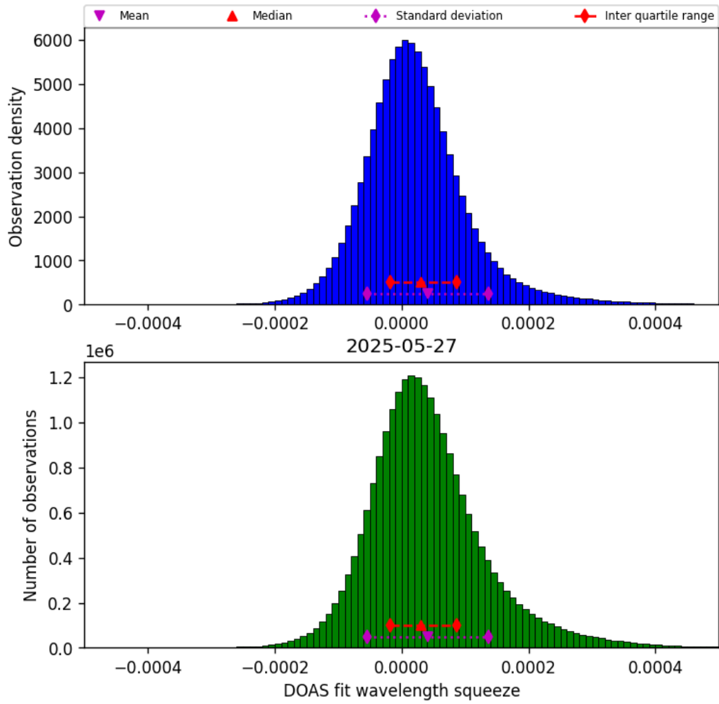
Figure 43: Histogram of “DOAS fit wavelength squeeze” for 2025-05-27 to 2025-05-28
