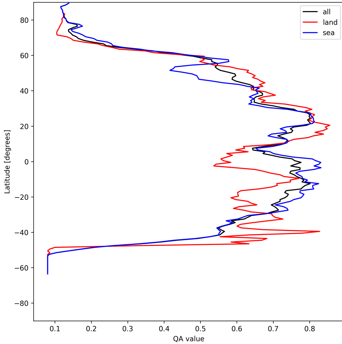
Figure 18: Zonal average of “QA value” for 2025-05-27 to 2025-05-28.
