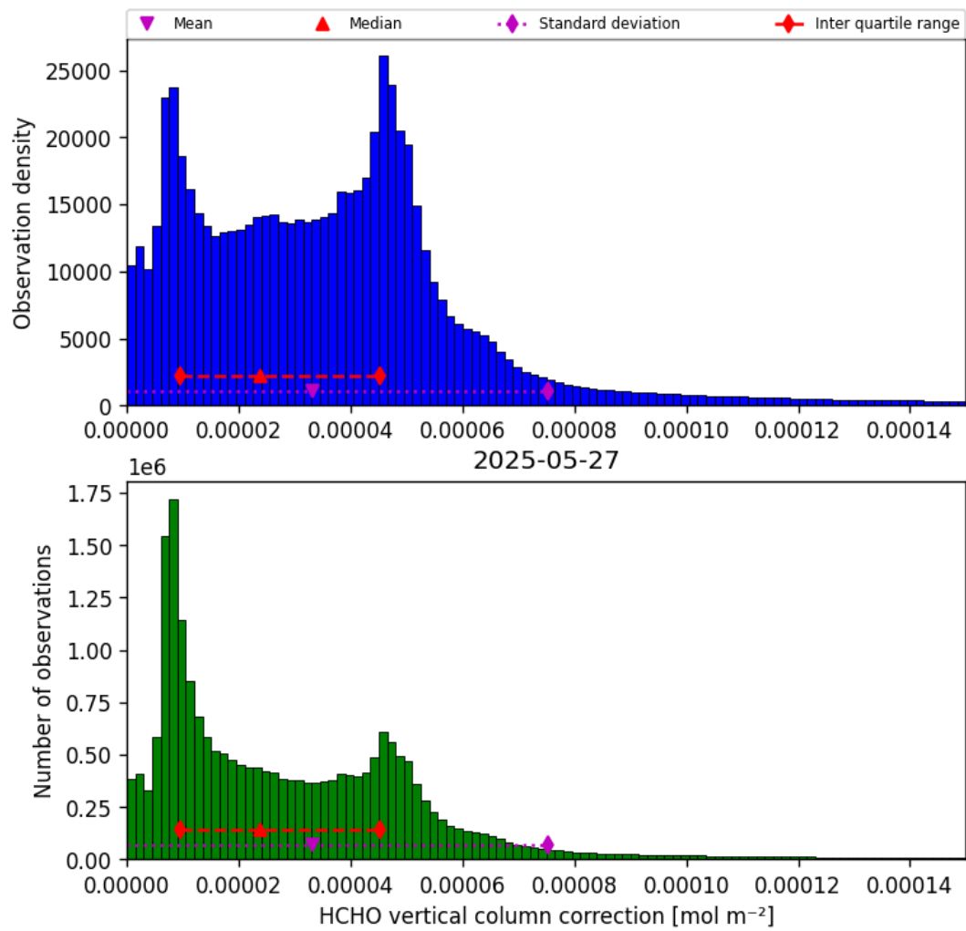
Figure 35: Histogram of “HCHO vertical column correction” for 2025-05-27 to 2025-05-28
