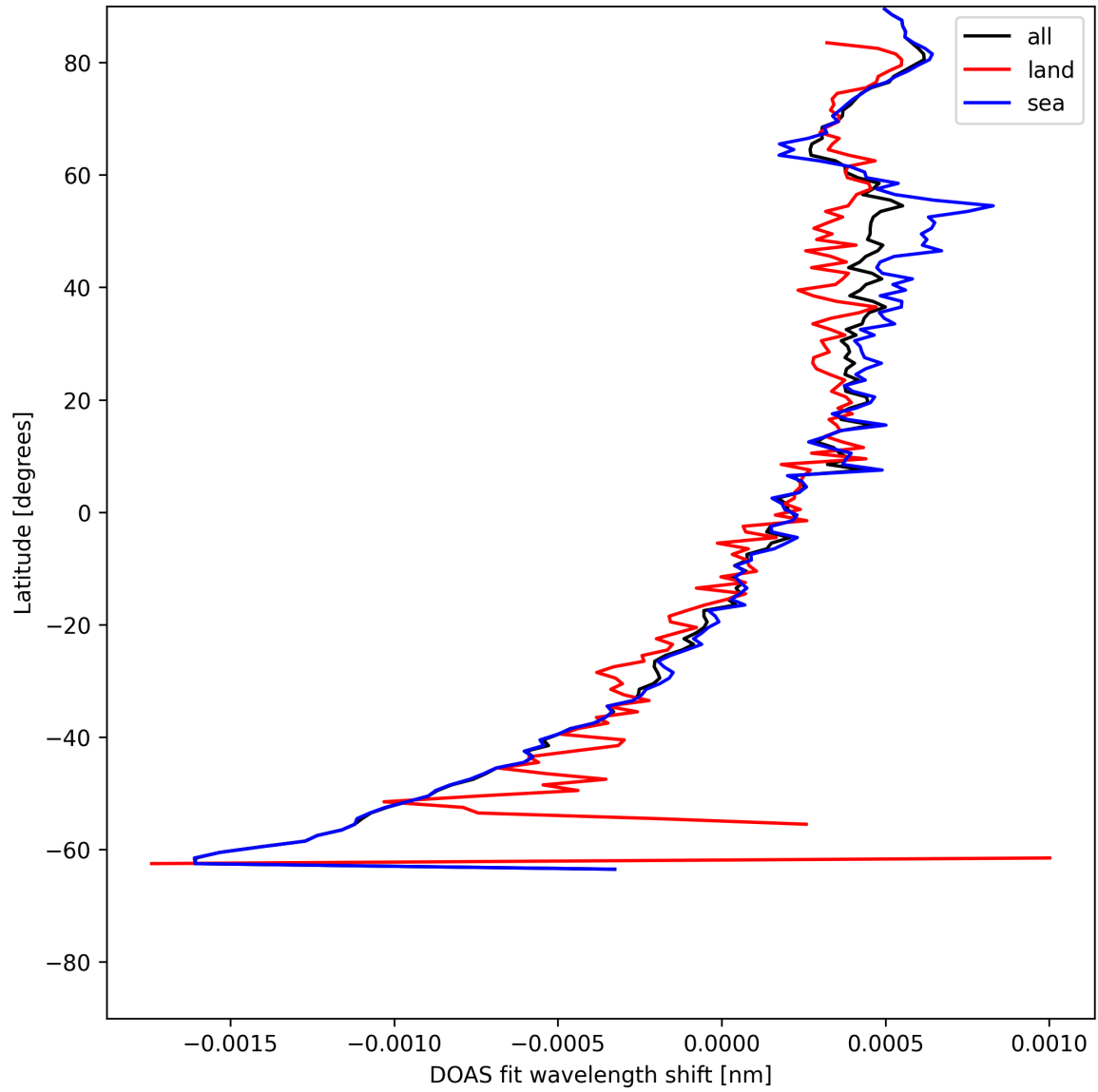
Figure 28: Zonal average of “DOAS fit wavelength shift” for 2025-05-27 to 2025-05-28.
