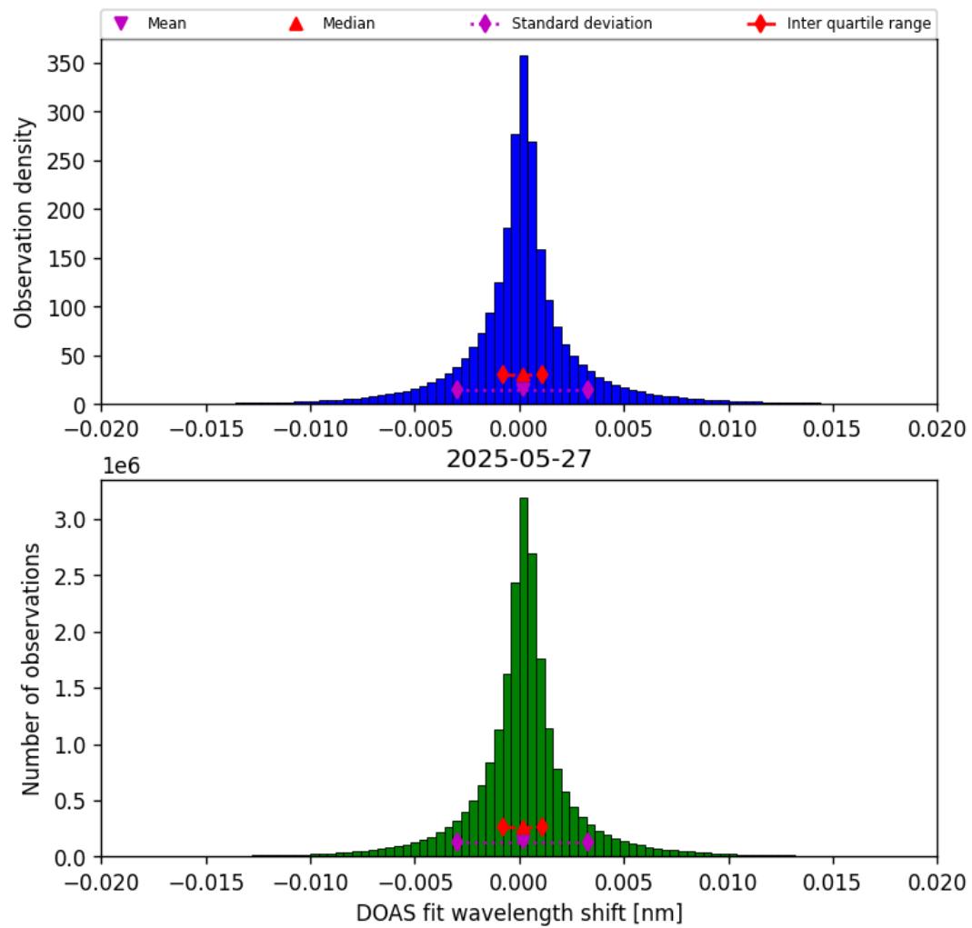
Figure 42: Histogram of “DOAS fit wavelength shift” for 2025-05-27 to 2025-05-28
