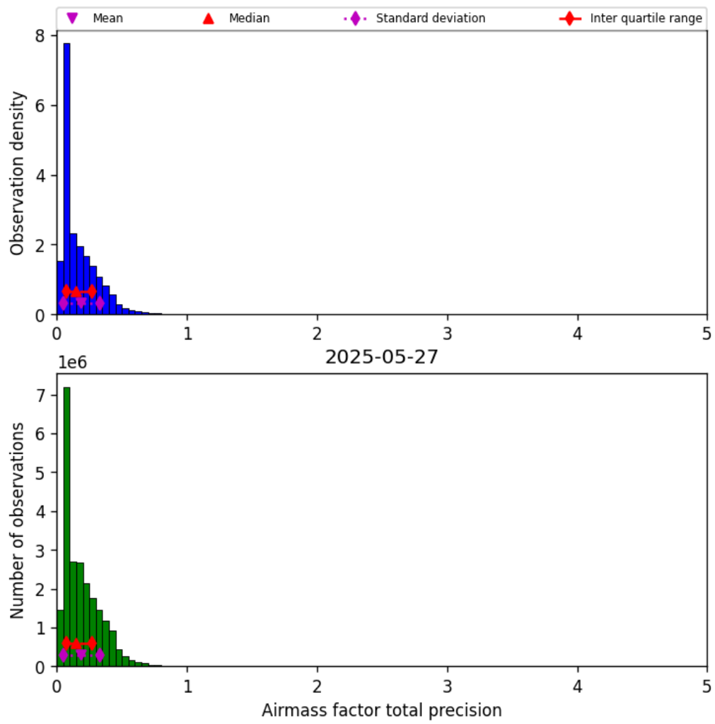
Figure 39: Histogram of “Airmass factor total precision” for 2025-05-27 to 2025-05-28
