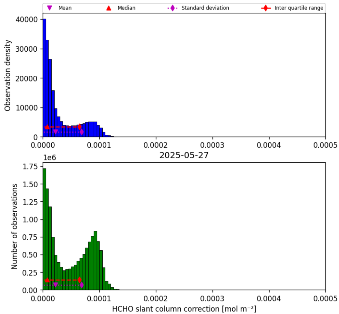
Figure 45: Histogram of “HCHO slant column correction” for 2025-05-27 to 2025-05-28
