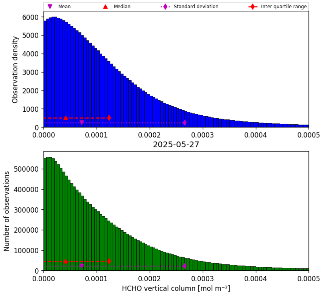
Figure 33: Histogram of “HCHO vertical column” for 2025-05-27 to 2025-05-28
