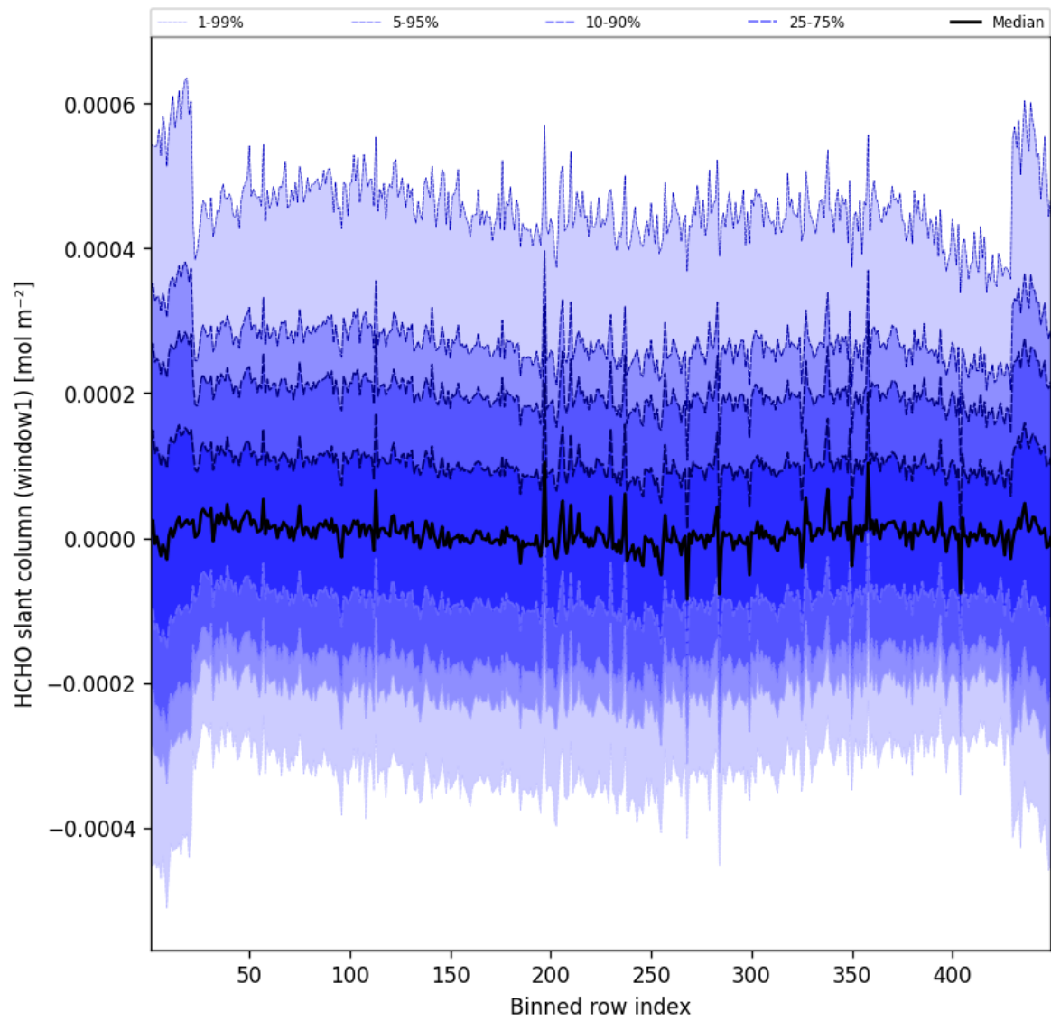
Figure 50: Along track statistics of “HCHO slant column (window1)” for 2025-05-27 to 2025-05-28
