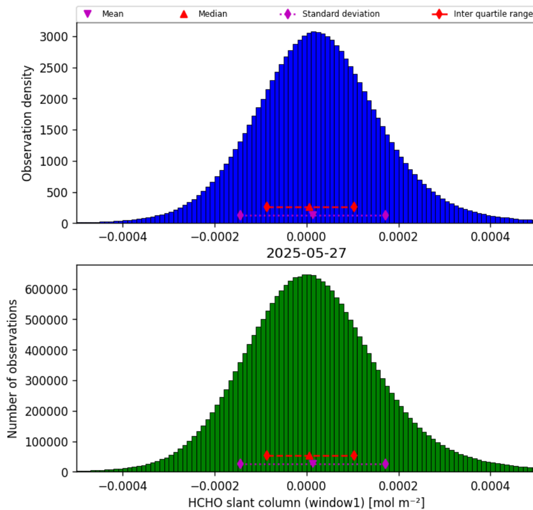
Figure 36: Histogram of “HCHO slant column (window1)” for 2025-05-27 to 2025-05-28
