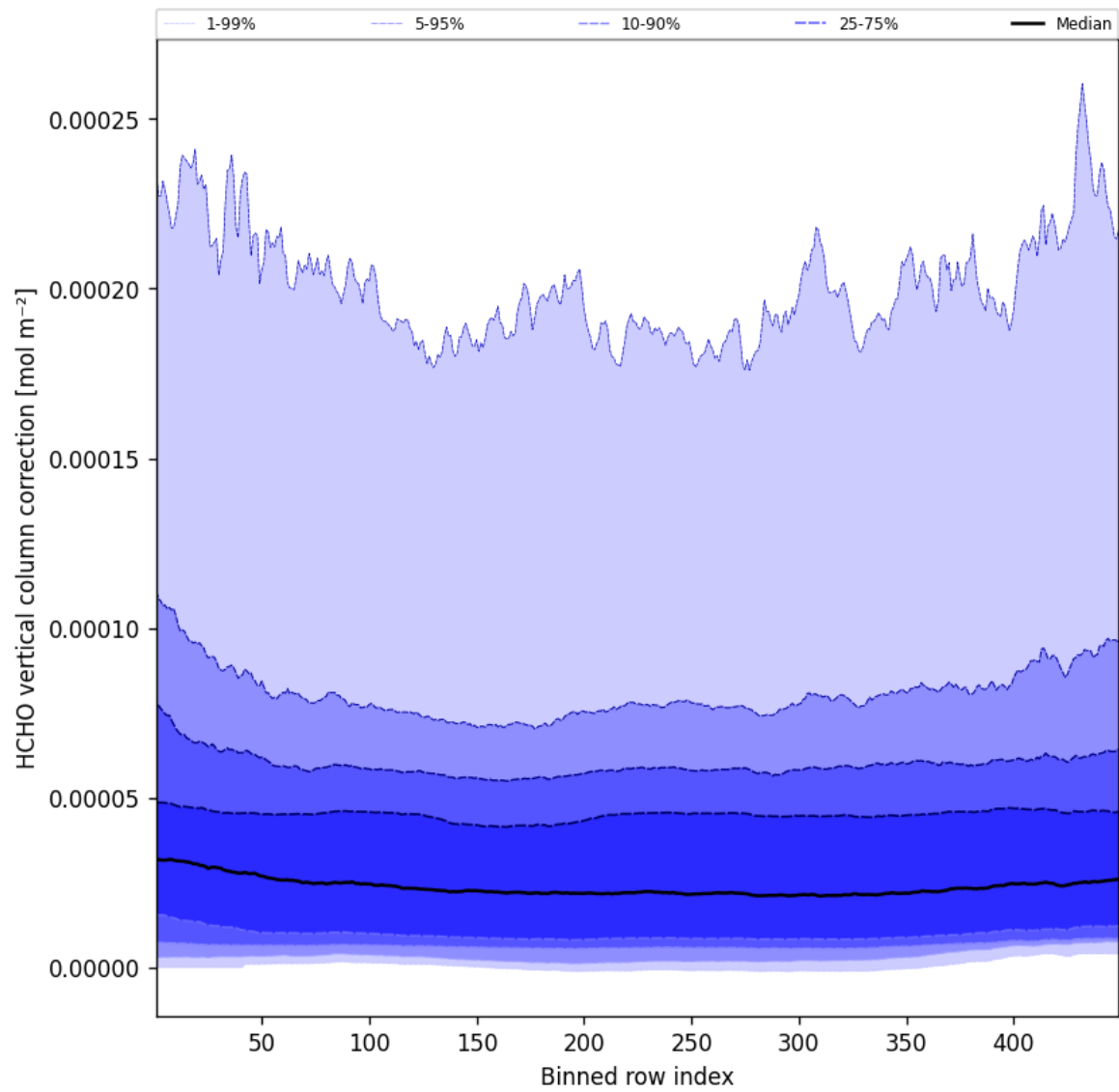
Figure 49: Along track statistics of “HCHO vertical column correction” for 2025-05-27 to 2025-05-28
