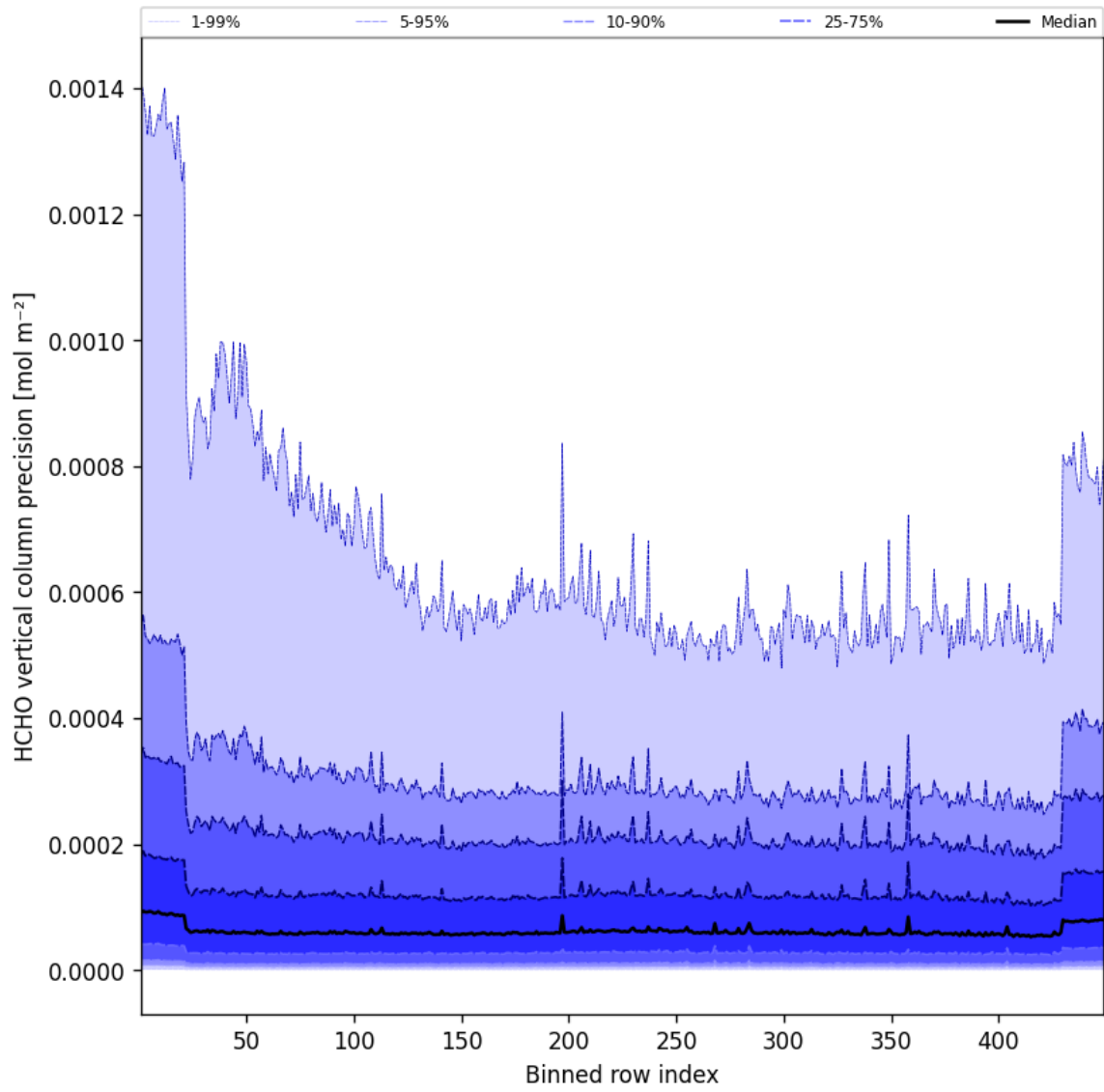
Figure 48: Along track statistics of “HCHO vertical column precision” for 2025-05-27 to 2025-05-28
