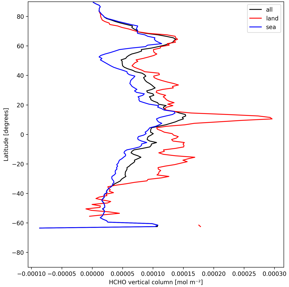
Figure 19: Zonal average of “HCHO vertical column” for 2025-05-27 to 2025-05-28.
