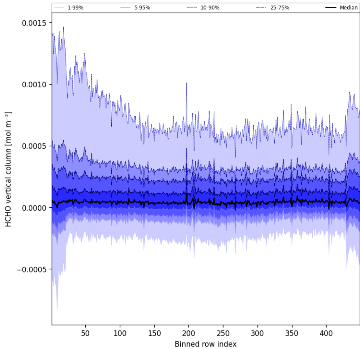
Figure 47: Along track statistics of “HCHO vertical column” for 2025-05-27 to 2025-05-28
