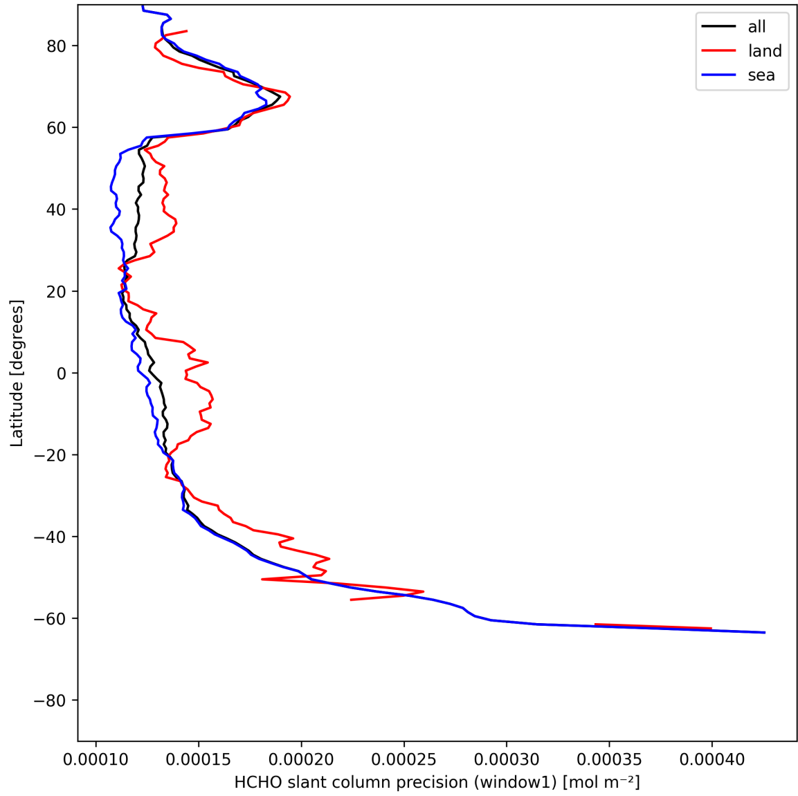
Figure 23: Zonal average of “HCHO slant column precision (window1)” for 2025-05-27 to 2025-05-28.
