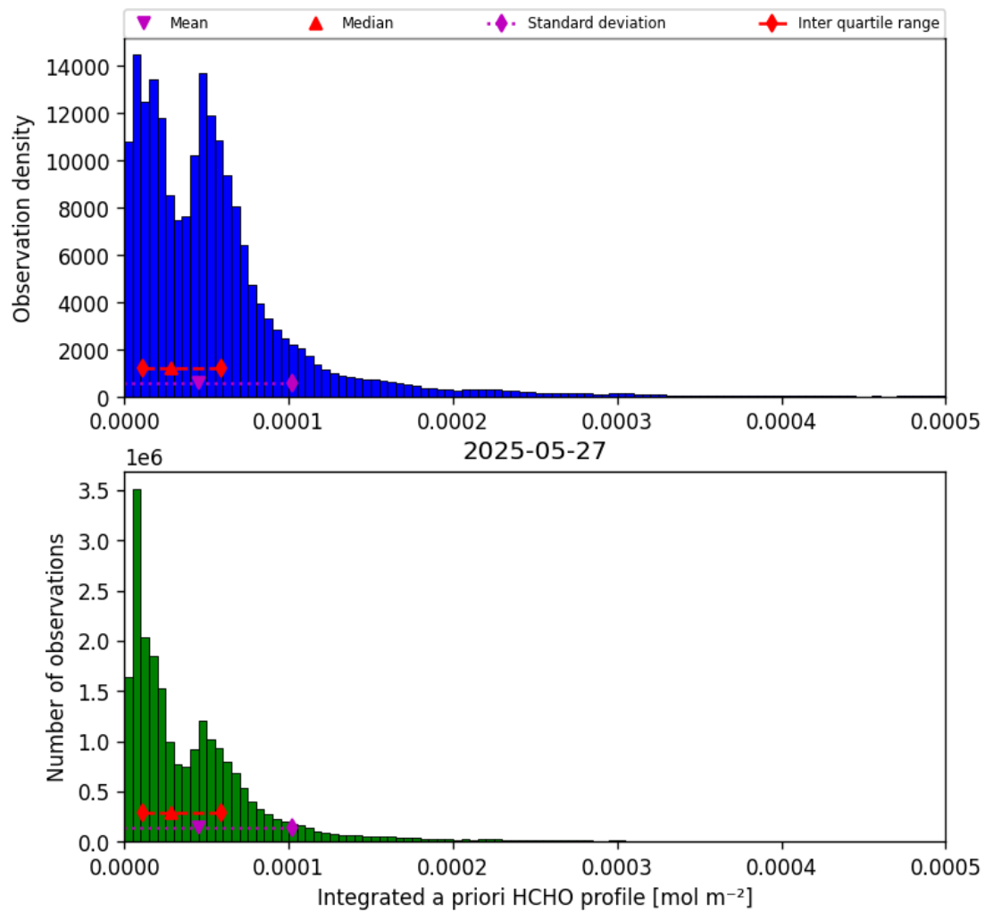
Figure 41: Histogram of “Integrated a priori HCHO profile” for 2025-05-27 to 2025-05-28
