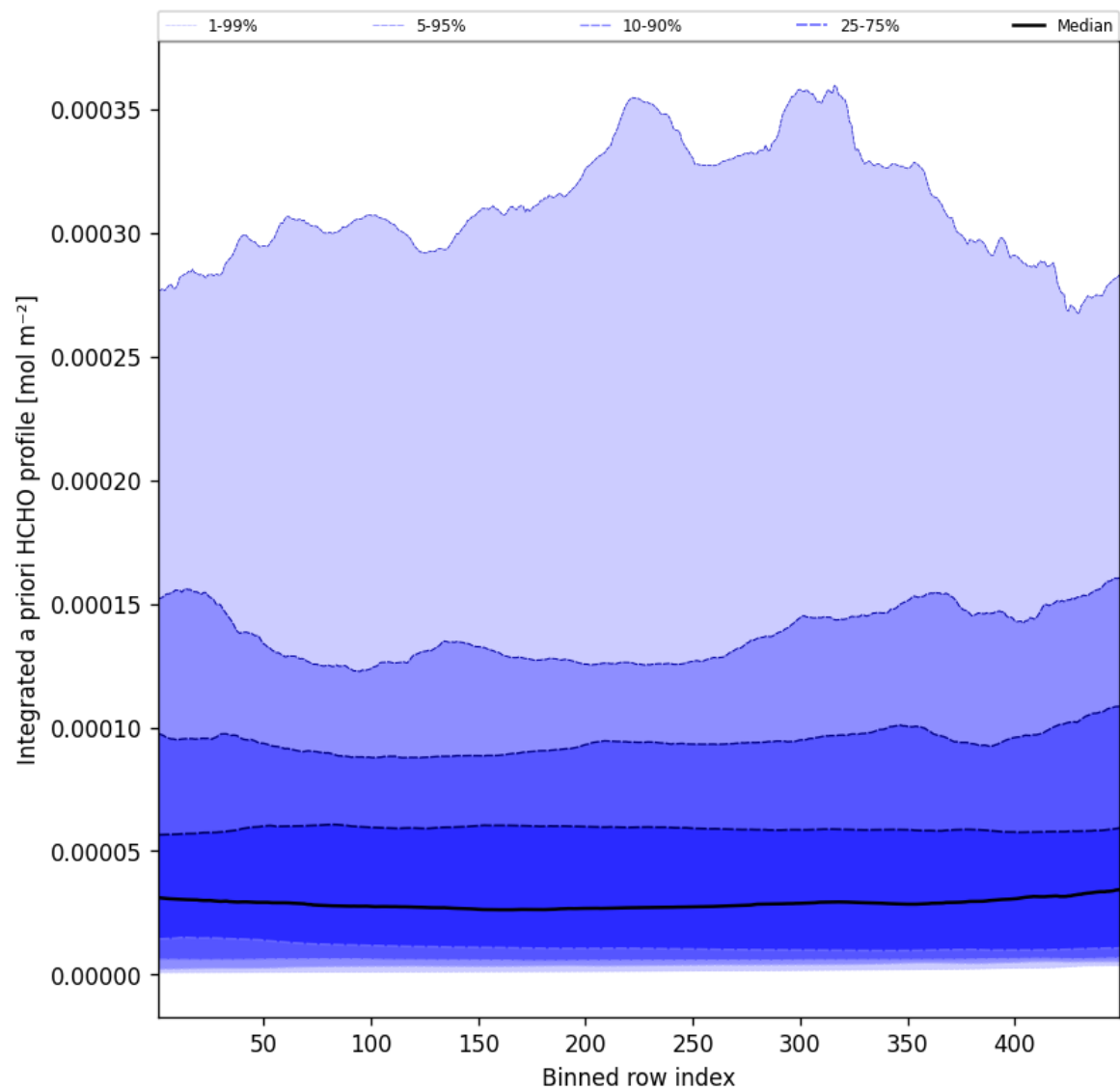
Figure 55: Along track statistics of “Integrated a priori HCHO profile” for 2025-05-27 to 2025-05-28
