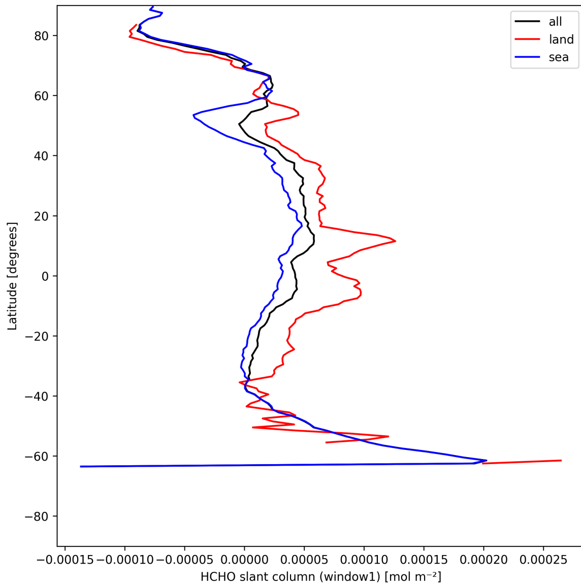
Figure 22: Zonal average of “HCHO slant column (window1)” for 2025-05-27 to 2025-05-28.
