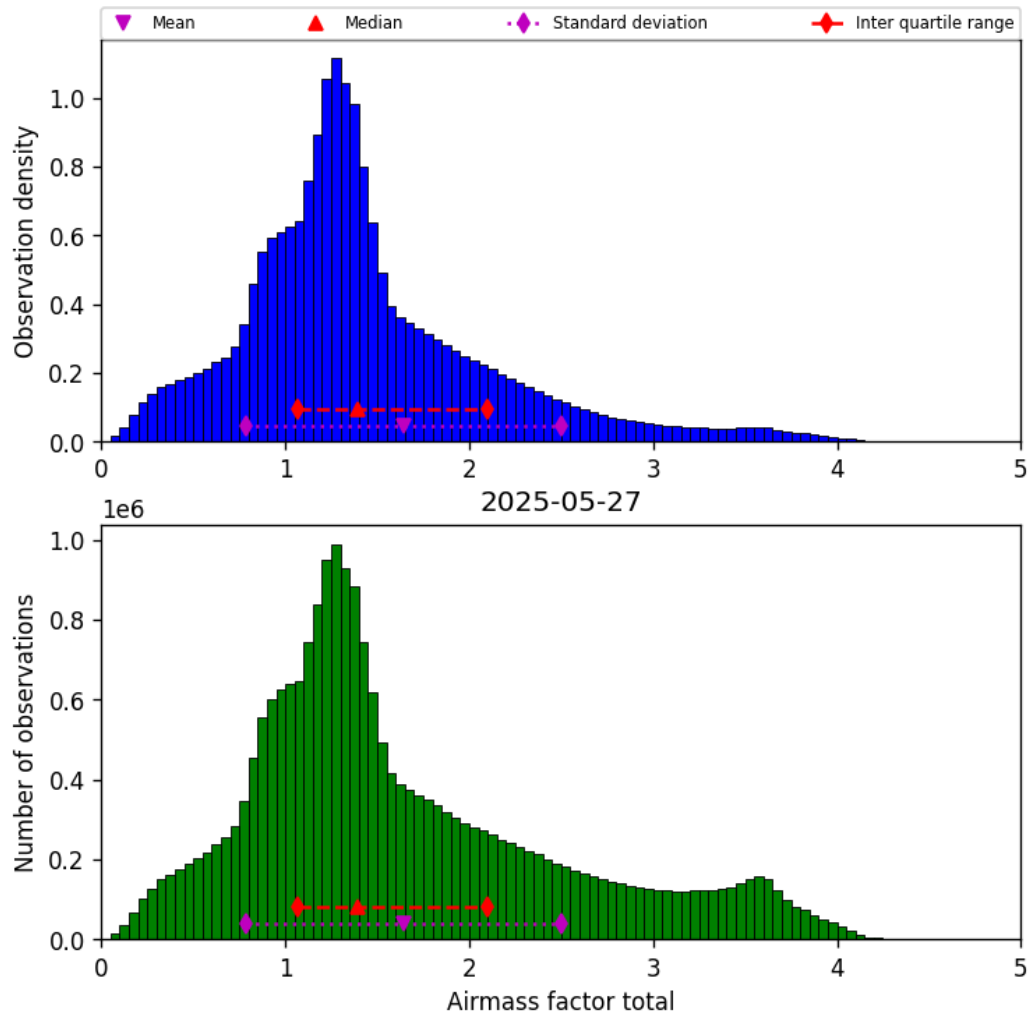
Figure 38: Histogram of “Airmass factor total” for 2025-05-27 to 2025-05-28
