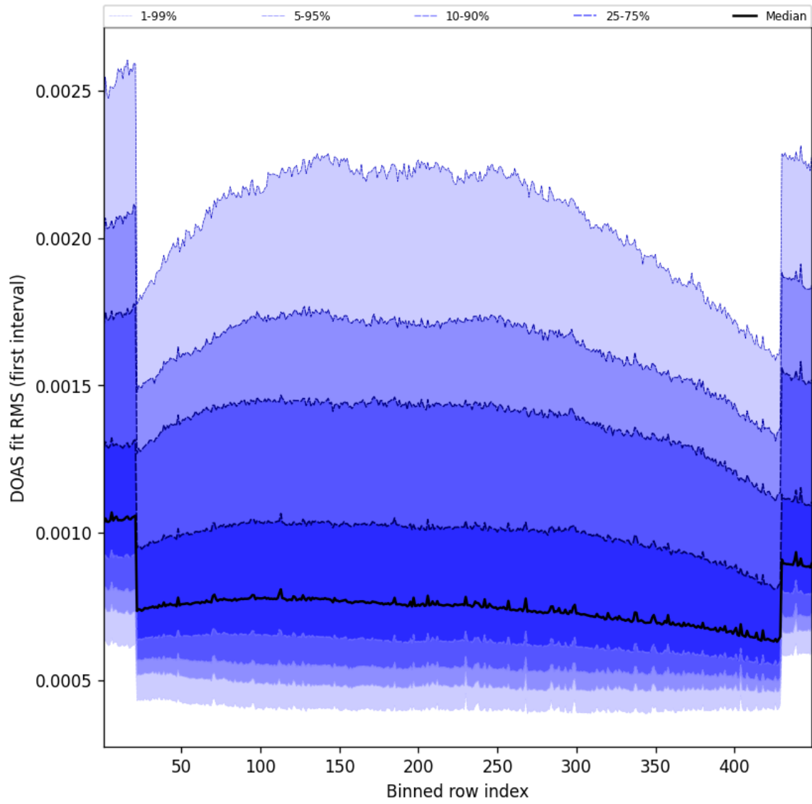
Figure 58: Along track statistics of “DOAS fit RMS (first interval)” for 2025-05-27 to 2025-05-28
