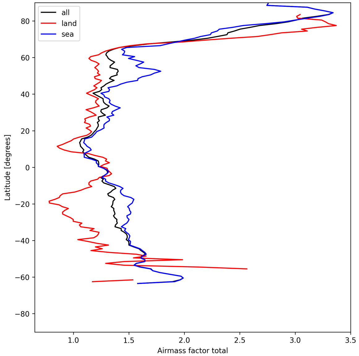
Figure 24: Zonal average of “Airmass factor total” for 2025-05-27 to 2025-05-28.
