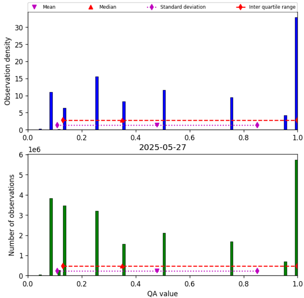
Figure 32: Histogram of “QA value” for 2025-05-27 to 2025-05-28
