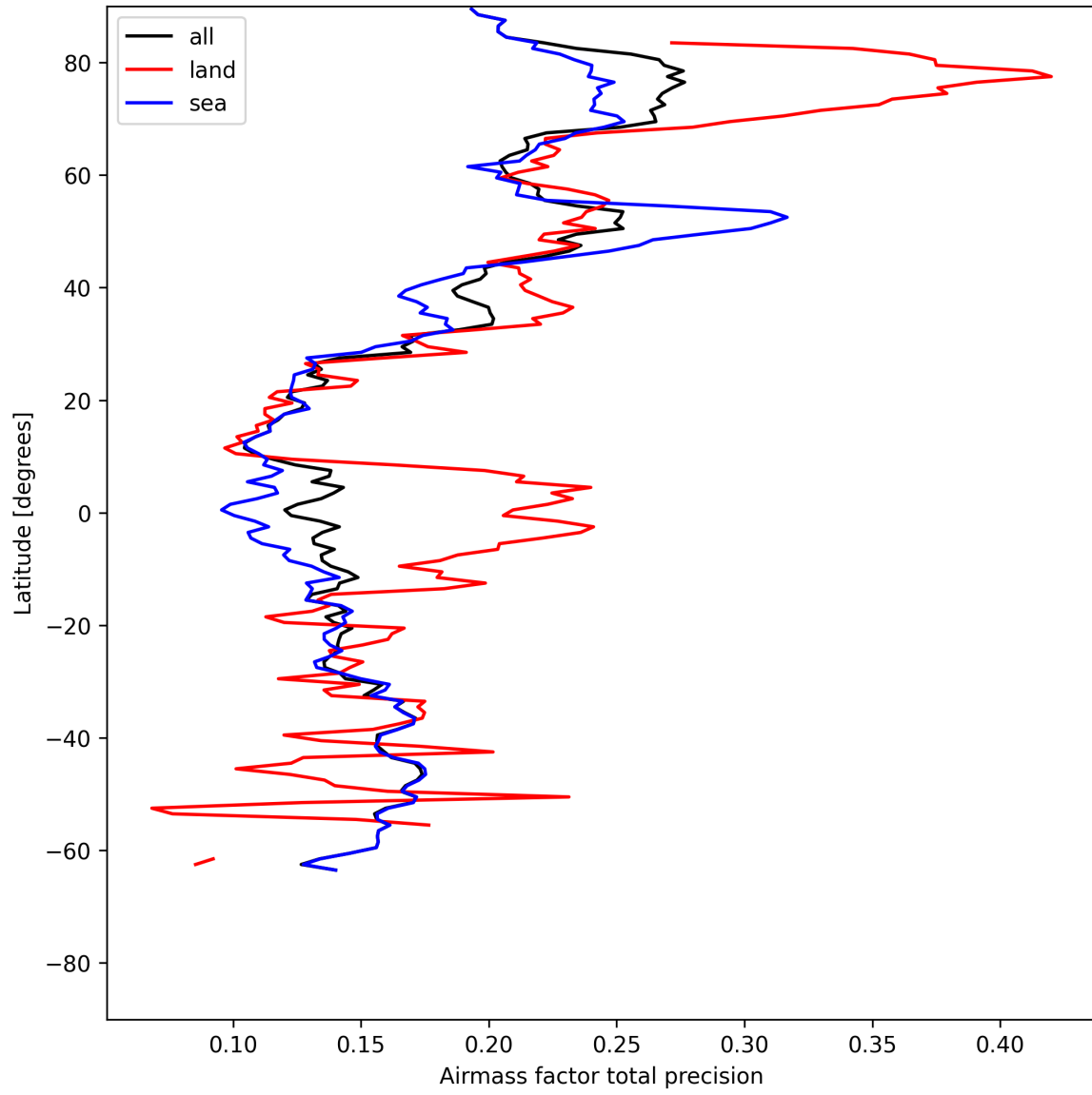
Figure 25: Zonal average of “Airmass factor total precision” for 2025-05-27 to 2025-05-28.
