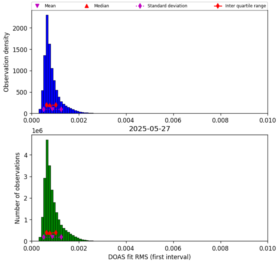
Figure 44: Histogram of "DOAS fit RMS (first interval)" for 2025-05-27 to 2025-05-28
