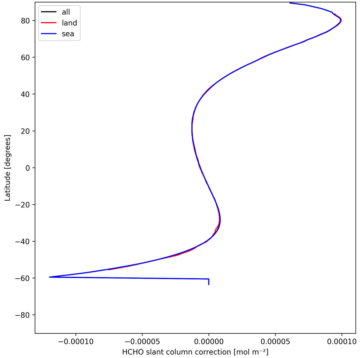
Figure 31: Zonal average of "HCHO slant column correction" for 2025-05-27 to 2025-05-28.
