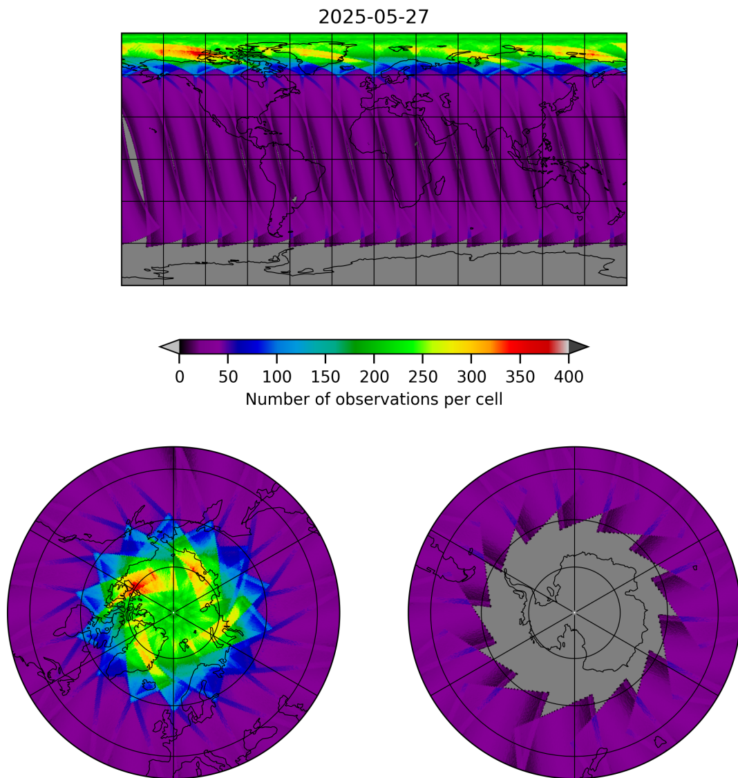
Figure 17: Map of the number of observations for 2025-05-27 to 2025-05-28
