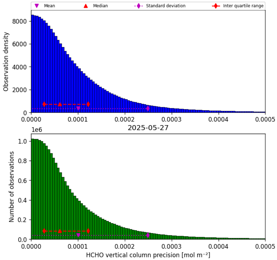
Figure 34: Histogram of “HCHO vertical column precision” for 2025-05-27 to 2025-05-28
