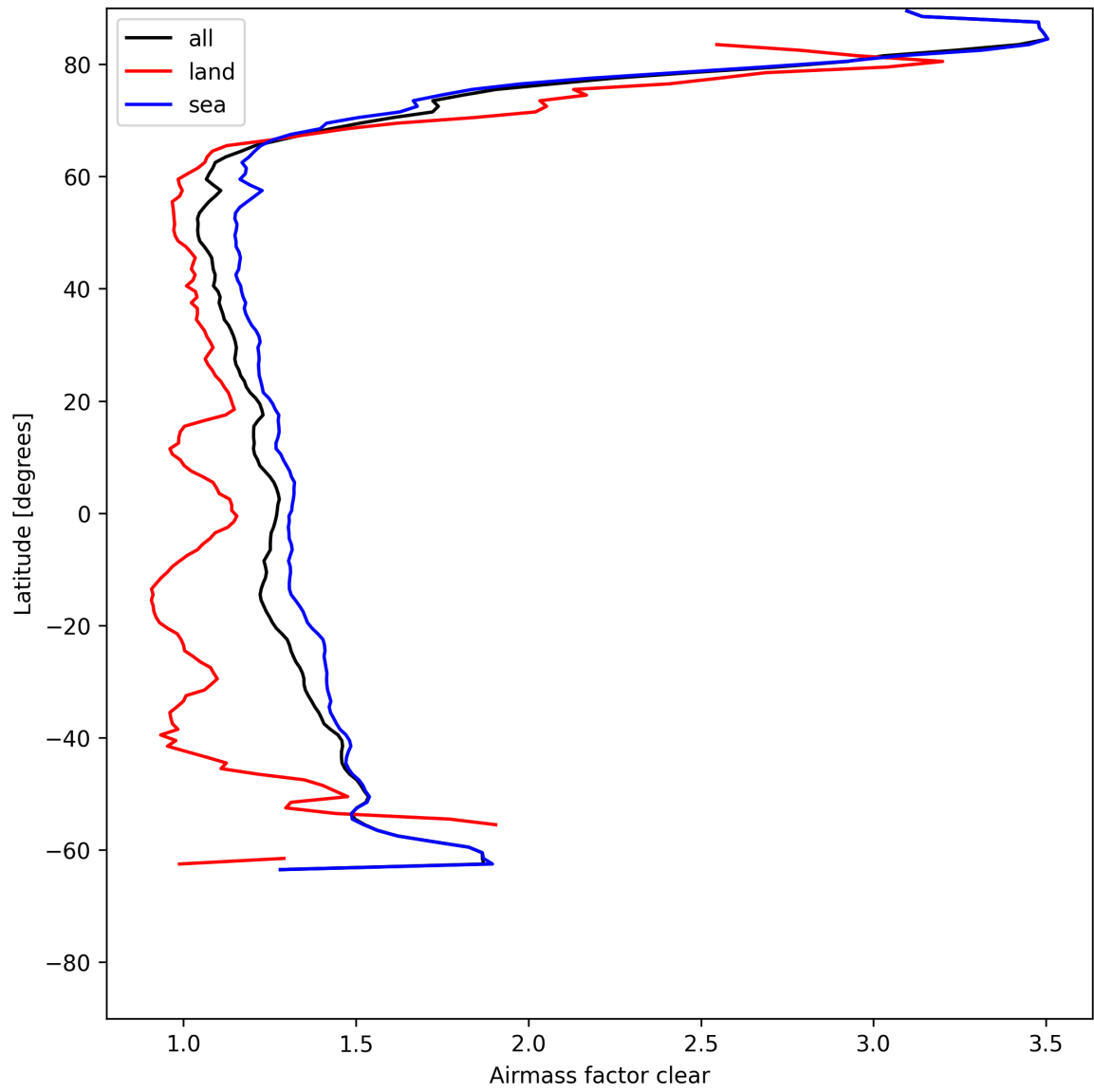
Figure 26: Zonal average of “Airmass factor clear” for 2025-05-27 to 2025-05-28.
