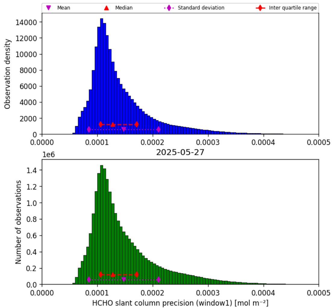
Figure 37: Histogram of “HCHO slant column precision (window1)” for 2025-05-27 to 2025-05-28
