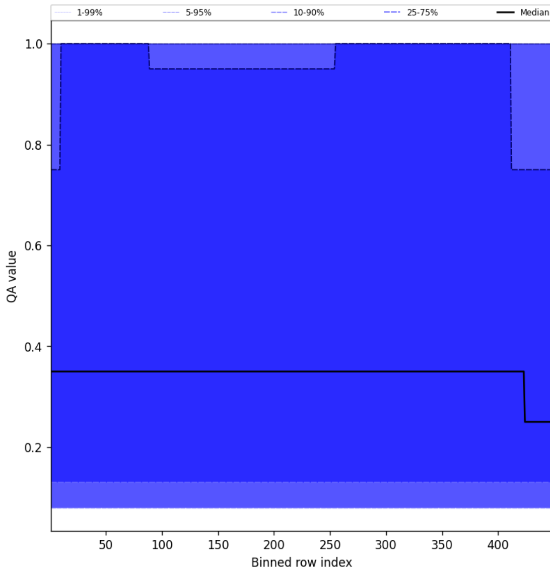
Figure 46: Along track statistics of “QA value” for 2025-05-27 to 2025-05-28
