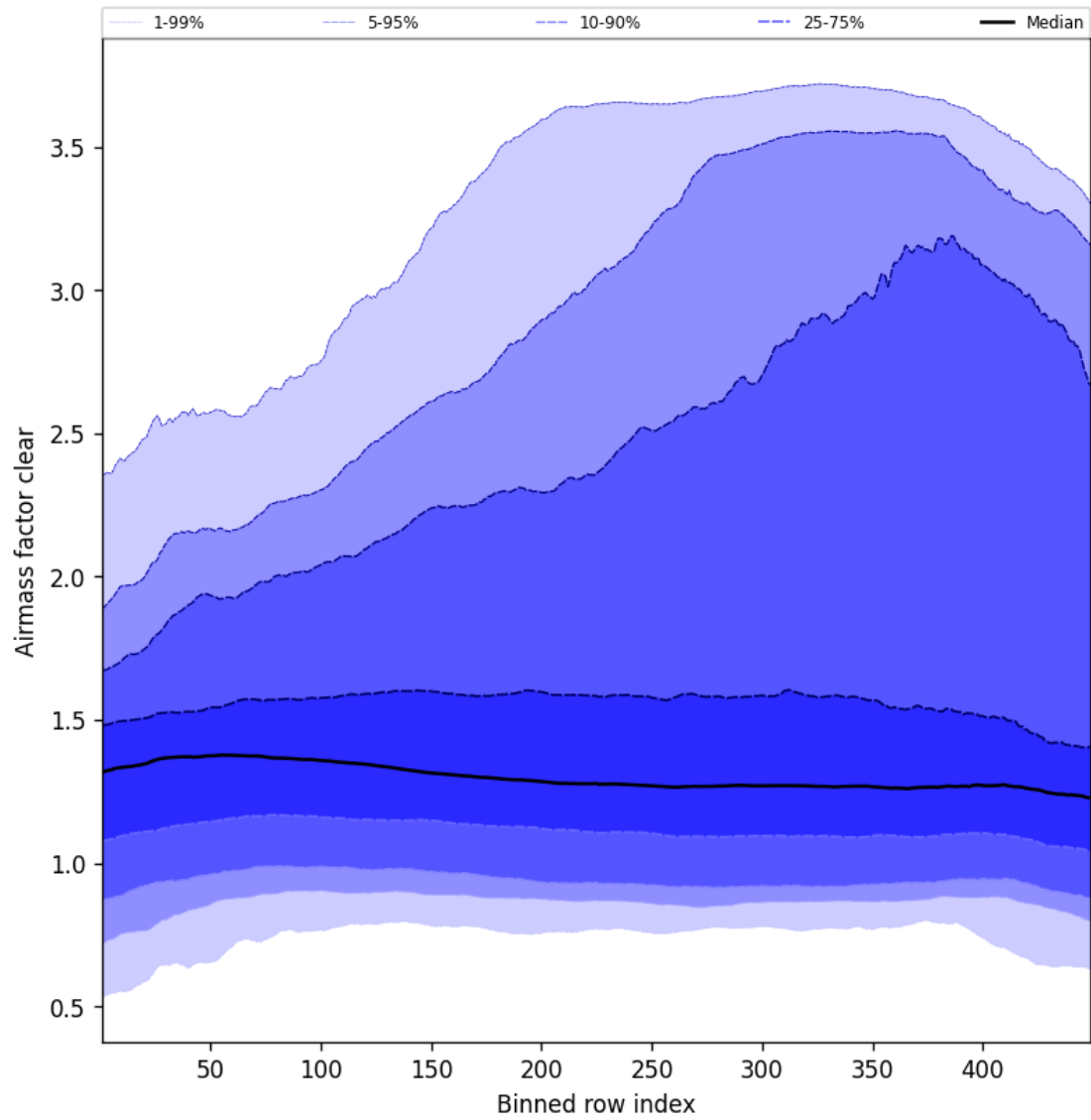
Figure 54: Along track statistics of “Airmass factor clear” for 2025-05-27 to 2025-05-28
