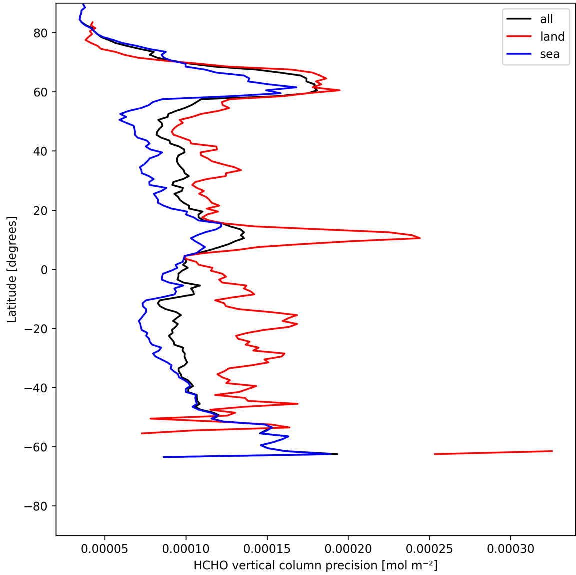
Figure 20: Zonal average of “HCHO vertical column precision” for 2025-05-27 to 2025-05-28.
