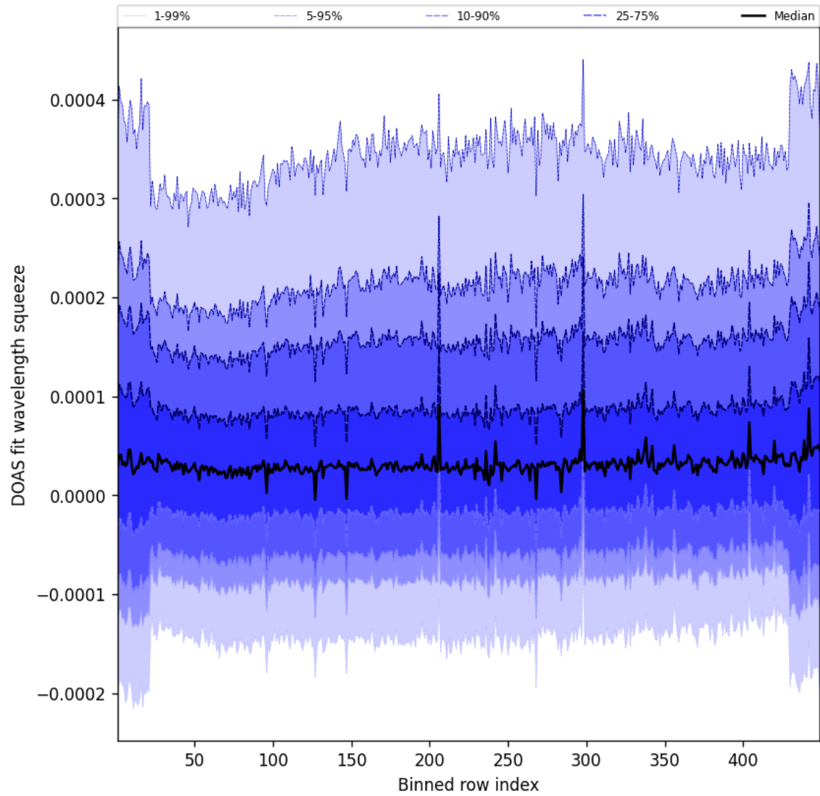
Figure 57: Along track statistics of “DOAS fit wavelength squeeze” for 2025-05-27 to 2025-05-28
