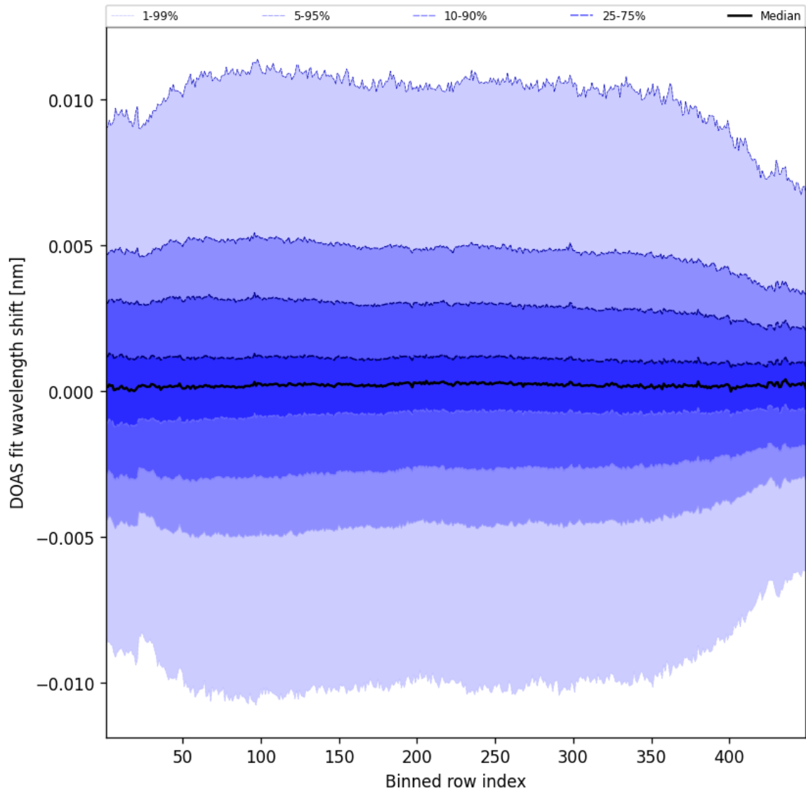
Figure 56: Along track statistics of “DOAS fit wavelength shift” for 2025-05-27 to 2025-05-28
