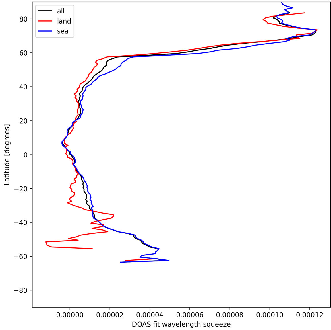
Figure 29: Zonal average of “DOAS fit wavelength squeeze” for 2025-05-27 to 2025-05-28.
