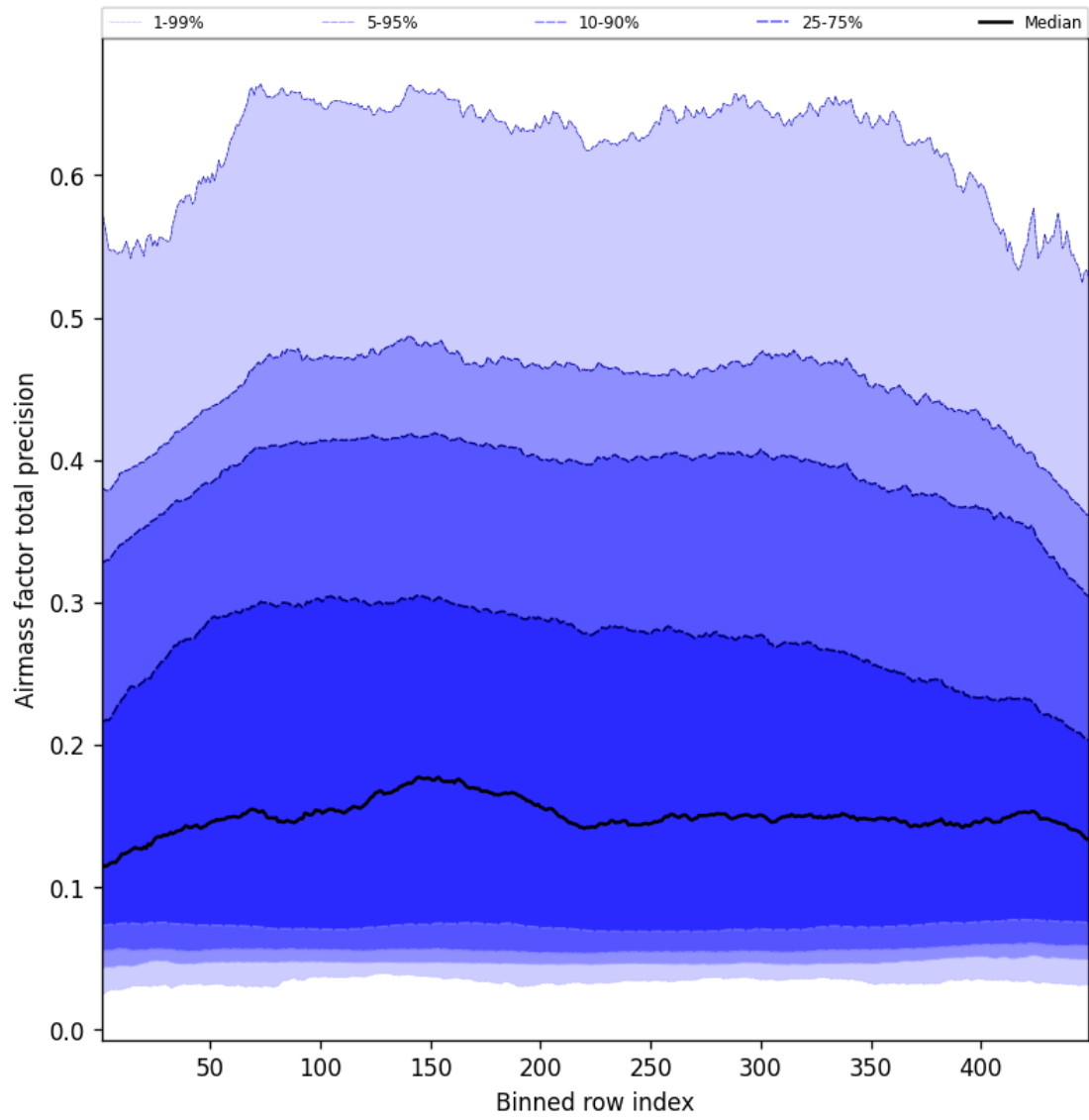
Figure 53: Along track statistics of “Airmass factor total precision” for 2025-05-27 to 2025-05-28
