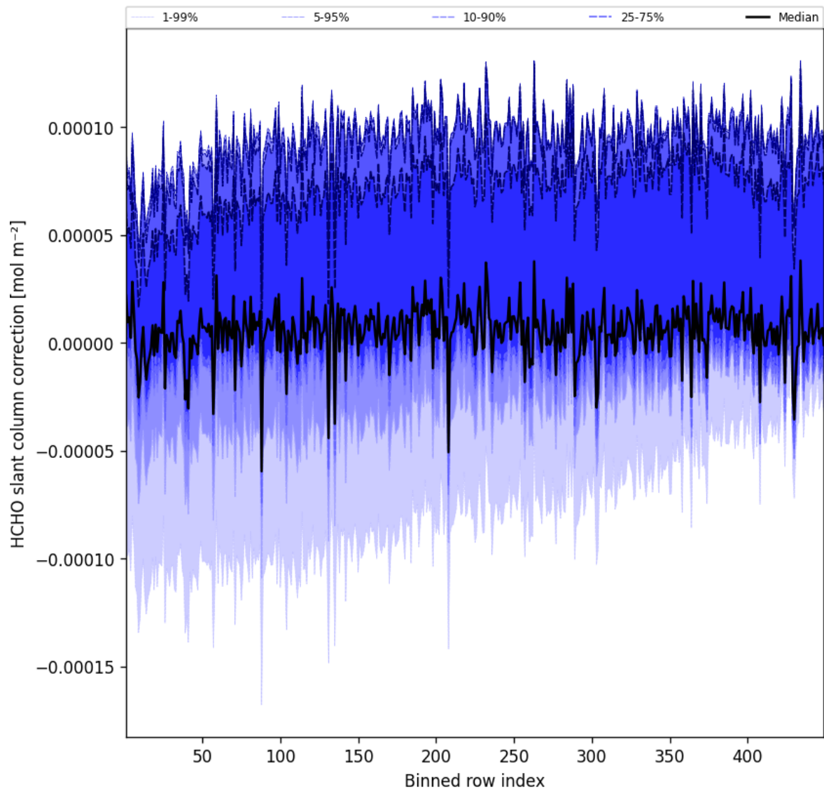
Figure 59: Along track statistics of “HCHO slant column correction” for 2025-05-27 to 2025-05-28
