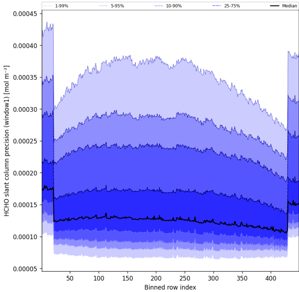
Figure 51: Along track statistics of “HCHO slant column precision (window1)” for 2025-05-27 to 2025-05-28
