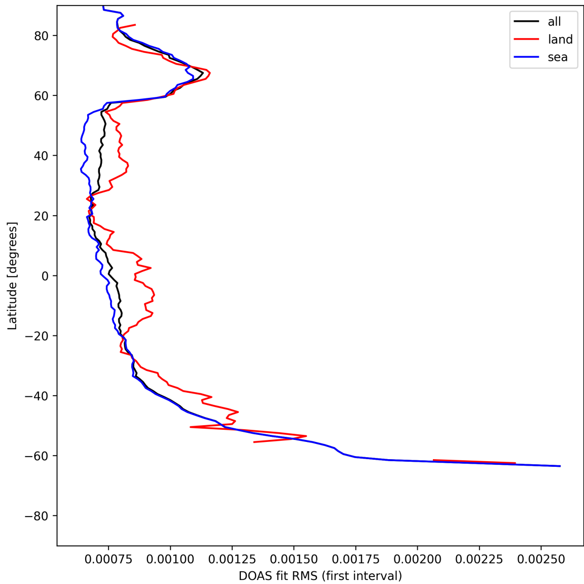
Figure 30: Zonal average of “DOAS fit RMS (first interval)” for 2025-05-27 to 2025-05-28.
