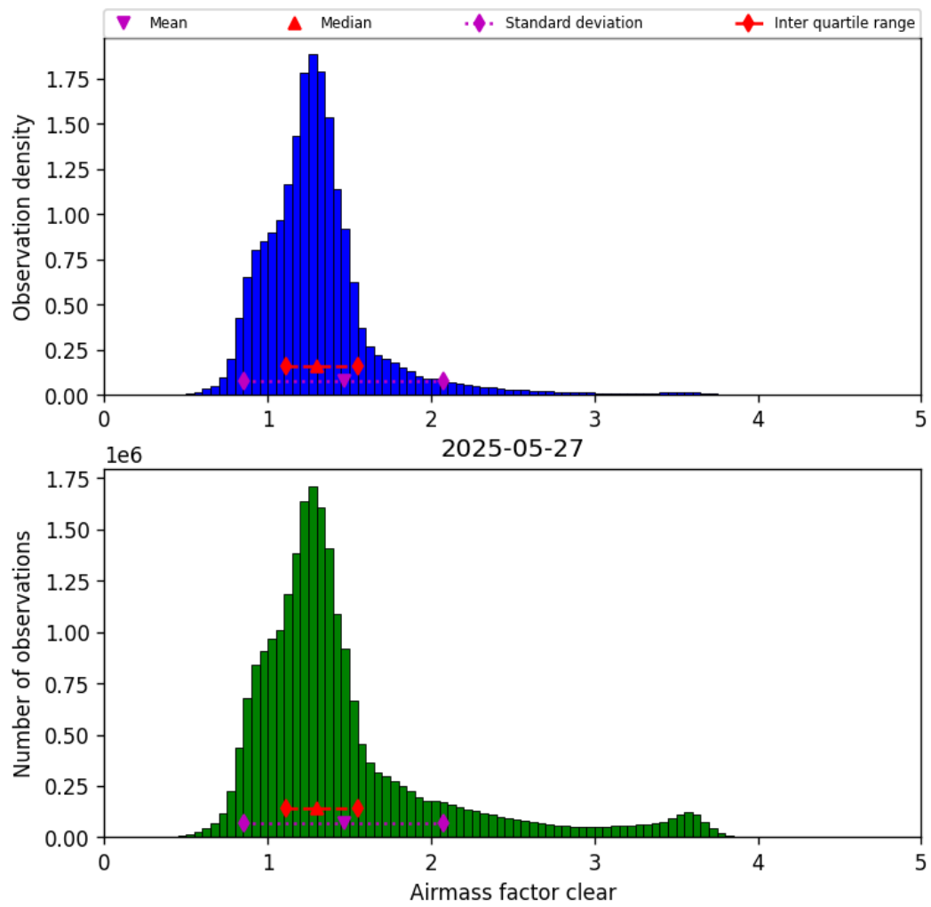
Figure 40: Histogram of “Airmass factor clear” for 2025-05-27 to 2025-05-28
