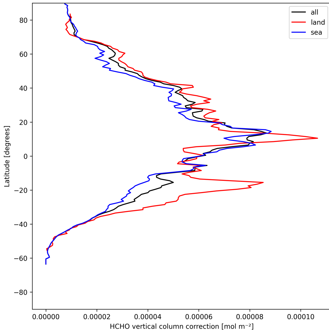
Figure 21: Zonal average of “HCHO vertical column correction” for 2025-05-27 to 2025-05-28.
