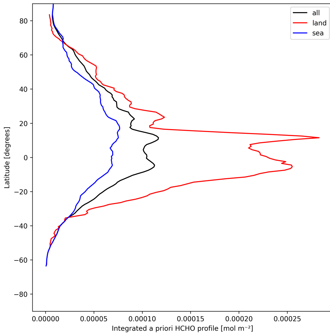
Figure 27: Zonal average of “Integrated a priori HCHO profile” for 2025-05-27 to 2025-05-28.
