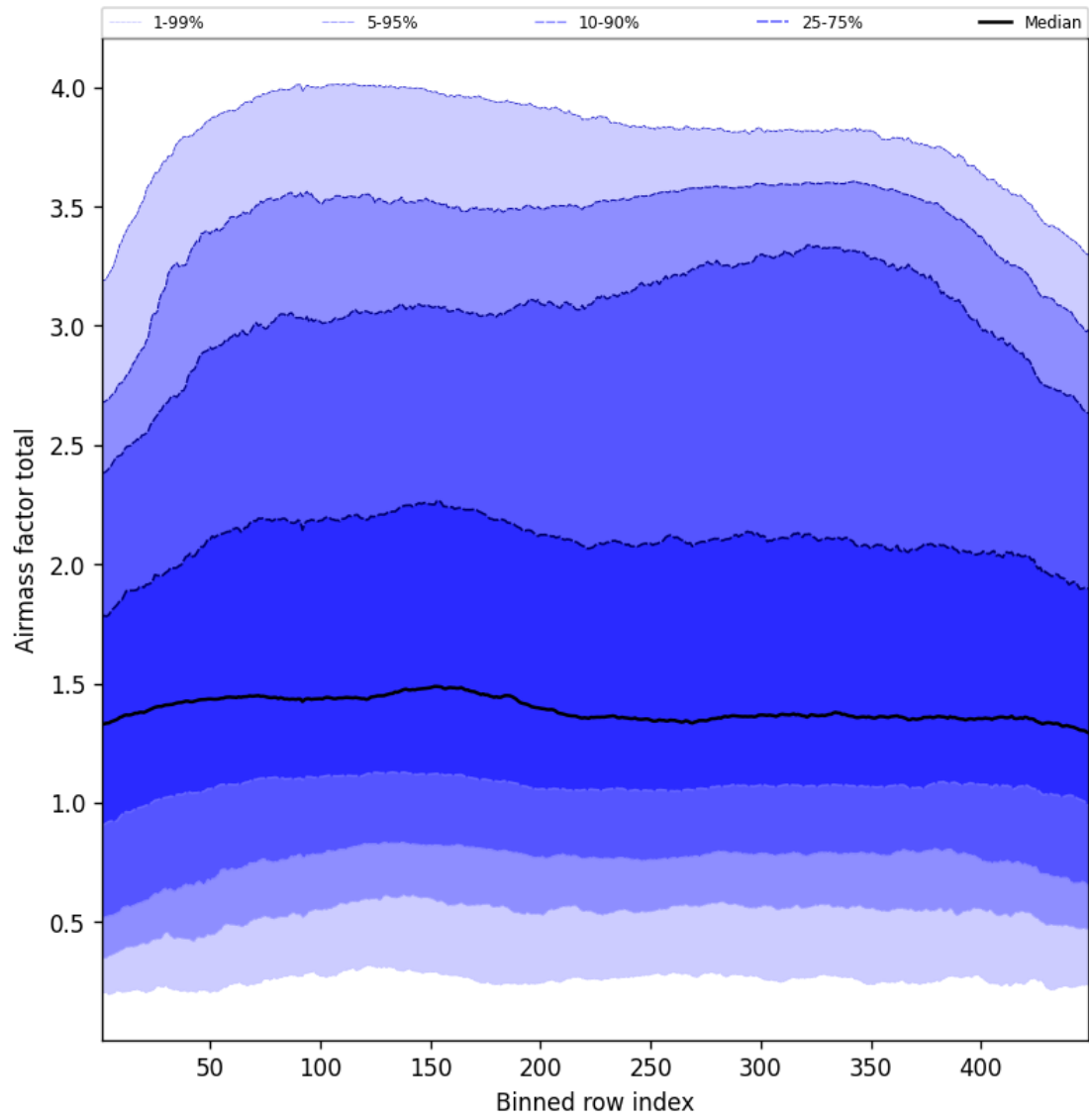
Figure 52: Along track statistics of “Airmass factor total” for 2025-05-27 to 2025-05-28
