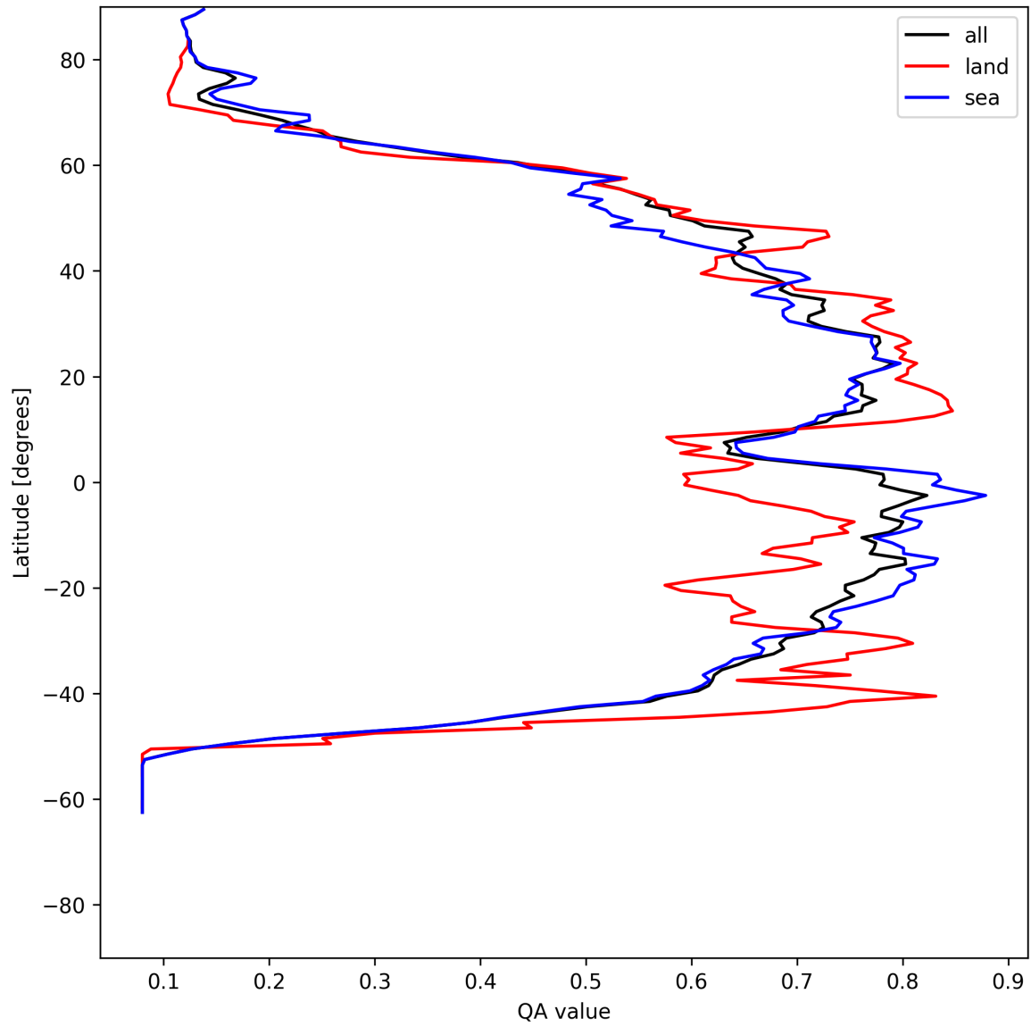
Figure 18: Zonal average of “QA value” for 2025-05-28 to 2025-05-29.
