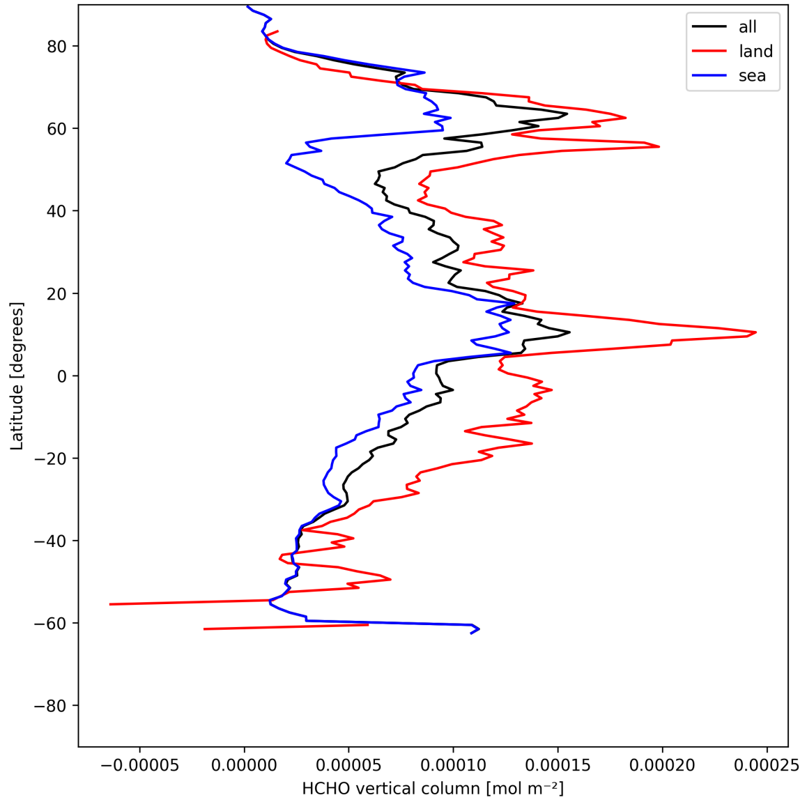
Figure 19: Zonal average of “HCHO vertical column” for 2025-05-28 to 2025-05-29.
