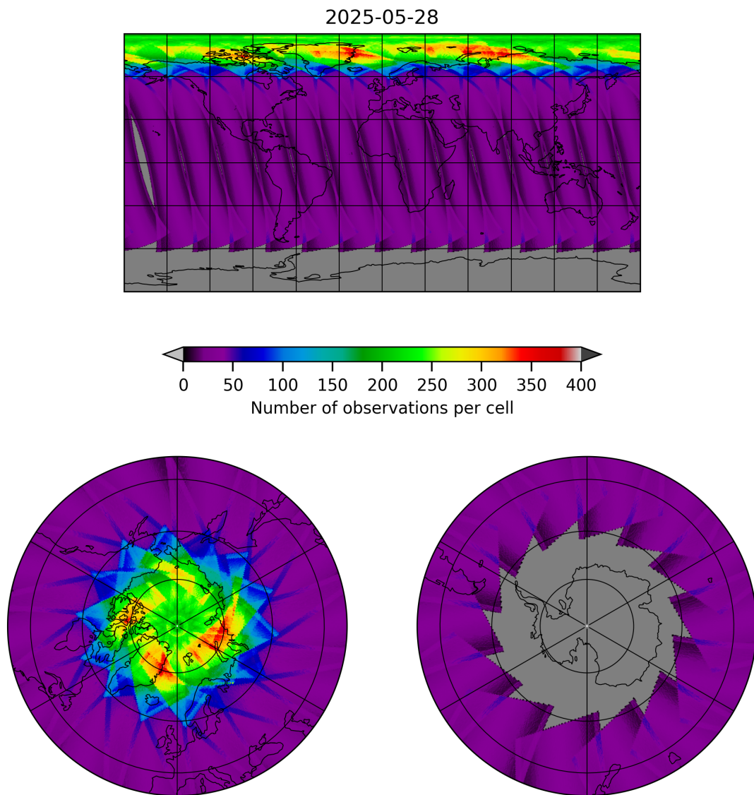
Figure 17: Map of the number of observations for 2025-05-28 to 2025-05-29
