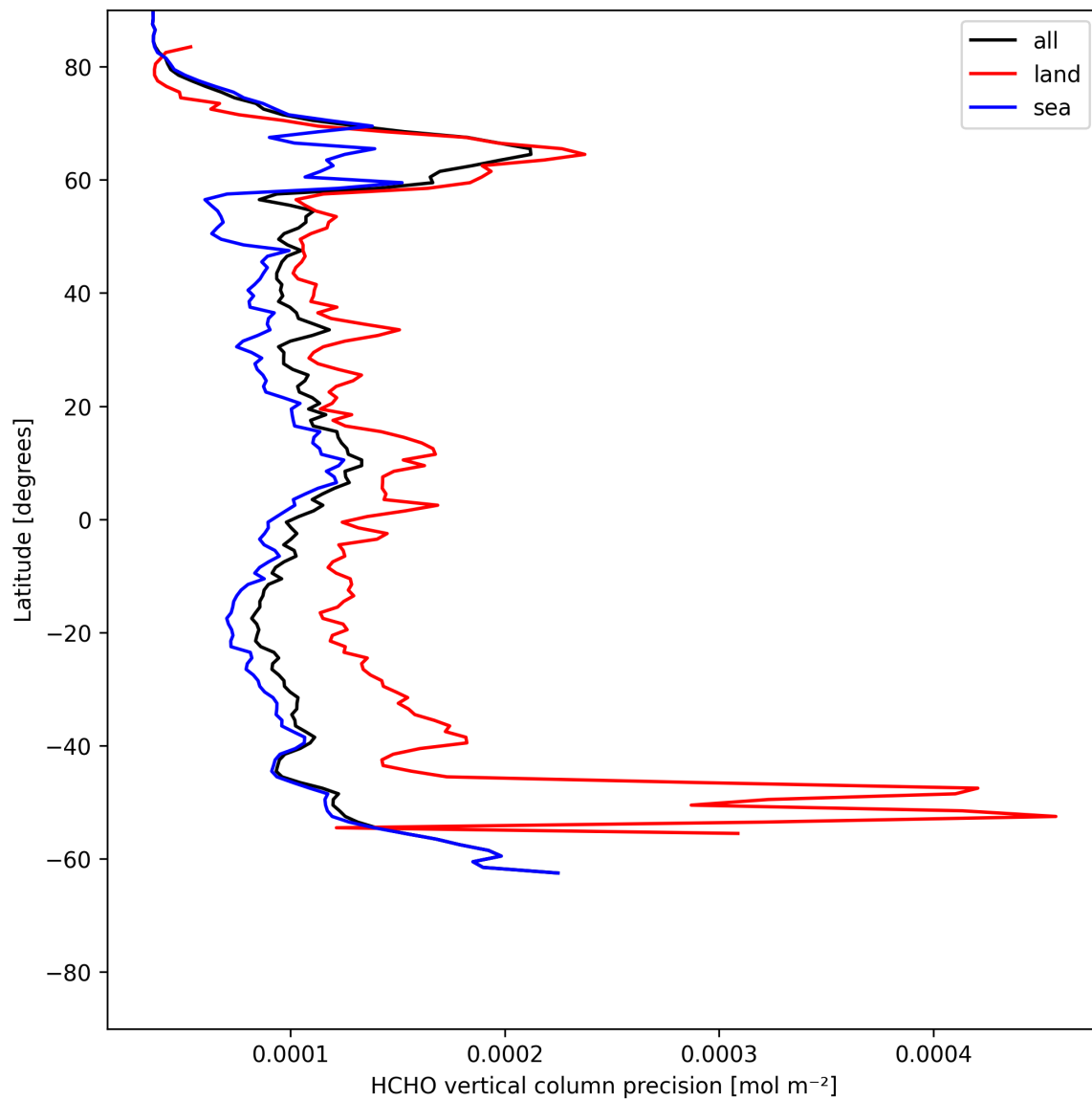
Figure 20: Zonal average of “HCHO vertical column precision” for 2025-05-29 to 2025-05-29.
