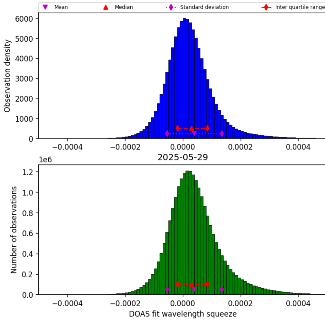
Figure 43: Histogram of “DOAS fit wavelength squeeze” for 2025-05-29 to 2025-05-29
