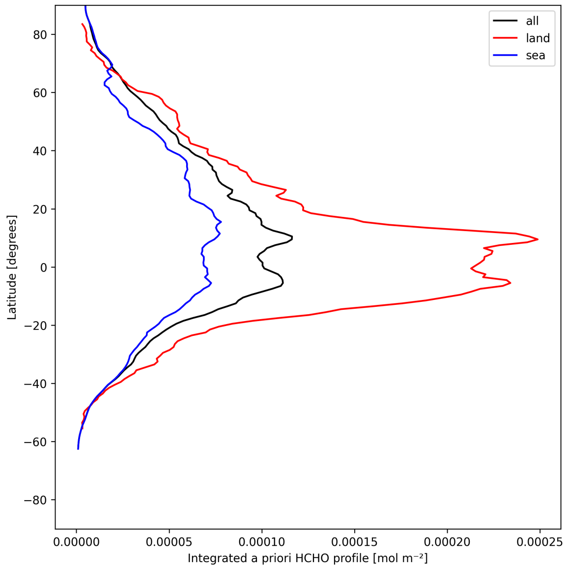
Figure 27: Zonal average of “Integrated a priori HCHO profile” for 2025-05-29 to 2025-05-29.
