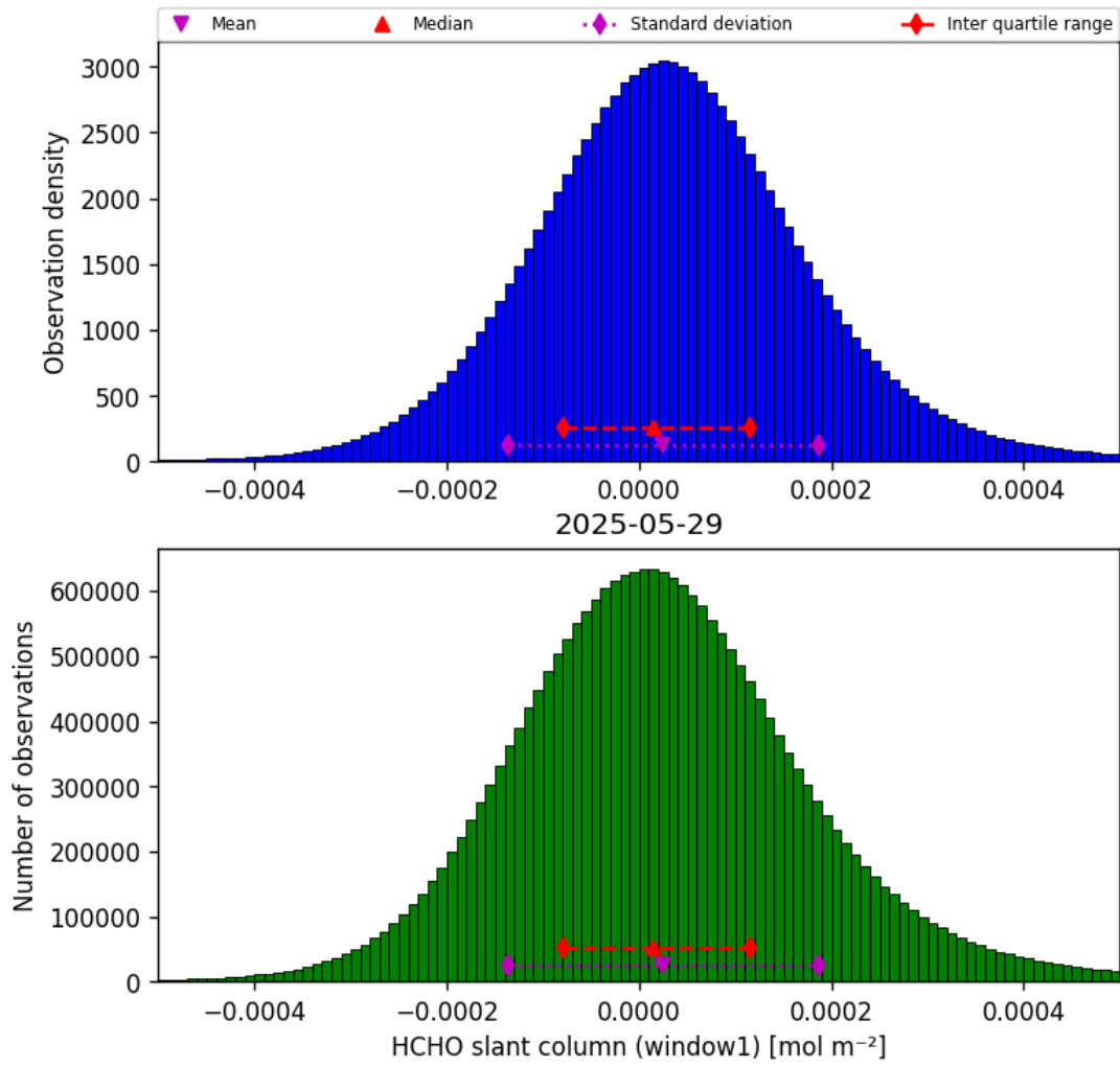
Figure 36: Histogram of “HCHO slant column (window1)” for 2025-05-29 to 2025-05-29
