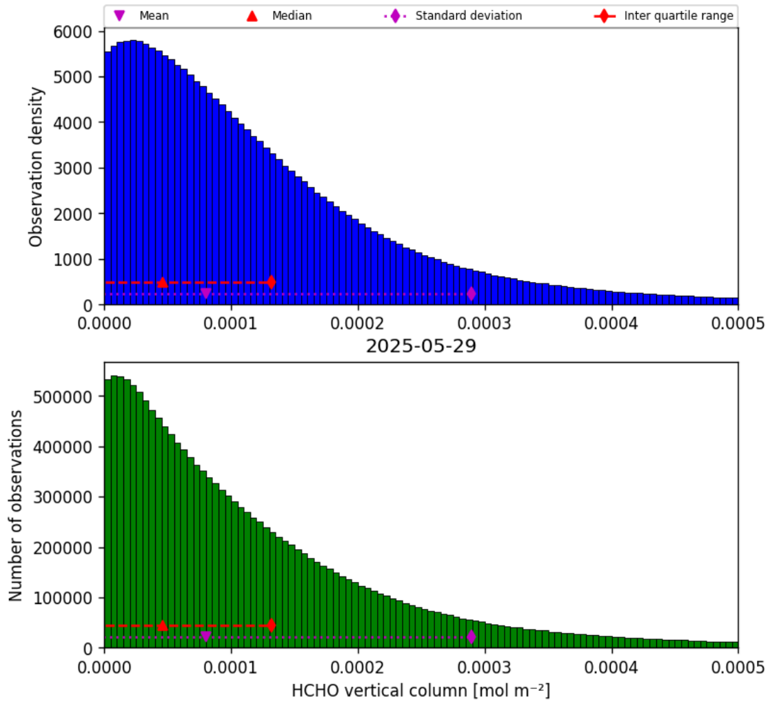
Figure 33: Histogram of “HCHO vertical column” for 2025-05-29 to 2025-05-29
