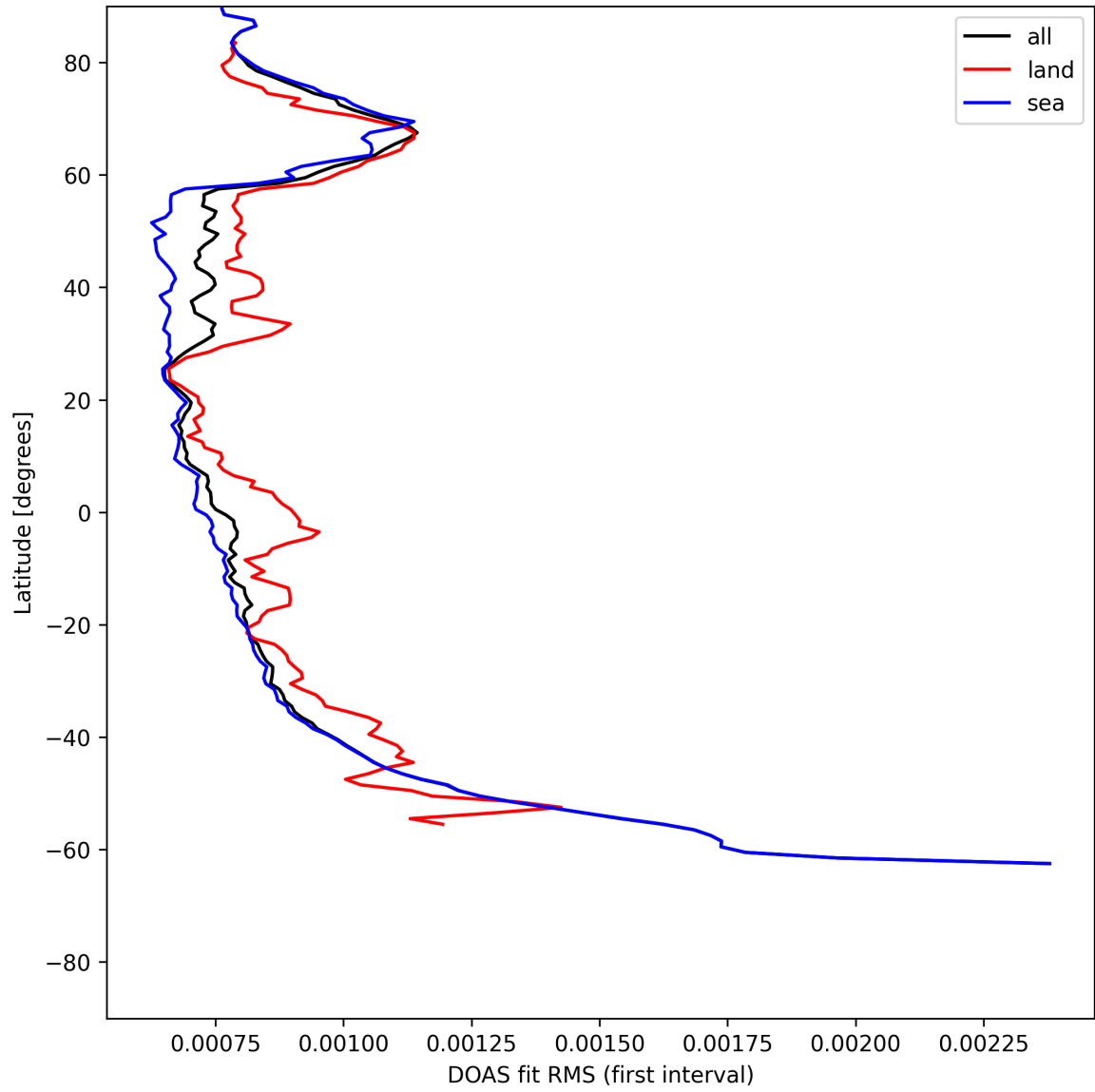
Figure 30: Zonal average of “DOAS fit RMS (first interval)” for 2025-05-29 to 2025-05-29.
