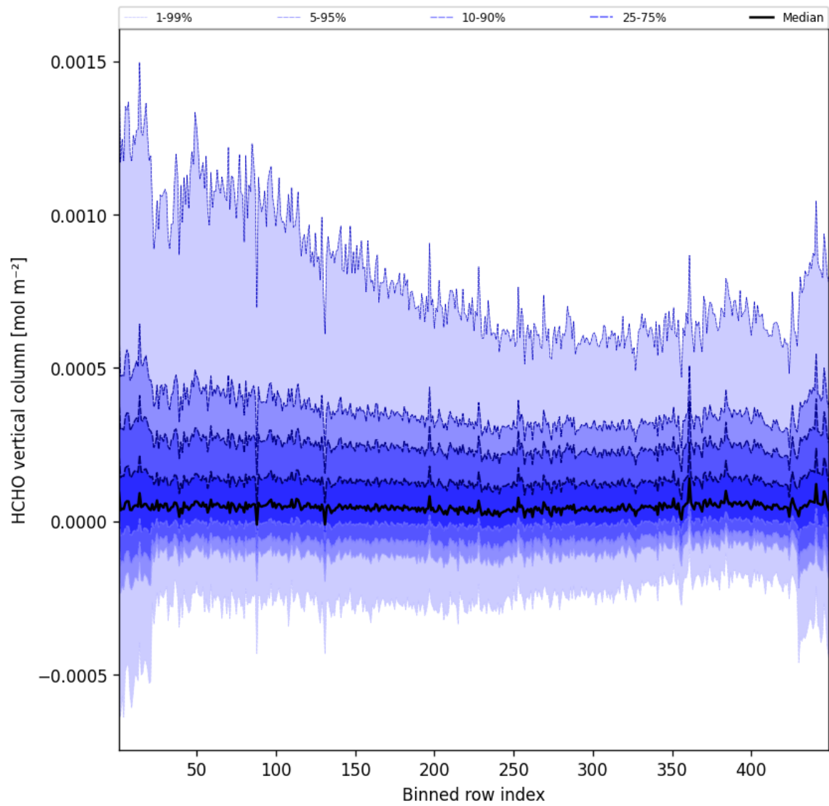
Figure 47: Along track statistics of “HCHO vertical column” for 2025-05-29 to 2025-05-29
