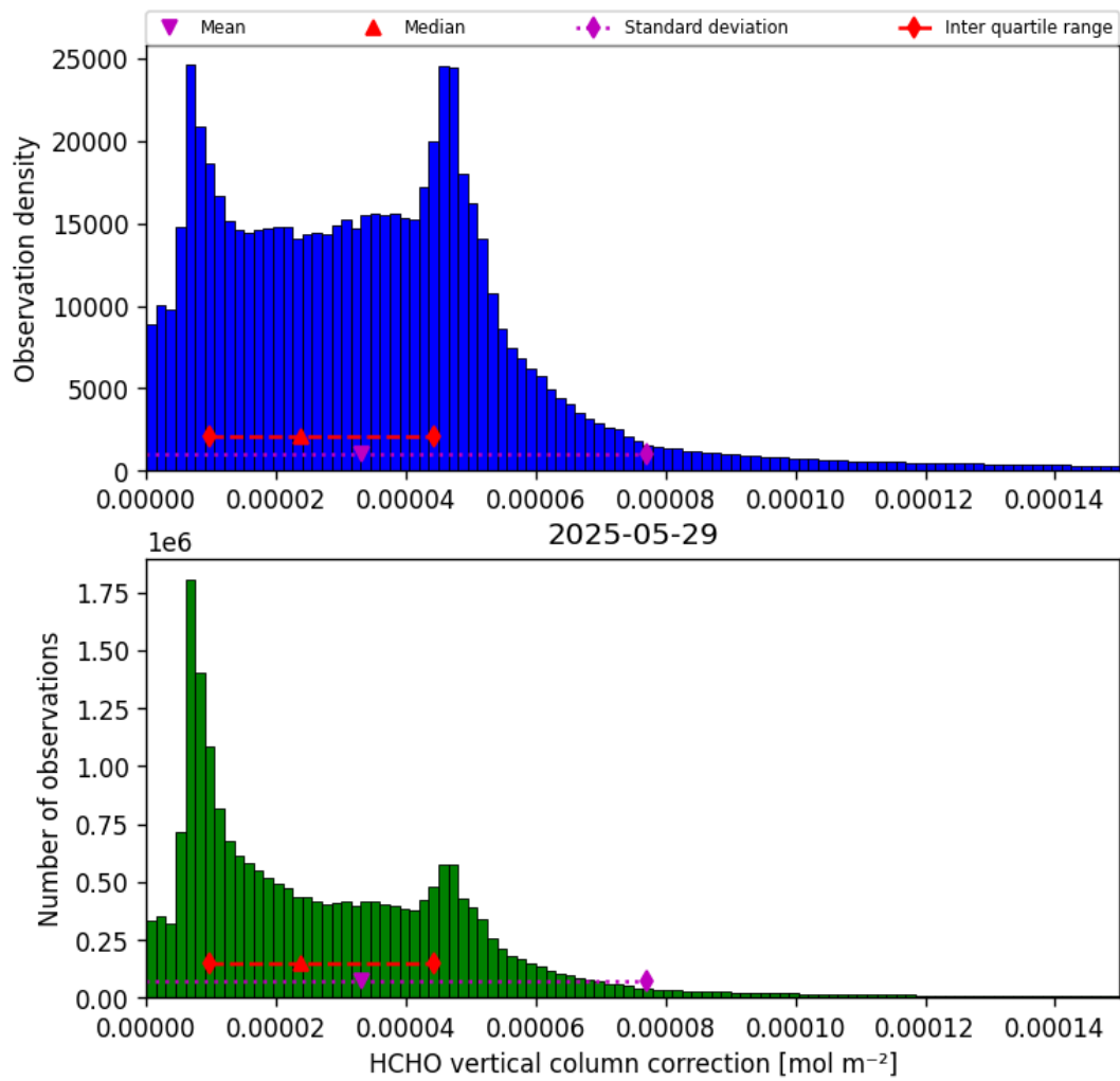
Figure 35: Histogram of “HCHO vertical column correction” for 2025-05-29 to 2025-05-29
