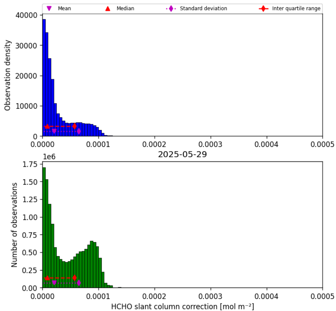
Figure 45: Histogram of “HCHO slant column correction” for 2025-05-29 to 2025-05-29
