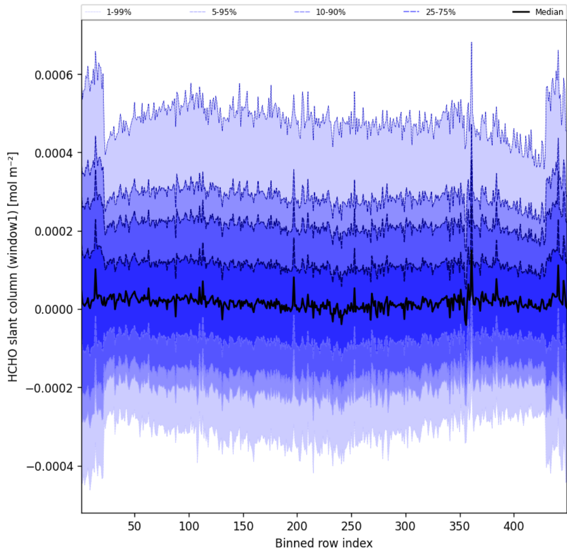
Figure 50: Along track statistics of “HCHO slant column (window1)” for 2025-05-29 to 2025-05-29
