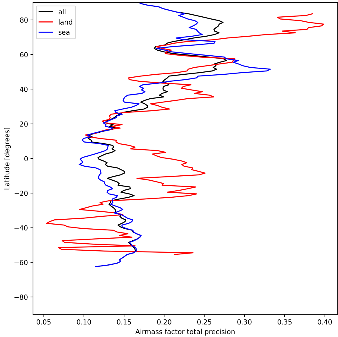
Figure 25: Zonal average of “Airmass factor total precision” for 2025-05-29 to 2025-05-29.
