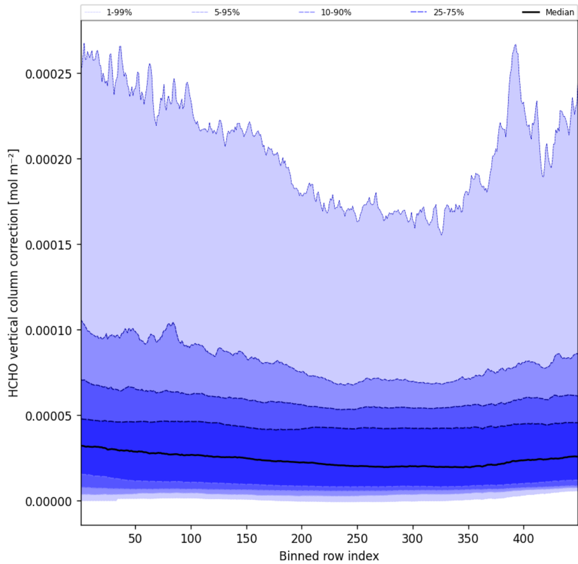
Figure 49: Along track statistics of "HCHO vertical column correction" for 2025-05-29 to 2025-05-29
