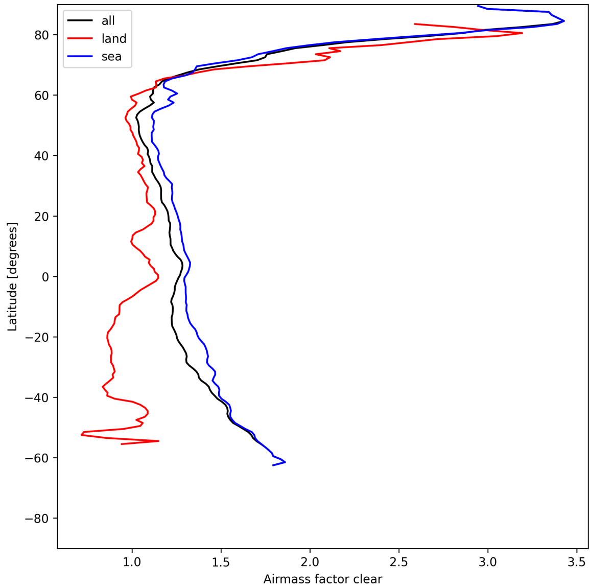
Figure 26: Zonal average of “Airmass factor clear” for 2025-05-29 to 2025-05-29.
