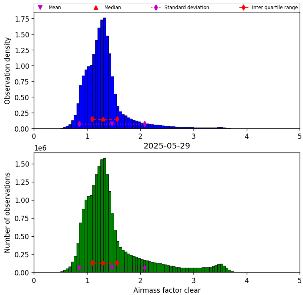
Figure 40: Histogram of “Airmass factor clear” for 2025-05-29 to 2025-05-29
