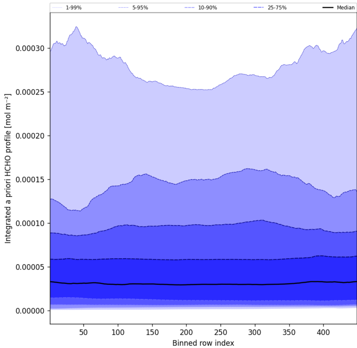
Figure 55: Along track statistics of "Integrated a priori HCHO profile" for 2025-05-29 to 2025-05-29
