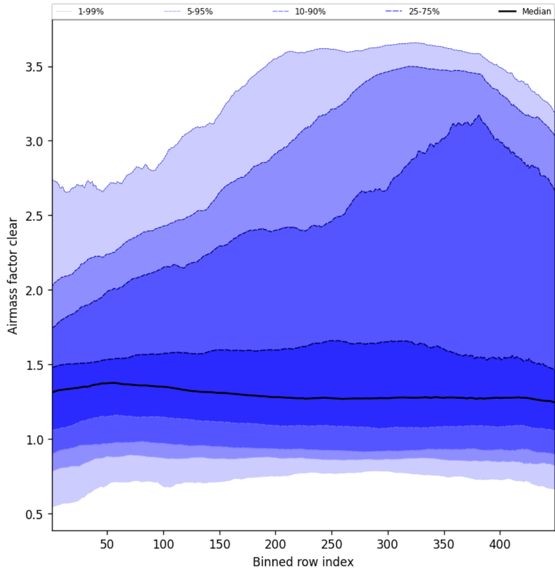
Figure 54: Along track statistics of “Airmass factor clear” for 2025-05-29 to 2025-05-29
