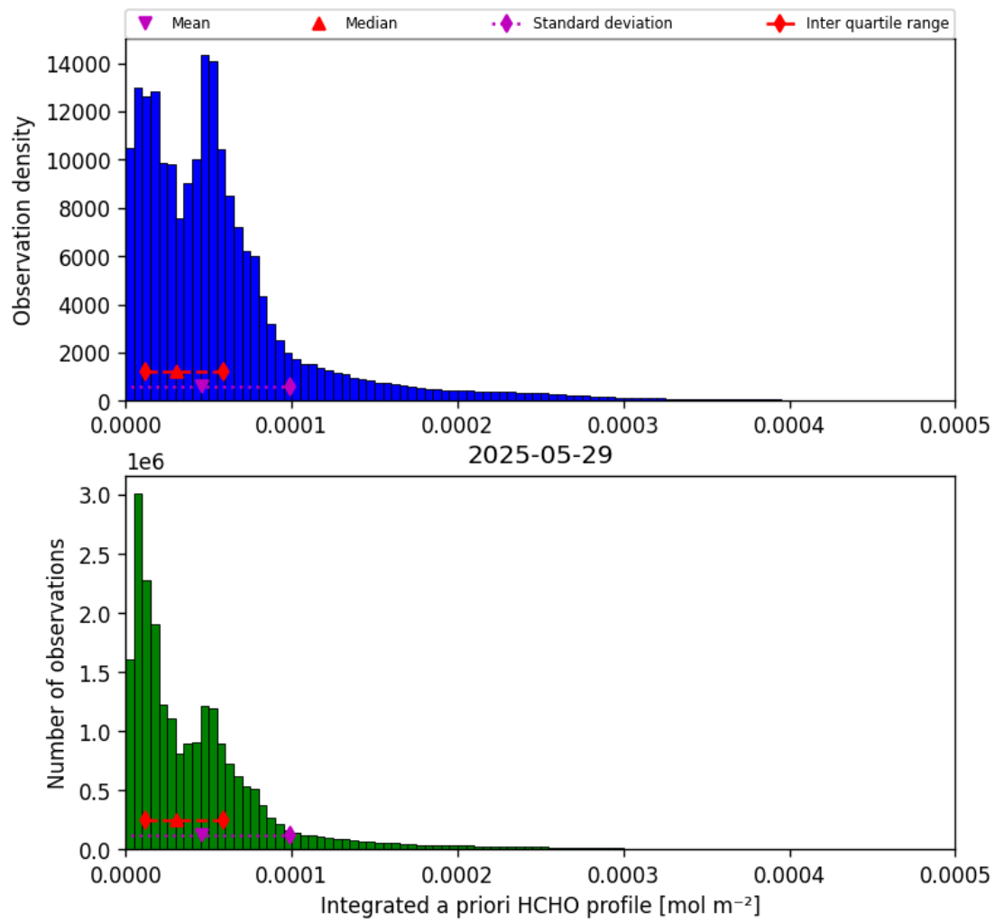
Figure 41: Histogram of “Integrated a priori HCHO profile” for 2025-05-29 to 2025-05-29
