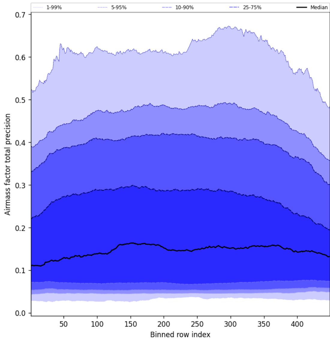
Figure 53: Along track statistics of “Airmass factor total precision” for 2025-05-29 to 2025-05-29
