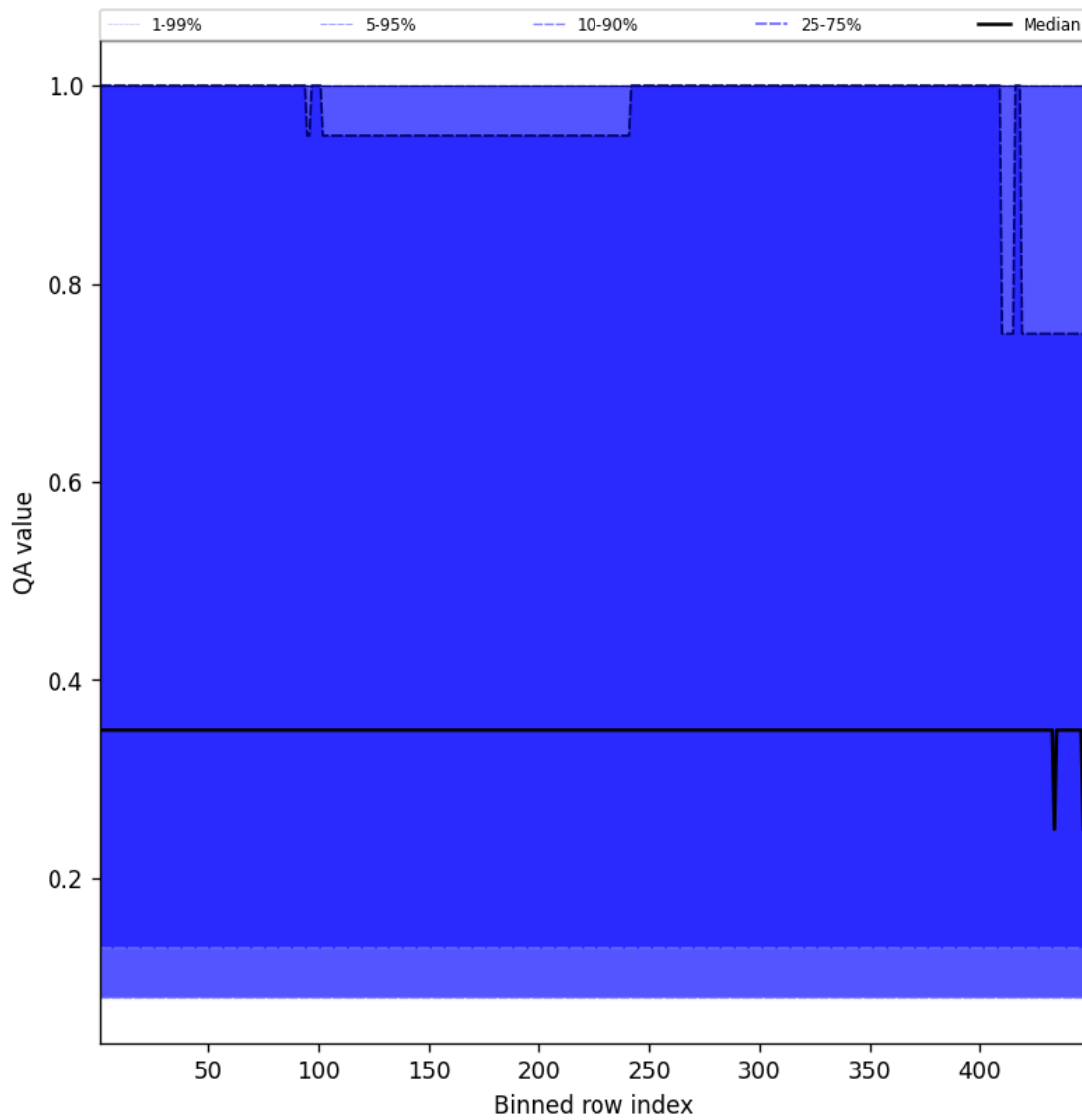
Figure 46: Along track statistics of “QA value” for 2025-05-29 to 2025-05-29
