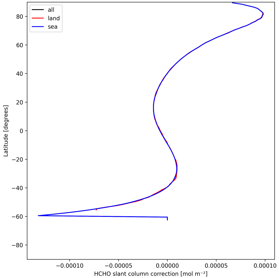
Figure 31: Zonal average of "HCHO slant column correction" for 2025-05-29 to 2025-05-29.
