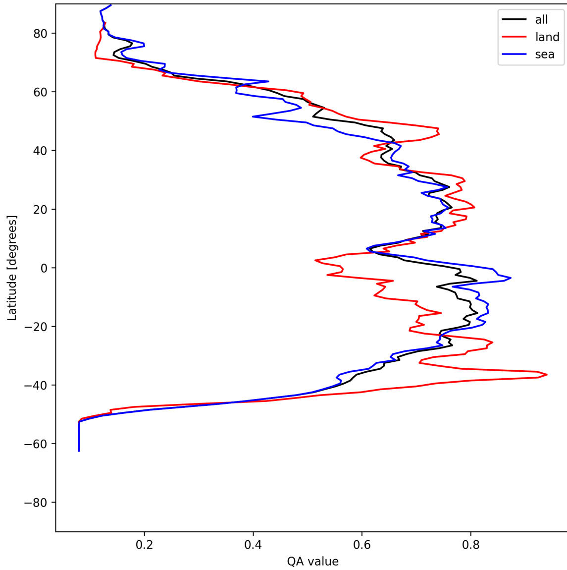
Figure 18: Zonal average of “QA value” for 2025-05-29 to 2025-05-29.
