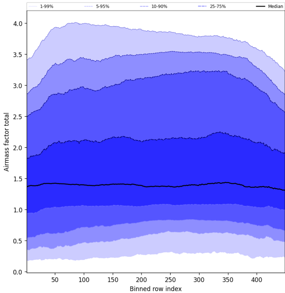
Figure 52: Along track statistics of “Airmass factor total” for 2025-05-29 to 2025-05-29
