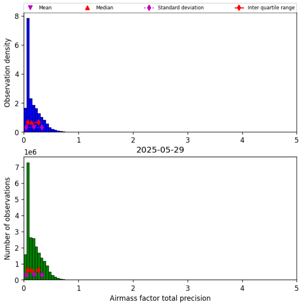
Figure 39: Histogram of “Airmass factor total precision” for 2025-05-29 to 2025-05-29
