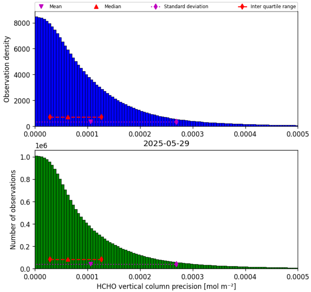
Figure 34: Histogram of “HCHO vertical column precision” for 2025-05-29 to 2025-05-29
