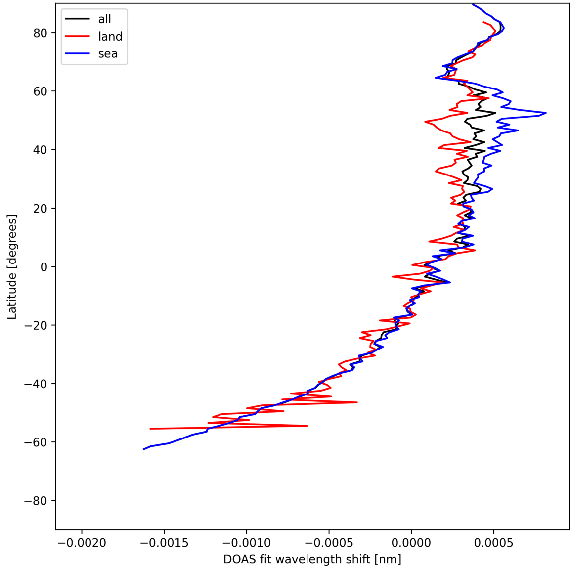
Figure 28: Zonal average of “DOAS fit wavelength shift” for 2025-05-29 to 2025-05-29.
