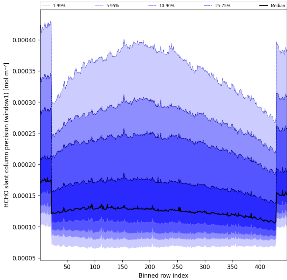
Figure 51: Along track statistics of “HCHO slant column precision (window1)” for 2025-05-29 to 2025-05-29
