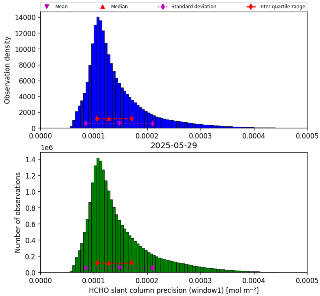
Figure 37: Histogram of “HCHO slant column precision (window1)” for 2025-05-29 to 2025-05-29
