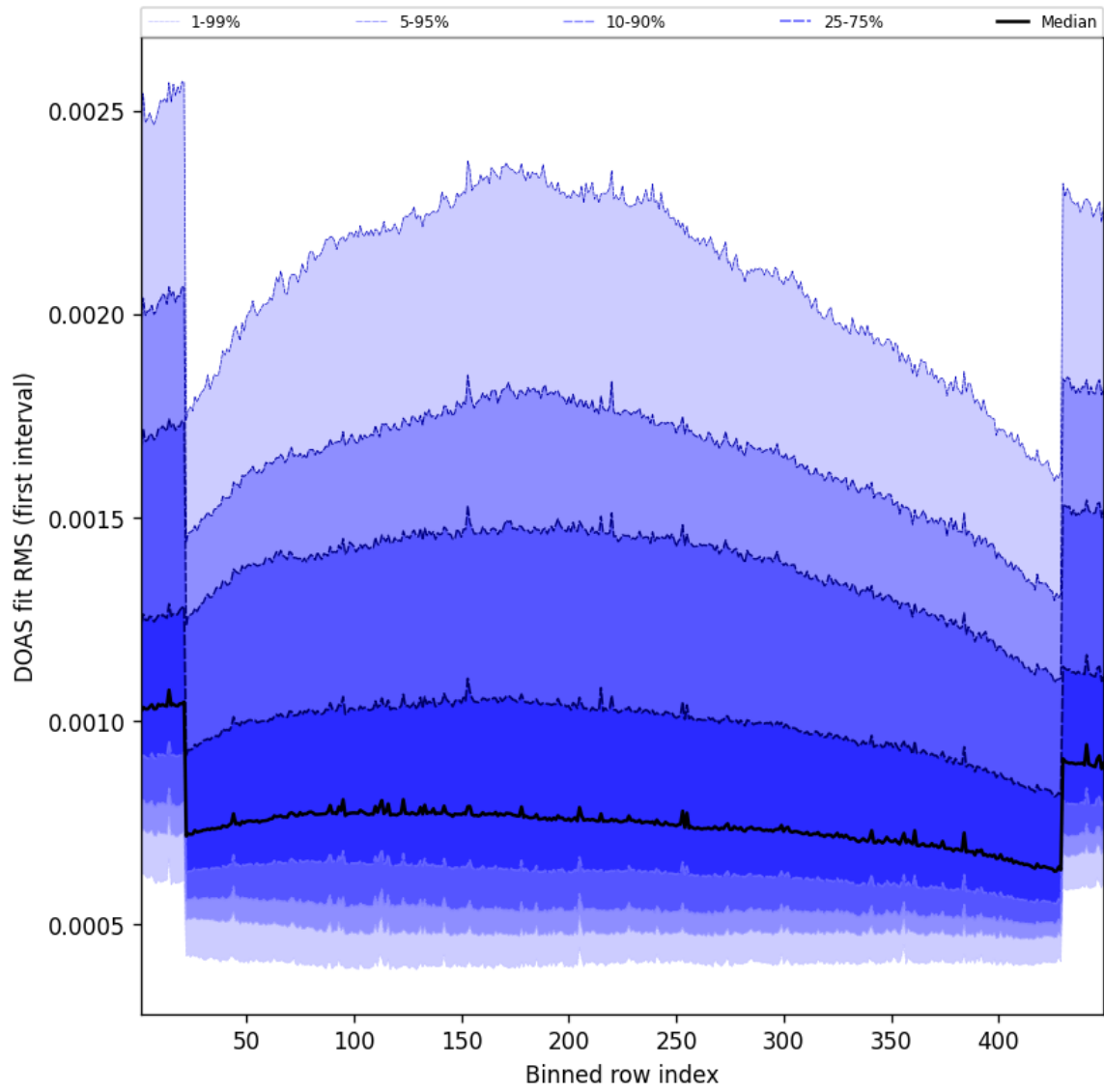
Figure 58: Along track statistics of “DOAS fit RMS (first interval)” for 2025-05-29 to 2025-05-29
