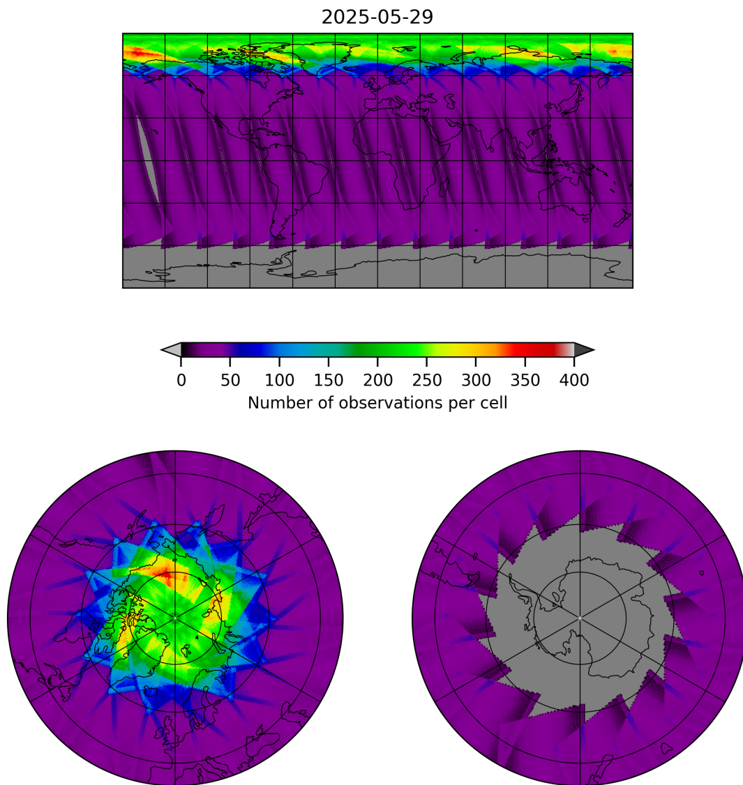
Figure 17: Map of the number of observations for 2025-05-29 to 2025-05-29
