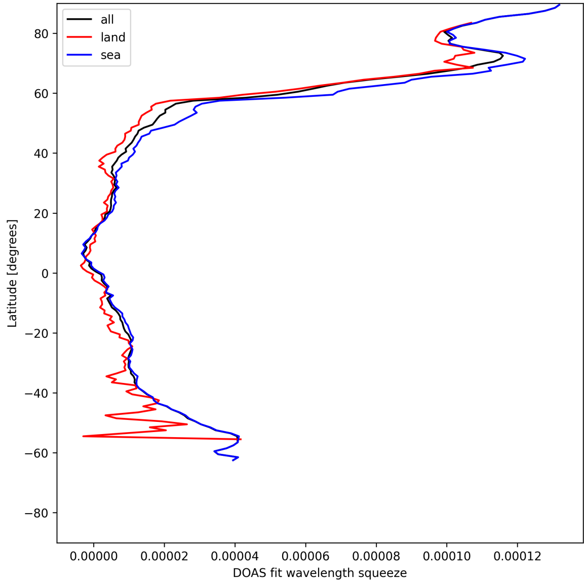
Figure 29: Zonal average of “DOAS fit wavelength squeeze” for 2025-05-29 to 2025-05-29.
