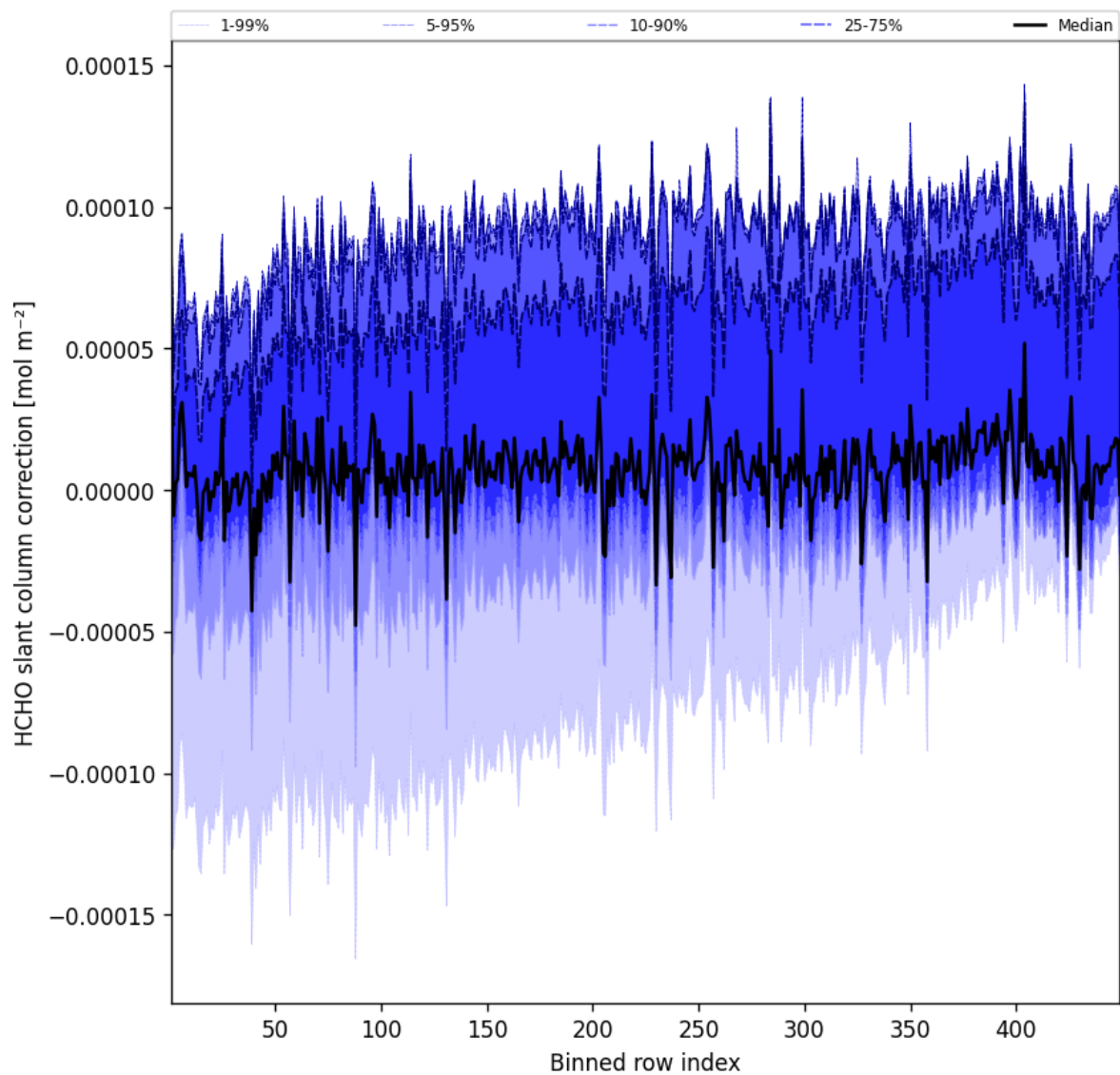
Figure 59: Along track statistics of “HCHO slant column correction” for 2025-05-29 to 2025-05-29
