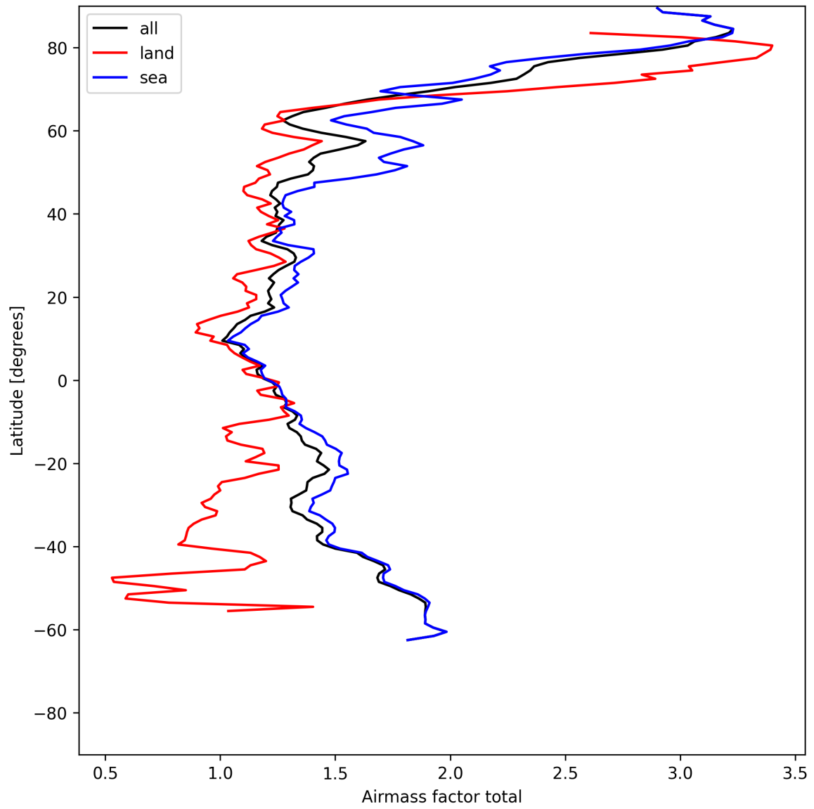
Figure 24: Zonal average of “Airmass factor total” for 2025-05-29 to 2025-05-29.
