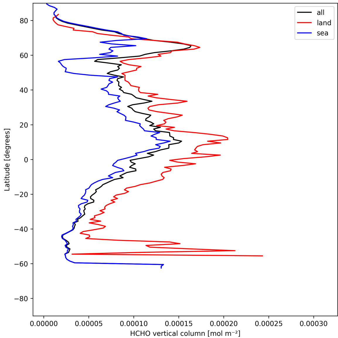
Figure 19: Zonal average of “HCHO vertical column” for 2025-05-29 to 2025-05-29.
