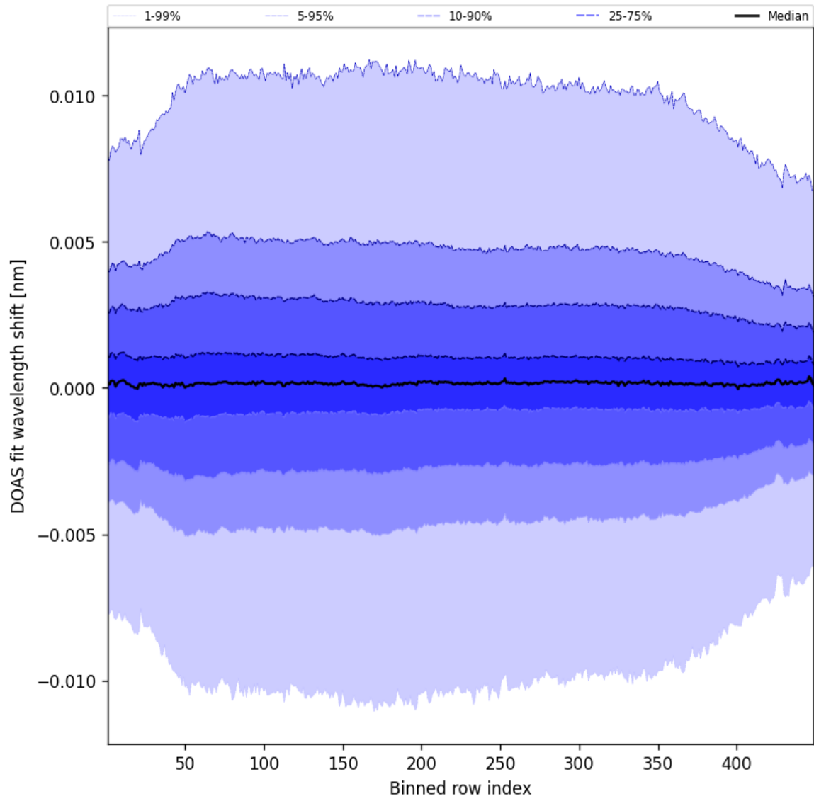
Figure 56: Along track statistics of “DOAS fit wavelength shift” for 2025-05-29 to 2025-05-29
