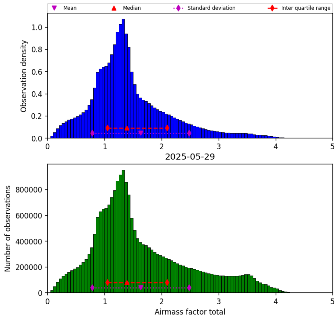
Figure 38: Histogram of “Airmass factor total” for 2025-05-29 to 2025-05-29
