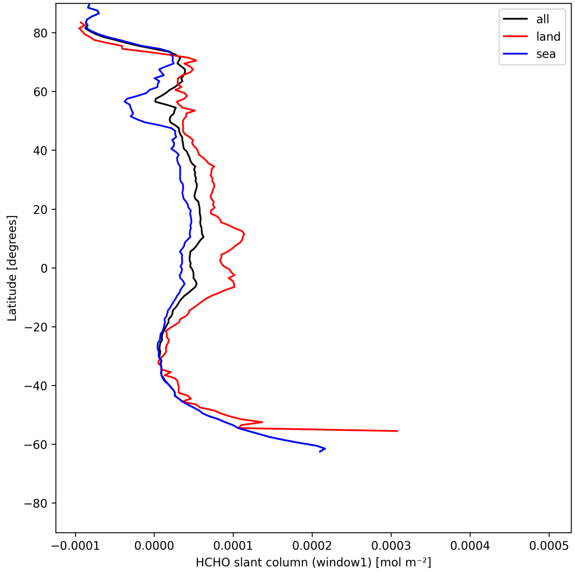
Figure 22: Zonal average of “HCHO slant column (window1)” for 2025-05-29 to 2025-05-29.
