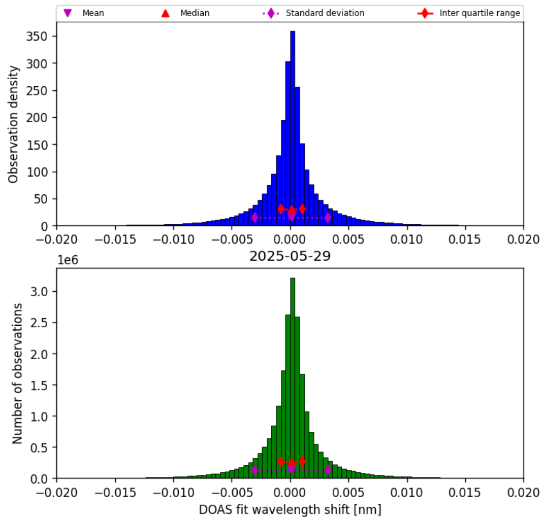
Figure 42: Histogram of “DOAS fit wavelength shift” for 2025-05-29 to 2025-05-29
