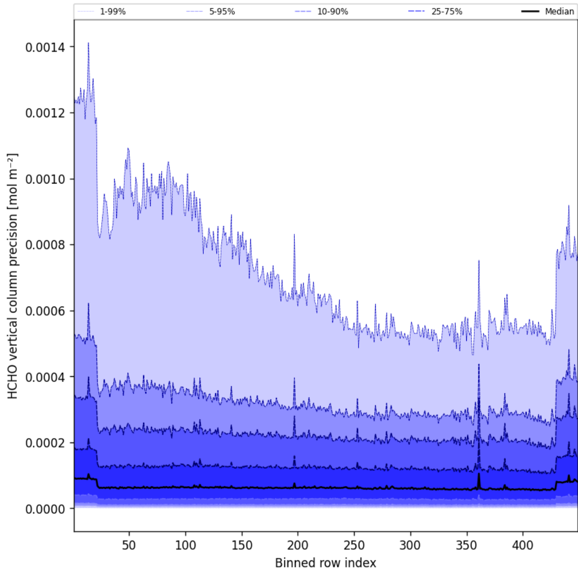
Figure 48: Along track statistics of “HCHO vertical column precision” for 2025-05-29 to 2025-05-29
