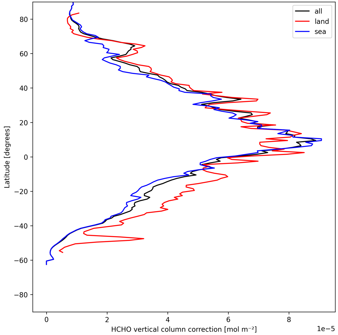
Figure 21: Zonal average of “HCHO vertical column correction” for 2025-05-29 to 2025-05-29.
