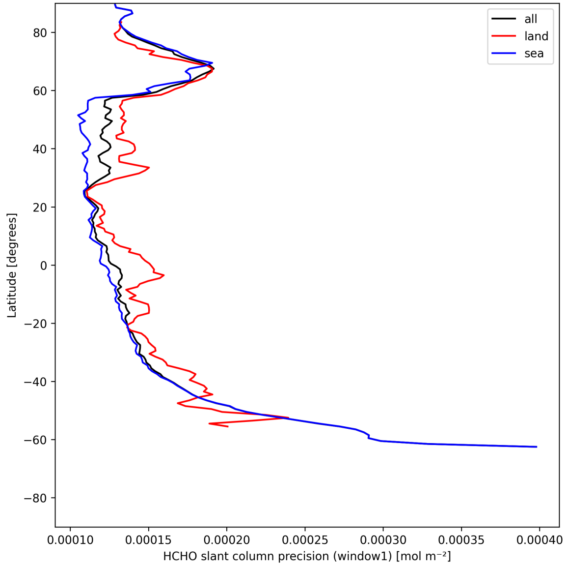
Figure 23: Zonal average of “HCHO slant column precision (window1)” for 2025-05-29 to 2025-05-29.
