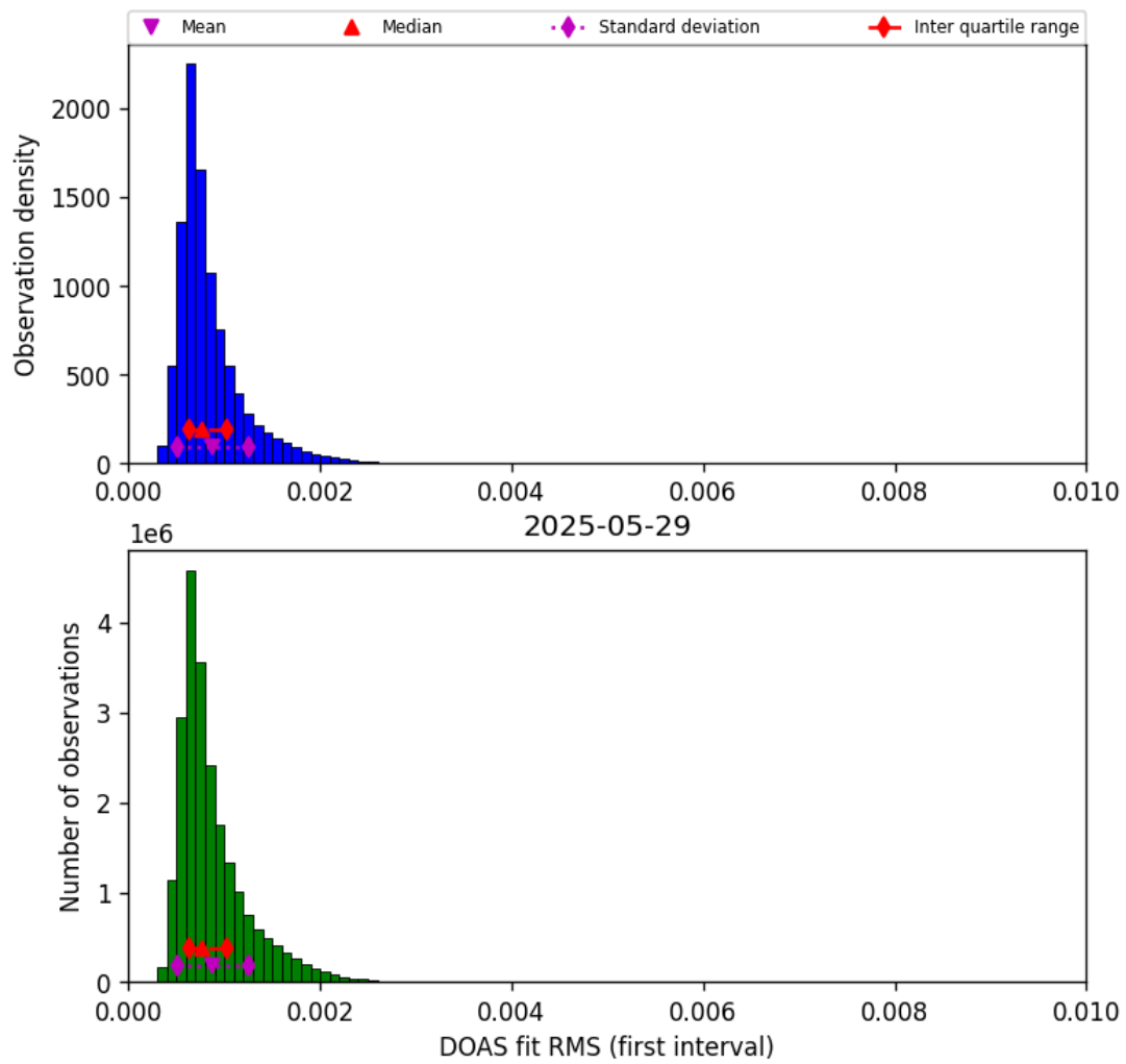
Figure 44: Histogram of “DOAS fit RMS (first interval)” for 2025-05-29 to 2025-05-29
