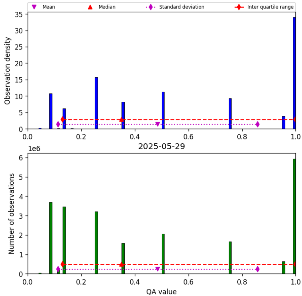
Figure 32: Histogram of “QA value” for 2025-05-29 to 2025-05-29
