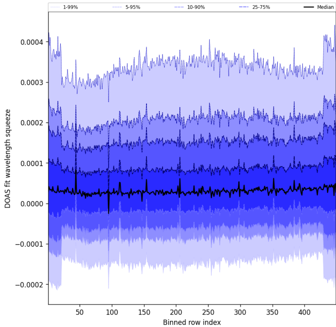
Figure 57: Along track statistics of “DOAS fit wavelength squeeze” for 2025-05-29 to 2025-05-29
