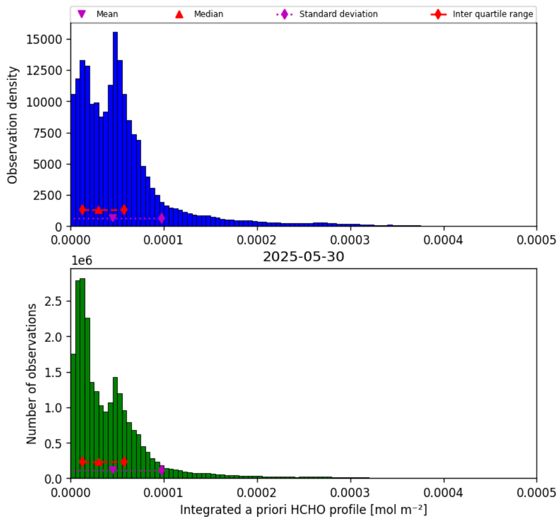
Figure 41: Histogram of “Integrated a priori HCHO profile” for 2025-05-30 to 2025-05-31
