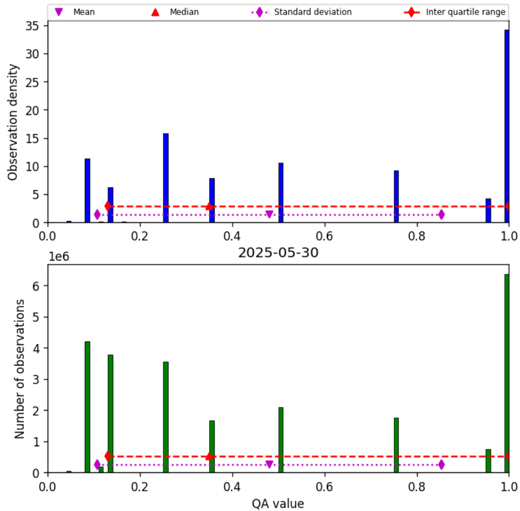
Figure 32: Histogram of “QA value” for 2025-05-30 to 2025-05-31
