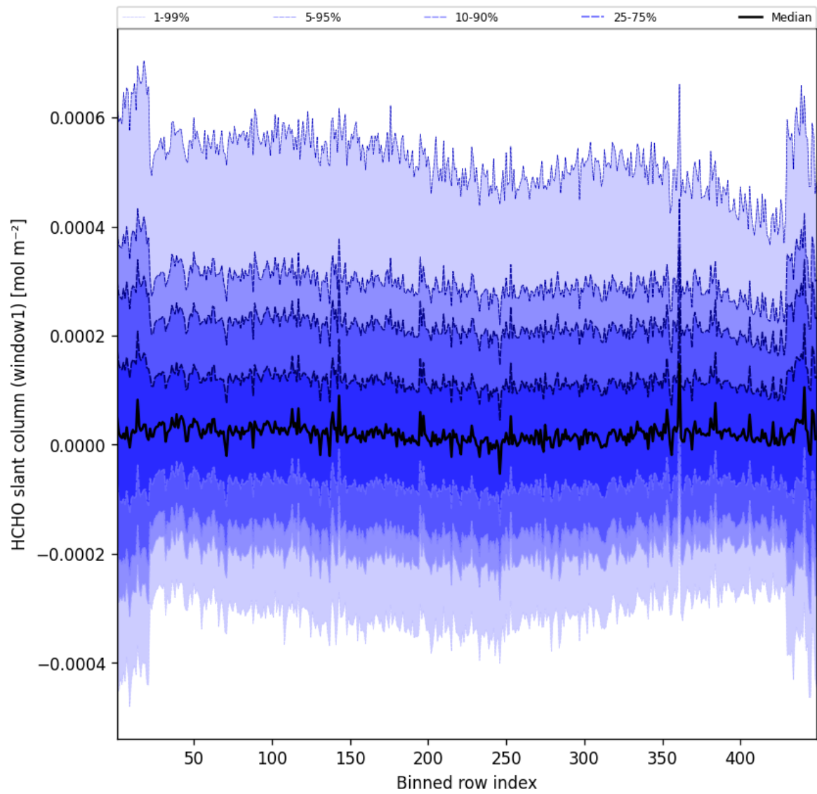
Figure 50: Along track statistics of “HCHO slant column (window1)” for 2025-05-30 to 2025-05-31
