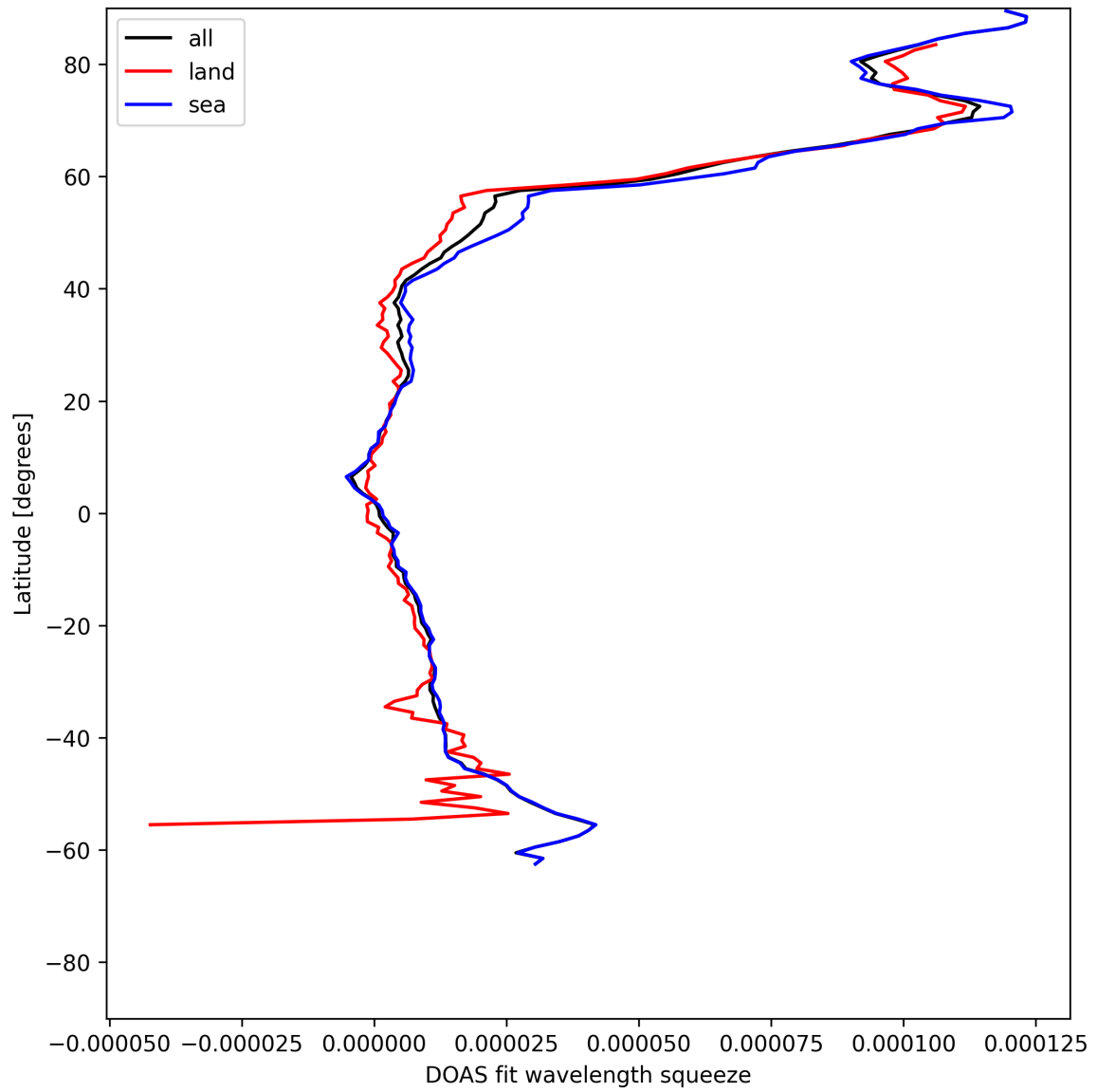
Figure 29: Zonal average of “DOAS fit wavelength squeeze” for 2025-05-30 to 2025-05-31.
