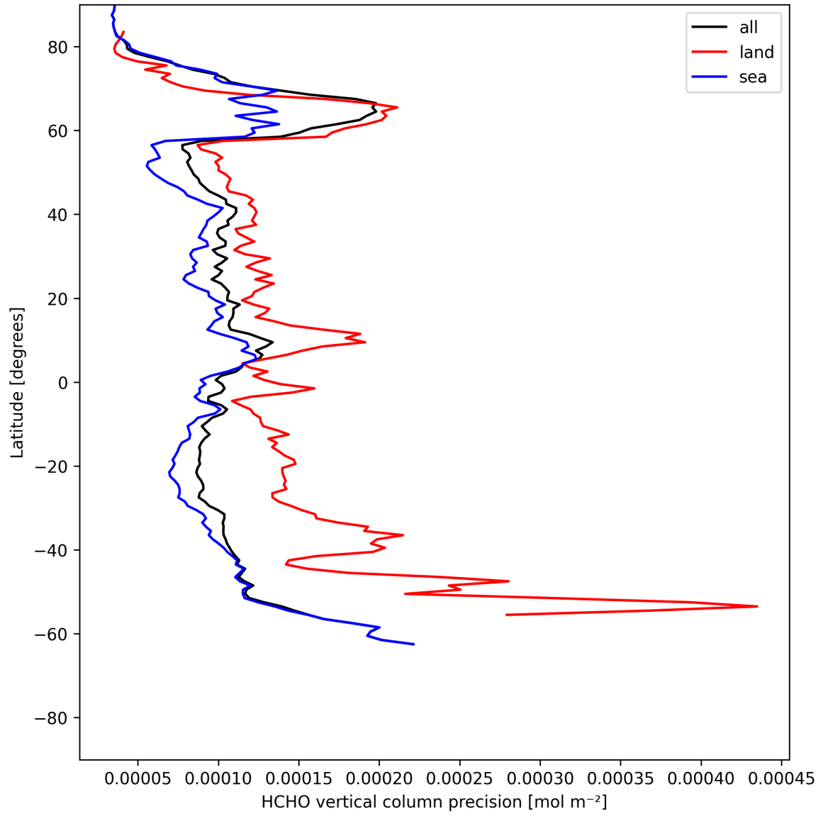
Figure 20: Zonal average of “HCHO vertical column precision” for 2025-05-30 to 2025-05-31.
