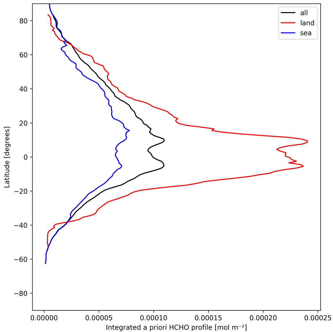
Figure 27: Zonal average of “Integrated a priori HCHO profile” for 2025-05-30 to 2025-05-31.
