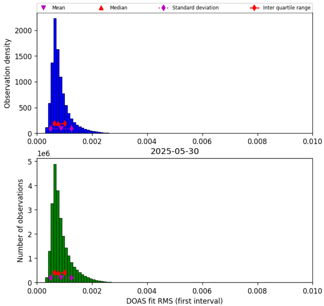
Figure 44: Histogram of “DOAS fit RMS (first interval)” for 2025-05-30 to 2025-05-31
