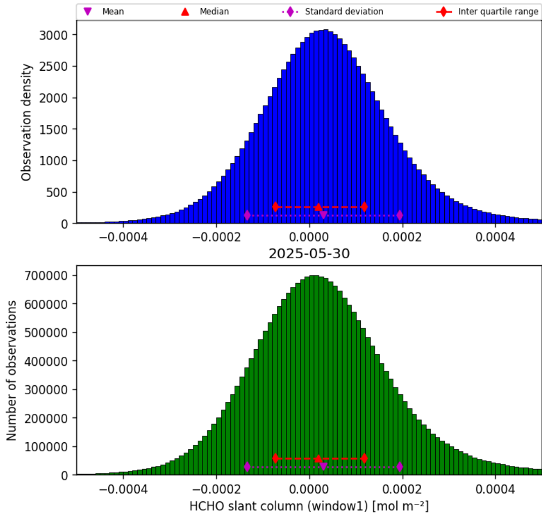
Figure 36: Histogram of “HCHO slant column (window1)” for 2025-05-30 to 2025-05-31
