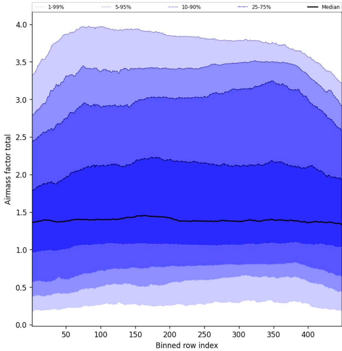
Figure 52: Along track statistics of “Airmass factor total” for 2025-05-30 to 2025-05-31
