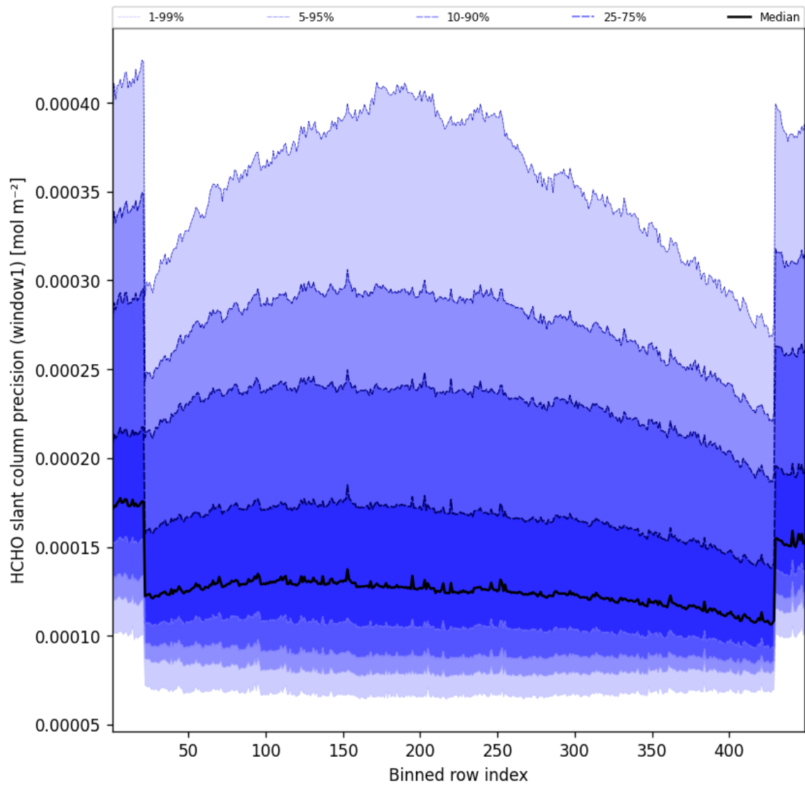
Figure 51: Along track statistics of “HCHO slant column precision (window1)” for 2025-05-30 to 2025-05-31
