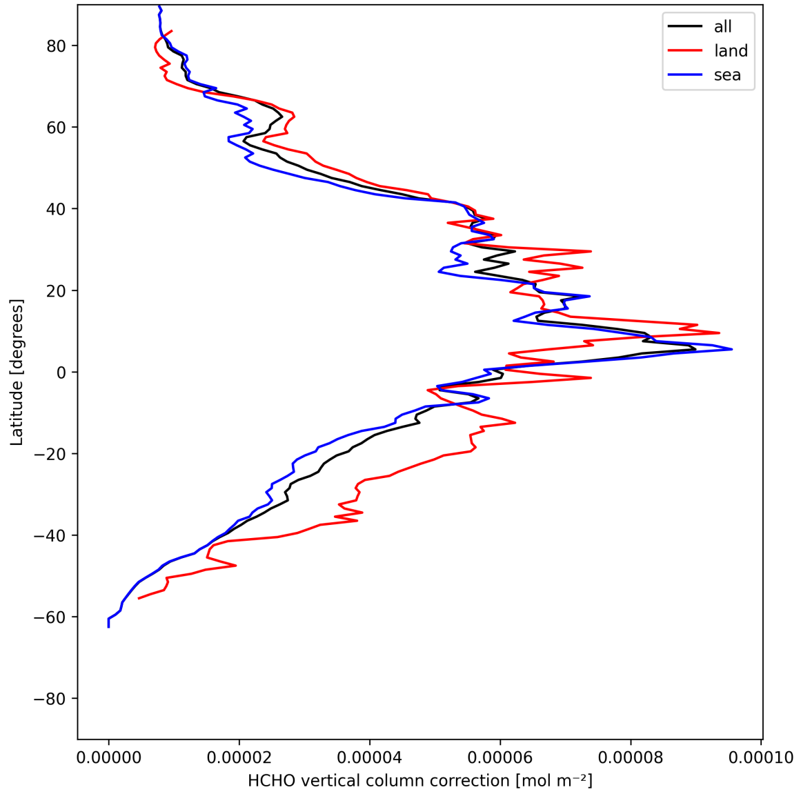
Figure 21: Zonal average of “HCHO vertical column correction” for 2025-05-30 to 2025-05-31.
