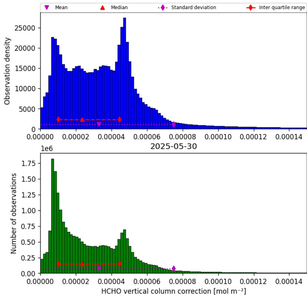
Figure 35: Histogram of “HCHO vertical column correction” for 2025-05-30 to 2025-05-31
