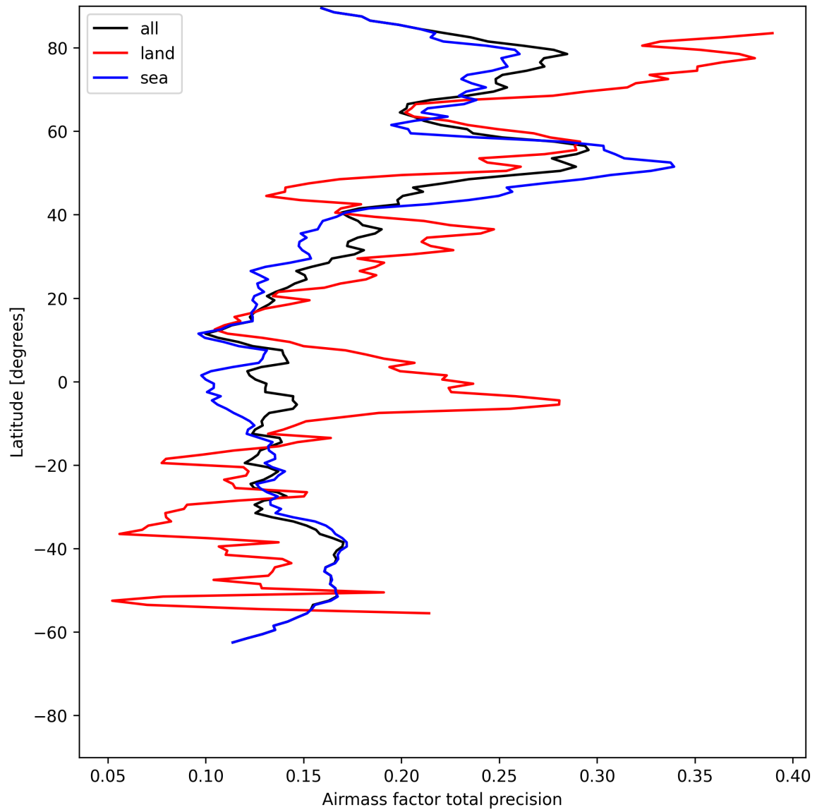
Figure 25: Zonal average of “Airmass factor total precision” for 2025-05-30 to 2025-05-31.
