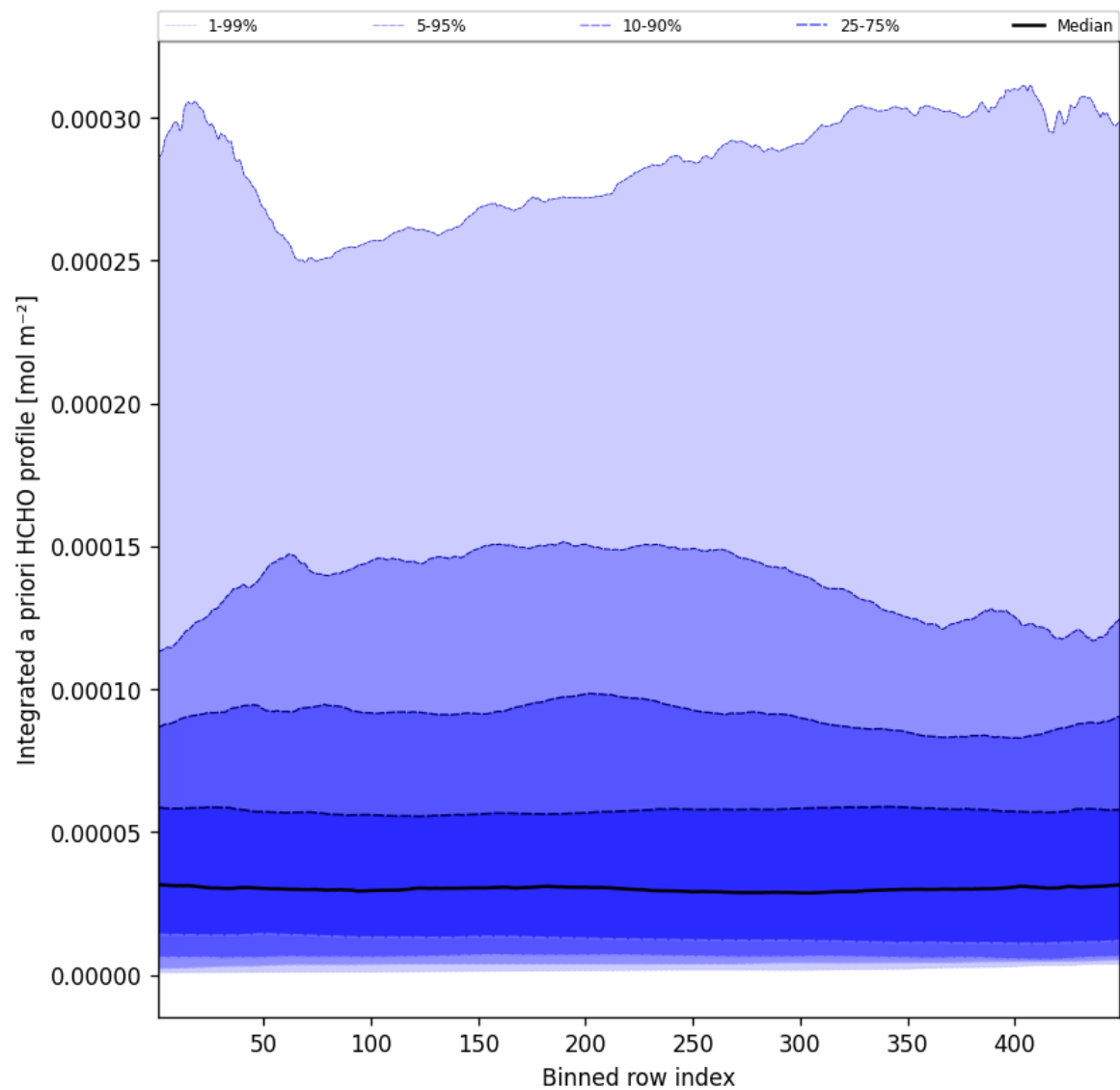
Figure 55: Along track statistics of “Integrated a priori HCHO profile” for 2025-05-30 to 2025-05-31
