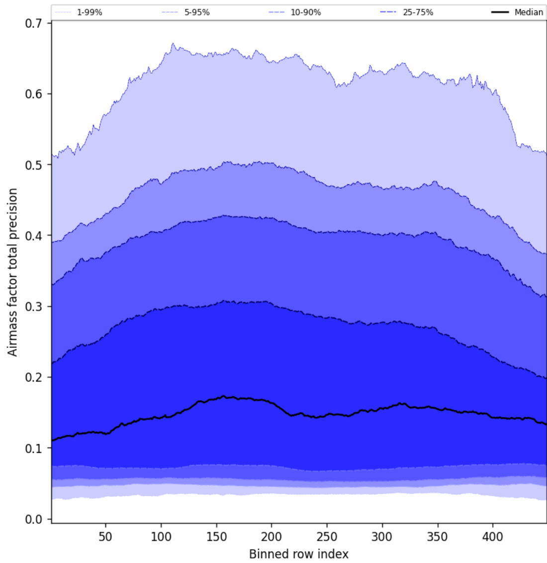
Figure 53: Along track statistics of “Airmass factor total precision” for 2025-05-30 to 2025-05-31
