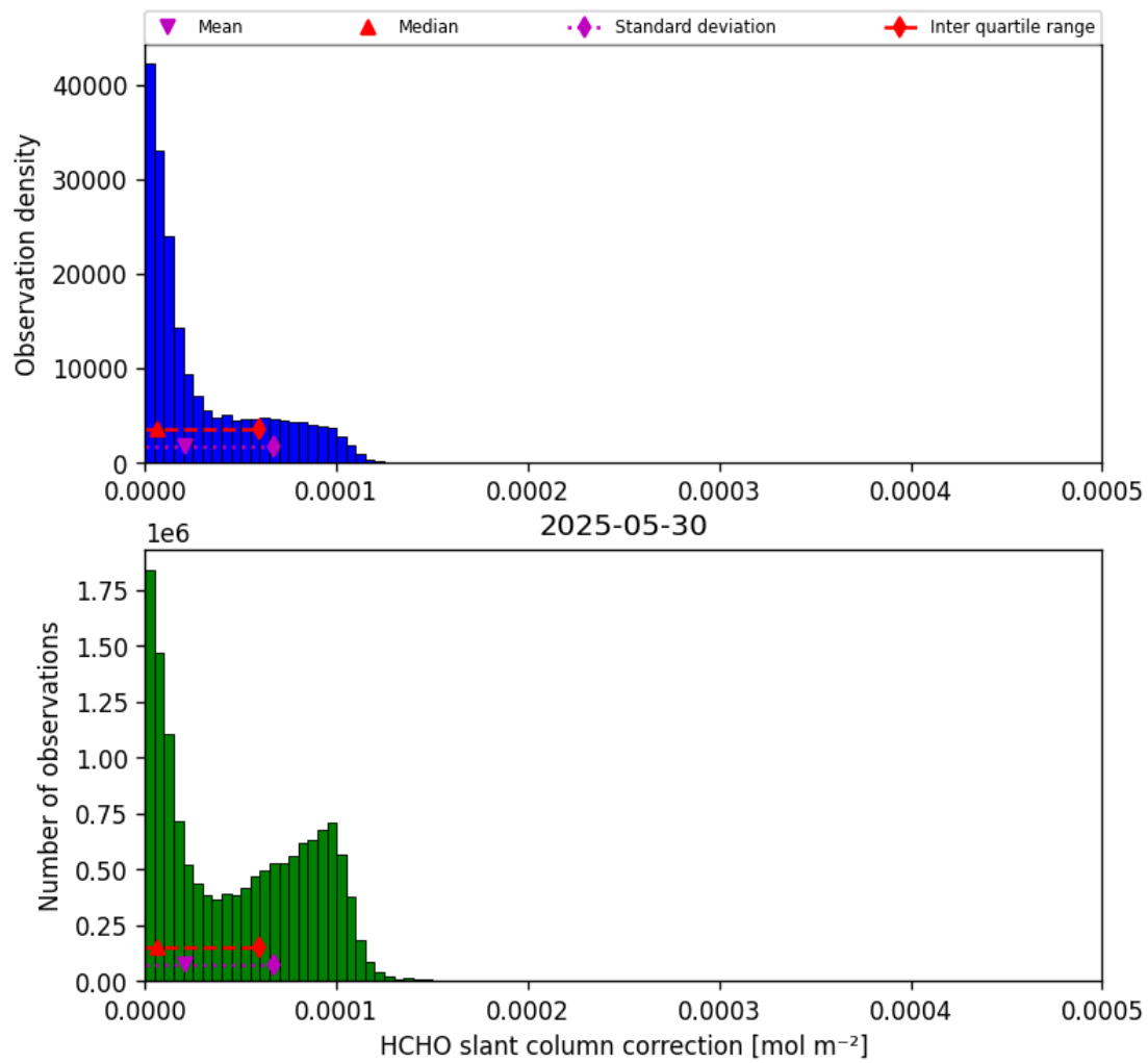
Figure 45: Histogram of “HCHO slant column correction” for 2025-05-30 to 2025-05-31
