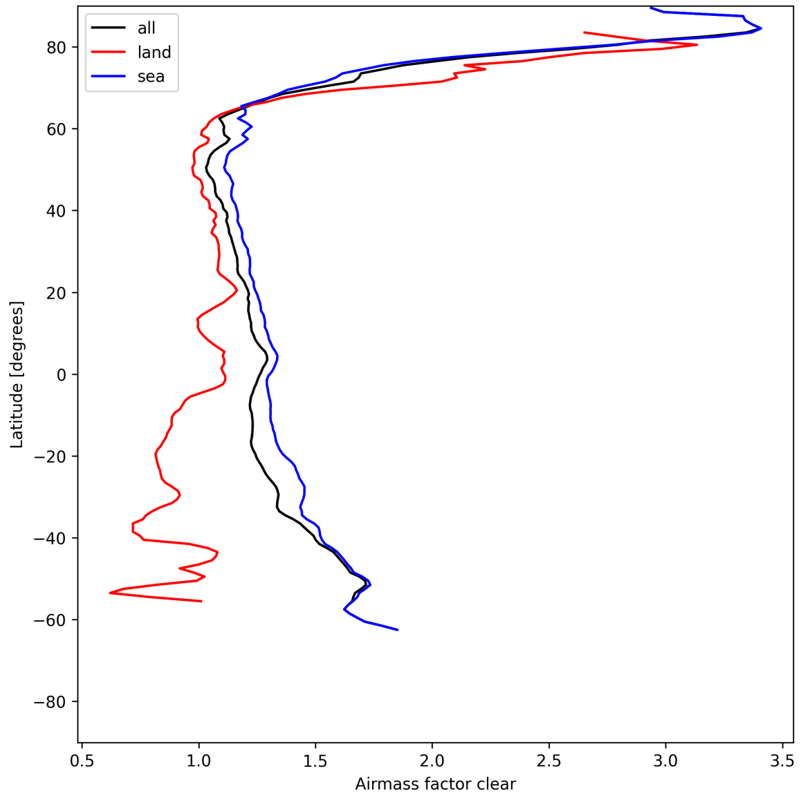
Figure 26: Zonal average of “Airmass factor clear” for 2025-05-30 to 2025-05-31.
