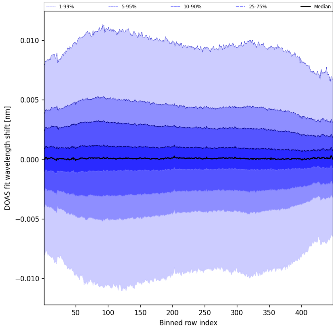
Figure 56: Along track statistics of “DOAS fit wavelength shift” for 2025-05-30 to 2025-05-31
