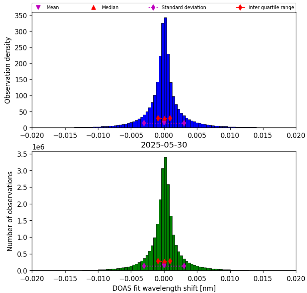
Figure 42: Histogram of “DOAS fit wavelength shift” for 2025-05-30 to 2025-05-31
