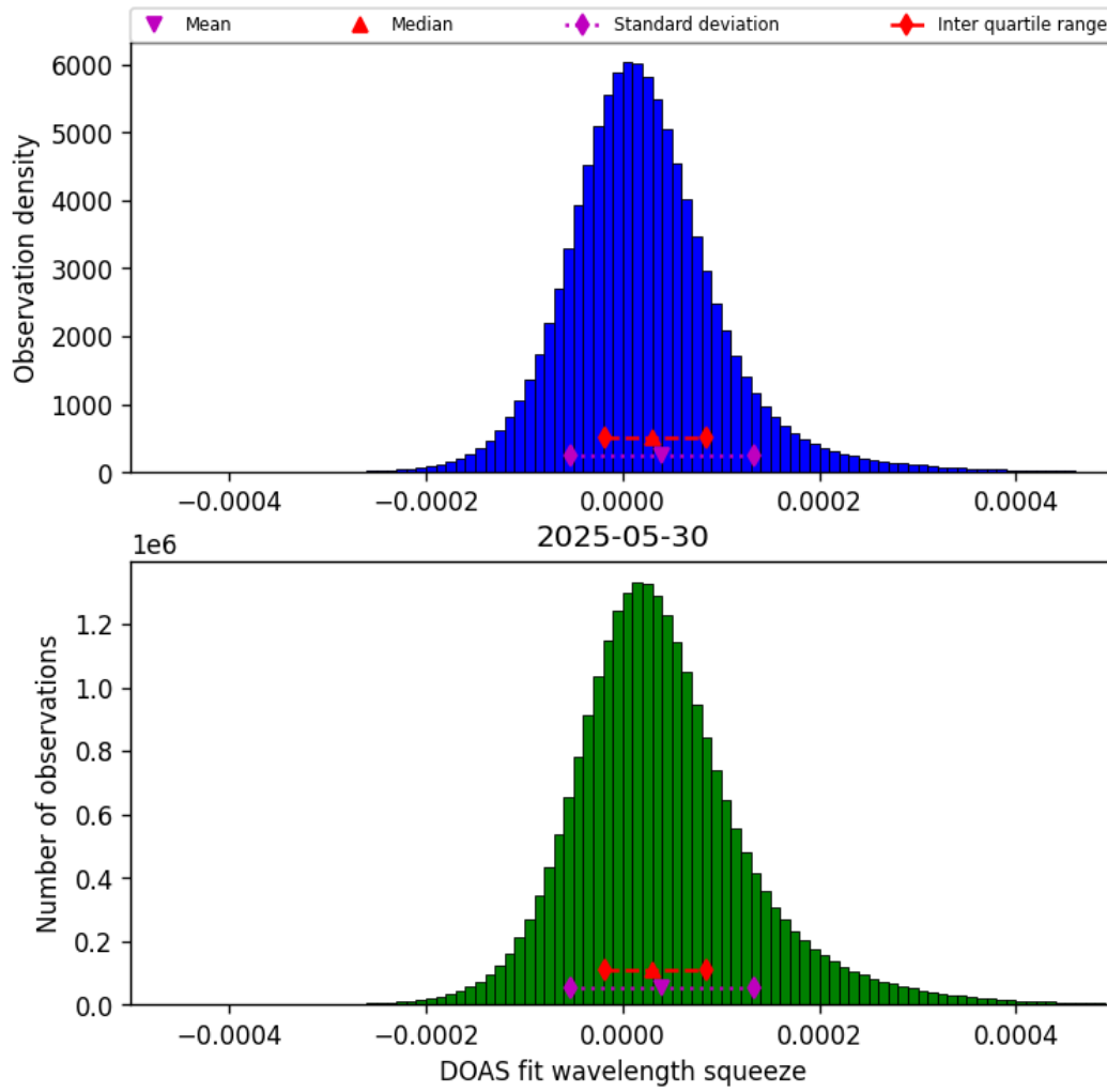
Figure 43: Histogram of “DOAS fit wavelength squeeze” for 2025-05-30 to 2025-05-31
