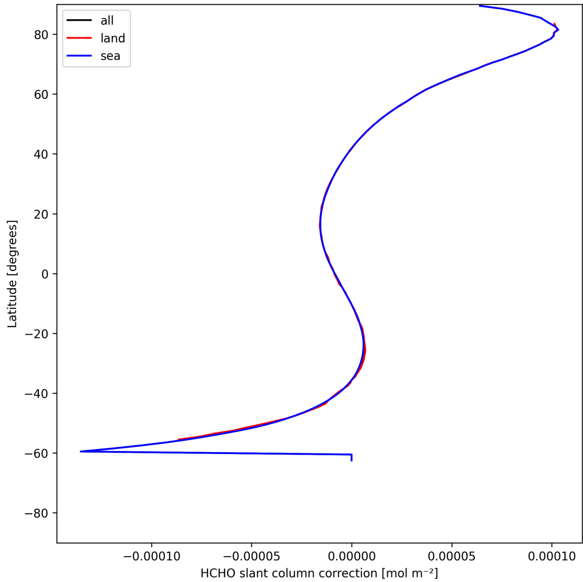
Figure 31: Zonal average of “HCHO slant column correction” for 2025-05-30 to 2025-05-31.
