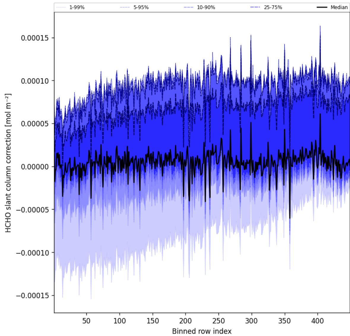
Figure 59: Along track statistics of “HCHO slant column correction” for 2025-05-30 to 2025-05-31
