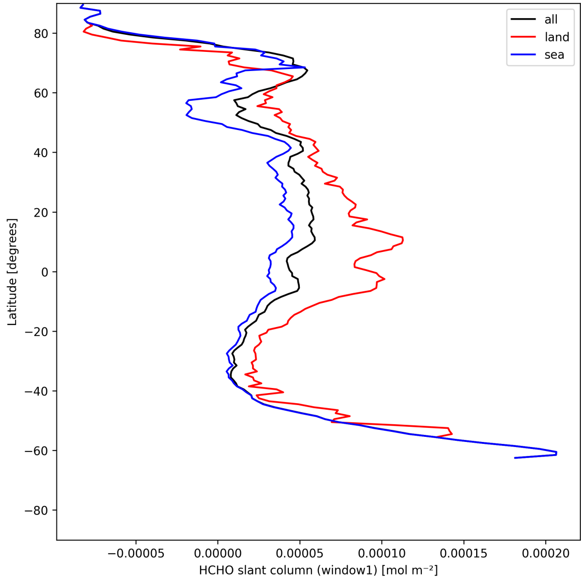
Figure 22: Zonal average of “HCHO slant column (window1)” for 2025-05-30 to 2025-05-31.
