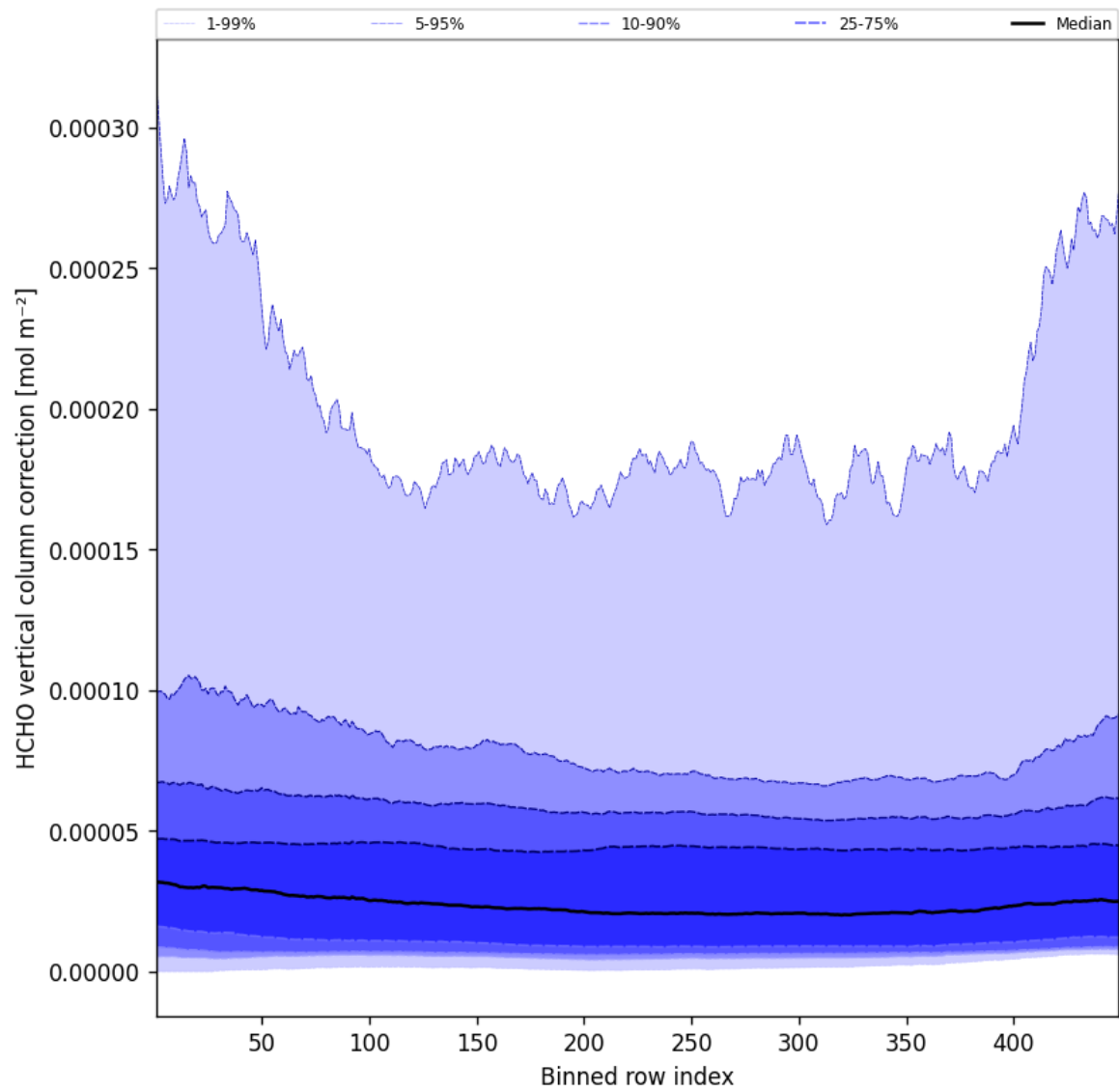
Figure 49: Along track statistics of “HCHO vertical column correction” for 2025-05-30 to 2025-05-31
