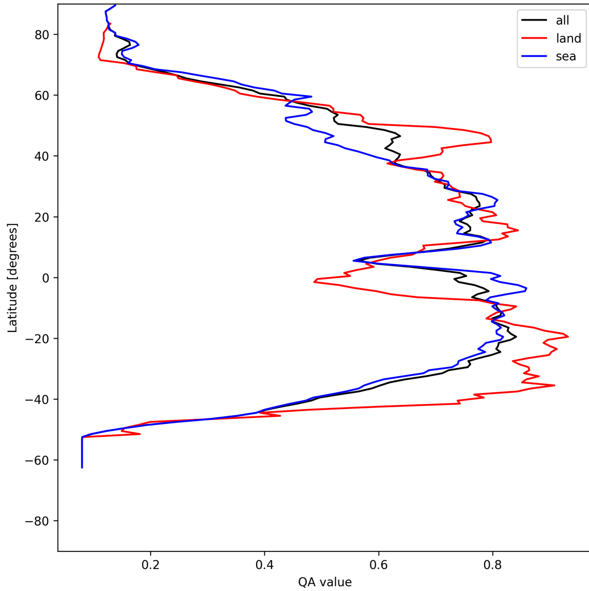
Figure 18: Zonal average of “QA value” for 2025-05-30 to 2025-05-31.
