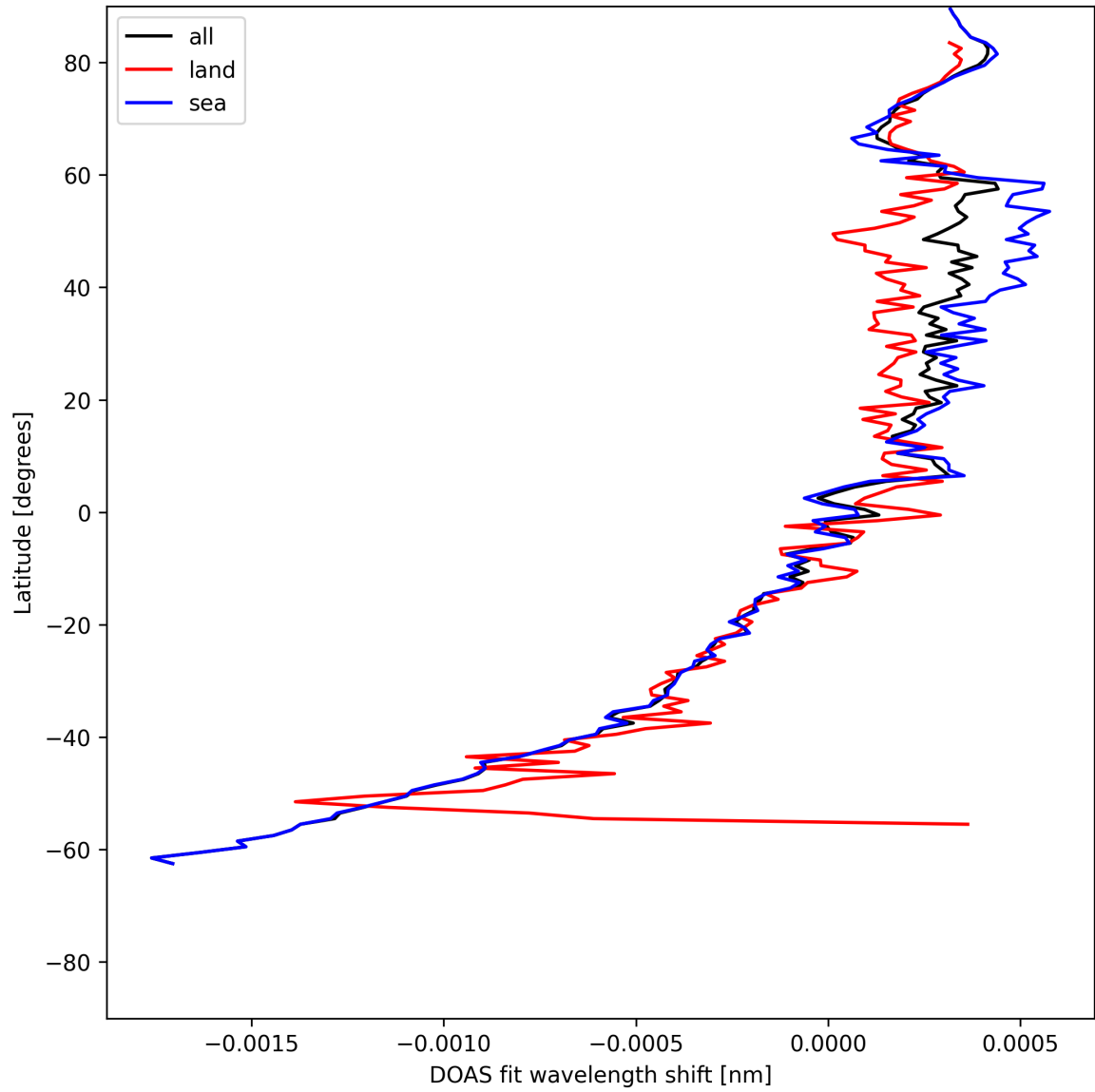
Figure 28: Zonal average of “DOAS fit wavelength shift” for 2025-05-30 to 2025-05-31.
