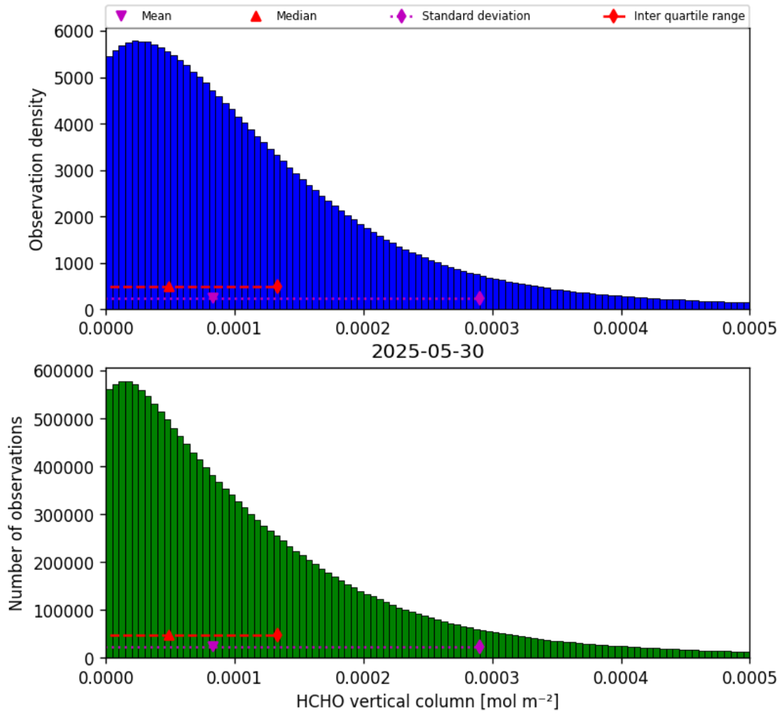
Figure 33: Histogram of “HCHO vertical column” for 2025-05-30 to 2025-05-31
