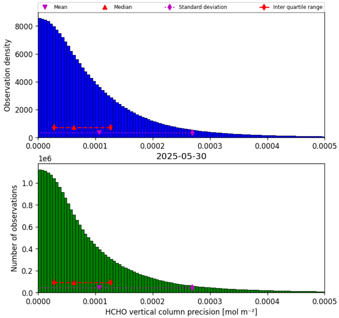
Figure 34: Histogram of “HCHO vertical column precision” for 2025-05-30 to 2025-05-31
