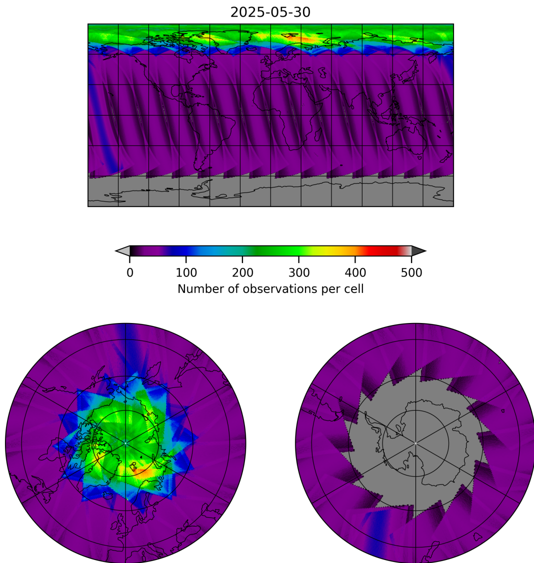
Figure 17: Map of the number of observations for 2025-05-30 to 2025-05-31
