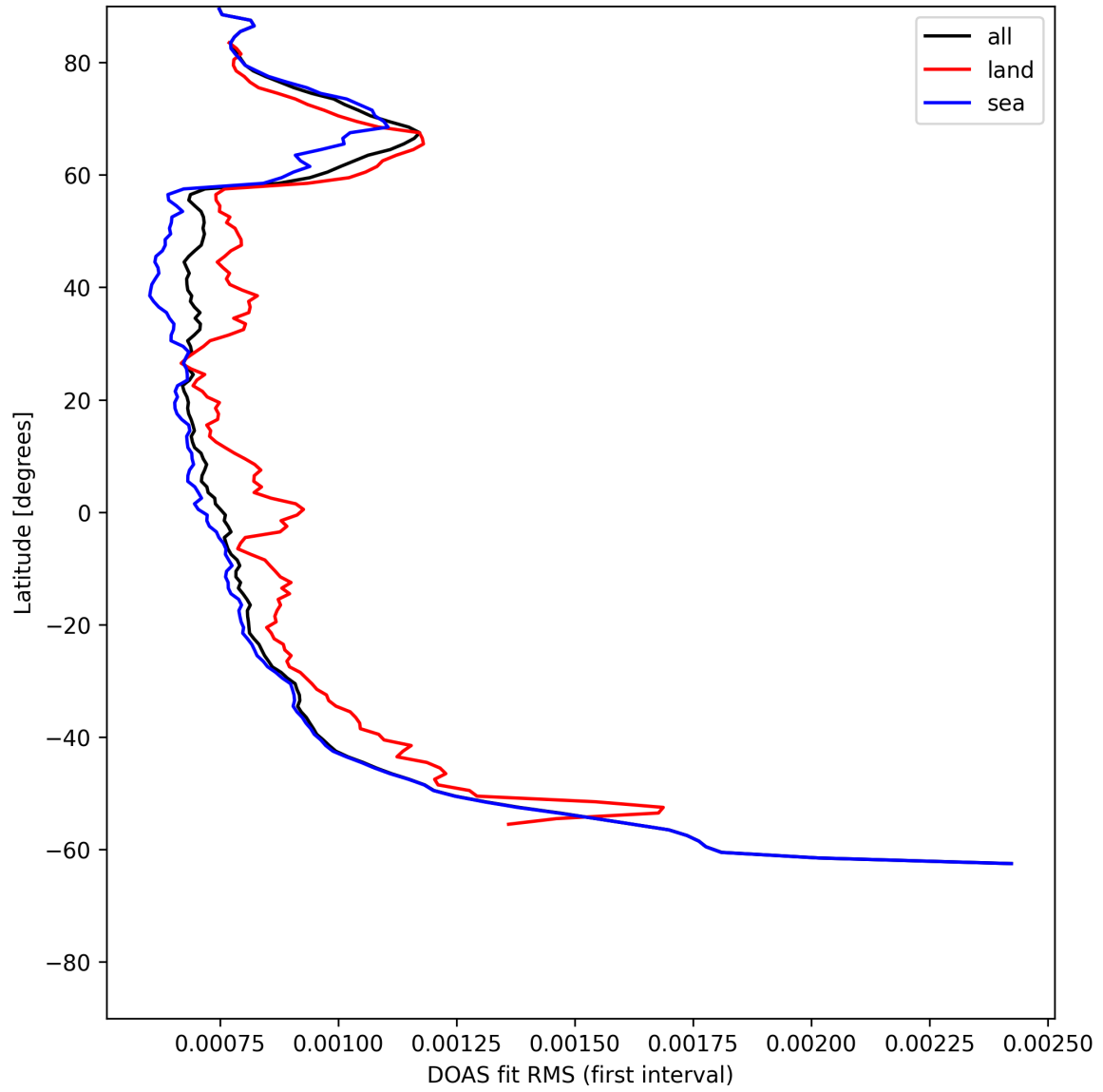
Figure 30: Zonal average of “DOAS fit RMS (first interval)” for 2025-05-30 to 2025-05-31.
