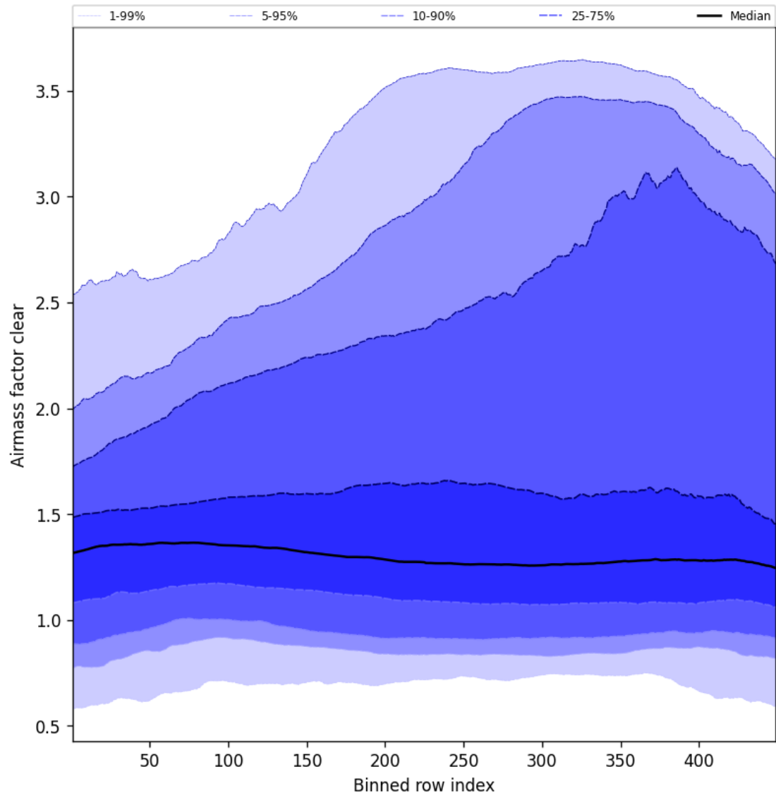
Figure 54: Along track statistics of “Air mass factor clear” for 2025-05-30 to 2025-05-31
