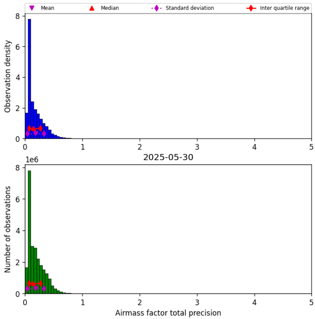
Figure 39: Histogram of “Airmass factor total precision” for 2025-05-30 to 2025-05-31
