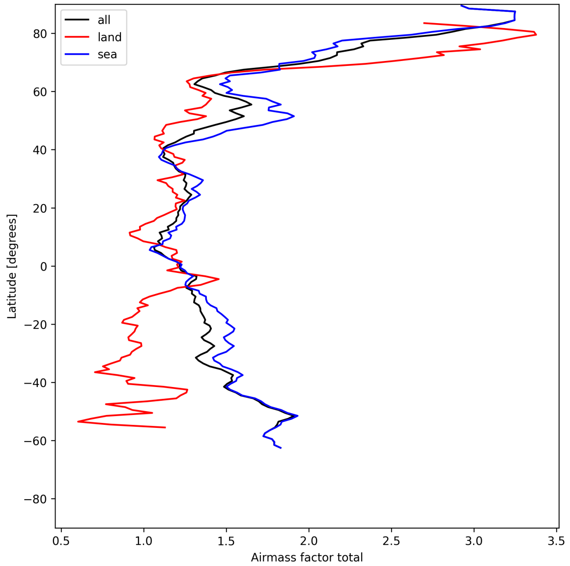
Figure 24: Zonal average of “Airmass factor total” for 2025-05-30 to 2025-05-31.
