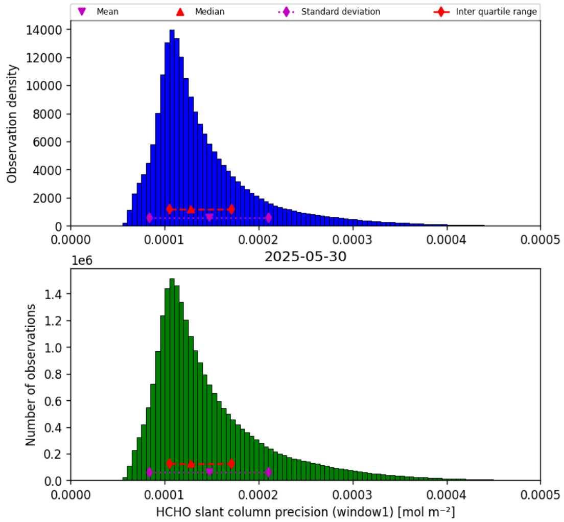
Figure 37: Histogram of “HCHO slant column precision (window1)” for 2025-05-30 to 2025-05-31
