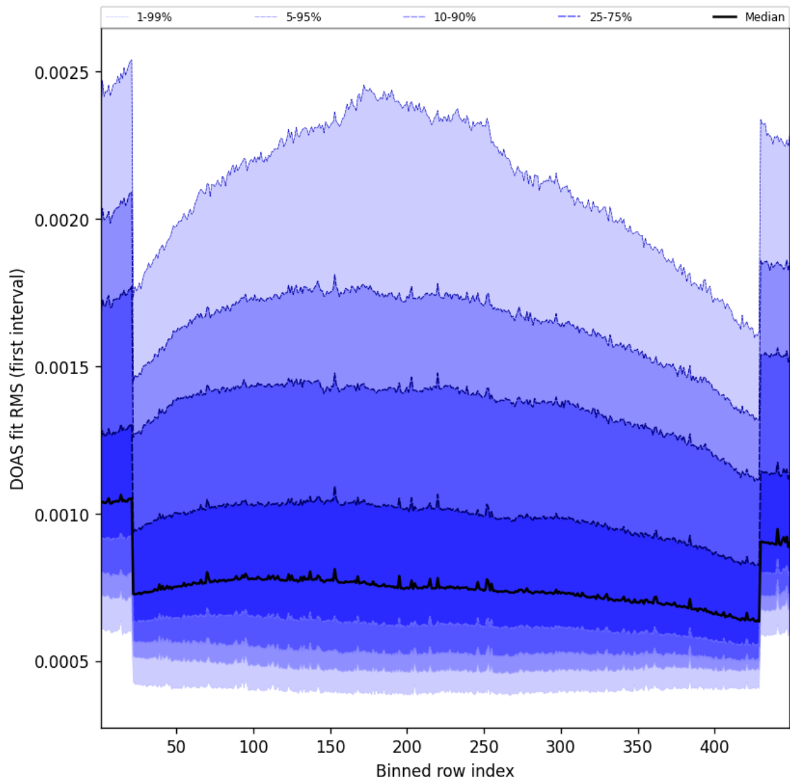
Figure 58: Along track statistics of “DOAS fit RMS (first interval)” for 2025-05-30 to 2025-05-31
