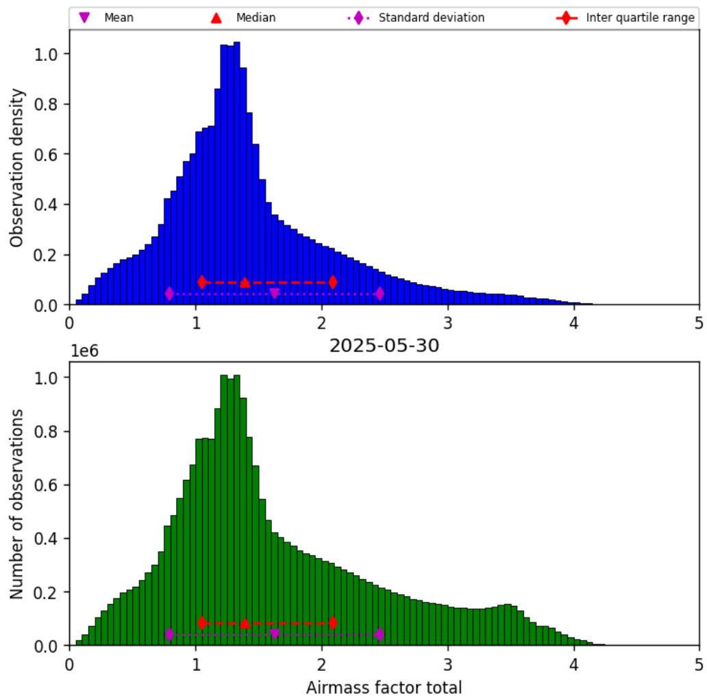
Figure 38: Histogram of “Airmass factor total” for 2025-05-30 to 2025-05-31
