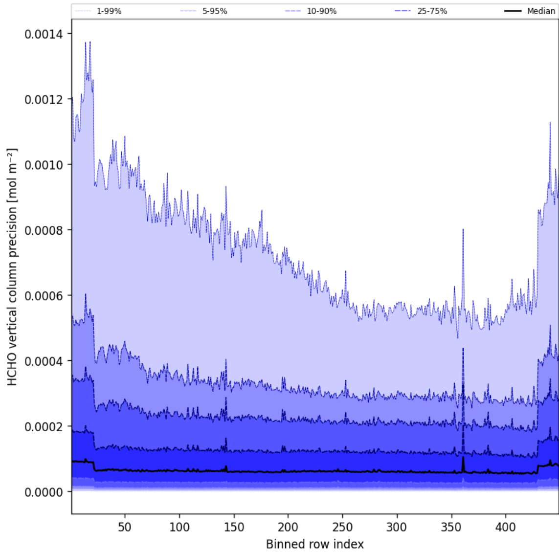
Figure 48: Along track statistics of “HCHO vertical column precision” for 2025-05-30 to 2025-05-31
