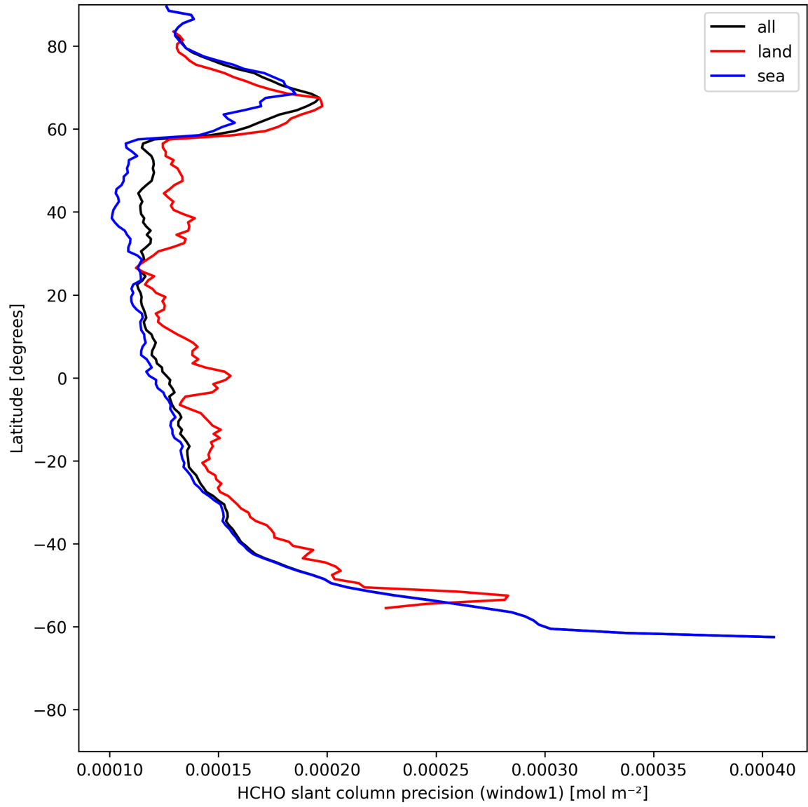
Figure 23: Zonal average of "HCHO slant column precision (window1)" for 2025-05-30 to 2025-05-31.
