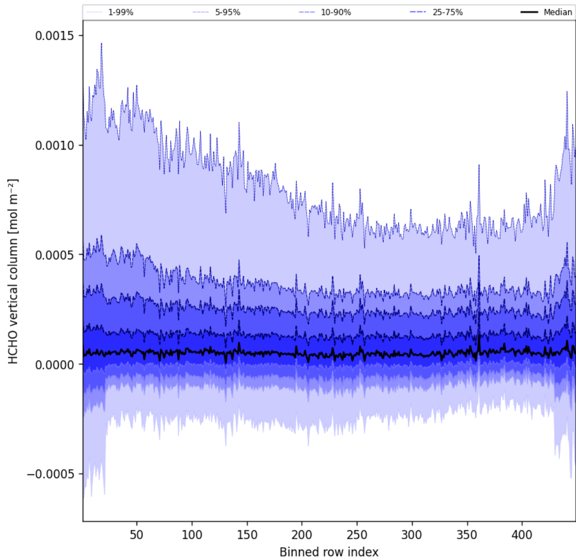
Figure 47: Along track statistics of “HCHO vertical column” for 2025-05-30 to 2025-05-31
