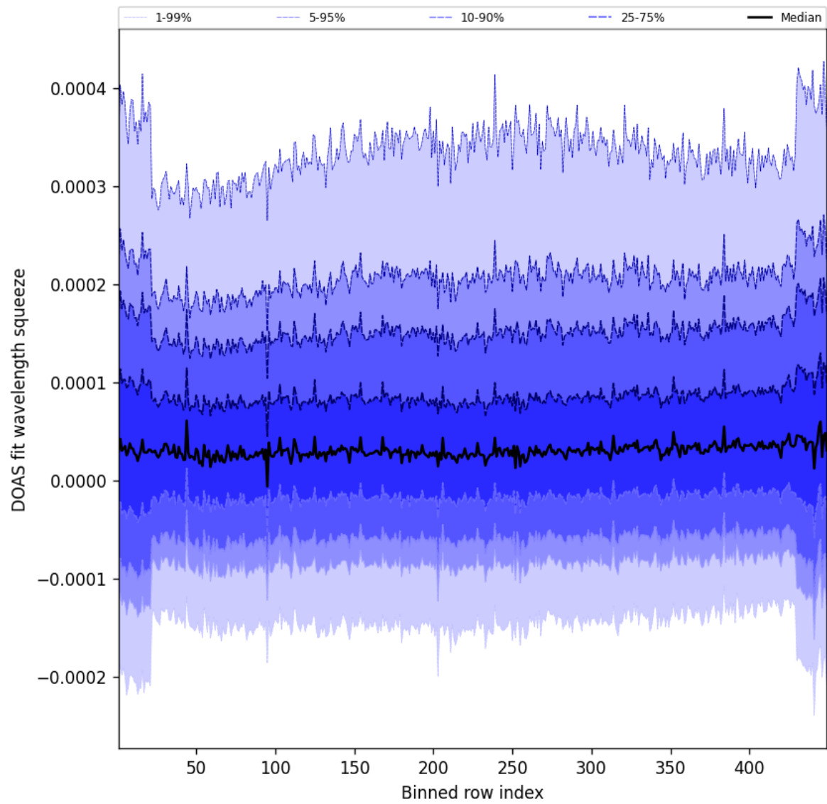
Figure 57: Along track statistics of “DOAS fit wavelength squeeze” for 2025-05-30 to 2025-05-31
