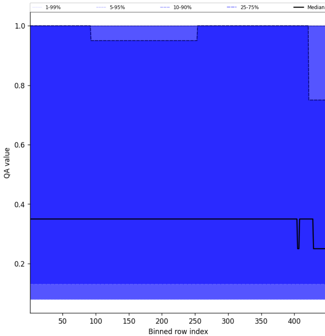
Figure 46: Along track statistics of “QA value” for 2025-05-30 to 2025-05-31
