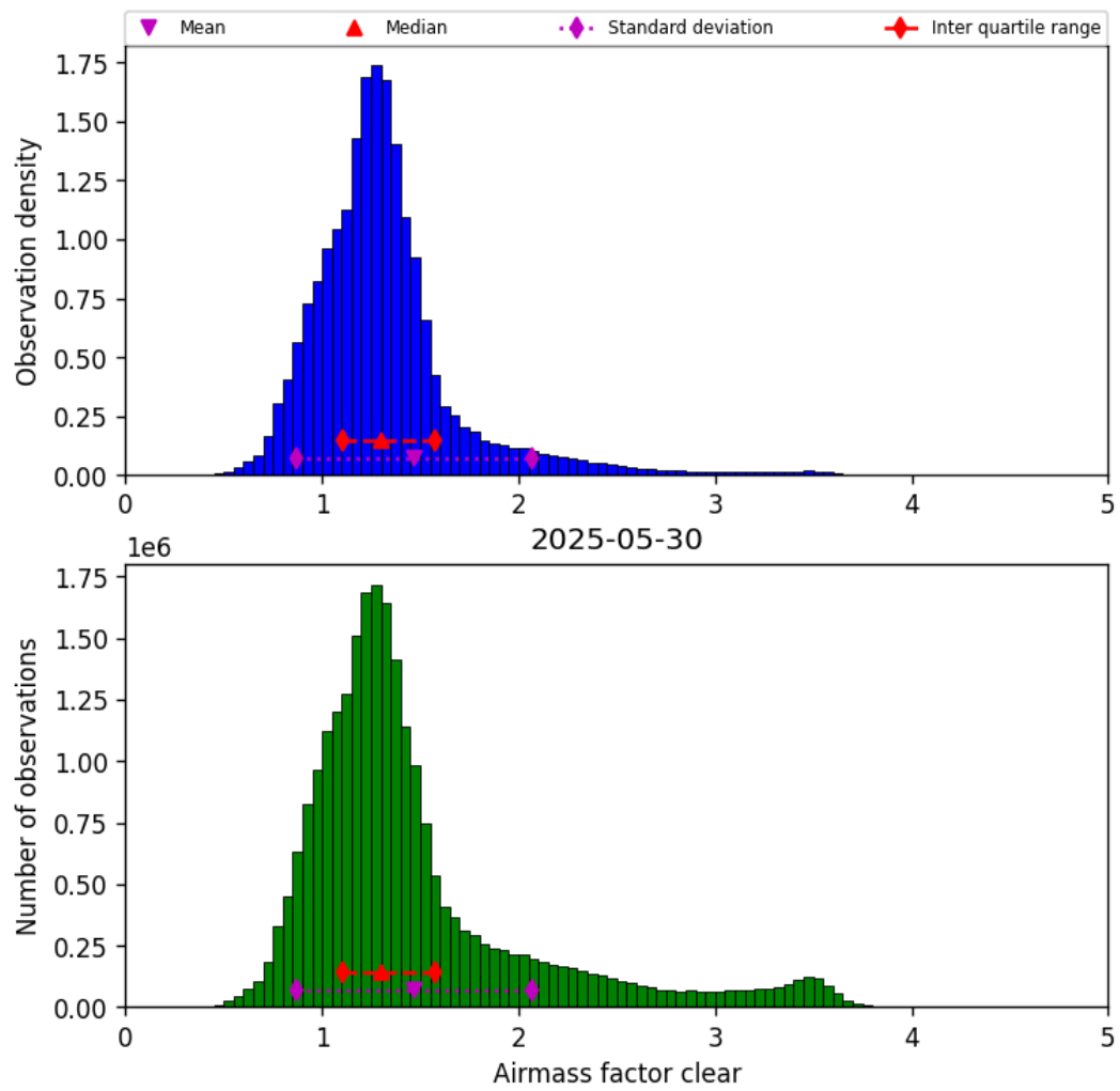
Figure 40: Histogram of “Airmass factor clear” for 2025-05-30 to 2025-05-31
