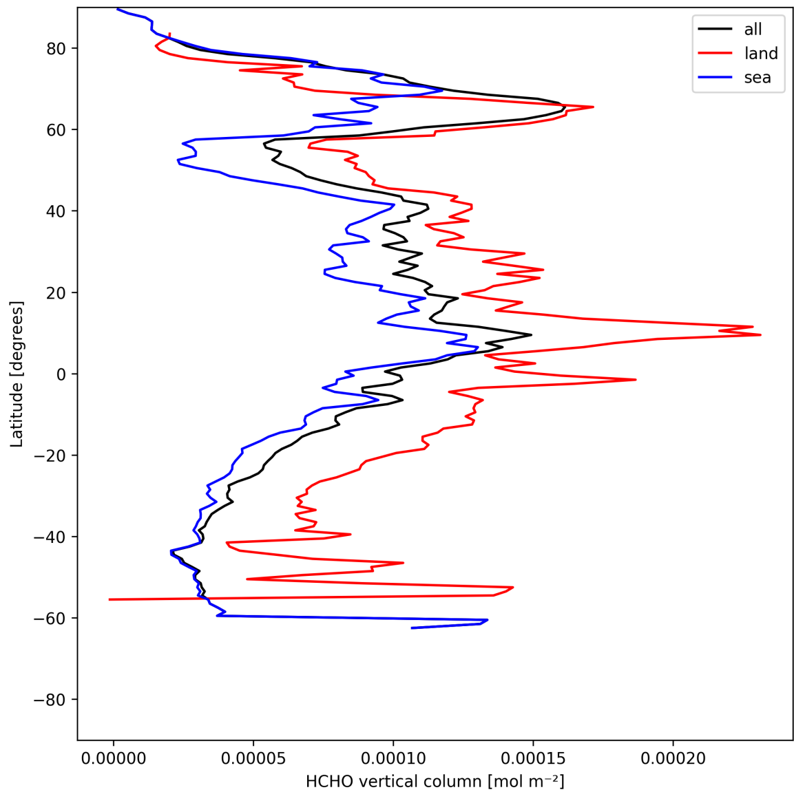
Figure 19: Zonal average of “HCHO vertical column” for 2025-05-30 to 2025-05-31.
