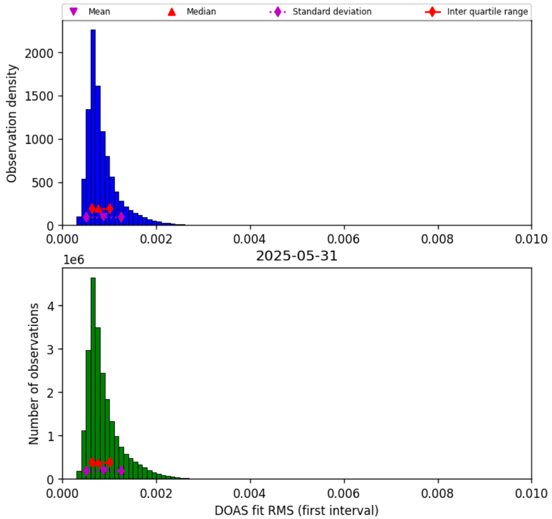
Figure 44: Histogram of “DOAS fit RMS (first interval)” for 2025-05-31 to 2025-06-01
