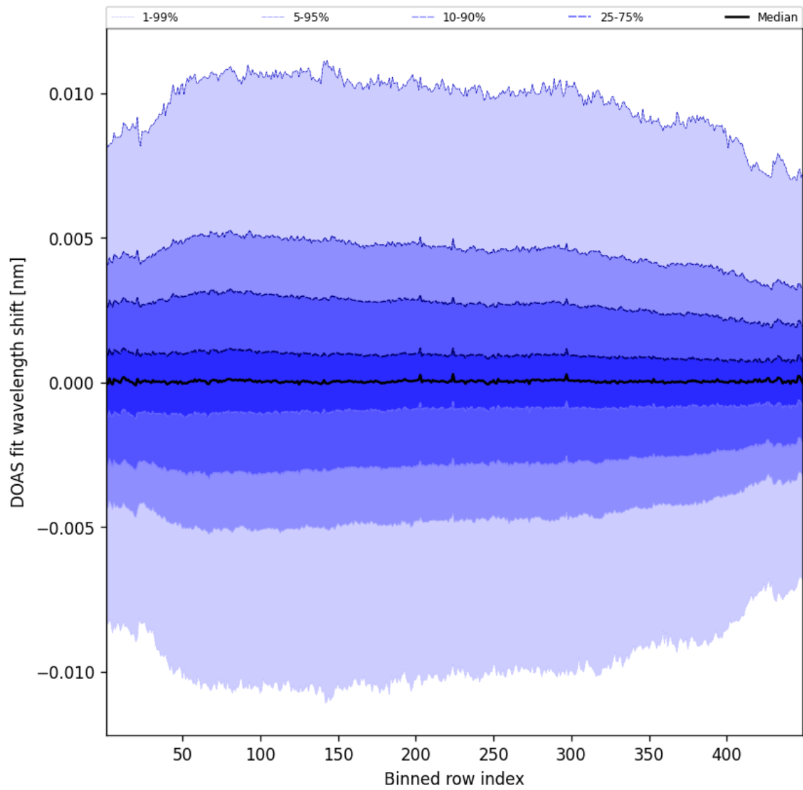
Figure 56: Along track statistics of “DOAS fit wavelength shift” for 2025-05-31 to 2025-06-01
