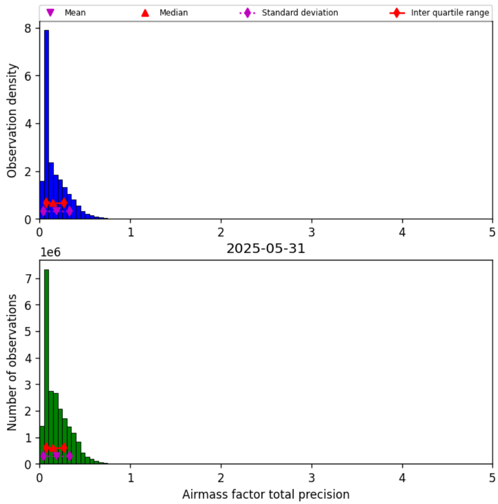
Figure 39: Histogram of “Airmass factor total precision” for 2025-05-31 to 2025-06-01
