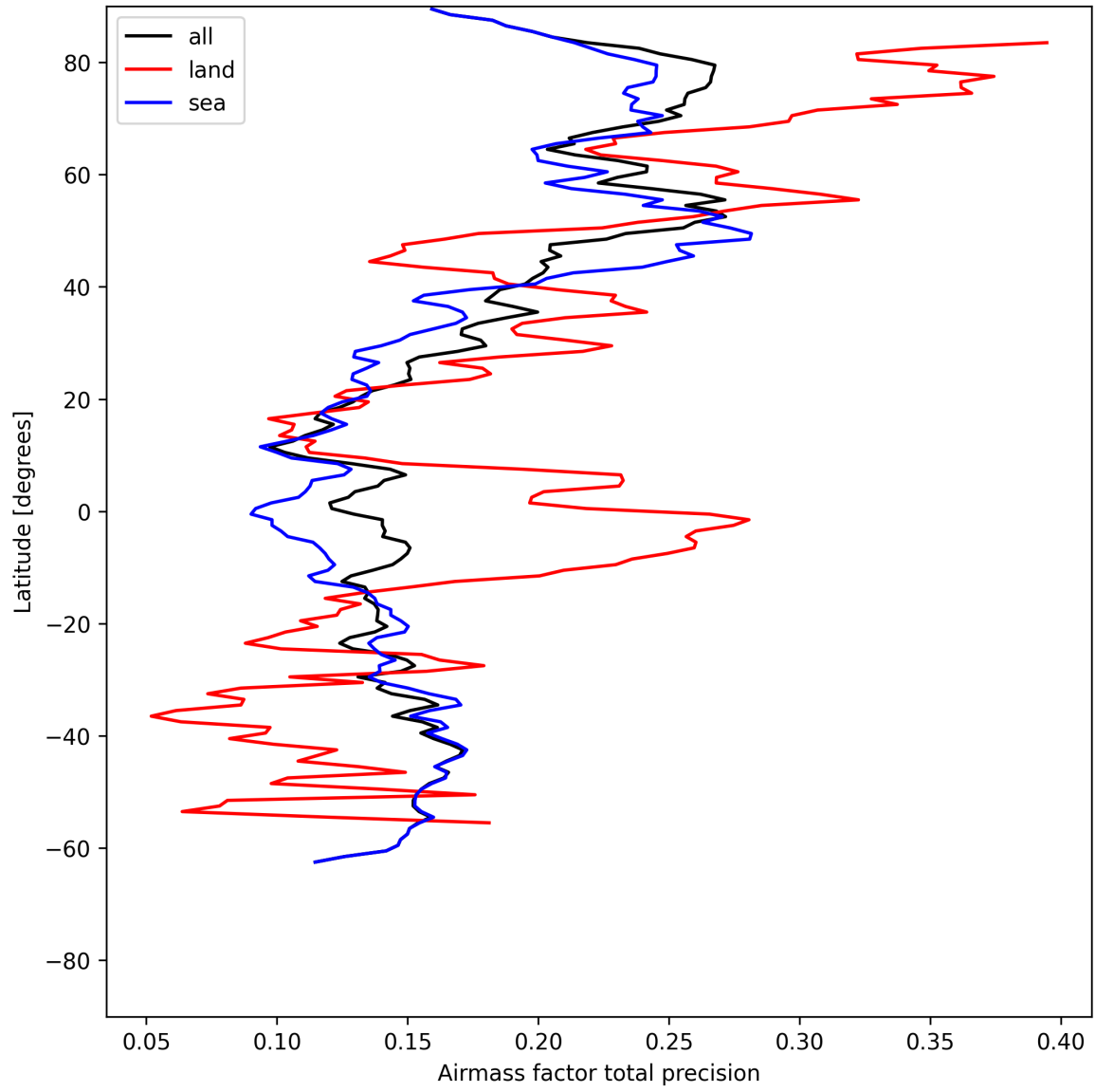
Figure 25: Zonal average of “Airmass factor total precision” for 2025-05-31 to 2025-06-01.
