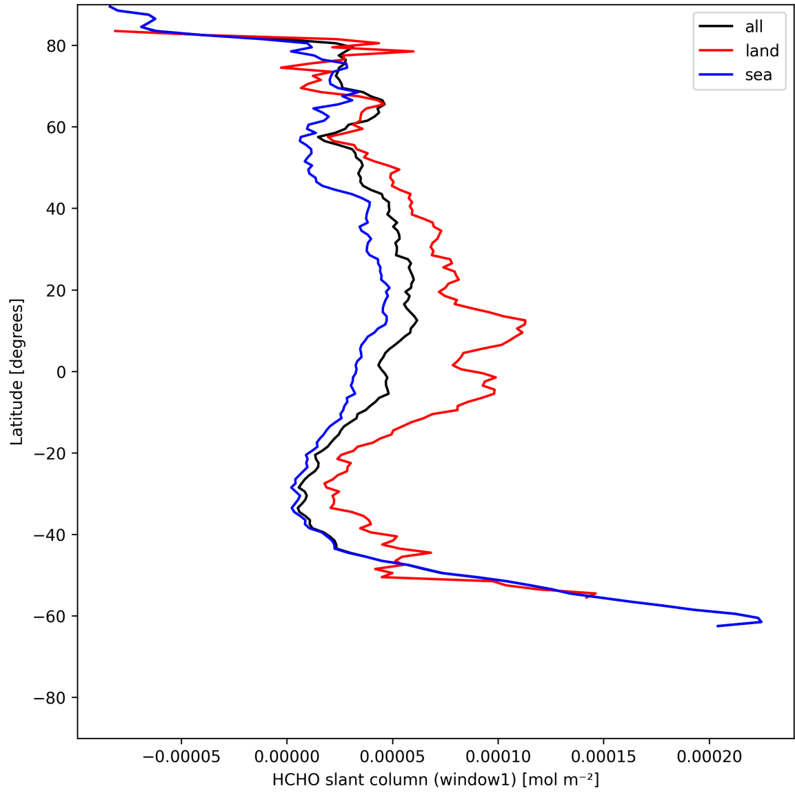
Figure 22: Zonal average of “HCHO slant column (window1)” for 2025-05-31 to 2025-06-01.
