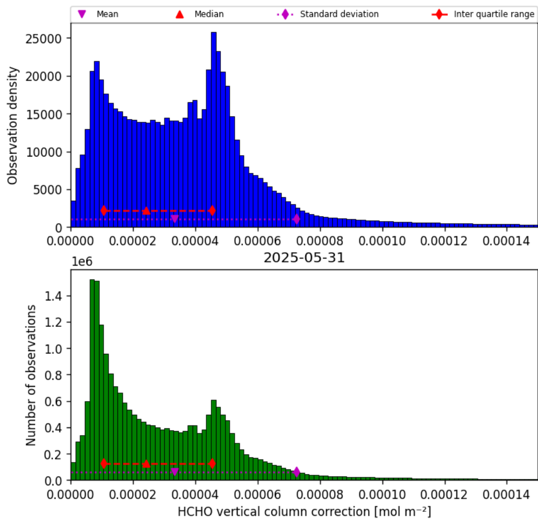
Figure 35: Histogram of “HCHO vertical column correction” for 2025-05-31 to 2025-06-01
