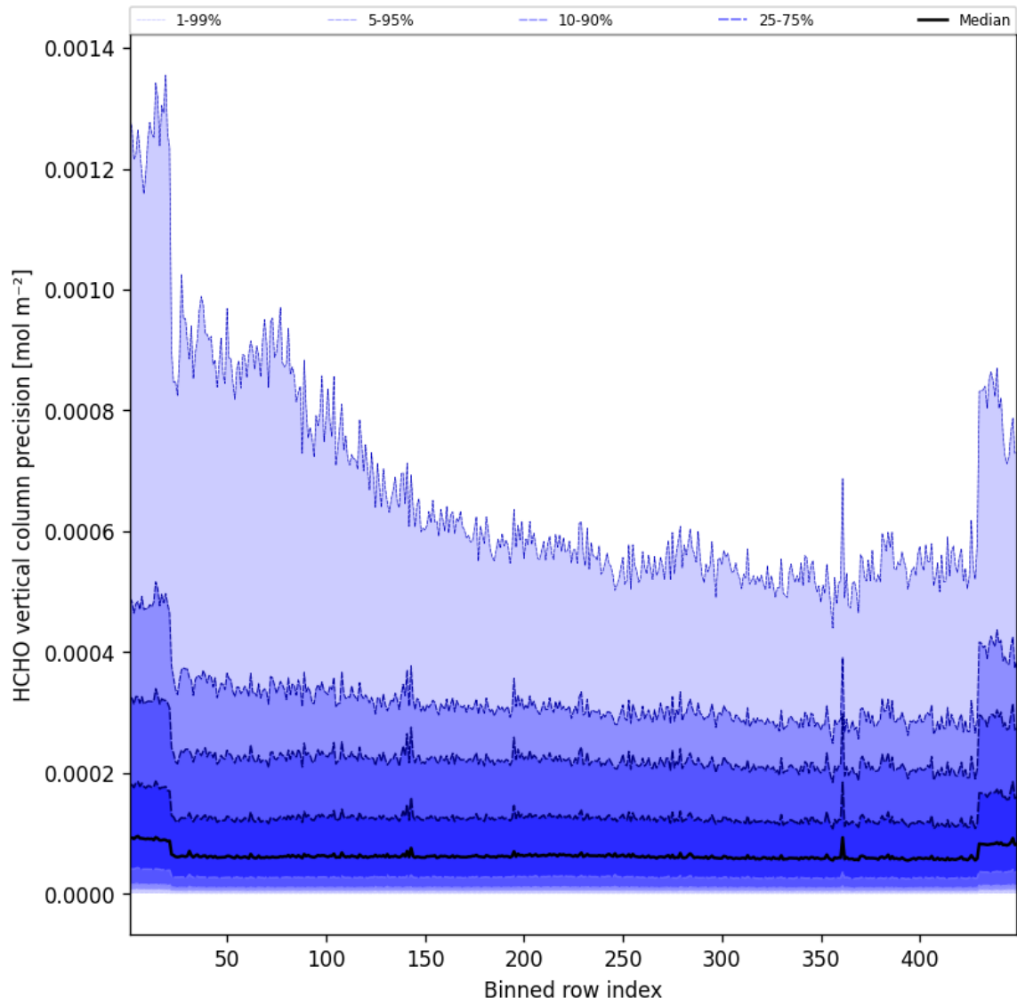
Figure 48: Along track statistics of “HCHO vertical column precision” for 2025-05-31 to 2025-06-01
