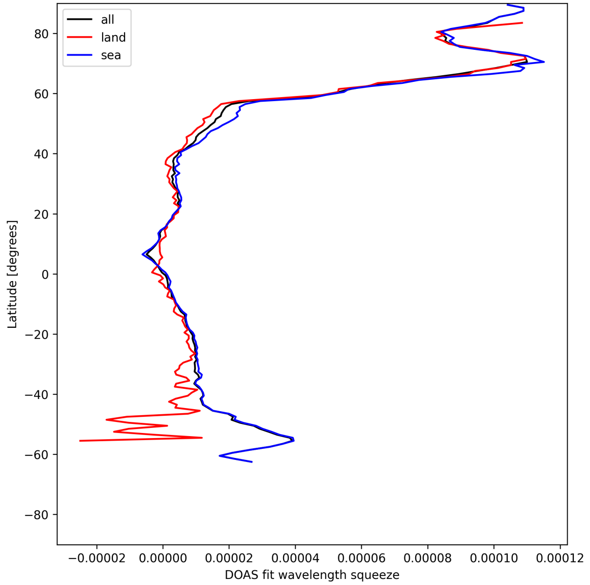
Figure 29: Zonal average of “DOAS fit wavelength squeeze” for 2025-05-31 to 2025-06-01.
