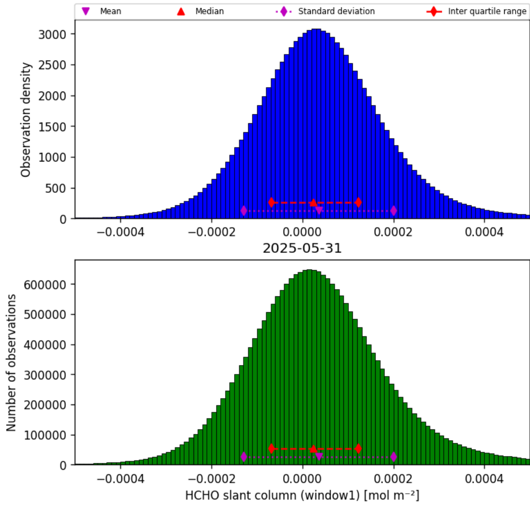
Figure 36: Histogram of “HCHO slant column (window1)” for 2025-05-31 to 2025-06-01
