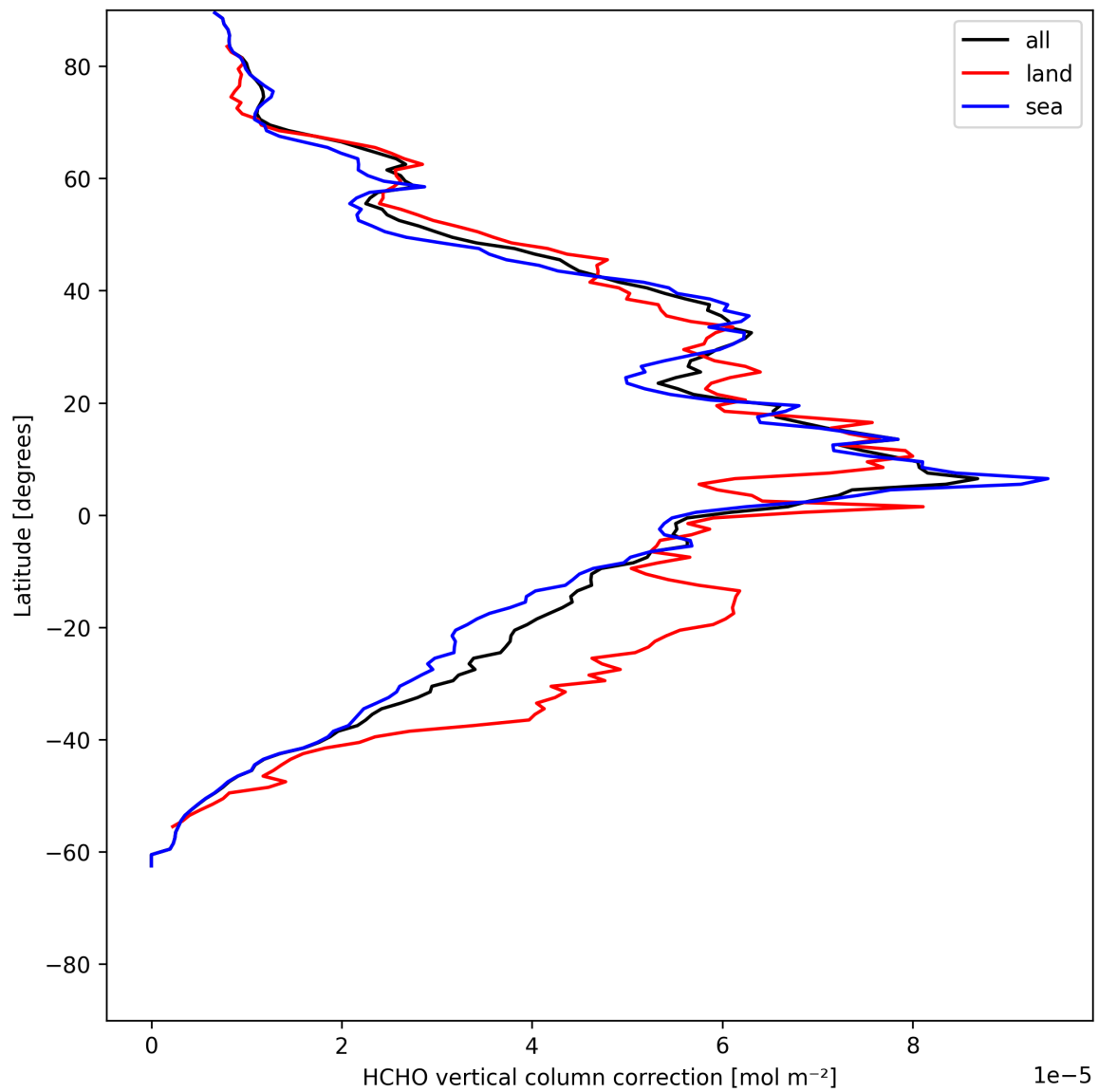
Figure 21: Zonal average of “HCHO vertical column correction” for 2025-05-31 to 2025-06-01.
