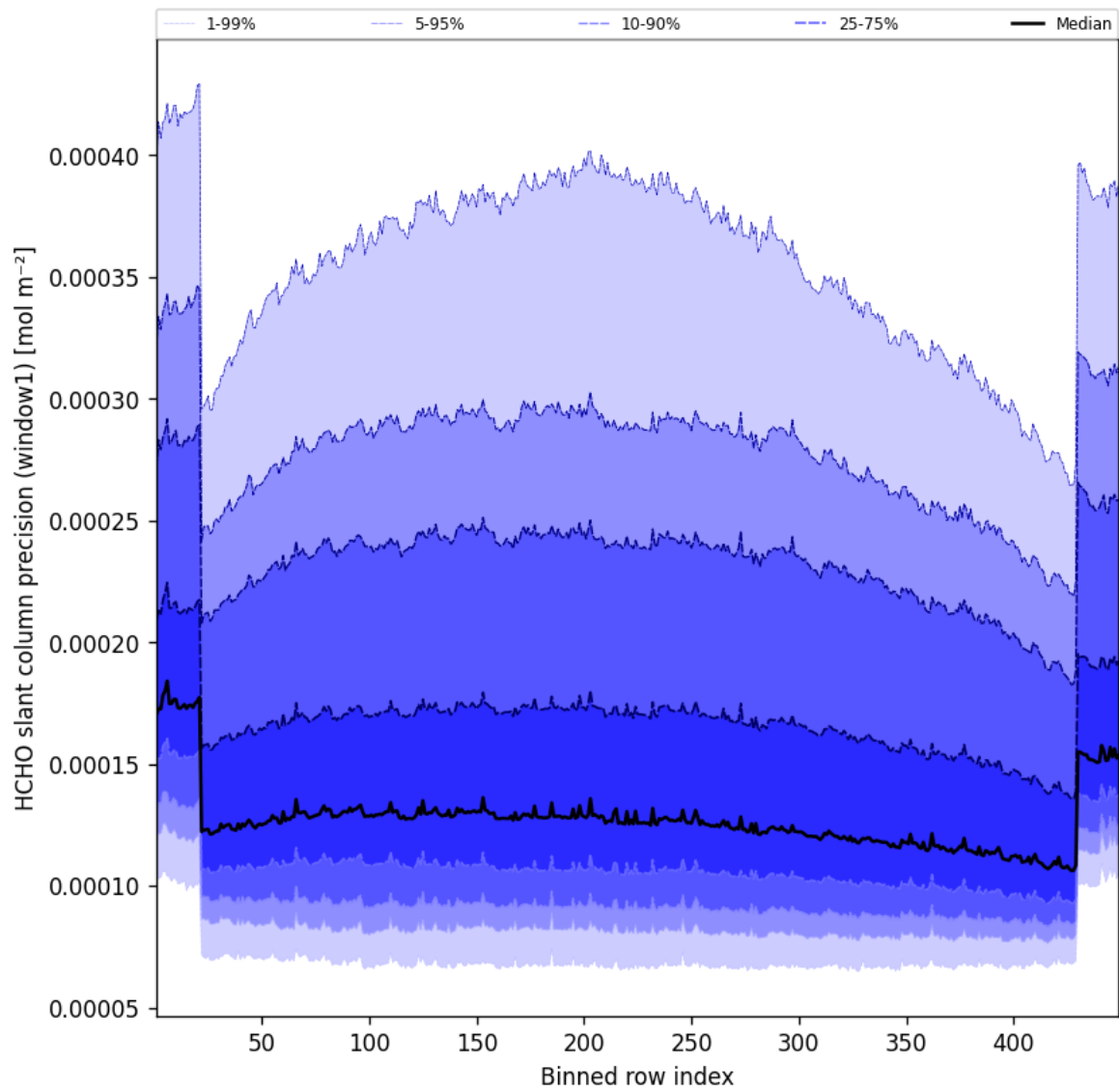
Figure 51: Along track statistics of “HCHO slant column precision (window1)” for 2025-05-31 to 2025-06-01
