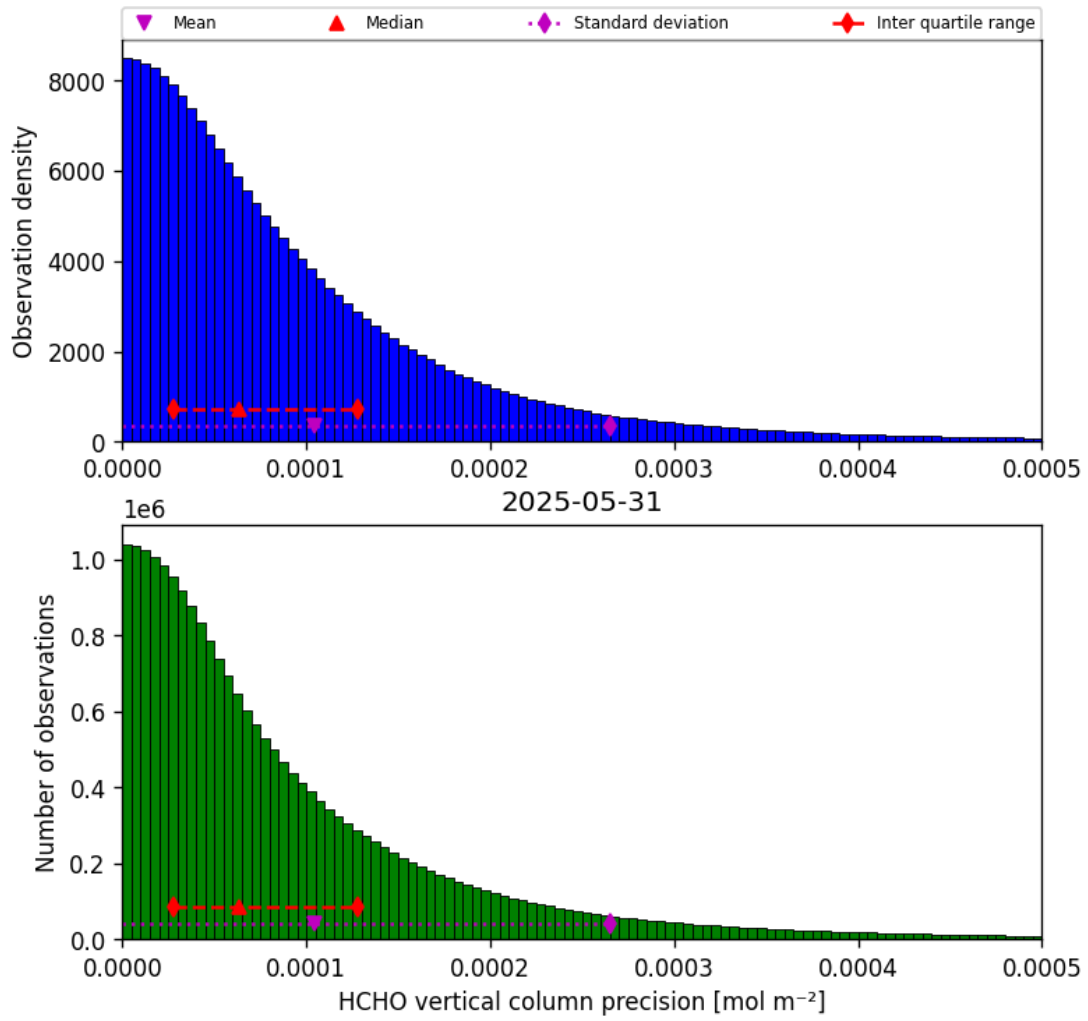
Figure 34: Histogram of “HCHO vertical column precision” for 2025-05-31 to 2025-06-01
