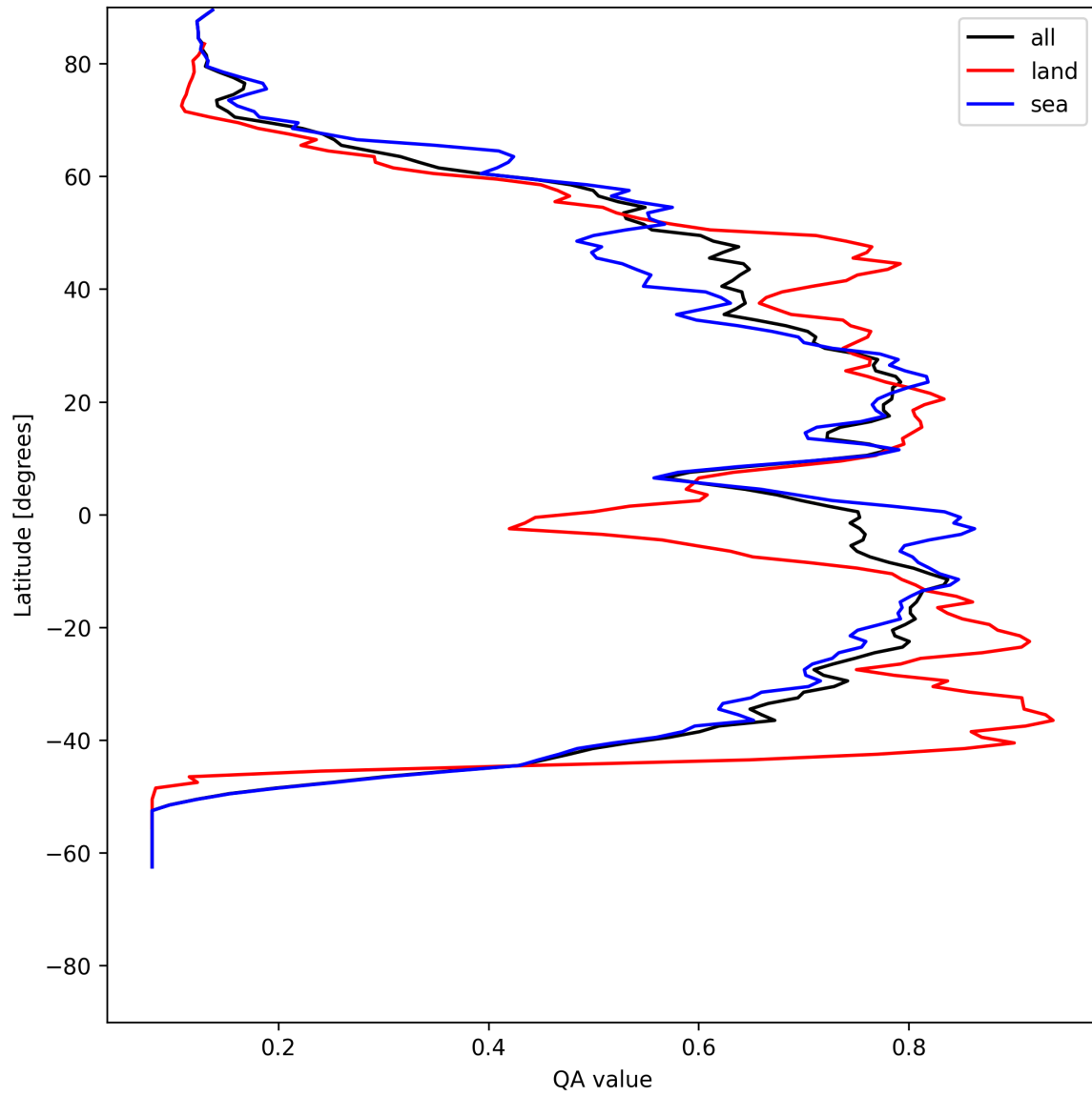
Figure 18: Zonal average of “QA value” for 2025-05-31 to 2025-06-01.
