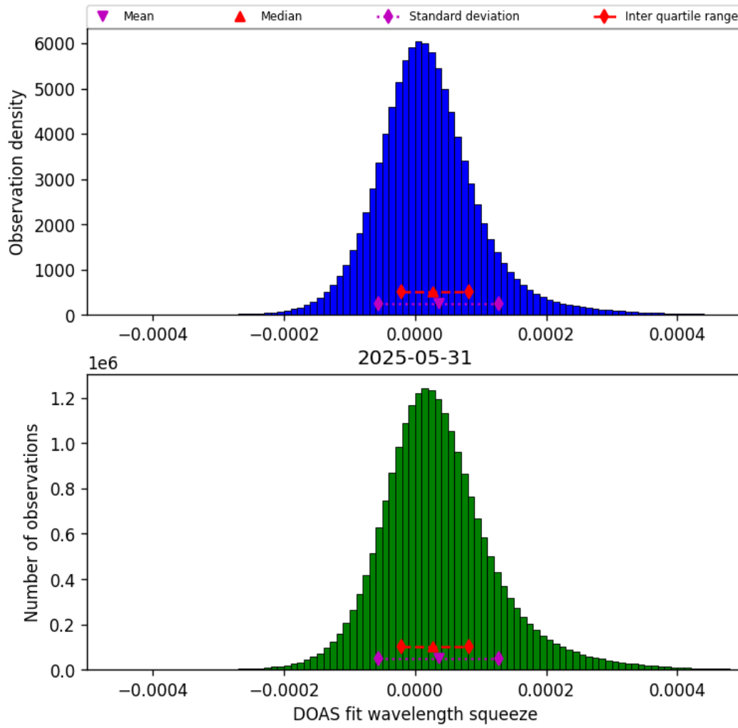
Figure 43: Histogram of “DOAS fit wavelength squeeze” for 2025-05-31 to 2025-06-01
