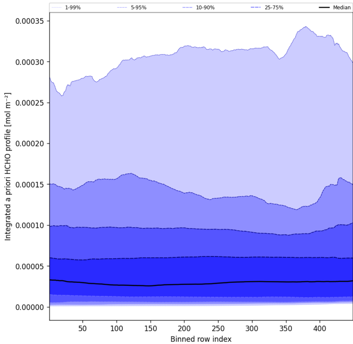
Figure 55: Along track statistics of “Integrated a priori HCHO profile” for 2025-05-31 to 2025-06-01
