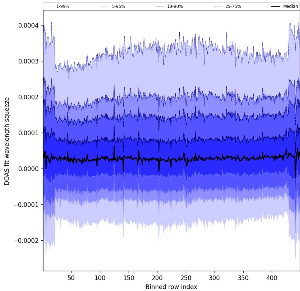
Figure 57: Along track statistics of “DOAS fit wavelength squeeze” for 2025-05-31 to 2025-06-01
