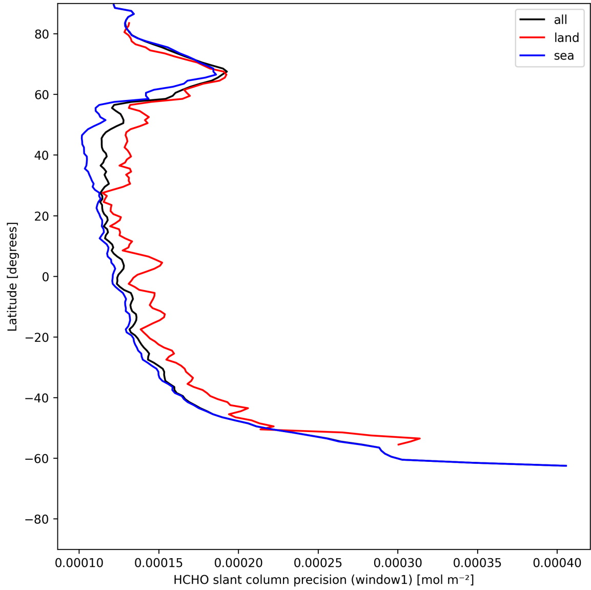
Figure 23: Zonal average of “HCHO slant column precision (window1)” for 2025-05-31 to 2025-06-01.
