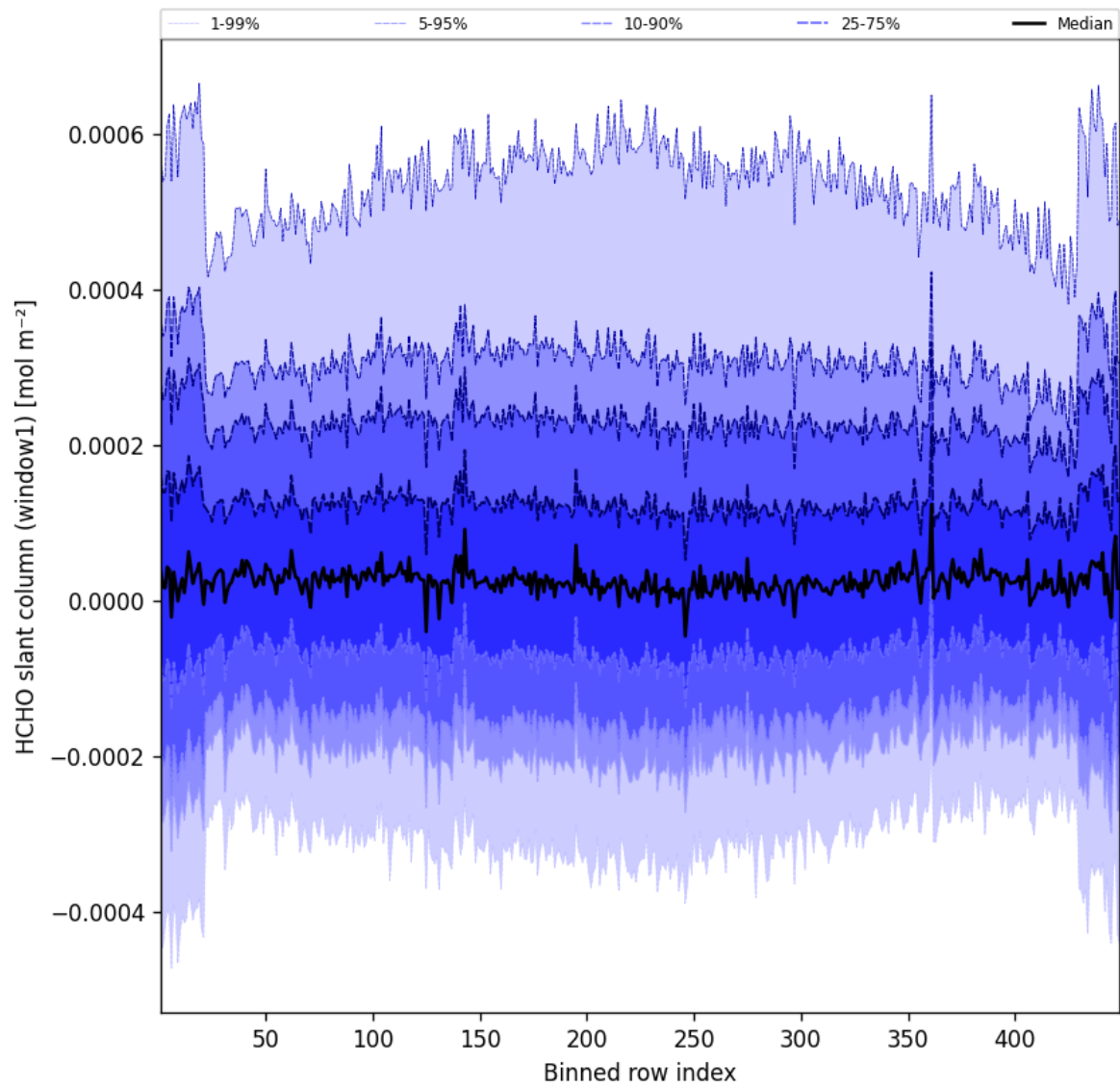
Figure 50: Along track statistics of “HCHO slant column (window1)” for 2025-05-31 to 2025-06-01
