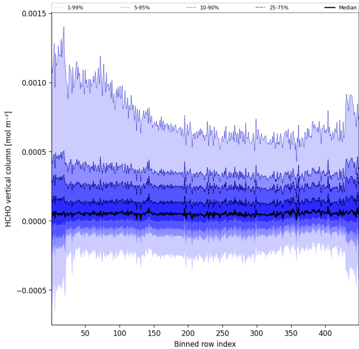
Figure 47: Along track statistics of “HCHO vertical column” for 2025-05-31 to 2025-06-01
