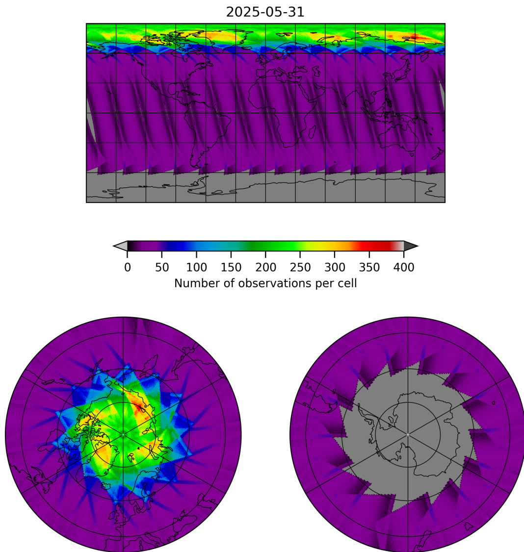
Figure 17: Map of the number of observations for 2025-05-31 to 2025-06-01
