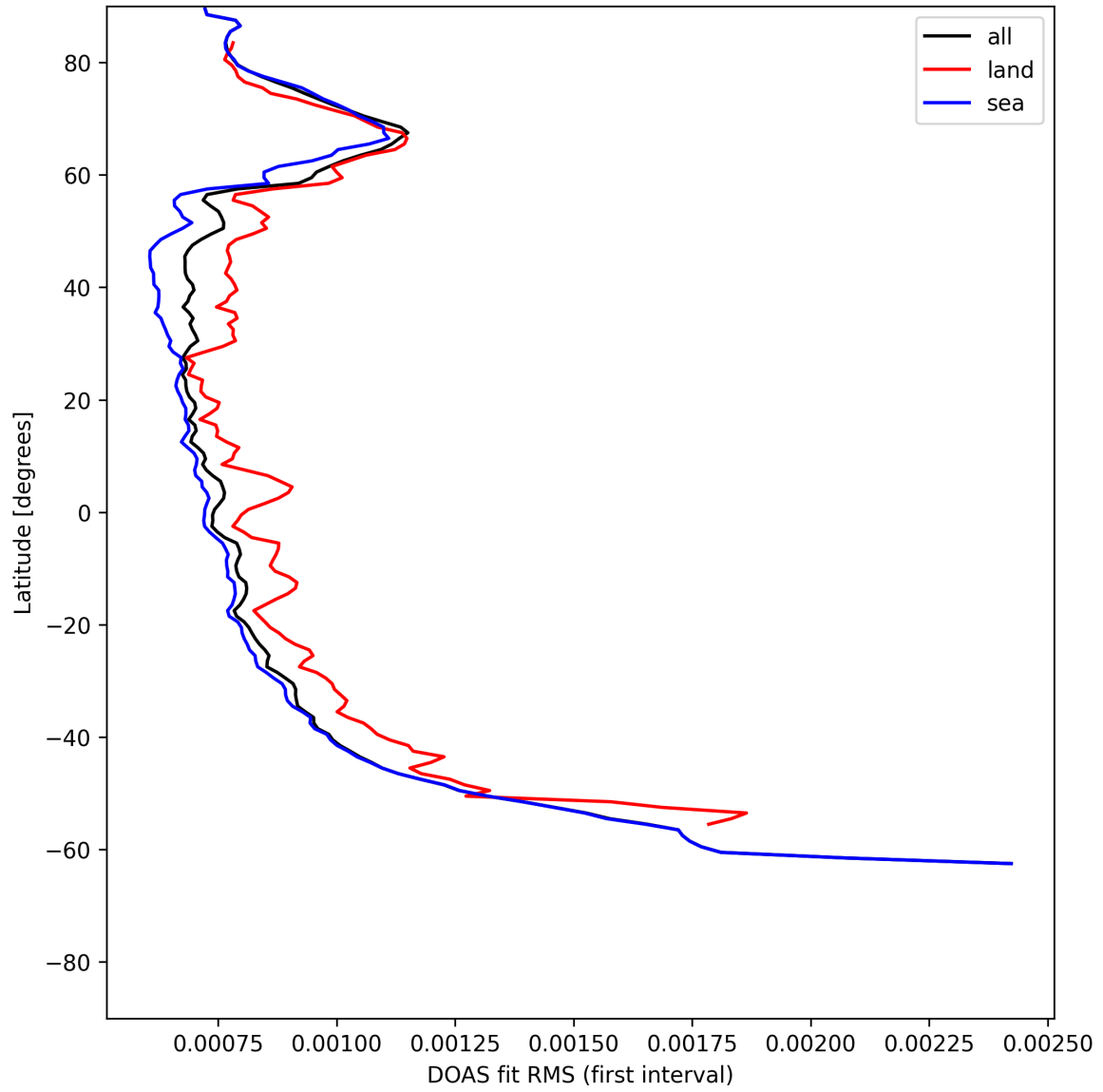
Figure 30: Zonal average of "DOAS fit RMS (first interval)" for 2025-05-31 to 2025-06-01.
