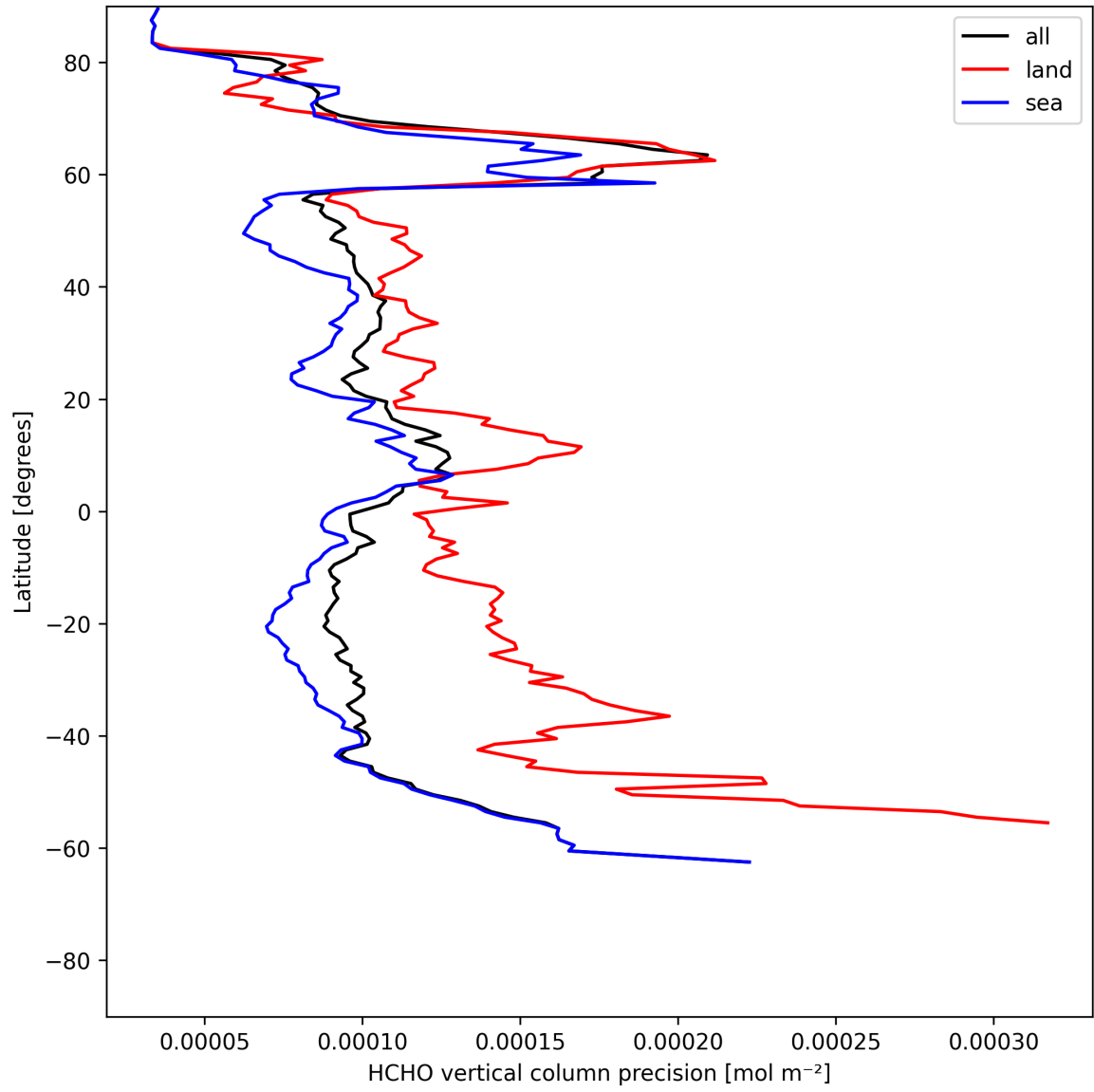
Figure 20: Zonal average of “HCHO vertical column precision” for 2025-05-31 to 2025-06-01.
