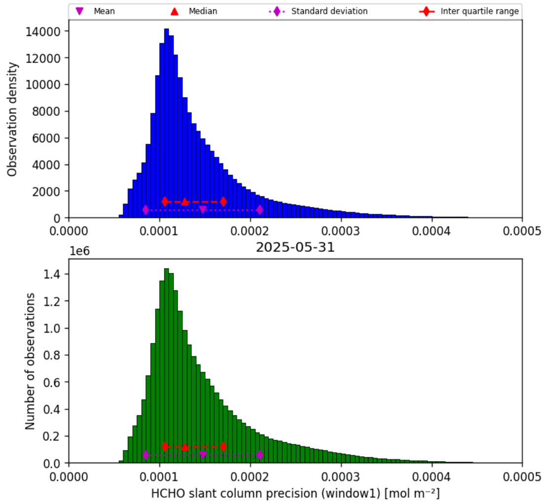
Figure 37: Histogram of “HCHO slant column precision (window1)” for 2025-05-31 to 2025-06-01
