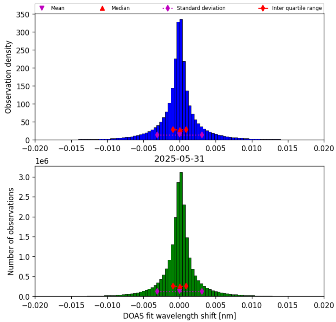
Figure 42: Histogram of “DOAS fit wavelength shift” for 2025-05-31 to 2025-06-01
