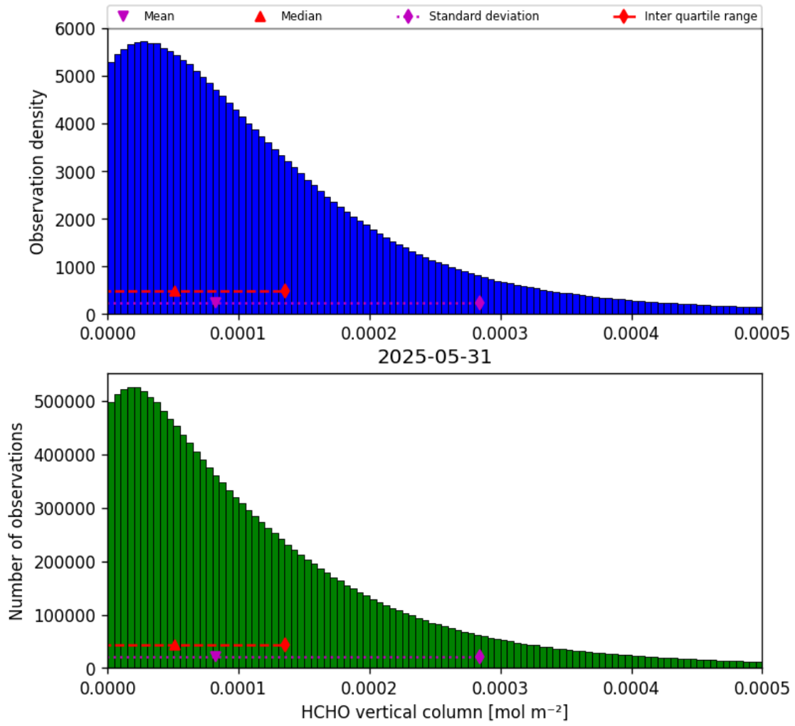
Figure 33: Histogram of “HCHO vertical column” for 2025-05-31 to 2025-06-01
