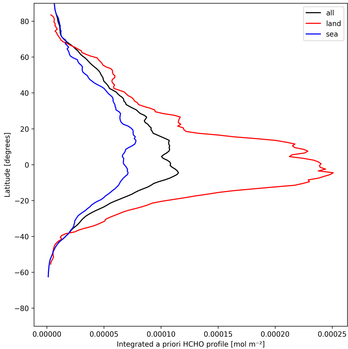
Figure 27: Zonal average of “Integrated a priori HCHO profile” for 2025-05-31 to 2025-06-01.
