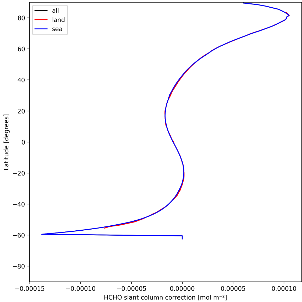
Figure 31: Zonal average of “HCHO slant column correction” for 2025-05-31 to 2025-06-01.
