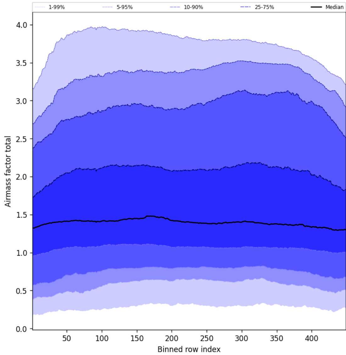
Figure 52: Along track statistics of “Airmass factor total” for 2025-05-31 to 2025-06-01
