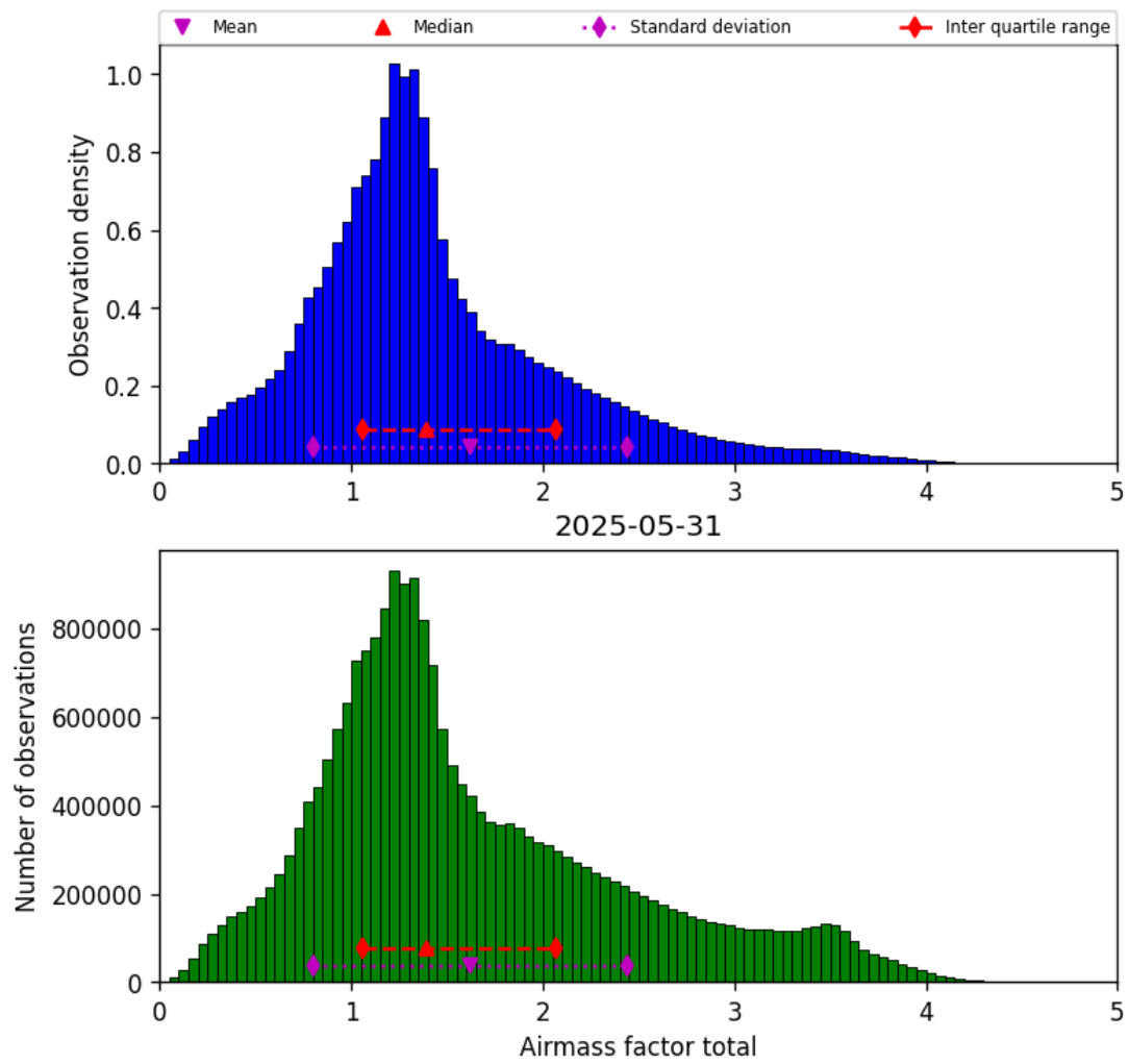
Figure 38: Histogram of “Airmass factor total” for 2025-05-31 to 2025-06-01
