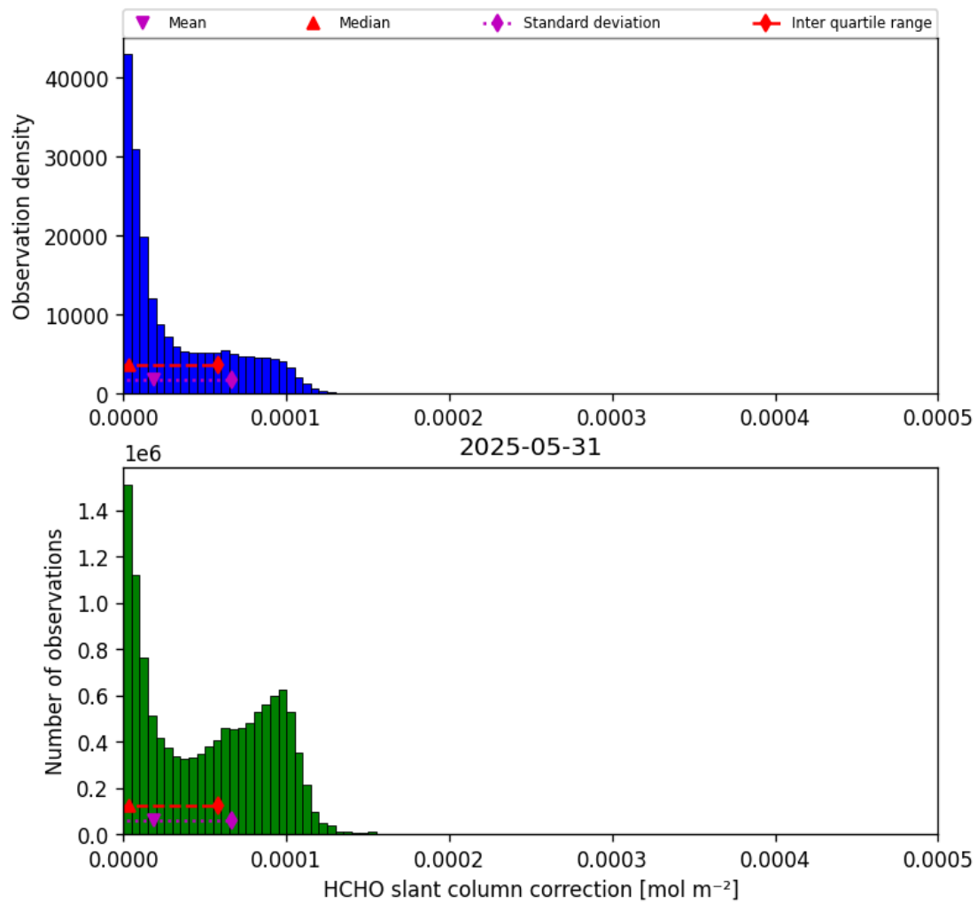
Figure 45: Histogram of “HCHO slant column correction” for 2025-05-31 to 2025-06-01
