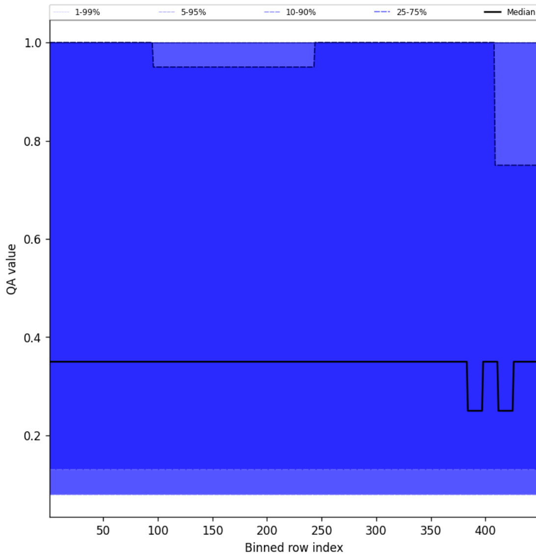
Figure 46: Along track statistics of “QA value” for 2025-05-31 to 2025-06-01
