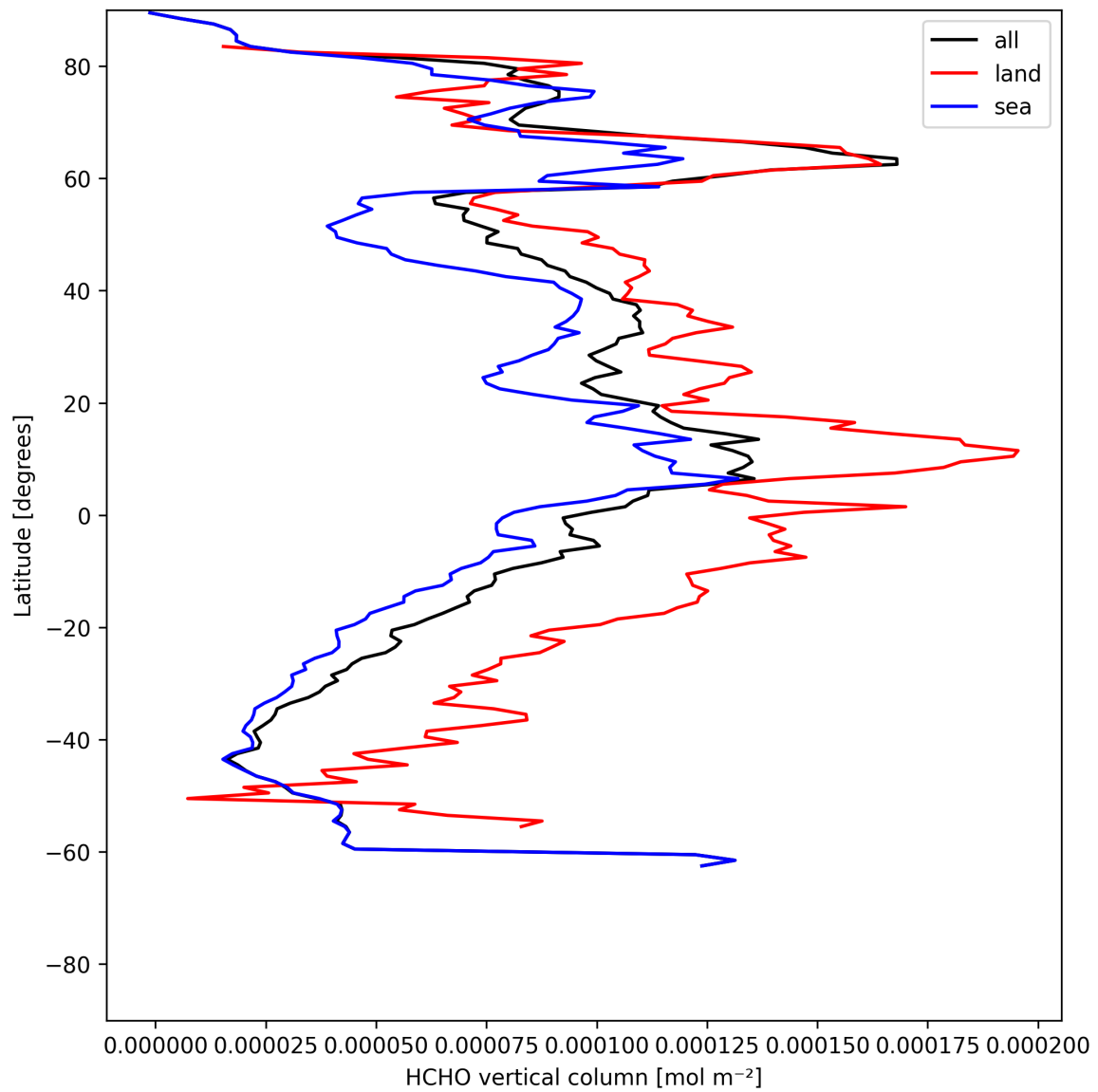
Figure 19: Zonal average of “HCHO vertical column” for 2025-05-31 to 2025-06-01.
