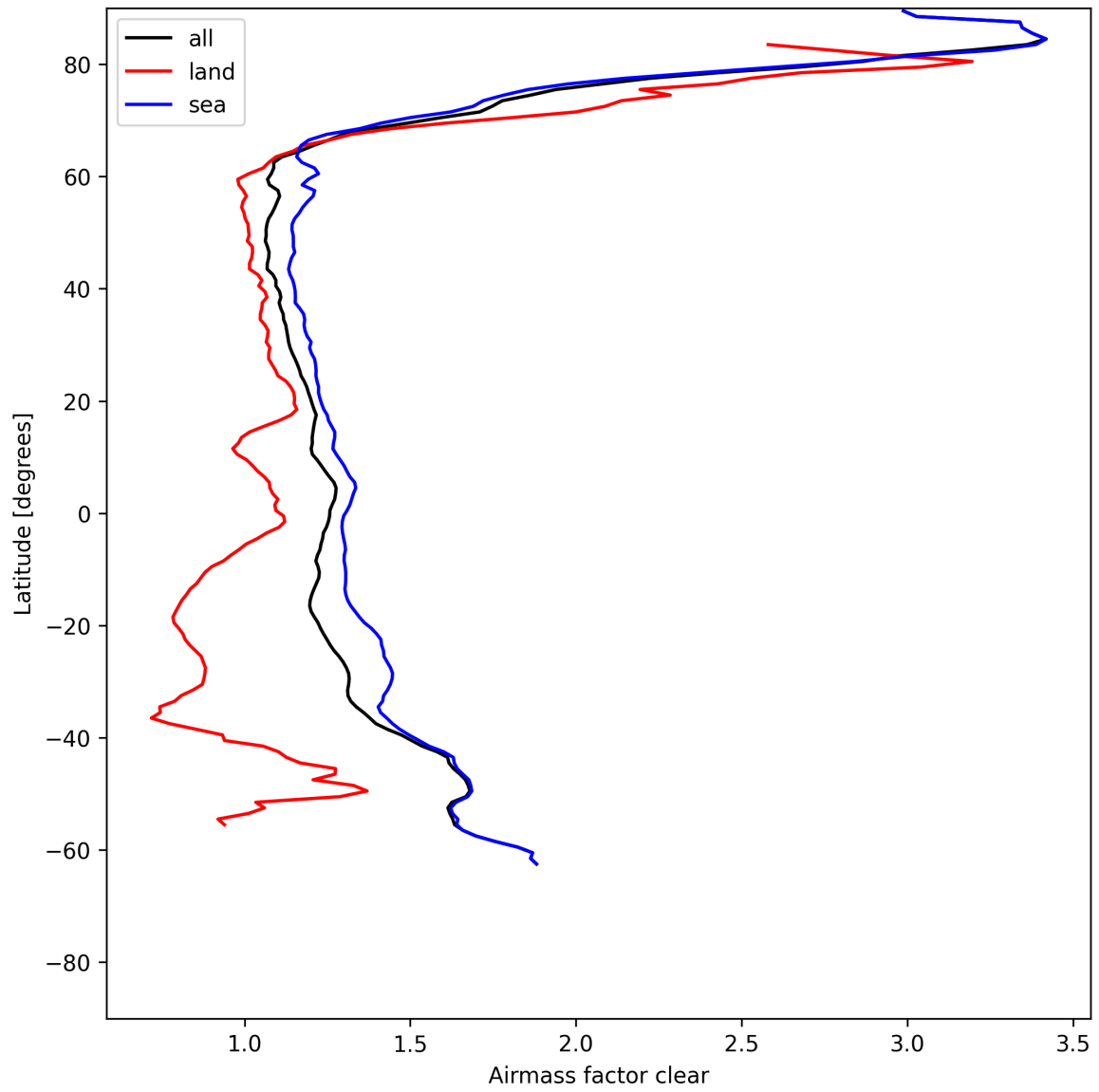
Figure 26: Zonal average of “Airmass factor clear” for 2025-05-31 to 2025-06-01.
