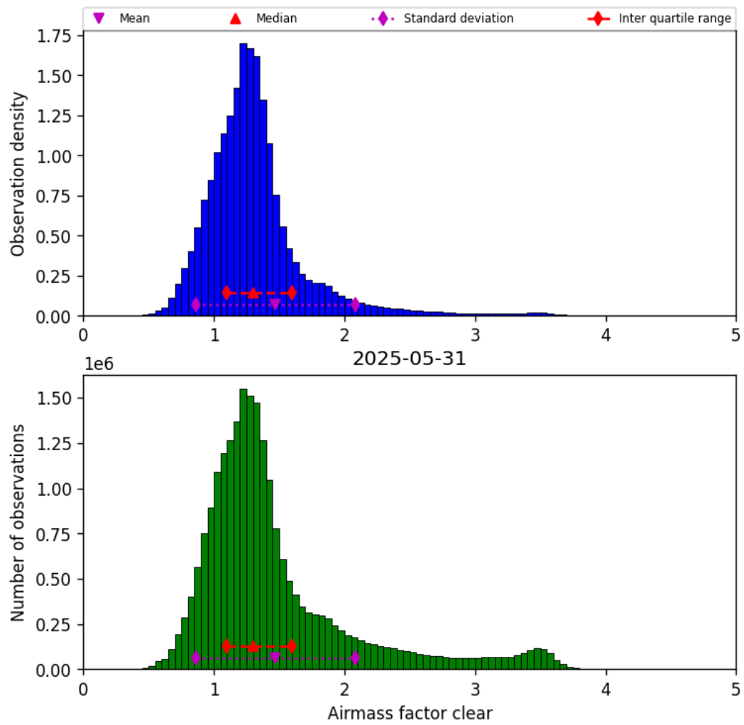
Figure 40: Histogram of “Airmass factor clear” for 2025-05-31 to 2025-06-01
