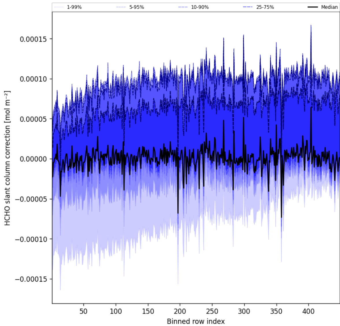
Figure 59: Along track statistics of “HCHO slant column correction” for 2025-05-31 to 2025-06-01
