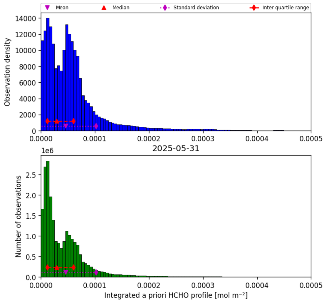
Figure 41: Histogram of “Integrated a priori HCHO profile” for 2025-05-31 to 2025-06-01
