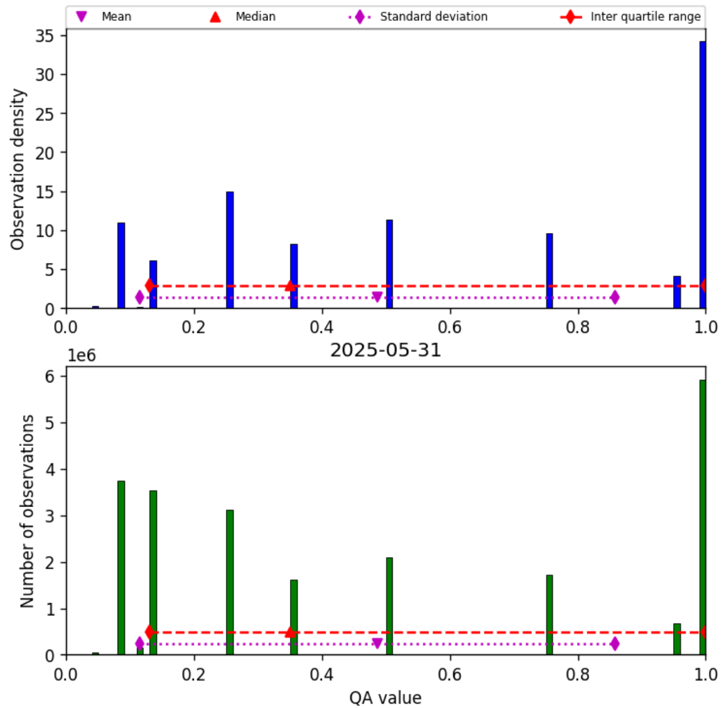
Figure 32: Histogram of “QA value” for 2025-05-31 to 2025-06-01
