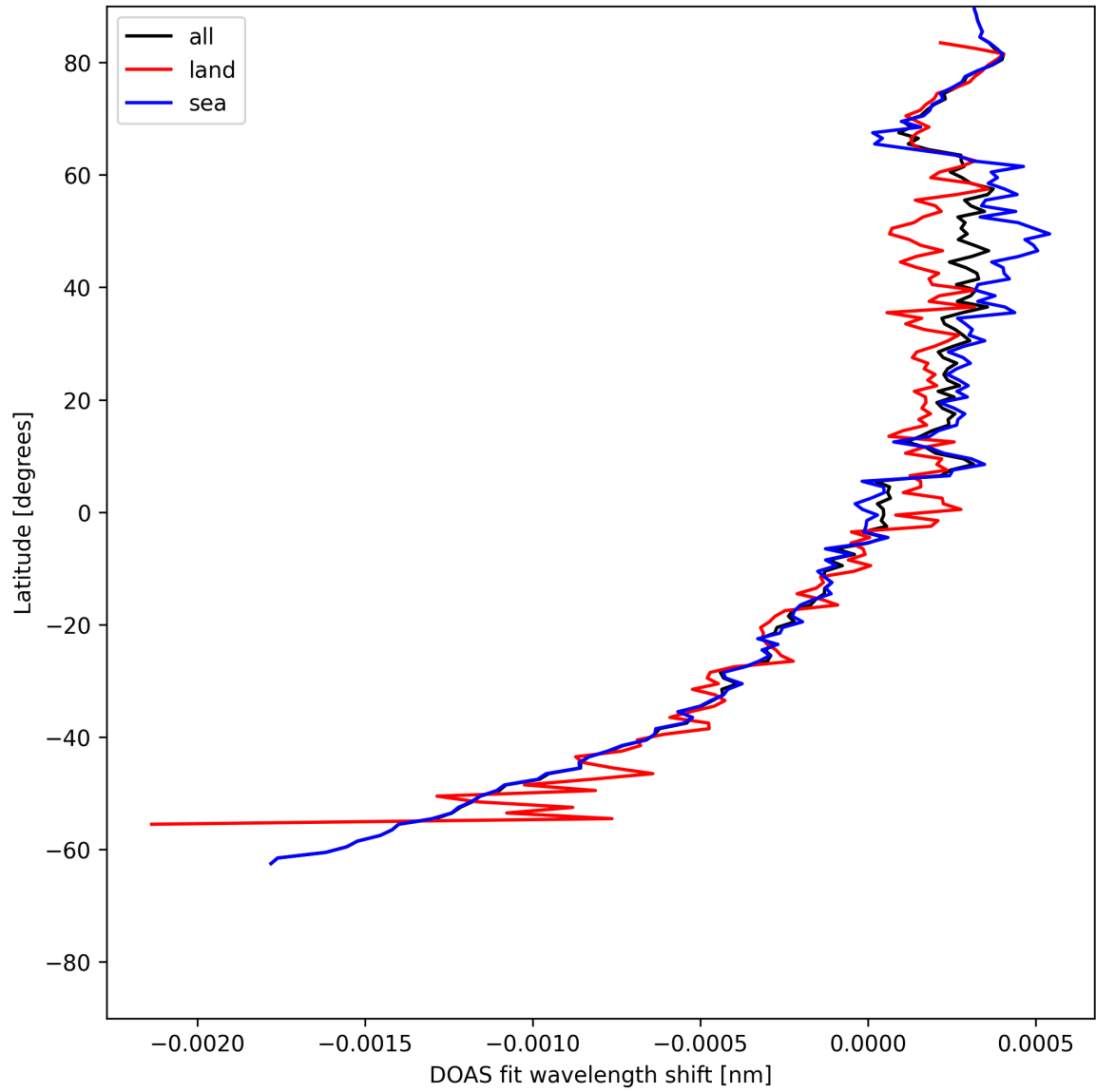
Figure 28: Zonal average of "DOAS fit wavelength shift" for 2025-05-31 to 2025-06-01.
