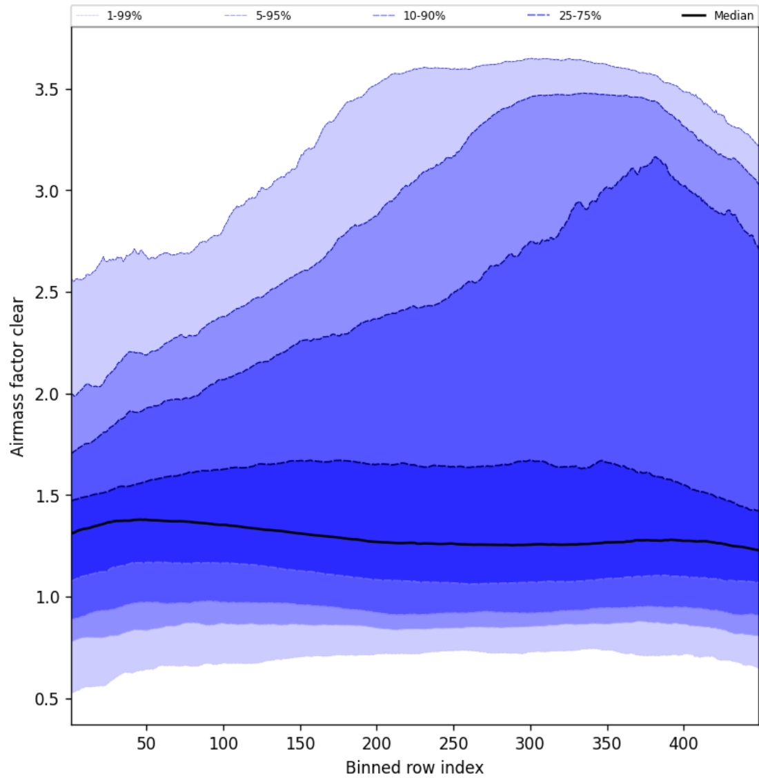
Figure 54: Along track statistics of “Airmass factor clear” for 2025-05-31 to 2025-06-01
