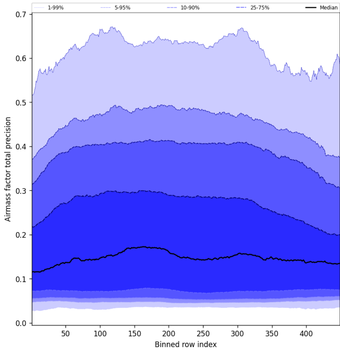
Figure 53: Along track statistics of “Airmass factor total precision” for 2025-05-31 to 2025-06-01
