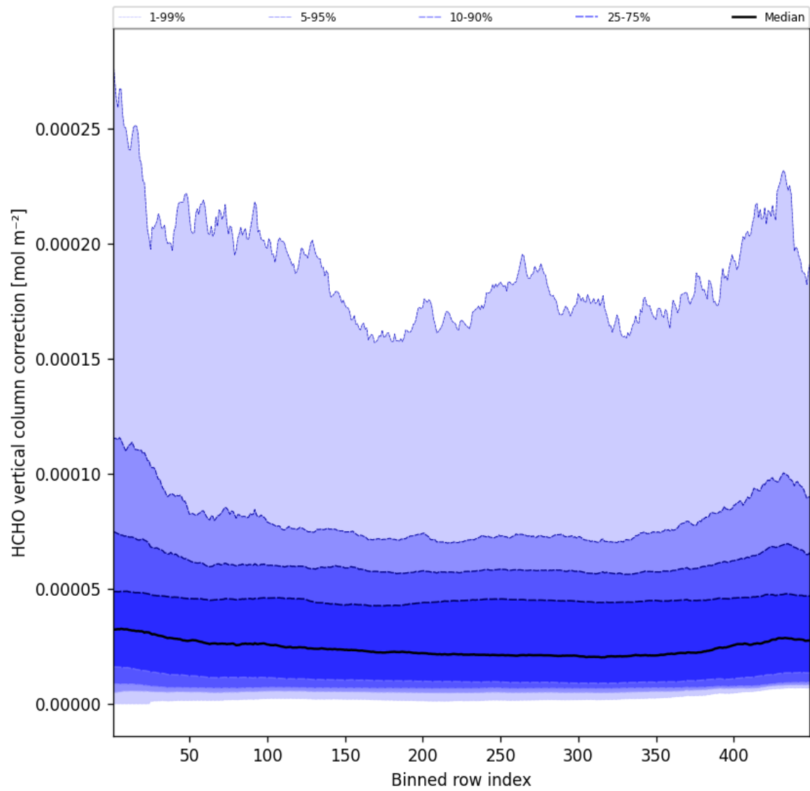
Figure 49: Along track statistics of “HCHO vertical column correction” for 2025-05-31 to 2025-06-01
