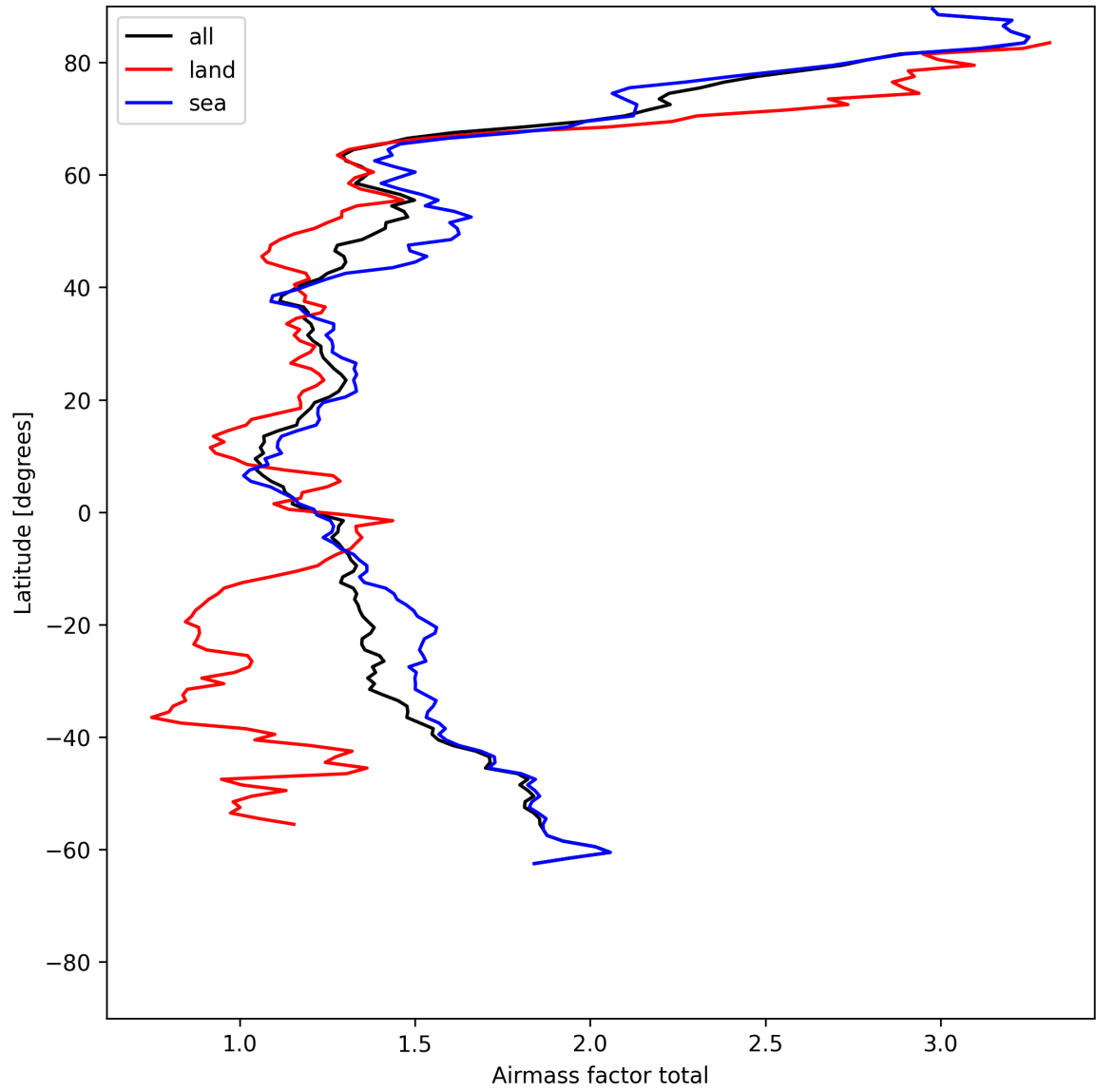
Figure 24: Zonal average of “Airmass factor total” for 2025-05-31 to 2025-06-01.
