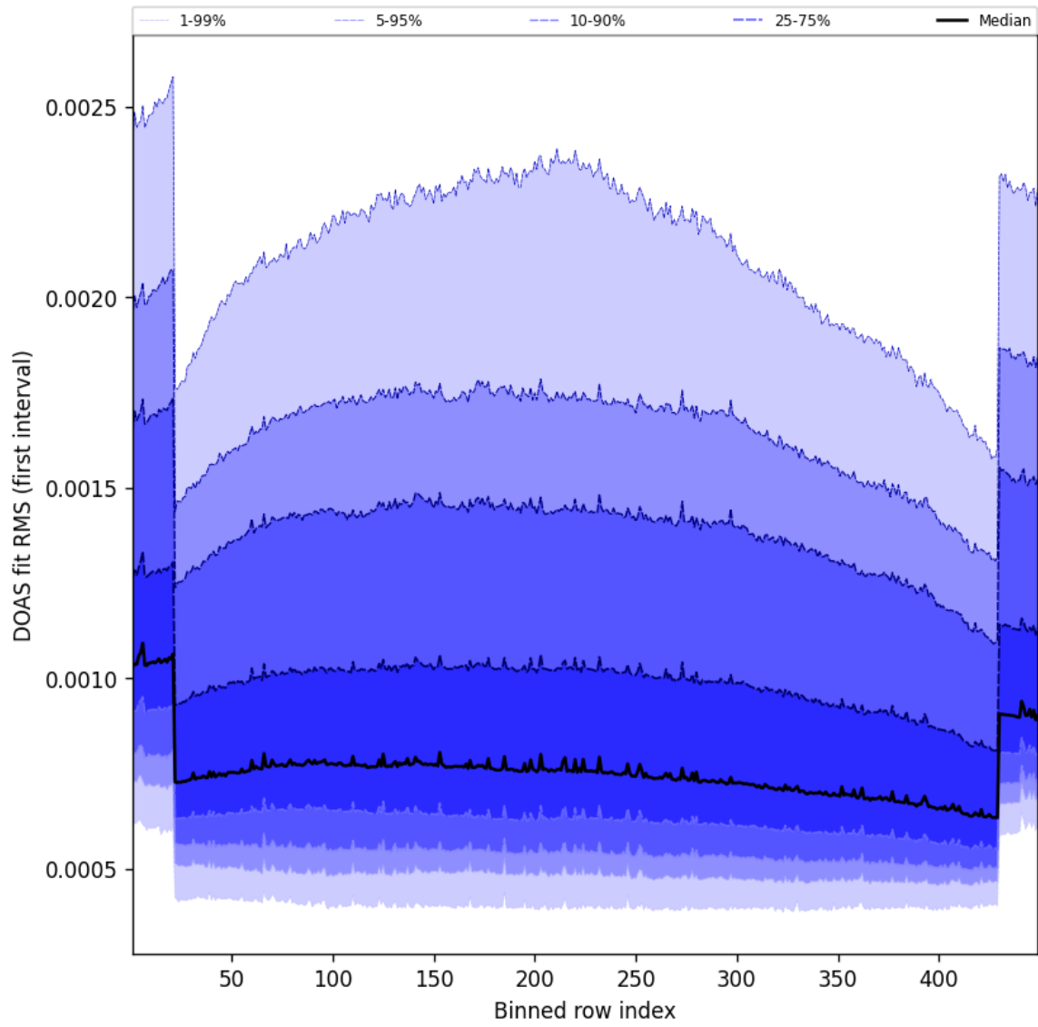
Figure 58: Along track statistics of “DOAS fit RMS (first interval)” for 2025-05-31 to 2025-06-01
