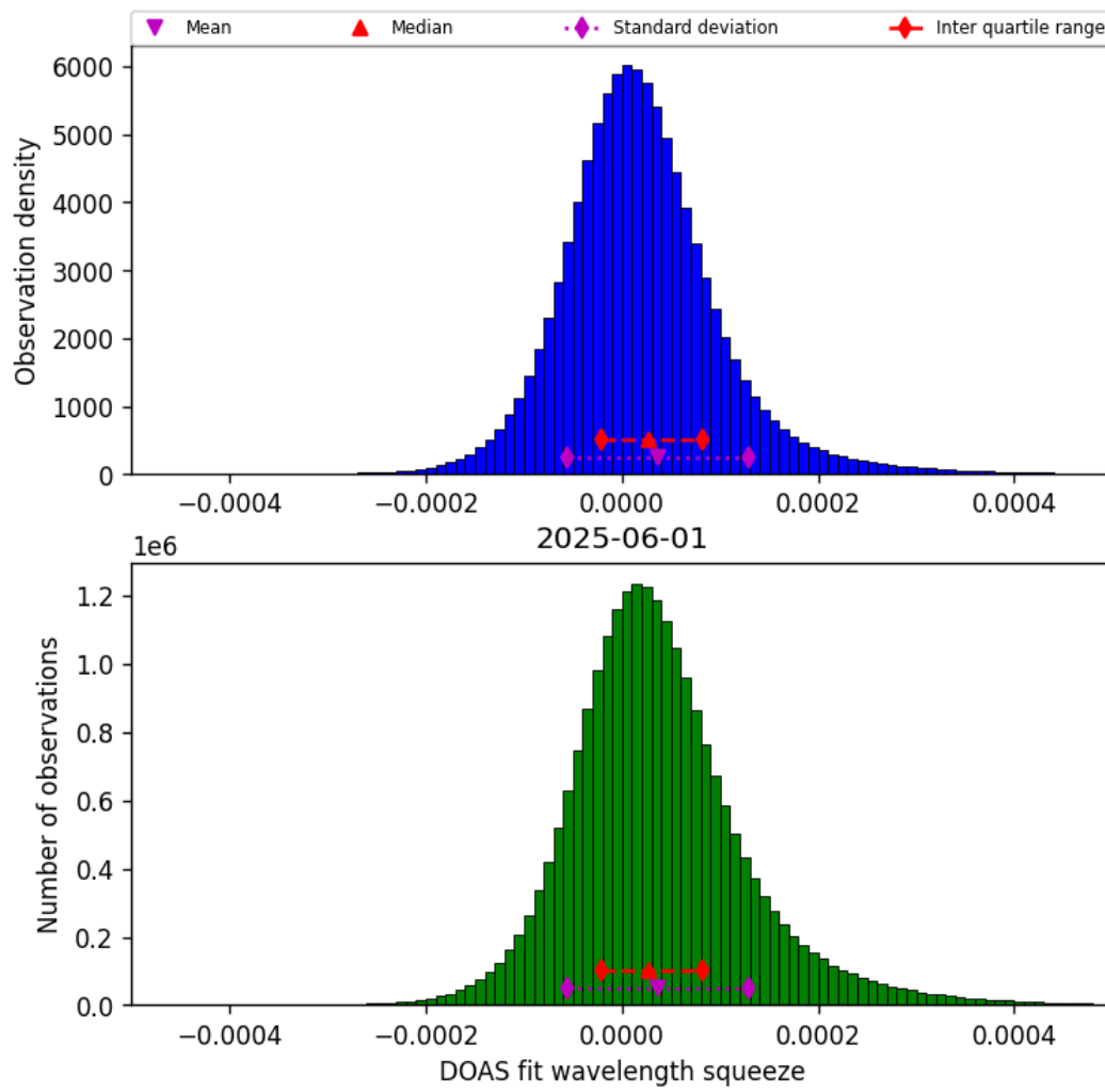
Figure 43: Histogram of “DOAS fit wavelength squeeze” for 2025-06-01 to 2025-06-02
