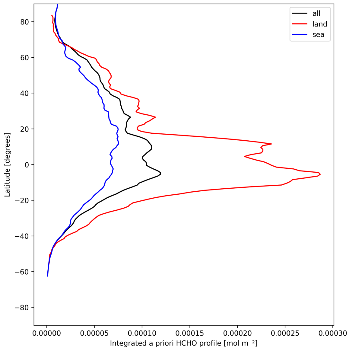
Figure 27: Zonal average of “Integrated a priori HCHO profile” for 2025-06-01 to 2025-06-02.
