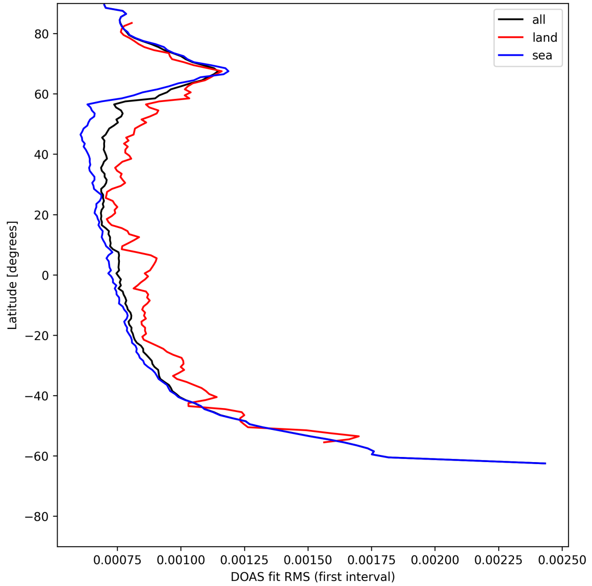
Figure 30: Zonal average of “DOAS fit RMS (first interval)” for 2025-06-01 to 2025-06-02.
