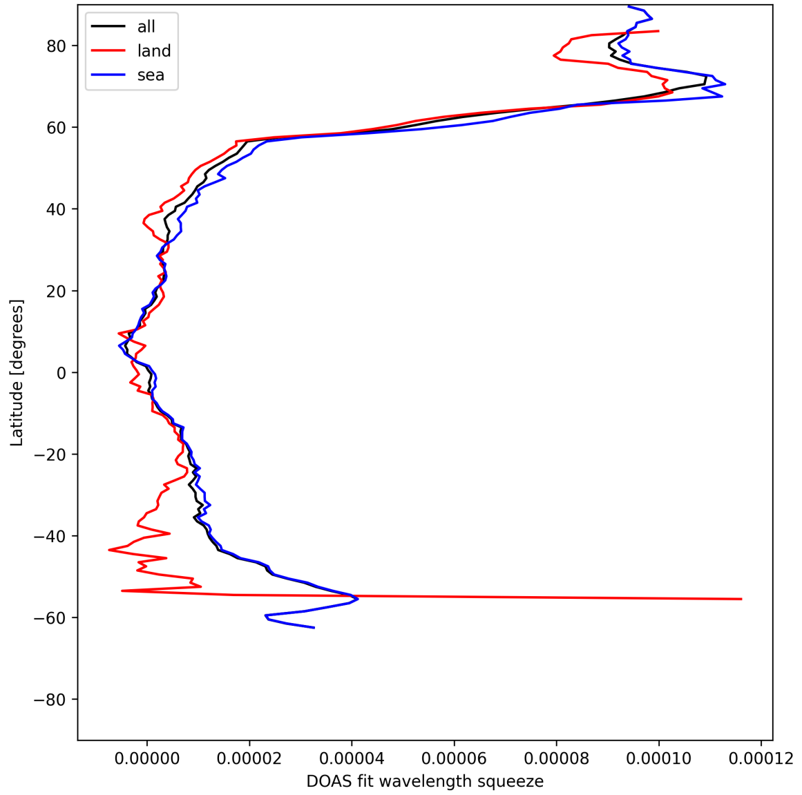
Figure 29: Zonal average of “DOAS fit wavelength squeeze” for 2025-06-01 to 2025-06-02.
