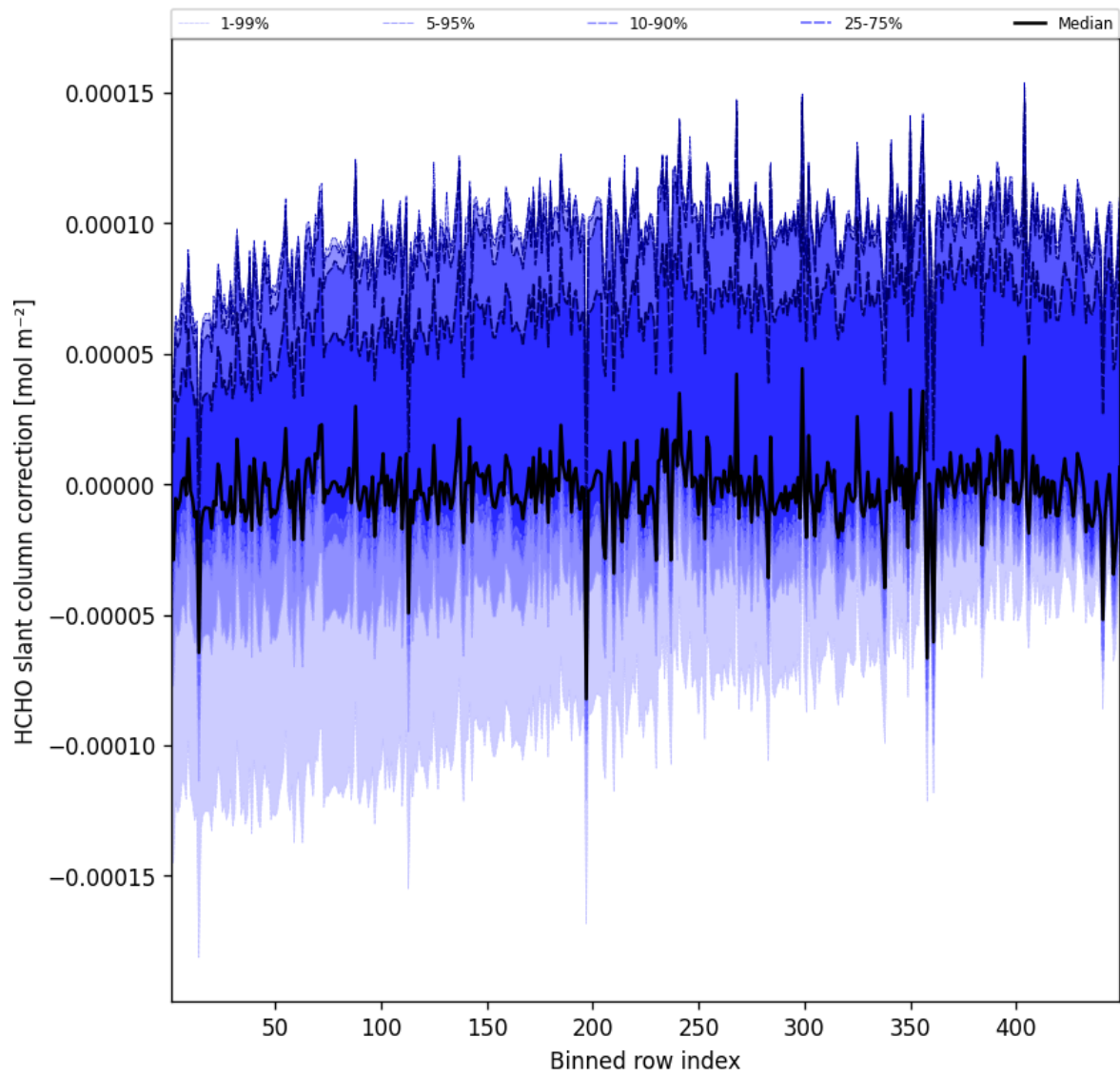
Figure 59: Along track statistics of “HCHO slant column correction” for 2025-06-01 to 2025-06-02
