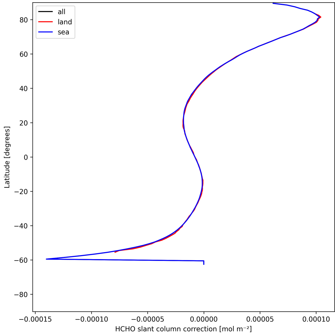
Figure 31: Zonal average of “HCHO slant column correction” for 2025-06-01 to 2025-06-02.
