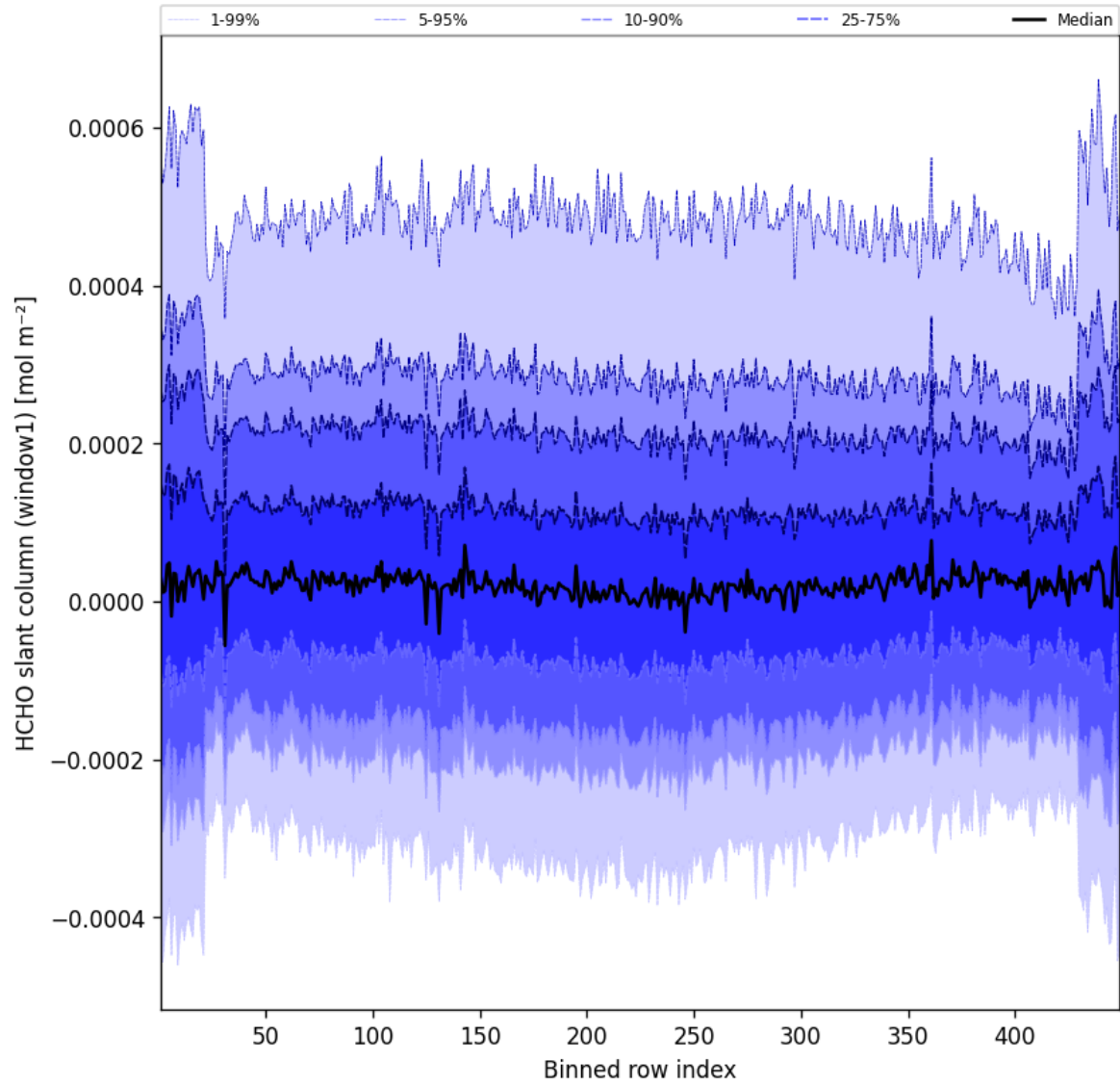
Figure 50: Along track statistics of “HCHO slant column (window1)” for 2025-06-01 to 2025-06-02
