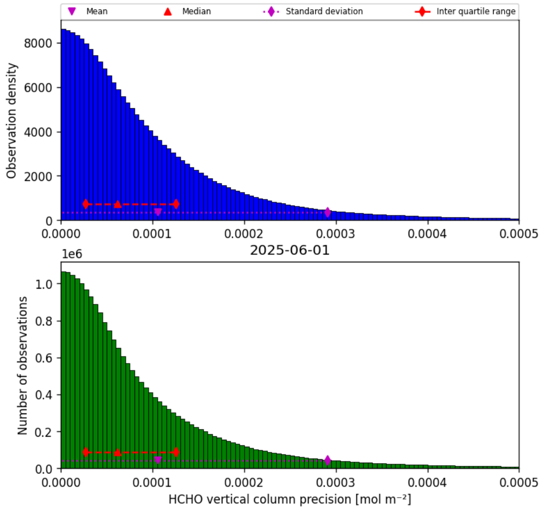
Figure 34: Histogram of “HCHO vertical column precision” for 2025-06-01 to 2025-06-02
