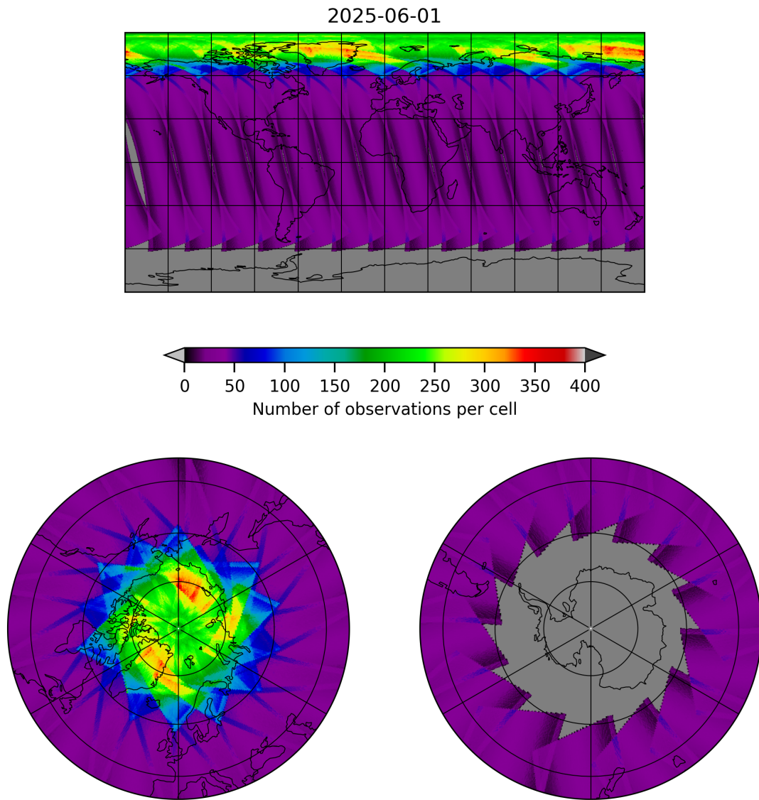
Figure 17: Map of the number of observations for 2025-06-01 to 2025-06-02
