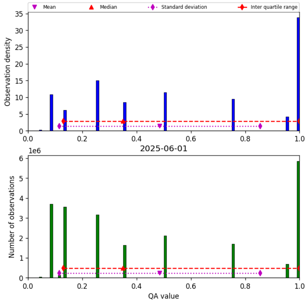
Figure 32: Histogram of “QA value” for 2025-06-01 to 2025-06-02
