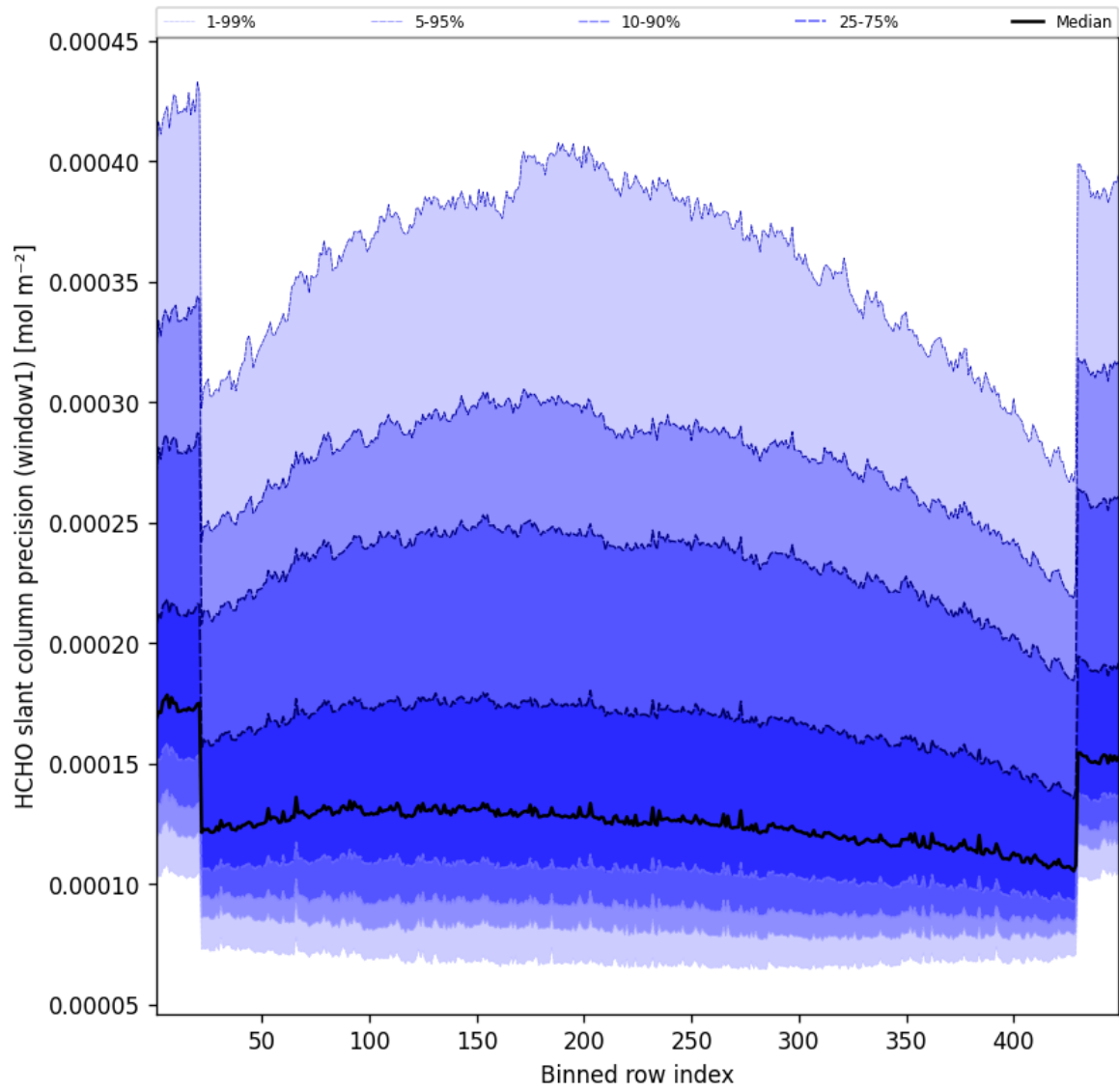
Figure 51: Along track statistics of “HCHO slant column precision (window1)” for 2025-06-01 to 2025-06-02
