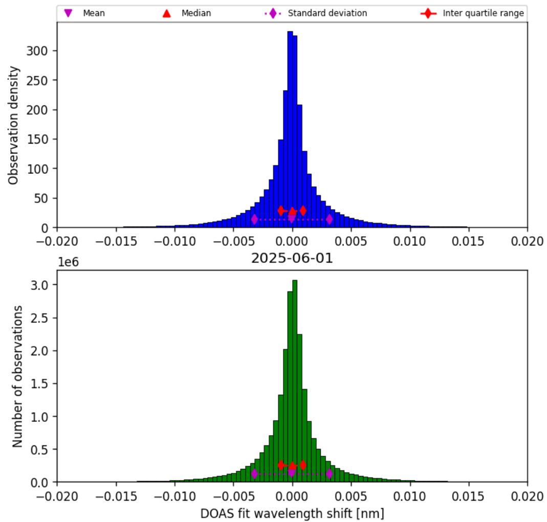
Figure 42: Histogram of “DOAS fit wavelength shift” for 2025-06-01 to 2025-06-02
