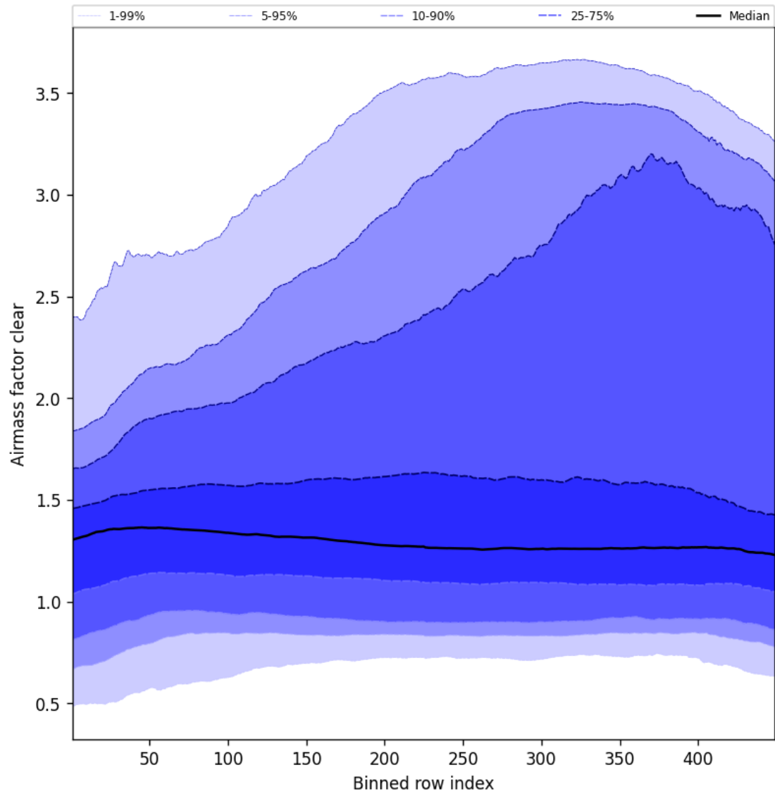
Figure 54: Along track statistics of “Airmass factor clear” for 2025-06-01 to 2025-06-02
