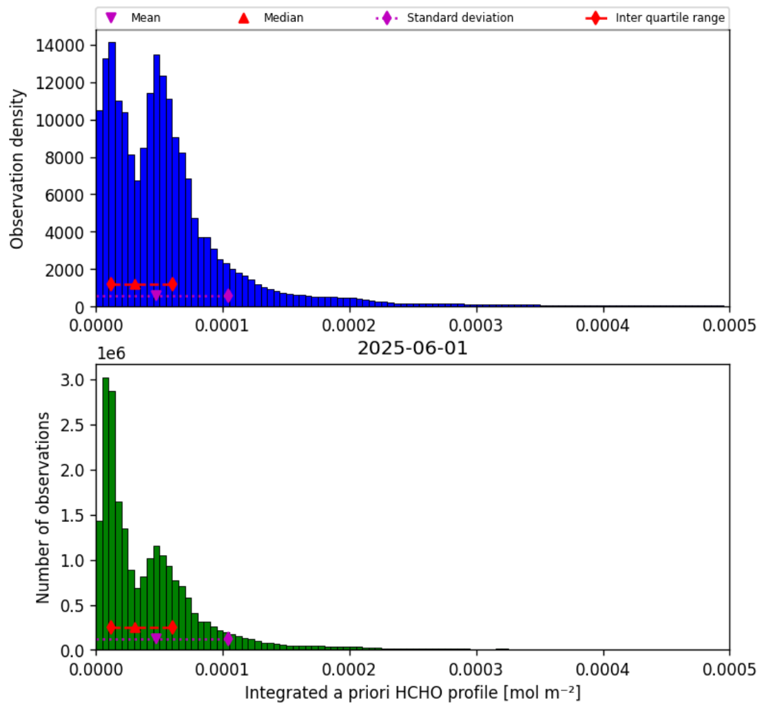
Figure 41: Histogram of “Integrated a priori HCHO profile” for 2025-06-01 to 2025-06-02
