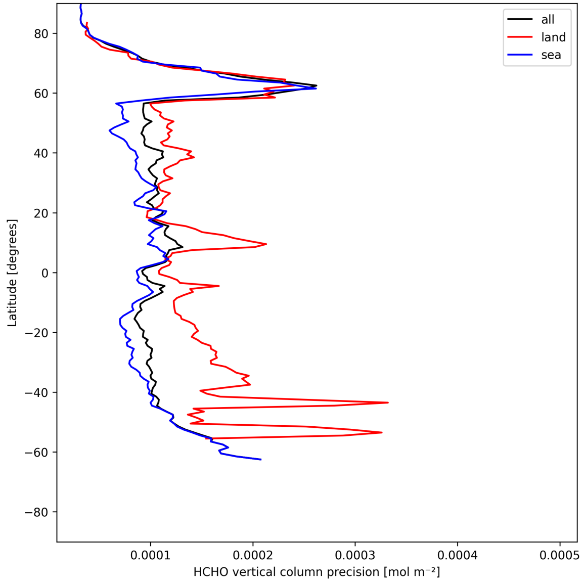
Figure 20: Zonal average of “HCHO vertical column precision” for 2025-06-01 to 2025-06-02.
