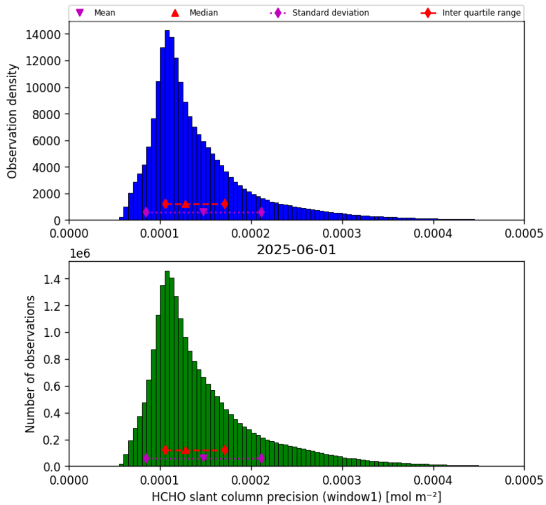
Figure 37: Histogram of “HCHO slant column precision (window1)” for 2025-06-01 to 2025-06-02
