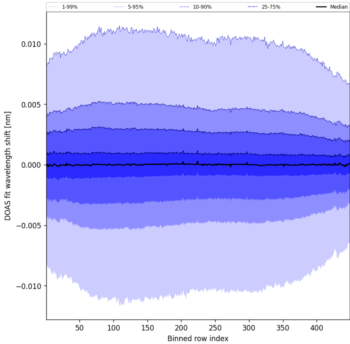
Figure 56: Along track statistics of “DOAS fit wavelength shift” for 2025-06-01 to 2025-06-02
