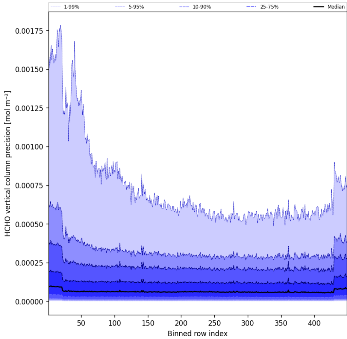
Figure 48: Along track statistics of “HCHO vertical column precision” for 2025-06-01 to 2025-06-02
