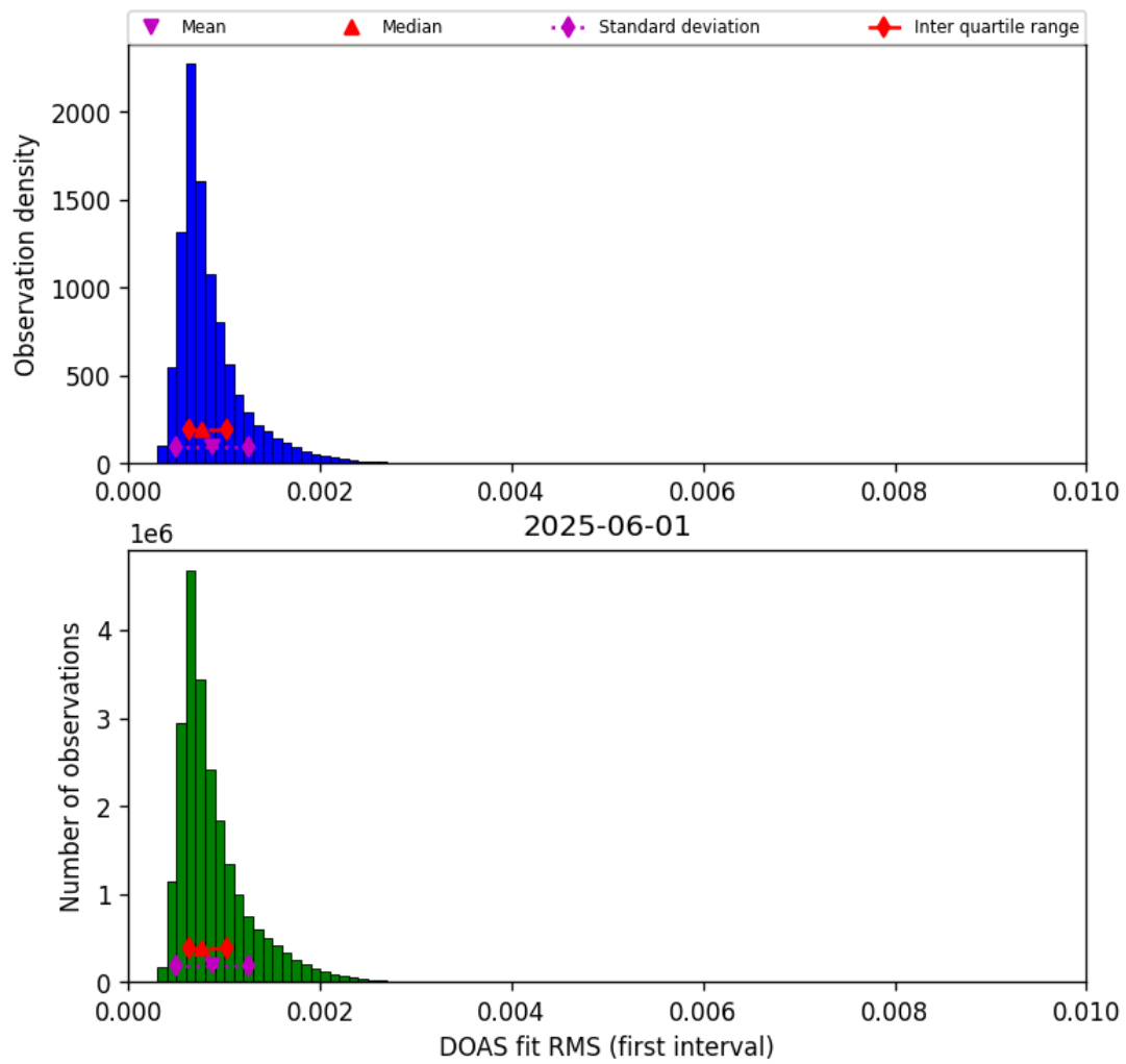
Figure 44: Histogram of “DOAS fit RMS (first interval)” for 2025-06-01 to 2025-06-02
