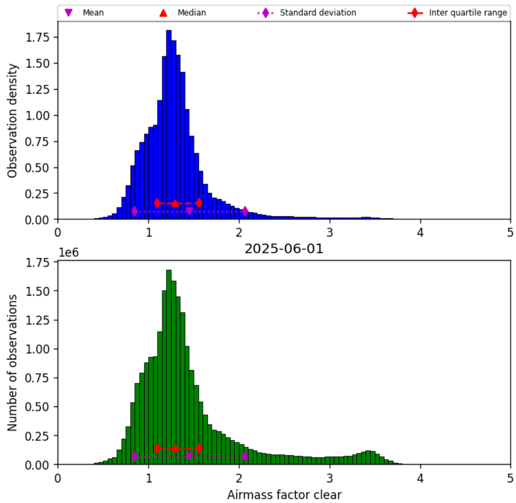
Figure 40: Histogram of “Airmass factor clear” for 2025-06-01 to 2025-06-02
