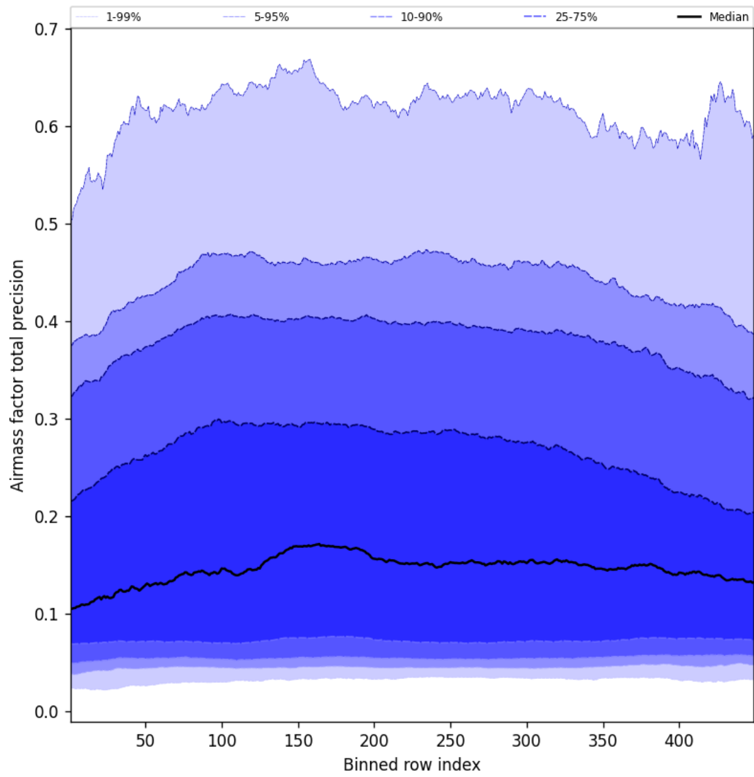
Figure 53: Along track statistics of “Airmass factor total precision” for 2025-06-01 to 2025-06-02
