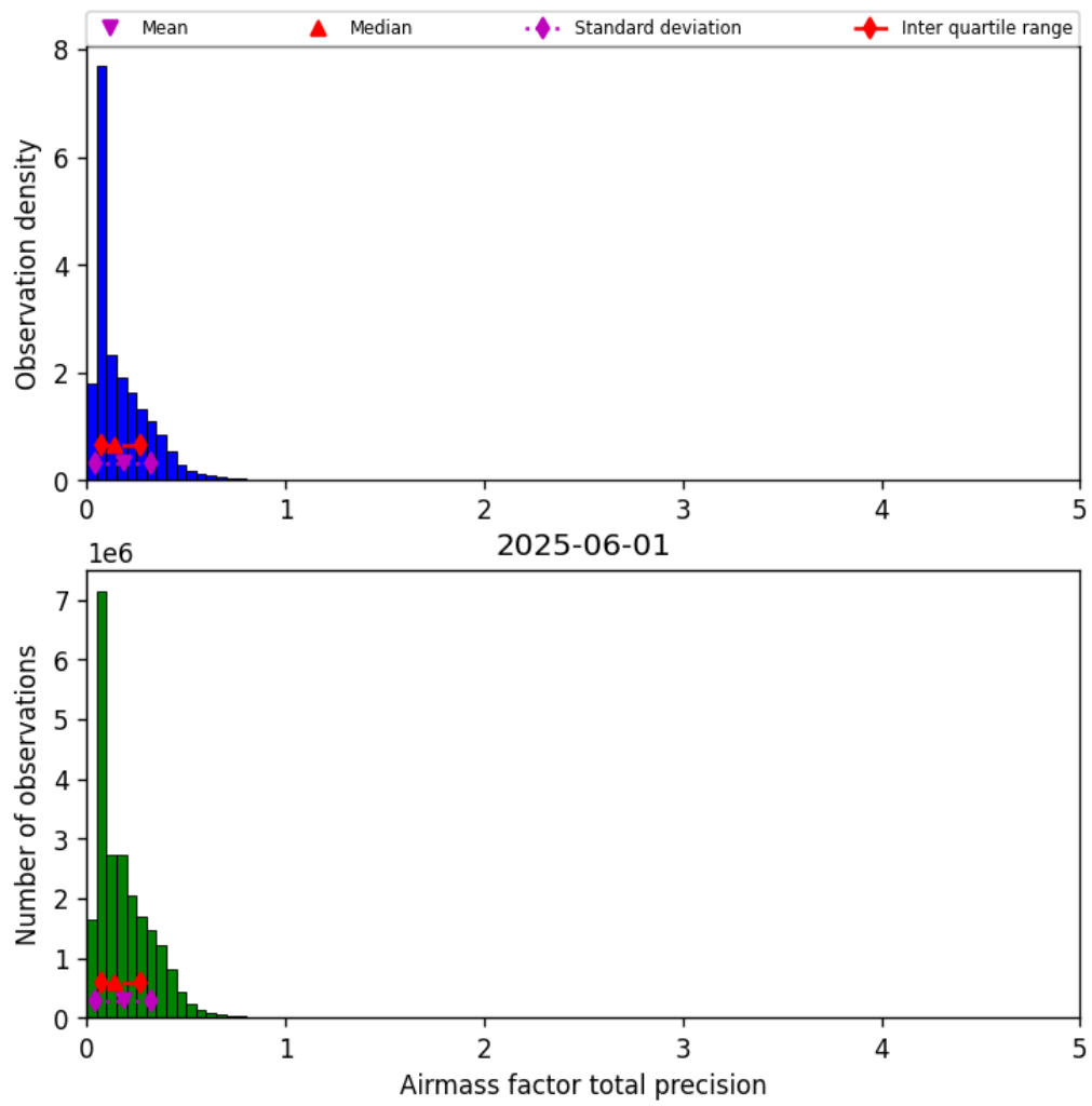
Figure 39: Histogram of “Airmass factor total precision” for 2025-06-01 to 2025-06-02
