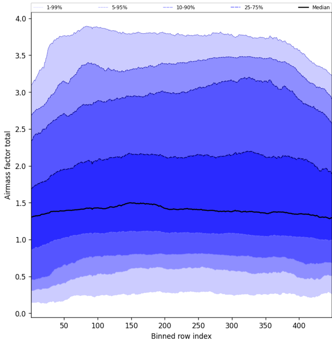
Figure 52: Along track statistics of “Airmass factor total” for 2025-06-01 to 2025-06-02
