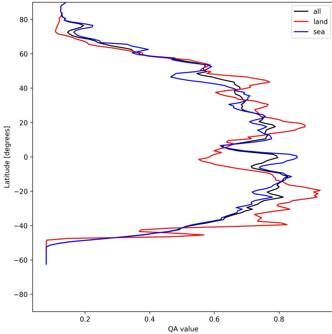
Figure 18: Zonal average of “QA value” for 2025-06-01 to 2025-06-02.
