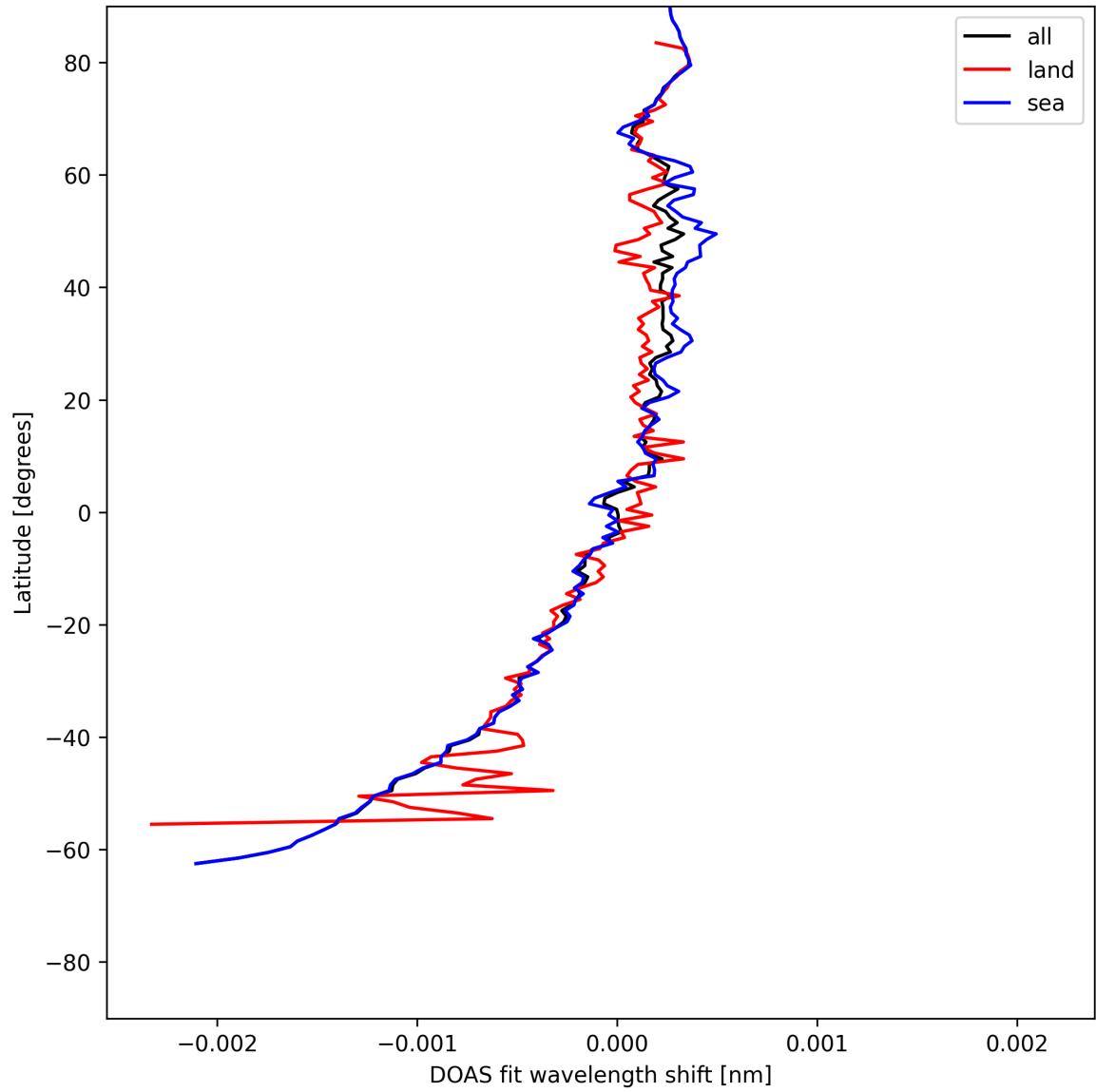
Figure 28: Zonal average of “DOAS fit wavelength shift” for 2025-06-01 to 2025-06-02.
