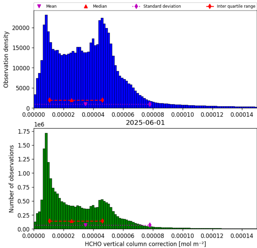
Figure 35: Histogram of “HCHO vertical column correction” for 2025-06-01 to 2025-06-02
