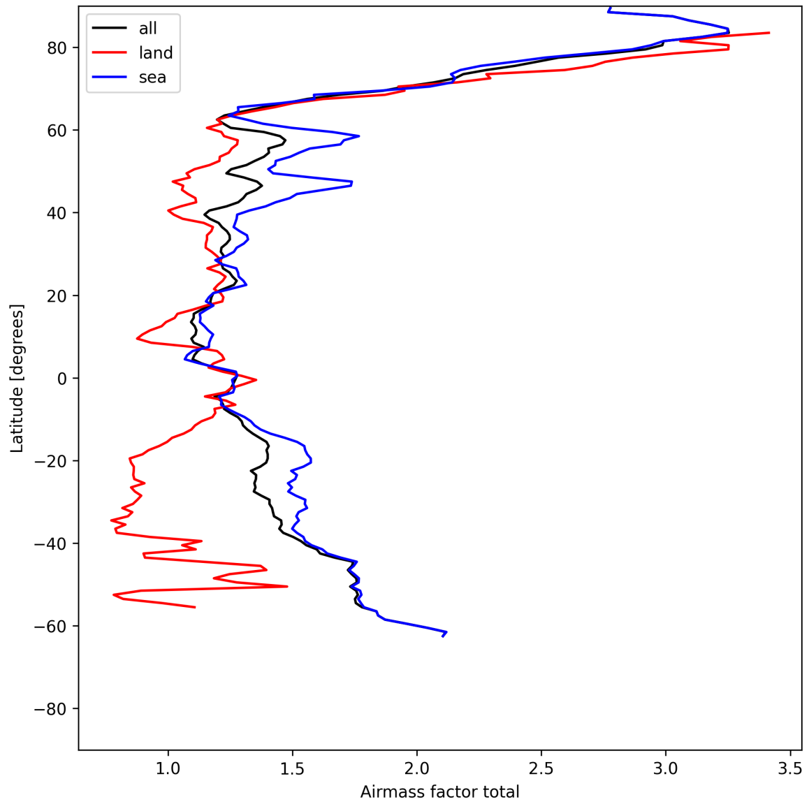
Figure 24: Zonal average of “Airmass factor total” for 2025-06-01 to 2025-06-02.
