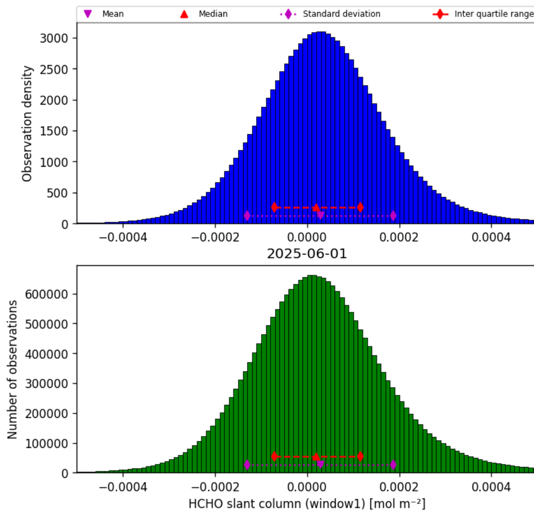
Figure 36: Histogram of “HCHO slant column (window1)” for 2025-06-01 to 2025-06-02
