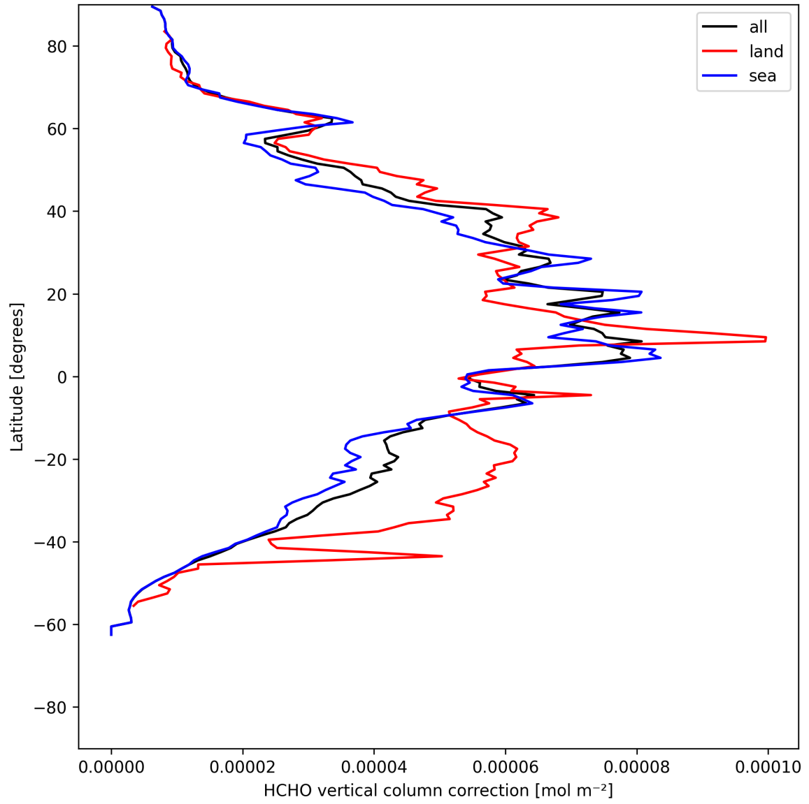
Figure 21: Zonal average of “HCHO vertical column correction” for 2025-06-01 to 2025-06-02.
