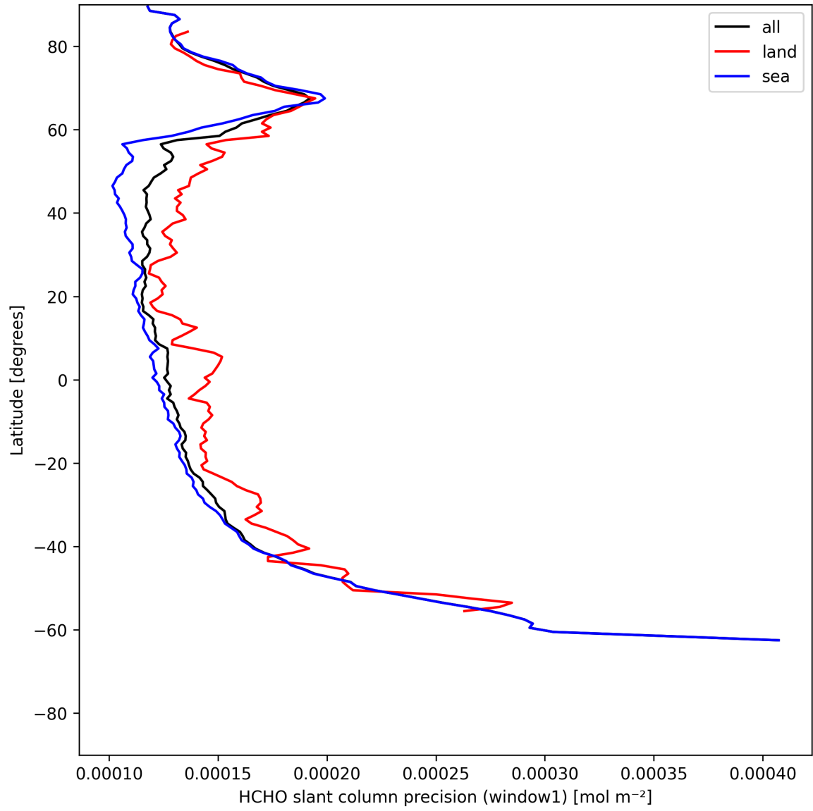
Figure 23: Zonal average of “HCHO slant column precision (window1)” for 2025-06-01 to 2025-06-02.
