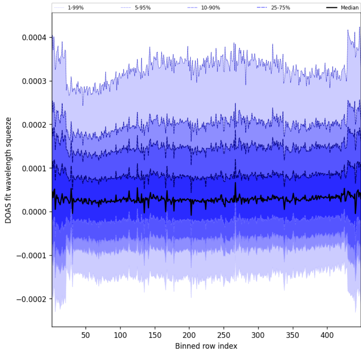
Figure 57: Along track statistics of “DOAS fit wavelength squeeze” for 2025-06-01 to 2025-06-02
