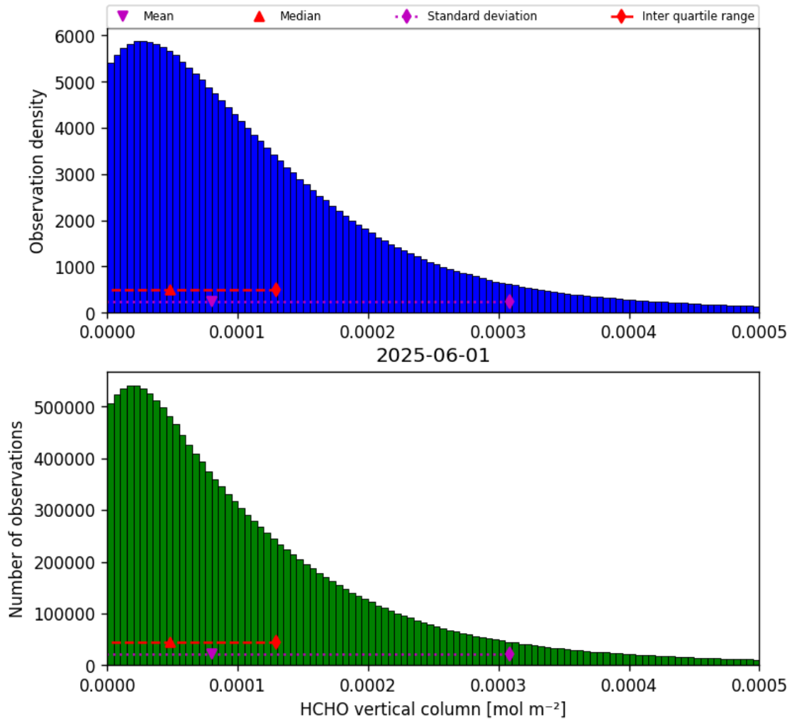
Figure 33: Histogram of “HCHO vertical column” for 2025-06-01 to 2025-06-02
