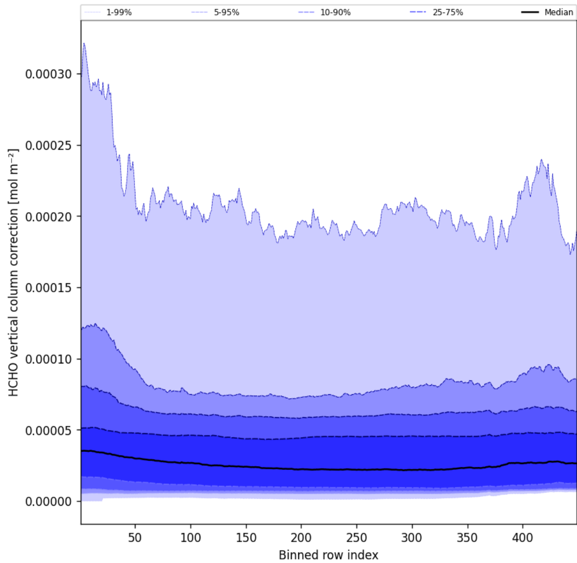
Figure 49: Along track statistics of “HCHO vertical column correction” for 2025-06-01 to 2025-06-02
