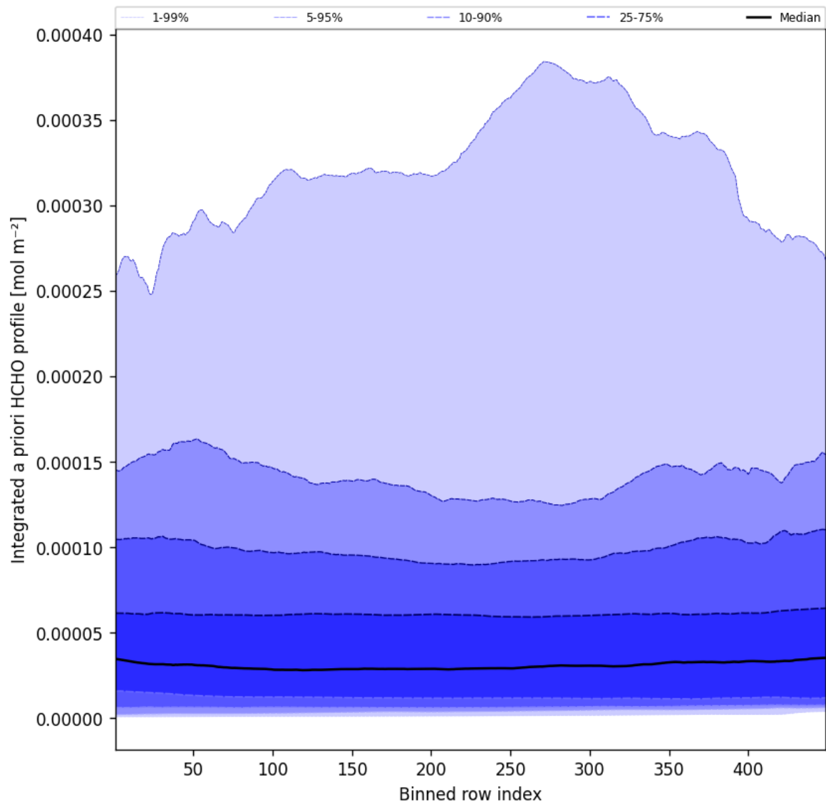
Figure 55: Along track statistics of “Integrated a priori HCHO profile” for 2025-06-01 to 2025-06-02
