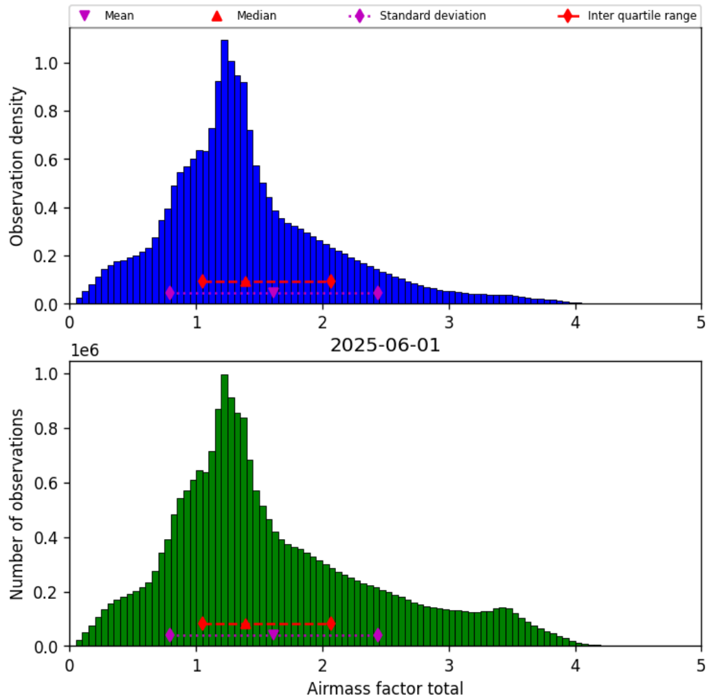
Figure 38: Histogram of “Airmass factor total” for 2025-06-01 to 2025-06-02
