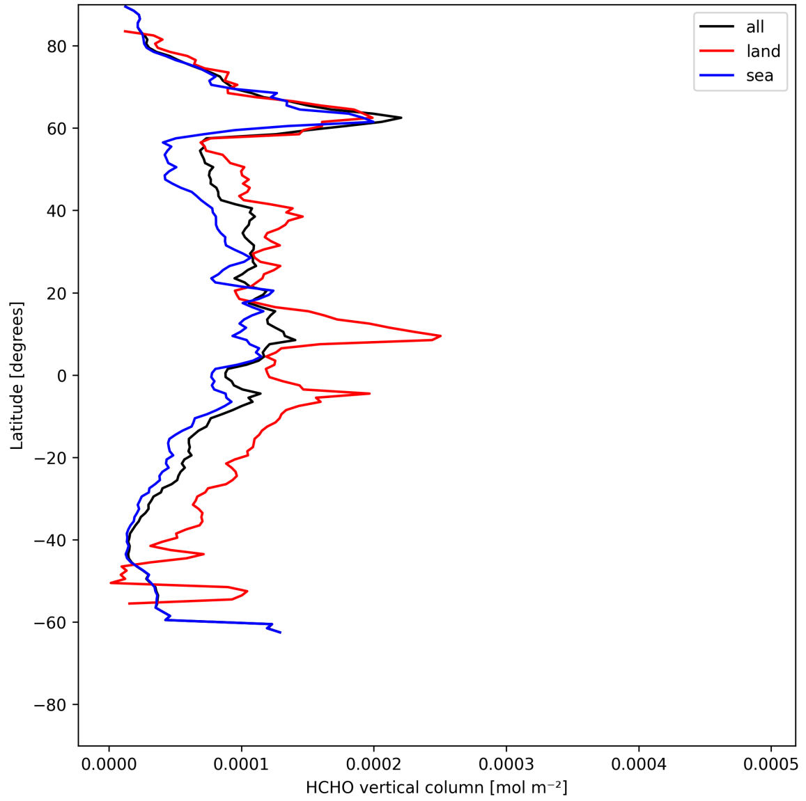
Figure 19: Zonal average of “HCHO vertical column” for 2025-06-01 to 2025-06-02.
