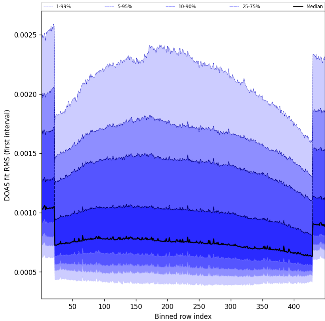
Figure 58: Along track statistics of “DOAS fit RMS (first interval)” for 2025-06-01 to 2025-06-02
