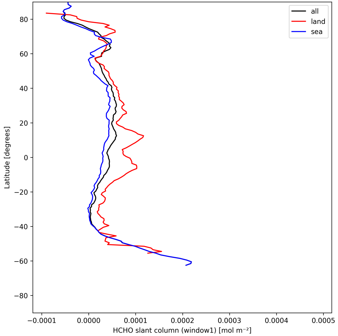
Figure 22: Zonal average of “HCHO slant column (window1)” for 2025-06-01 to 2025-06-02.
