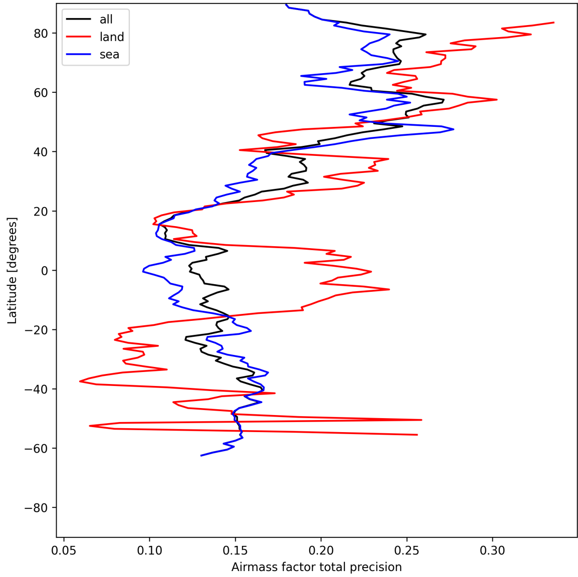
Figure 25: Zonal average of “Airmass factor total precision” for 2025-06-01 to 2025-06-02.
