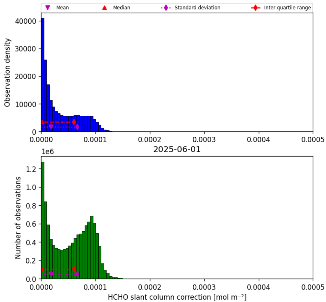
Figure 45: Histogram of “HCHO slant column correction” for 2025-06-01 to 2025-06-02
