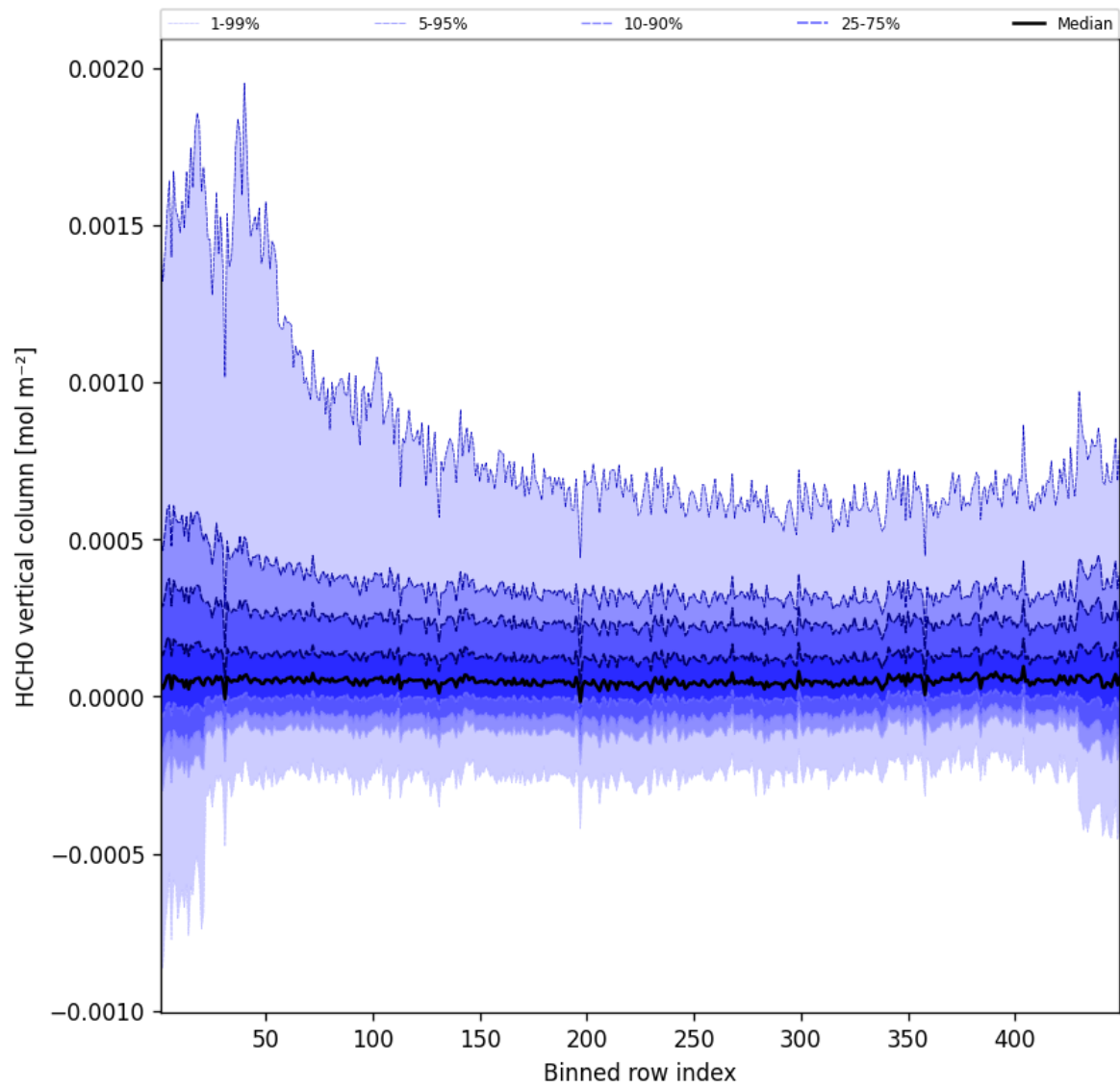
Figure 47: Along track statistics of “HCHO vertical column” for 2025-06-01 to 2025-06-02
