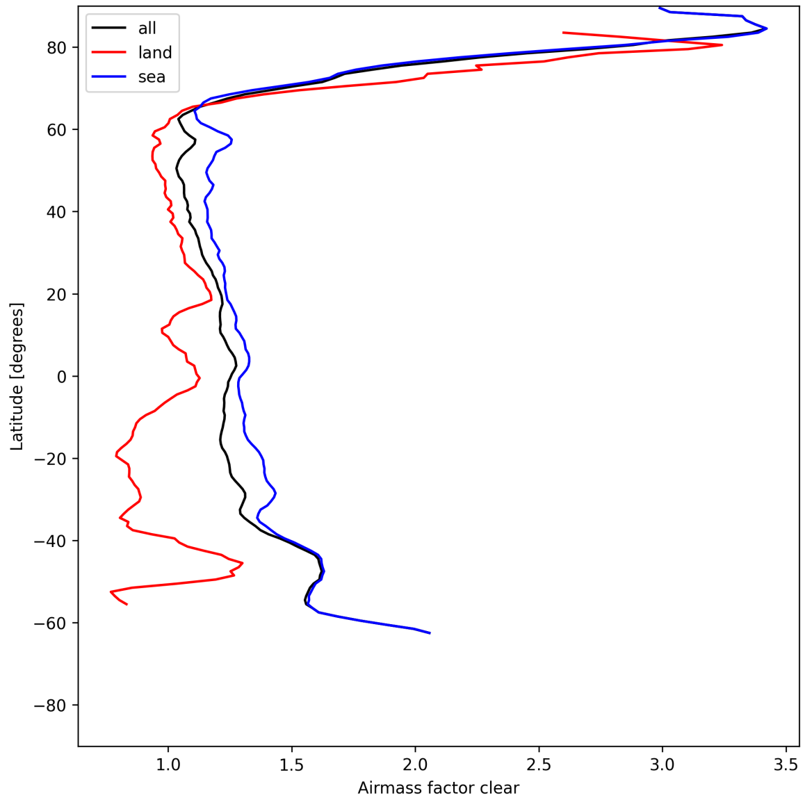
Figure 26: Zonal average of “Airmass factor clear” for 2025-06-01 to 2025-06-02.
