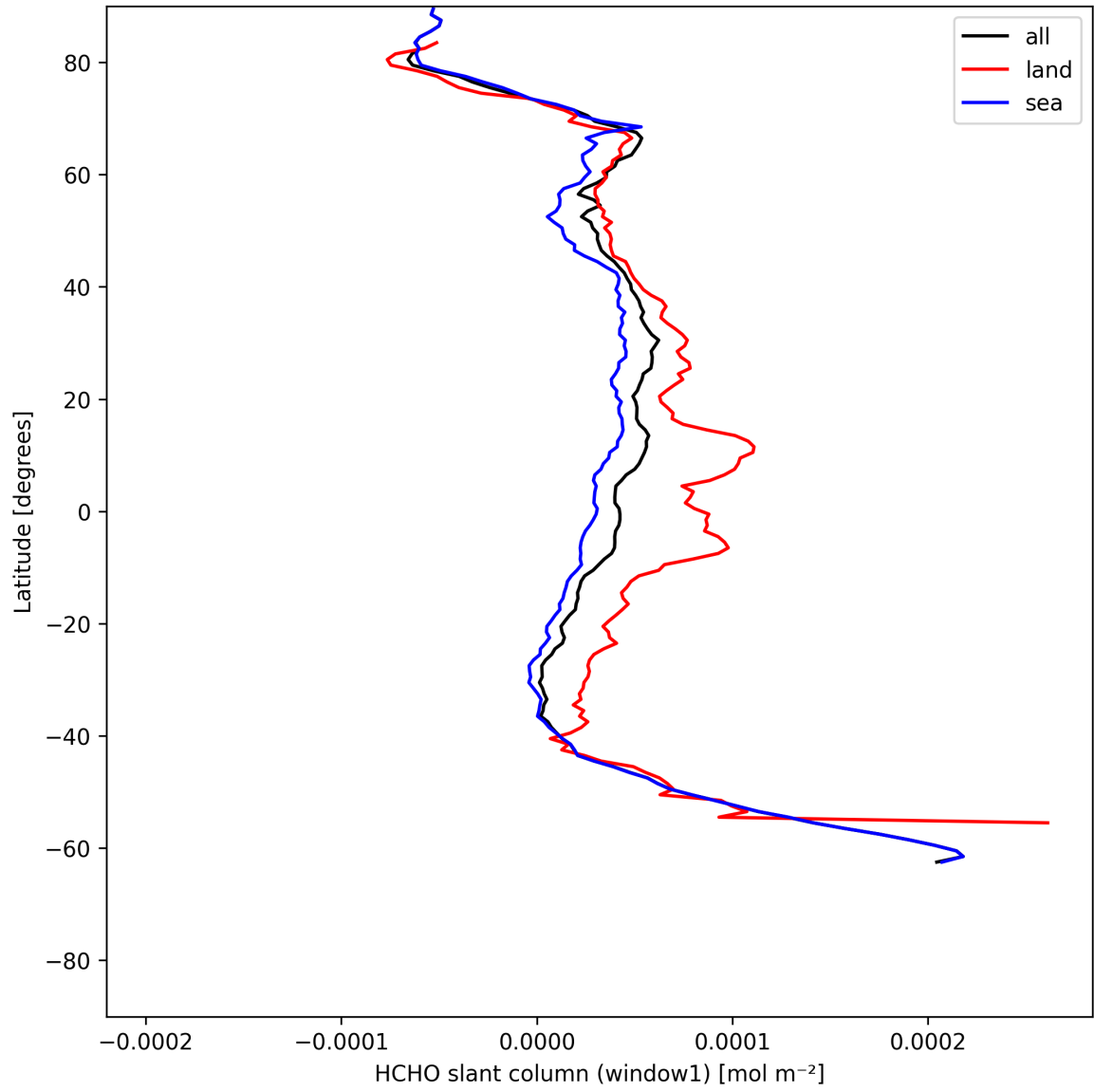
Figure 22: Zonal average of “HCHO slant column (window1)” for 2025-06-02 to 2025-06-03.
