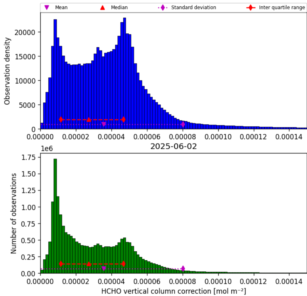
Figure 35: Histogram of “HCHO vertical column correction” for 2025-06-02 to 2025-06-03
