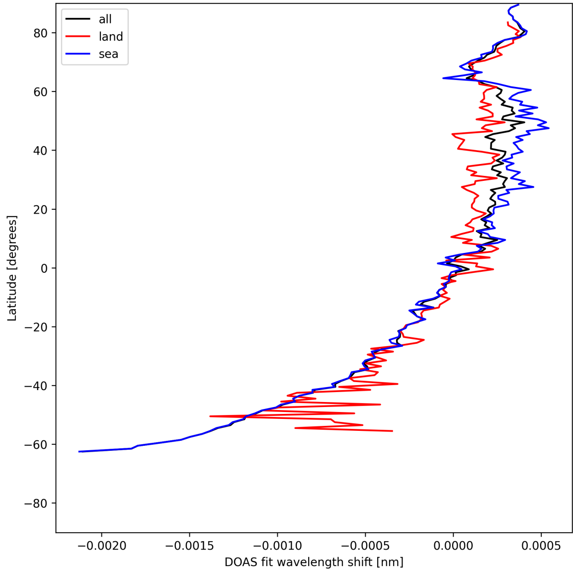
Figure 28: Zonal average of “DOAS fit wavelength shift” for 2025-06-02 to 2025-06-03.
