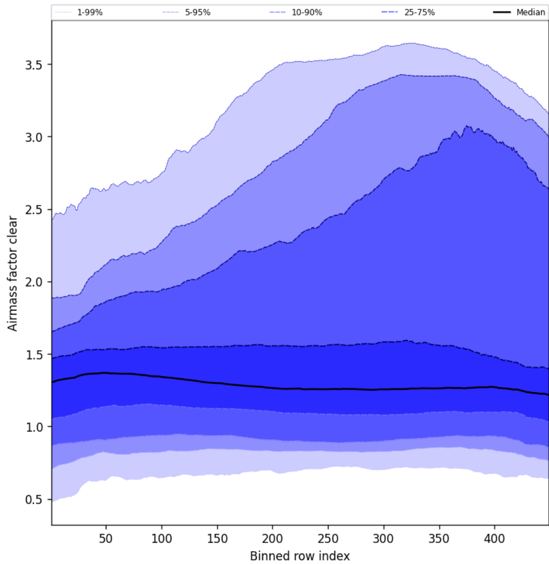
Figure 54: Along track statistics of “Airmass factor clear” for 2025-06-02 to 2025-06-03
