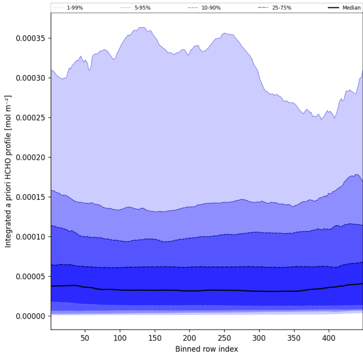
Figure 55: Along track statistics of "Integrated a priori HCHO profile" for 2025-06-02 to 2025-06-03
