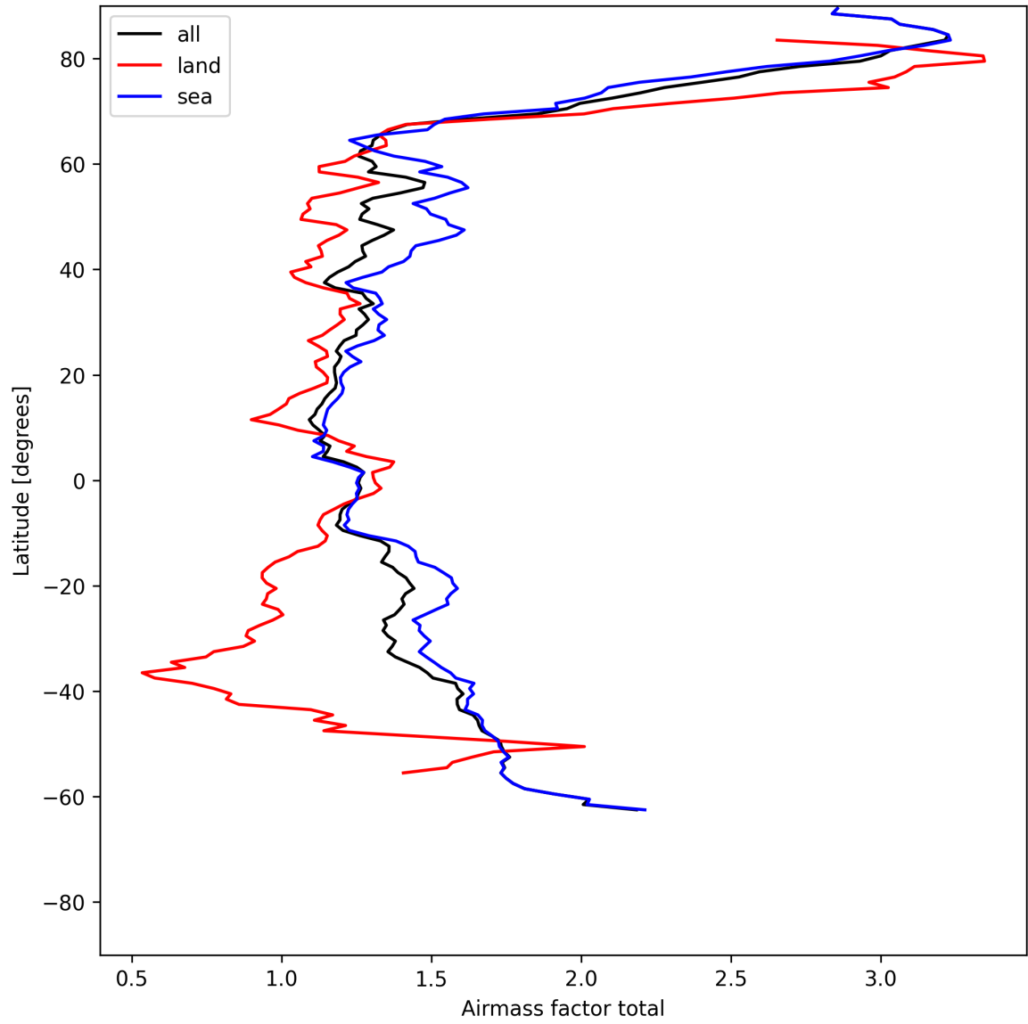
Figure 24: Zonal average of “Airmass factor total” for 2025-06-02 to 2025-06-03.
