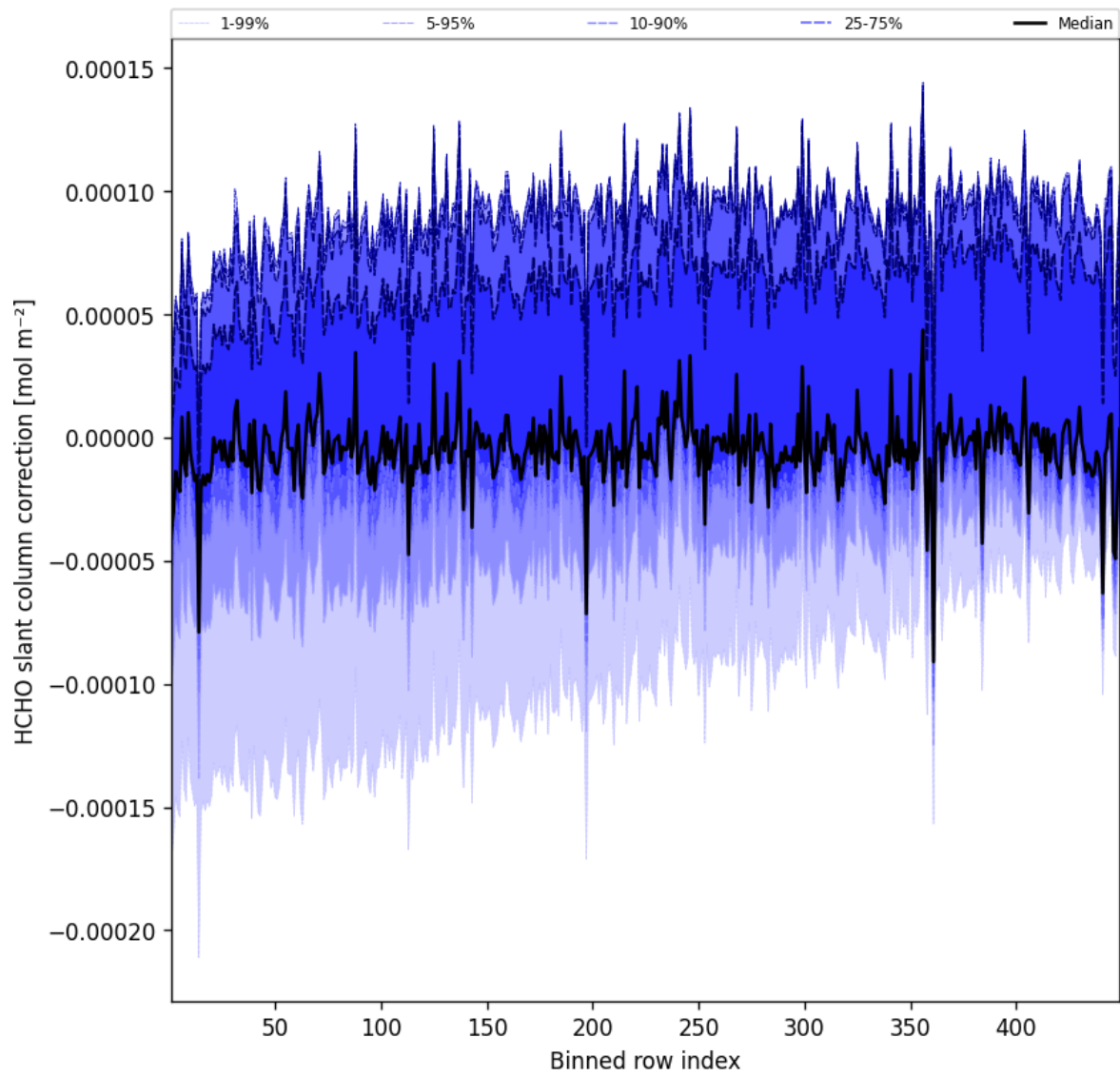
Figure 59: Along track statistics of “HCHO slant column correction” for 2025-06-02 to 2025-06-03
