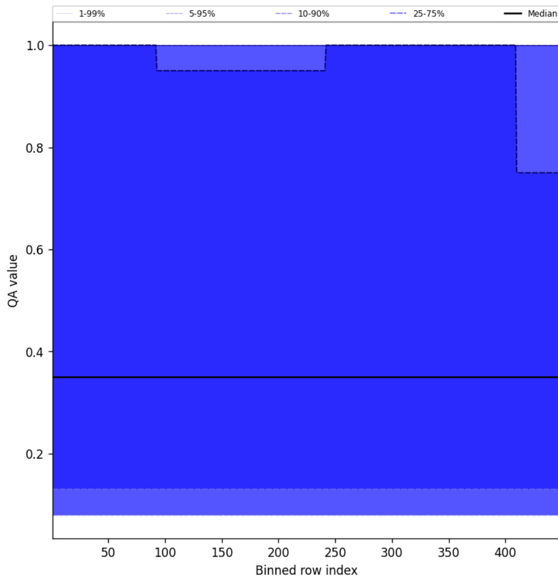
Figure 46: Along track statistics of “QA value” for 2025-06-02 to 2025-06-03
