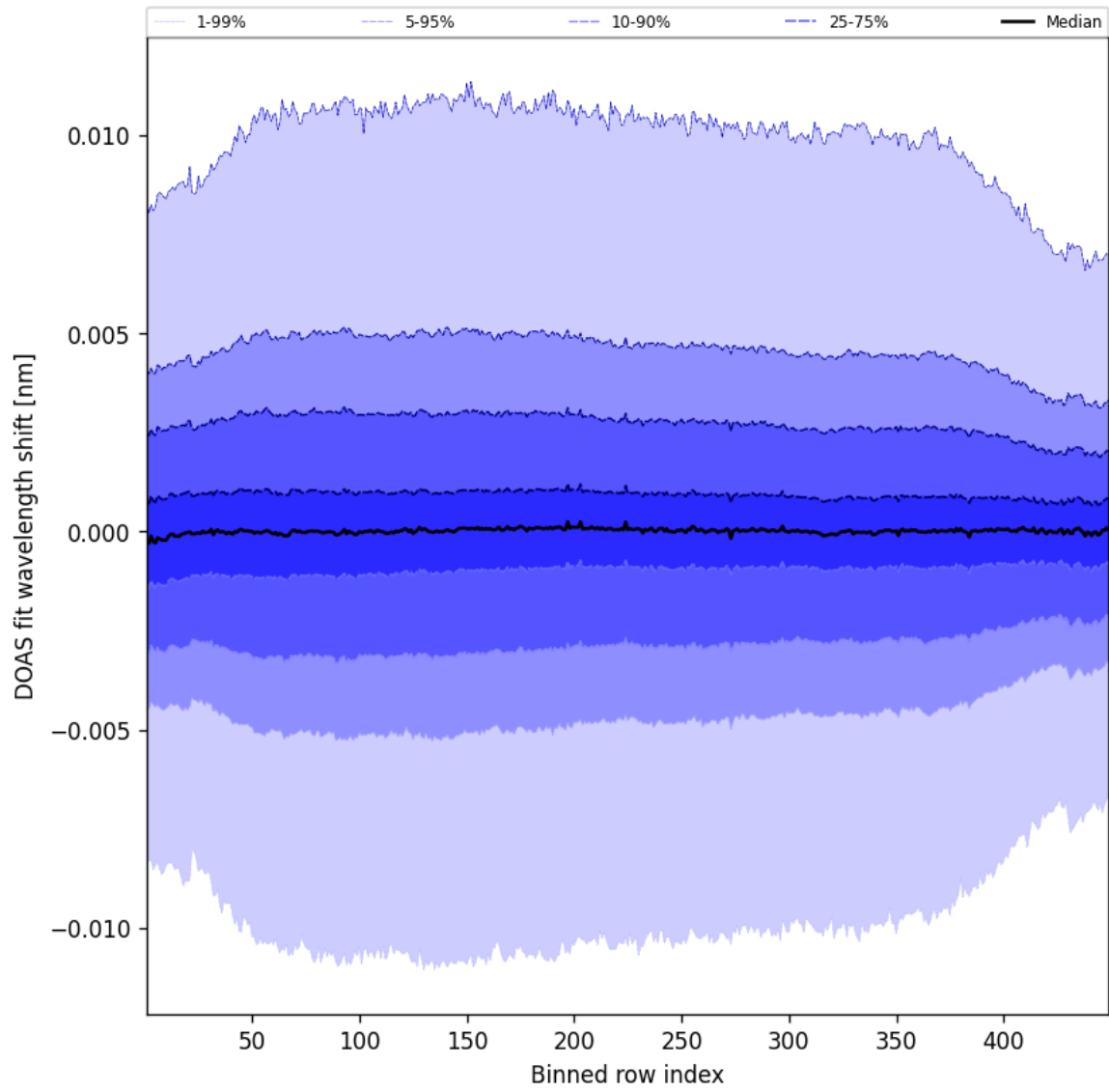
Figure 56: Along track statistics of “DOAS fit wavelength shift” for 2025-06-02 to 2025-06-03
