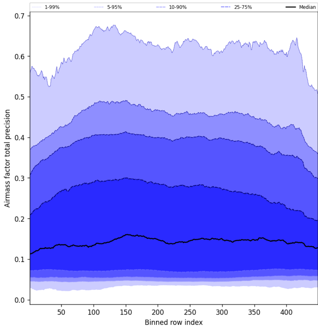
Figure 53: Along track statistics of “Airmass factor total precision” for 2025-06-02 to 2025-06-03
