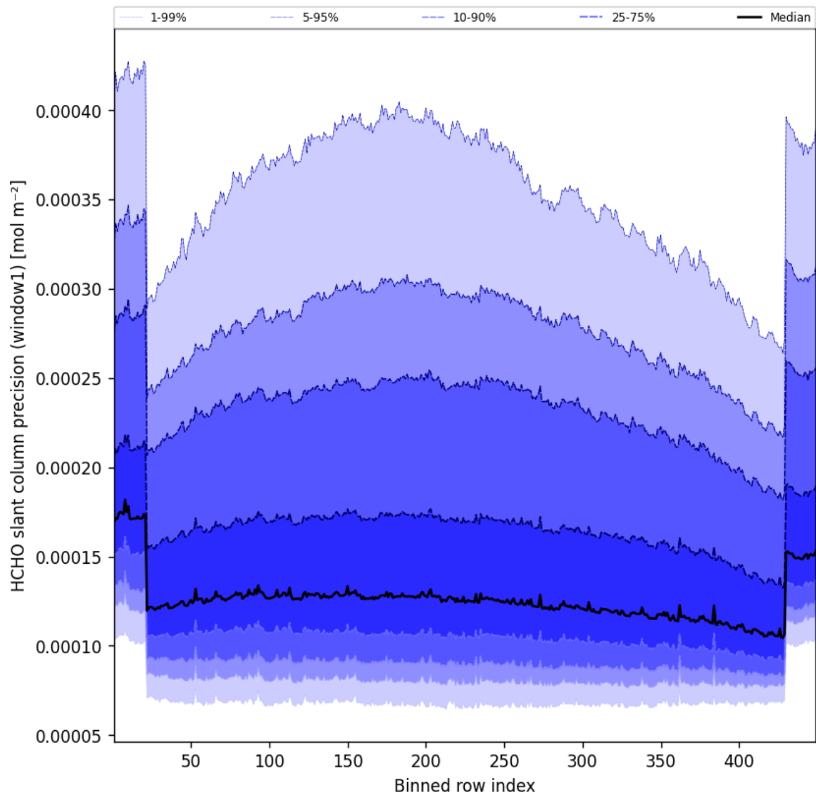
Figure 51: Along track statistics of “HCHO slant column precision (window1)” for 2025-06-02 to 2025-06-03
