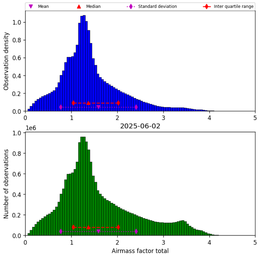
Figure 38: Histogram of “Airmass factor total” for 2025-06-02 to 2025-06-03
