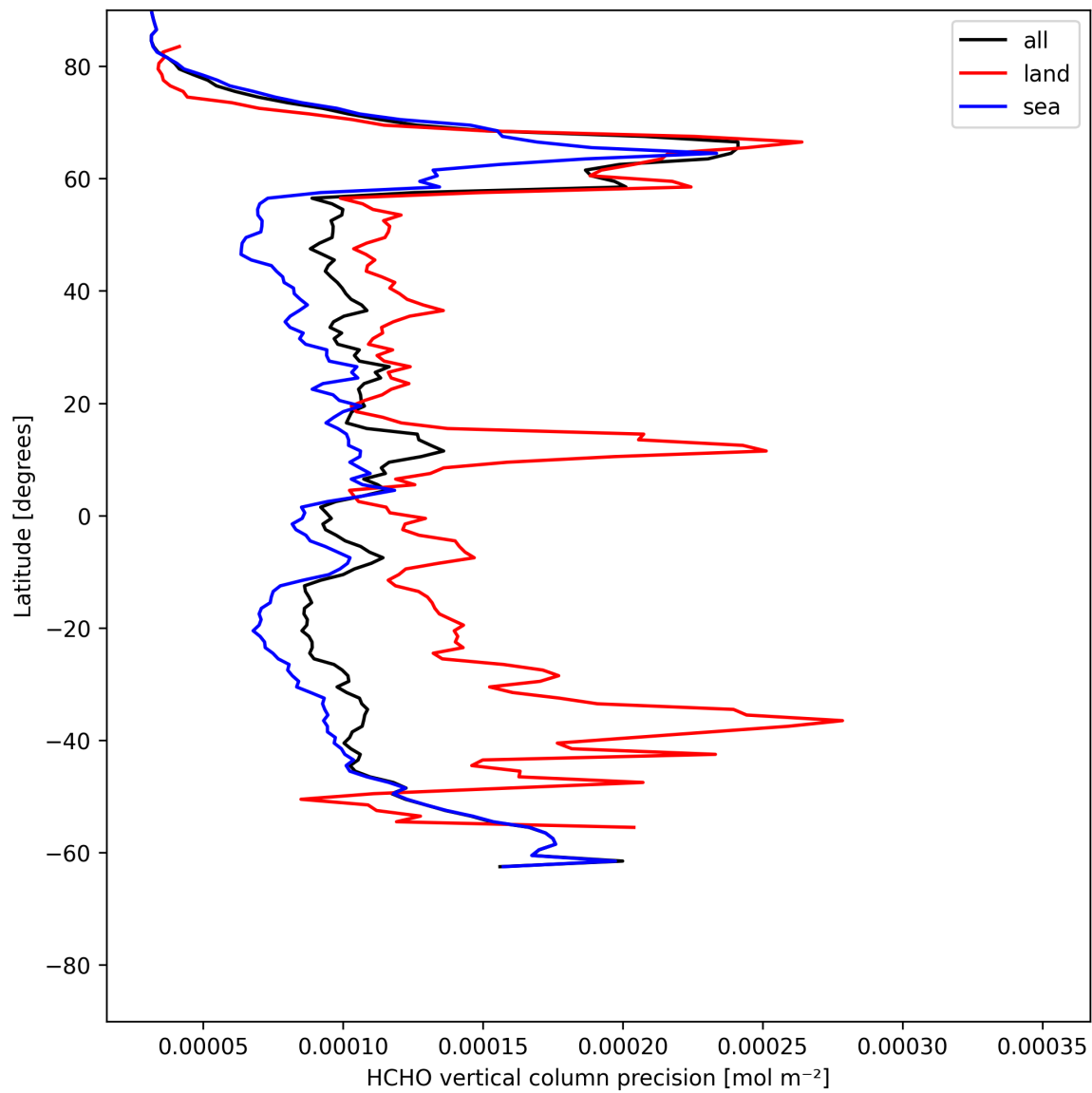
Figure 20: Zonal average of “HCHO vertical column precision” for 2025-06-02 to 2025-06-03.
