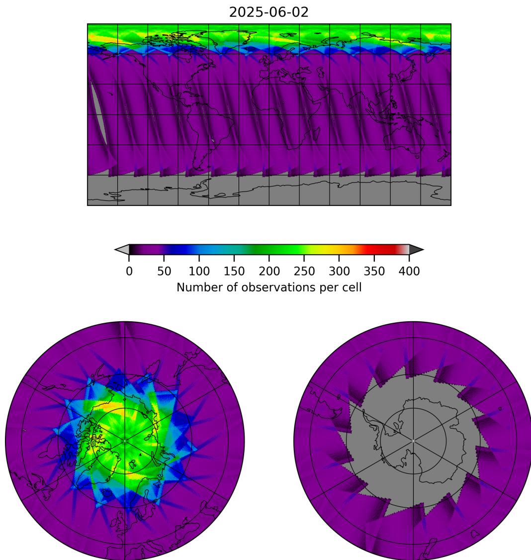
Figure 17: Map of the number of observations for 2025-06-02 to 2025-06-03
