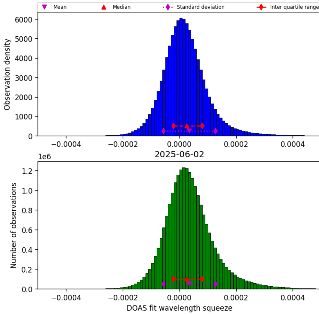
Figure 43: Histogram of “DOAS fit wavelength squeeze” for 2025-06-02 to 2025-06-03
