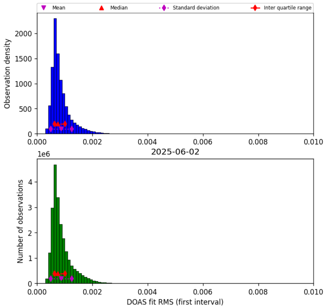
Figure 44: Histogram of “DOAS fit RMS (first interval)” for 2025-06-02 to 2025-06-03
