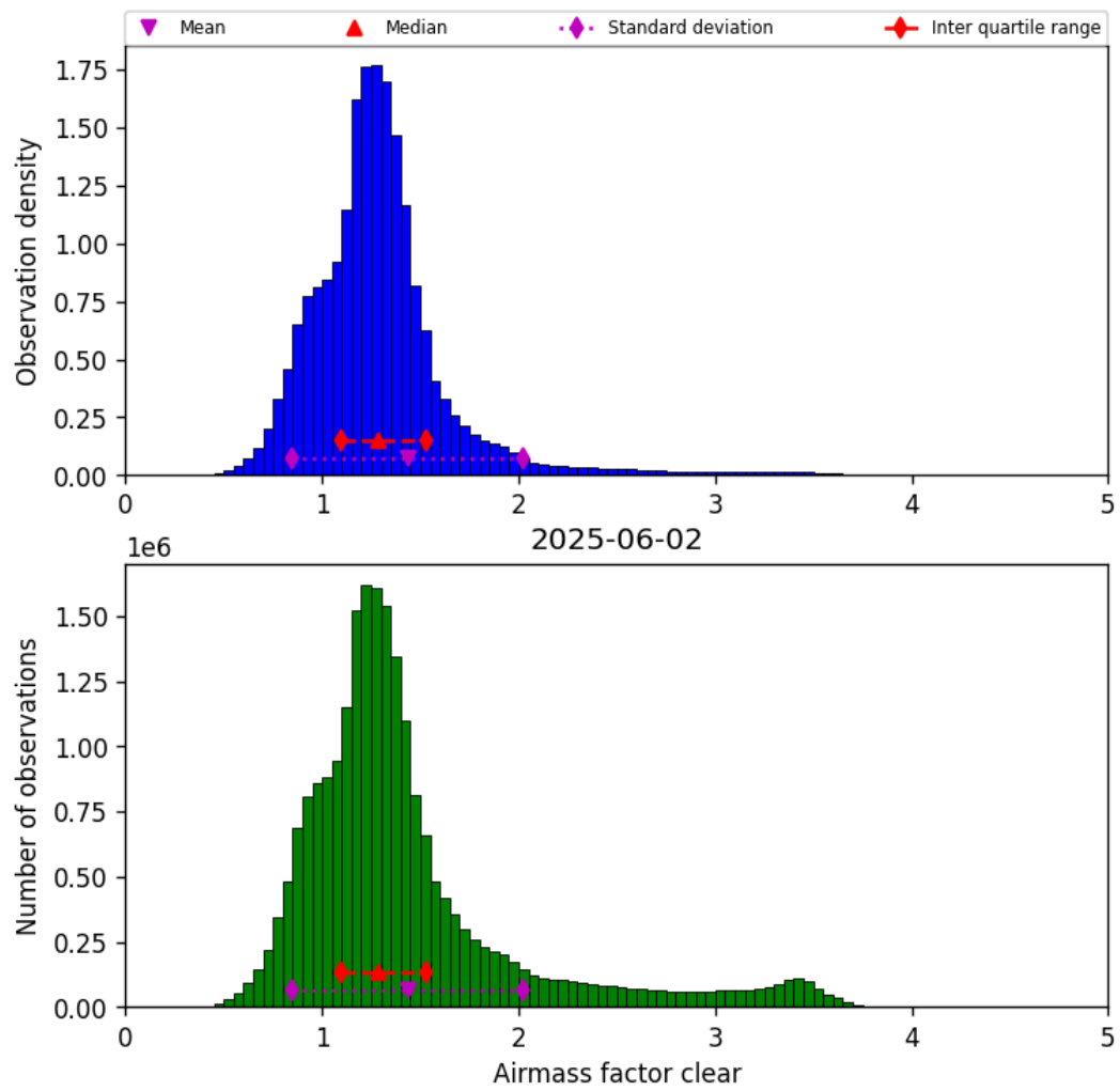
Figure 40: Histogram of “Airmass factor clear” for 2025-06-02 to 2025-06-03
