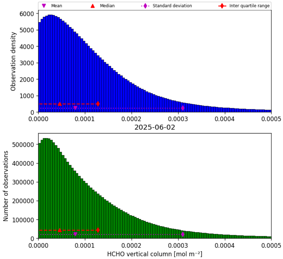
Figure 33: Histogram of “HCHO vertical column” for 2025-06-02 to 2025-06-03
