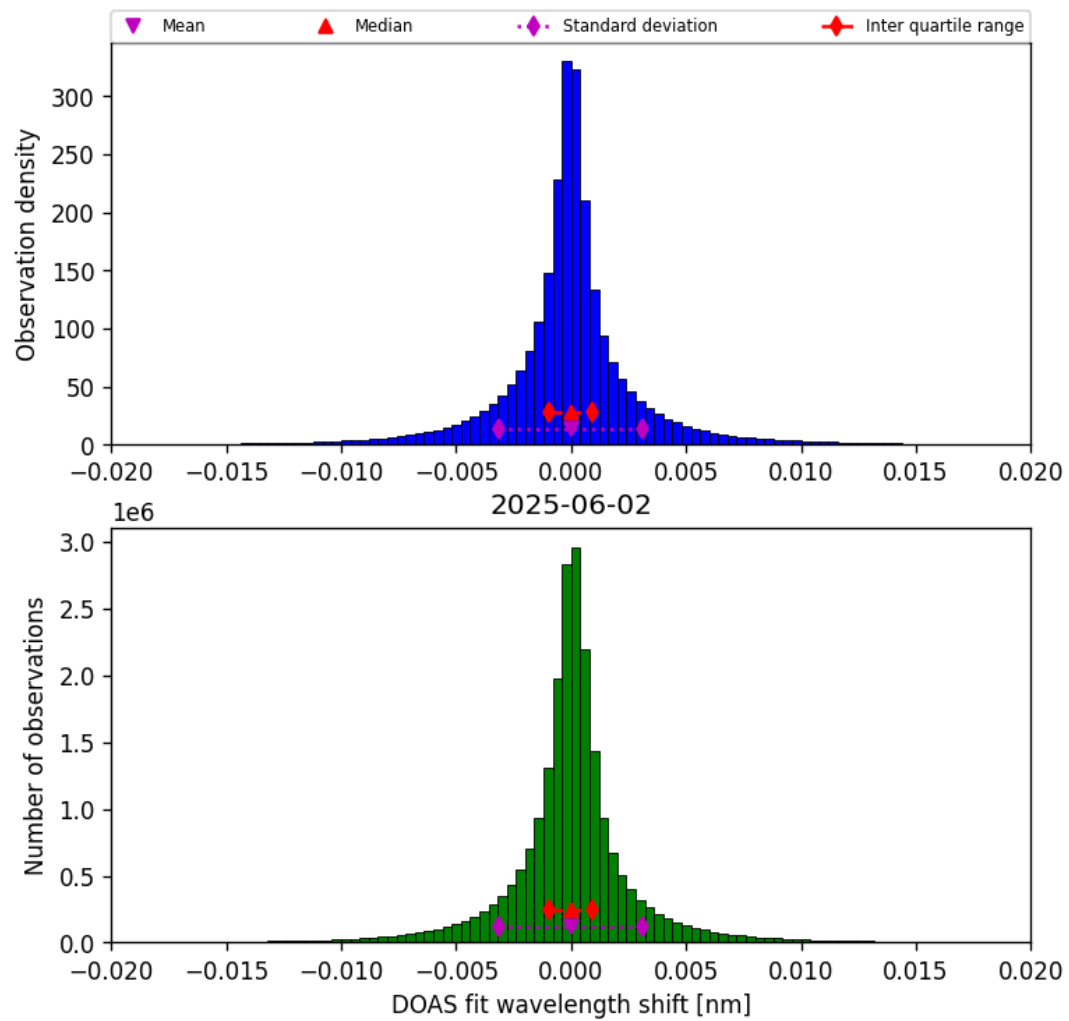
Figure 42: Histogram of “DOAS fit wavelength shift” for 2025-06-02 to 2025-06-03
