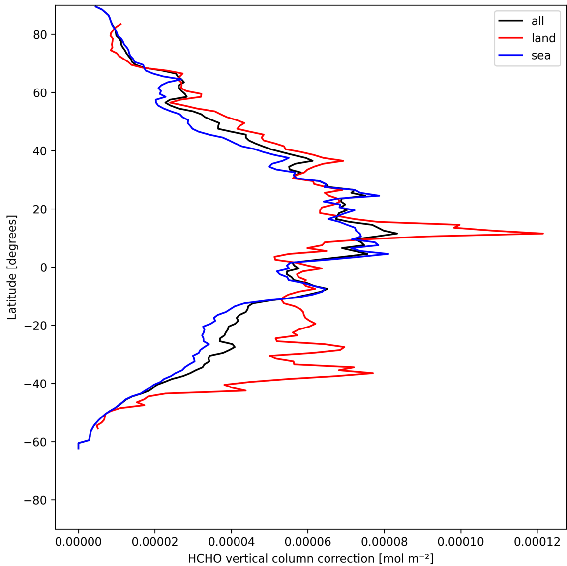
Figure 21: Zonal average of “HCHO vertical column correction” for 2025-06-02 to 2025-06-03.
