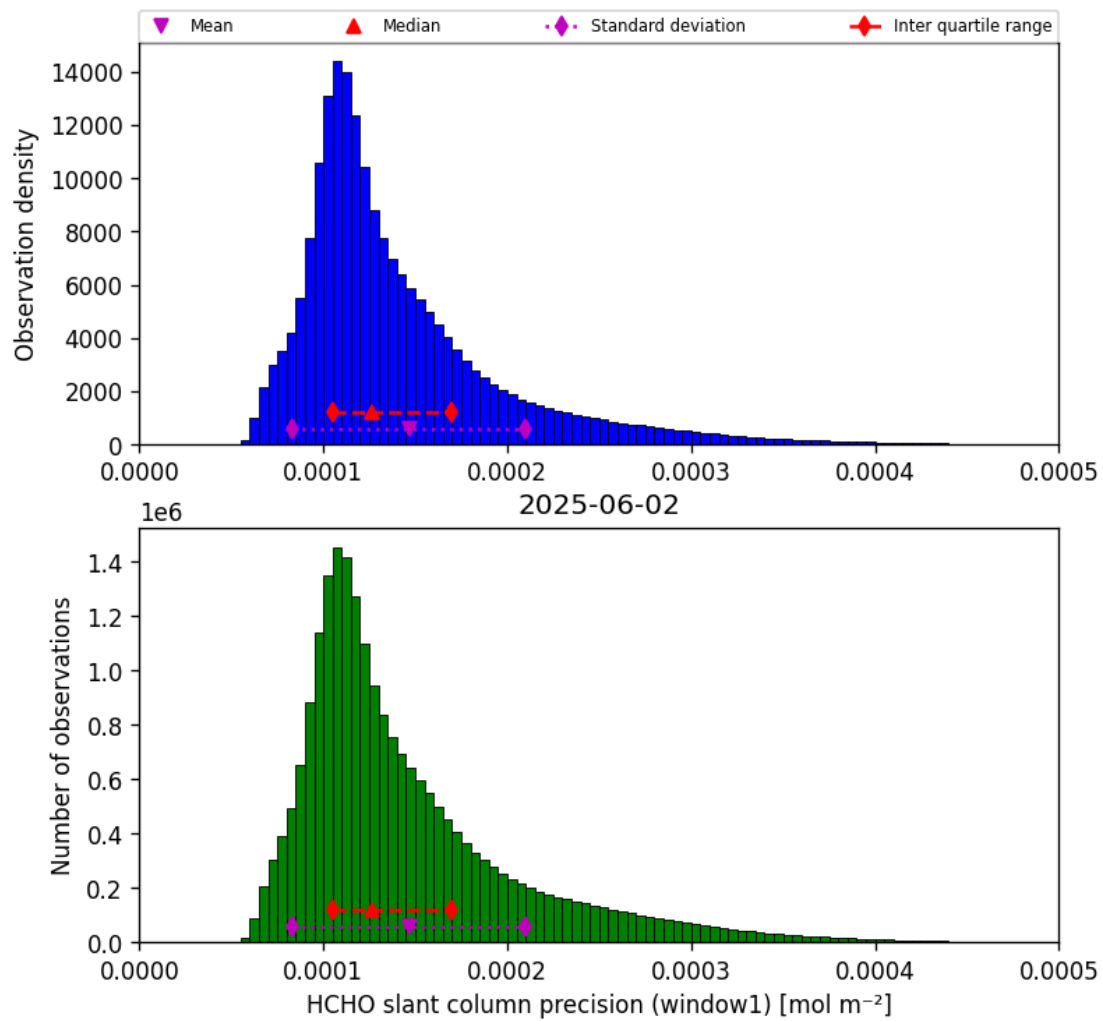
Figure 37: Histogram of “HCHO slant column precision (window1)” for 2025-06-02 to 2025-06-03
