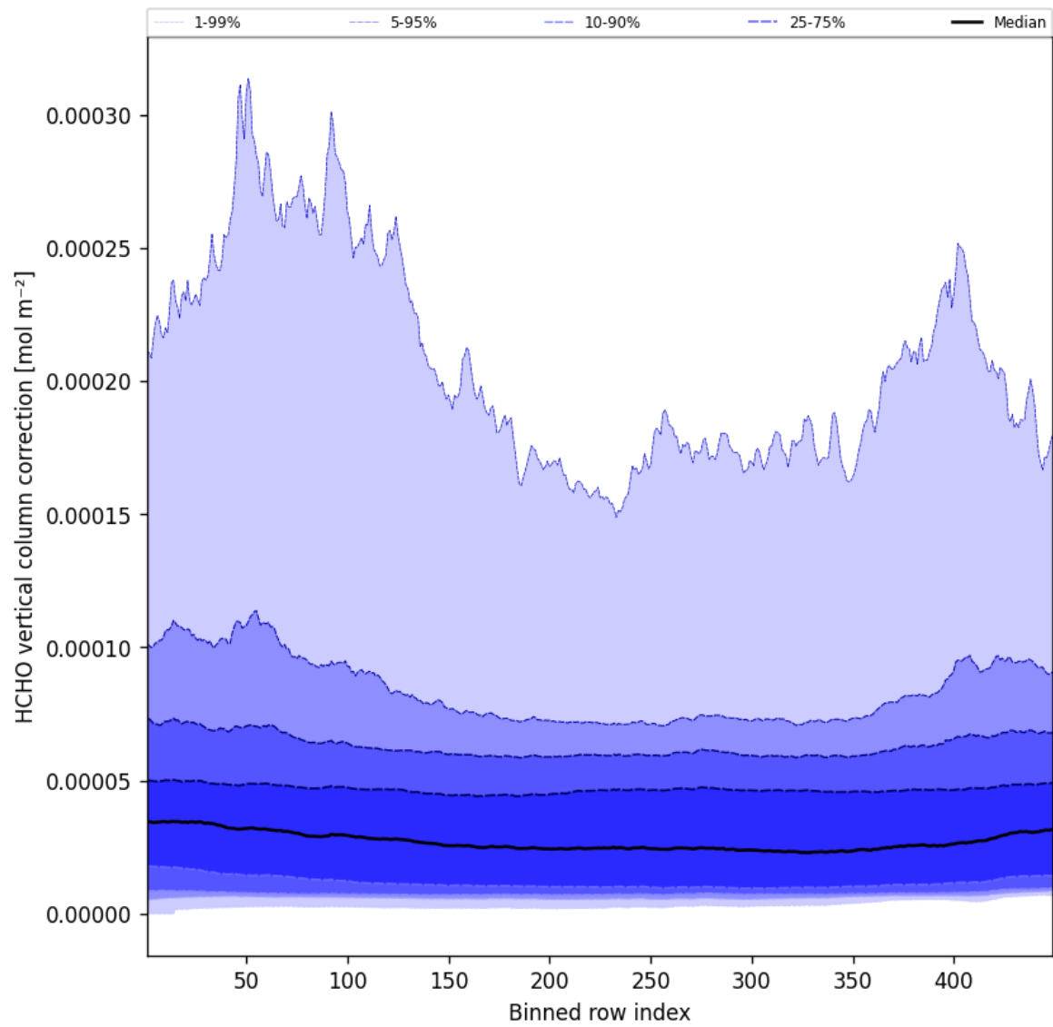
Figure 49: Along track statistics of “HCHO vertical column correction” for 2025-06-02 to 2025-06-03
