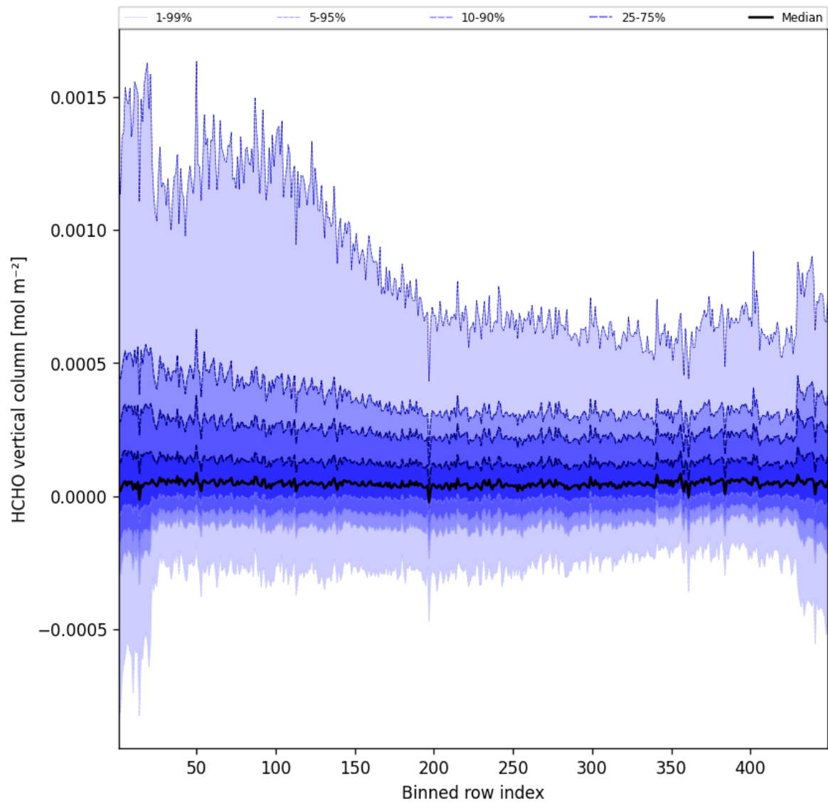
Figure 47: Along track statistics of “HCHO vertical column” for 2025-06-02 to 2025-06-03
