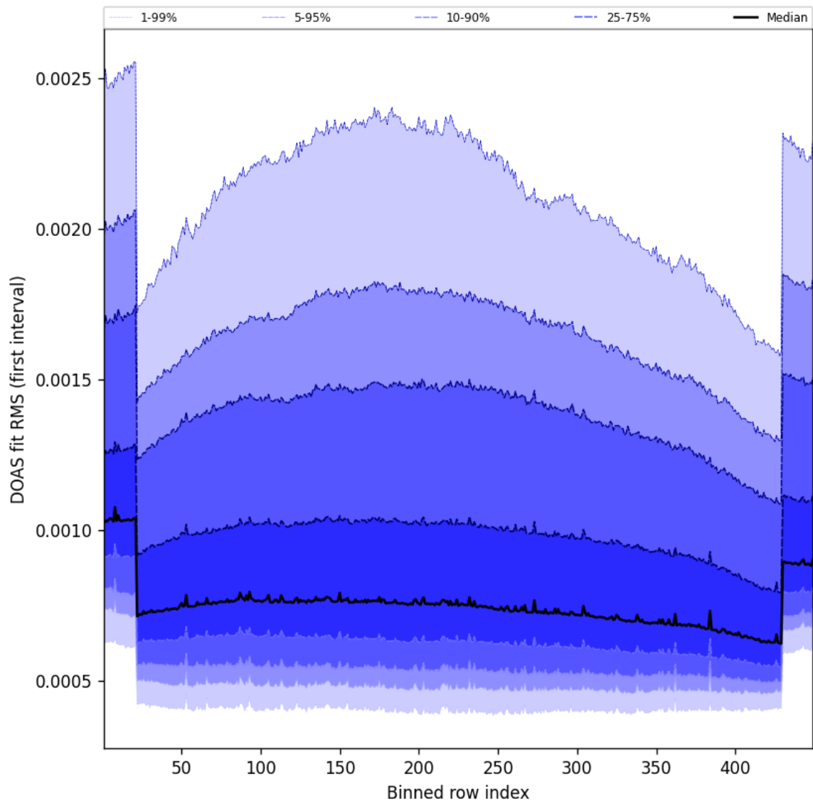
Figure 58: Along track statistics of “DOAS fit RMS (first interval)” for 2025-06-02 to 2025-06-03
