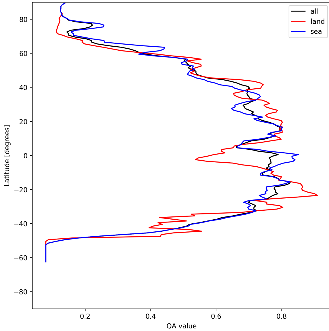
Figure 18: Zonal average of “QA value” for 2025-06-02 to 2025-06-03.
