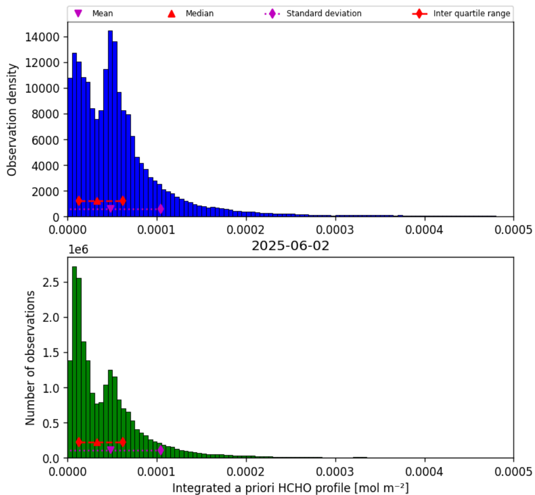
Figure 41: Histogram of “Integrated a priori HCHO profile” for 2025-06-02 to 2025-06-03
