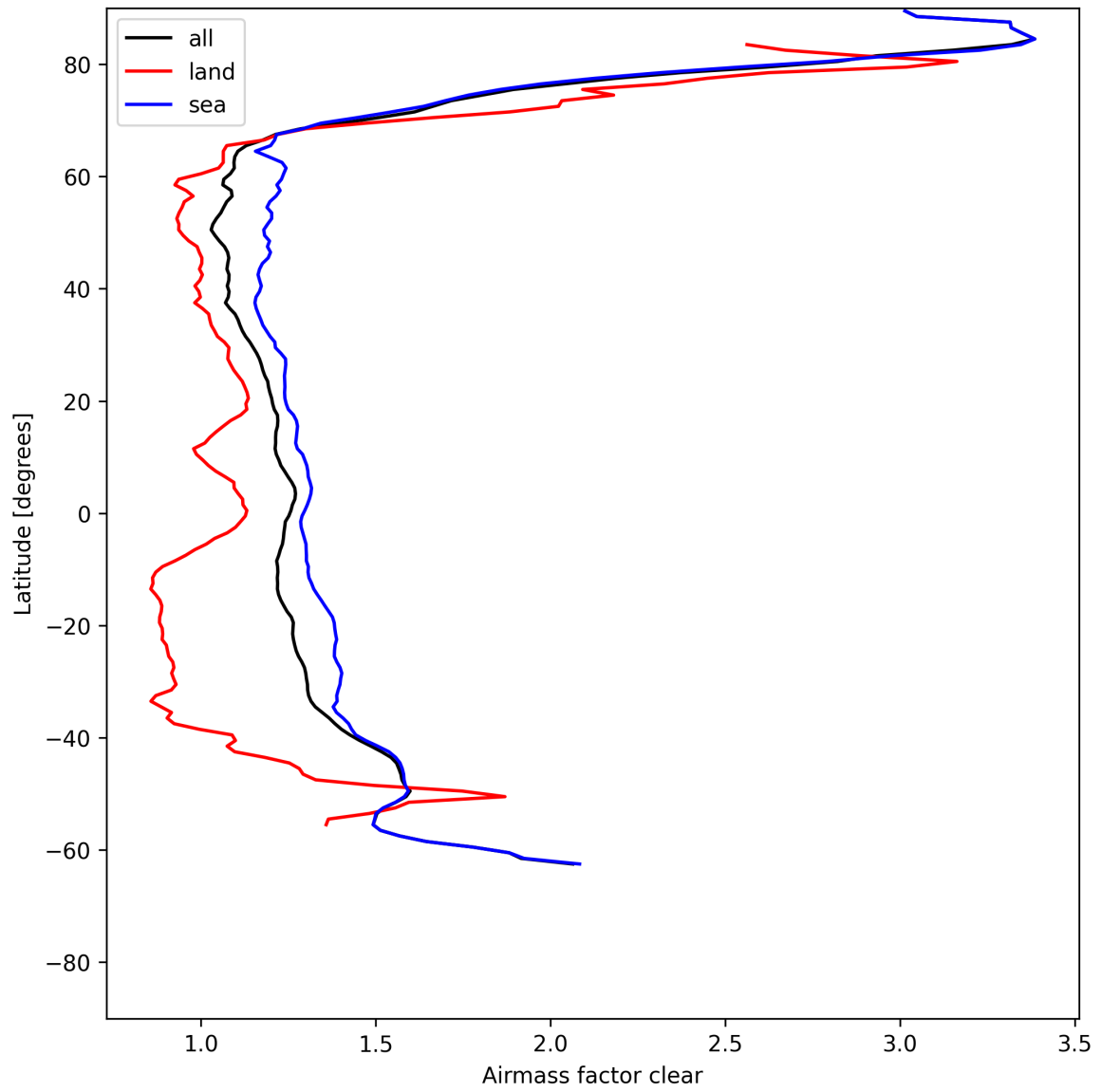
Figure 26: Zonal average of “Airmass factor clear” for 2025-06-02 to 2025-06-03.
