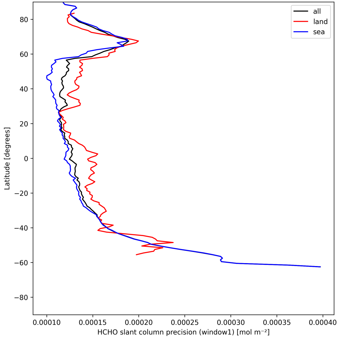
Figure 23: Zonal average of “HCHO slant column precision (window1)” for 2025-06-02 to 2025-06-03.
