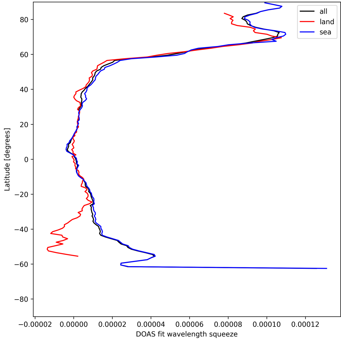
Figure 29: Zonal average of “DOAS fit wavelength squeeze” for 2025-06-02 to 2025-06-03.
