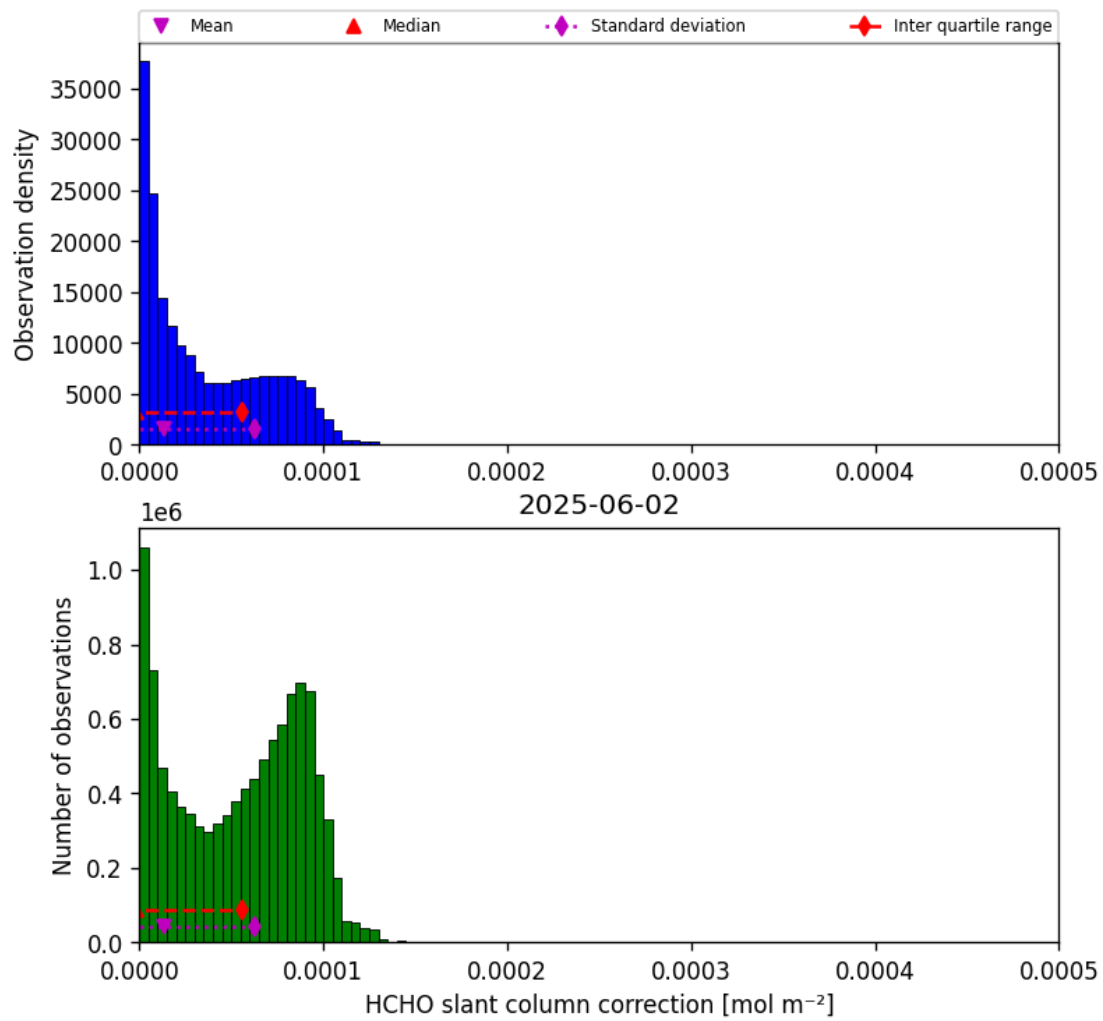
Figure 45: Histogram of “HCHO slant column correction” for 2025-06-02 to 2025-06-03
