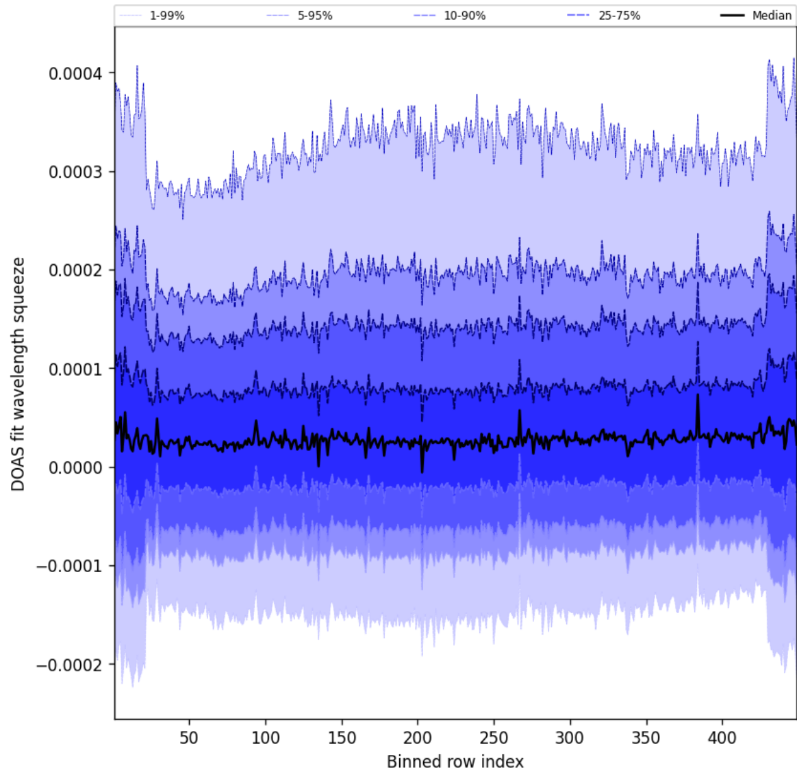
Figure 57: Along track statistics of “DOAS fit wavelength squeeze” for 2025-06-02 to 2025-06-03
