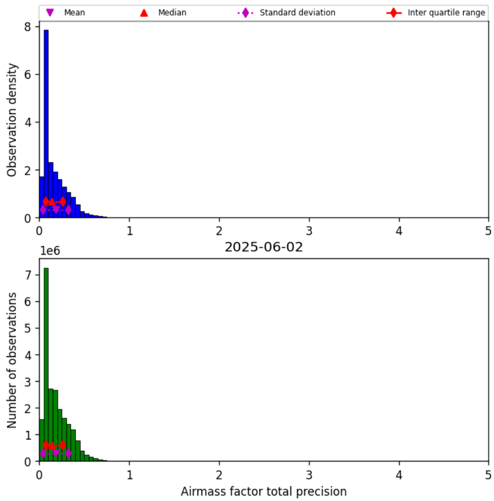
Figure 39: Histogram of “Airmass factor total precision” for 2025-06-02 to 2025-06-03
