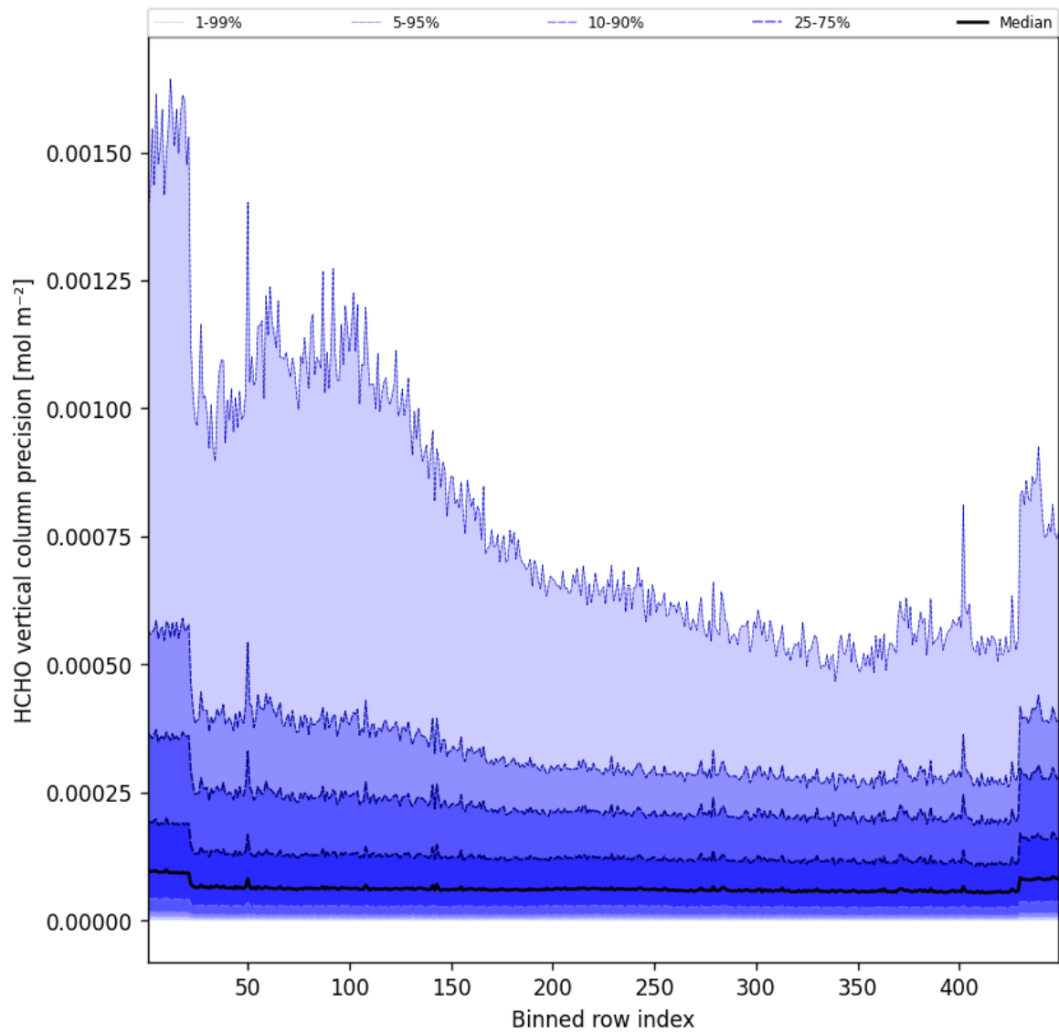
Figure 48: Along track statistics of “HCHO vertical column precision” for 2025-06-02 to 2025-06-03
