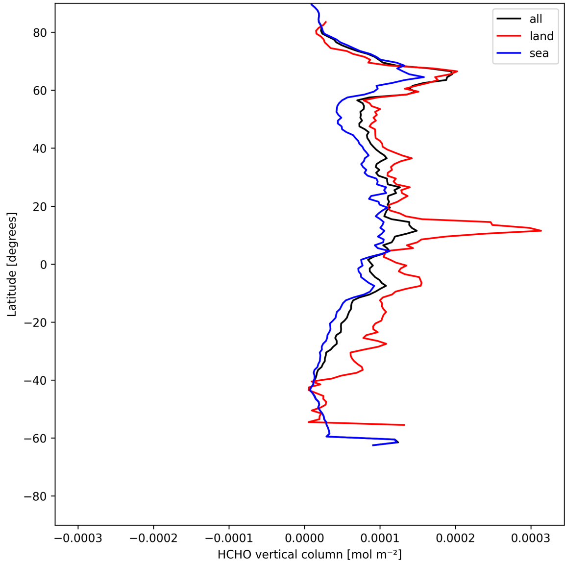
Figure 19: Zonal average of “HCHO vertical column” for 2025-06-02 to 2025-06-03.
