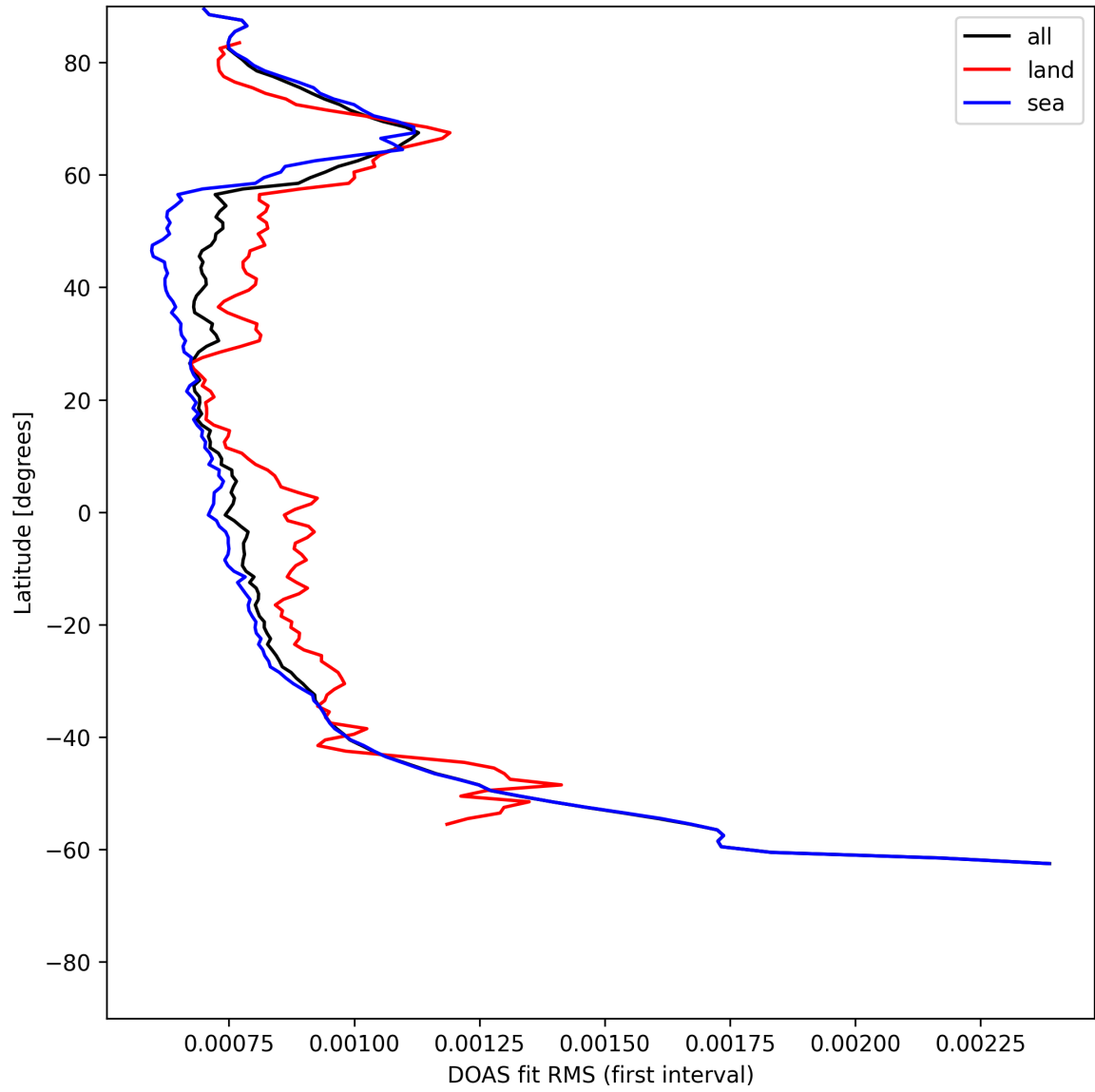
Figure 30: Zonal average of "DOAS fit RMS (first interval)" for 2025-06-02 to 2025-06-03.
