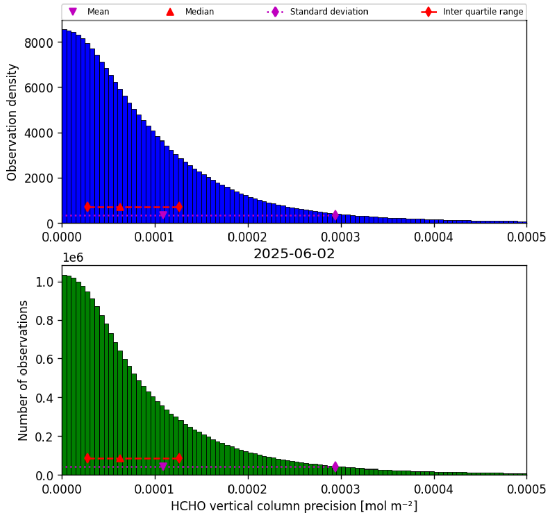
Figure 34: Histogram of “HCHO vertical column precision” for 2025-06-02 to 2025-06-03
