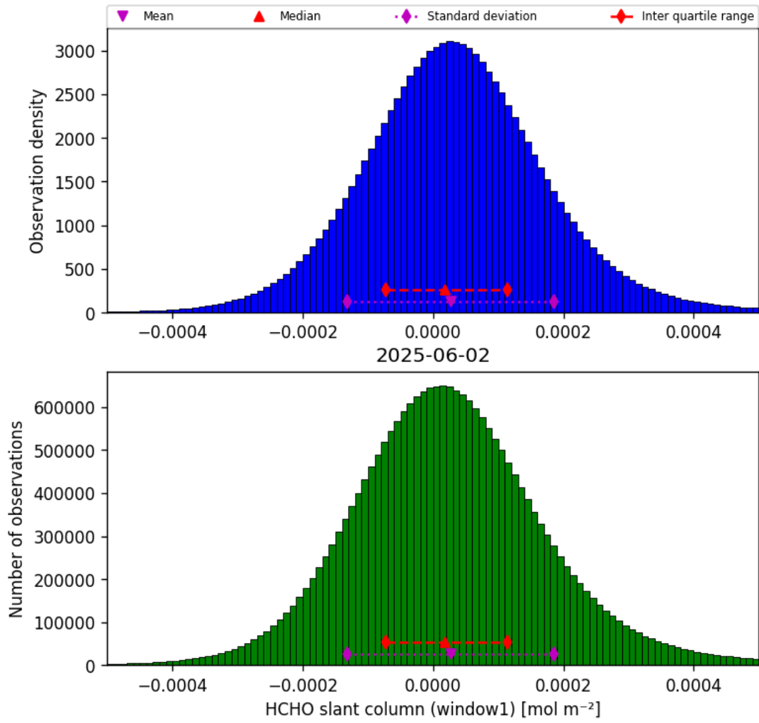
Figure 36: Histogram of “HCHO slant column (window1)” for 2025-06-02 to 2025-06-03
