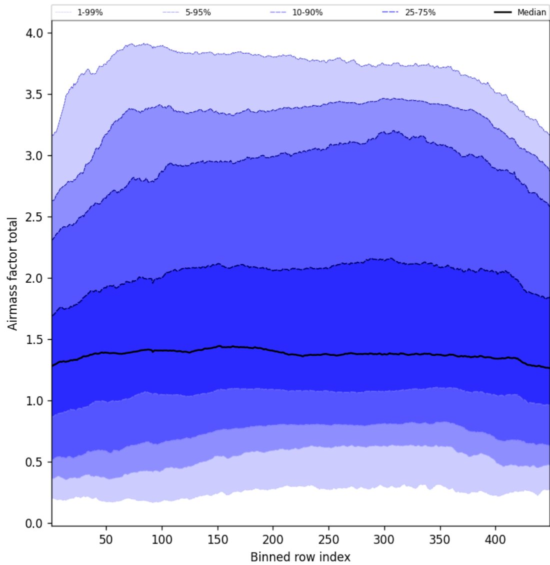
Figure 52: Along track statistics of “Airmass factor total” for 2025-06-02 to 2025-06-03
