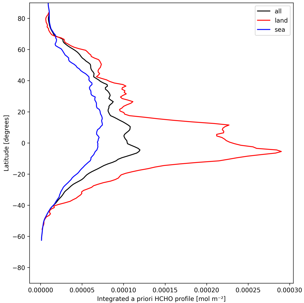
Figure 27: Zonal average of “Integrated a priori HCHO profile” for 2025-06-02 to 2025-06-03.
