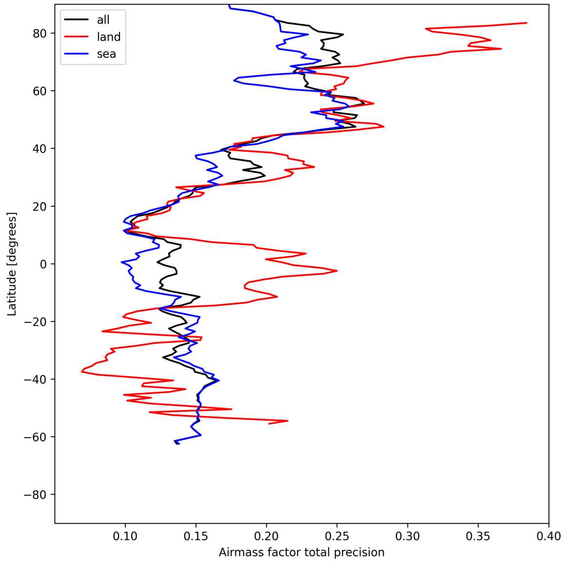
Figure 25: Zonal average of “Airmass factor total precision” for 2025-06-02 to 2025-06-03.
