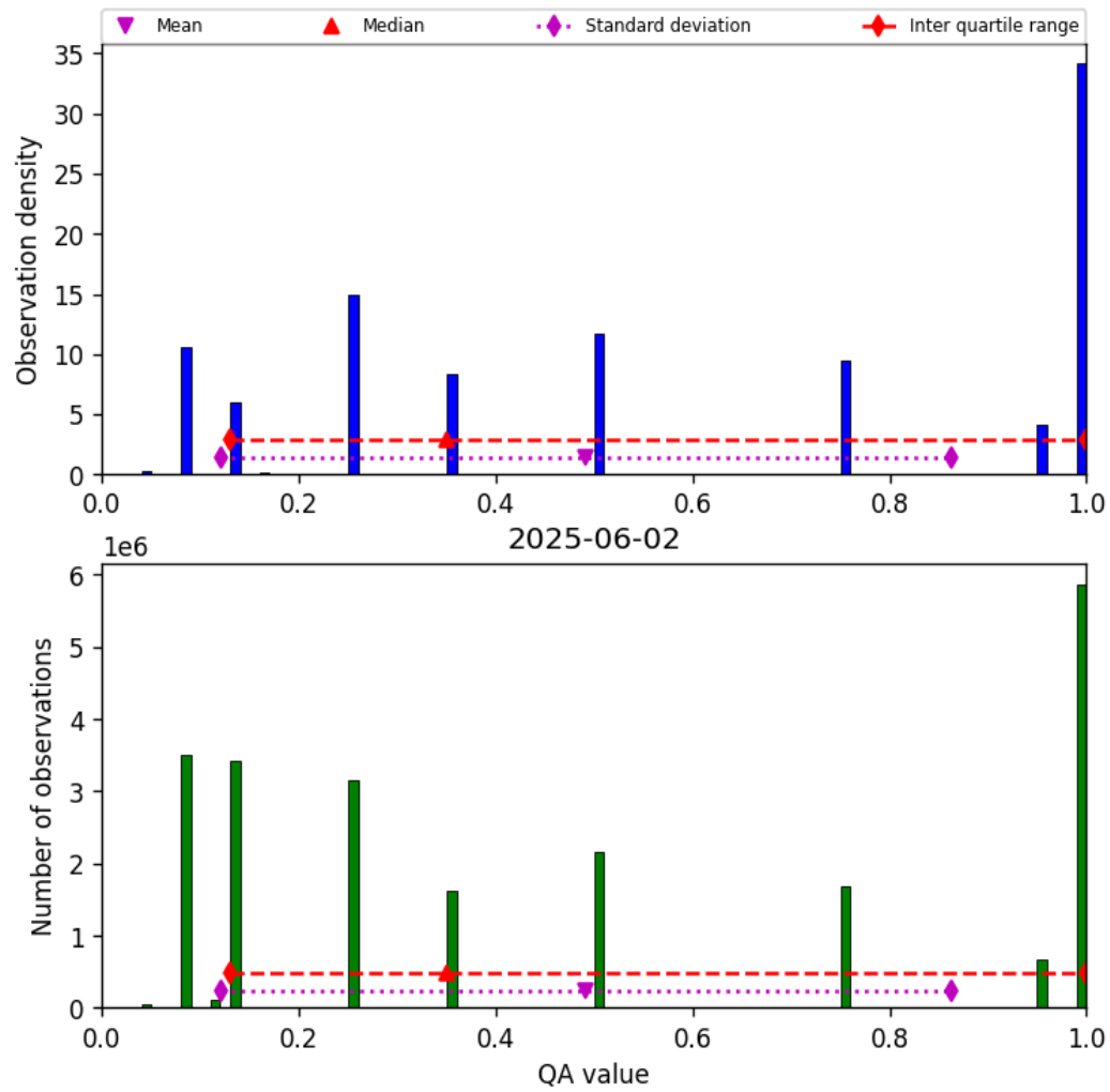
Figure 32: Histogram of “QA value” for 2025-06-02 to 2025-06-03
