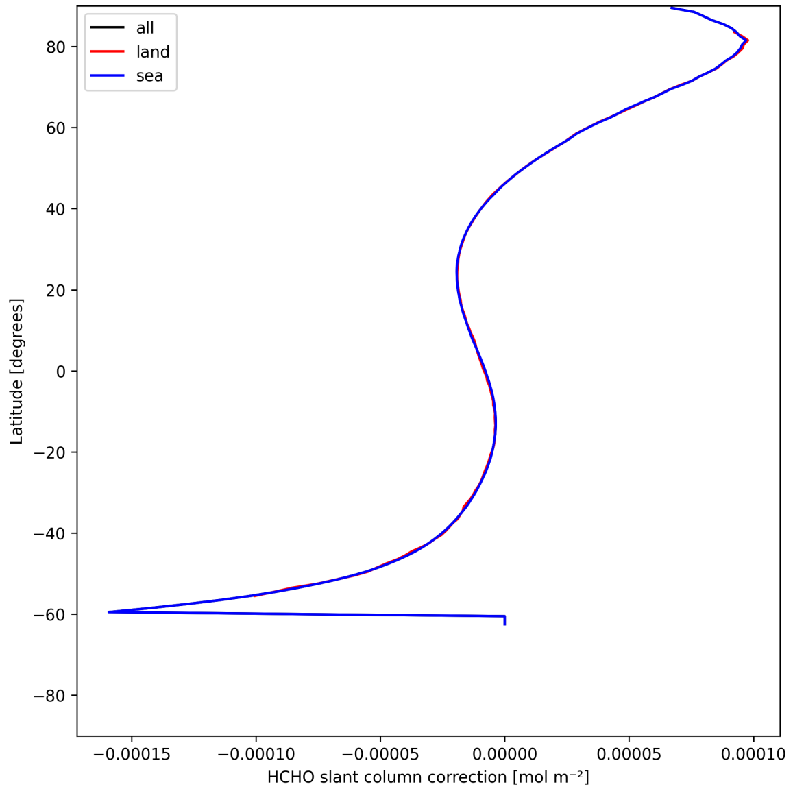
Figure 31: Zonal average of “HCHO slant column correction” for 2025-06-02 to 2025-06-03.
