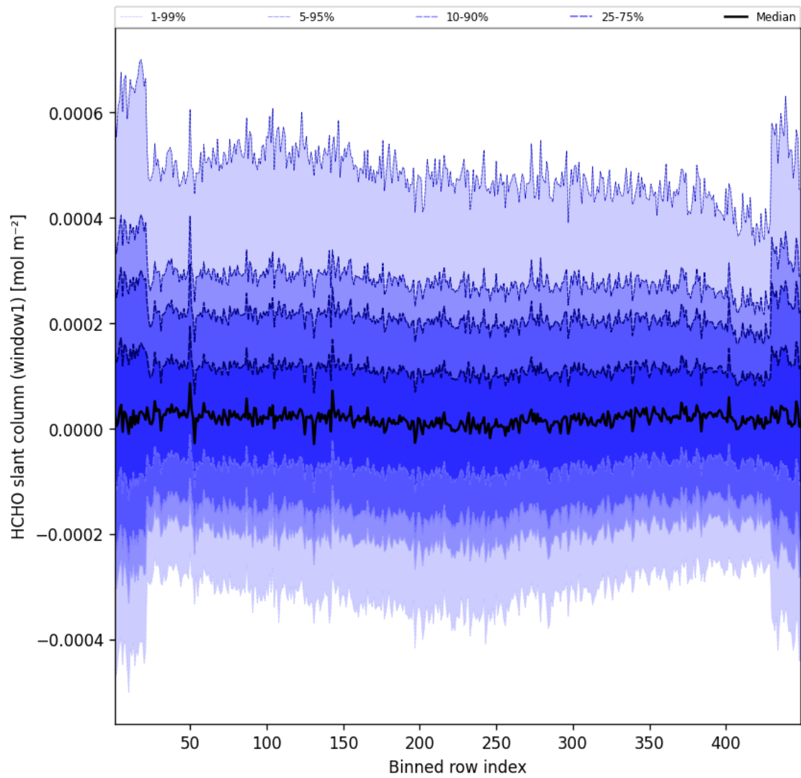
Figure 50: Along track statistics of “HCHO slant column (window1)” for 2025-06-02 to 2025-06-03
