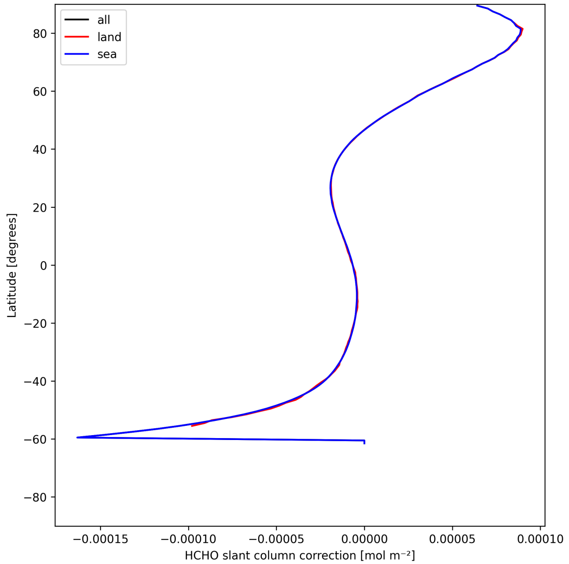
Figure 31: Zonal average of “HCHO slant column correction” for 2025-06-03 to 2025-06-04.
