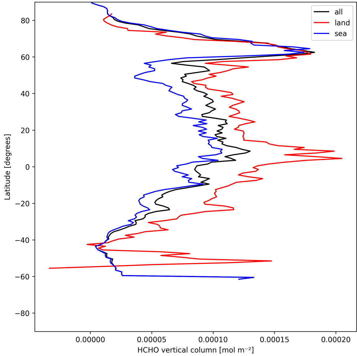
Figure 19: Zonal average of “HCHO vertical column” for 2025-06-03 to 2025-06-04.
