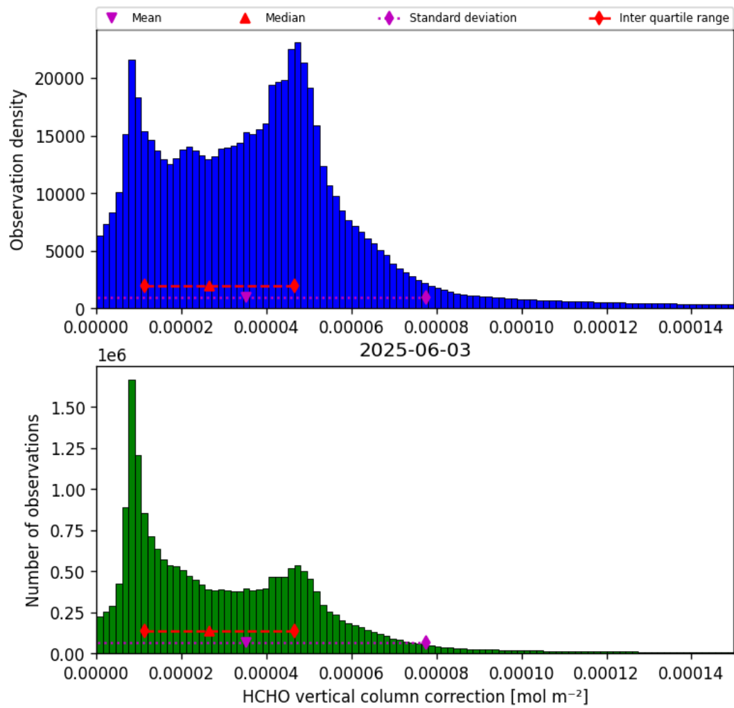
Figure 35: Histogram of “HCHO vertical column correction” for 2025-06-03 to 2025-06-04
