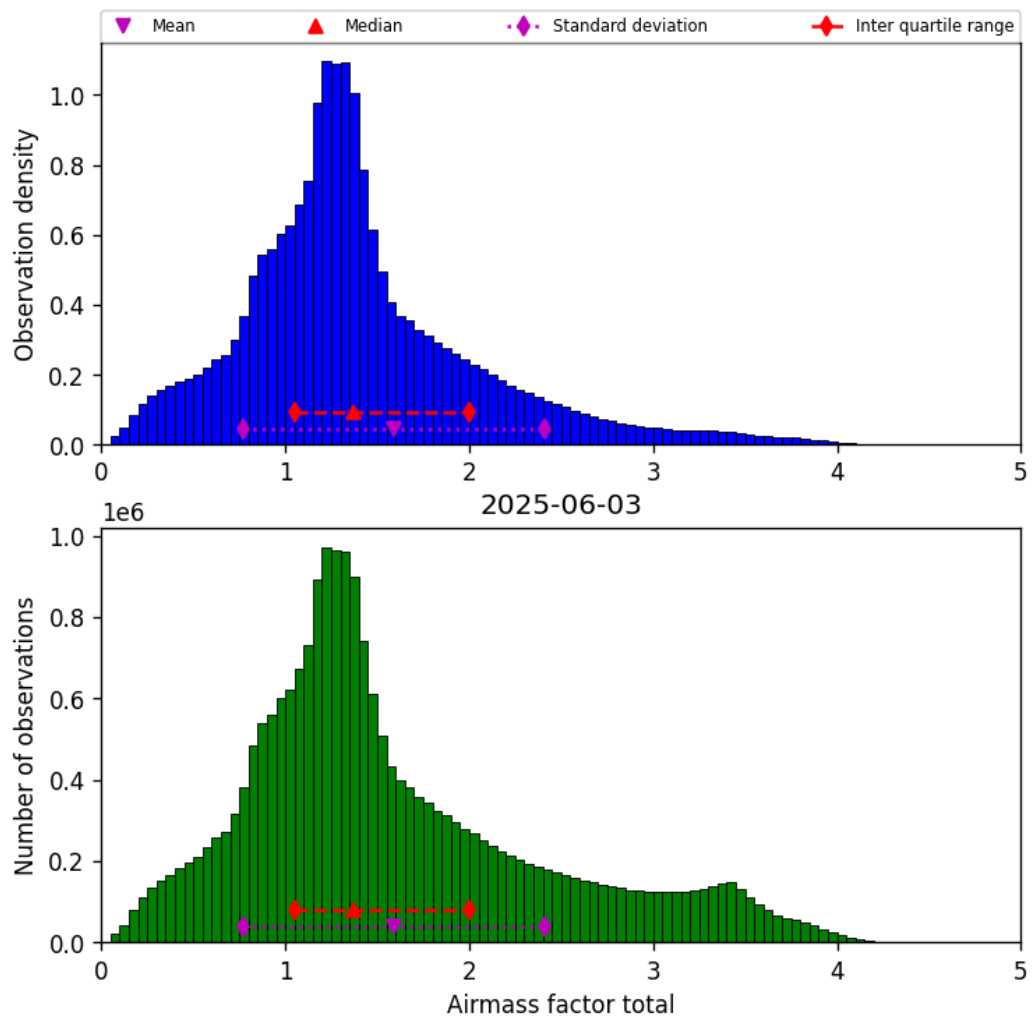
Figure 38: Histogram of “Airmass factor total” for 2025-06-03 to 2025-06-04
