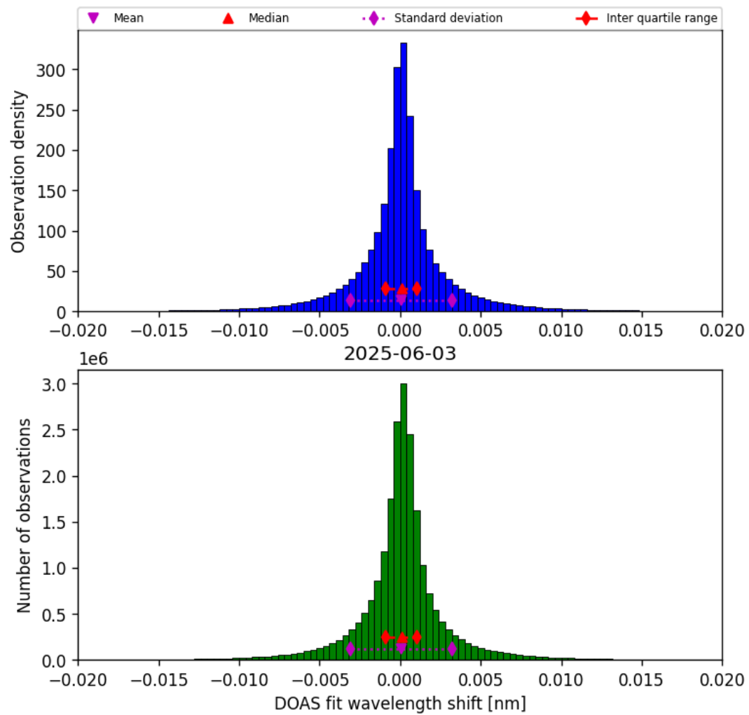
Figure 42: Histogram of “DOAS fit wavelength shift” for 2025-06-03 to 2025-06-04
