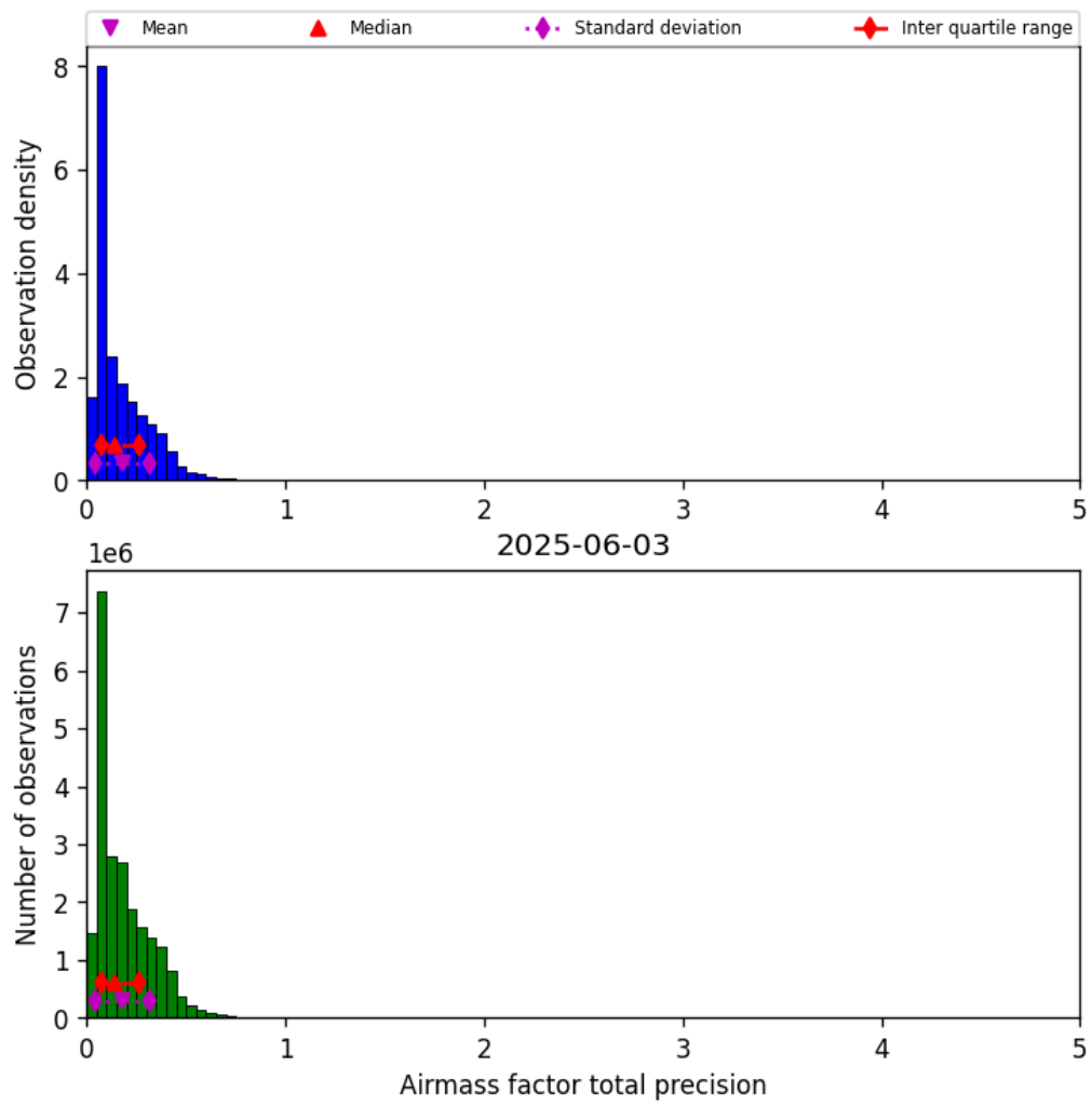
Figure 39: Histogram of “Airmass factor total precision” for 2025-06-03 to 2025-06-04
