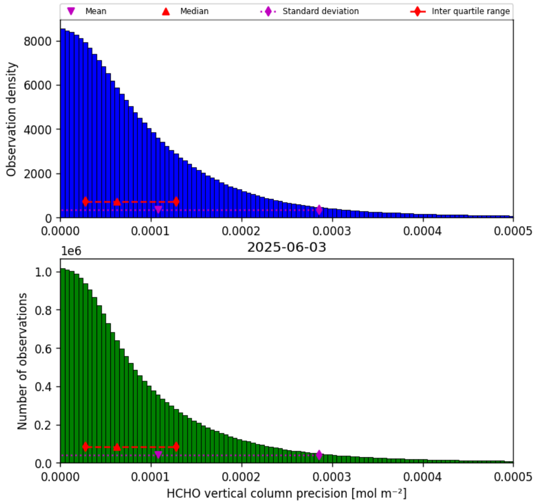
Figure 34: Histogram of “HCHO vertical column precision” for 2025-06-03 to 2025-06-04
