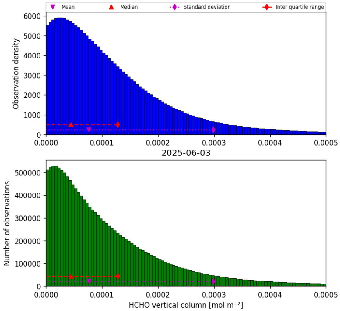
Figure 33: Histogram of “HCHO vertical column” for 2025-06-03 to 2025-06-04
