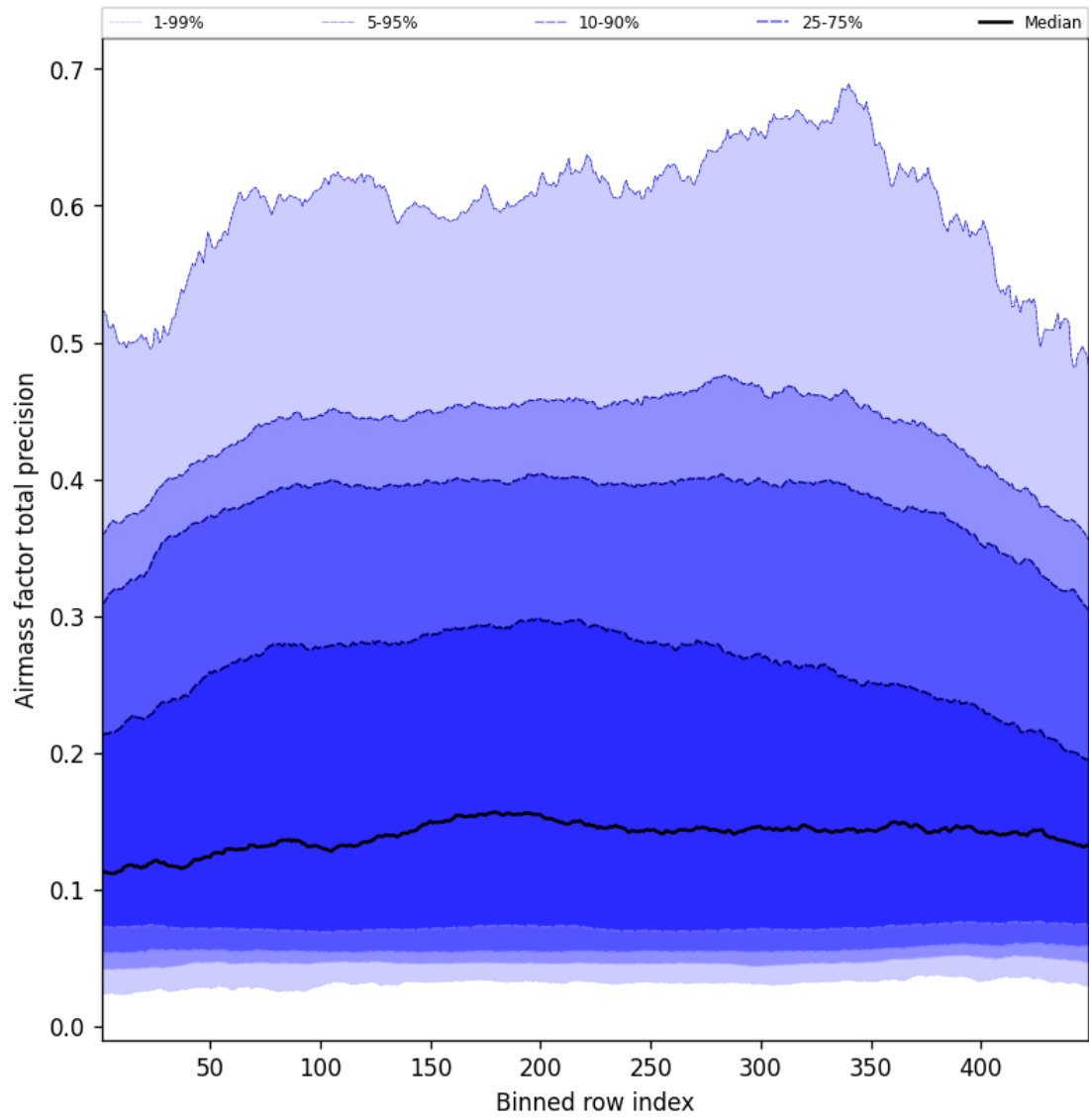
Figure 53: Along track statistics of “Airmass factor total precision” for 2025-06-03 to 2025-06-04
