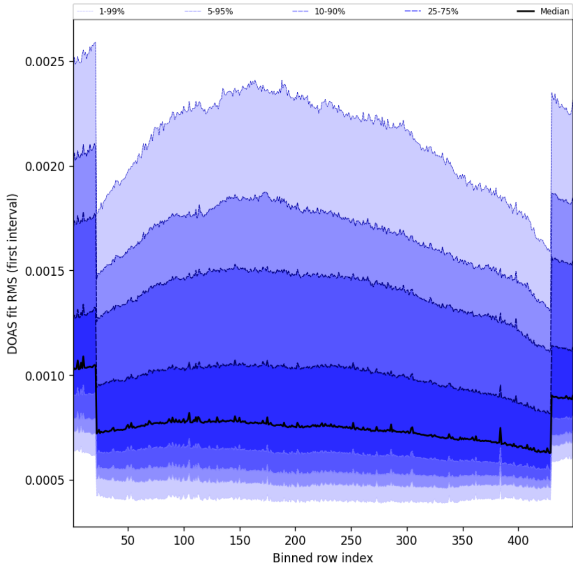
Figure 58: Along track statistics of “DOAS fit RMS (first interval)” for 2025-06-03 to 2025-06-04
