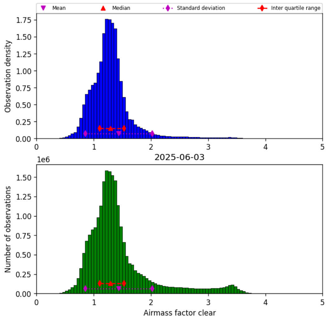
Figure 40: Histogram of “Airmass factor clear” for 2025-06-03 to 2025-06-04
