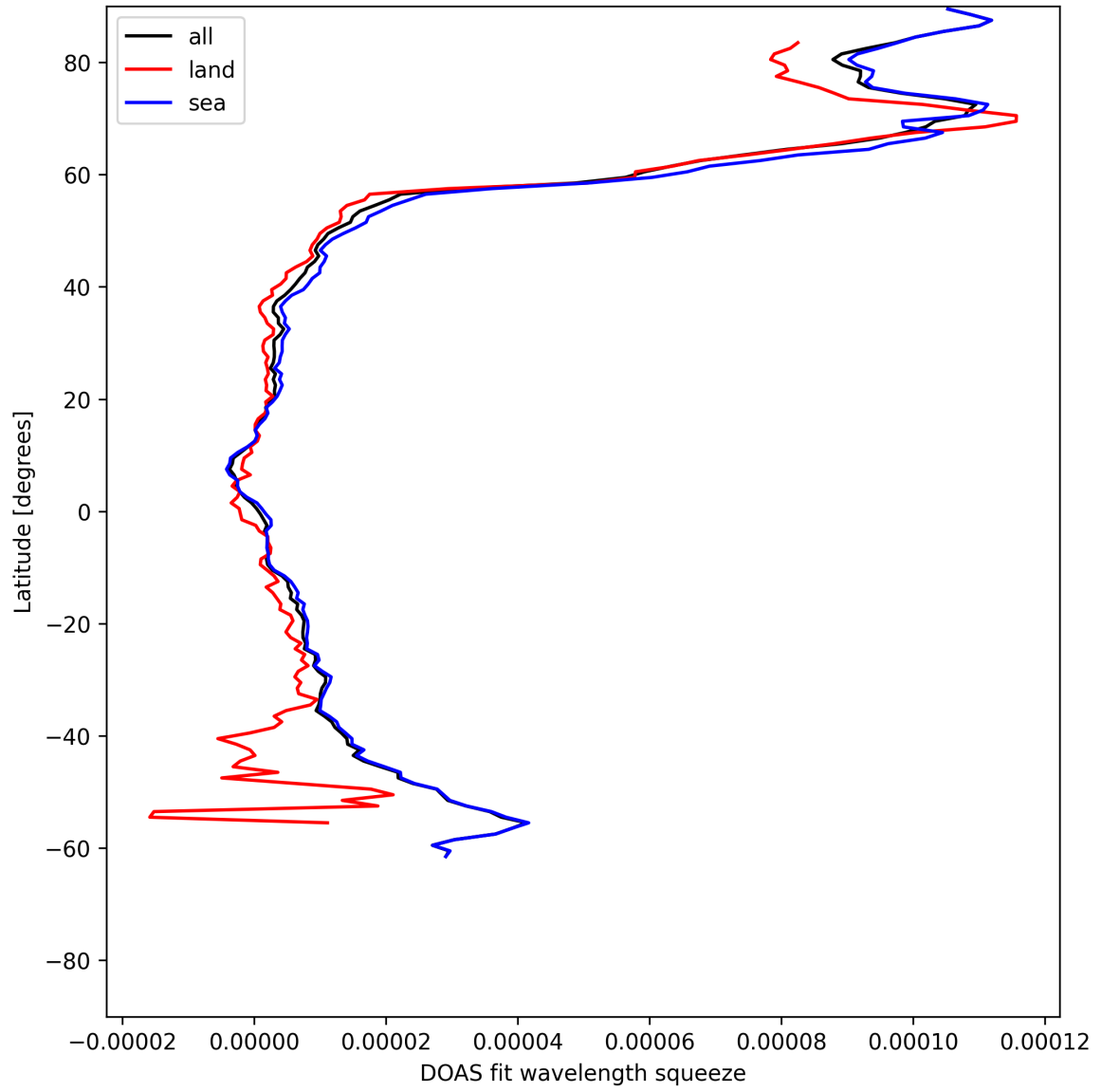
Figure 29: Zonal average of “DOAS fit wavelength squeeze” for 2025-06-03 to 2025-06-04.
