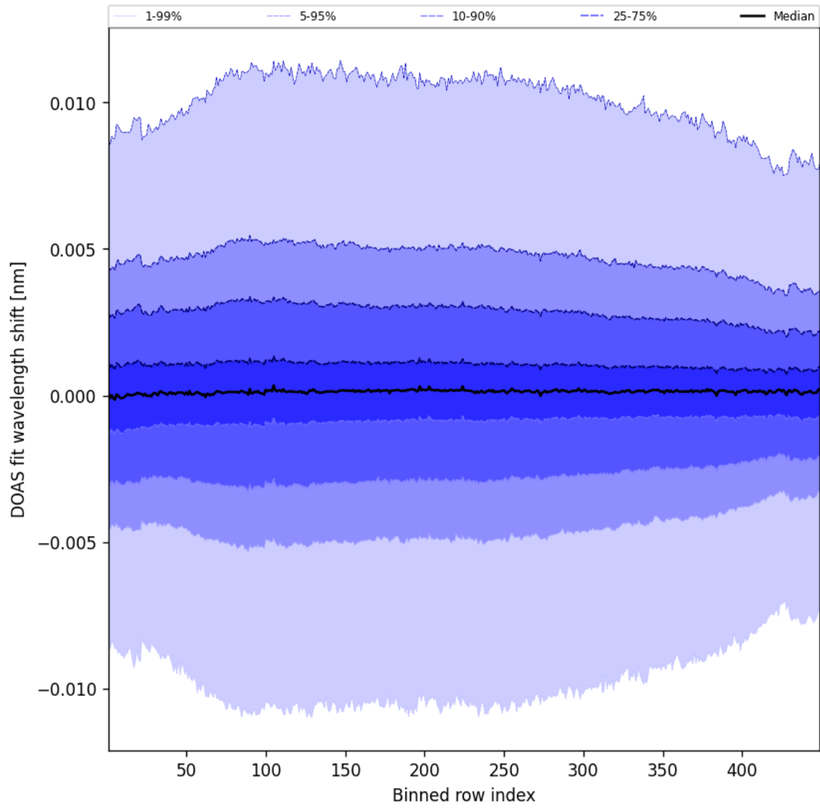
Figure 56: Along track statistics of “DOAS fit wavelength shift” for 2025-06-03 to 2025-06-04
