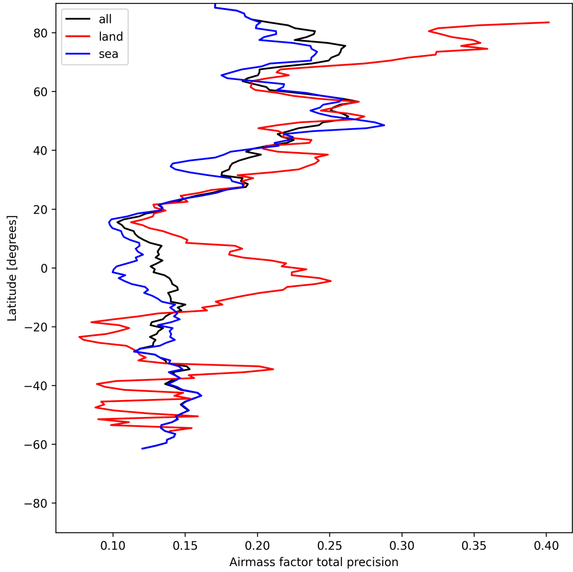
Figure 25: Zonal average of “Airmass factor total precision” for 2025-06-03 to 2025-06-04.
