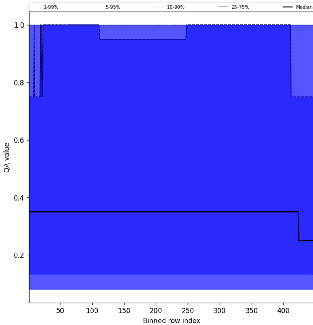
Figure 46: Along track statistics of "QA value" for 2025-06-03 to 2025-06-04
