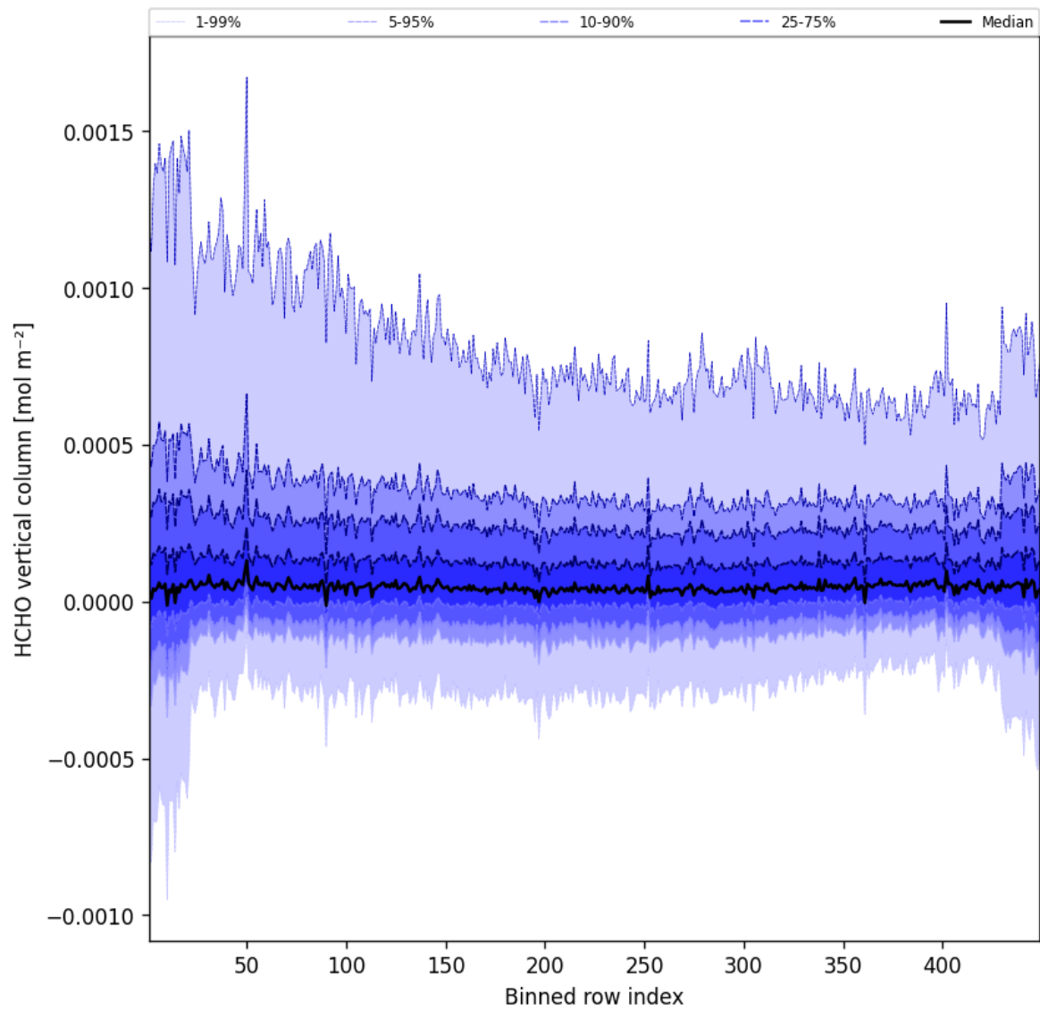
Figure 47: Along track statistics of “HCHO vertical column” for 2025-06-03 to 2025-06-04
