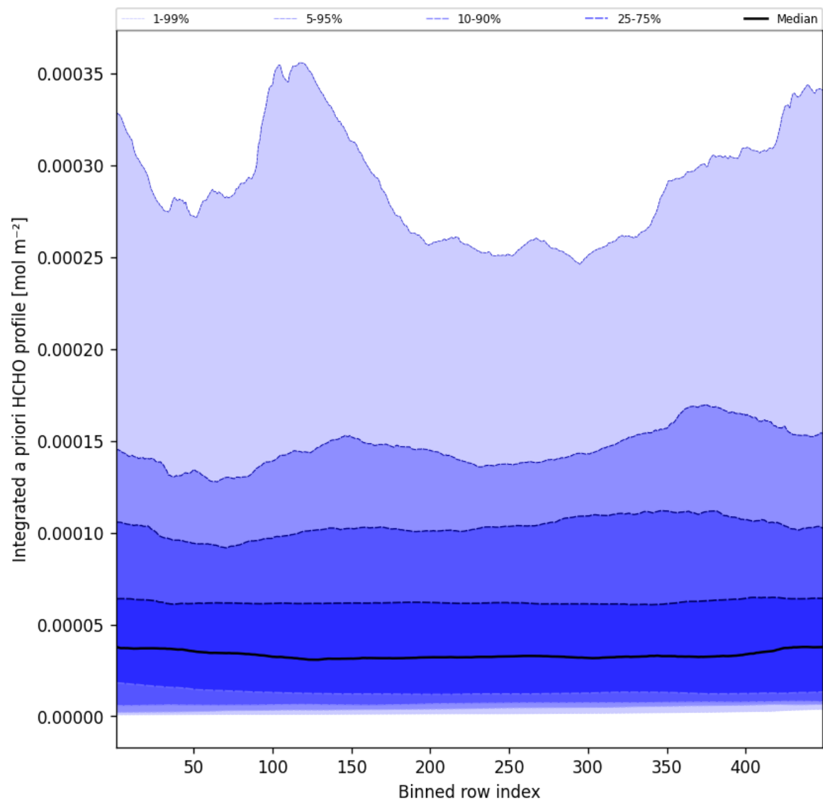
Figure 55: Along track statistics of “Integrated a priori HCHO profile” for 2025-06-03 to 2025-06-04
