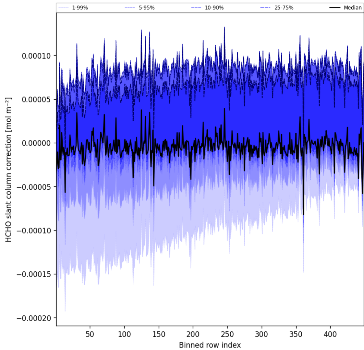
Figure 59: Along track statistics of “HCHO slant column correction” for 2025-06-03 to 2025-06-04
