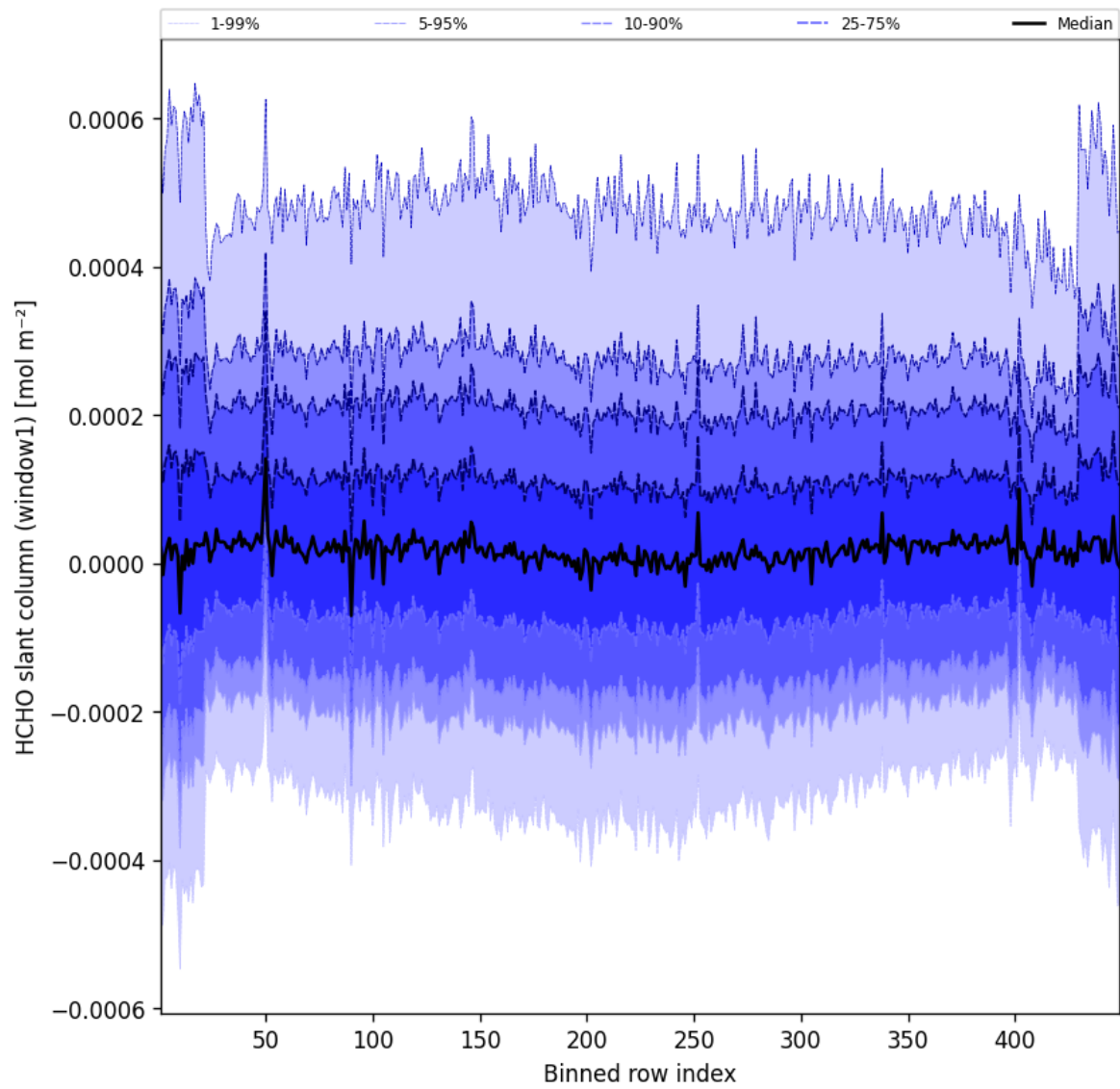
Figure 50: Along track statistics of “HCHO slant column (window1)” for 2025-06-03 to 2025-06-04
