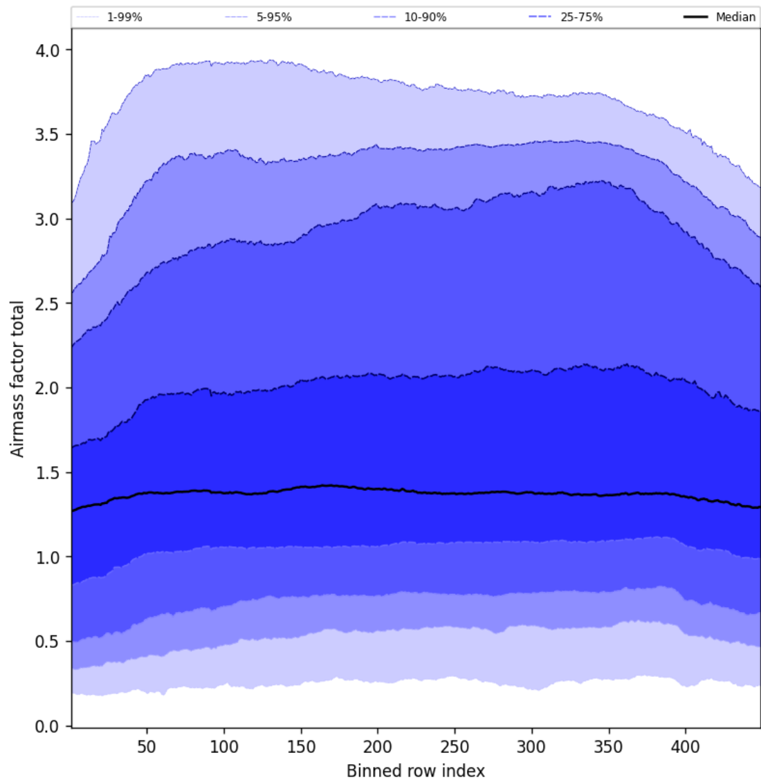
Figure 52: Along track statistics of “Airmass factor total” for 2025-06-03 to 2025-06-04
