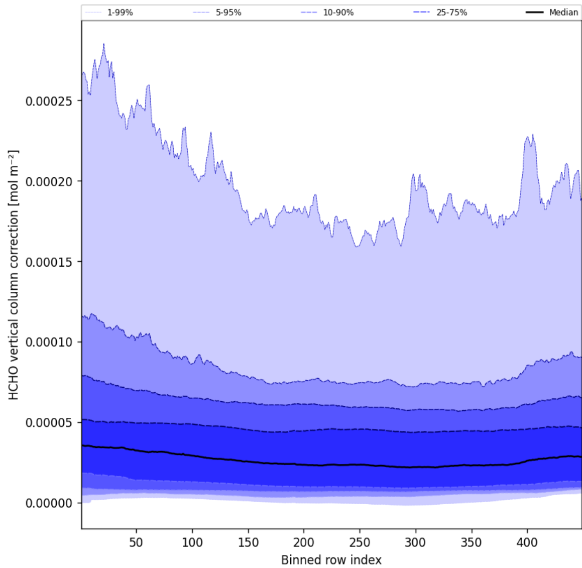
Figure 49: Along track statistics of “HCHO vertical column correction” for 2025-06-03 to 2025-06-04
