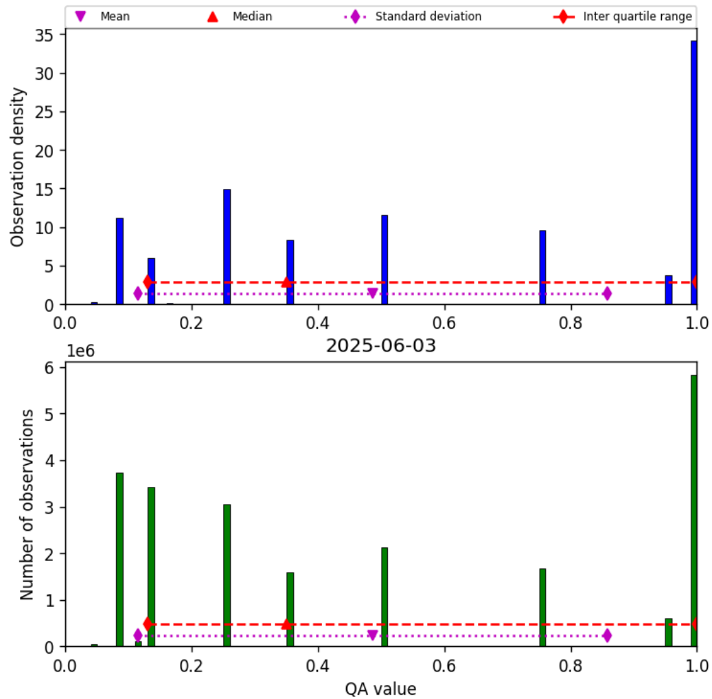
Figure 32: Histogram of “QA value” for 2025-06-03 to 2025-06-04
