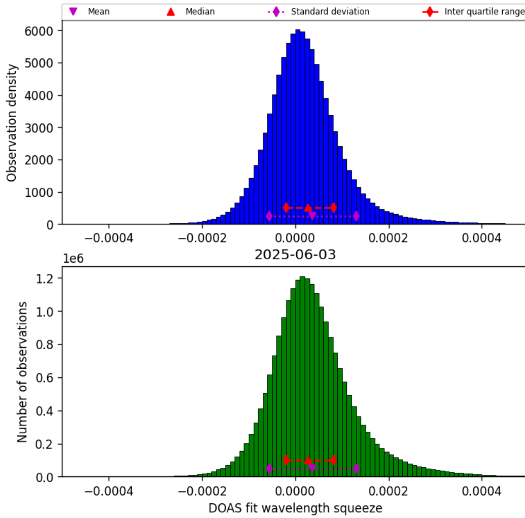
Figure 43: Histogram of “DOAS fit wavelength squeeze” for 2025-06-03 to 2025-06-04
