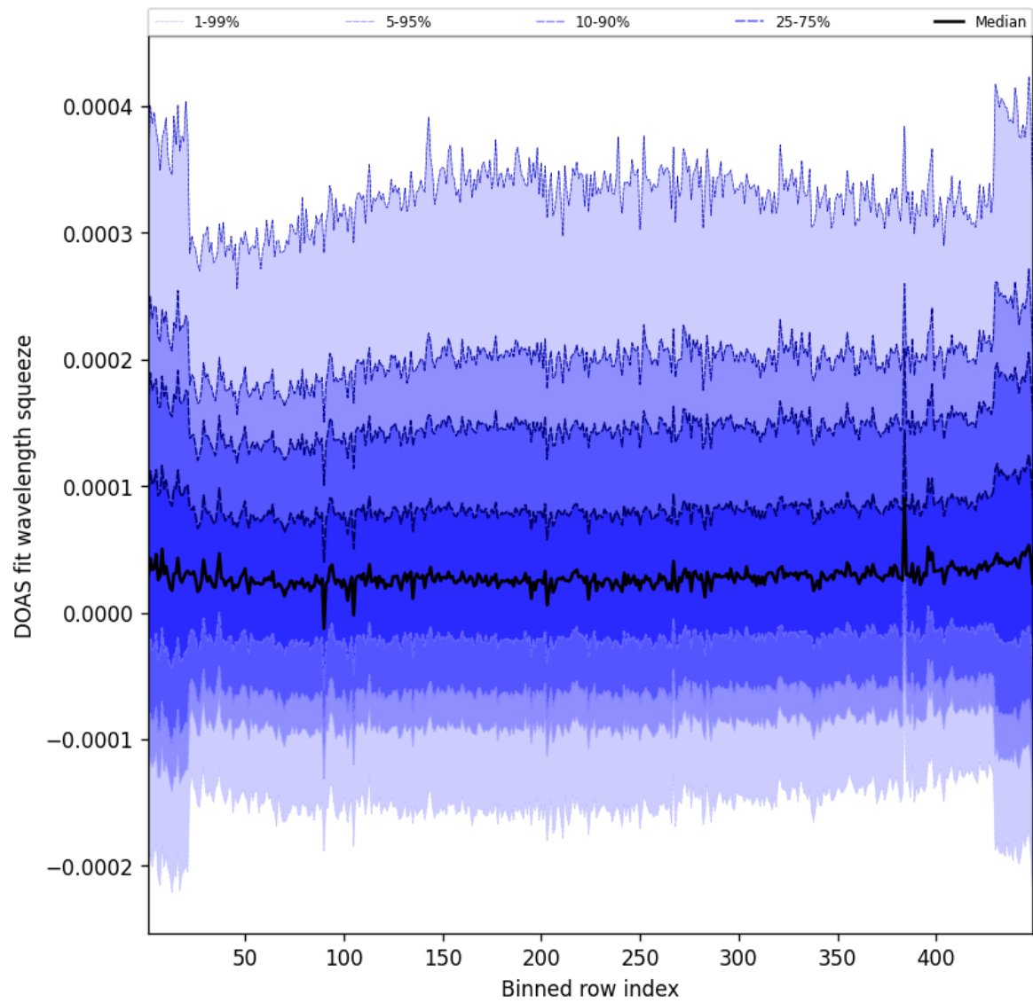
Figure 57: Along track statistics of “DOAS fit wavelength squeeze” for 2025-06-03 to 2025-06-04
