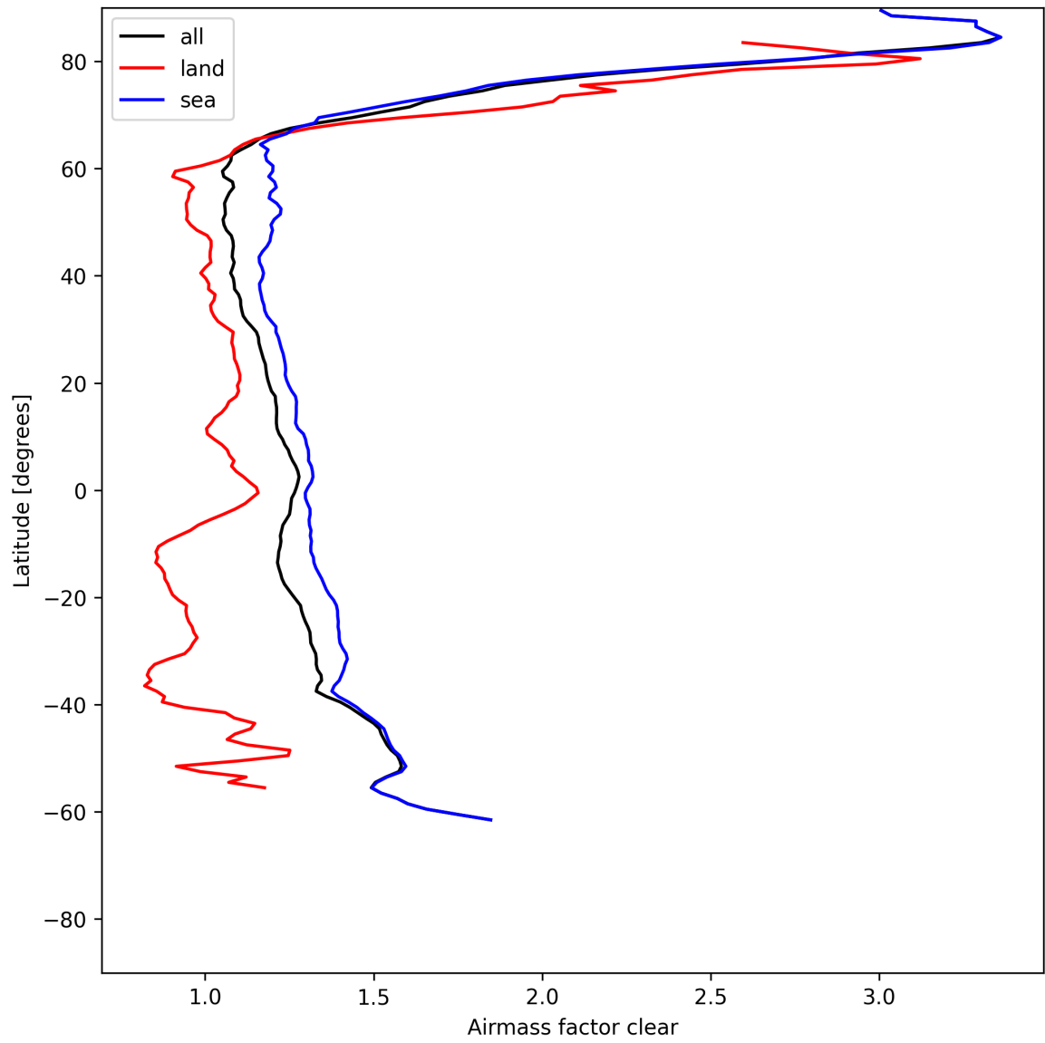
Figure 26: Zonal average of “Airmass factor clear” for 2025-06-03 to 2025-06-04.
