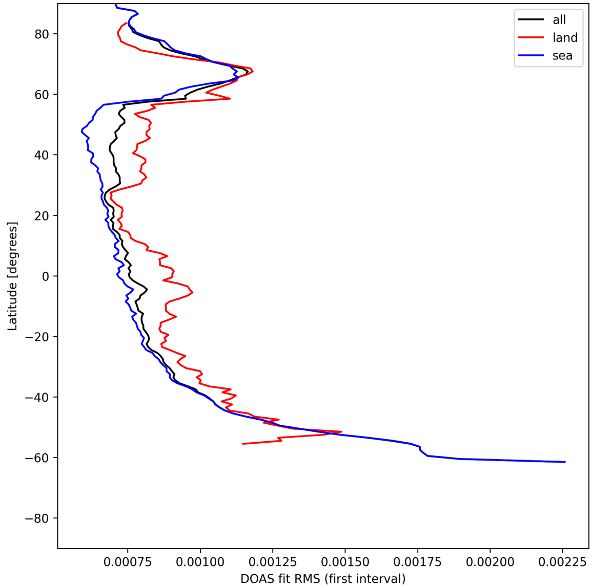
Figure 30: Zonal average of "DOAS fit RMS (first interval)" for 2025-06-03 to 2025-06-04.
