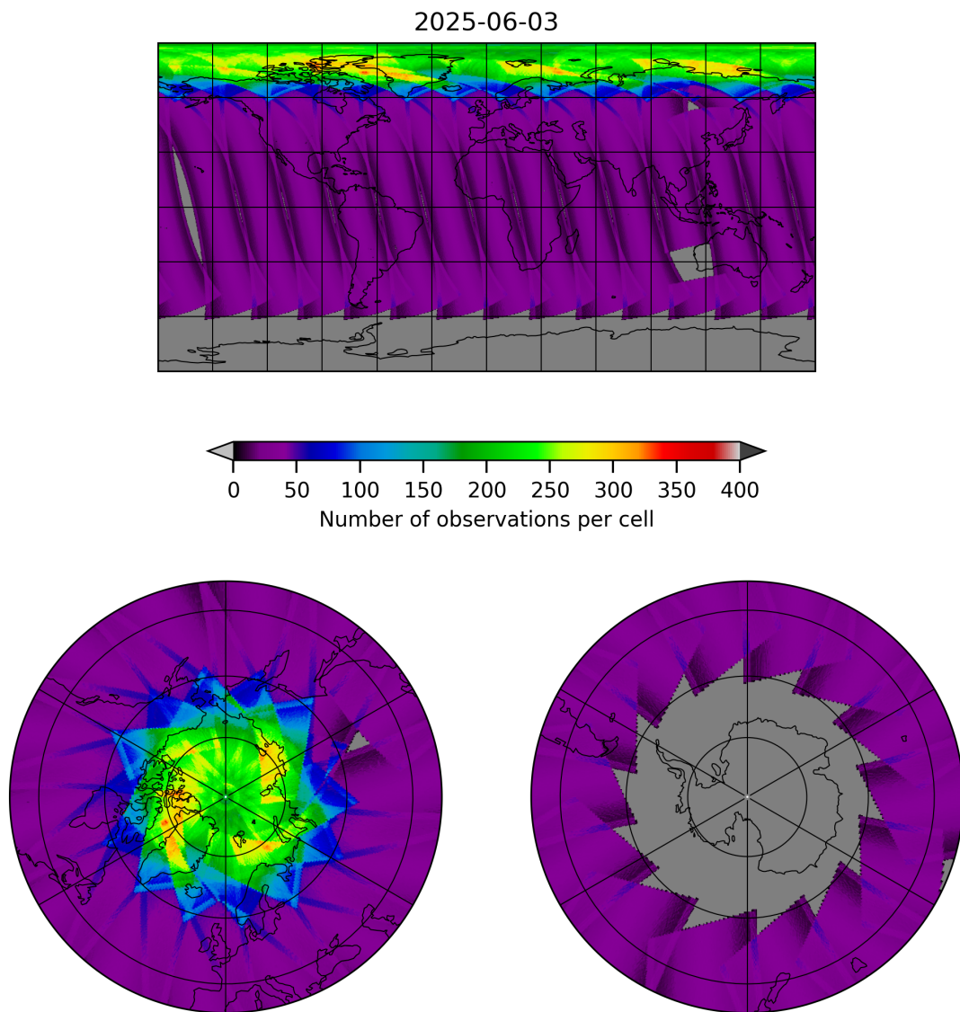
Figure 17: Map of the number of observations for 2025-06-03 to 2025-06-04
