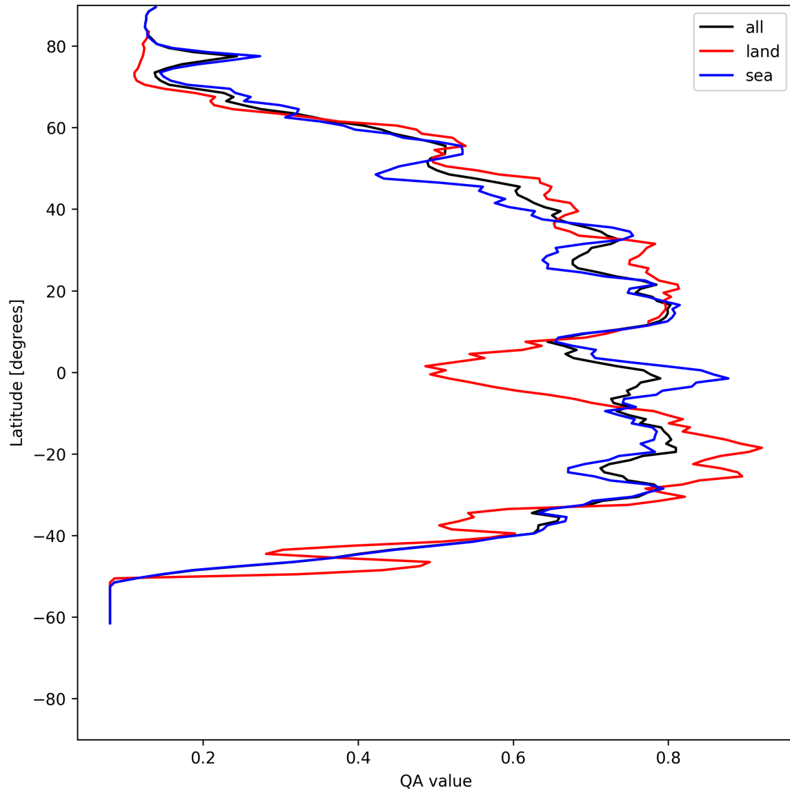
Figure 18: Zonal average of “QA value” for 2025-06-03 to 2025-06-04.
