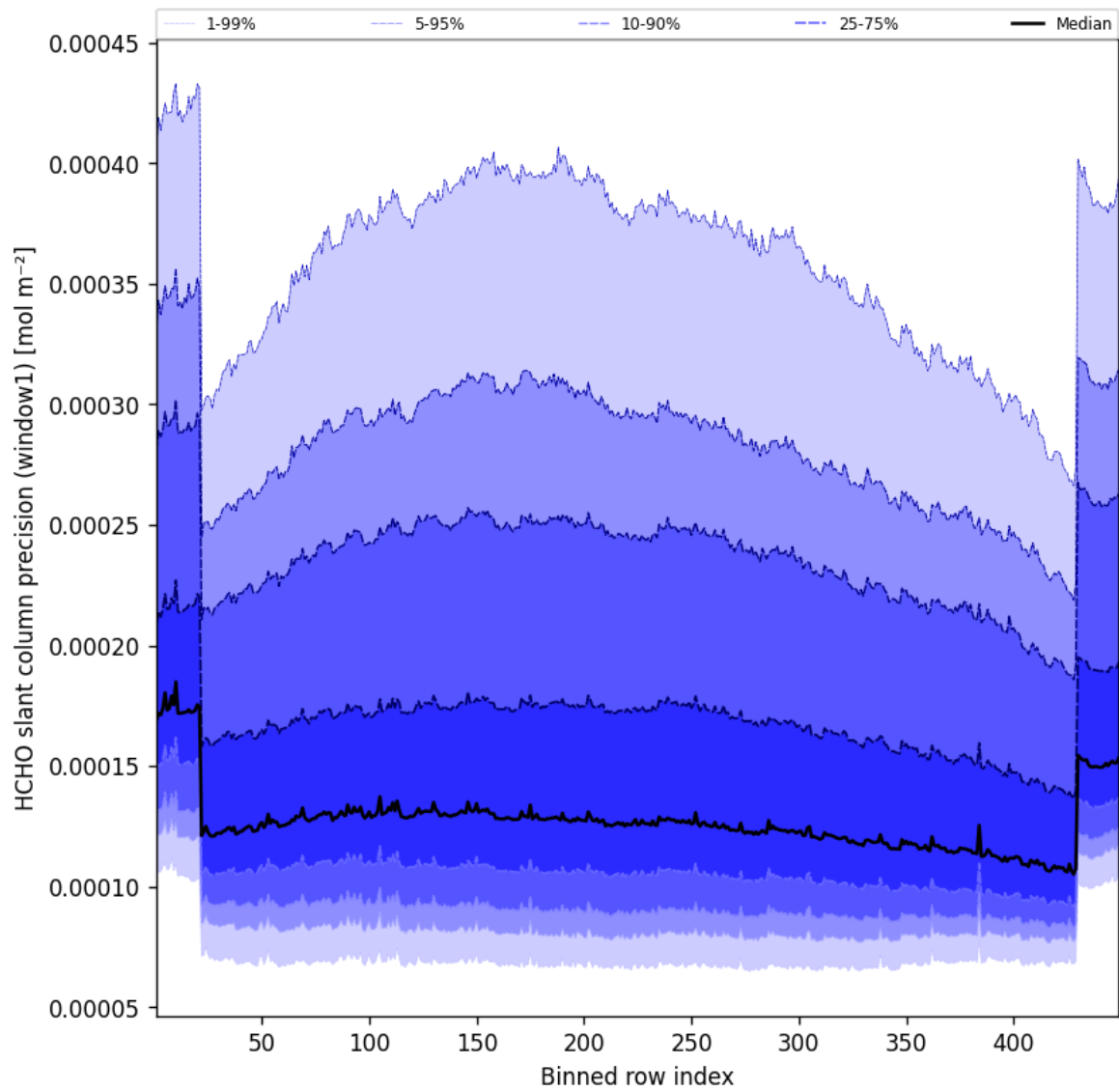
Figure 51: Along track statistics of “HCHO slant column precision (window1)” for 2025-06-03 to 2025-06-04
