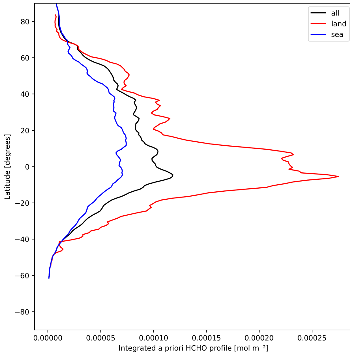
Figure 27: Zonal average of “Integrated a priori HCHO profile” for 2025-06-03 to 2025-06-04.
