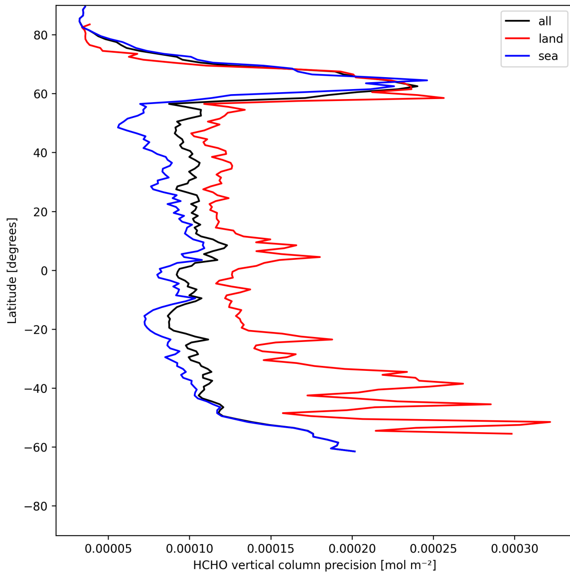
Figure 20: Zonal average of “HCHO vertical column precision” for 2025-06-03 to 2025-06-04.
