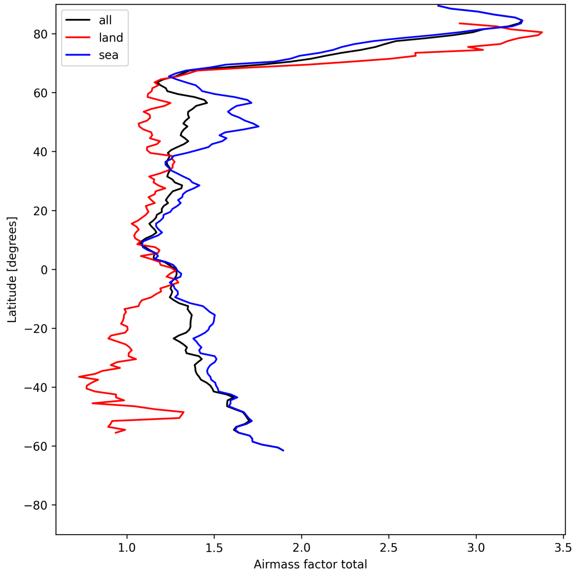
Figure 24: Zonal average of “Airmass factor total” for 2025-06-03 to 2025-06-04.
