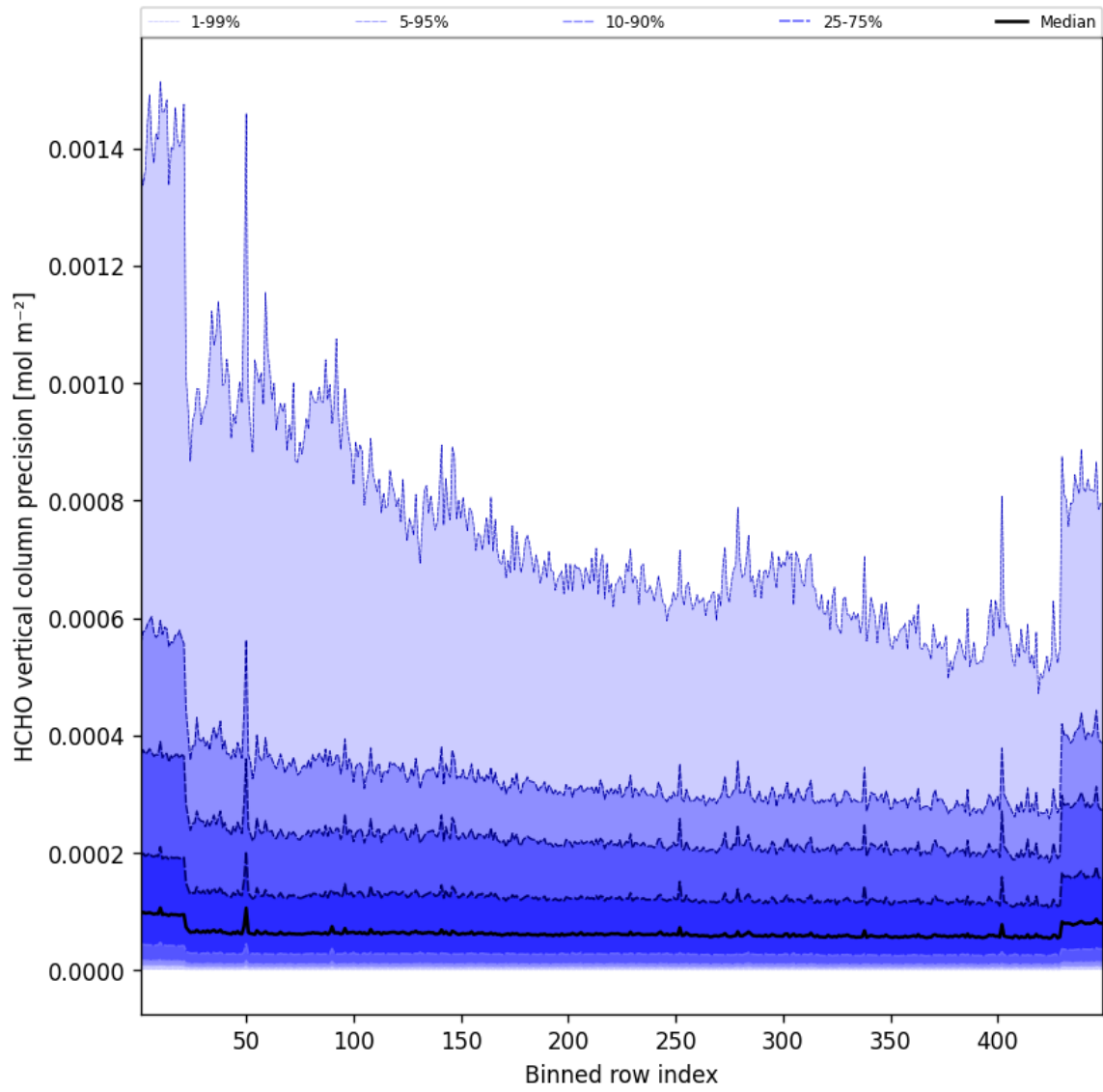
Figure 48: Along track statistics of “HCHO vertical column precision” for 2025-06-03 to 2025-06-04
