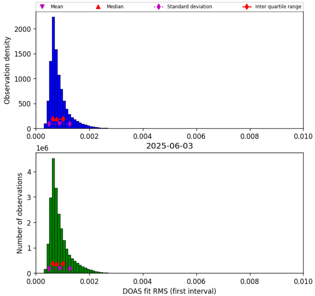
Figure 44: Histogram of "DOAS fit RMS (first interval)" for 2025-06-03 to 2025-06-04
