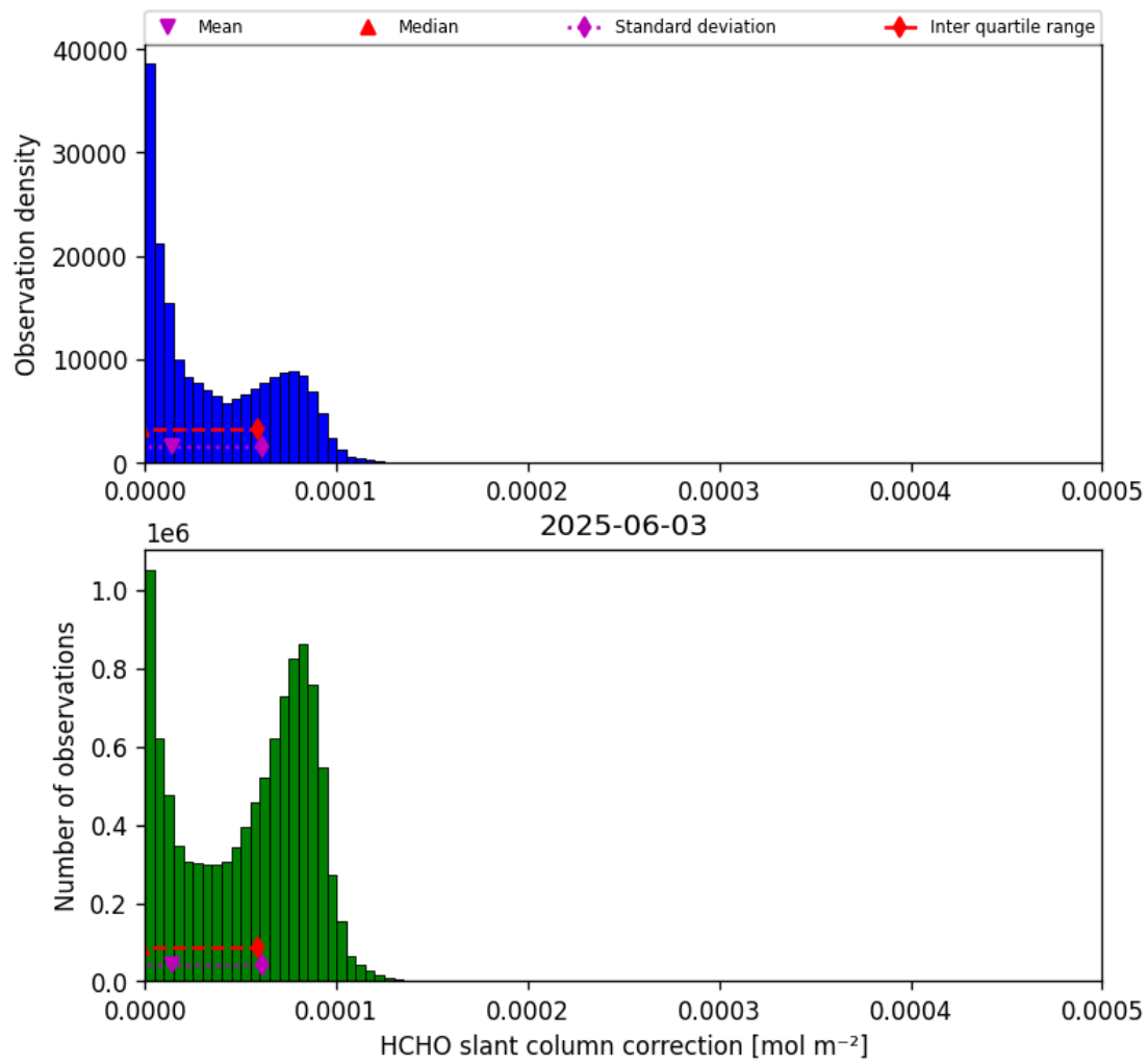
Figure 45: Histogram of “HCHO slant column correction” for 2025-06-03 to 2025-06-04
