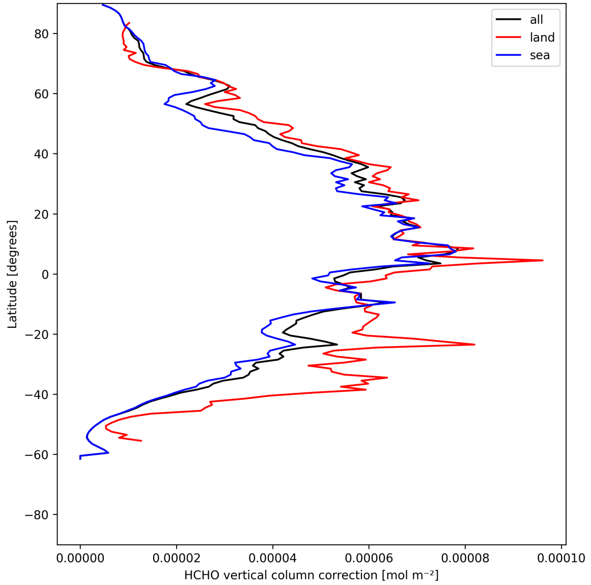
Figure 21: Zonal average of “HCHO vertical column correction” for 2025-06-03 to 2025-06-04.
