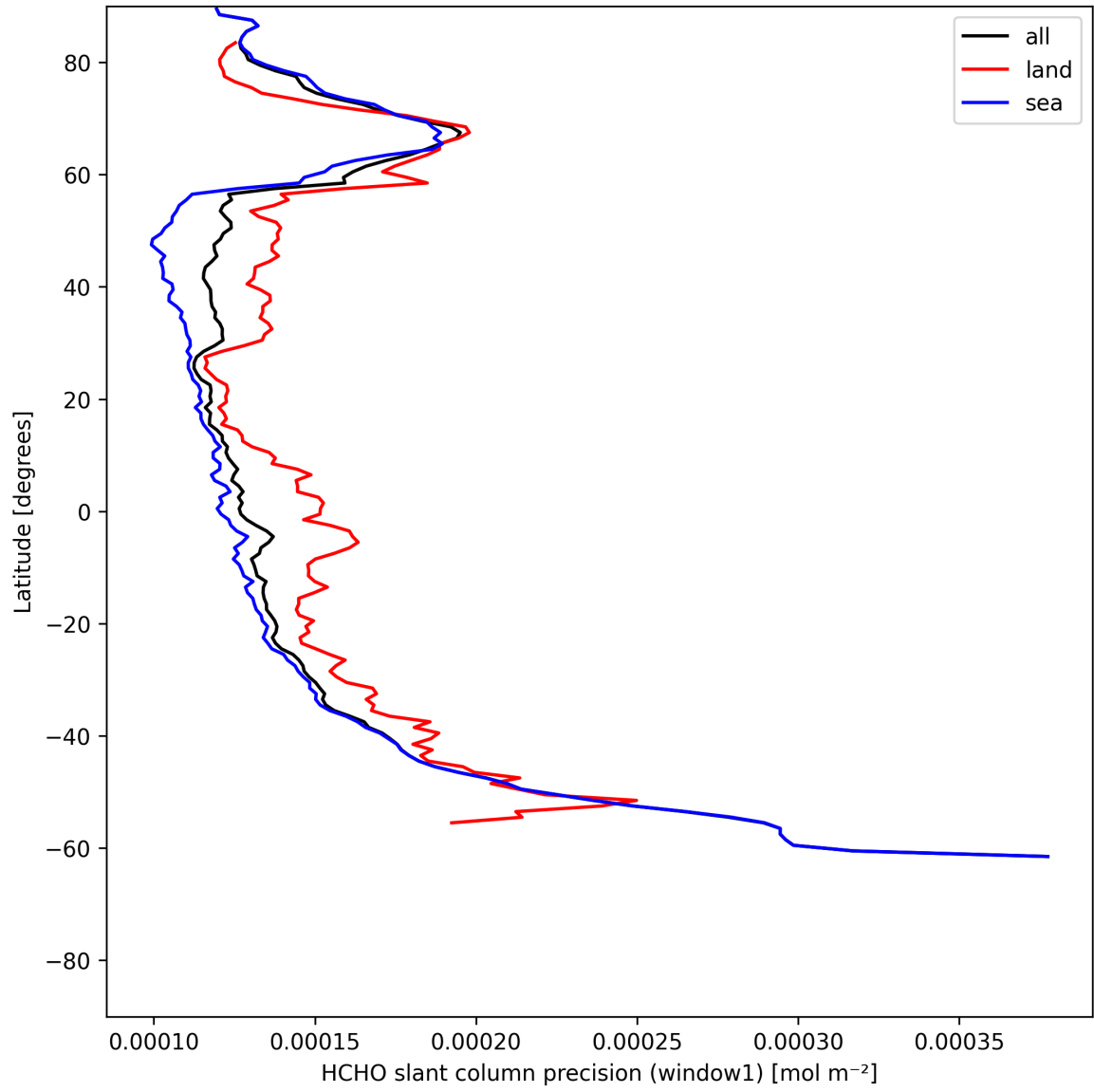
Figure 23: Zonal average of "HCHO slant column precision (window1)" for 2025-06-03 to 2025-06-04.
