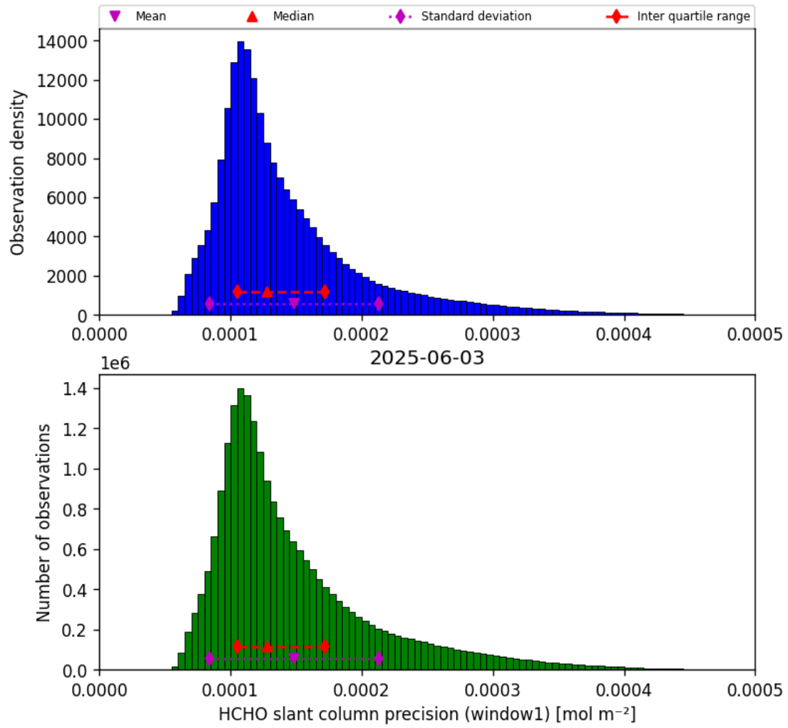
Figure 37: Histogram of “HCHO slant column precision (window1)” for 2025-06-03 to 2025-06-04
