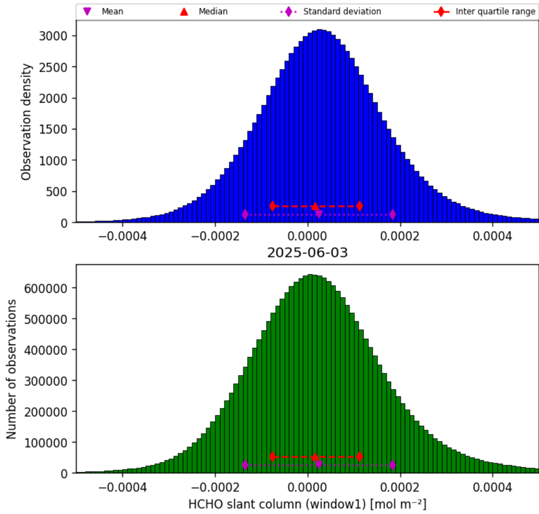
Figure 36: Histogram of “HCHO slant column (window1)” for 2025-06-03 to 2025-06-04
