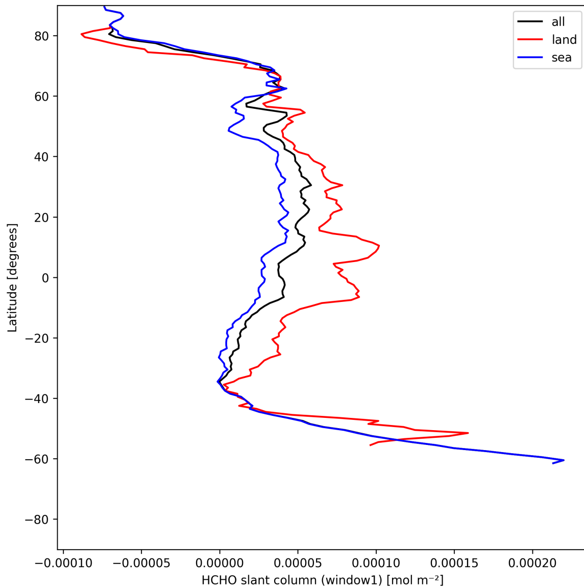
Figure 22: Zonal average of “HCHO slant column (window1)” for 2025-06-03 to 2025-06-04.
