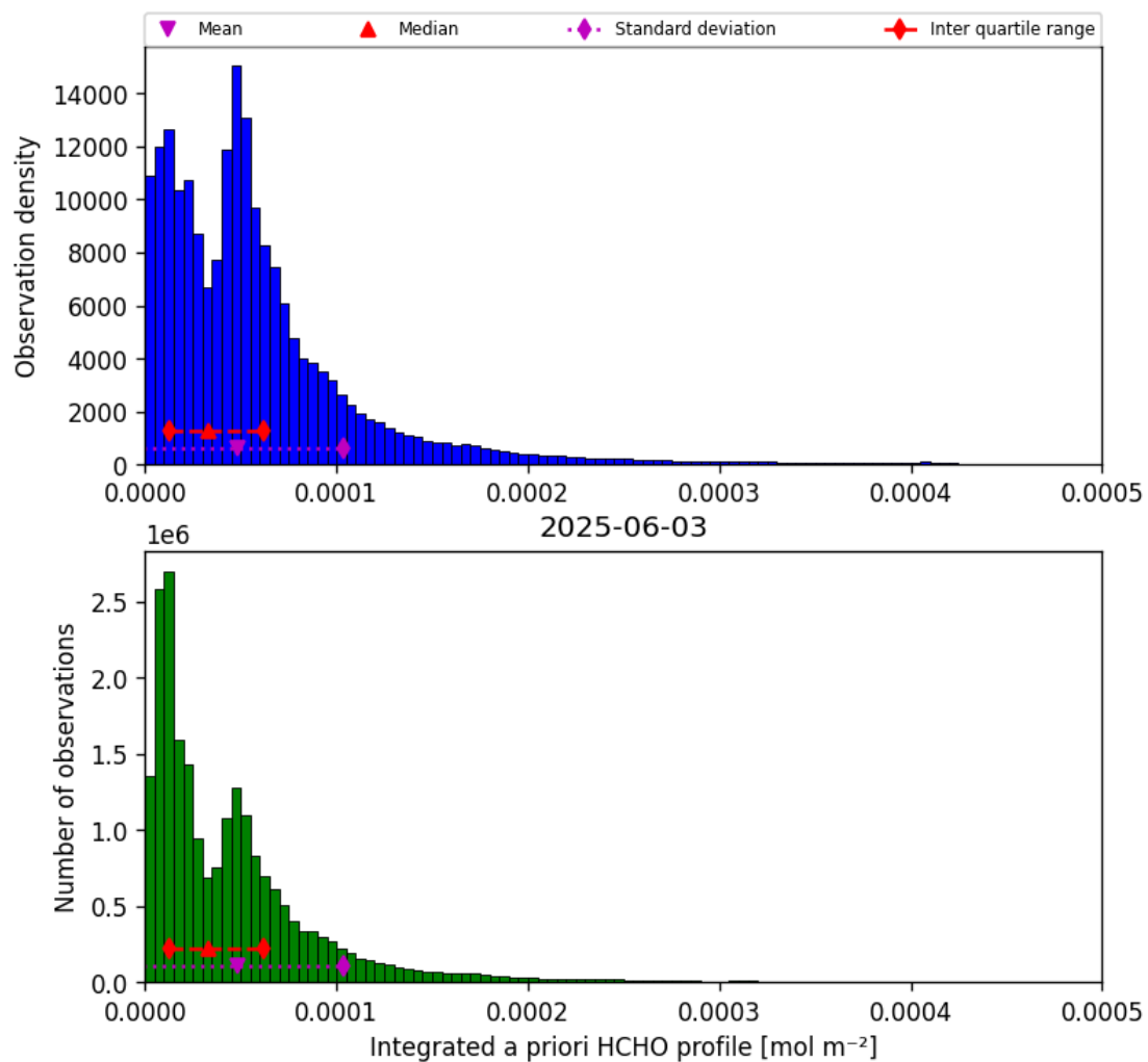
Figure 41: Histogram of “Integrated a priori HCHO profile” for 2025-06-03 to 2025-06-04
