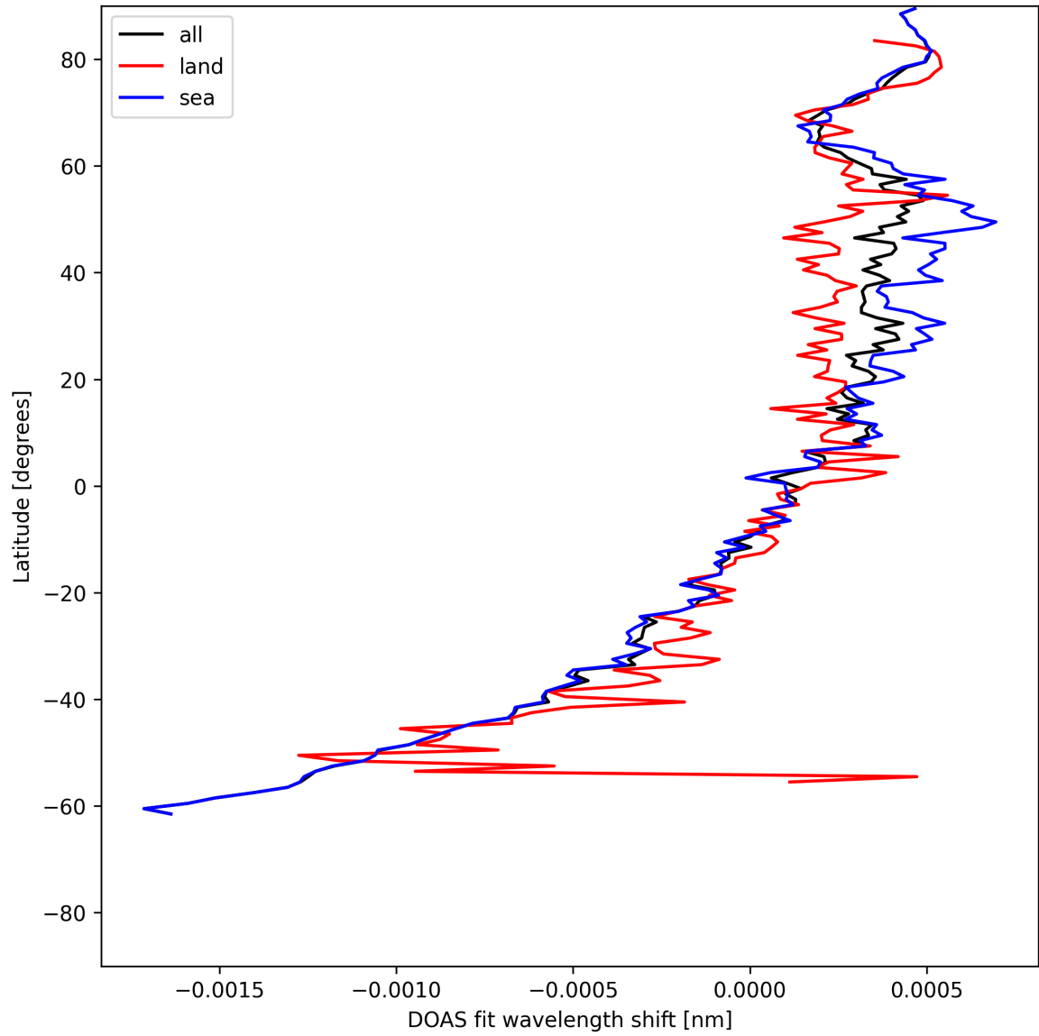
Figure 28: Zonal average of “DOAS fit wavelength shift” for 2025-06-03 to 2025-06-04.
