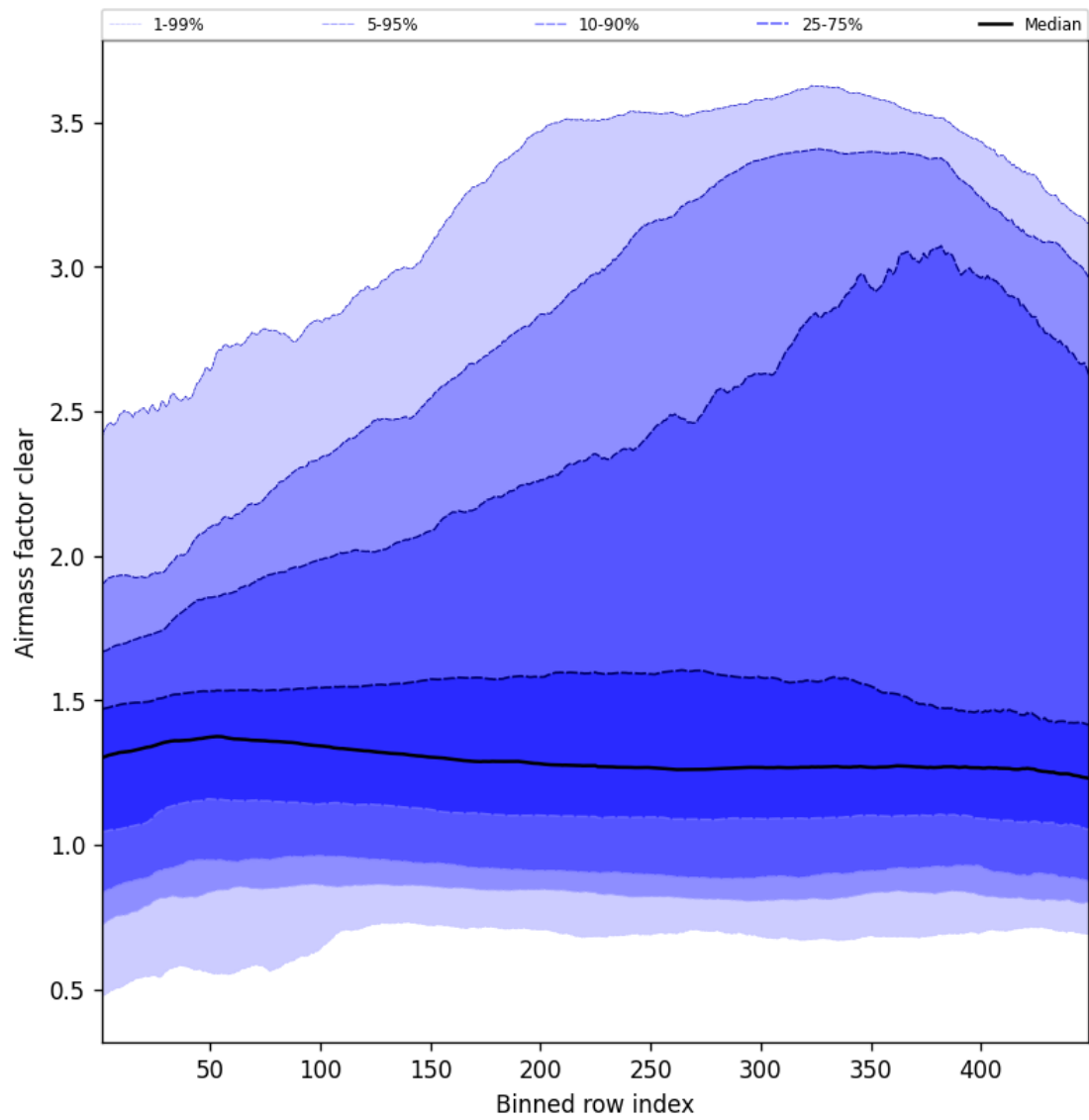
Figure 54: Along track statistics of “Air mass factor clear” for 2025-06-03 to 2025-06-04
