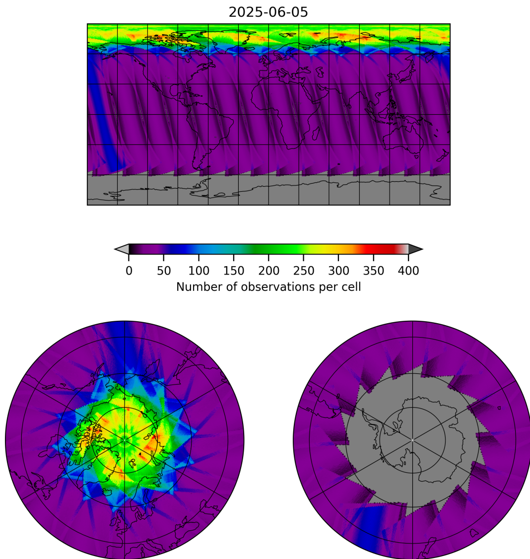
Figure 17: Map of the number of observations for 2025-06-05 to 2025-06-06
