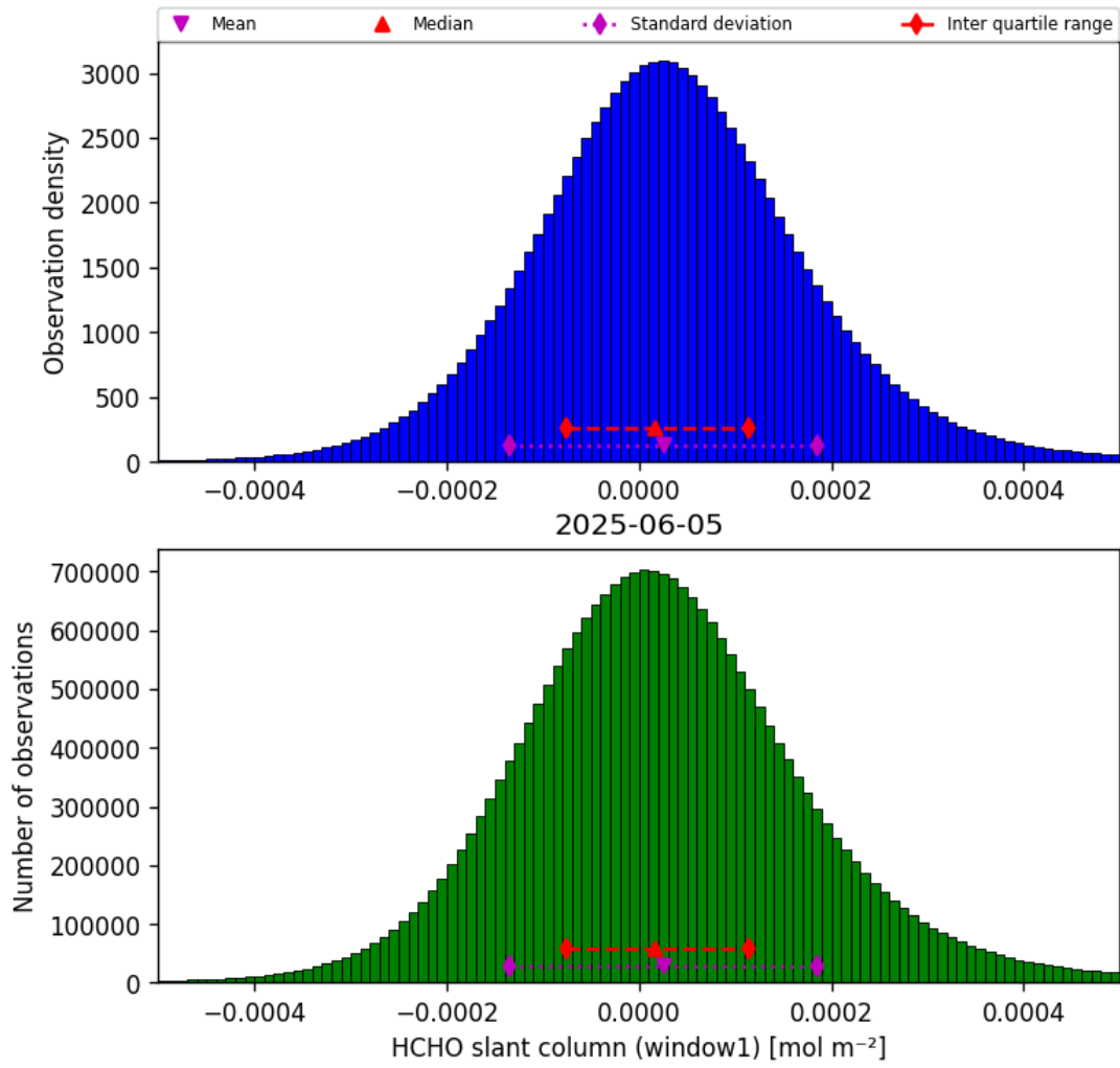
Figure 36: Histogram of “HCHO slant column (window1)” for 2025-06-05 to 2025-06-06
