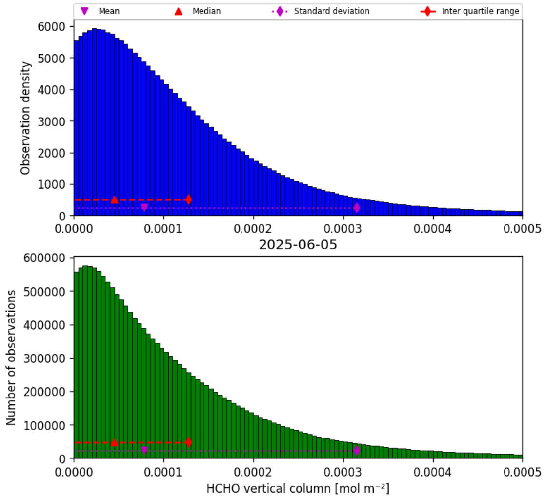
Figure 33: Histogram of “HCHO vertical column” for 2025-06-05 to 2025-06-06
