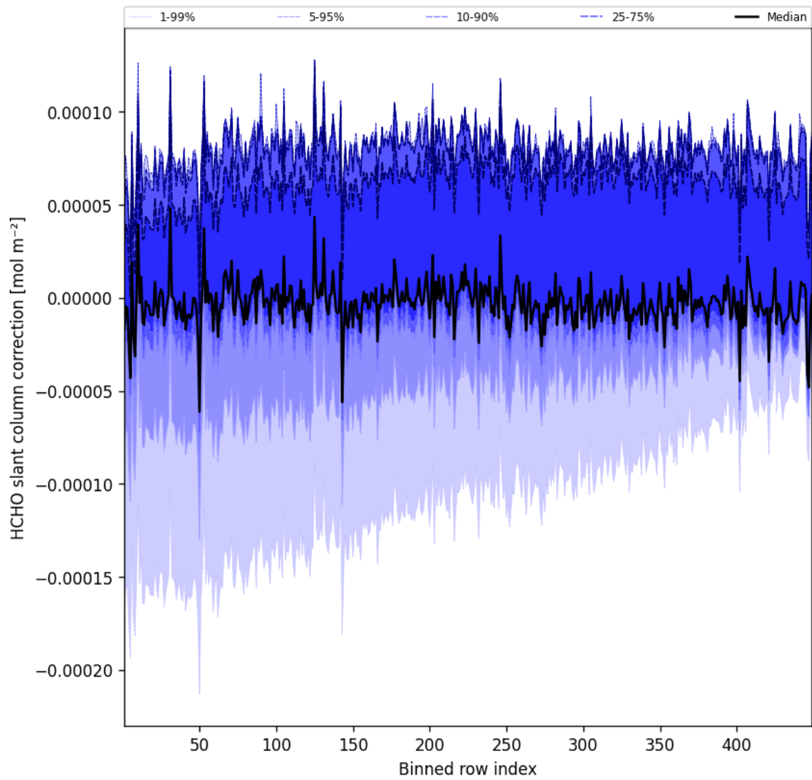
Figure 59: Along track statistics of “HCHO slant column correction” for 2025-06-05 to 2025-06-06
