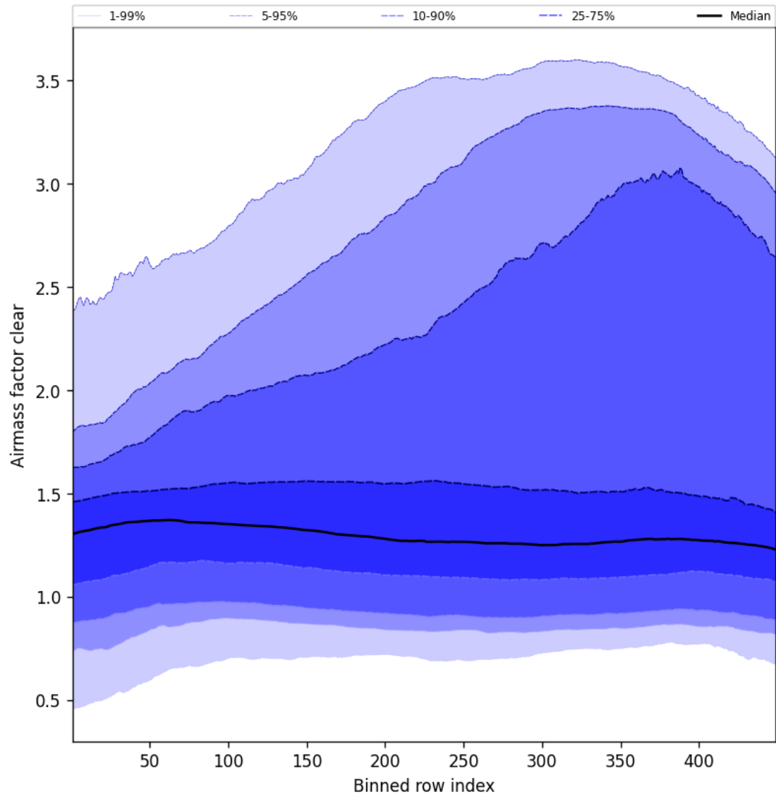
Figure 54: Along track statistics of “Airmass factor clear” for 2025-06-05 to 2025-06-06
