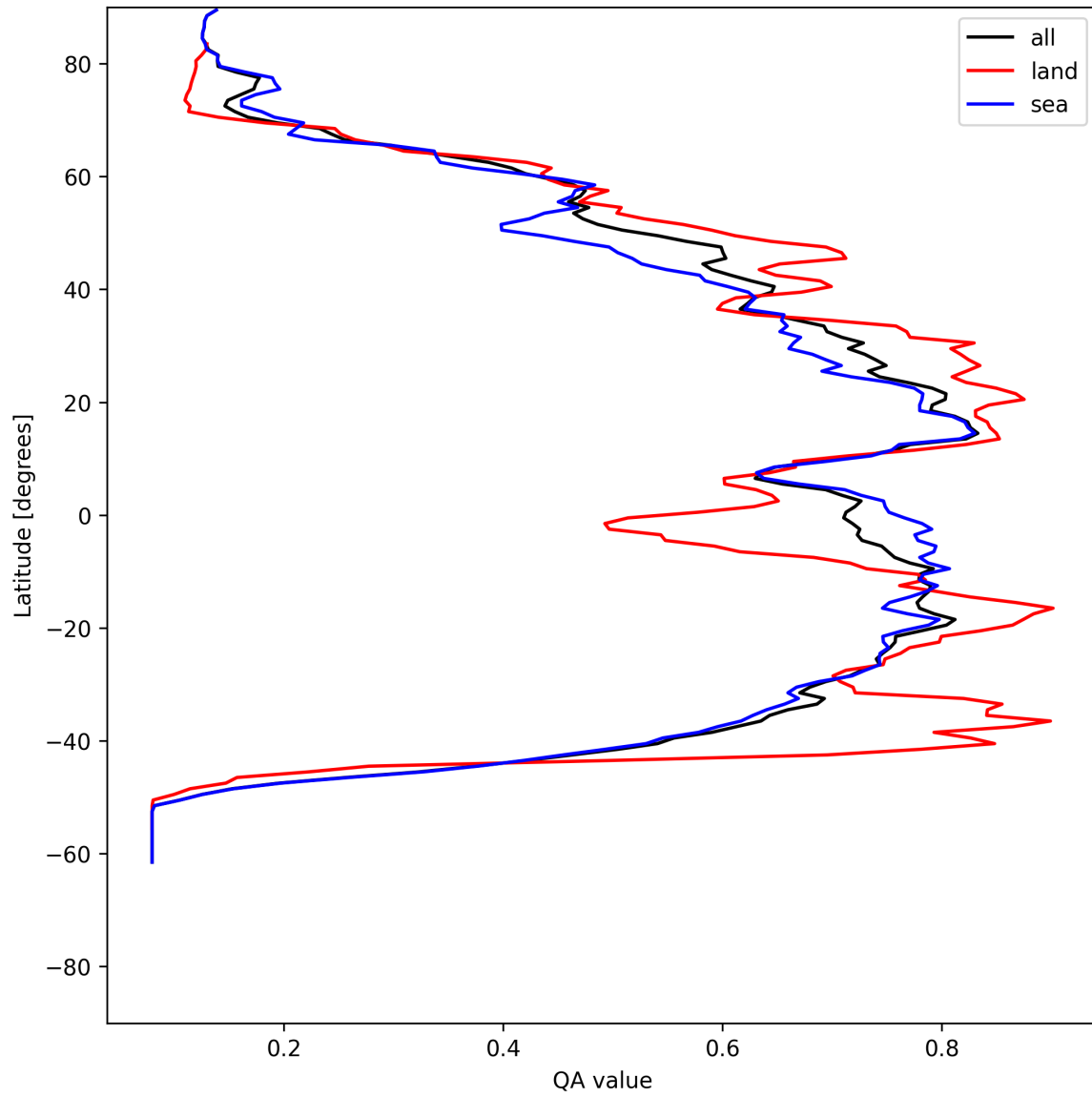
Figure 18: Zonal average of “QA value” for 2025-06-05 to 2025-06-06.
