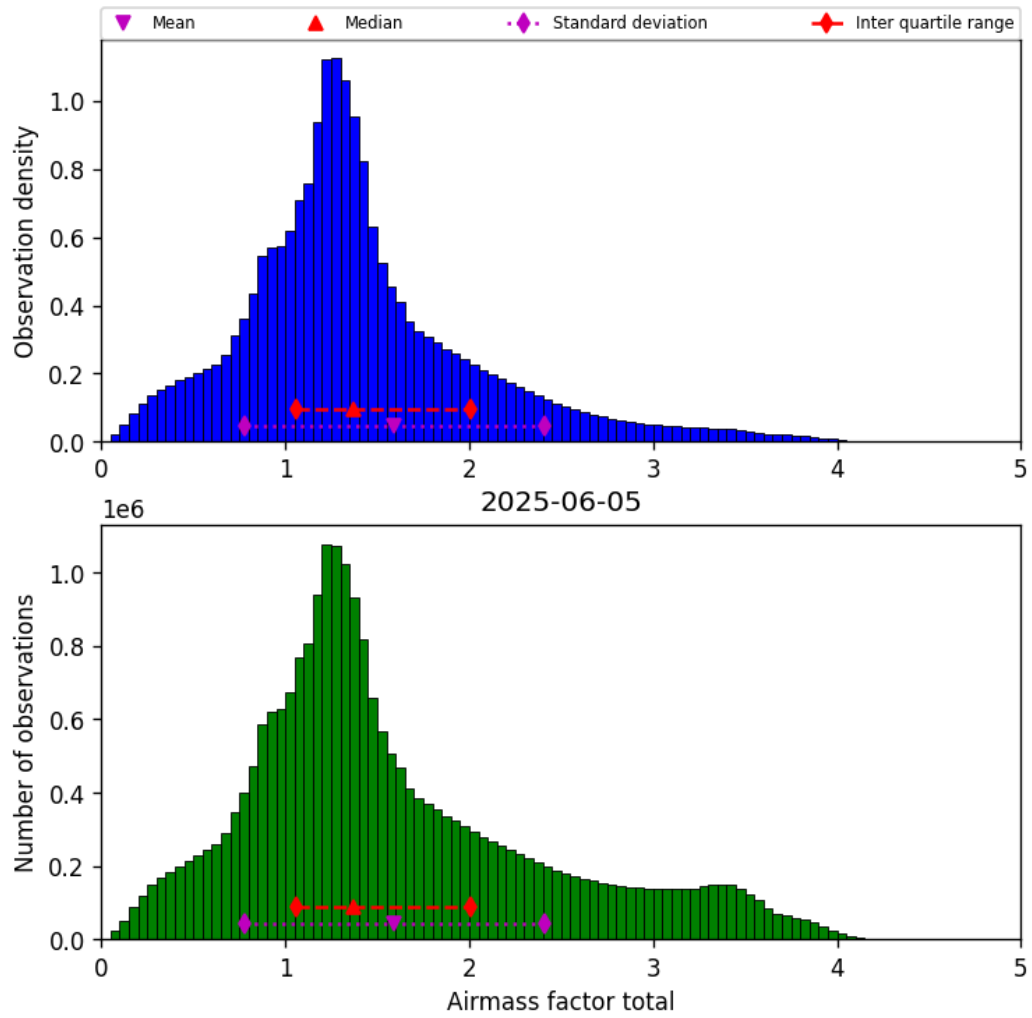
Figure 38: Histogram of “Airmass factor total” for 2025-06-05 to 2025-06-06
