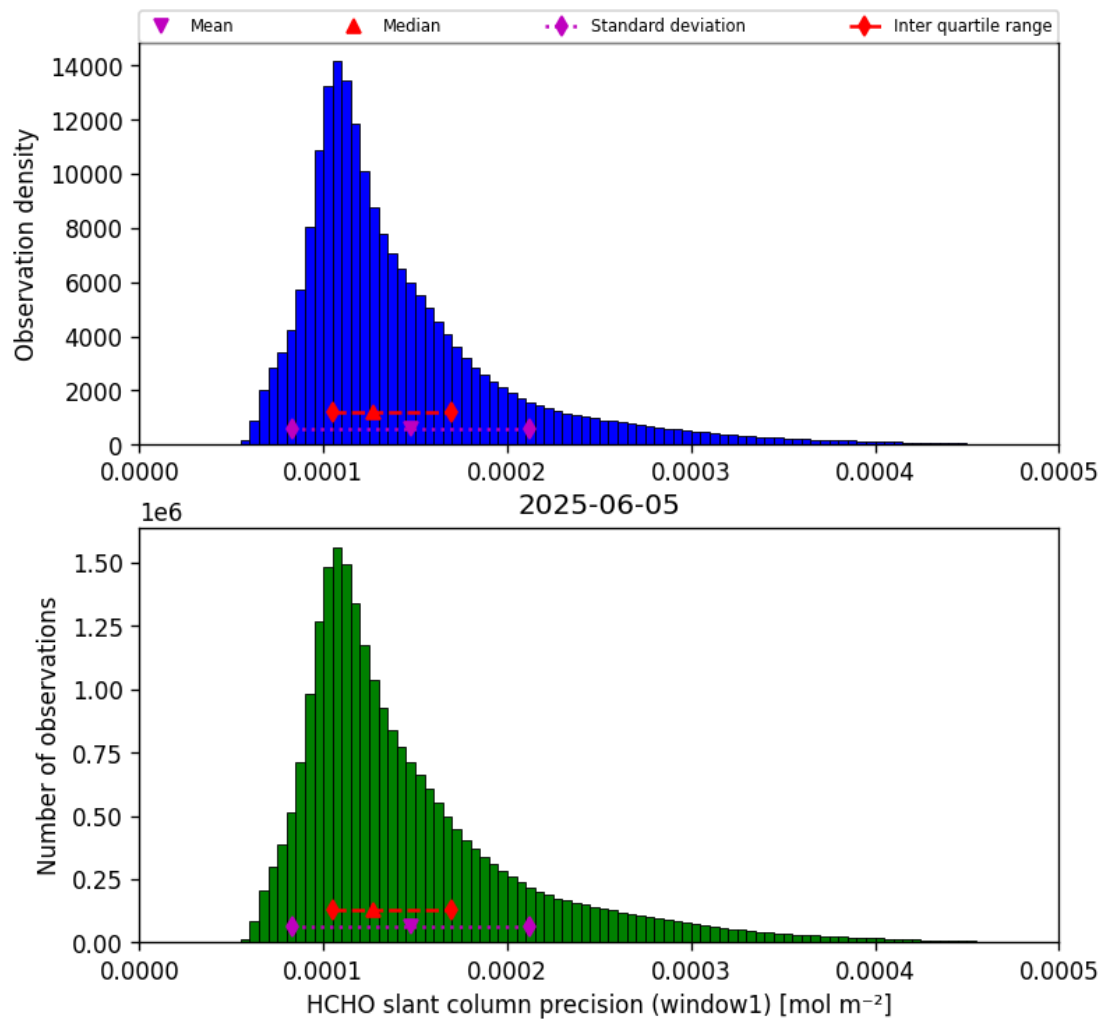
Figure 37: Histogram of “HCHO slant column precision (window1)” for 2025-06-05 to 2025-06-06
