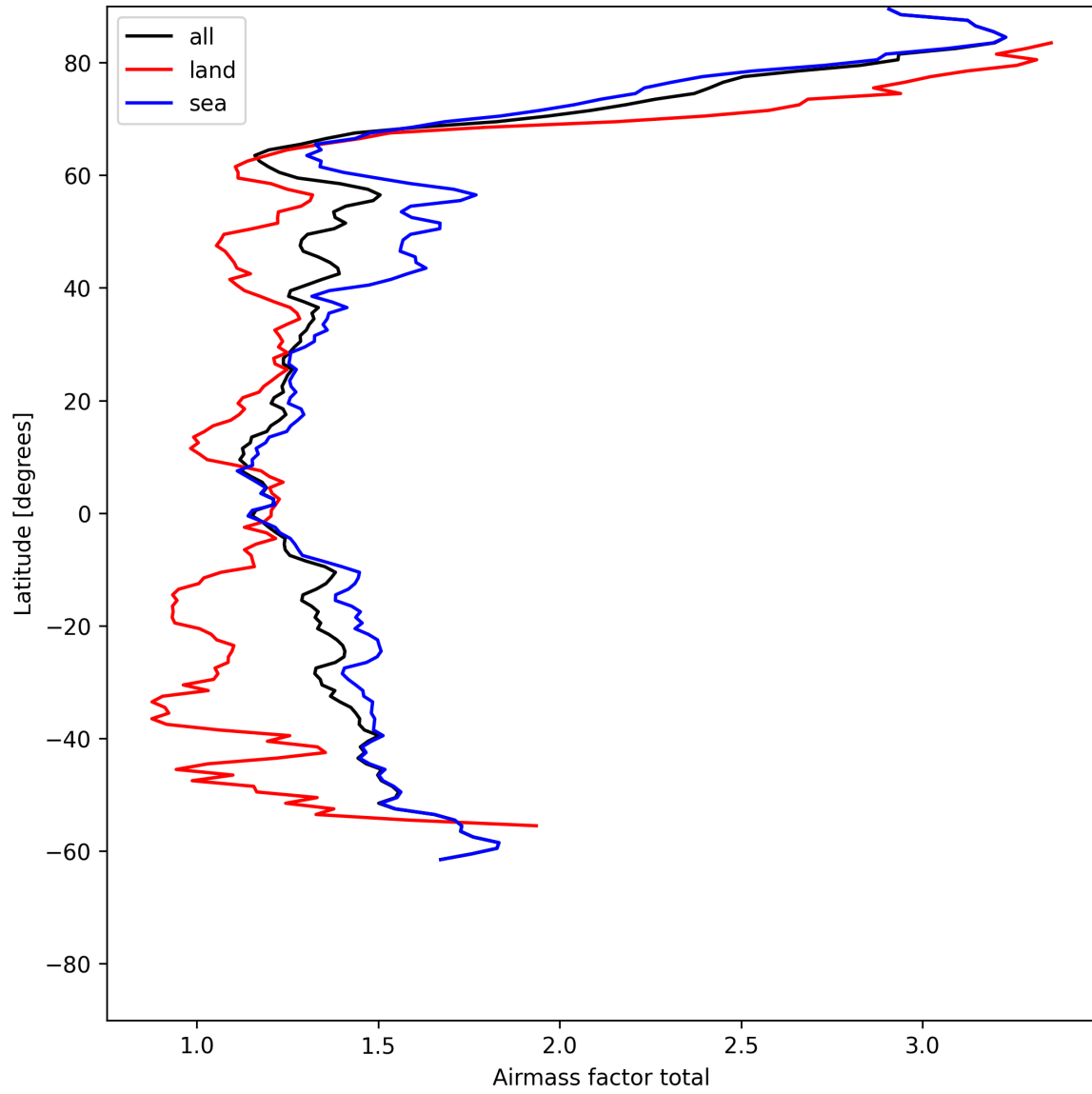
Figure 24: Zonal average of “Airmass factor total” for 2025-06-05 to 2025-06-06.
