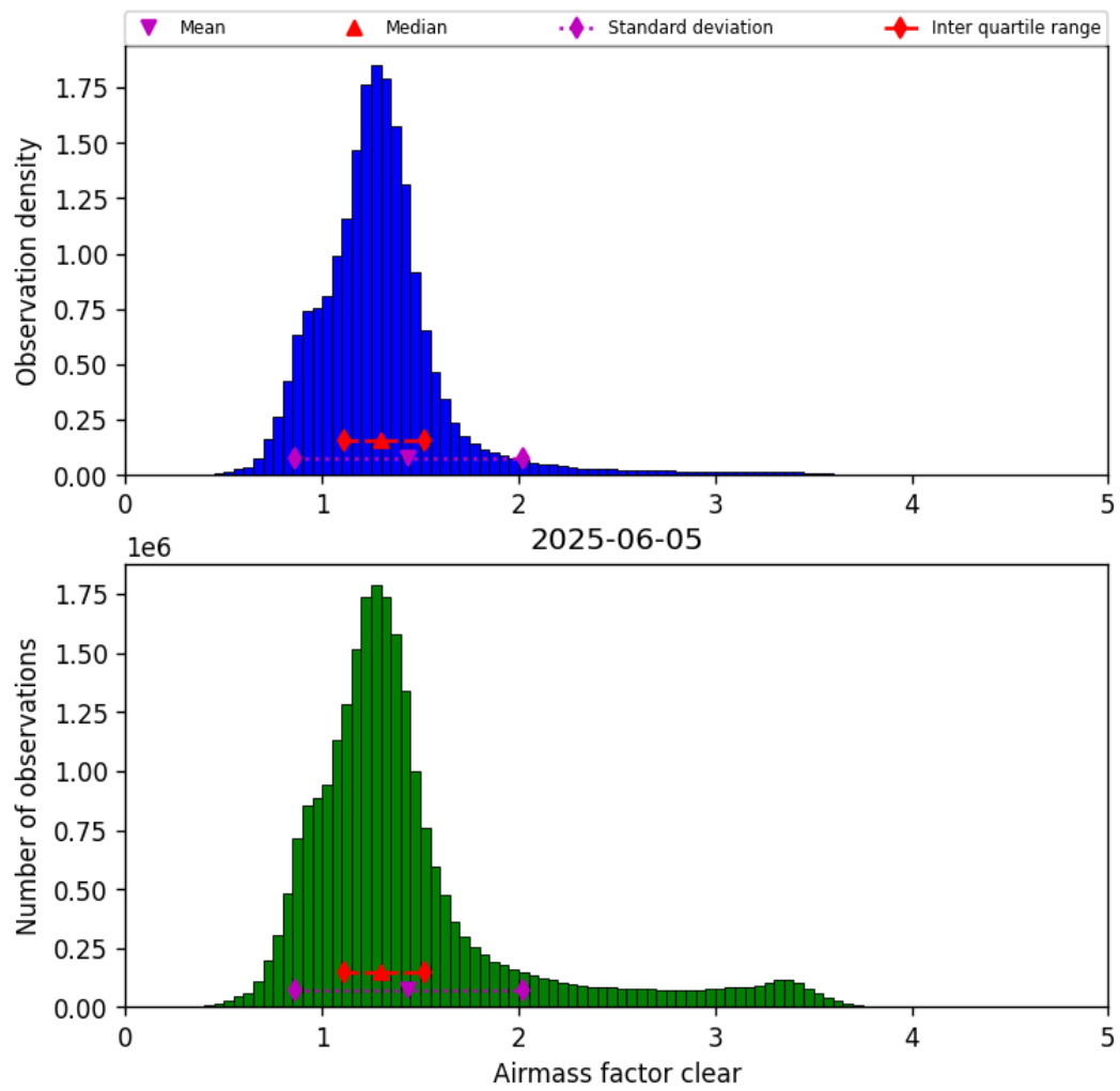
Figure 40: Histogram of “Airmass factor clear” for 2025-06-05 to 2025-06-06
