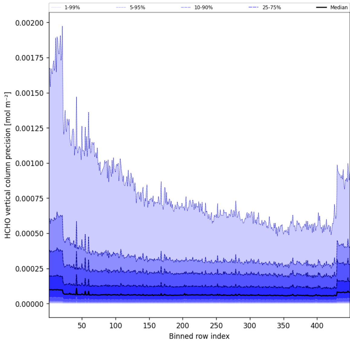
Figure 48: Along track statistics of “HCHO vertical column precision” for 2025-06-05 to 2025-06-06
