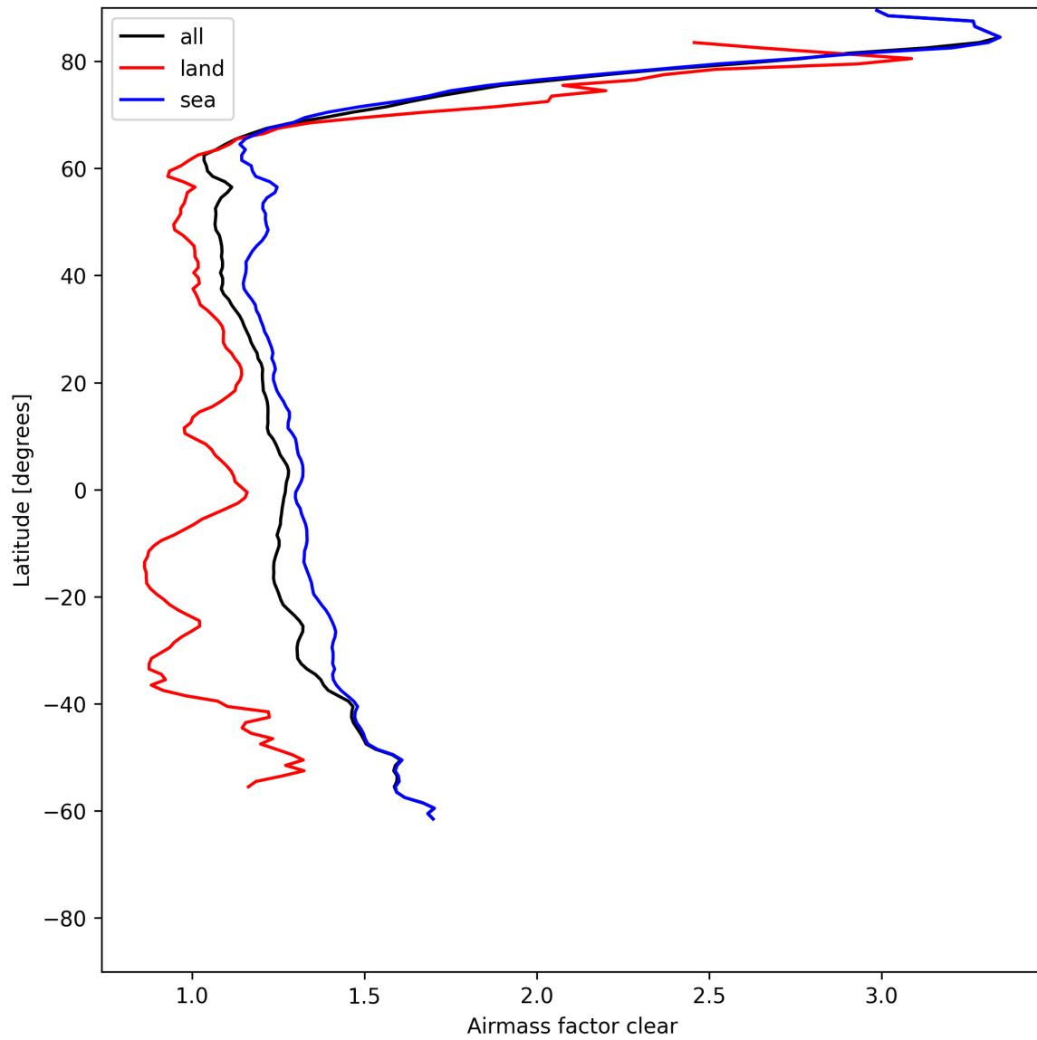
Figure 26: Zonal average of “Airmass factor clear” for 2025-06-05 to 2025-06-06.
