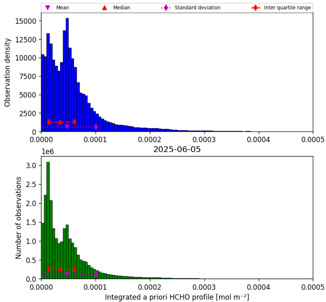
Figure 41: Histogram of “Integrated a priori HCHO profile” for 2025-06-05 to 2025-06-06
