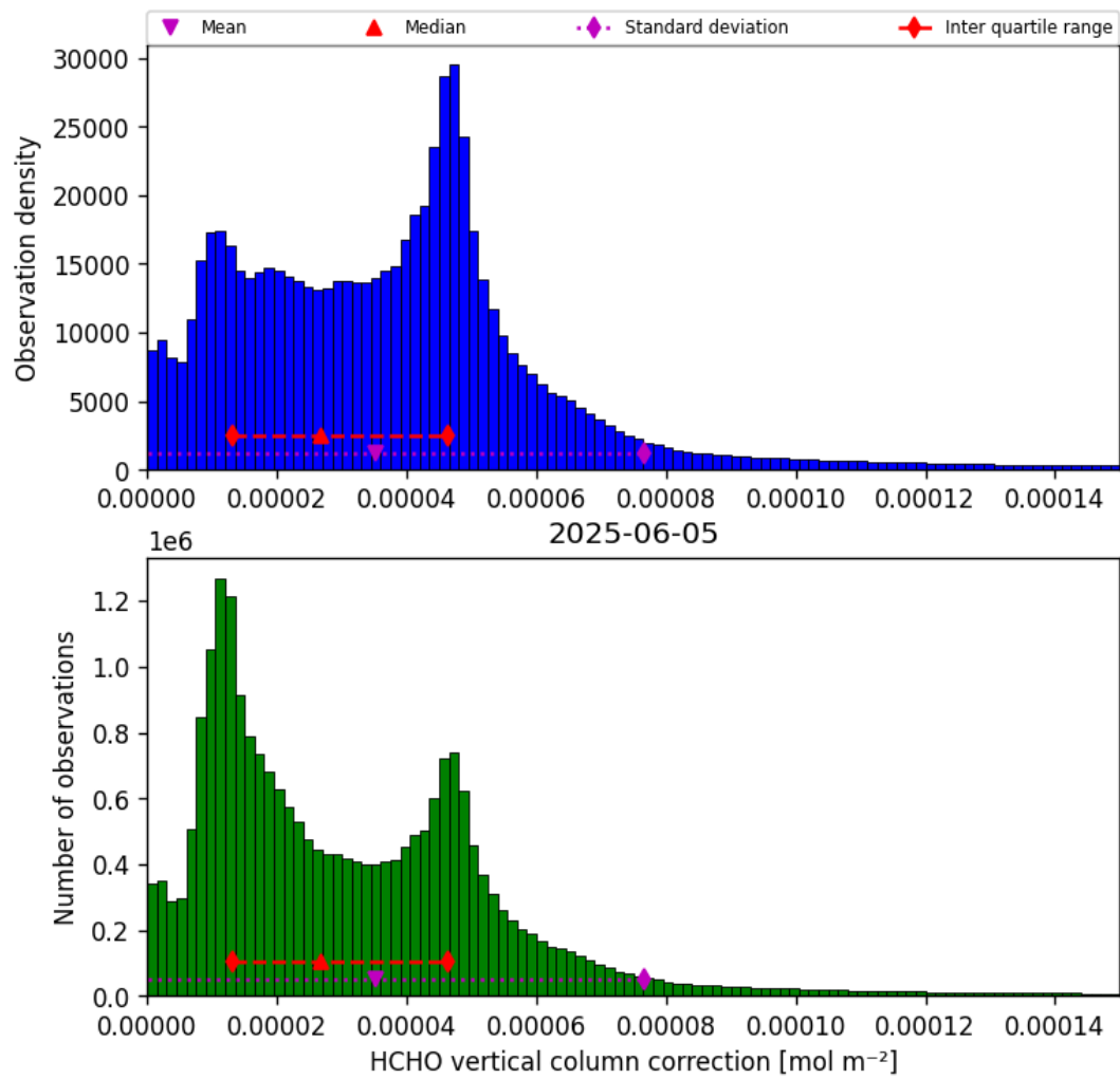
Figure 35: Histogram of “HCHO vertical column correction” for 2025-06-05 to 2025-06-06
