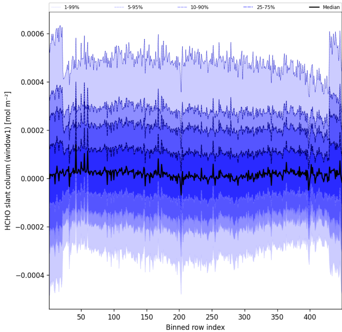
Figure 50: Along track statistics of “HCHO slant column (window1)” for 2025-06-05 to 2025-06-06
