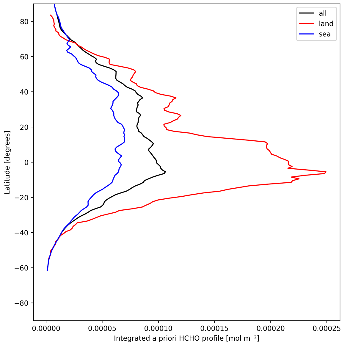
Figure 27: Zonal average of “Integrated a priori HCHO profile” for 2025-06-05 to 2025-06-06.
