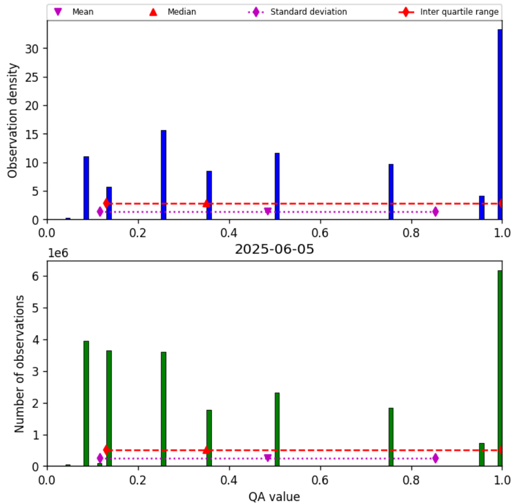
Figure 32: Histogram of “QA value” for 2025-06-05 to 2025-06-06
