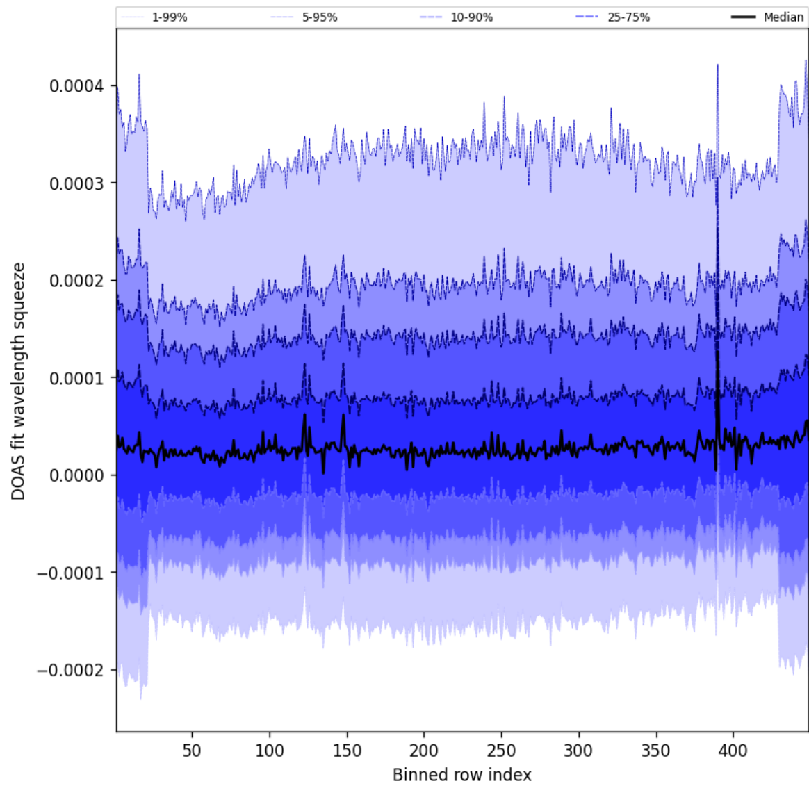
Figure 57: Along track statistics of “DOAS fit wavelength squeeze” for 2025-06-07 to 2025-06-08
