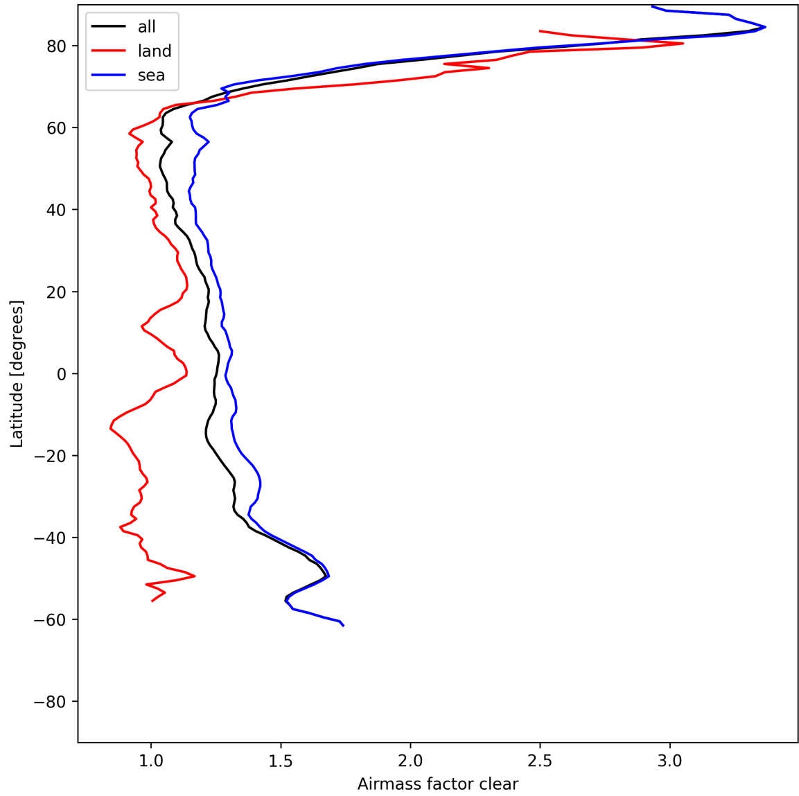
Figure 26: Zonal average of “Airmass factor clear” for 2025-06-07 to 2025-06-08.
