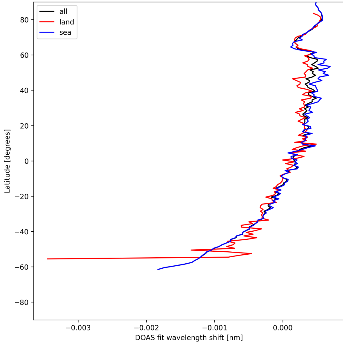
Figure 28: Zonal average of “DOAS fit wavelength shift” for 2025-06-07 to 2025-06-08.
