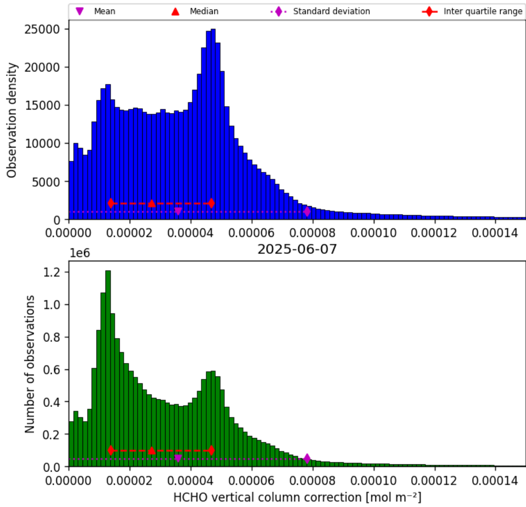
Figure 35: Histogram of “HCHO vertical column correction” for 2025-06-07 to 2025-06-08
