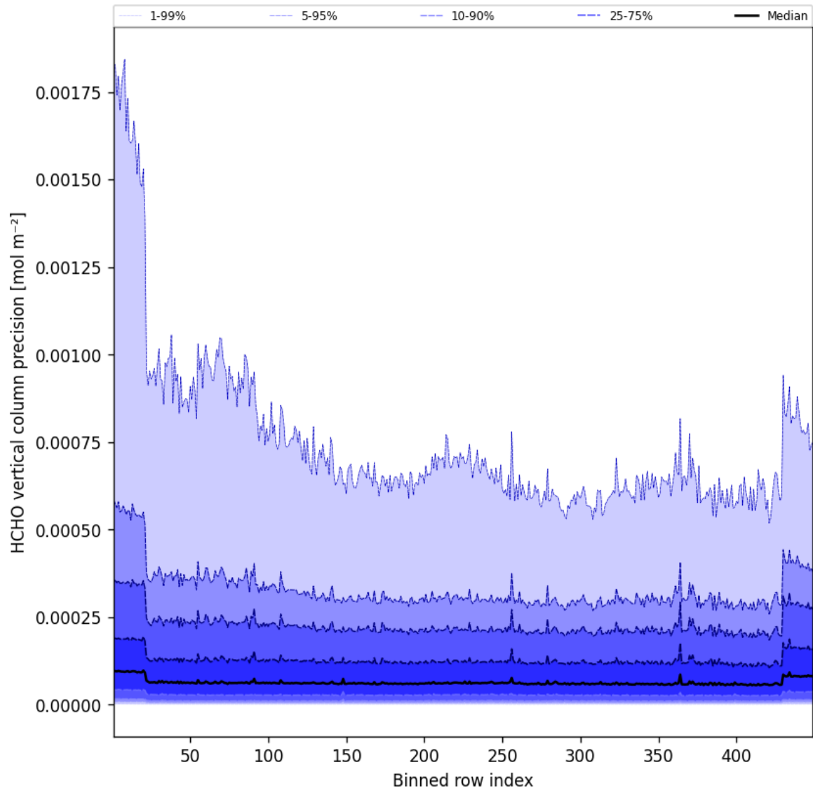
Figure 48: Along track statistics of “HCHO vertical column precision” for 2025-06-07 to 2025-06-08
