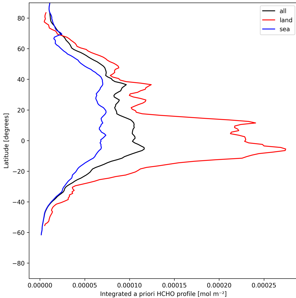
Figure 27: Zonal average of “Integrated a priori HCHO profile” for 2025-06-07 to 2025-06-08.
