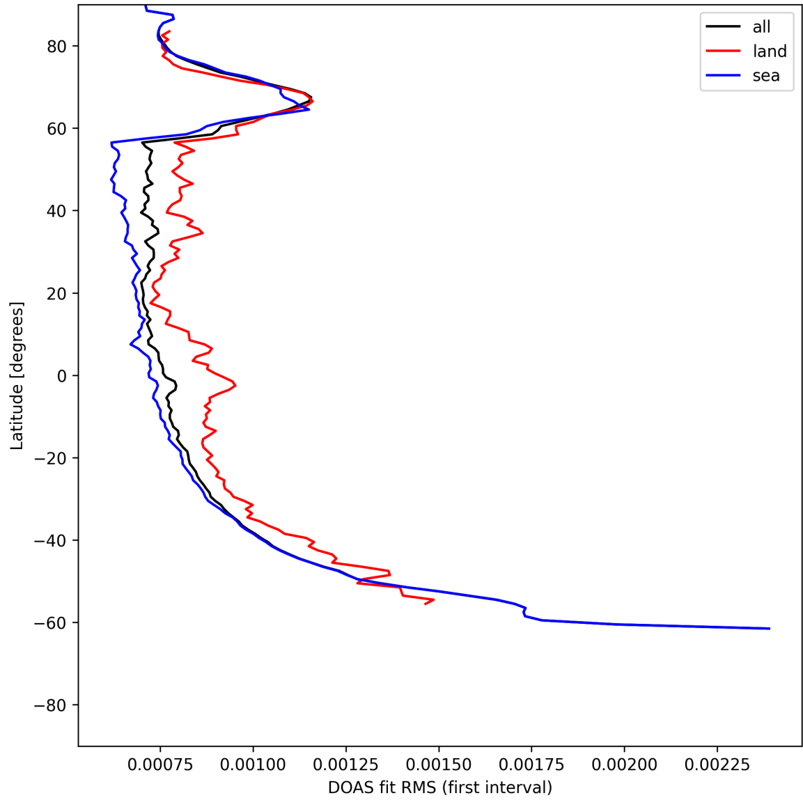
Figure 30: Zonal average of "DOAS fit RMS (first interval)" for 2025-06-07 to 2025-06-08.
