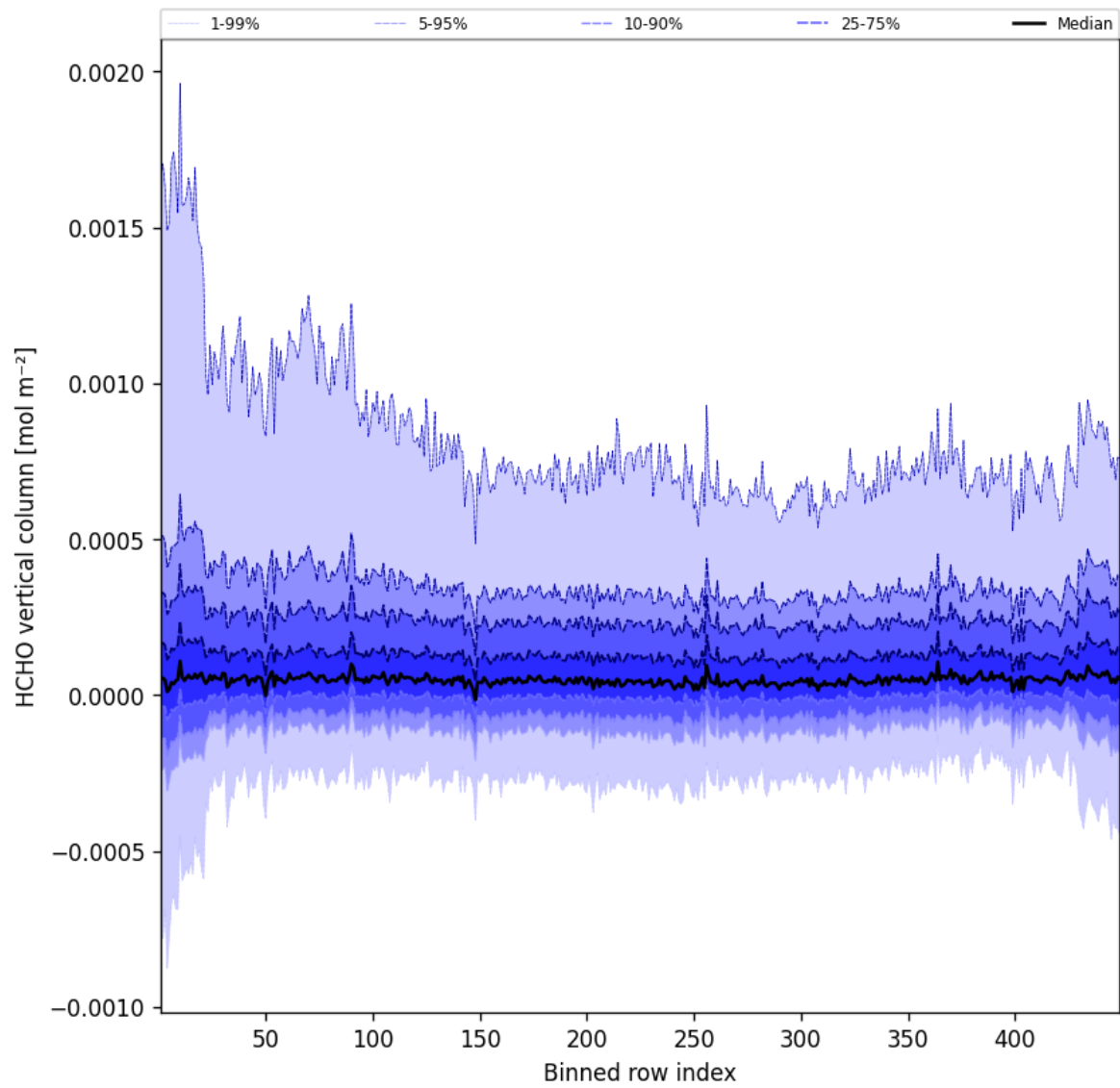
Figure 47: Along track statistics of “HCHO vertical column” for 2025-06-07 to 2025-06-08
