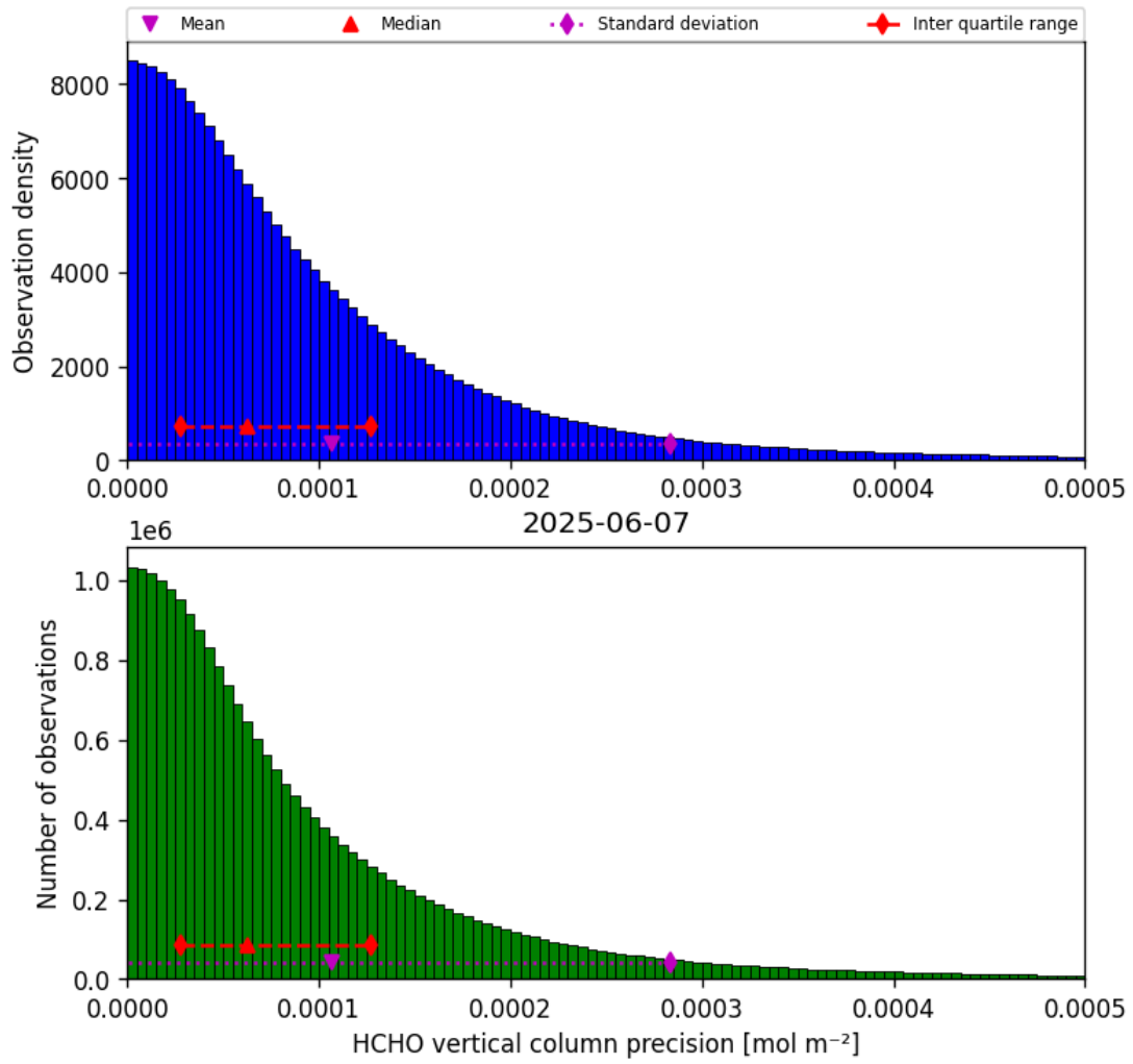
Figure 34: Histogram of “HCHO vertical column precision” for 2025-06-07 to 2025-06-08
