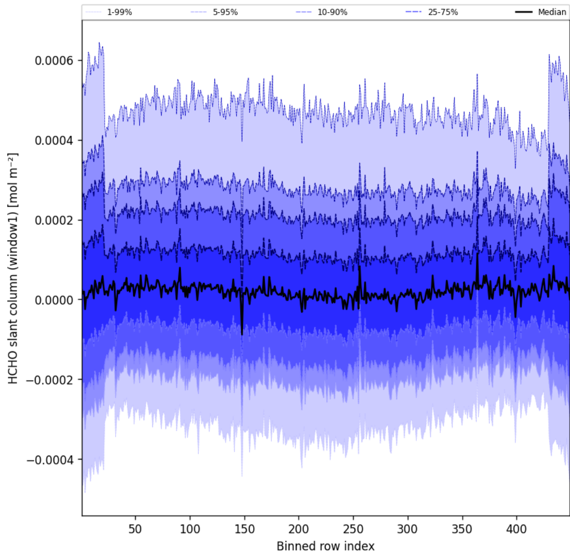
Figure 50: Along track statistics of “HCHO slant column (window1)” for 2025-06-07 to 2025-06-08
