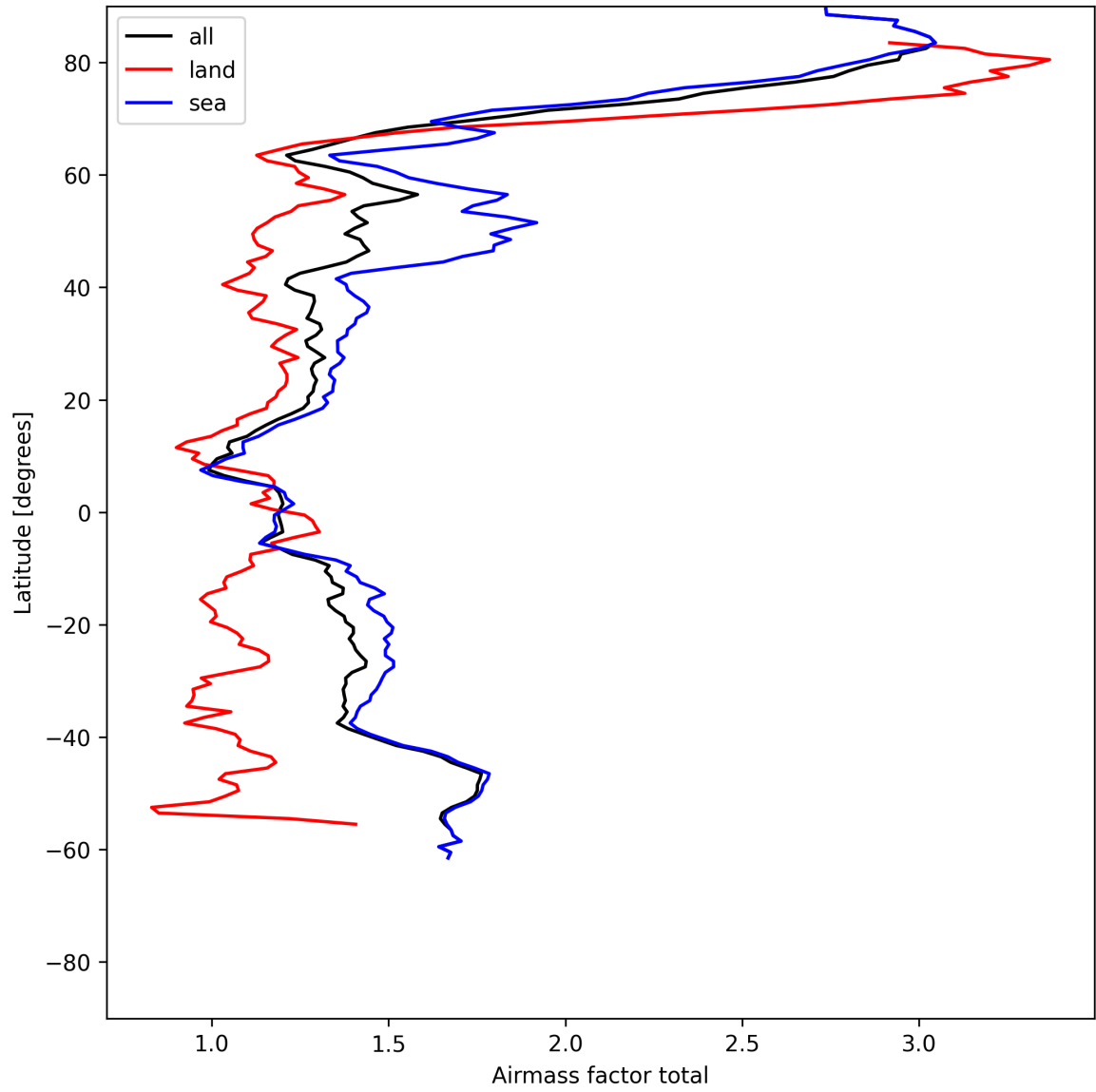
Figure 24: Zonal average of “Airmass factor total” for 2025-06-07 to 2025-06-08.
