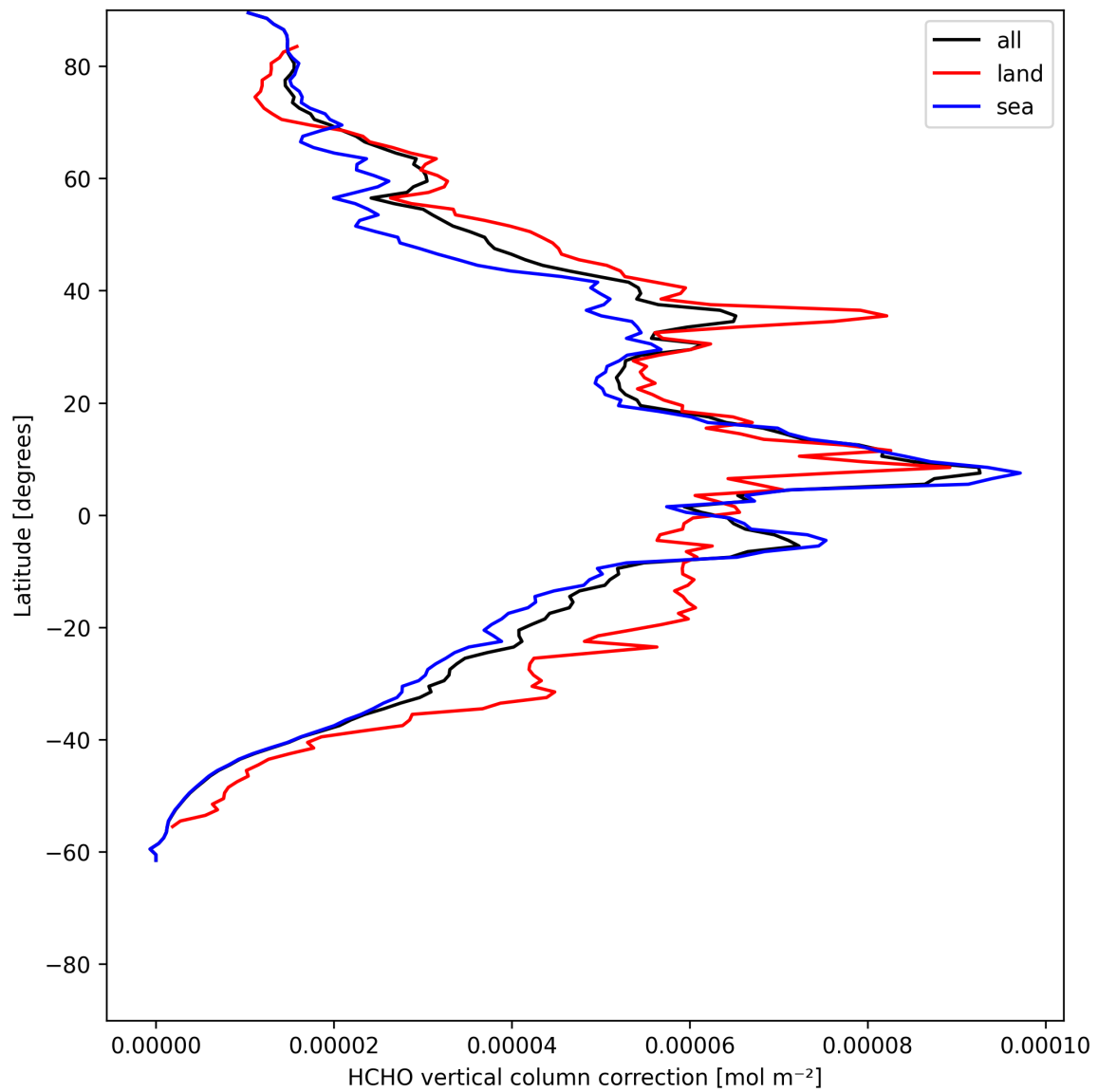
Figure 21: Zonal average of “HCHO vertical column correction” for 2025-06-07 to 2025-06-08.
