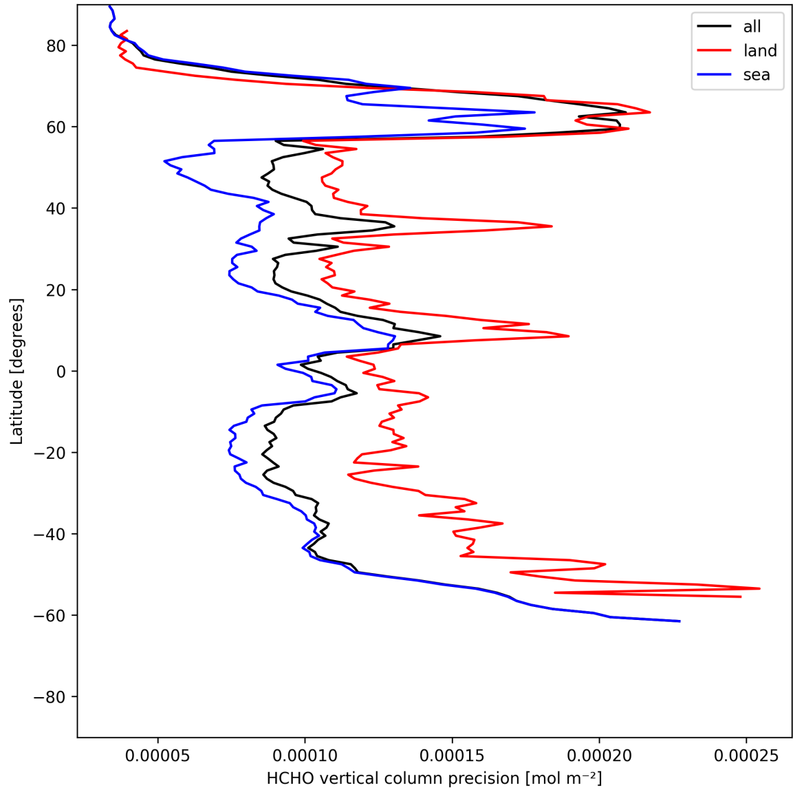
Figure 20: Zonal average of “HCHO vertical column precision” for 2025-06-07 to 2025-06-08.
