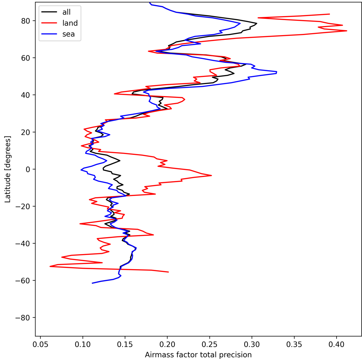
Figure 25: Zonal average of “Airmass factor total precision” for 2025-06-07 to 2025-06-08.
