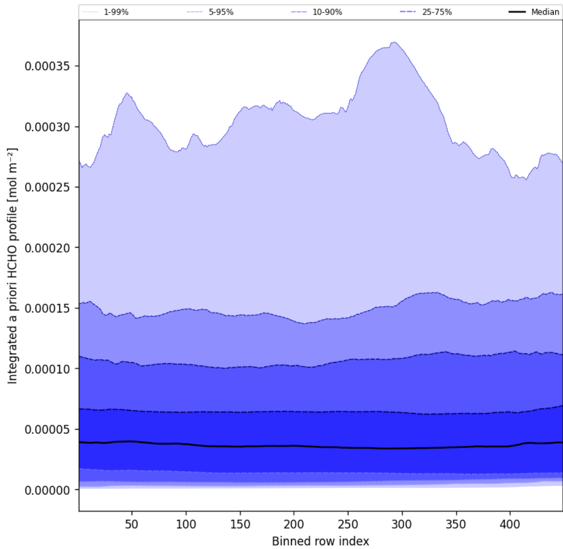
Figure 55: Along track statistics of "Integrated a priori HCHO profile" for 2025-06-07 to 2025-06-08
