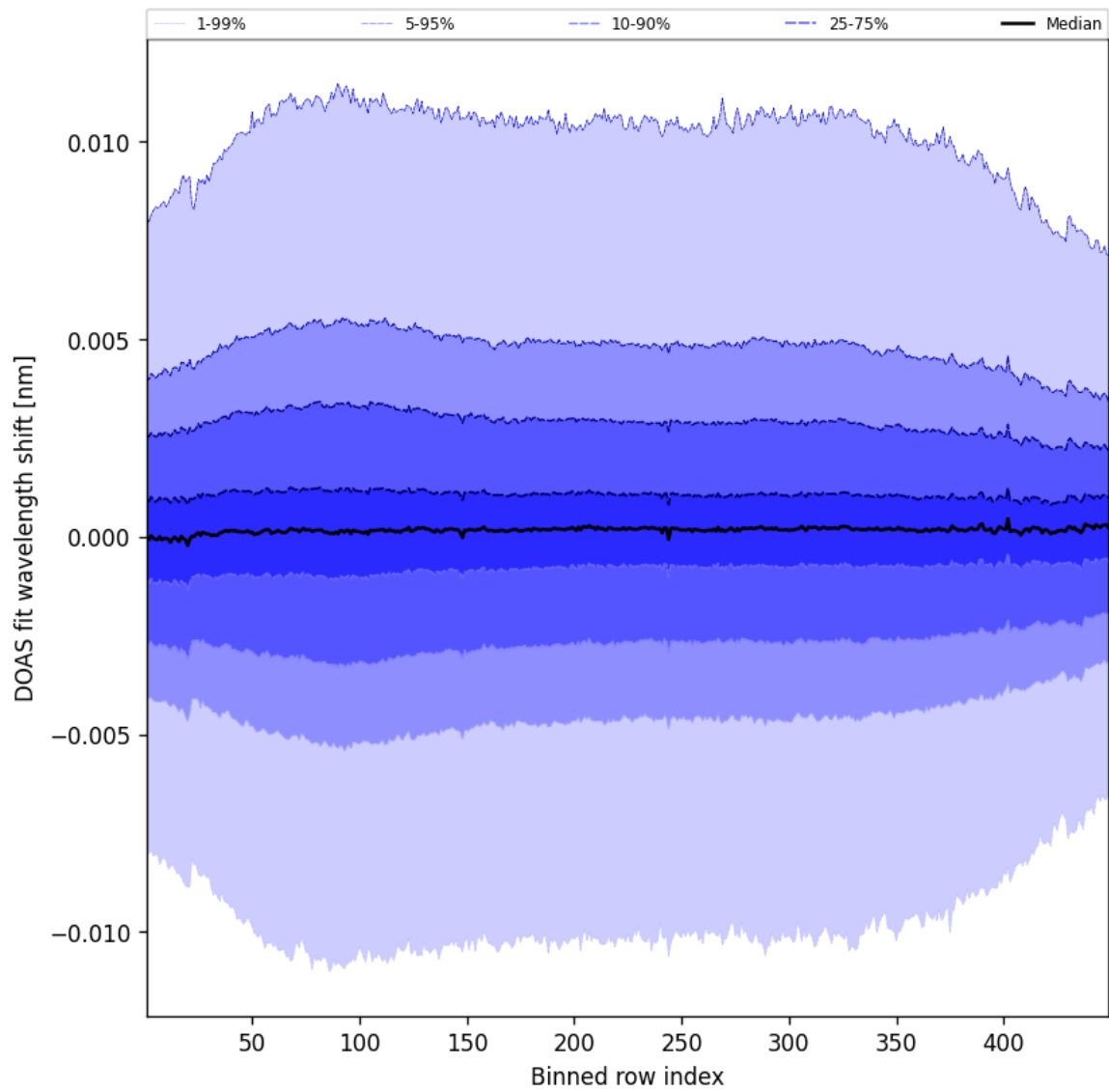
Figure 56: Along track statistics of “DOAS fit wavelength shift” for 2025-06-07 to 2025-06-08
