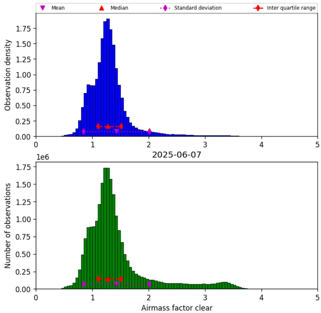
Figure 40: Histogram of “Airmass factor clear” for 2025-06-07 to 2025-06-08
