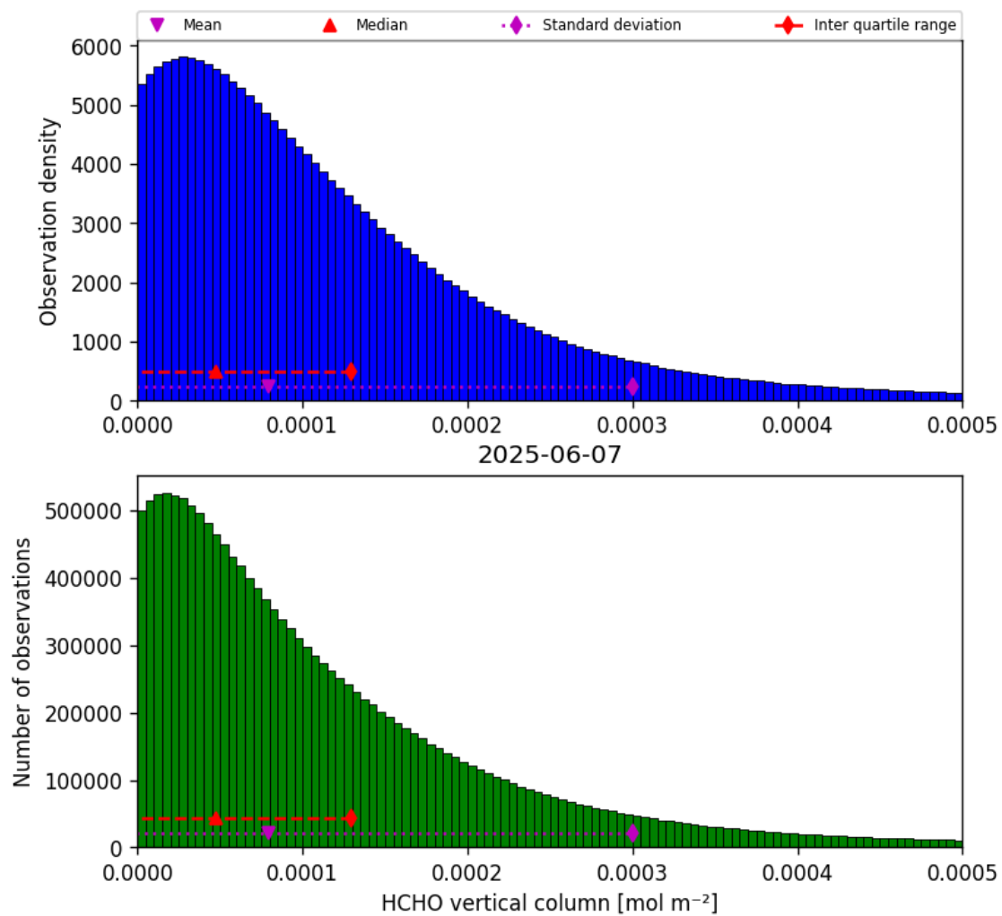
Figure 33: Histogram of “HCHO vertical column” for 2025-06-07 to 2025-06-08
