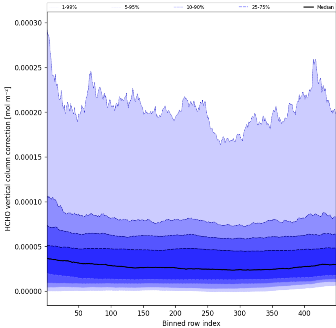
Figure 49: Along track statistics of “HCHO vertical column correction” for 2025-06-07 to 2025-06-08
