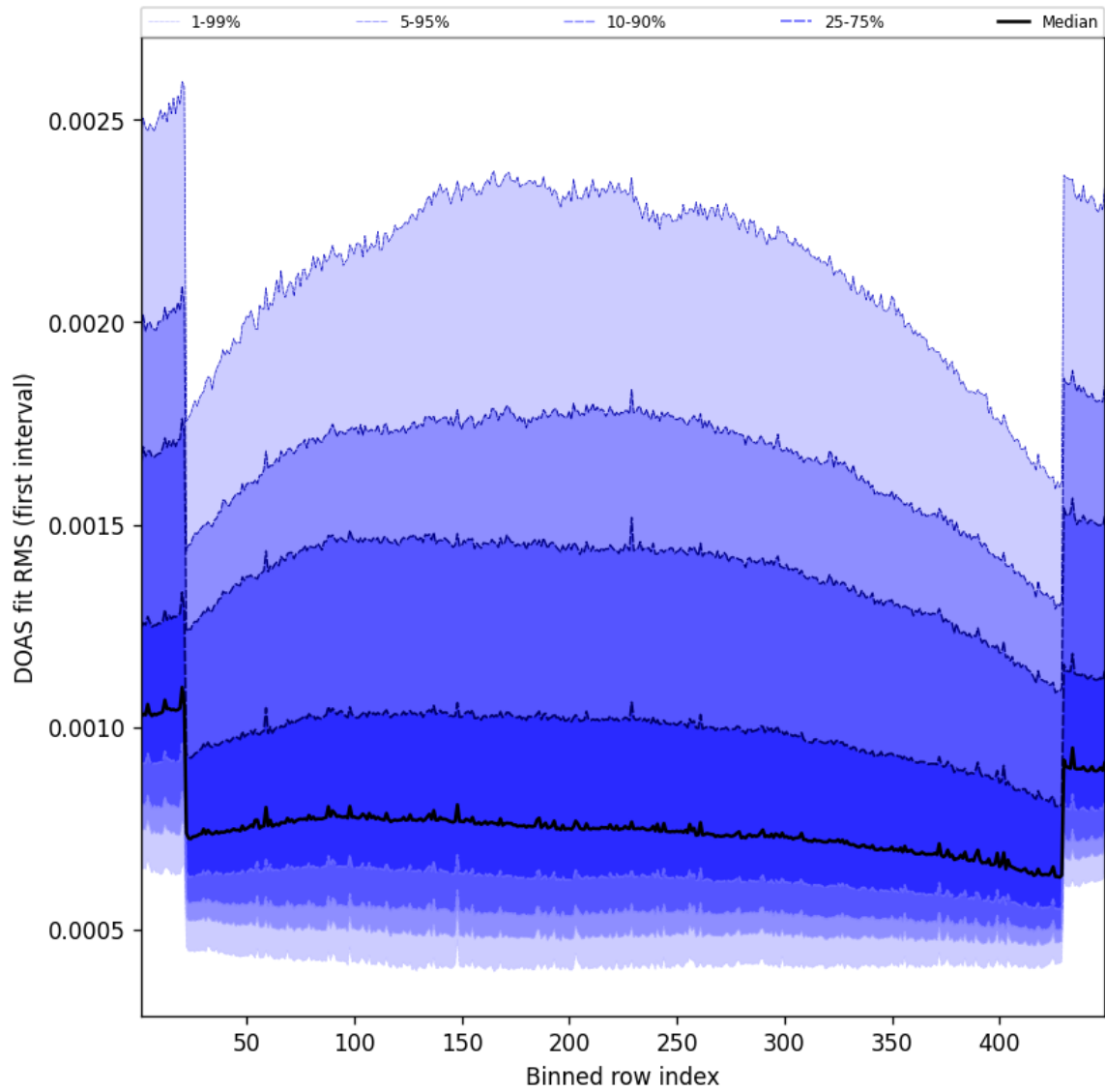
Figure 58: Along track statistics of “DOAS fit RMS (first interval)” for 2025-06-07 to 2025-06-08
