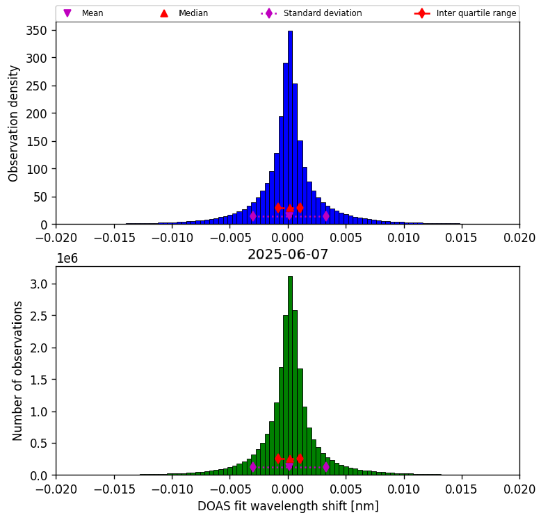
Figure 42: Histogram of “DOAS fit wavelength shift” for 2025-06-07 to 2025-06-08
