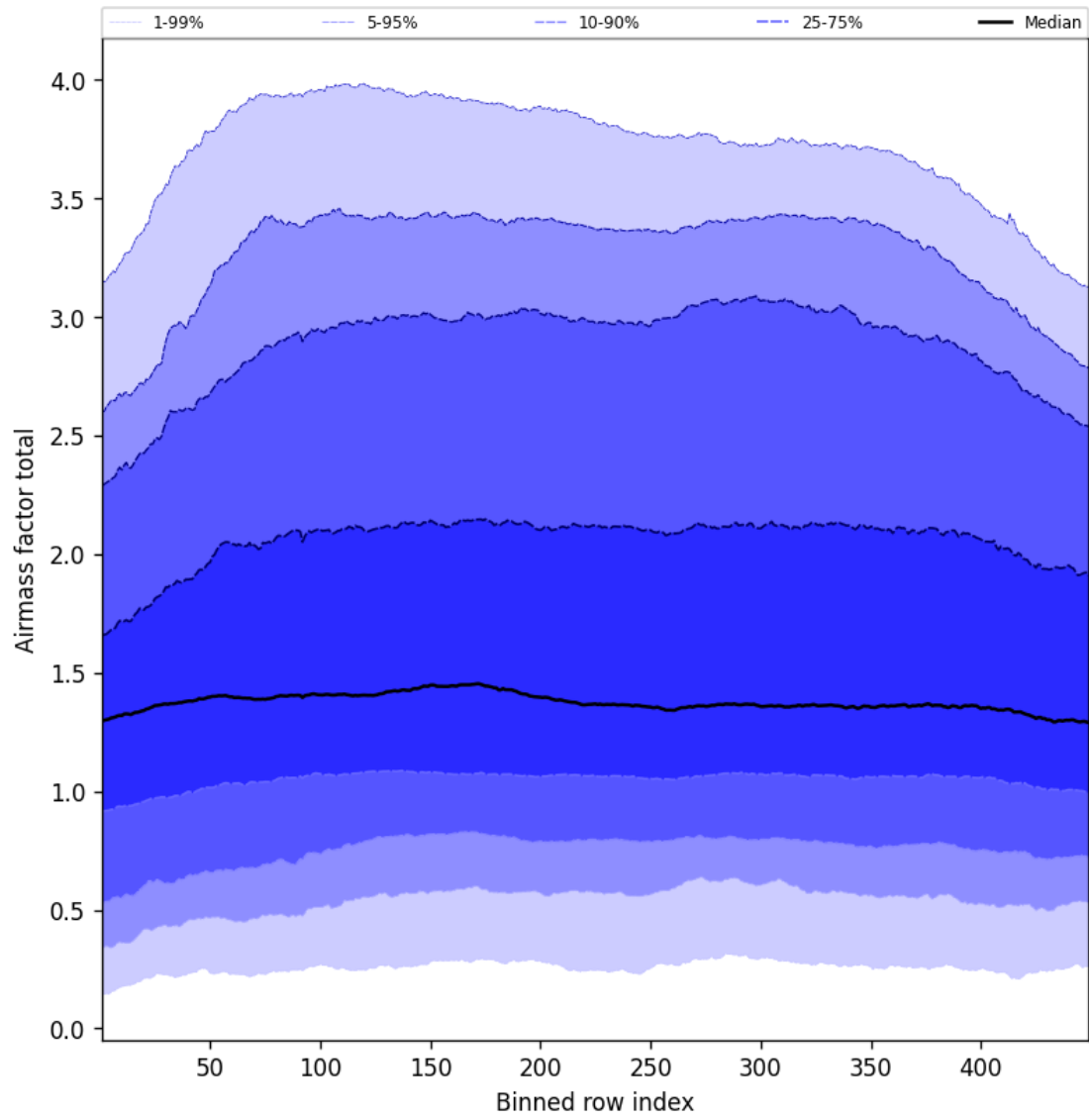
Figure 52: Along track statistics of “Airmass factor total” for 2025-06-07 to 2025-06-08
