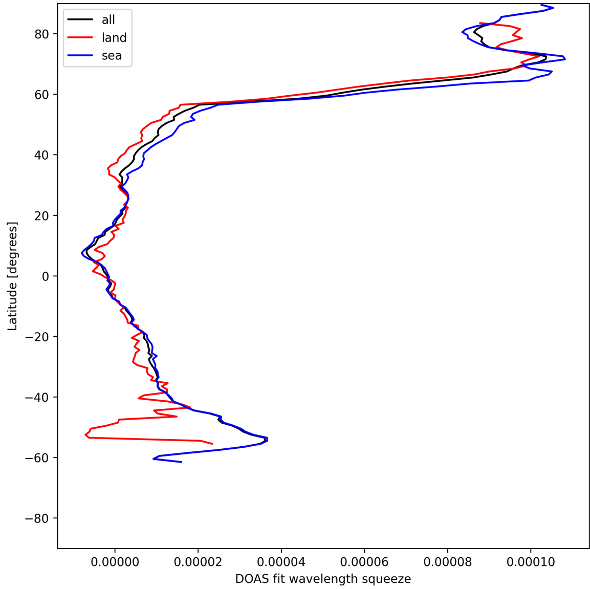
Figure 29: Zonal average of “DOAS fit wavelength squeeze” for 2025-06-07 to 2025-06-08.
