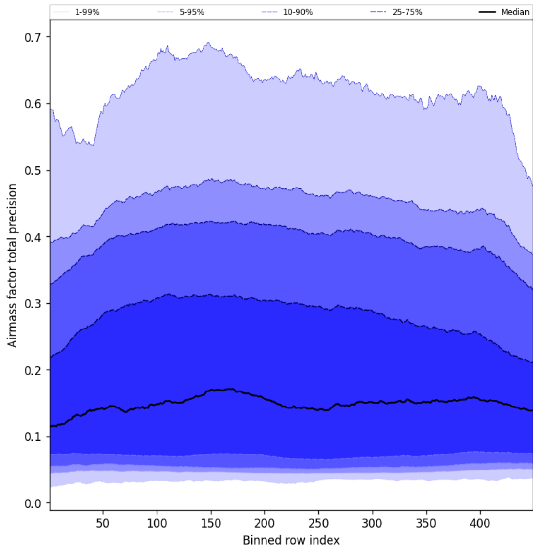
Figure 53: Along track statistics of “Airmass factor total precision” for 2025-06-07 to 2025-06-08
