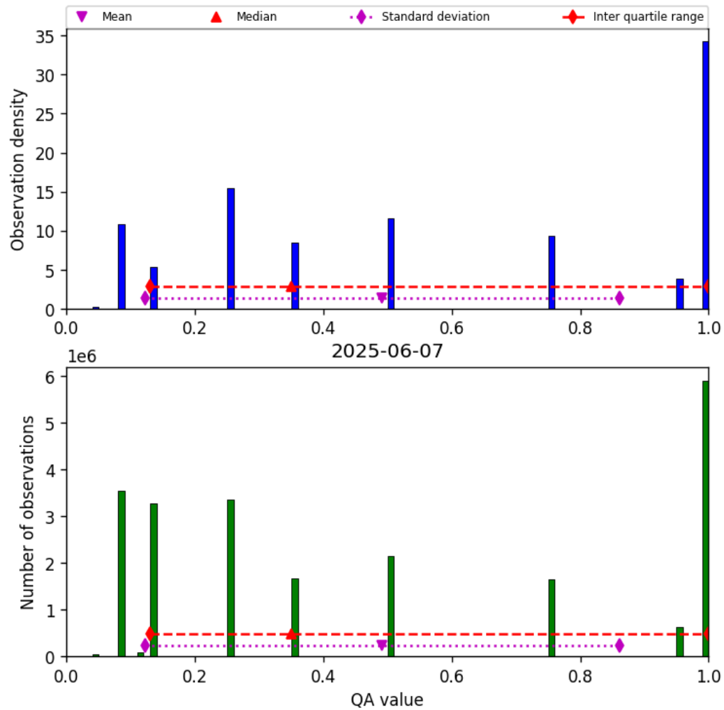
Figure 32: Histogram of “QA value” for 2025-06-07 to 2025-06-08
