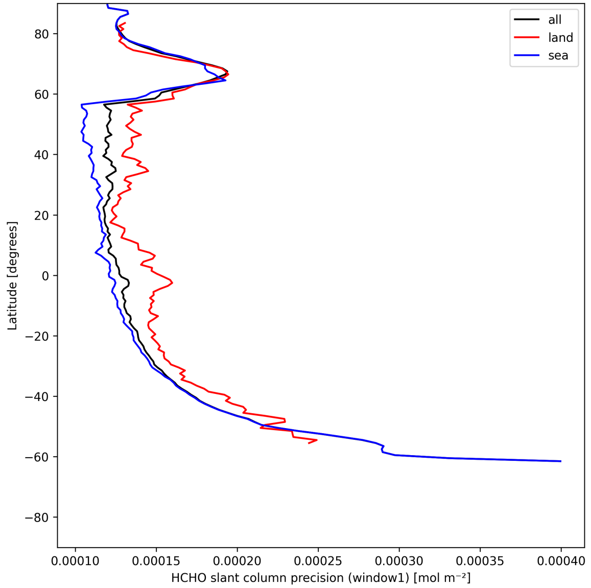
Figure 23: Zonal average of “HCHO slant column precision (window1)” for 2025-06-07 to 2025-06-08.
