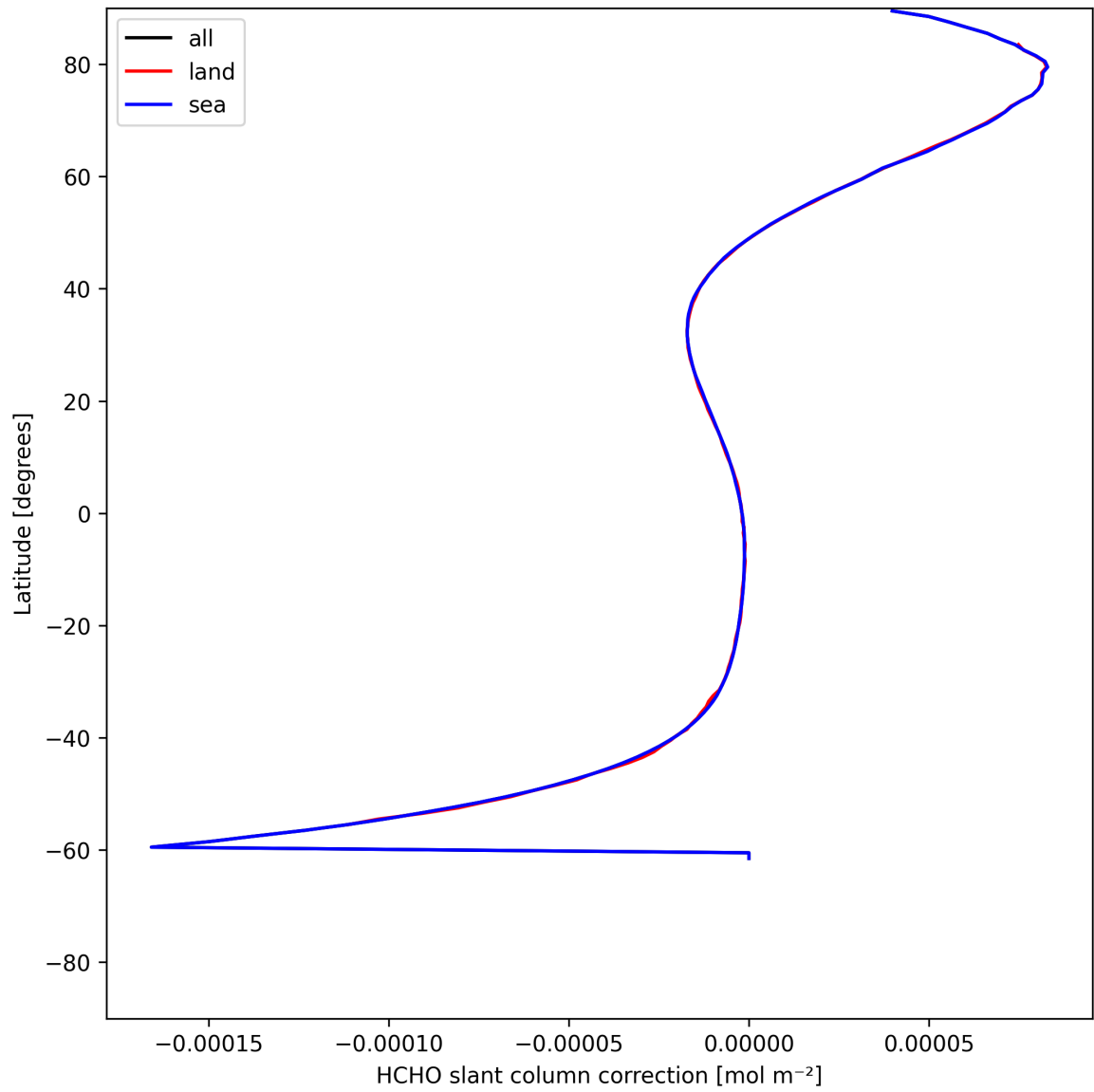
Figure 31: Zonal average of “HCHO slant column correction” for 2025-06-07 to 2025-06-08.
