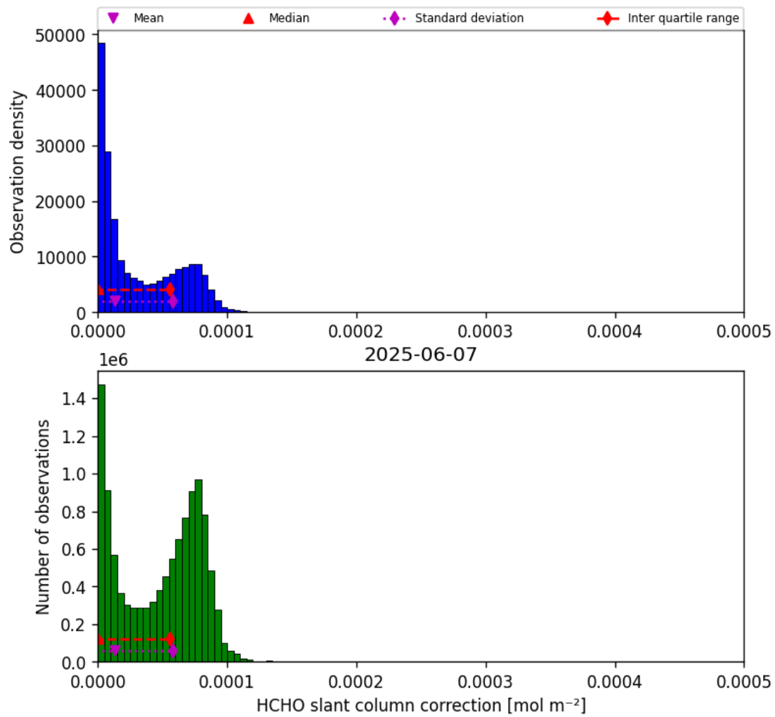
Figure 45: Histogram of “HCHO slant column correction” for 2025-06-07 to 2025-06-08
