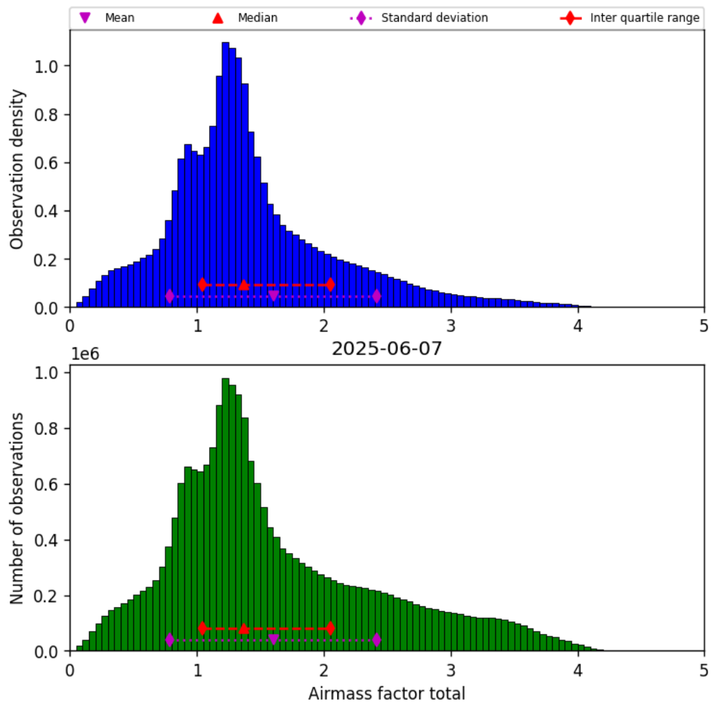
Figure 38: Histogram of “Airmass factor total” for 2025-06-07 to 2025-06-08
