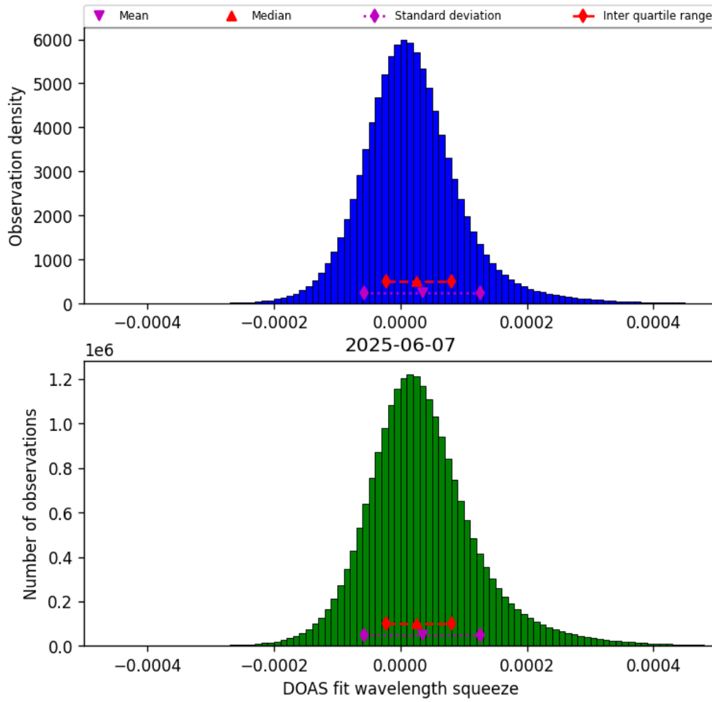
Figure 43: Histogram of “DOAS fit wavelength squeeze” for 2025-06-07 to 2025-06-08
