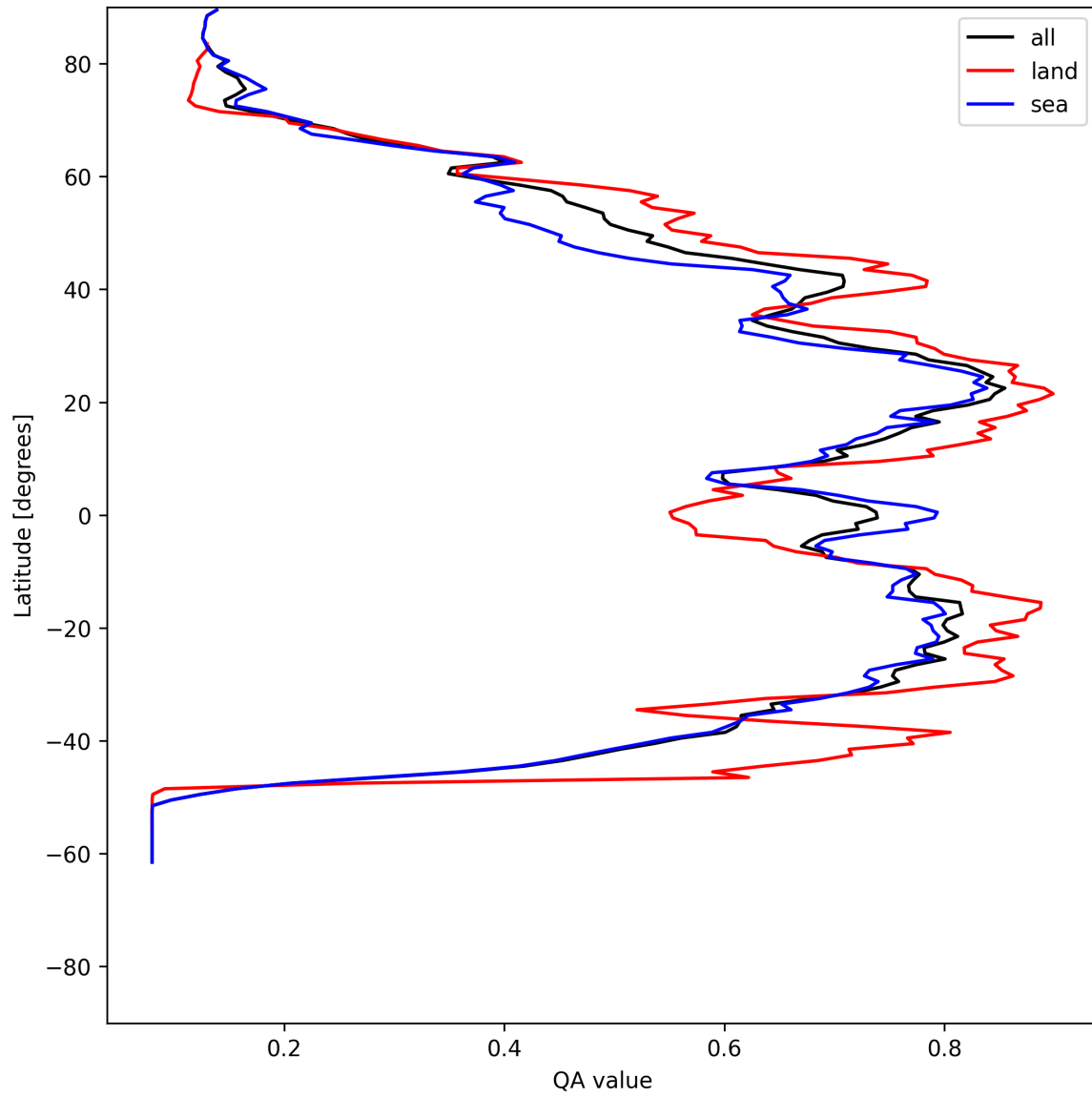
Figure 18: Zonal average of “QA value” for 2025-06-07 to 2025-06-08.
