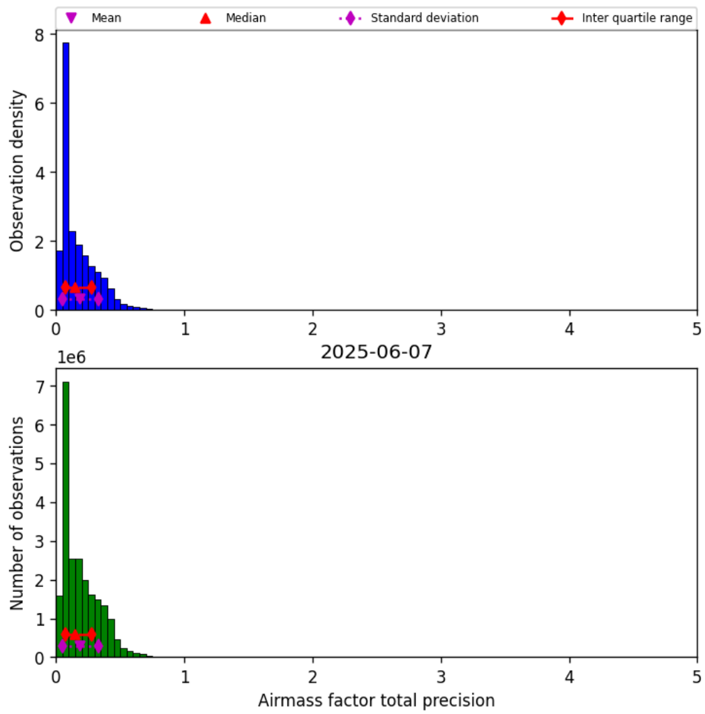
Figure 39: Histogram of “Airmass factor total precision” for 2025-06-07 to 2025-06-08
