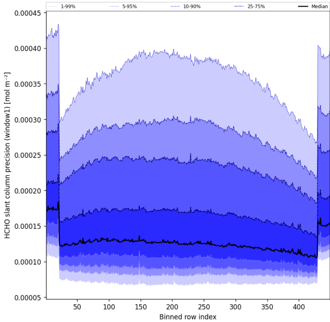
Figure 51: Along track statistics of “HCHO slant column precision (window1)” for 2025-06-07 to 2025-06-08
