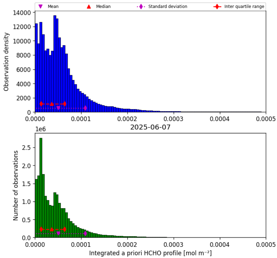
Figure 41: Histogram of “Integrated a priori HCHO profile” for 2025-06-07 to 2025-06-08
