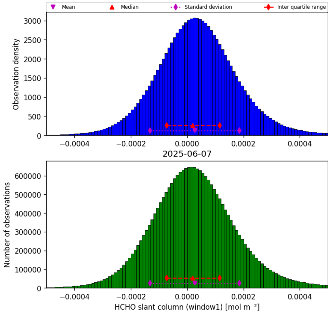
Figure 36: Histogram of “HCHO slant column (window1)” for 2025-06-07 to 2025-06-08
