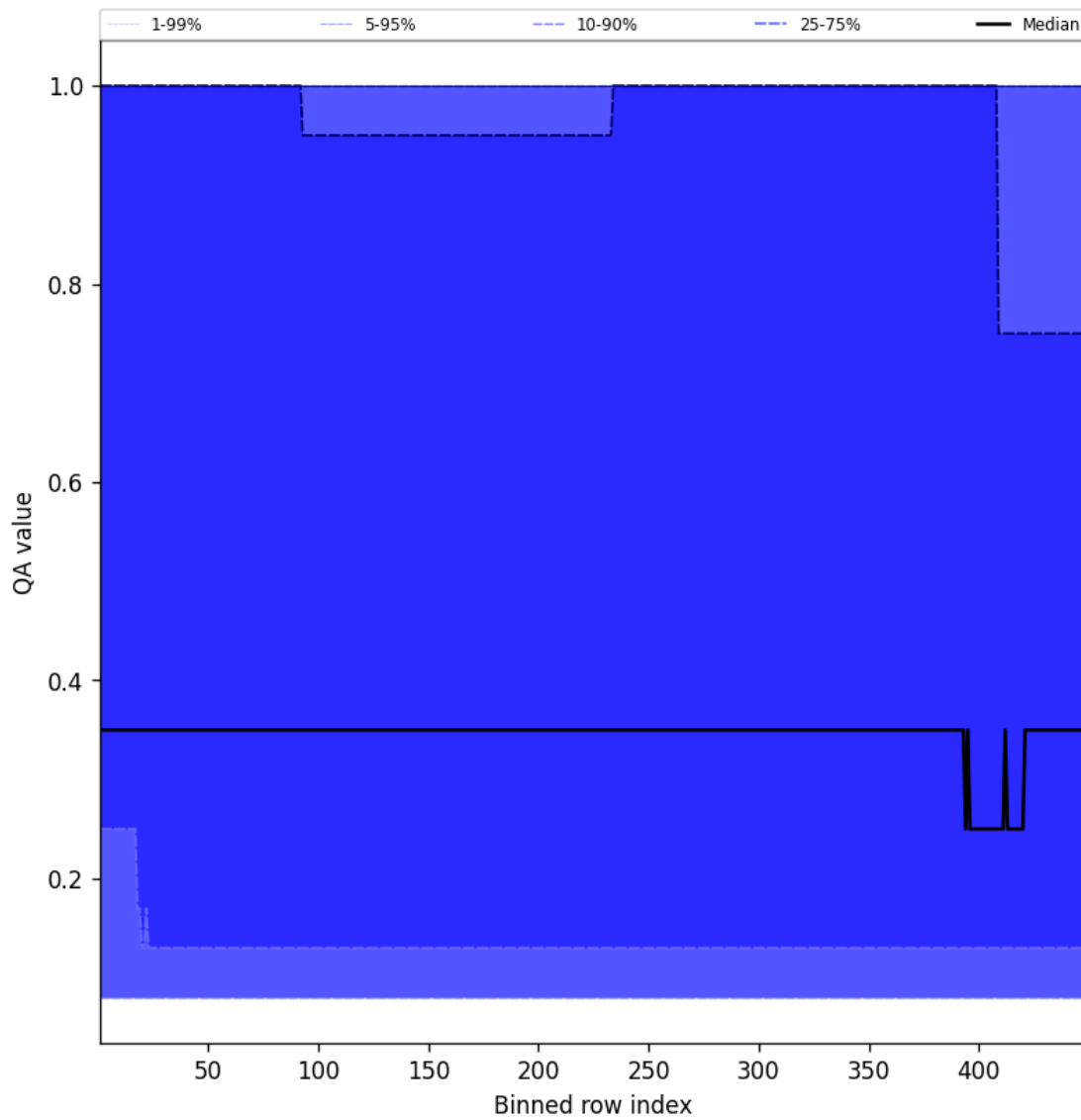
Figure 46: Along track statistics of “QA value” for 2025-06-07 to 2025-06-08
