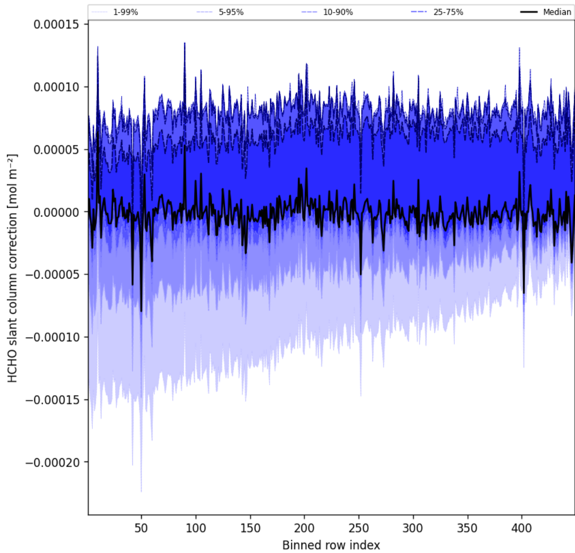
Figure 59: Along track statistics of “HCHO slant column correction” for 2025-06-07 to 2025-06-08
