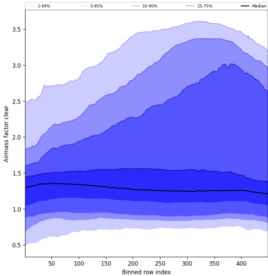
Figure 54: Along track statistics of “Airmass factor clear” for 2025-06-07 to 2025-06-08
