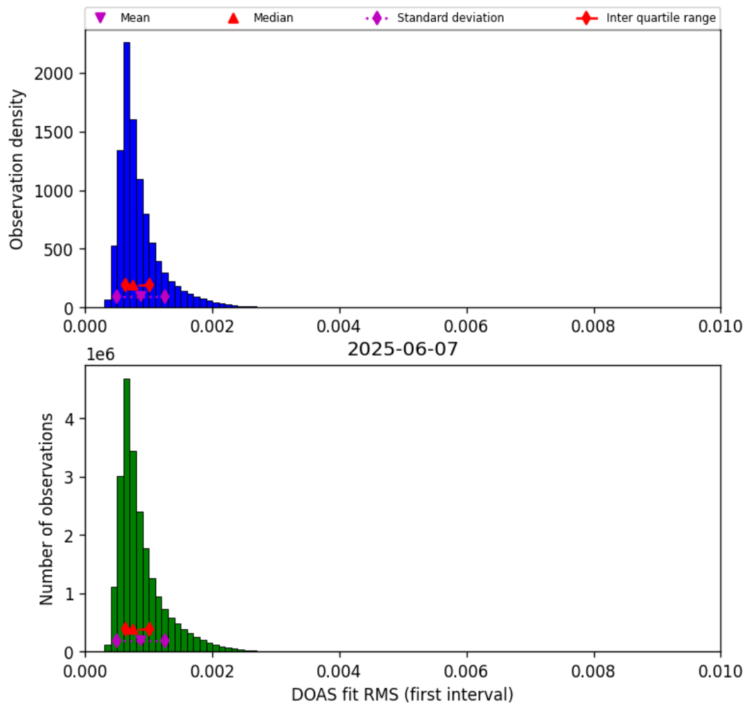
Figure 44: Histogram of “DOAS fit RMS (first interval)” for 2025-06-07 to 2025-06-08
