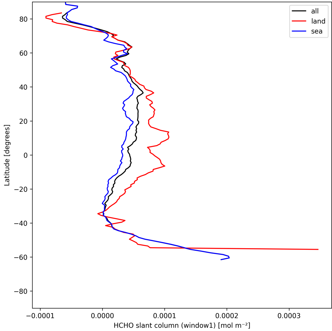
Figure 22: Zonal average of “HCHO slant column (window1)” for 2025-06-07 to 2025-06-08.
