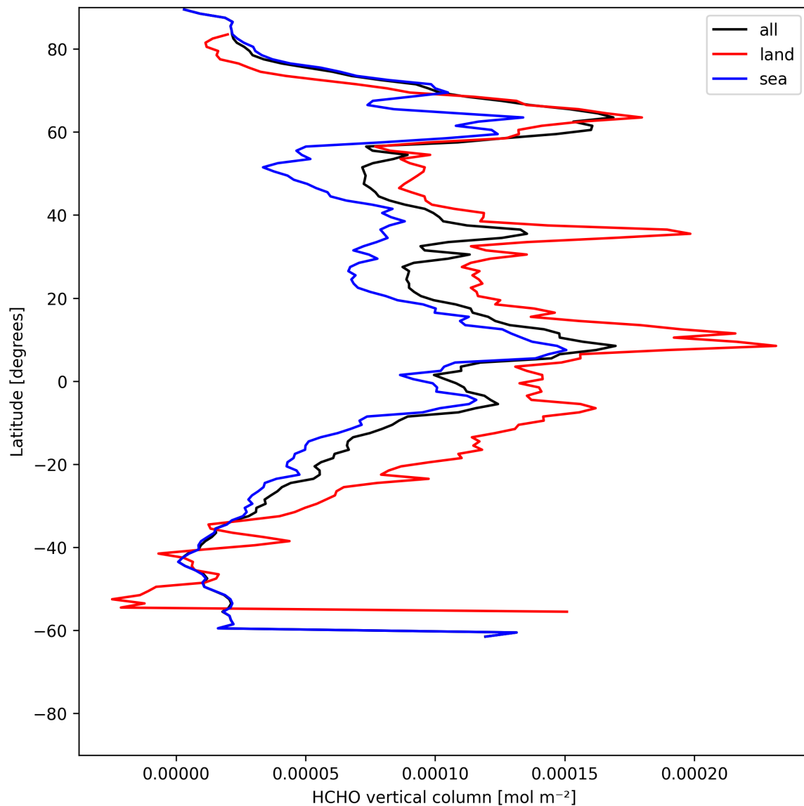
Figure 19: Zonal average of “HCHO vertical column” for 2025-06-07 to 2025-06-08.
