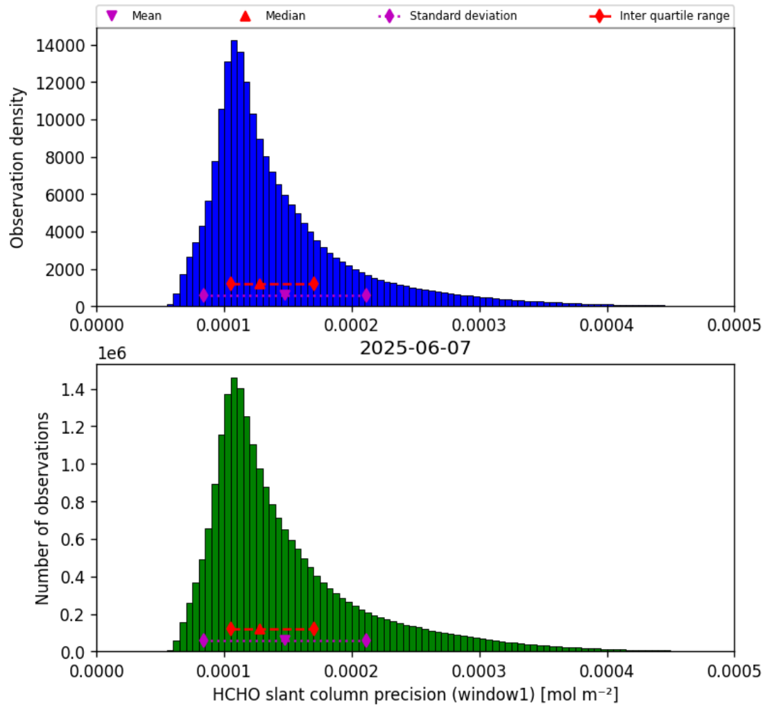
Figure 37: Histogram of “HCHO slant column precision (window1)” for 2025-06-07 to 2025-06-08
