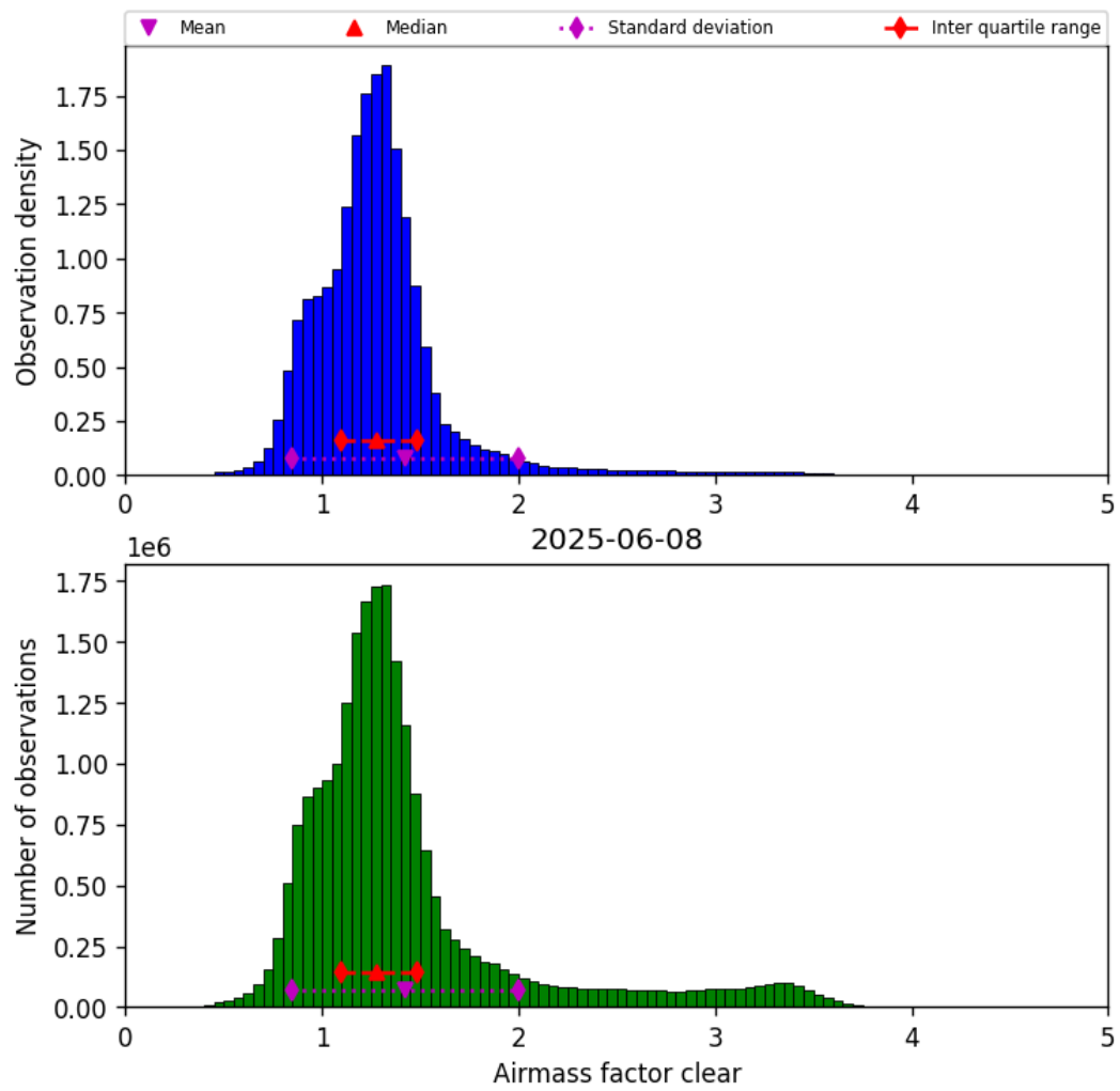
Figure 40: Histogram of “Airmass factor clear” for 2025-06-08 to 2025-06-09
