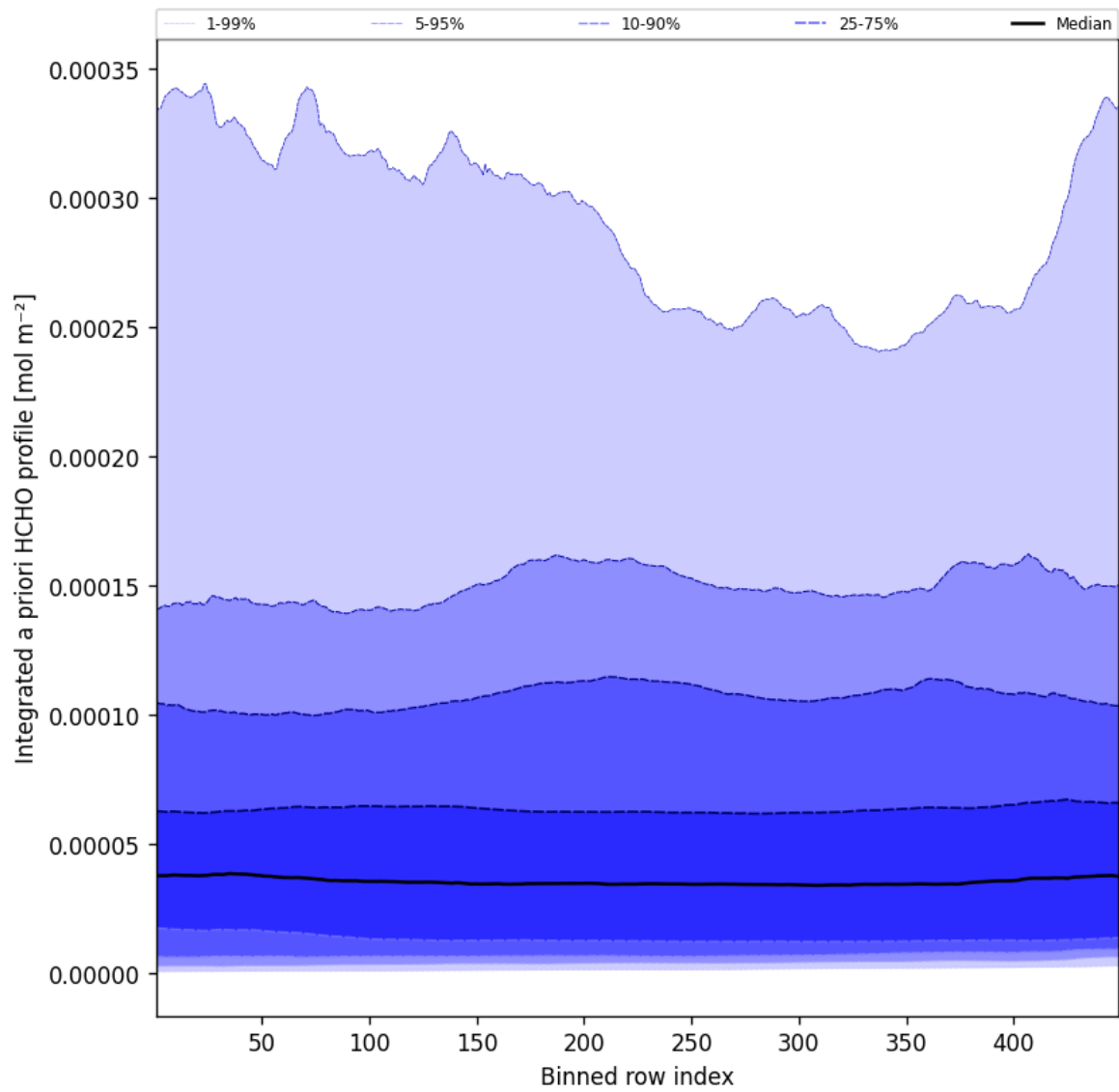
Figure 55: Along track statistics of "Integrated a priori HCHO profile" for 2025-06-08 to 2025-06-09
