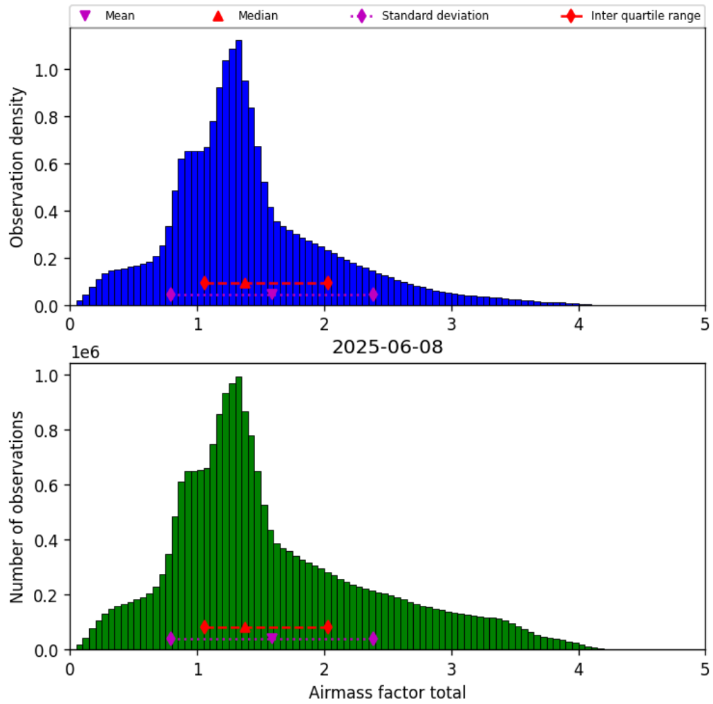
Figure 38: Histogram of “Airmass factor total” for 2025-06-08 to 2025-06-09
