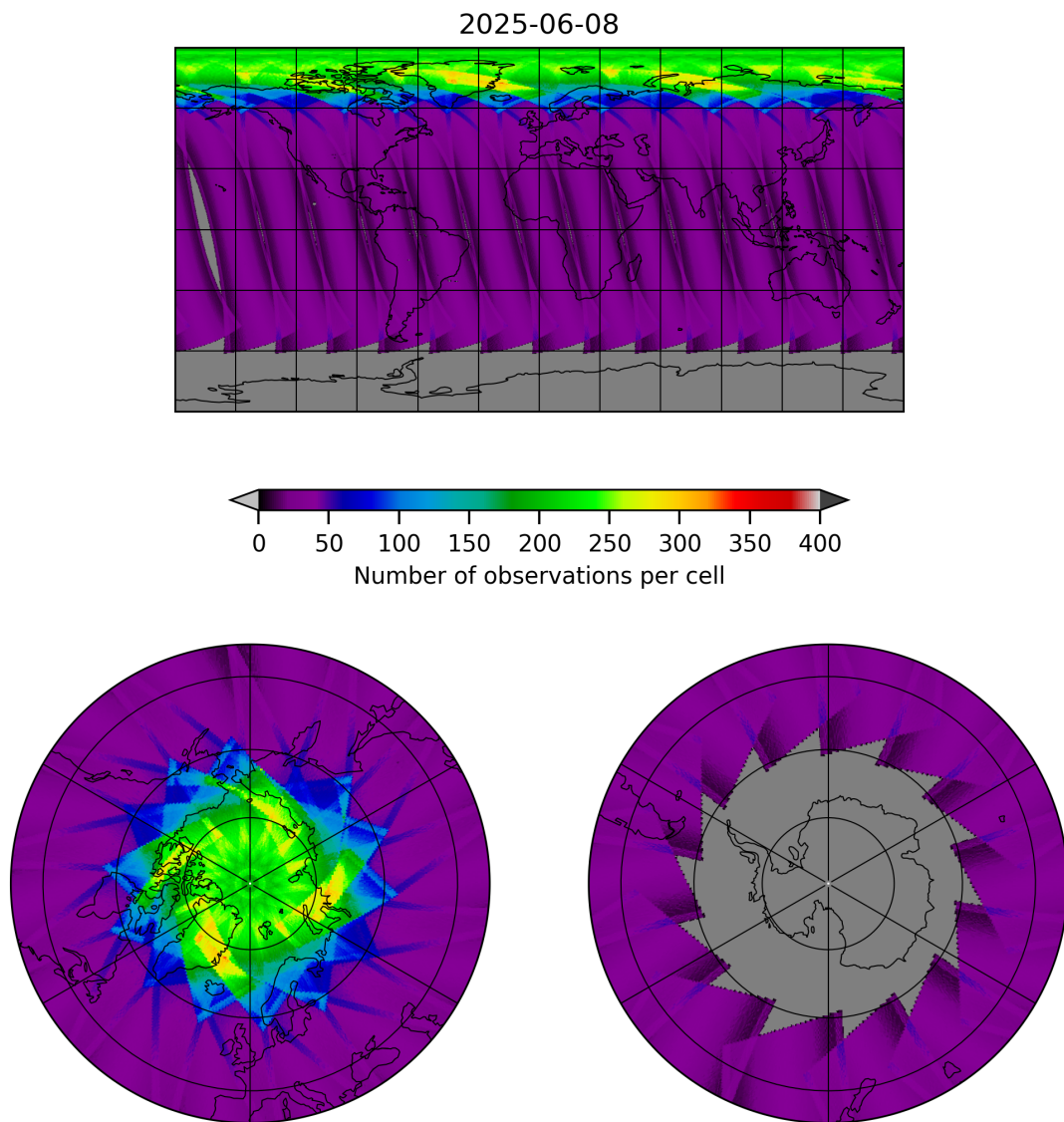
Figure 17: Map of the number of observations for 2025-06-08 to 2025-06-09
