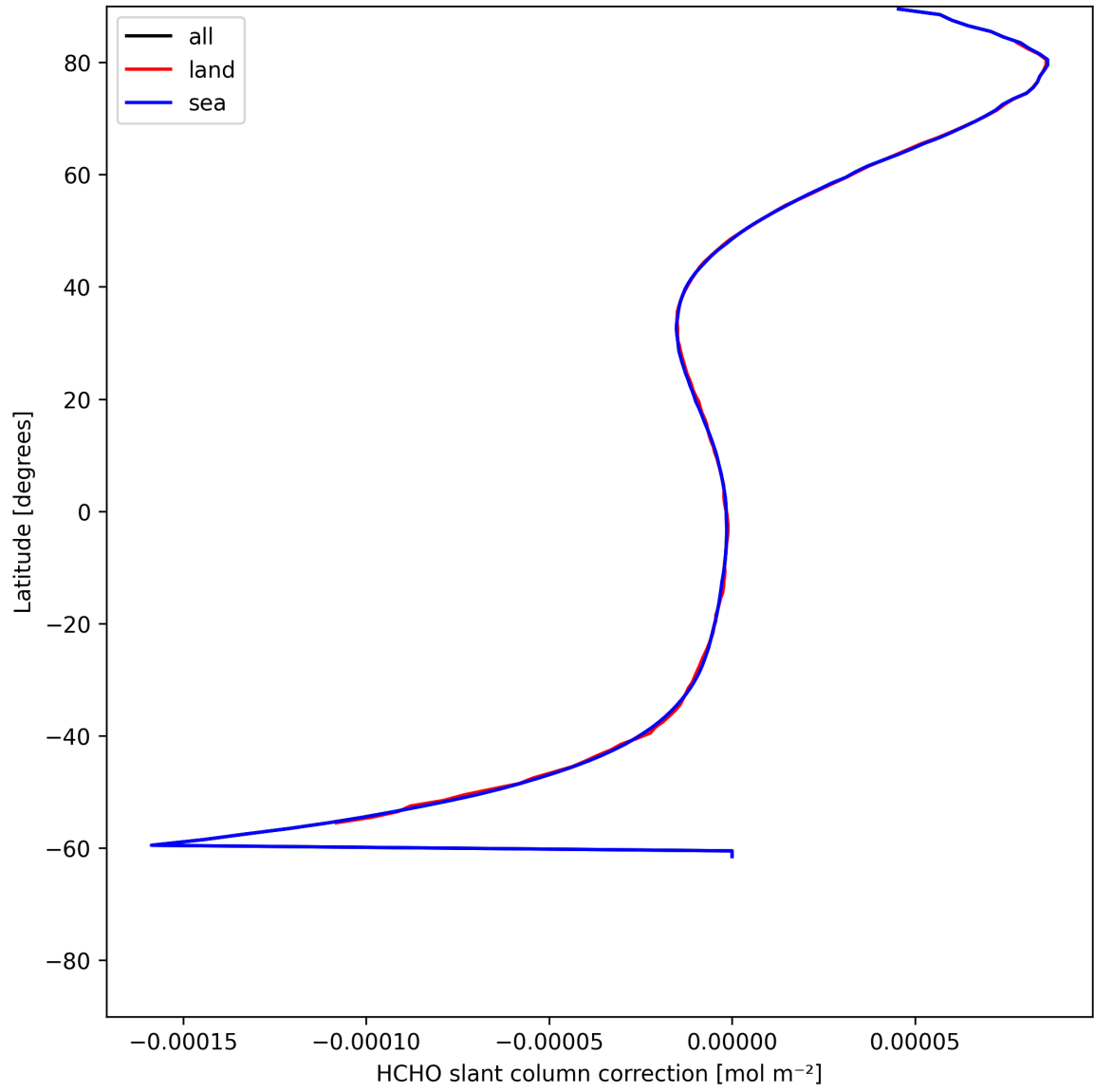
Figure 31: Zonal average of “HCHO slant column correction” for 2025-06-08 to 2025-06-09.
