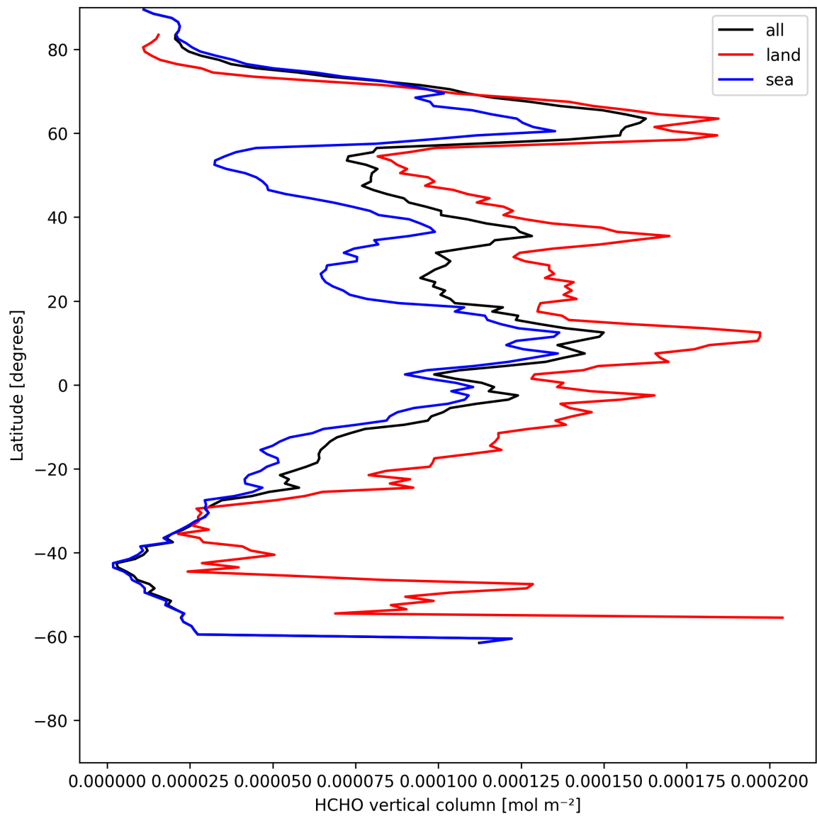
Figure 19: Zonal average of “HCHO vertical column” for 2025-06-08 to 2025-06-09.
