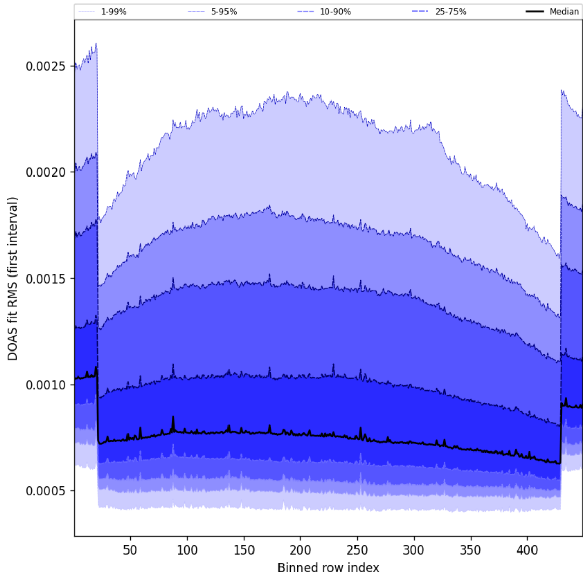
Figure 58: Along track statistics of “DOAS fit RMS (first interval)” for 2025-06-08 to 2025-06-09
