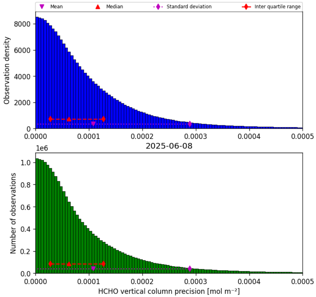
Figure 34: Histogram of “HCHO vertical column precision” for 2025-06-08 to 2025-06-09
