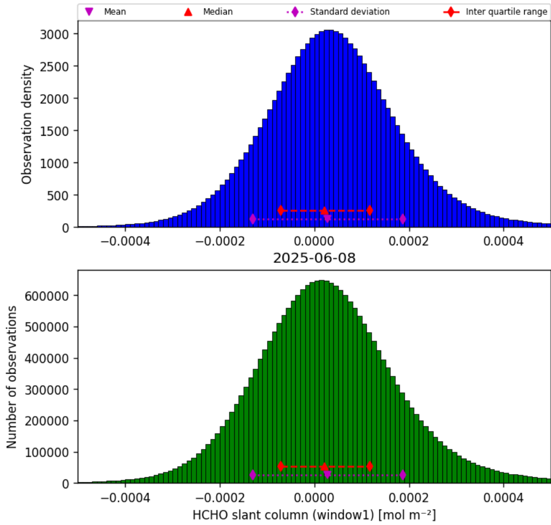
Figure 36: Histogram of “HCHO slant column (window1)” for 2025-06-08 to 2025-06-09
