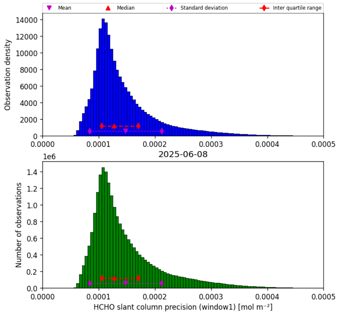
Figure 37: Histogram of “HCHO slant column precision (window1)” for 2025-06-08 to 2025-06-09
