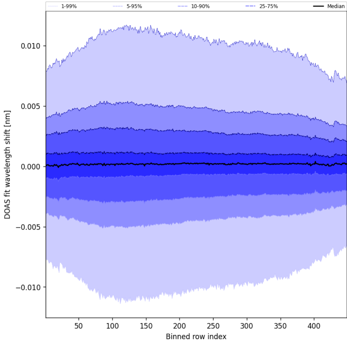
Figure 56: Along track statistics of “DOAS fit wavelength shift” for 2025-06-08 to 2025-06-09
