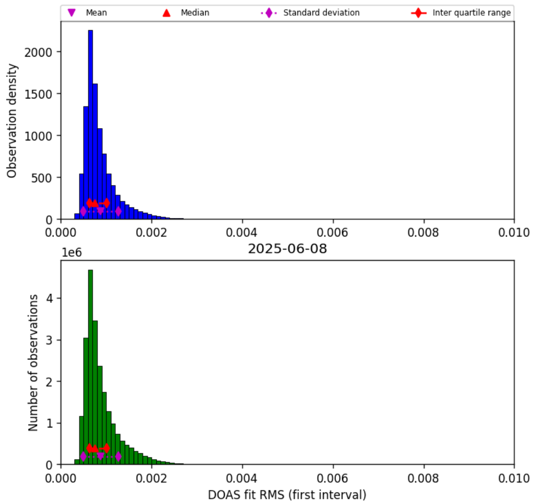
Figure 44: Histogram of “DOAS fit RMS (first interval)” for 2025-06-08 to 2025-06-09
