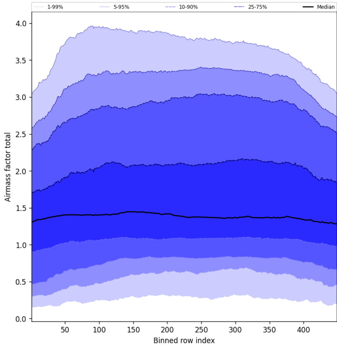
Figure 52: Along track statistics of “Airmass factor total” for 2025-06-08 to 2025-06-09
