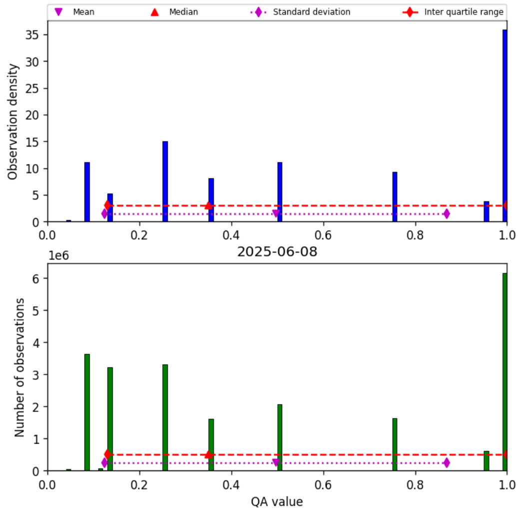
Figure 32: Histogram of “QA value” for 2025-06-08 to 2025-06-09
