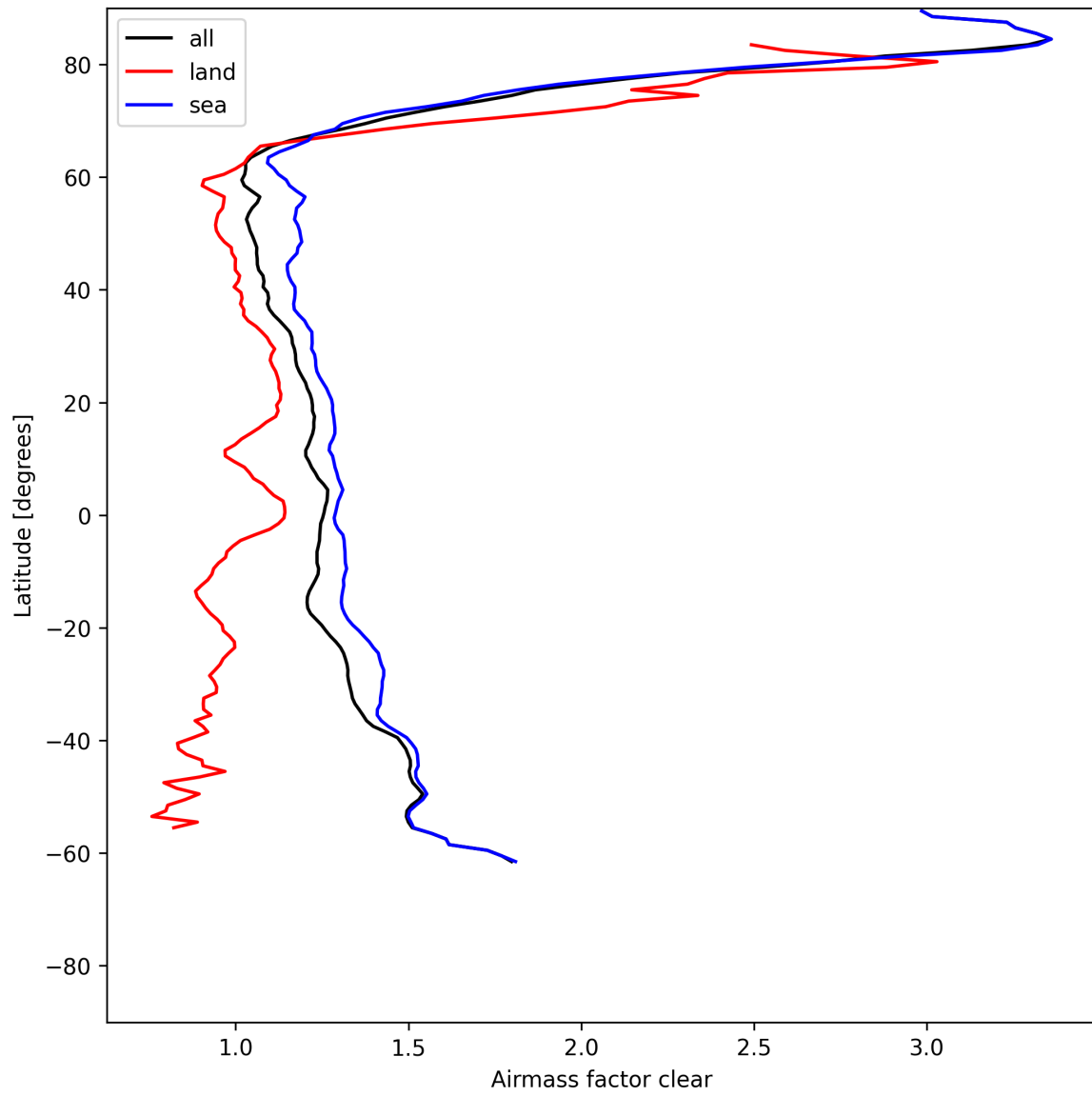
Figure 26: Zonal average of “Airmass factor clear” for 2025-06-08 to 2025-06-09.
