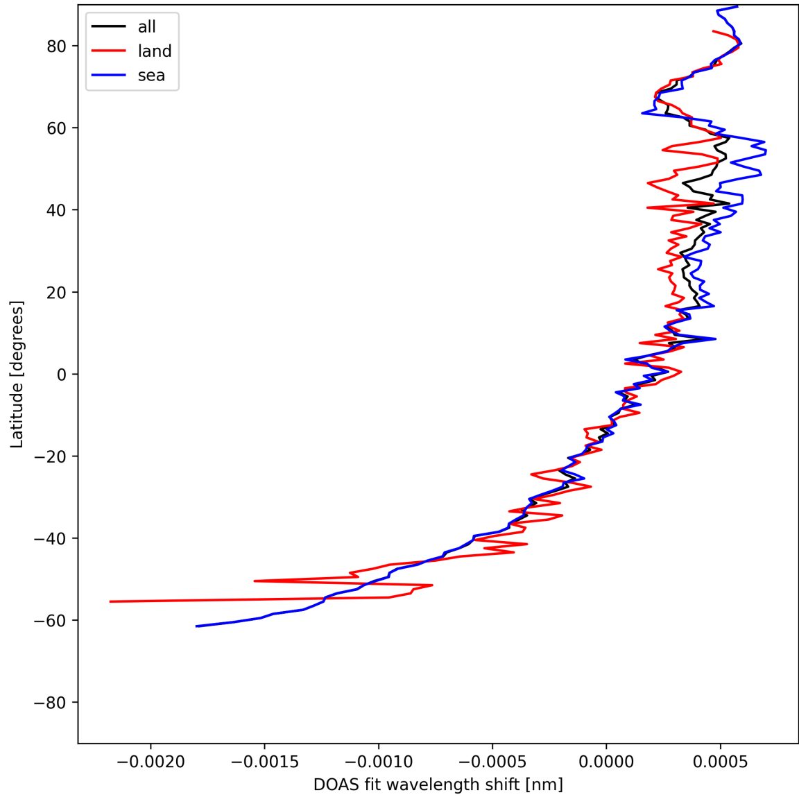
Figure 28: Zonal average of “DOAS fit wavelength shift” for 2025-06-08 to 2025-06-09.
