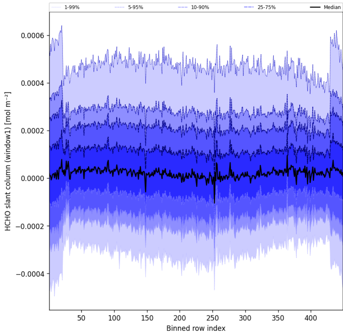
Figure 50: Along track statistics of “HCHO slant column (window1)” for 2025-06-08 to 2025-06-09
