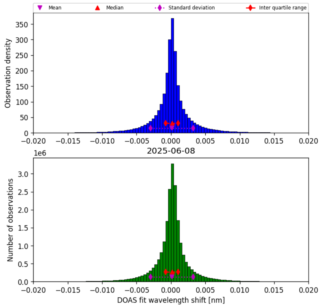
Figure 42: Histogram of “DOAS fit wavelength shift” for 2025-06-08 to 2025-06-09
