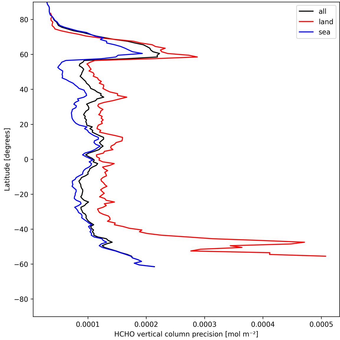
Figure 20: Zonal average of "HCHO vertical column precision" for 2025-06-08 to 2025-06-09.
