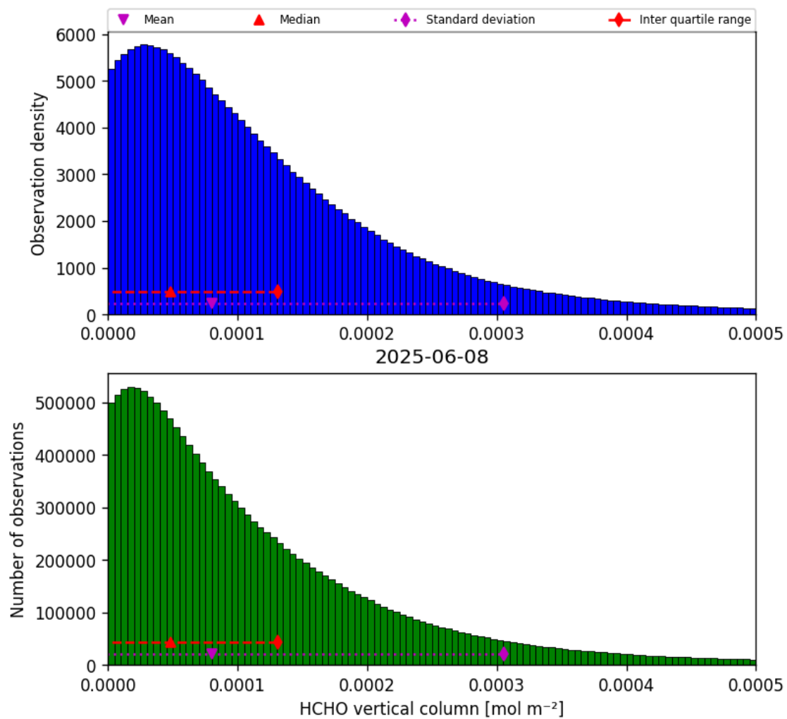
Figure 33: Histogram of “HCHO vertical column” for 2025-06-08 to 2025-06-09
