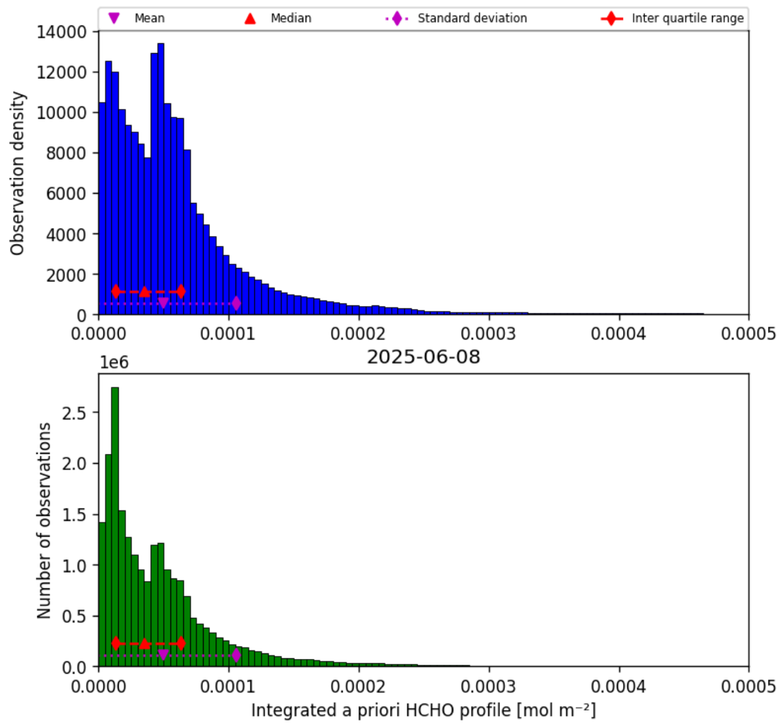
Figure 41: Histogram of “Integrated a priori HCHO profile” for 2025-06-08 to 2025-06-09
