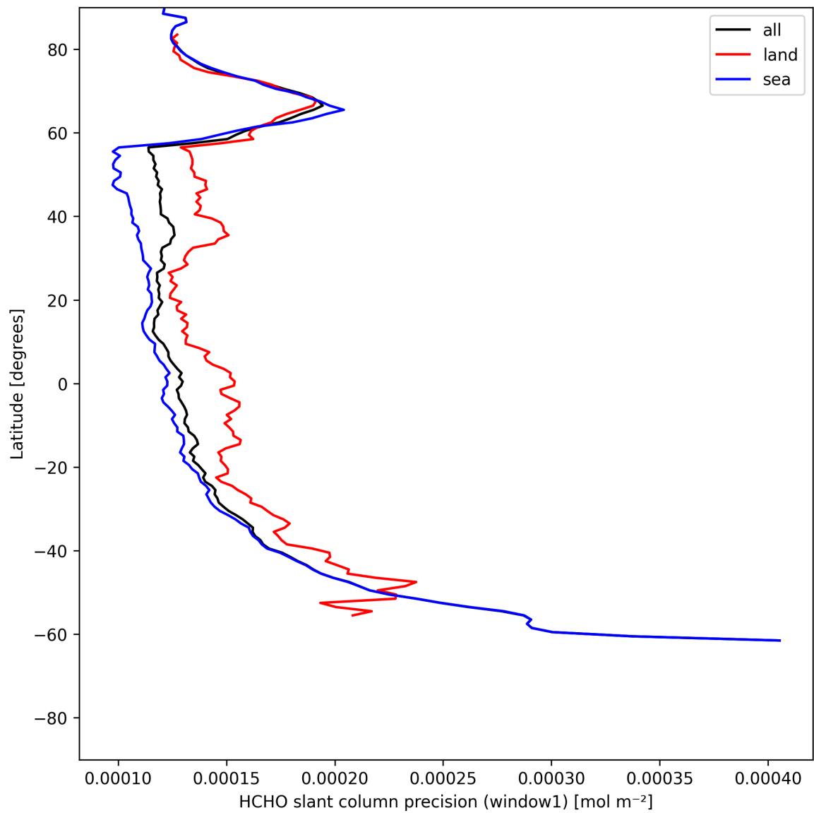
Figure 23: Zonal average of “HCHO slant column precision (window1)” for 2025-06-08 to 2025-06-09.
