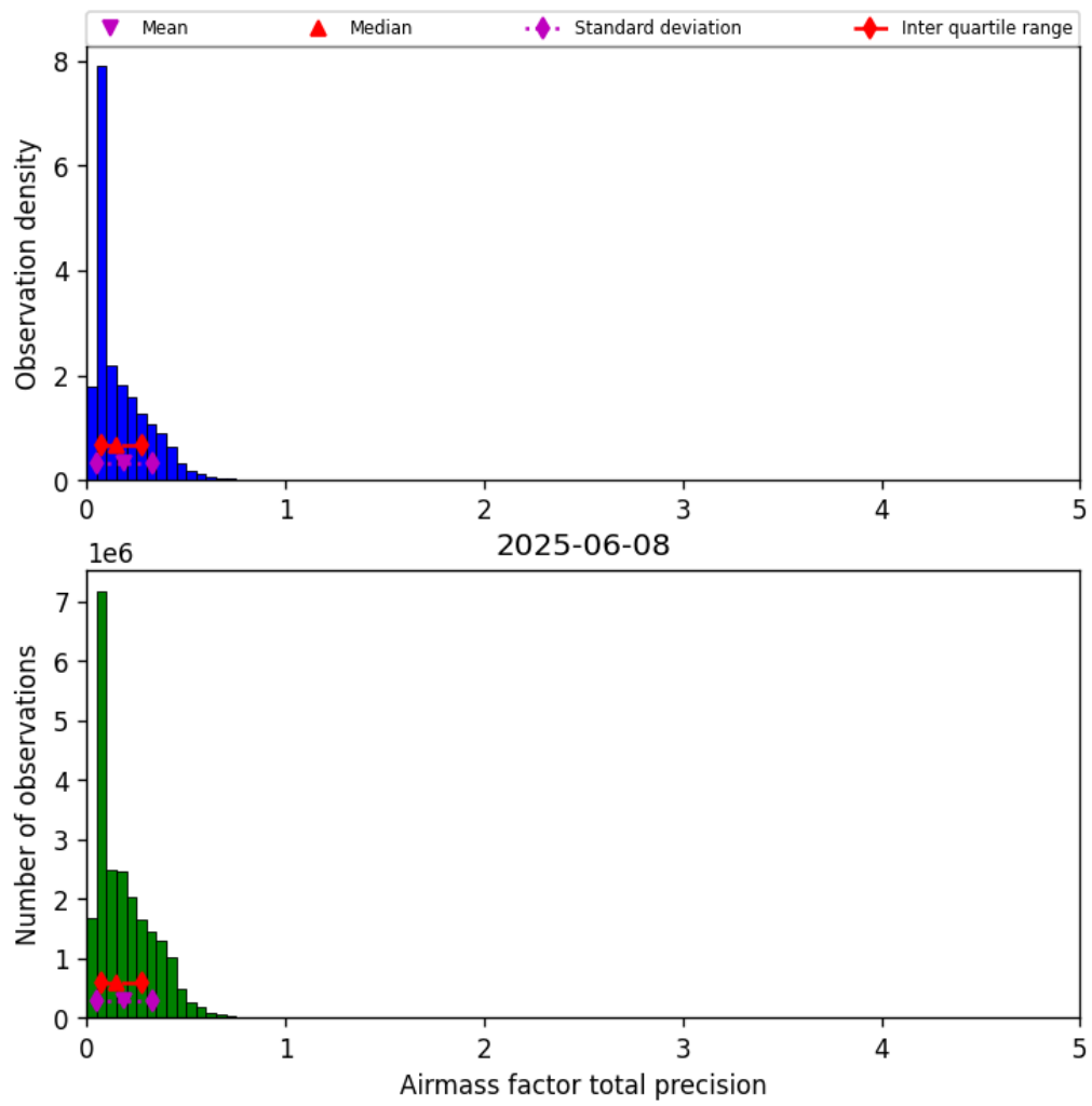
Figure 39: Histogram of “Airmass factor total precision” for 2025-06-08 to 2025-06-09
