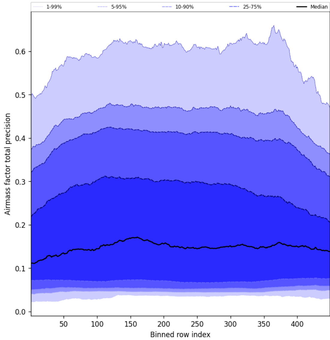
Figure 53: Along track statistics of “Airmass factor total precision” for 2025-06-08 to 2025-06-09
