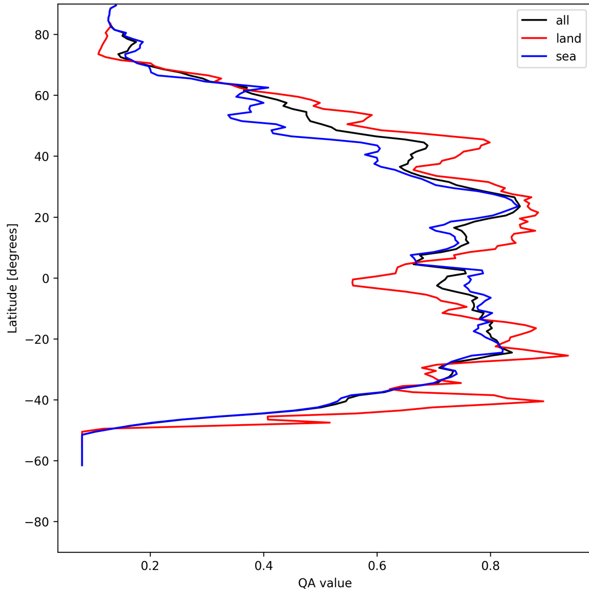
Figure 18: Zonal average of “QA value” for 2025-06-08 to 2025-06-09.
