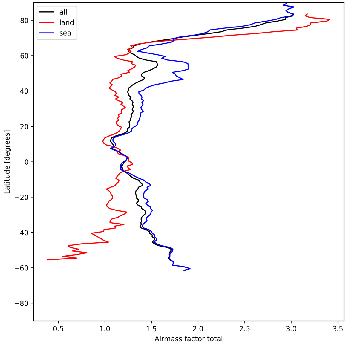
Figure 24: Zonal average of “Airmass factor total” for 2025-06-08 to 2025-06-09.
