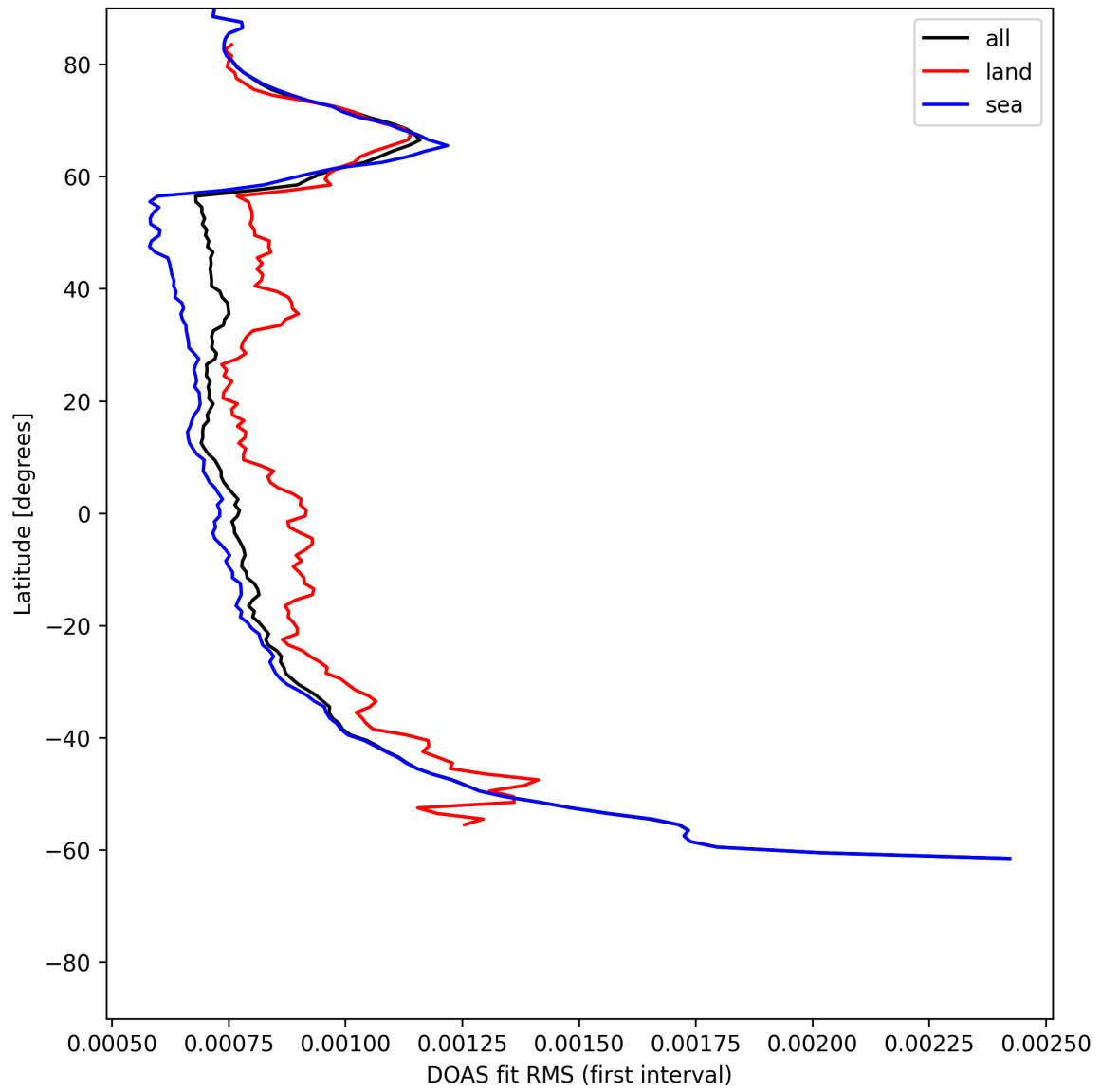
Figure 30: Zonal average of “DOAS fit RMS (first interval)” for 2025-06-08 to 2025-06-09.
