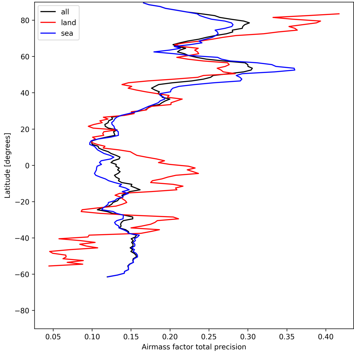
Figure 25: Zonal average of “Airmass factor total precision” for 2025-06-08 to 2025-06-09.
