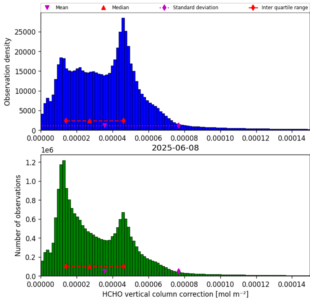
Figure 35: Histogram of “HCHO vertical column correction” for 2025-06-08 to 2025-06-09
