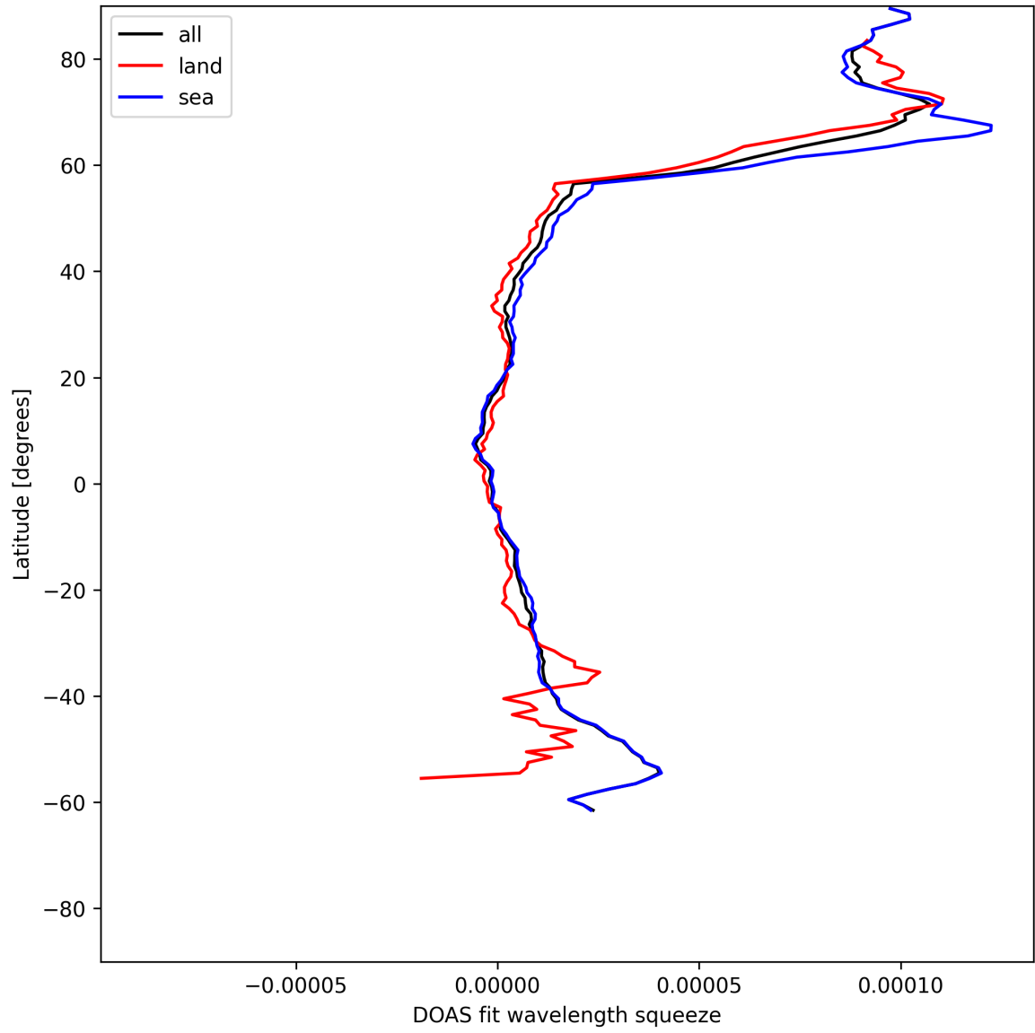
Figure 29: Zonal average of “DOAS fit wavelength squeeze” for 2025-06-08 to 2025-06-09.
