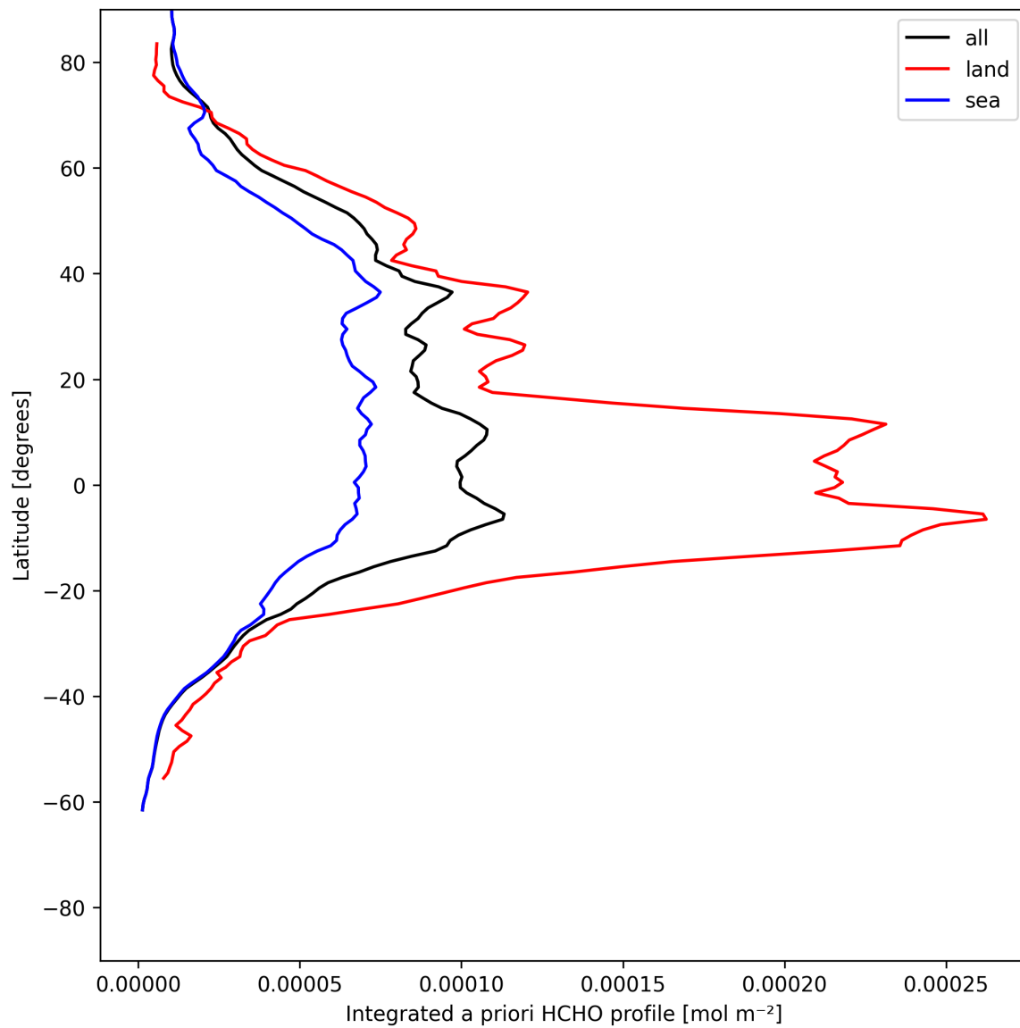
Figure 27: Zonal average of “Integrated a priori HCHO profile” for 2025-06-08 to 2025-06-09.
