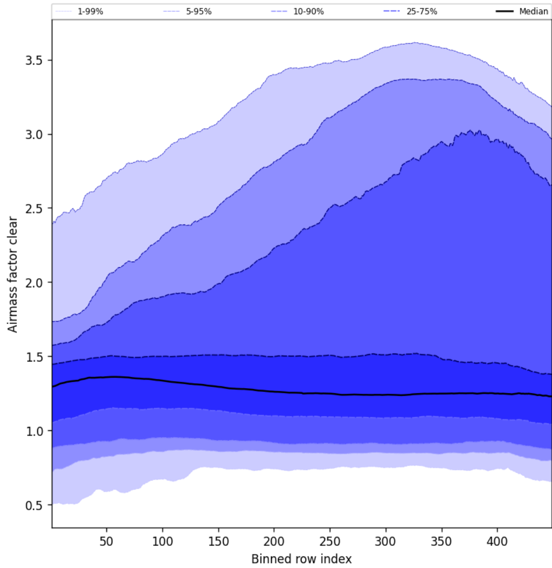
Figure 54: Along track statistics of “Air mass factor clear” for 2025-06-08 to 2025-06-09
