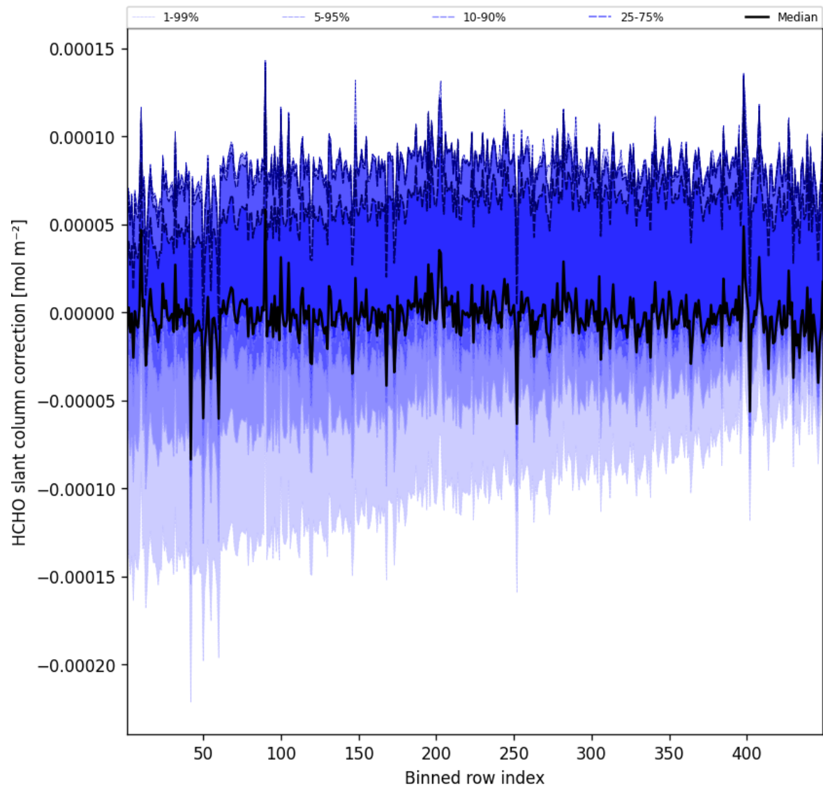
Figure 59: Along track statistics of “HCHO slant column correction” for 2025-06-08 to 2025-06-09
