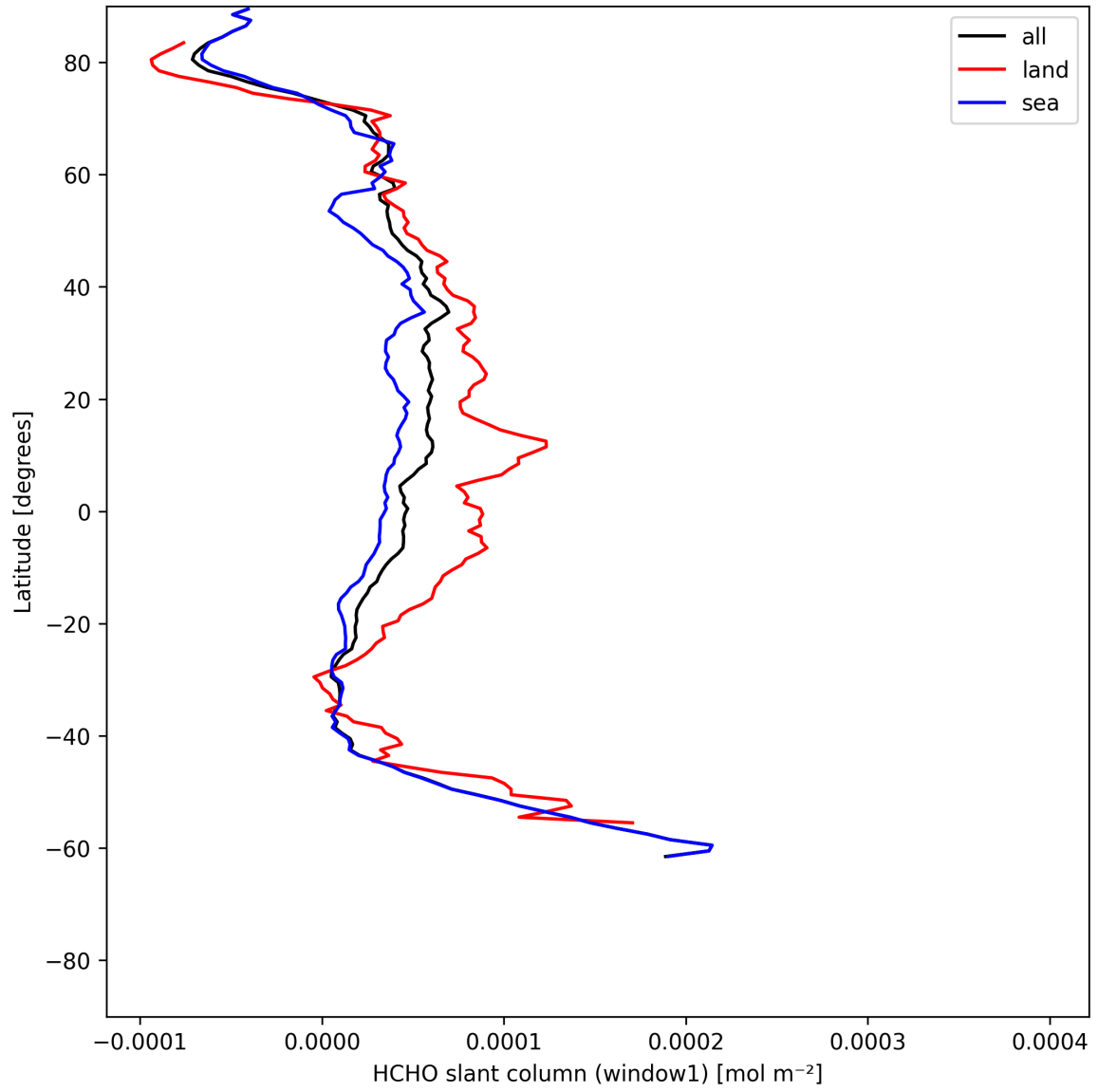
Figure 22: Zonal average of “HCHO slant column (window1)” for 2025-06-08 to 2025-06-09.
