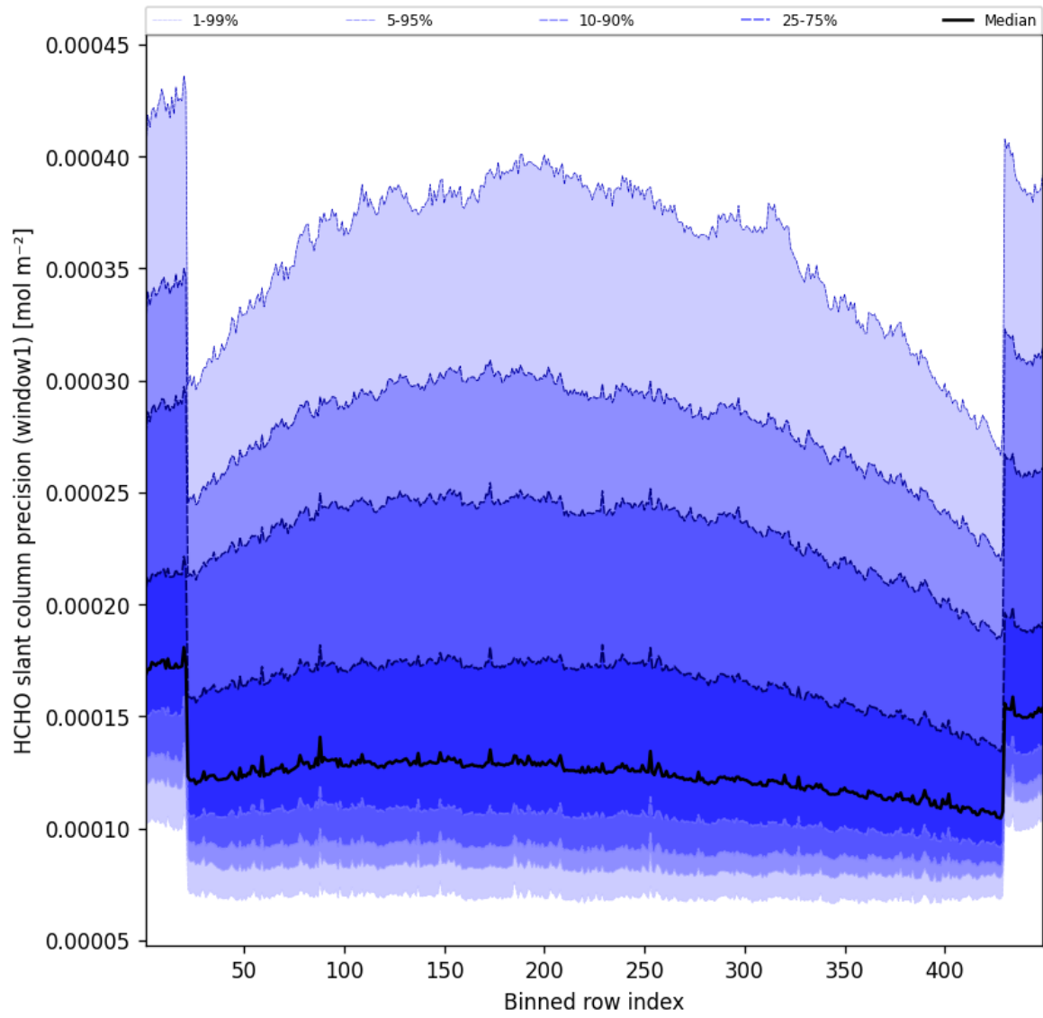
Figure 51: Along track statistics of “HCHO slant column precision (window1)” for 2025-06-08 to 2025-06-09
