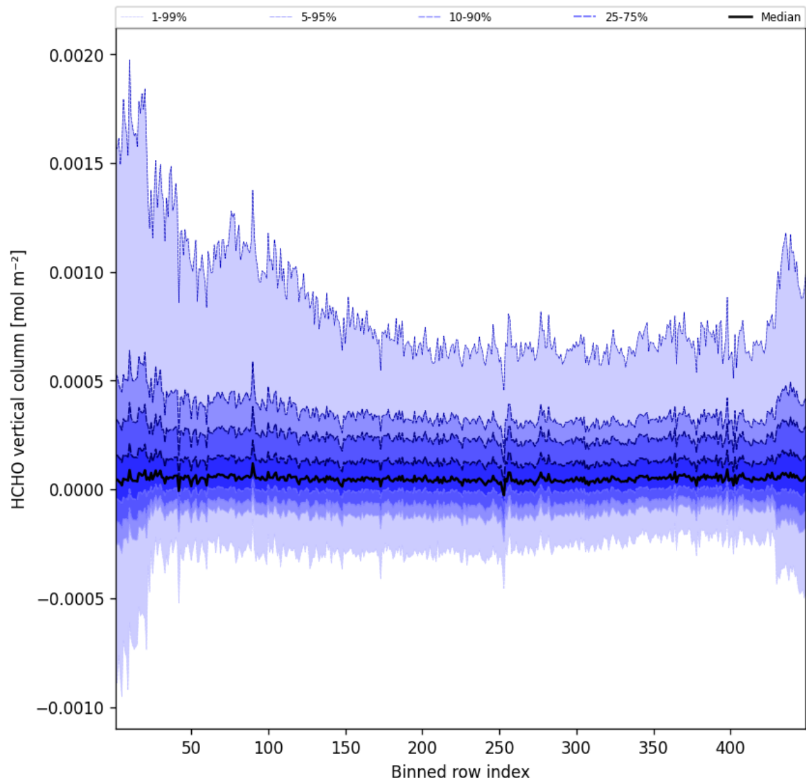
Figure 47: Along track statistics of “HCHO vertical column” for 2025-06-08 to 2025-06-09
