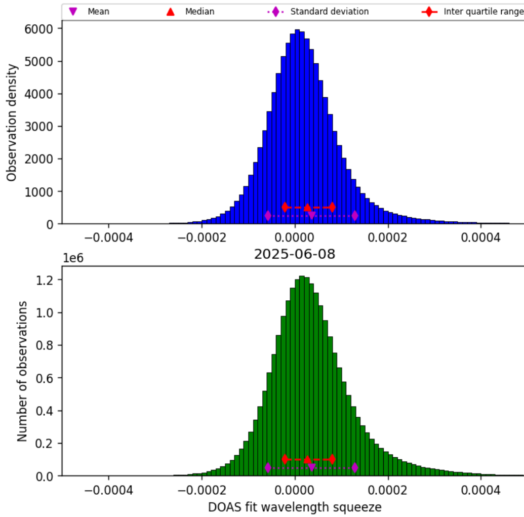
Figure 43: Histogram of “DOAS fit wavelength squeeze” for 2025-06-08 to 2025-06-09
