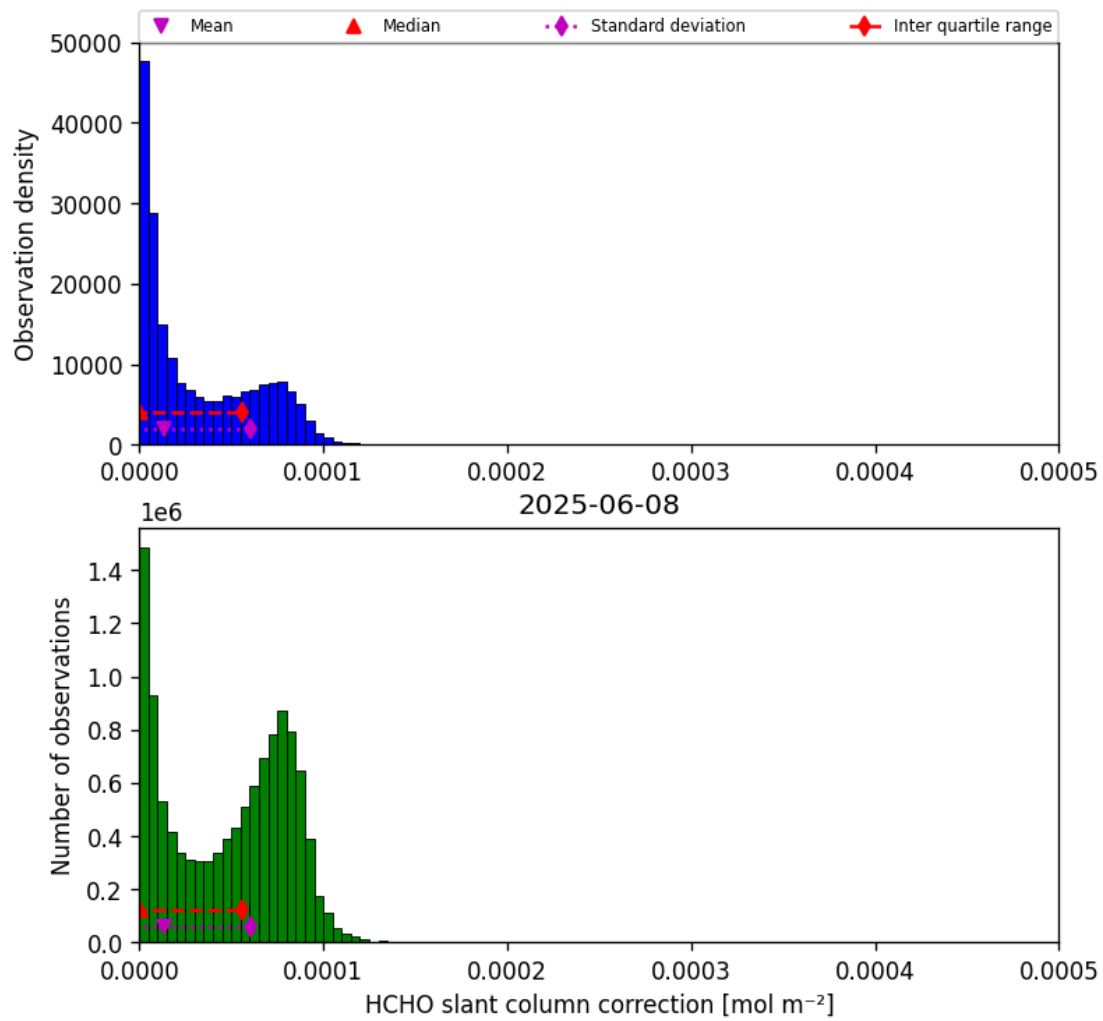
Figure 45: Histogram of “HCHO slant column correction” for 2025-06-08 to 2025-06-09
