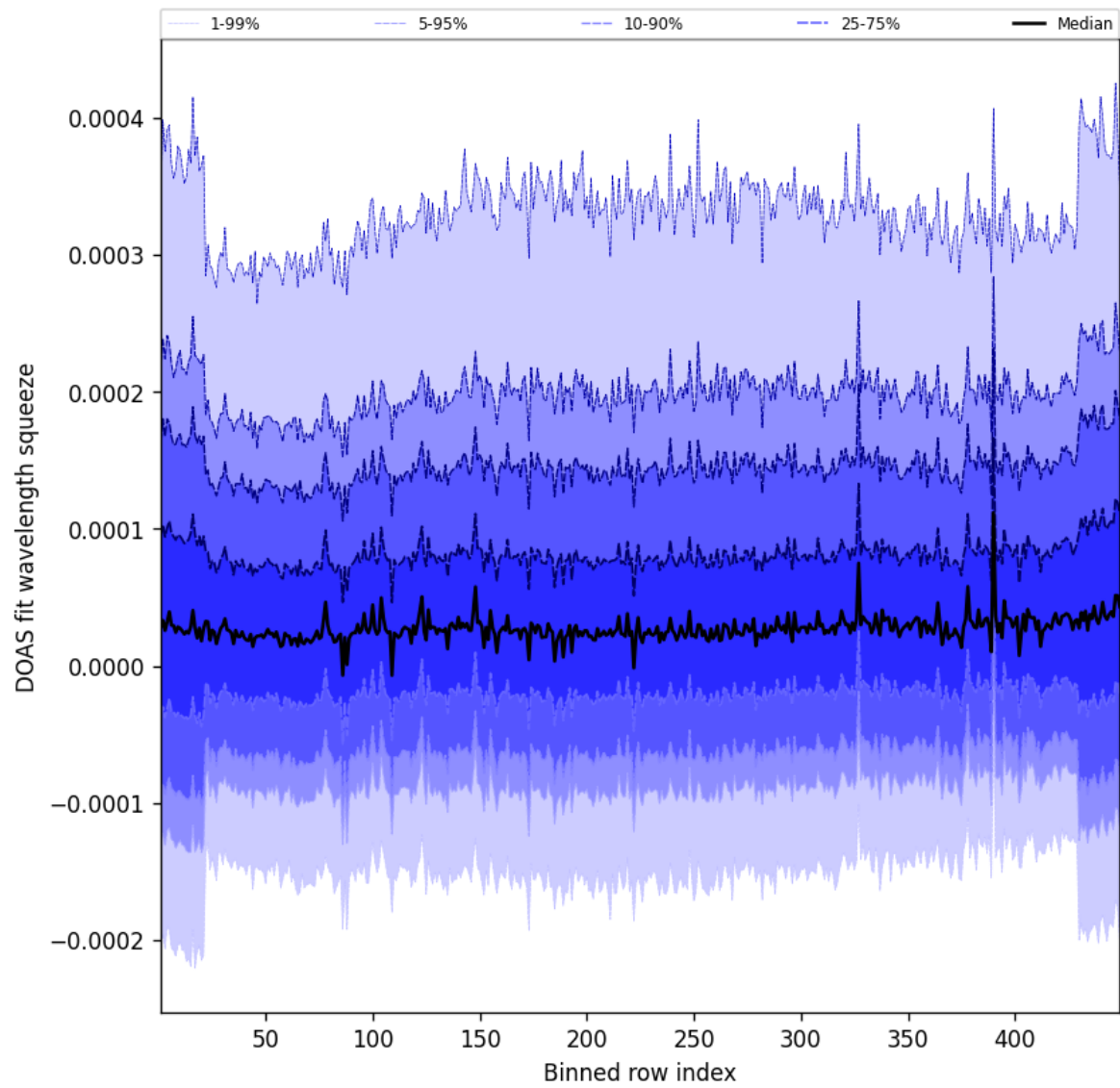
Figure 57: Along track statistics of “DOAS fit wavelength squeeze” for 2025-06-08 to 2025-06-09
