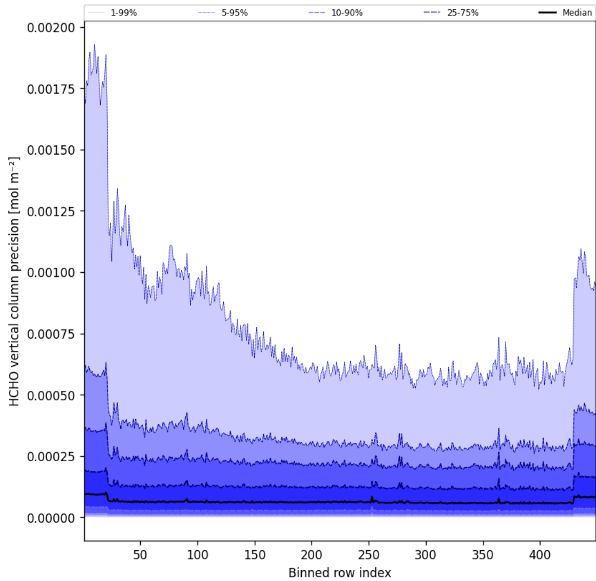
Figure 48: Along track statistics of “HCHO vertical column precision” for 2025-06-08 to 2025-06-09
