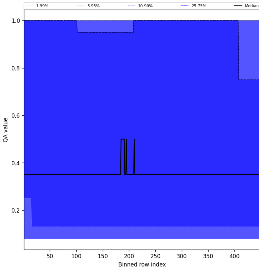
Figure 46: Along track statistics of “QA value” for 2025-06-08 to 2025-06-09
