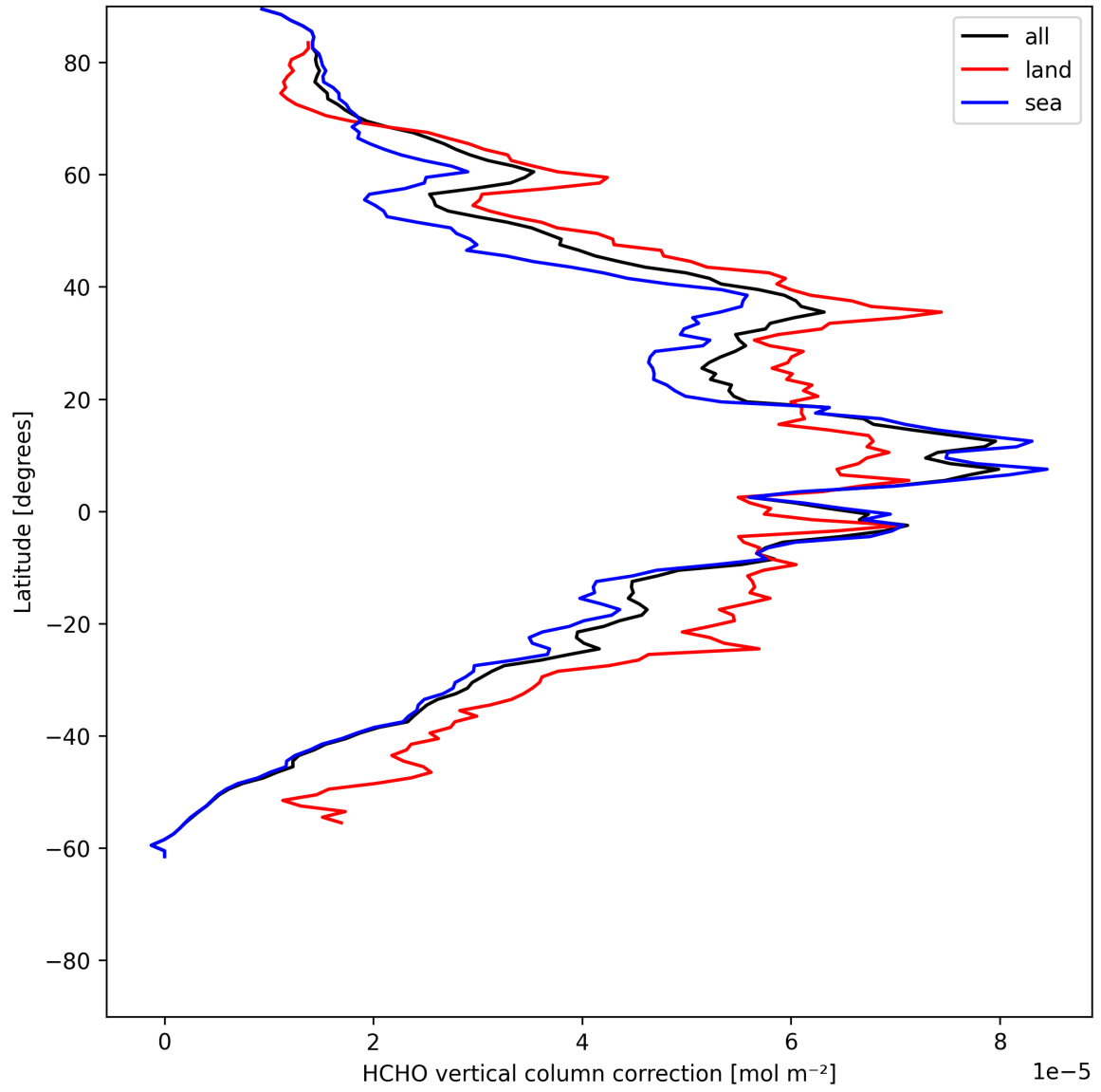
Figure 21: Zonal average of “HCHO vertical column correction” for 2025-06-08 to 2025-06-09.
