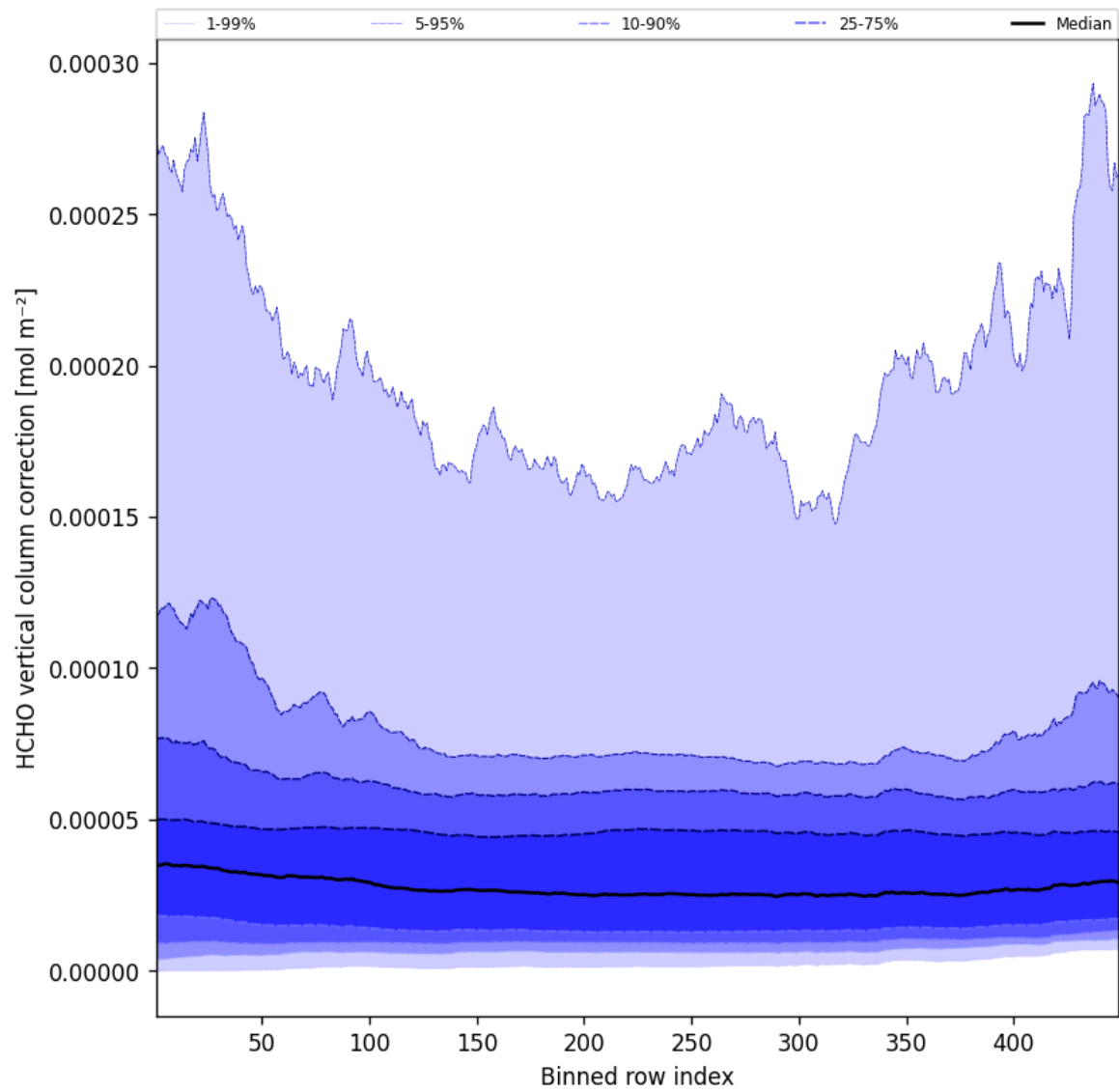
Figure 49: Along track statistics of “HCHO vertical column correction” for 2025-06-08 to 2025-06-09
