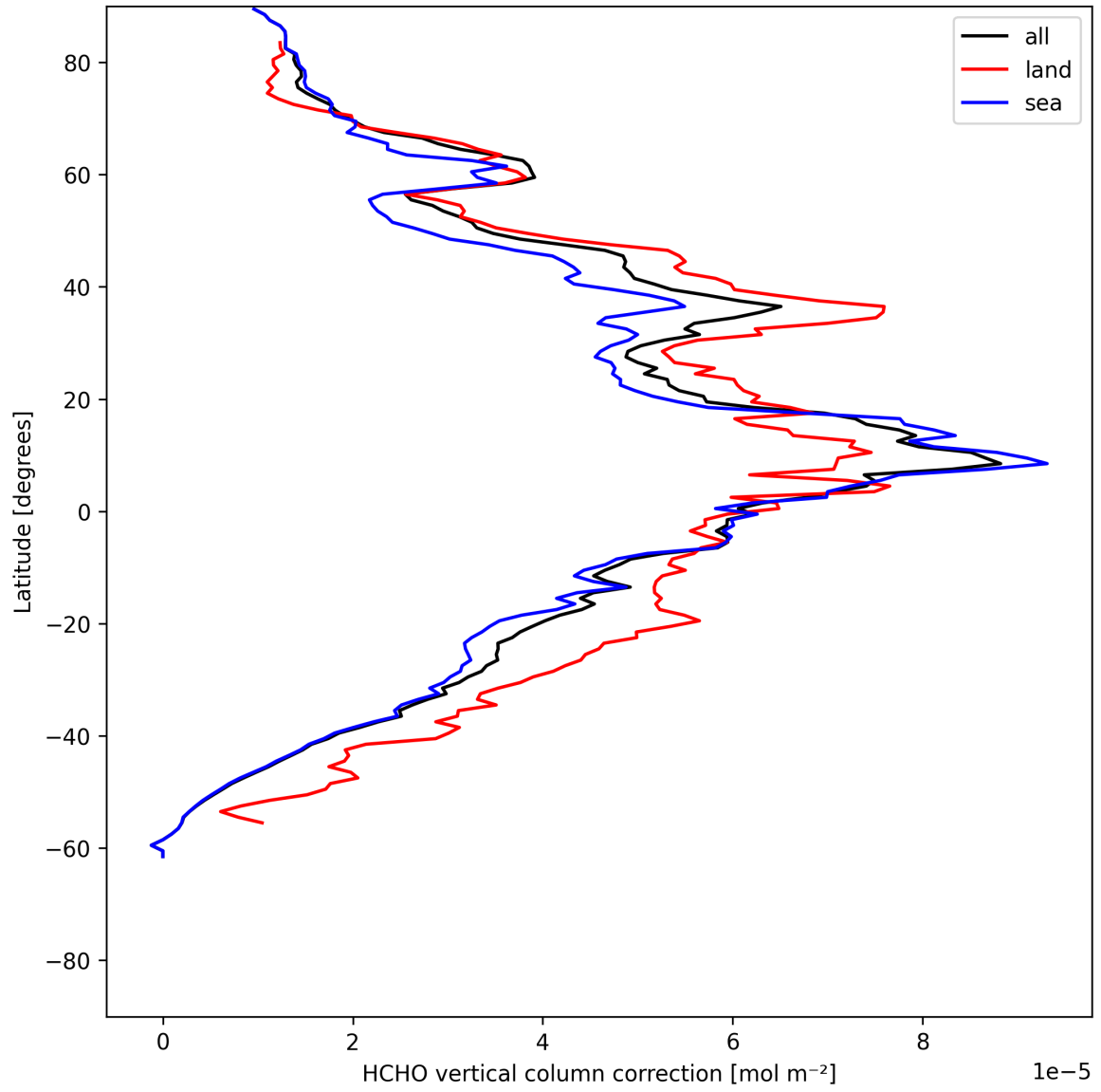
Figure 21: Zonal average of "HCHO vertical column correction" for 2025-06-09 to 2025-06-09.
