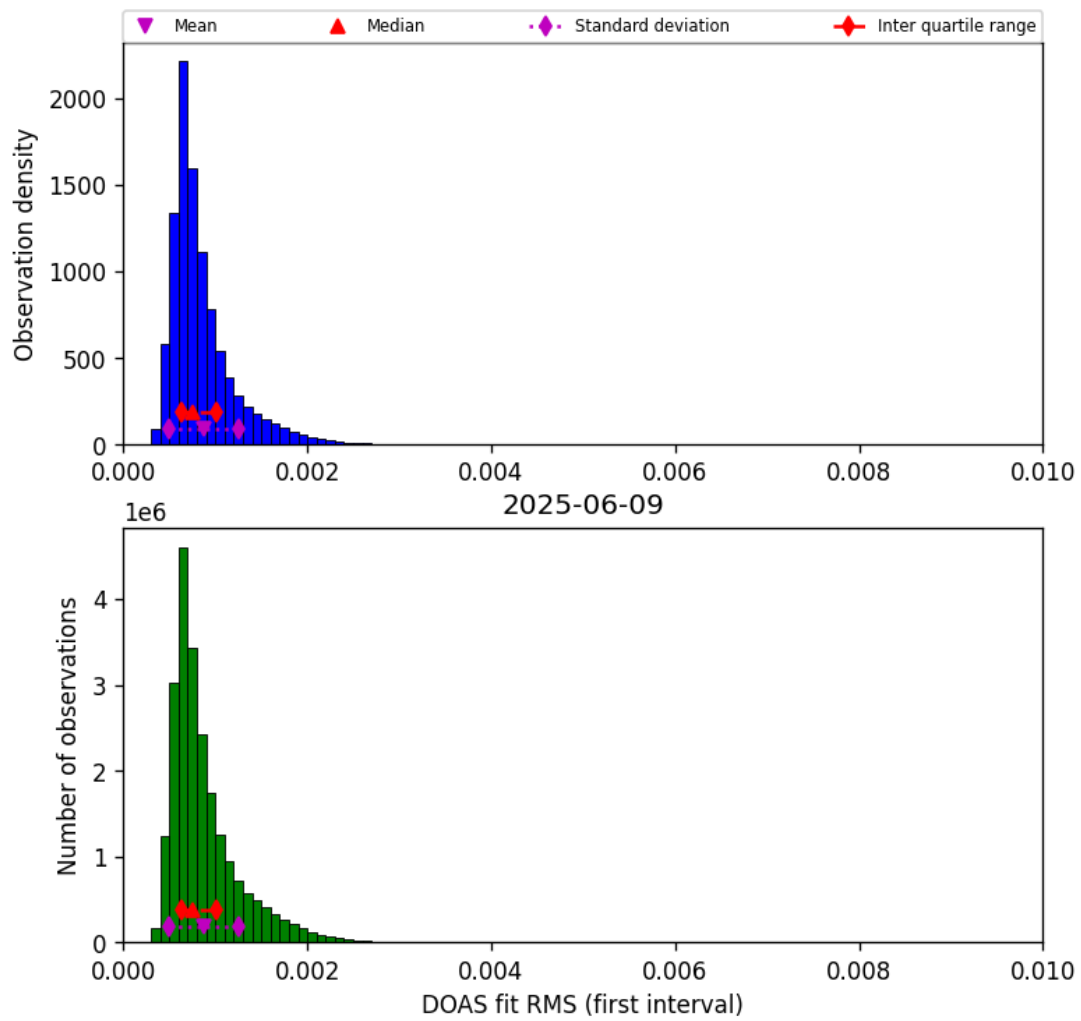
Figure 44: Histogram of “DOAS fit RMS (first interval)” for 2025-06-09 to 2025-06-09
