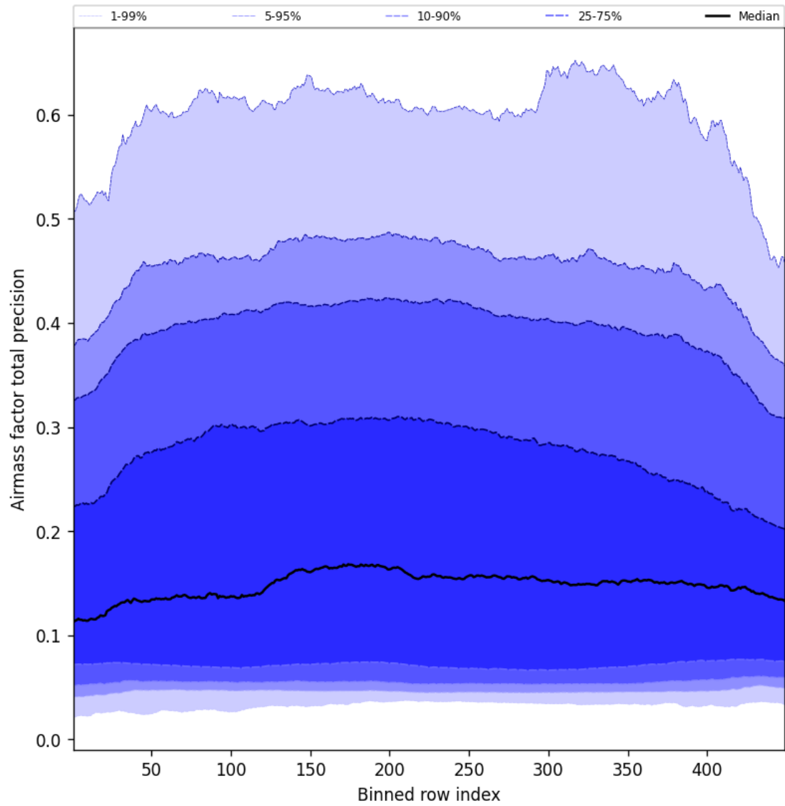
Figure 53: Along track statistics of “Airmass factor total precision” for 2025-06-09 to 2025-06-09
