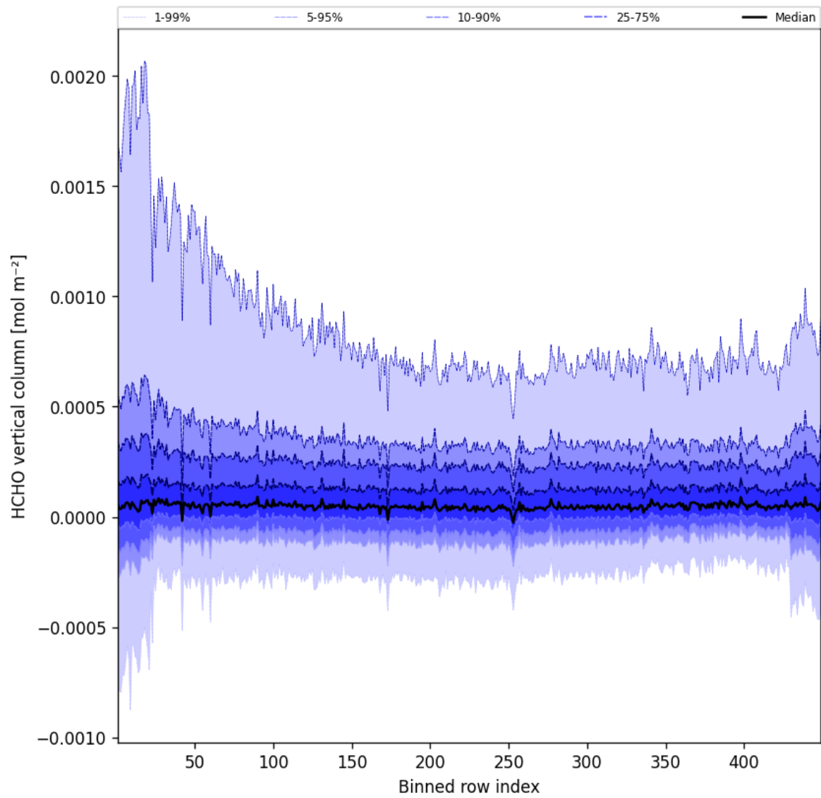
Figure 47: Along track statistics of “HCHO vertical column” for 2025-06-09 to 2025-06-09
