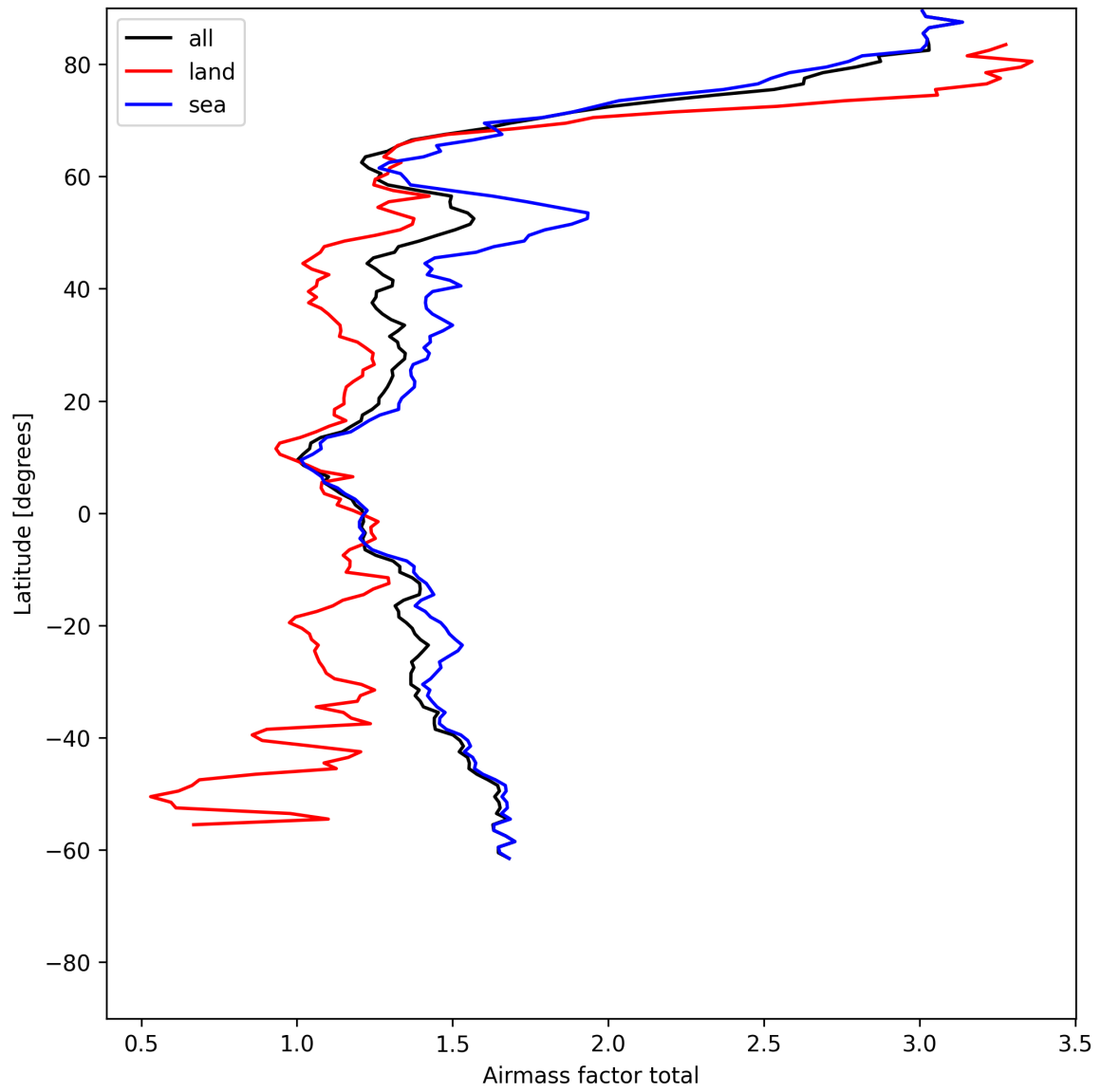
Figure 24: Zonal average of “Airmass factor total” for 2025-06-09 to 2025-06-09.
