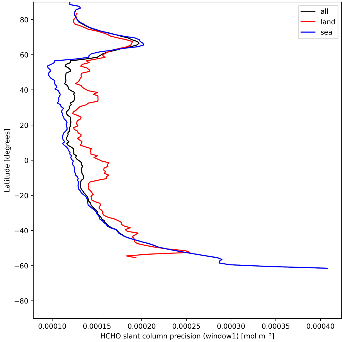
Figure 23: Zonal average of “HCHO slant column precision (window1)” for 2025-06-09 to 2025-06-09.
