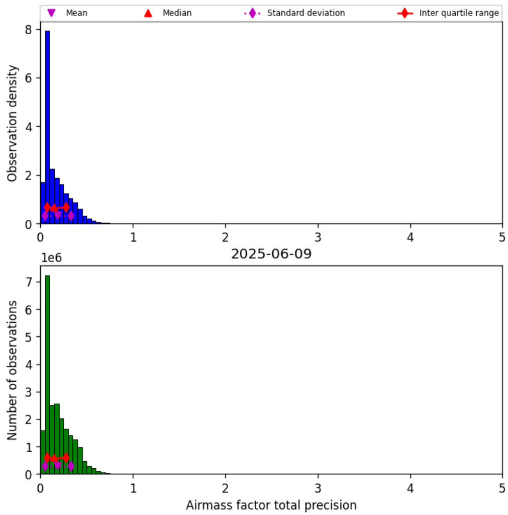
Figure 39: Histogram of “Airmass factor total precision” for 2025-06-09 to 2025-06-09
