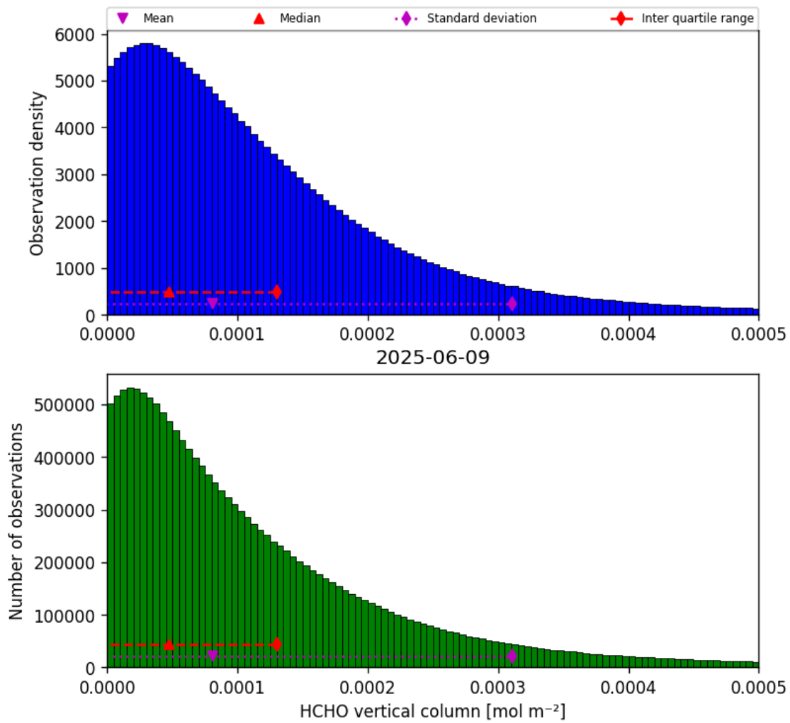
Figure 33: Histogram of “HCHO vertical column” for 2025-06-09 to 2025-06-09
