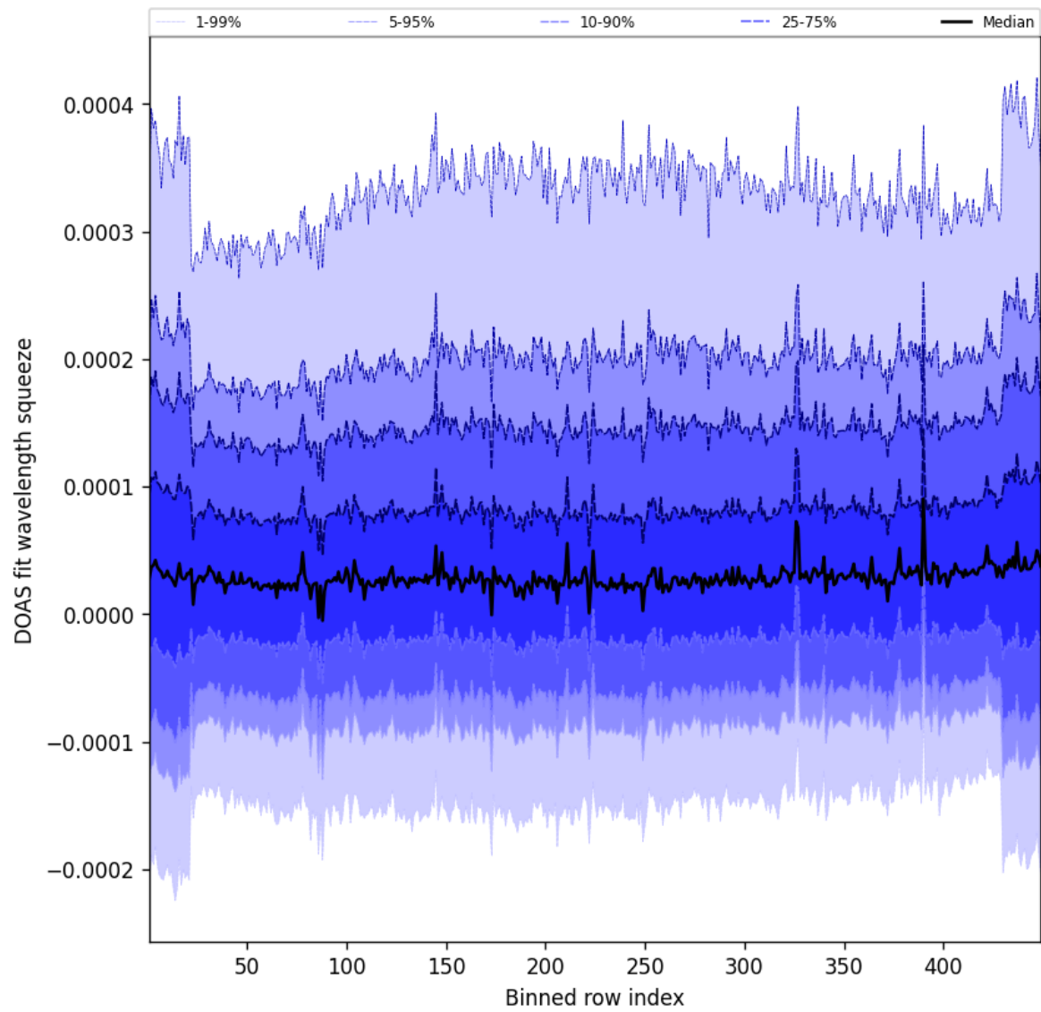
Figure 57: Along track statistics of “DOAS fit wavelength squeeze” for 2025-06-09 to 2025-06-09
