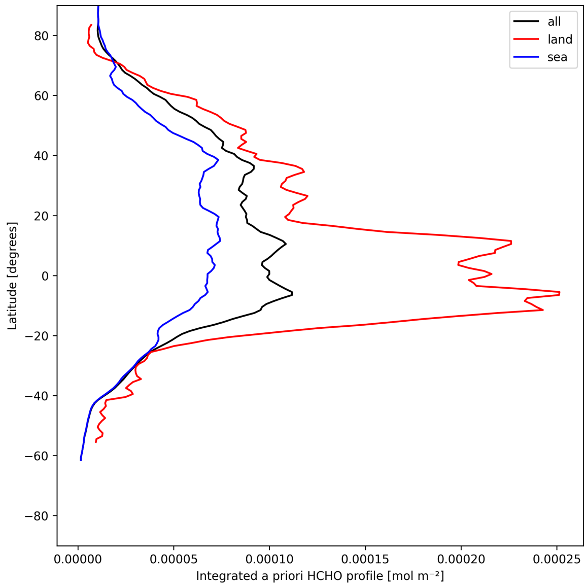
Figure 27: Zonal average of “Integrated a priori HCHO profile” for 2025-06-09 to 2025-06-09.
