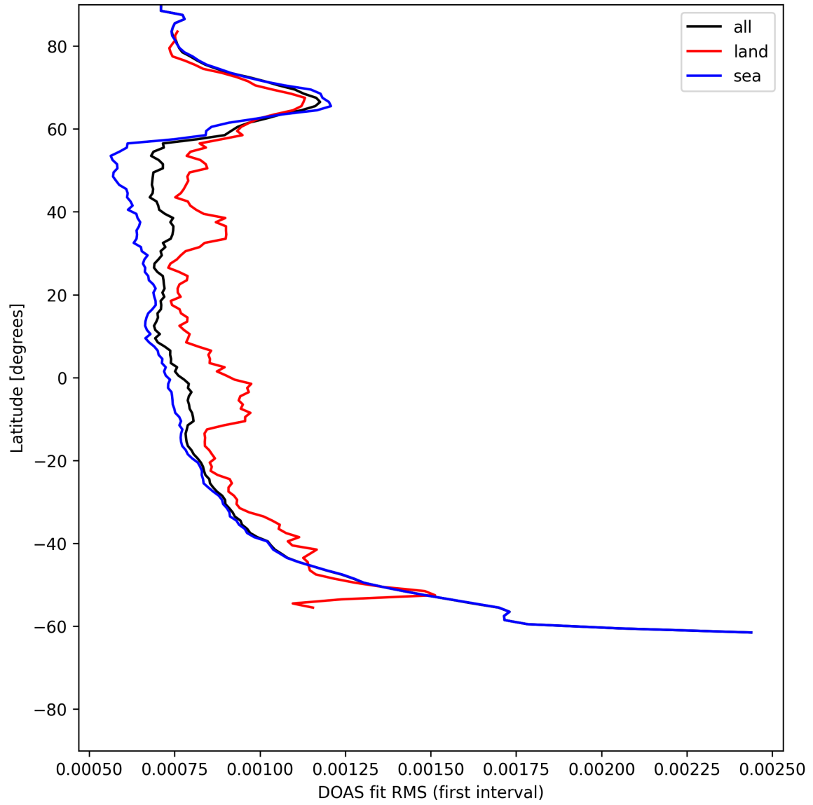
Figure 30: Zonal average of “DOAS fit RMS (first interval)” for 2025-06-09 to 2025-06-09.
