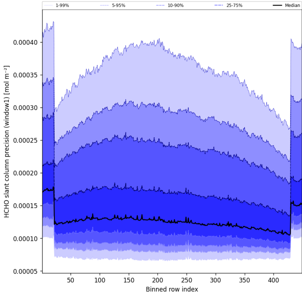
Figure 51: Along track statistics of “HCHO slant column precision (window1)” for 2025-06-09 to 2025-06-09
