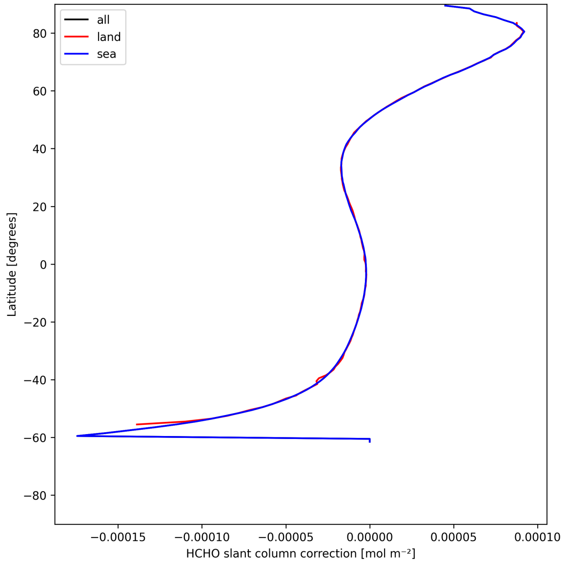
Figure 31: Zonal average of “HCHO slant column correction” for 2025-06-09 to 2025-06-09.
