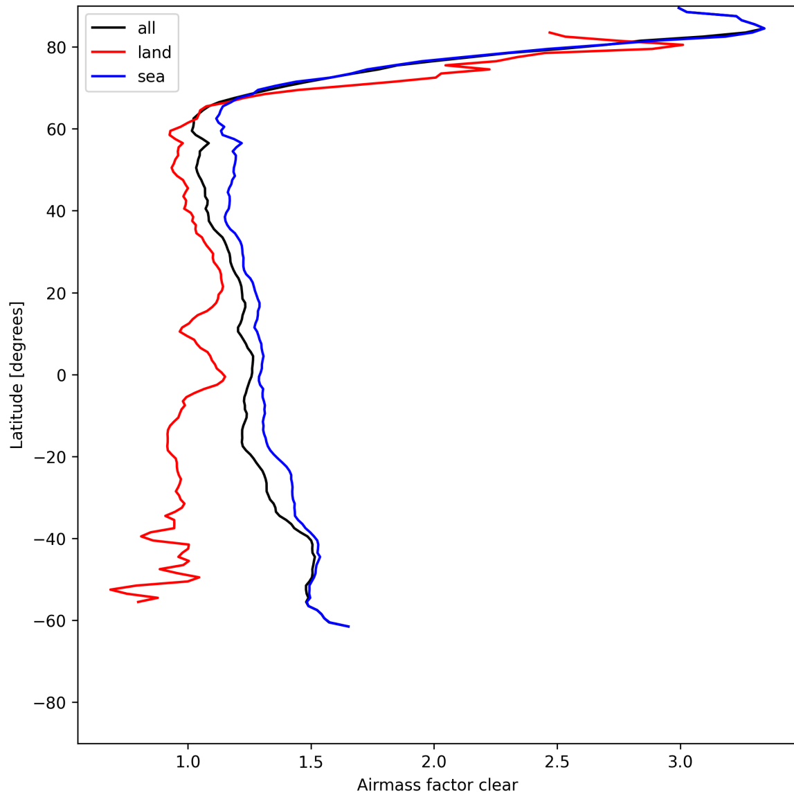
Figure 26: Zonal average of “Airmass factor clear” for 2025-06-09 to 2025-06-09.
