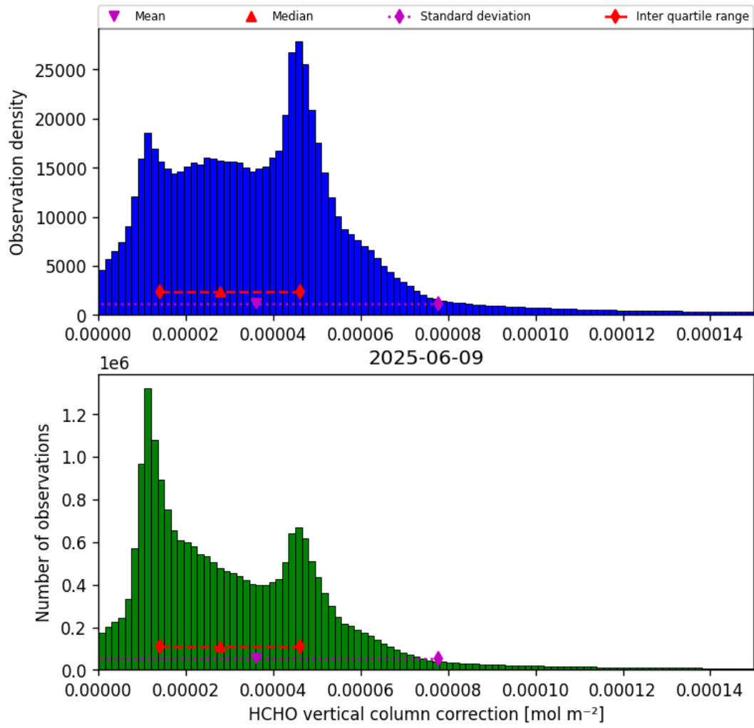
Figure 35: Histogram of “HCHO vertical column correction” for 2025-06-09 to 2025-06-09
