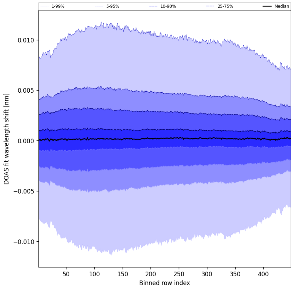
Figure 56: Along track statistics of “DOAS fit wavelength shift” for 2025-06-09 to 2025-06-09
