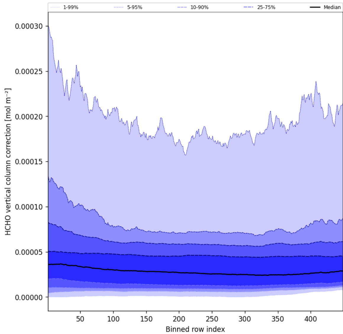
Figure 49: Along track statistics of “HCHO vertical column correction” for 2025-06-09 to 2025-06-09
