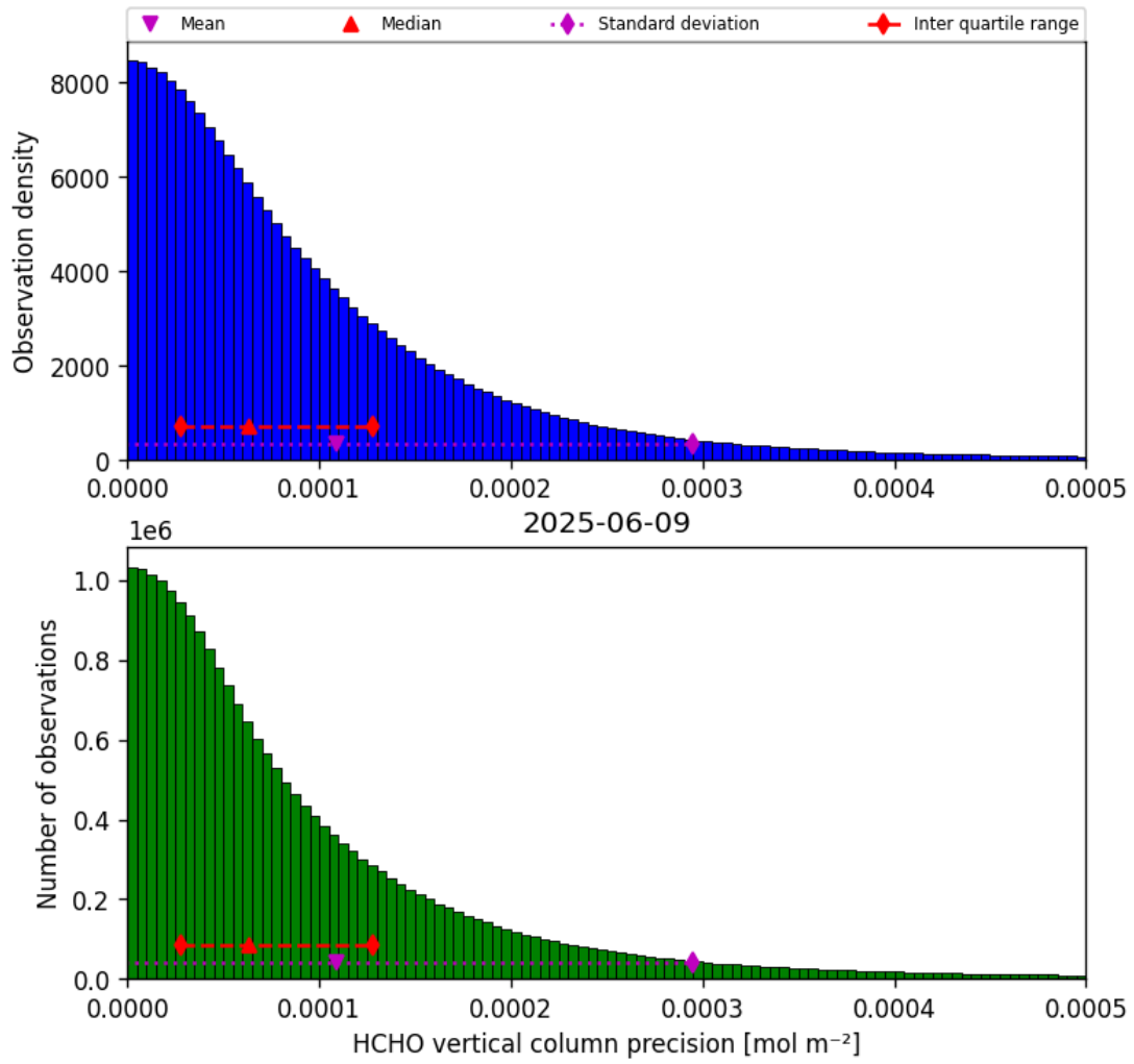
Figure 34: Histogram of “HCHO vertical column precision” for 2025-06-09 to 2025-06-09
