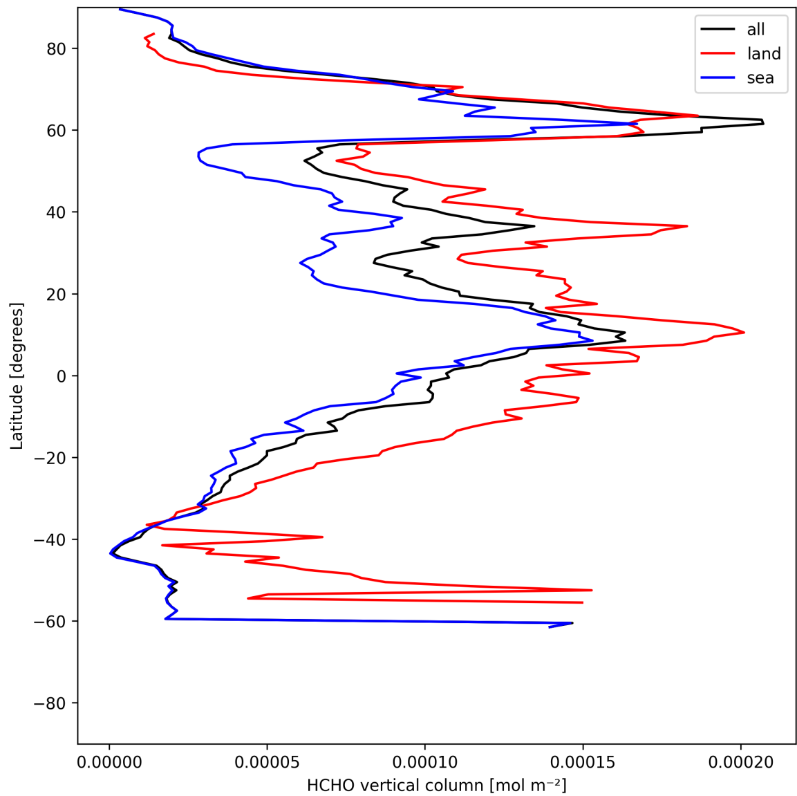
Figure 19: Zonal average of “HCHO vertical column” for 2025-06-09 to 2025-06-09.
