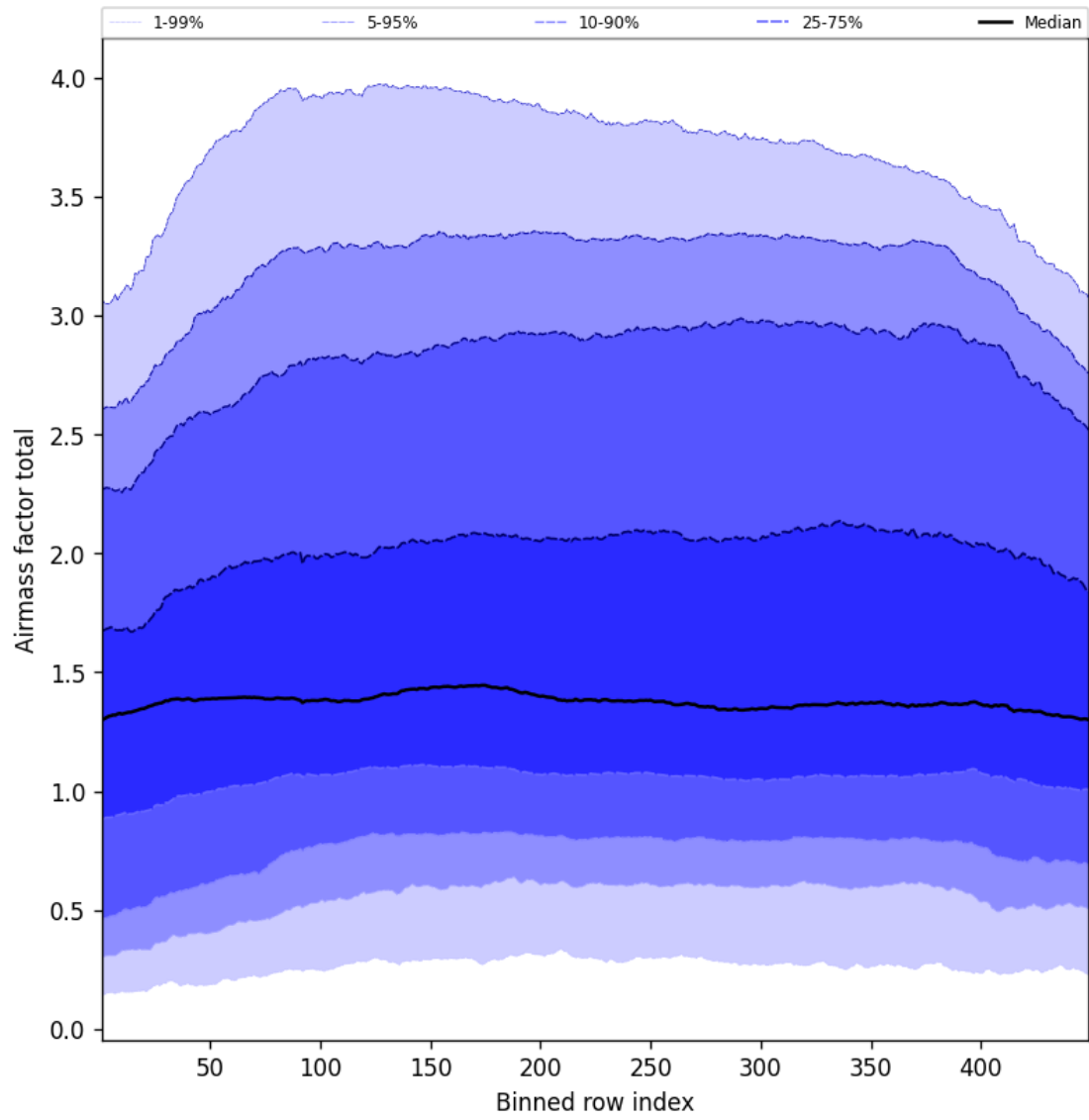
Figure 52: Along track statistics of “Airmass factor total” for 2025-06-09 to 2025-06-09
