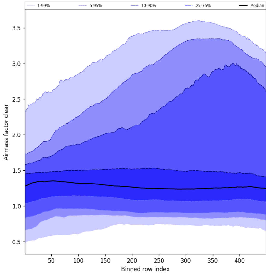
Figure 54: Along track statistics of “Airmass factor clear” for 2025-06-09 to 2025-06-09
