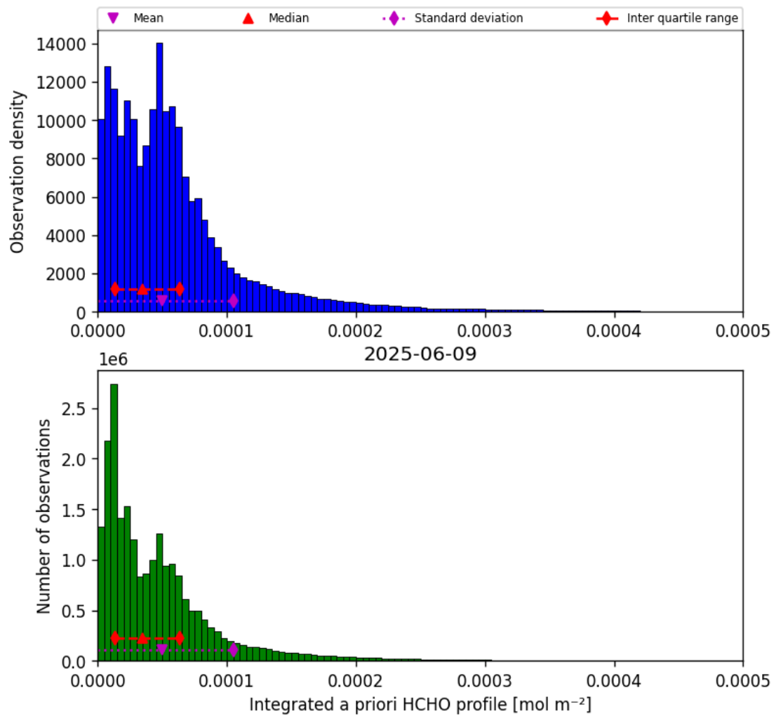
Figure 41: Histogram of “Integrated a priori HCHO profile” for 2025-06-09 to 2025-06-09
