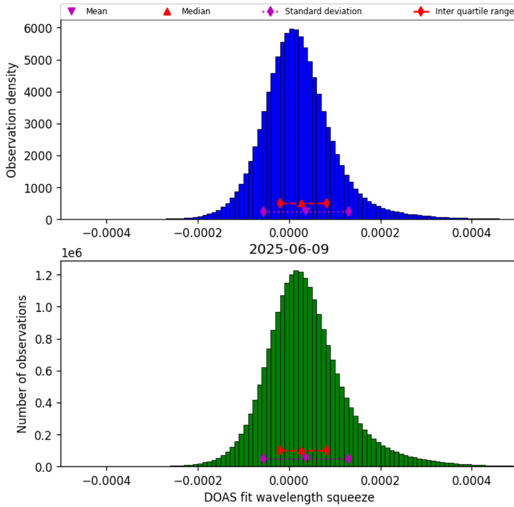
Figure 43: Histogram of “DOAS fit wavelength squeeze” for 2025-06-09 to 2025-06-09
