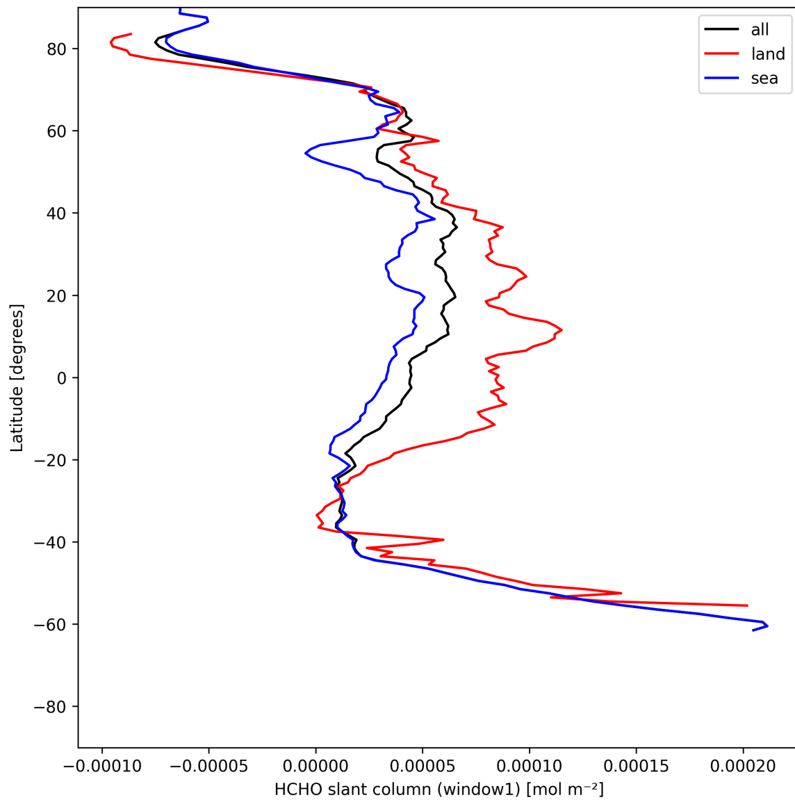
Figure 22: Zonal average of “HCHO slant column (window1)” for 2025-06-09 to 2025-06-09.
