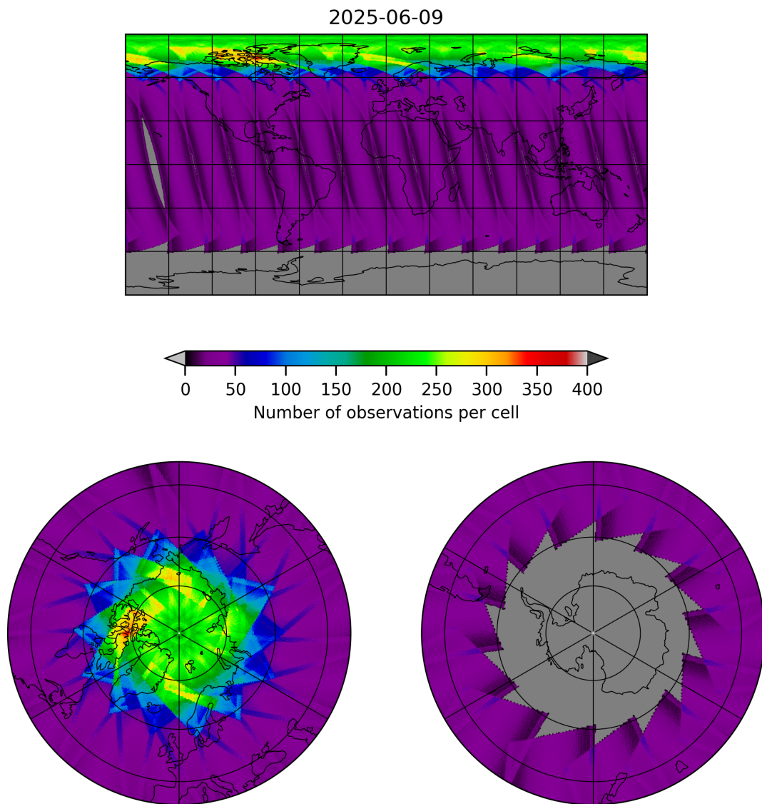
Figure 17: Map of the number of observations for 2025-06-09 to 2025-06-09
