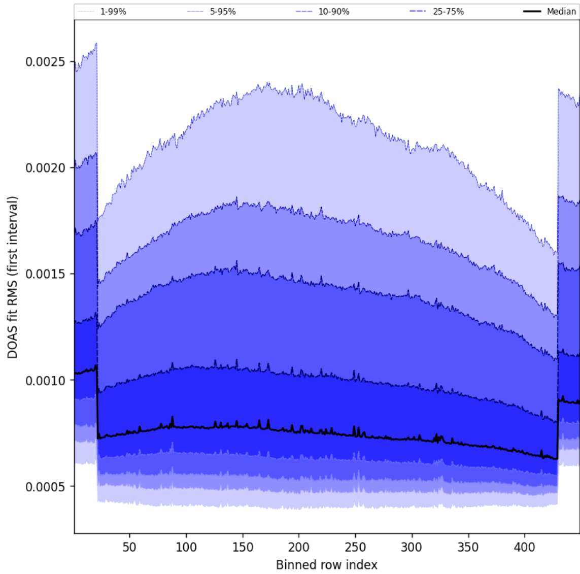
Figure 58: Along track statistics of “DOAS fit RMS (first interval)” for 2025-06-09 to 2025-06-09
