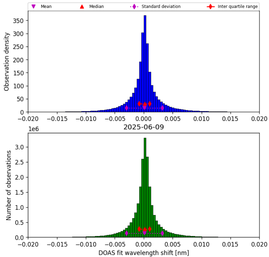
Figure 42: Histogram of “DOAS fit wavelength shift” for 2025-06-09 to 2025-06-09
