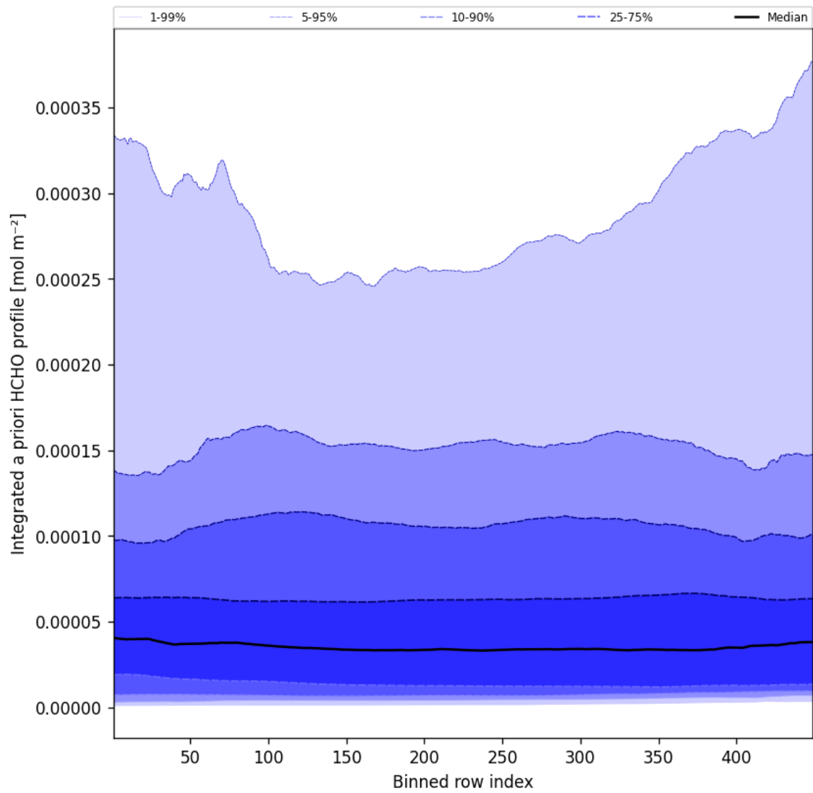
Figure 55: Along track statistics of “Integrated a priori HCHO profile” for 2025-06-09 to 2025-06-09
