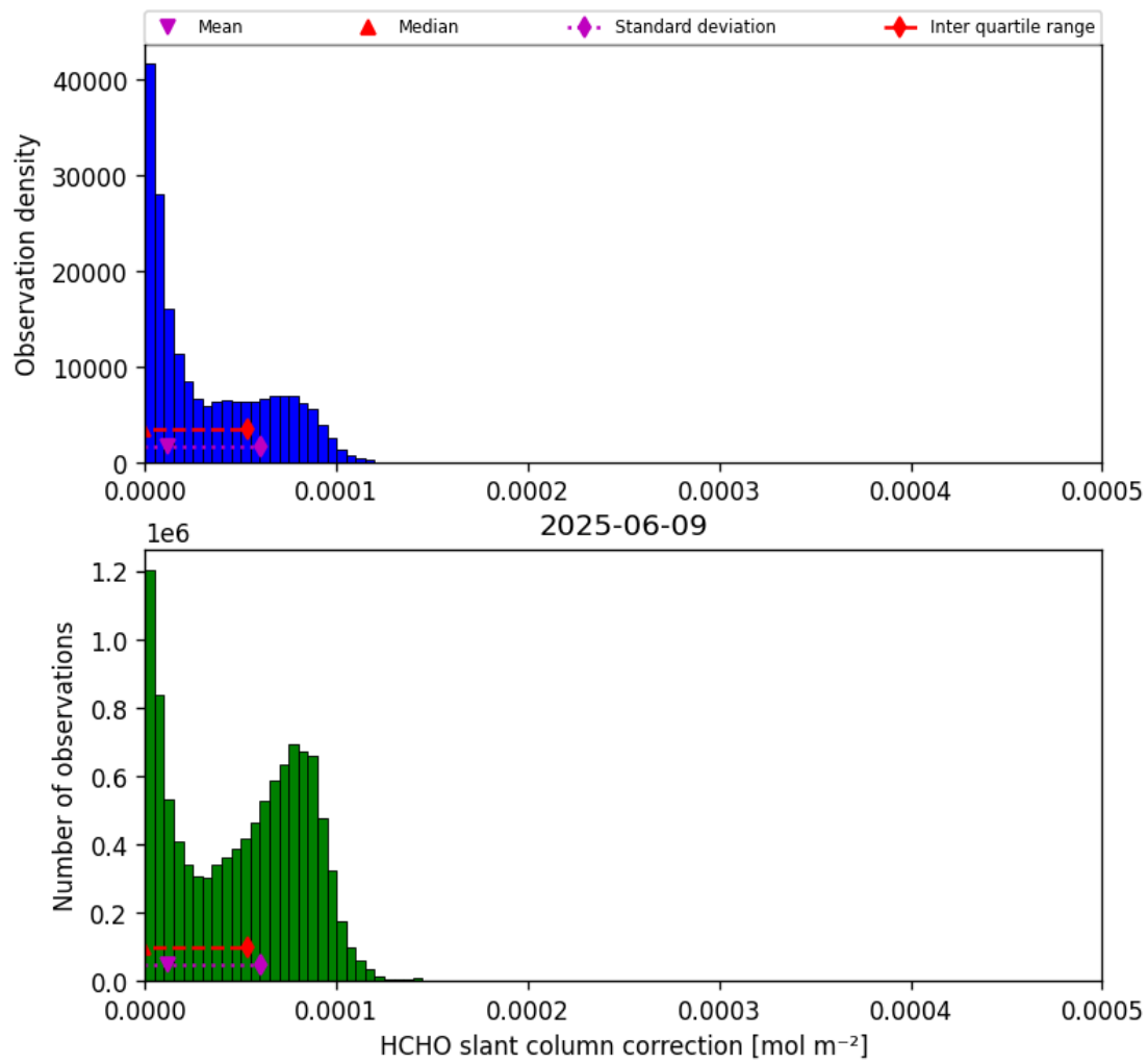
Figure 45: Histogram of “HCHO slant column correction” for 2025-06-09 to 2025-06-09
