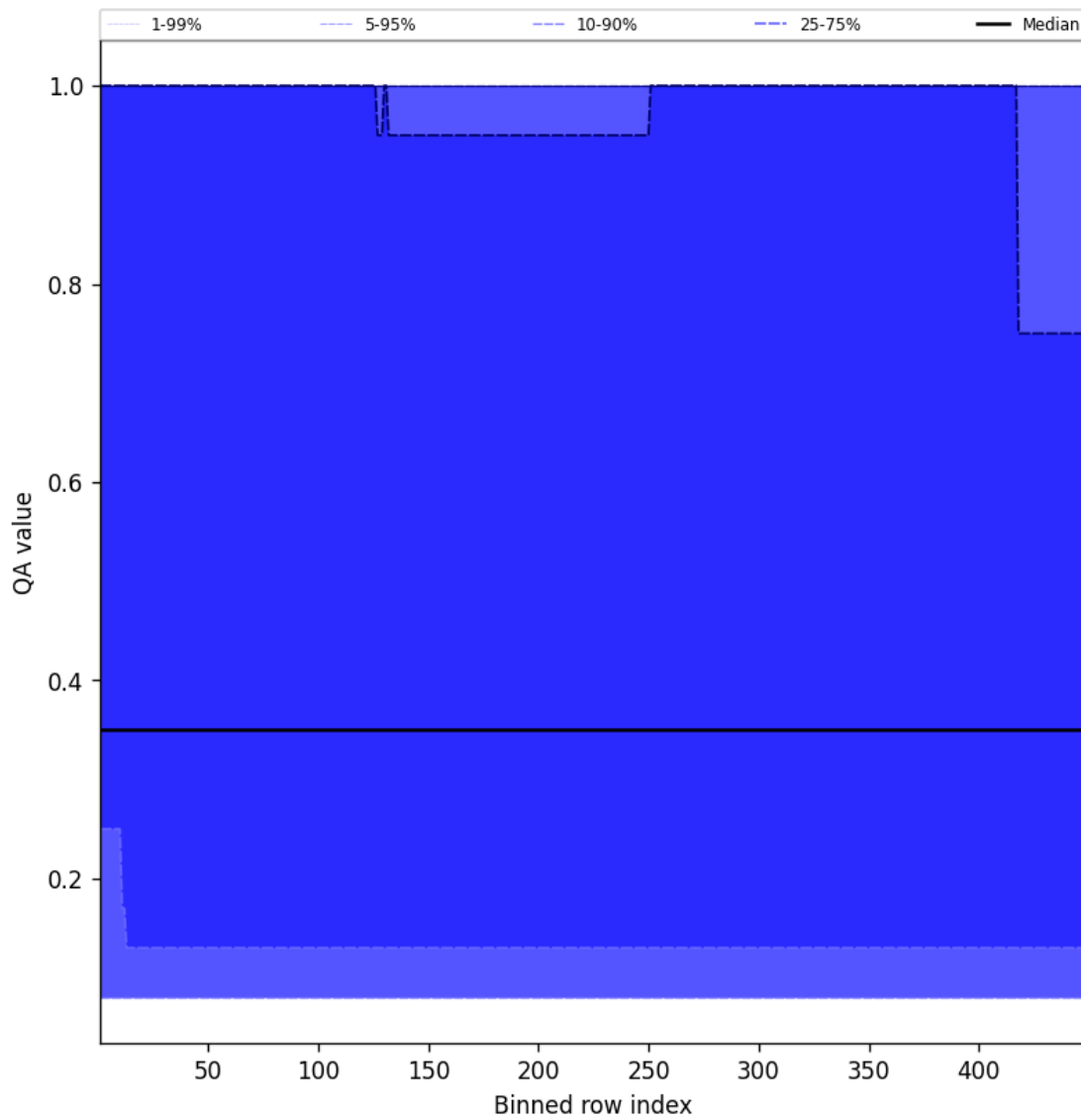
Figure 46: Along track statistics of "QA value" for 2025-06-09 to 2025-06-09
