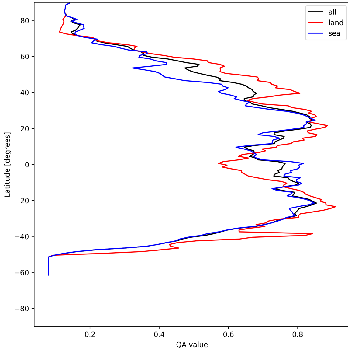
Figure 18: Zonal average of “QA value” for 2025-06-09 to 2025-06-09.
