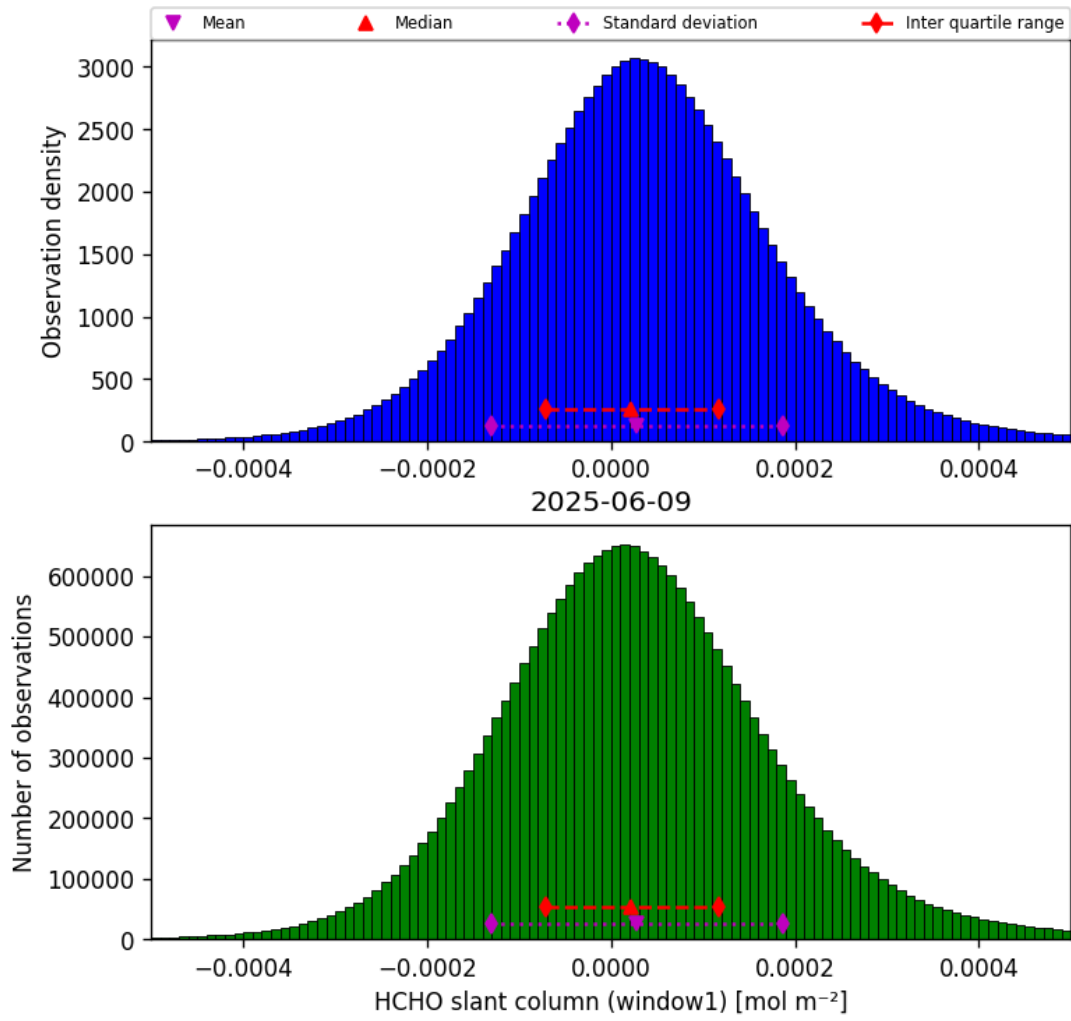
Figure 36: Histogram of “HCHO slant column (window1)” for 2025-06-09 to 2025-06-09
