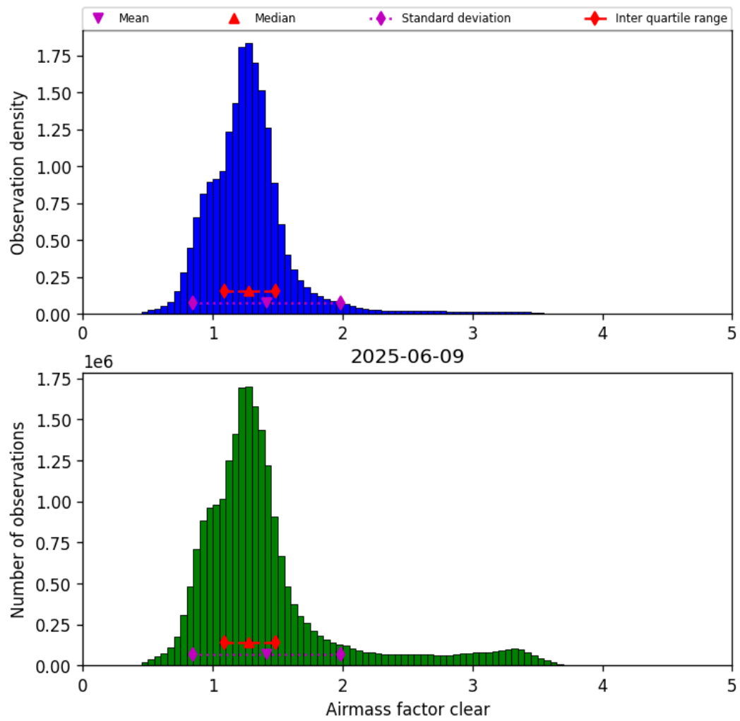
Figure 40: Histogram of “Airmass factor clear” for 2025-06-09 to 2025-06-09
