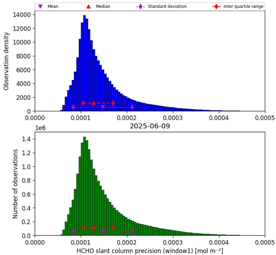
Figure 37: Histogram of “HCHO slant column precision (window1)” for 2025-06-09 to 2025-06-09
