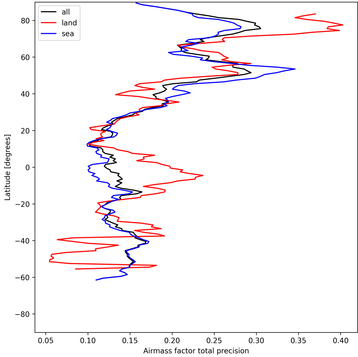
Figure 25: Zonal average of “Airmass factor total precision” for 2025-06-09 to 2025-06-09.
