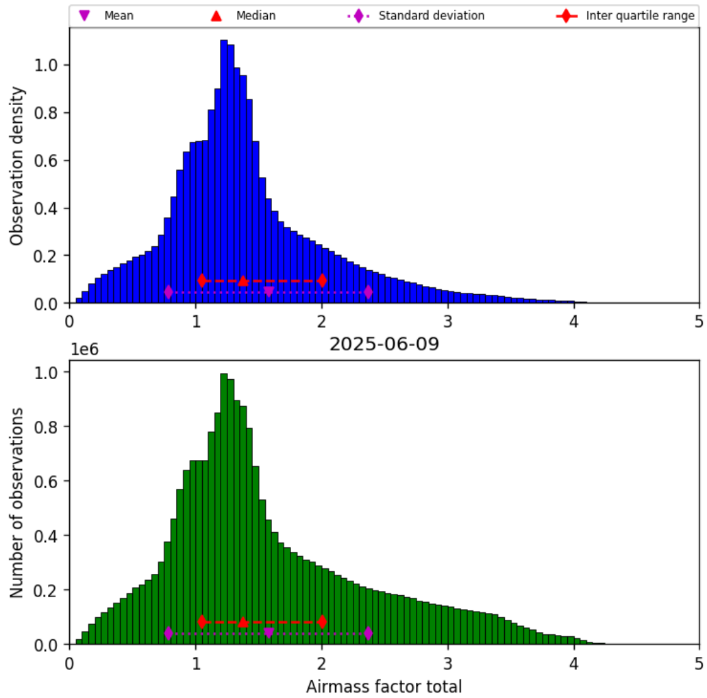
Figure 38: Histogram of “Airmass factor total” for 2025-06-09 to 2025-06-09
