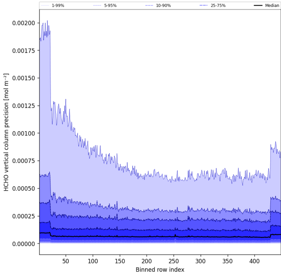
Figure 48: Along track statistics of “HCHO vertical column precision” for 2025-06-09 to 2025-06-09
