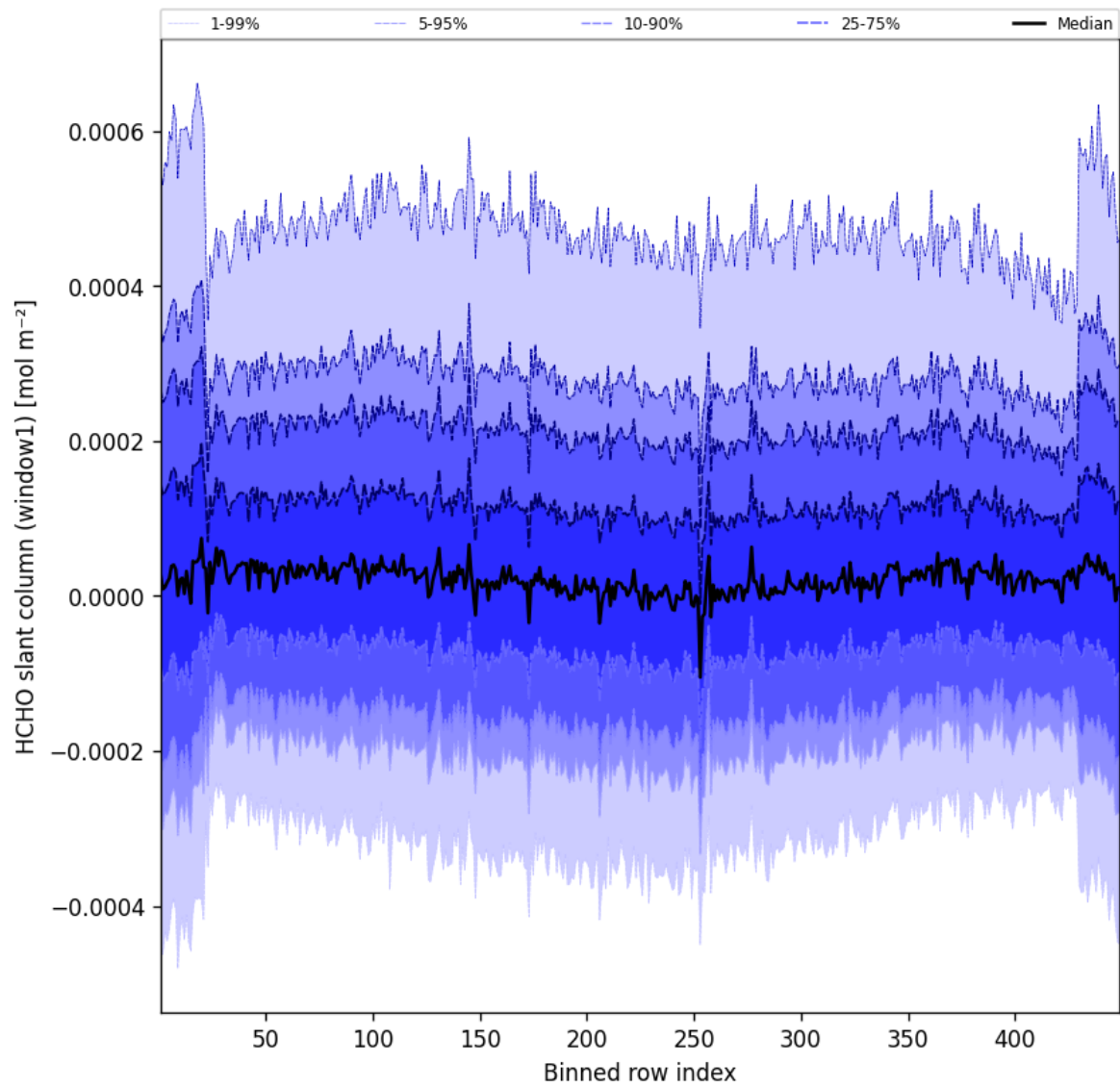
Figure 50: Along track statistics of “HCHO slant column (window1)” for 2025-06-09 to 2025-06-09
