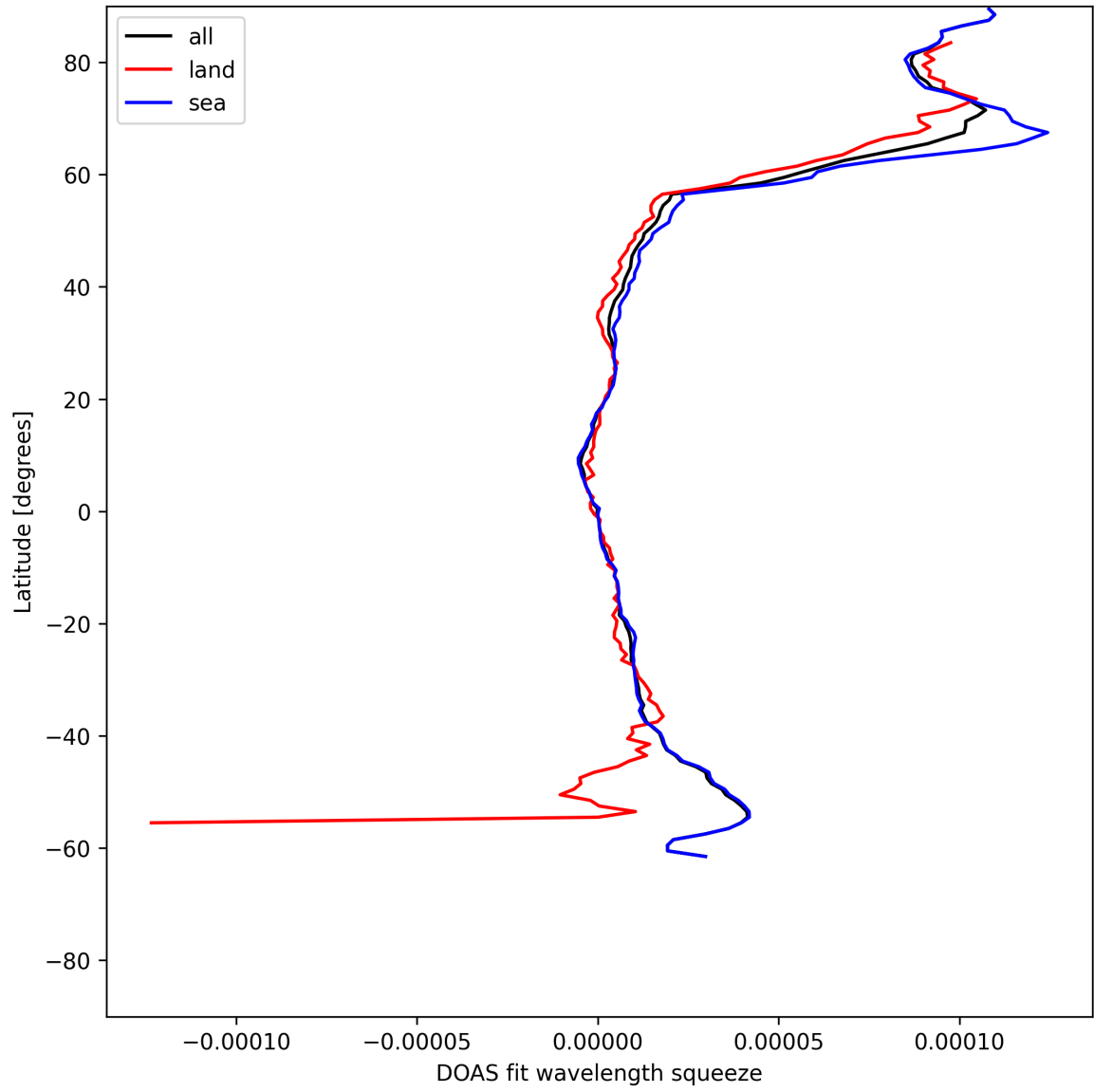
Figure 29: Zonal average of “DOAS fit wavelength squeeze” for 2025-06-09 to 2025-06-09.
