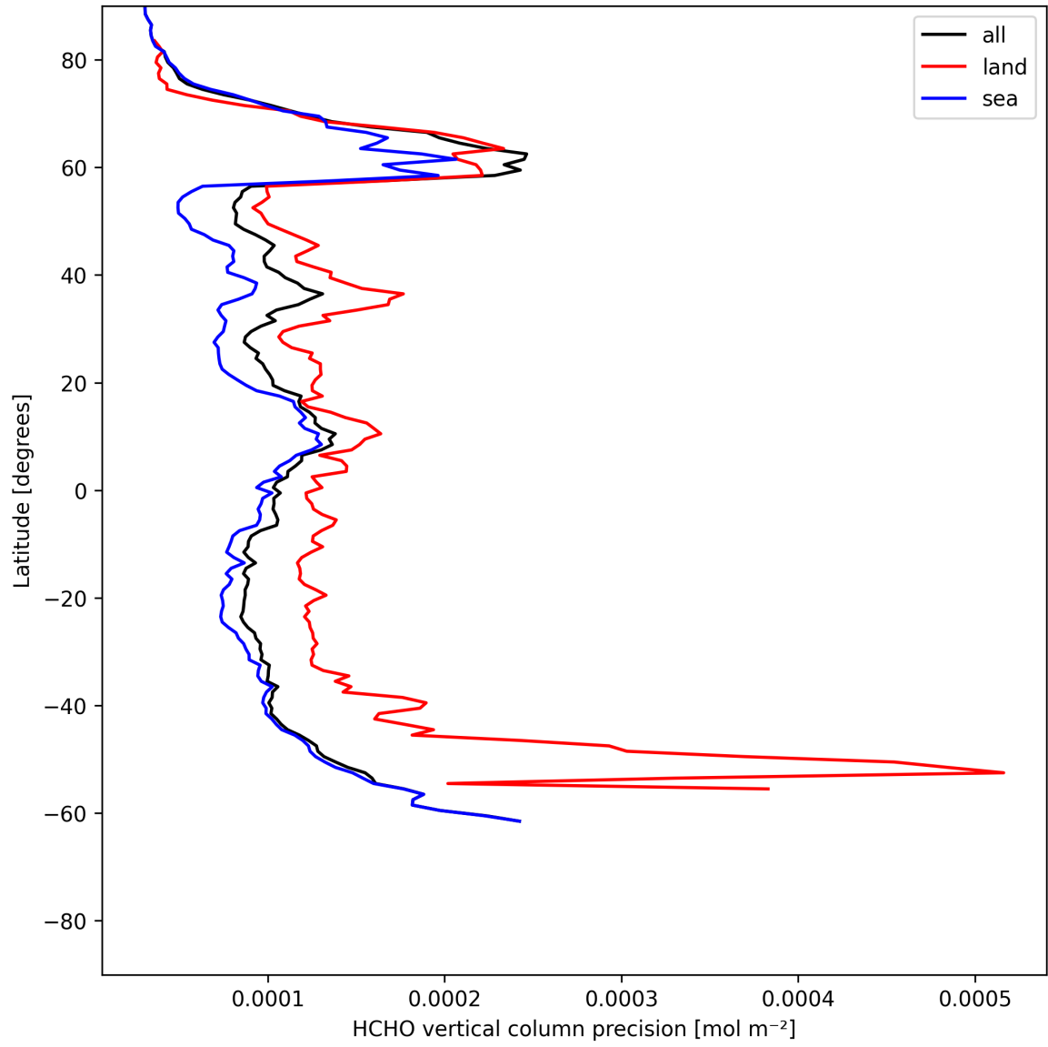
Figure 20: Zonal average of “HCHO vertical column precision” for 2025-06-09 to 2025-06-09.
