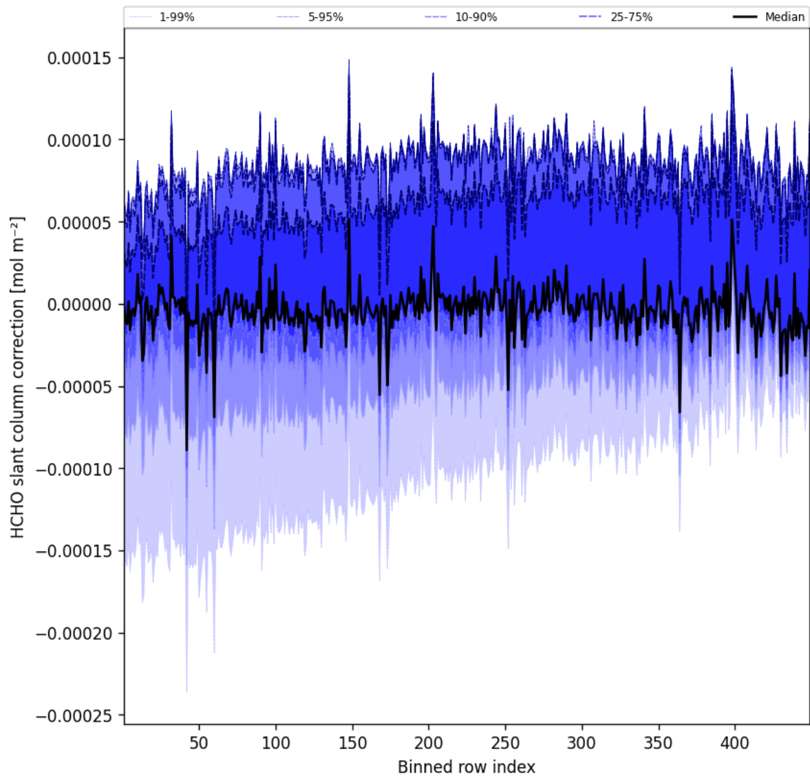
Figure 59: Along track statistics of “HCHO slant column correction” for 2025-06-09 to 2025-06-09
