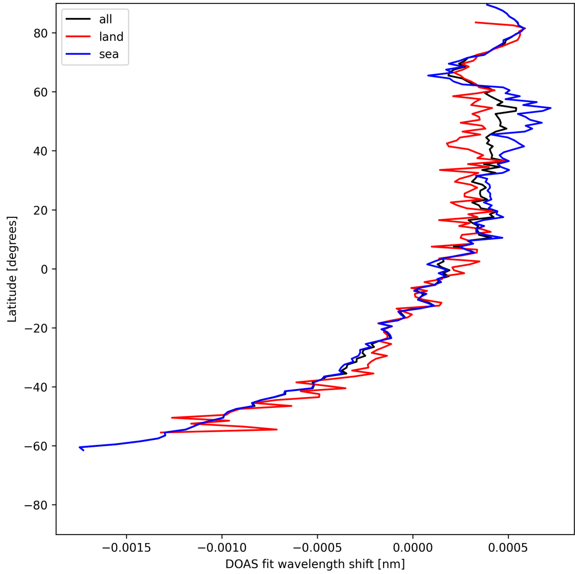
Figure 28: Zonal average of “DOAS fit wavelength shift” for 2025-06-09 to 2025-06-09.
