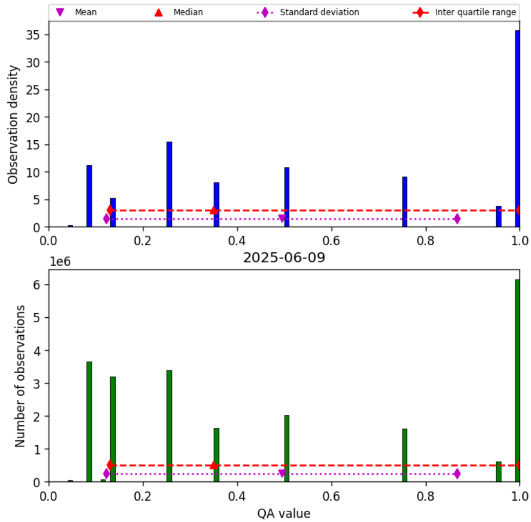
Figure 32: Histogram of “QA value” for 2025-06-09 to 2025-06-09
