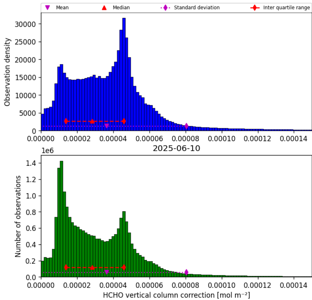
Figure 35: Histogram of “HCHO vertical column correction” for 2025-06-10 to 2025-06-11
