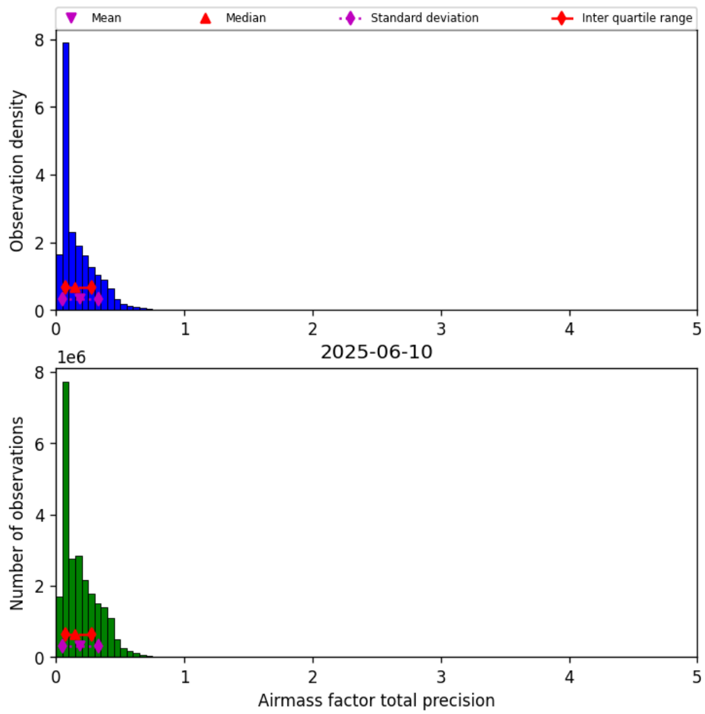
Figure 39: Histogram of “Airmass factor total precision” for 2025-06-10 to 2025-06-11
