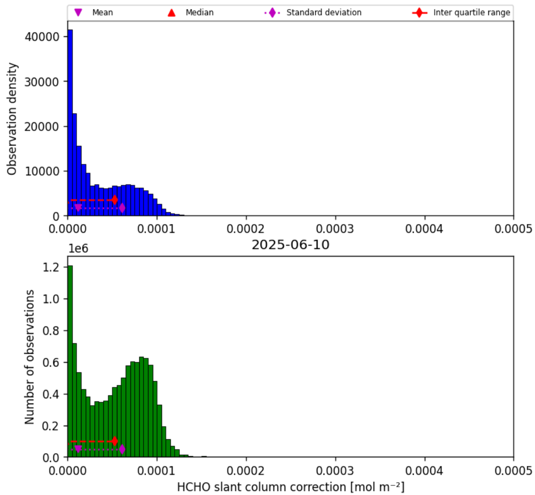
Figure 45: Histogram of “HCHO slant column correction” for 2025-06-10 to 2025-06-11
