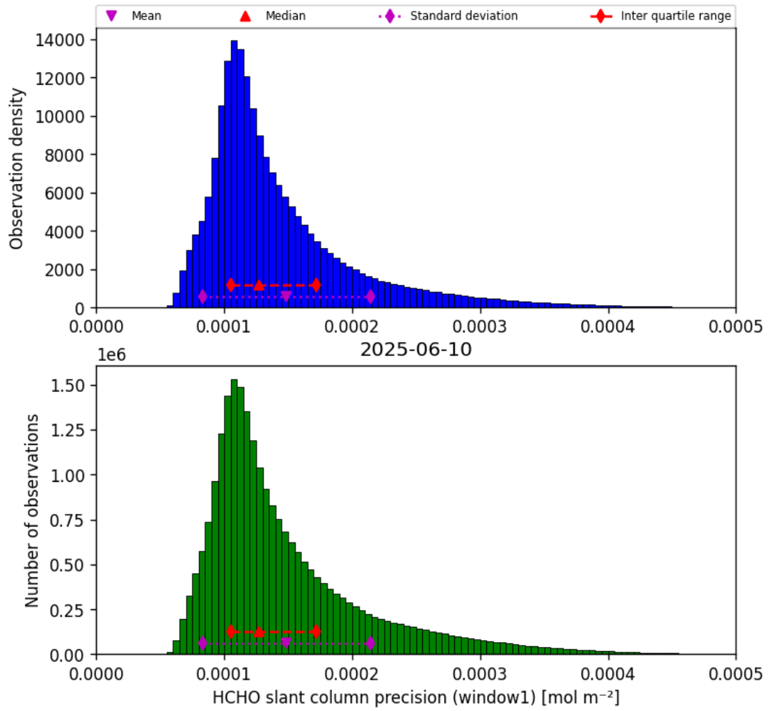
Figure 37: Histogram of “HCHO slant column precision (window1)” for 2025-06-10 to 2025-06-11
