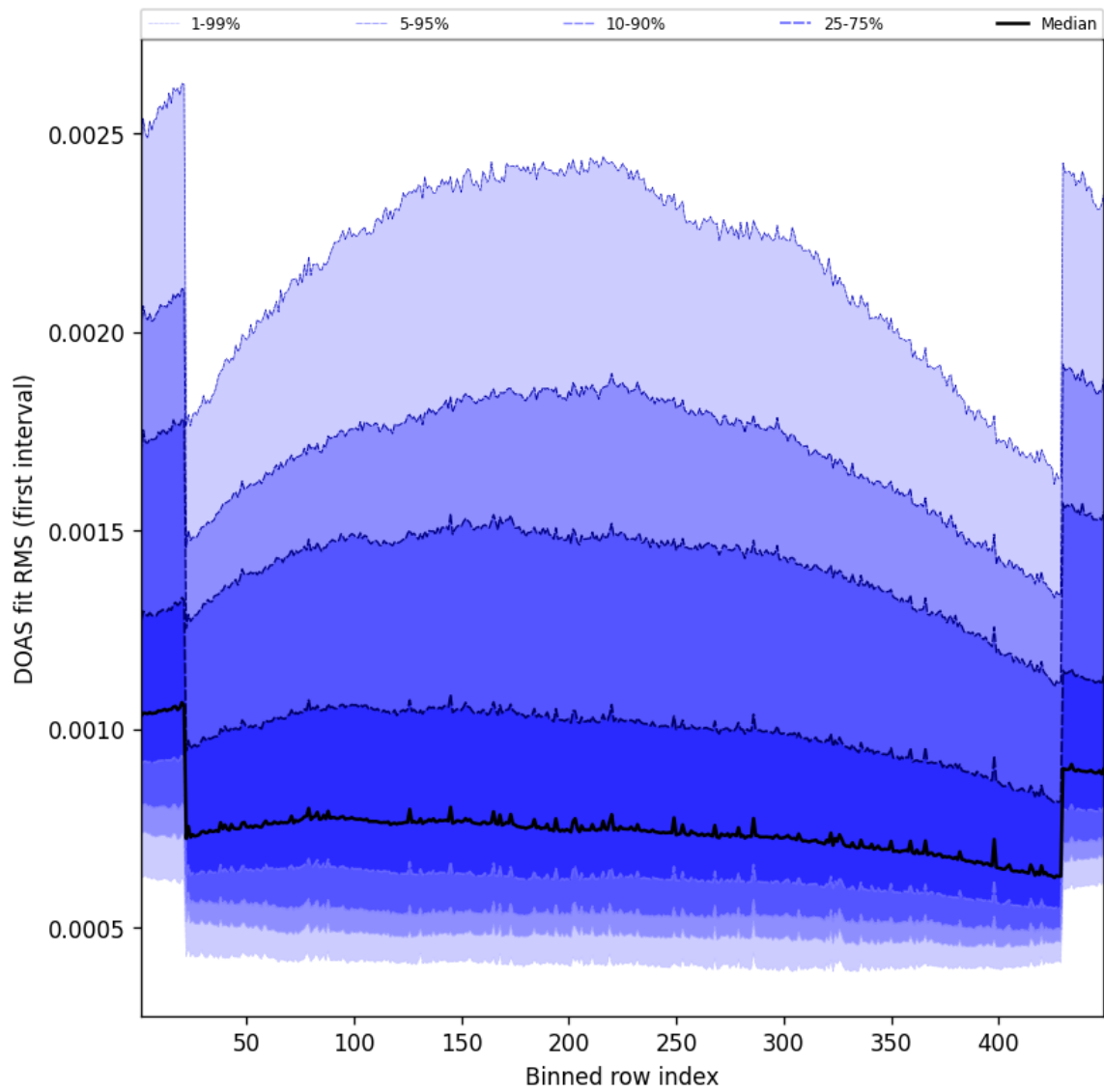
Figure 58: Along track statistics of “DOAS fit RMS (first interval)” for 2025-06-10 to 2025-06-11
