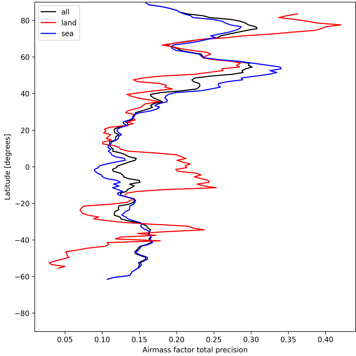
Figure 25: Zonal average of “Airmass factor total precision” for 2025-06-10 to 2025-06-11.
