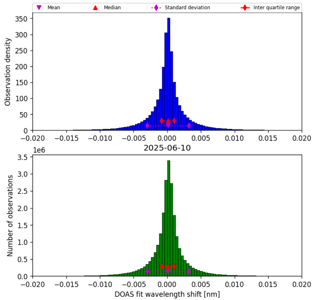
Figure 42: Histogram of “DOAS fit wavelength shift” for 2025-06-10 to 2025-06-11
