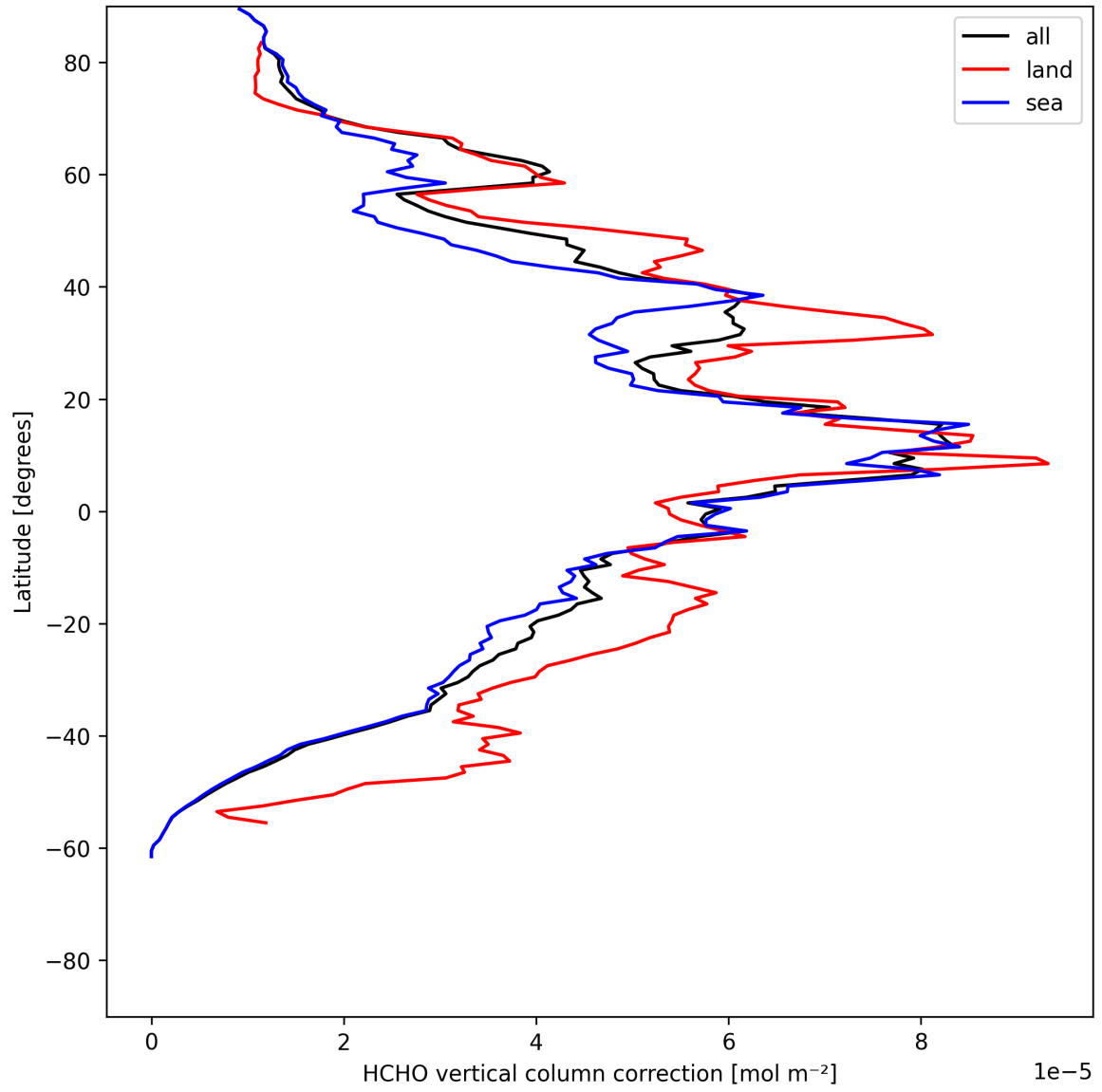
Figure 21: Zonal average of “HCHO vertical column correction” for 2025-06-10 to 2025-06-11.
