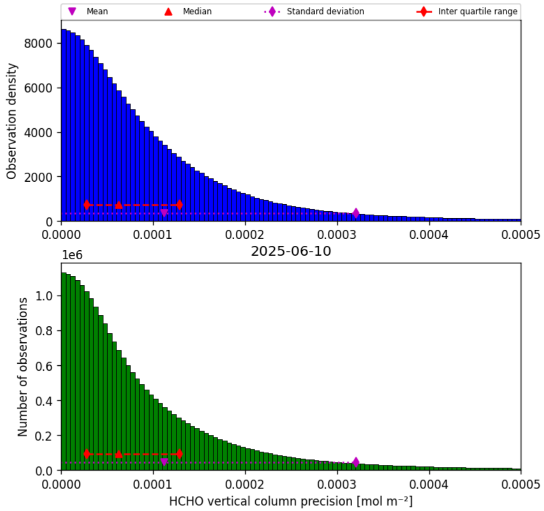
Figure 34: Histogram of “HCHO vertical column precision” for 2025-06-10 to 2025-06-11
