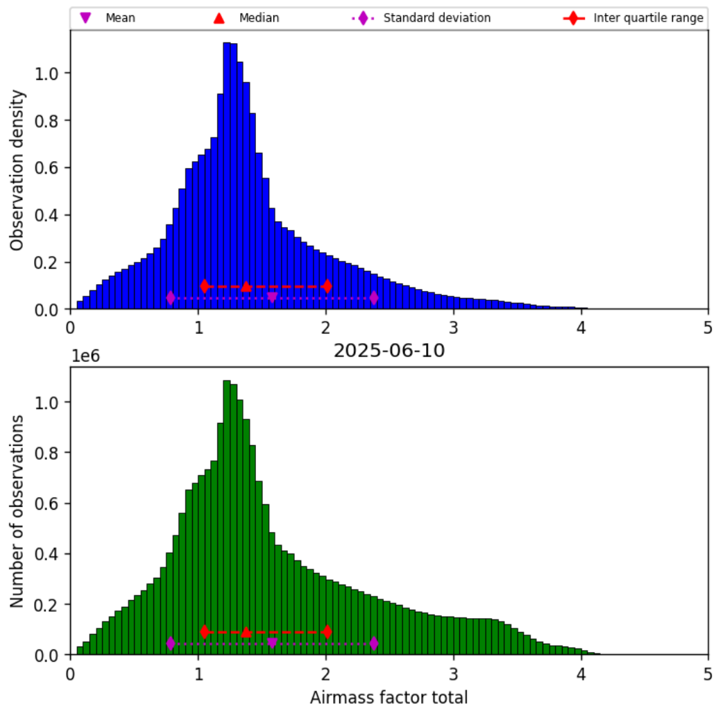
Figure 38: Histogram of “Airmass factor total” for 2025-06-10 to 2025-06-11
