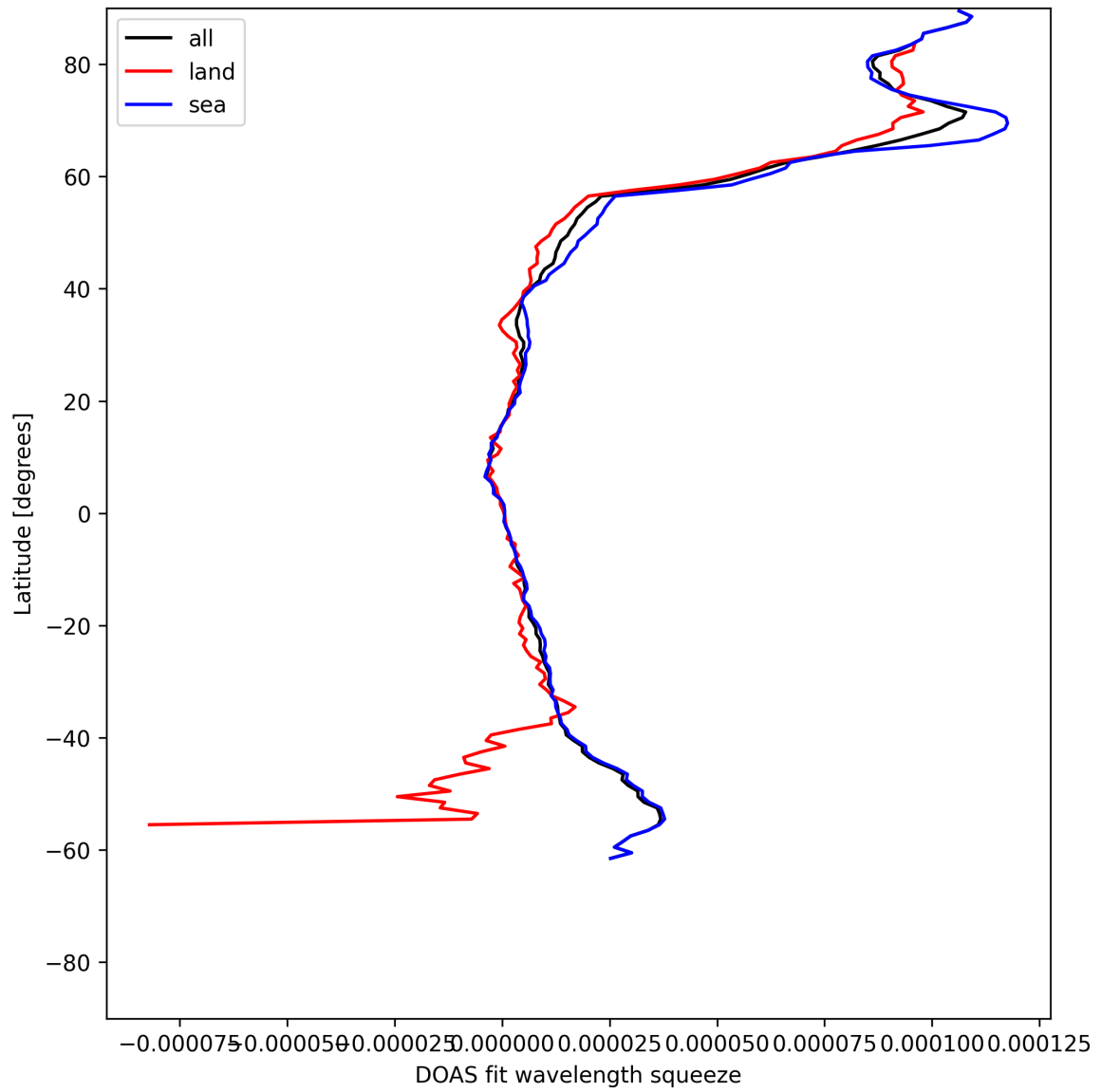
Figure 29: Zonal average of “DOAS fit wavelength squeeze” for 2025-06-10 to 2025-06-11.
