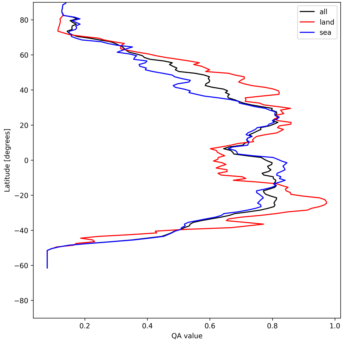
Figure 18: Zonal average of “QA value” for 2025-06-10 to 2025-06-11.
