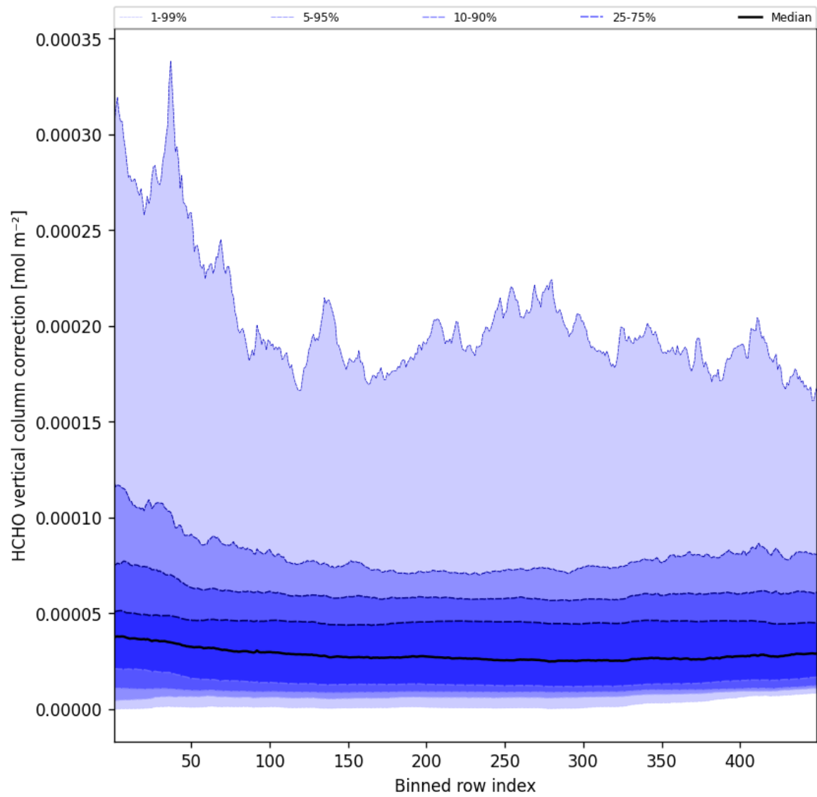
Figure 49: Along track statistics of “HCHO vertical column correction” for 2025-06-10 to 2025-06-11
