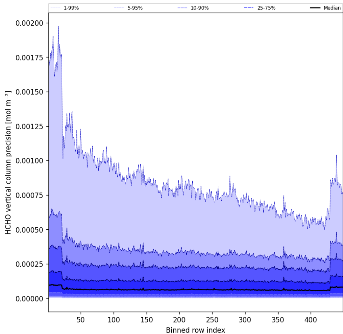
Figure 48: Along track statistics of “HCHO vertical column precision” for 2025-06-10 to 2025-06-11
