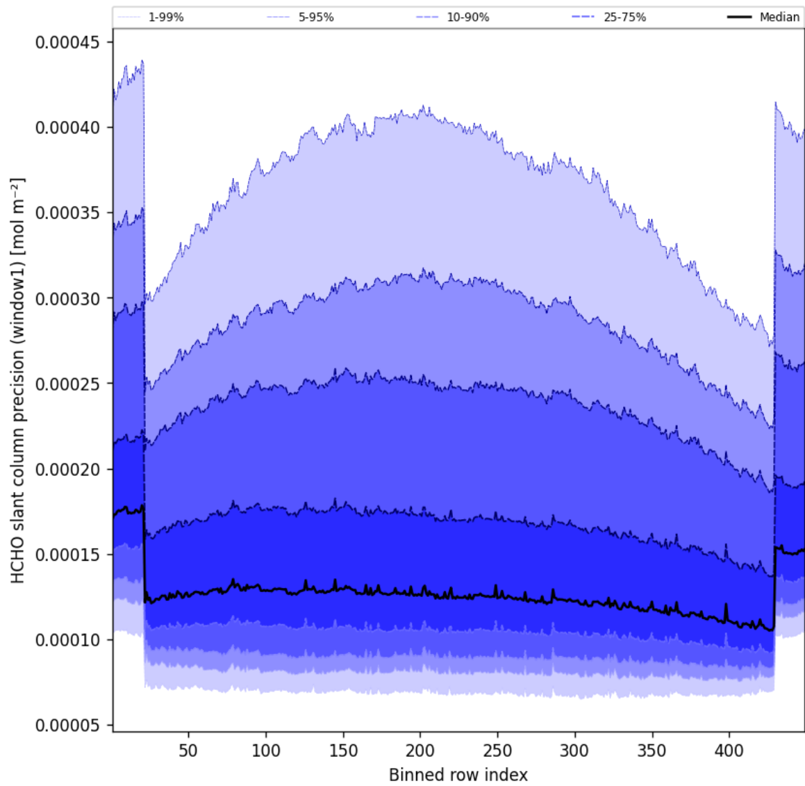
Figure 51: Along track statistics of “HCHO slant column precision (window1)” for 2025-06-10 to 2025-06-11
