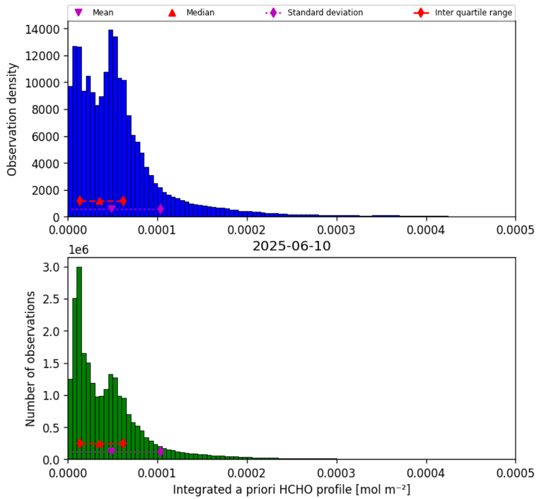
Figure 41: Histogram of “Integrated a priori HCHO profile” for 2025-06-10 to 2025-06-11
