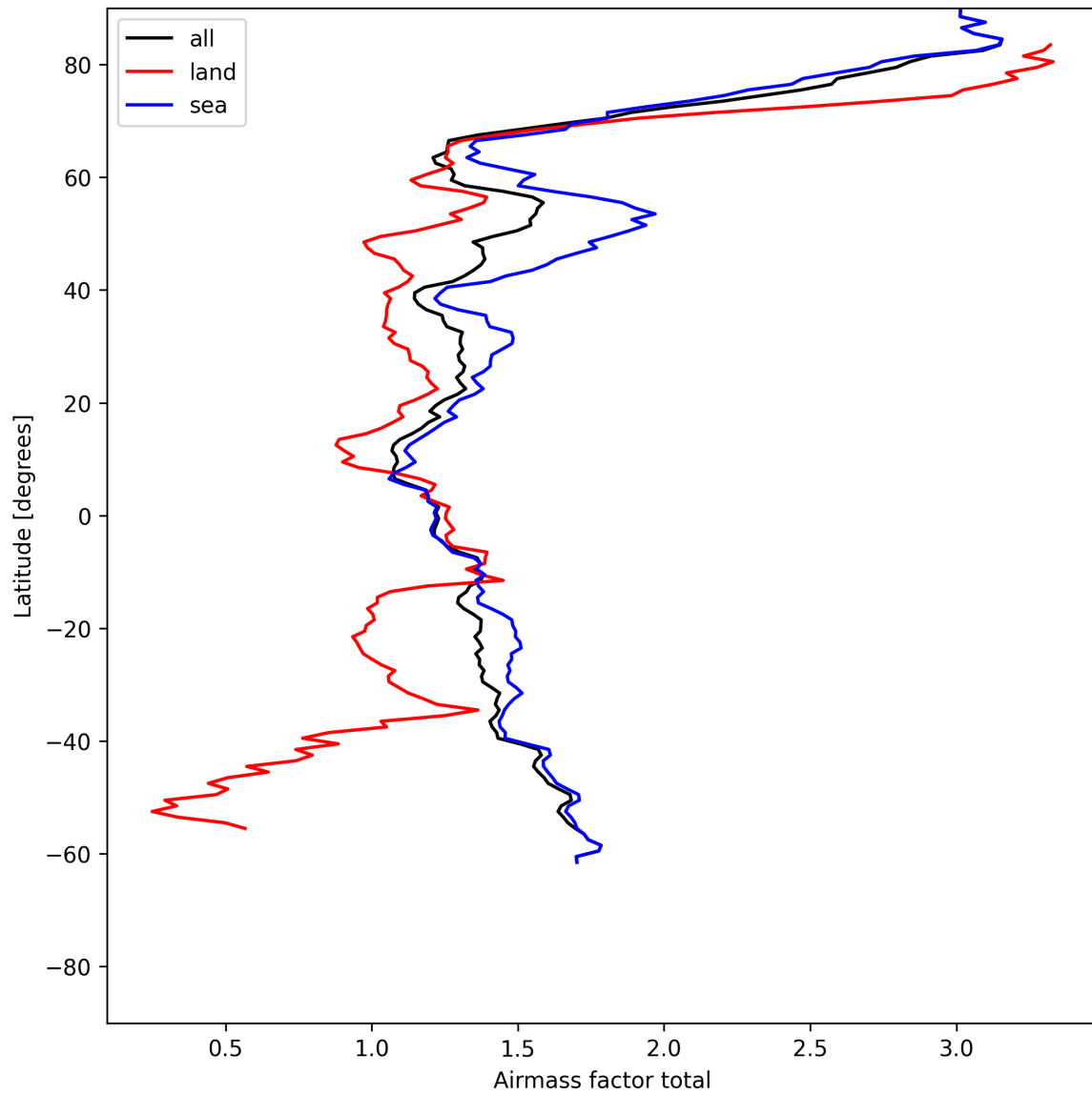
Figure 24: Zonal average of “Airmass factor total” for 2025-06-10 to 2025-06-11.
