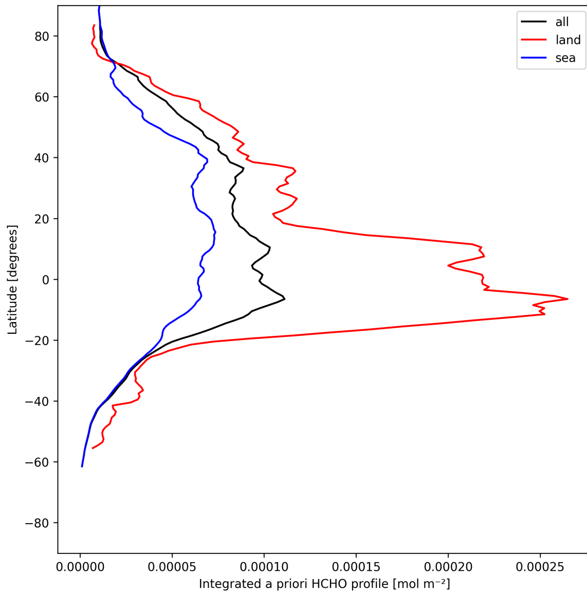
Figure 27: Zonal average of “Integrated a priori HCHO profile” for 2025-06-10 to 2025-06-11.
