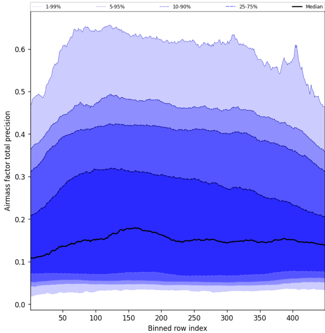
Figure 53: Along track statistics of “Airmass factor total precision” for 2025-06-10 to 2025-06-11
