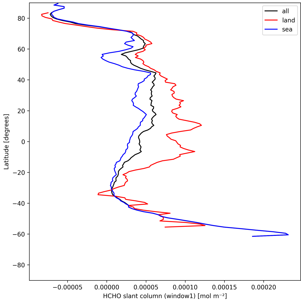
Figure 22: Zonal average of “HCHO slant column (window1)” for 2025-06-10 to 2025-06-11.
