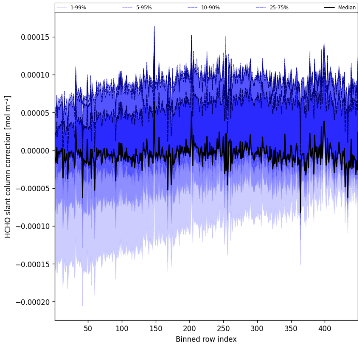
Figure 59: Along track statistics of “HCHO slant column correction” for 2025-06-10 to 2025-06-11
