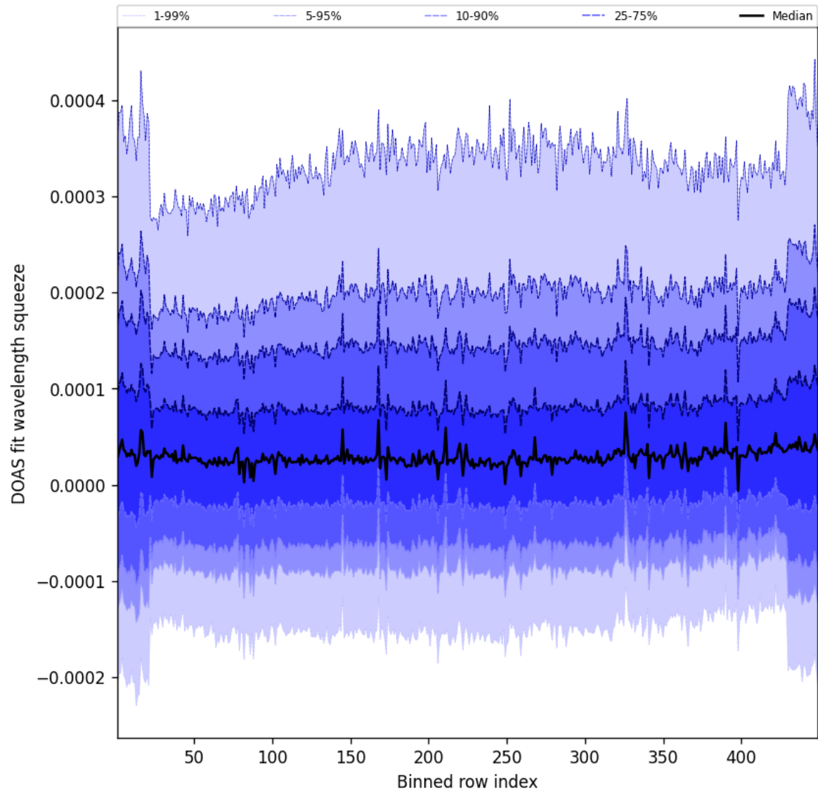
Figure 57: Along track statistics of “DOAS fit wavelength squeeze” for 2025-06-10 to 2025-06-11
