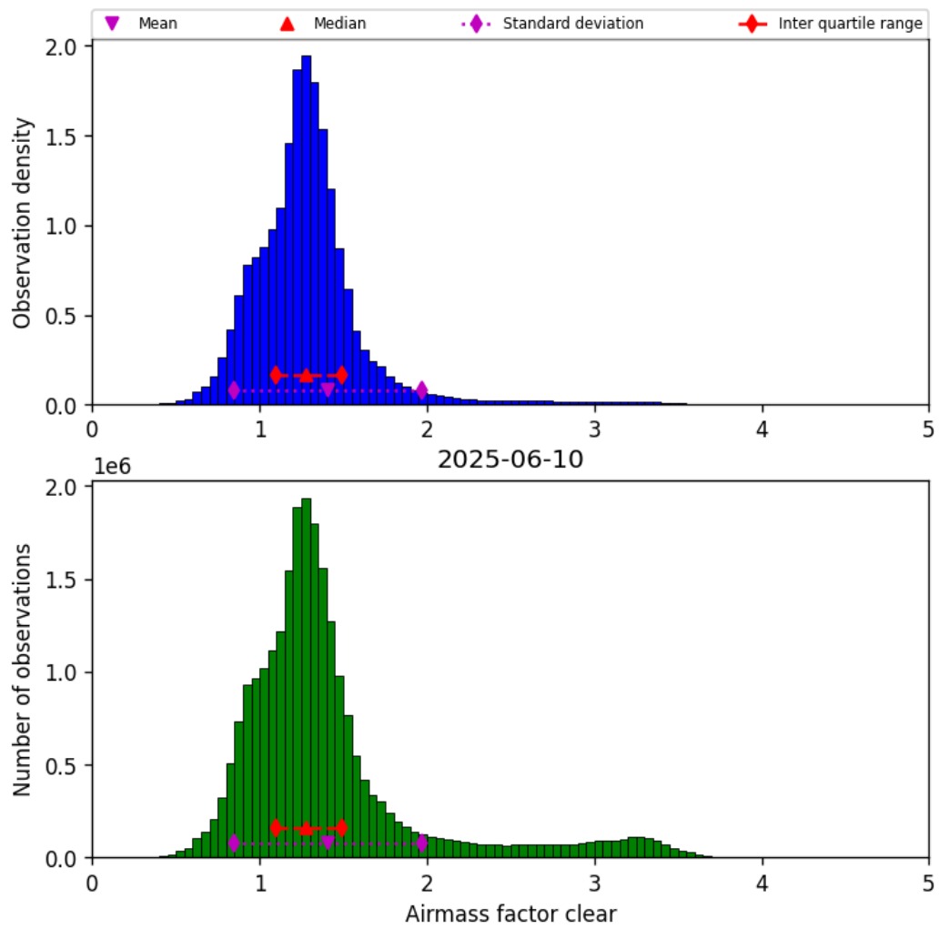
Figure 40: Histogram of “Airmass factor clear” for 2025-06-10 to 2025-06-11
