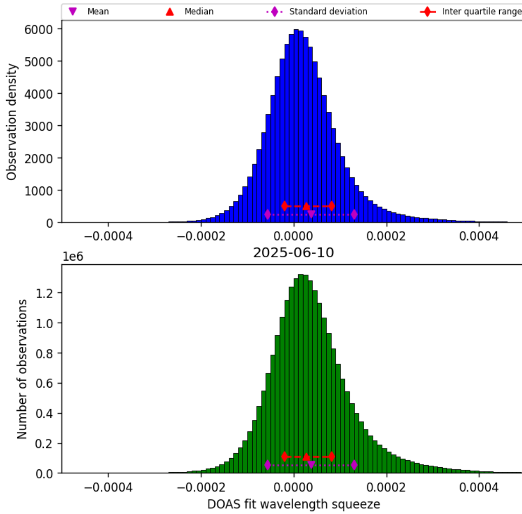
Figure 43: Histogram of “DOAS fit wavelength squeeze” for 2025-06-10 to 2025-06-11
