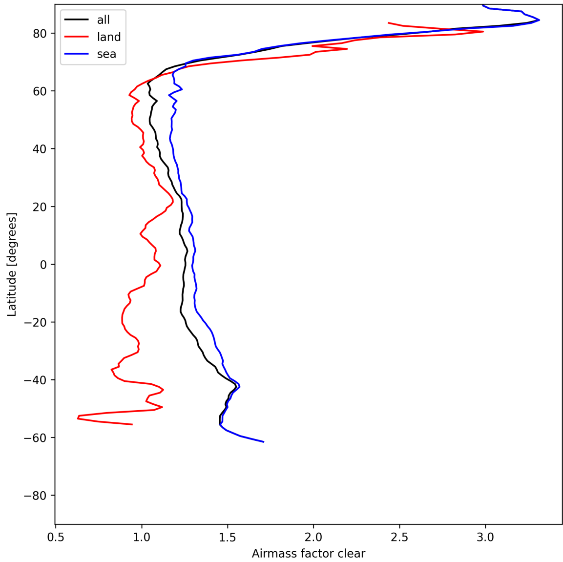
Figure 26: Zonal average of “Airmass factor clear” for 2025-06-10 to 2025-06-11.
