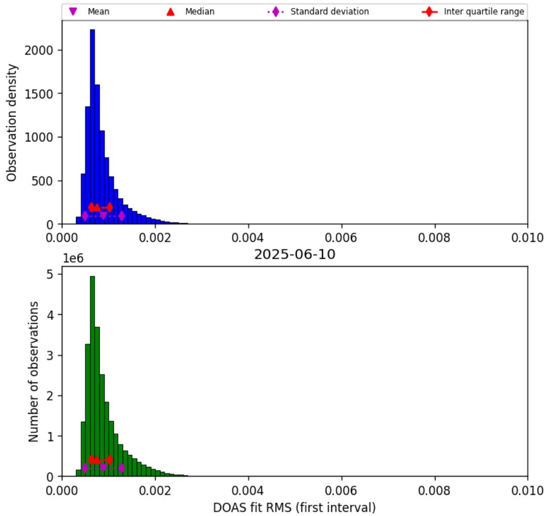
Figure 44: Histogram of “DOAS fit RMS (first interval)” for 2025-06-10 to 2025-06-11
