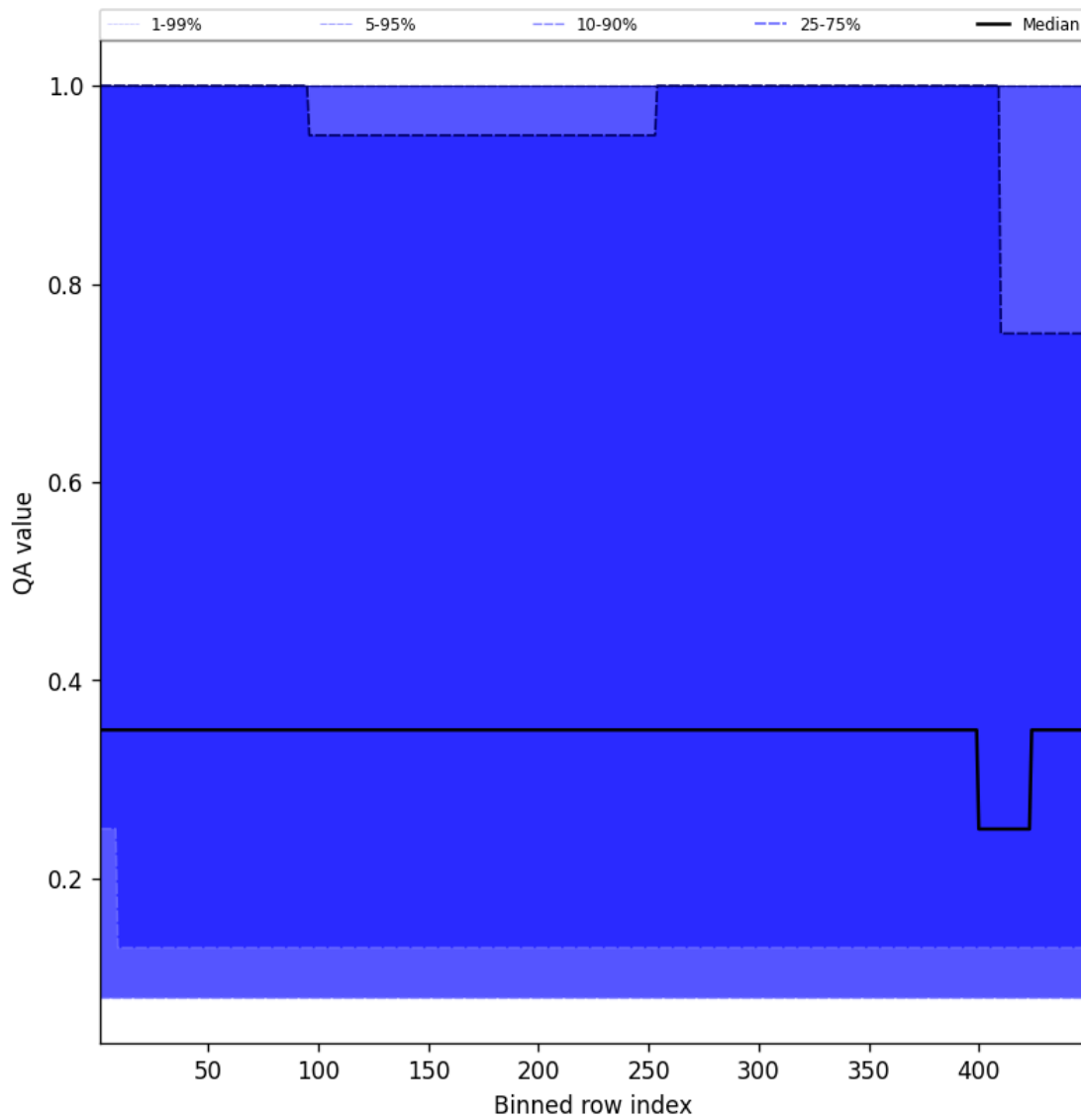
Figure 46: Along track statistics of “QA value” for 2025-06-10 to 2025-06-11
