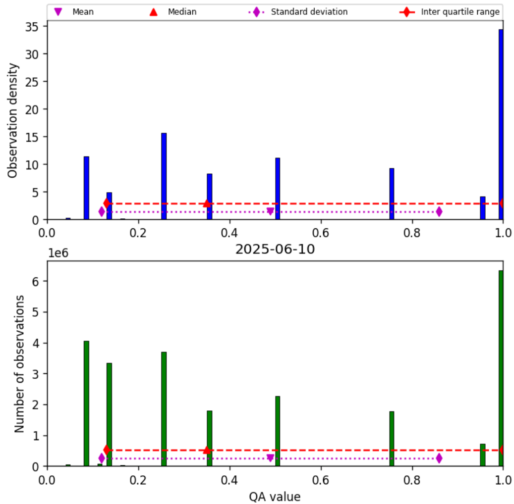
Figure 32: Histogram of “QA value” for 2025-06-10 to 2025-06-11
