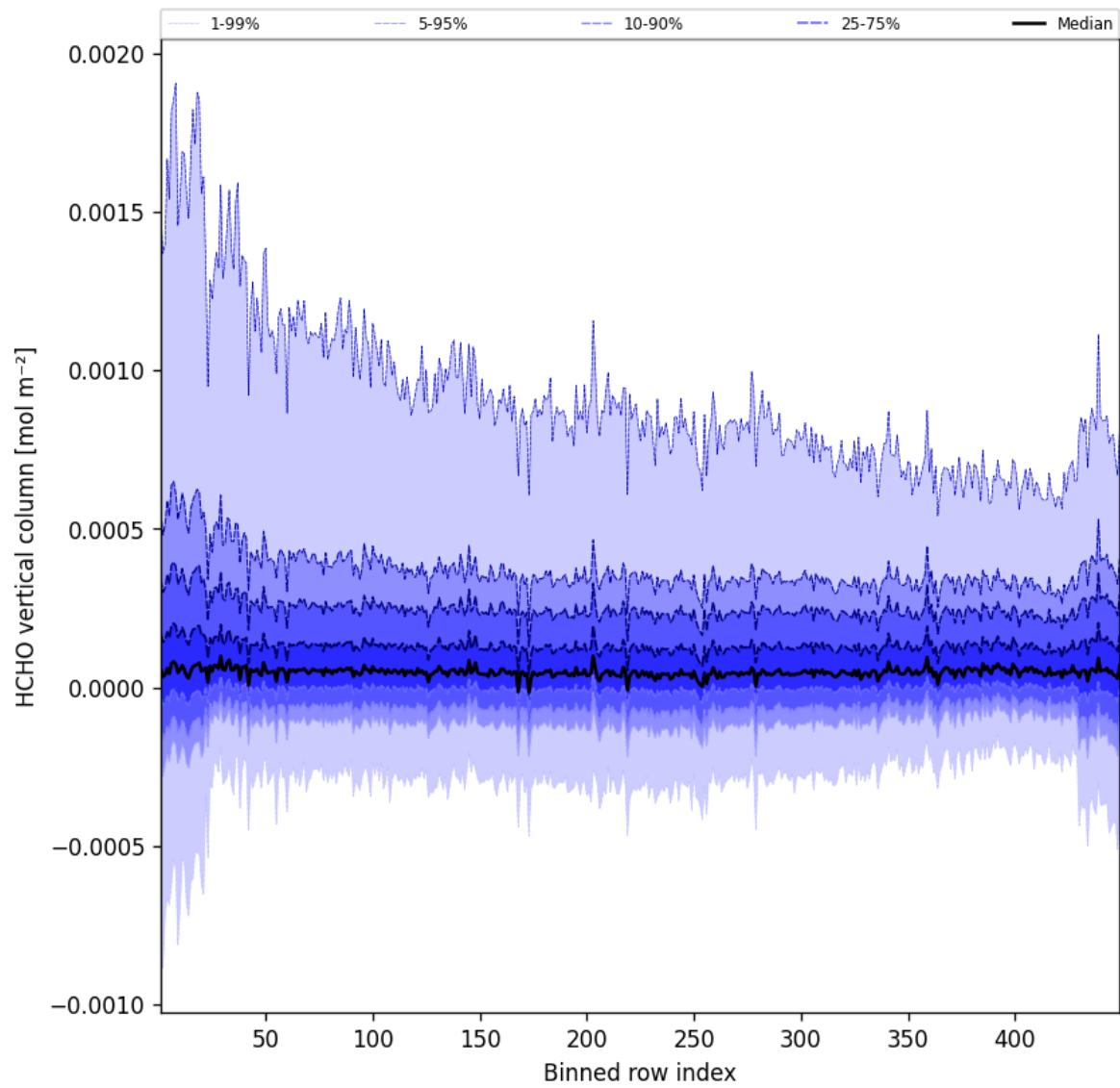
Figure 47: Along track statistics of “HCHO vertical column” for 2025-06-10 to 2025-06-11
