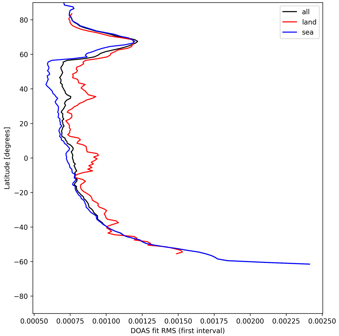
Figure 30: Zonal average of “DOAS fit RMS (first interval)” for 2025-06-10 to 2025-06-11.
