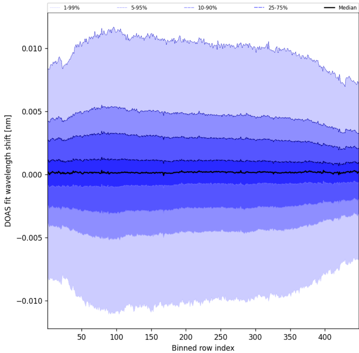
Figure 56: Along track statistics of “DOAS fit wavelength shift” for 2025-06-10 to 2025-06-11
