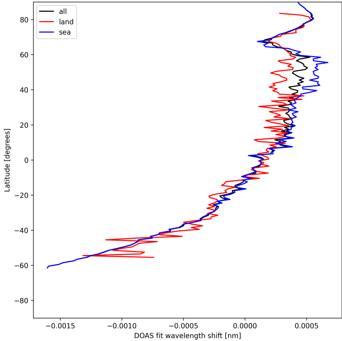
Figure 28: Zonal average of “DOAS fit wavelength shift” for 2025-06-10 to 2025-06-11.
