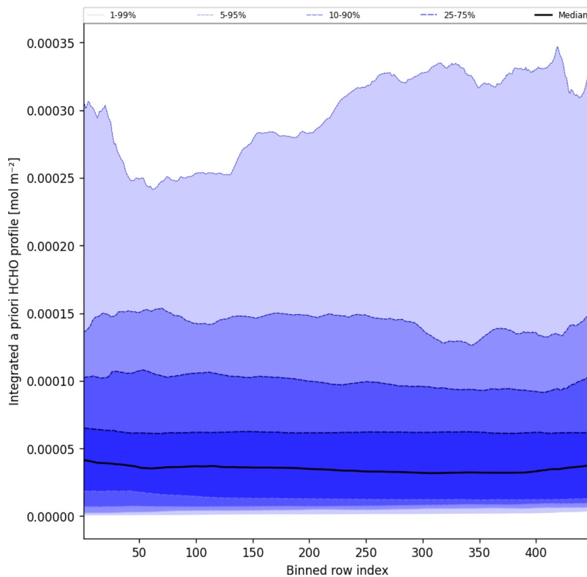
Figure 55: Along track statistics of “Integrated a priori HCHO profile” for 2025-06-10 to 2025-06-11
