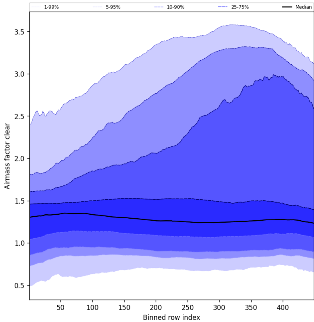
Figure 54: Along track statistics of “Airmass factor clear” for 2025-06-10 to 2025-06-11
