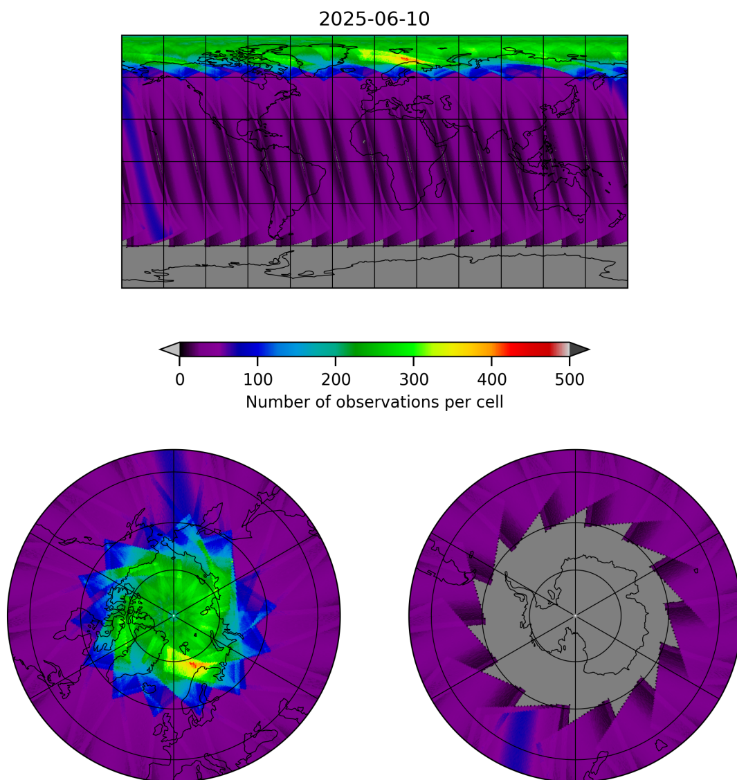
Figure 17: Map of the number of observations for 2025-06-10 to 2025-06-11
