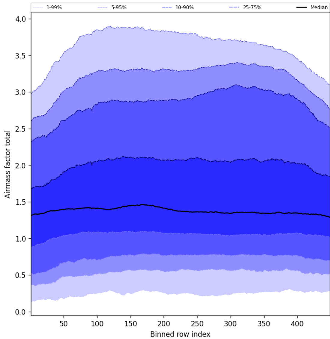
Figure 52: Along track statistics of “Airmass factor total” for 2025-06-10 to 2025-06-11
