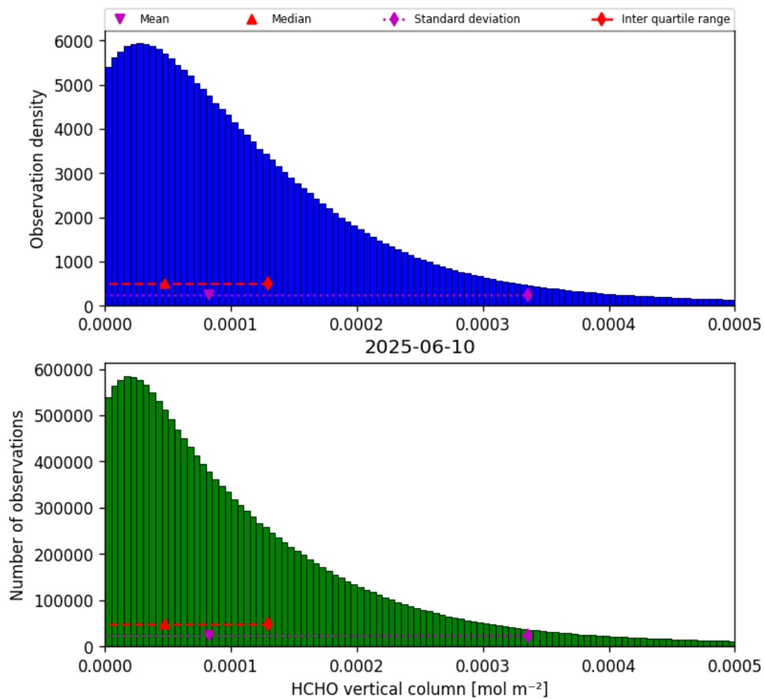
Figure 33: Histogram of “HCHO vertical column” for 2025-06-10 to 2025-06-11
