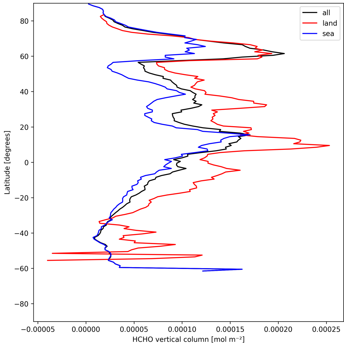
Figure 19: Zonal average of “HCHO vertical column” for 2025-06-10 to 2025-06-11.
