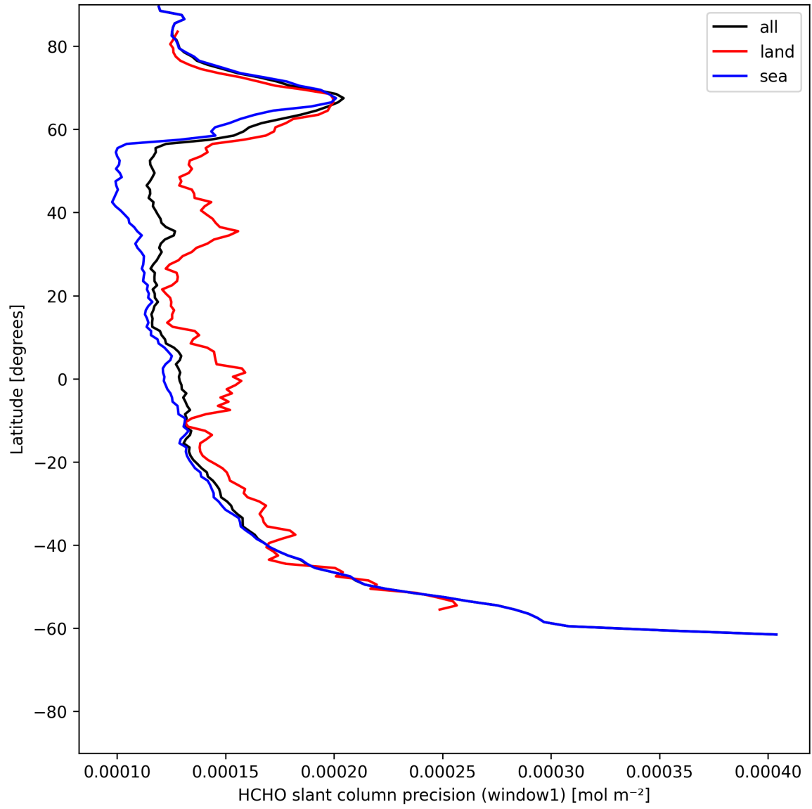
Figure 23: Zonal average of “HCHO slant column precision (window1)” for 2025-06-10 to 2025-06-11.
