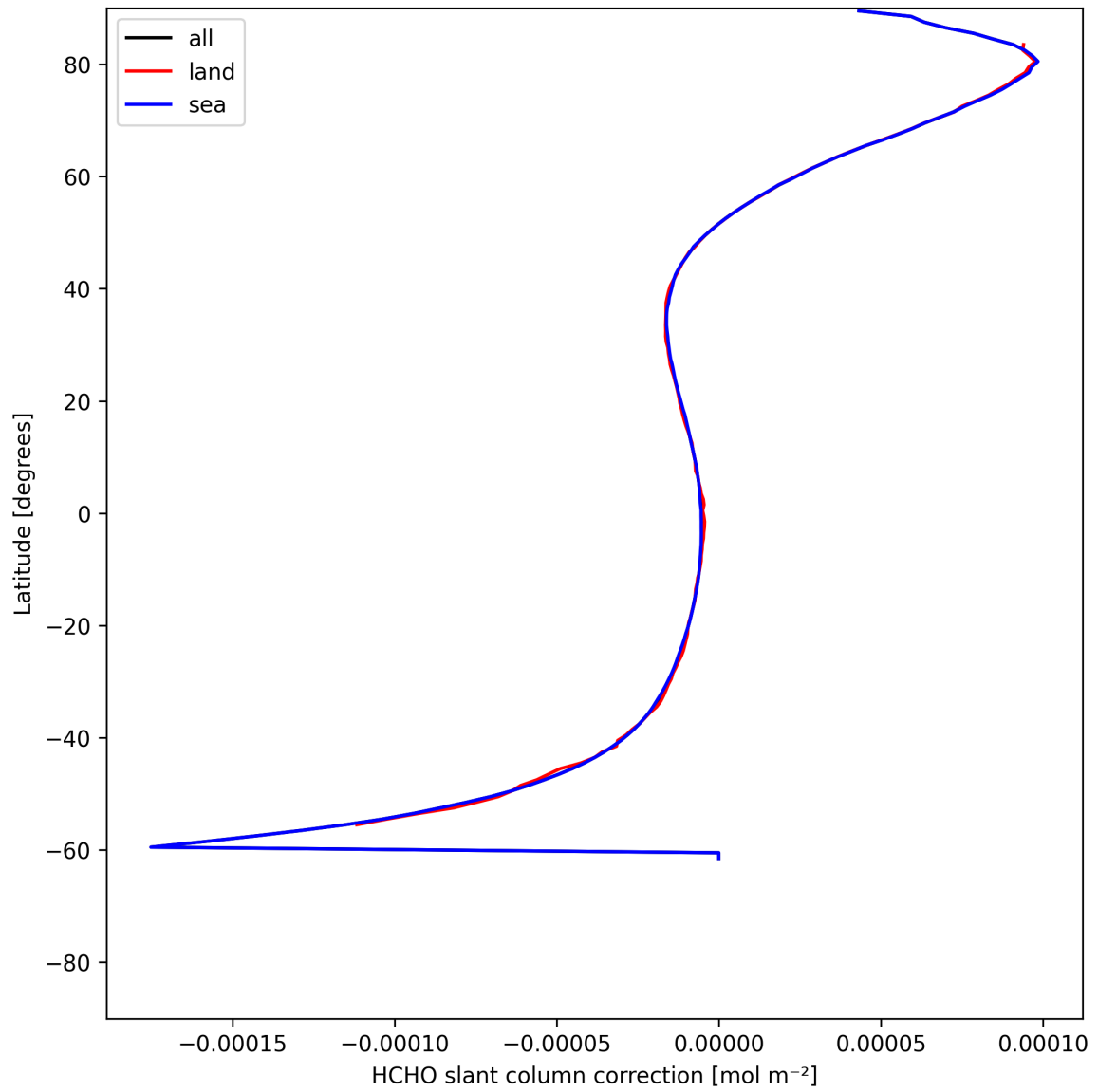
Figure 31: Zonal average of “HCHO slant column correction” for 2025-06-10 to 2025-06-11.
