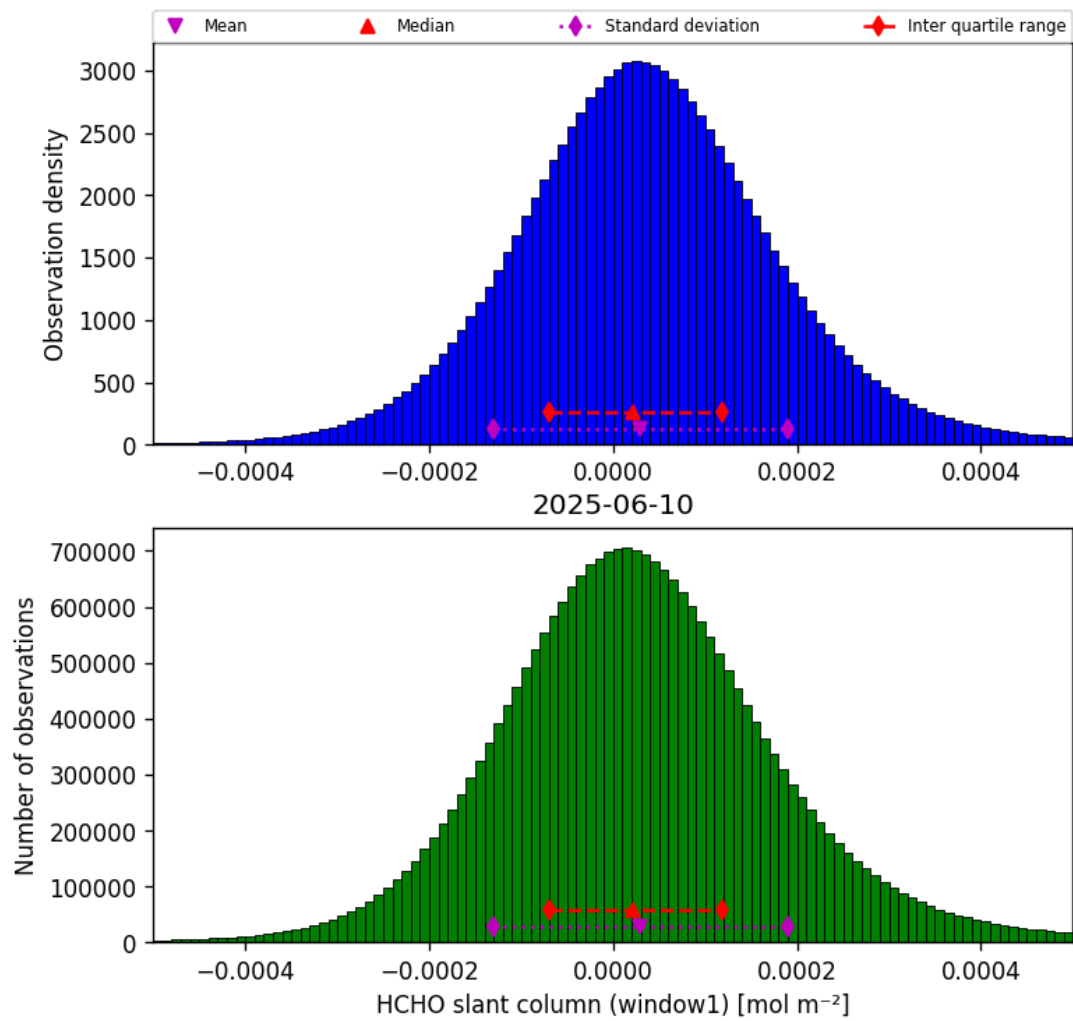
Figure 36: Histogram of “HCHO slant column (window1)” for 2025-06-10 to 2025-06-11
