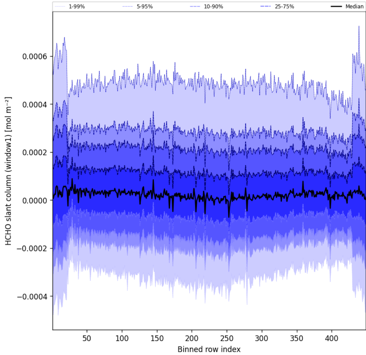
Figure 50: Along track statistics of “HCHO slant column (window1)” for 2025-06-10 to 2025-06-11
