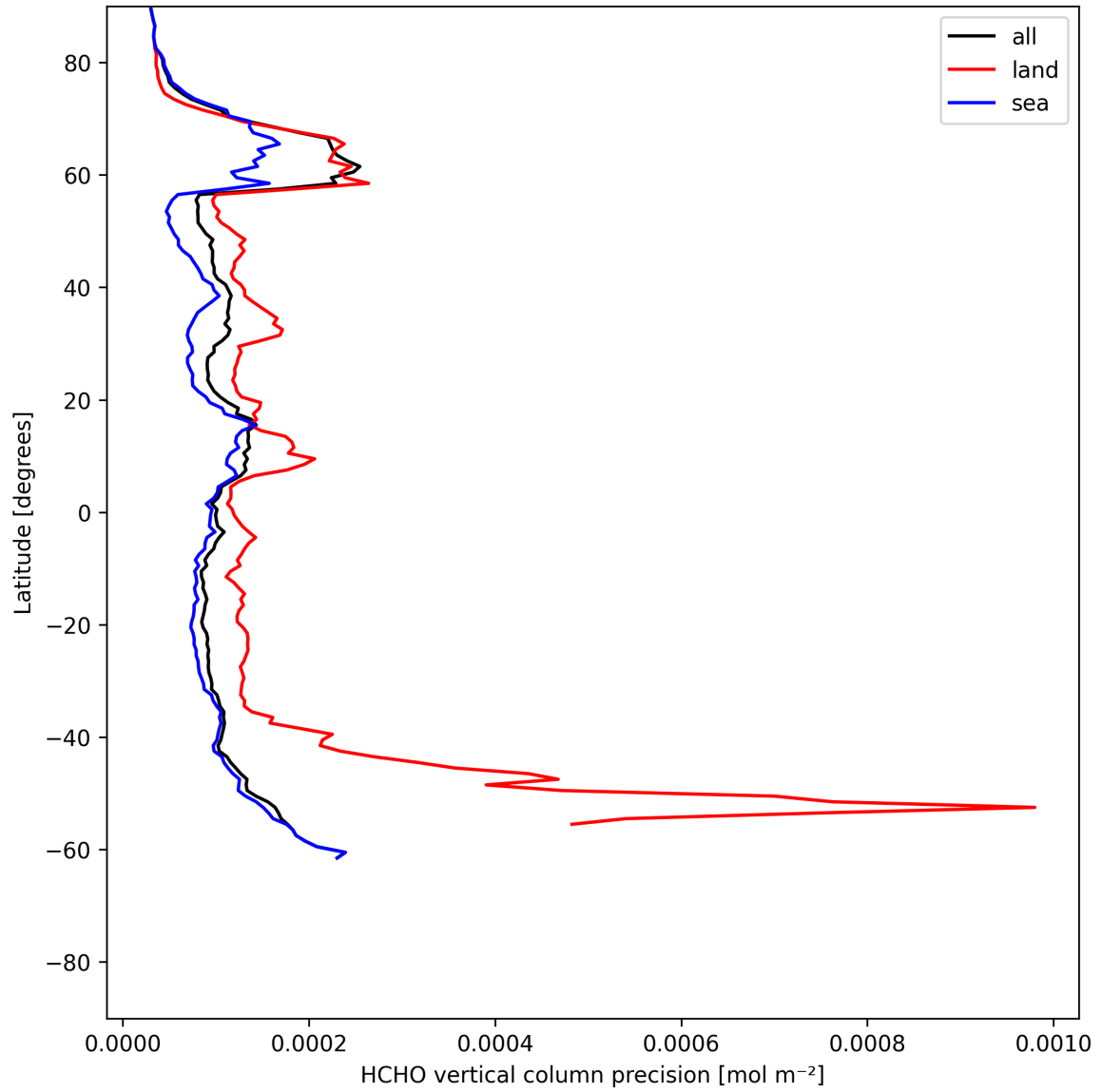
Figure 20: Zonal average of “HCHO vertical column precision” for 2025-06-10 to 2025-06-11.
