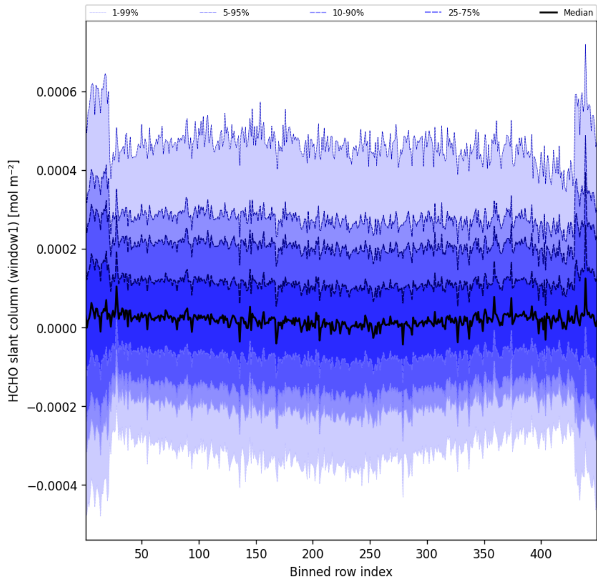
Figure 50: Along track statistics of “HCHO slant column (window1)” for 2025-06-12 to 2025-06-13
