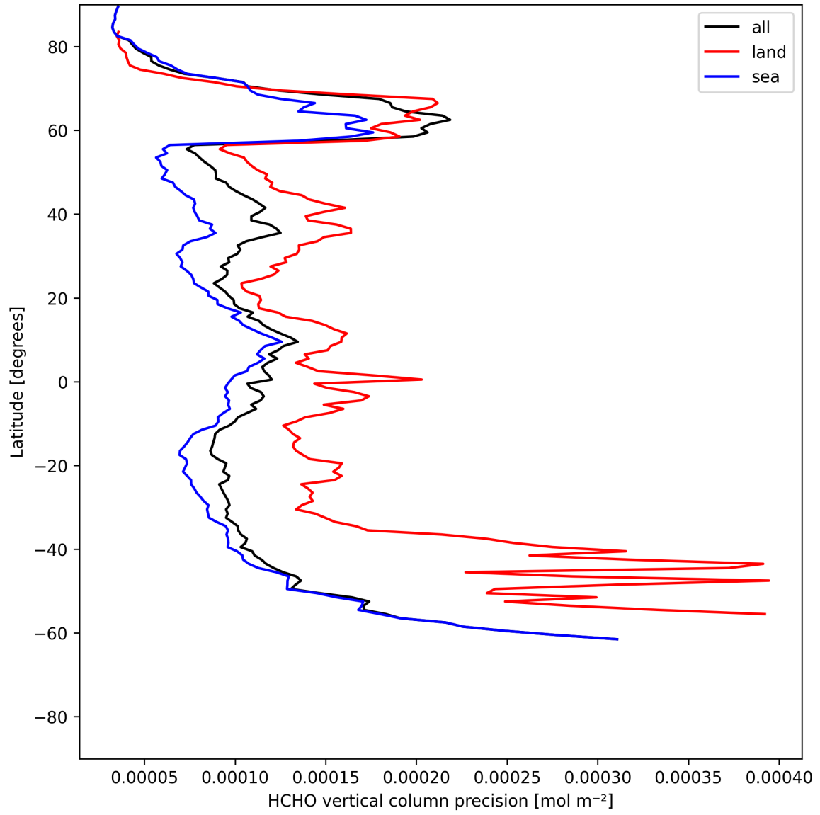
Figure 20: Zonal average of “HCHO vertical column precision” for 2025-06-12 to 2025-06-13.
