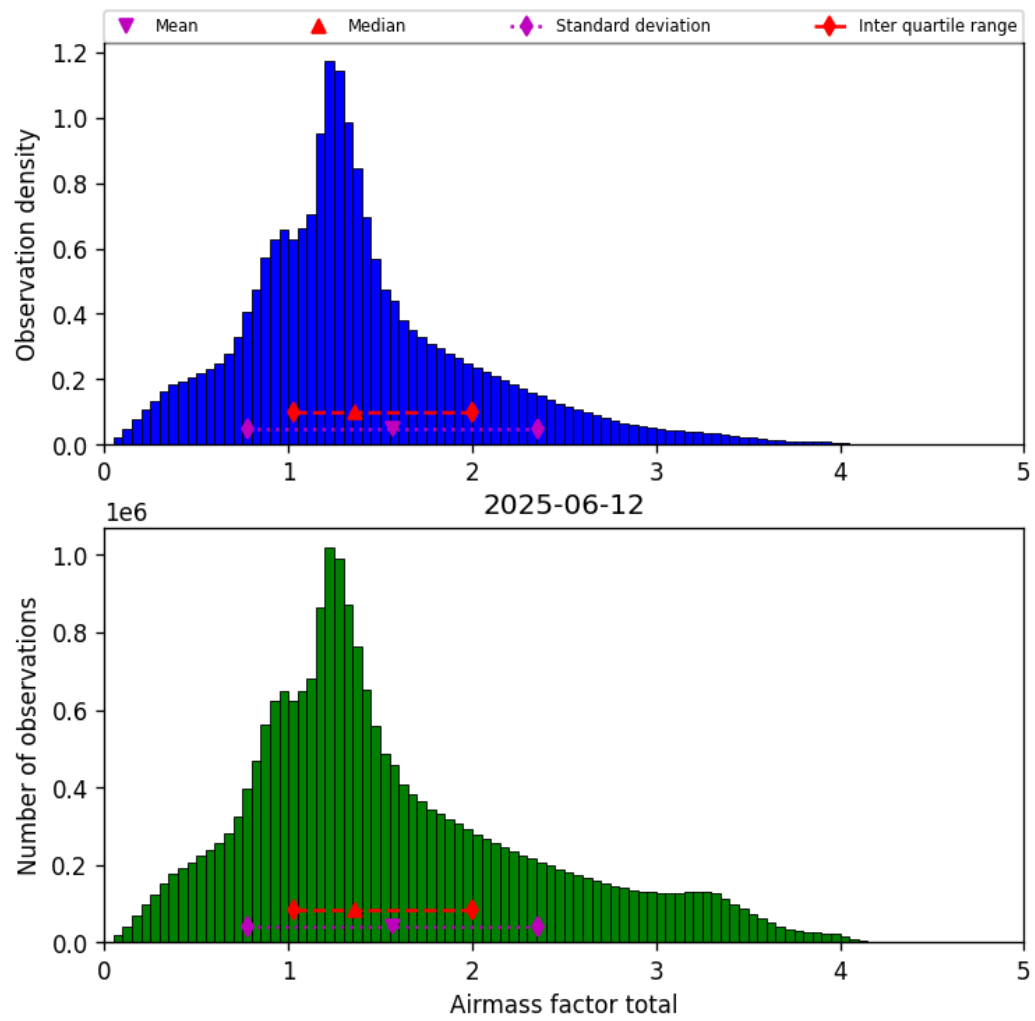
Figure 38: Histogram of “Airmass factor total” for 2025-06-12 to 2025-06-13
