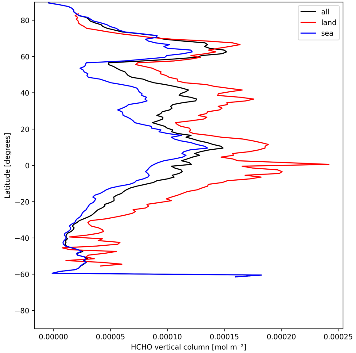
Figure 19: Zonal average of “HCHO vertical column” for 2025-06-12 to 2025-06-13.
