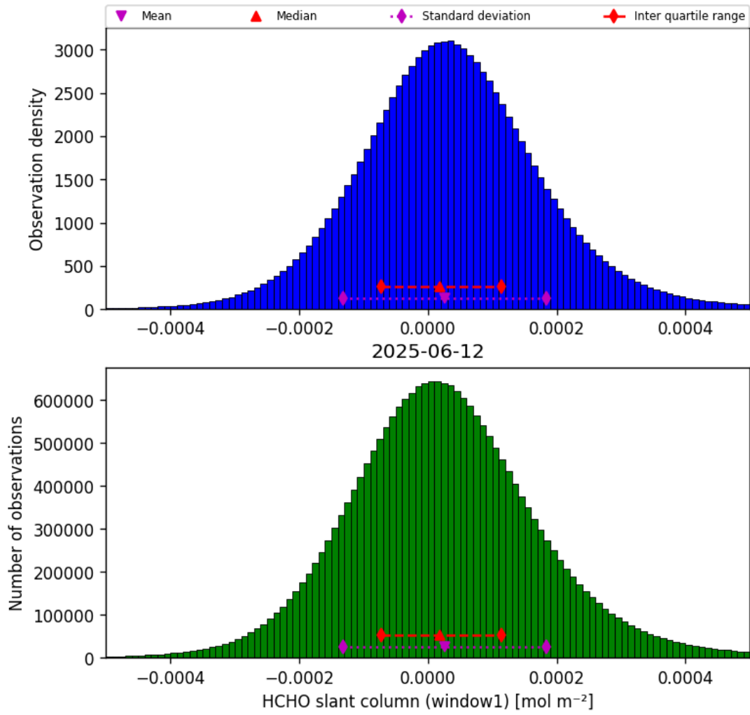
Figure 36: Histogram of “HCHO slant column (window1)” for 2025-06-12 to 2025-06-13
