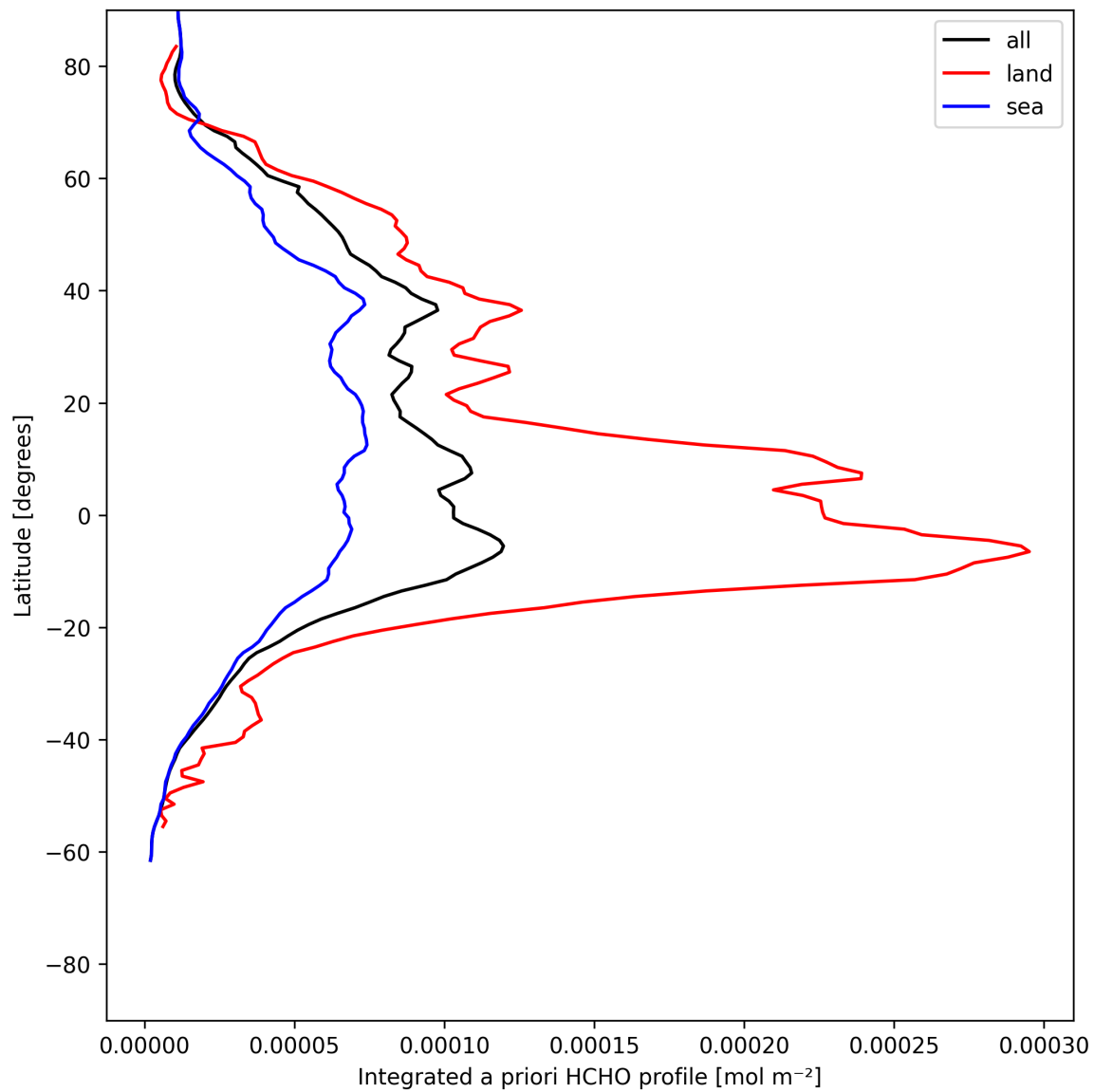
Figure 27: Zonal average of “Integrated a priori HCHO profile” for 2025-06-12 to 2025-06-13.
