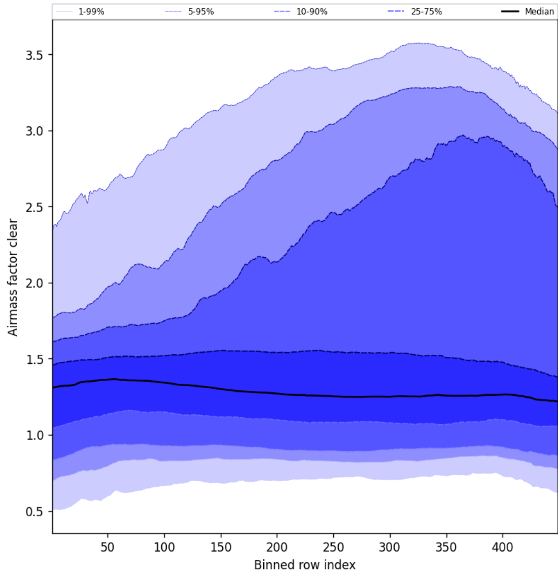
Figure 54: Along track statistics of “Airmass factor clear” for 2025-06-12 to 2025-06-13
