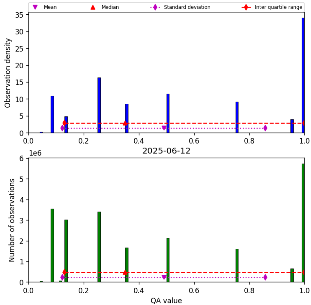
Figure 32: Histogram of “QA value” for 2025-06-12 to 2025-06-13
