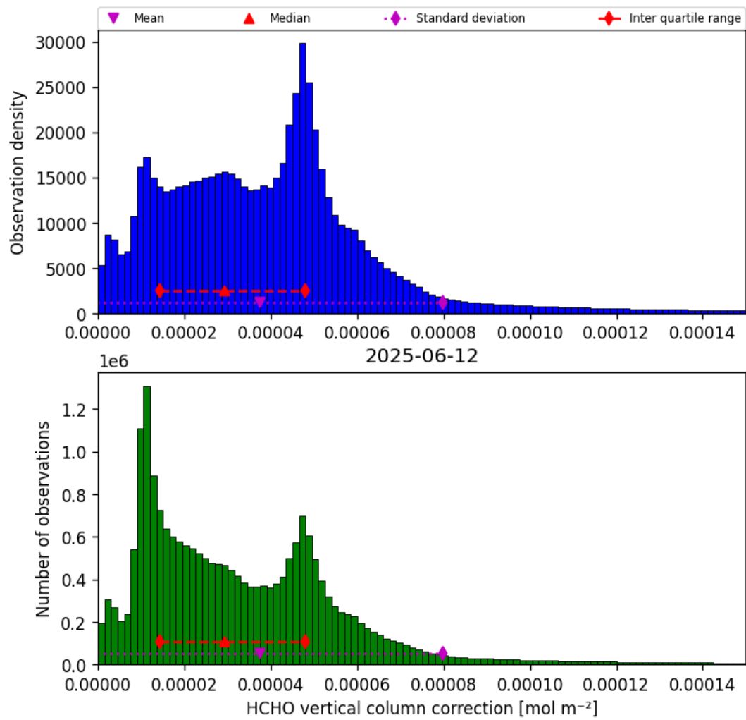
Figure 35: Histogram of “HCHO vertical column correction” for 2025-06-12 to 2025-06-13
