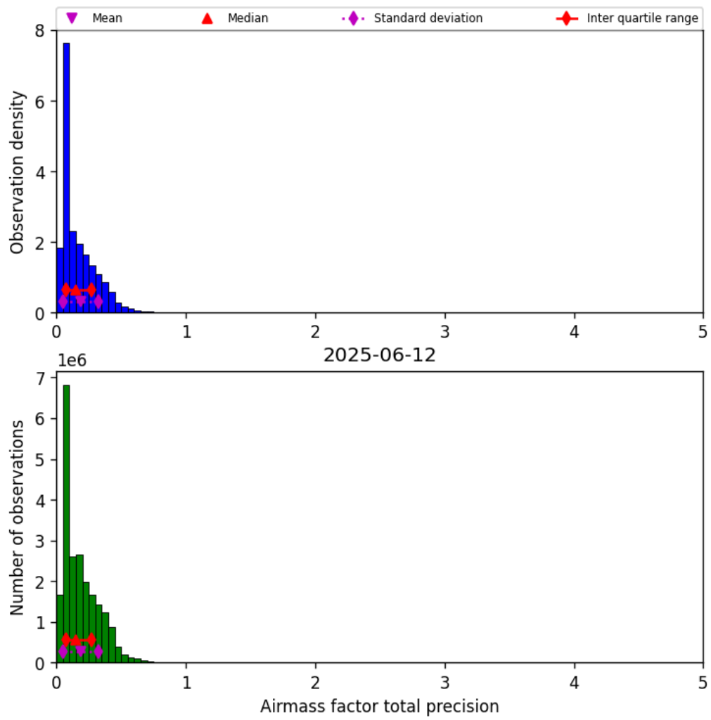
Figure 39: Histogram of “Airmass factor total precision” for 2025-06-12 to 2025-06-13
