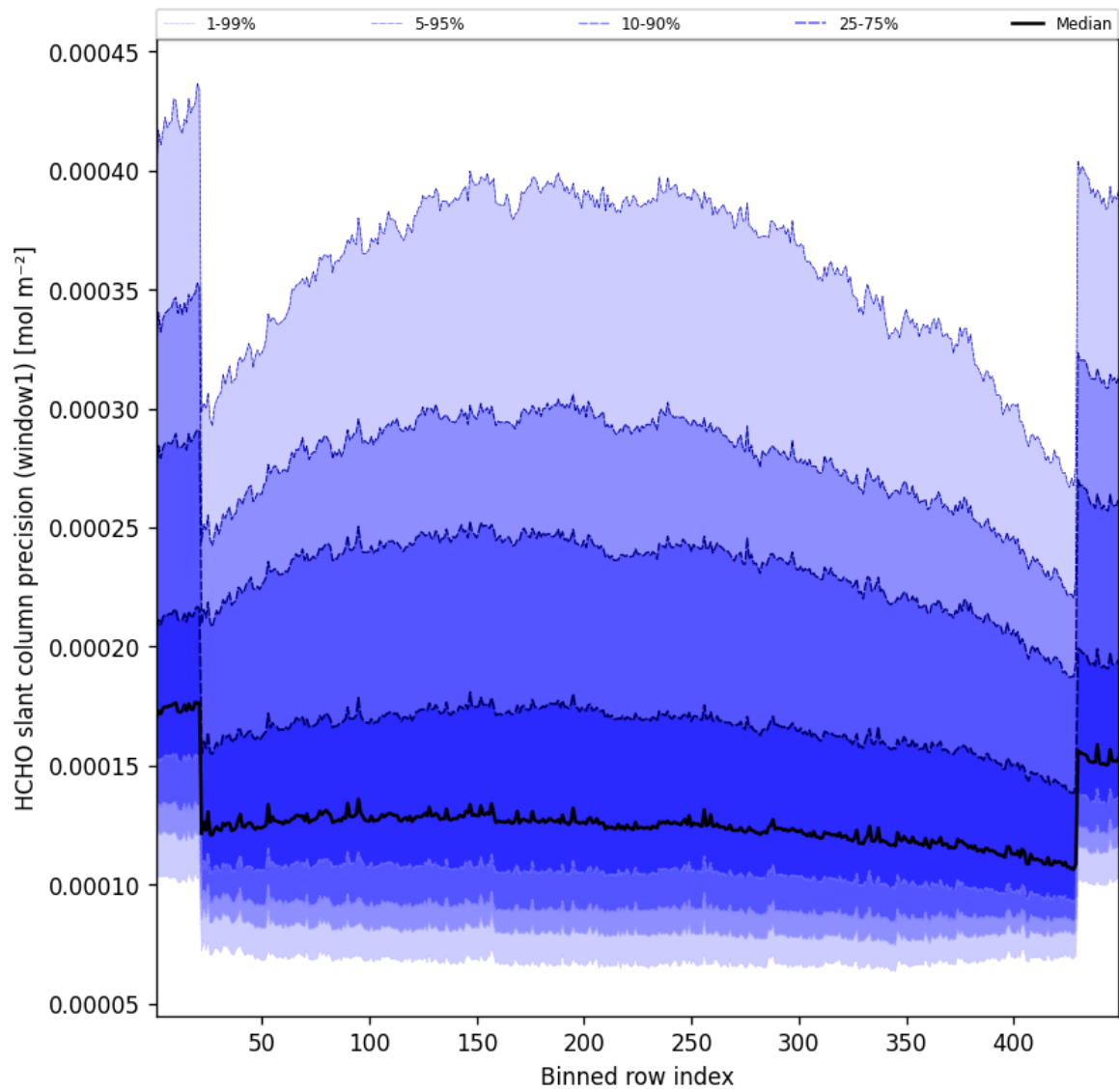
Figure 51: Along track statistics of “HCHO slant column precision (window1)” for 2025-06-12 to 2025-06-13
