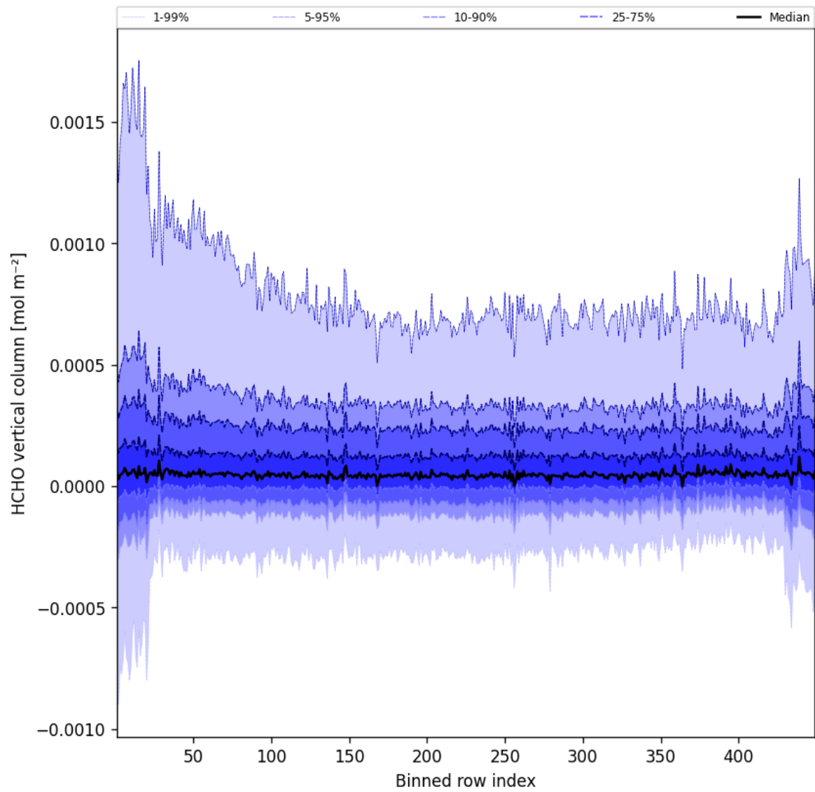
Figure 47: Along track statistics of “HCHO vertical column” for 2025-06-12 to 2025-06-13
