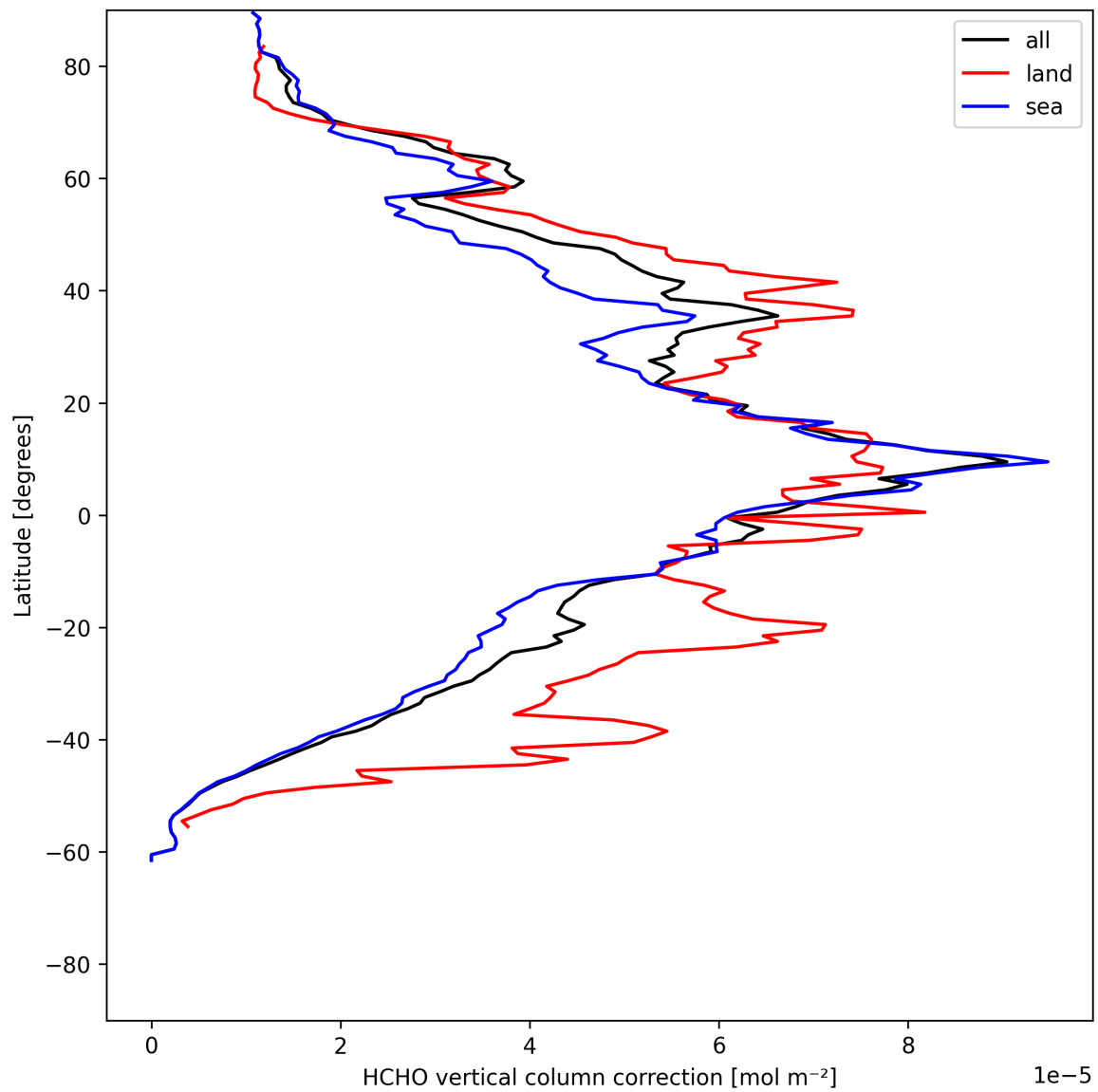
Figure 21: Zonal average of “HCHO vertical column correction” for 2025-06-12 to 2025-06-13.
