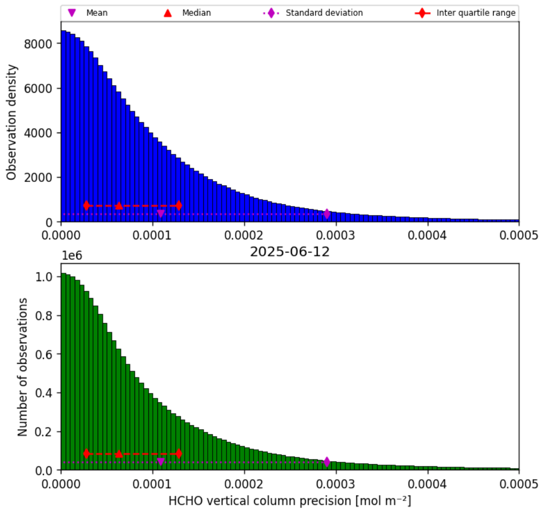
Figure 34: Histogram of “HCHO vertical column precision” for 2025-06-12 to 2025-06-13
