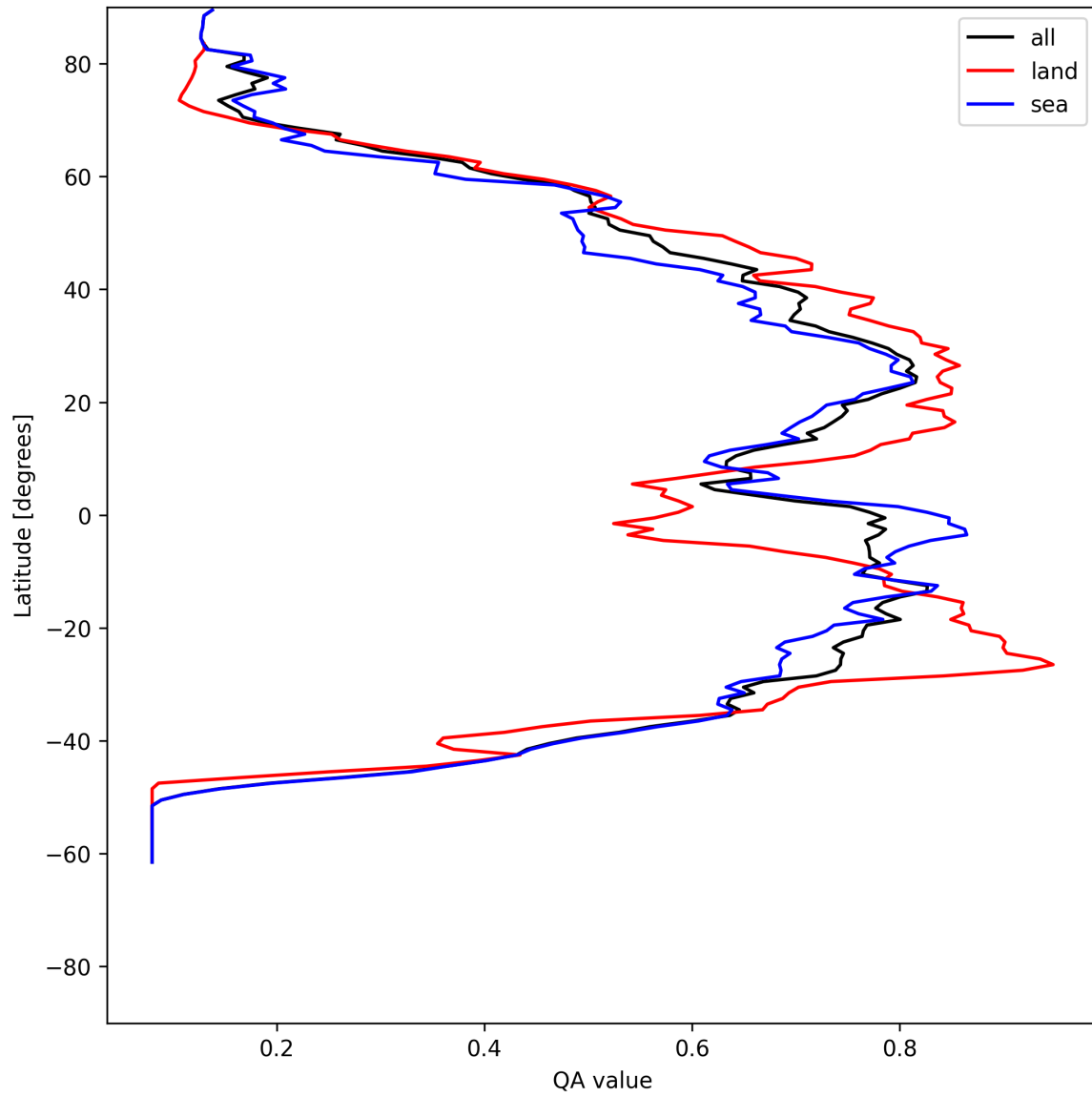
Figure 18: Zonal average of “QA value” for 2025-06-12 to 2025-06-13.
