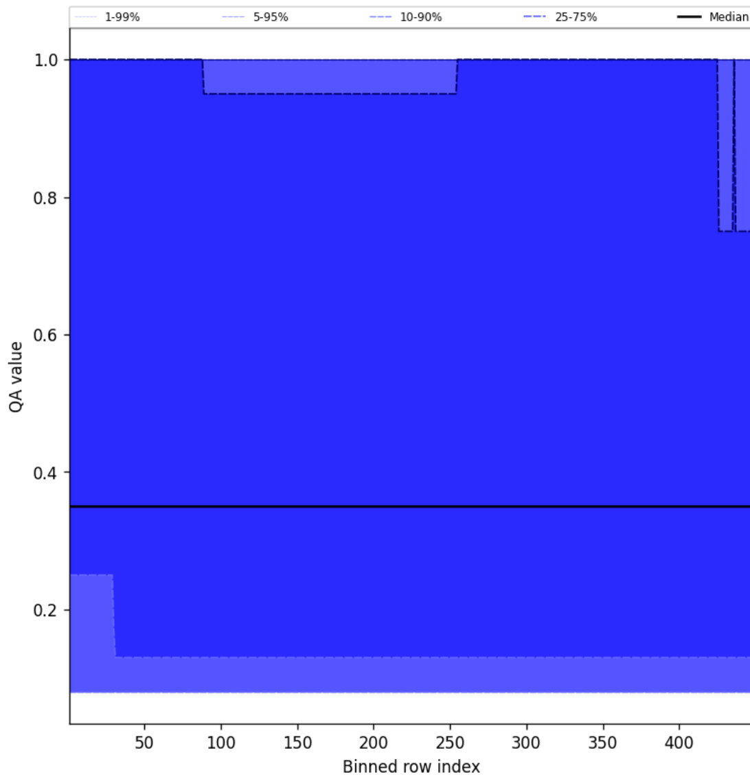
Figure 46: Along track statistics of "QA value" for 2025-06-12 to 2025-06-13
