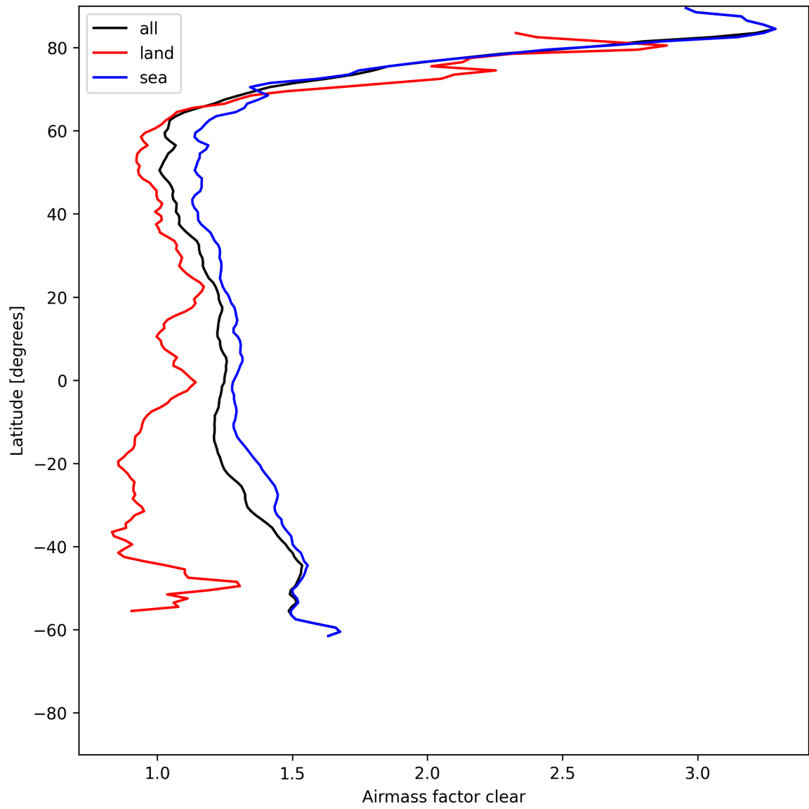
Figure 26: Zonal average of “Airmass factor clear” for 2025-06-12 to 2025-06-13.
