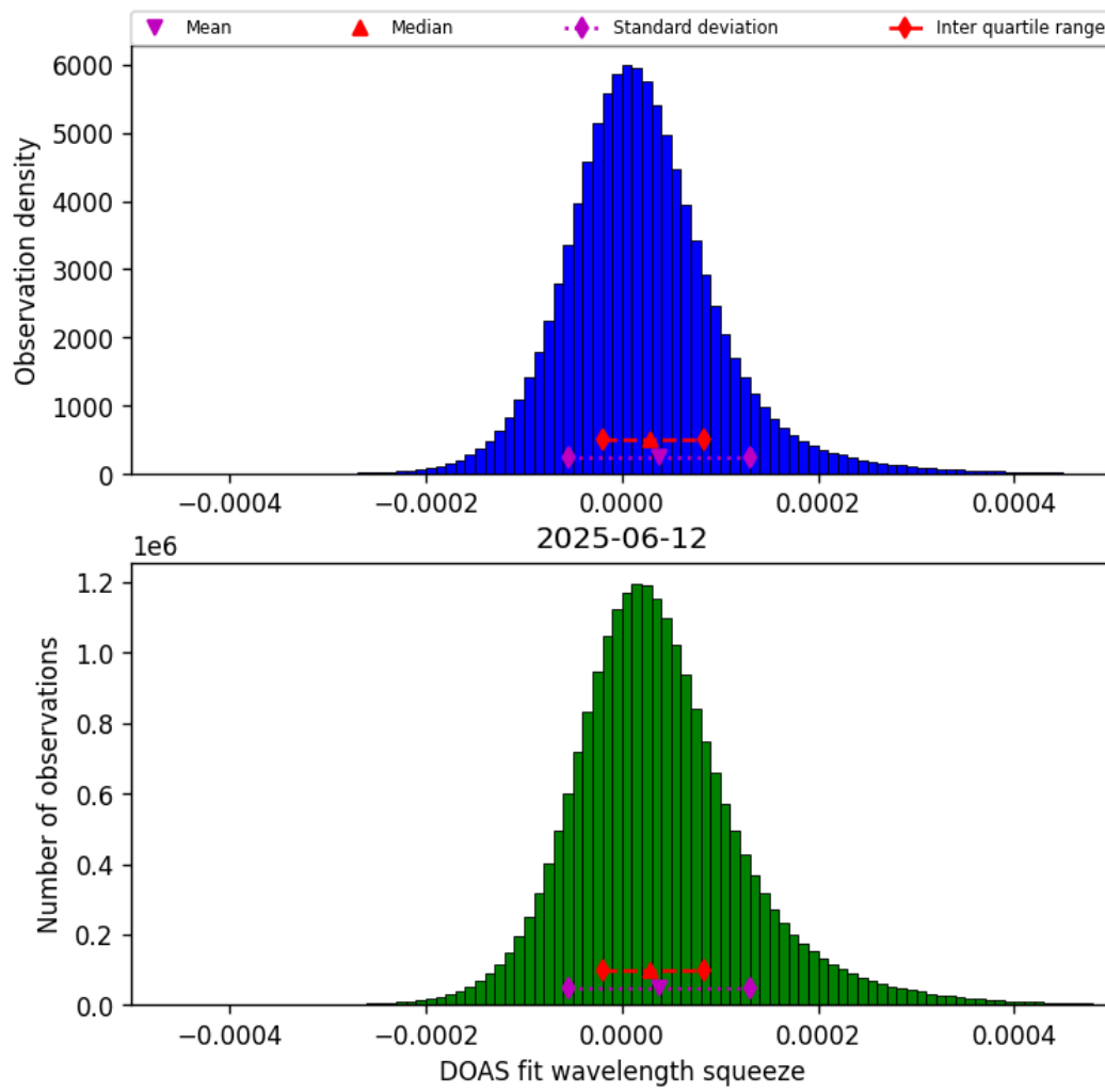
Figure 43: Histogram of “DOAS fit wavelength squeeze” for 2025-06-12 to 2025-06-13
