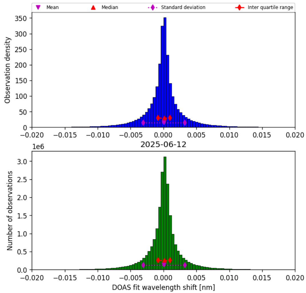
Figure 42: Histogram of “DOAS fit wavelength shift” for 2025-06-12 to 2025-06-13
