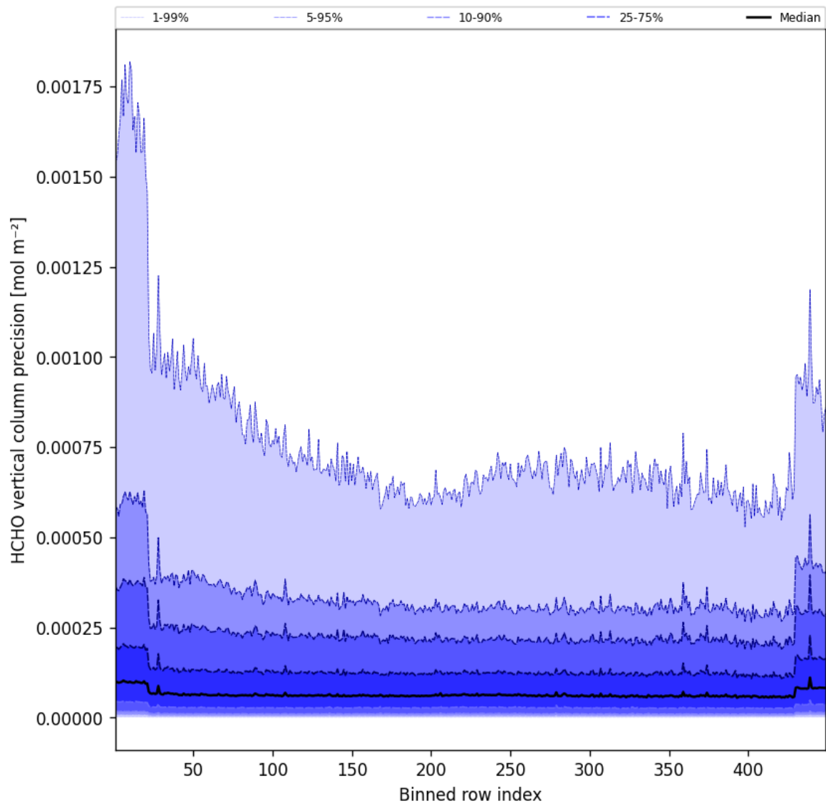
Figure 48: Along track statistics of “HCHO vertical column precision” for 2025-06-12 to 2025-06-13
