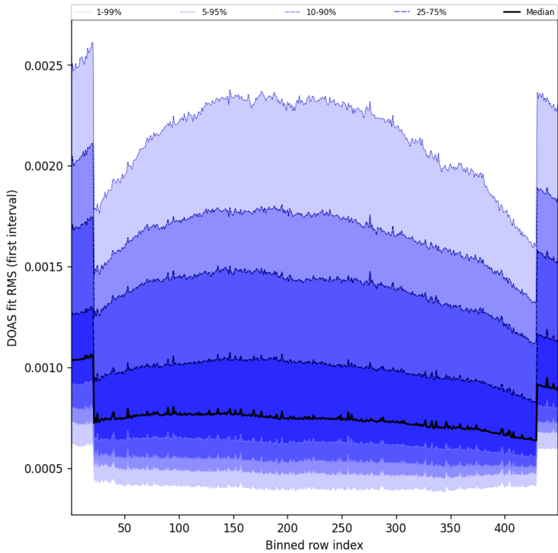
Figure 58: Along track statistics of “DOAS fit RMS (first interval)” for 2025-06-12 to 2025-06-13
