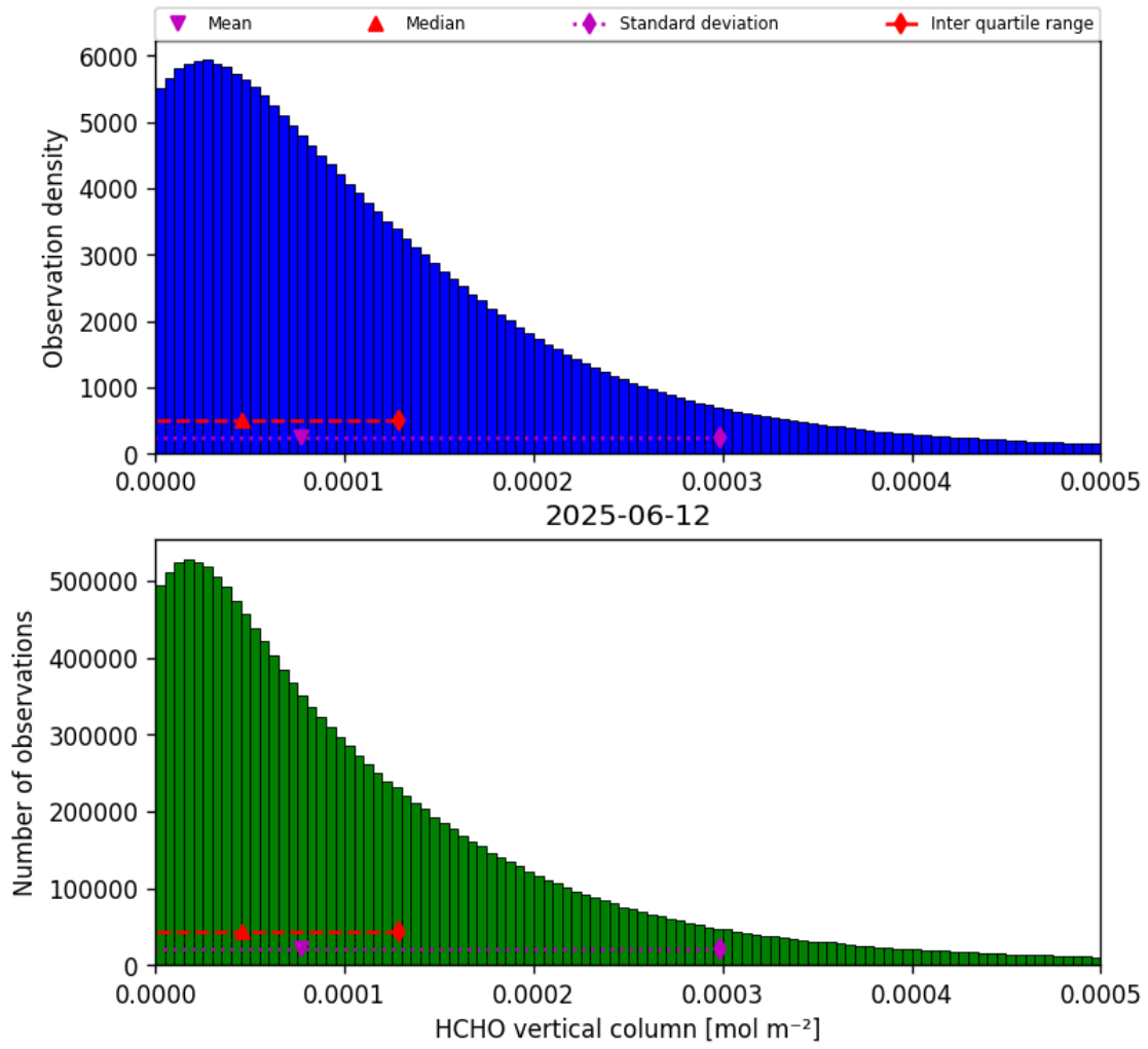
Figure 33: Histogram of “HCHO vertical column” for 2025-06-12 to 2025-06-13
