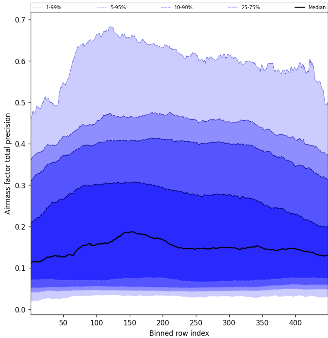
Figure 53: Along track statistics of “Airmass factor total precision” for 2025-06-12 to 2025-06-13
