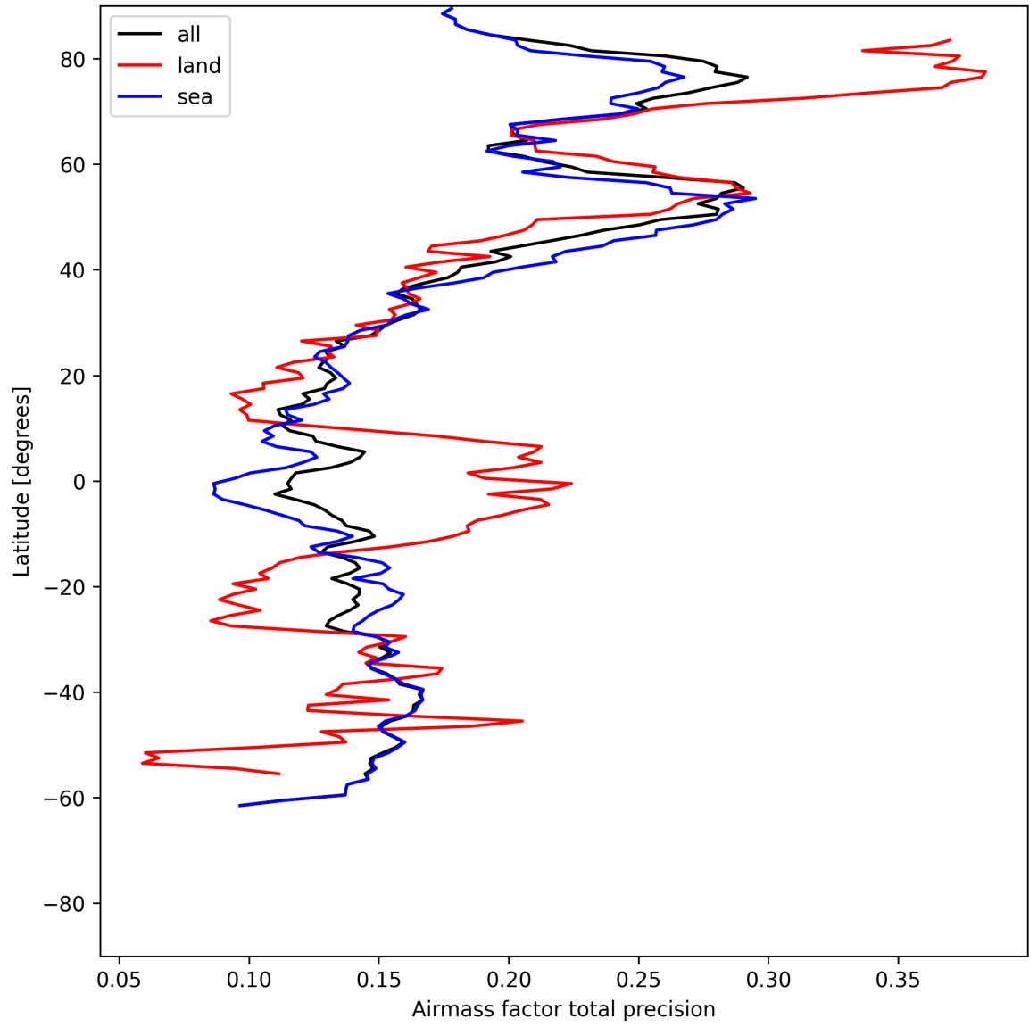
Figure 25: Zonal average of “Airmass factor total precision” for 2025-06-12 to 2025-06-13.
