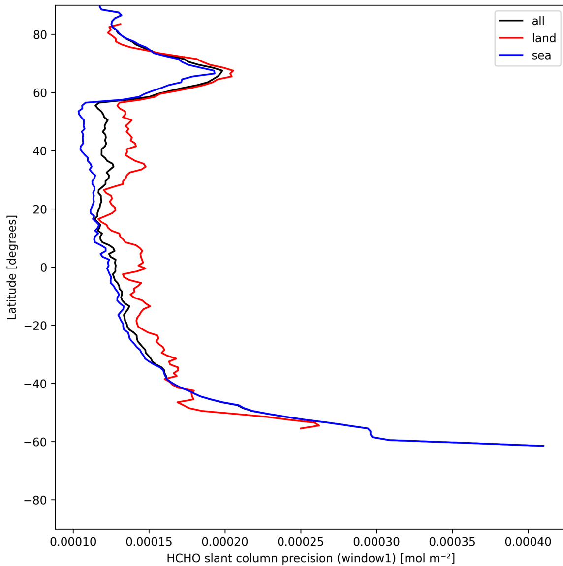
Figure 23: Zonal average of “HCHO slant column precision (window1)” for 2025-06-12 to 2025-06-13.
