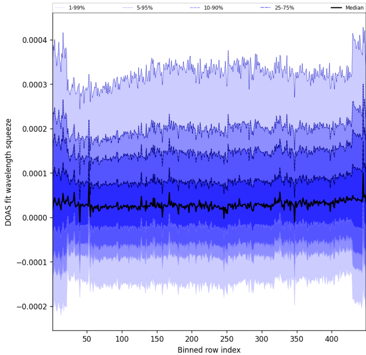
Figure 57: Along track statistics of “DOAS fit wavelength squeeze” for 2025-06-12 to 2025-06-13
