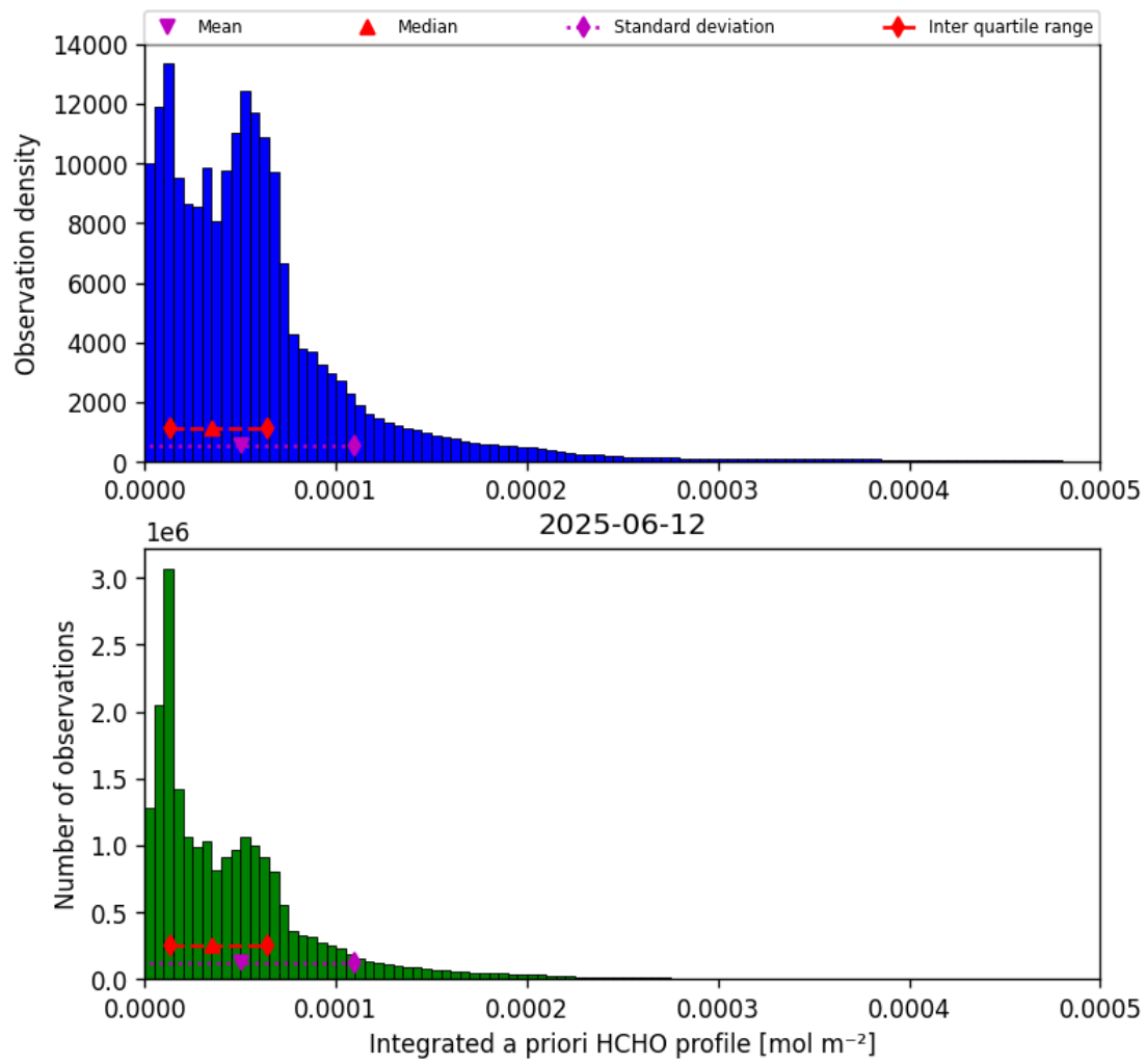
Figure 41: Histogram of “Integrated a priori HCHO profile” for 2025-06-12 to 2025-06-13
