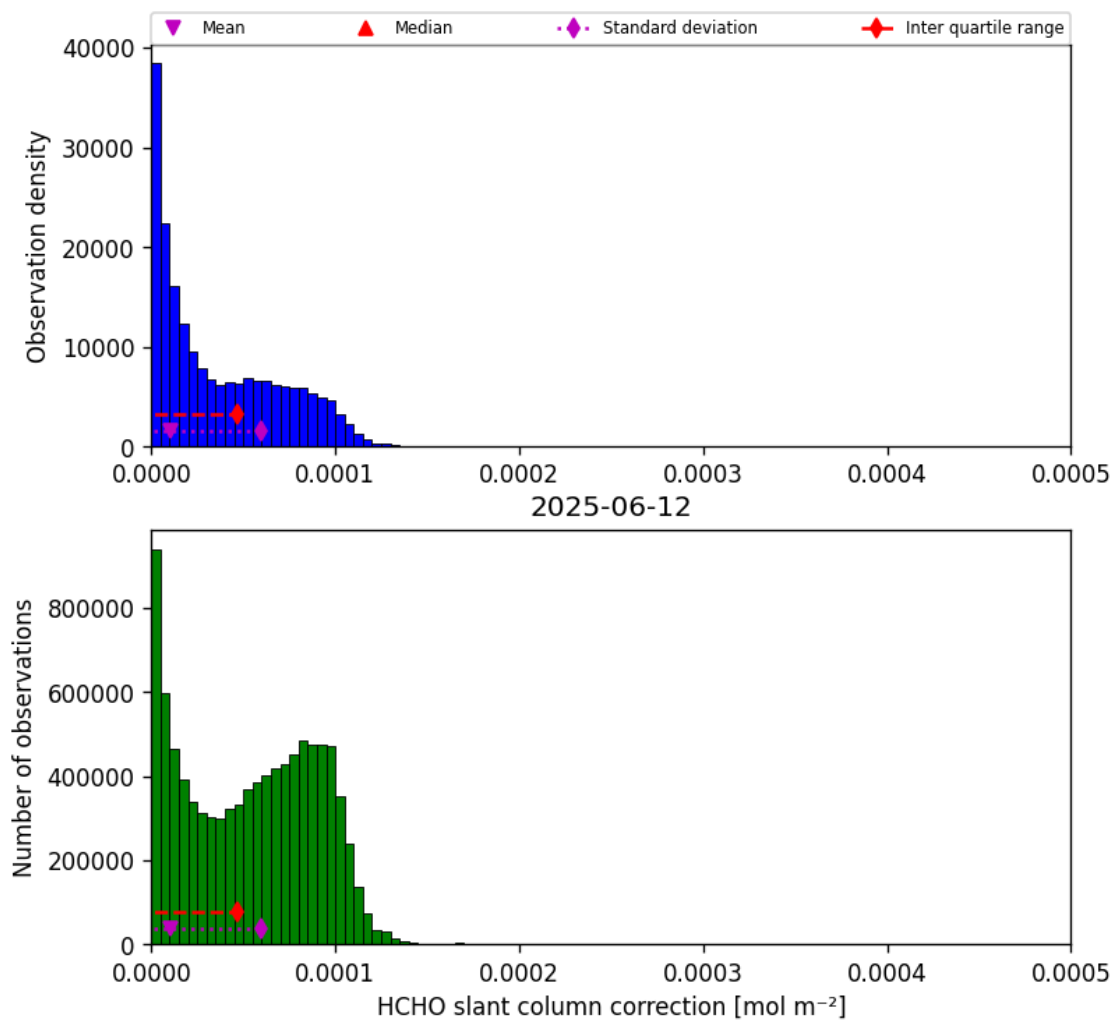
Figure 45: Histogram of “HCHO slant column correction” for 2025-06-12 to 2025-06-13
