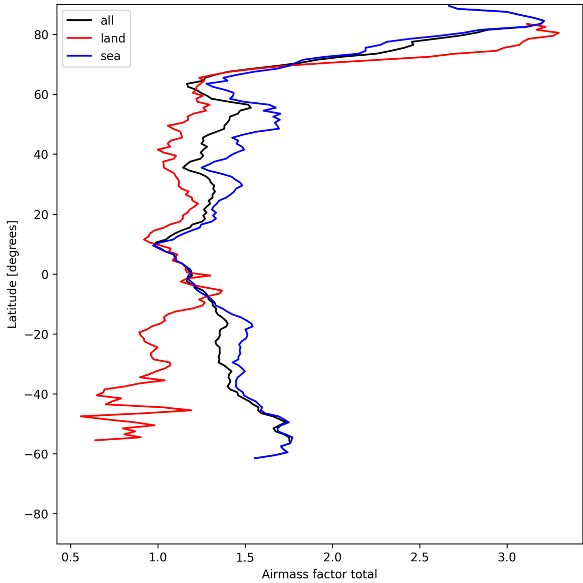
Figure 24: Zonal average of “Airmass factor total” for 2025-06-12 to 2025-06-13.
