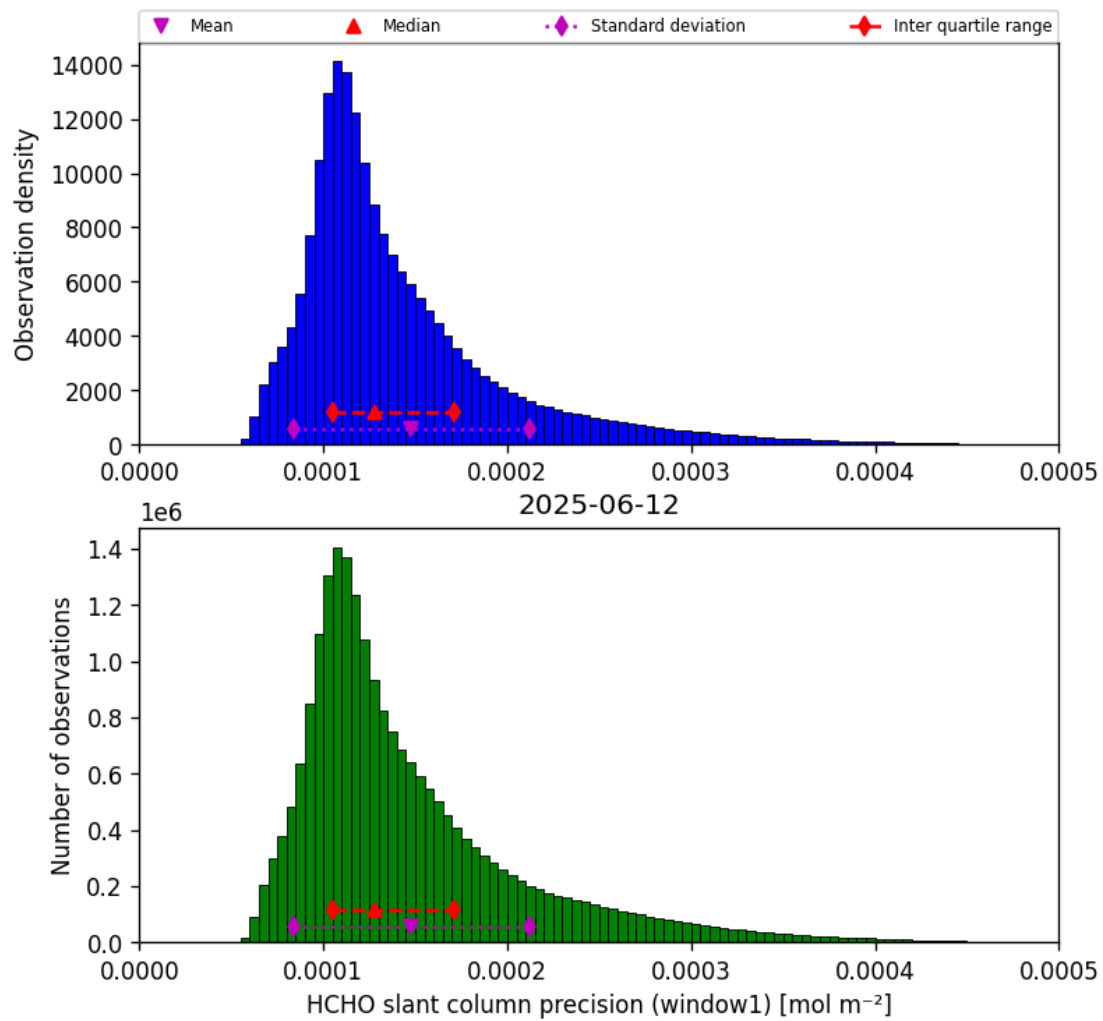
Figure 37: Histogram of “HCHO slant column precision (window1)” for 2025-06-12 to 2025-06-13
