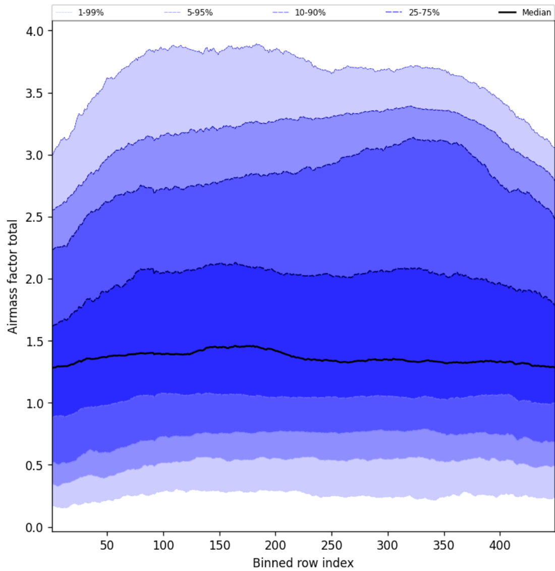
Figure 52: Along track statistics of “Airmass factor total” for 2025-06-12 to 2025-06-13
