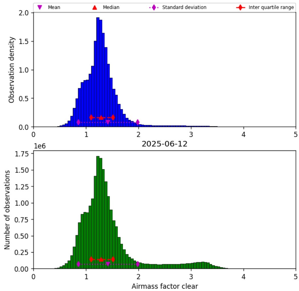
Figure 40: Histogram of “Airmass factor clear” for 2025-06-12 to 2025-06-13
