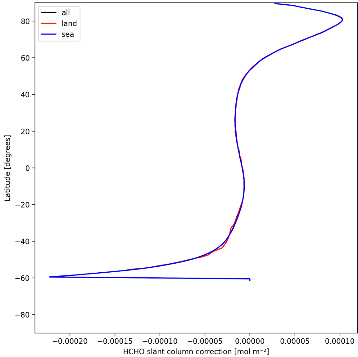
Figure 31: Zonal average of “HCHO slant column correction” for 2025-06-12 to 2025-06-13.
