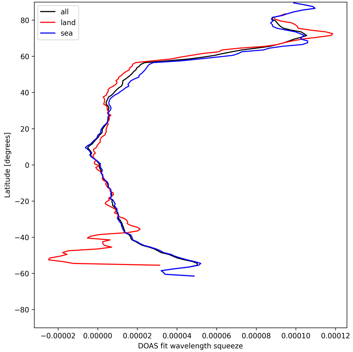
Figure 29: Zonal average of “DOAS fit wavelength squeeze” for 2025-06-12 to 2025-06-13.
