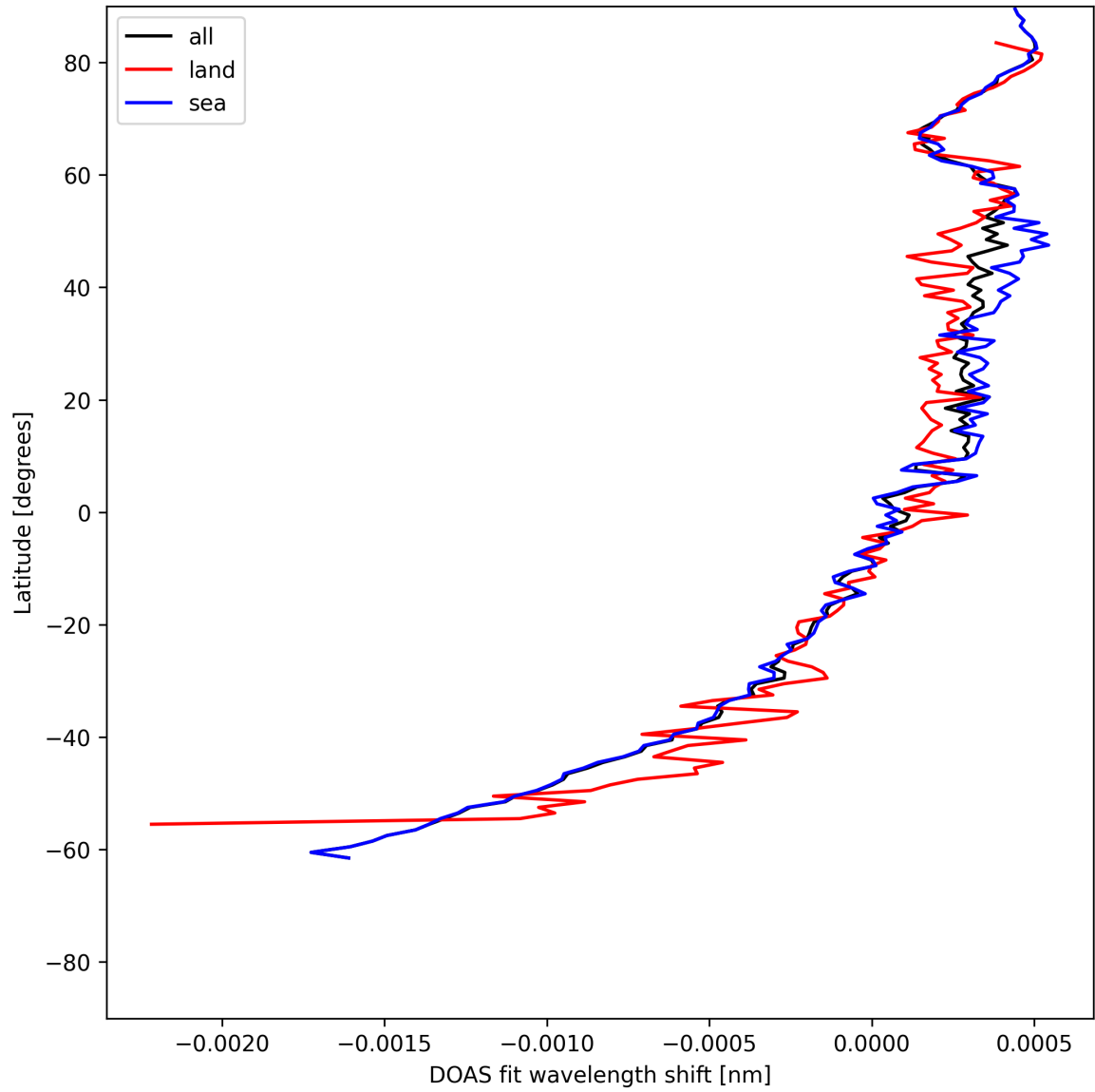
Figure 28: Zonal average of “DOAS fit wavelength shift” for 2025-06-12 to 2025-06-13.
