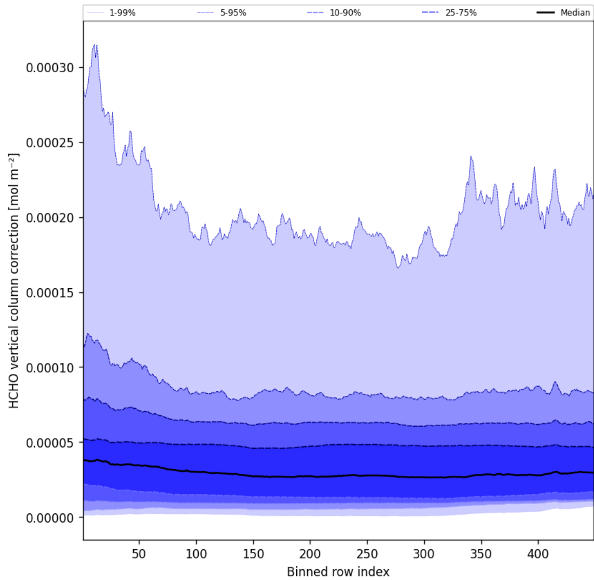
Figure 49: Along track statistics of “HCHO vertical column correction” for 2025-06-12 to 2025-06-13
