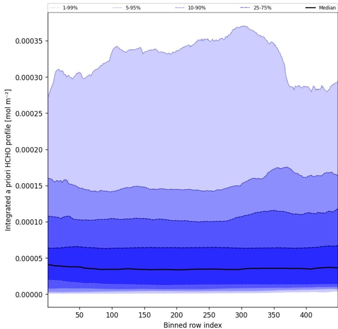
Figure 55: Along track statistics of "Integrated a priori HCHO profile" for 2025-06-12 to 2025-06-13
