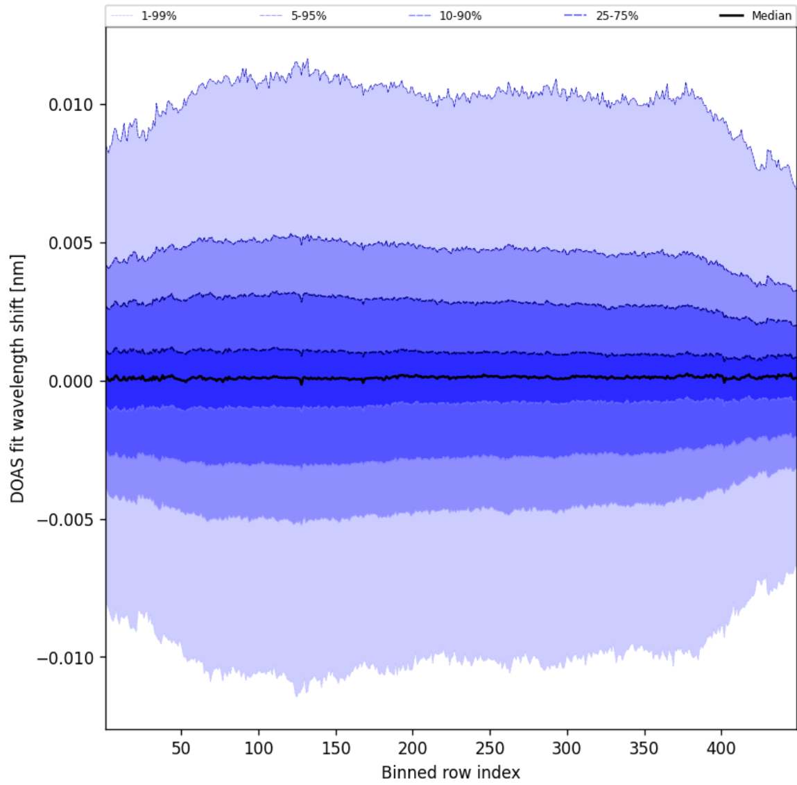
Figure 56: Along track statistics of “DOAS fit wavelength shift” for 2025-06-12 to 2025-06-13
