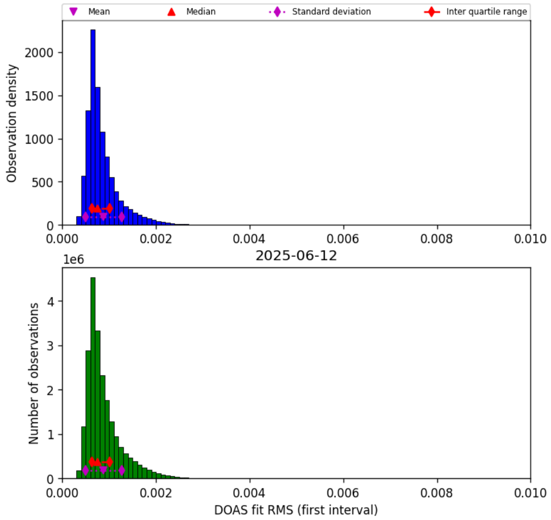
Figure 44: Histogram of “DOAS fit RMS (first interval)” for 2025-06-12 to 2025-06-13
