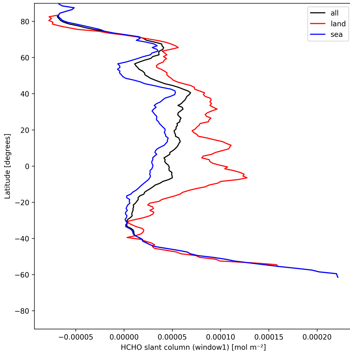
Figure 22: Zonal average of “HCHO slant column (window1)” for 2025-06-12 to 2025-06-13.
