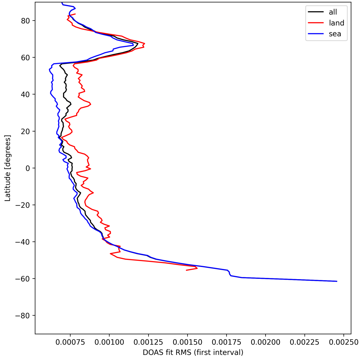
Figure 30: Zonal average of “DOAS fit RMS (first interval)” for 2025-06-12 to 2025-06-13.
