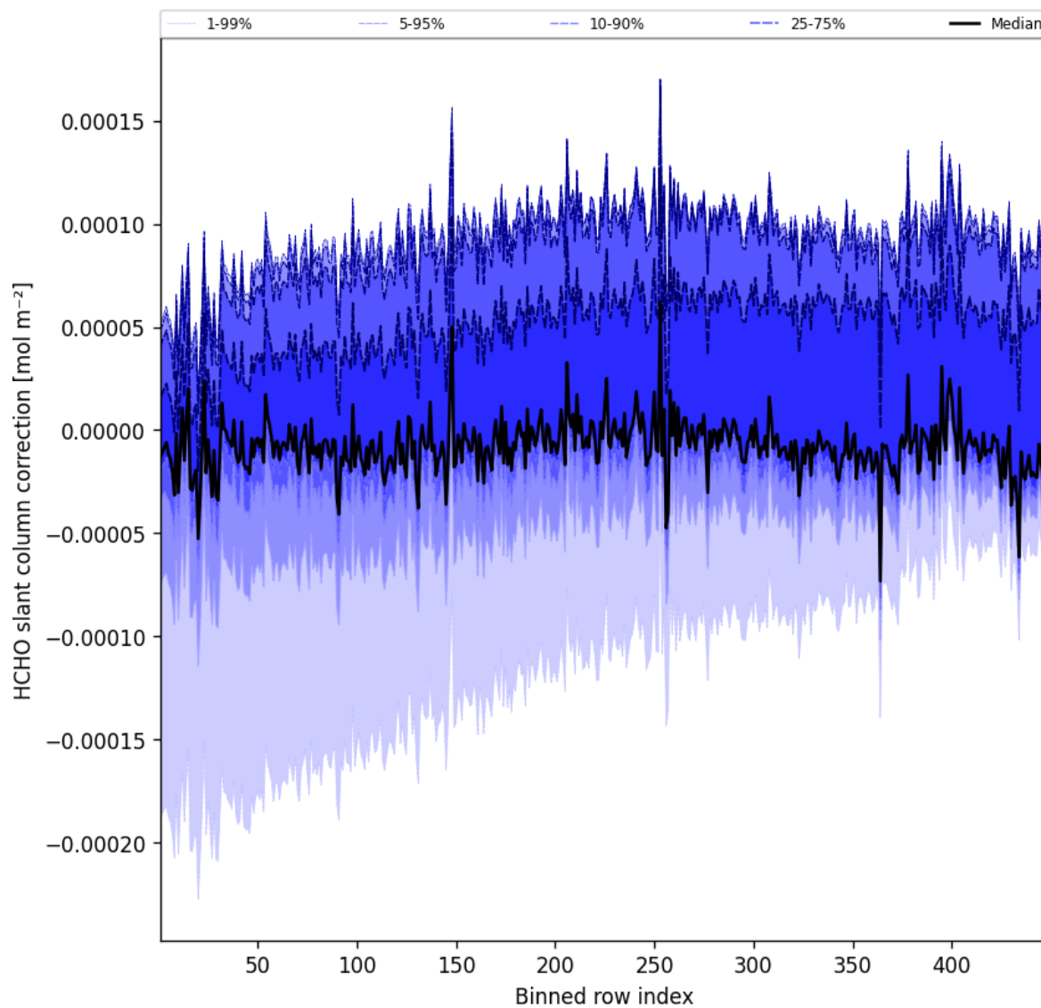
Figure 59: Along track statistics of “HCHO slant column correction” for 2025-06-12 to 2025-06-13
