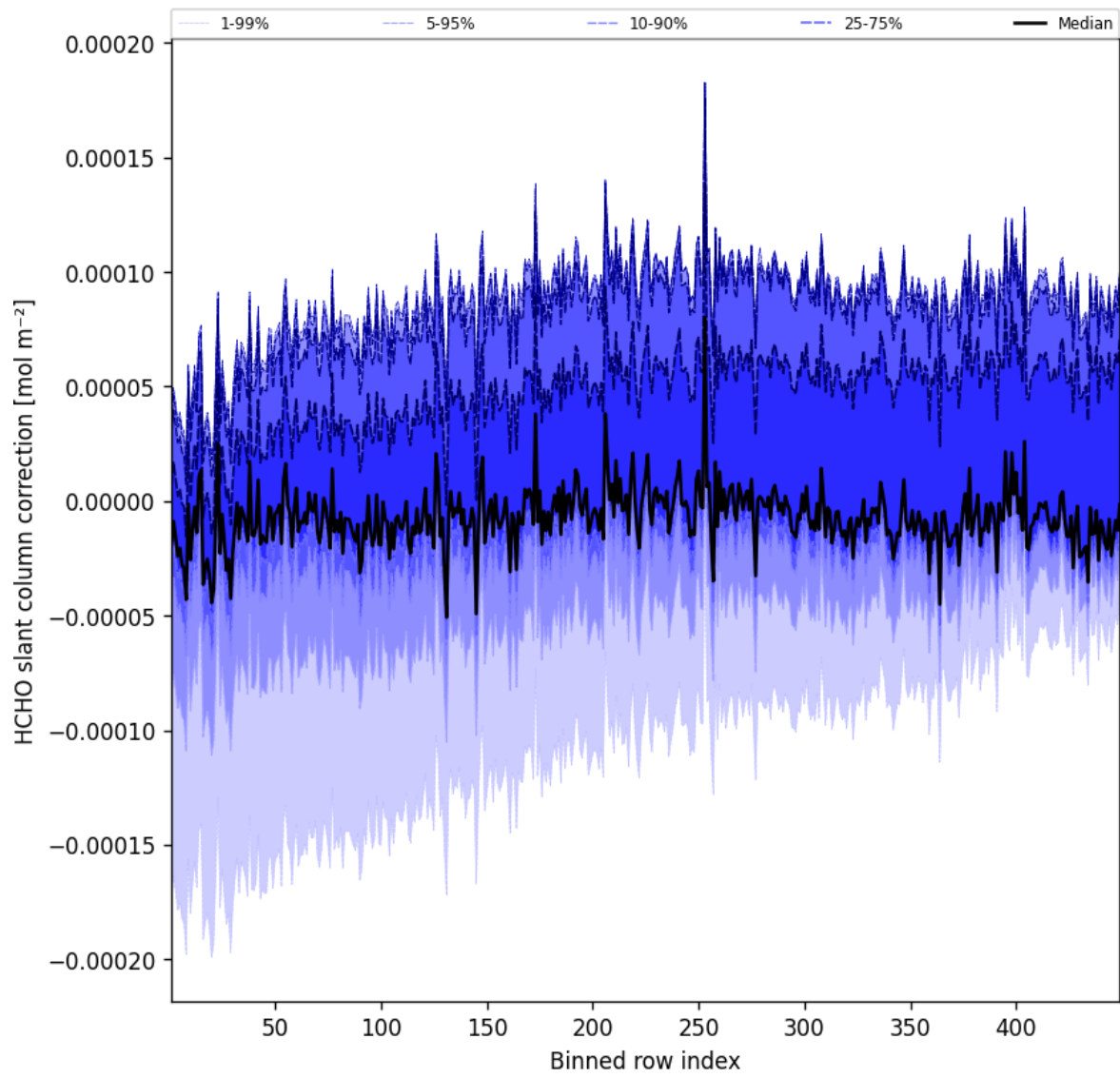
Figure 59: Along track statistics of “HCHO slant column correction” for 2025-06-13 to 2025-06-14
