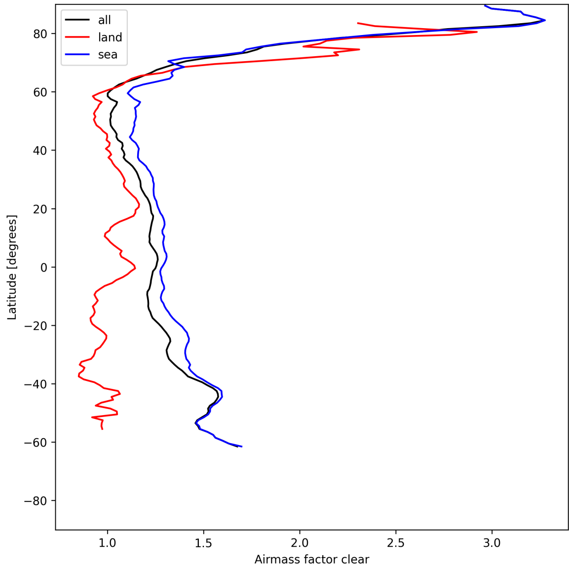
Figure 26: Zonal average of “Airmass factor clear” for 2025-06-13 to 2025-06-14.
