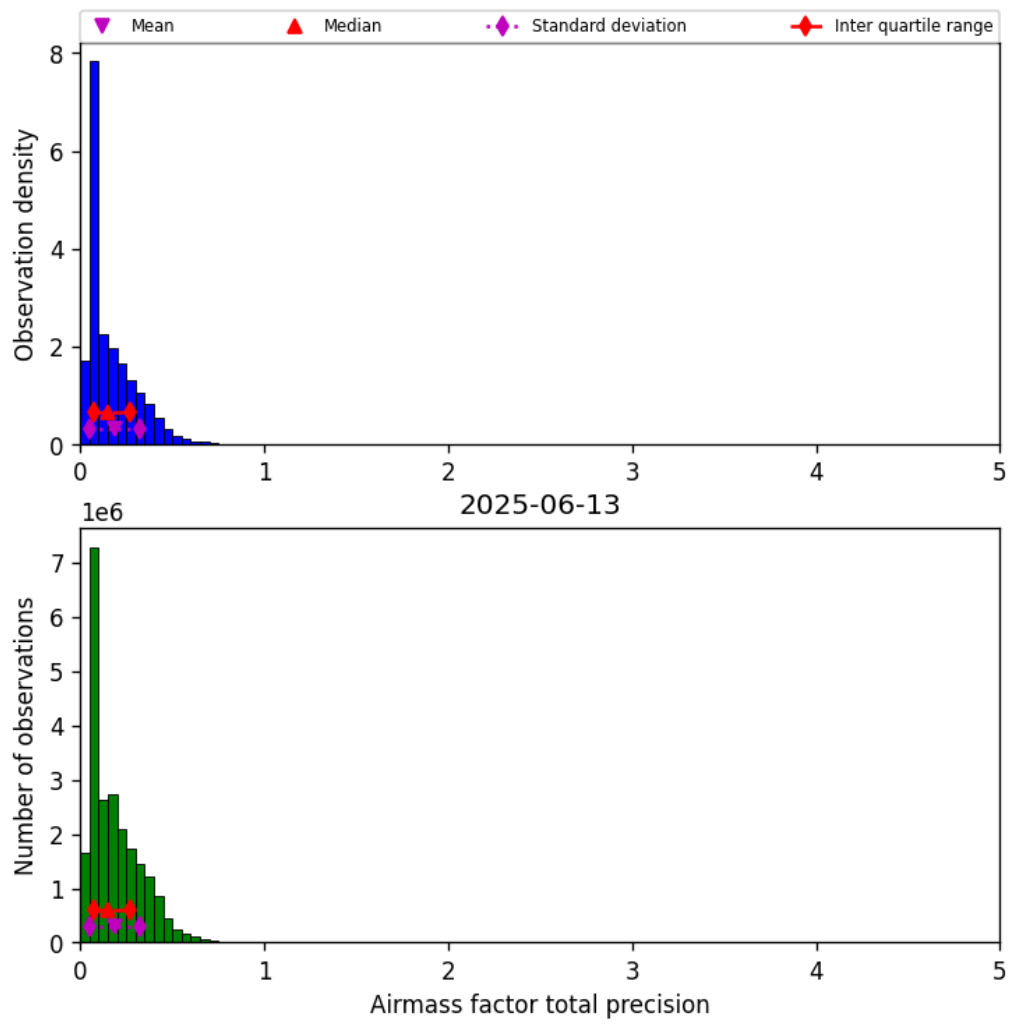
Figure 39: Histogram of “Airmass factor total precision” for 2025-06-13 to 2025-06-14
