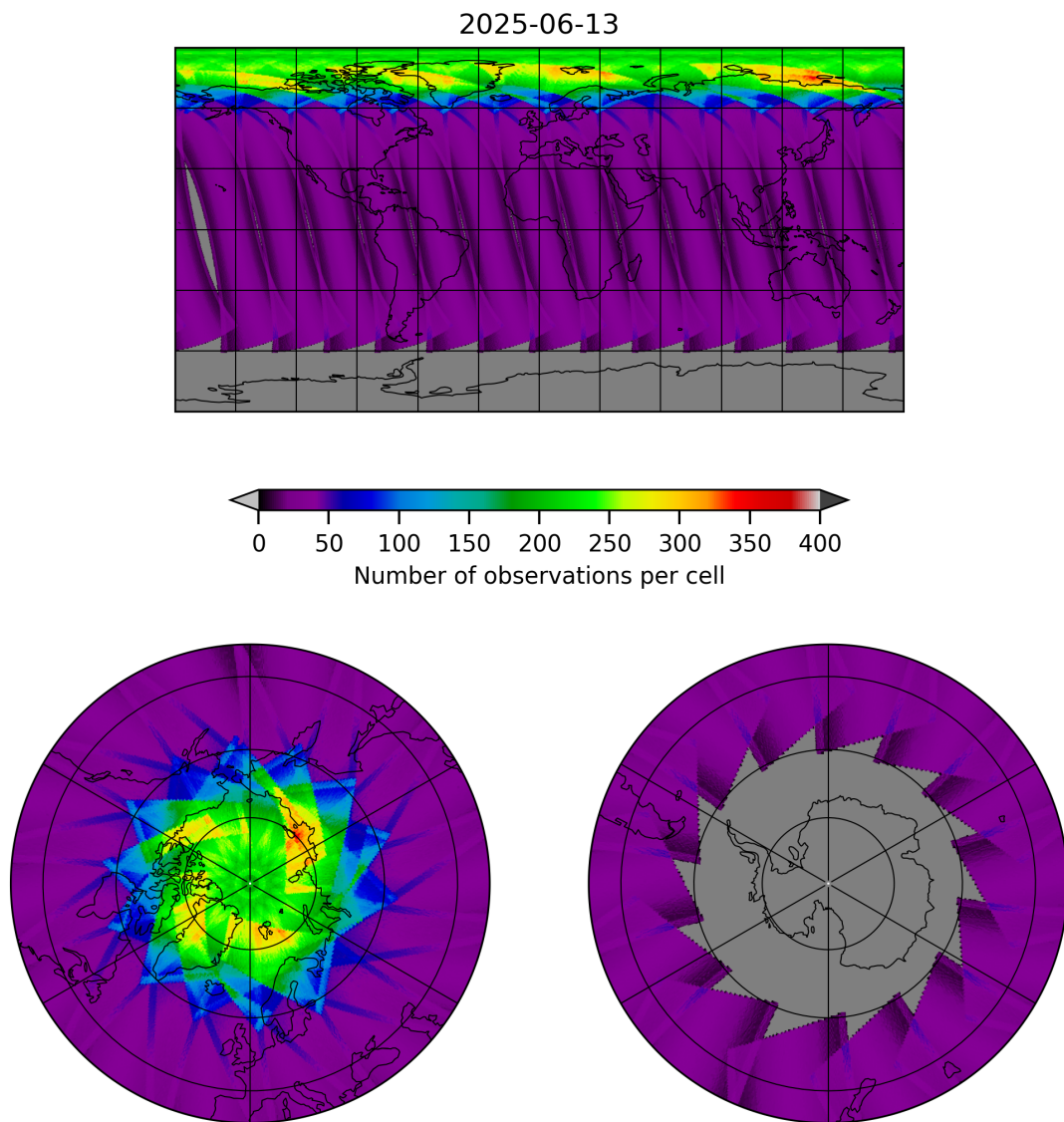
Figure 17: Map of the number of observations for 2025-06-13 to 2025-06-14
