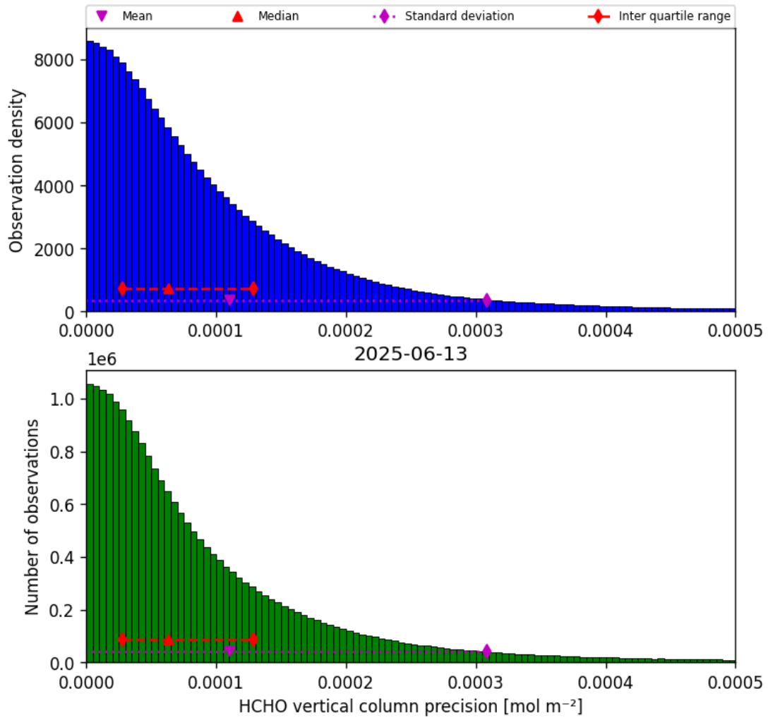
Figure 34: Histogram of “HCHO vertical column precision” for 2025-06-13 to 2025-06-14
