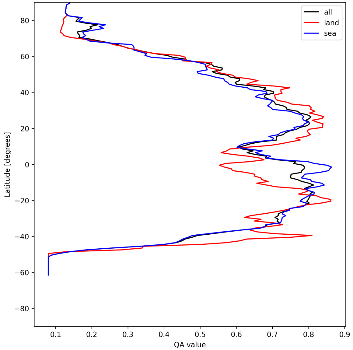
Figure 18: Zonal average of “QA value” for 2025-06-13 to 2025-06-14.
