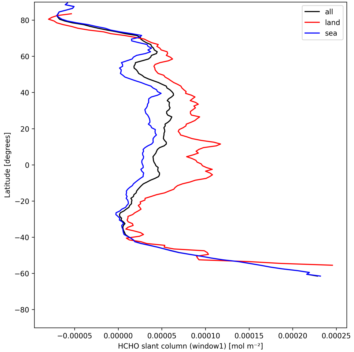
Figure 22: Zonal average of “HCHO slant column (window1)” for 2025-06-13 to 2025-06-14.
