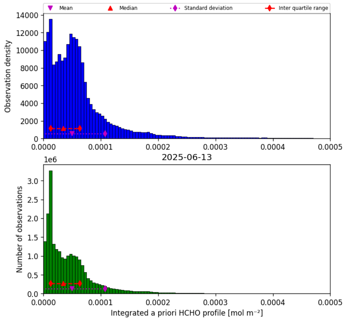
Figure 41: Histogram of “Integrated a priori HCHO profile” for 2025-06-13 to 2025-06-14
