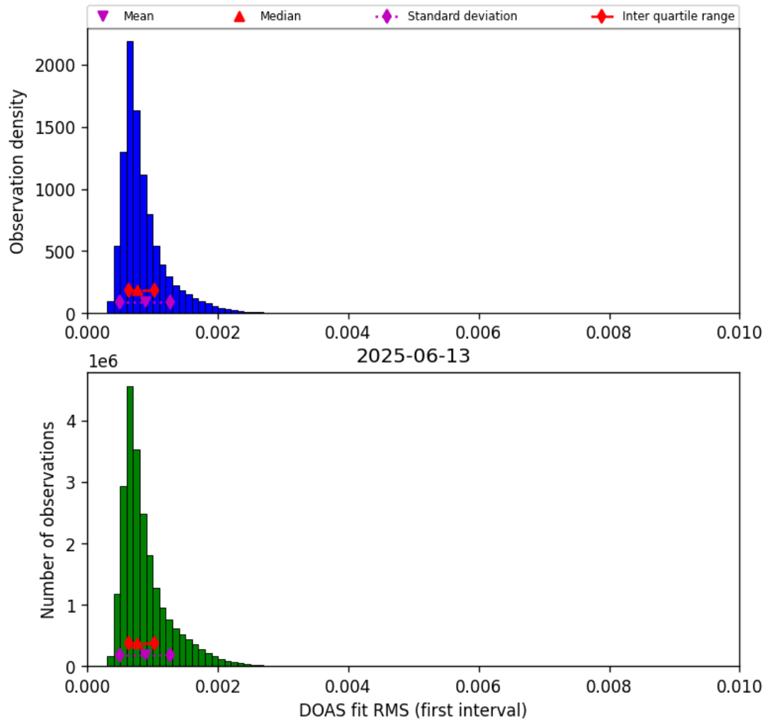
Figure 44: Histogram of “DOAS fit RMS (first interval)” for 2025-06-13 to 2025-06-14
