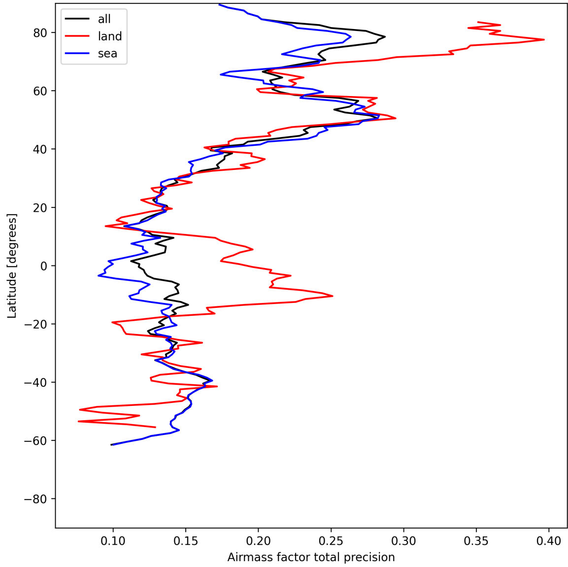
Figure 25: Zonal average of “Airmass factor total precision” for 2025-06-13 to 2025-06-14.
