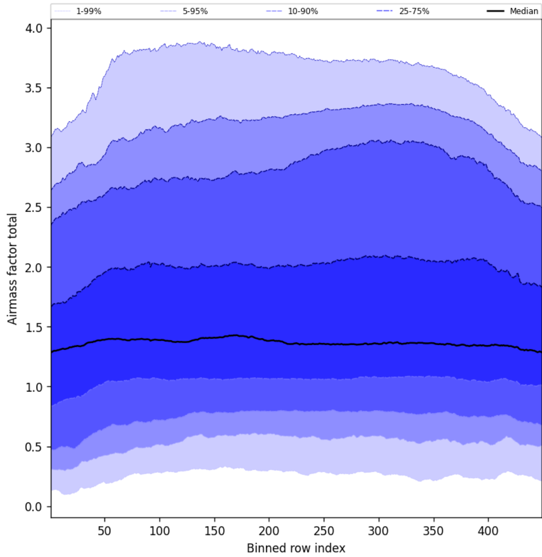
Figure 52: Along track statistics of “Airmass factor total” for 2025-06-13 to 2025-06-14
