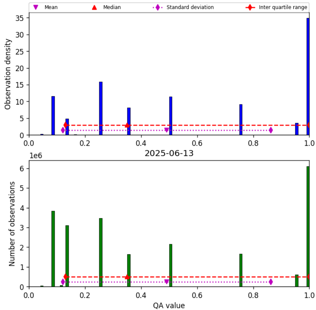
Figure 32: Histogram of “QA value” for 2025-06-13 to 2025-06-14
