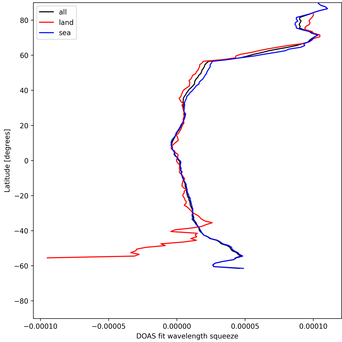
Figure 29: Zonal average of “DOAS fit wavelength squeeze” for 2025-06-13 to 2025-06-14.
