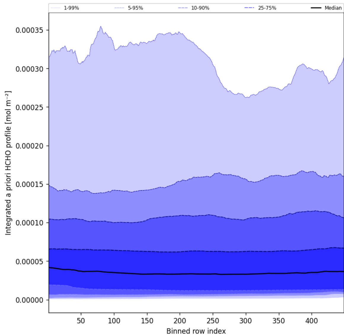
Figure 55: Along track statistics of “Integrated a priori HCHO profile” for 2025-06-13 to 2025-06-14
