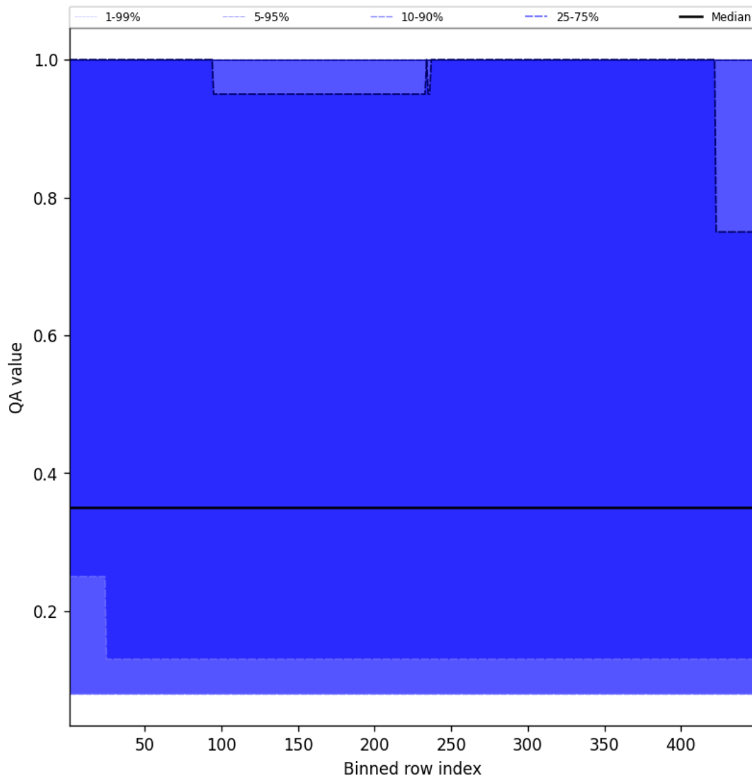
Figure 46: Along track statistics of “QA value” for 2025-06-13 to 2025-06-14
