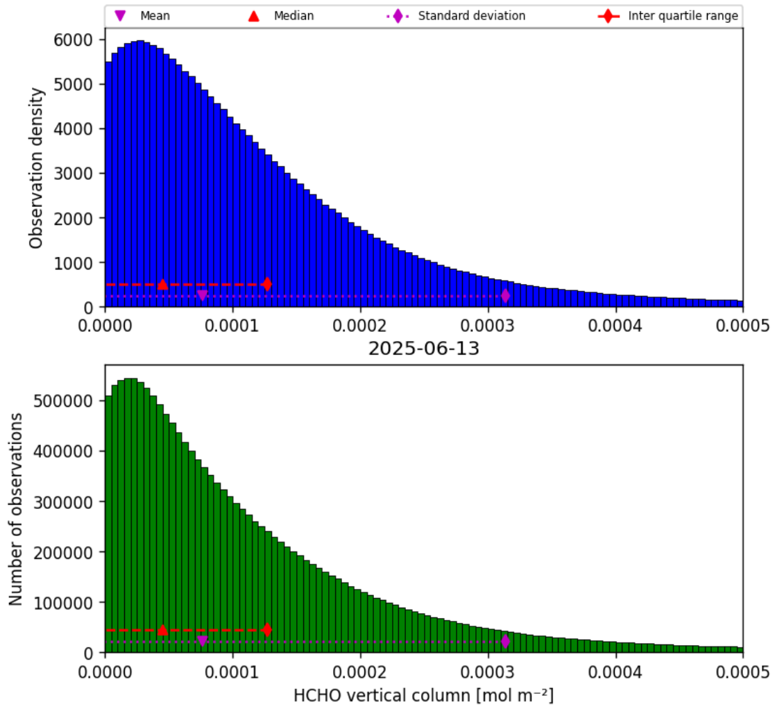
Figure 33: Histogram of “HCHO vertical column” for 2025-06-13 to 2025-06-14
