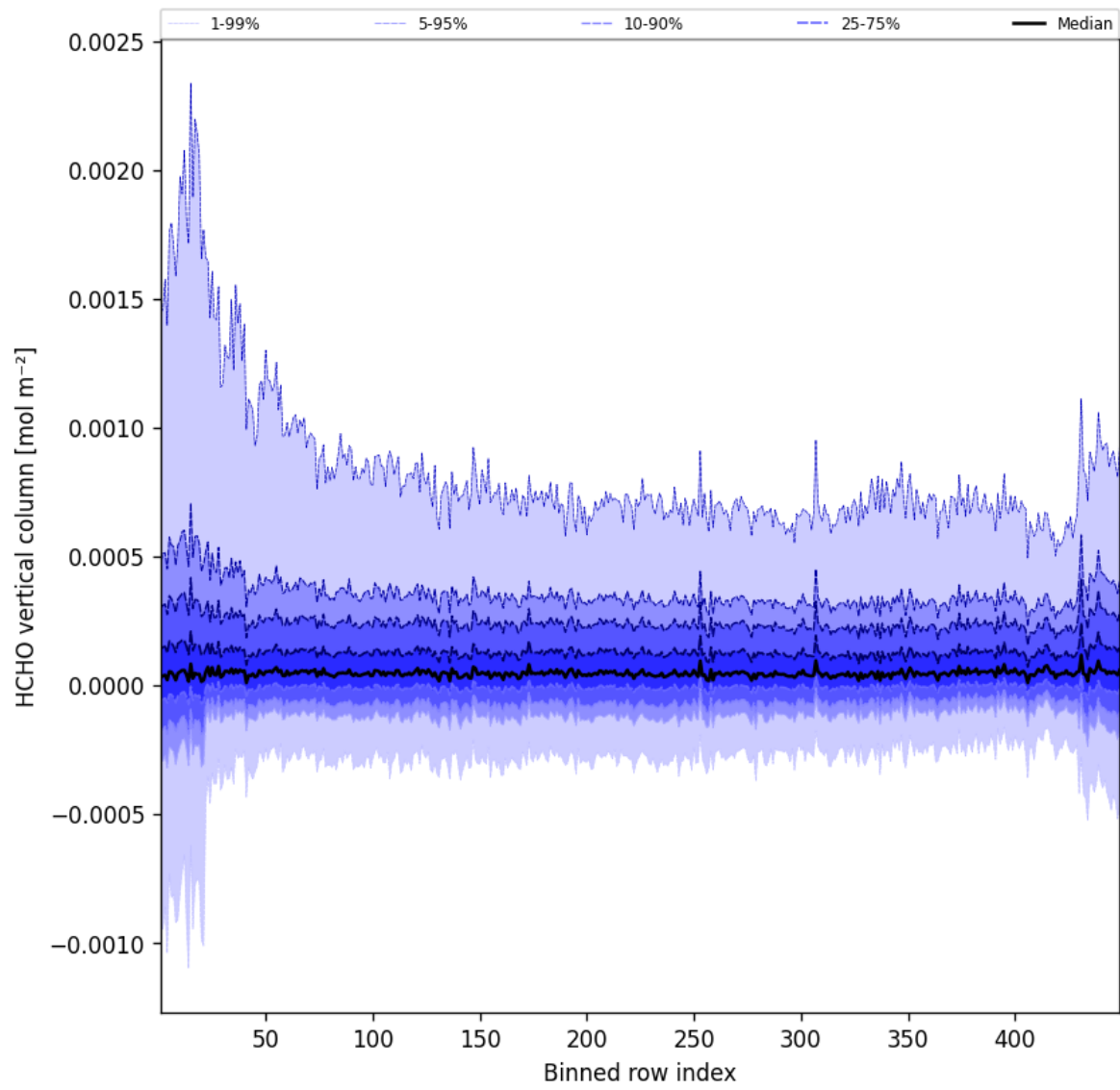
Figure 47: Along track statistics of “HCHO vertical column” for 2025-06-13 to 2025-06-14
