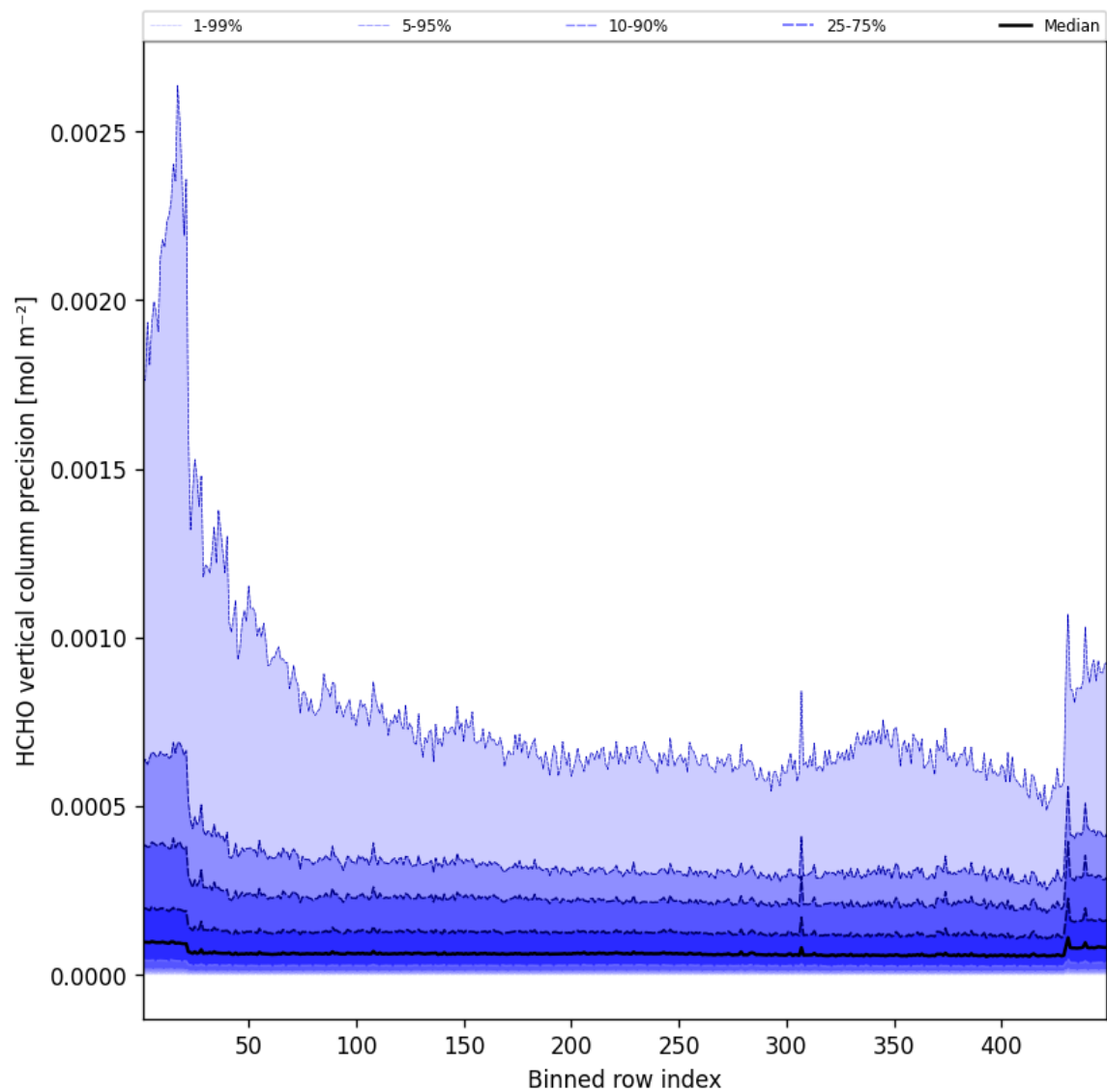
Figure 48: Along track statistics of “HCHO vertical column precision” for 2025-06-13 to 2025-06-14
