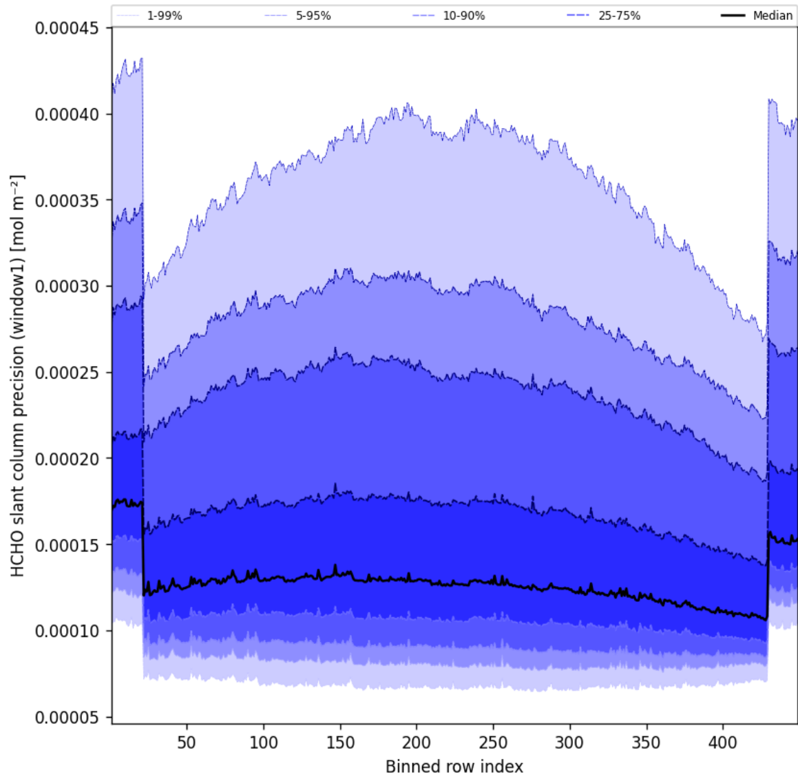
Figure 51: Along track statistics of “HCHO slant column precision (window1)” for 2025-06-13 to 2025-06-14
