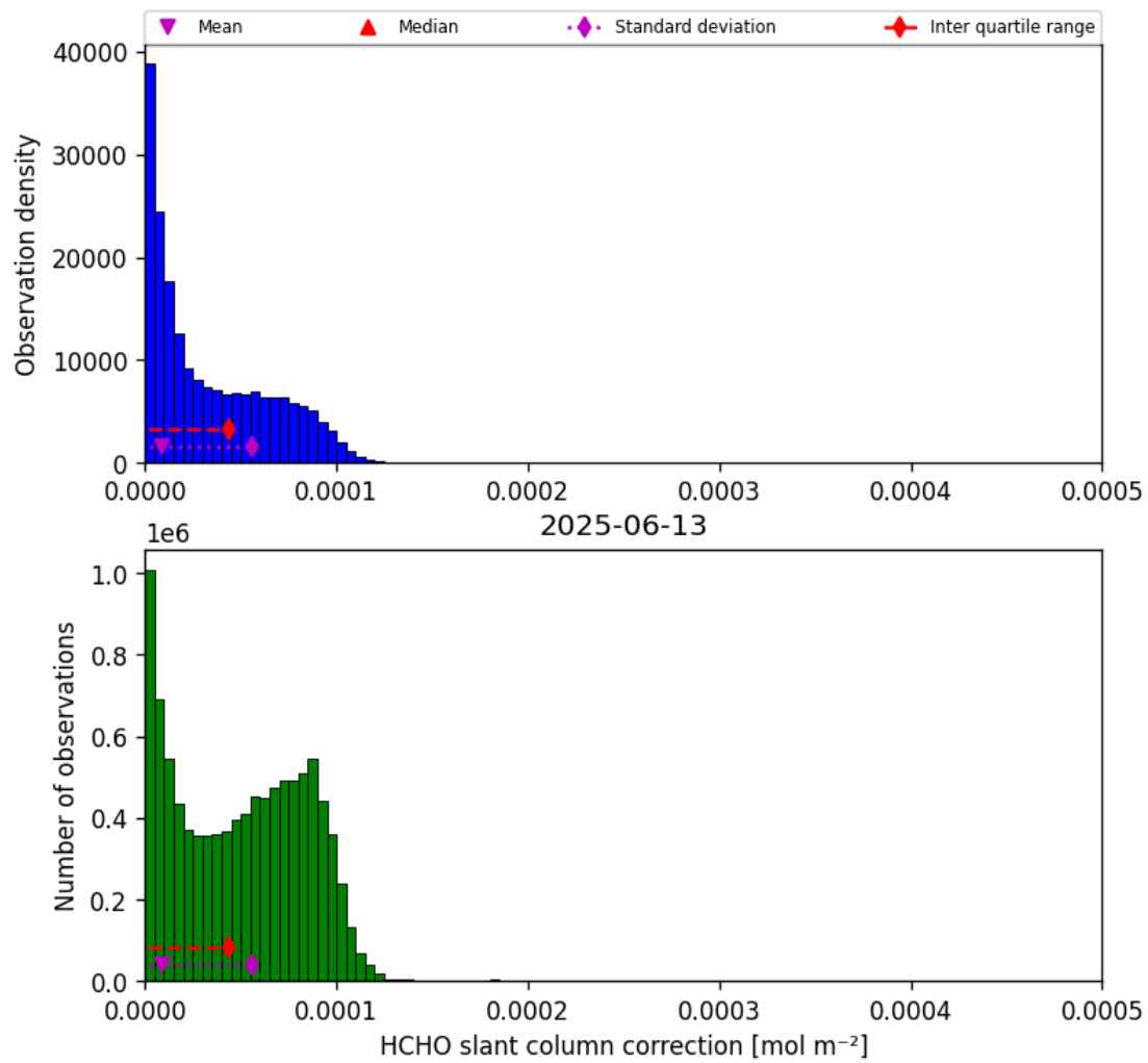
Figure 45: Histogram of “HCHO slant column correction” for 2025-06-13 to 2025-06-14
