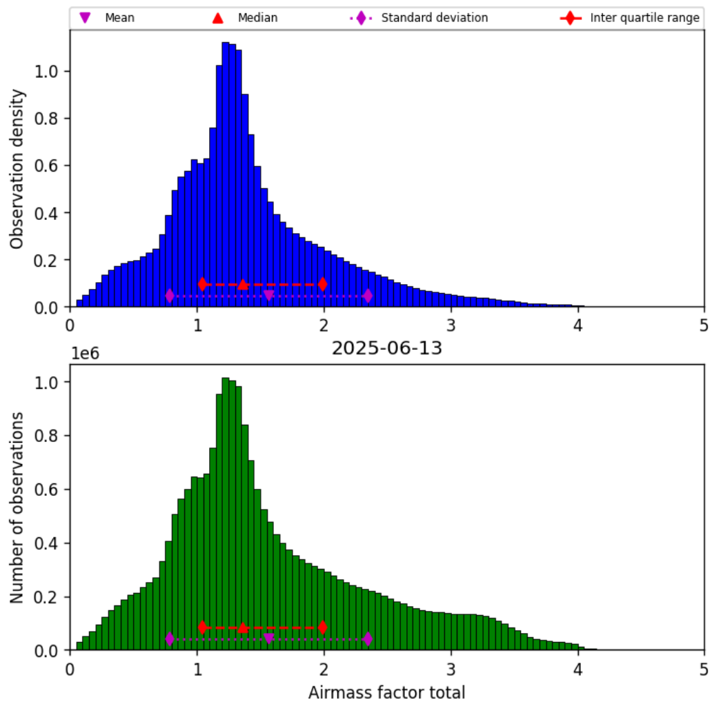
Figure 38: Histogram of “Airmass factor total” for 2025-06-13 to 2025-06-14
