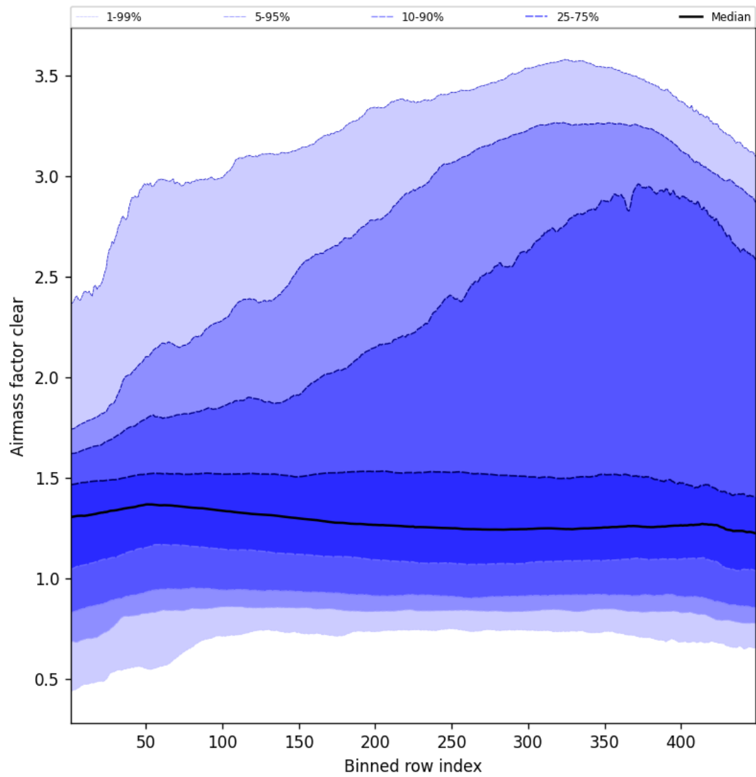
Figure 54: Along track statistics of “Airmass factor clear” for 2025-06-13 to 2025-06-14
