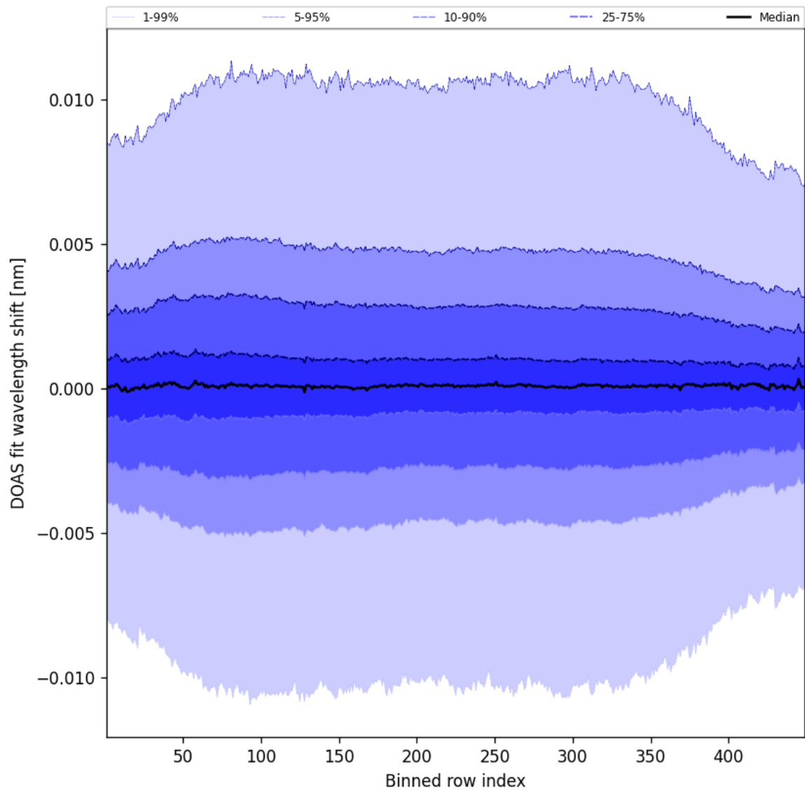
Figure 56: Along track statistics of “DOAS fit wavelength shift” for 2025-06-13 to 2025-06-14
