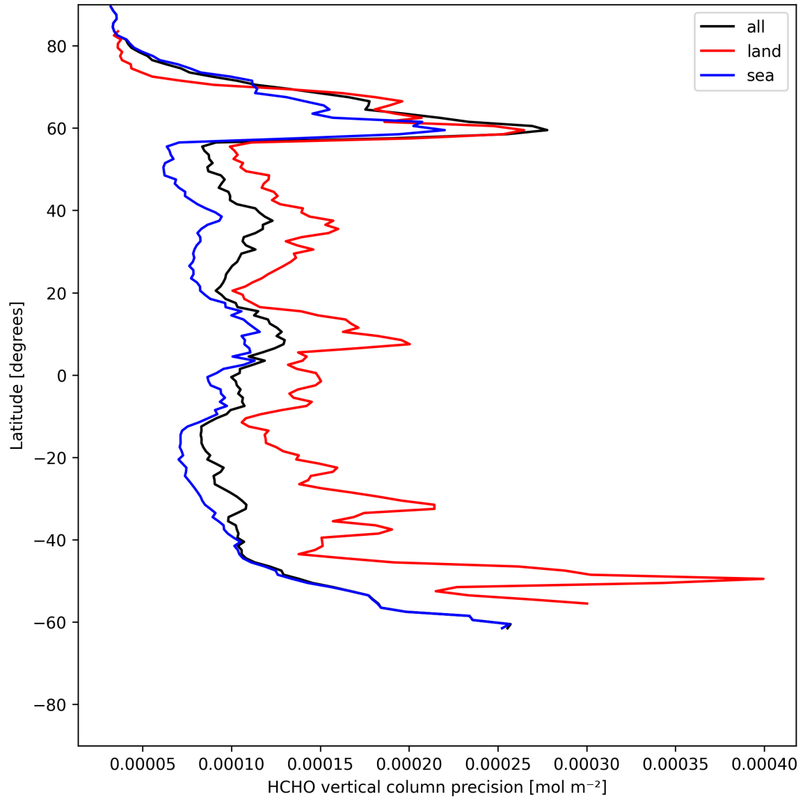
Figure 20: Zonal average of “HCHO vertical column precision” for 2025-06-13 to 2025-06-14.
