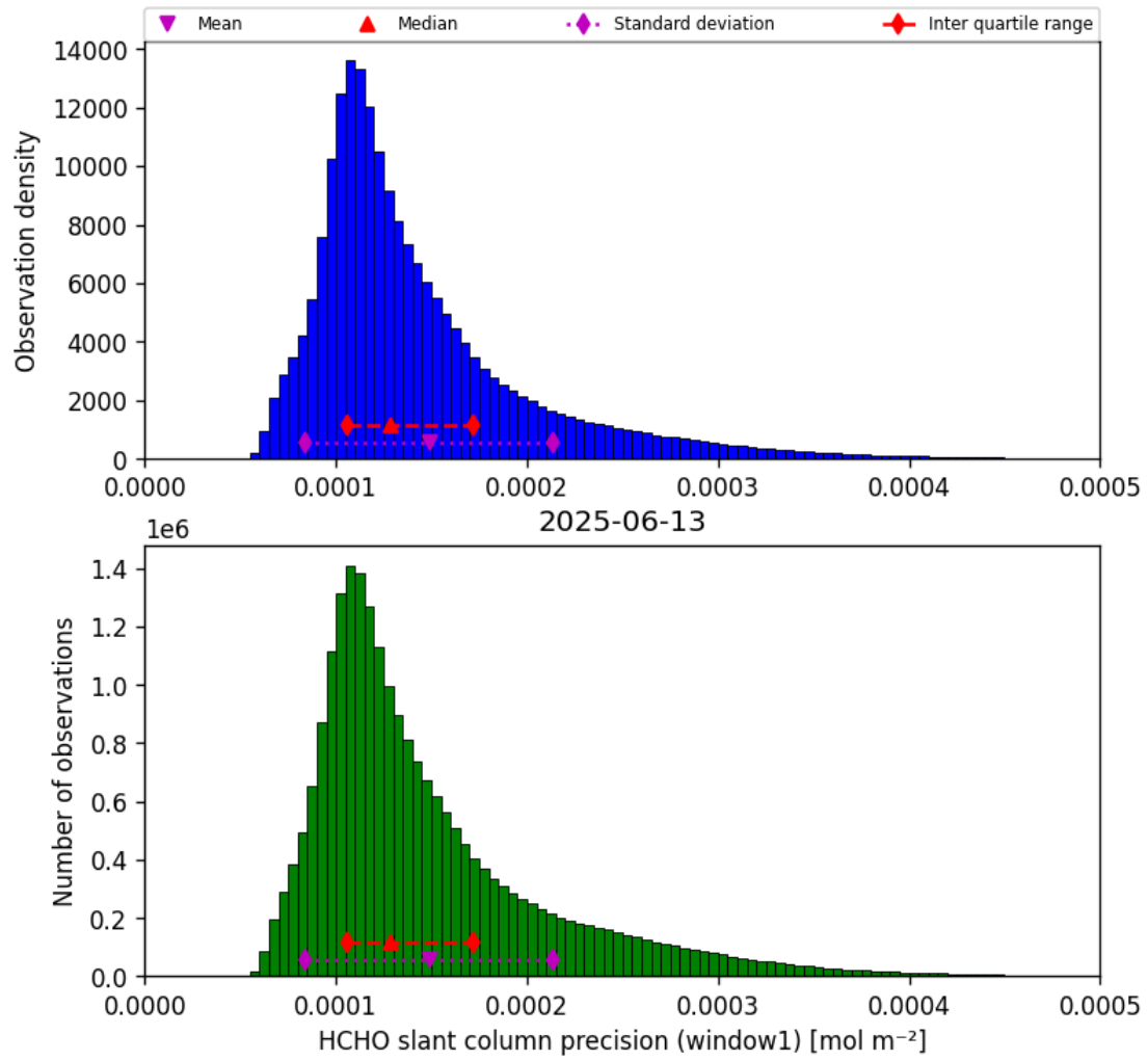
Figure 37: Histogram of “HCHO slant column precision (window1)” for 2025-06-13 to 2025-06-14
