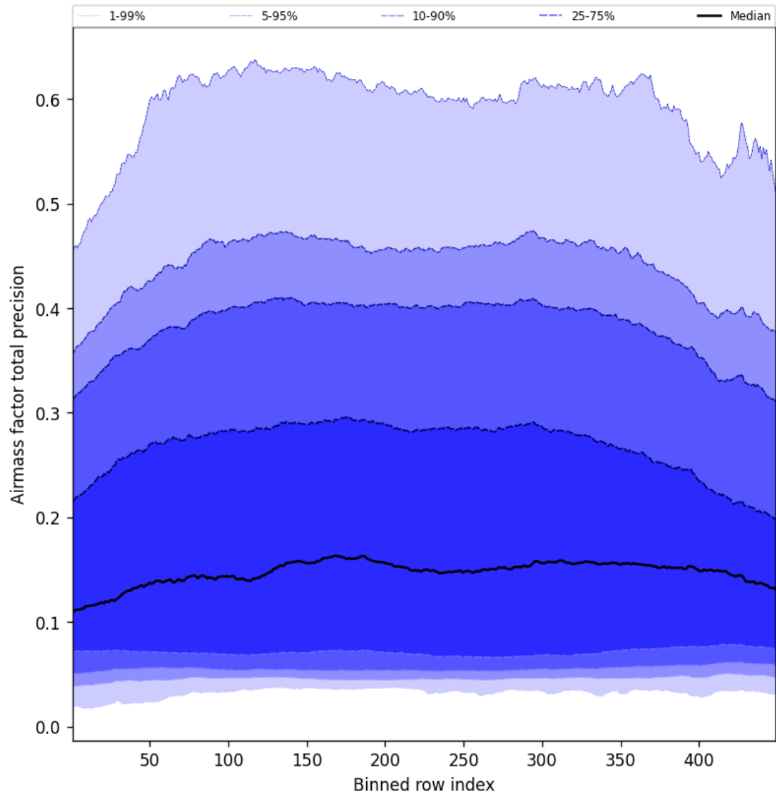
Figure 53: Along track statistics of “Airmass factor total precision” for 2025-06-13 to 2025-06-14
