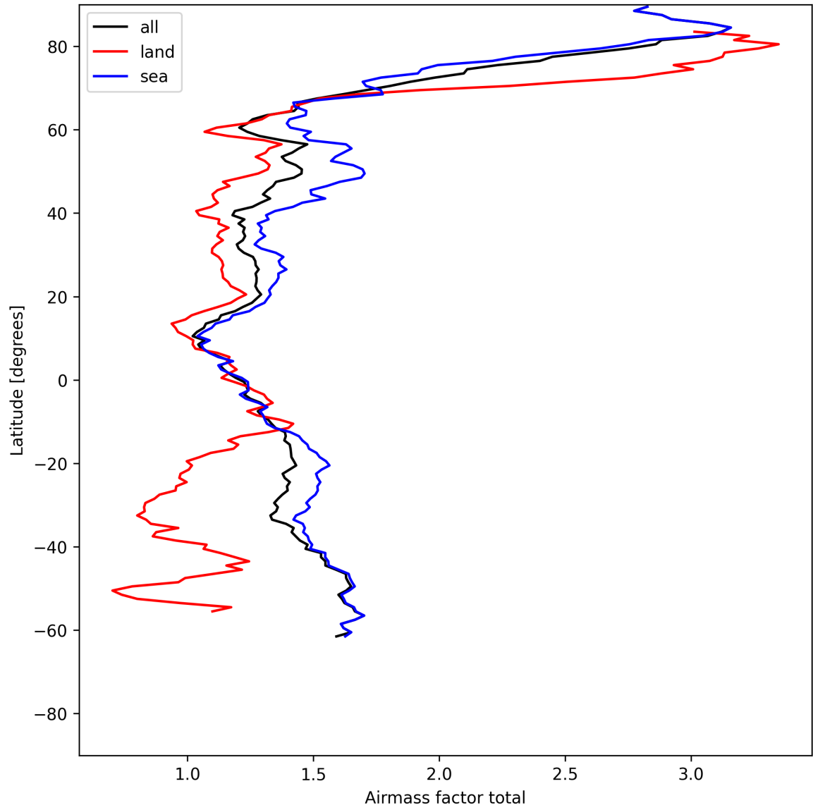
Figure 24: Zonal average of “Airmass factor total” for 2025-06-13 to 2025-06-14.
