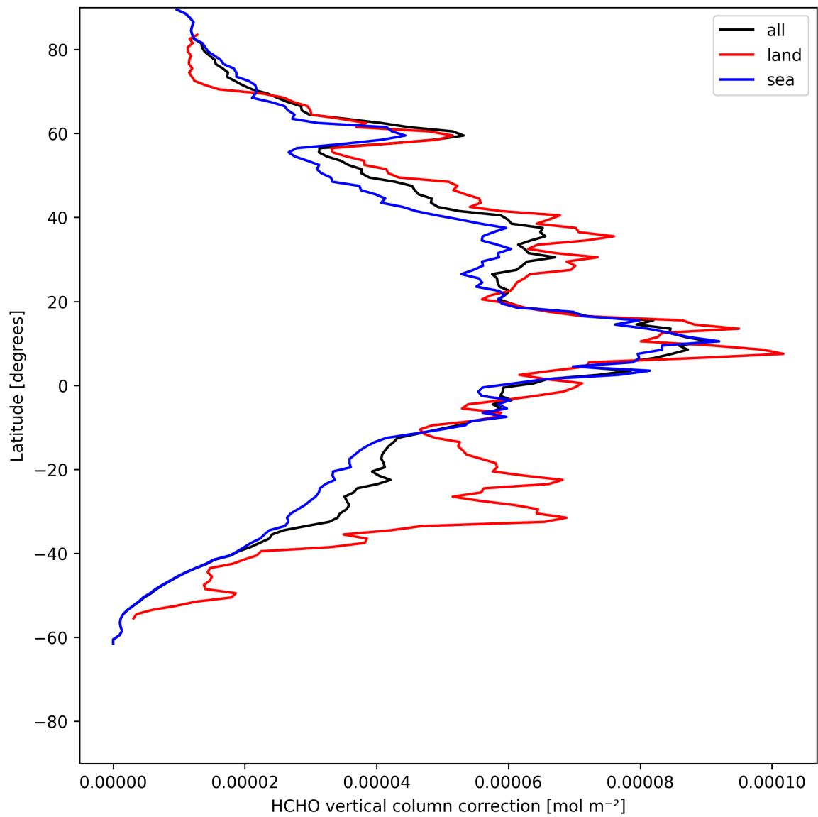
Figure 21: Zonal average of “HCHO vertical column correction” for 2025-06-13 to 2025-06-14.
