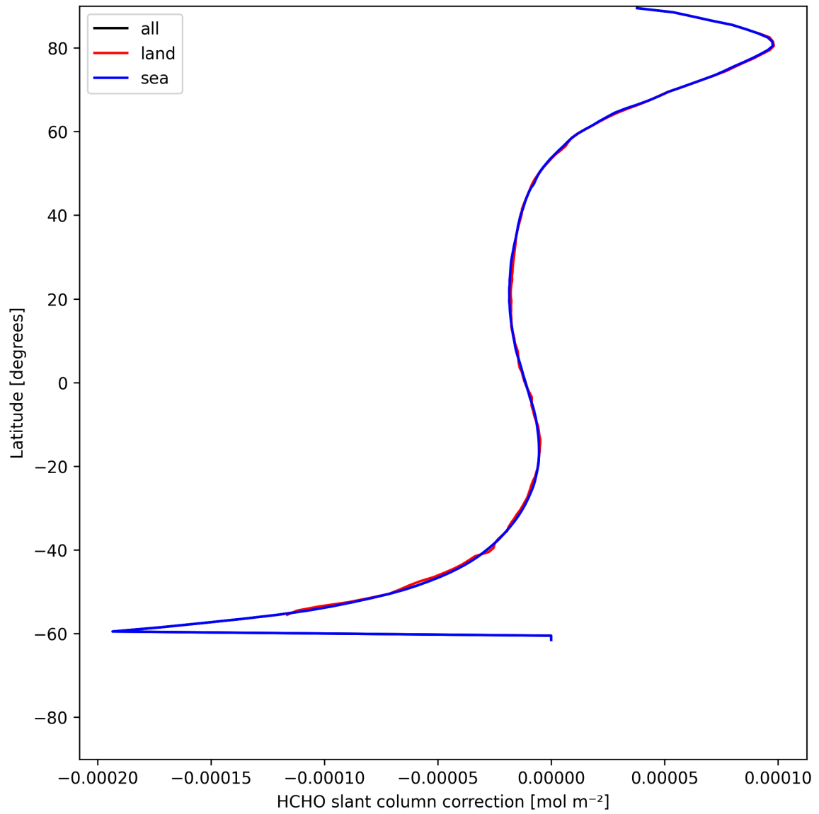
Figure 31: Zonal average of “HCHO slant column correction” for 2025-06-13 to 2025-06-14.
