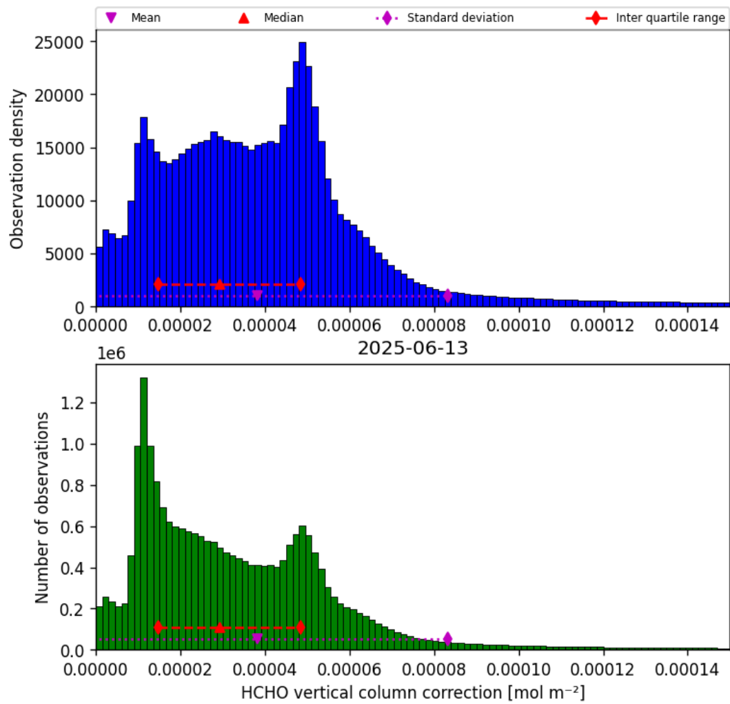
Figure 35: Histogram of “HCHO vertical column correction” for 2025-06-13 to 2025-06-14
