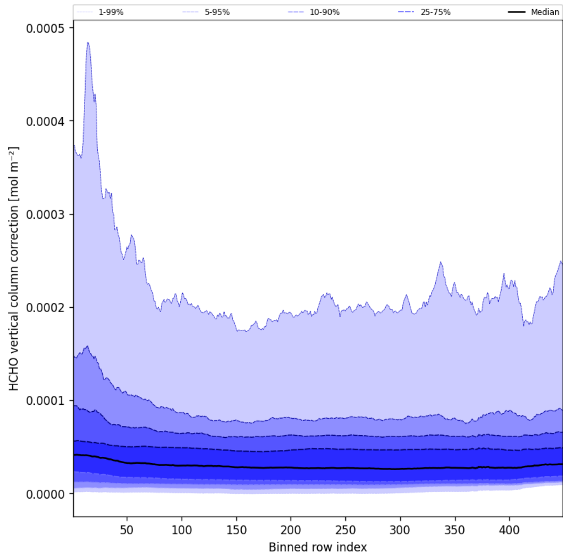
Figure 49: Along track statistics of “HCHO vertical column correction” for 2025-06-13 to 2025-06-14
