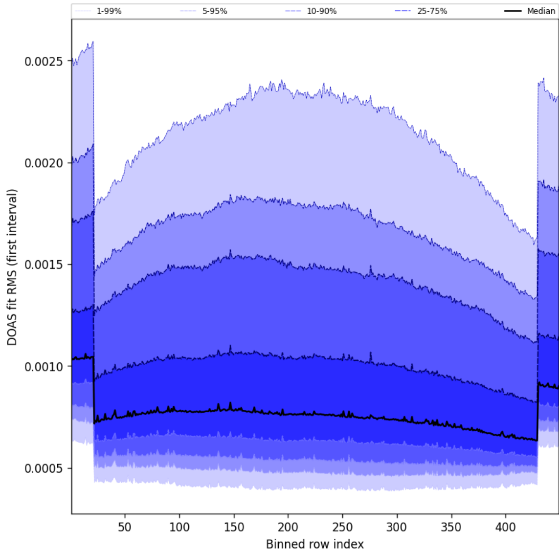
Figure 58: Along track statistics of “DOAS fit RMS (first interval)” for 2025-06-13 to 2025-06-14
