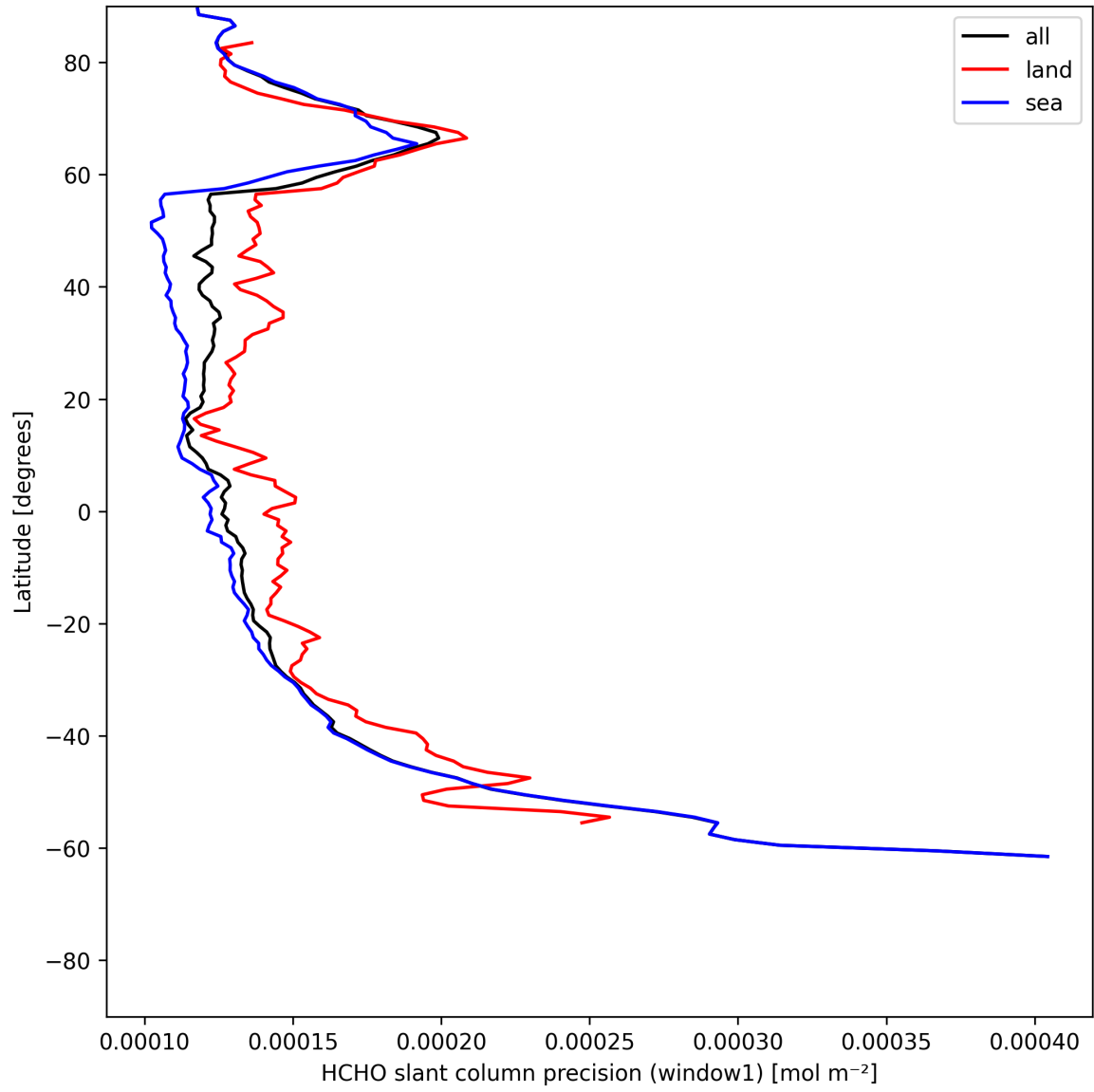
Figure 23: Zonal average of "HCHO slant column precision (window1)" for 2025-06-13 to 2025-06-14.
