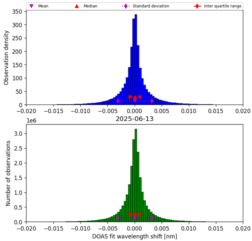
Figure 42: Histogram of “DOAS fit wavelength shift” for 2025-06-13 to 2025-06-14
