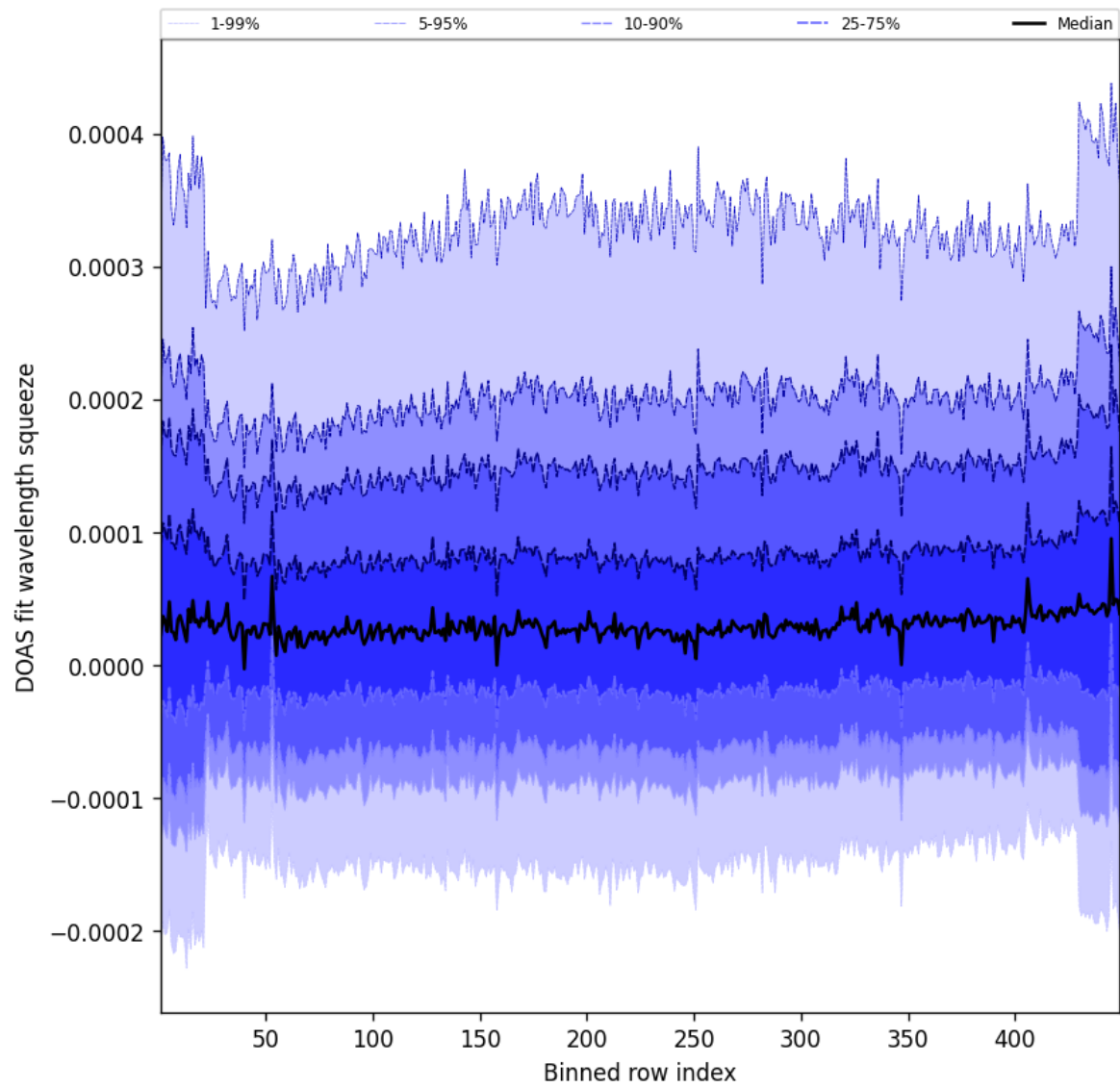
Figure 57: Along track statistics of “DOAS fit wavelength squeeze” for 2025-06-13 to 2025-06-14
