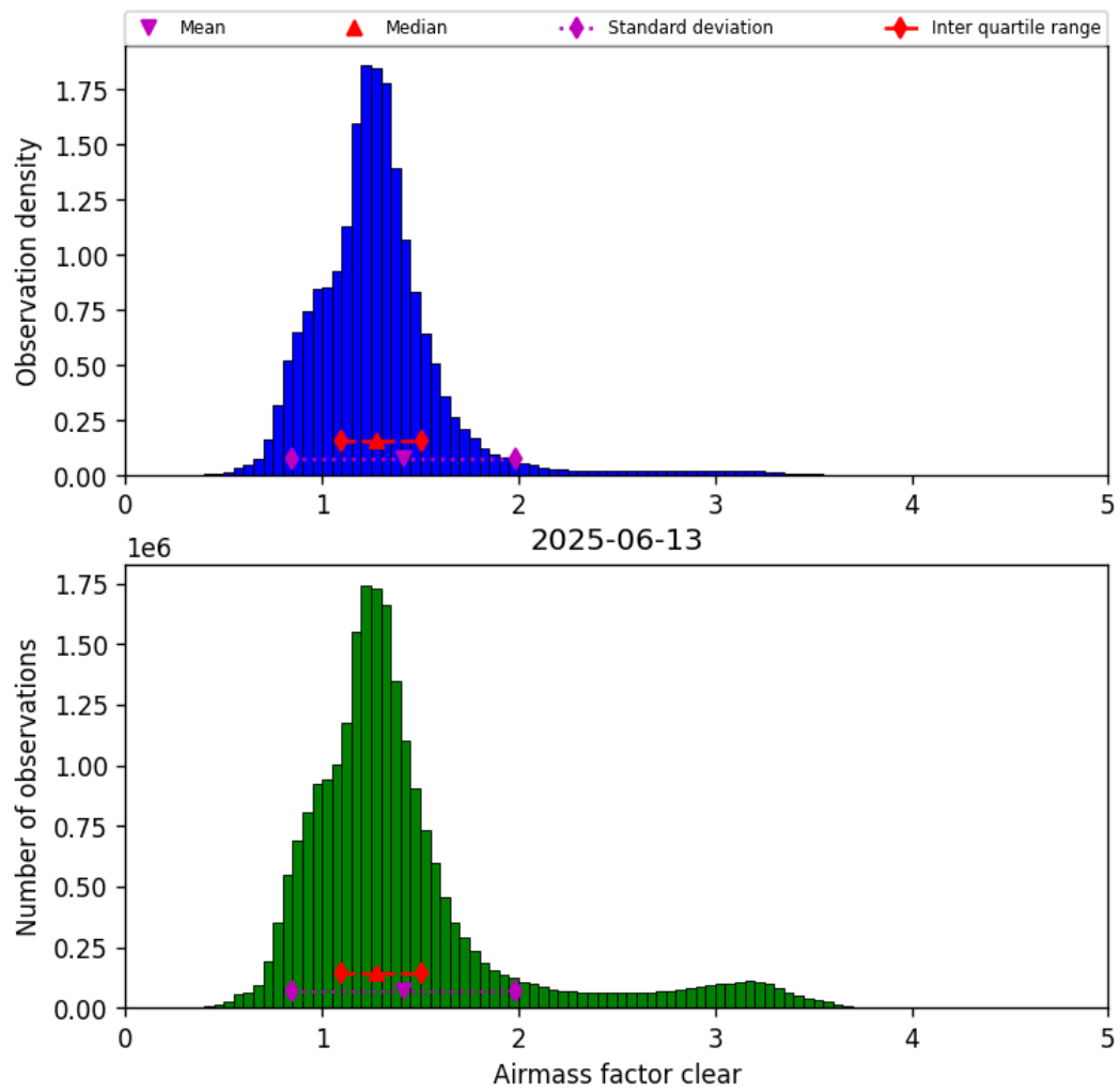
Figure 40: Histogram of “Airmass factor clear” for 2025-06-13 to 2025-06-14
