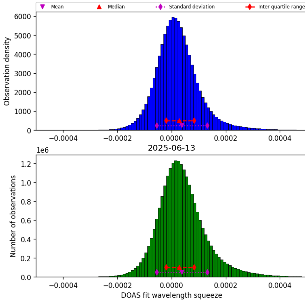
Figure 43: Histogram of “DOAS fit wavelength squeeze” for 2025-06-13 to 2025-06-14
