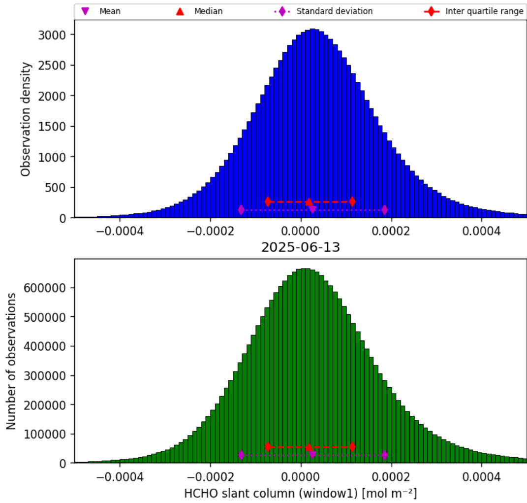
Figure 36: Histogram of “HCHO slant column (window1)” for 2025-06-13 to 2025-06-14
