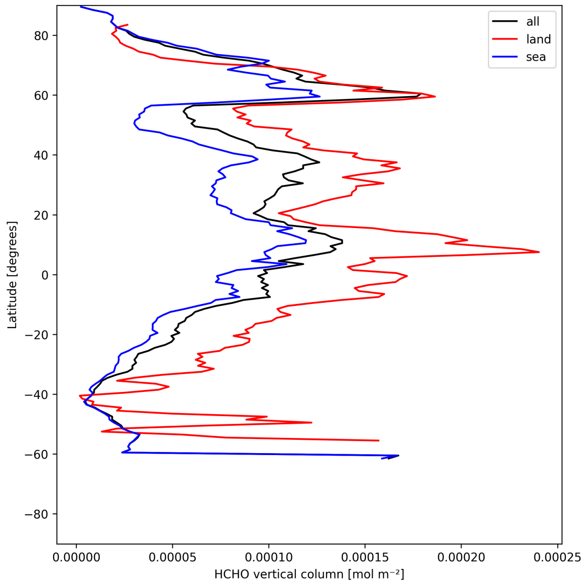
Figure 19: Zonal average of “HCHO vertical column” for 2025-06-13 to 2025-06-14.
