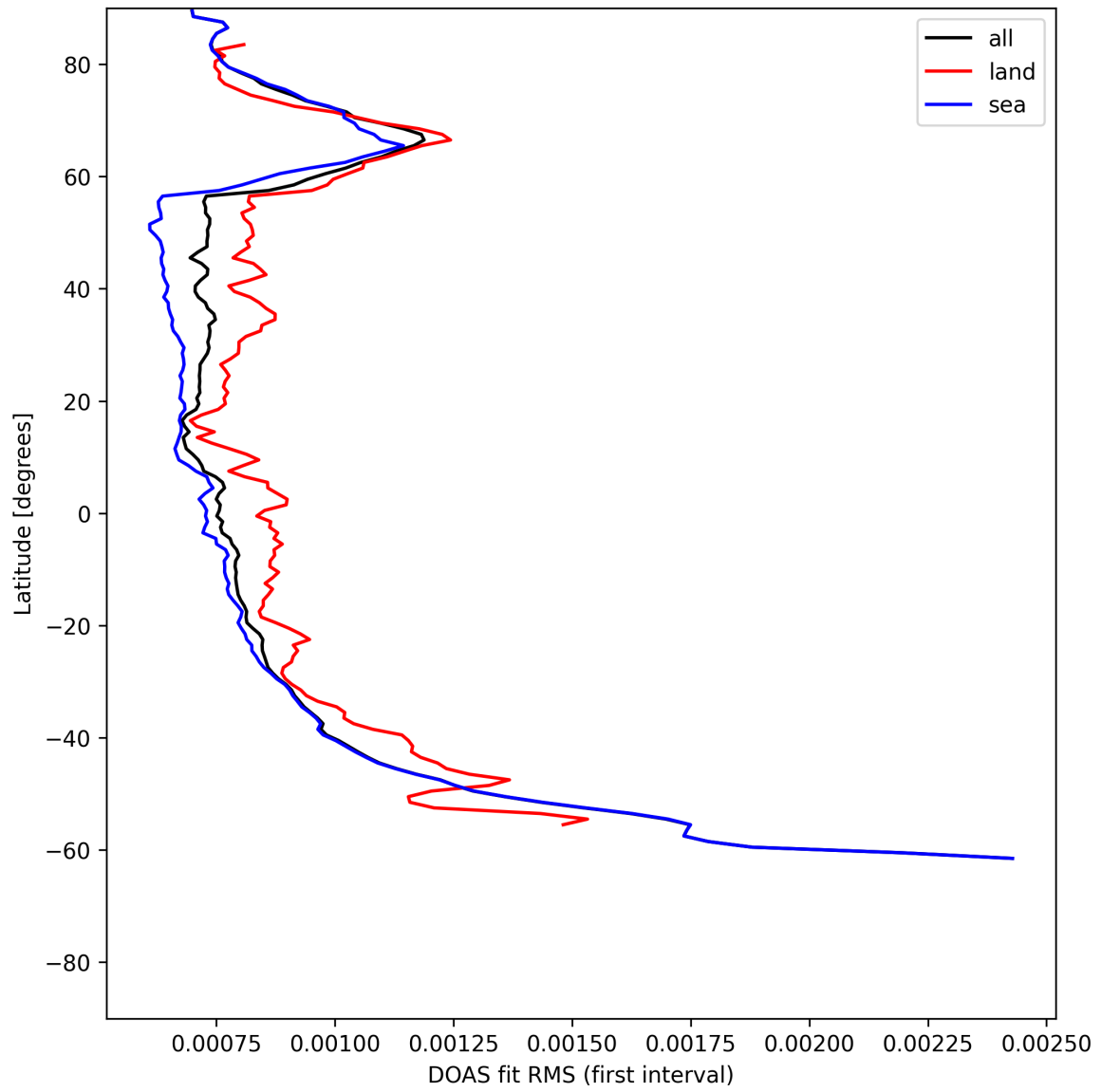
Figure 30: Zonal average of “DOAS fit RMS (first interval)” for 2025-06-13 to 2025-06-14.
