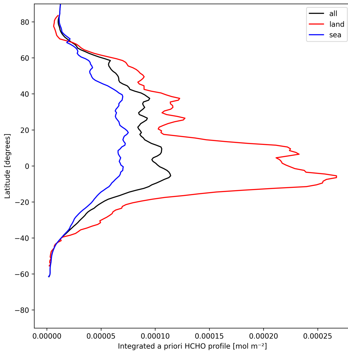
Figure 27: Zonal average of “Integrated a priori HCHO profile” for 2025-06-13 to 2025-06-14.
