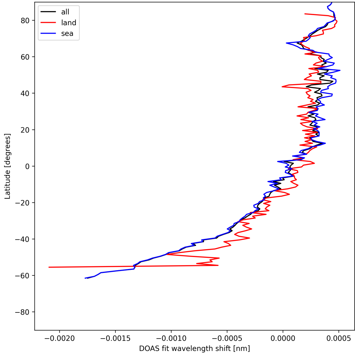
Figure 28: Zonal average of “DOAS fit wavelength shift” for 2025-06-13 to 2025-06-14.
