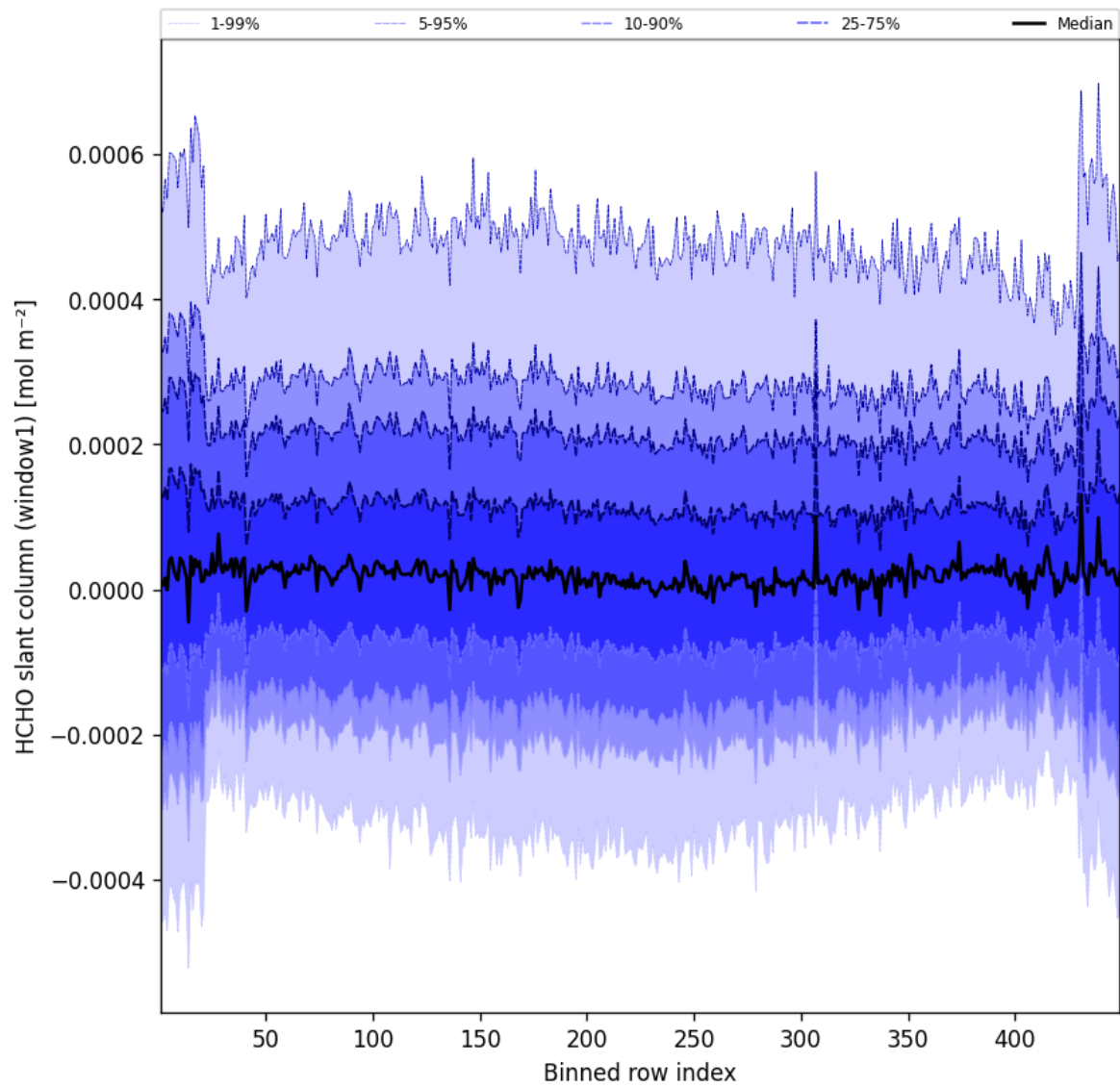
Figure 50: Along track statistics of “HCHO slant column (window1)” for 2025-06-13 to 2025-06-14
