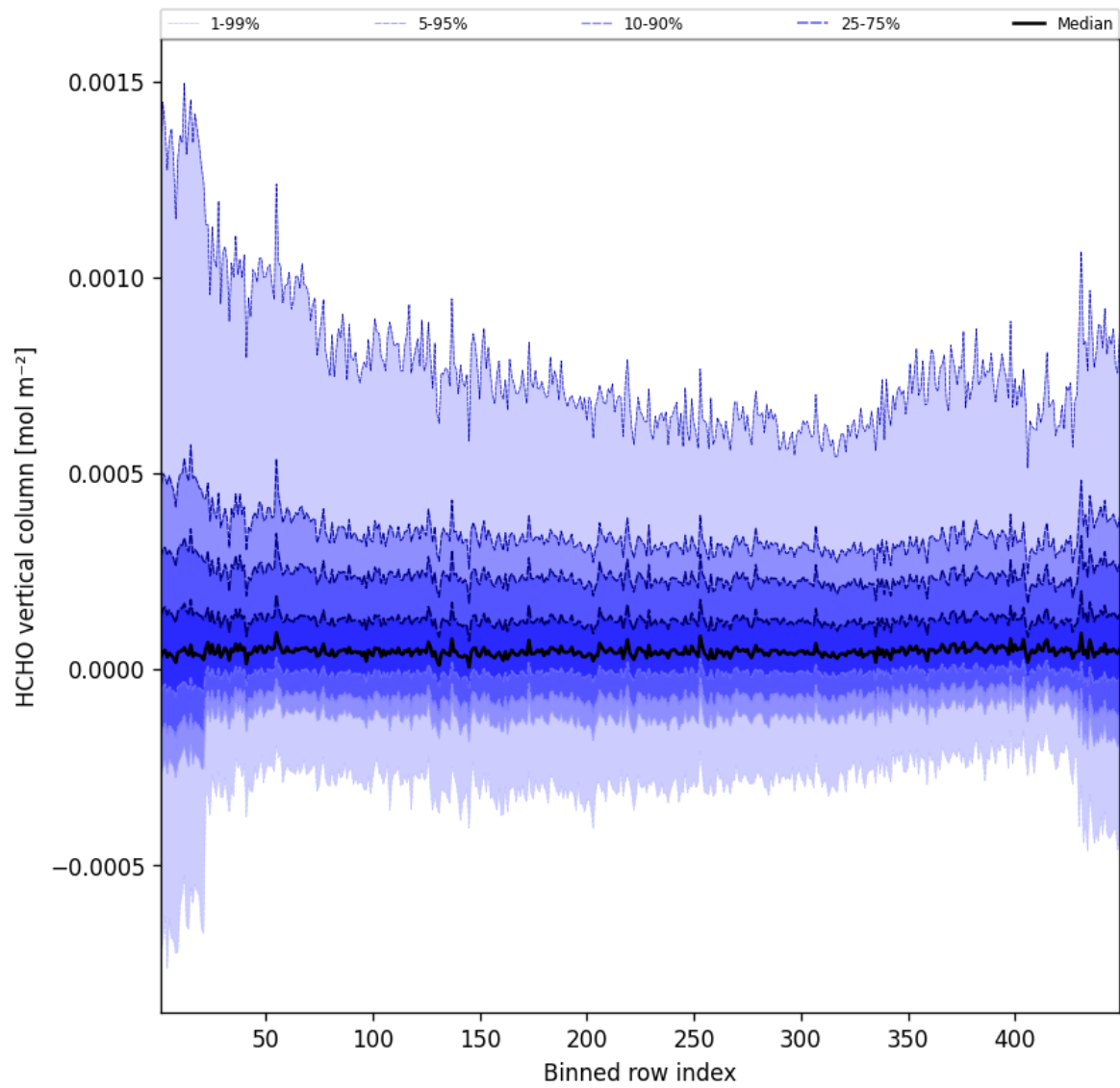
Figure 47: Along track statistics of “HCHO vertical column” for 2025-06-14 to 2025-06-14
