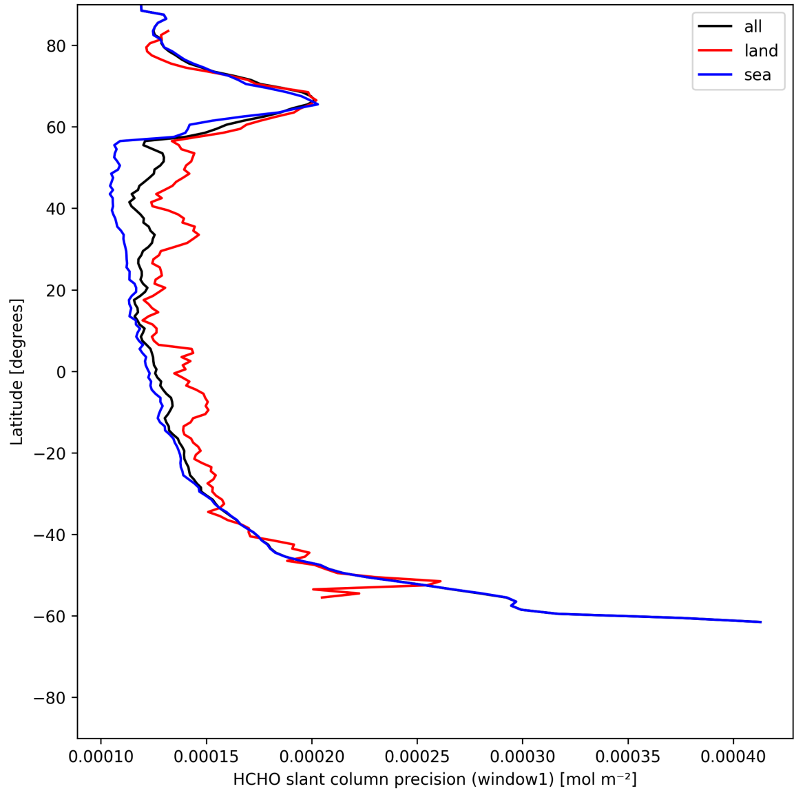
Figure 23: Zonal average of "HCHO slant column precision (window1)" for 2025-06-14 to 2025-06-14.
