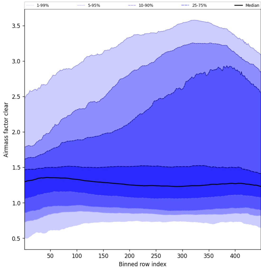
Figure 54: Along track statistics of “Air mass factor clear” for 2025-06-14 to 2025-06-14
