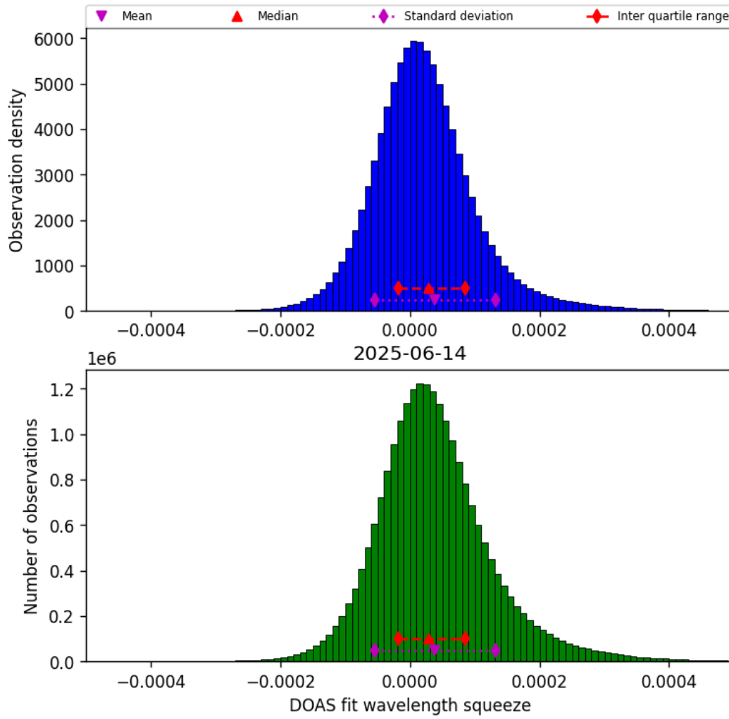
Figure 43: Histogram of “DOAS fit wavelength squeeze” for 2025-06-14 to 2025-06-14
