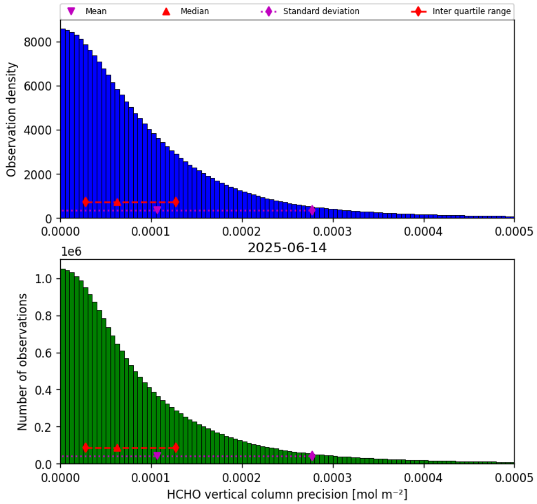
Figure 34: Histogram of “HCHO vertical column precision” for 2025-06-14 to 2025-06-14
