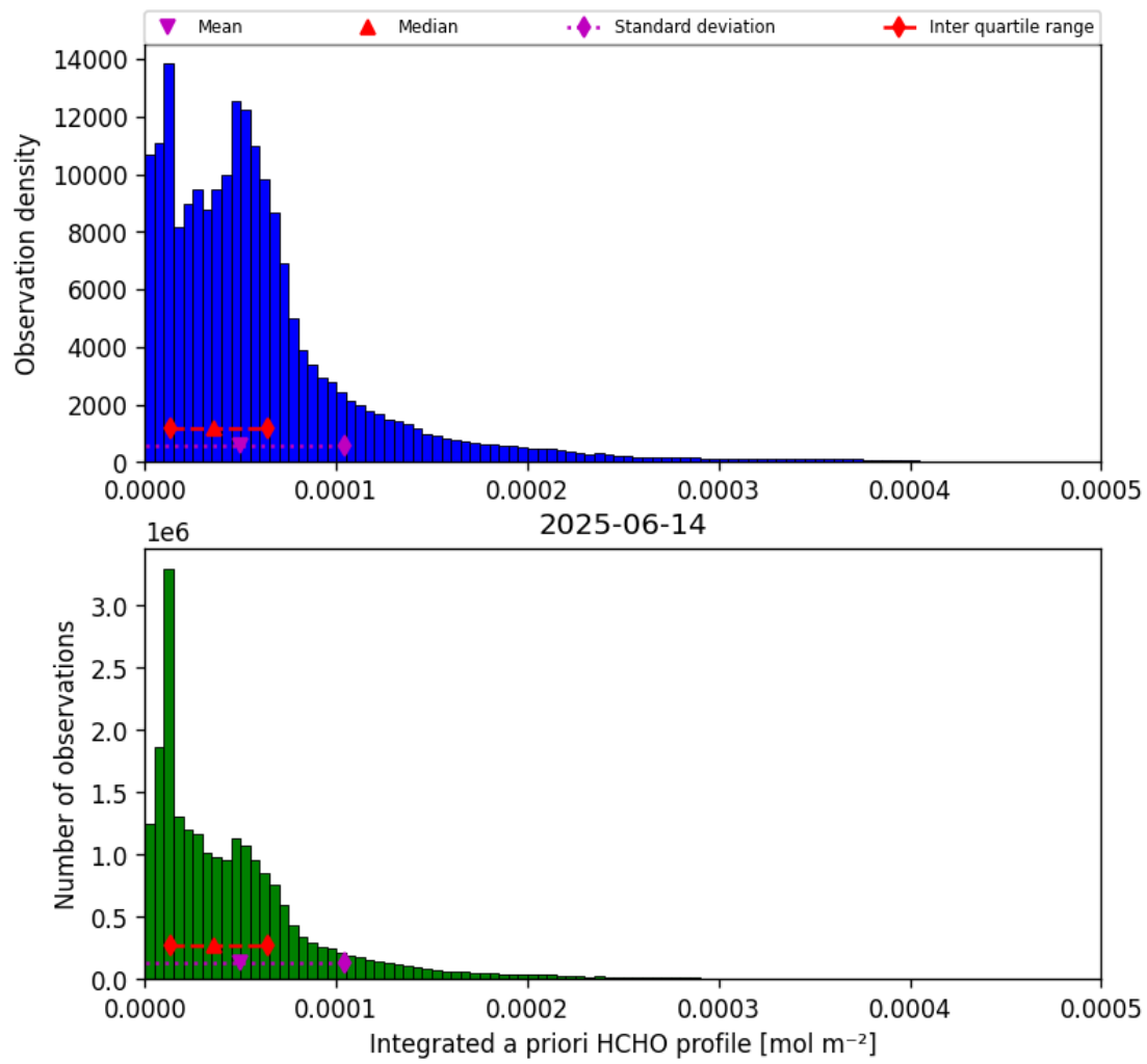
Figure 41: Histogram of “Integrated a priori HCHO profile” for 2025-06-14 to 2025-06-14
