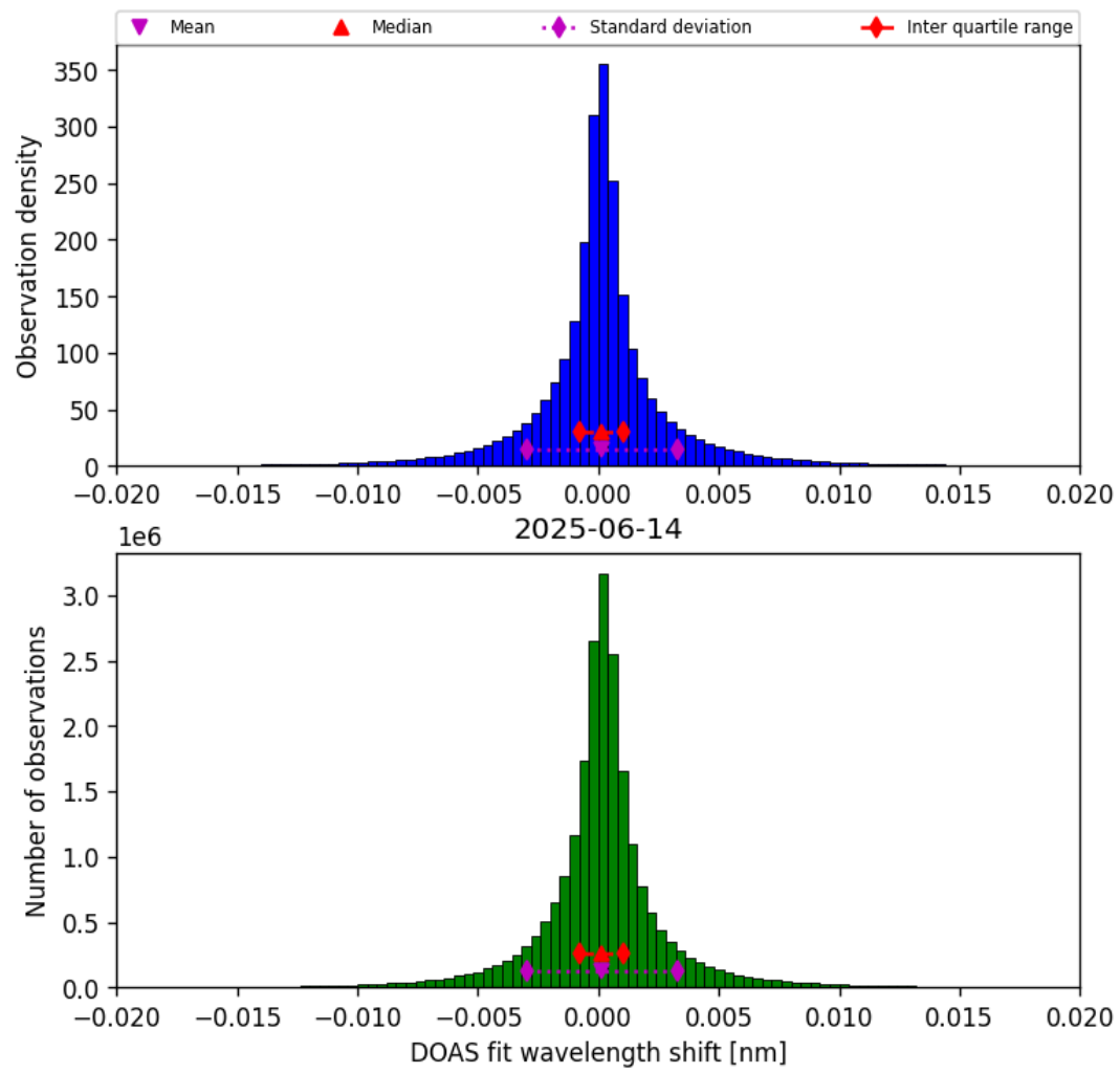
Figure 42: Histogram of “DOAS fit wavelength shift” for 2025-06-14 to 2025-06-14
