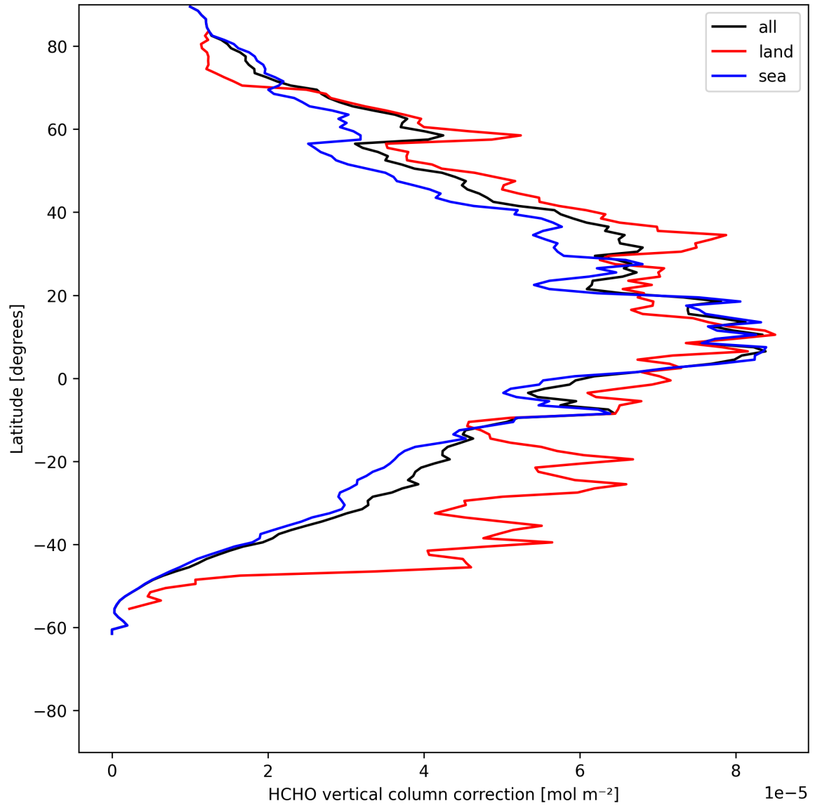
Figure 21: Zonal average of “HCHO vertical column correction” for 2025-06-14 to 2025-06-14.
