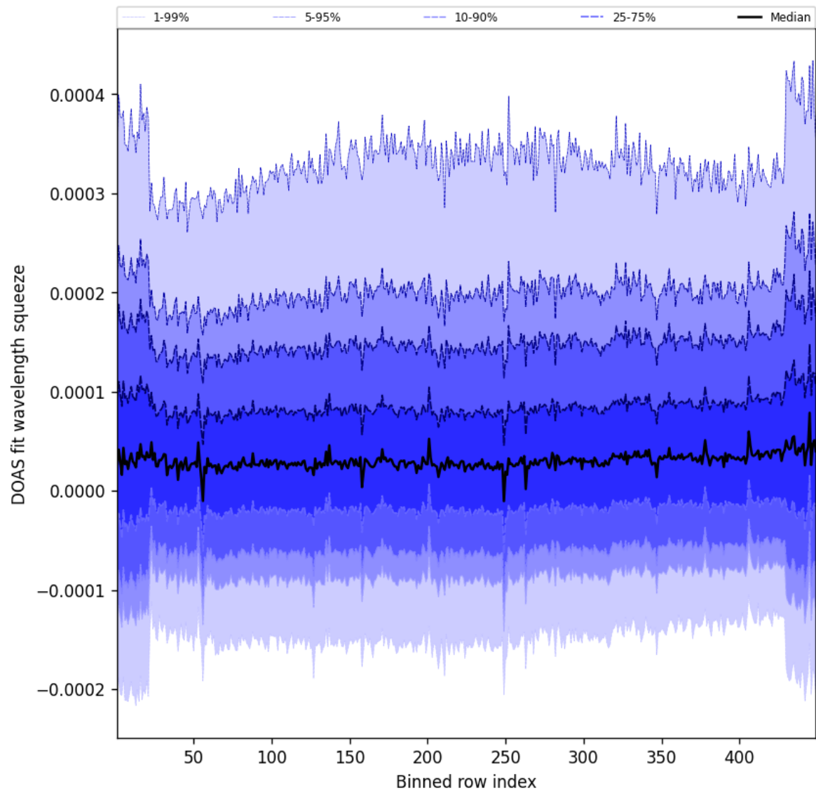
Figure 57: Along track statistics of “DOAS fit wavelength squeeze” for 2025-06-14 to 2025-06-14
