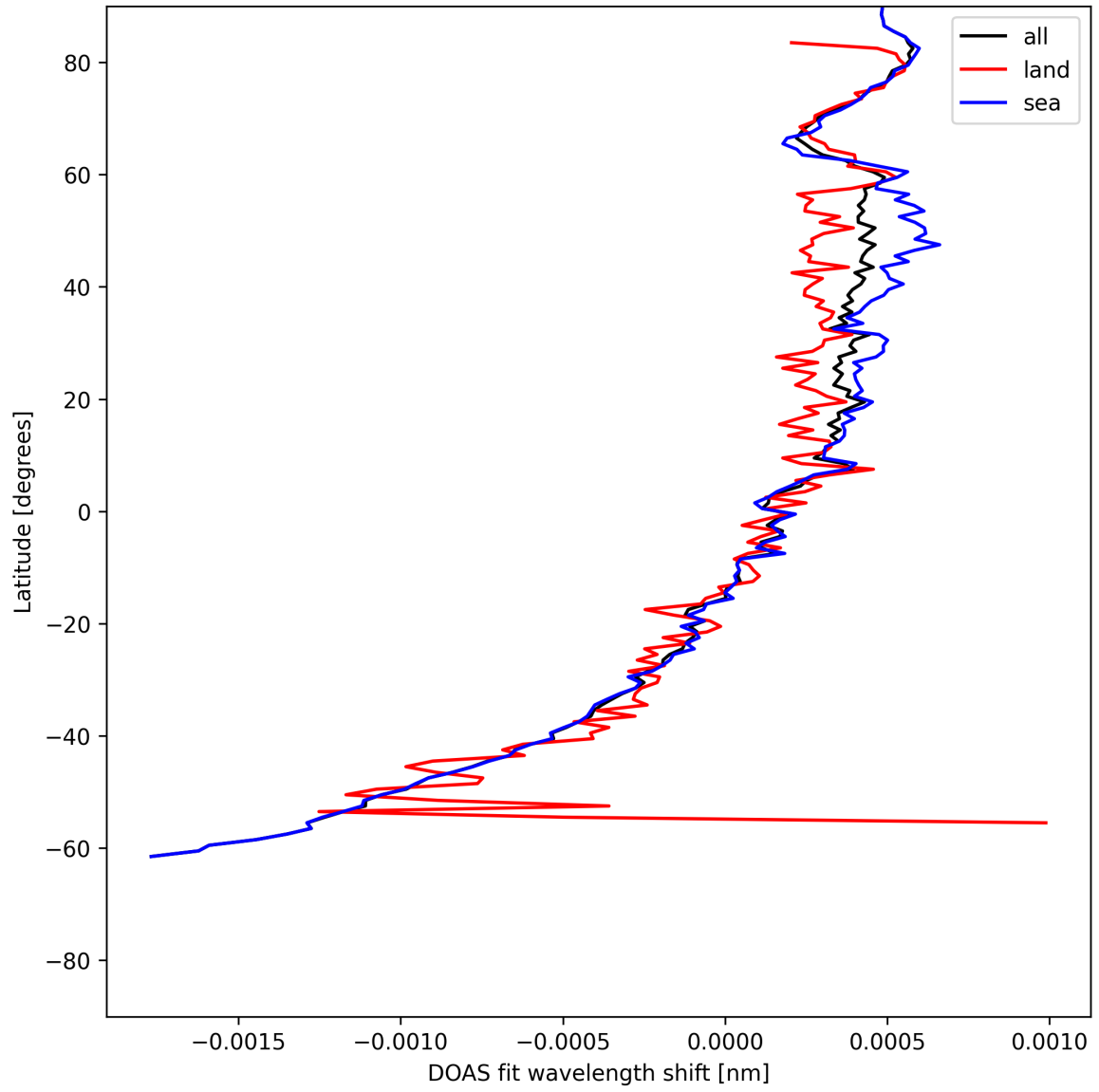
Figure 28: Zonal average of “DOAS fit wavelength shift” for 2025-06-14 to 2025-06-14.
