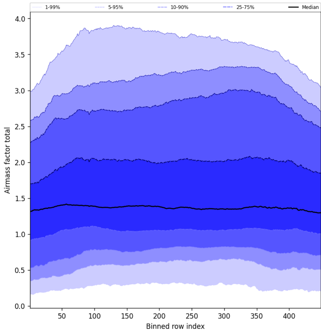
Figure 52: Along track statistics of “Airmass factor total” for 2025-06-14 to 2025-06-14
