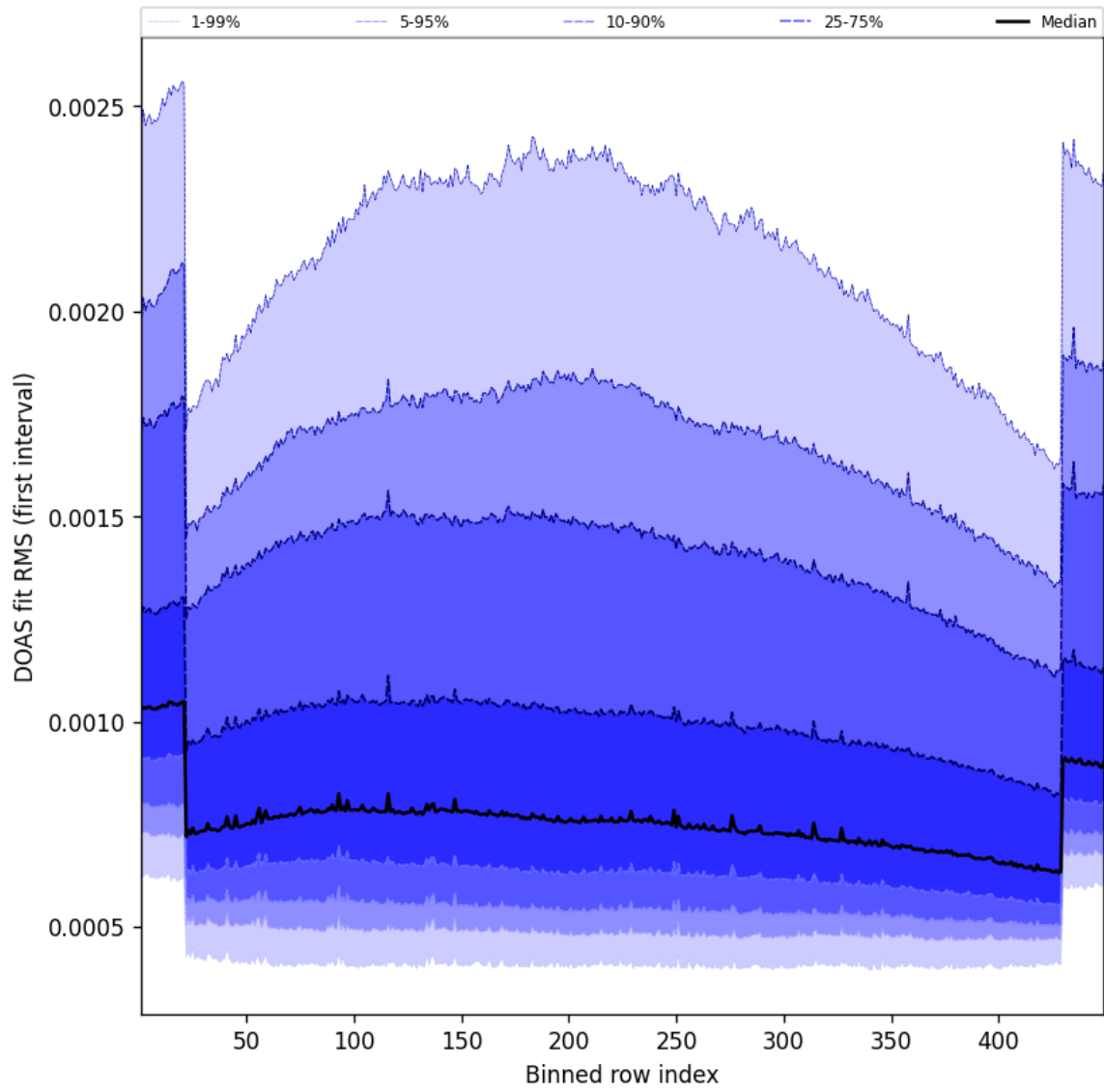
Figure 58: Along track statistics of “DOAS fit RMS (first interval)” for 2025-06-14 to 2025-06-14
