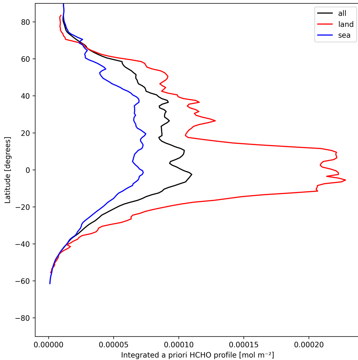
Figure 27: Zonal average of “Integrated a priori HCHO profile” for 2025-06-14 to 2025-06-14.
