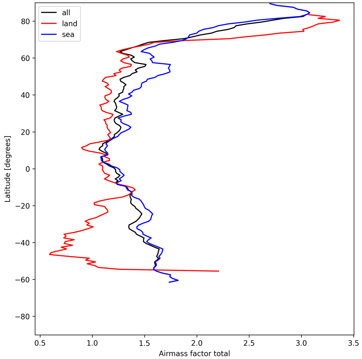
Figure 24: Zonal average of “Airmass factor total” for 2025-06-14 to 2025-06-14.
