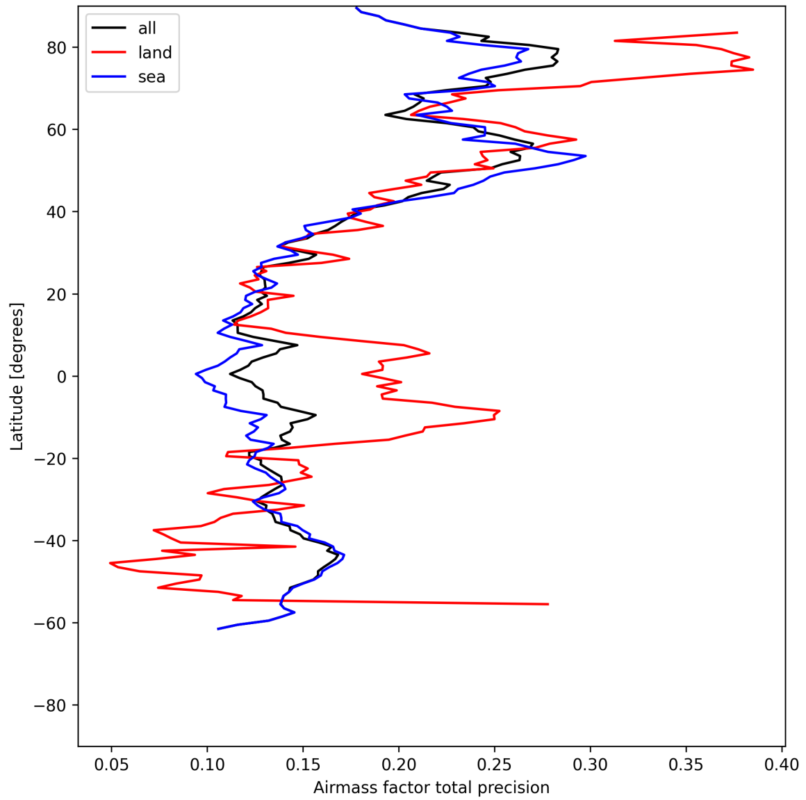
Figure 25: Zonal average of “Airmass factor total precision” for 2025-06-14 to 2025-06-14.
