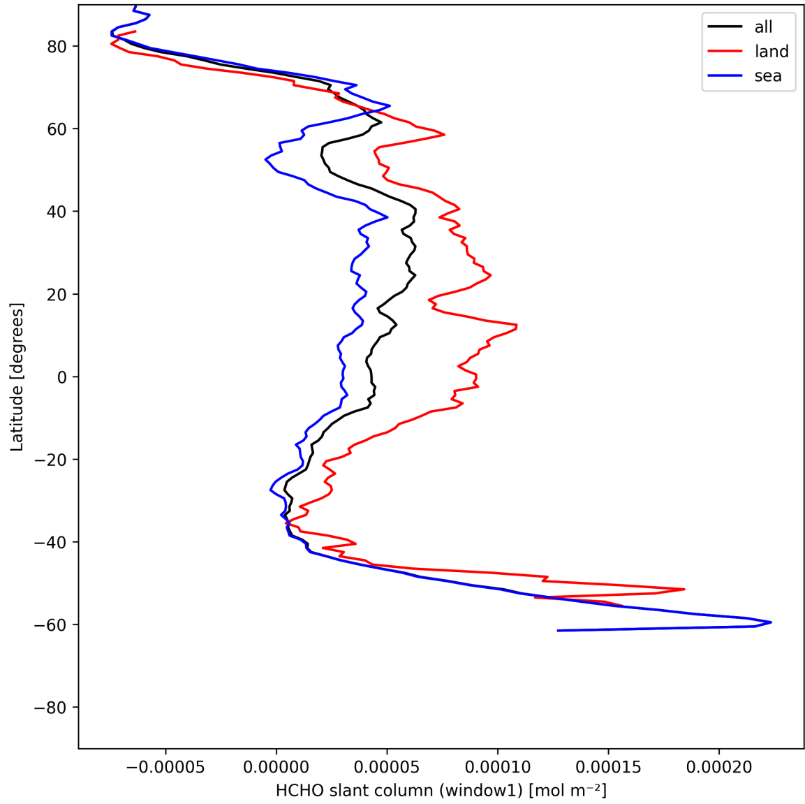
Figure 22: Zonal average of “HCHO slant column (window1)” for 2025-06-14 to 2025-06-14.
