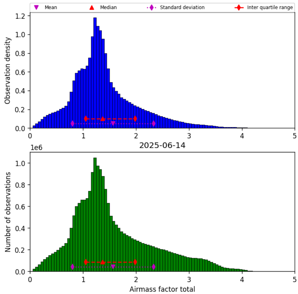
Figure 38: Histogram of “Airmass factor total” for 2025-06-14 to 2025-06-14
