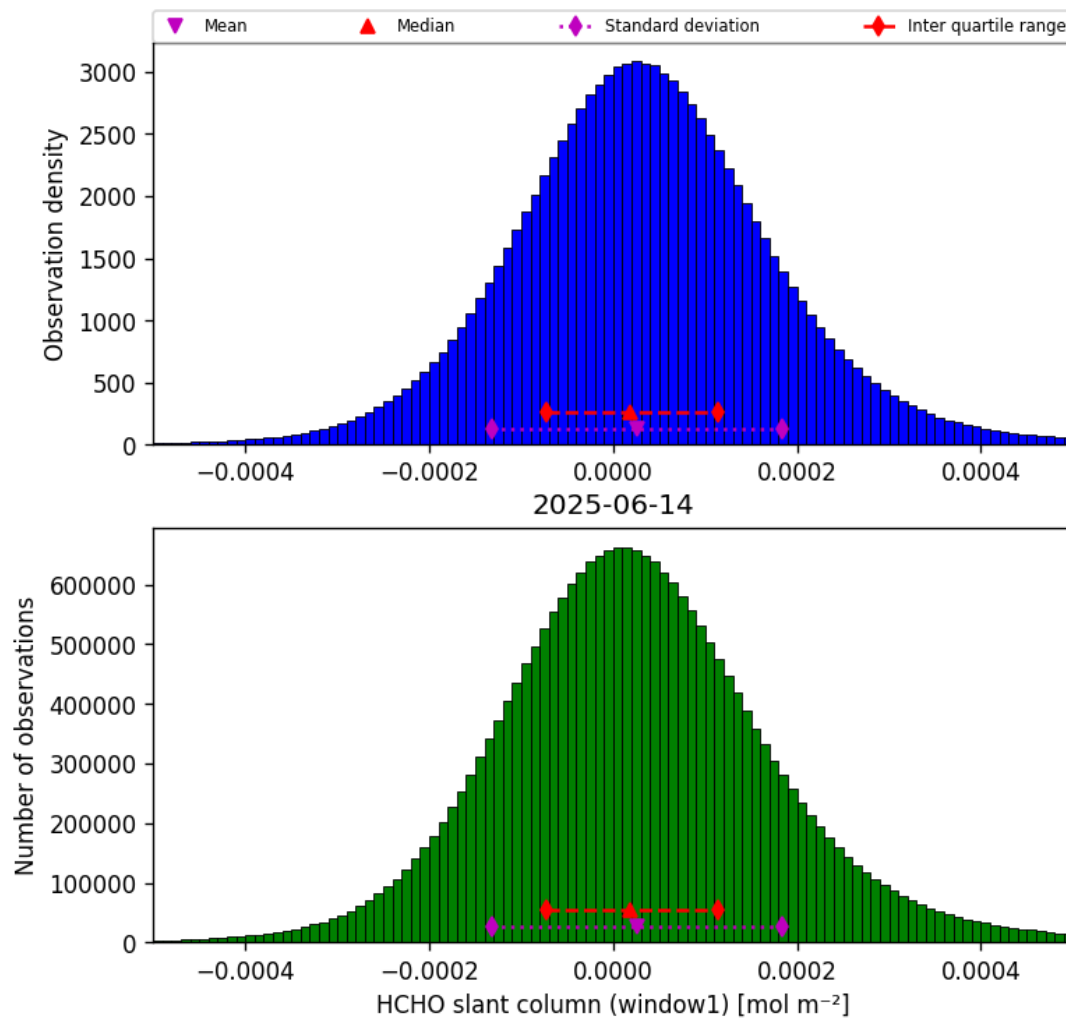
Figure 36: Histogram of “HCHO slant column (window1)” for 2025-06-14 to 2025-06-14
