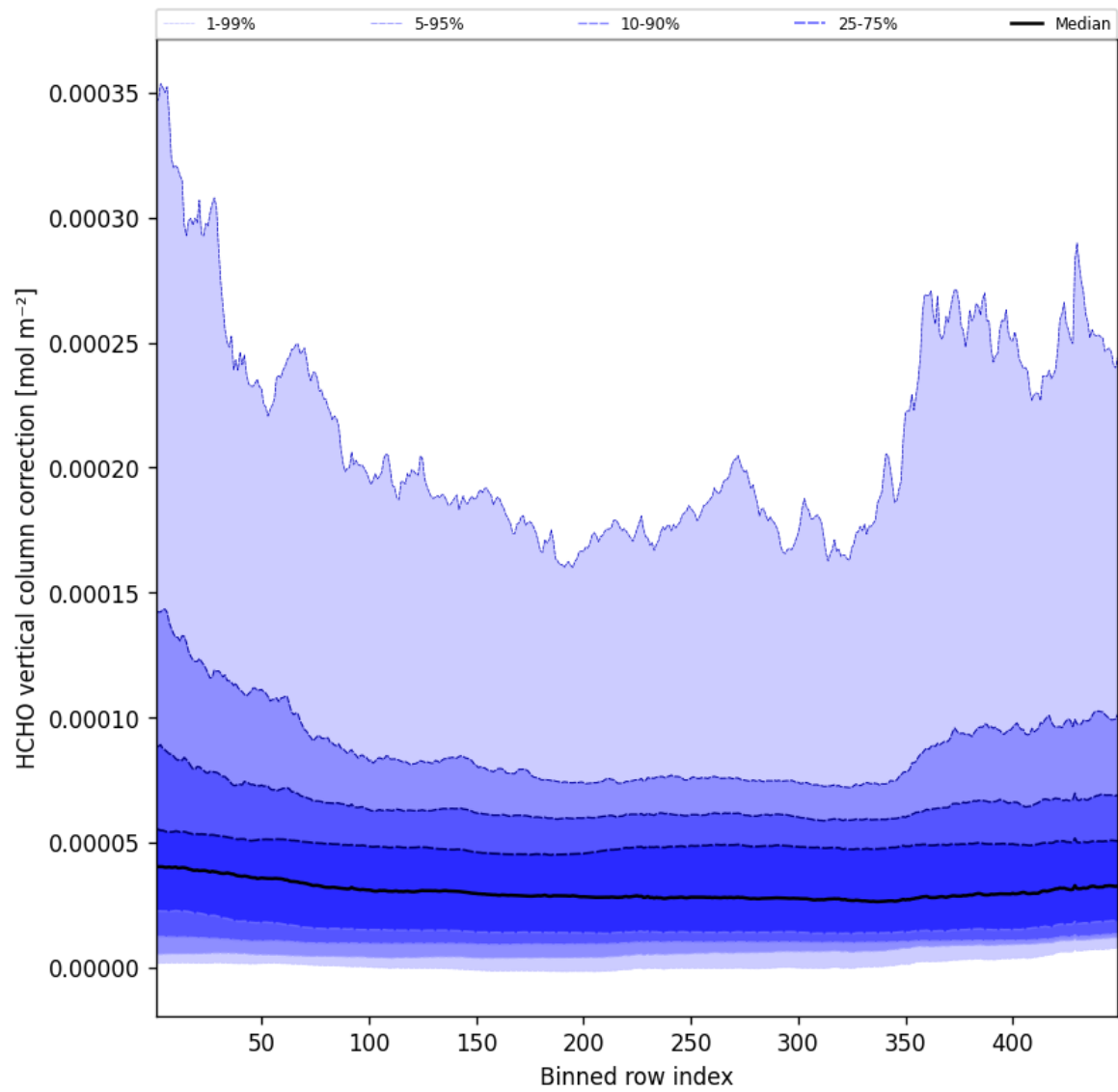
Figure 49: Along track statistics of “HCHO vertical column correction” for 2025-06-14 to 2025-06-14
