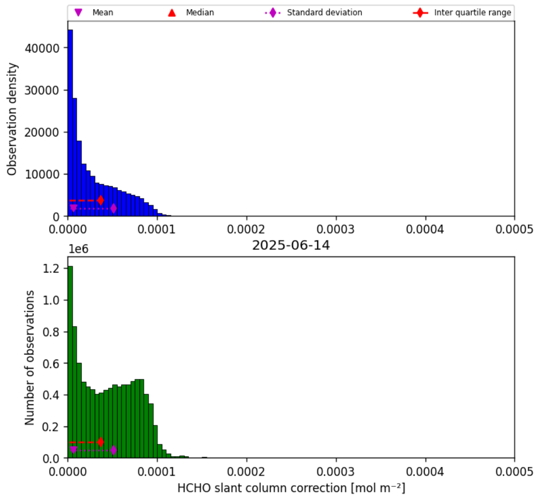
Figure 45: Histogram of “HCHO slant column correction” for 2025-06-14 to 2025-06-14
