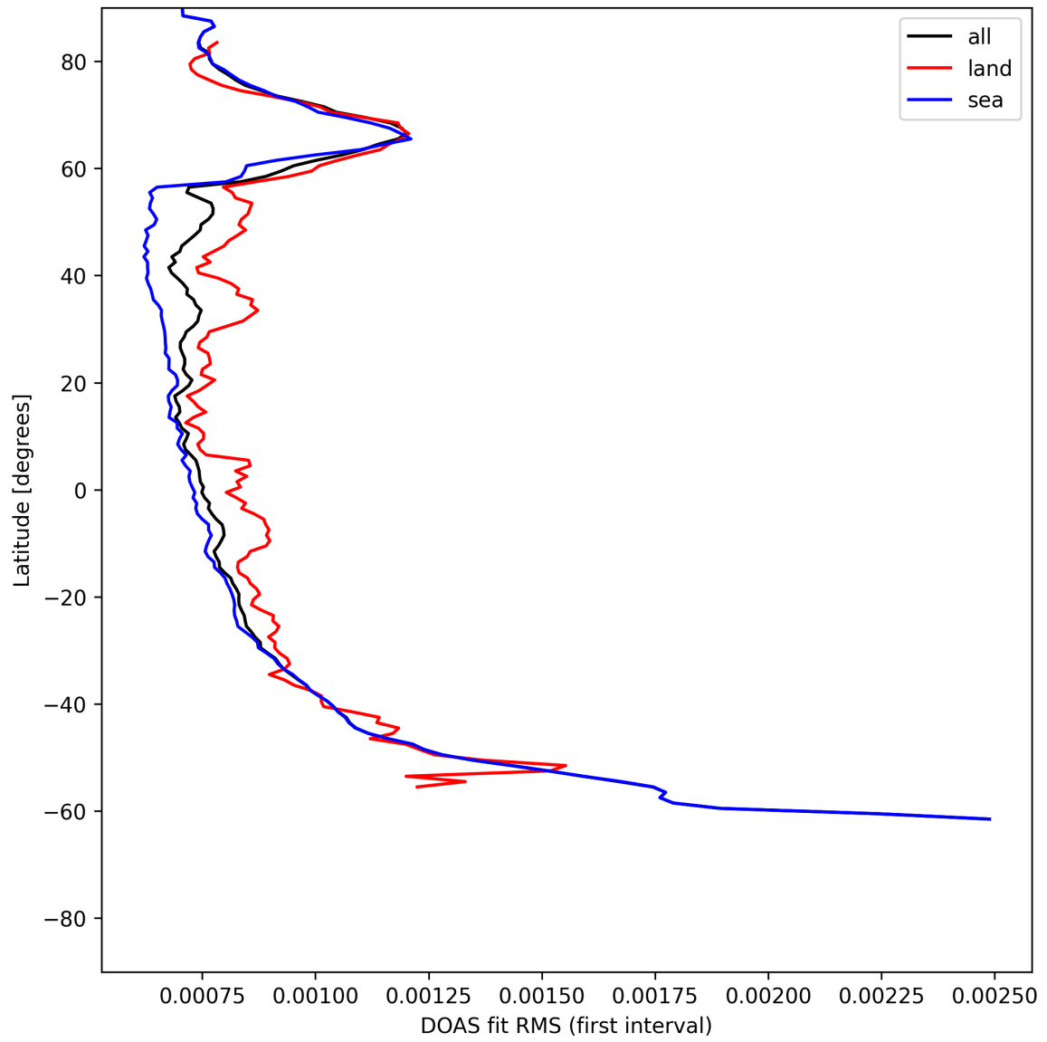
Figure 30: Zonal average of “DOAS fit RMS (first interval)” for 2025-06-14 to 2025-06-14.
