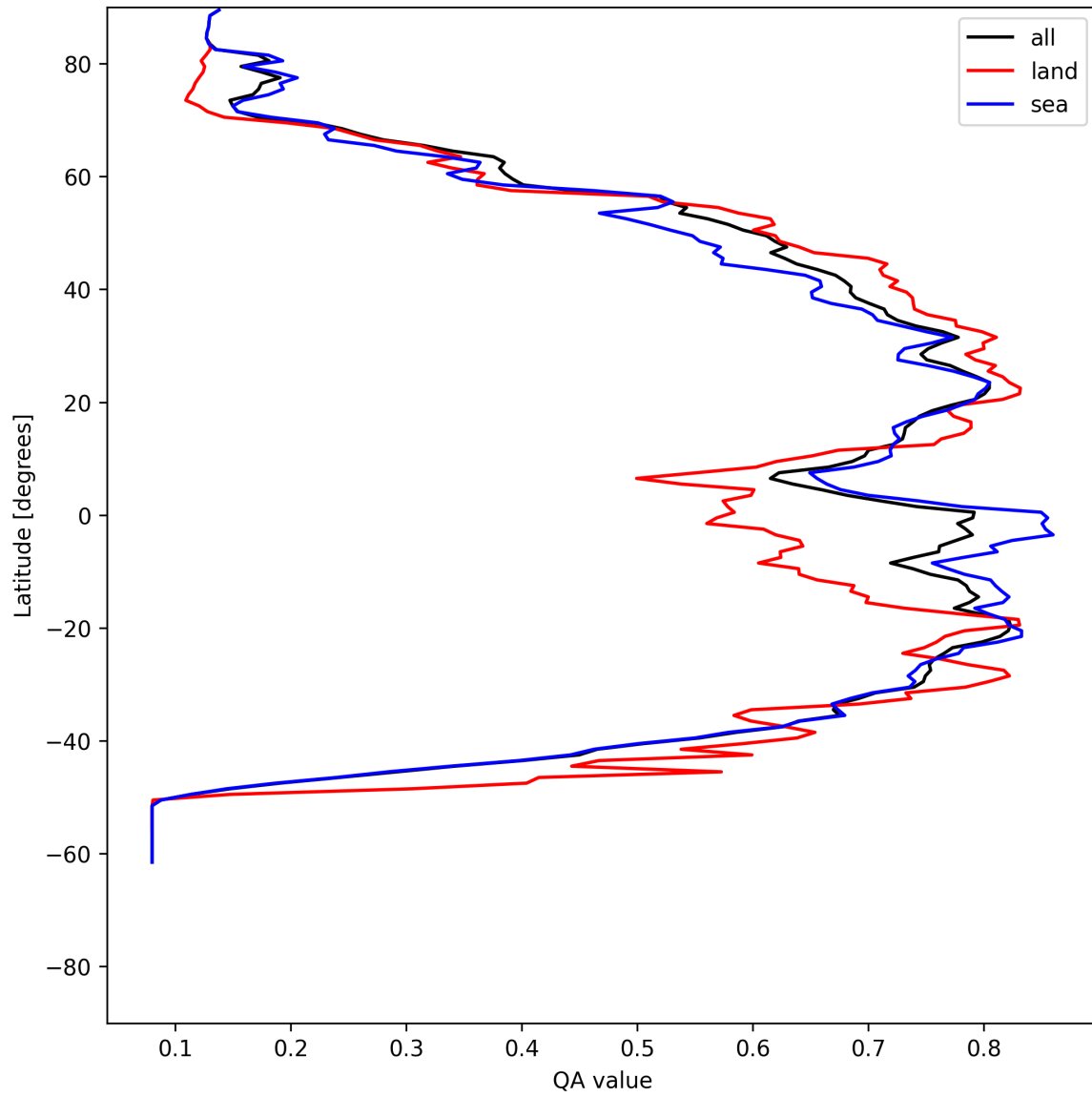
Figure 18: Zonal average of “QA value” for 2025-06-14 to 2025-06-14.
