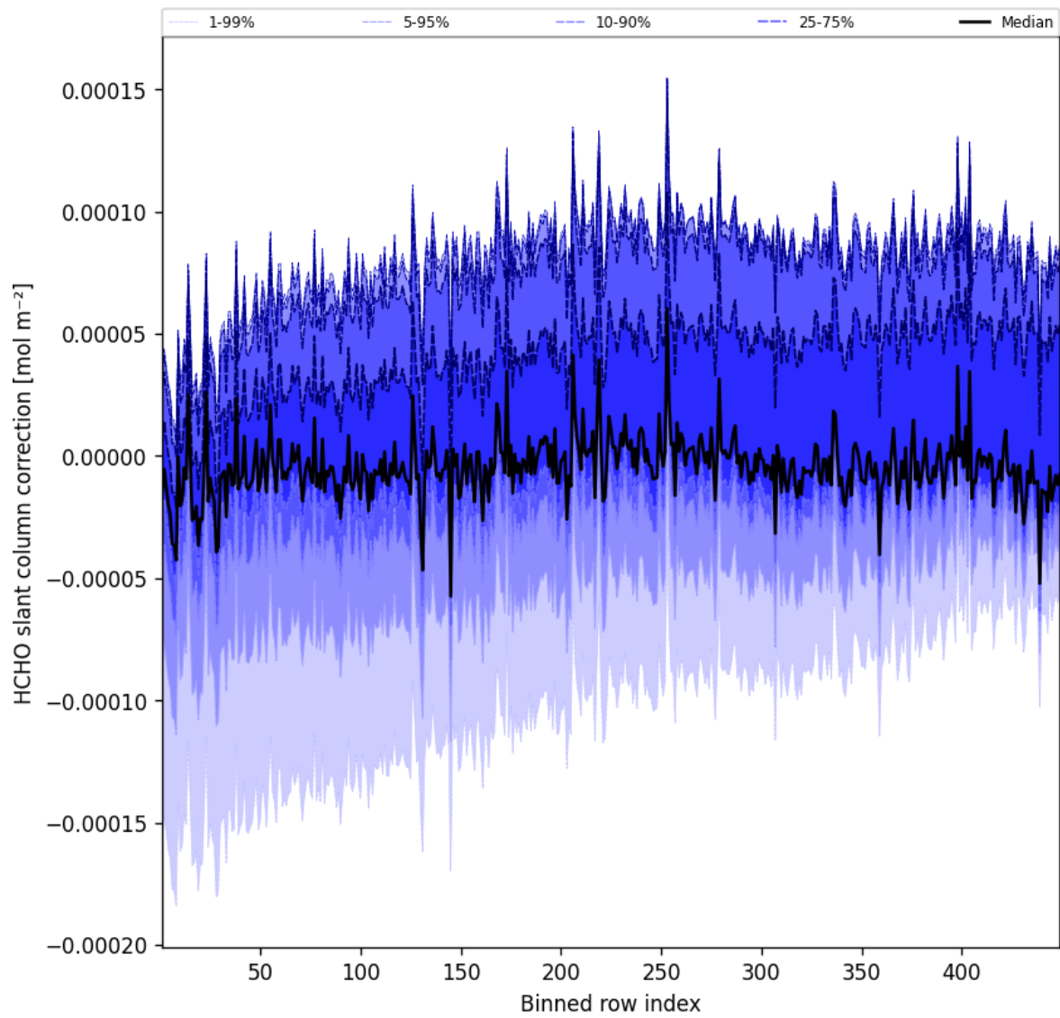
Figure 59: Along track statistics of “HCHO slant column correction” for 2025-06-14 to 2025-06-14
