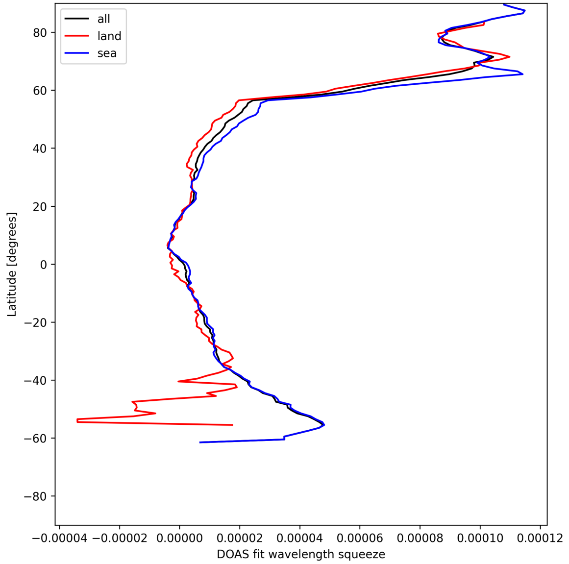
Figure 29: Zonal average of “DOAS fit wavelength squeeze” for 2025-06-14 to 2025-06-14.
