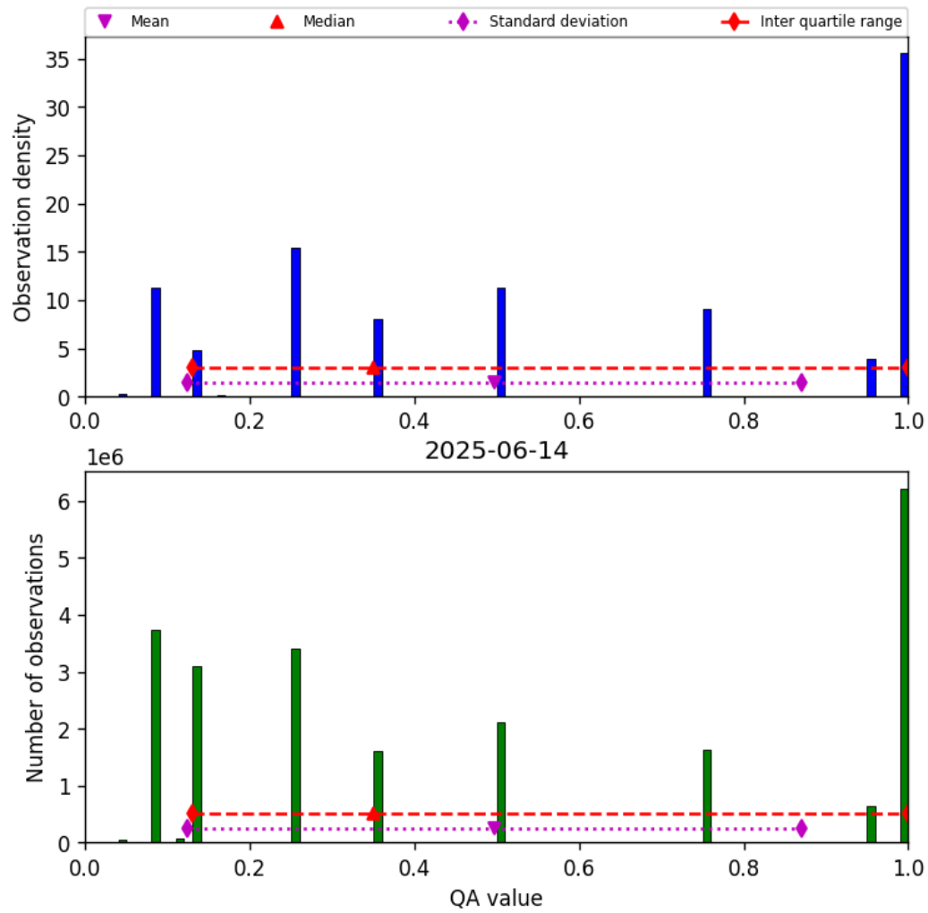
Figure 32: Histogram of “QA value” for 2025-06-14 to 2025-06-14
