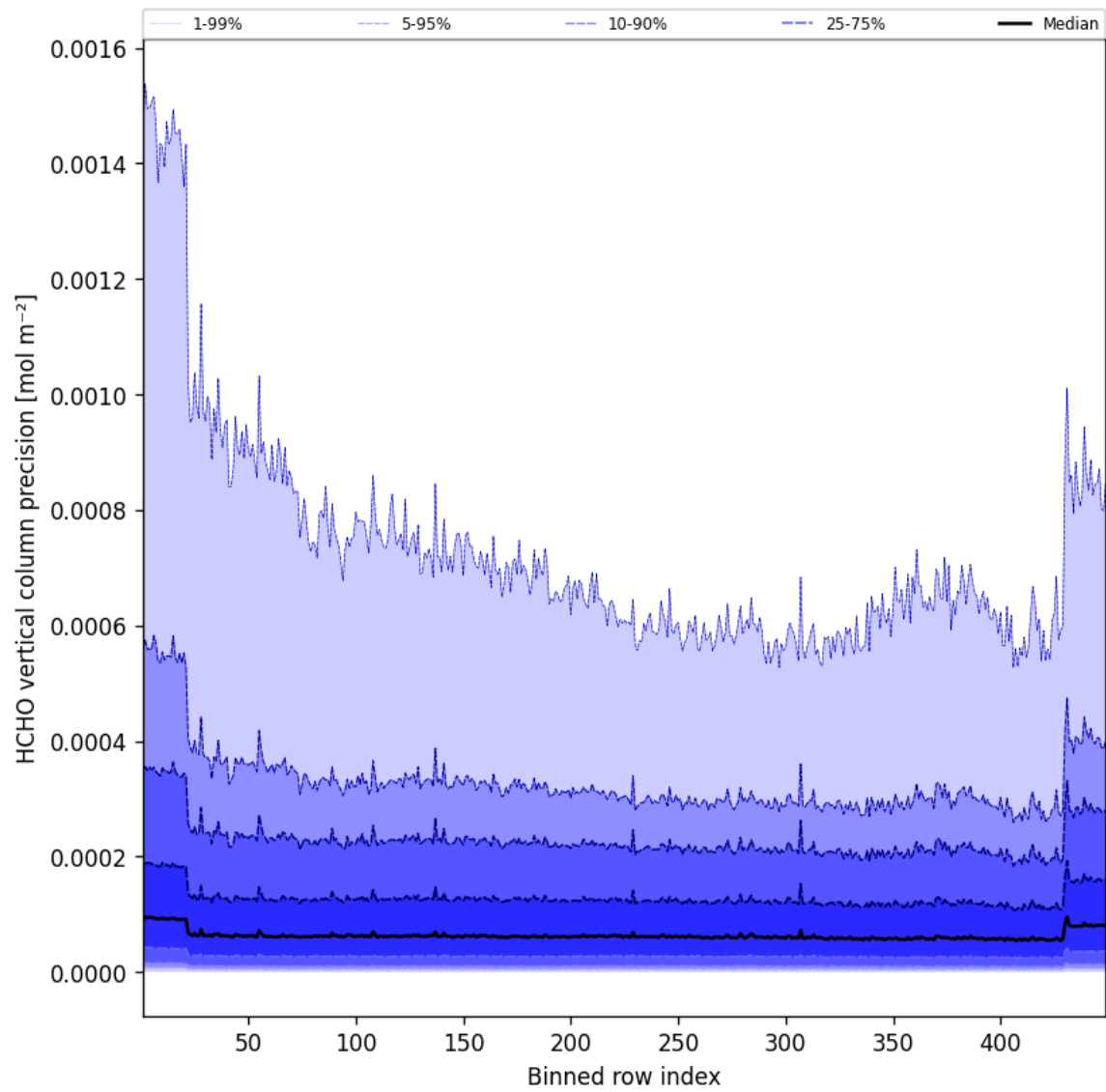
Figure 48: Along track statistics of “HCHO vertical column precision” for 2025-06-14 to 2025-06-14
