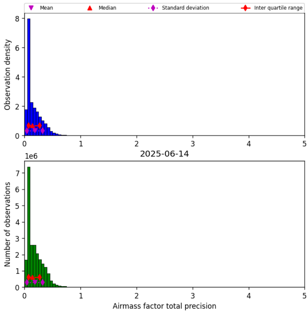
Figure 39: Histogram of “Airmass factor total precision” for 2025-06-14 to 2025-06-14
