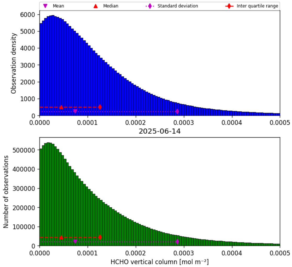
Figure 33: Histogram of “HCHO vertical column” for 2025-06-14 to 2025-06-14
