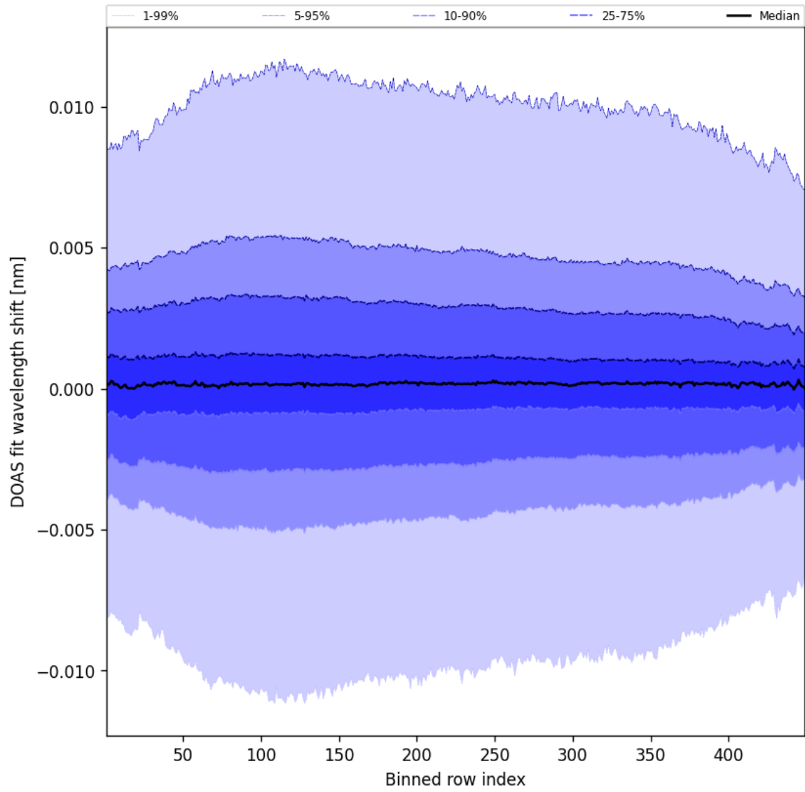
Figure 56: Along track statistics of “DOAS fit wavelength shift” for 2025-06-14 to 2025-06-14
