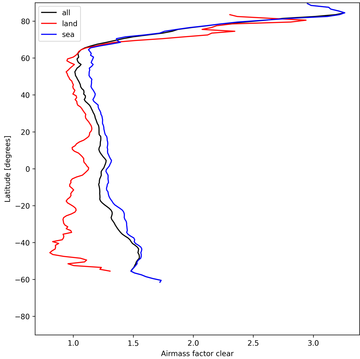
Figure 26: Zonal average of “Airmass factor clear” for 2025-06-14 to 2025-06-14.
