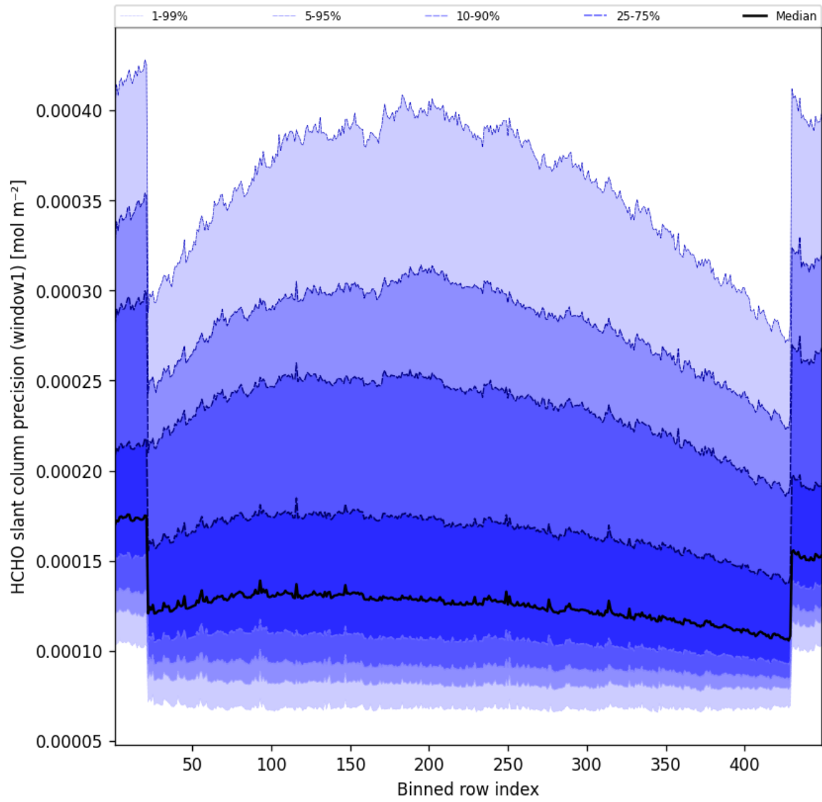
Figure 51: Along track statistics of “HCHO slant column precision (window1)” for 2025-06-14 to 2025-06-14
