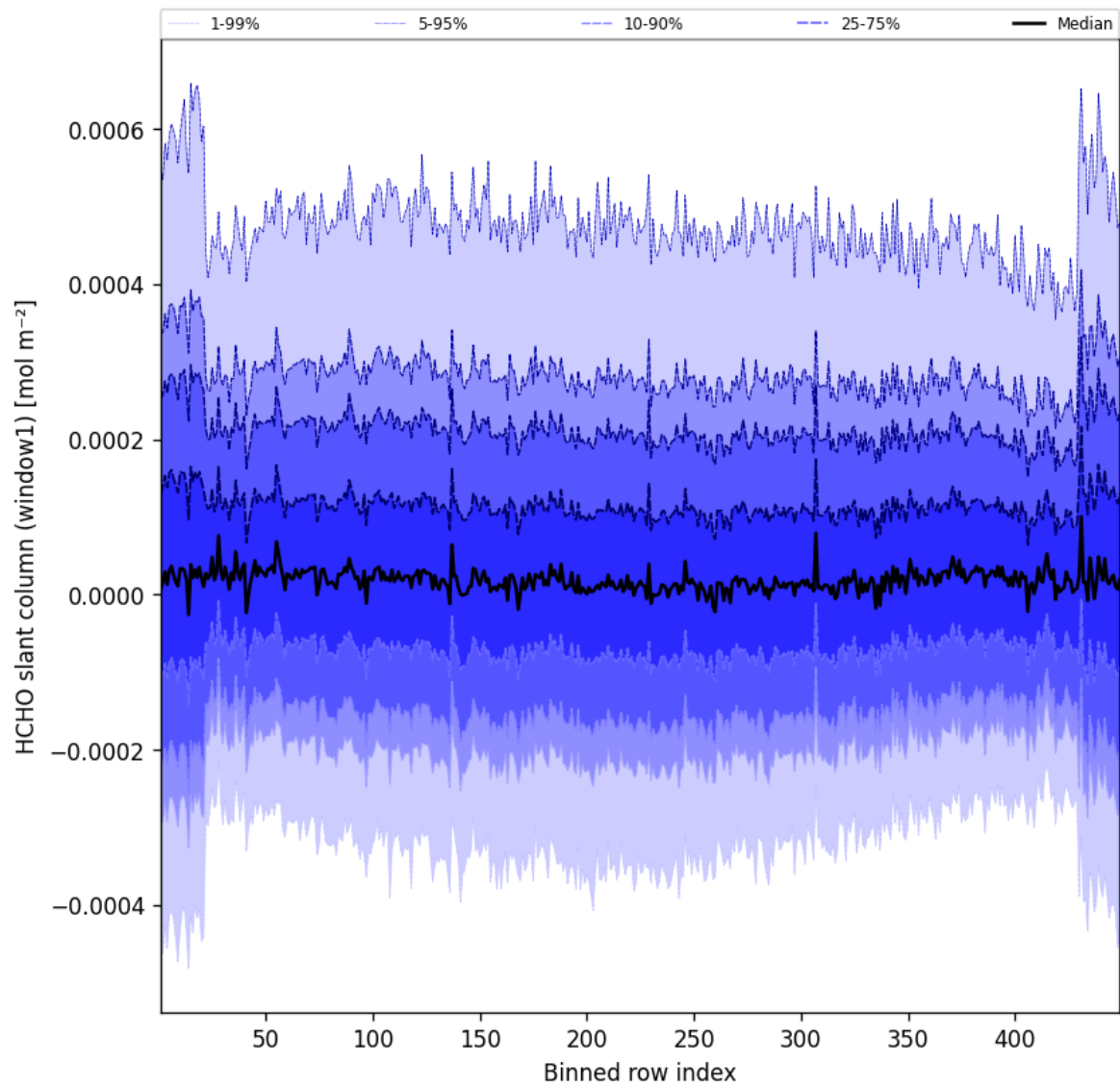
Figure 50: Along track statistics of “HCHO slant column (window1)” for 2025-06-14 to 2025-06-14
