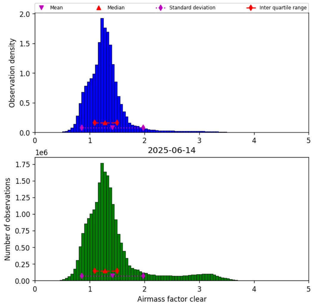
Figure 40: Histogram of “Airmass factor clear” for 2025-06-14 to 2025-06-14
