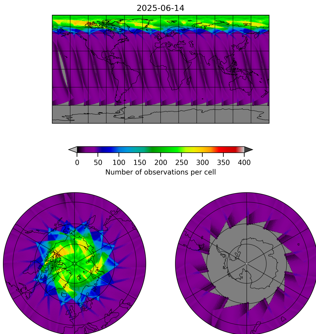
Figure 17: Map of the number of observations for 2025-06-14 to 2025-06-14
