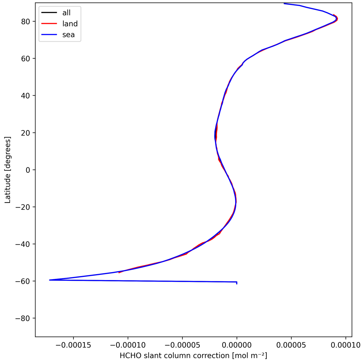
Figure 31: Zonal average of “HCHO slant column correction” for 2025-06-14 to 2025-06-14.
