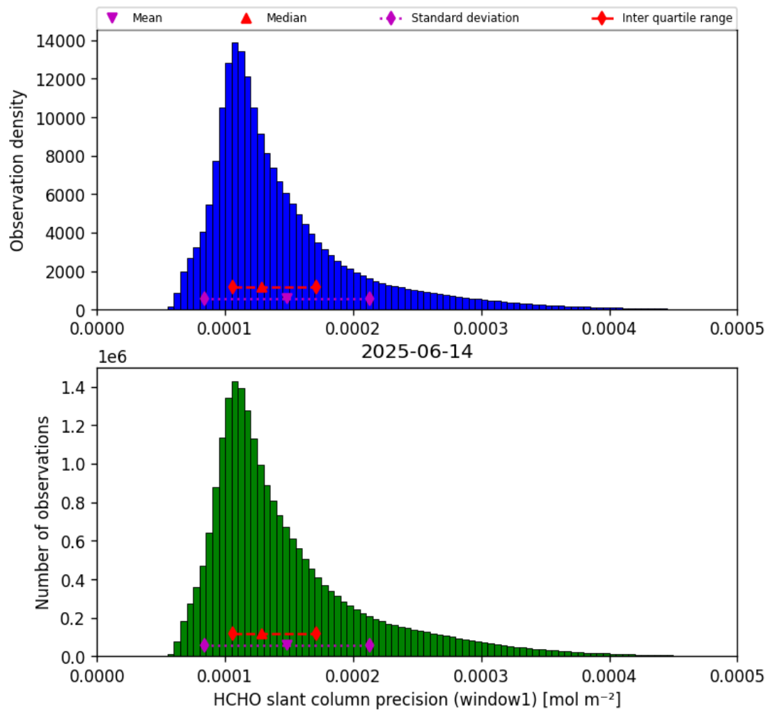
Figure 37: Histogram of “HCHO slant column precision (window1)” for 2025-06-14 to 2025-06-14
