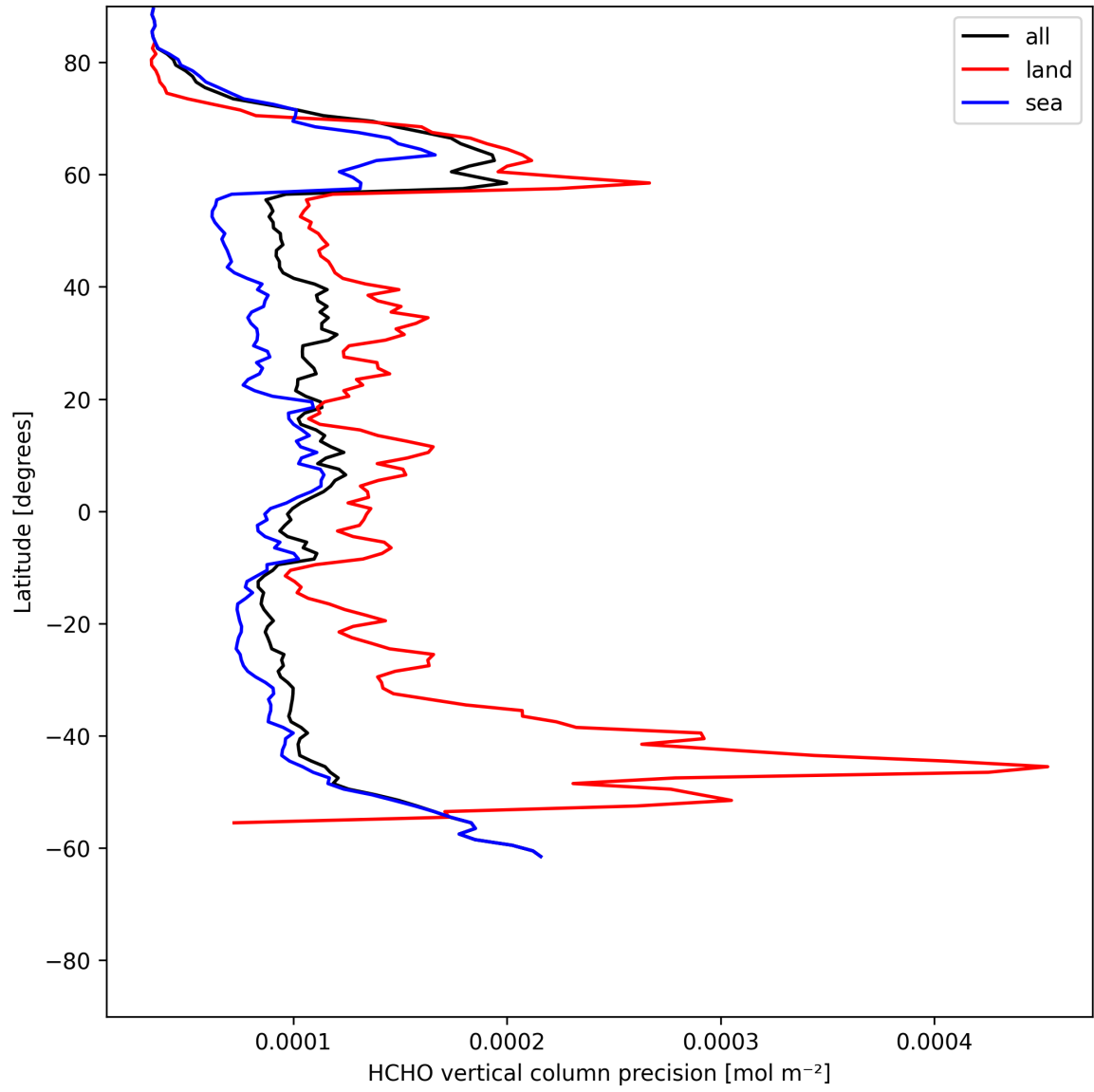
Figure 20: Zonal average of “HCHO vertical column precision” for 2025-06-14 to 2025-06-14.
