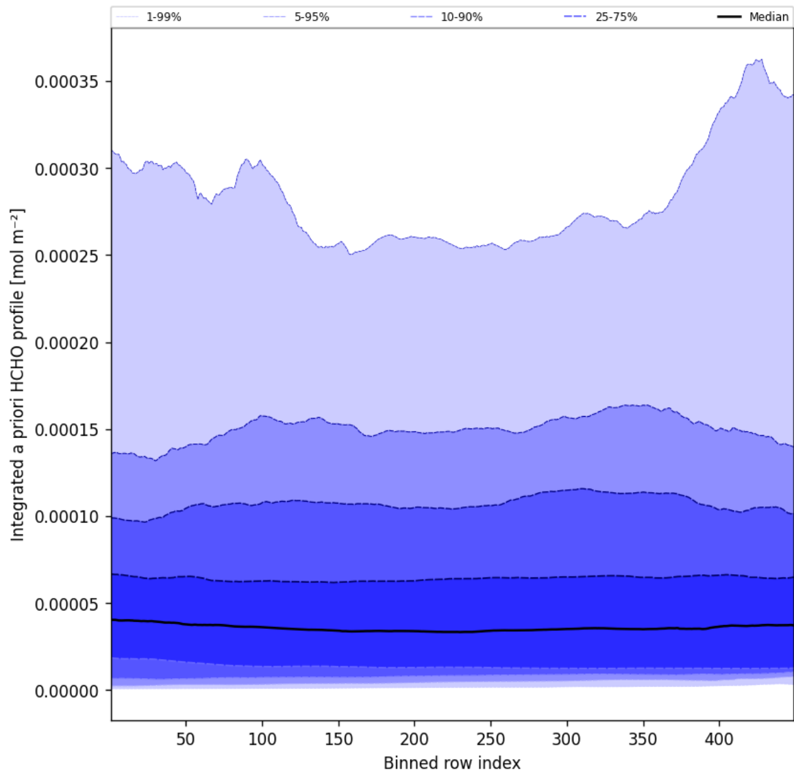
Figure 55: Along track statistics of "Integrated a priori HCHO profile" for 2025-06-14 to 2025-06-14
