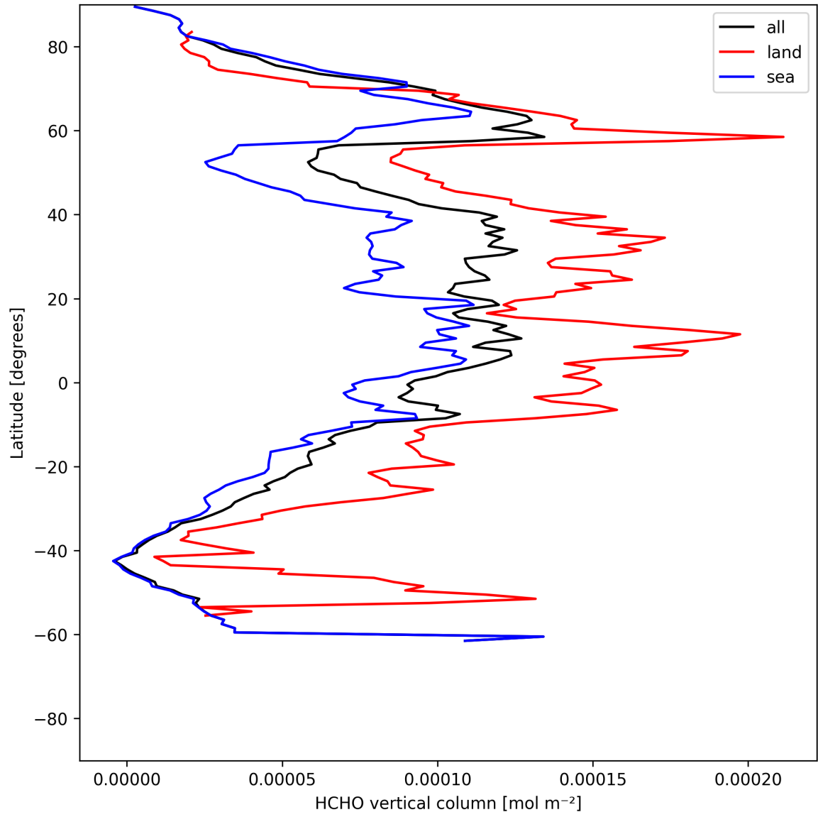
Figure 19: Zonal average of “HCHO vertical column” for 2025-06-14 to 2025-06-14.
