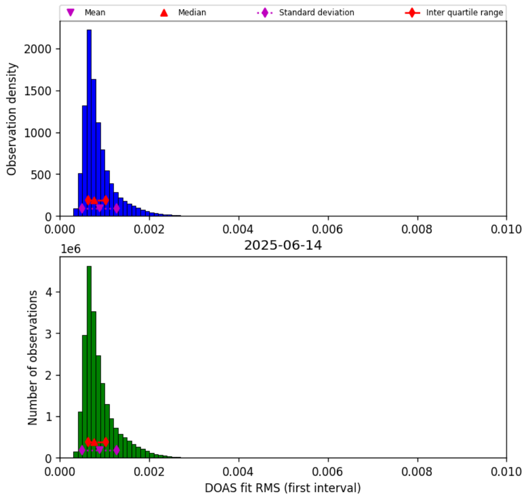
Figure 44: Histogram of “DOAS fit RMS (first interval)” for 2025-06-14 to 2025-06-14
