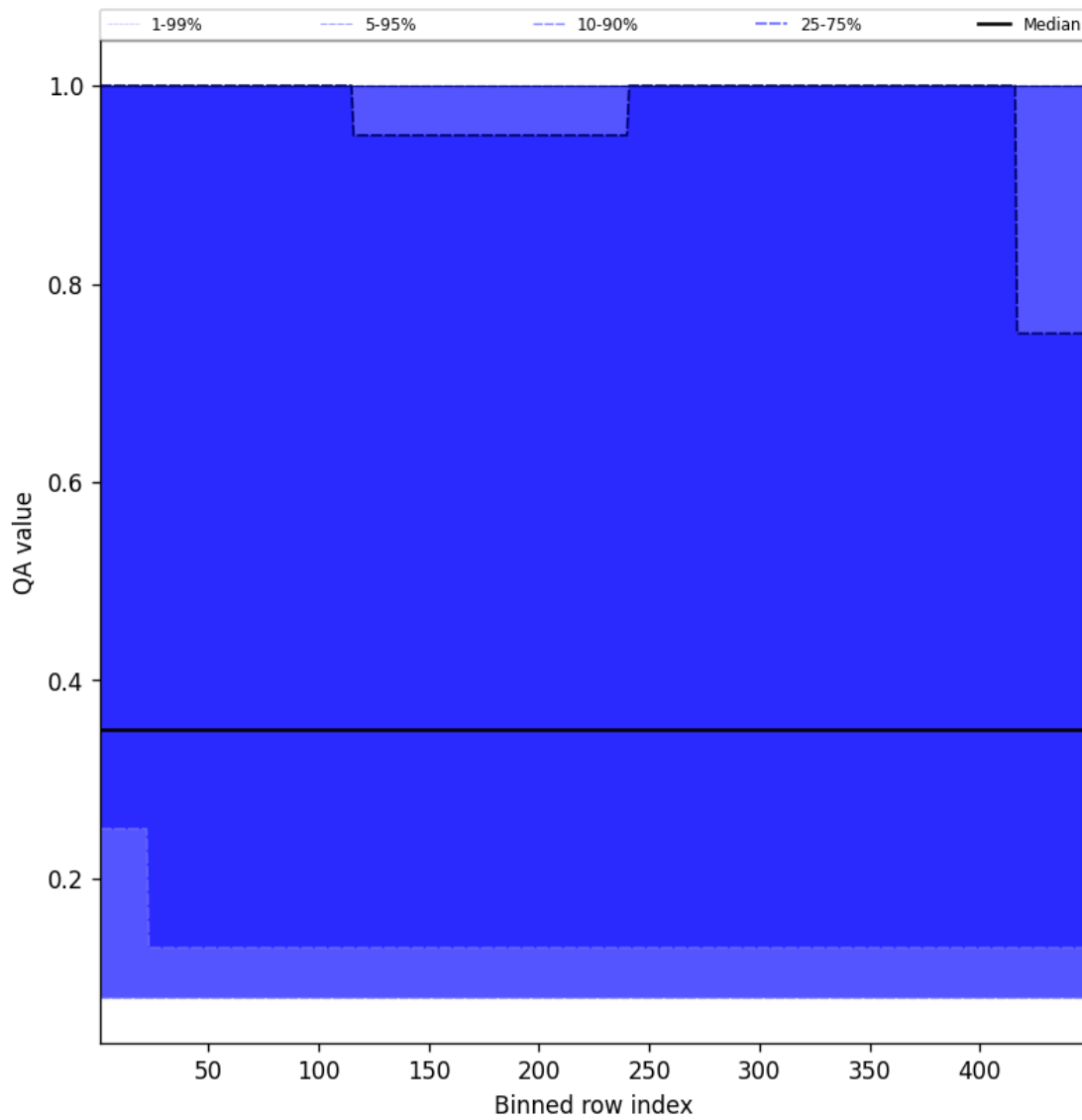
Figure 46: Along track statistics of “QA value” for 2025-06-14 to 2025-06-14
