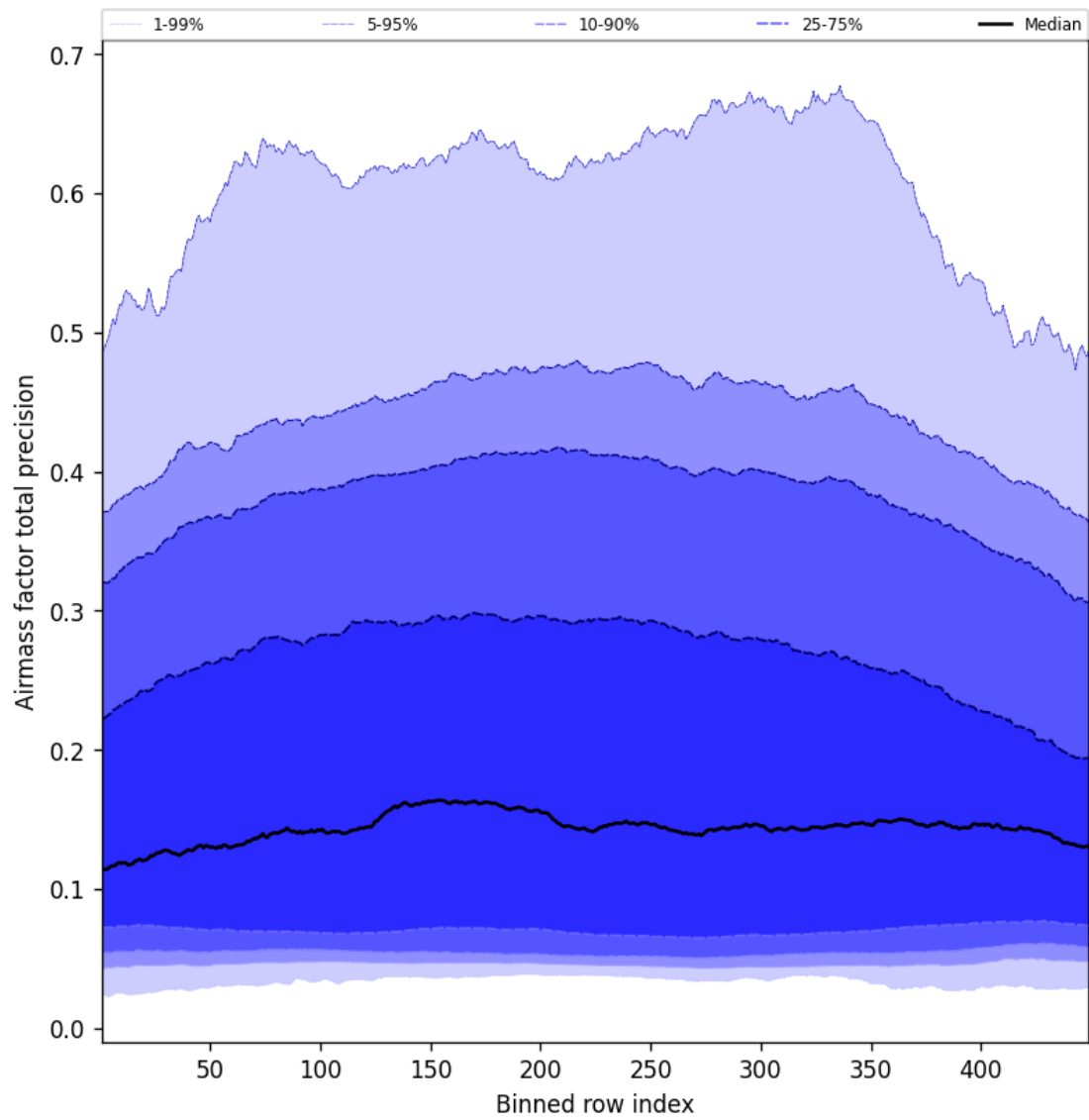
Figure 53: Along track statistics of “Airmass factor total precision” for 2025-06-14 to 2025-06-14
