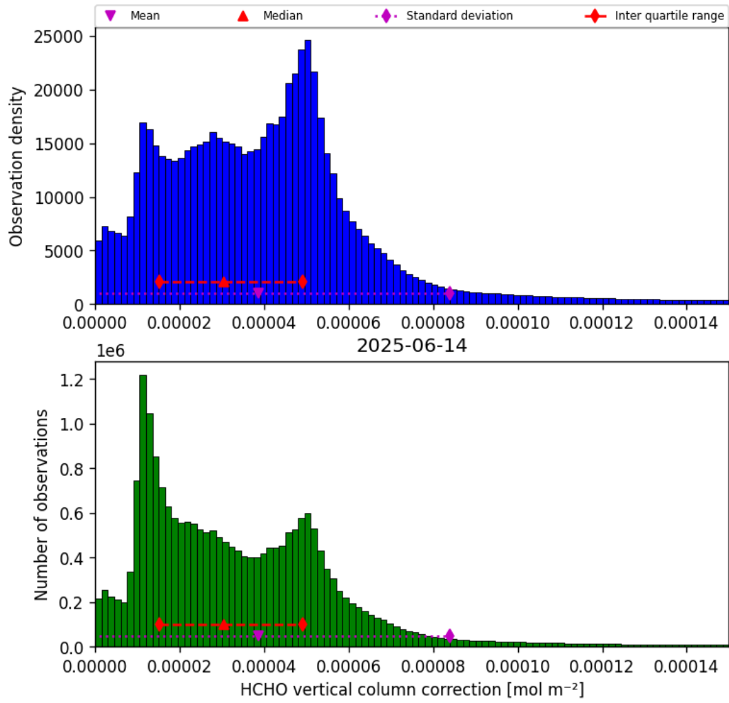
Figure 35: Histogram of “HCHO vertical column correction” for 2025-06-14 to 2025-06-14
