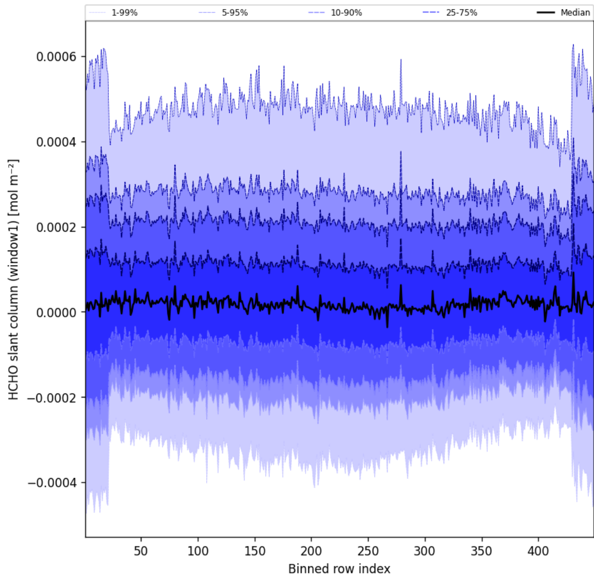
Figure 50: Along track statistics of “HCHO slant column (window1)” for 2025-06-15 to 2025-06-16
