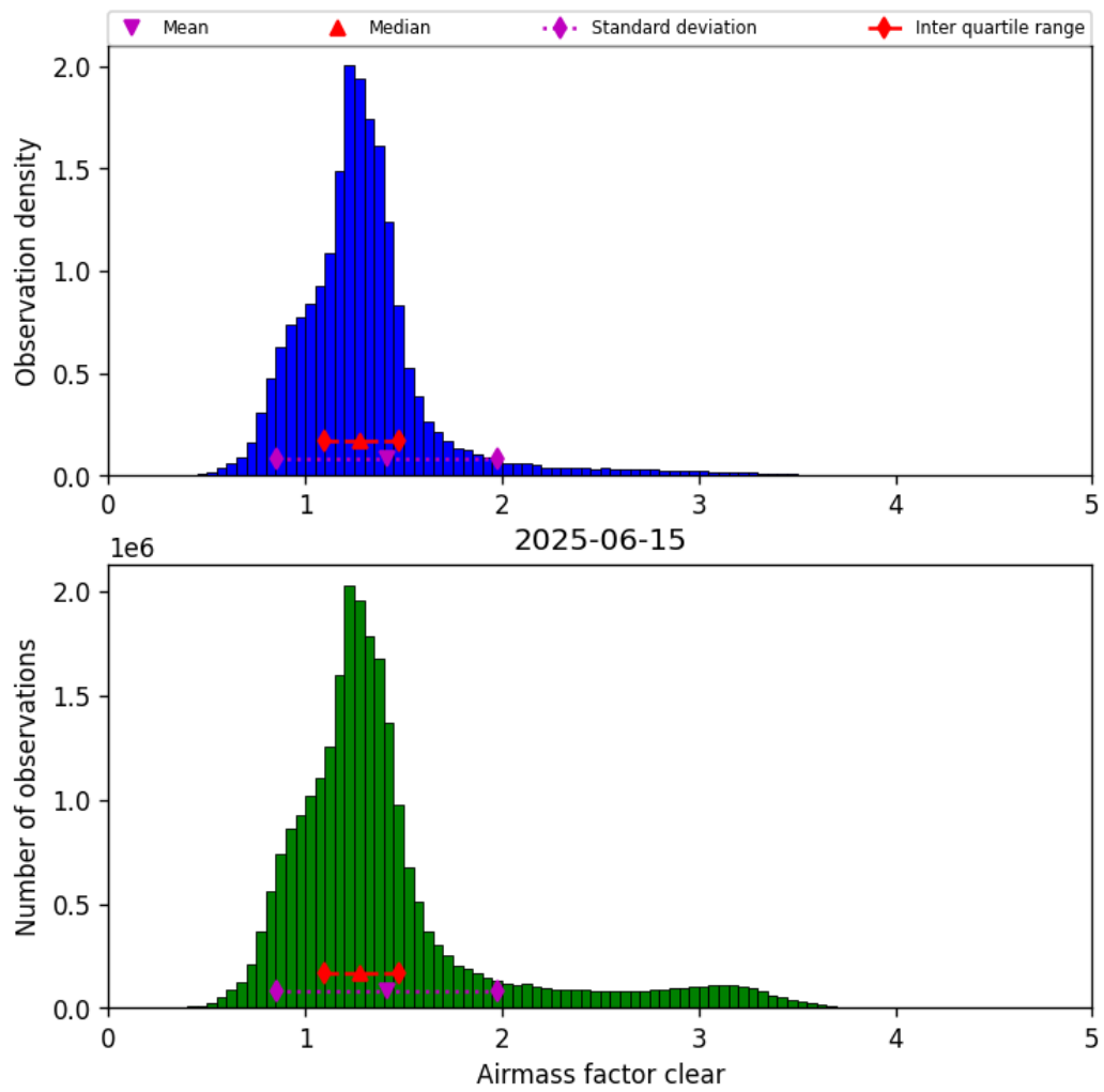
Figure 40: Histogram of “Airmass factor clear” for 2025-06-15 to 2025-06-16
