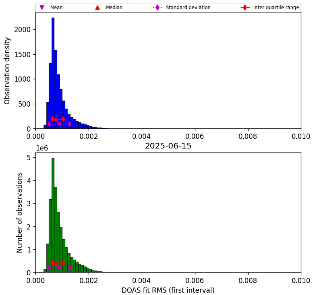
Figure 44: Histogram of “DOAS fit RMS (first interval)” for 2025-06-15 to 2025-06-16
