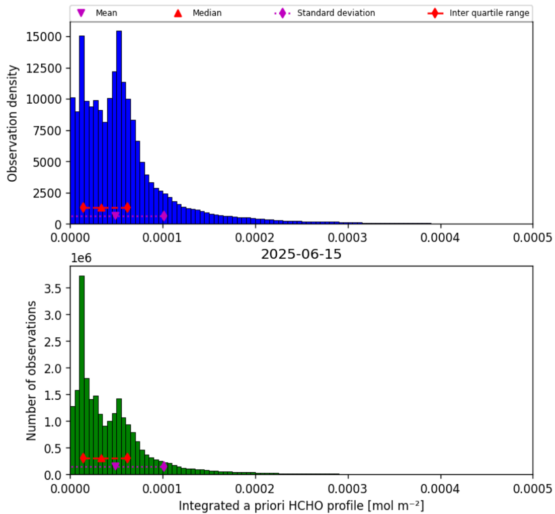
Figure 41: Histogram of “Integrated a priori HCHO profile” for 2025-06-15 to 2025-06-16
