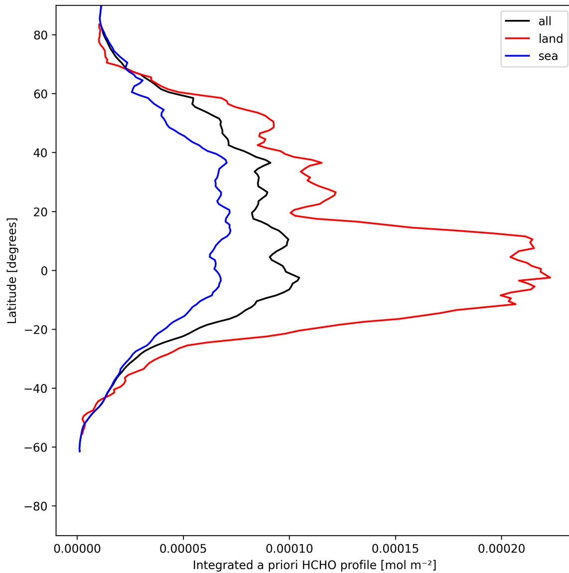
Figure 27: Zonal average of “Integrated a priori HCHO profile” for 2025-06-15 to 2025-06-16.
