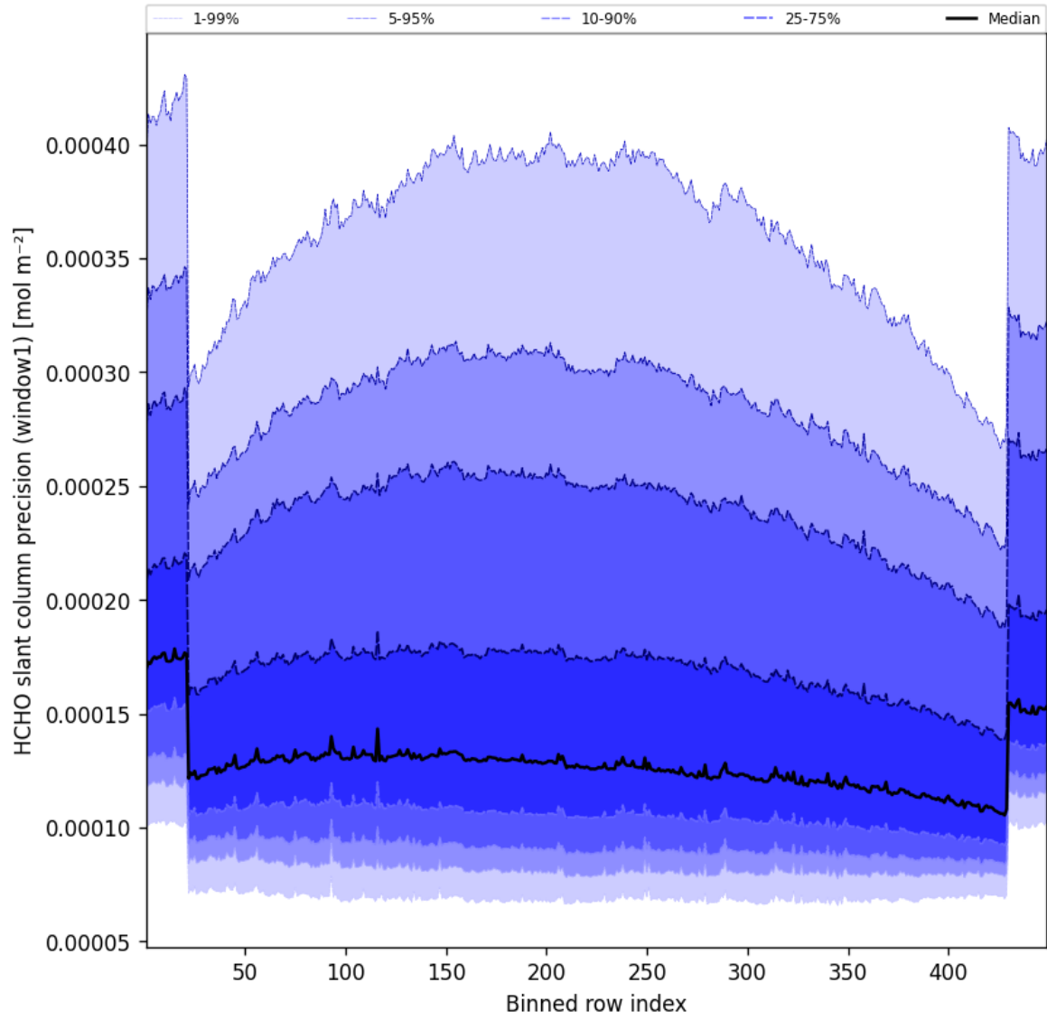
Figure 51: Along track statistics of “HCHO slant column precision (window1)” for 2025-06-15 to 2025-06-16
