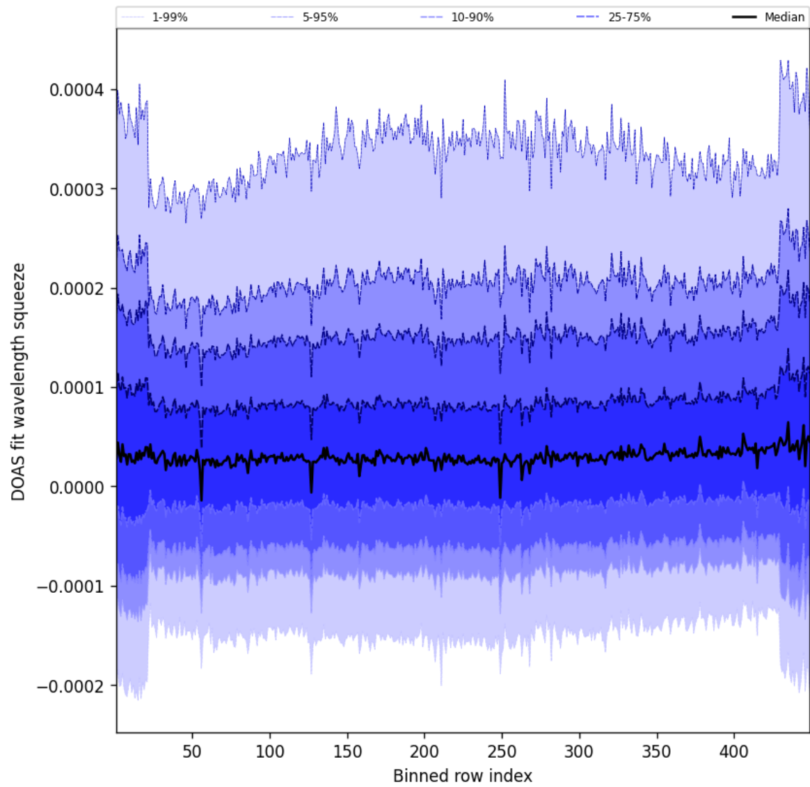
Figure 57: Along track statistics of “DOAS fit wavelength squeeze” for 2025-06-15 to 2025-06-16
