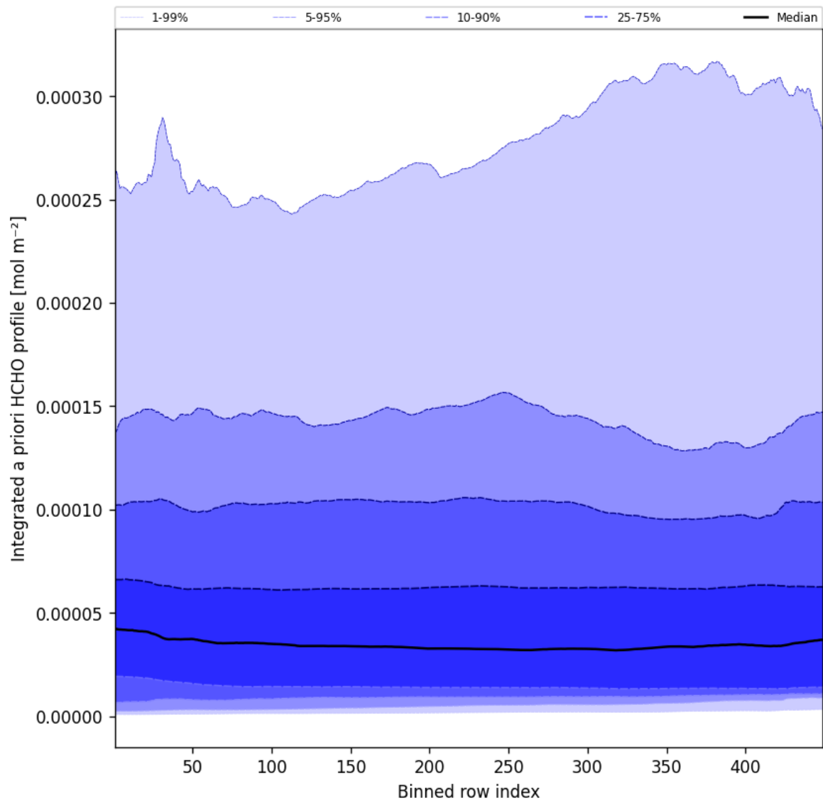
Figure 55: Along track statistics of “Integrated a priori HCHO profile” for 2025-06-15 to 2025-06-16
