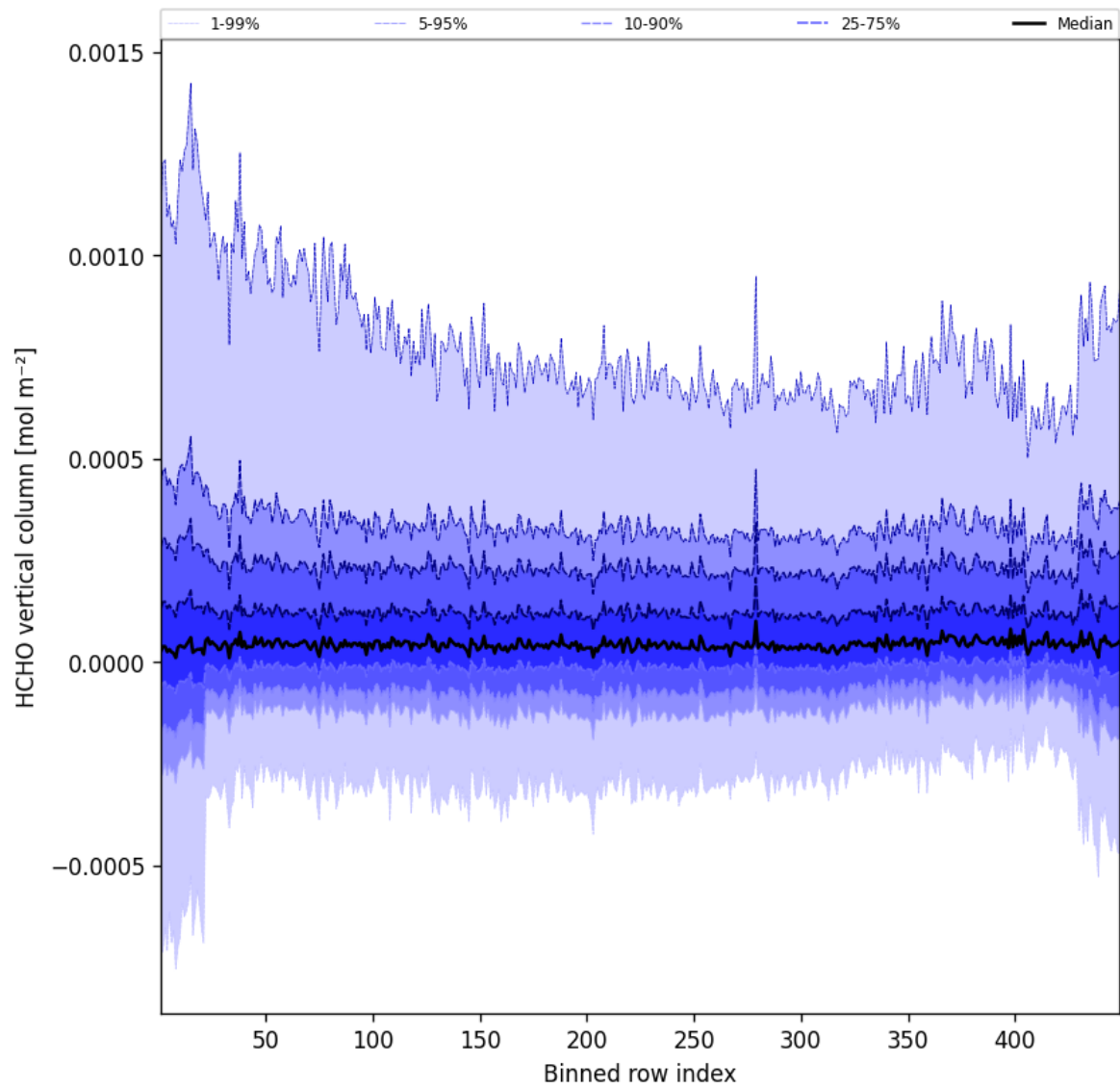
Figure 47: Along track statistics of “HCHO vertical column” for 2025-06-15 to 2025-06-16
