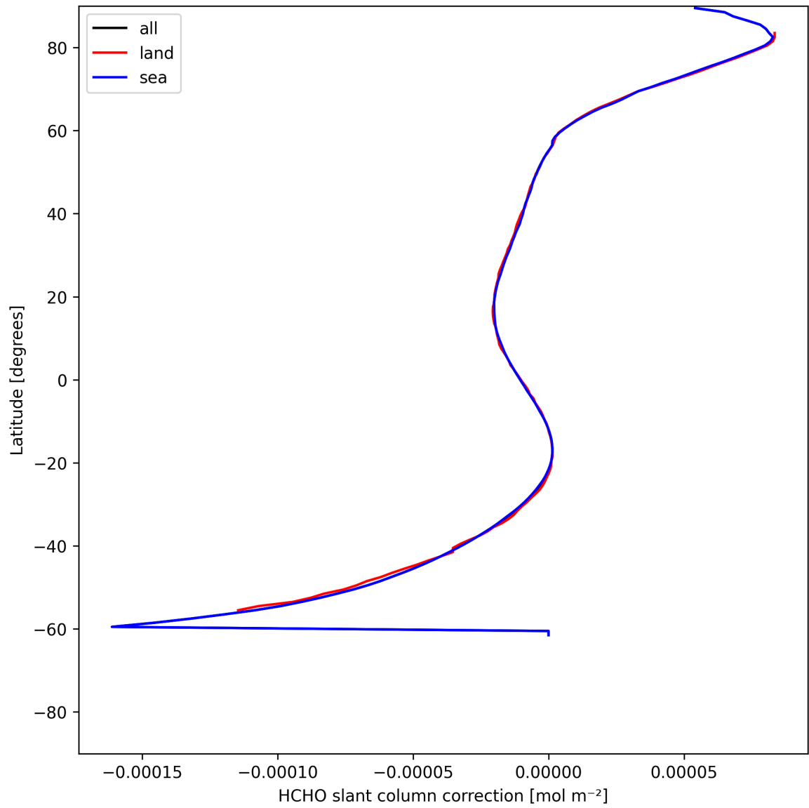
Figure 31: Zonal average of “HCHO slant column correction” for 2025-06-15 to 2025-06-16.
