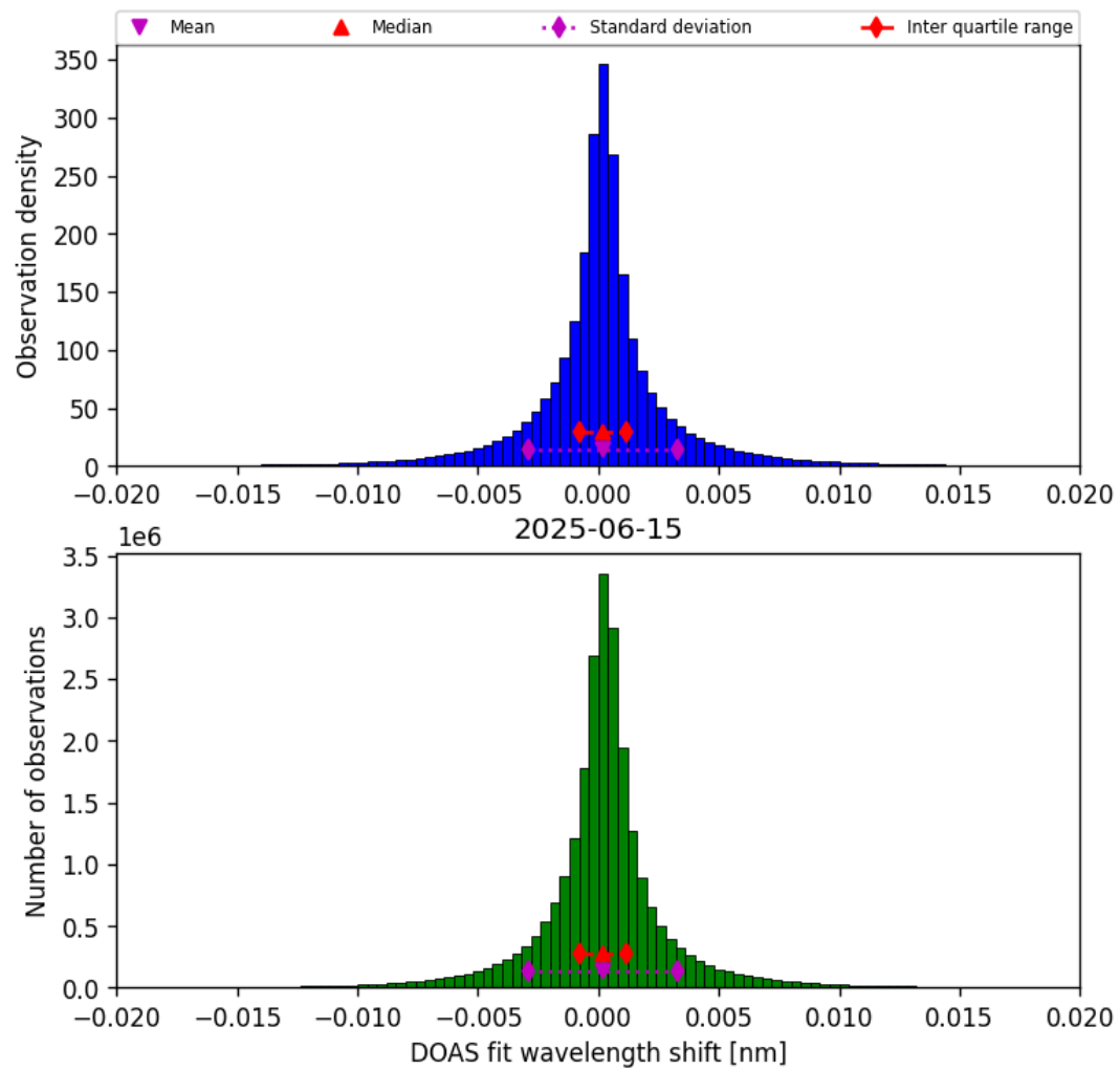
Figure 42: Histogram of “DOAS fit wavelength shift” for 2025-06-15 to 2025-06-16
