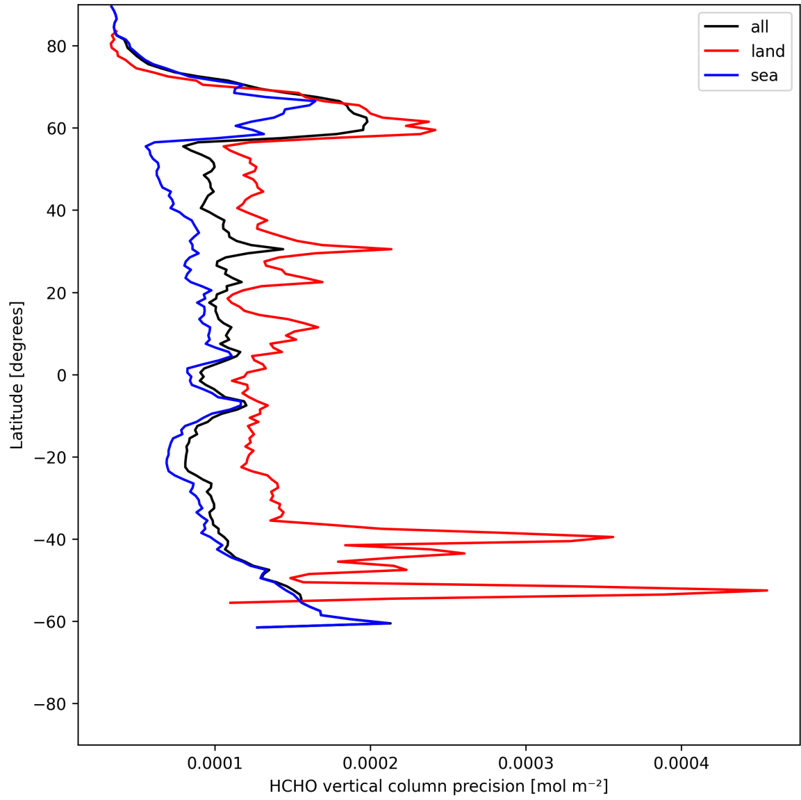
Figure 20: Zonal average of “HCHO vertical column precision” for 2025-06-15 to 2025-06-16.
