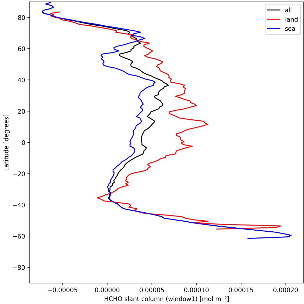
Figure 22: Zonal average of “HCHO slant column (window1)” for 2025-06-15 to 2025-06-16.
