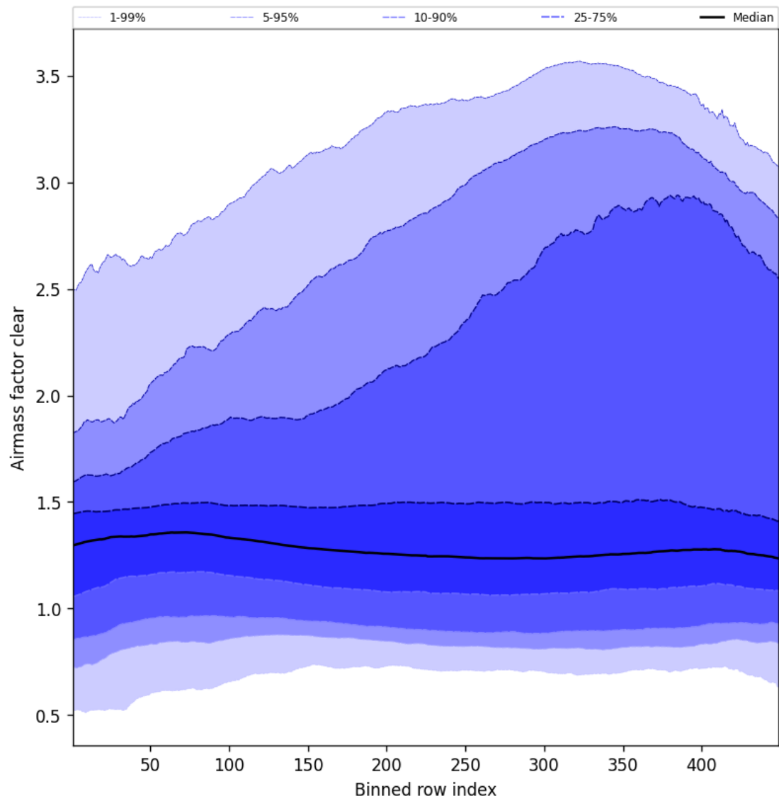
Figure 54: Along track statistics of “Airmass factor clear” for 2025-06-15 to 2025-06-16
