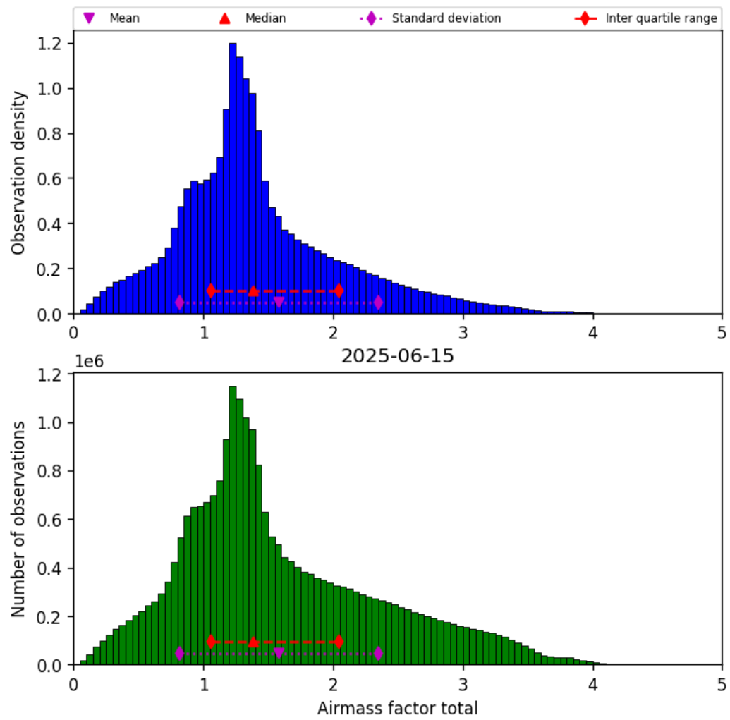
Figure 38: Histogram of “Airmass factor total” for 2025-06-15 to 2025-06-16
