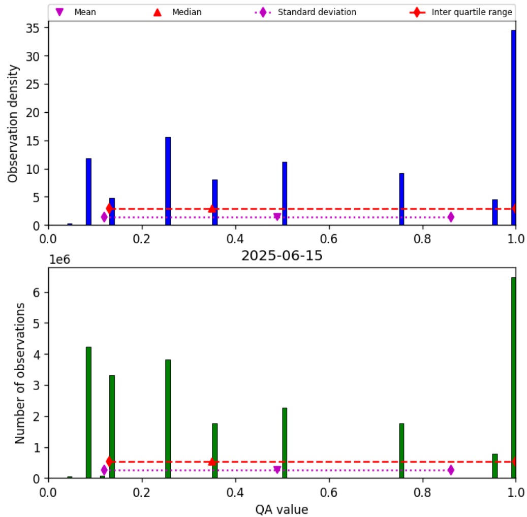
Figure 32: Histogram of “QA value” for 2025-06-15 to 2025-06-16
