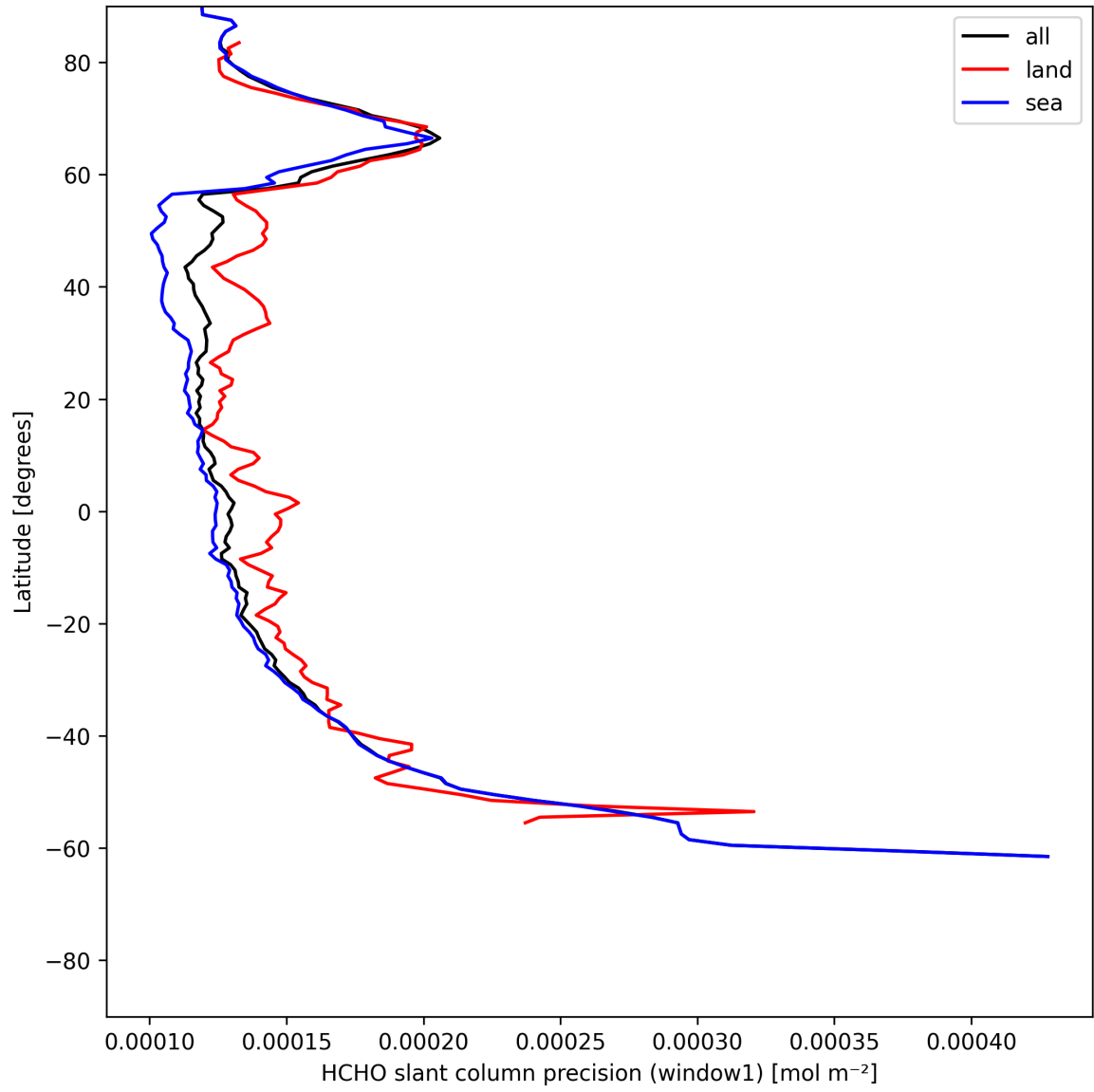
Figure 23: Zonal average of “HCHO slant column precision (window1)” for 2025-06-15 to 2025-06-16.
