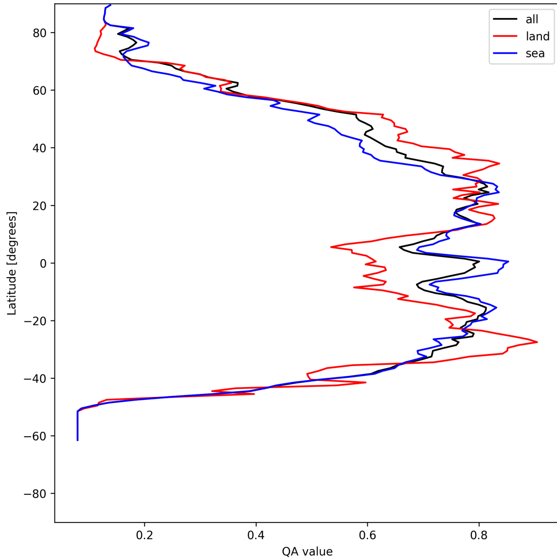
Figure 18: Zonal average of “QA value” for 2025-06-15 to 2025-06-16.
