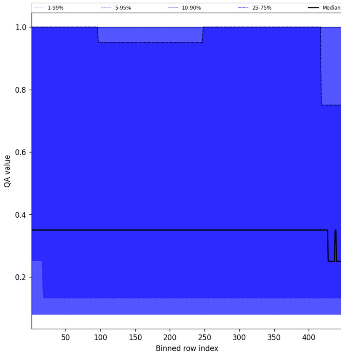
Figure 46: Along track statistics of “QA value” for 2025-06-15 to 2025-06-16
