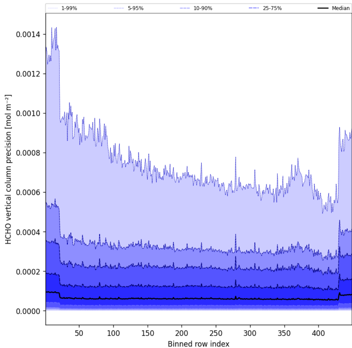
Figure 48: Along track statistics of “HCHO vertical column precision” for 2025-06-15 to 2025-06-16
