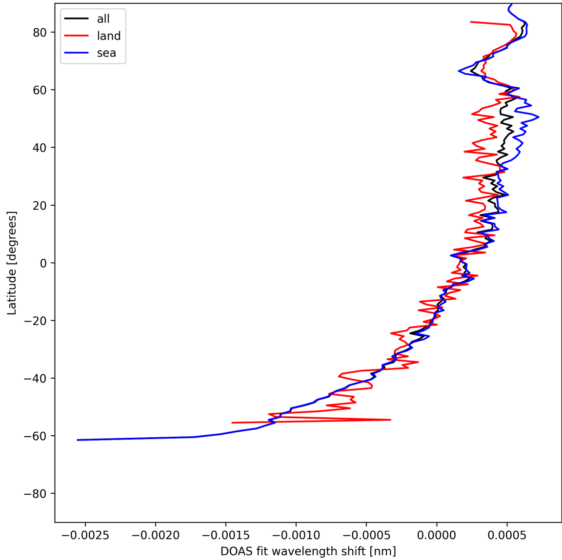
Figure 28: Zonal average of “DOAS fit wavelength shift” for 2025-06-15 to 2025-06-16.
