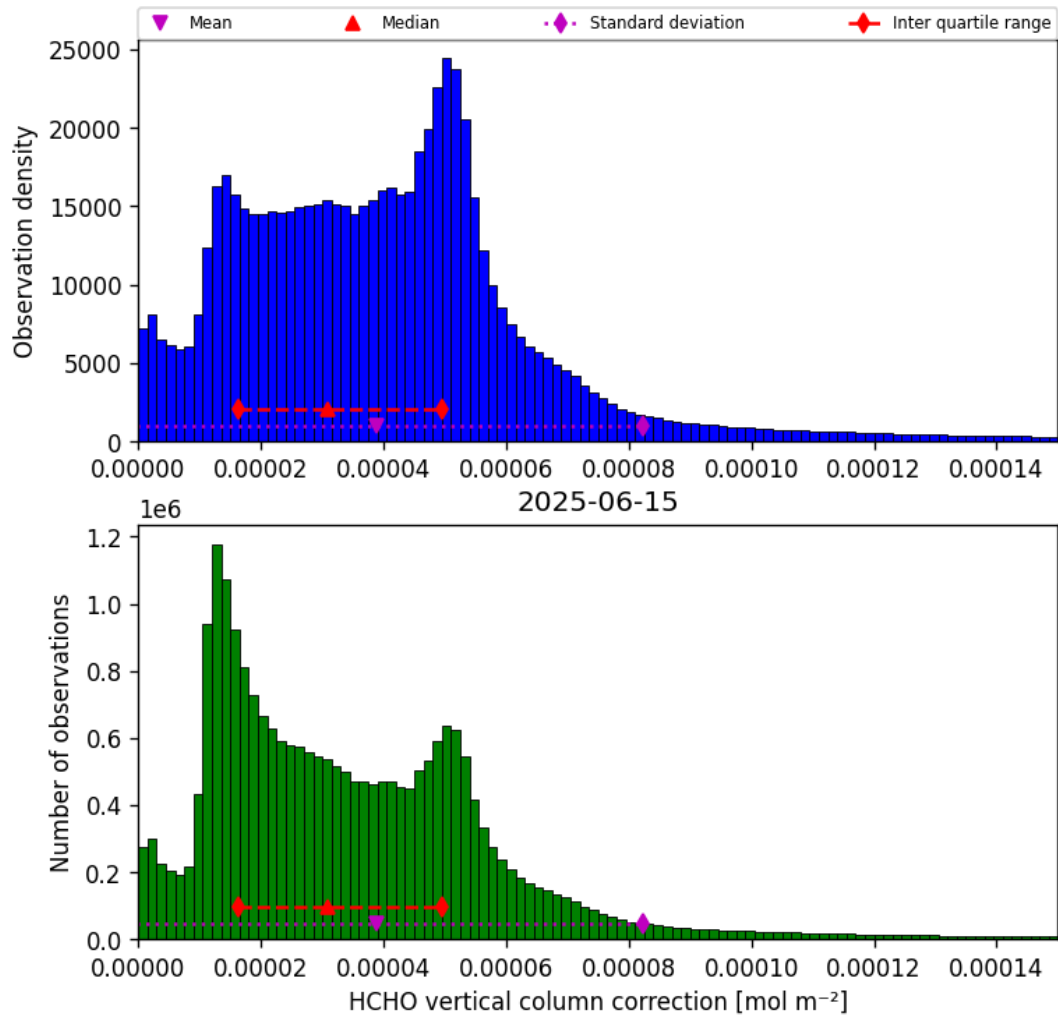
Figure 35: Histogram of “HCHO vertical column correction” for 2025-06-15 to 2025-06-16
