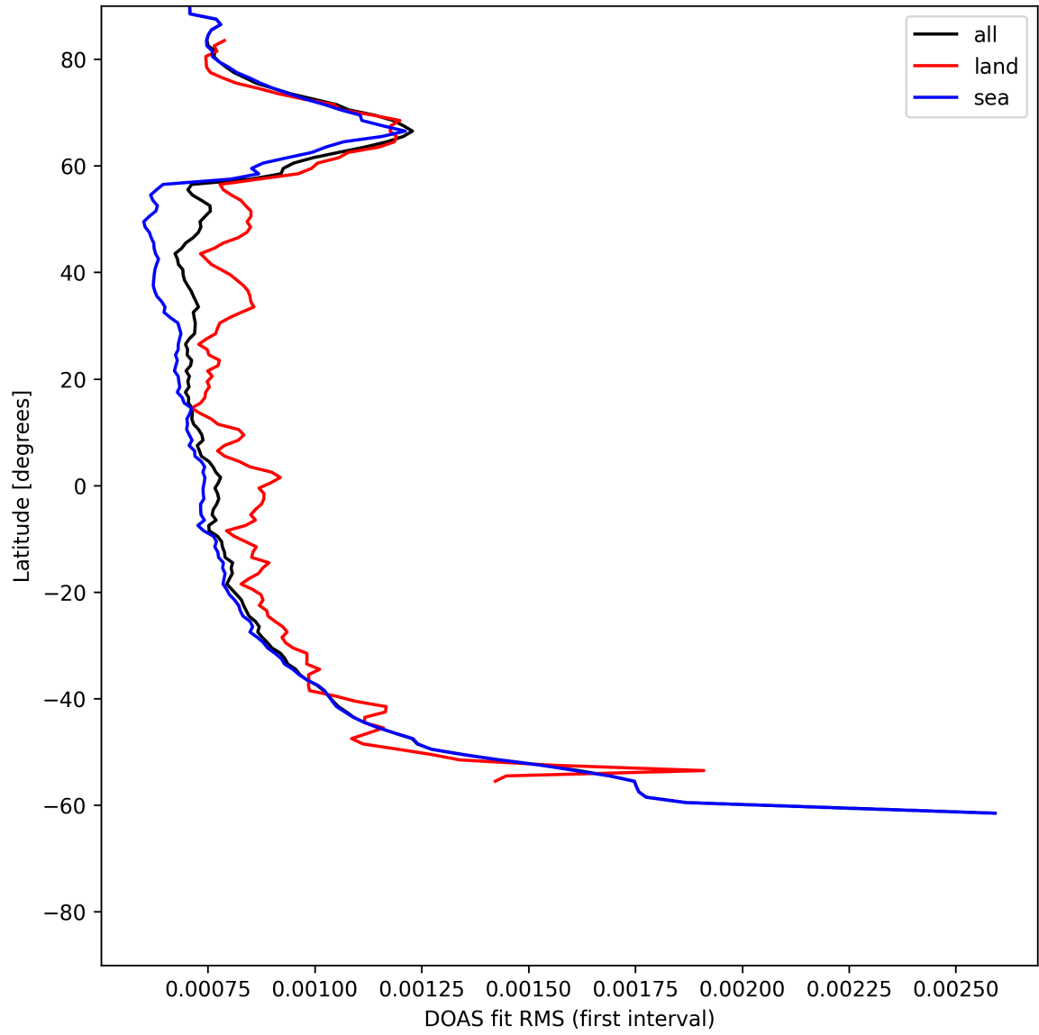
Figure 30: Zonal average of "DOAS fit RMS (first interval)" for 2025-06-15 to 2025-06-16.
