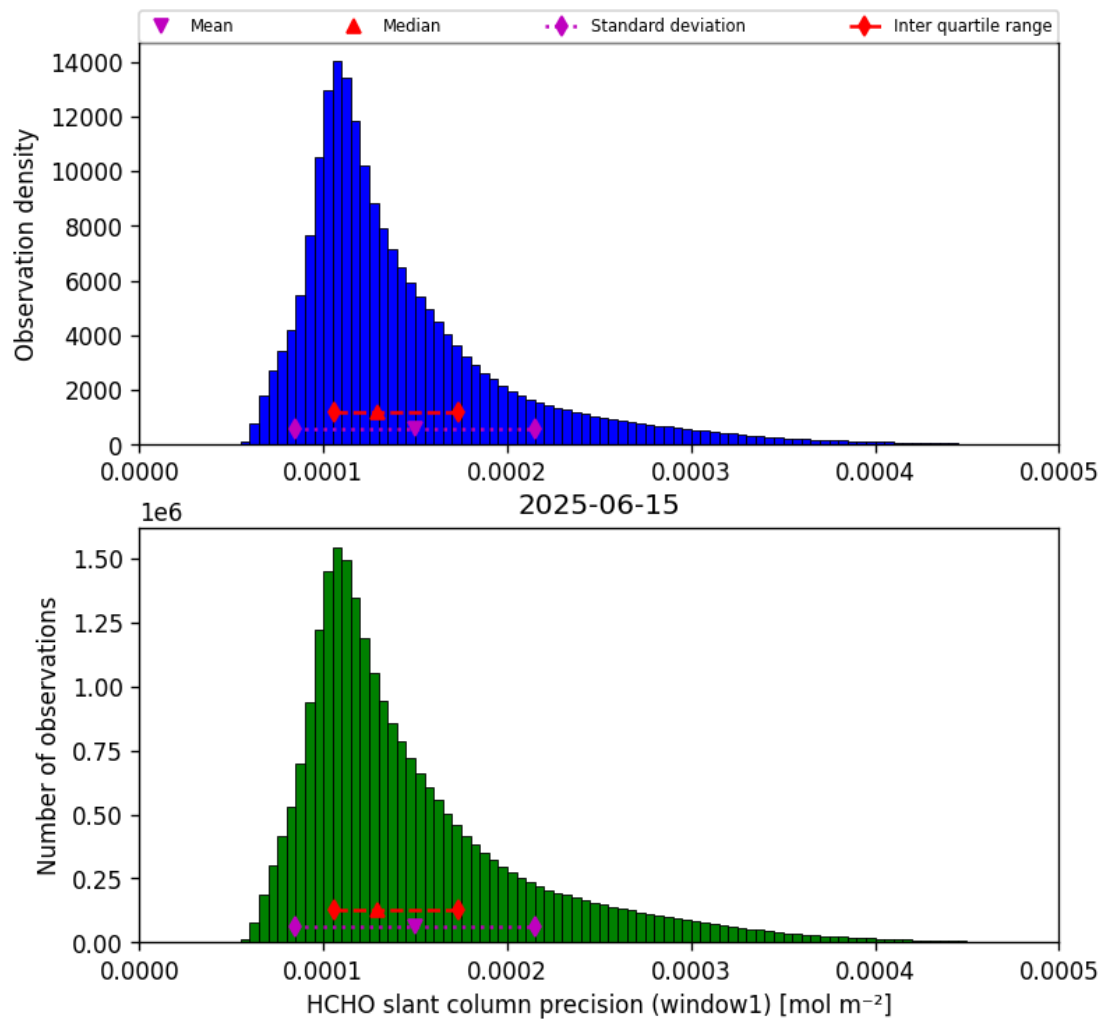
Figure 37: Histogram of “HCHO slant column precision (window1)” for 2025-06-15 to 2025-06-16
