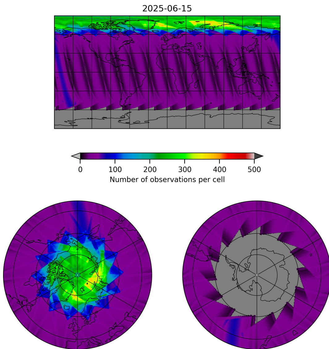
Figure 17: Map of the number of observations for 2025-06-15 to 2025-06-16
