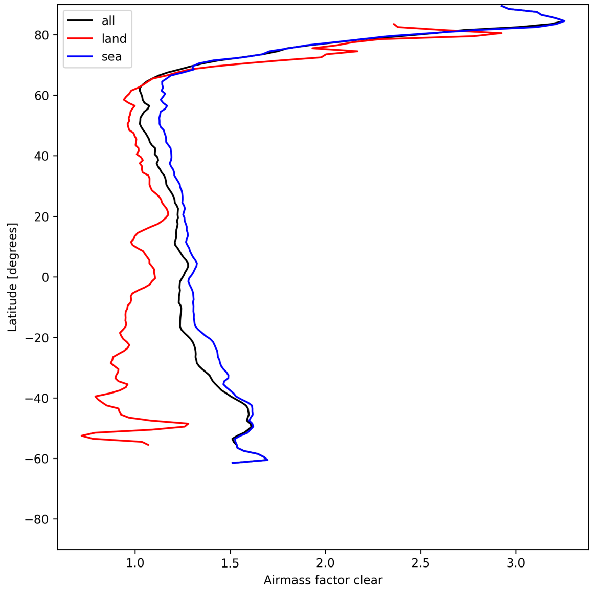
Figure 26: Zonal average of “Airmass factor clear” for 2025-06-15 to 2025-06-16.
