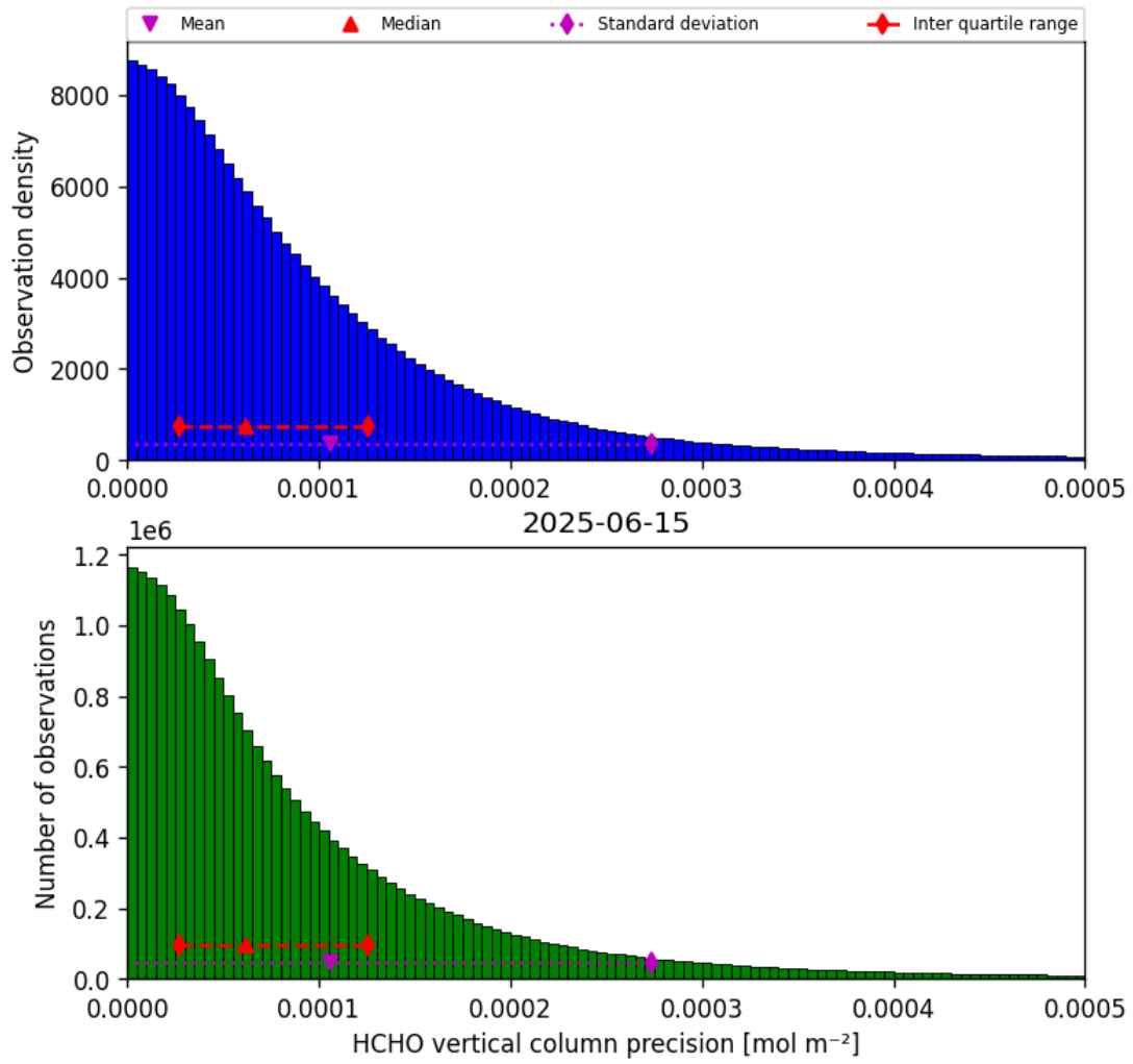
Figure 34: Histogram of “HCHO vertical column precision” for 2025-06-15 to 2025-06-16
