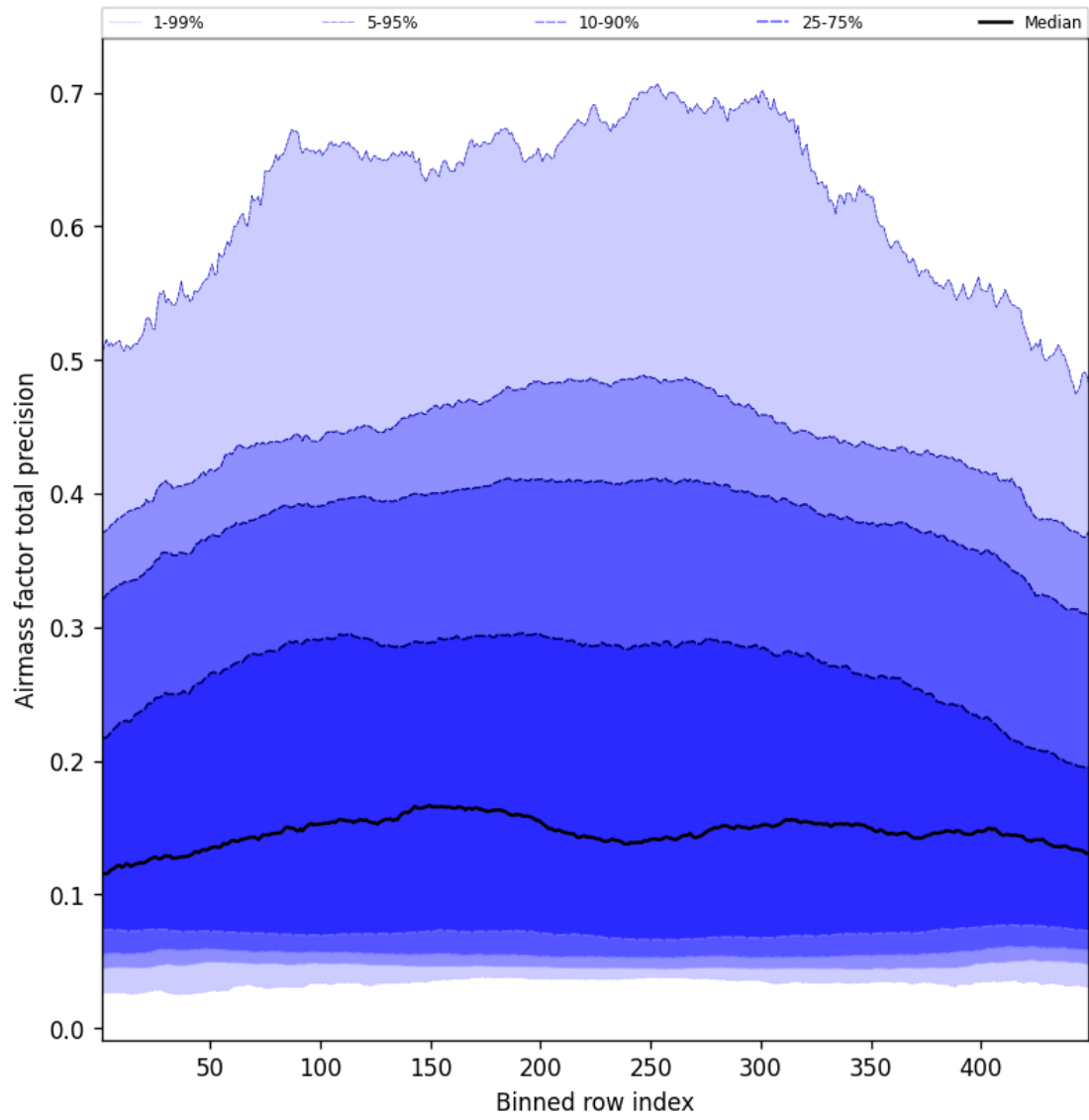
Figure 53: Along track statistics of “Airmass factor total precision” for 2025-06-15 to 2025-06-16
