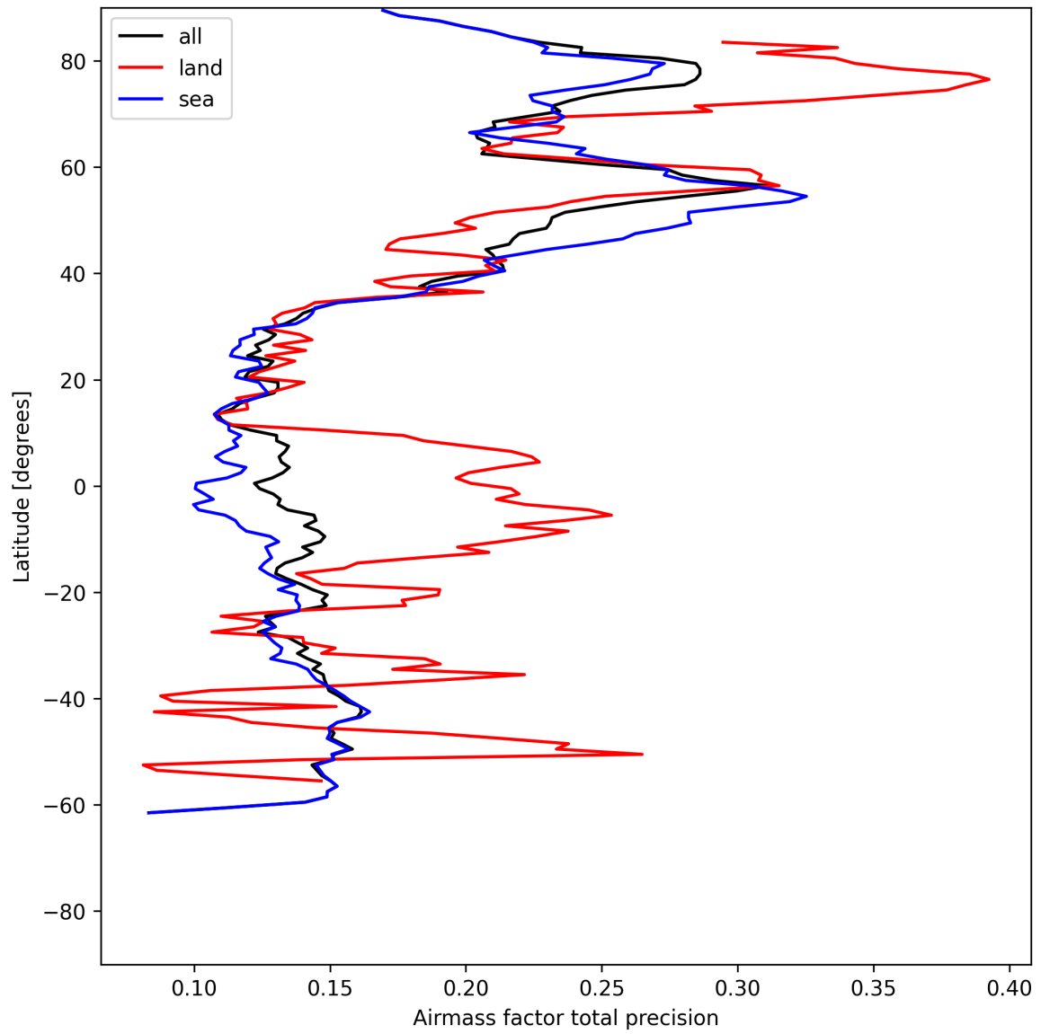
Figure 25: Zonal average of “Airmass factor total precision” for 2025-06-15 to 2025-06-16.
