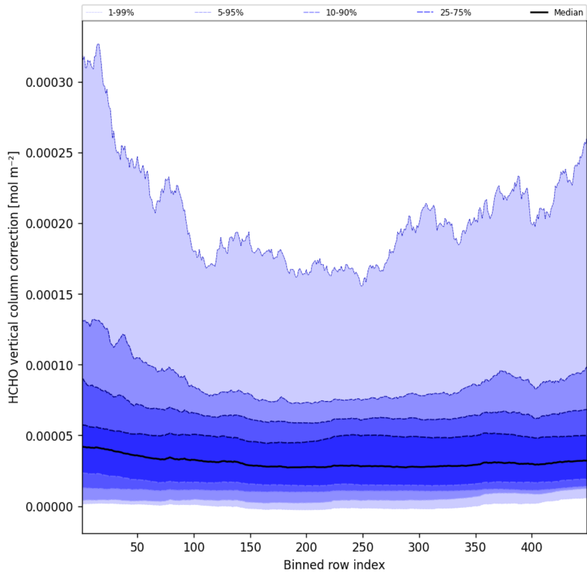
Figure 49: Along track statistics of “HCHO vertical column correction” for 2025-06-15 to 2025-06-16
