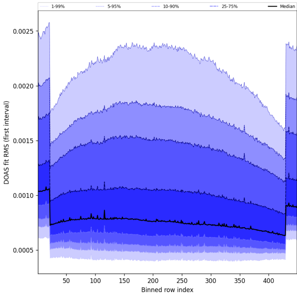
Figure 58: Along track statistics of “DOAS fit RMS (first interval)” for 2025-06-15 to 2025-06-16
