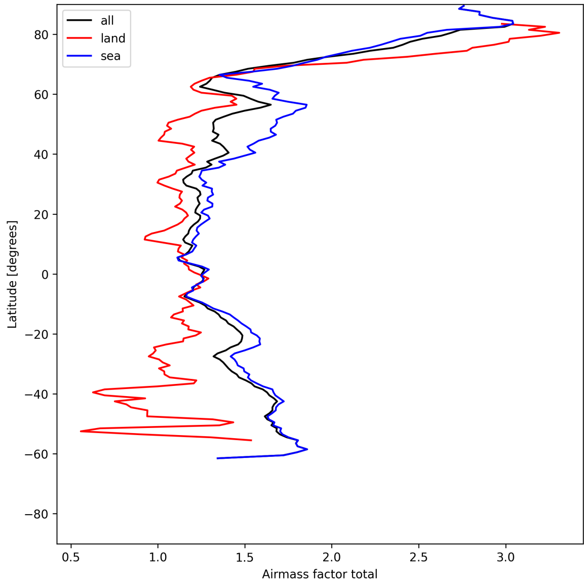
Figure 24: Zonal average of “Airmass factor total” for 2025-06-15 to 2025-06-16.
