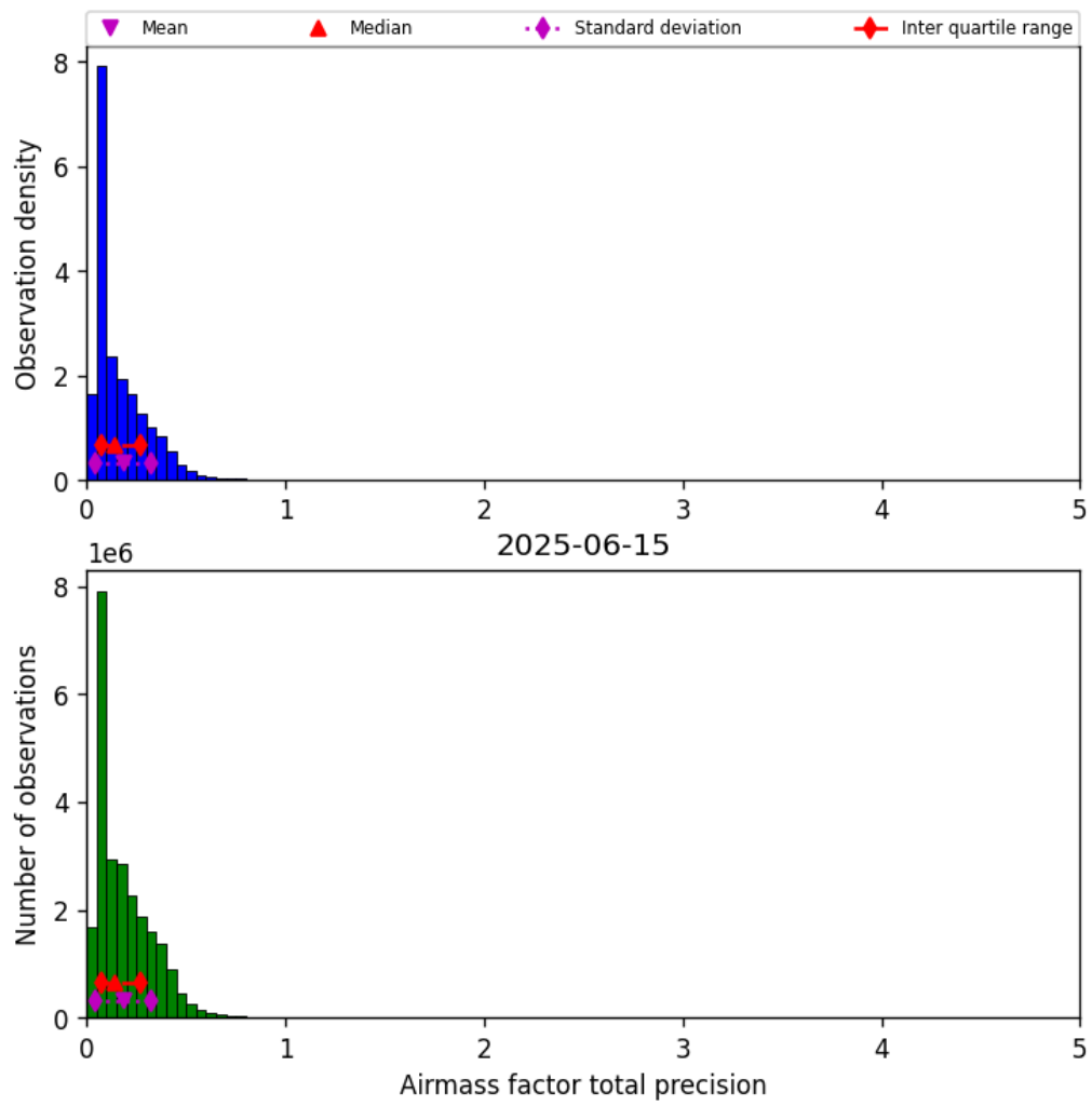
Figure 39: Histogram of “Airmass factor total precision” for 2025-06-15 to 2025-06-16
