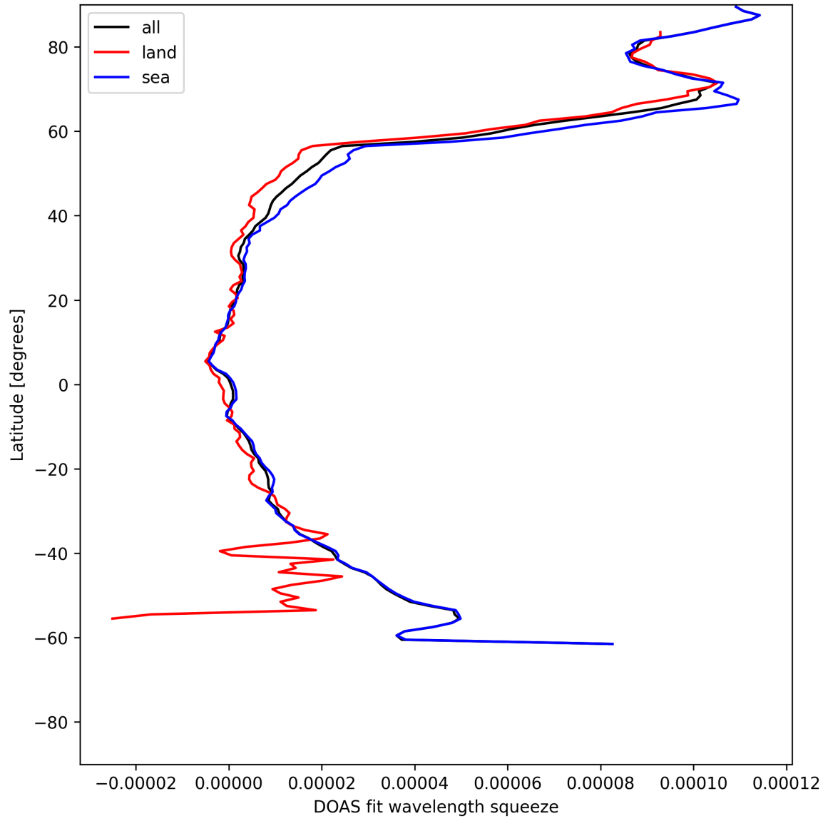
Figure 29: Zonal average of “DOAS fit wavelength squeeze” for 2025-06-15 to 2025-06-16.
