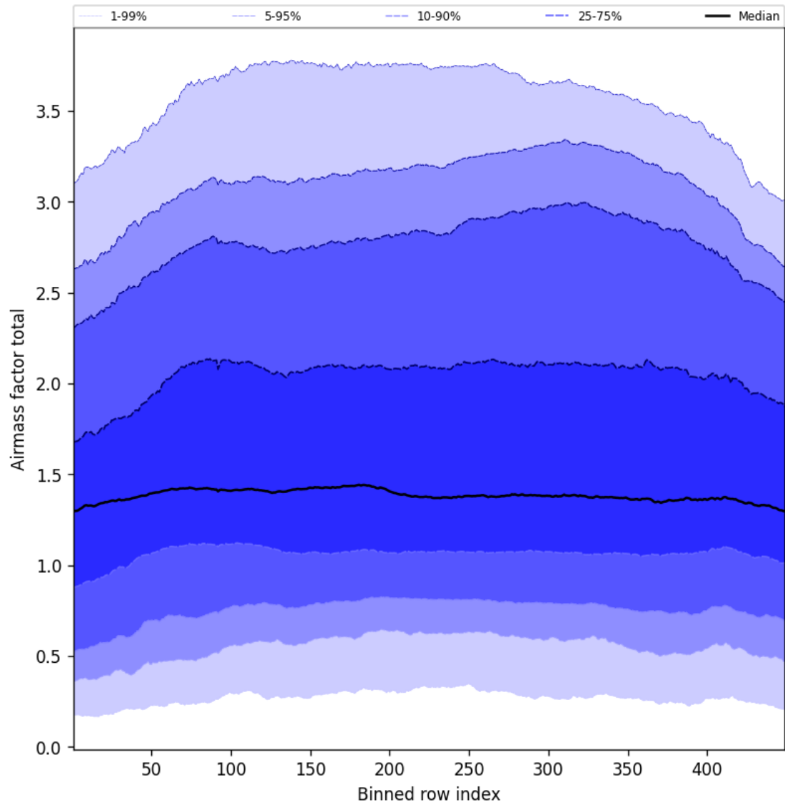
Figure 52: Along track statistics of “Airmass factor total” for 2025-06-15 to 2025-06-16
