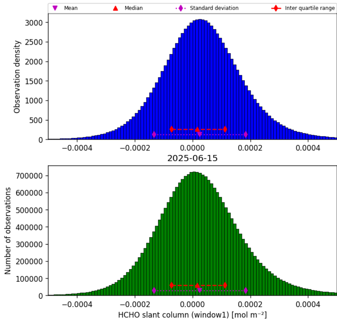
Figure 36: Histogram of “HCHO slant column (window1)” for 2025-06-15 to 2025-06-16
