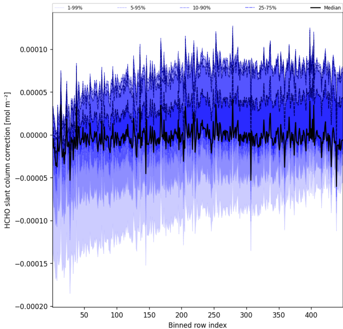
Figure 59: Along track statistics of “HCHO slant column correction” for 2025-06-15 to 2025-06-16
