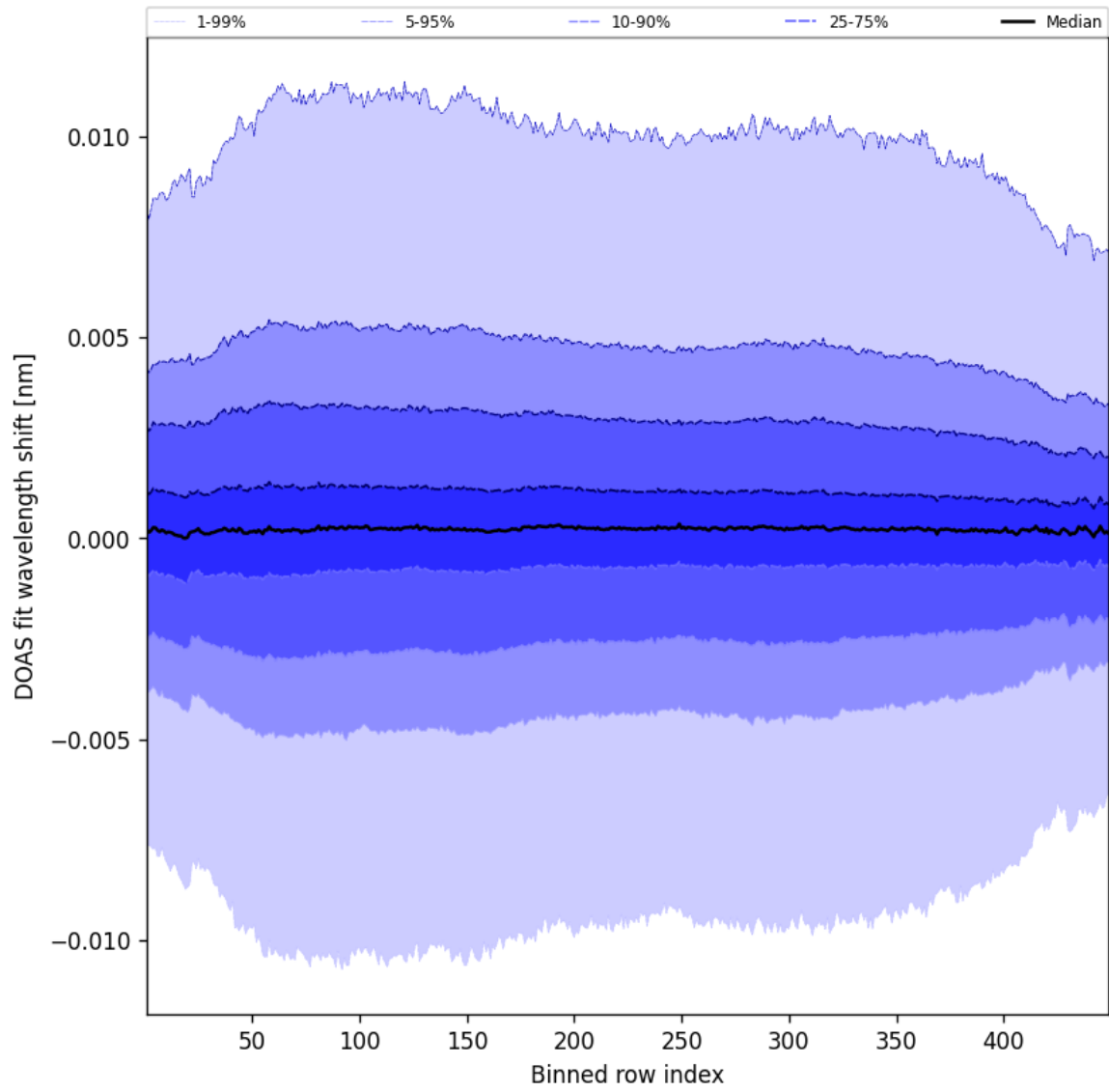
Figure 56: Along track statistics of “DOAS fit wavelength shift” for 2025-06-15 to 2025-06-16
