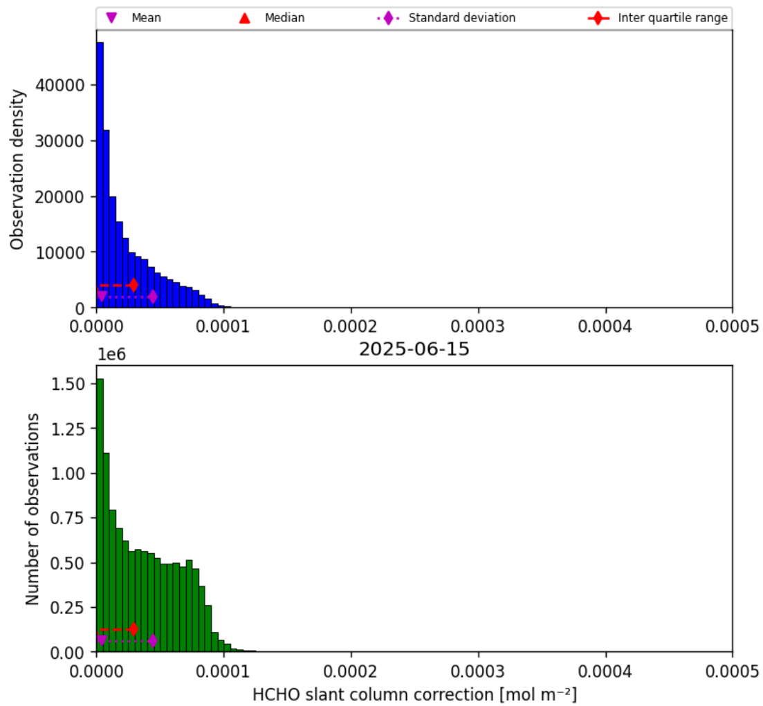
Figure 45: Histogram of “HCHO slant column correction” for 2025-06-15 to 2025-06-16
