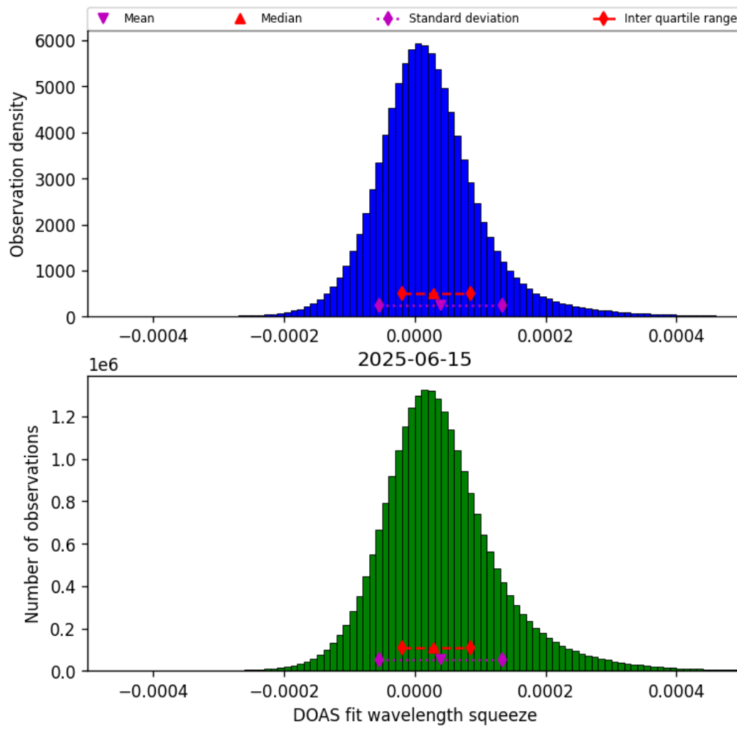
Figure 43: Histogram of “DOAS fit wavelength squeeze” for 2025-06-15 to 2025-06-16
