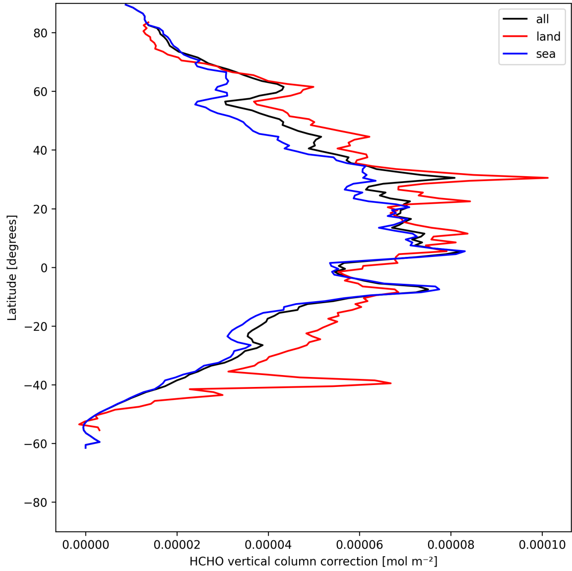
Figure 21: Zonal average of “HCHO vertical column correction” for 2025-06-15 to 2025-06-16.
