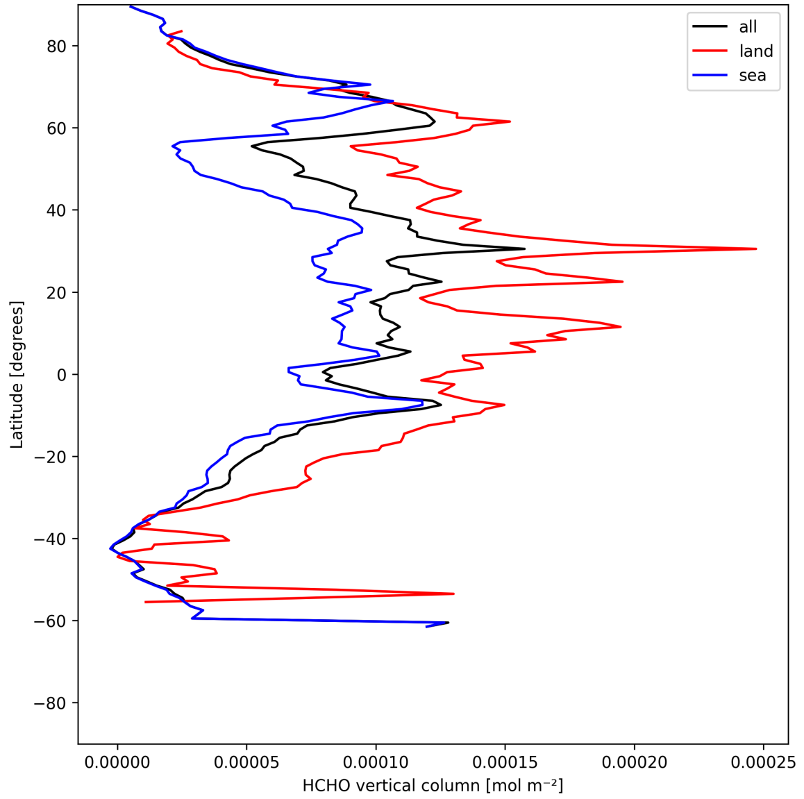
Figure 19: Zonal average of “HCHO vertical column” for 2025-06-15 to 2025-06-16.
