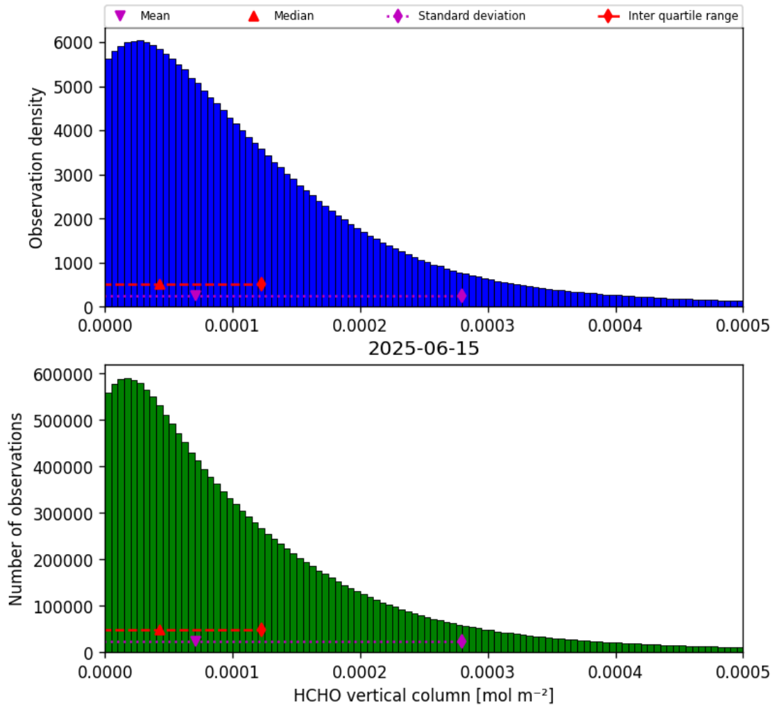
Figure 33: Histogram of “HCHO vertical column” for 2025-06-15 to 2025-06-16
