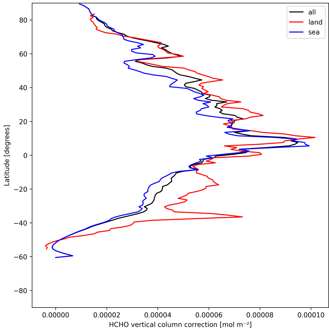
Figure 21: Zonal average of “HCHO vertical column correction” for 2025-06-16 to 2025-06-17.
