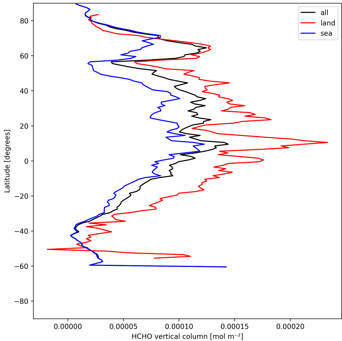
Figure 19: Zonal average of “HCHO vertical column” for 2025-06-16 to 2025-06-17.
