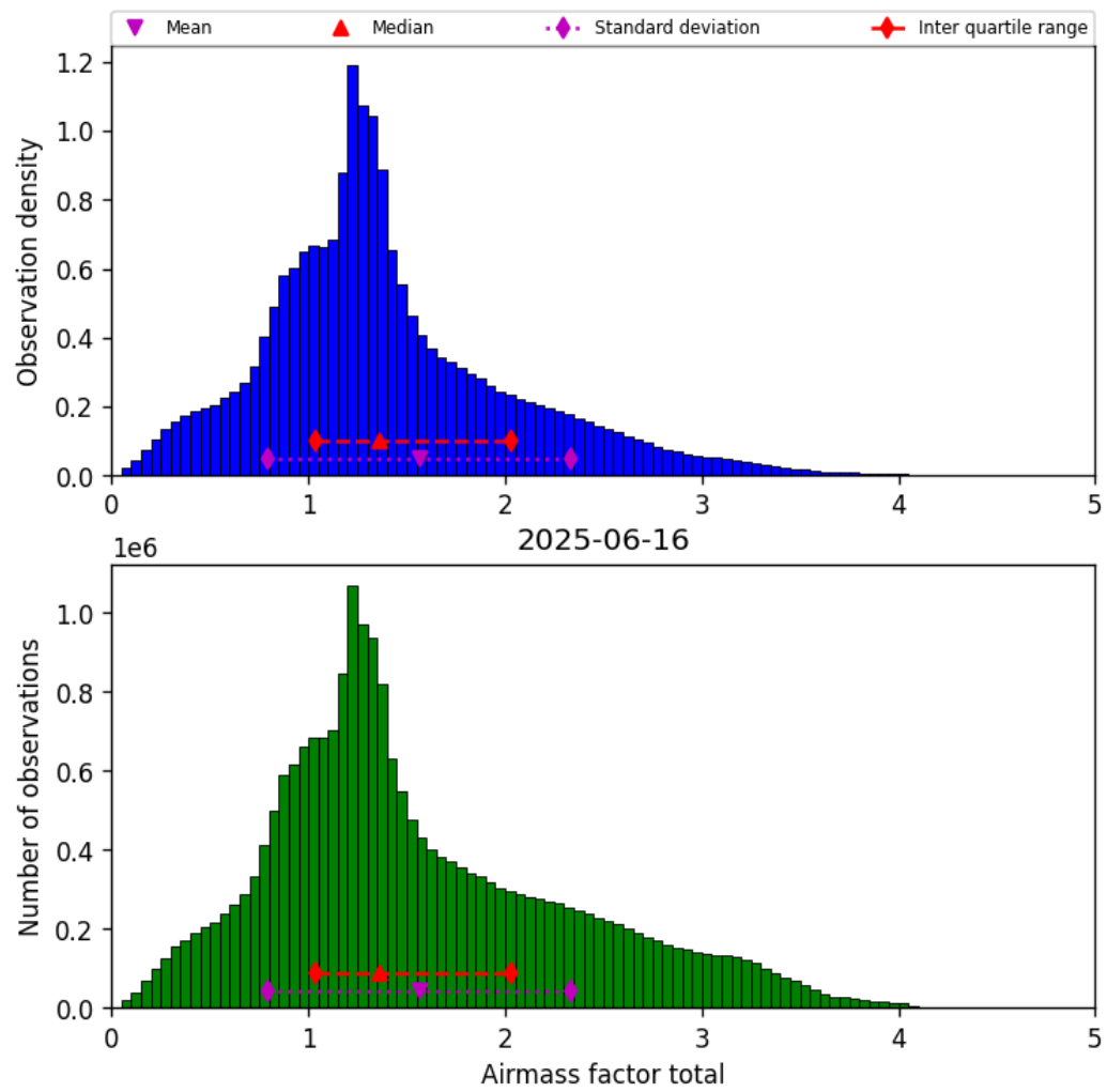
Figure 38: Histogram of “Airmass factor total” for 2025-06-16 to 2025-06-17
