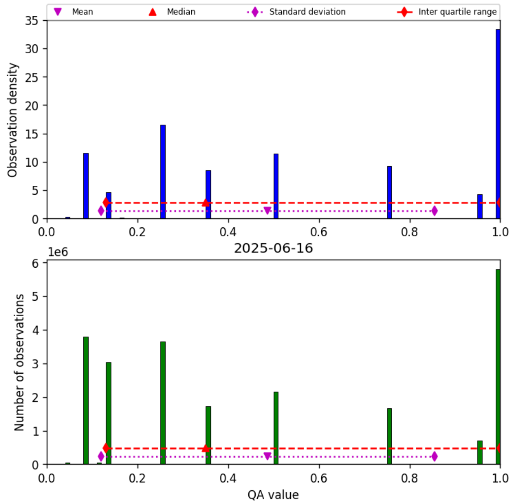
Figure 32: Histogram of “QA value” for 2025-06-16 to 2025-06-17
