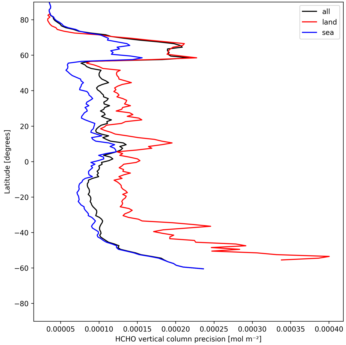
Figure 20: Zonal average of “HCHO vertical column precision” for 2025-06-16 to 2025-06-17.
