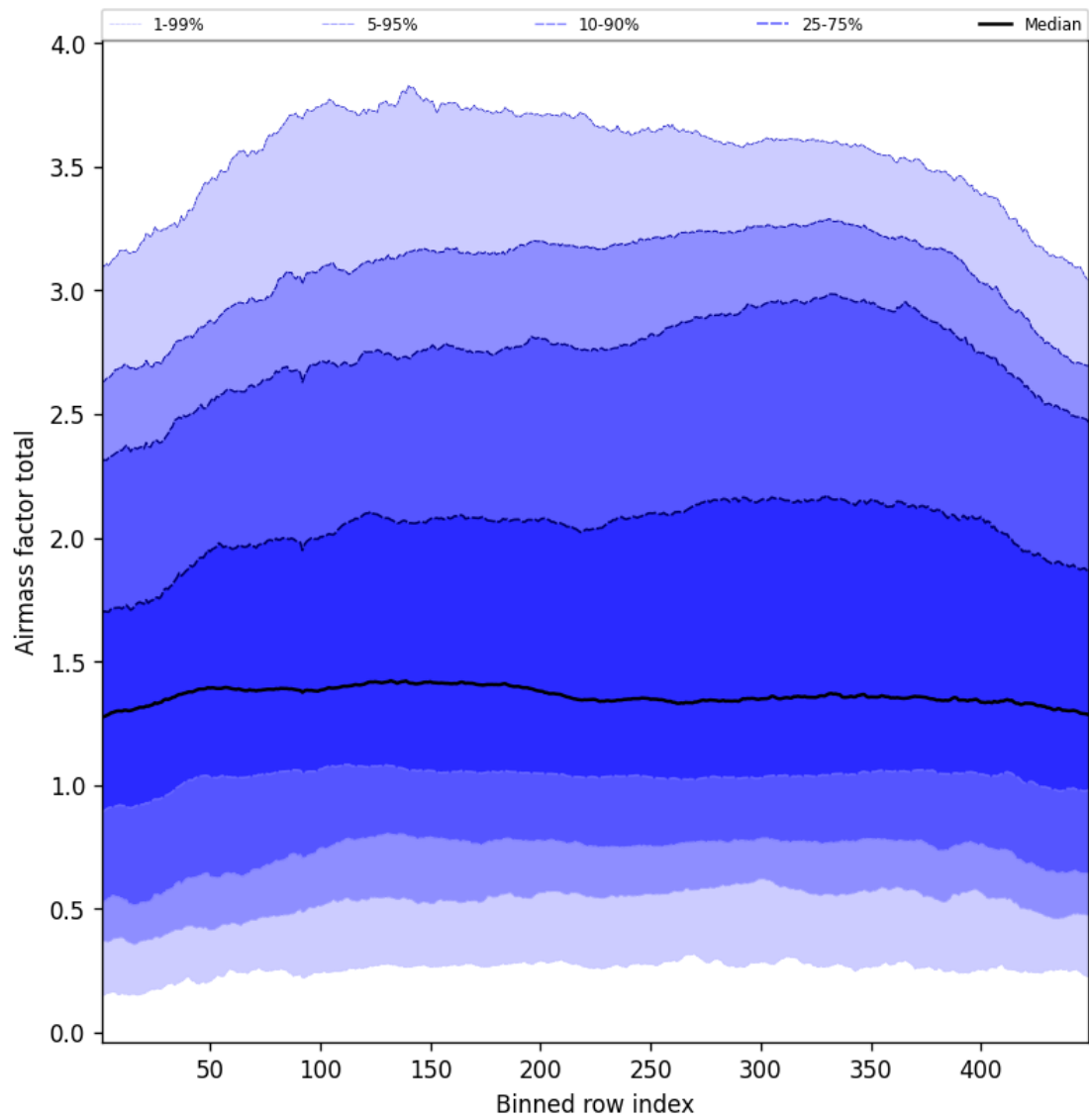
Figure 52: Along track statistics of “Airmass factor total” for 2025-06-16 to 2025-06-17
