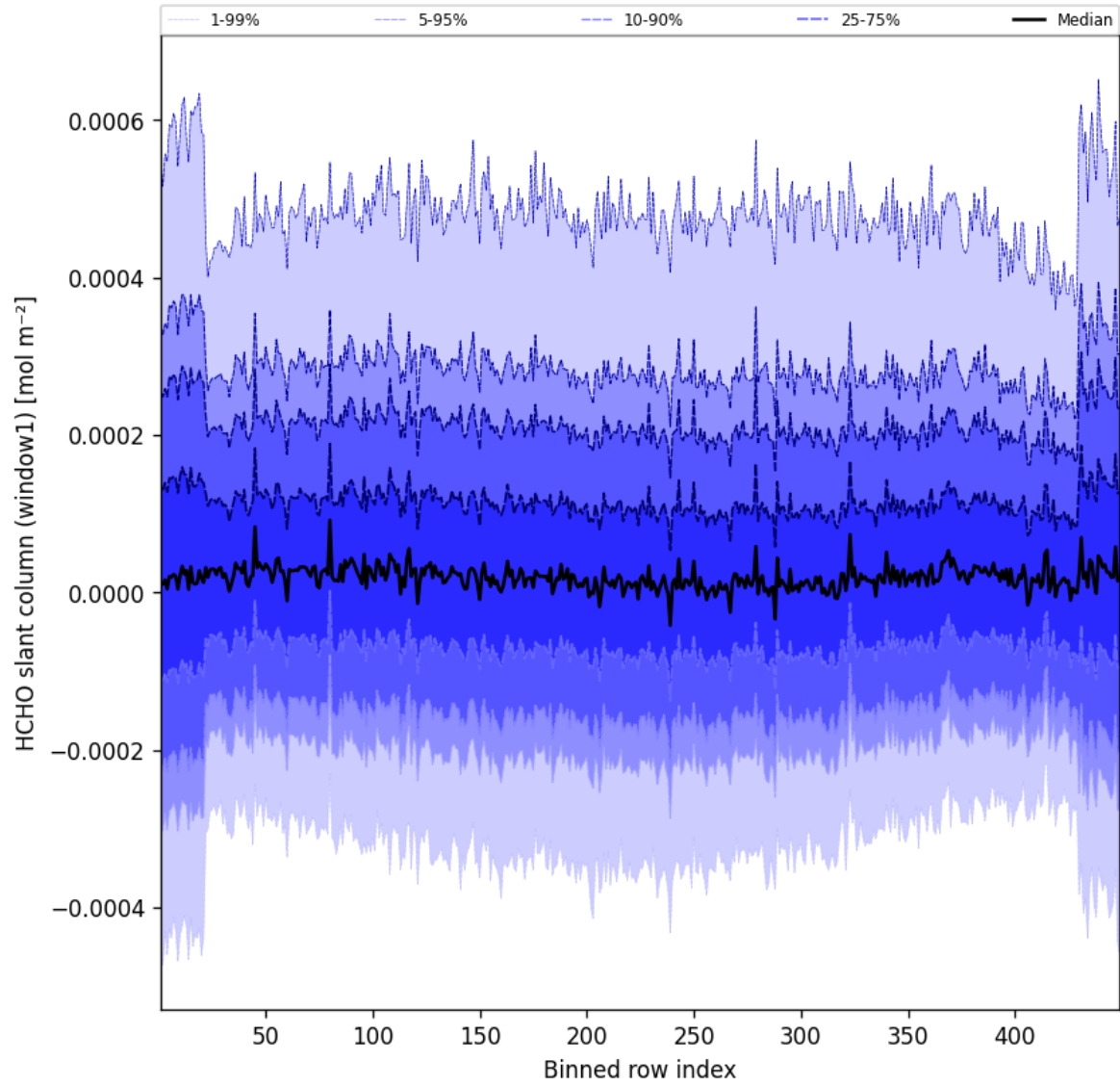
Figure 50: Along track statistics of “HCHO slant column (window1)” for 2025-06-16 to 2025-06-17
