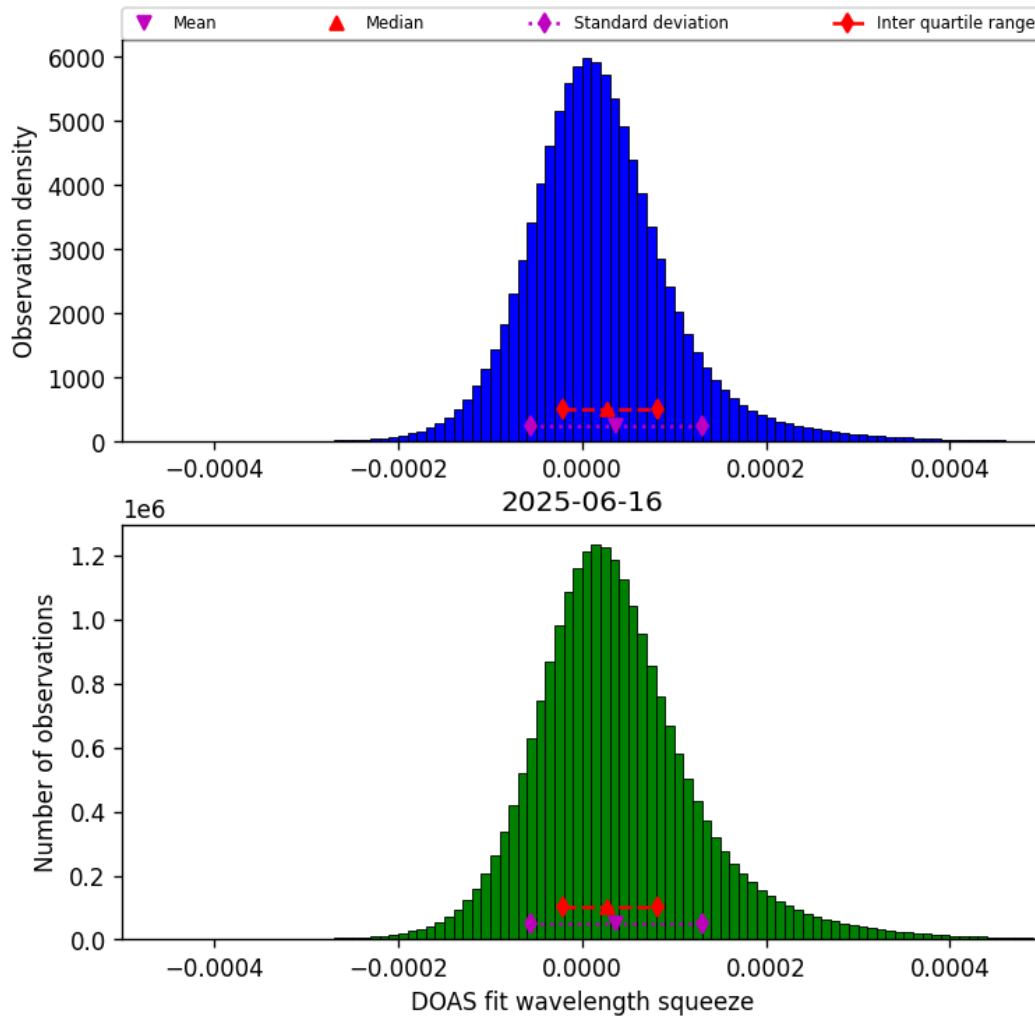
Figure 43: Histogram of “DOAS fit wavelength squeeze” for 2025-06-16 to 2025-06-17
