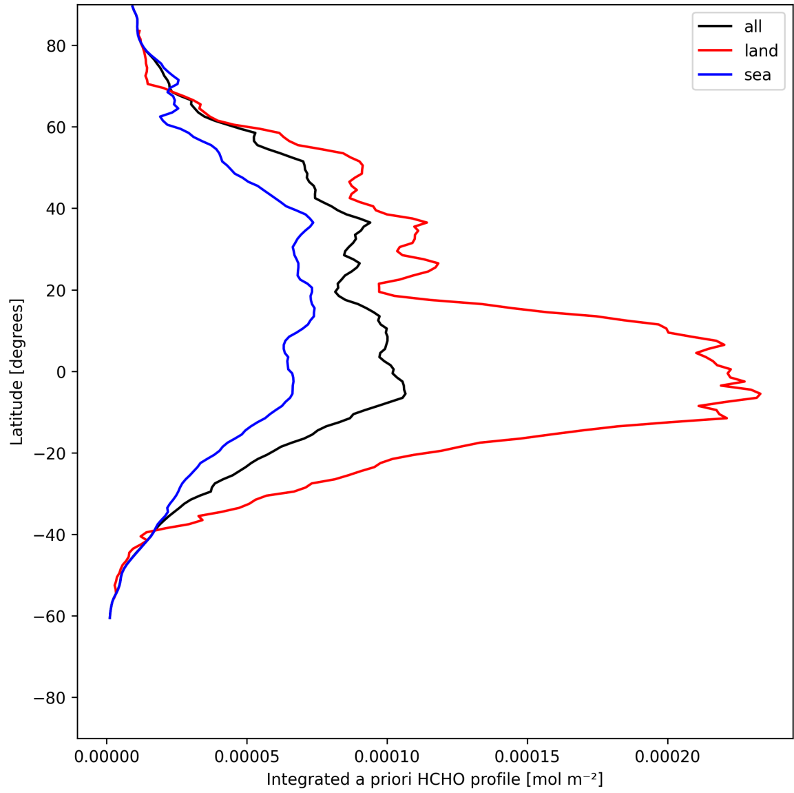
Figure 27: Zonal average of “Integrated a priori HCHO profile” for 2025-06-16 to 2025-06-17.
