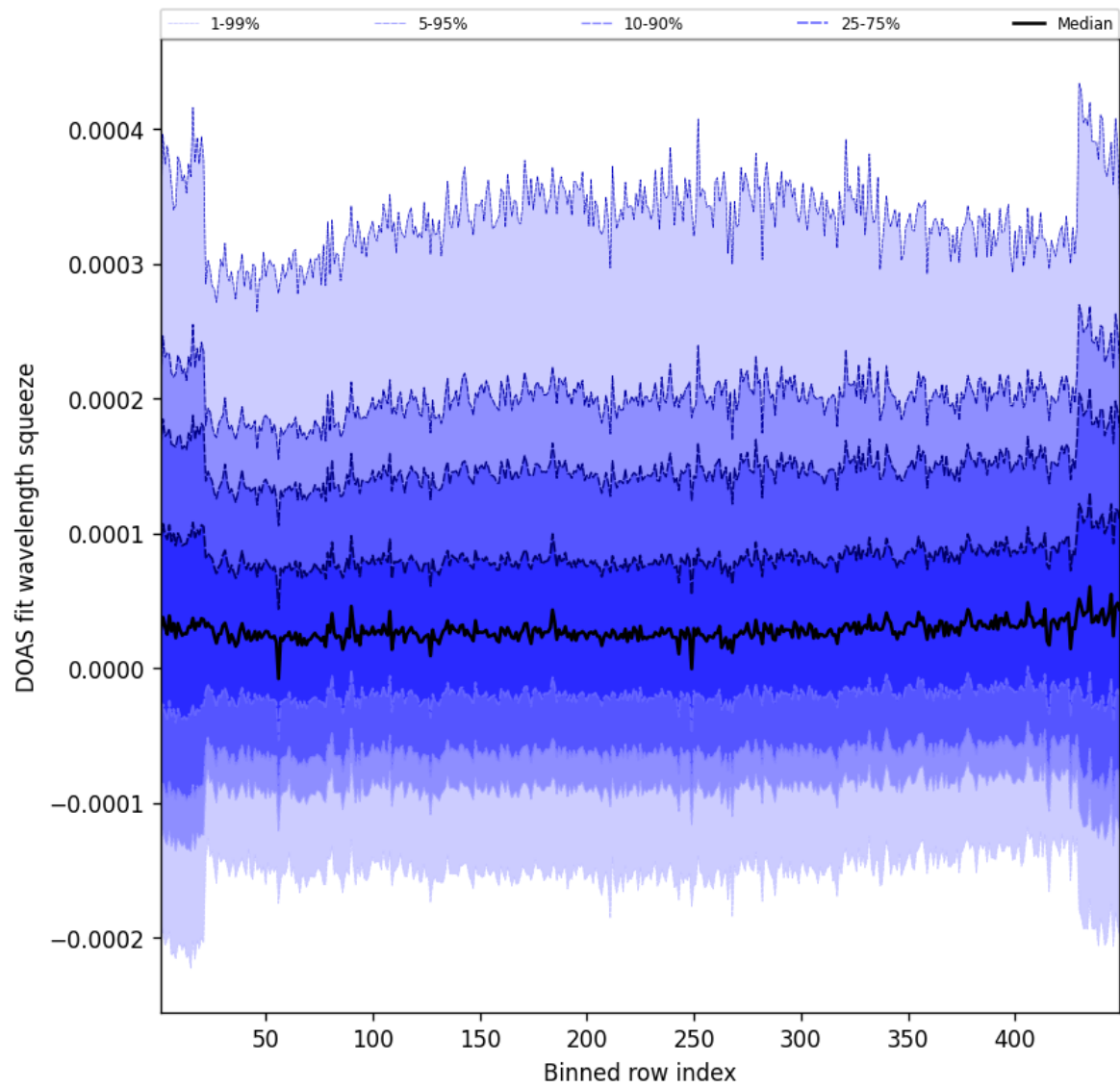
Figure 57: Along track statistics of “DOAS fit wavelength squeeze” for 2025-06-16 to 2025-06-17
