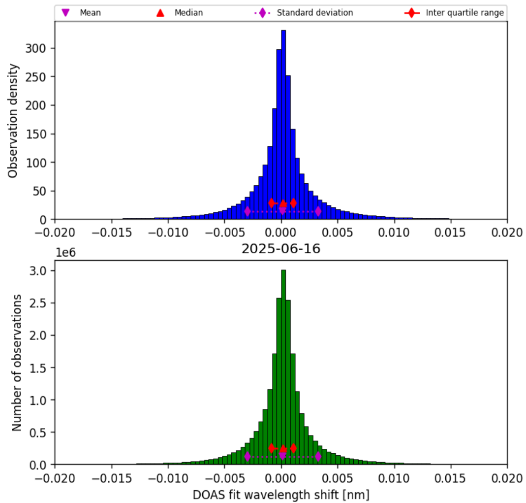
Figure 42: Histogram of “DOAS fit wavelength shift” for 2025-06-16 to 2025-06-17
