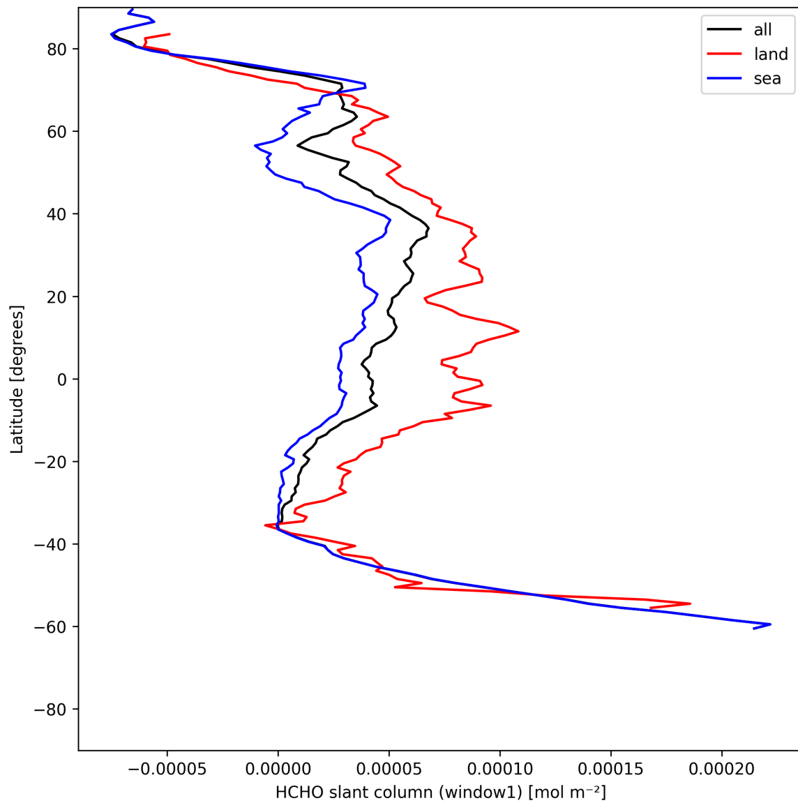
Figure 22: Zonal average of “HCHO slant column (window1)” for 2025-06-16 to 2025-06-17.
