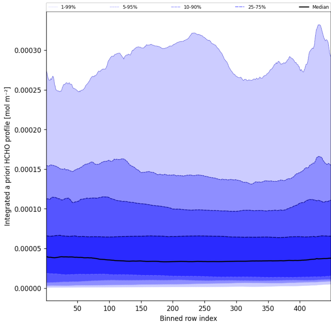
Figure 55: Along track statistics of "Integrated a priori HCHO profile" for 2025-06-16 to 2025-06-17
