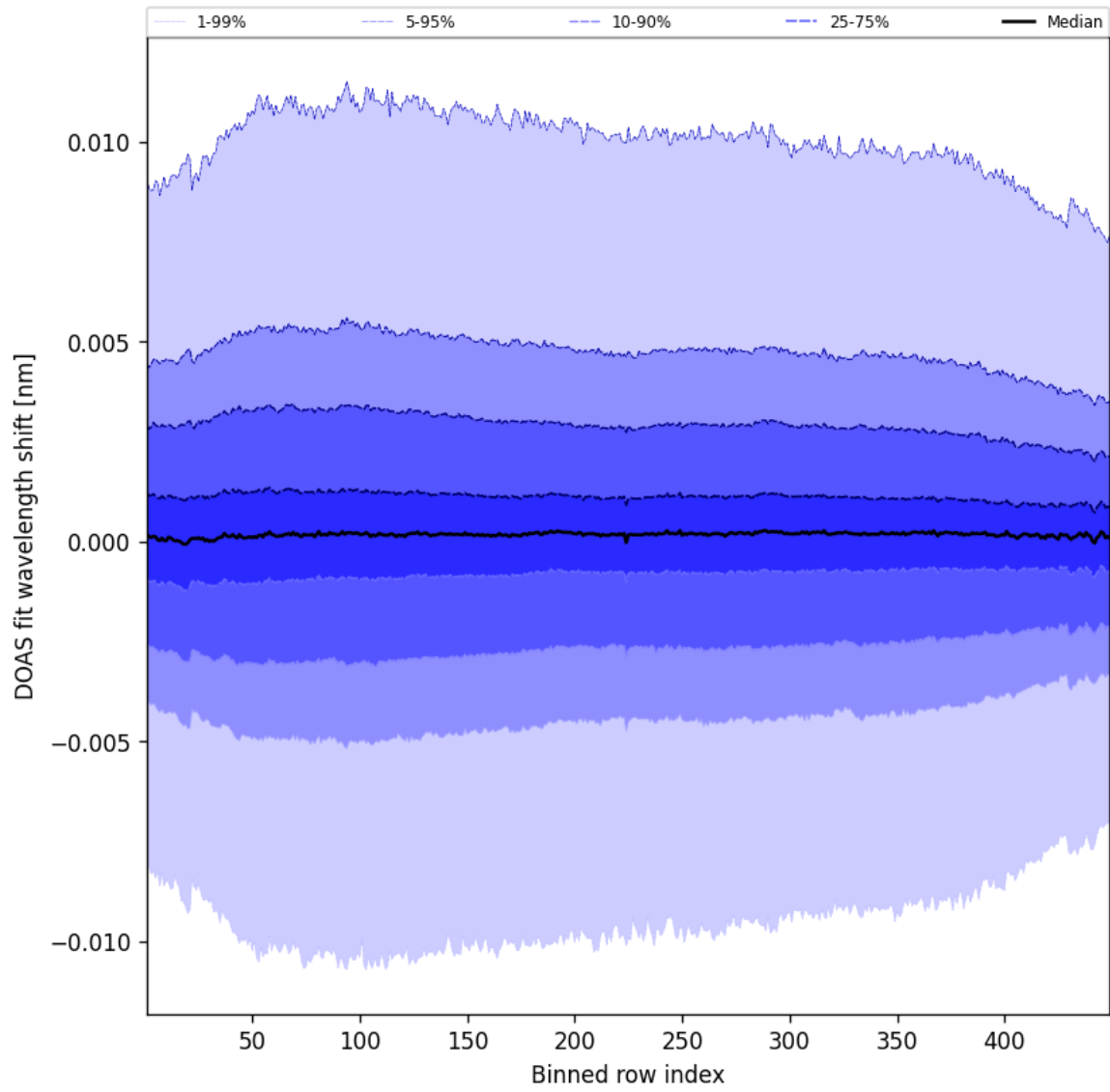
Figure 56: Along track statistics of “DOAS fit wavelength shift” for 2025-06-16 to 2025-06-17
