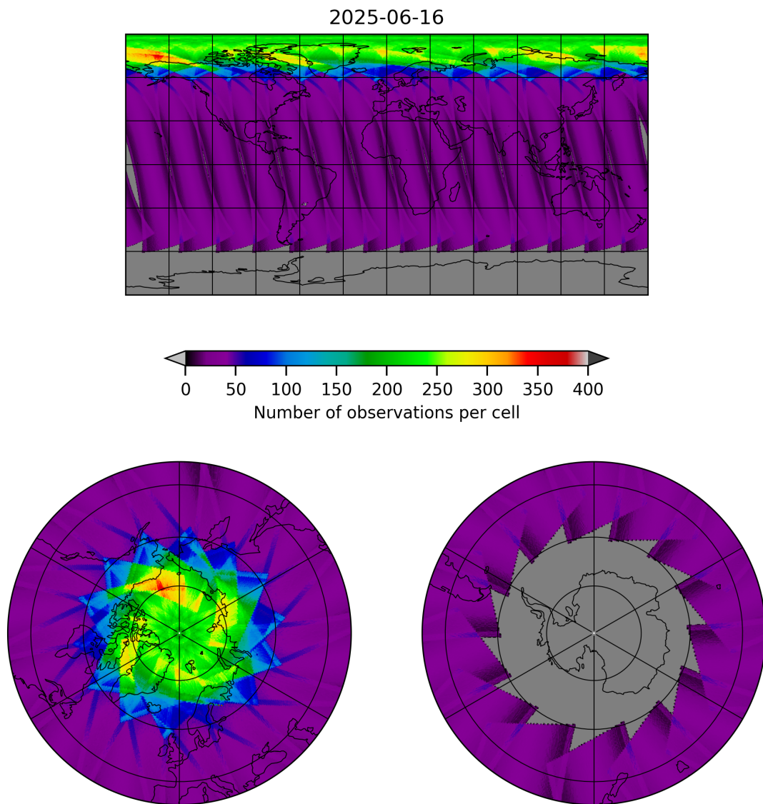
Figure 17: Map of the number of observations for 2025-06-16 to 2025-06-17
