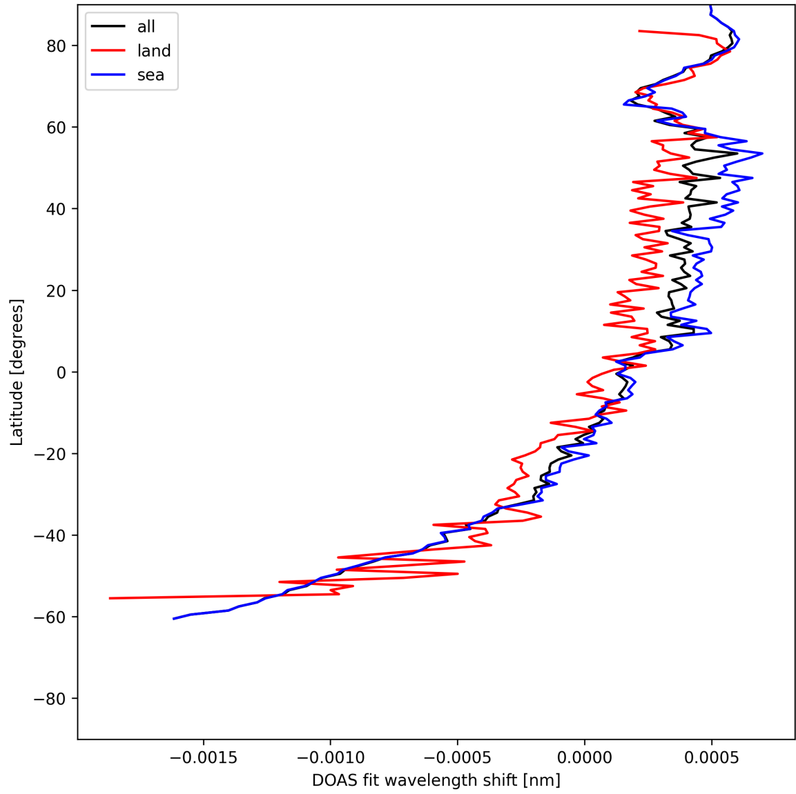
Figure 28: Zonal average of “DOAS fit wavelength shift” for 2025-06-16 to 2025-06-17.
