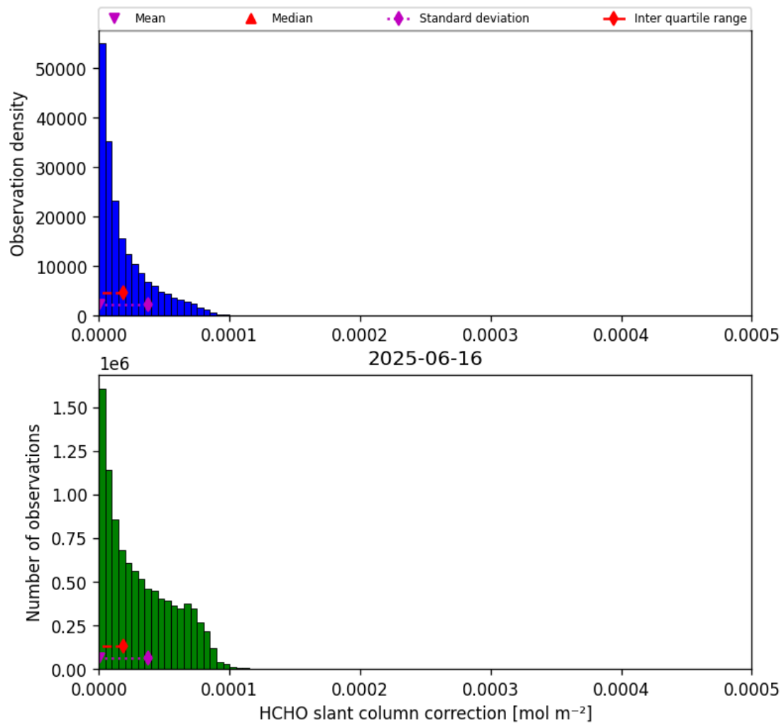
Figure 45: Histogram of “HCHO slant column correction” for 2025-06-16 to 2025-06-17
