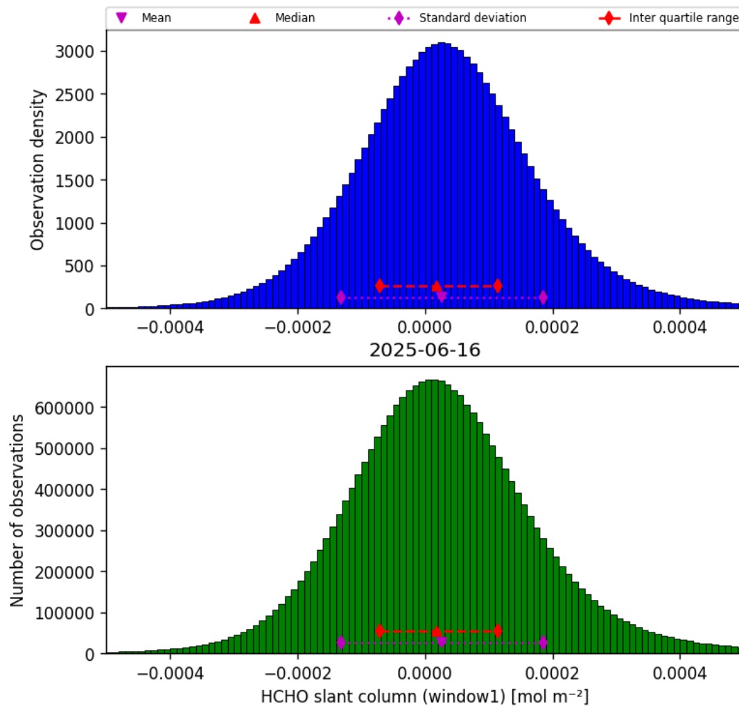
Figure 36: Histogram of “HCHO slant column (window1)” for 2025-06-16 to 2025-06-17
