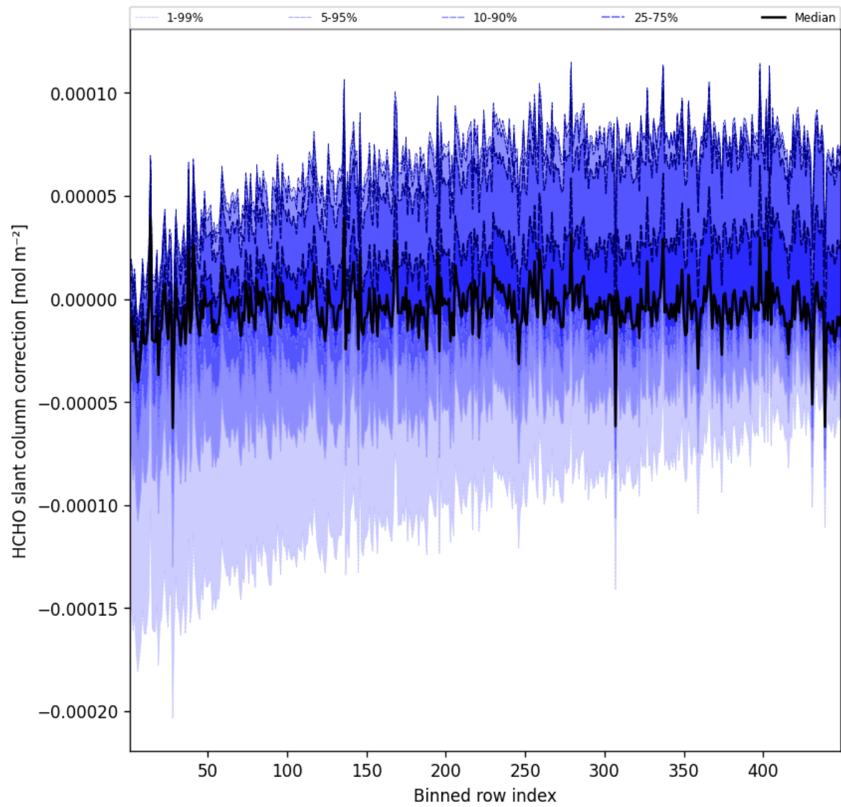
Figure 59: Along track statistics of “HCHO slant column correction” for 2025-06-16 to 2025-06-17
