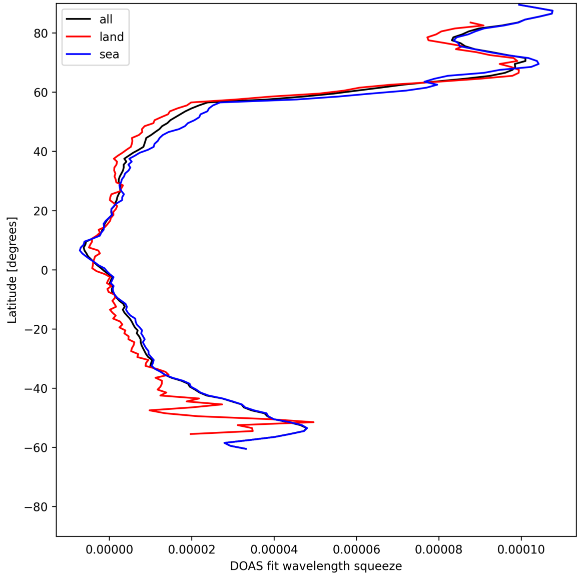
Figure 29: Zonal average of “DOAS fit wavelength squeeze” for 2025-06-16 to 2025-06-17.
