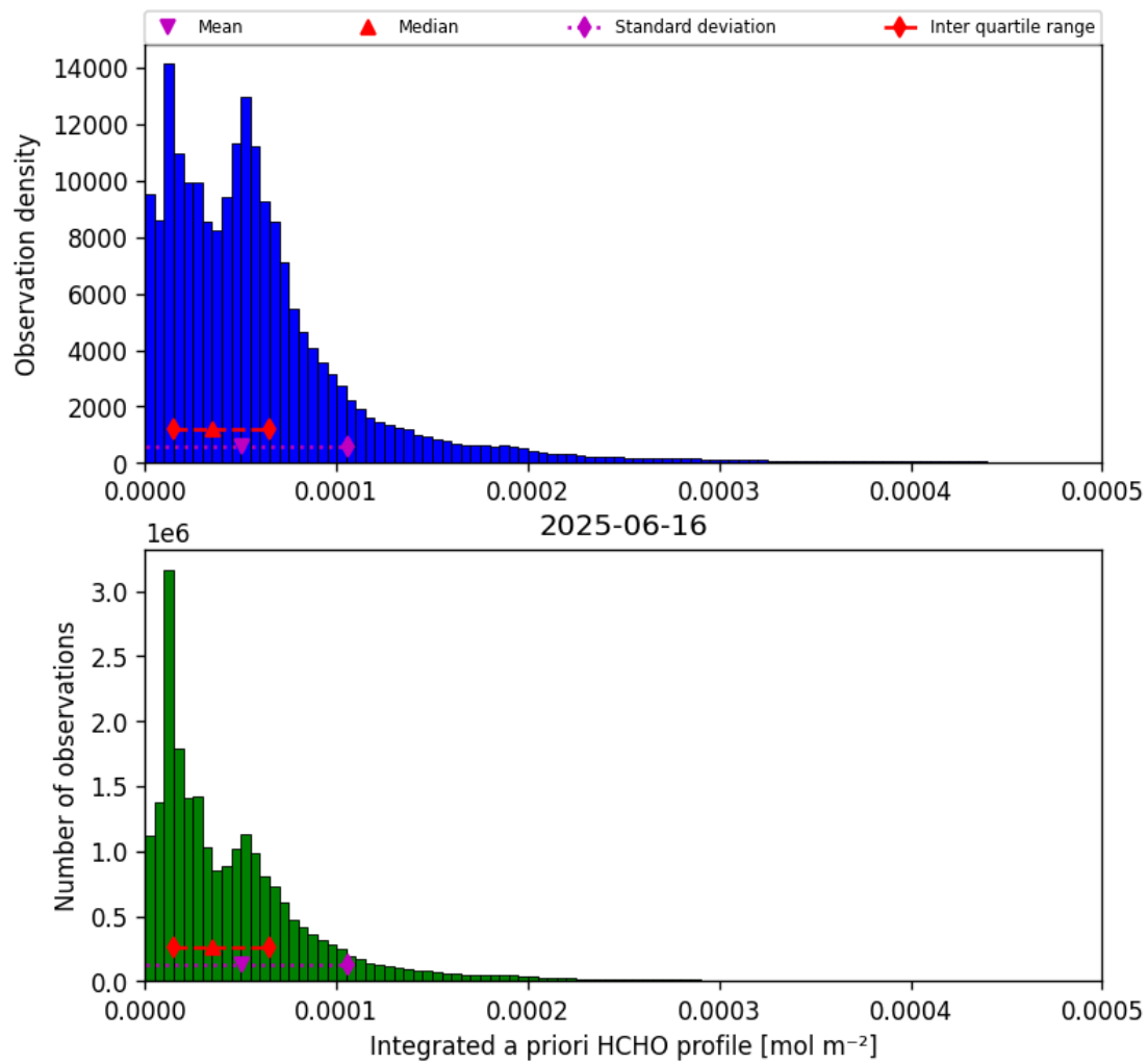
Figure 41: Histogram of “Integrated a priori HCHO profile” for 2025-06-16 to 2025-06-17
