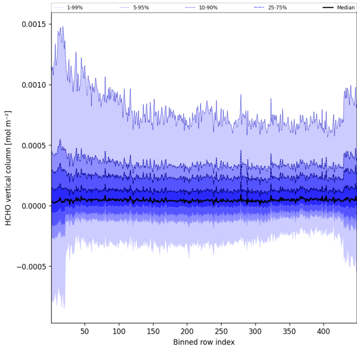
Figure 47: Along track statistics of “HCHO vertical column” for 2025-06-16 to 2025-06-17
