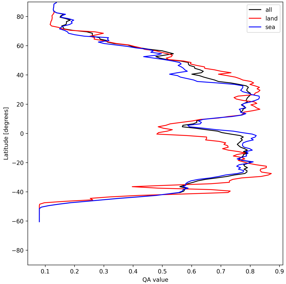
Figure 18: Zonal average of “QA value” for 2025-06-16 to 2025-06-17.
