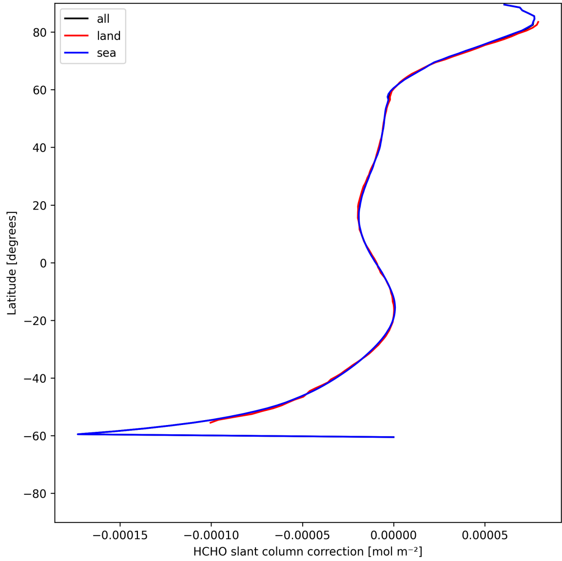
Figure 31: Zonal average of “HCHO slant column correction” for 2025-06-16 to 2025-06-17.
