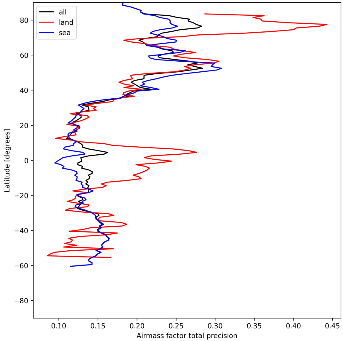
Figure 25: Zonal average of “Airmass factor total precision” for 2025-06-16 to 2025-06-17.
