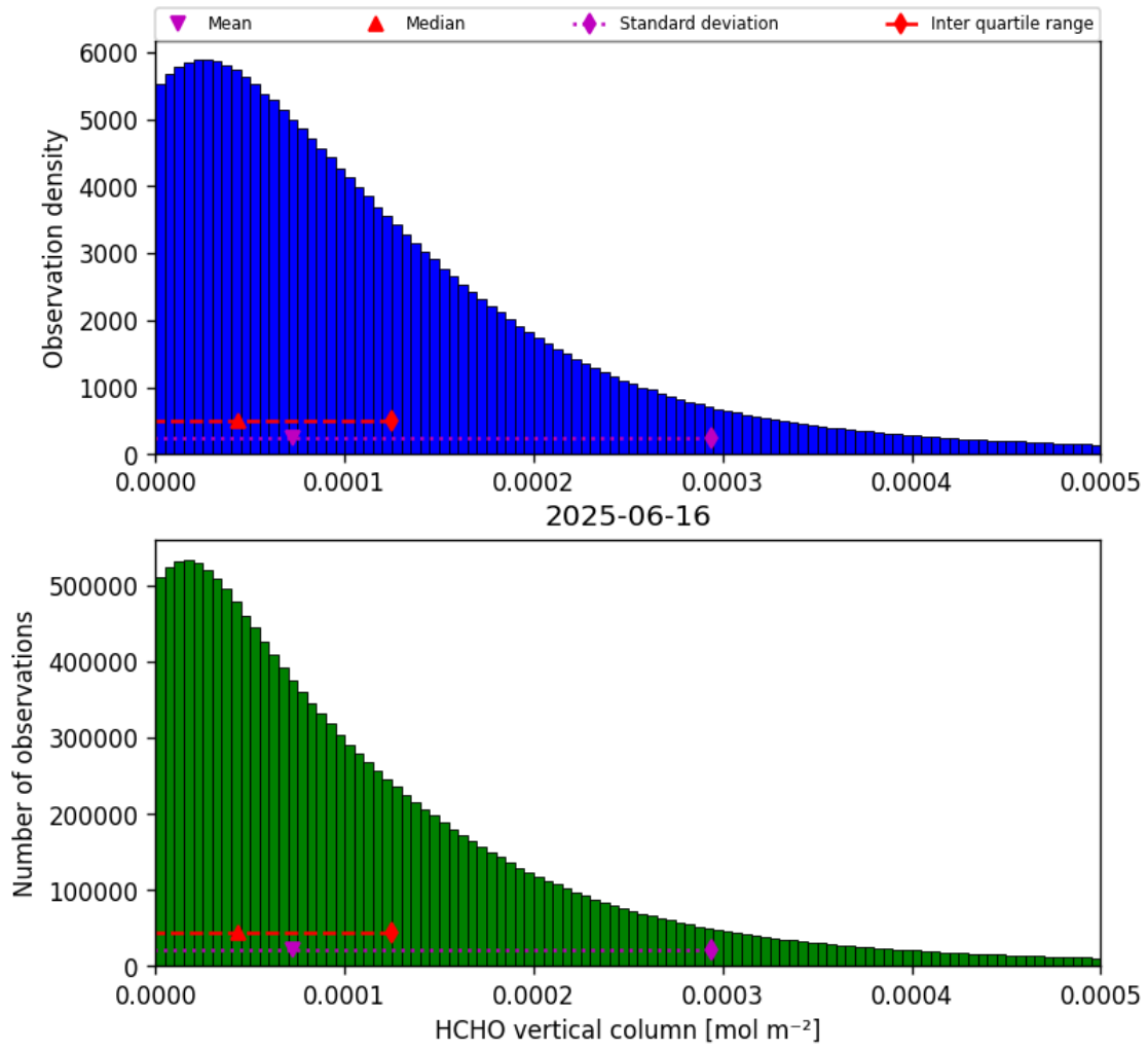
Figure 33: Histogram of “HCHO vertical column” for 2025-06-16 to 2025-06-17
