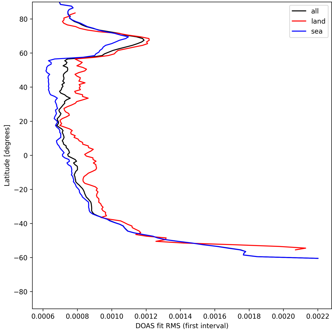
Figure 30: Zonal average of "DOAS fit RMS (first interval)" for 2025-06-16 to 2025-06-17.
