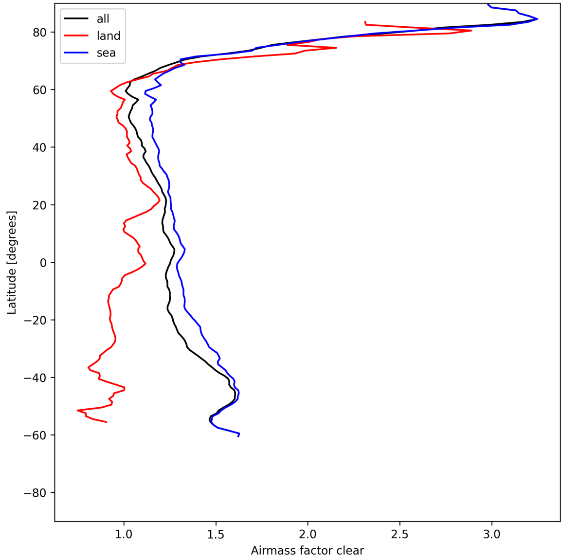
Figure 26: Zonal average of “Airmass factor clear” for 2025-06-16 to 2025-06-17.
