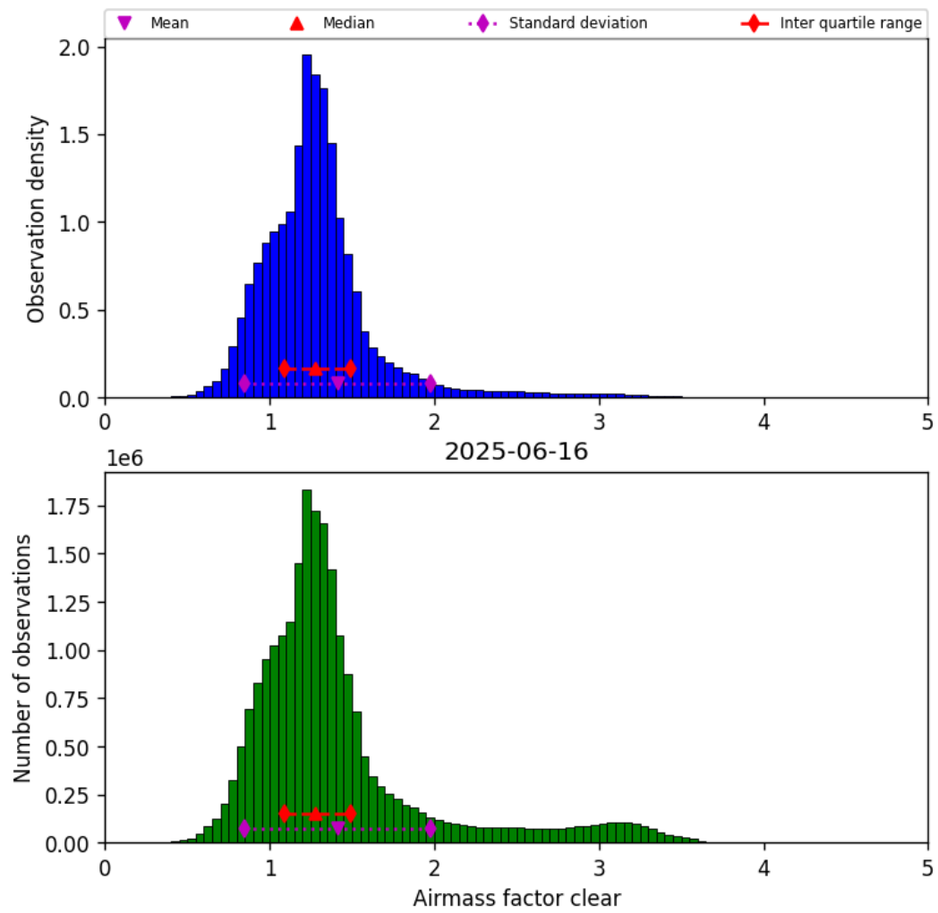
Figure 40: Histogram of “Airmass factor clear” for 2025-06-16 to 2025-06-17
