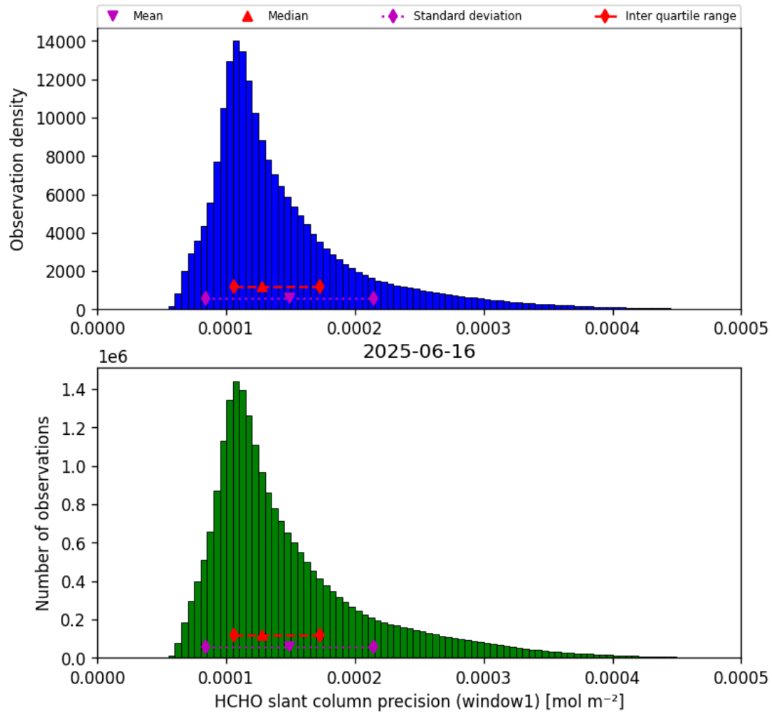
Figure 37: Histogram of “HCHO slant column precision (window1)” for 2025-06-16 to 2025-06-17
