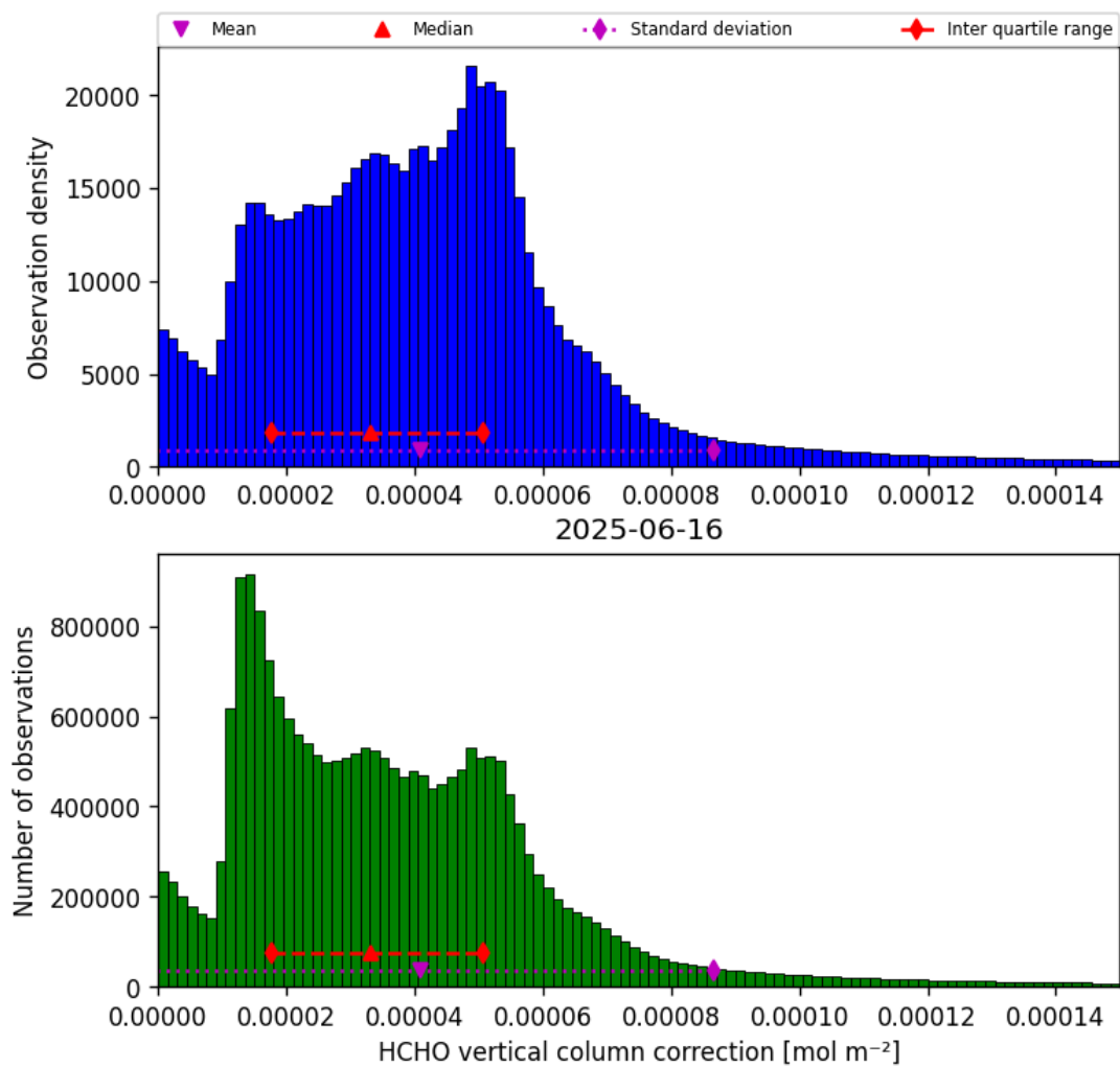
Figure 35: Histogram of “HCHO vertical column correction” for 2025-06-16 to 2025-06-17
