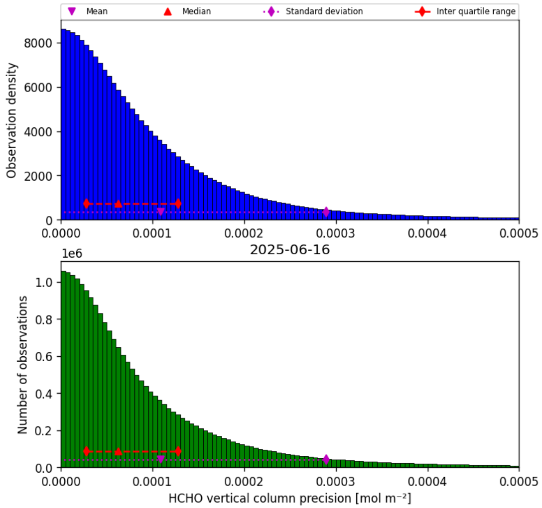
Figure 34: Histogram of “HCHO vertical column precision” for 2025-06-16 to 2025-06-17
