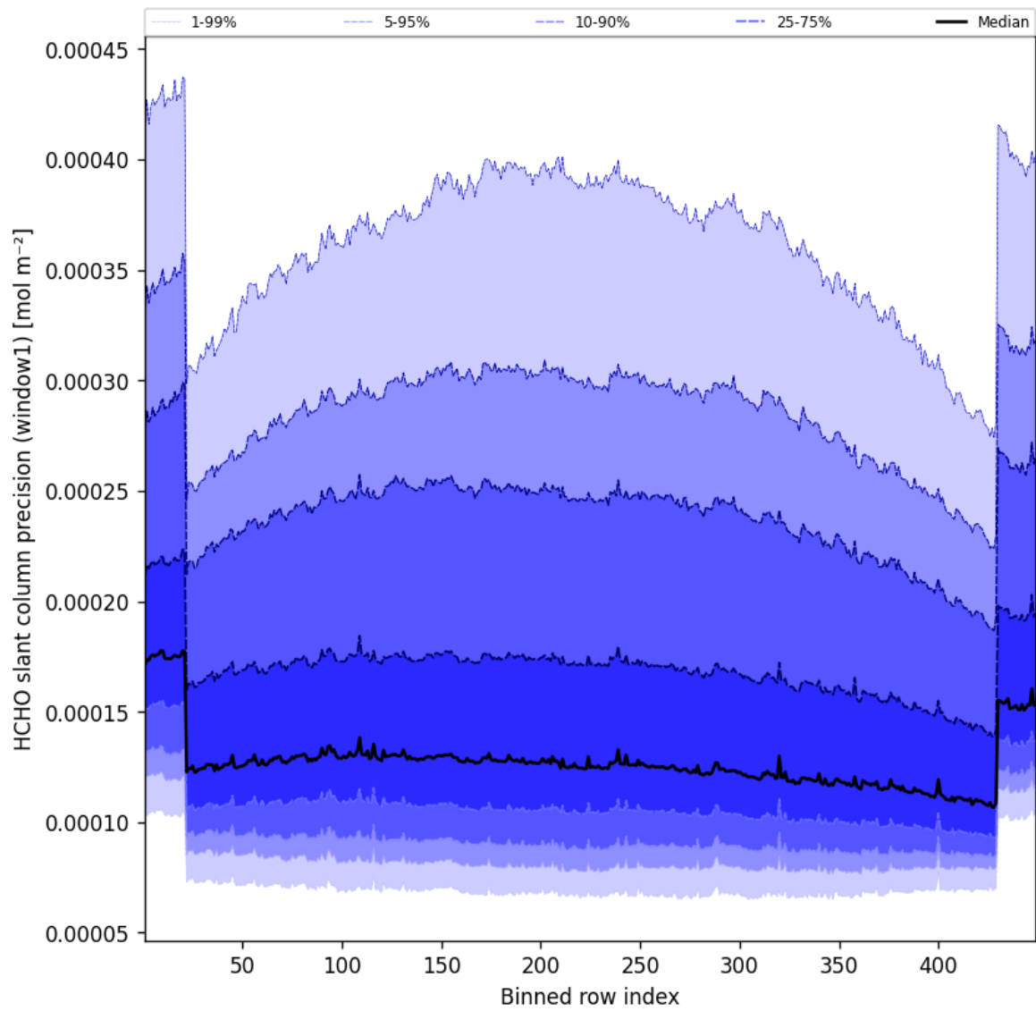
Figure 51: Along track statistics of “HCHO slant column precision (window1)” for 2025-06-16 to 2025-06-17
