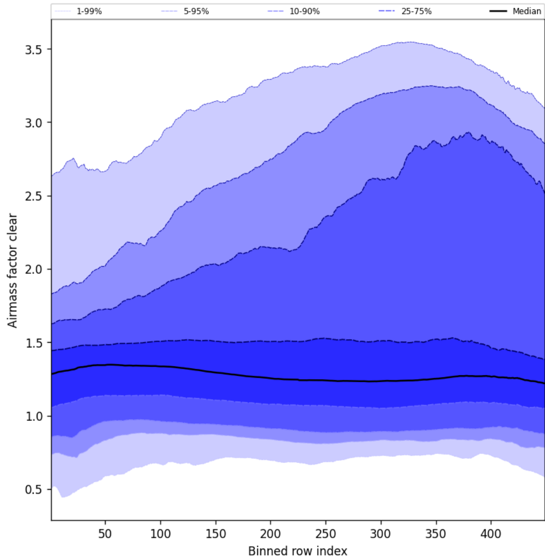
Figure 54: Along track statistics of “Airmass factor clear” for 2025-06-16 to 2025-06-17
