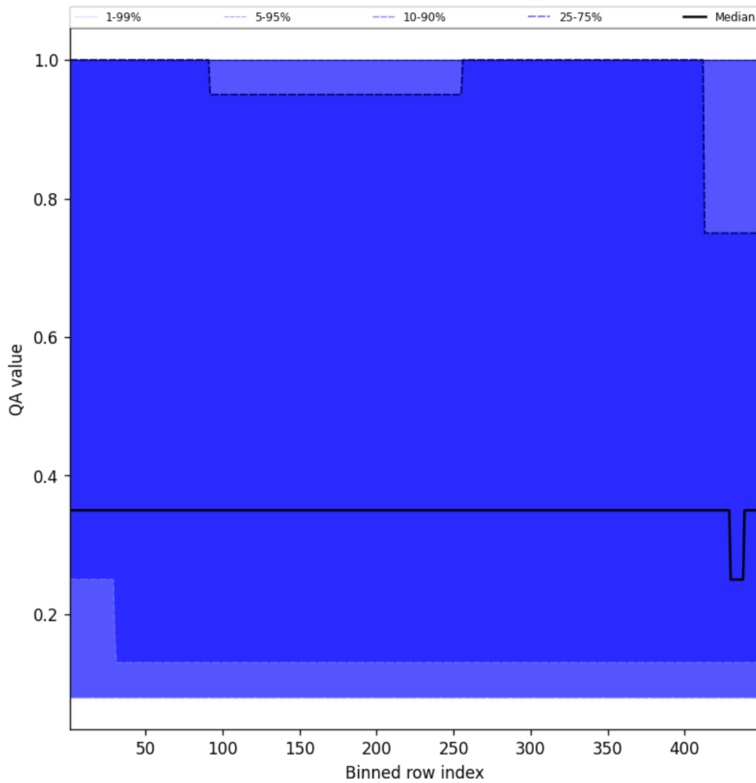
Figure 46: Along track statistics of “QA value” for 2025-06-16 to 2025-06-17
