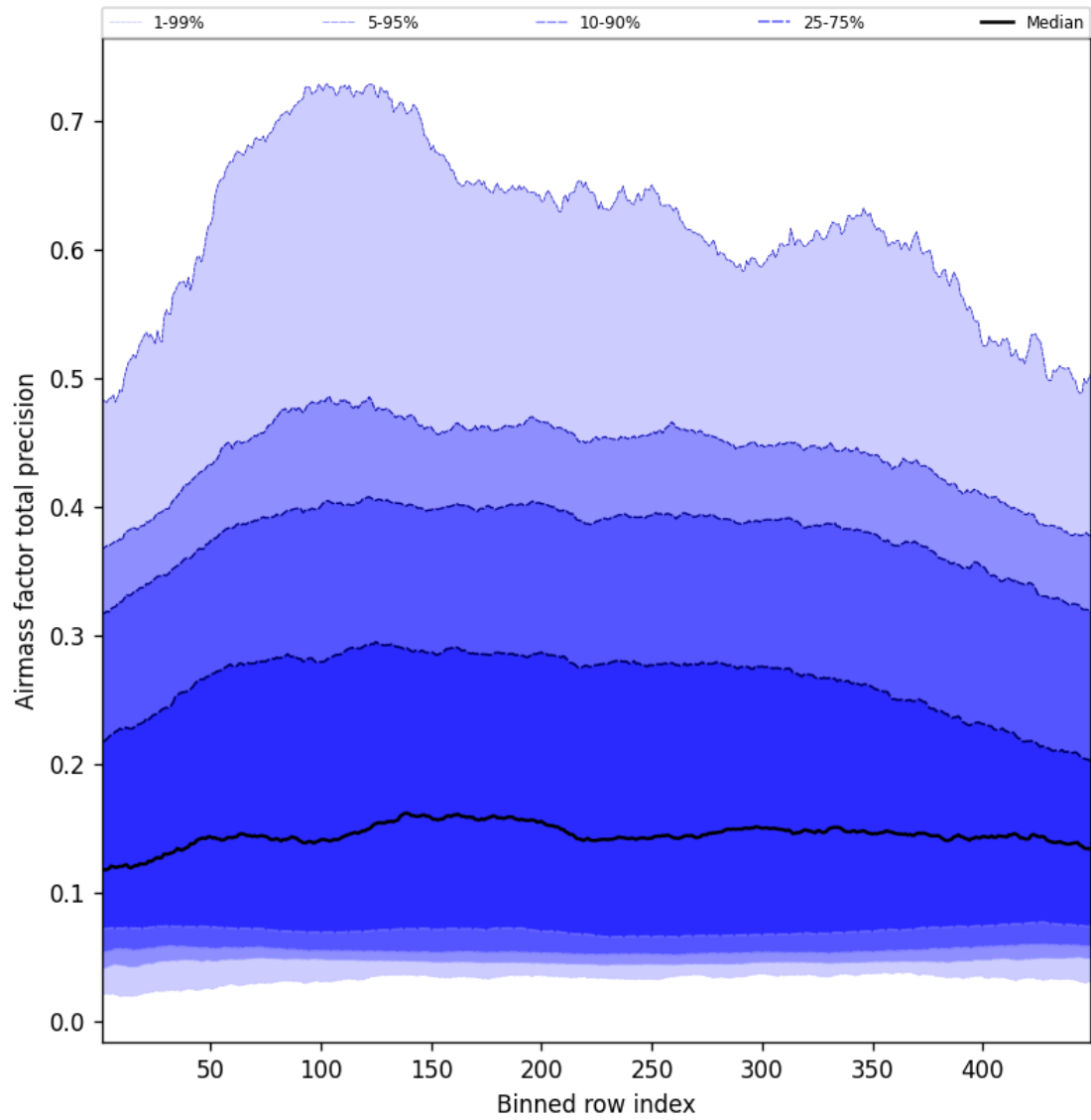
Figure 53: Along track statistics of “Airmass factor total precision” for 2025-06-16 to 2025-06-17
