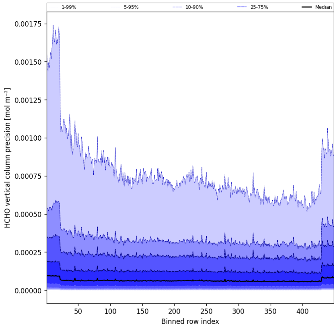
Figure 48: Along track statistics of “HCHO vertical column precision” for 2025-06-16 to 2025-06-17
