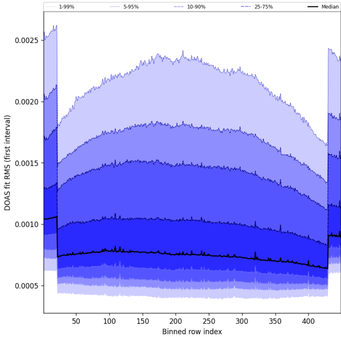
Figure 58: Along track statistics of “DOAS fit RMS (first interval)” for 2025-06-16 to 2025-06-17
