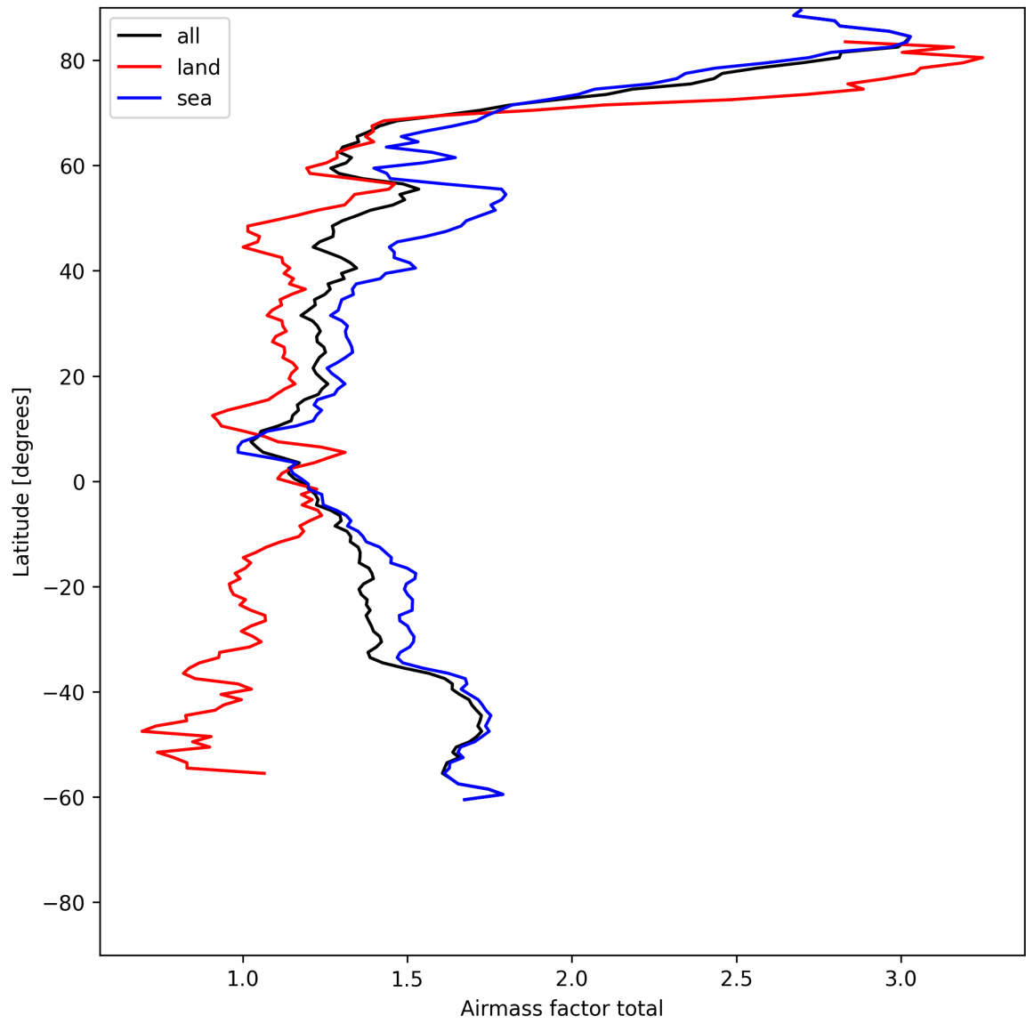
Figure 24: Zonal average of “Airmass factor total” for 2025-06-16 to 2025-06-17.
