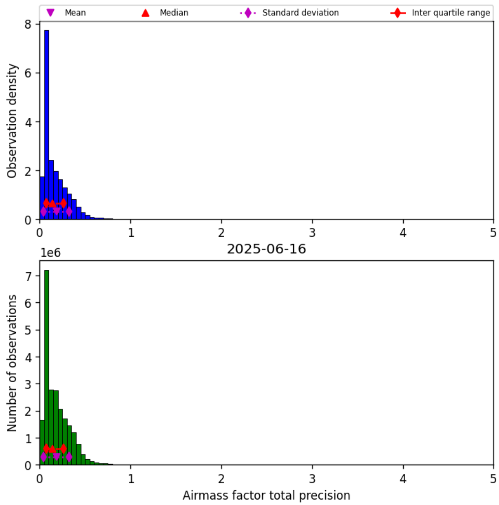
Figure 39: Histogram of “Airmass factor total precision” for 2025-06-16 to 2025-06-17
