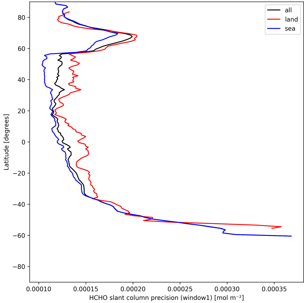
Figure 23: Zonal average of “HCHO slant column precision (window1)” for 2025-06-16 to 2025-06-17.
