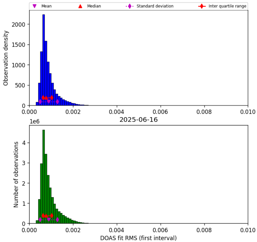
Figure 44: Histogram of “DOAS fit RMS (first interval)” for 2025-06-16 to 2025-06-17
