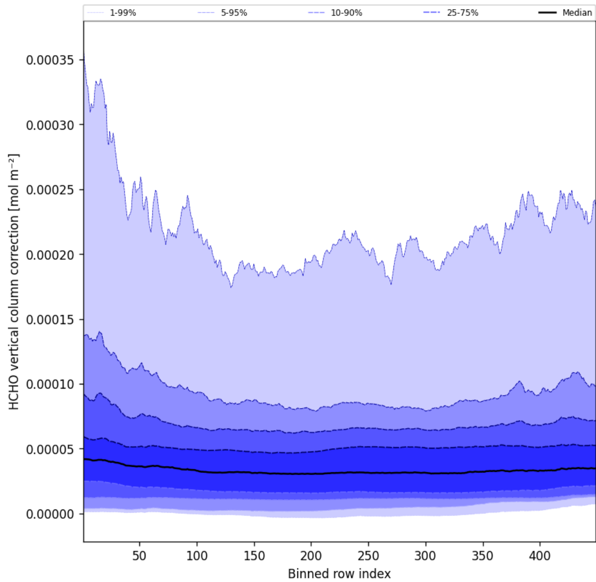
Figure 49: Along track statistics of “HCHO vertical column correction” for 2025-06-16 to 2025-06-17
