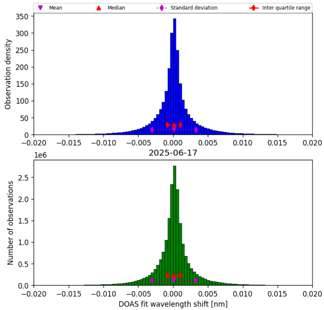
Figure 42: Histogram of “DOAS fit wavelength shift” for 2025-06-17 to 2025-06-17
