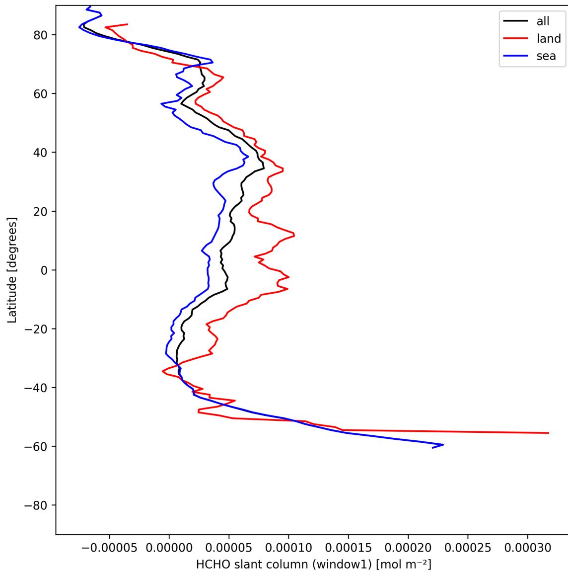
Figure 22: Zonal average of “HCHO slant column (window1)” for 2025-06-17 to 2025-06-17.
