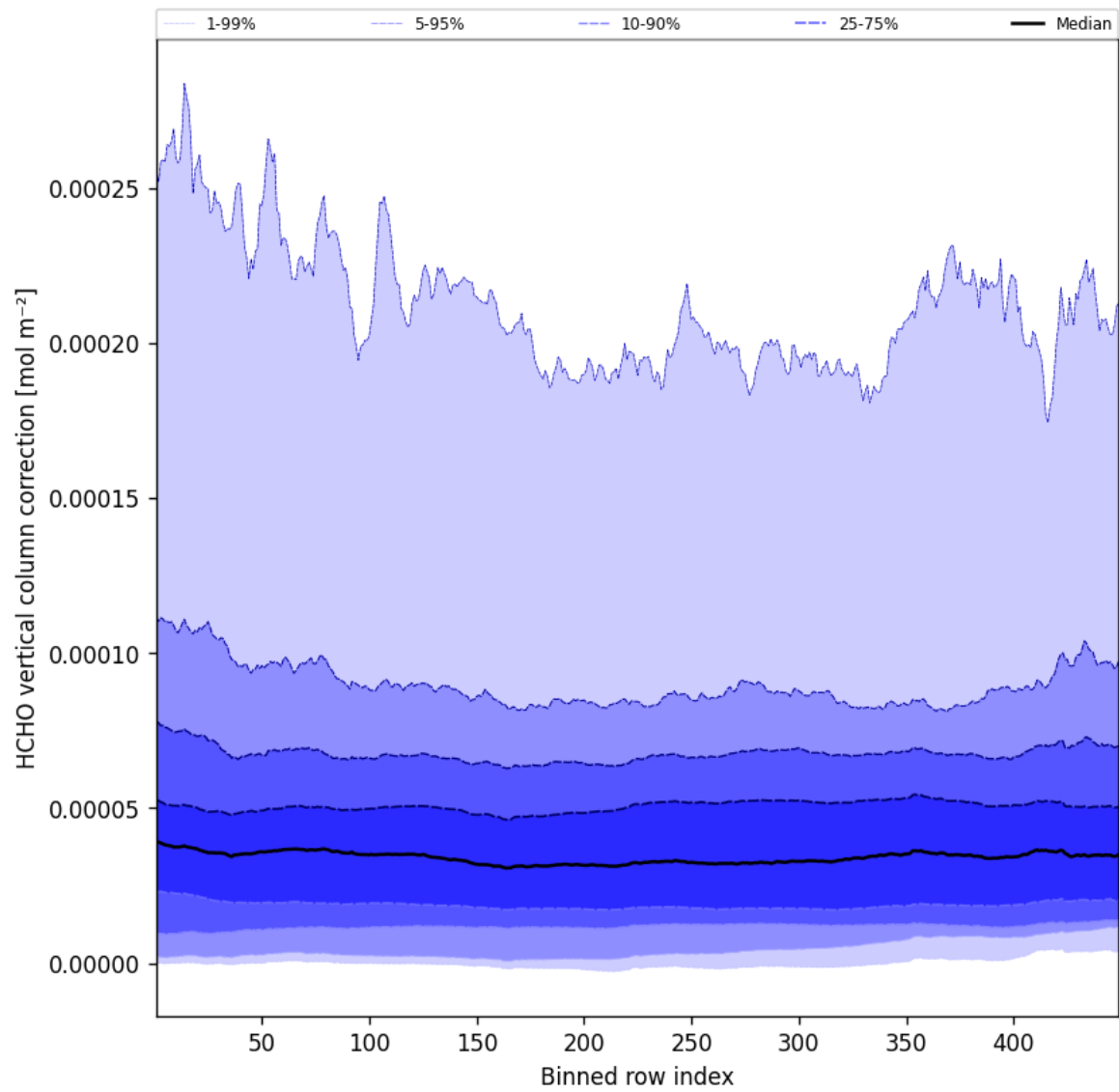
Figure 49: Along track statistics of “HCHO vertical column correction” for 2025-06-17 to 2025-06-17
