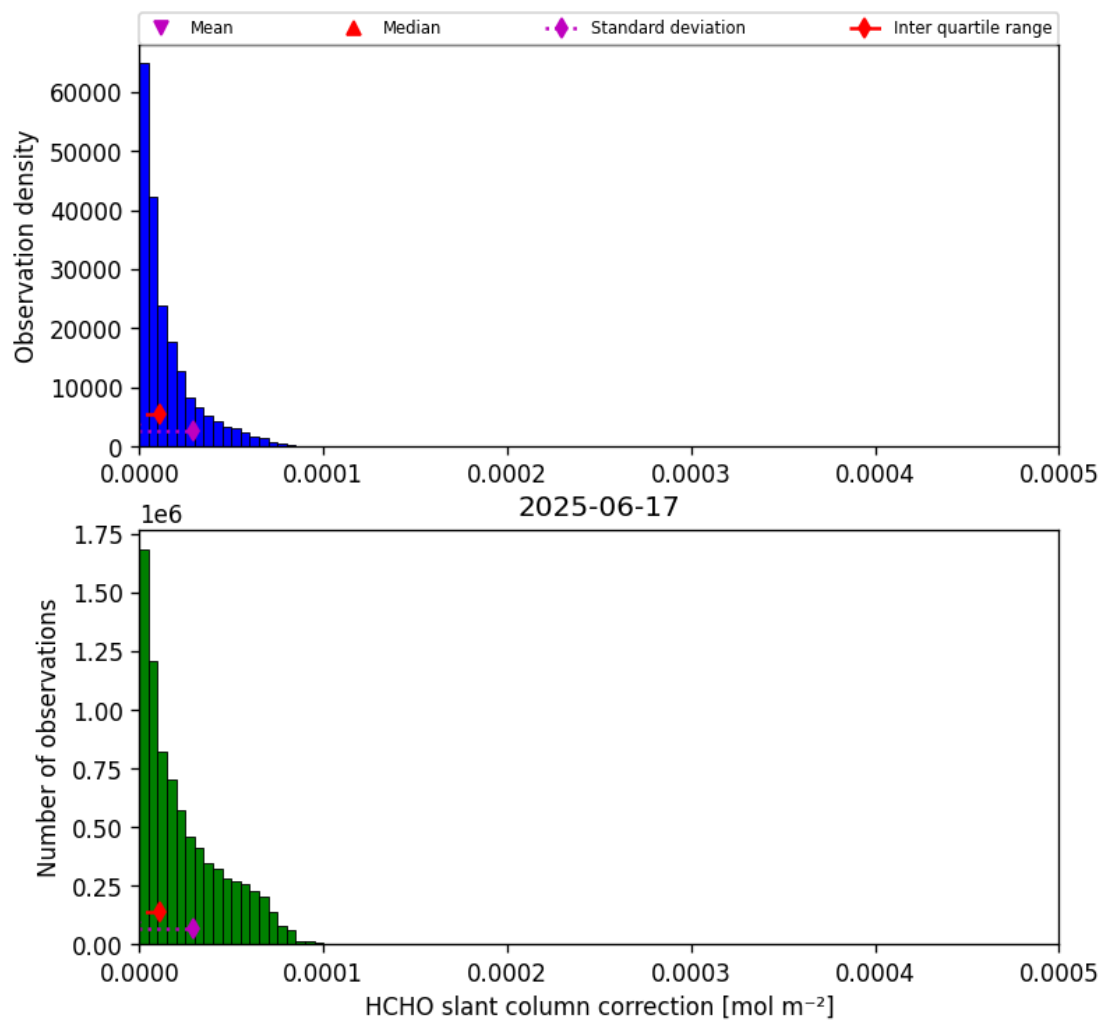
Figure 45: Histogram of “HCHO slant column correction” for 2025-06-17 to 2025-06-17
