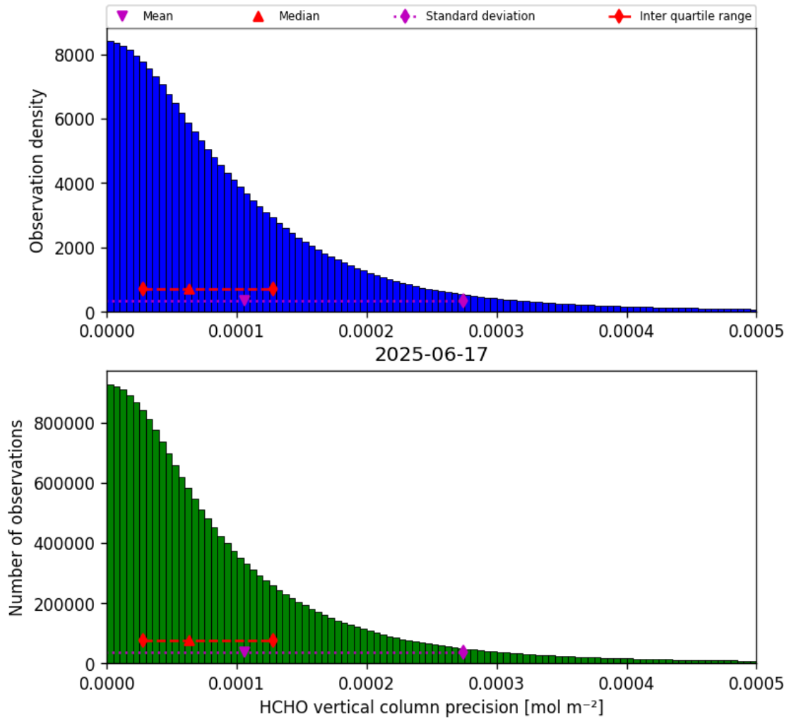
Figure 34: Histogram of “HCHO vertical column precision” for 2025-06-17 to 2025-06-17
