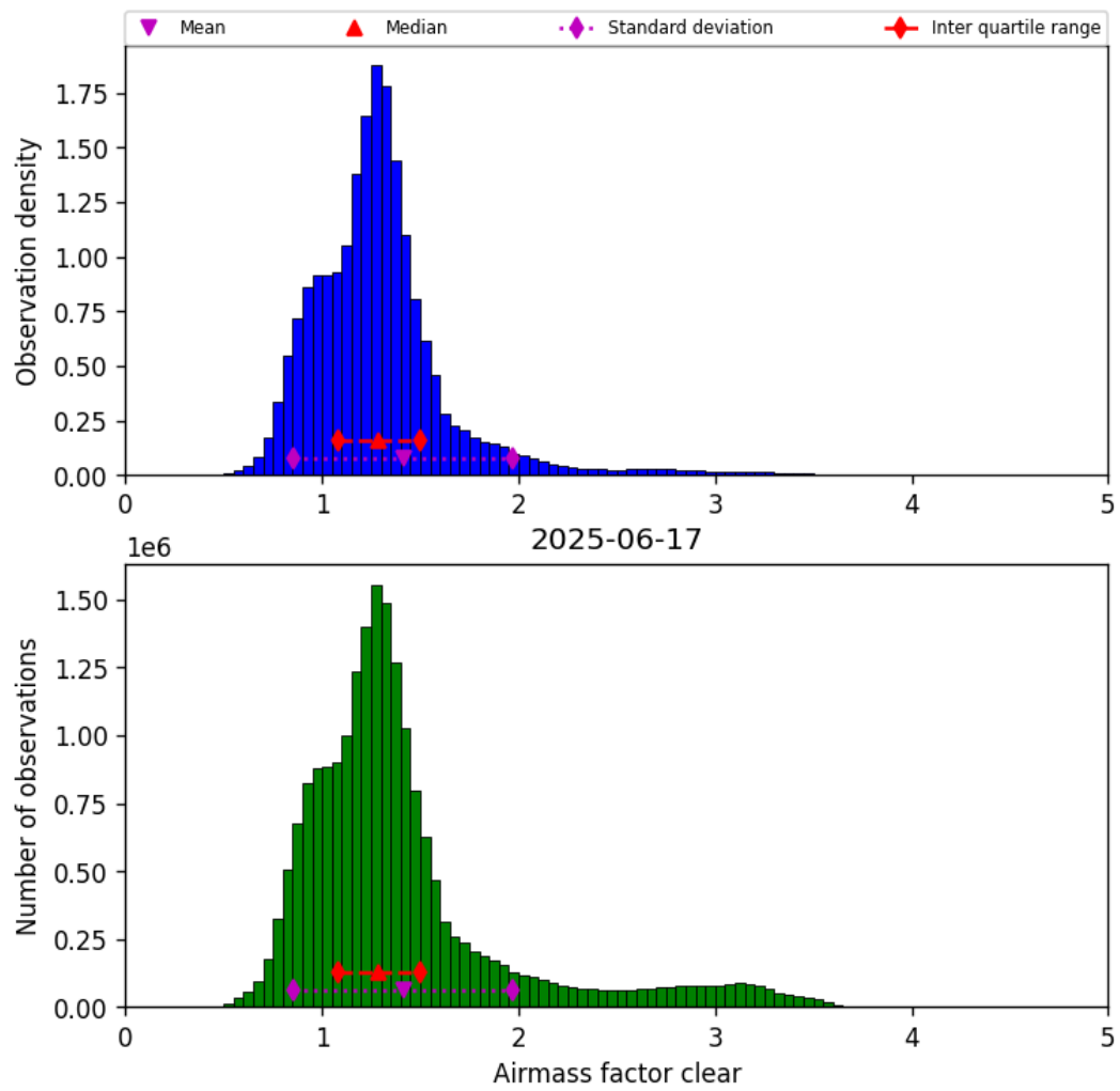
Figure 40: Histogram of “Airmass factor clear” for 2025-06-17 to 2025-06-17
