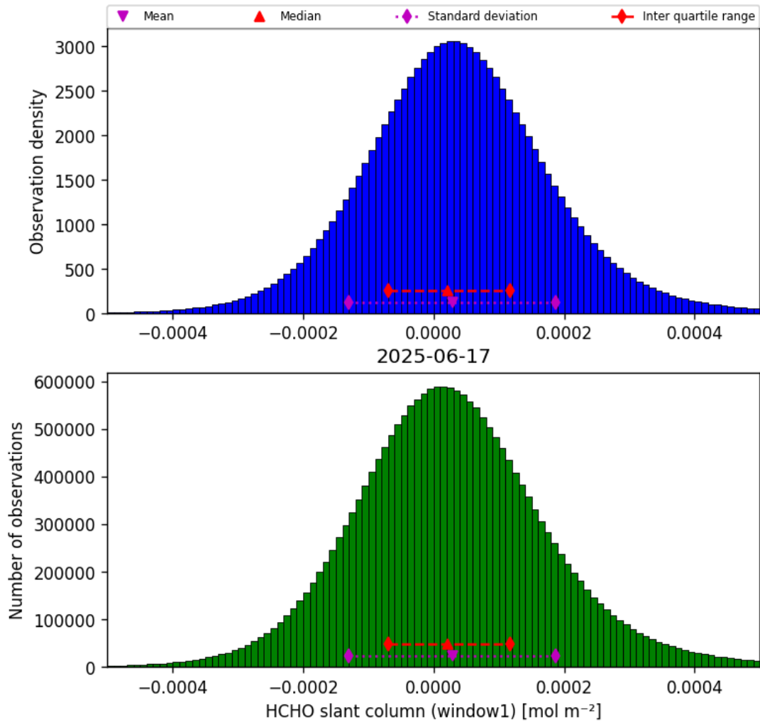
Figure 36: Histogram of “HCHO slant column (window1)” for 2025-06-17 to 2025-06-17
