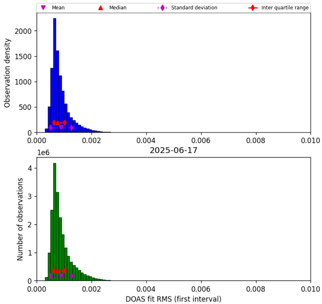
Figure 44: Histogram of “DOAS fit RMS (first interval)” for 2025-06-17 to 2025-06-17
