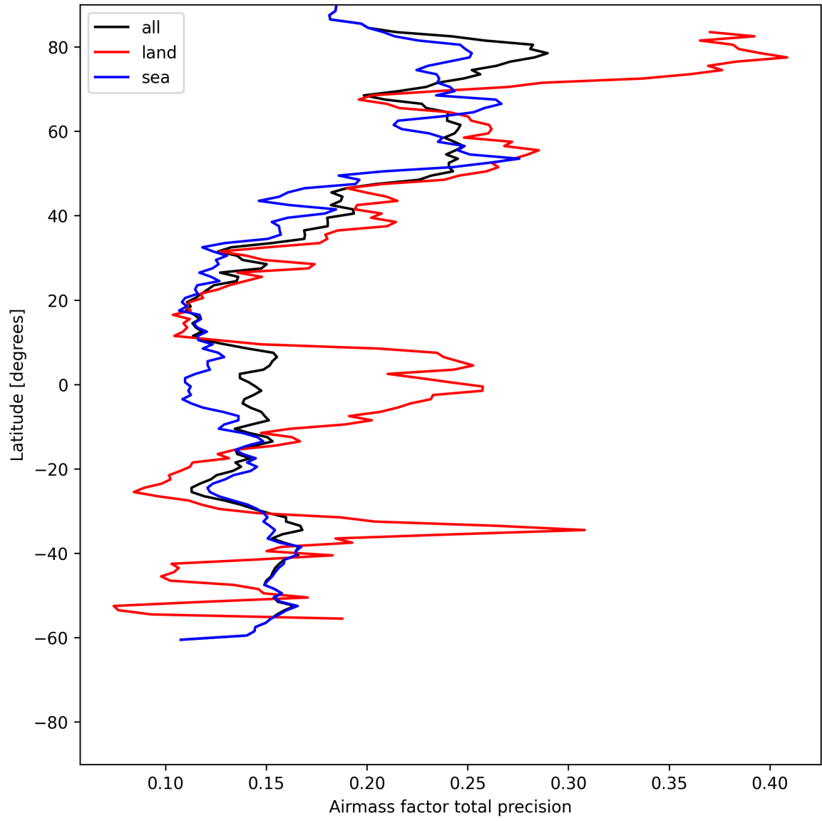
Figure 25: Zonal average of “Airmass factor total precision” for 2025-06-17 to 2025-06-17.
