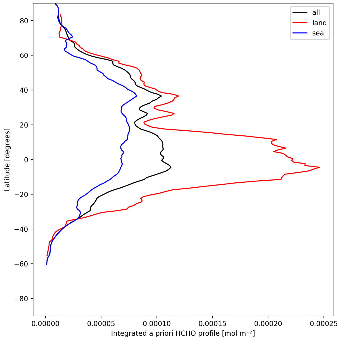
Figure 27: Zonal average of “Integrated a priori HCHO profile” for 2025-06-17 to 2025-06-17.
