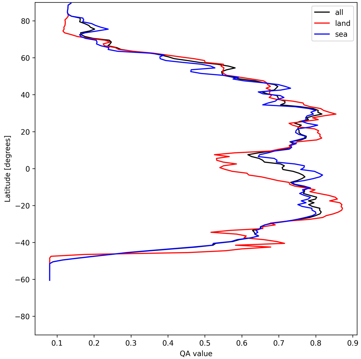
Figure 18: Zonal average of “QA value” for 2025-06-17 to 2025-06-17.
