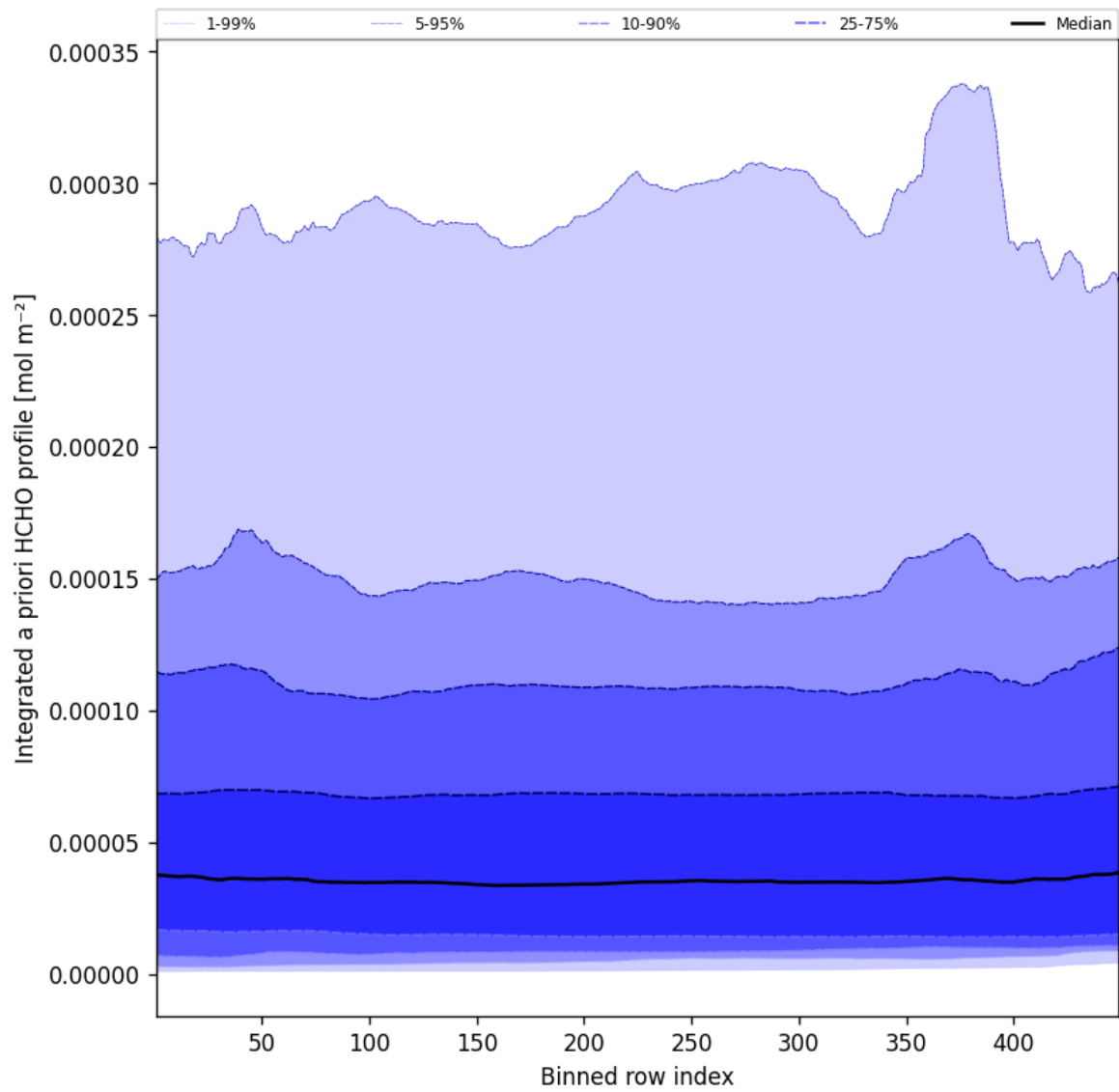
Figure 55: Along track statistics of "Integrated a priori HCHO profile" for 2025-06-17 to 2025-06-17
