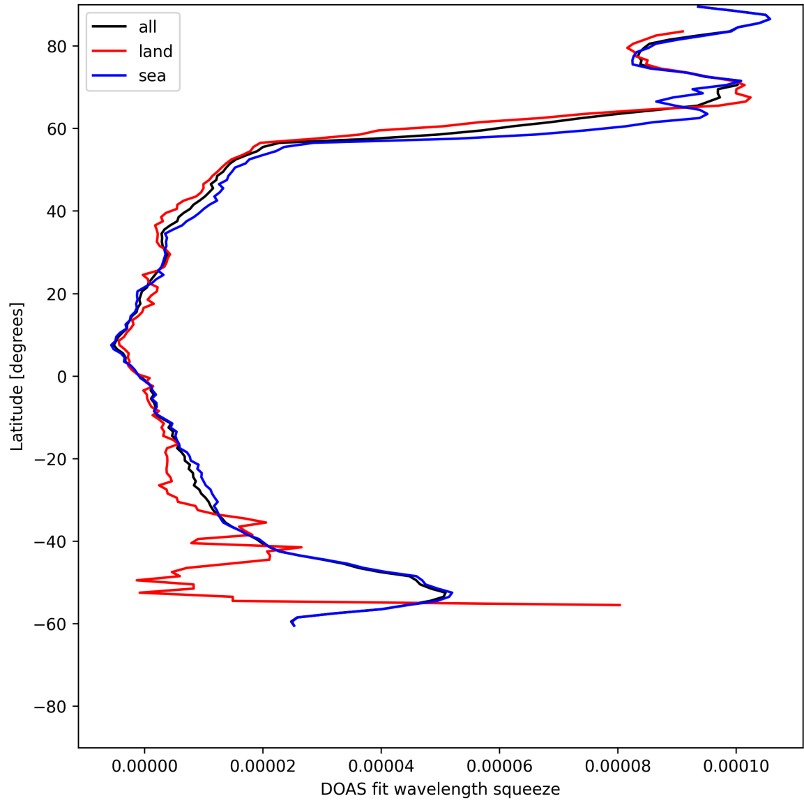
Figure 29: Zonal average of “DOAS fit wavelength squeeze” for 2025-06-17 to 2025-06-17.
