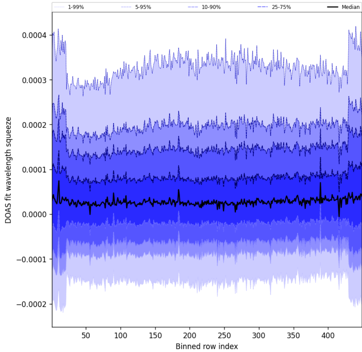
Figure 57: Along track statistics of “DOAS fit wavelength squeeze” for 2025-06-17 to 2025-06-17
