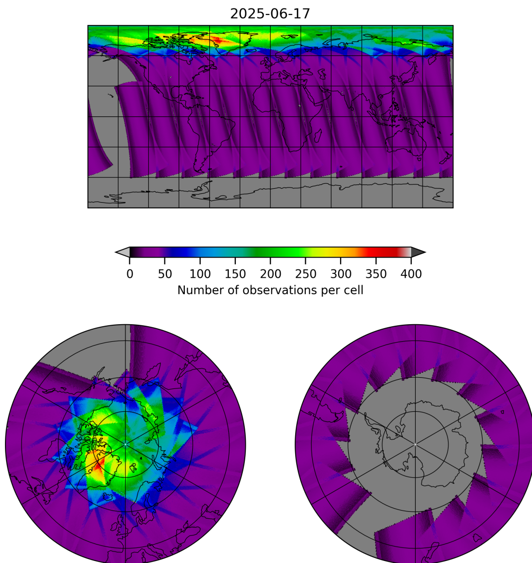
Figure 17: Map of the number of observations for 2025-06-17 to 2025-06-17
