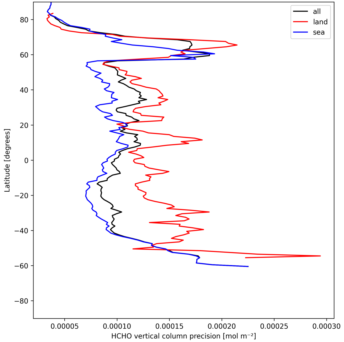
Figure 20: Zonal average of “HCHO vertical column precision” for 2025-06-17 to 2025-06-17.
