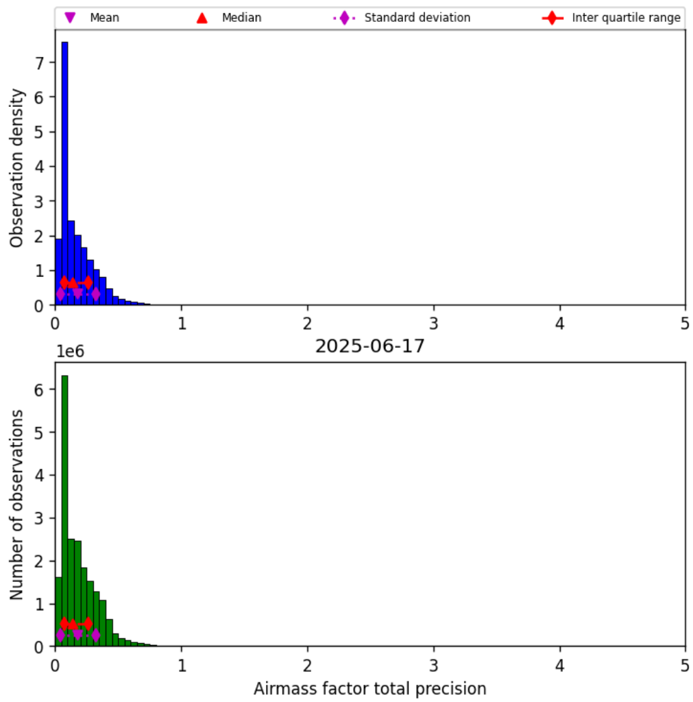
Figure 39: Histogram of “Airmass factor total precision” for 2025-06-17 to 2025-06-17
