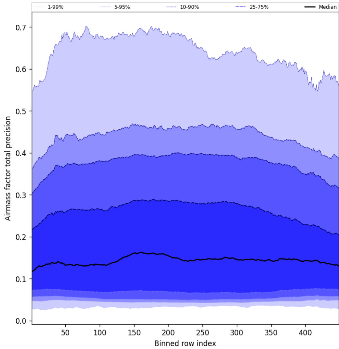
Figure 53: Along track statistics of “Airmass factor total precision” for 2025-06-17 to 2025-06-17
