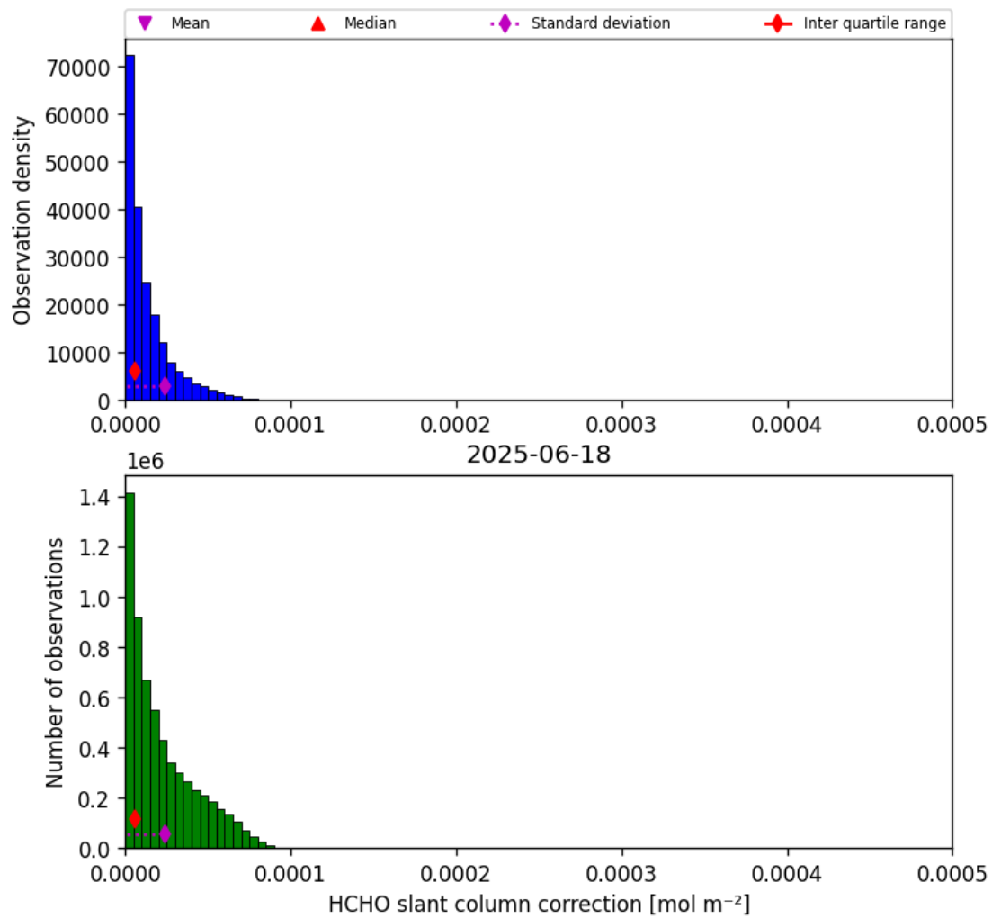
Figure 45: Histogram of “HCHO slant column correction” for 2025-06-18 to 2025-06-19
