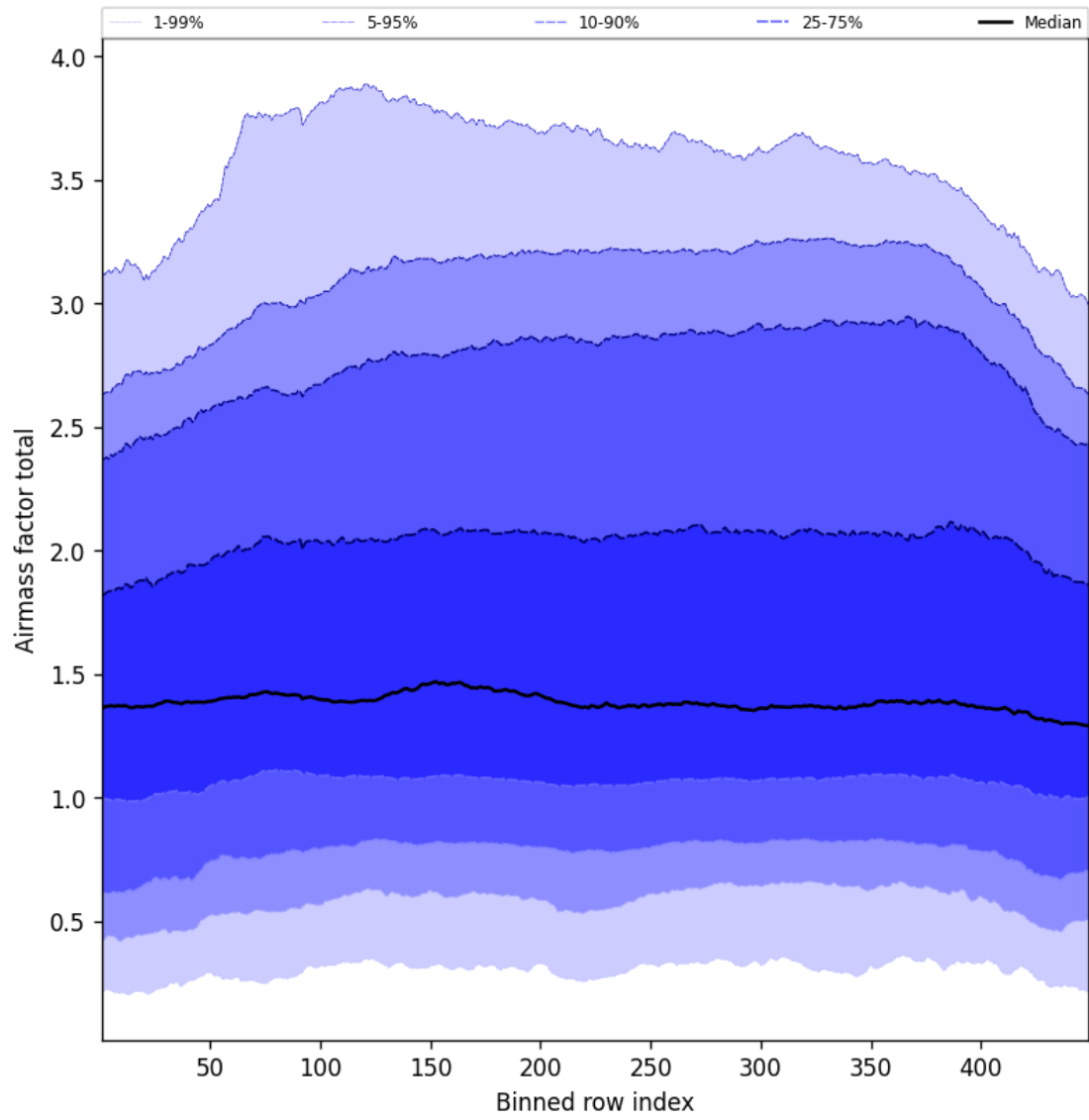
Figure 52: Along track statistics of “Airmass factor total” for 2025-06-18 to 2025-06-19
