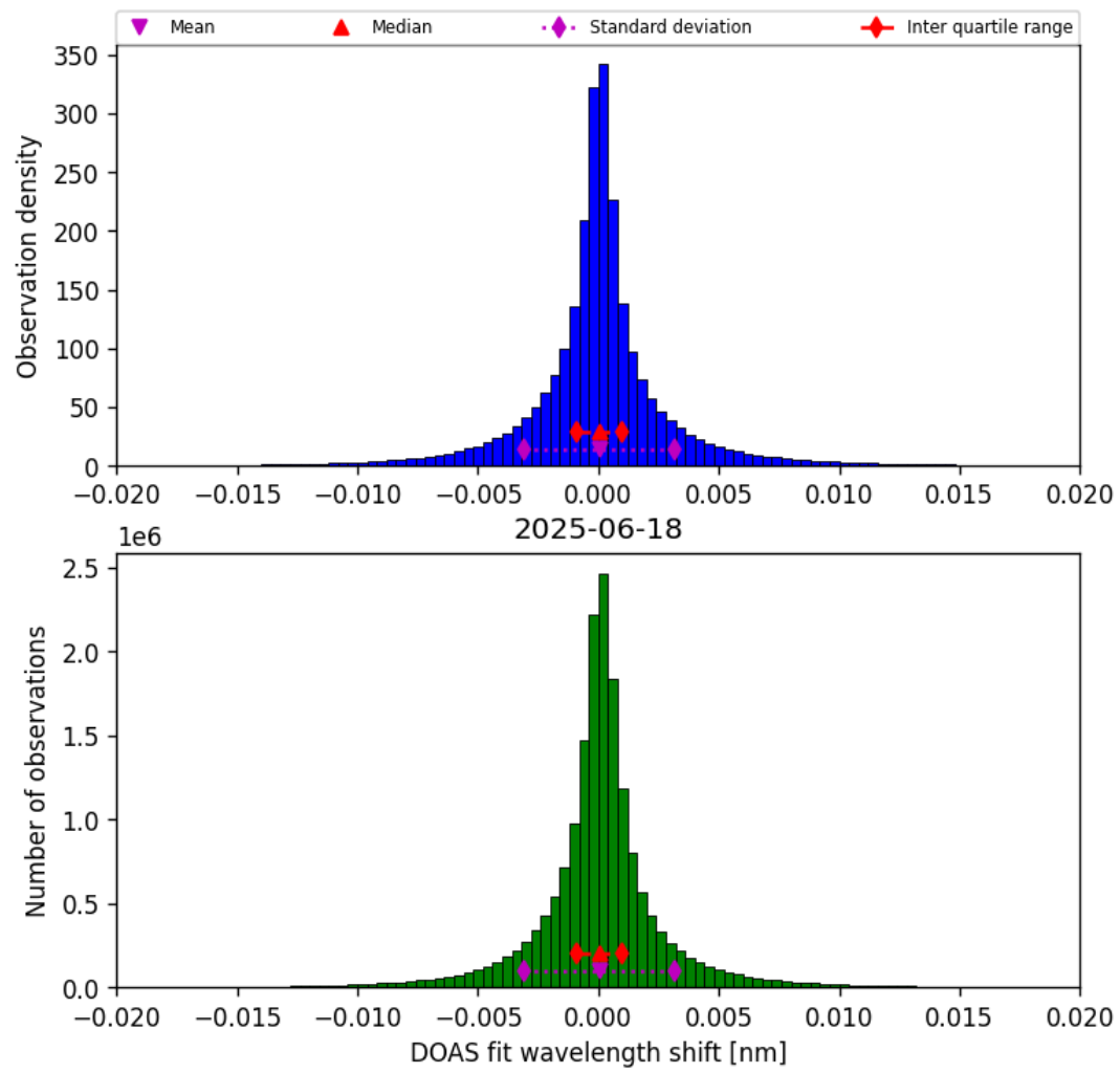
Figure 42: Histogram of “DOAS fit wavelength shift” for 2025-06-18 to 2025-06-19
