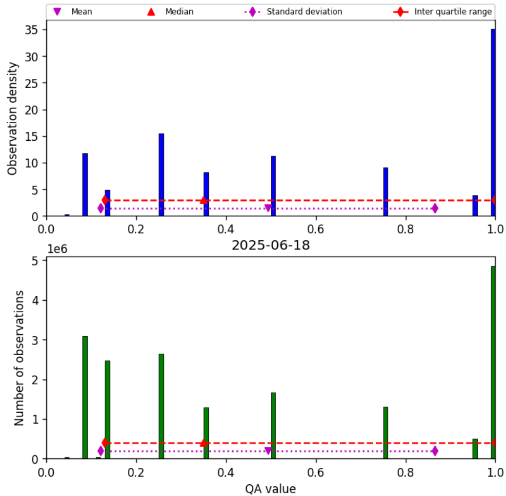
Figure 32: Histogram of “QA value” for 2025-06-18 to 2025-06-19
