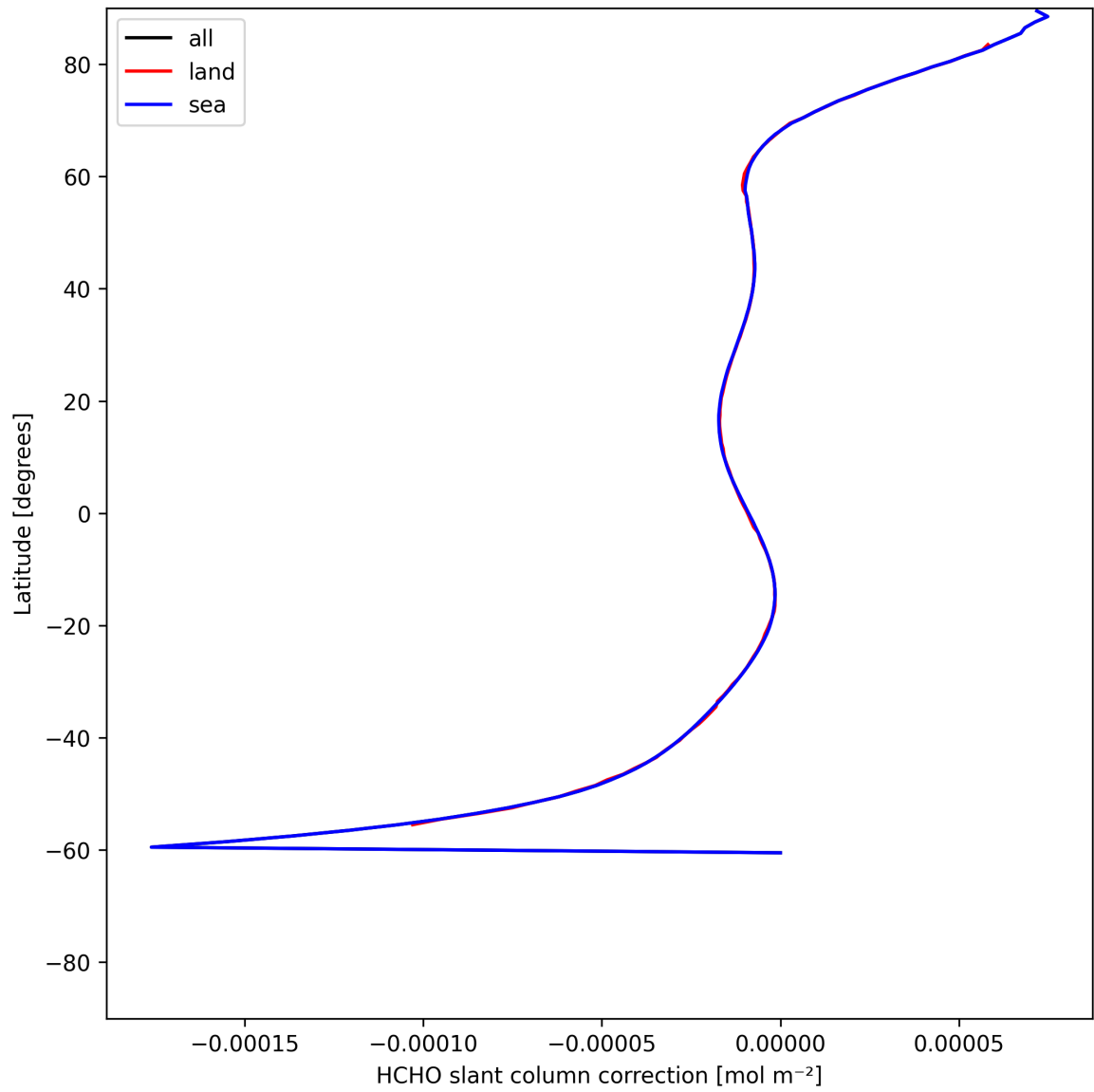
Figure 31: Zonal average of “HCHO slant column correction” for 2025-06-18 to 2025-06-19.
