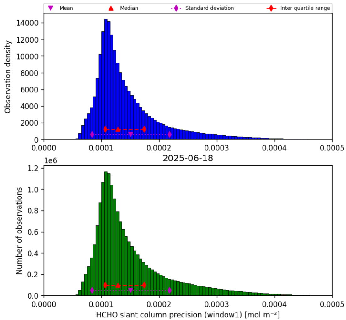
Figure 37: Histogram of “HCHO slant column precision (window1)” for 2025-06-18 to 2025-06-19
