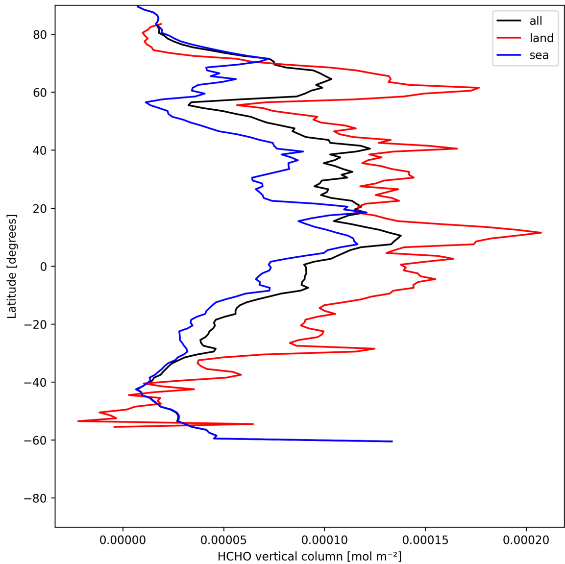
Figure 19: Zonal average of “HCHO vertical column” for 2025-06-18 to 2025-06-19.
