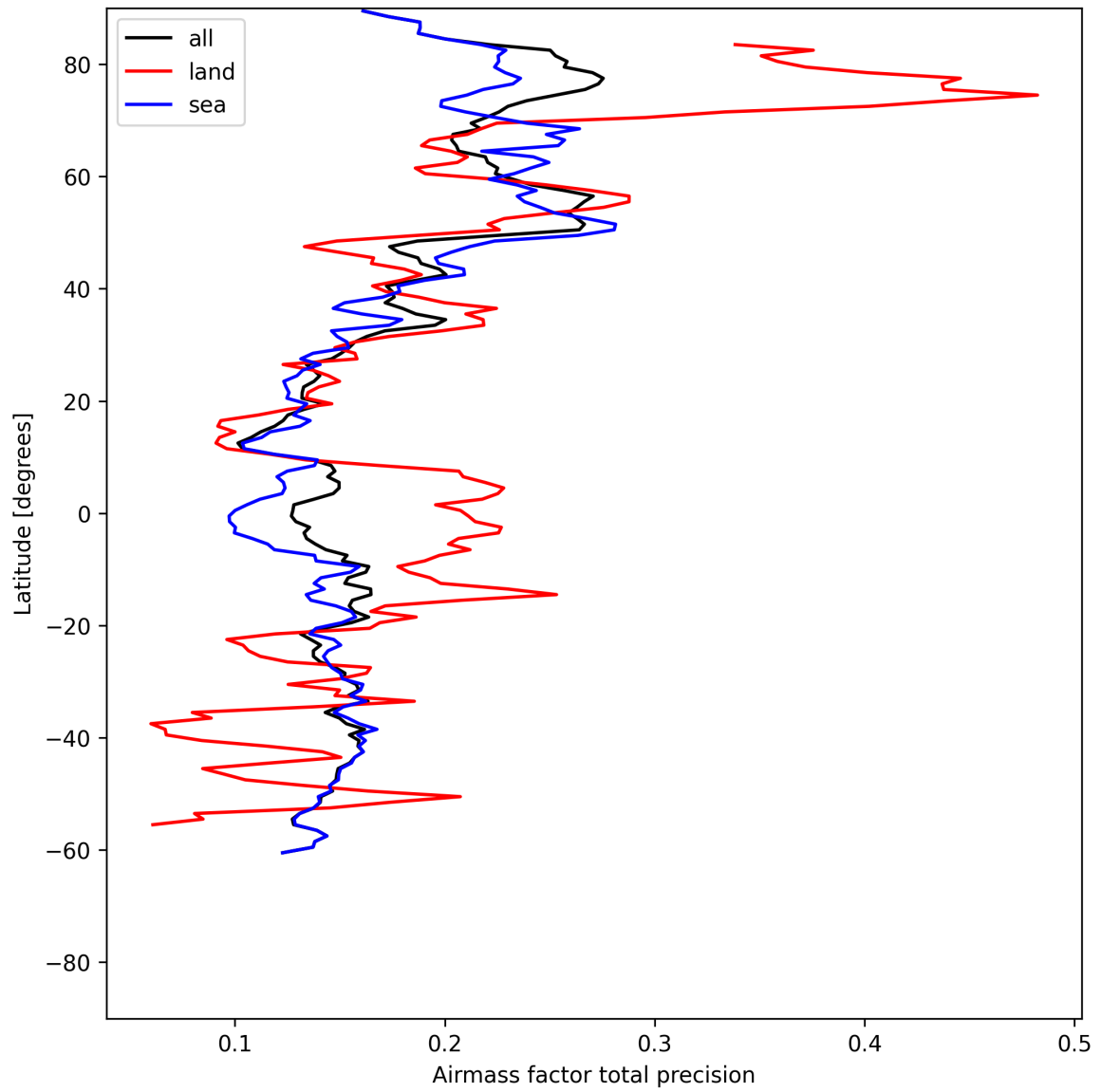
Figure 25: Zonal average of “Airmass factor total precision” for 2025-06-18 to 2025-06-19.
