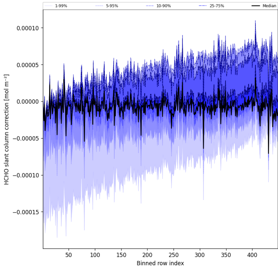
Figure 59: Along track statistics of “HCHO slant column correction” for 2025-06-18 to 2025-06-19
