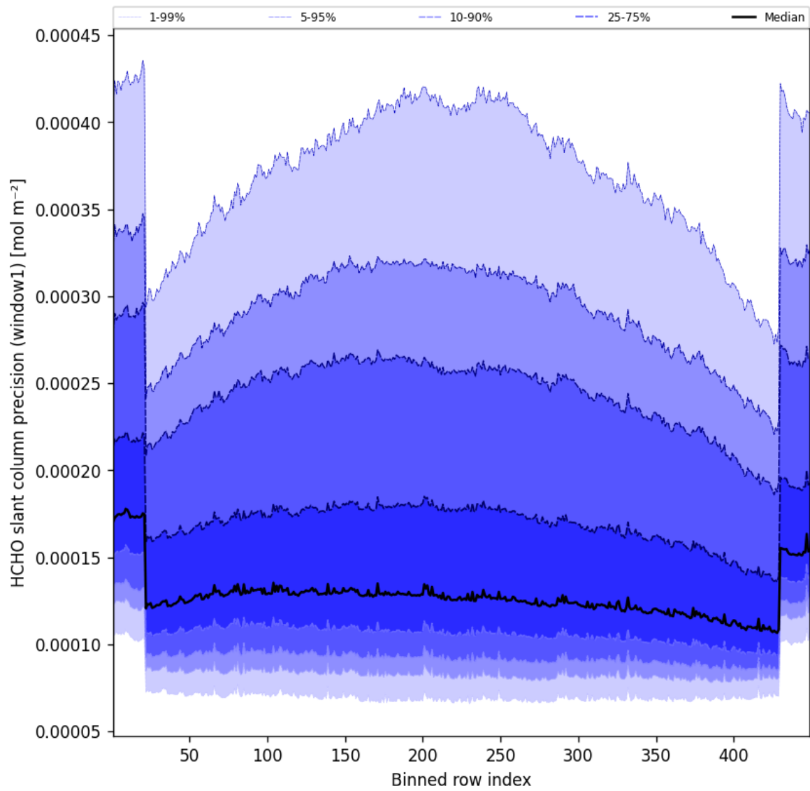
Figure 51: Along track statistics of “HCHO slant column precision (window1)” for 2025-06-18 to 2025-06-19
