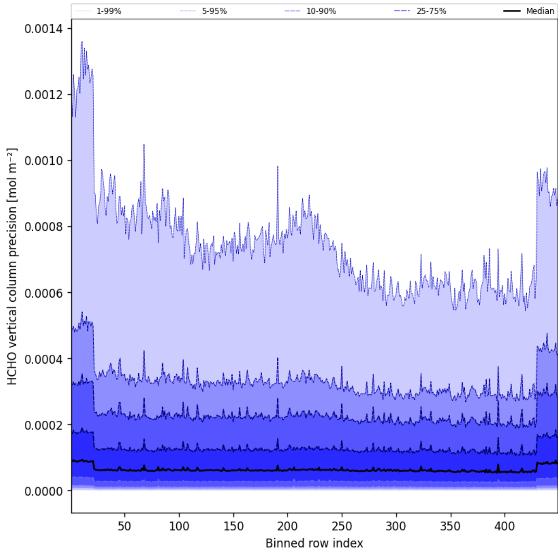
Figure 48: Along track statistics of “HCHO vertical column precision” for 2025-06-18 to 2025-06-19
