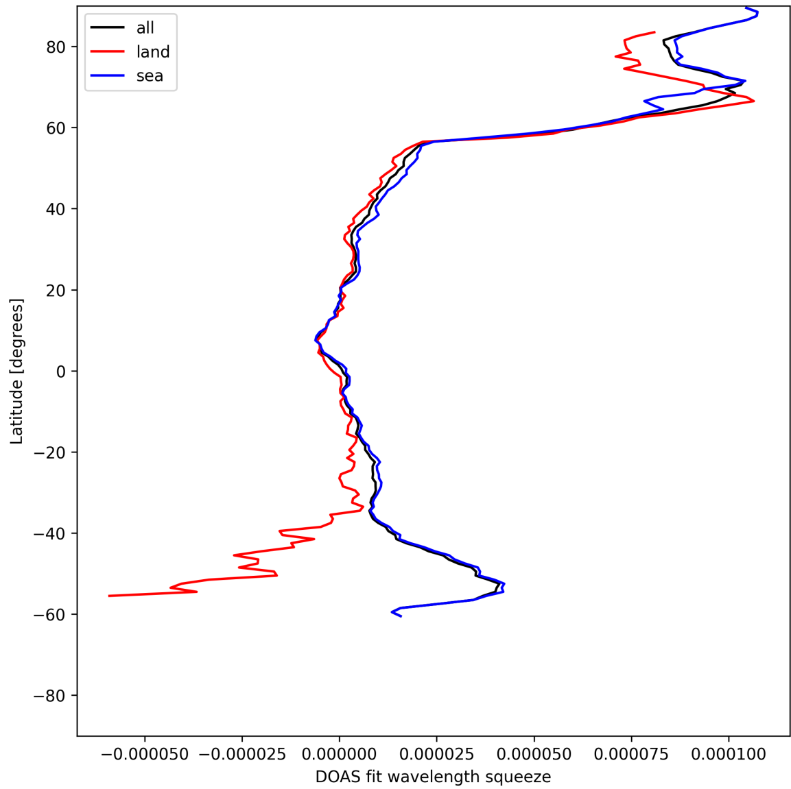
Figure 29: Zonal average of “DOAS fit wavelength squeeze” for 2025-06-18 to 2025-06-19.
