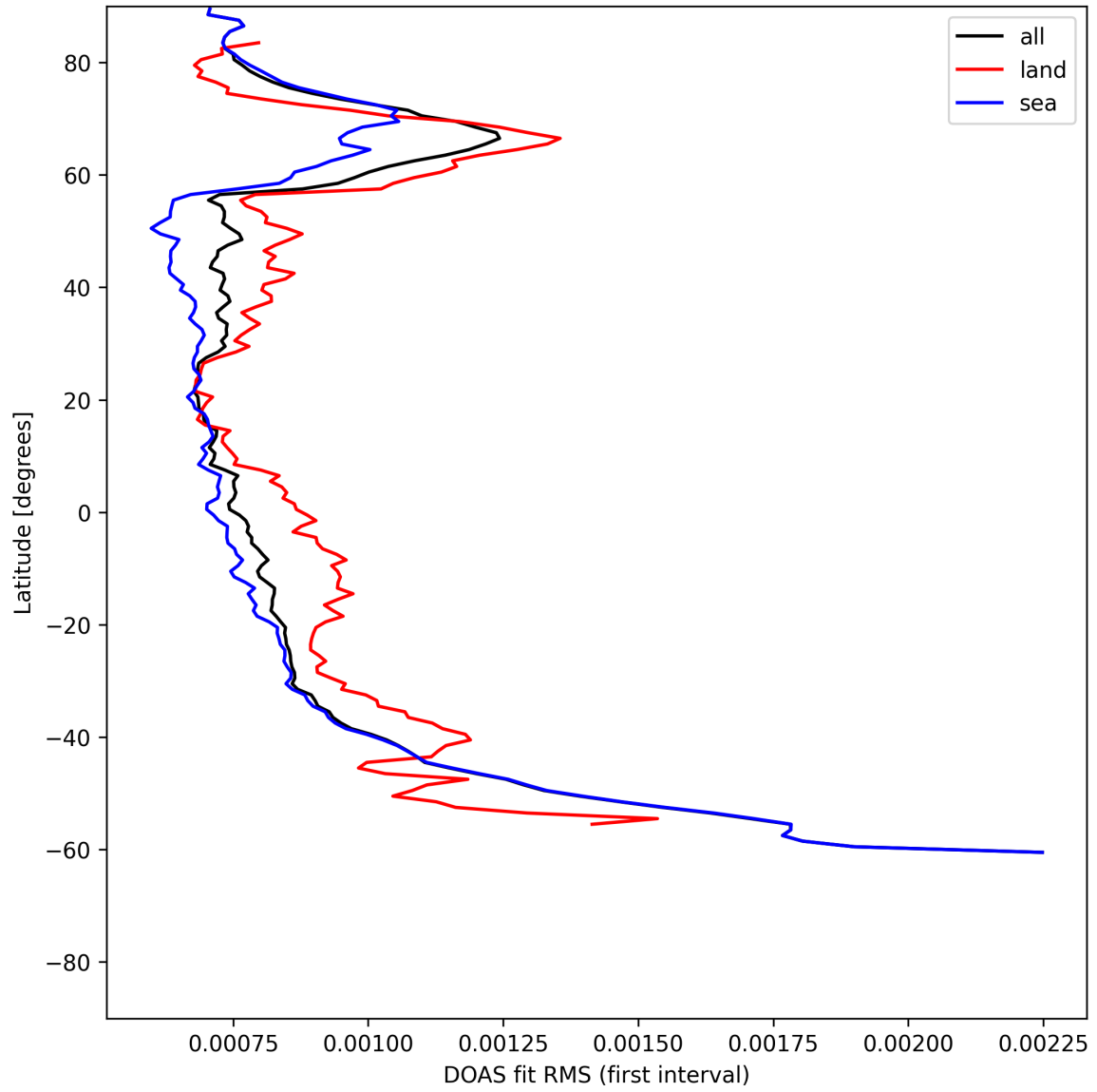
Figure 30: Zonal average of "DOAS fit RMS (first interval)" for 2025-06-18 to 2025-06-19.
