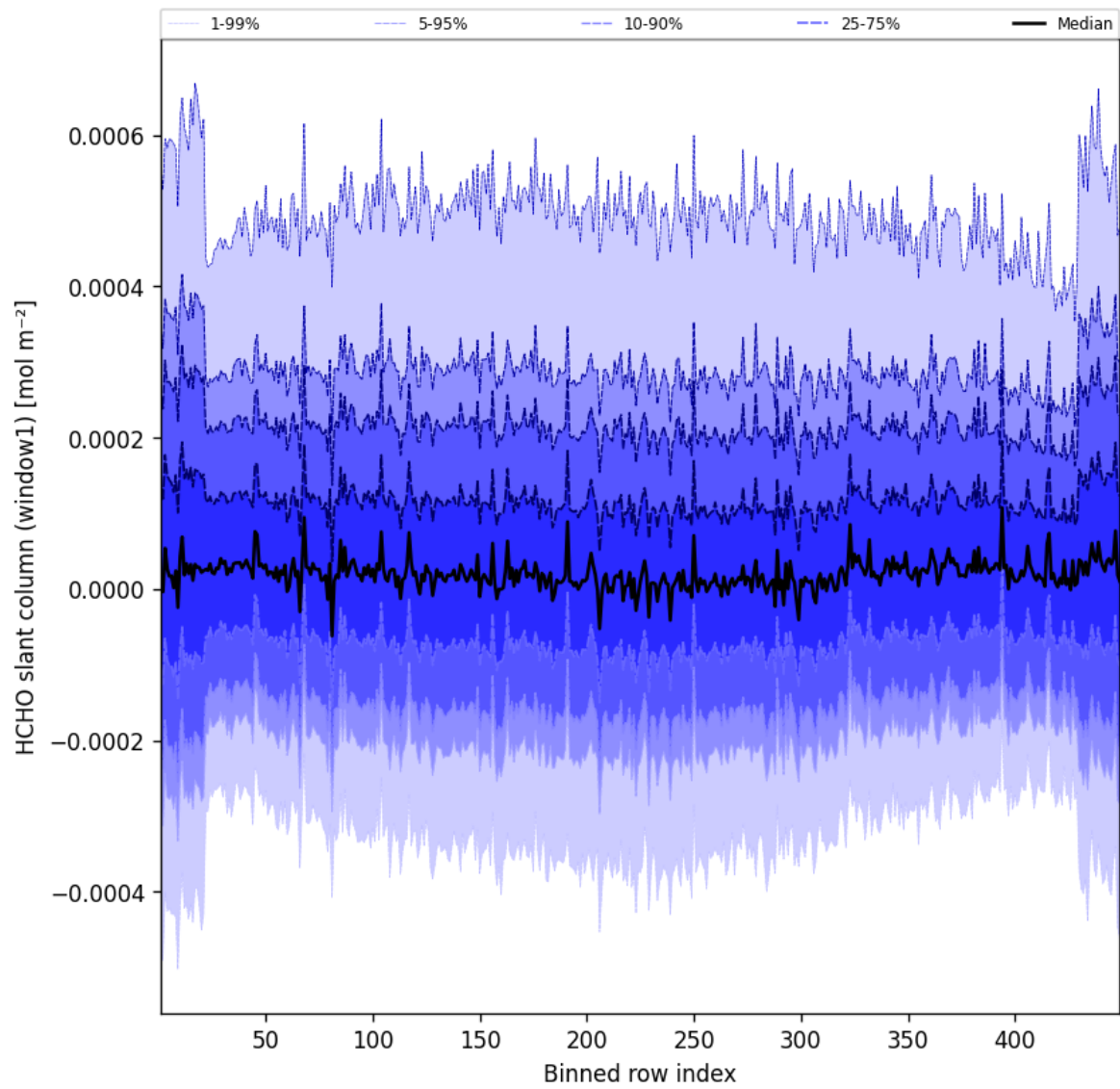
Figure 50: Along track statistics of “HCHO slant column (window1)” for 2025-06-18 to 2025-06-19
