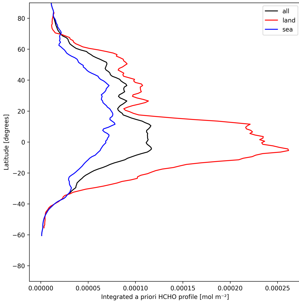
Figure 27: Zonal average of “Integrated a priori HCHO profile” for 2025-06-18 to 2025-06-19.
