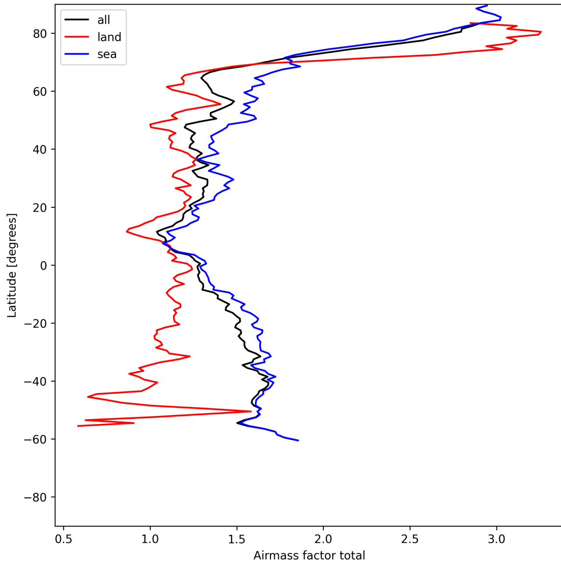
Figure 24: Zonal average of “Airmass factor total” for 2025-06-18 to 2025-06-19.
