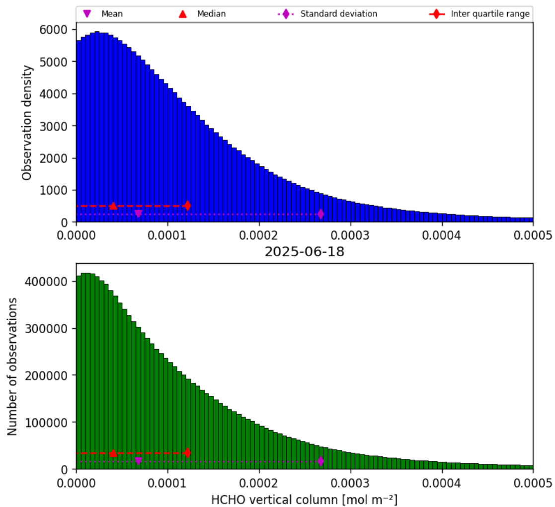
Figure 33: Histogram of “HCHO vertical column” for 2025-06-18 to 2025-06-19
