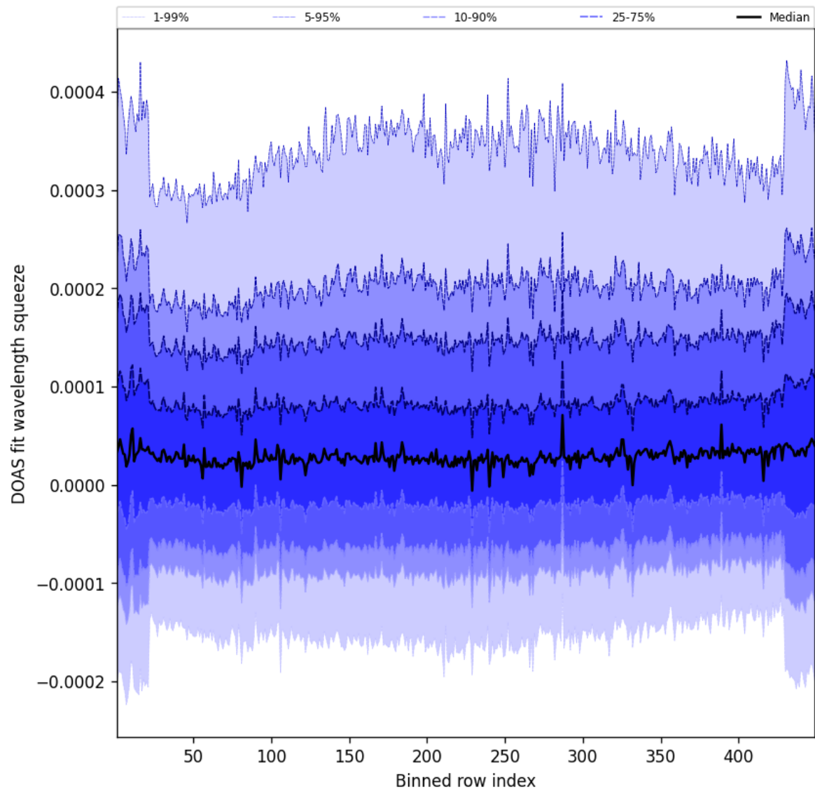
Figure 57: Along track statistics of “DOAS fit wavelength squeeze” for 2025-06-18 to 2025-06-19
