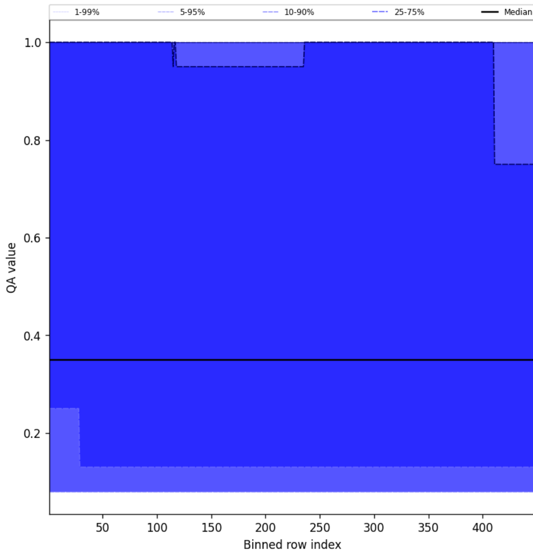
Figure 46: Along track statistics of “QA value” for 2025-06-18 to 2025-06-19
