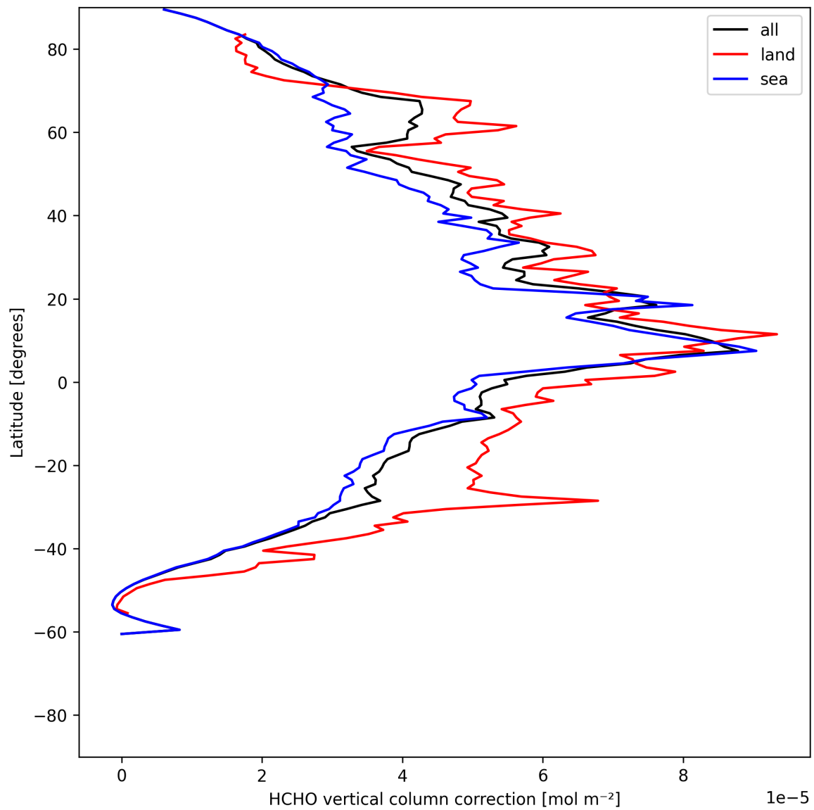
Figure 21: Zonal average of “HCHO vertical column correction” for 2025-06-18 to 2025-06-19.
