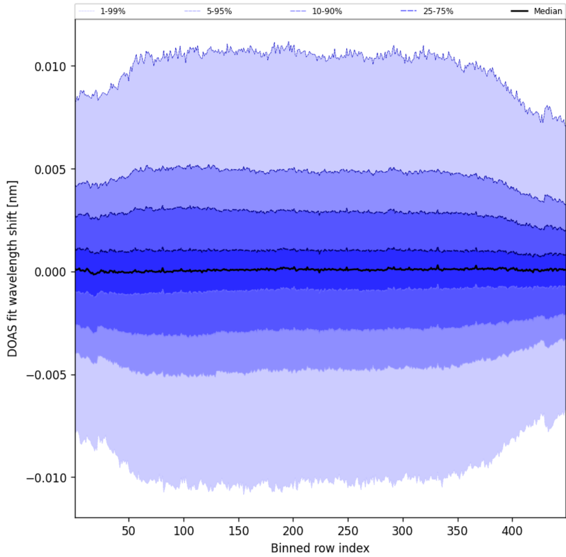
Figure 56: Along track statistics of “DOAS fit wavelength shift” for 2025-06-18 to 2025-06-19
