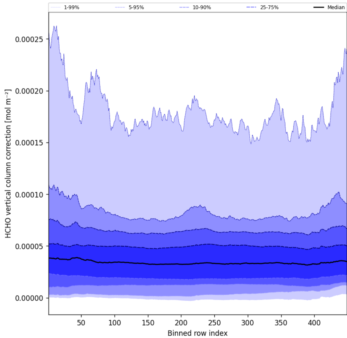
Figure 49: Along track statistics of “HCHO vertical column correction” for 2025-06-18 to 2025-06-19
