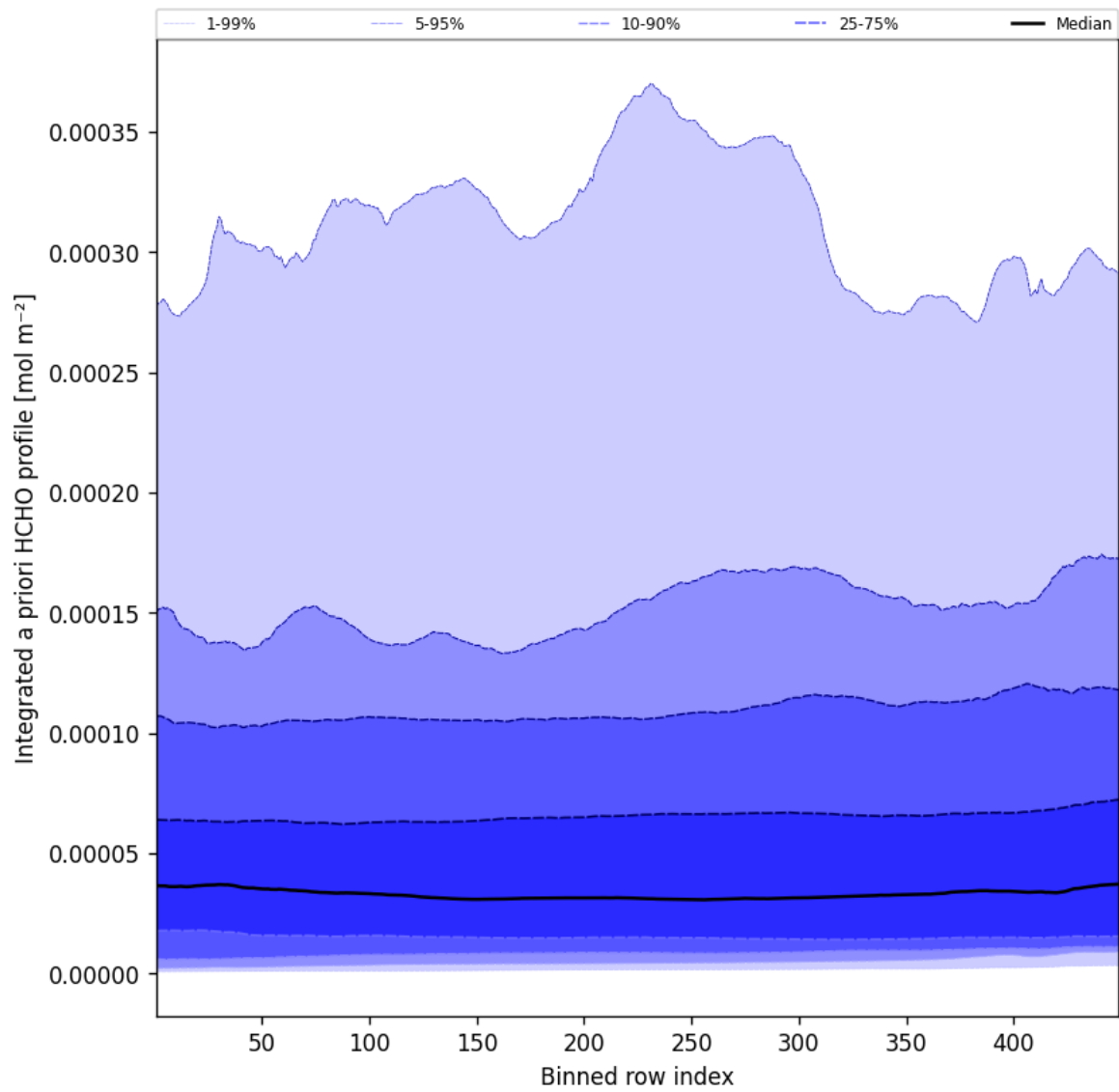
Figure 55: Along track statistics of “Integrated a priori HCHO profile” for 2025-06-18 to 2025-06-19
