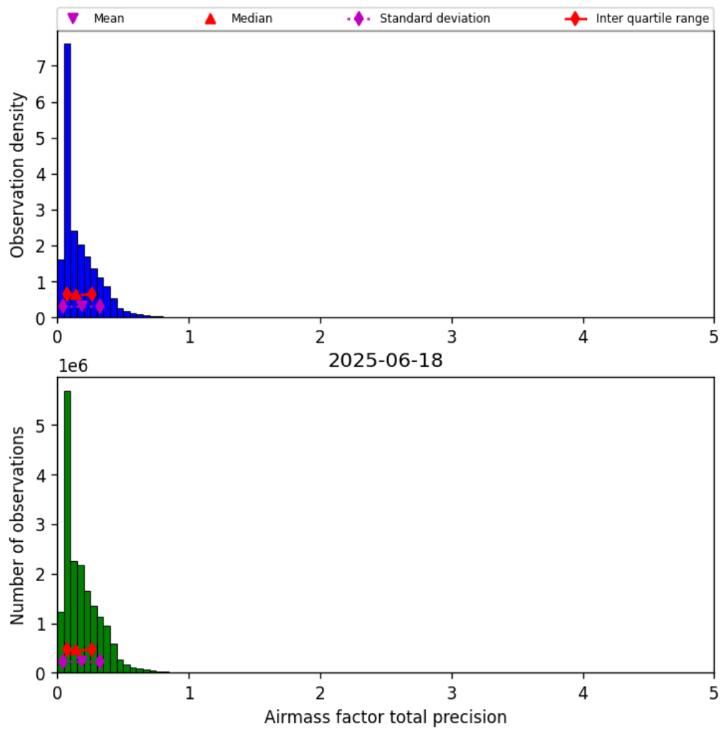
Figure 39: Histogram of “Airmass factor total precision” for 2025-06-18 to 2025-06-19
