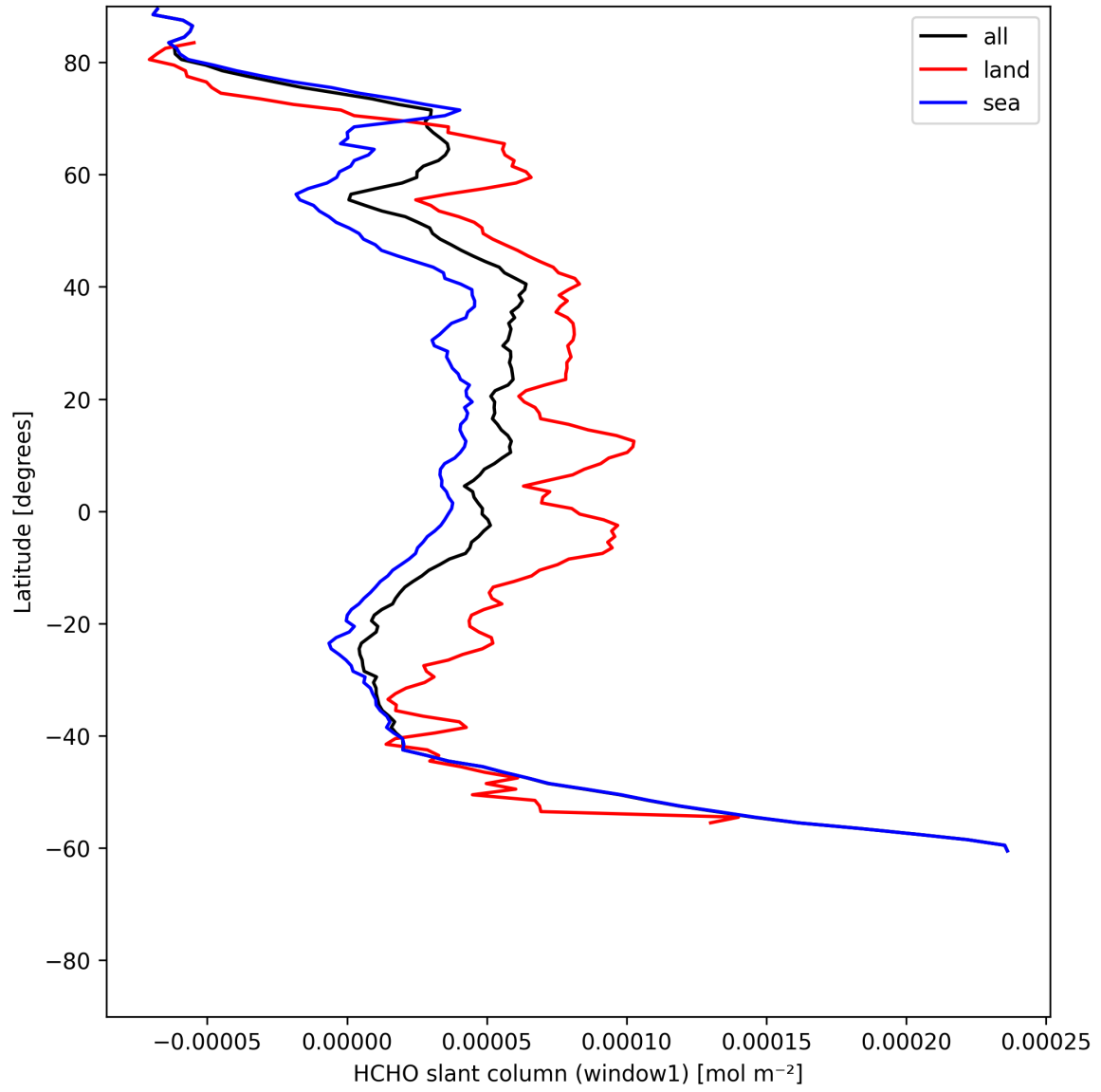
Figure 22: Zonal average of “HCHO slant column (window1)” for 2025-06-18 to 2025-06-19.
