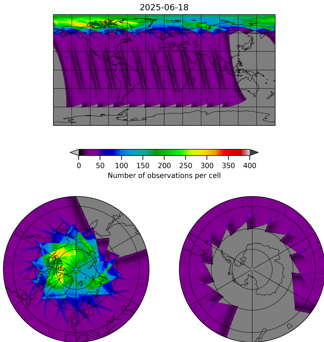
Figure 17: Map of the number of observations for 2025-06-18 to 2025-06-19
