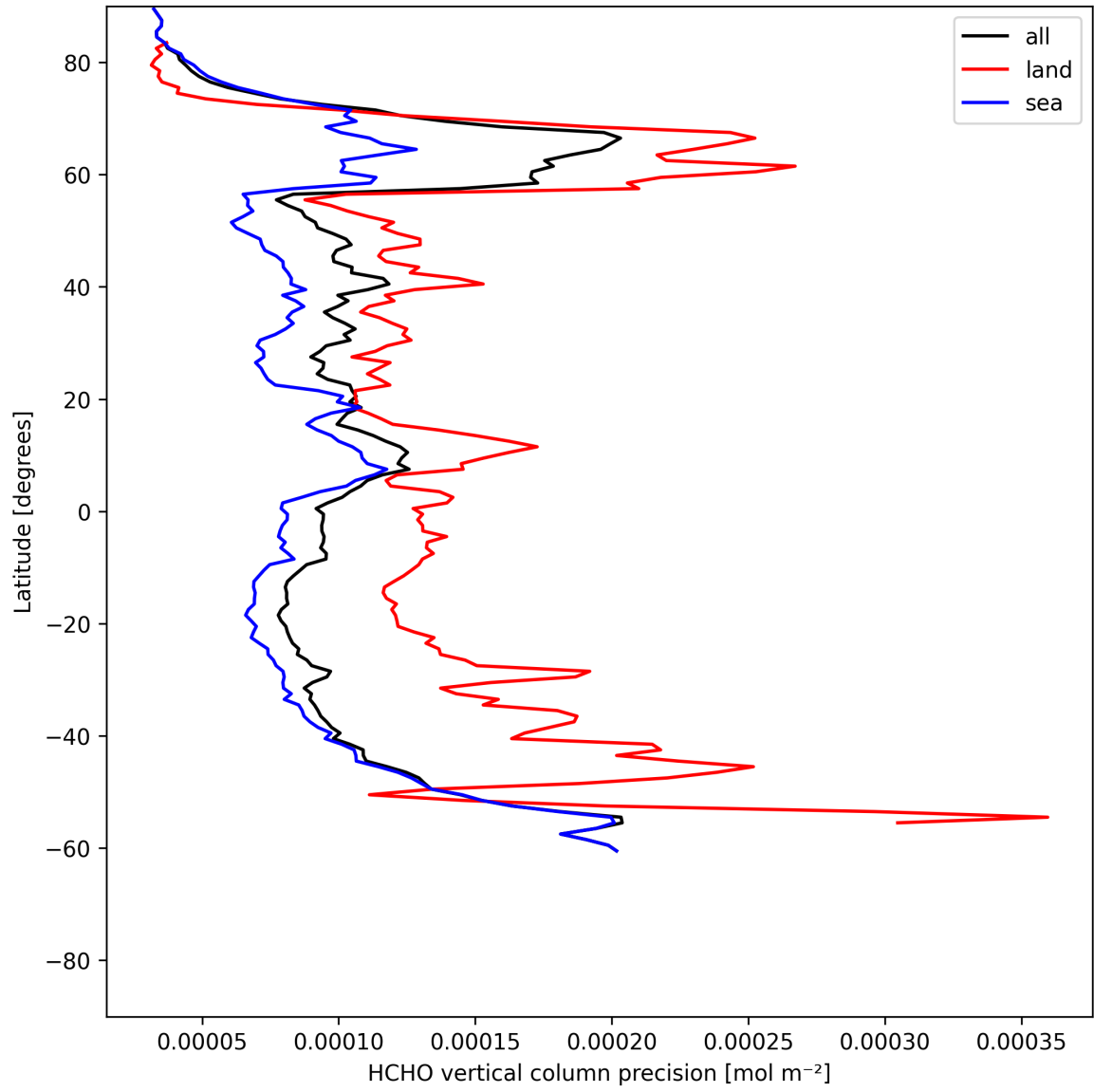
Figure 20: Zonal average of “HCHO vertical column precision” for 2025-06-18 to 2025-06-19.
