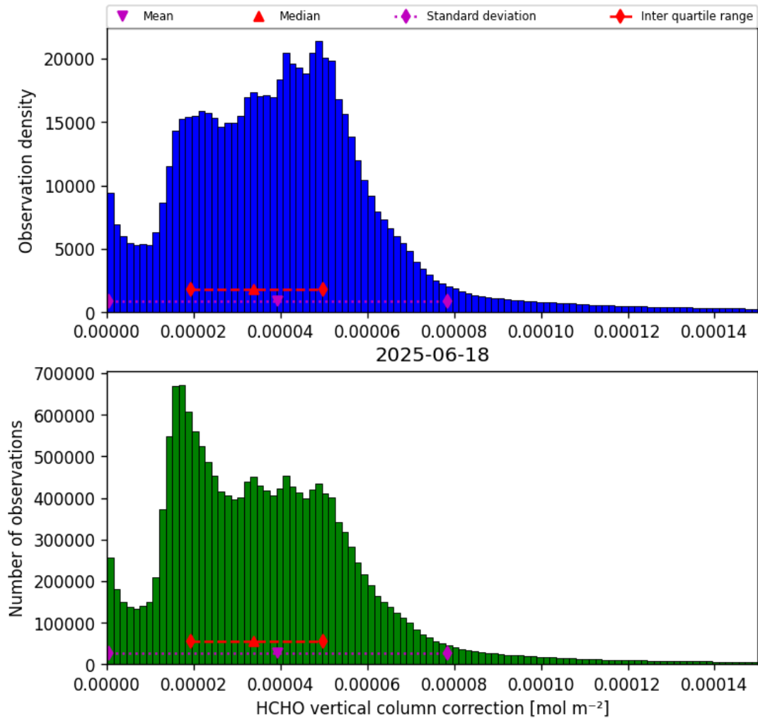
Figure 35: Histogram of “HCHO vertical column correction” for 2025-06-18 to 2025-06-19
