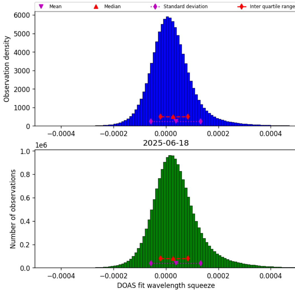
Figure 43: Histogram of “DOAS fit wavelength squeeze” for 2025-06-18 to 2025-06-19
