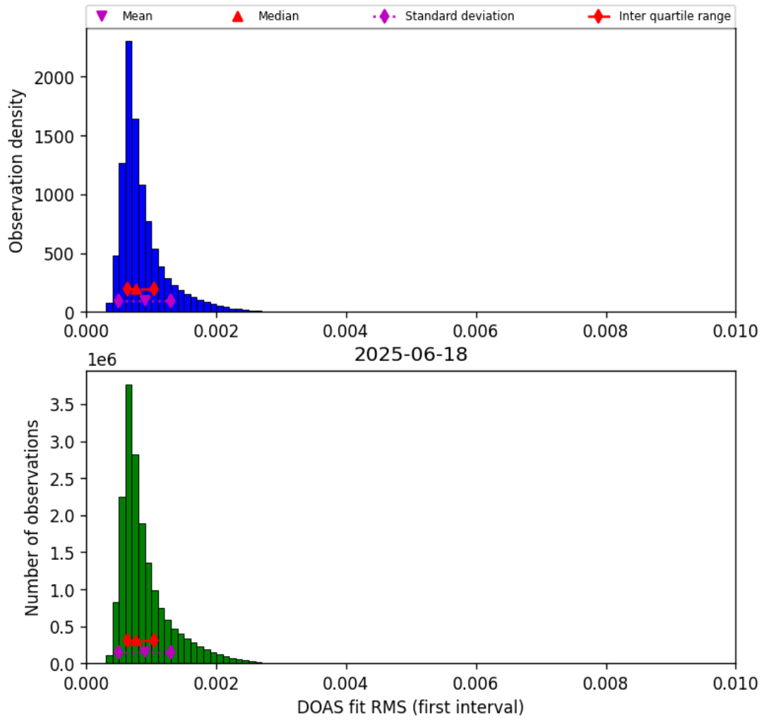
Figure 44: Histogram of “DOAS fit RMS (first interval)” for 2025-06-18 to 2025-06-19
