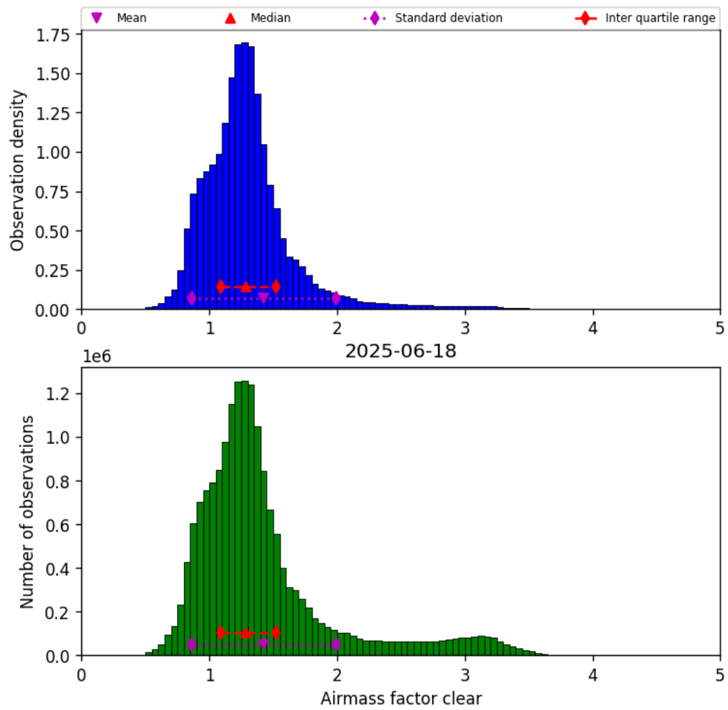
Figure 40: Histogram of “Airmass factor clear” for 2025-06-18 to 2025-06-19
