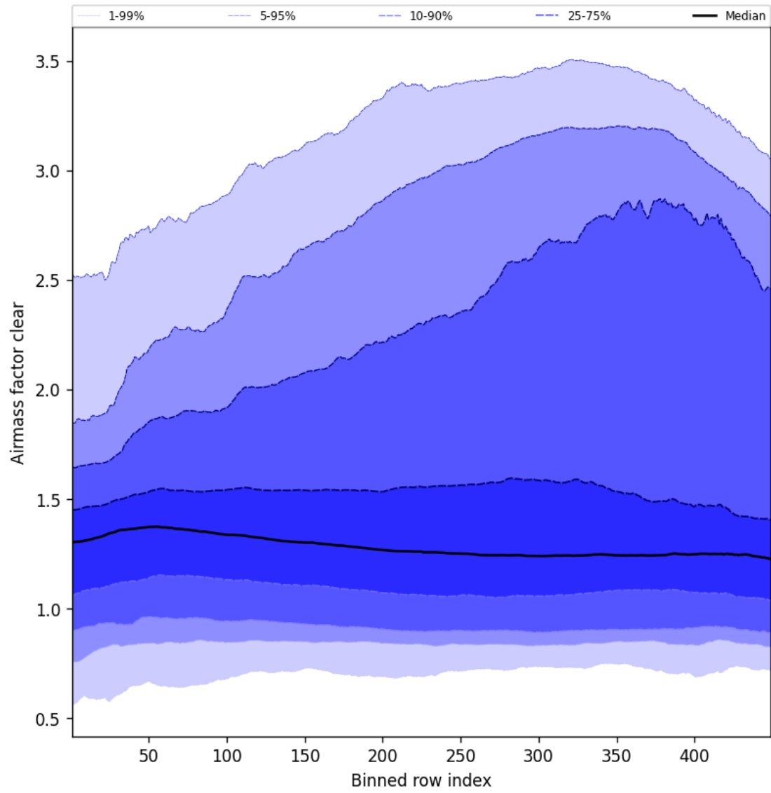
Figure 54: Along track statistics of “Airmass factor clear” for 2025-06-18 to 2025-06-19
