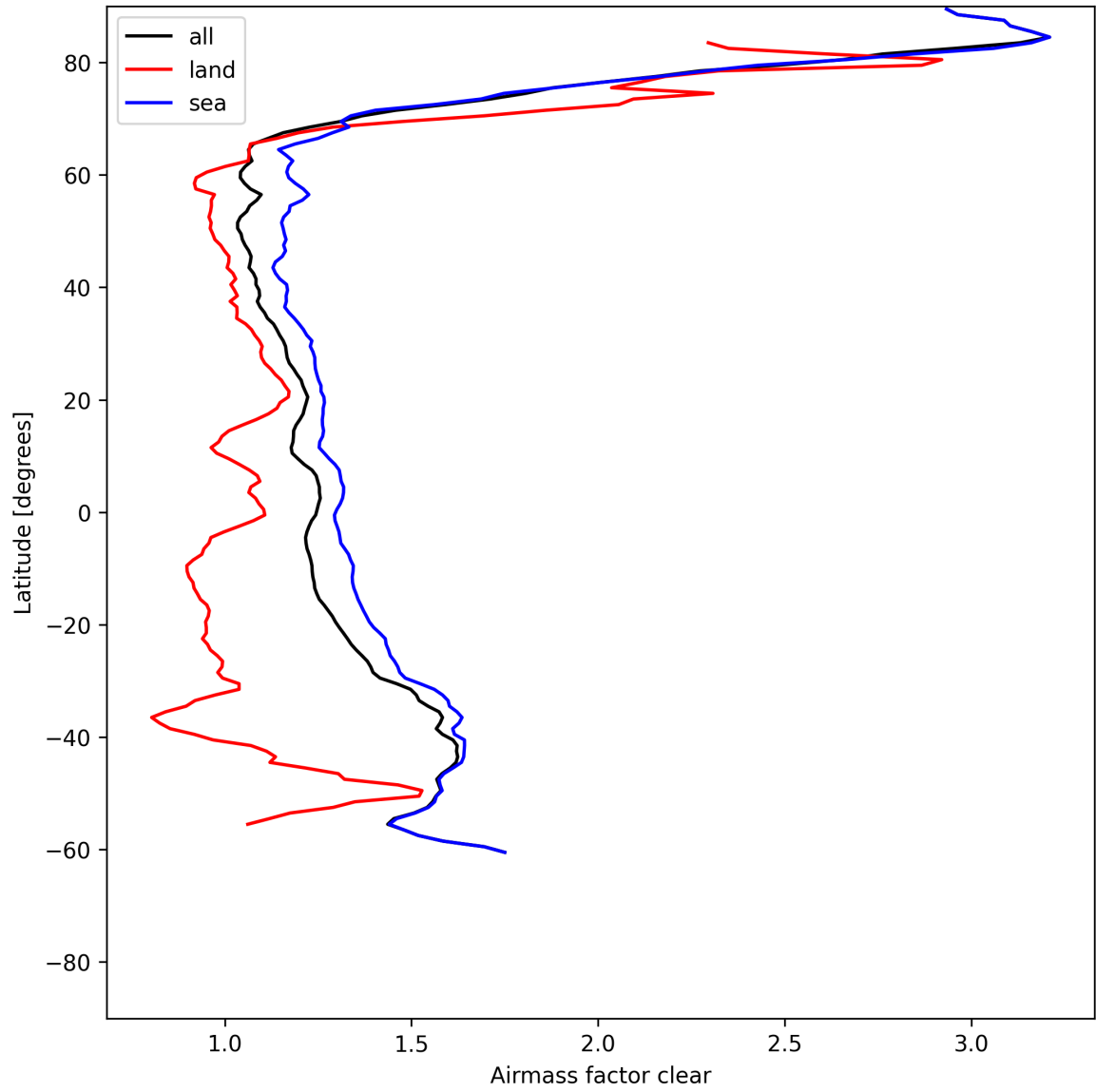
Figure 26: Zonal average of “Airmass factor clear” for 2025-06-18 to 2025-06-19.
