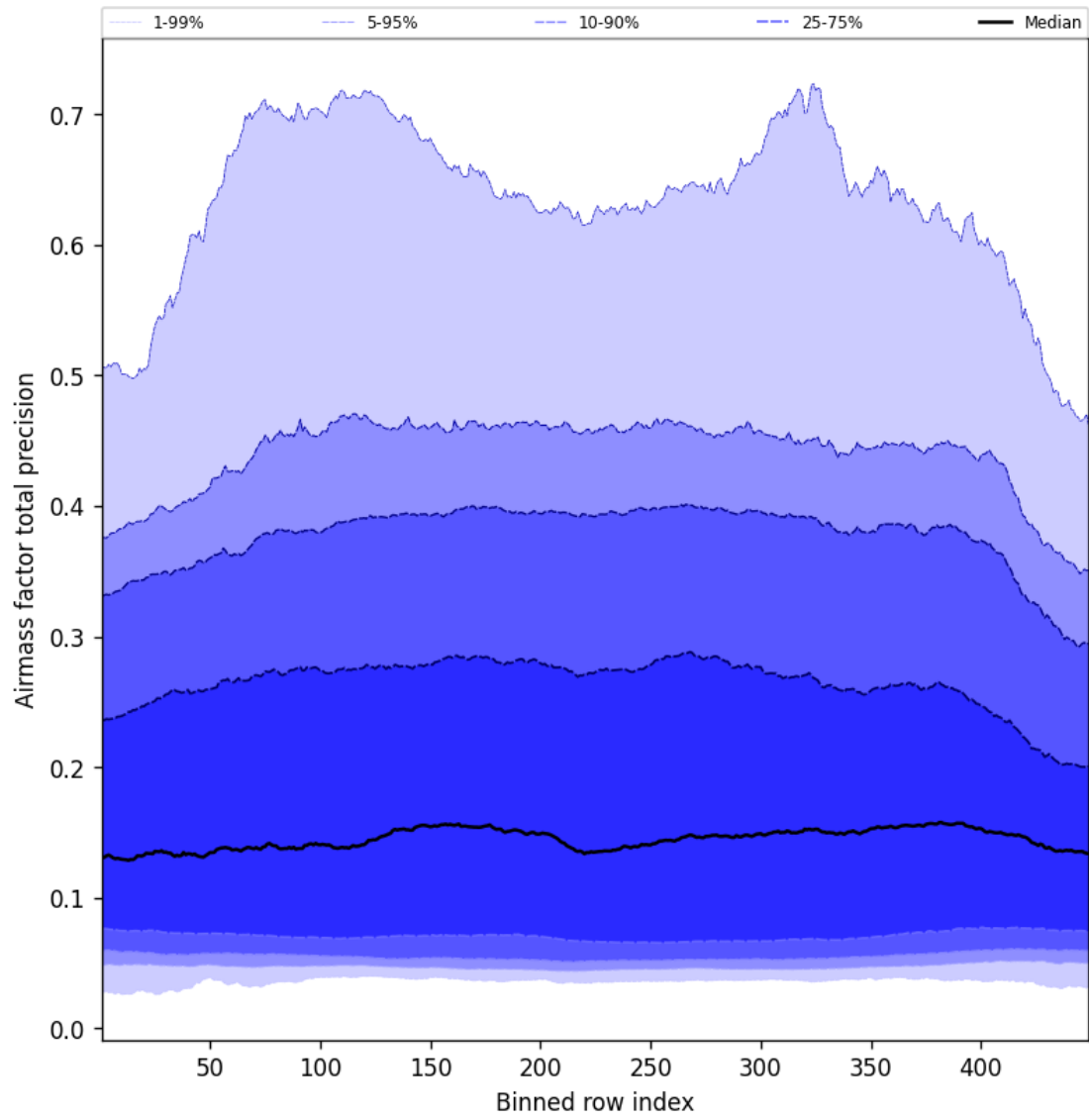
Figure 53: Along track statistics of “Airmass factor total precision” for 2025-06-18 to 2025-06-19
