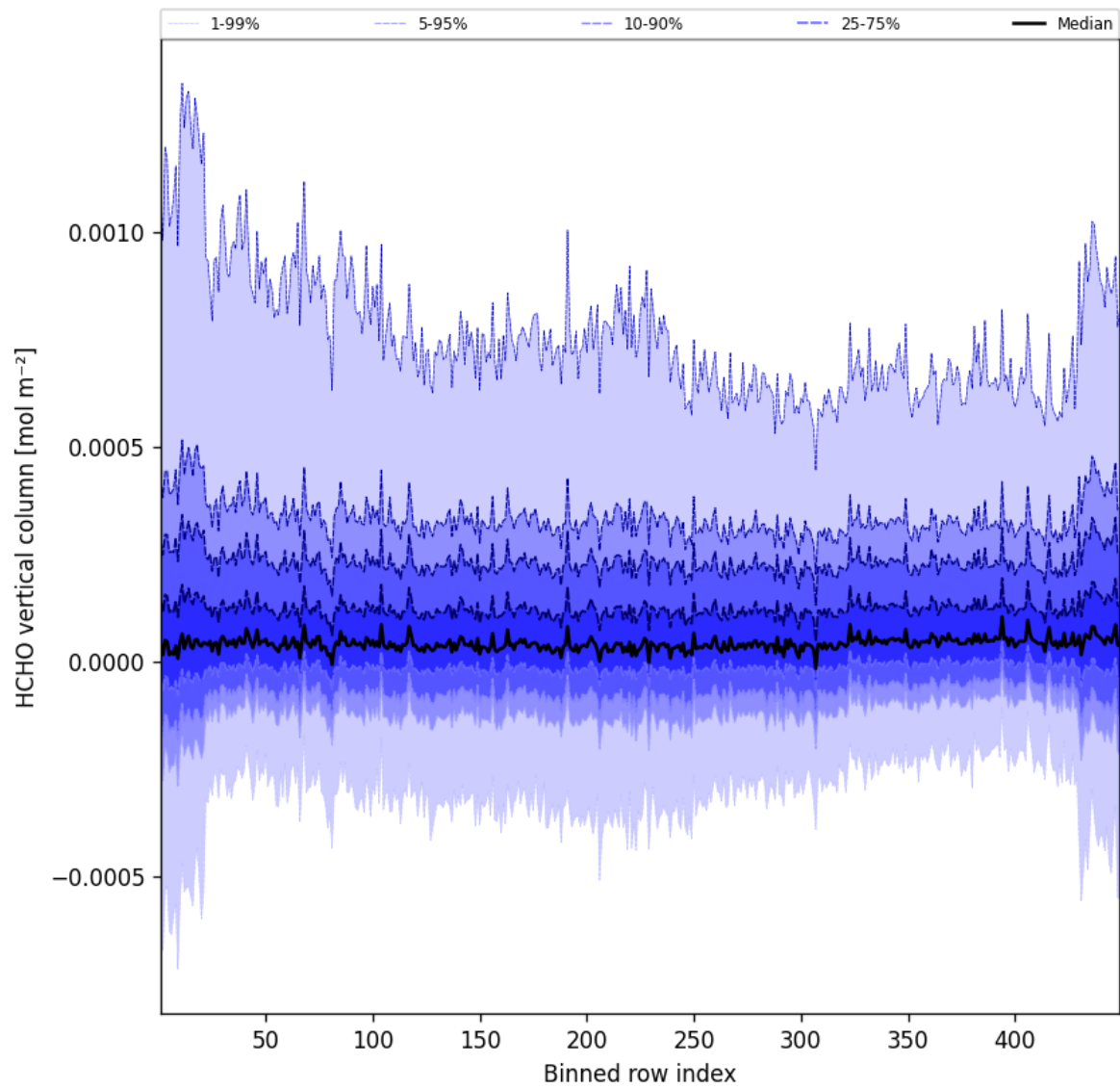
Figure 47: Along track statistics of “HCHO vertical column” for 2025-06-18 to 2025-06-19
