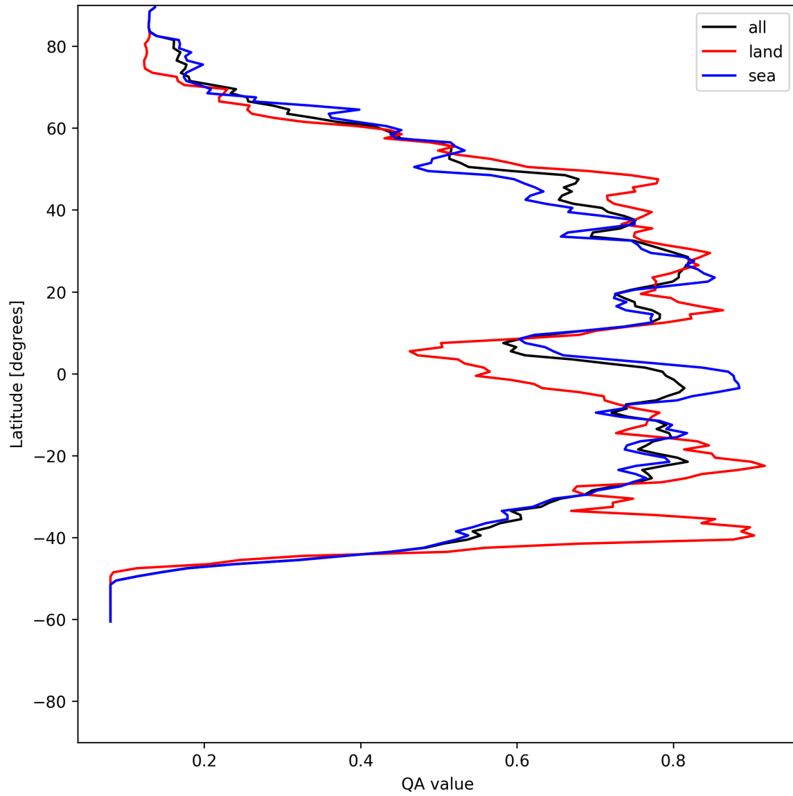
Figure 18: Zonal average of “QA value” for 2025-06-18 to 2025-06-19.
