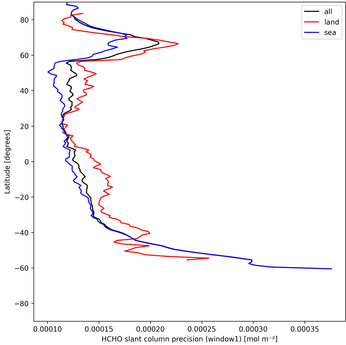
Figure 23: Zonal average of “HCHO slant column precision (window1)” for 2025-06-18 to 2025-06-19.
