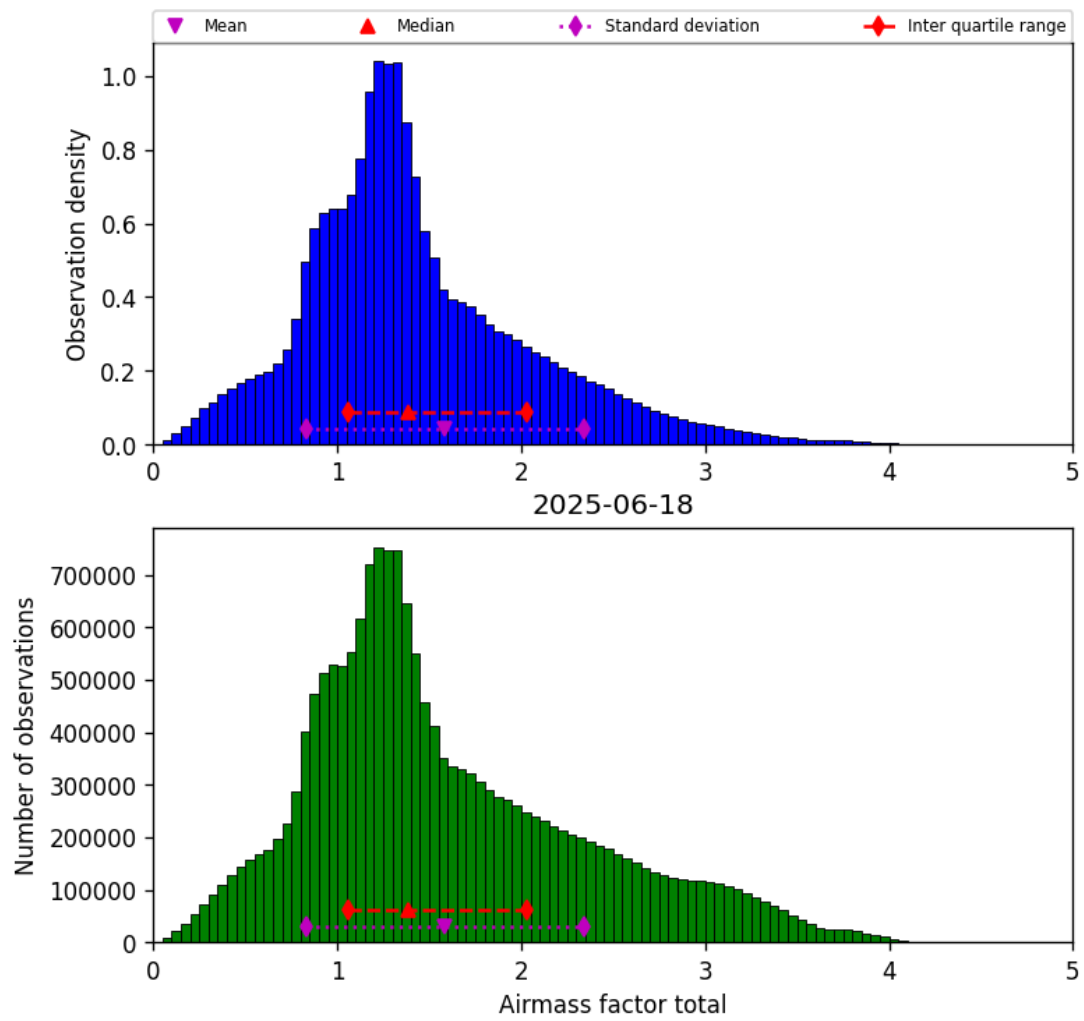
Figure 38: Histogram of “Airmass factor total” for 2025-06-18 to 2025-06-19
