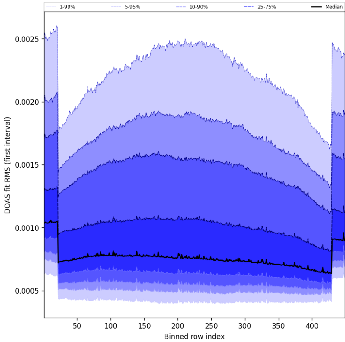
Figure 58: Along track statistics of “DOAS fit RMS (first interval)” for 2025-06-18 to 2025-06-19
