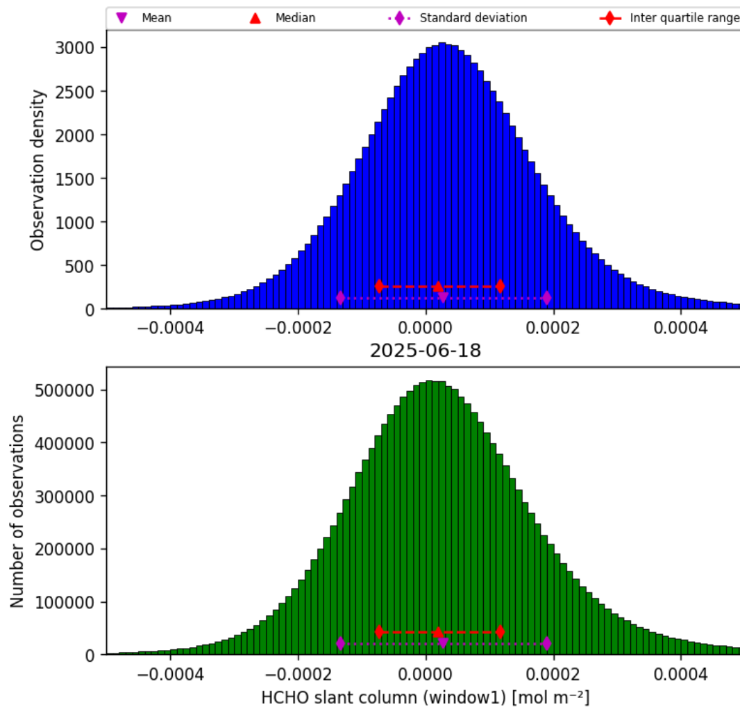
Figure 36: Histogram of “HCHO slant column (window1)” for 2025-06-18 to 2025-06-19
