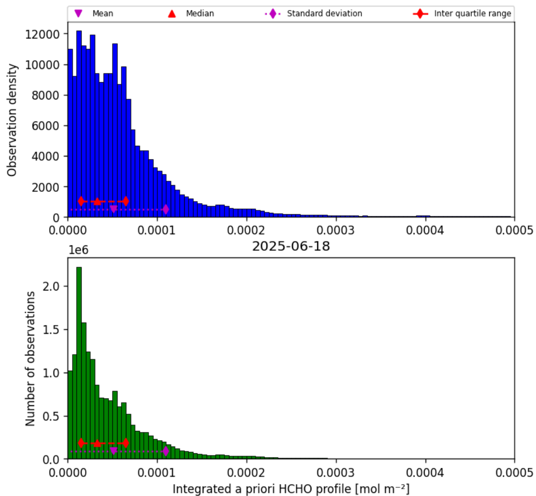
Figure 41: Histogram of “Integrated a priori HCHO profile” for 2025-06-18 to 2025-06-19
