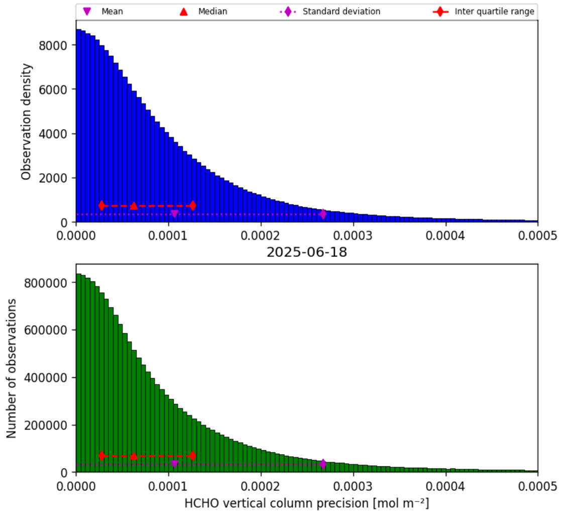
Figure 34: Histogram of “HCHO vertical column precision” for 2025-06-18 to 2025-06-19
