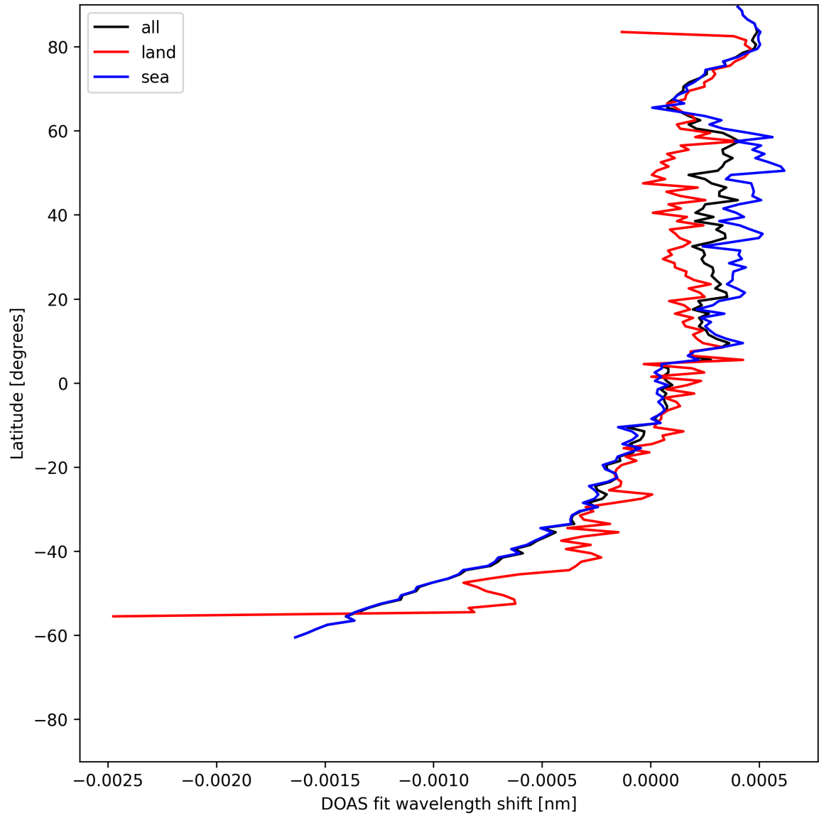
Figure 28: Zonal average of “DOAS fit wavelength shift” for 2025-06-18 to 2025-06-19.
