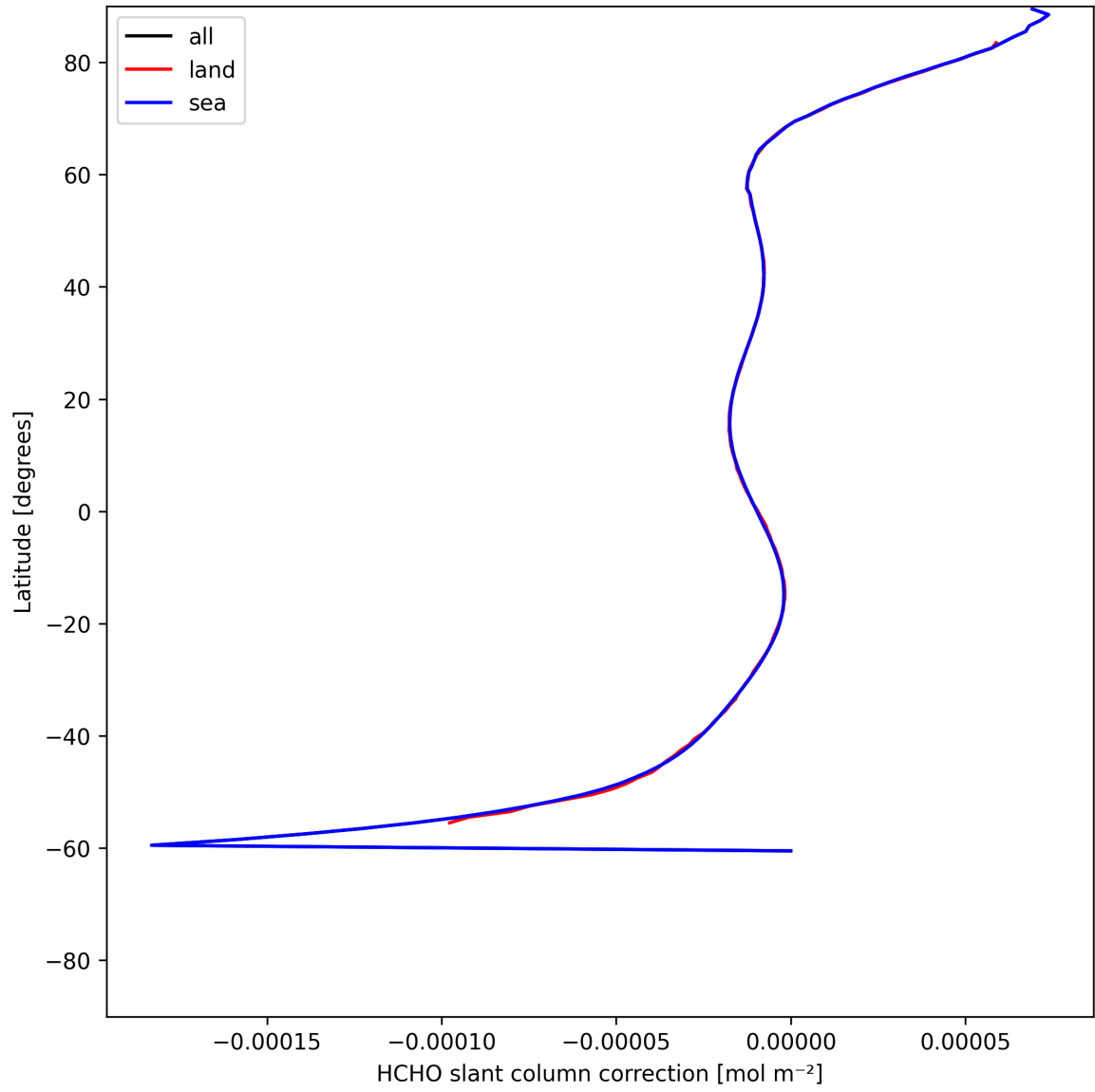
Figure 31: Zonal average of “HCHO slant column correction” for 2025-06-19 to 2025-06-20.
