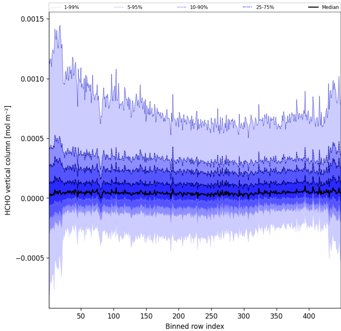
Figure 47: Along track statistics of “HCHO vertical column” for 2025-06-19 to 2025-06-20
