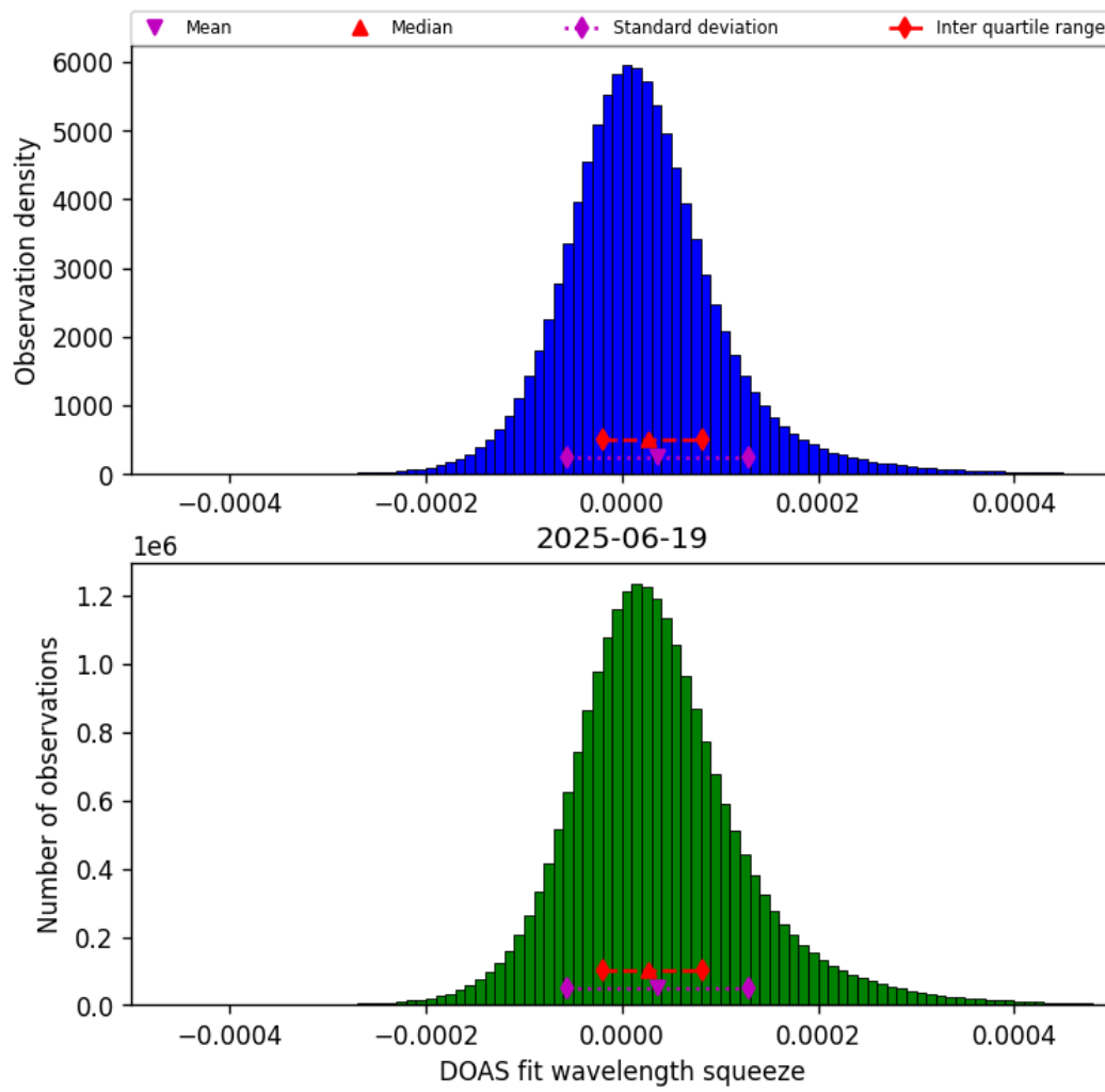
Figure 43: Histogram of “DOAS fit wavelength squeeze” for 2025-06-19 to 2025-06-20
