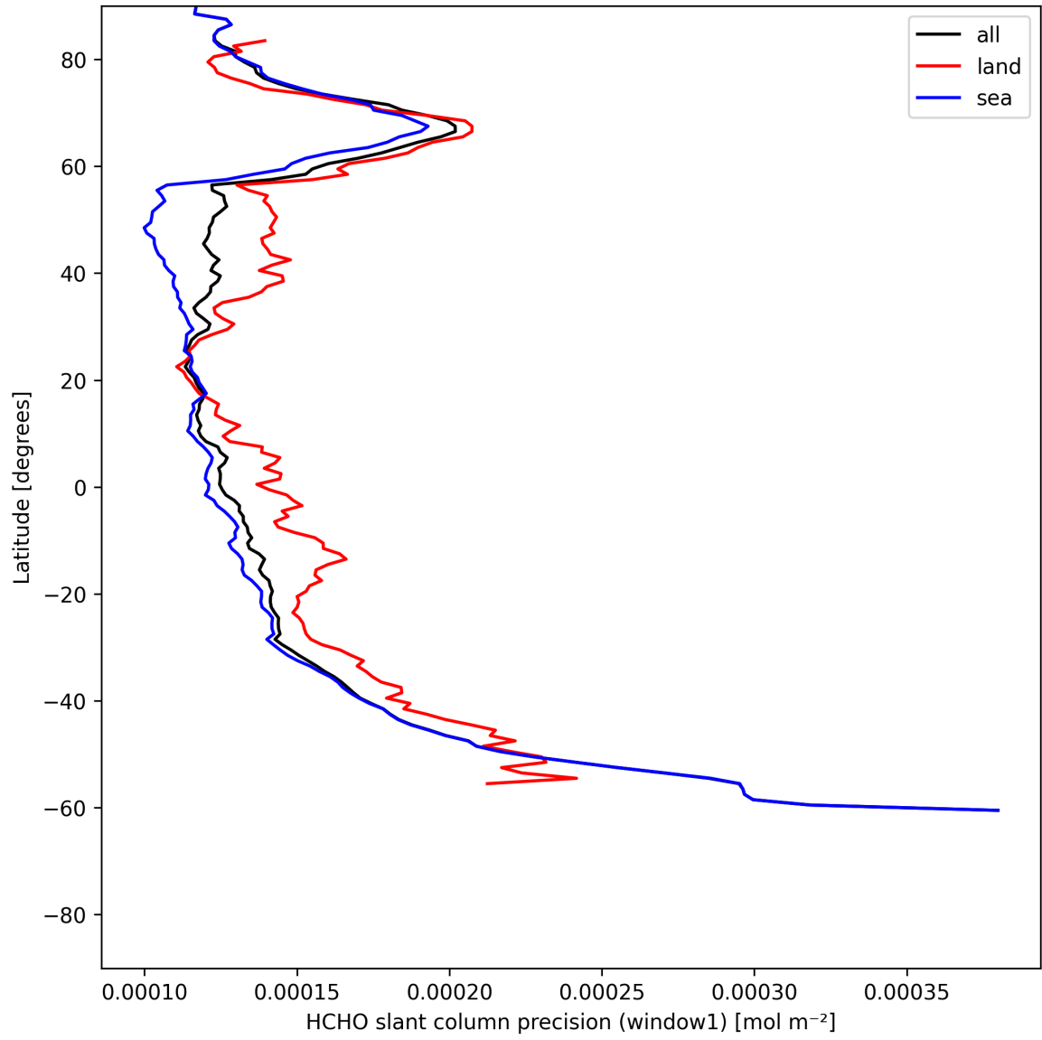
Figure 23: Zonal average of "HCHO slant column precision (window1)" for 2025-06-19 to 2025-06-20.
