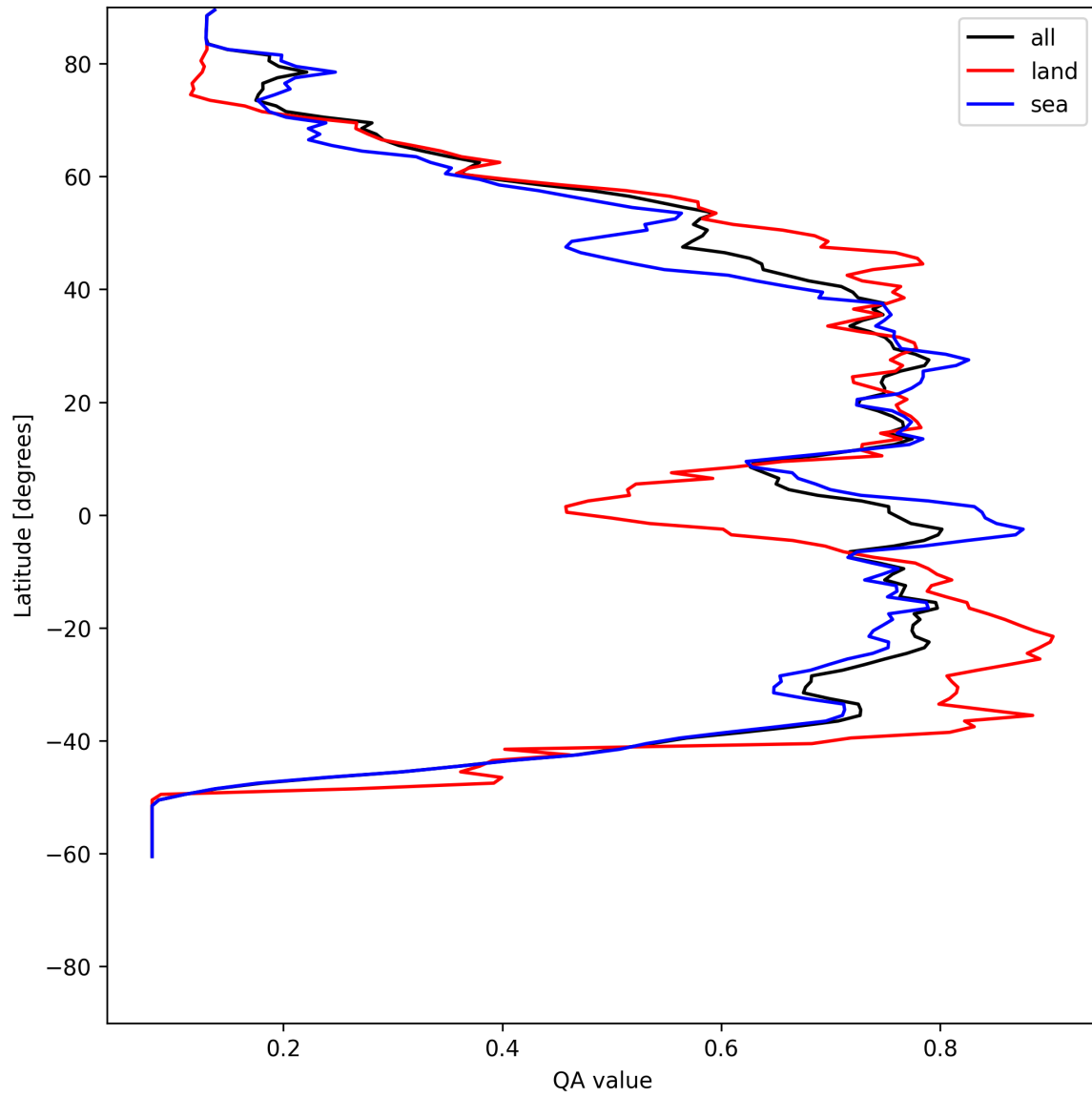
Figure 18: Zonal average of “QA value” for 2025-06-19 to 2025-06-20.
