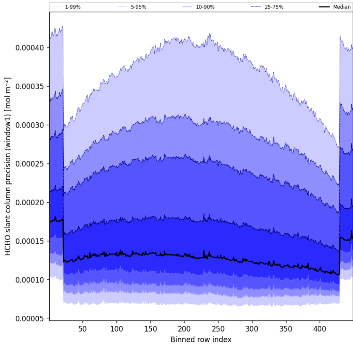
Figure 51: Along track statistics of “HCHO slant column precision (window1)” for 2025-06-19 to 2025-06-20
