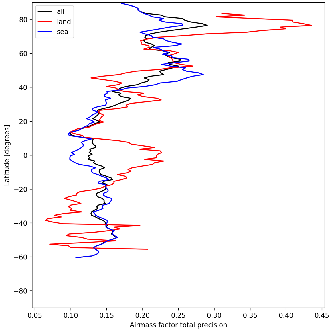
Figure 25: Zonal average of “Airmass factor total precision” for 2025-06-19 to 2025-06-20.
