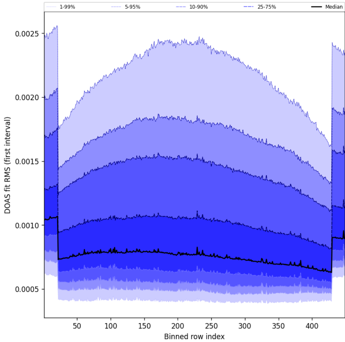
Figure 58: Along track statistics of “DOAS fit RMS (first interval)” for 2025-06-19 to 2025-06-20
