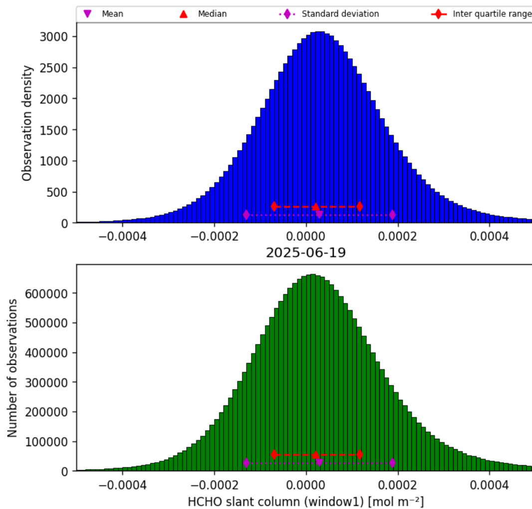
Figure 36: Histogram of “HCHO slant column (window1)” for 2025-06-19 to 2025-06-20
