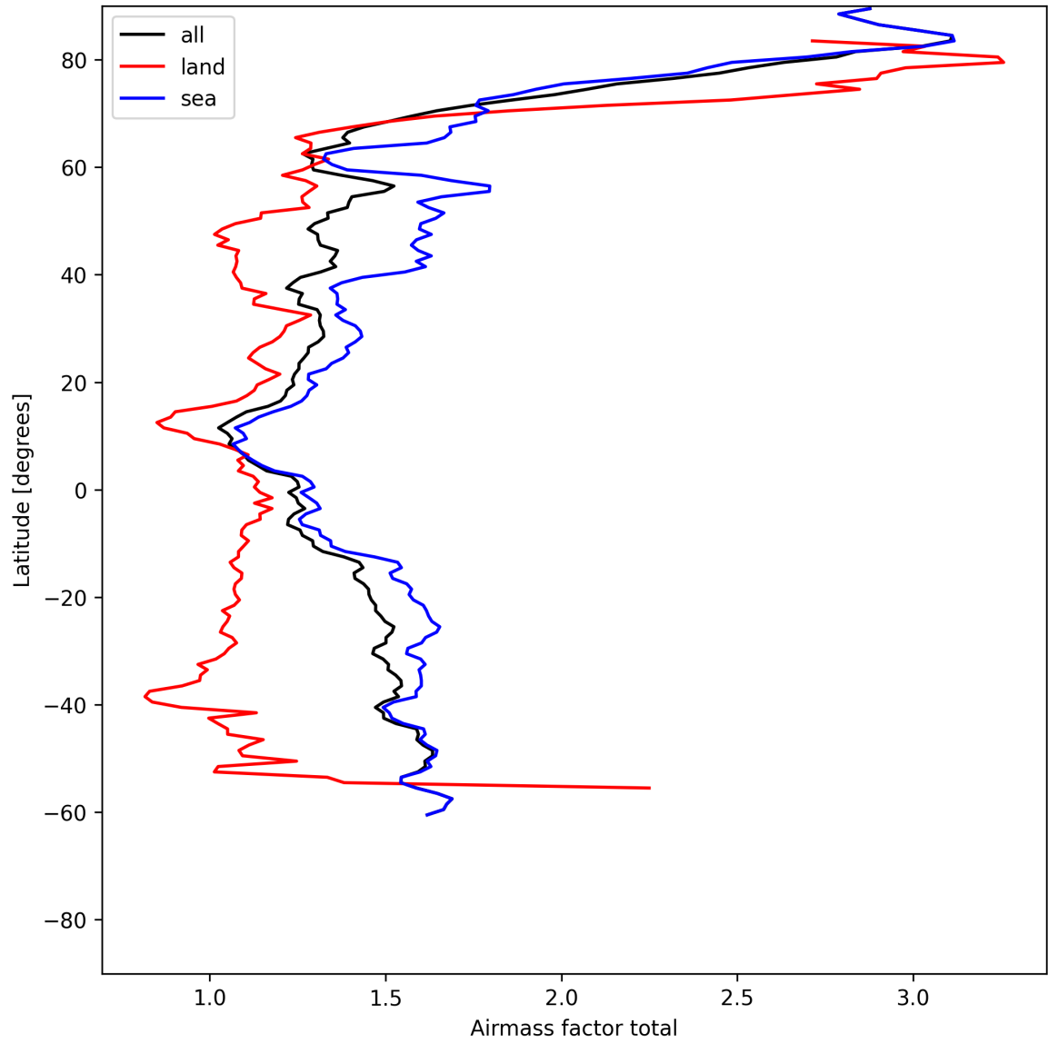
Figure 24: Zonal average of “Airmass factor total” for 2025-06-19 to 2025-06-20.
