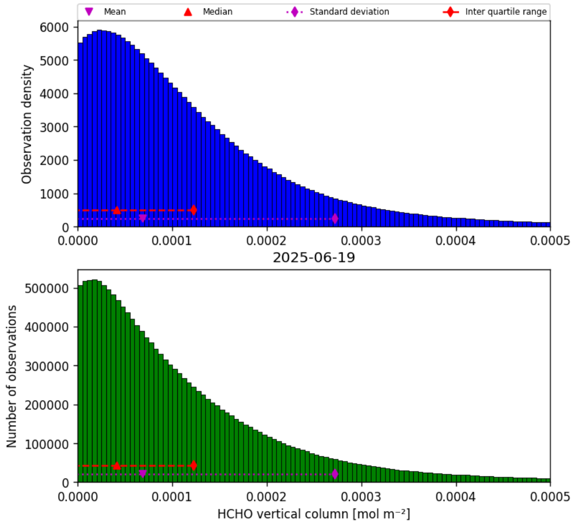
Figure 33: Histogram of “HCHO vertical column” for 2025-06-19 to 2025-06-20
