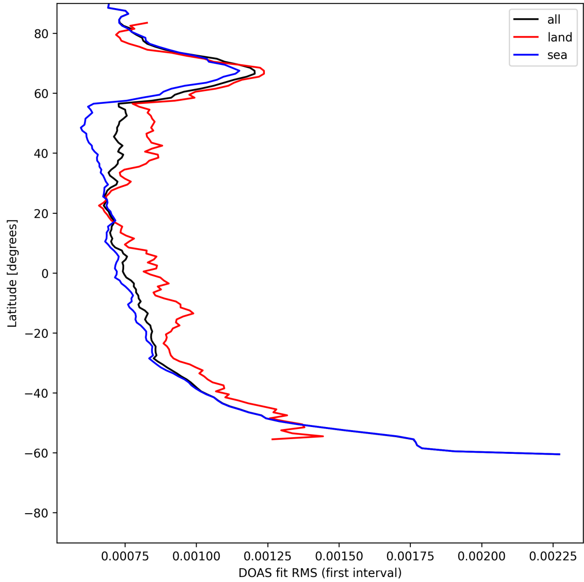
Figure 30: Zonal average of "DOAS fit RMS (first interval)" for 2025-06-19 to 2025-06-20.
