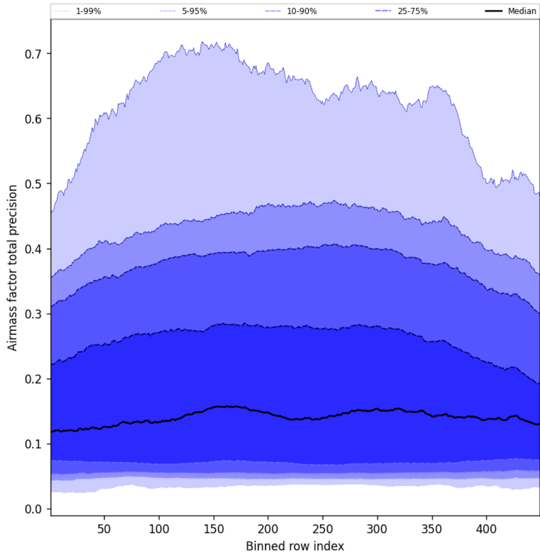
Figure 53: Along track statistics of “Airmass factor total precision” for 2025-06-19 to 2025-06-20
