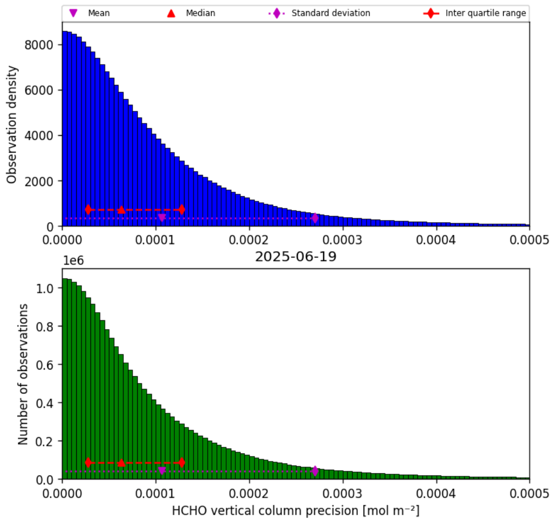
Figure 34: Histogram of “HCHO vertical column precision” for 2025-06-19 to 2025-06-20
