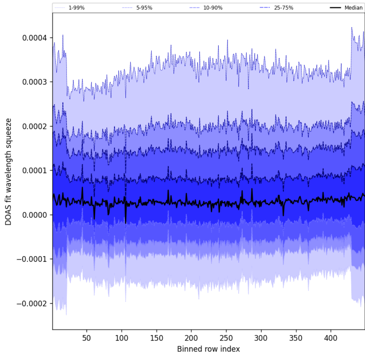
Figure 57: Along track statistics of “DOAS fit wavelength squeeze” for 2025-06-19 to 2025-06-20
