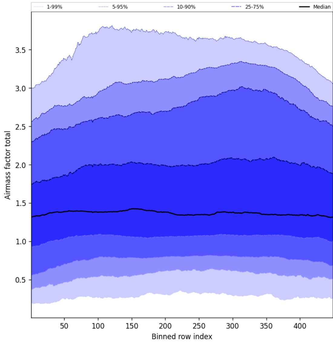
Figure 52: Along track statistics of “Airmass factor total” for 2025-06-19 to 2025-06-20
