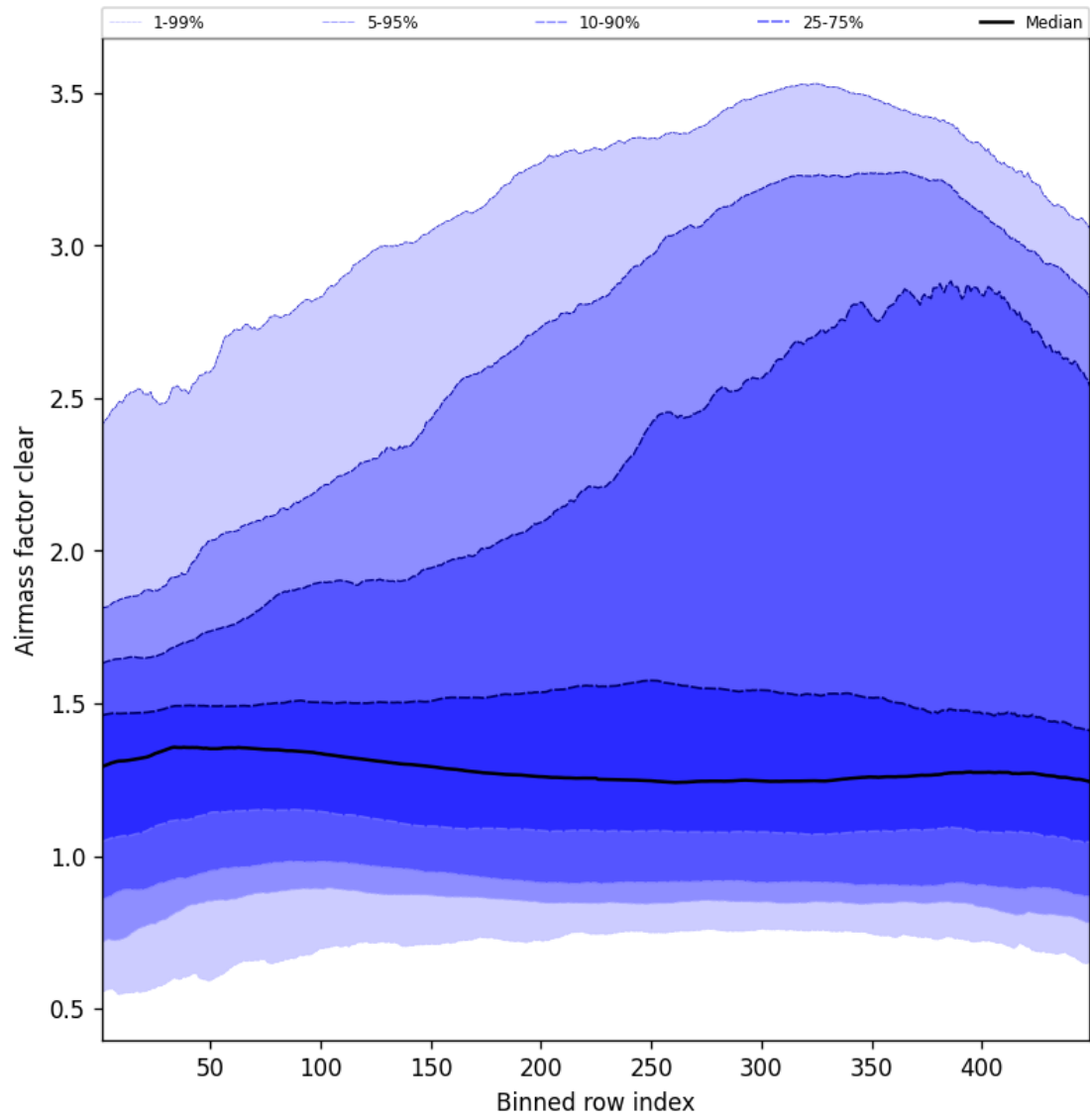
Figure 54: Along track statistics of “Airmass factor clear” for 2025-06-19 to 2025-06-20
