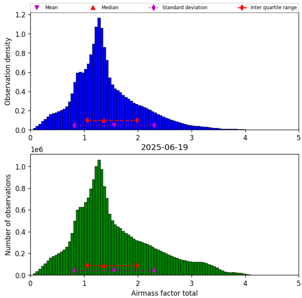
Figure 38: Histogram of “Airmass factor total” for 2025-06-19 to 2025-06-20
