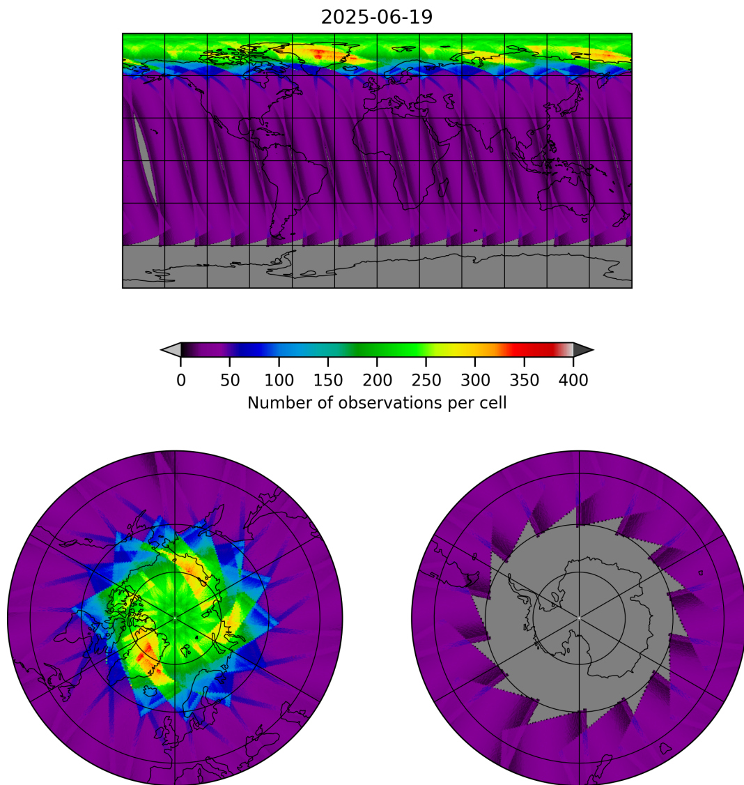
Figure 17: Map of the number of observations for 2025-06-19 to 2025-06-20
