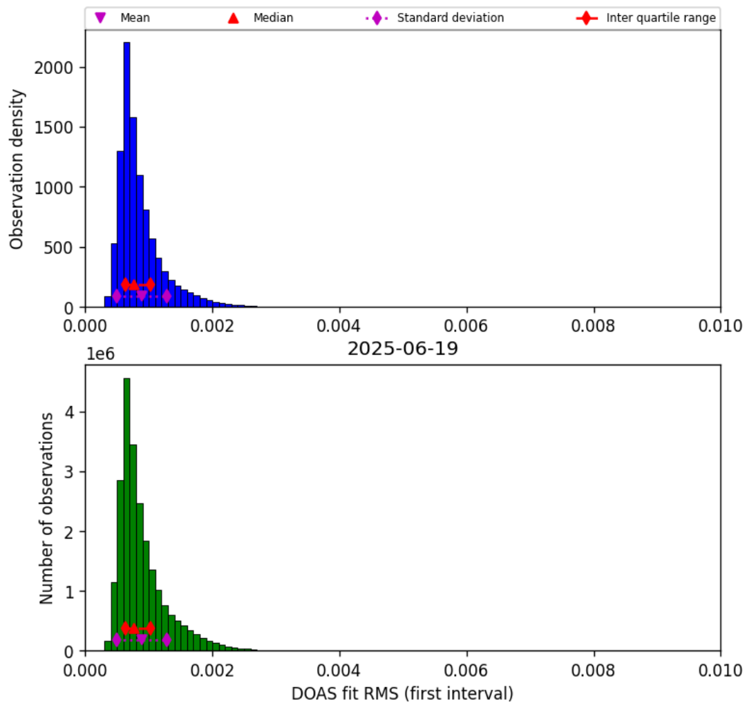
Figure 44: Histogram of “DOAS fit RMS (first interval)” for 2025-06-19 to 2025-06-20
