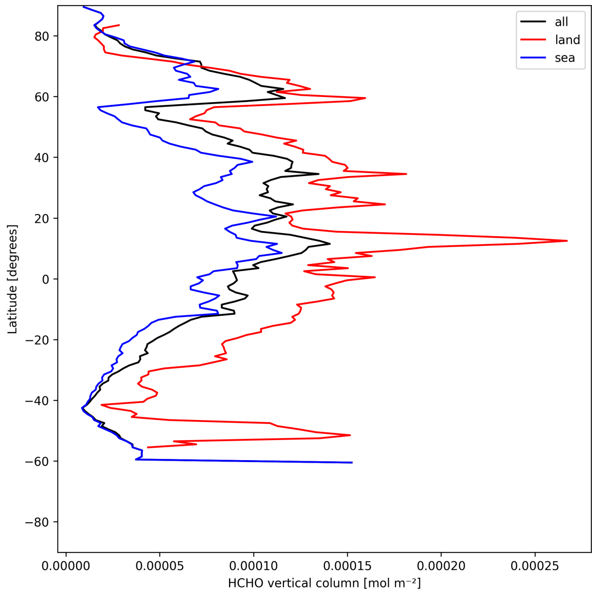
Figure 19: Zonal average of “HCHO vertical column” for 2025-06-19 to 2025-06-20.
