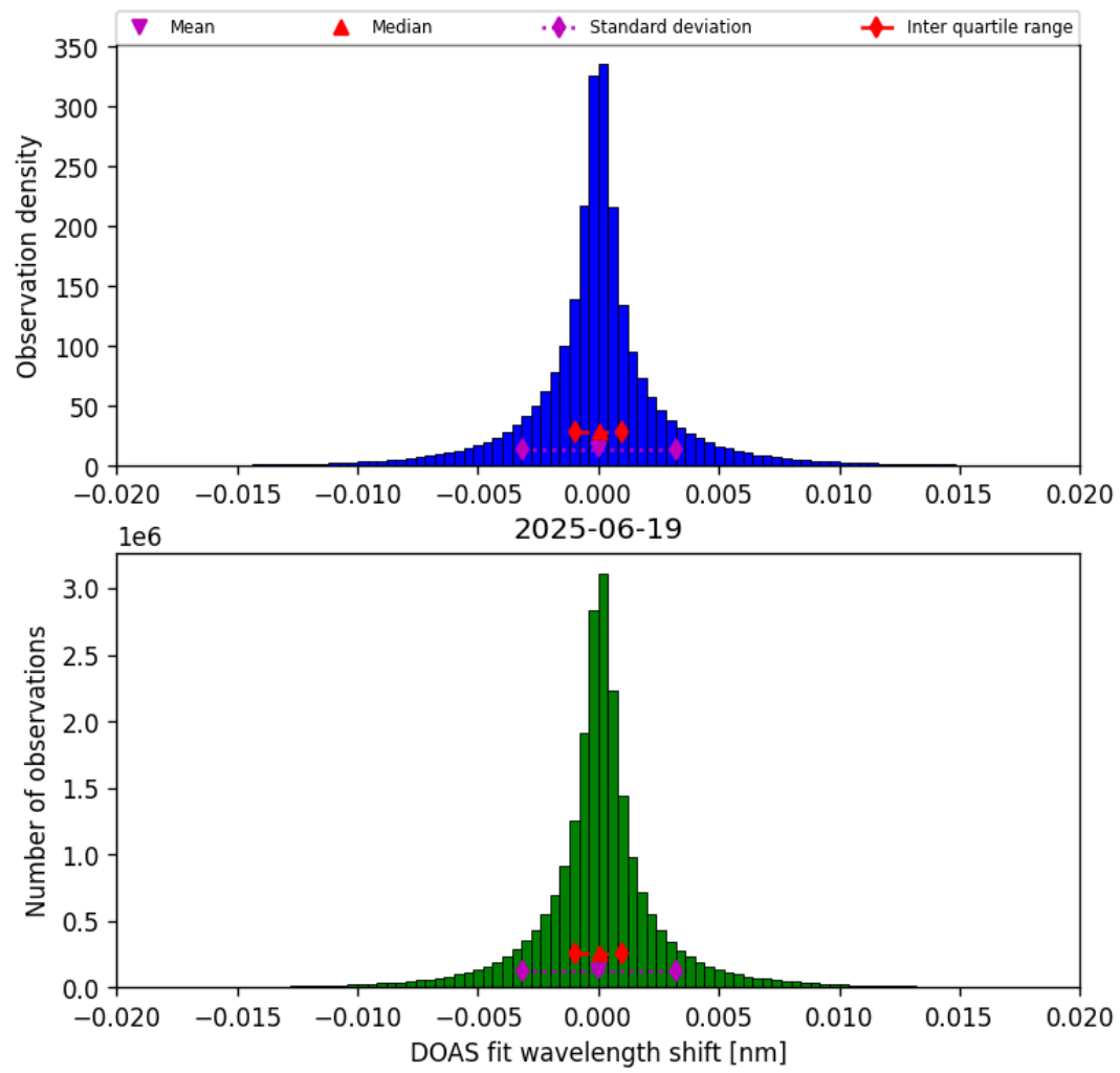
Figure 42: Histogram of “DOAS fit wavelength shift” for 2025-06-19 to 2025-06-20
