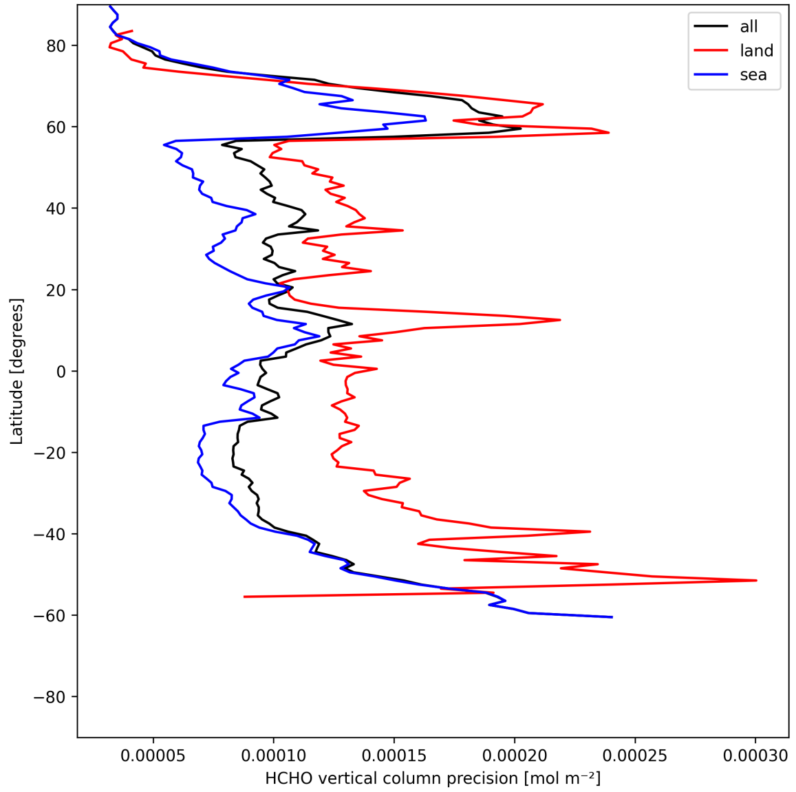
Figure 20: Zonal average of “HCHO vertical column precision” for 2025-06-19 to 2025-06-20.
