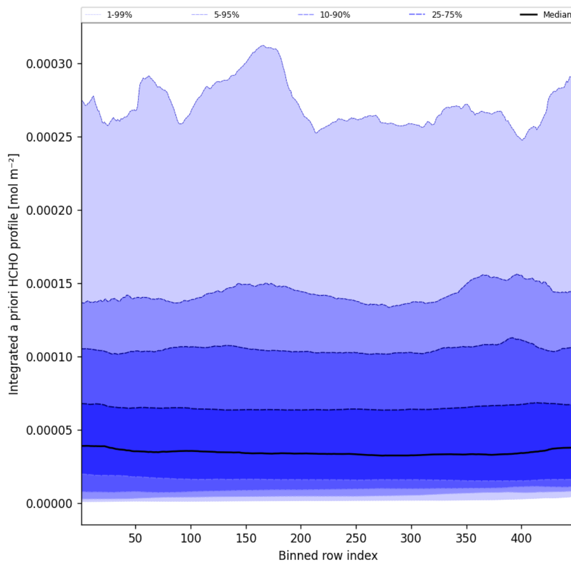
Figure 55: Along track statistics of "Integrated a priori HCHO profile" for 2025-06-19 to 2025-06-20
