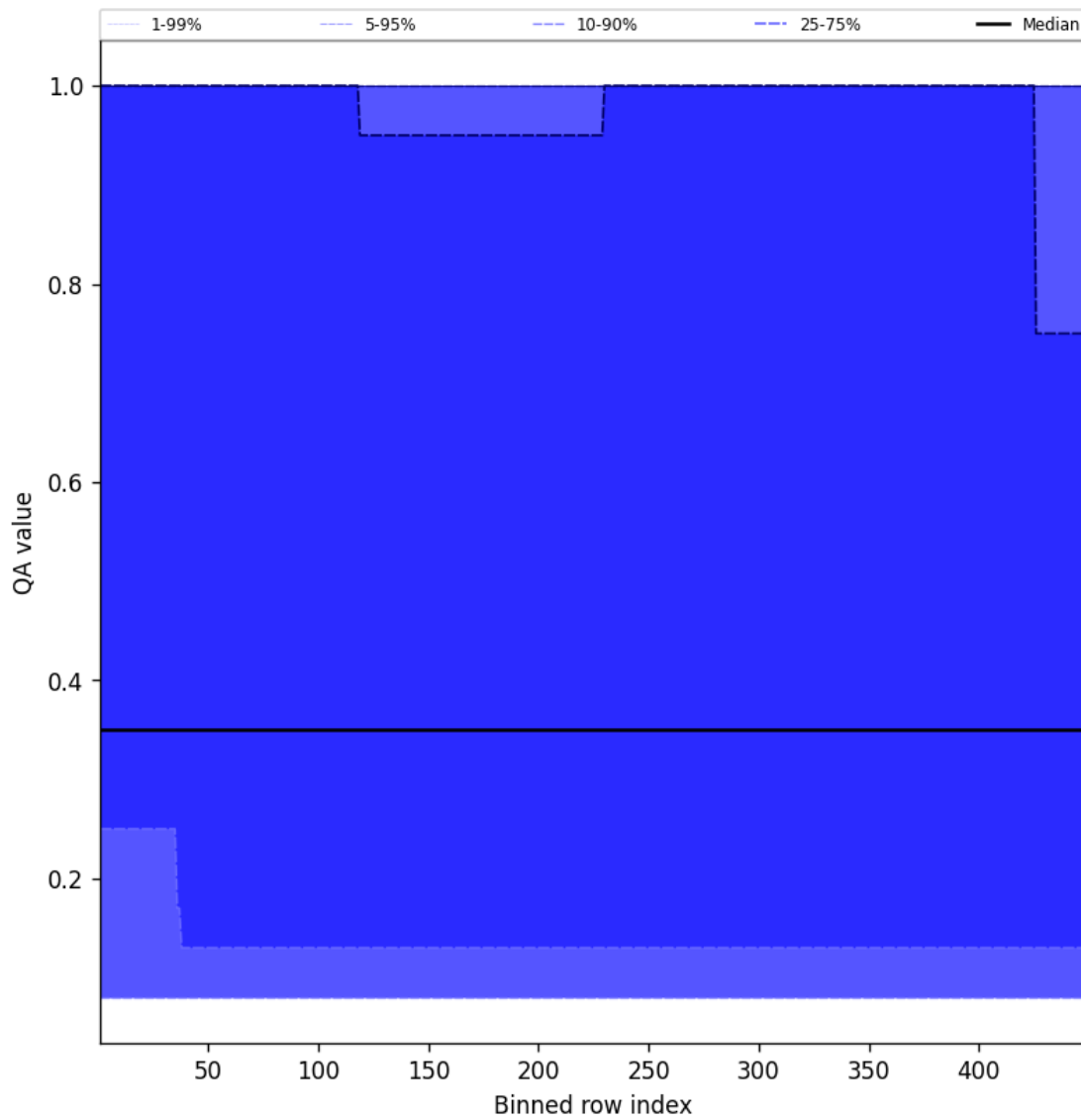
Figure 46: Along track statistics of “QA value” for 2025-06-19 to 2025-06-20
