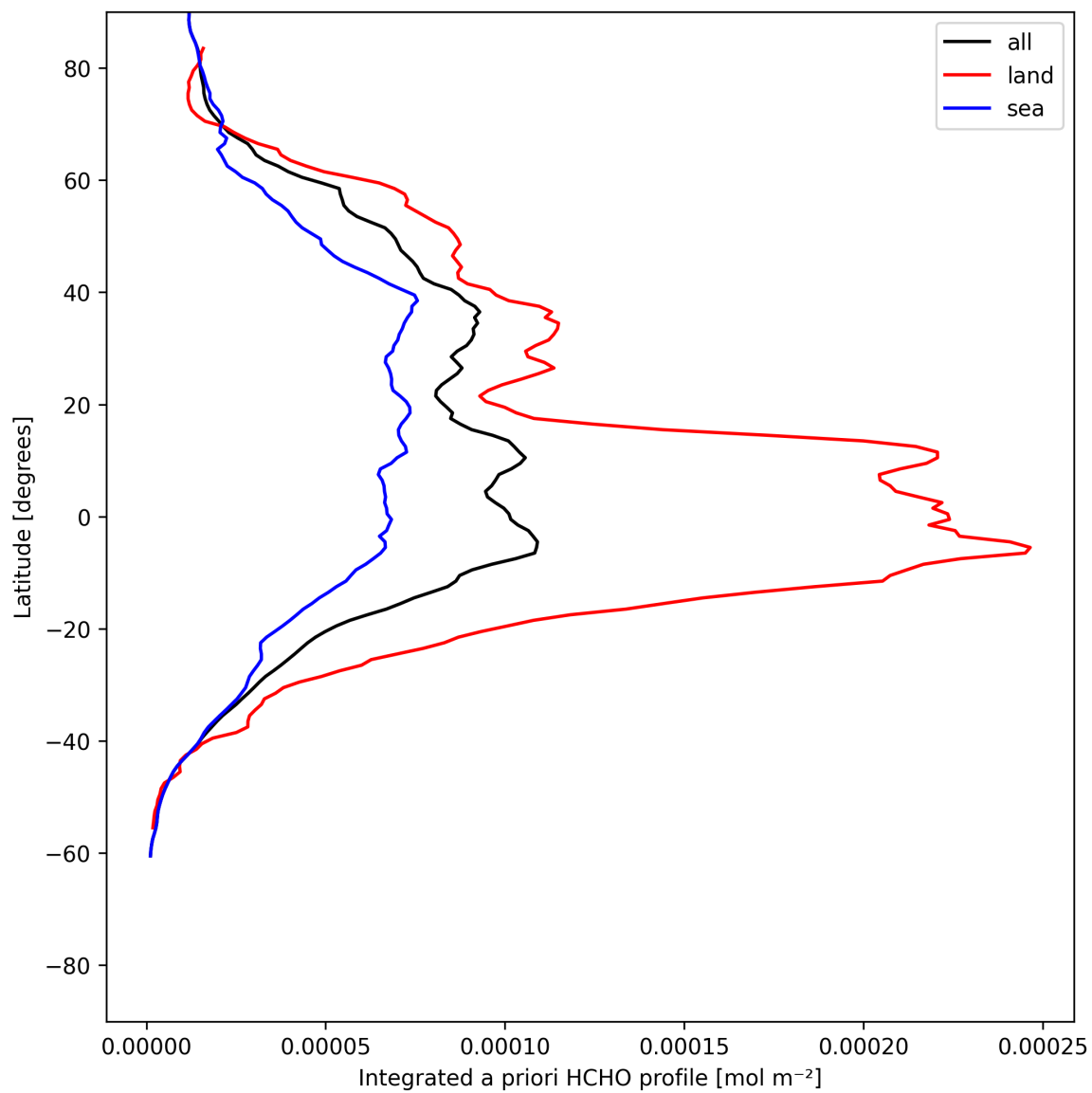
Figure 27: Zonal average of “Integrated a priori HCHO profile” for 2025-06-19 to 2025-06-20.
