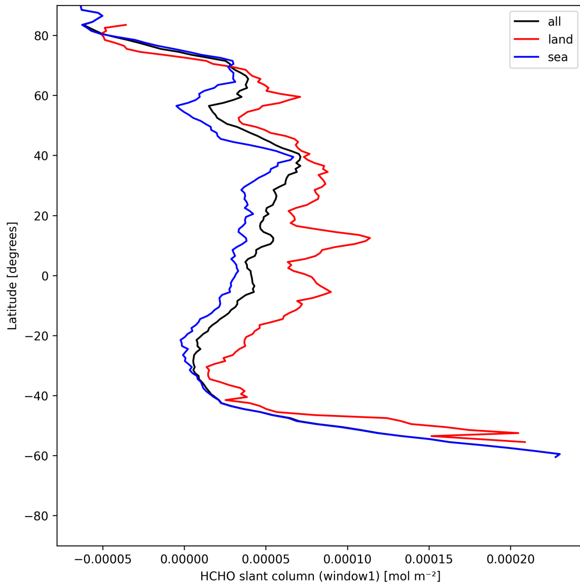
Figure 22: Zonal average of “HCHO slant column (window1)” for 2025-06-19 to 2025-06-20.
