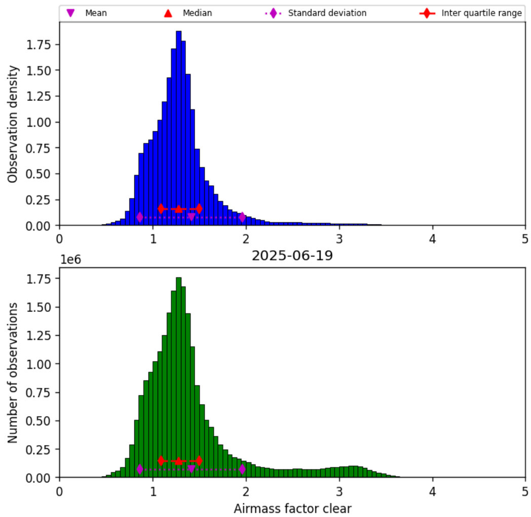
Figure 40: Histogram of “Airmass factor clear” for 2025-06-19 to 2025-06-20
