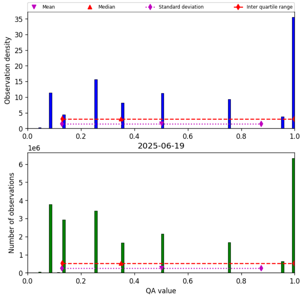
Figure 32: Histogram of “QA value” for 2025-06-19 to 2025-06-20
