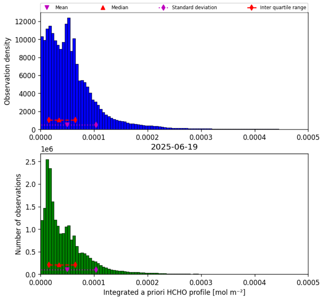
Figure 41: Histogram of “Integrated a priori HCHO profile” for 2025-06-19 to 2025-06-20
