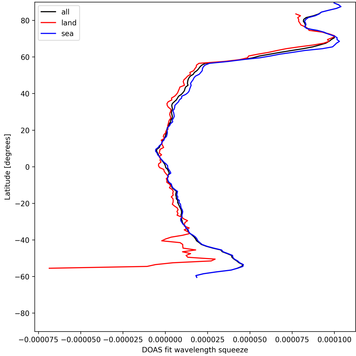
Figure 29: Zonal average of “DOAS fit wavelength squeeze” for 2025-06-19 to 2025-06-20.
