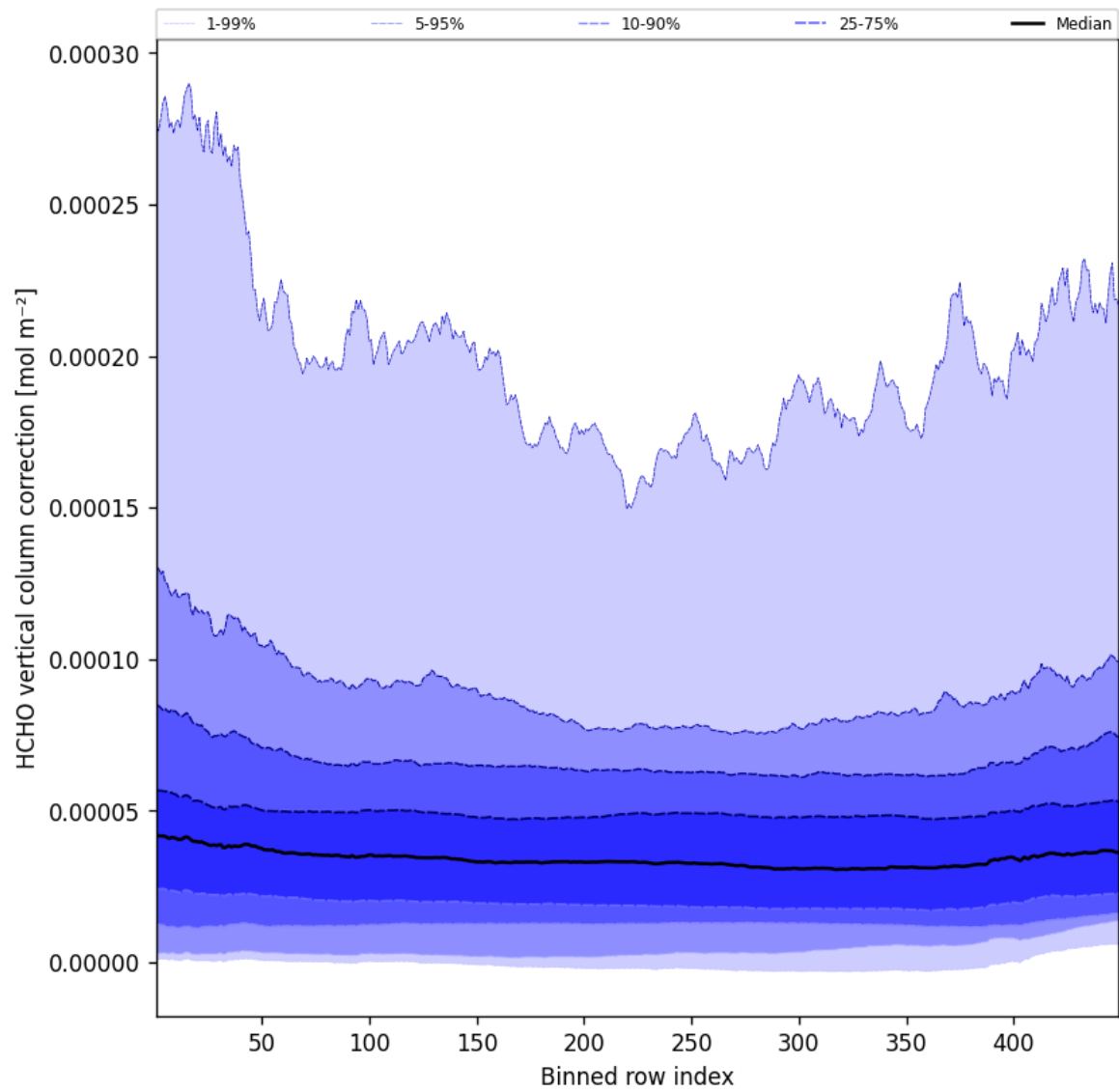
Figure 49: Along track statistics of “HCHO vertical column correction” for 2025-06-19 to 2025-06-20
