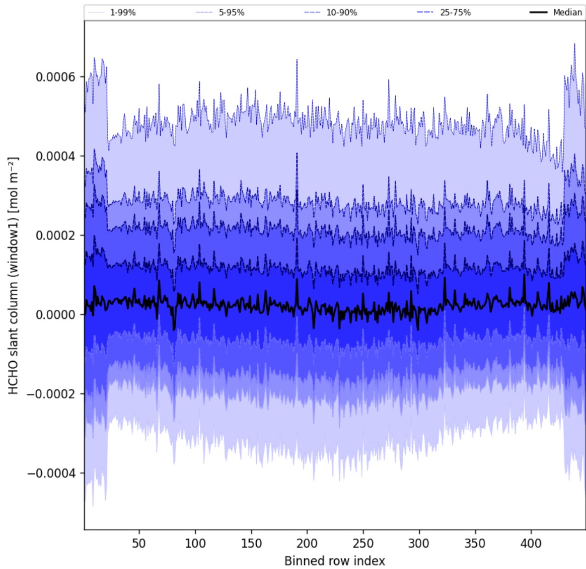
Figure 50: Along track statistics of “HCHO slant column (window1)” for 2025-06-19 to 2025-06-20
