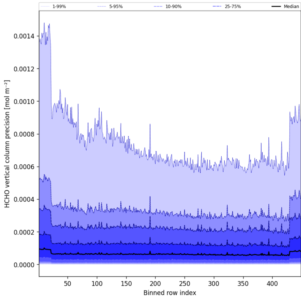
Figure 48: Along track statistics of “HCHO vertical column precision” for 2025-06-19 to 2025-06-20
