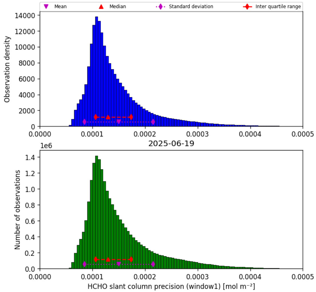
Figure 37: Histogram of “HCHO slant column precision (window1)” for 2025-06-19 to 2025-06-20
