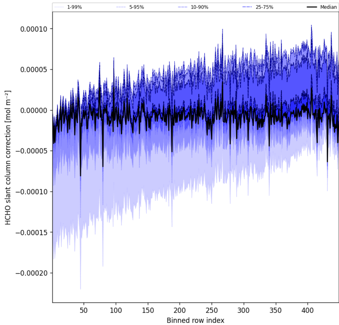
Figure 59: Along track statistics of “HCHO slant column correction” for 2025-06-19 to 2025-06-20
