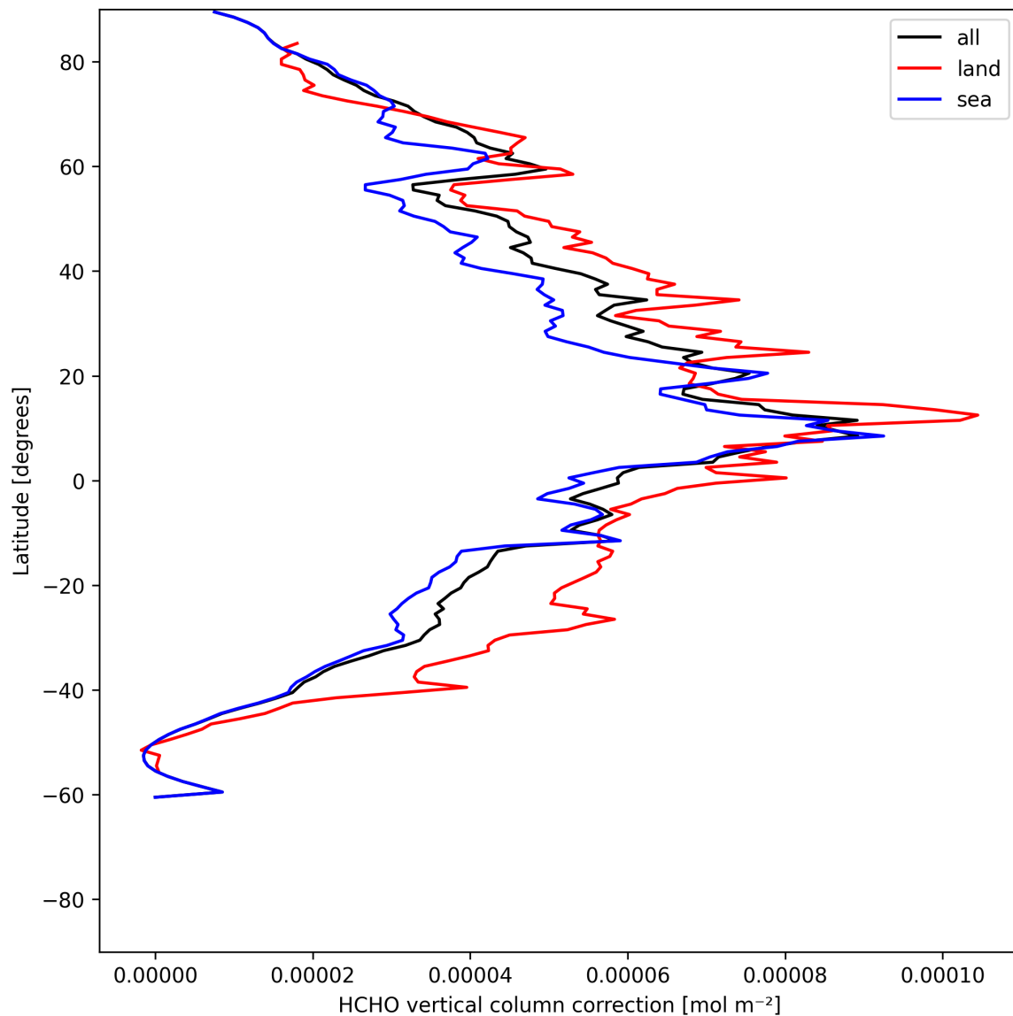
Figure 21: Zonal average of “HCHO vertical column correction” for 2025-06-19 to 2025-06-20.
