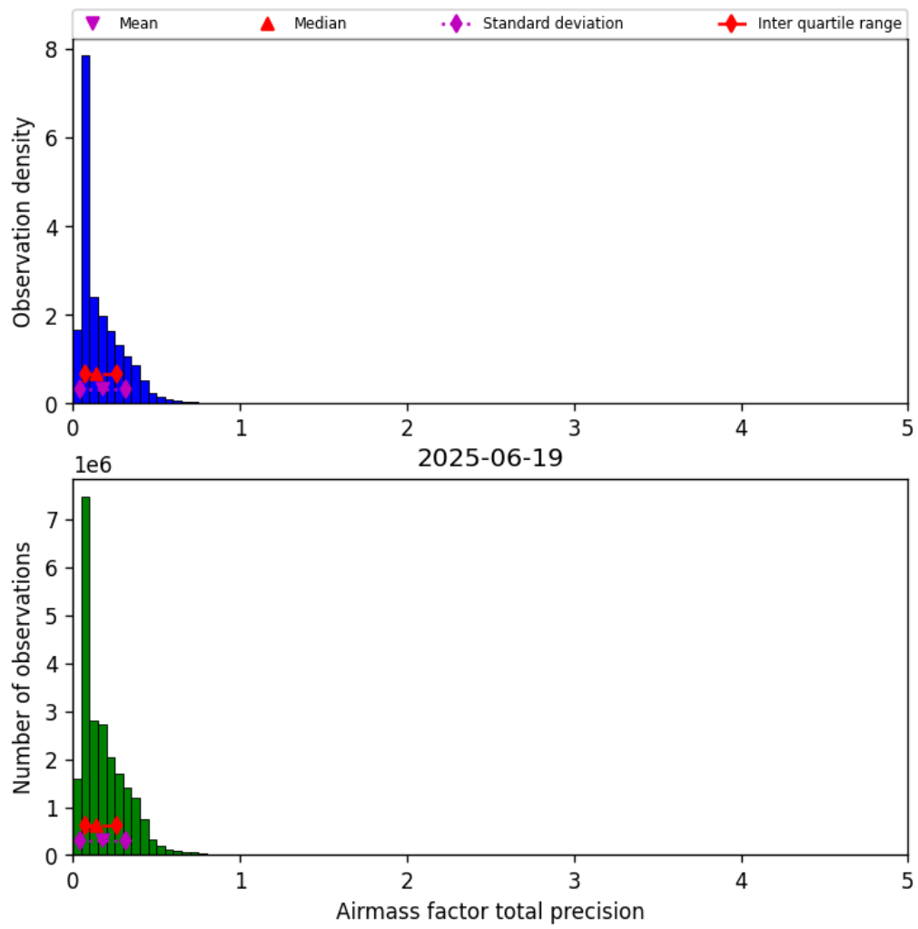
Figure 39: Histogram of “Airmass factor total precision” for 2025-06-19 to 2025-06-20
