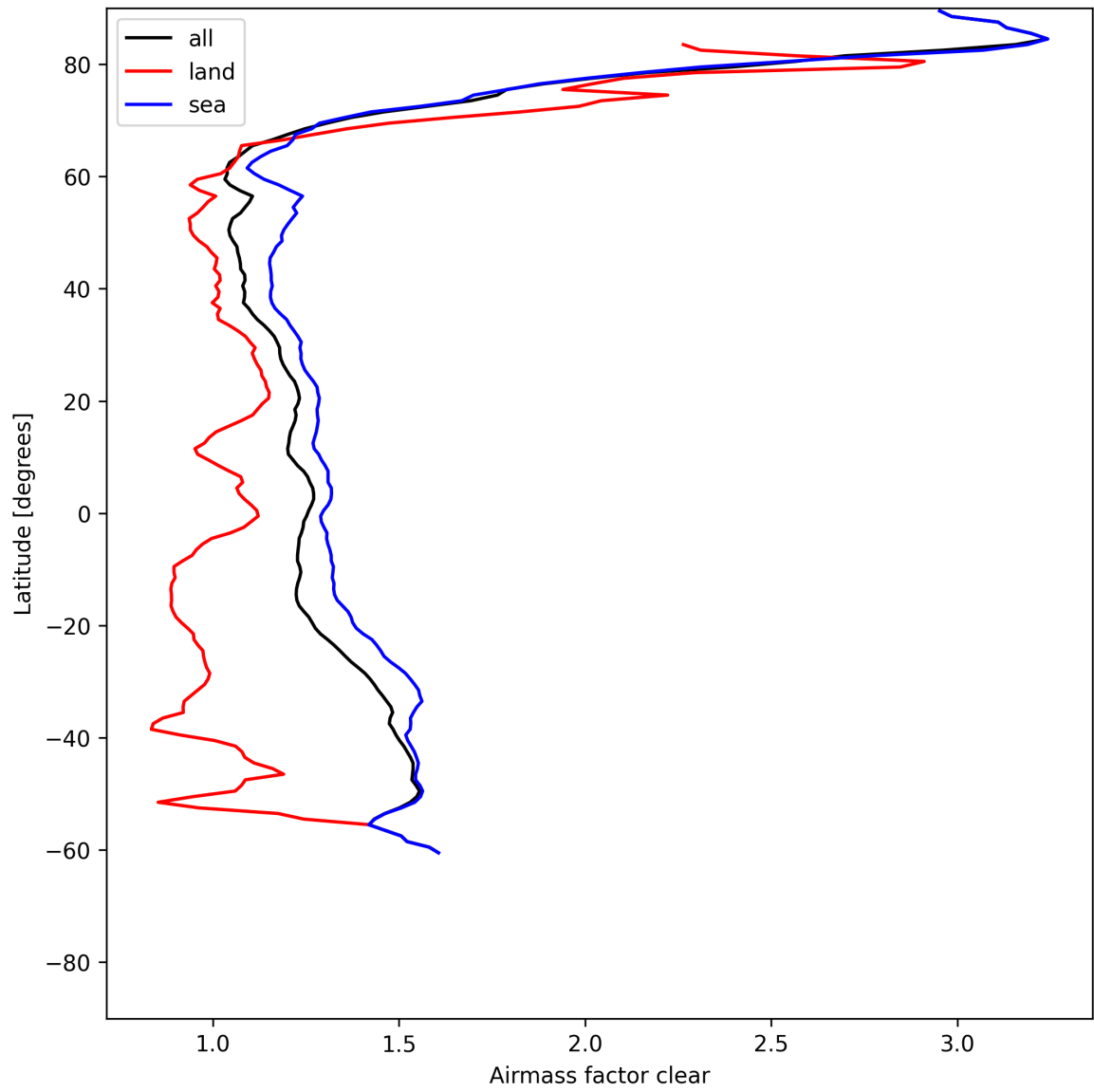
Figure 26: Zonal average of “Airmass factor clear” for 2025-06-19 to 2025-06-20.
