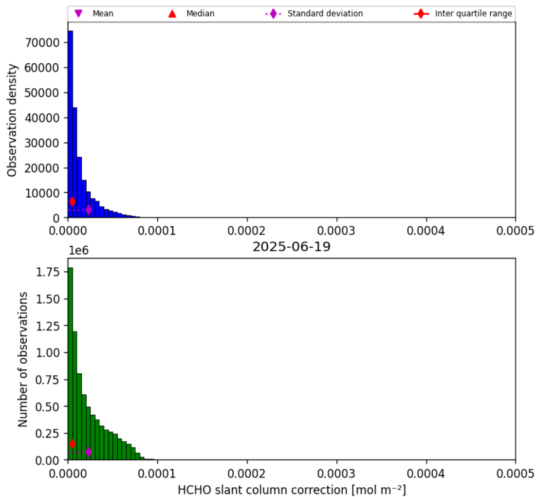
Figure 45: Histogram of “HCHO slant column correction” for 2025-06-19 to 2025-06-20
