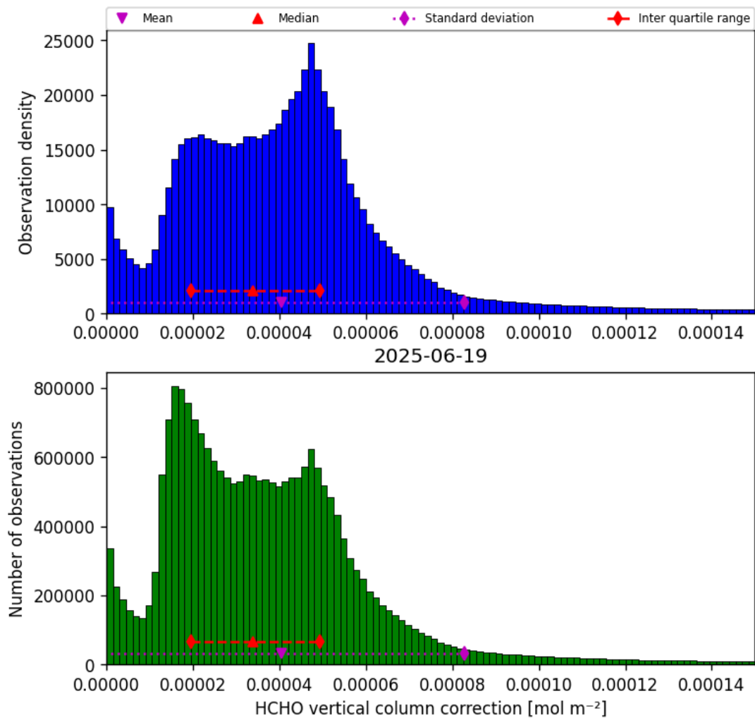
Figure 35: Histogram of “HCHO vertical column correction” for 2025-06-19 to 2025-06-20
