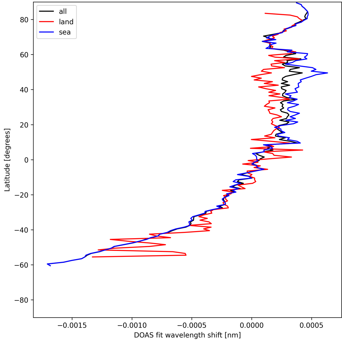
Figure 28: Zonal average of “DOAS fit wavelength shift” for 2025-06-19 to 2025-06-20.
