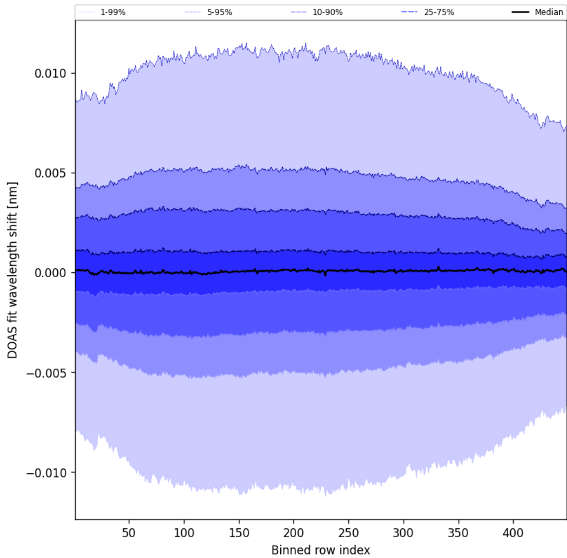
Figure 56: Along track statistics of “DOAS fit wavelength shift” for 2025-06-19 to 2025-06-20
