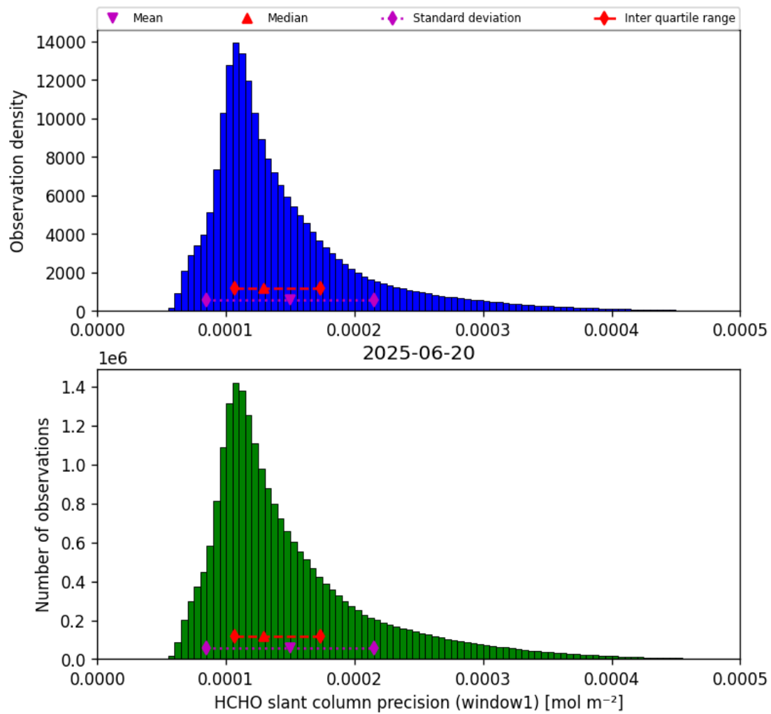
Figure 37: Histogram of “HCHO slant column precision (window1)” for 2025-06-20 to 2025-06-20
