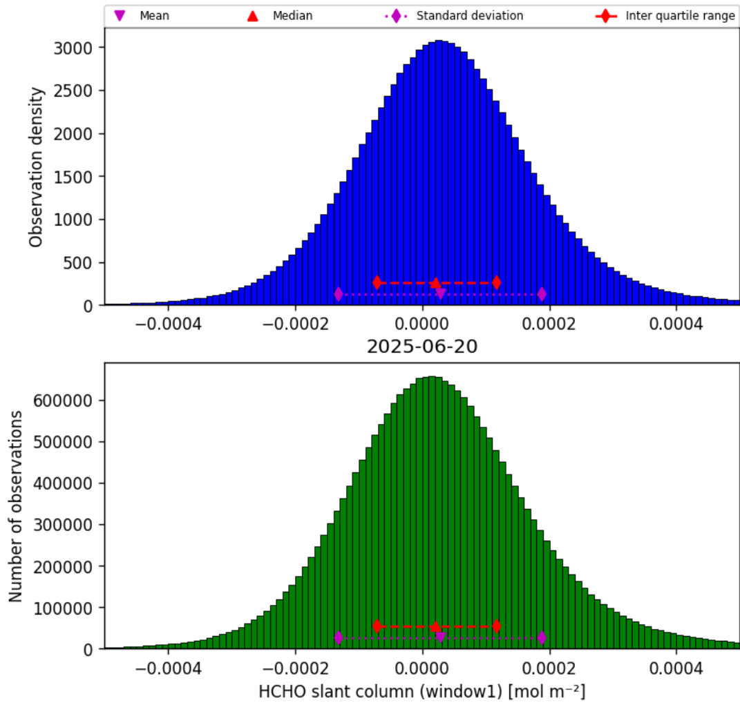
Figure 36: Histogram of “HCHO slant column (window1)” for 2025-06-20 to 2025-06-20
