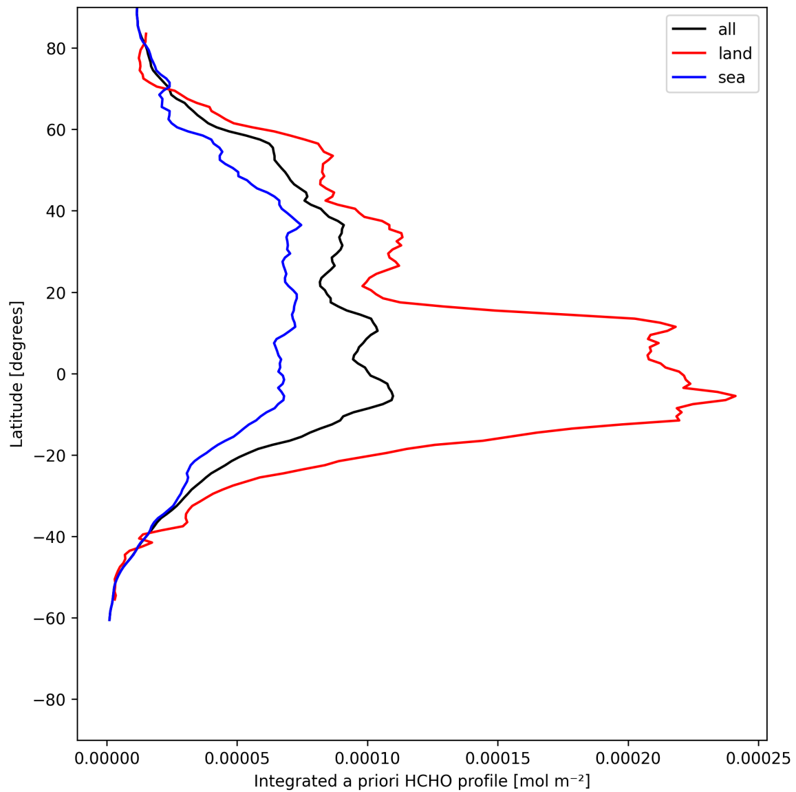
Figure 27: Zonal average of “Integrated a priori HCHO profile” for 2025-06-20 to 2025-06-20.
