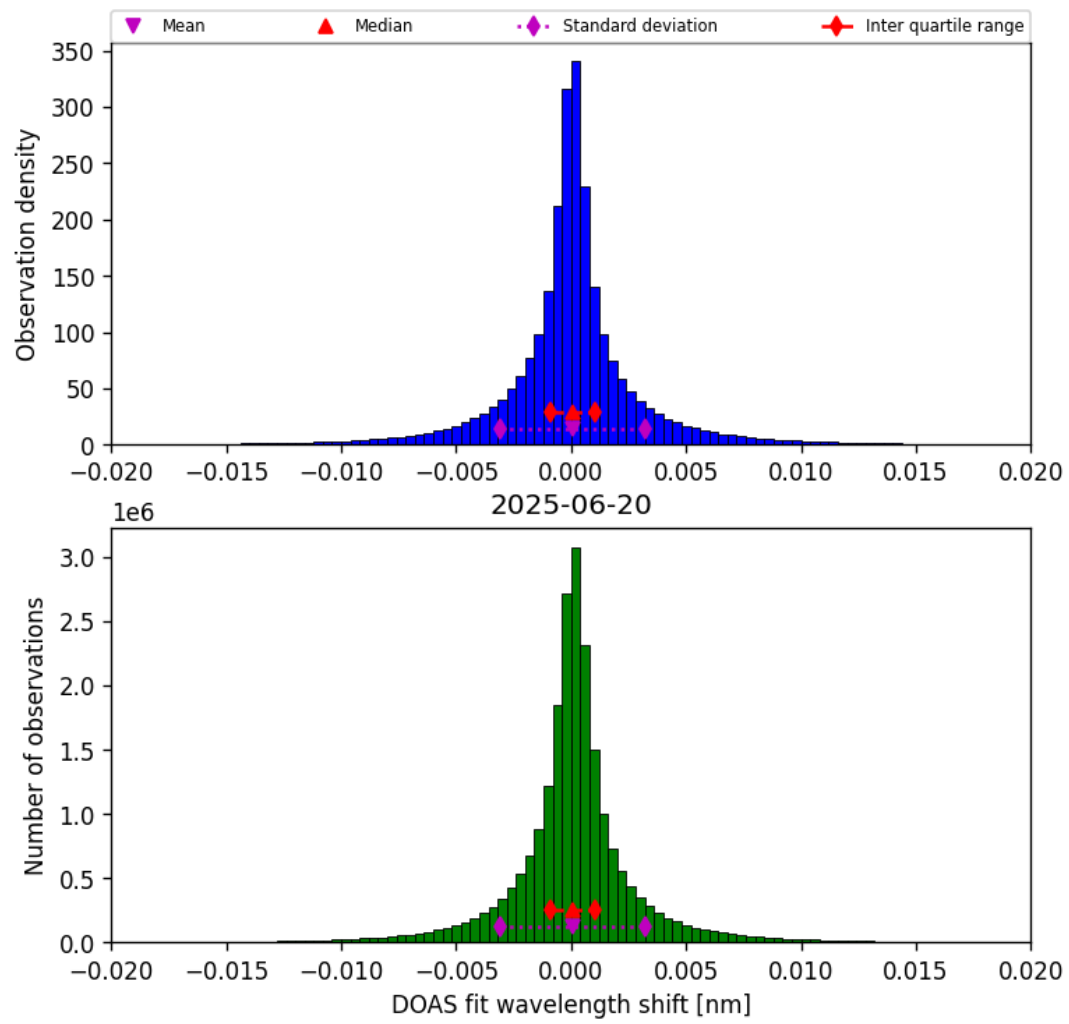
Figure 42: Histogram of “DOAS fit wavelength shift” for 2025-06-20 to 2025-06-20
