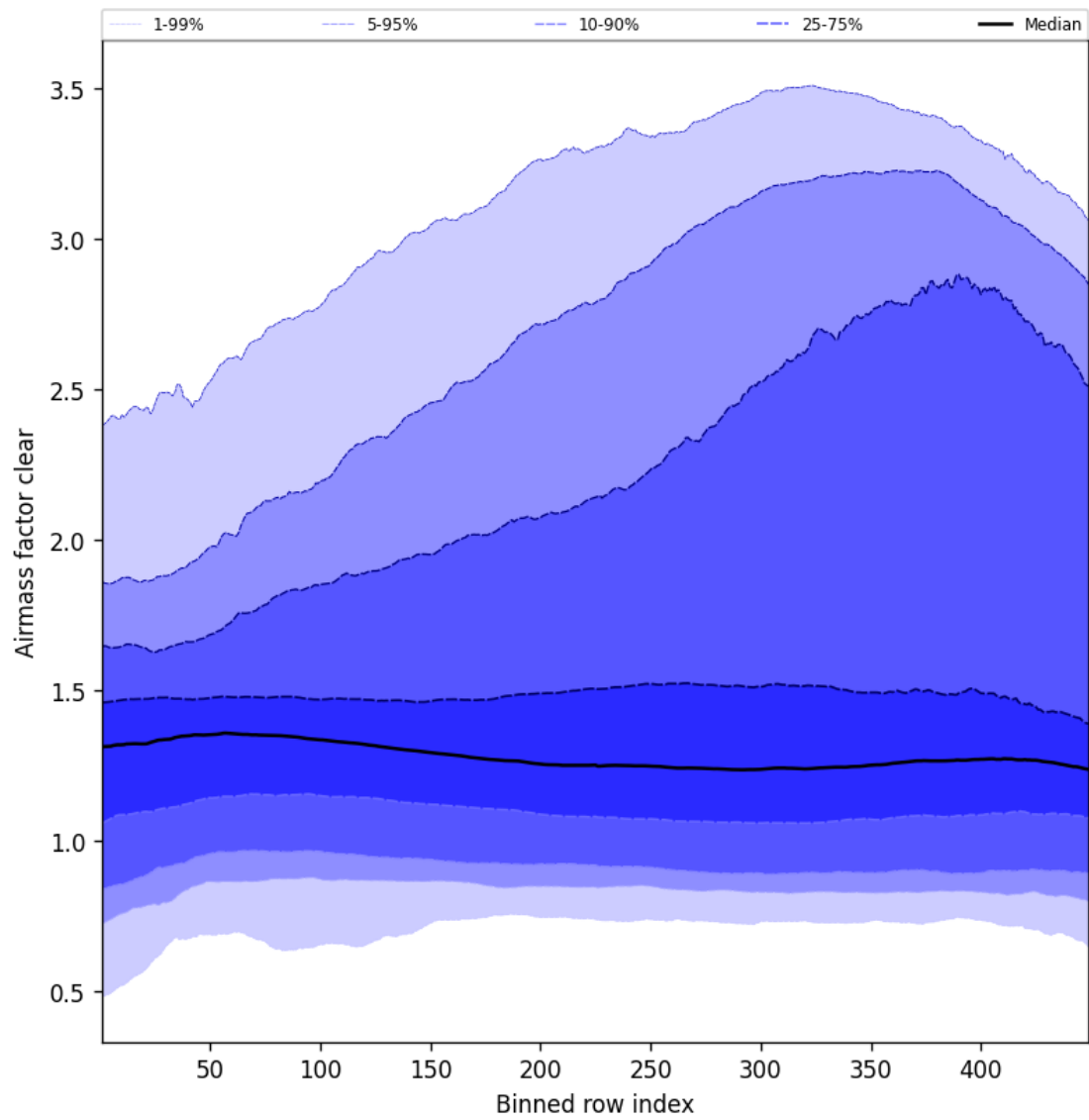
Figure 54: Along track statistics of “Airmass factor clear” for 2025-06-20 to 2025-06-20
