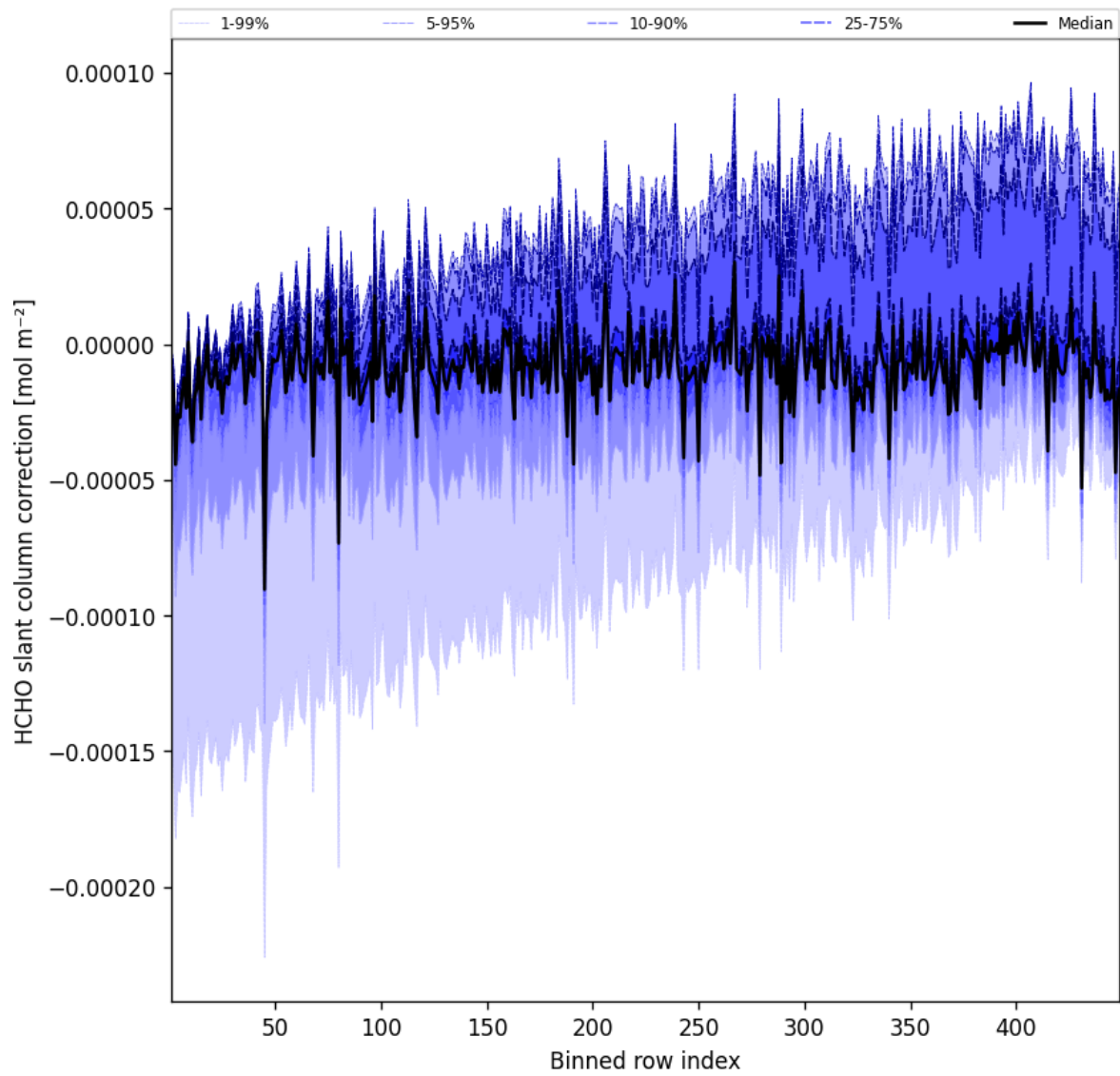
Figure 59: Along track statistics of “HCHO slant column correction” for 2025-06-20 to 2025-06-20
