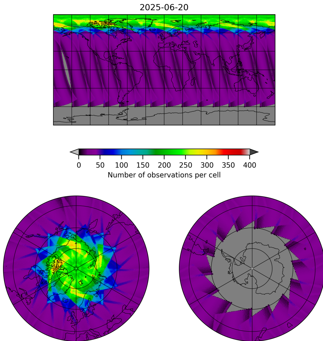
Figure 17: Map of the number of observations for 2025-06-20 to 2025-06-20
