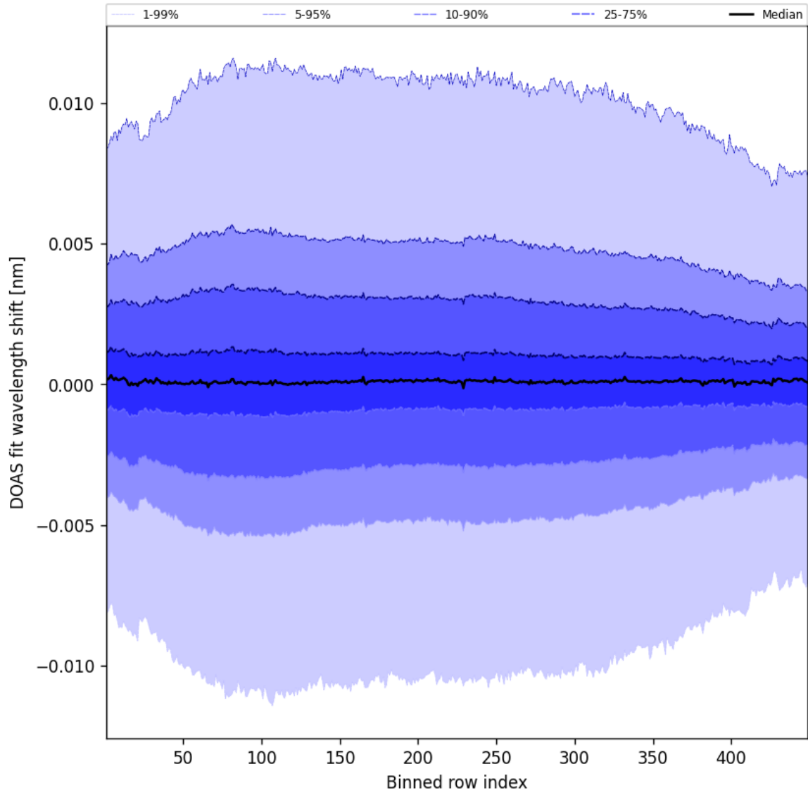
Figure 56: Along track statistics of “DOAS fit wavelength shift” for 2025-06-20 to 2025-06-20
