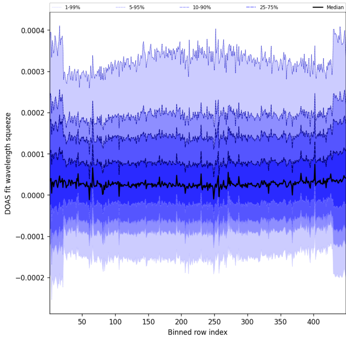
Figure 57: Along track statistics of “DOAS fit wavelength squeeze” for 2025-06-20 to 2025-06-20
