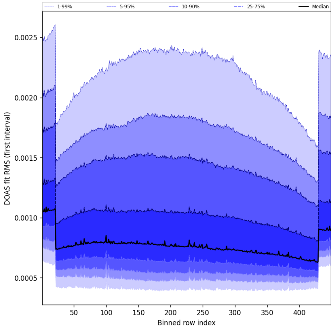
Figure 58: Along track statistics of “DOAS fit RMS (first interval)” for 2025-06-20 to 2025-06-20
