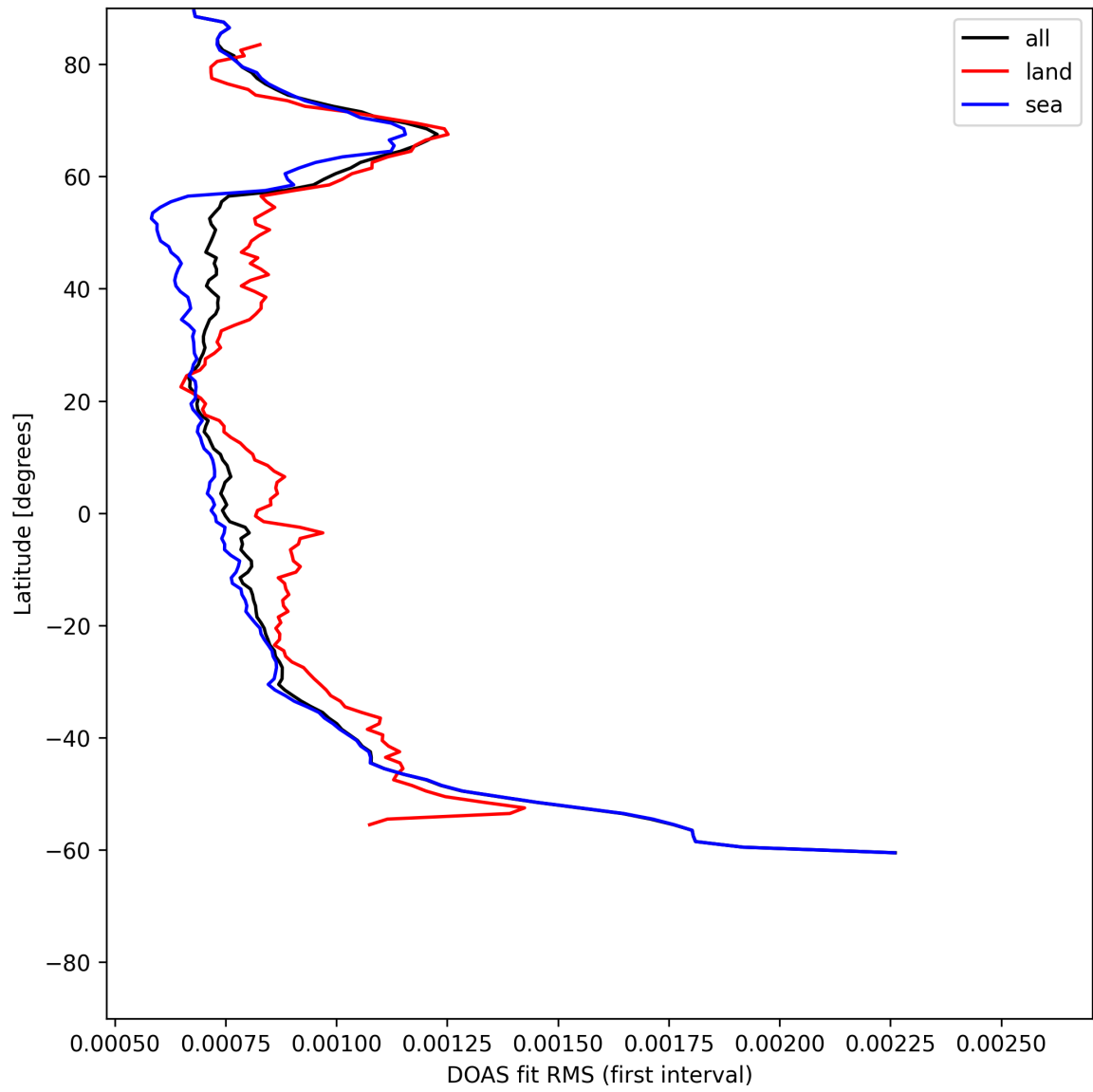
Figure 30: Zonal average of "DOAS fit RMS (first interval)" for 2025-06-20 to 2025-06-20.
