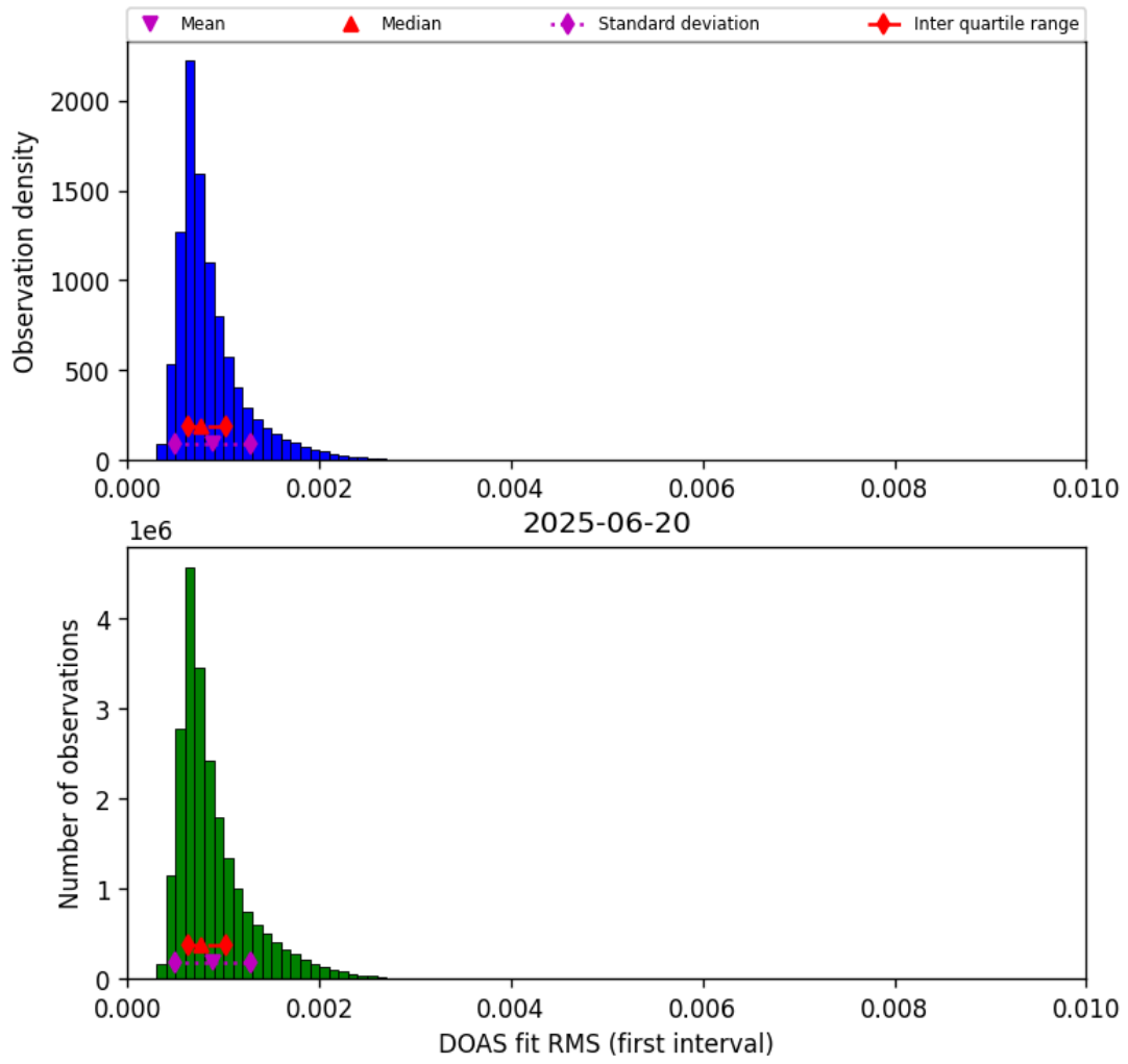
Figure 44: Histogram of “DOAS fit RMS (first interval)” for 2025-06-20 to 2025-06-20
