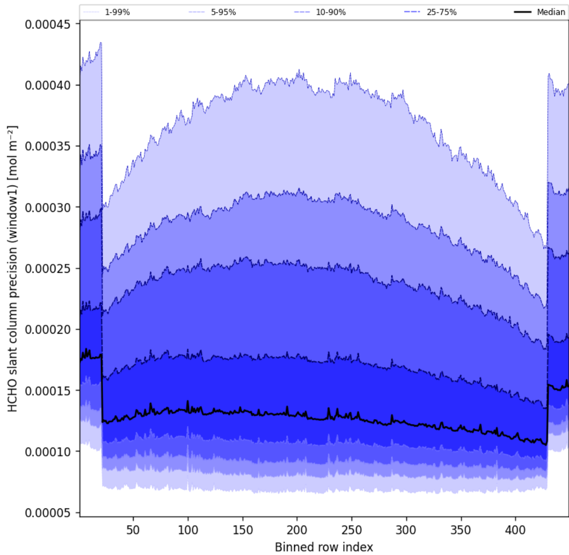
Figure 51: Along track statistics of “HCHO slant column precision (window1)” for 2025-06-20 to 2025-06-20
