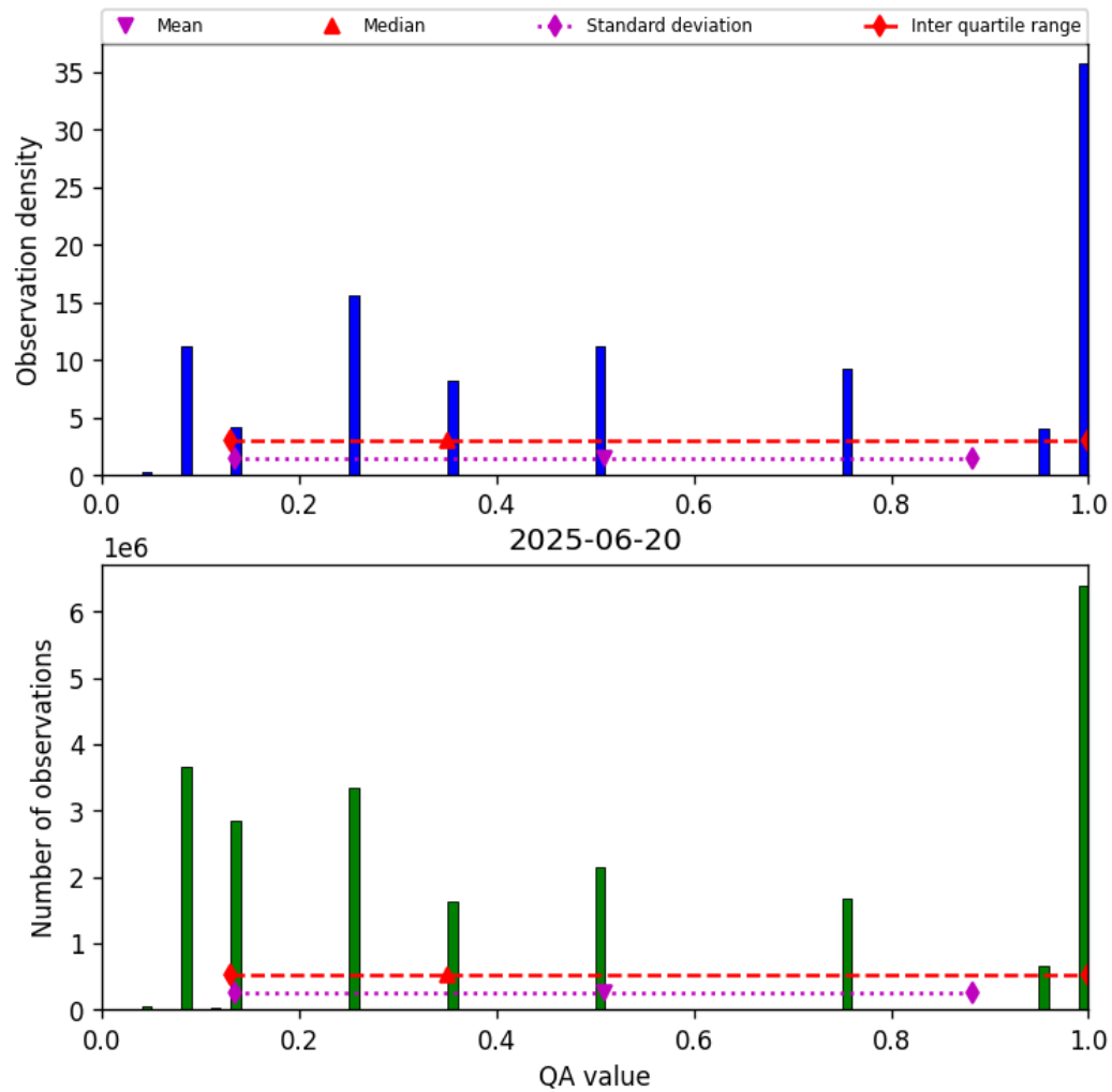
Figure 32: Histogram of “QA value” for 2025-06-20 to 2025-06-20
