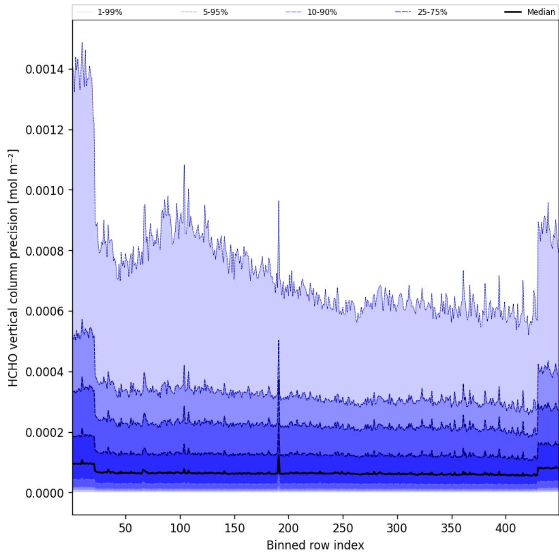
Figure 48: Along track statistics of “HCHO vertical column precision” for 2025-06-20 to 2025-06-20
