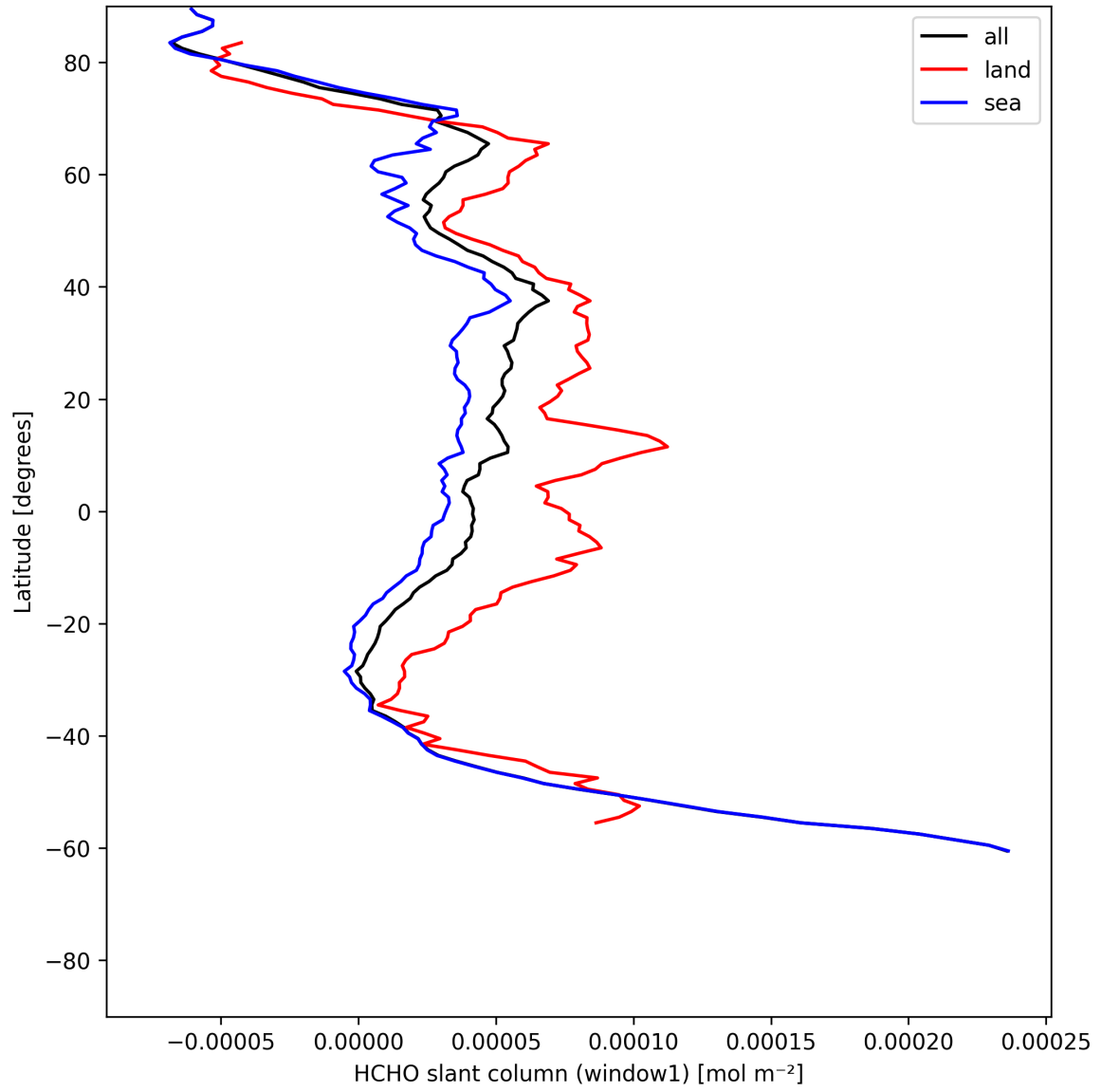
Figure 22: Zonal average of “HCHO slant column (window1)” for 2025-06-20 to 2025-06-20.
