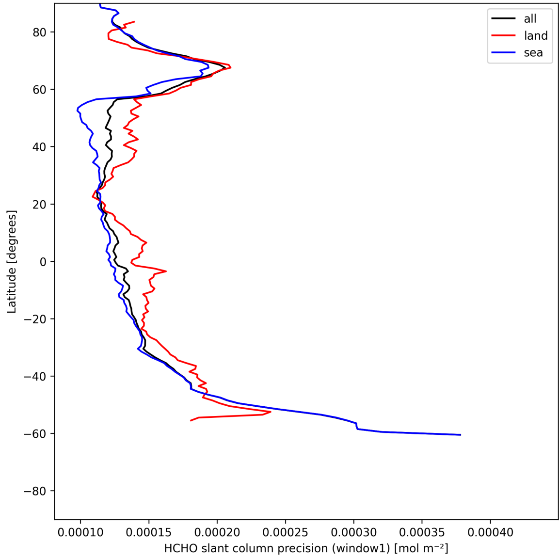
Figure 23: Zonal average of “HCHO slant column precision (window1)” for 2025-06-20 to 2025-06-20.
