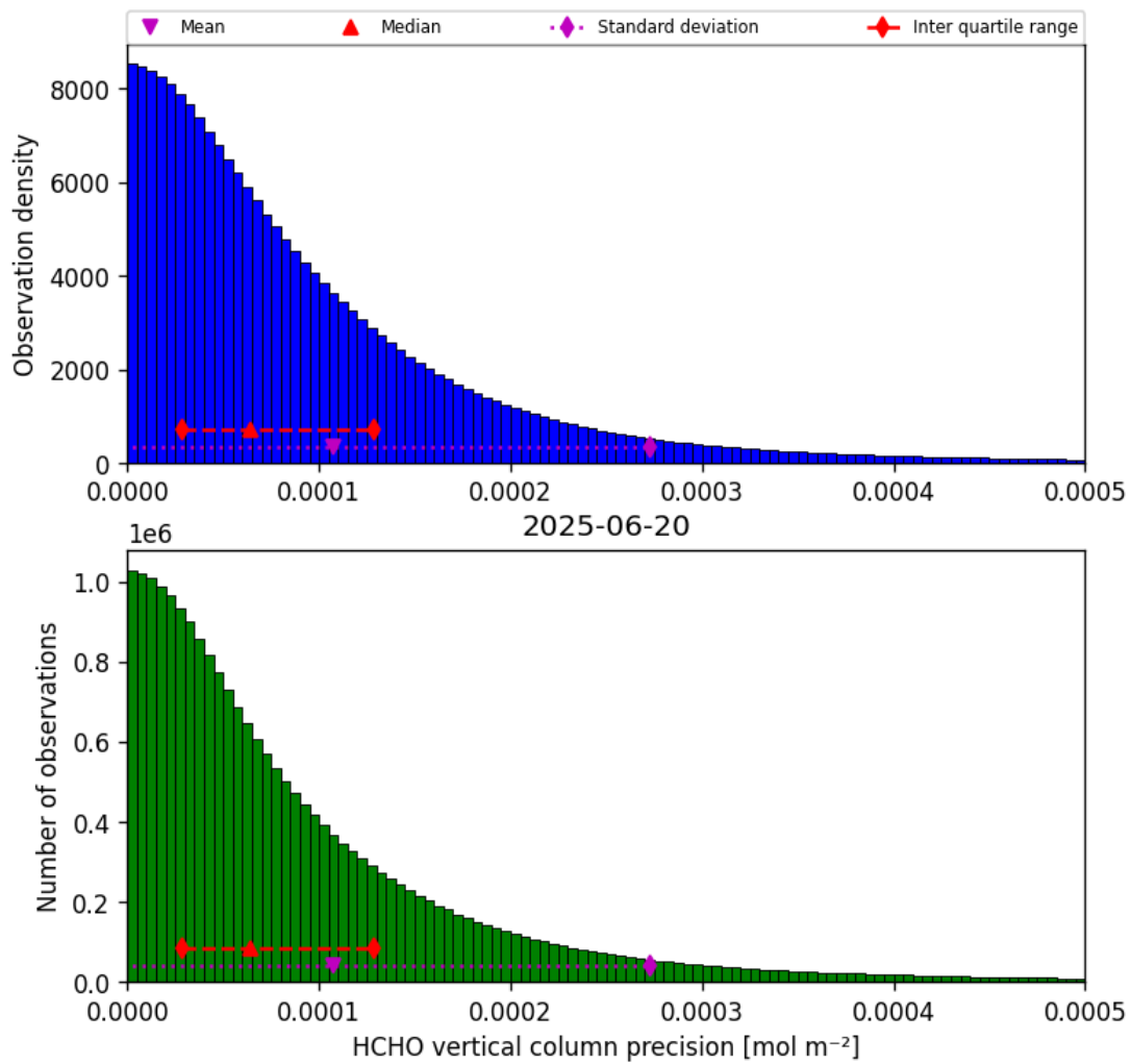
Figure 34: Histogram of “HCHO vertical column precision” for 2025-06-20 to 2025-06-20
