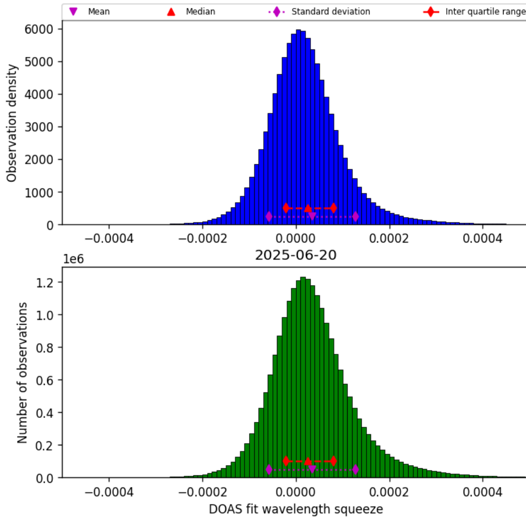
Figure 43: Histogram of “DOAS fit wavelength squeeze” for 2025-06-20 to 2025-06-20
