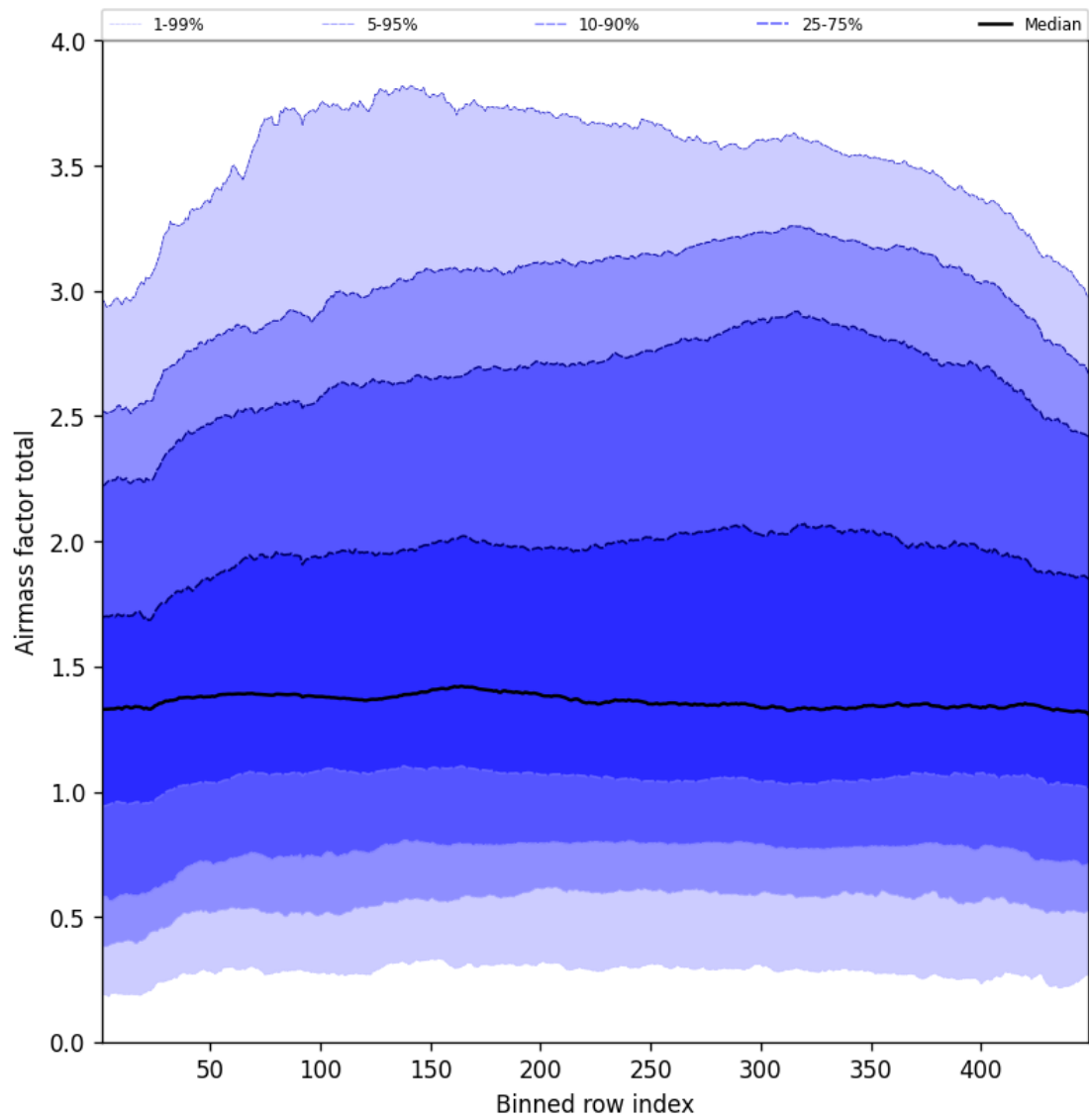
Figure 52: Along track statistics of “Airmass factor total” for 2025-06-20 to 2025-06-20
