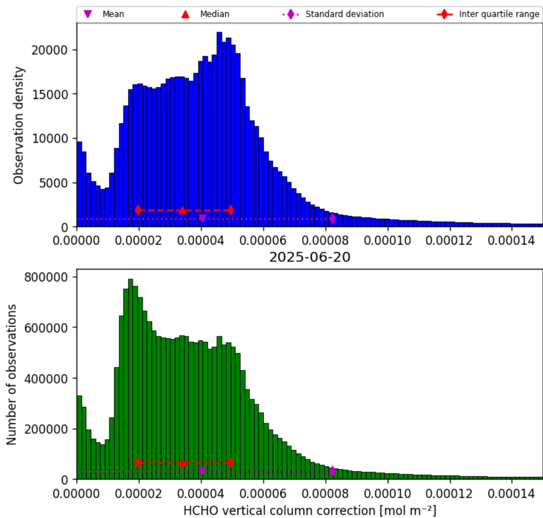
Figure 35: Histogram of “HCHO vertical column correction” for 2025-06-20 to 2025-06-20
