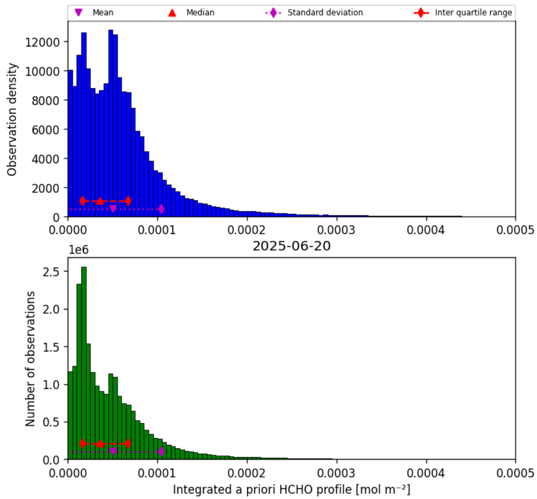
Figure 41: Histogram of “Integrated a priori HCHO profile” for 2025-06-20 to 2025-06-20
