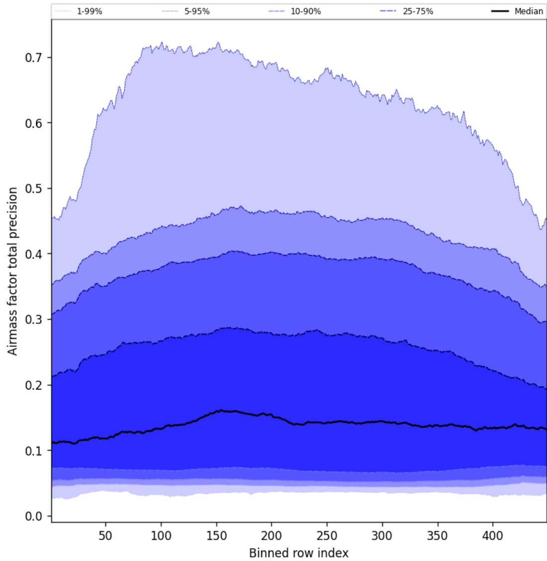
Figure 53: Along track statistics of “Airmass factor total precision” for 2025-06-20 to 2025-06-20
