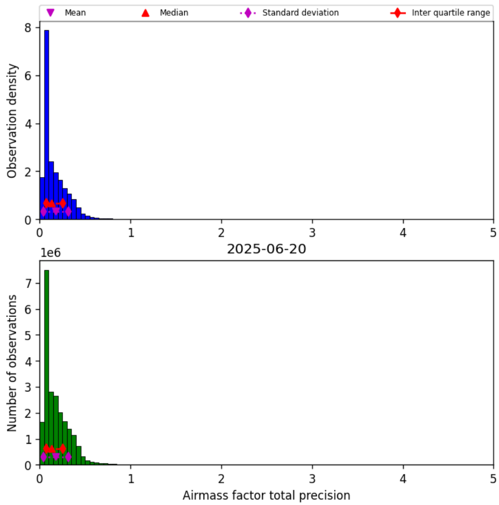
Figure 39: Histogram of “Airmass factor total precision” for 2025-06-20 to 2025-06-20
