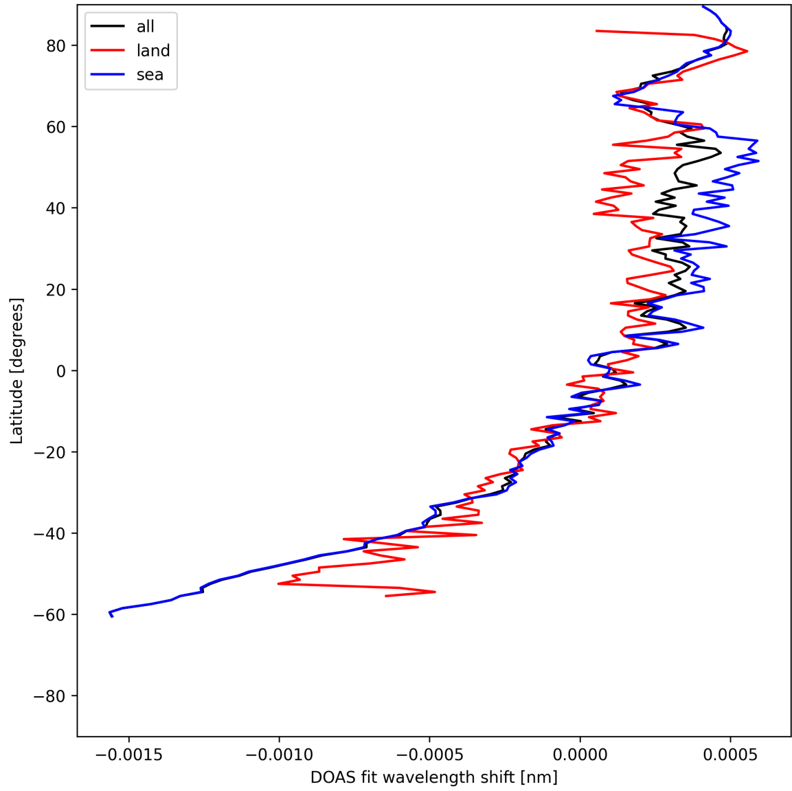
Figure 28: Zonal average of “DOAS fit wavelength shift” for 2025-06-20 to 2025-06-20.
