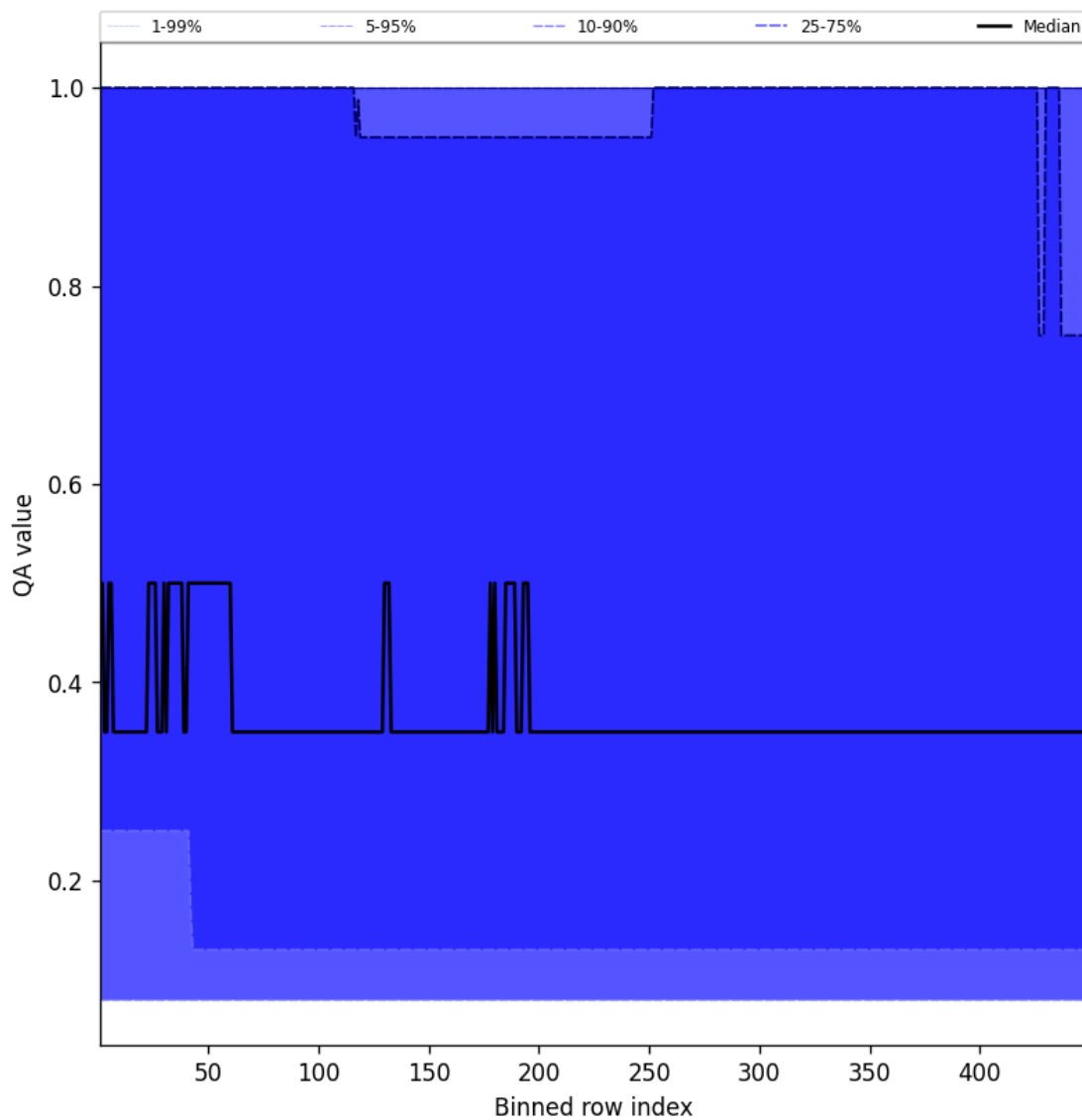
Figure 46: Along track statistics of “QA value” for 2025-06-20 to 2025-06-20
