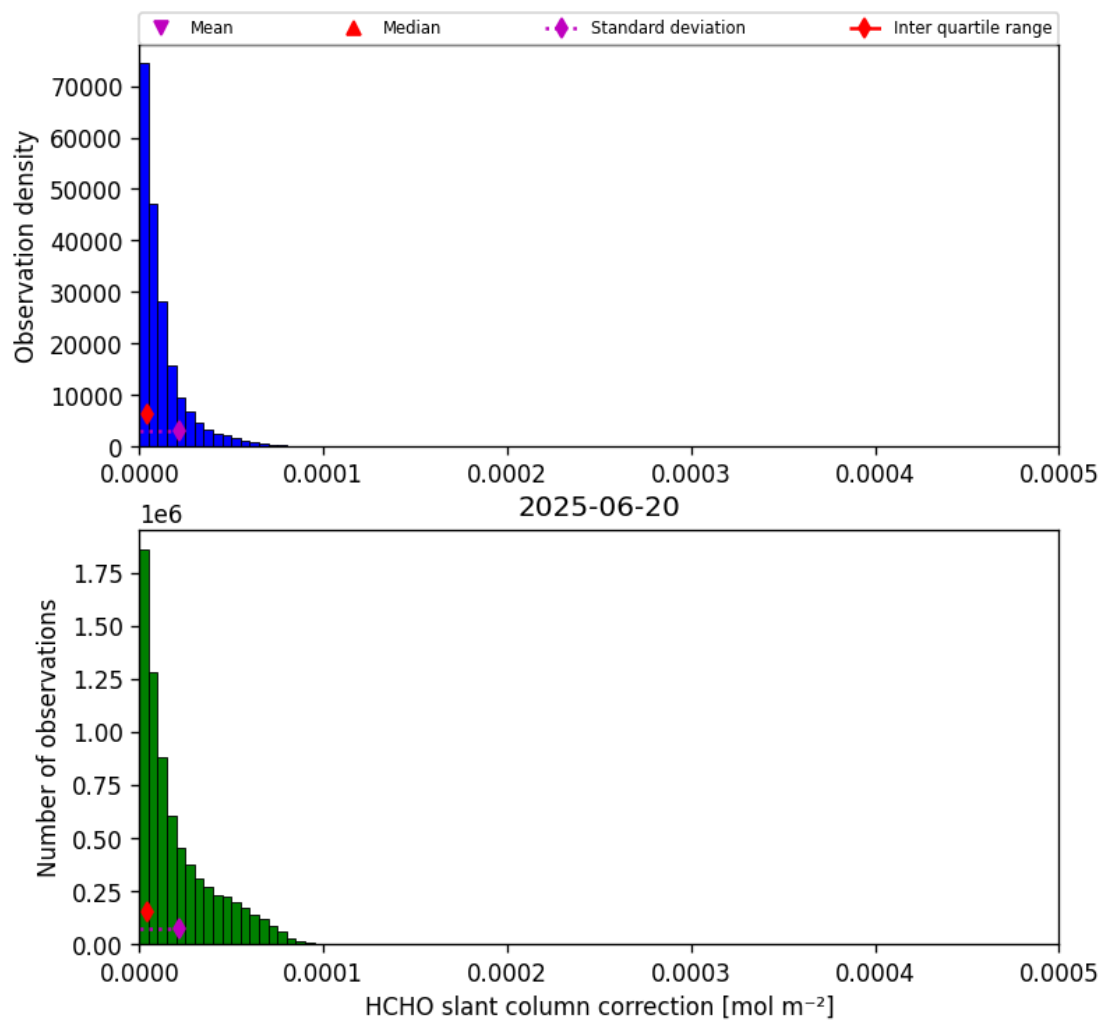
Figure 45: Histogram of “HCHO slant column correction” for 2025-06-20 to 2025-06-20
