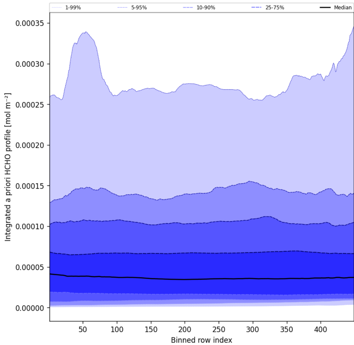
Figure 55: Along track statistics of “Integrated a priori HCHO profile” for 2025-06-20 to 2025-06-20
