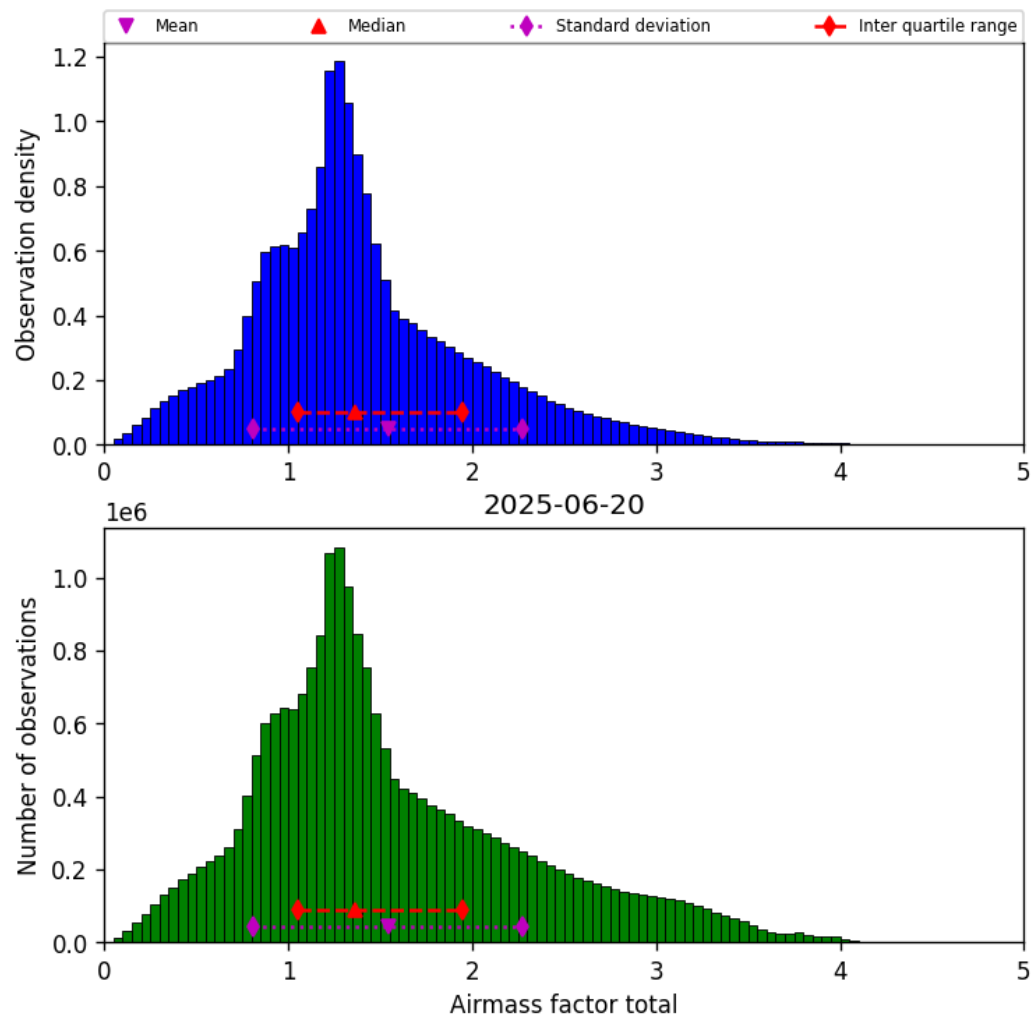
Figure 38: Histogram of “Airmass factor total” for 2025-06-20 to 2025-06-20
