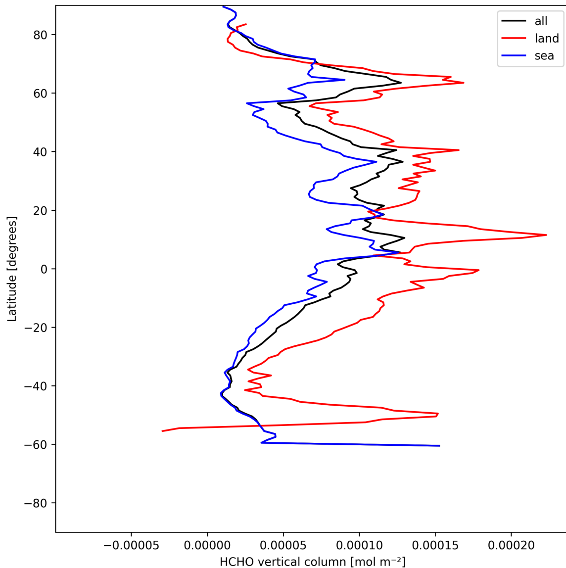
Figure 19: Zonal average of “HCHO vertical column” for 2025-06-20 to 2025-06-20.
