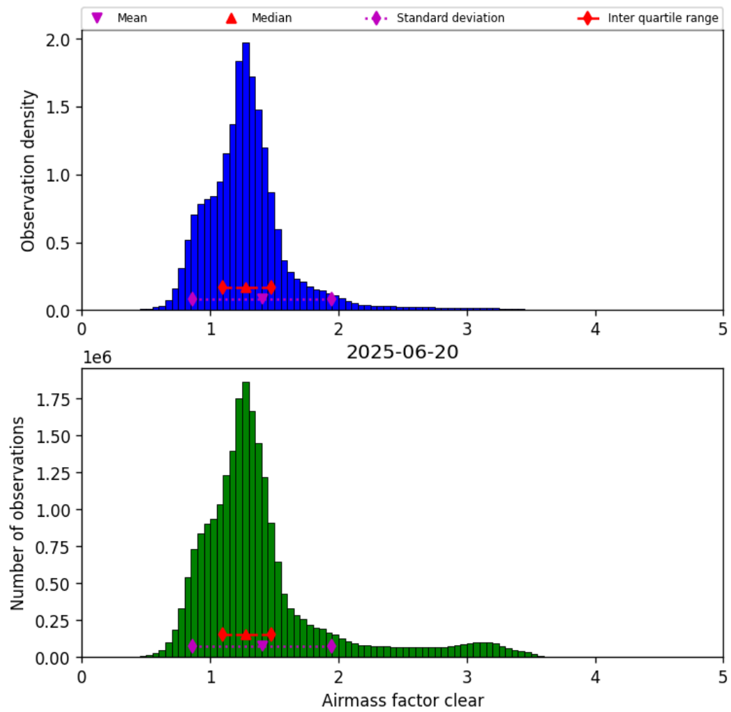
Figure 40: Histogram of “Airmass factor clear” for 2025-06-20 to 2025-06-20
