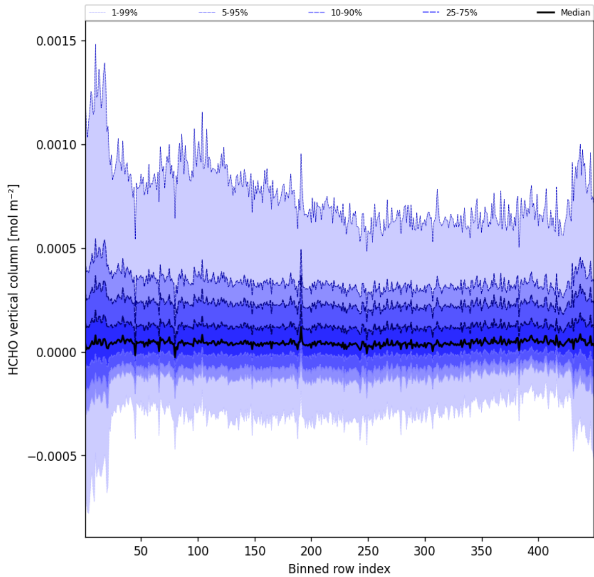
Figure 47: Along track statistics of “HCHO vertical column” for 2025-06-20 to 2025-06-20
