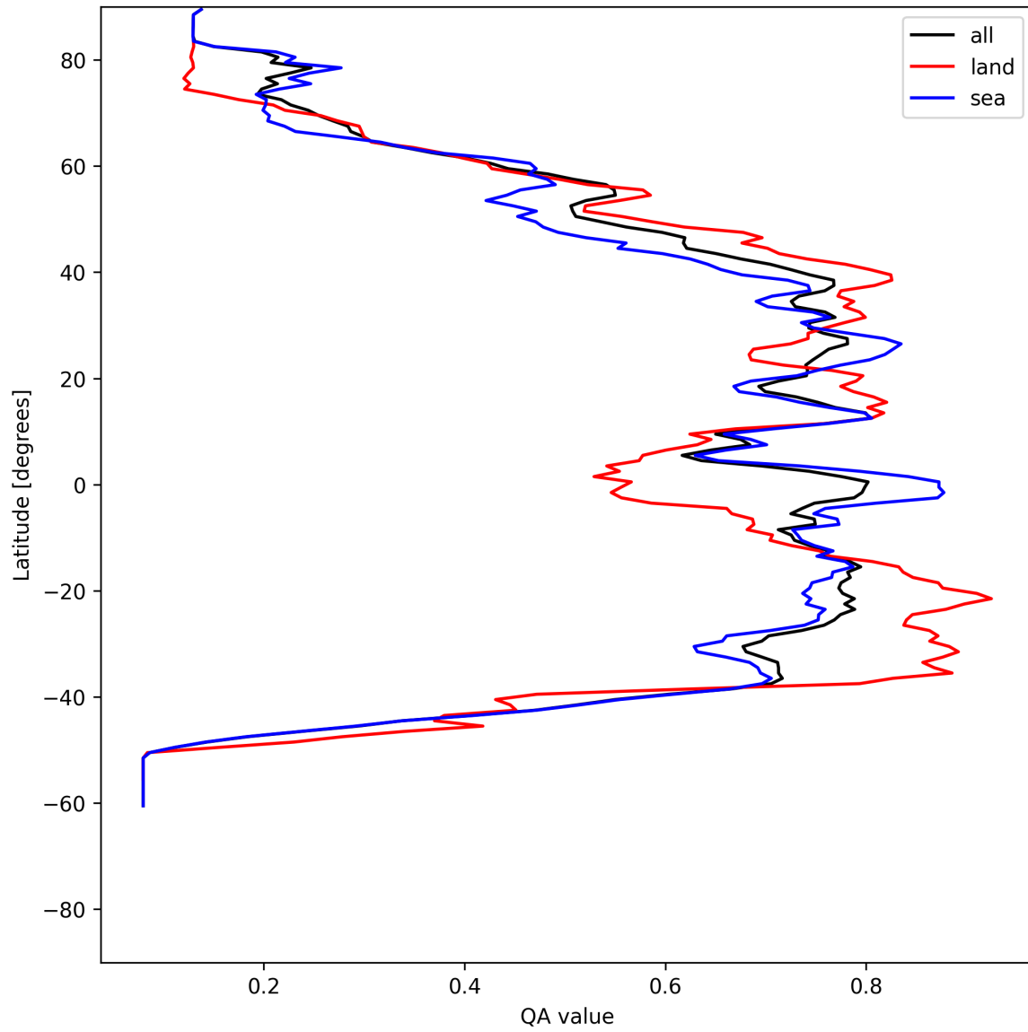
Figure 18: Zonal average of “QA value” for 2025-06-20 to 2025-06-20.
