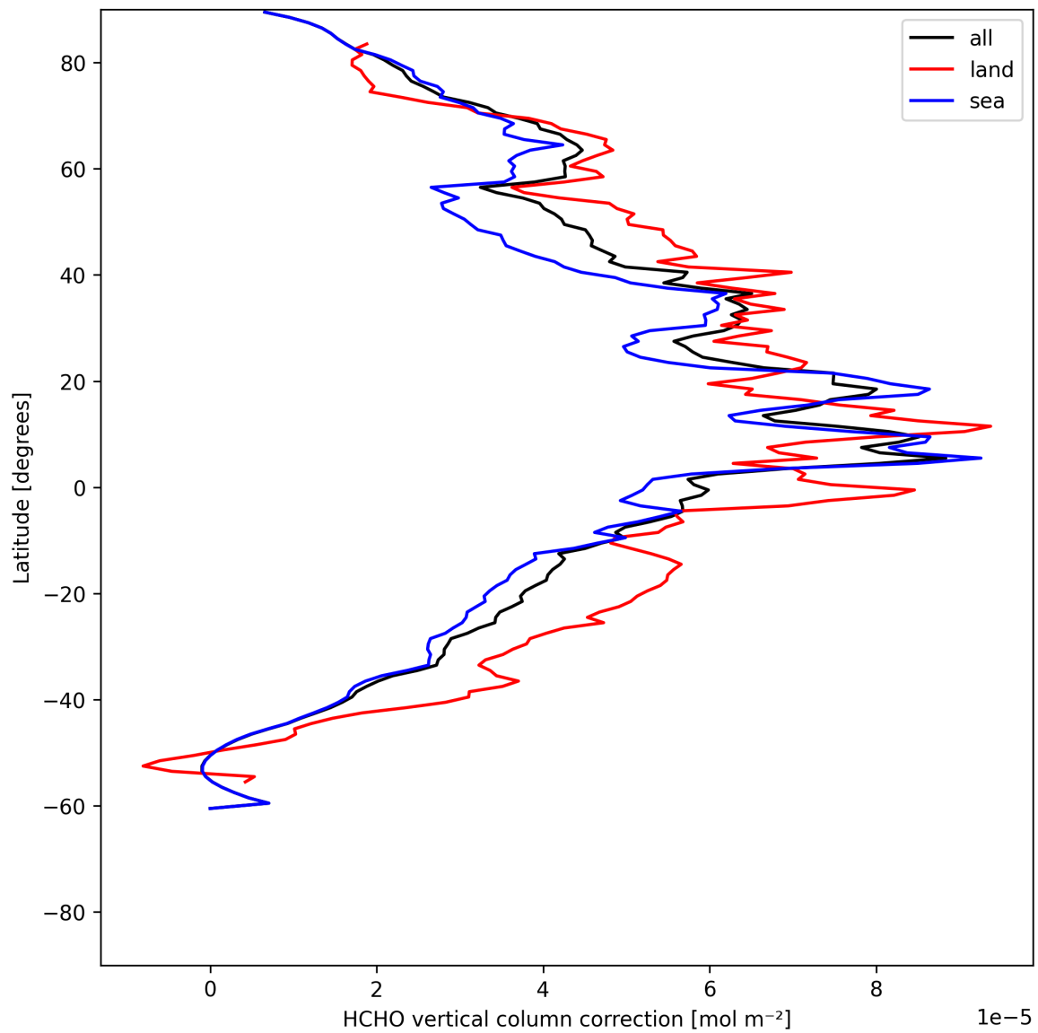
Figure 21: Zonal average of “HCHO vertical column correction” for 2025-06-20 to 2025-06-20.
