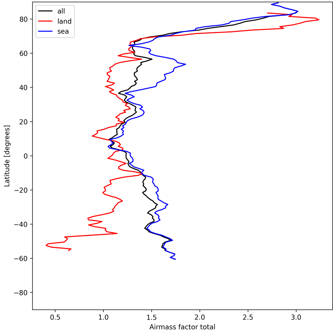
Figure 24: Zonal average of “Airmass factor total” for 2025-06-20 to 2025-06-20.
