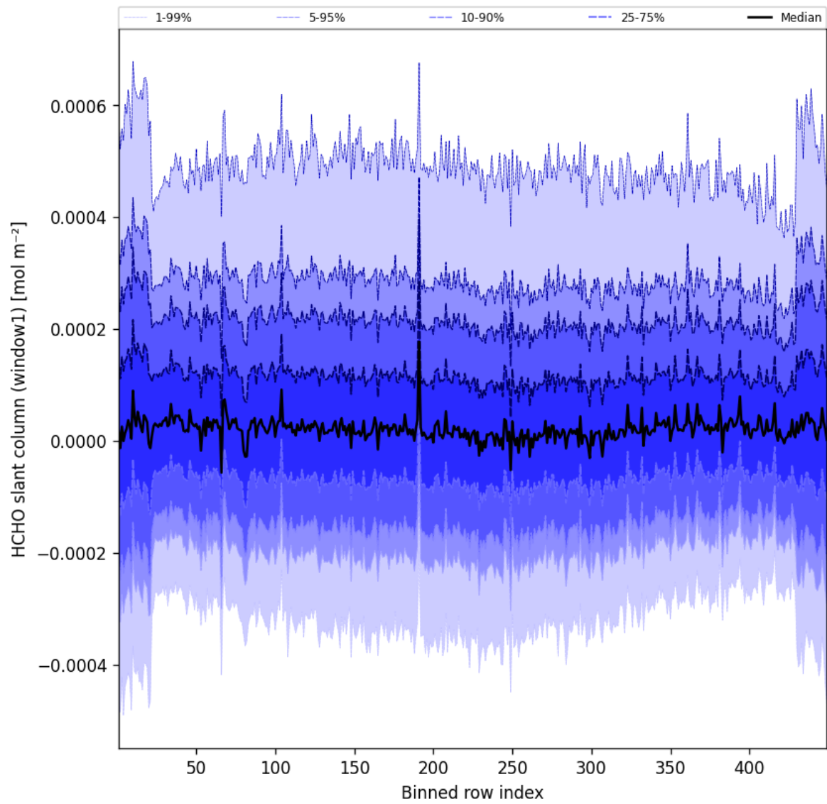
Figure 50: Along track statistics of “HCHO slant column (window1)” for 2025-06-20 to 2025-06-20
