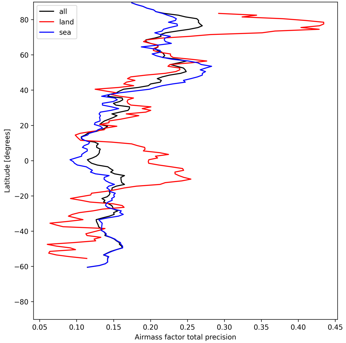
Figure 25: Zonal average of “Airmass factor total precision” for 2025-06-20 to 2025-06-20.
