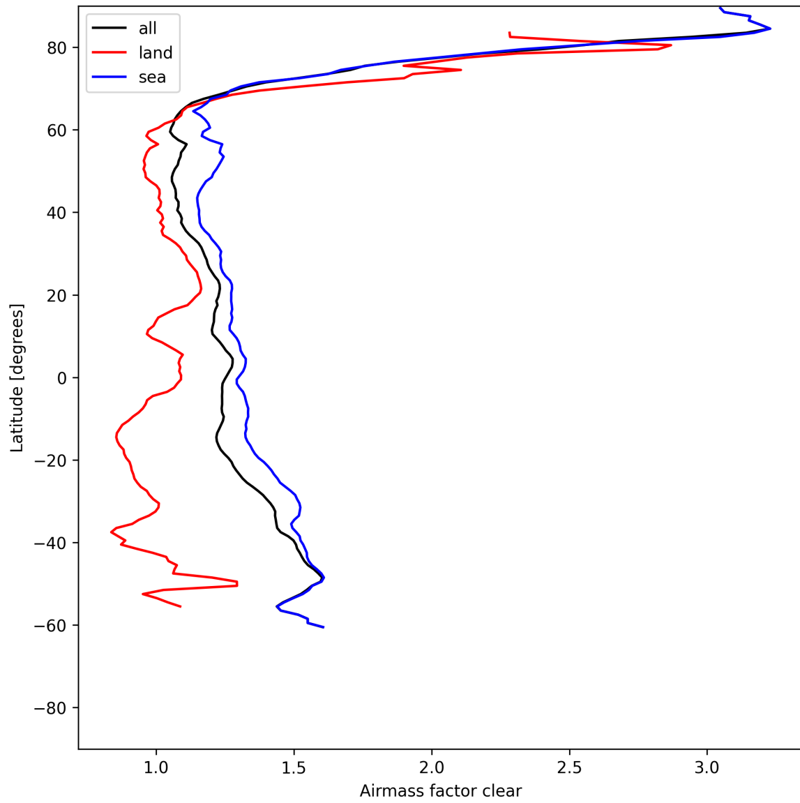
Figure 26: Zonal average of “Airmass factor clear” for 2025-06-20 to 2025-06-20.
