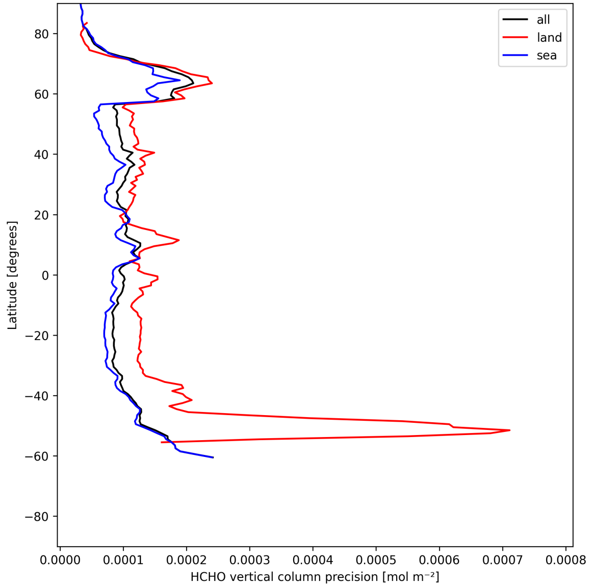
Figure 20: Zonal average of “HCHO vertical column precision” for 2025-06-20 to 2025-06-20.
