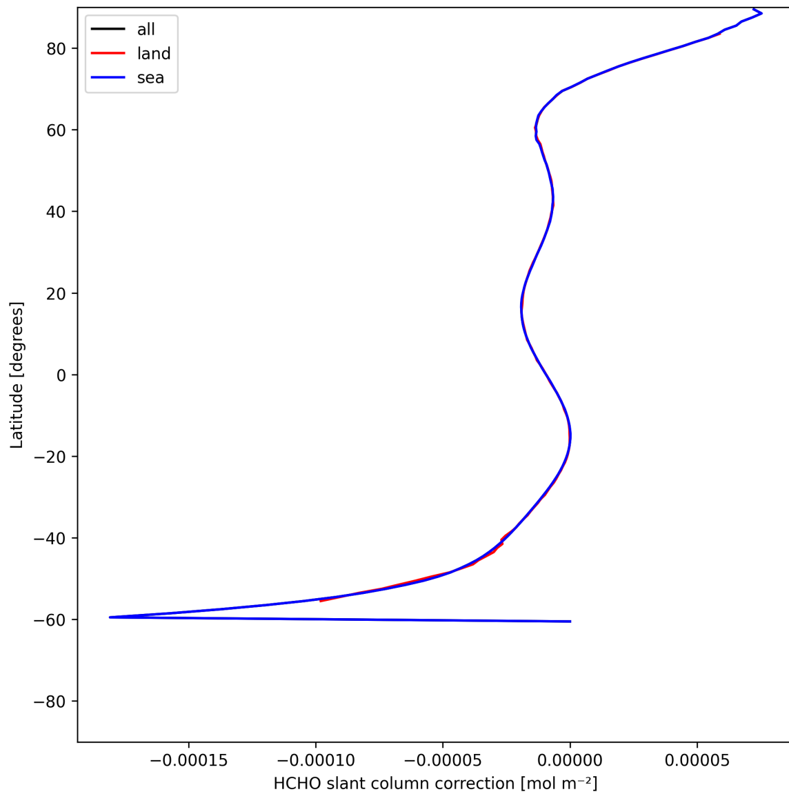
Figure 31: Zonal average of “HCHO slant column correction” for 2025-06-20 to 2025-06-20.
