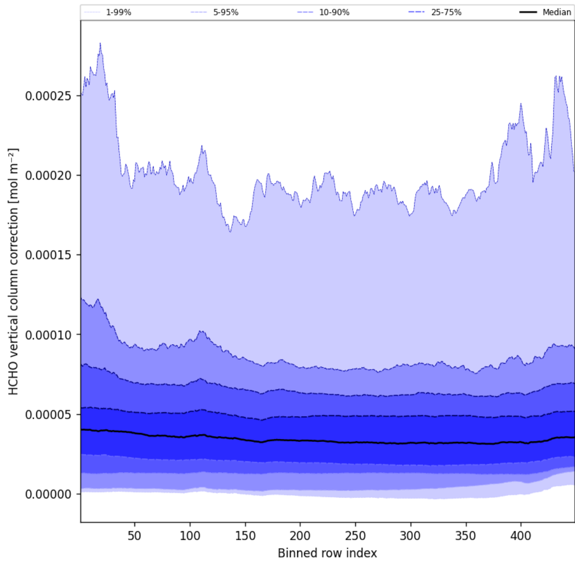
Figure 49: Along track statistics of “HCHO vertical column correction” for 2025-06-20 to 2025-06-20
