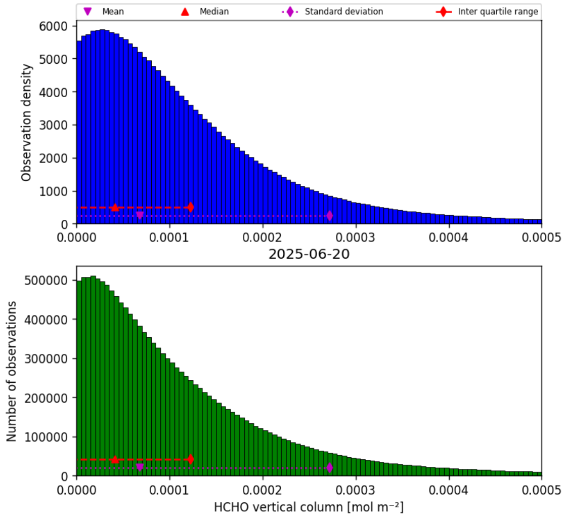
Figure 33: Histogram of “HCHO vertical column” for 2025-06-20 to 2025-06-20
