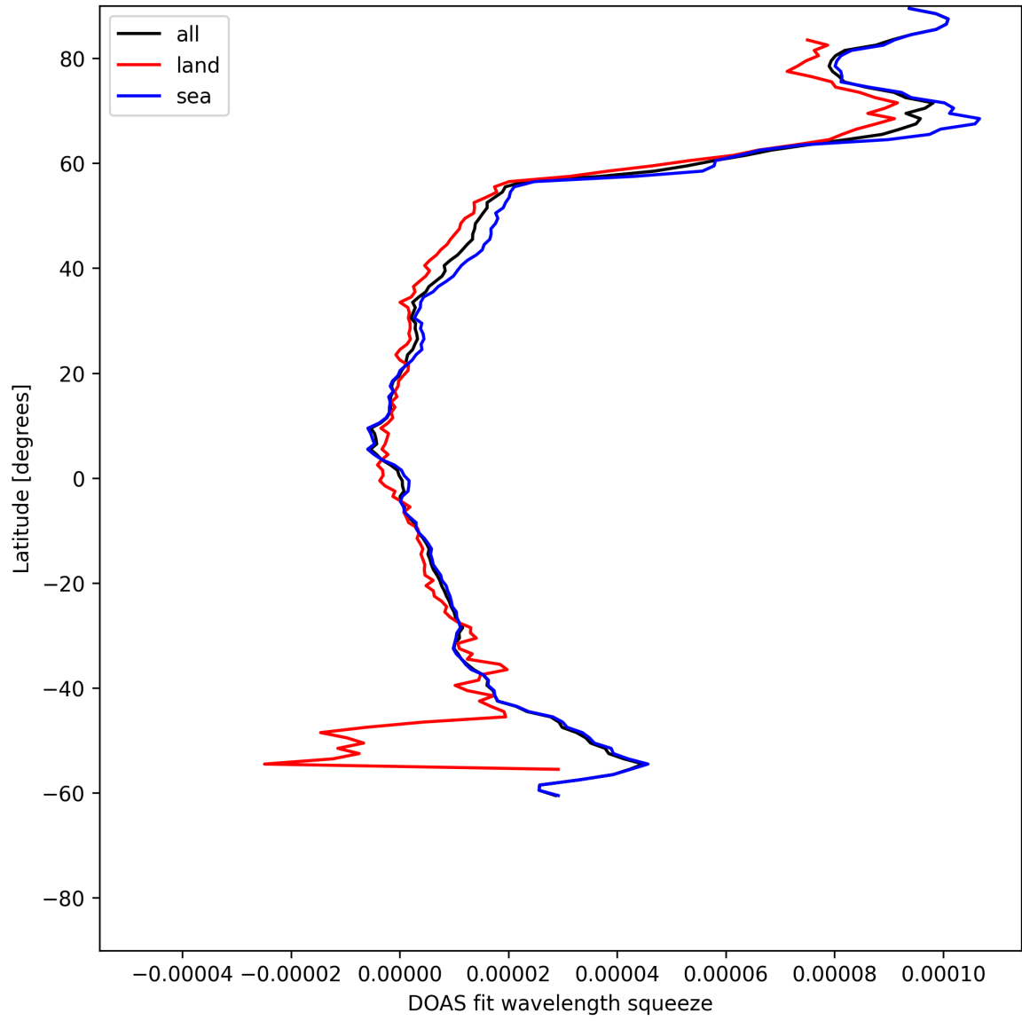
Figure 29: Zonal average of “DOAS fit wavelength squeeze” for 2025-06-20 to 2025-06-20.
