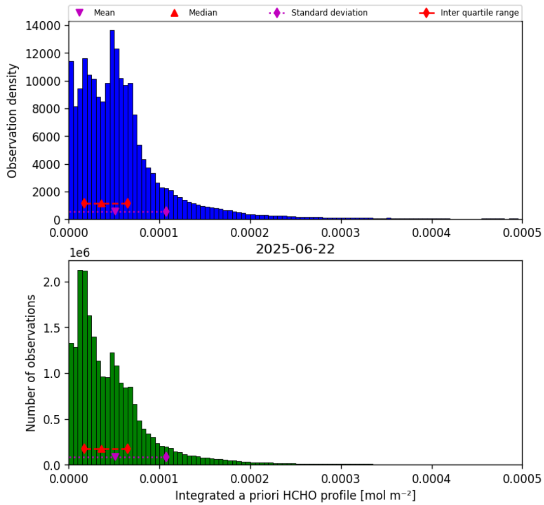
Figure 41: Histogram of “Integrated a priori HCHO profile” for 2025-06-22 to 2025-06-23
