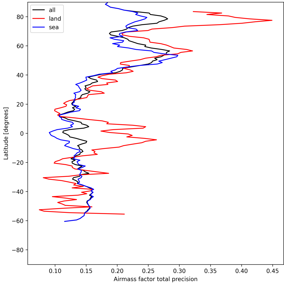
Figure 25: Zonal average of “Airmass factor total precision” for 2025-06-22 to 2025-06-23.
