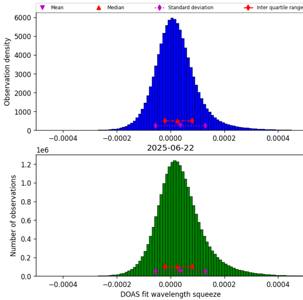
Figure 43: Histogram of “DOAS fit wavelength squeeze” for 2025-06-22 to 2025-06-23
