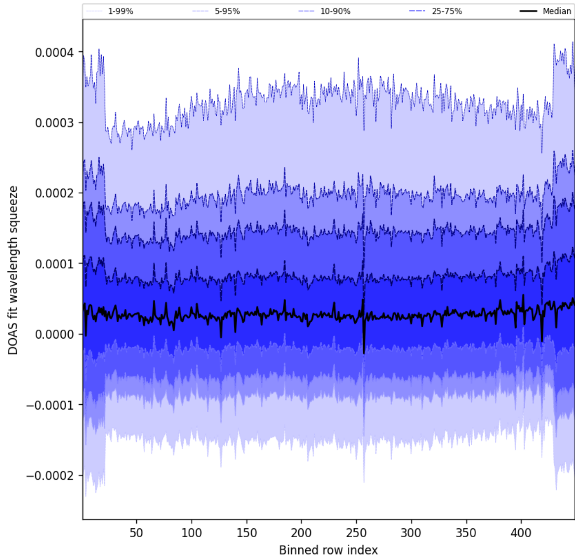
Figure 57: Along track statistics of “DOAS fit wavelength squeeze” for 2025-06-22 to 2025-06-23
