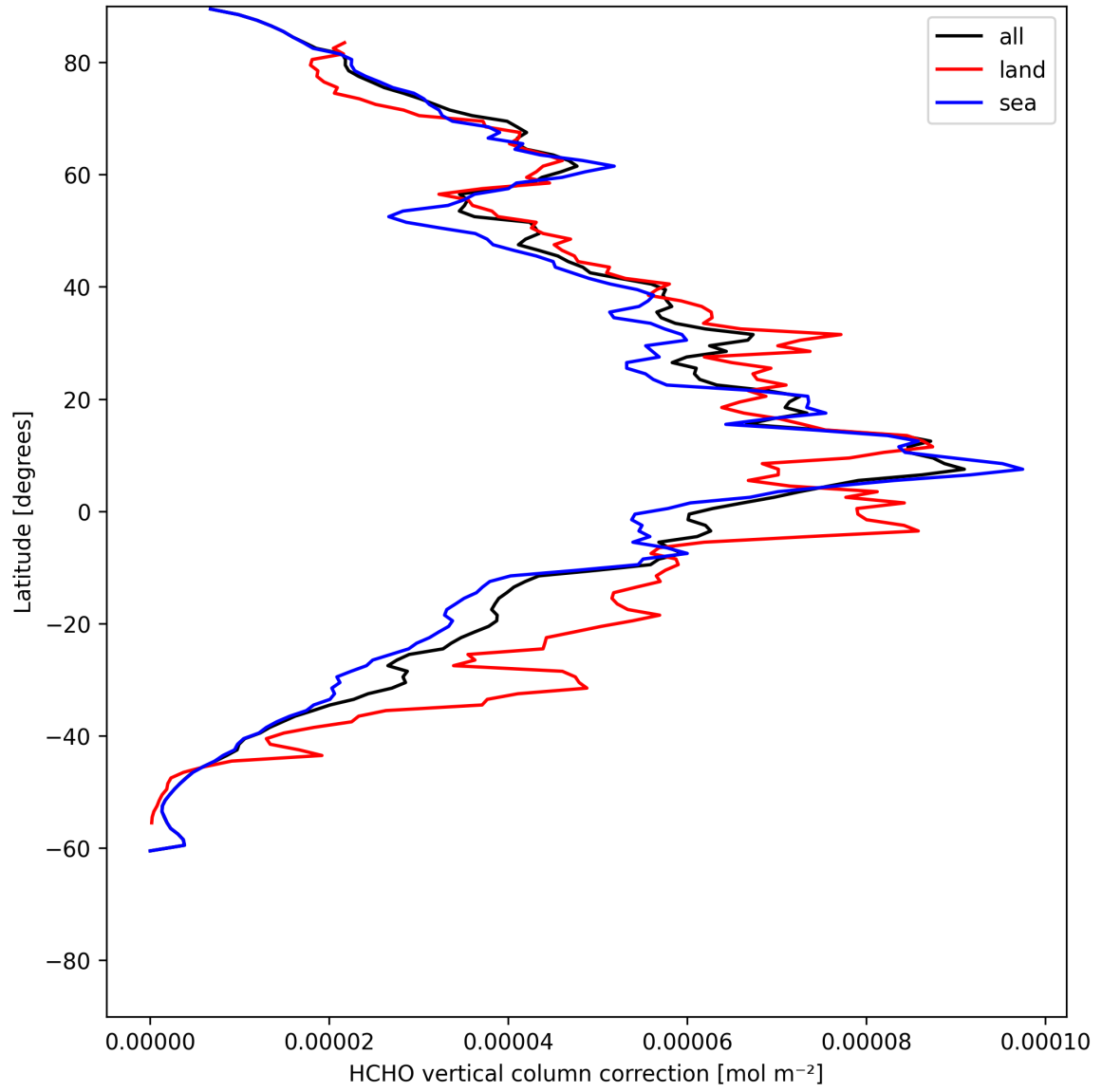
Figure 21: Zonal average of “HCHO vertical column correction” for 2025-06-22 to 2025-06-23.
