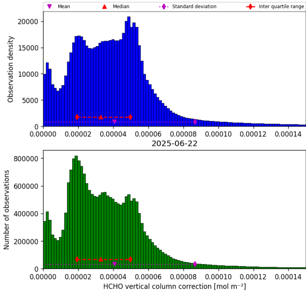
Figure 35: Histogram of “HCHO vertical column correction” for 2025-06-22 to 2025-06-23
