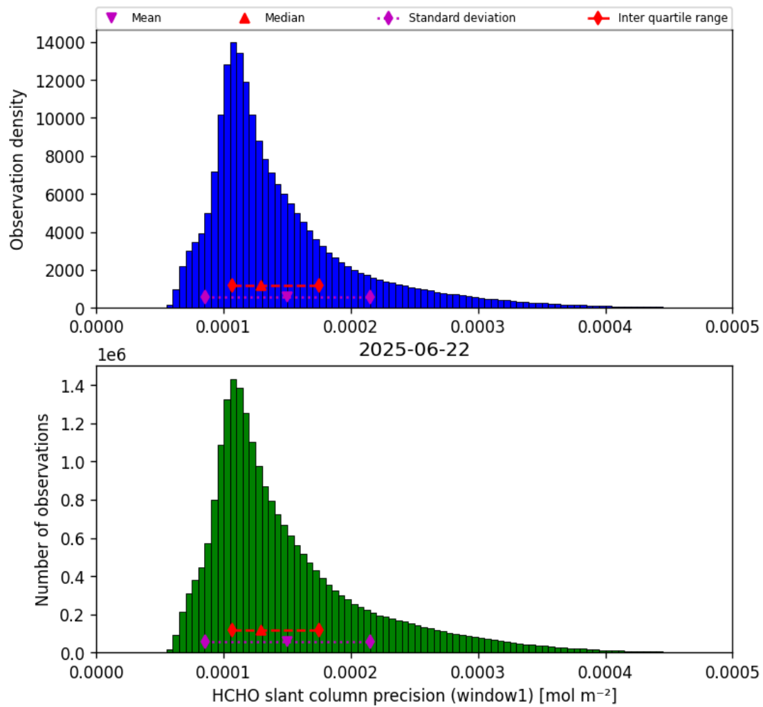
Figure 37: Histogram of “HCHO slant column precision (window1)” for 2025-06-22 to 2025-06-23
