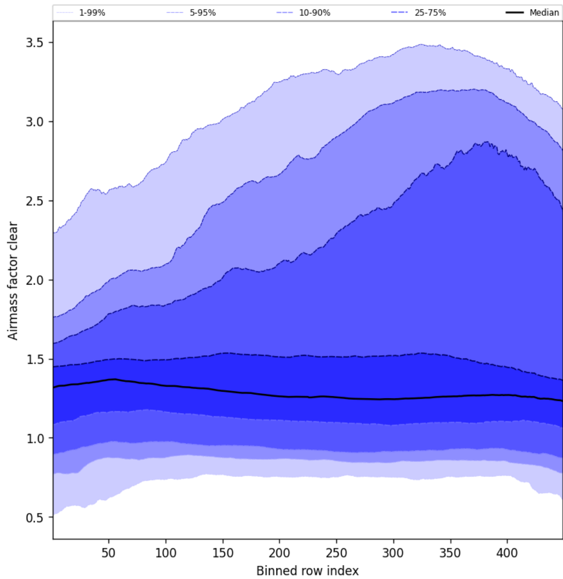
Figure 54: Along track statistics of “Airmass factor clear” for 2025-06-22 to 2025-06-23
