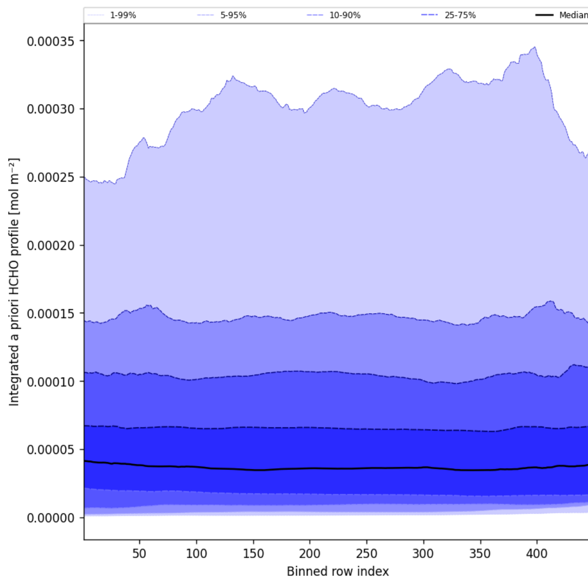
Figure 55: Along track statistics of “Integrated a priori HCHO profile” for 2025-06-22 to 2025-06-23
