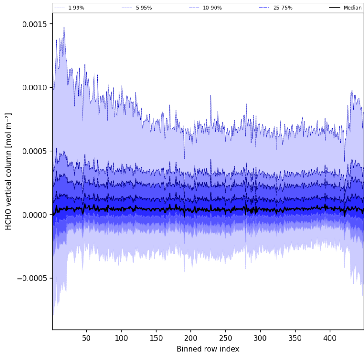
Figure 47: Along track statistics of “HCHO vertical column” for 2025-06-22 to 2025-06-23
