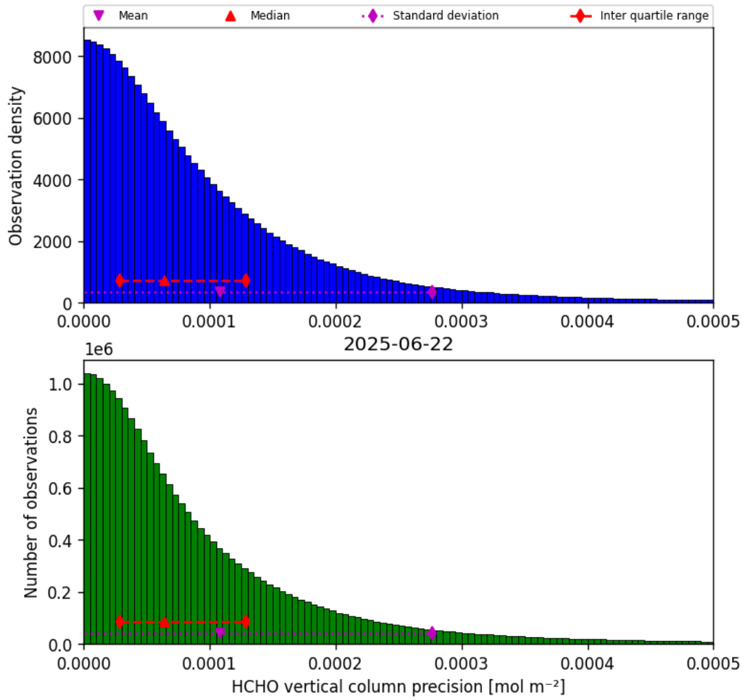
Figure 34: Histogram of “HCHO vertical column precision” for 2025-06-22 to 2025-06-23
