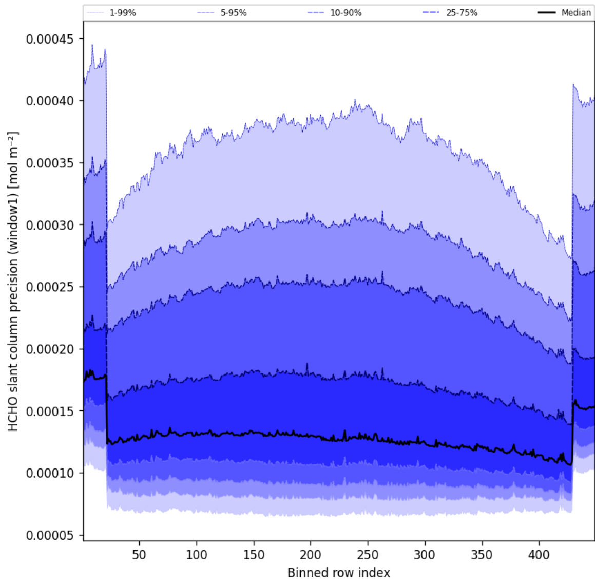
Figure 51: Along track statistics of “HCHO slant column precision (window1)” for 2025-06-22 to 2025-06-23
