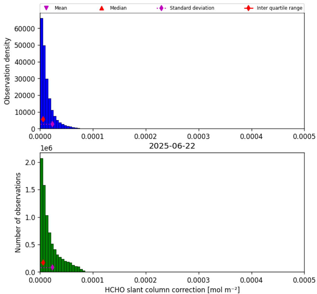
Figure 45: Histogram of “HCHO slant column correction” for 2025-06-22 to 2025-06-23
