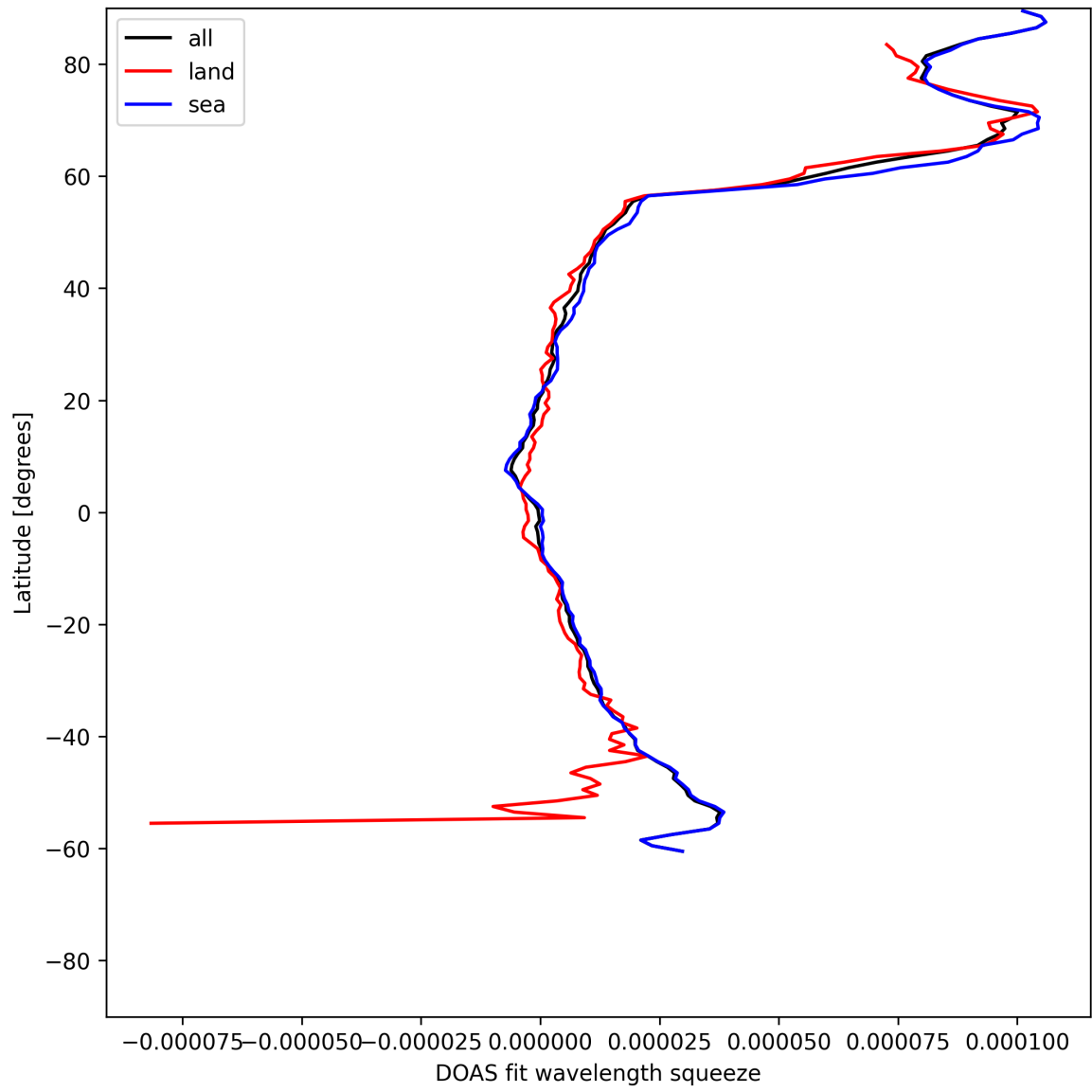
Figure 29: Zonal average of “DOAS fit wavelength squeeze” for 2025-06-22 to 2025-06-23.
