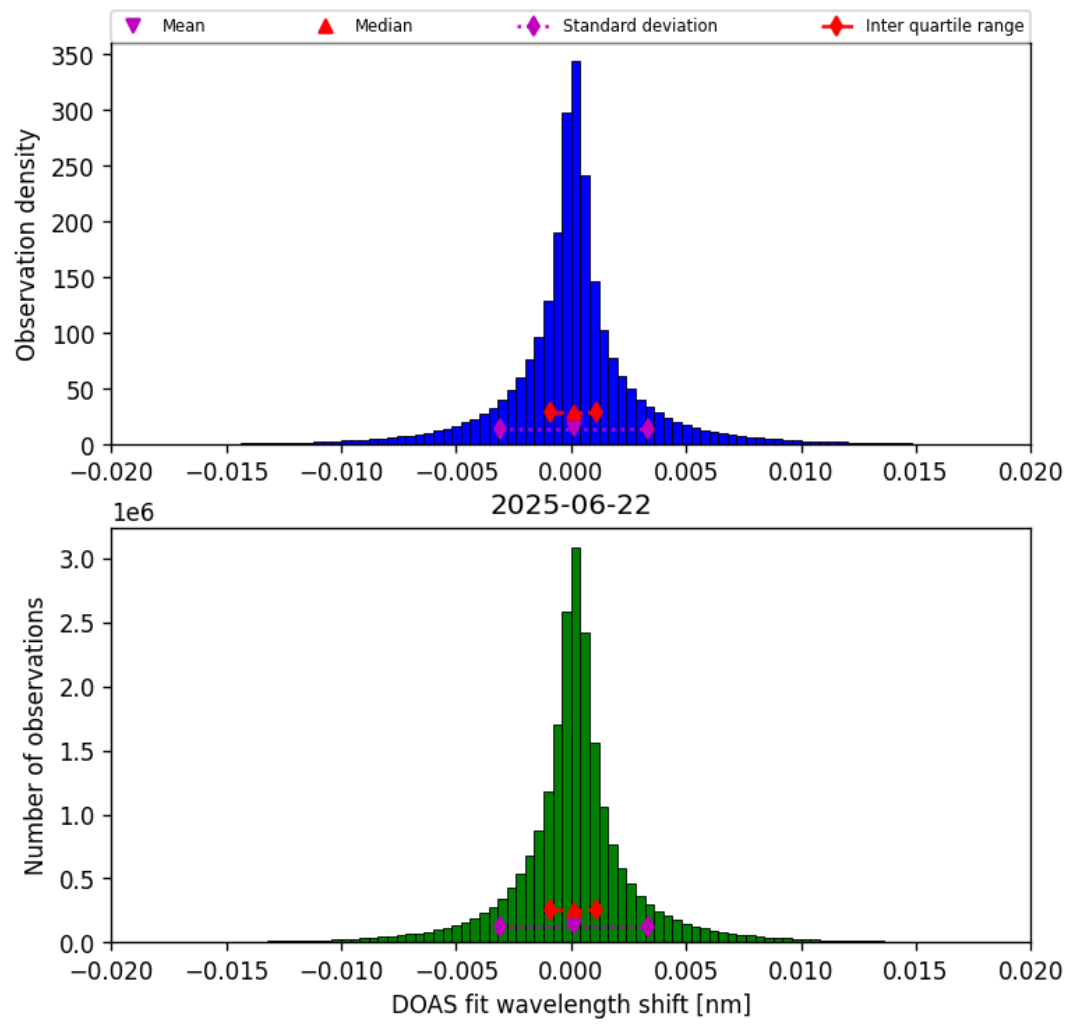
Figure 42: Histogram of “DOAS fit wavelength shift” for 2025-06-22 to 2025-06-23
