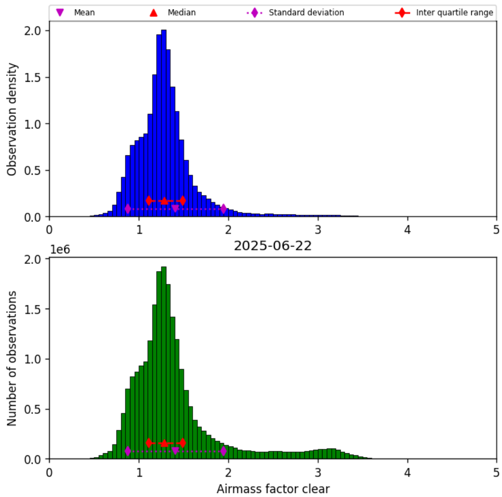
Figure 40: Histogram of “Airmass factor clear” for 2025-06-22 to 2025-06-23
