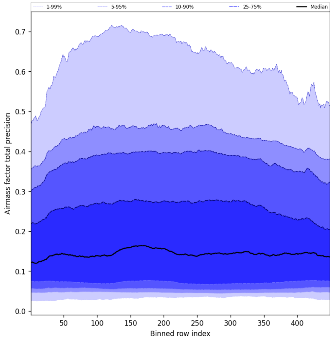
Figure 53: Along track statistics of “Airmass factor total precision” for 2025-06-22 to 2025-06-23
