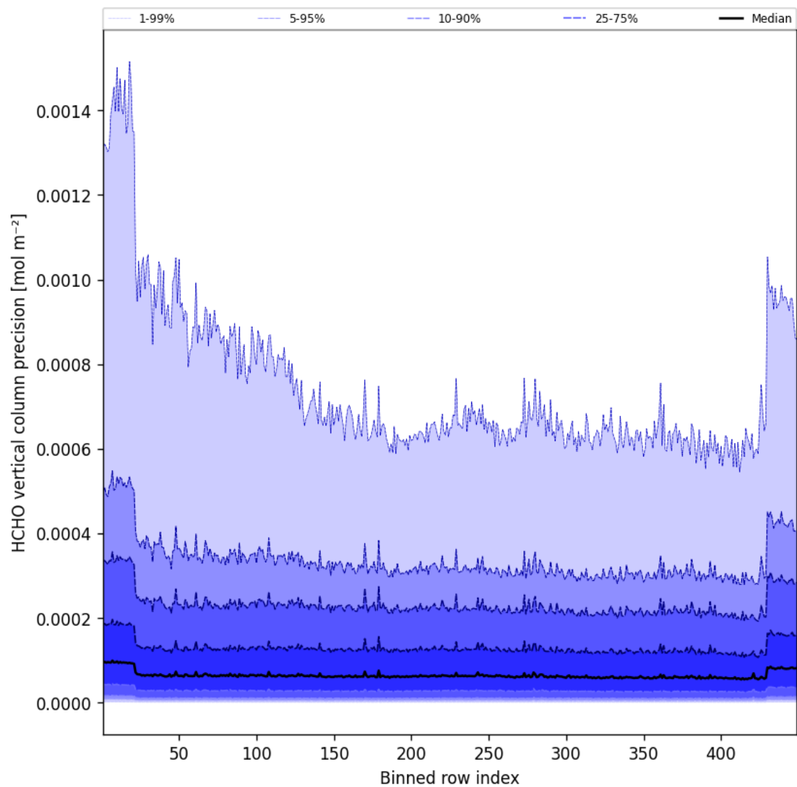
Figure 48: Along track statistics of “HCHO vertical column precision” for 2025-06-22 to 2025-06-23
