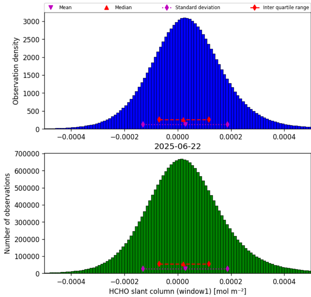
Figure 36: Histogram of “HCHO slant column (window1)” for 2025-06-22 to 2025-06-23
