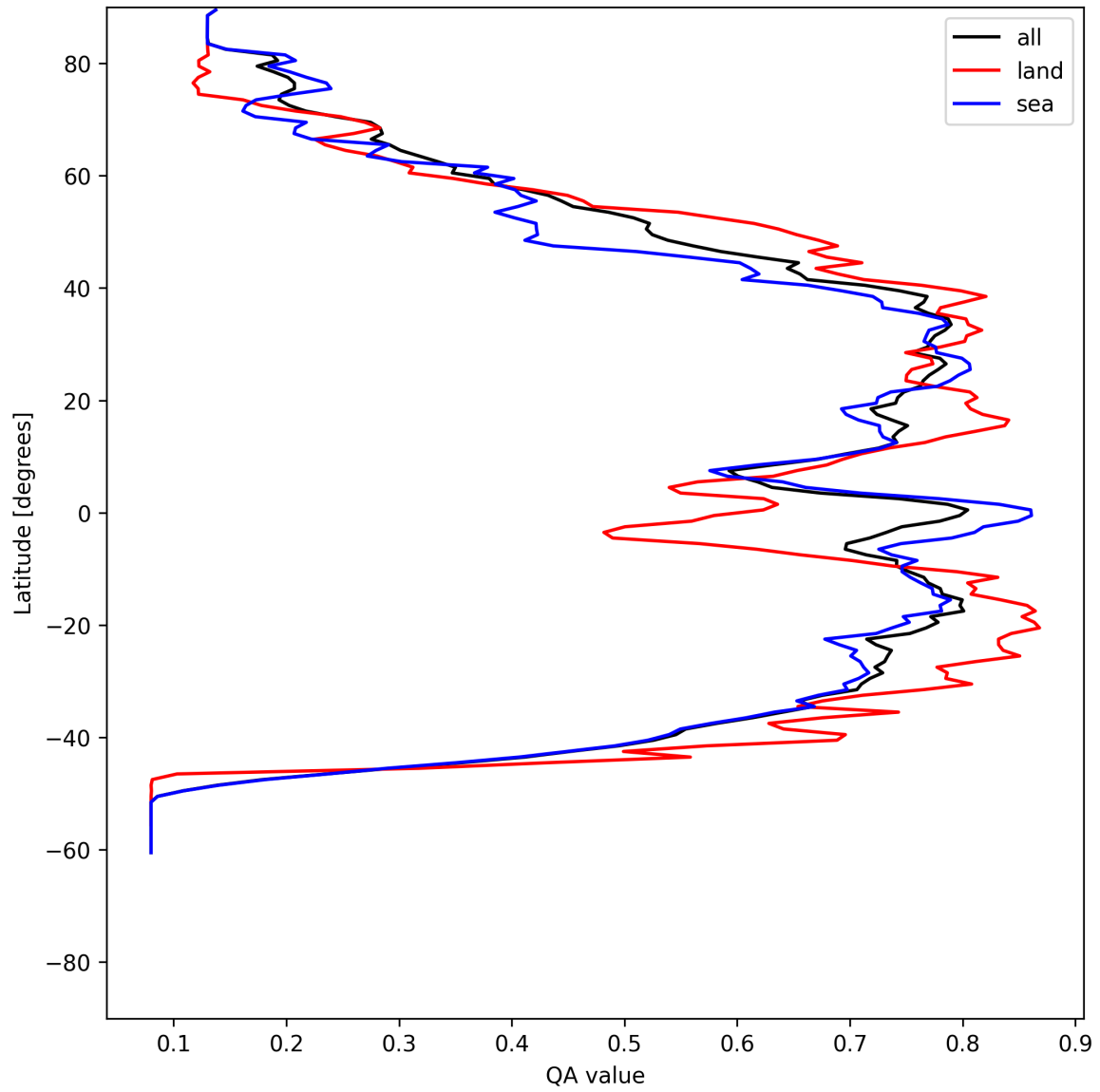
Figure 18: Zonal average of “QA value” for 2025-06-22 to 2025-06-23.
