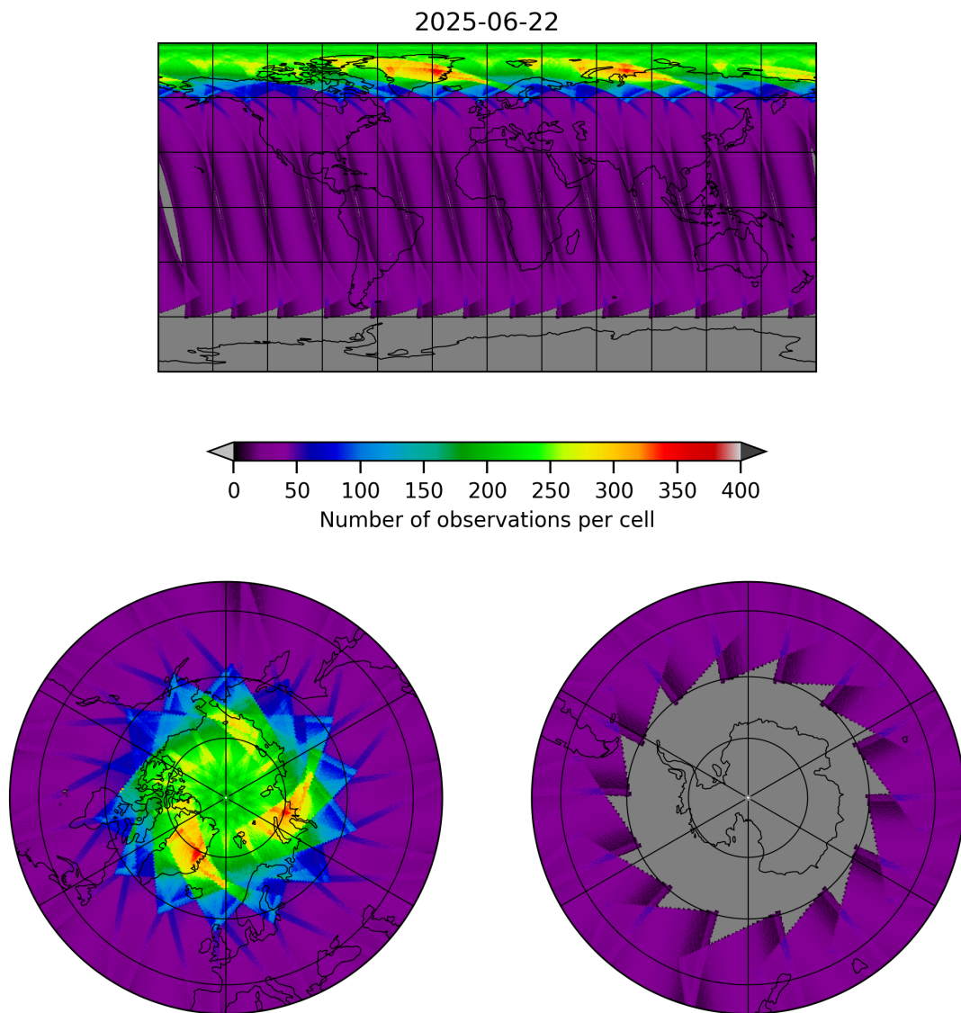
Figure 17: Map of the number of observations for 2025-06-22 to 2025-06-23
