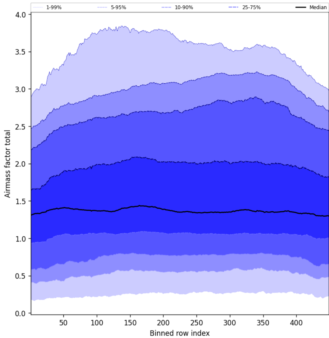
Figure 52: Along track statistics of “Airmass factor total” for 2025-06-22 to 2025-06-23
