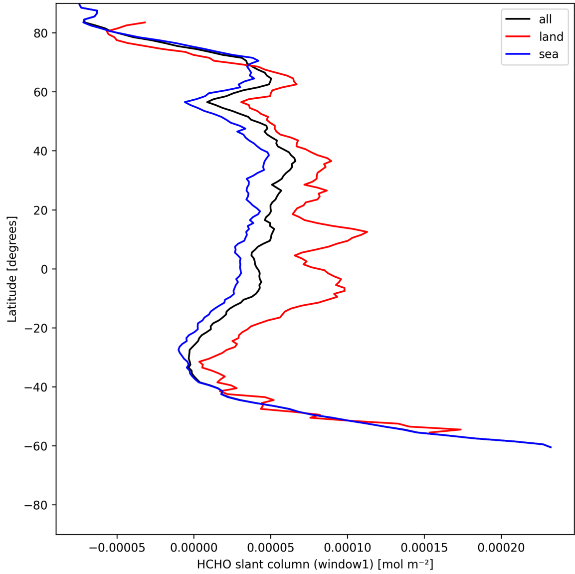
Figure 22: Zonal average of “HCHO slant column (window1)” for 2025-06-22 to 2025-06-23.
