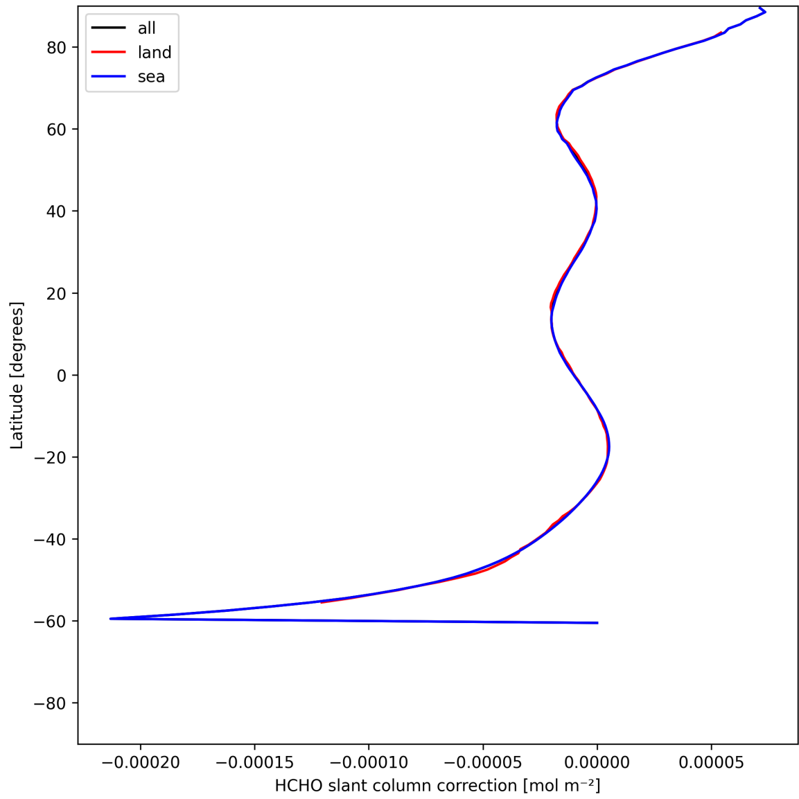
Figure 31: Zonal average of “HCHO slant column correction” for 2025-06-22 to 2025-06-23.
