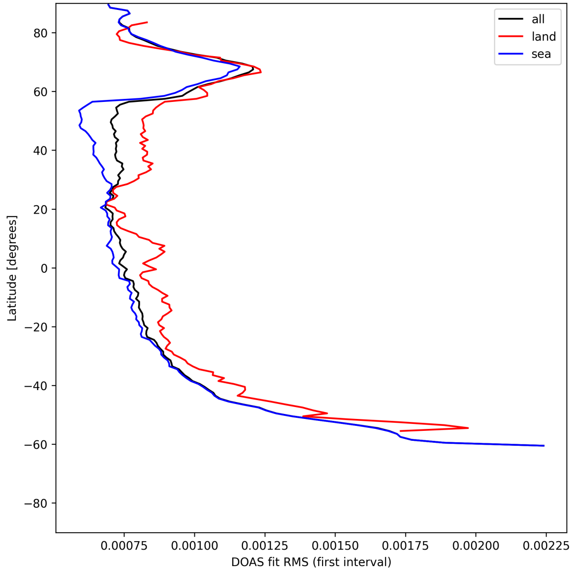
Figure 30: Zonal average of “DOAS fit RMS (first interval)” for 2025-06-22 to 2025-06-23.
