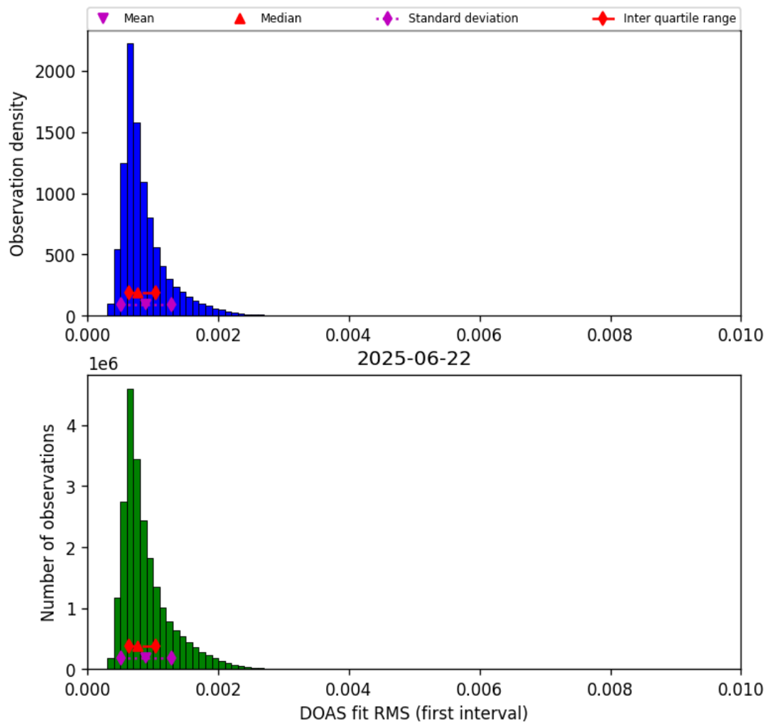
Figure 44: Histogram of “DOAS fit RMS (first interval)” for 2025-06-22 to 2025-06-23
