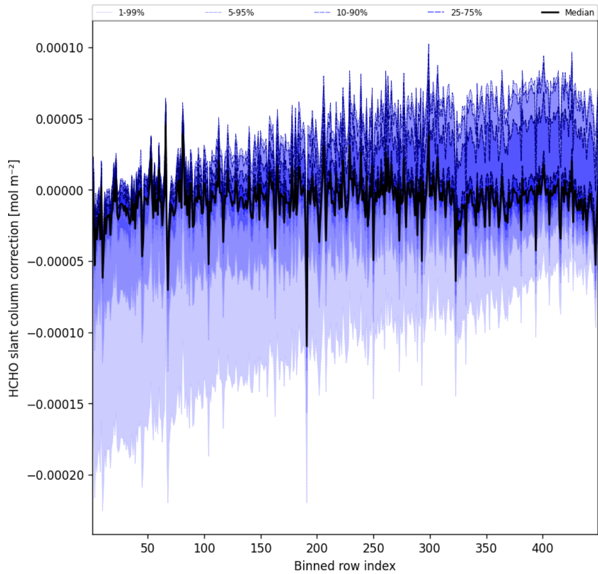
Figure 59: Along track statistics of “HCHO slant column correction” for 2025-06-22 to 2025-06-23
