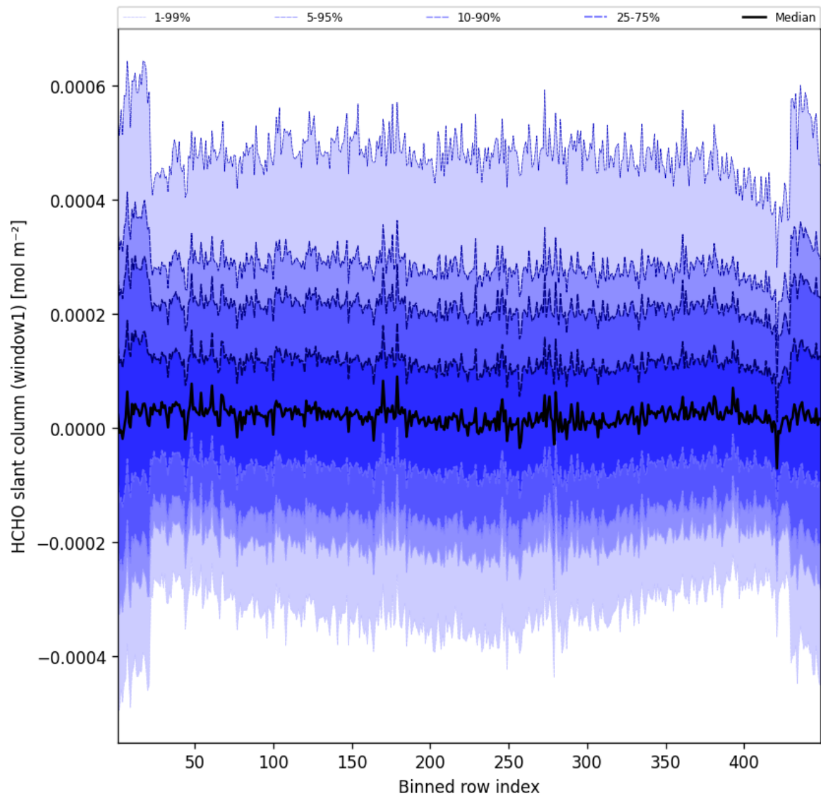
Figure 50: Along track statistics of “HCHO slant column (window1)” for 2025-06-22 to 2025-06-23
