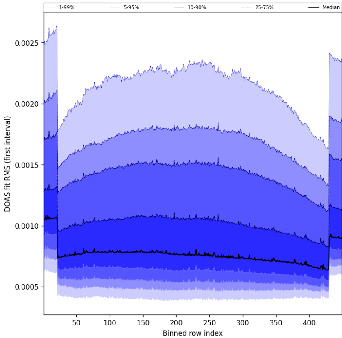
Figure 58: Along track statistics of “DOAS fit RMS (first interval)” for 2025-06-22 to 2025-06-23
