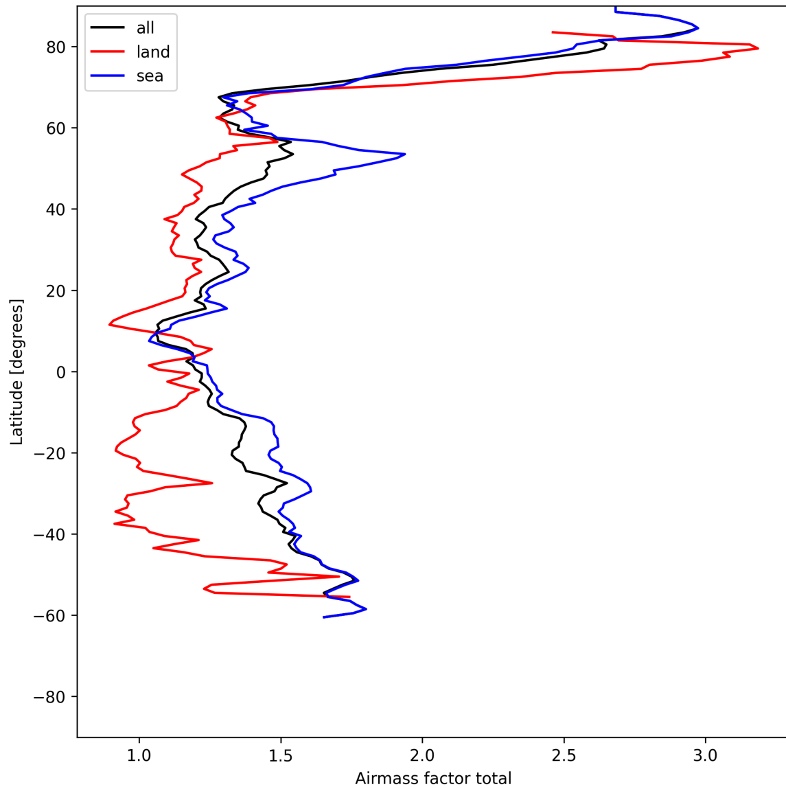
Figure 24: Zonal average of “Airmass factor total” for 2025-06-22 to 2025-06-23.
