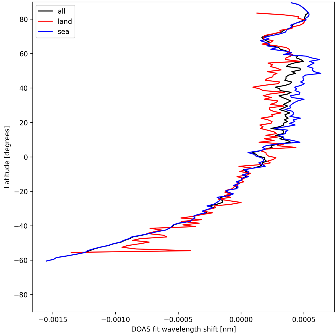
Figure 28: Zonal average of “DOAS fit wavelength shift” for 2025-06-22 to 2025-06-23.
