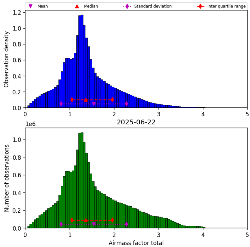
Figure 38: Histogram of “Airmass factor total” for 2025-06-22 to 2025-06-23
