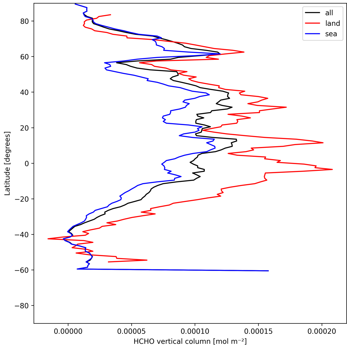
Figure 19: Zonal average of “HCHO vertical column” for 2025-06-22 to 2025-06-23.
