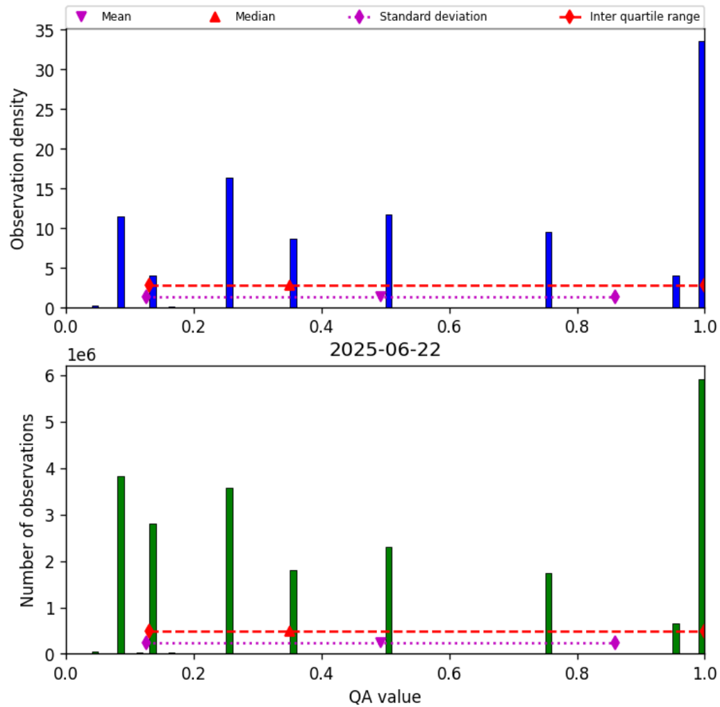
Figure 32: Histogram of “QA value” for 2025-06-22 to 2025-06-23
