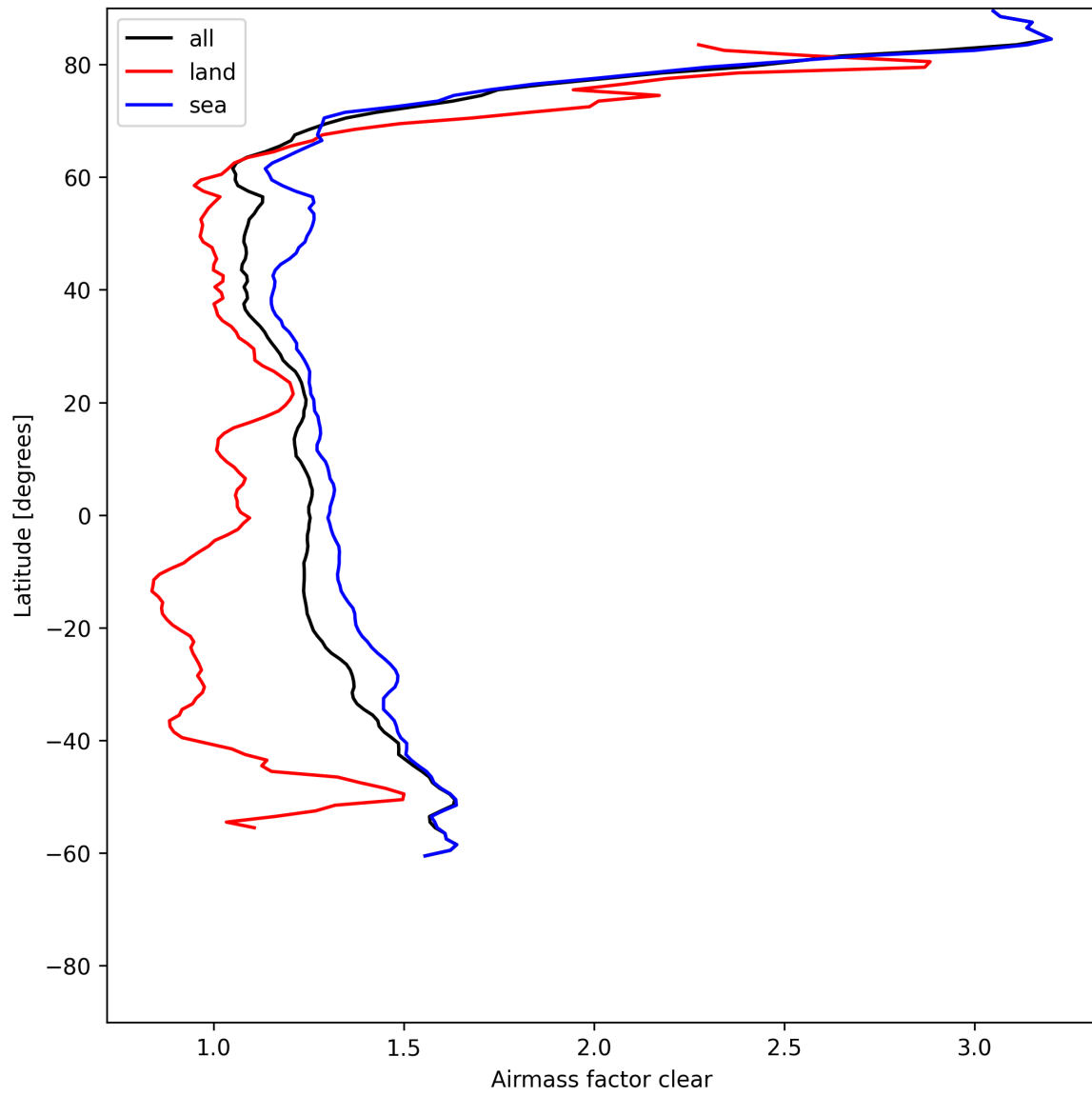
Figure 26: Zonal average of “Airmass factor clear” for 2025-06-22 to 2025-06-23.
