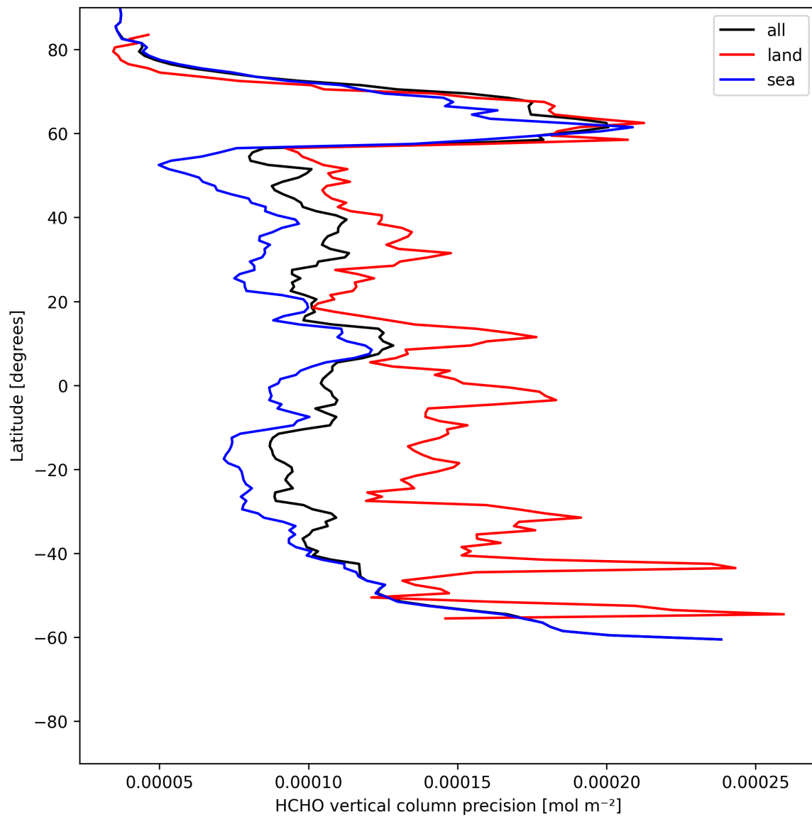
Figure 20: Zonal average of “HCHO vertical column precision” for 2025-06-22 to 2025-06-23.
