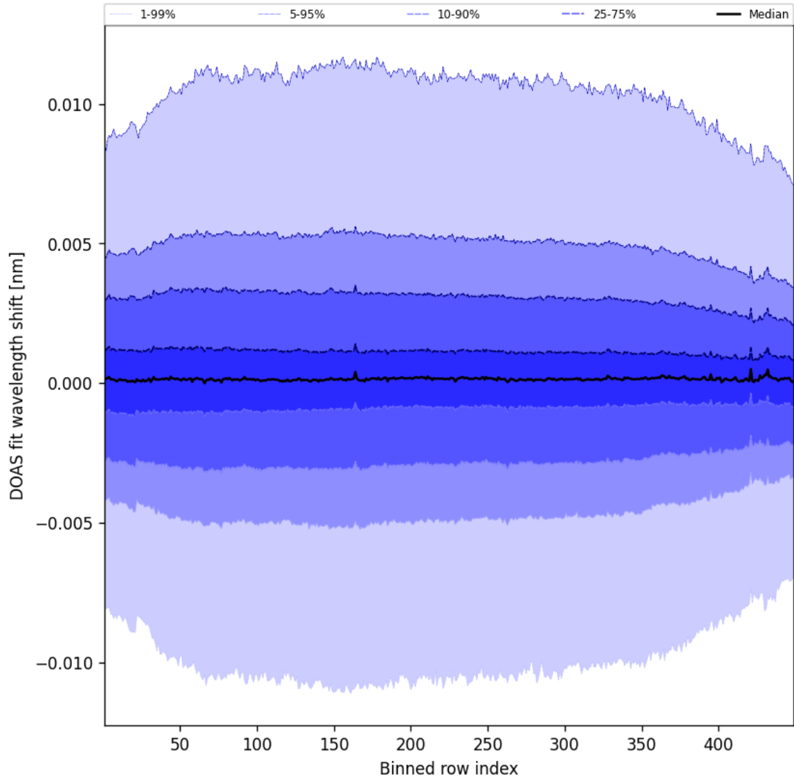
Figure 56: Along track statistics of “DOAS fit wavelength shift” for 2025-06-22 to 2025-06-23
