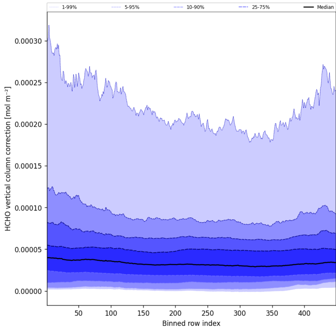
Figure 49: Along track statistics of “HCHO vertical column correction” for 2025-06-22 to 2025-06-23
