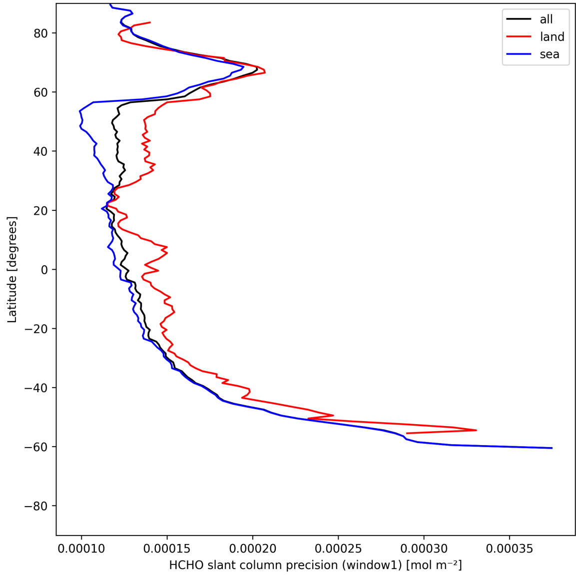
Figure 23: Zonal average of “HCHO slant column precision (window1)” for 2025-06-22 to 2025-06-23.
