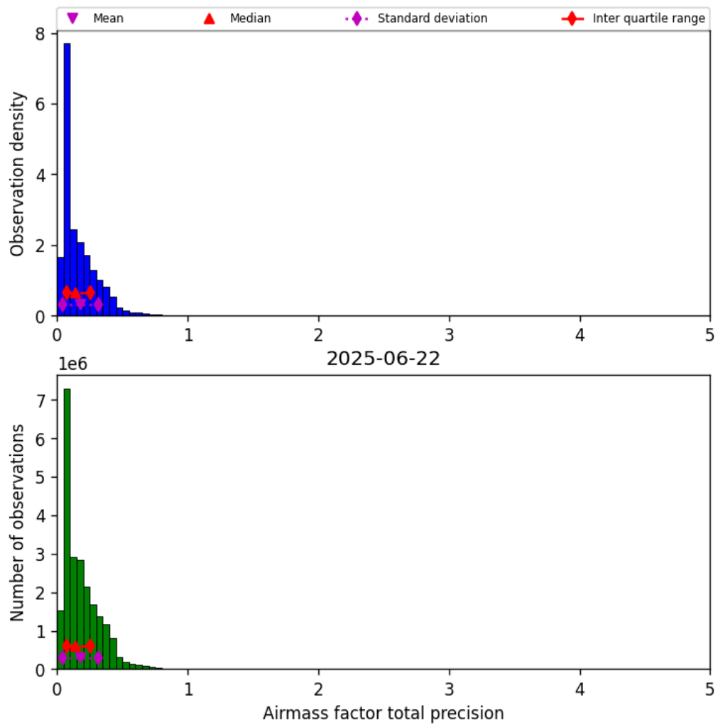
Figure 39: Histogram of “Airmass factor total precision” for 2025-06-22 to 2025-06-23
