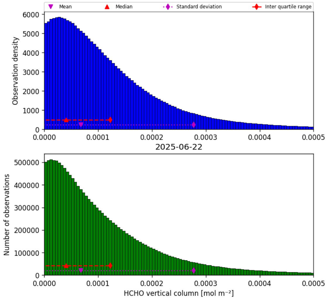
Figure 33: Histogram of “HCHO vertical column” for 2025-06-22 to 2025-06-23
