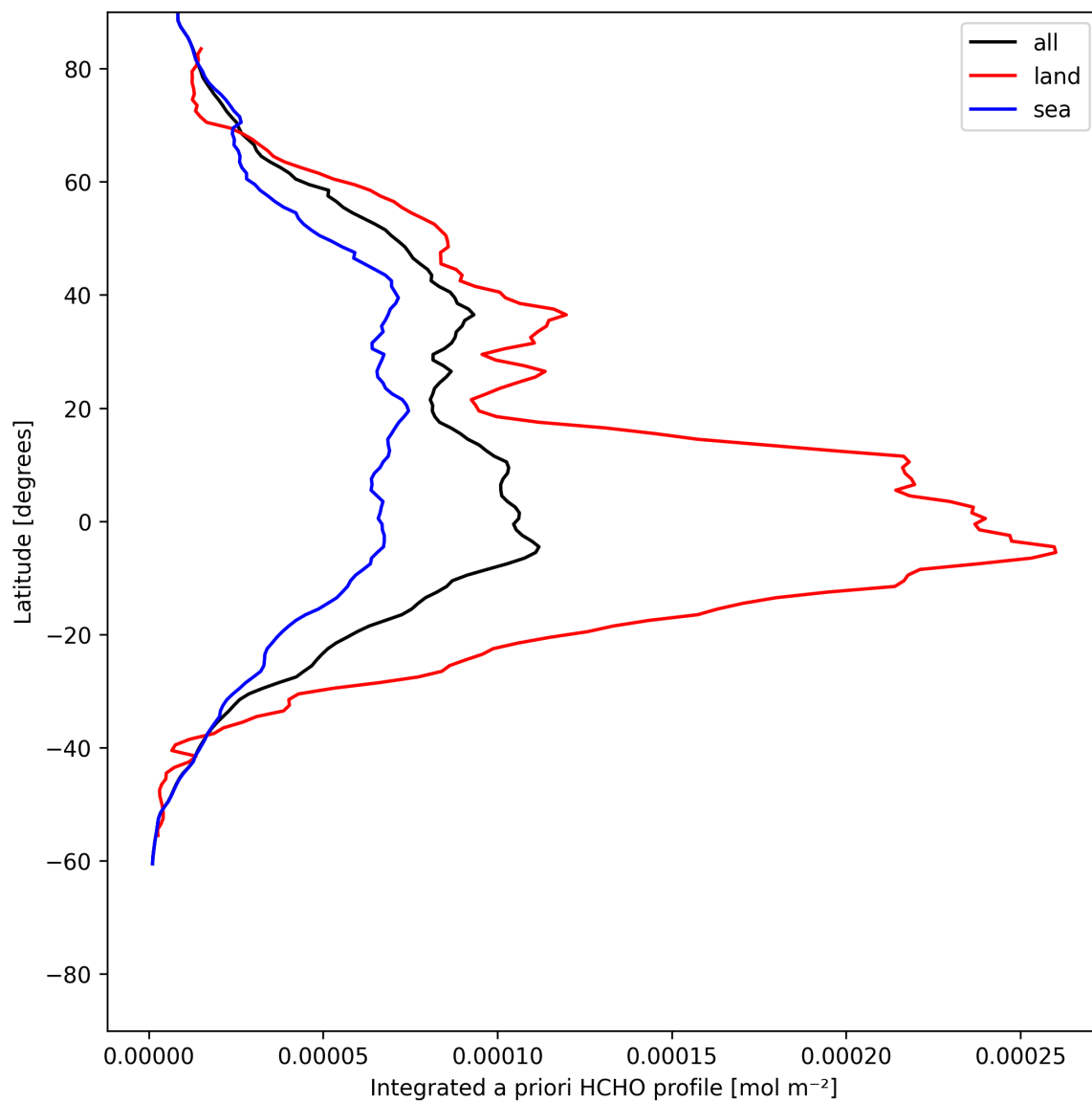
Figure 27: Zonal average of “Integrated a priori HCHO profile” for 2025-06-22 to 2025-06-23.
