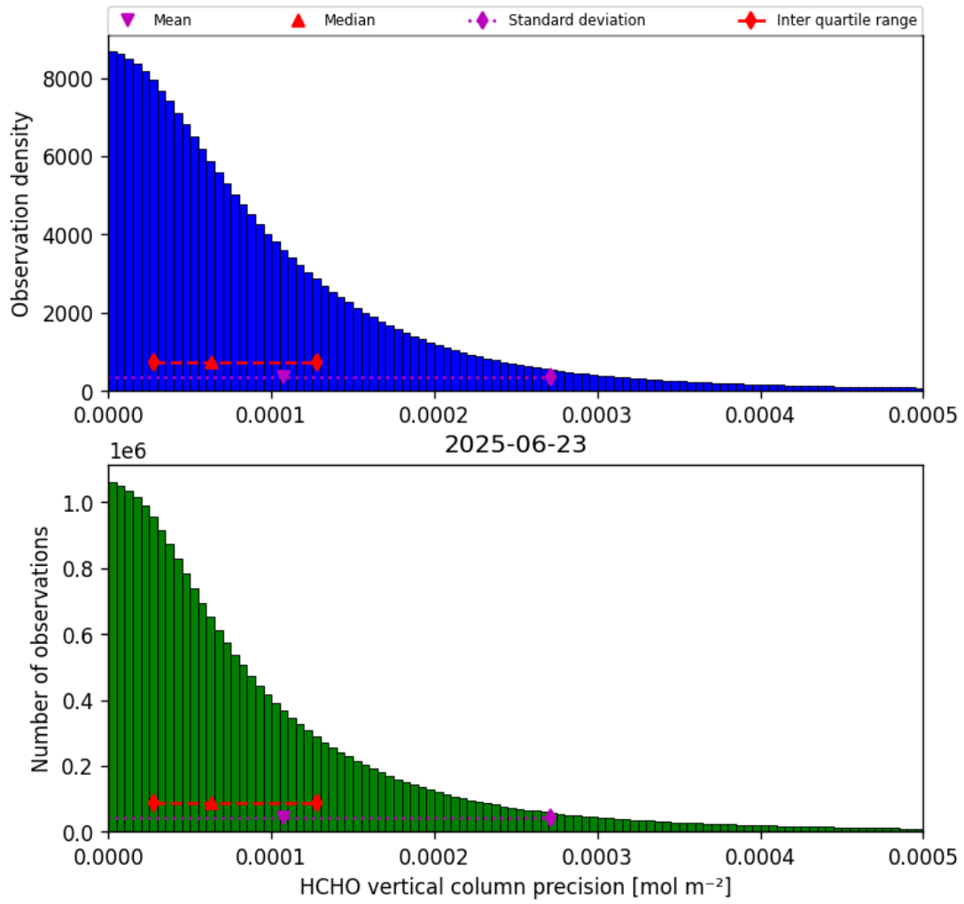
Figure 34: Histogram of “HCHO vertical column precision” for 2025-06-23 to 2025-06-24
