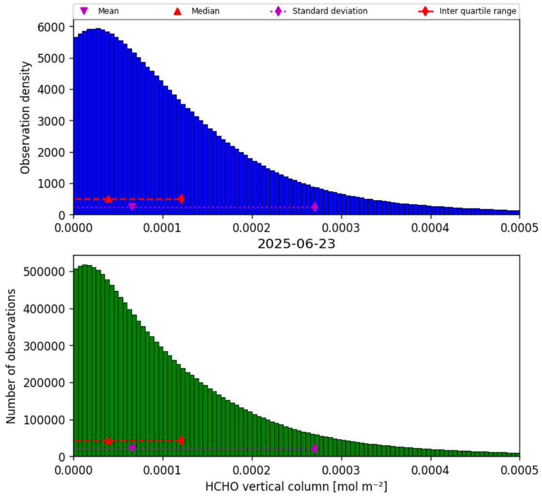
Figure 33: Histogram of “HCHO vertical column” for 2025-06-23 to 2025-06-24
