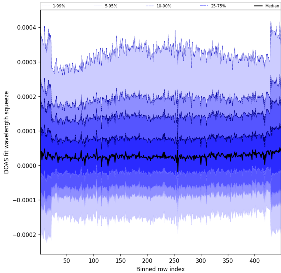
Figure 57: Along track statistics of “DOAS fit wavelength squeeze” for 2025-06-23 to 2025-06-24
