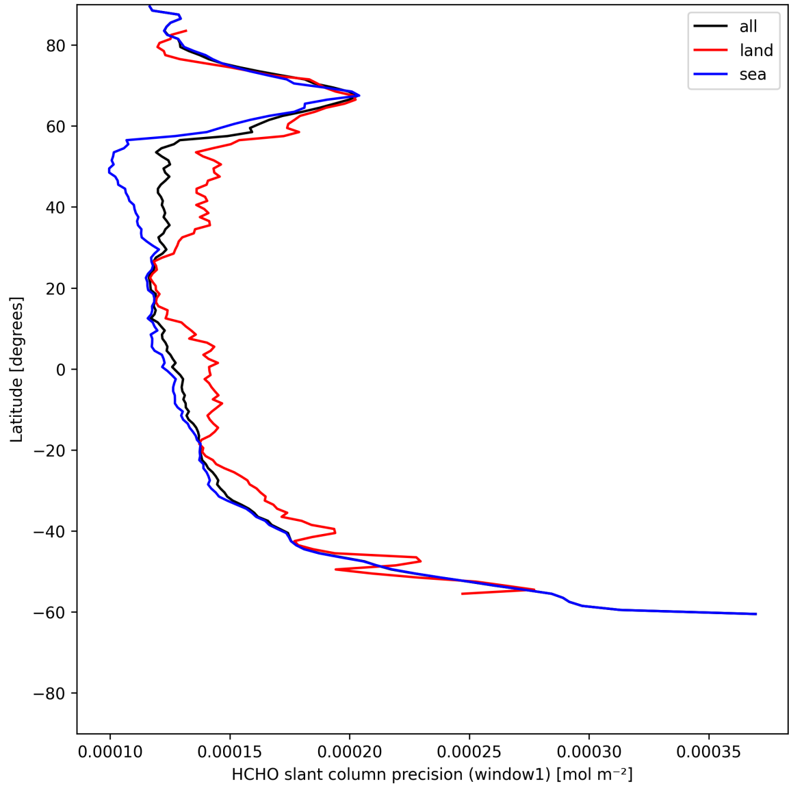
Figure 23: Zonal average of “HCHO slant column precision (window1)” for 2025-06-23 to 2025-06-24.
