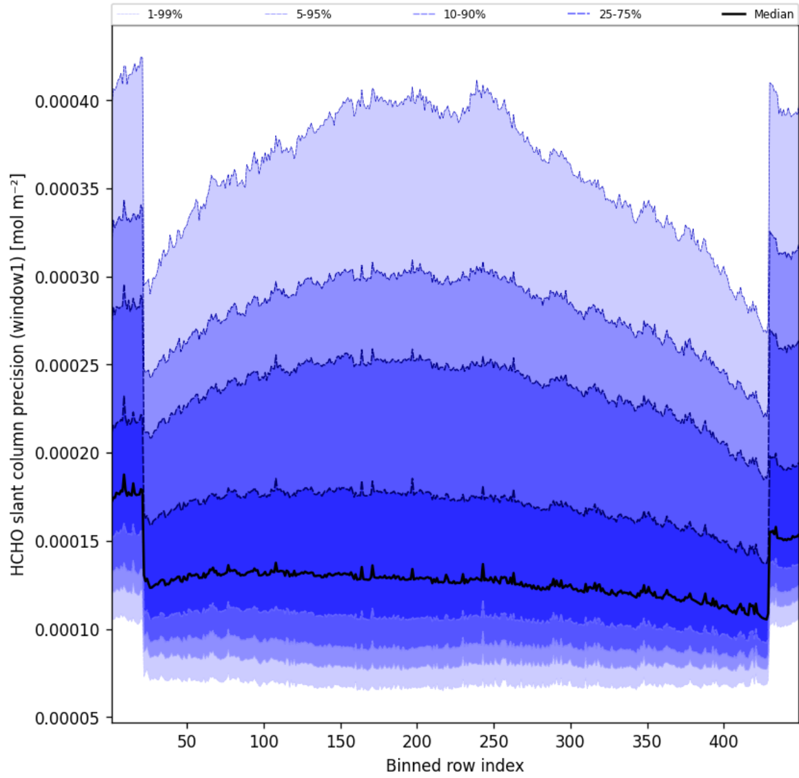
Figure 51: Along track statistics of “HCHO slant column precision (window1)” for 2025-06-23 to 2025-06-24
