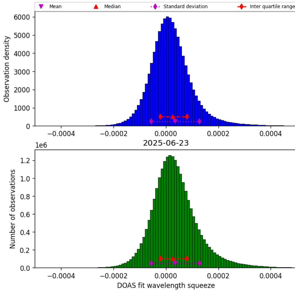
Figure 43: Histogram of “DOAS fit wavelength squeeze” for 2025-06-23 to 2025-06-24
