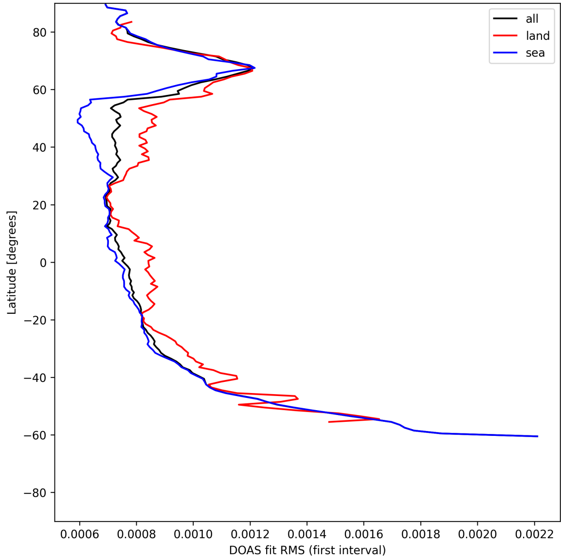
Figure 30: Zonal average of "DOAS fit RMS (first interval)" for 2025-06-23 to 2025-06-24.
