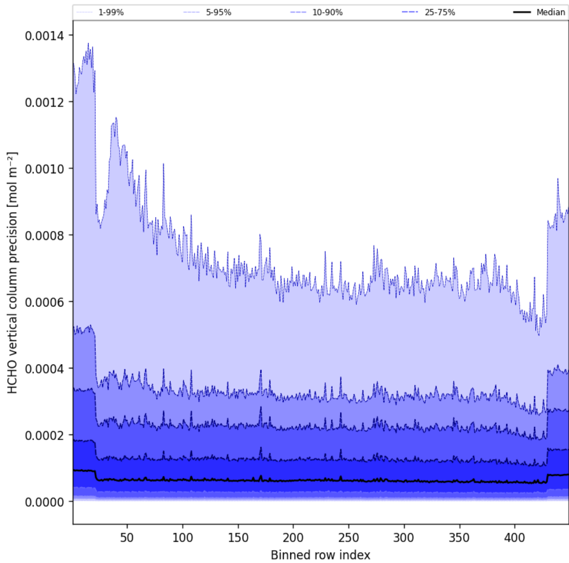
Figure 48: Along track statistics of “HCHO vertical column precision” for 2025-06-23 to 2025-06-24
