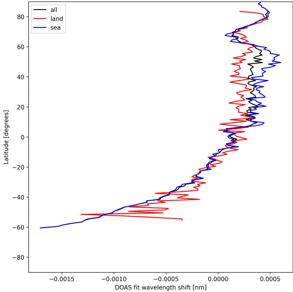
Figure 28: Zonal average of “DOAS fit wavelength shift” for 2025-06-23 to 2025-06-24.
