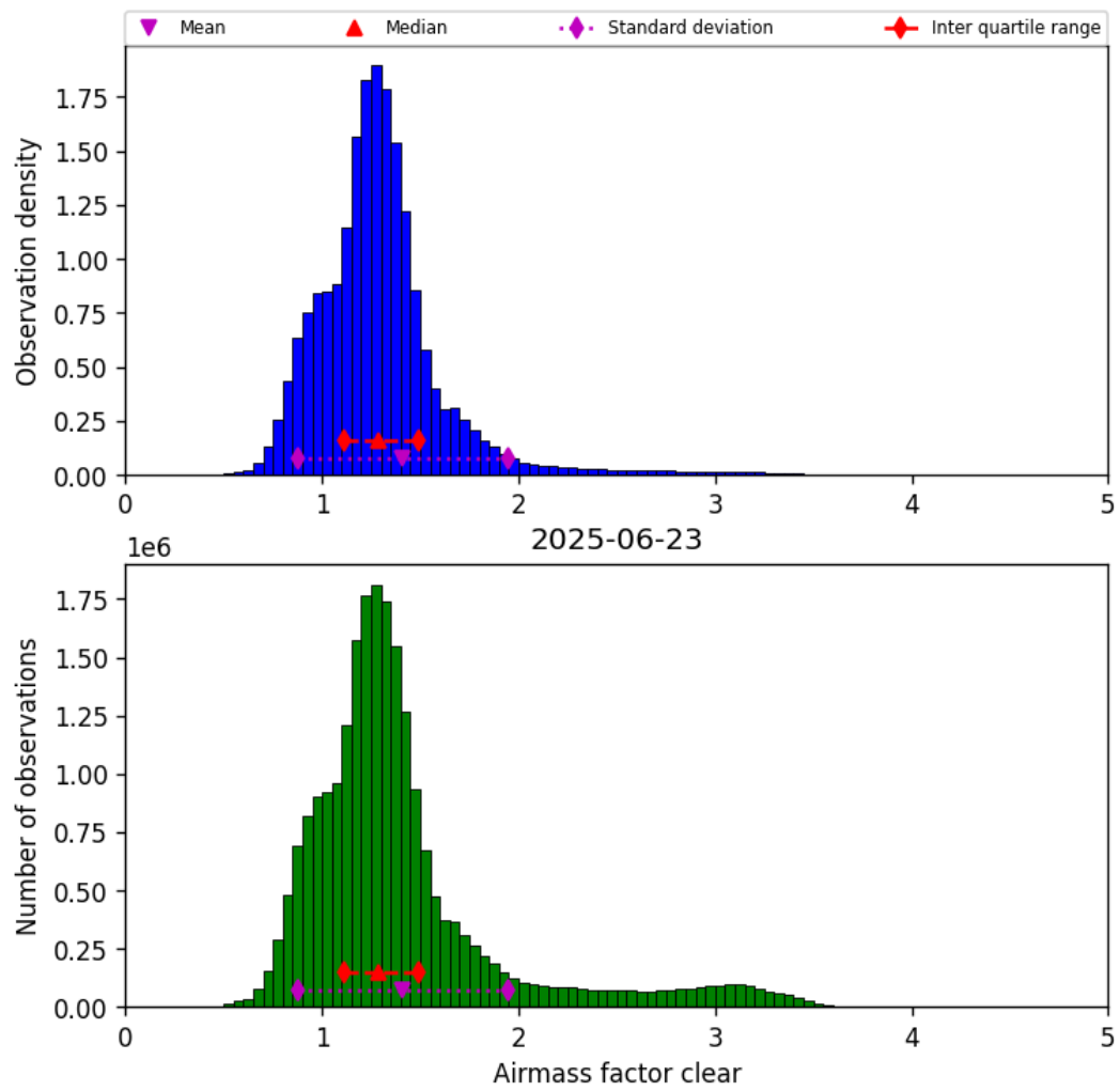
Figure 40: Histogram of “Airmass factor clear” for 2025-06-23 to 2025-06-24
