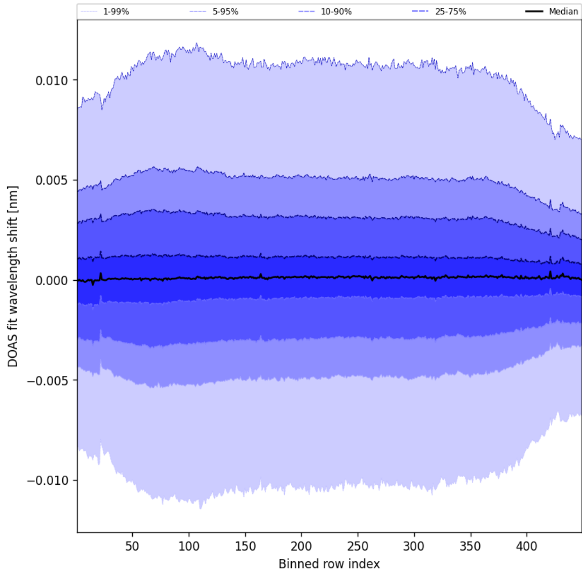
Figure 56: Along track statistics of “DOAS fit wavelength shift” for 2025-06-23 to 2025-06-24
