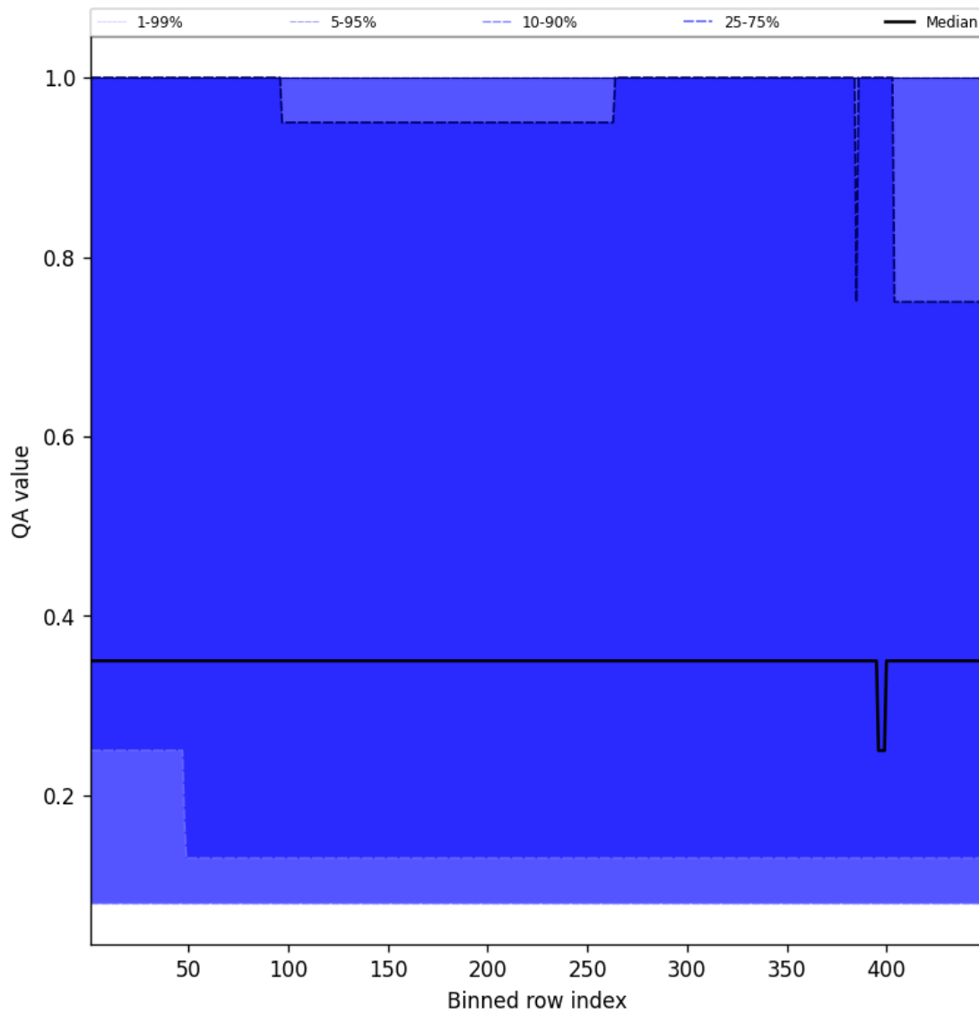
Figure 46: Along track statistics of “QA value” for 2025-06-23 to 2025-06-24
