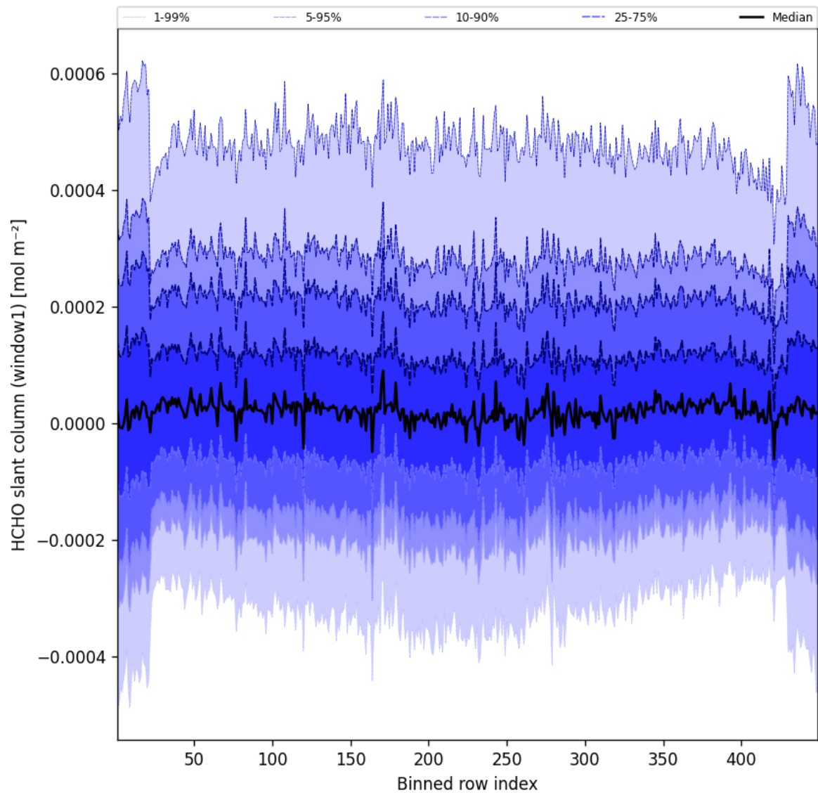
Figure 50: Along track statistics of “HCHO slant column (window1)” for 2025-06-23 to 2025-06-24
