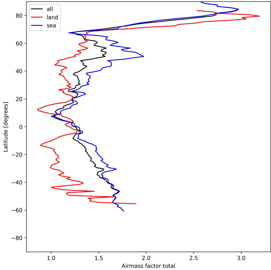
Figure 24: Zonal average of “Airmass factor total” for 2025-06-23 to 2025-06-24.
