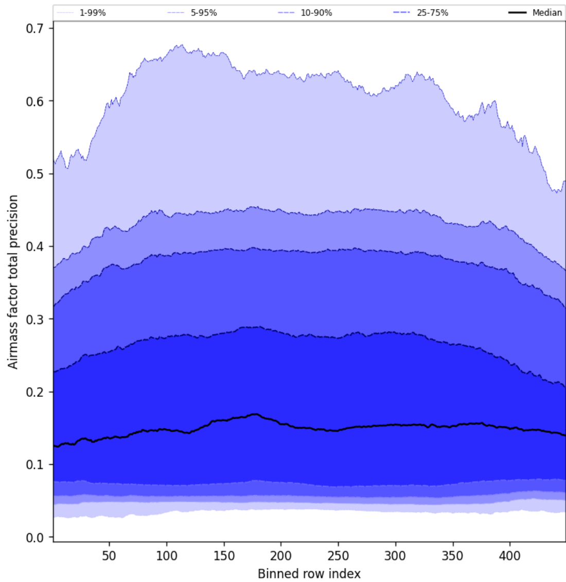
Figure 53: Along track statistics of “Airmass factor total precision” for 2025-06-23 to 2025-06-24
