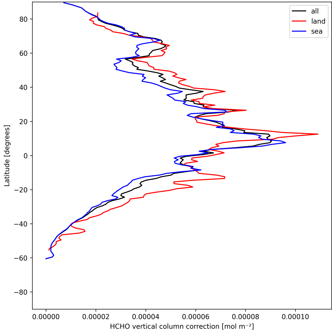
Figure 21: Zonal average of “HCHO vertical column correction” for 2025-06-23 to 2025-06-24.
