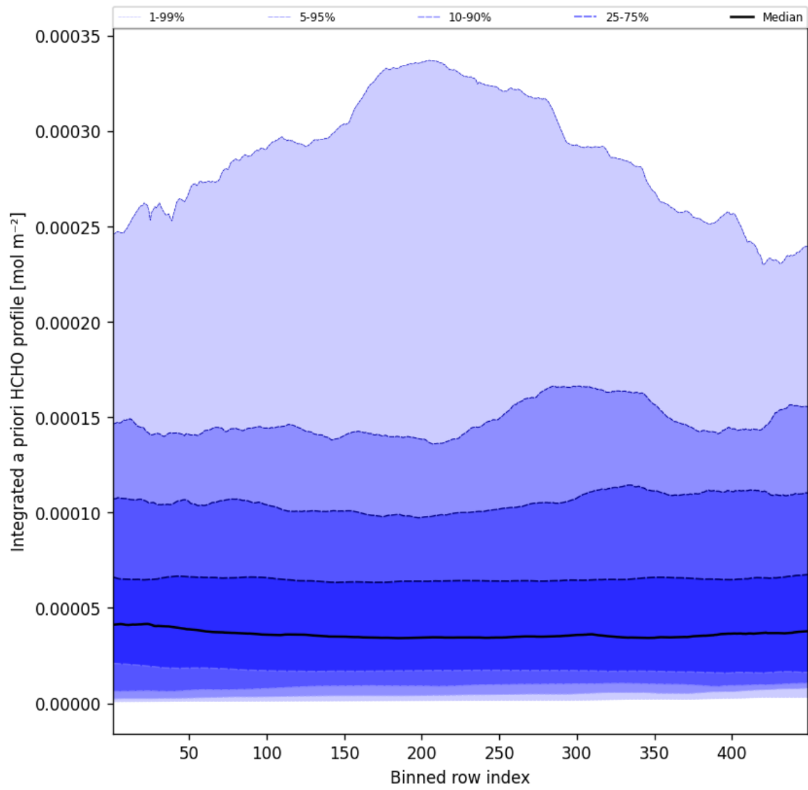
Figure 55: Along track statistics of "Integrated a priori HCHO profile" for 2025-06-23 to 2025-06-24
