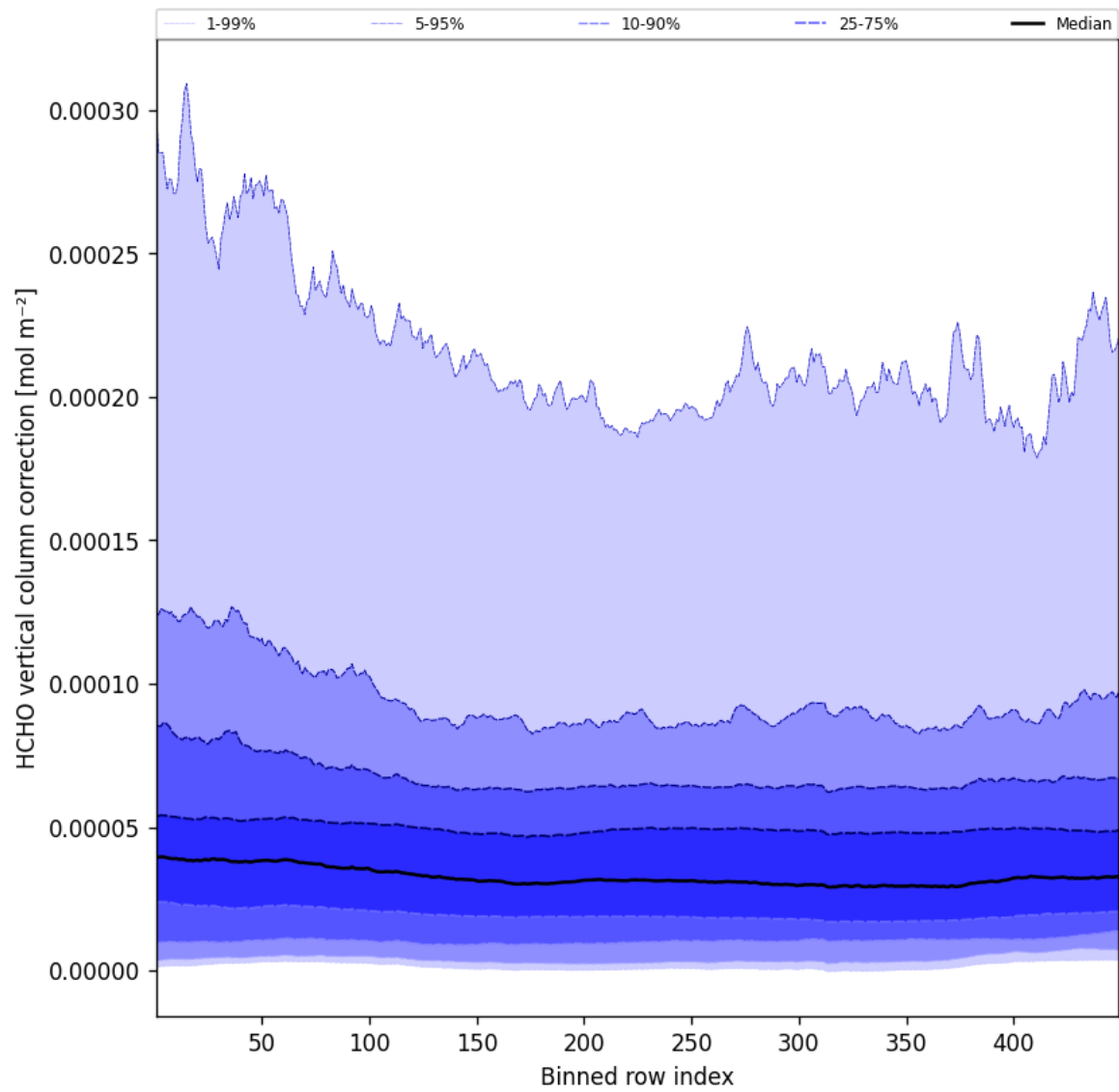
Figure 49: Along track statistics of “HCHO vertical column correction” for 2025-06-23 to 2025-06-24
