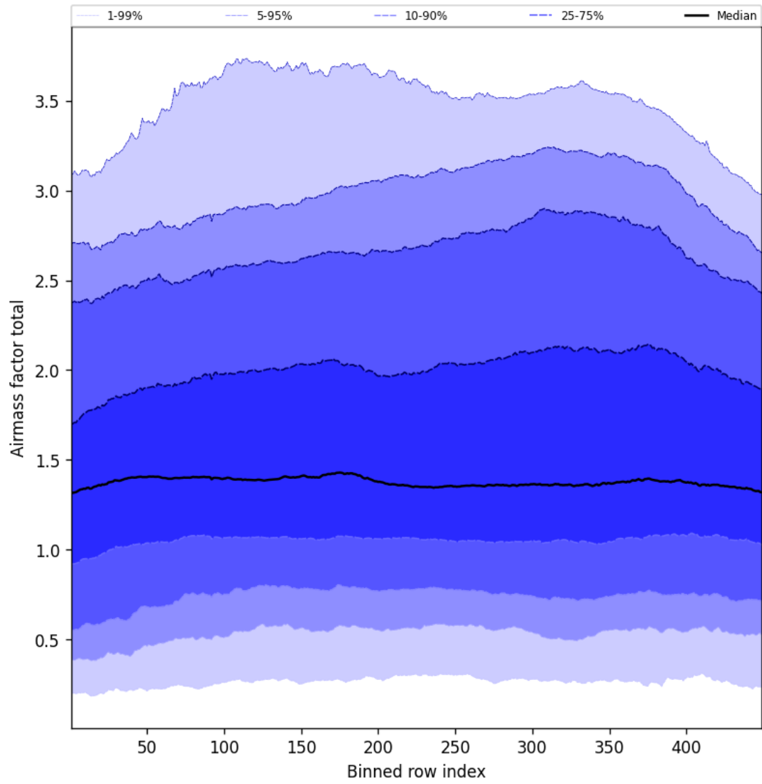
Figure 52: Along track statistics of “Airmass factor total” for 2025-06-23 to 2025-06-24
