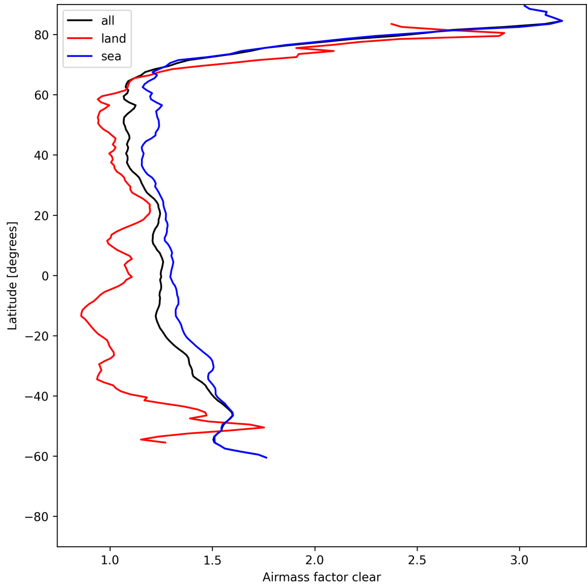
Figure 26: Zonal average of “Airmass factor clear” for 2025-06-23 to 2025-06-24.
