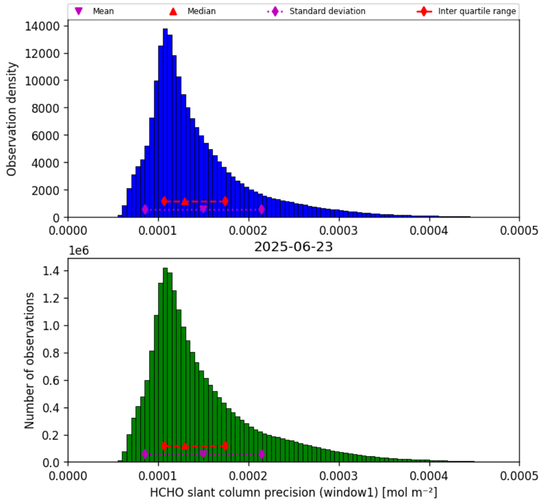
Figure 37: Histogram of “HCHO slant column precision (window1)” for 2025-06-23 to 2025-06-24
