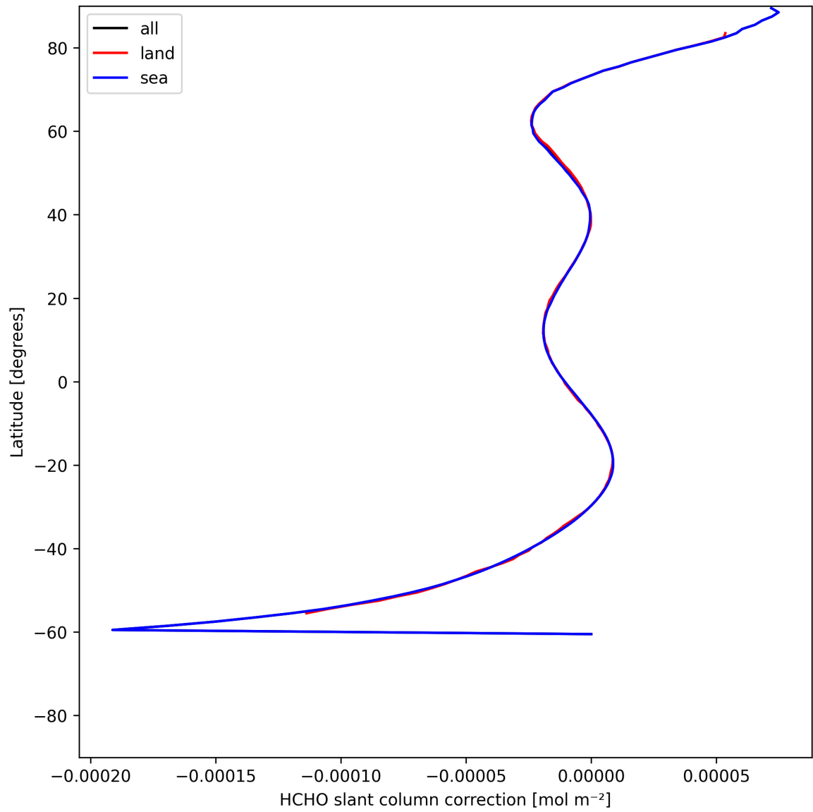
Figure 31: Zonal average of “HCHO slant column correction” for 2025-06-23 to 2025-06-24.
