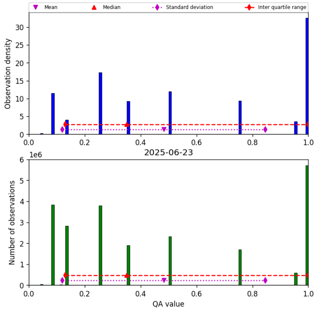
Figure 32: Histogram of “QA value” for 2025-06-23 to 2025-06-24
