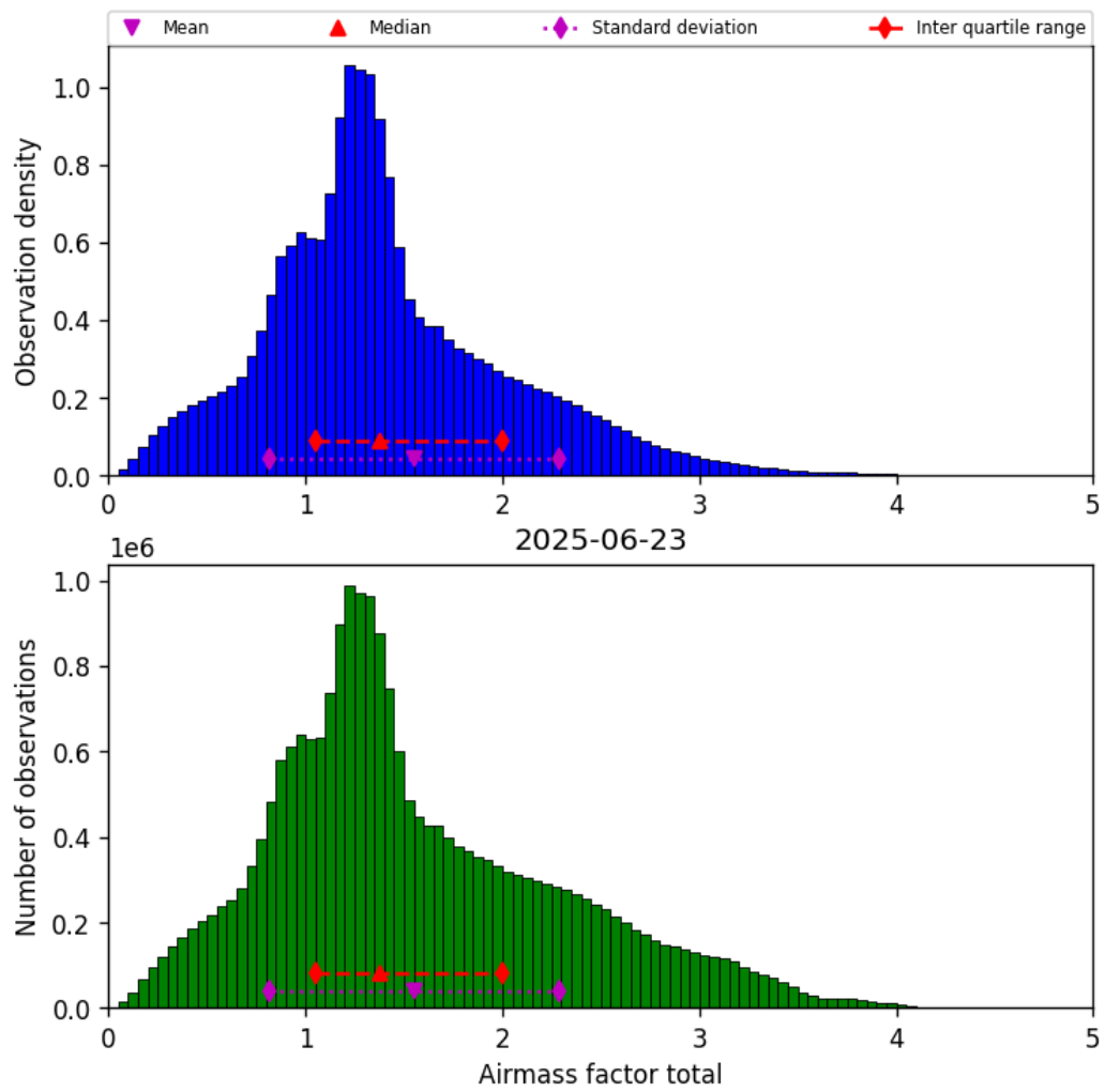
Figure 38: Histogram of “Airmass factor total” for 2025-06-23 to 2025-06-24
