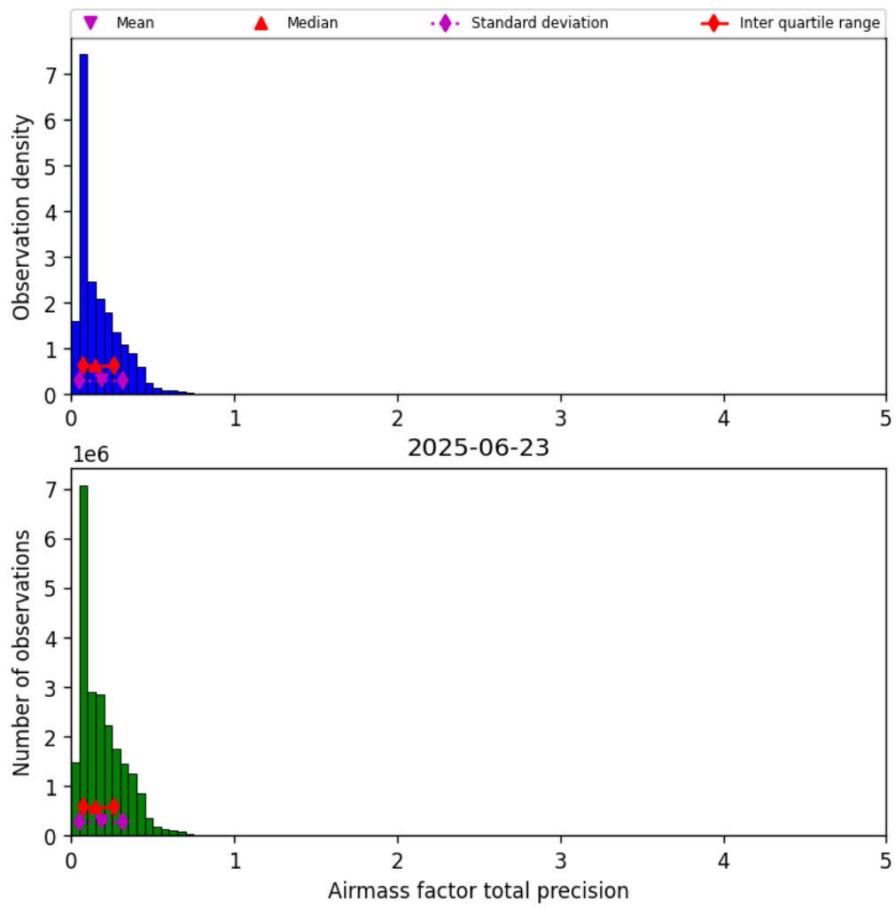
Figure 39: Histogram of “Airmass factor total precision” for 2025-06-23 to 2025-06-24
