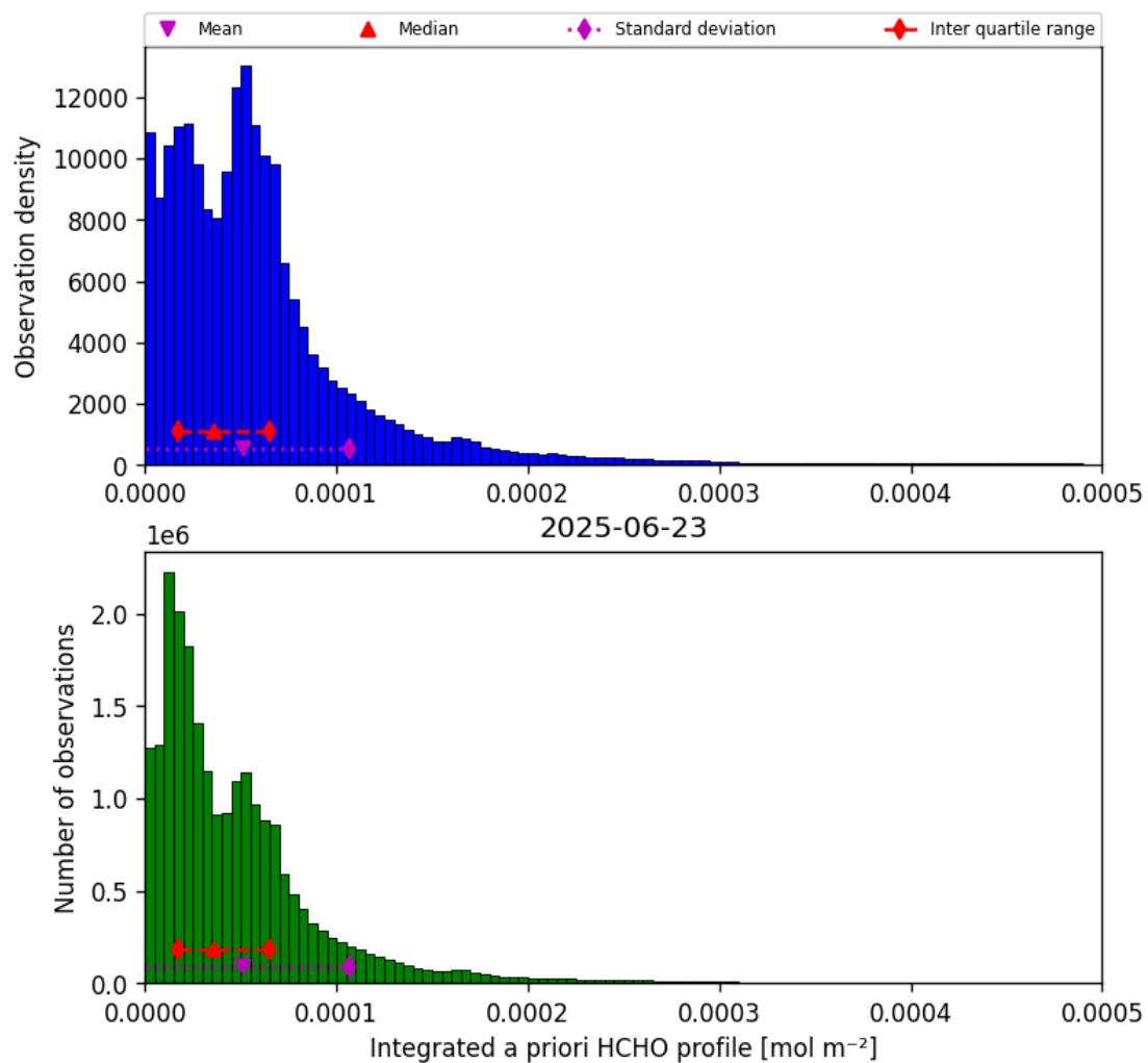
Figure 41: Histogram of “Integrated a priori HCHO profile” for 2025-06-23 to 2025-06-24
