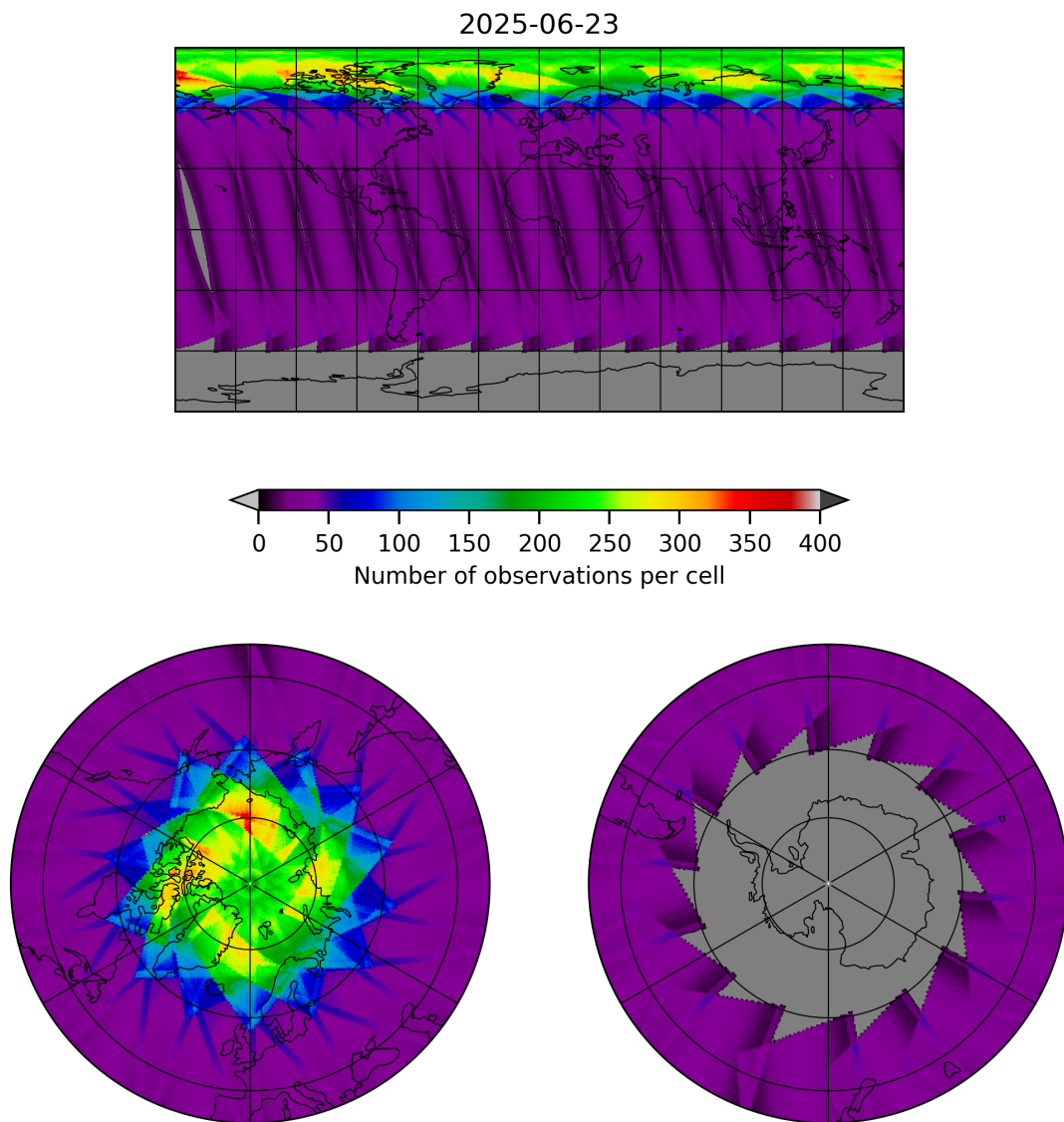
Figure 17: Map of the number of observations for 2025-06-23 to 2025-06-24
