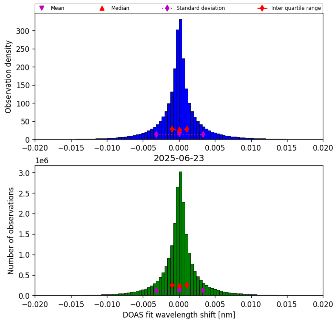
Figure 42: Histogram of “DOAS fit wavelength shift” for 2025-06-23 to 2025-06-24
