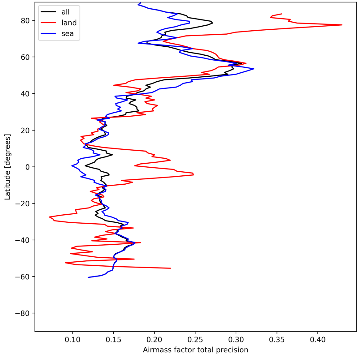
Figure 25: Zonal average of “Airmass factor total precision” for 2025-06-23 to 2025-06-24.
