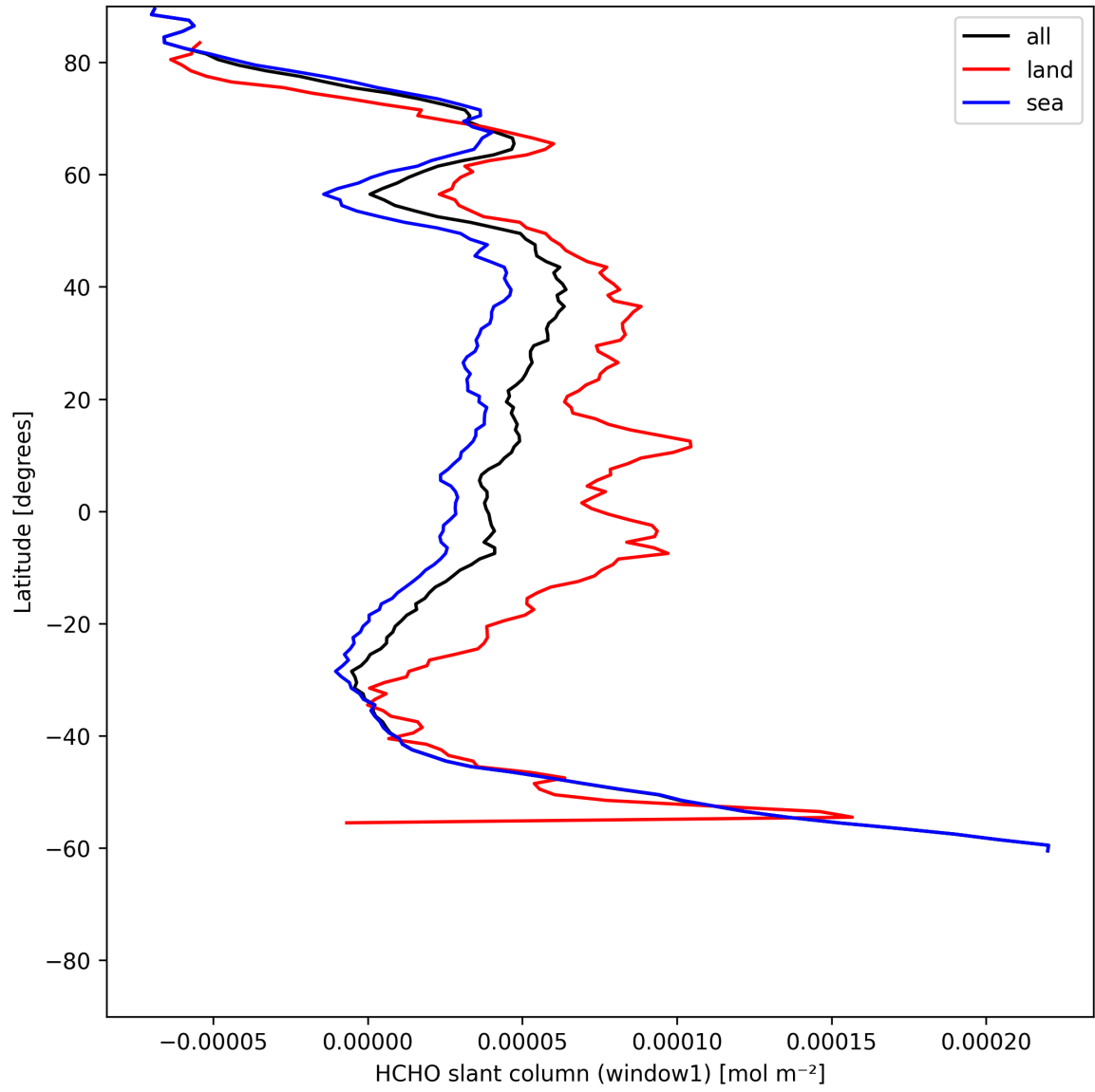
Figure 22: Zonal average of “HCHO slant column (window1)” for 2025-06-23 to 2025-06-24.
