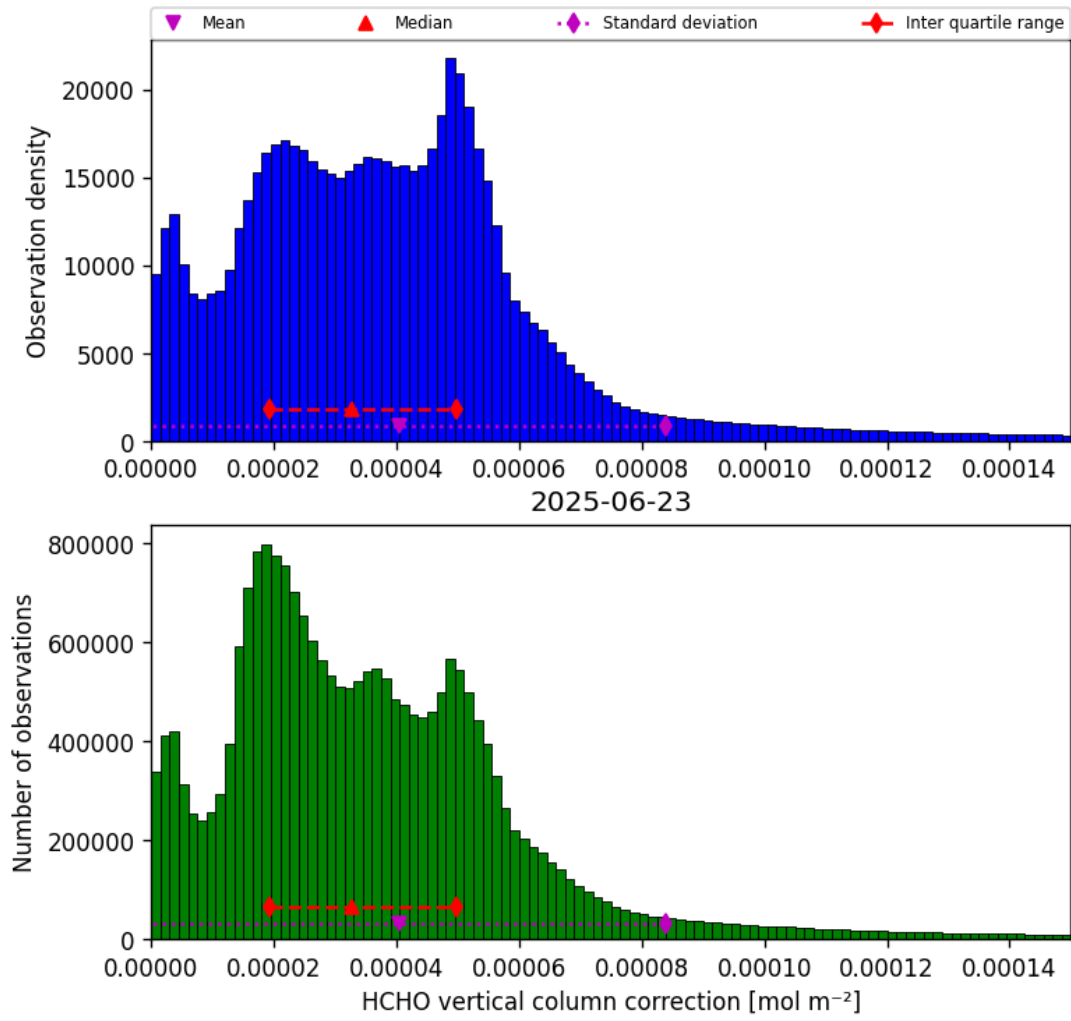
Figure 35: Histogram of “HCHO vertical column correction” for 2025-06-23 to 2025-06-24
