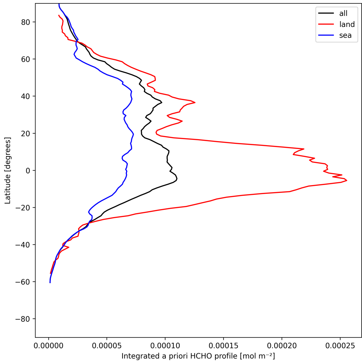
Figure 27: Zonal average of “Integrated a priori HCHO profile” for 2025-06-23 to 2025-06-24.
