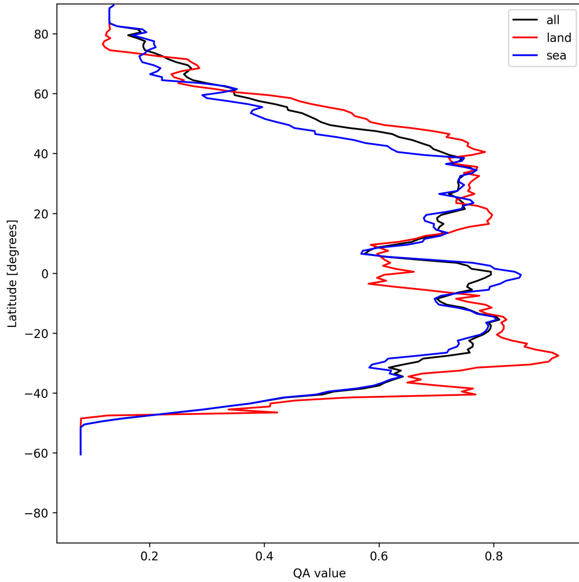
Figure 18: Zonal average of “QA value” for 2025-06-23 to 2025-06-24.
