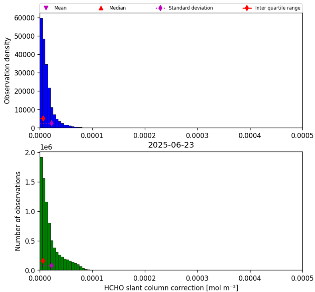
Figure 45: Histogram of “HCHO slant column correction” for 2025-06-23 to 2025-06-24
