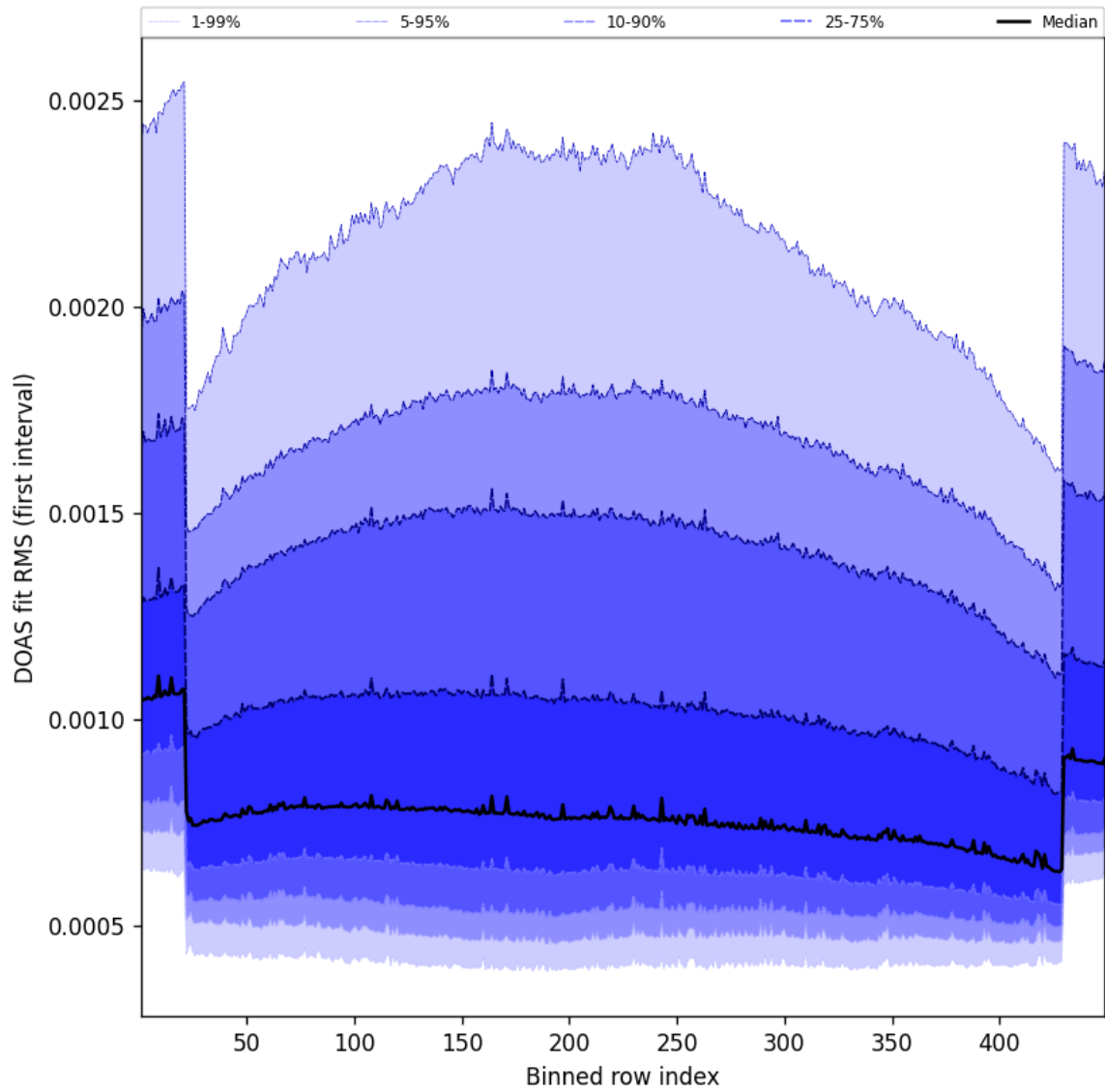
Figure 58: Along track statistics of “DOAS fit RMS (first interval)” for 2025-06-23 to 2025-06-24
