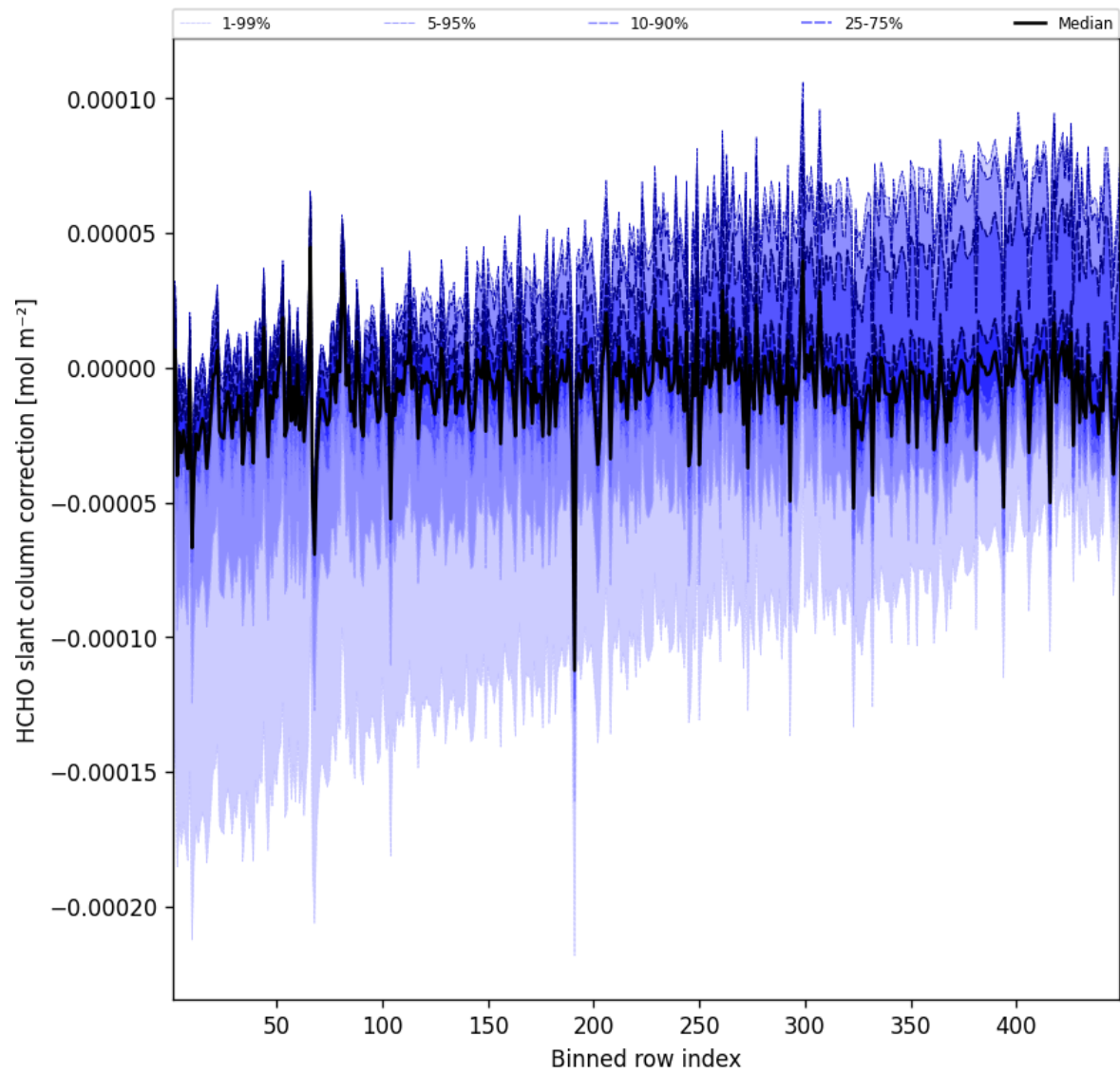
Figure 59: Along track statistics of “HCHO slant column correction” for 2025-06-23 to 2025-06-24
