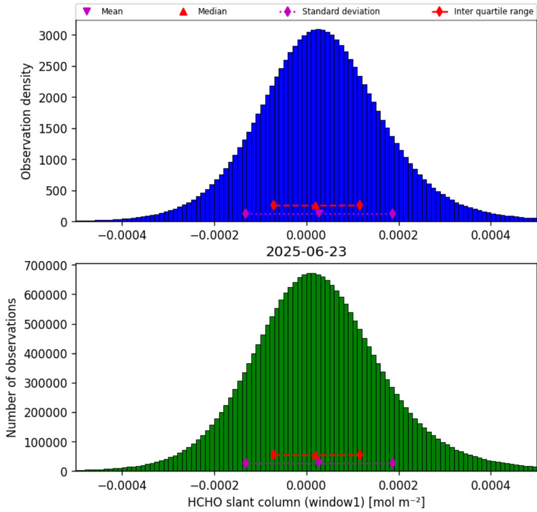
Figure 36: Histogram of “HCHO slant column (window1)” for 2025-06-23 to 2025-06-24
