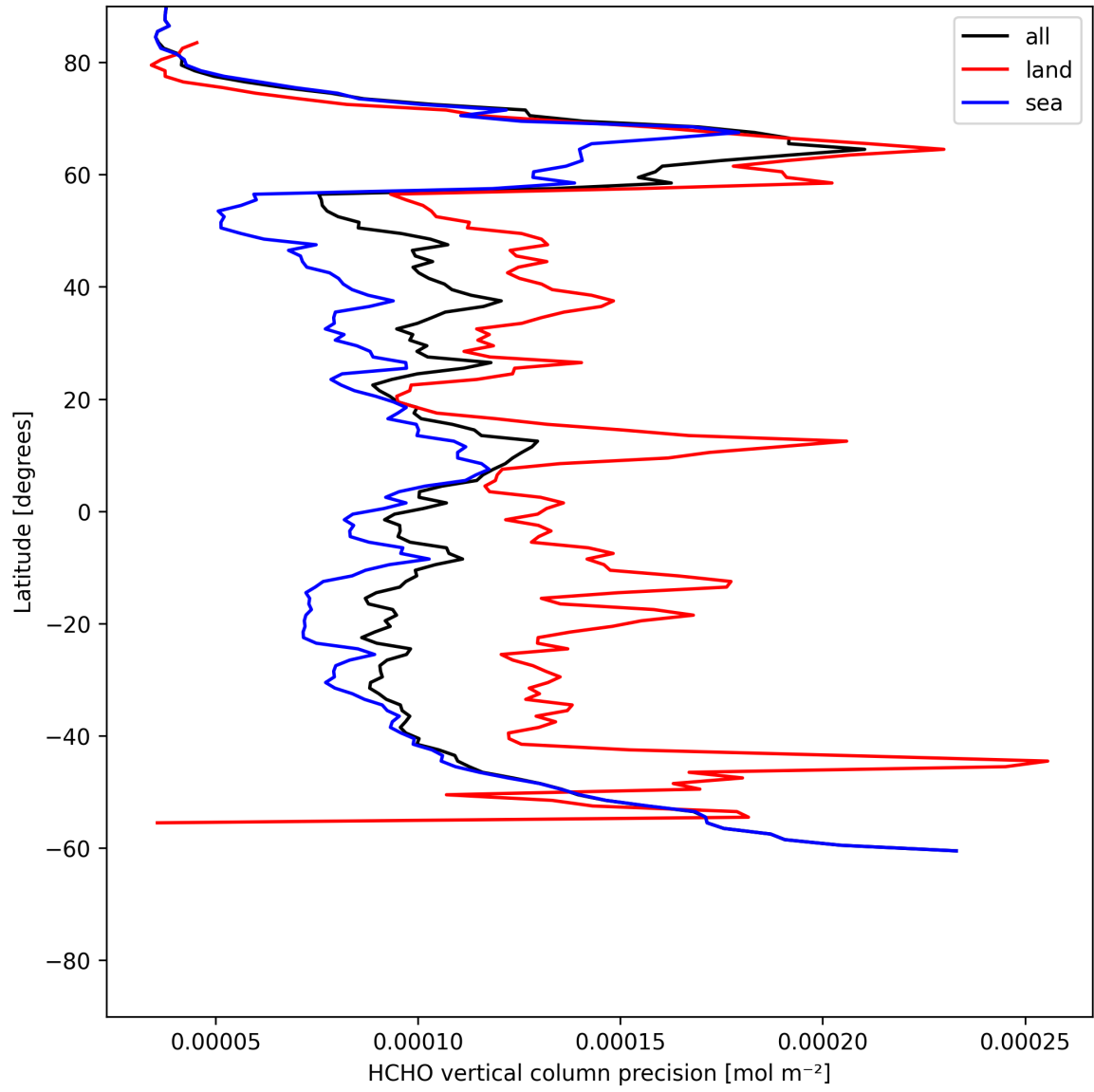
Figure 20: Zonal average of “HCHO vertical column precision” for 2025-06-23 to 2025-06-24.
