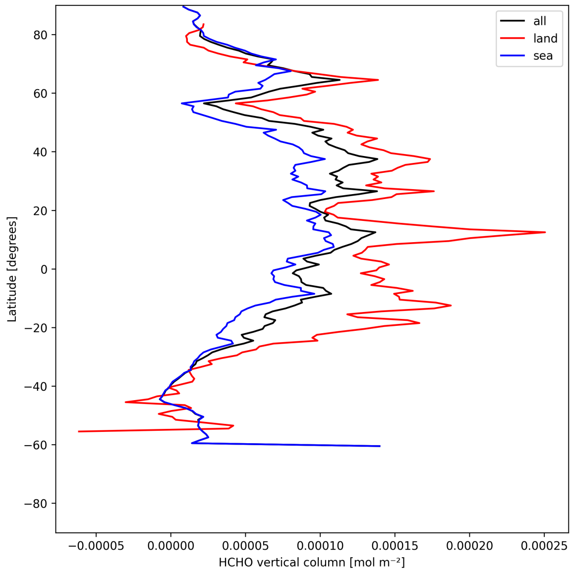
Figure 19: Zonal average of “HCHO vertical column” for 2025-06-23 to 2025-06-24.
