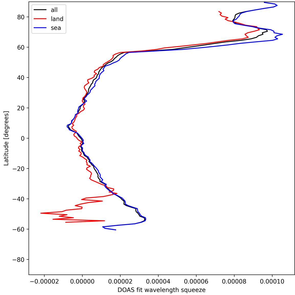
Figure 29: Zonal average of “DOAS fit wavelength squeeze” for 2025-06-23 to 2025-06-24.
