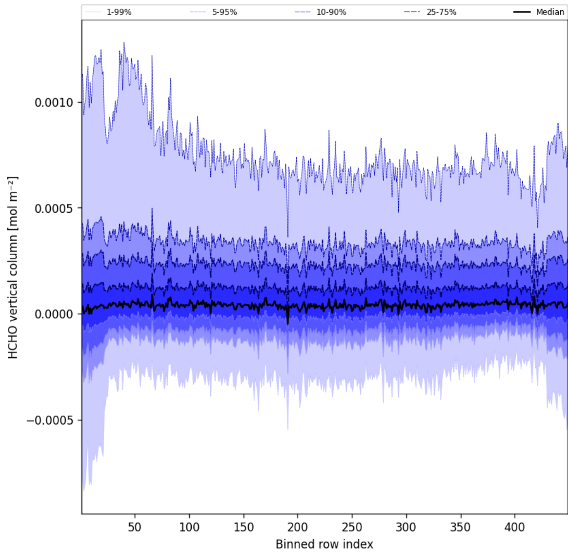
Figure 47: Along track statistics of “HCHO vertical column” for 2025-06-23 to 2025-06-24
