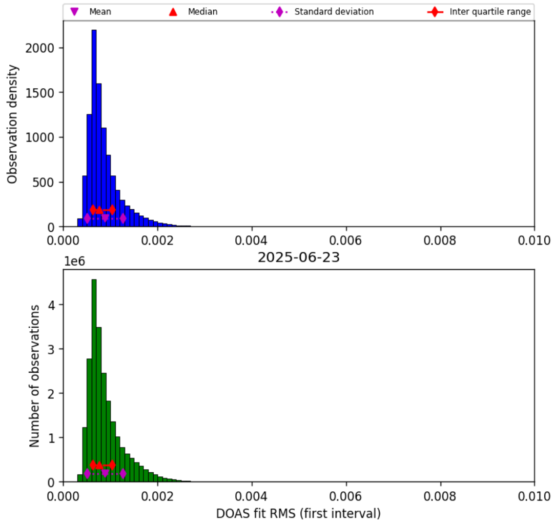
Figure 44: Histogram of “DOAS fit RMS (first interval)” for 2025-06-23 to 2025-06-24
