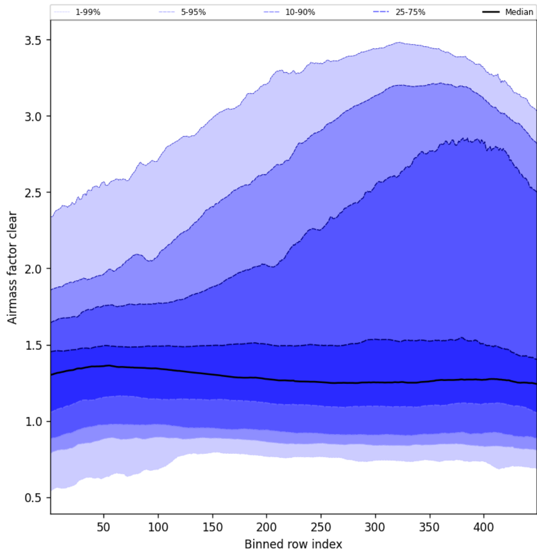
Figure 54: Along track statistics of “Airmass factor clear” for 2025-06-23 to 2025-06-24
