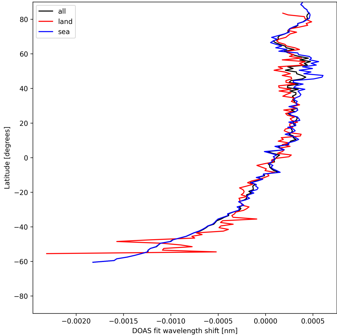
Figure 28: Zonal average of “DOAS fit wavelength shift” for 2025-06-24 to 2025-06-25.
