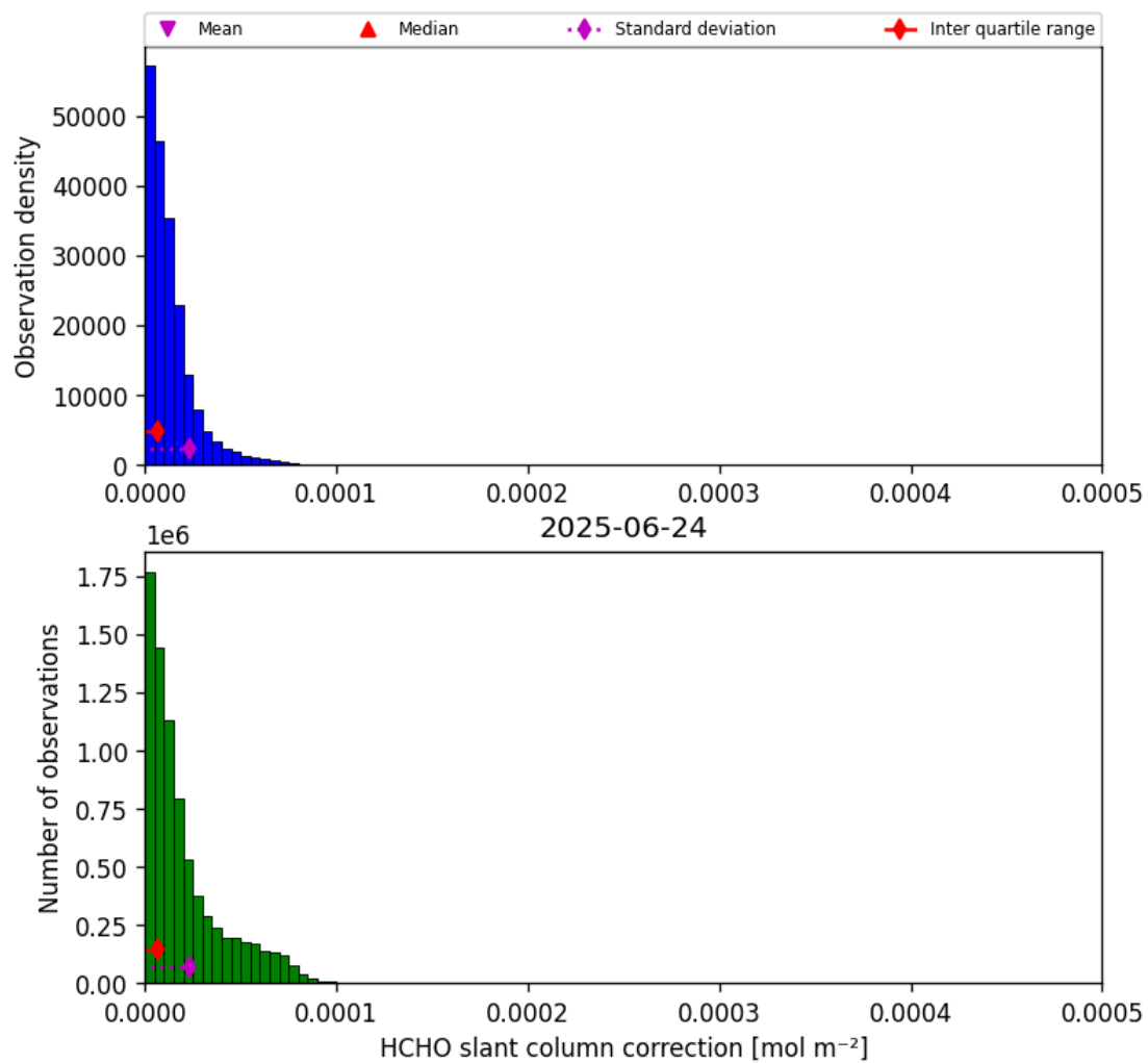
Figure 45: Histogram of “HCHO slant column correction” for 2025-06-24 to 2025-06-25
