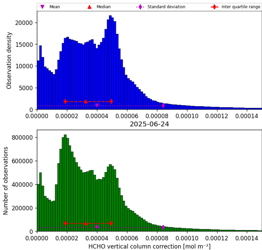
Figure 35: Histogram of “HCHO vertical column correction” for 2025-06-24 to 2025-06-25
