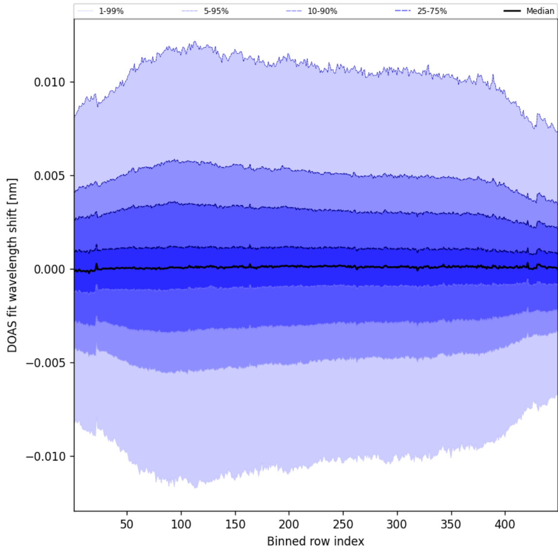
Figure 56: Along track statistics of “DOAS fit wavelength shift” for 2025-06-24 to 2025-06-25
