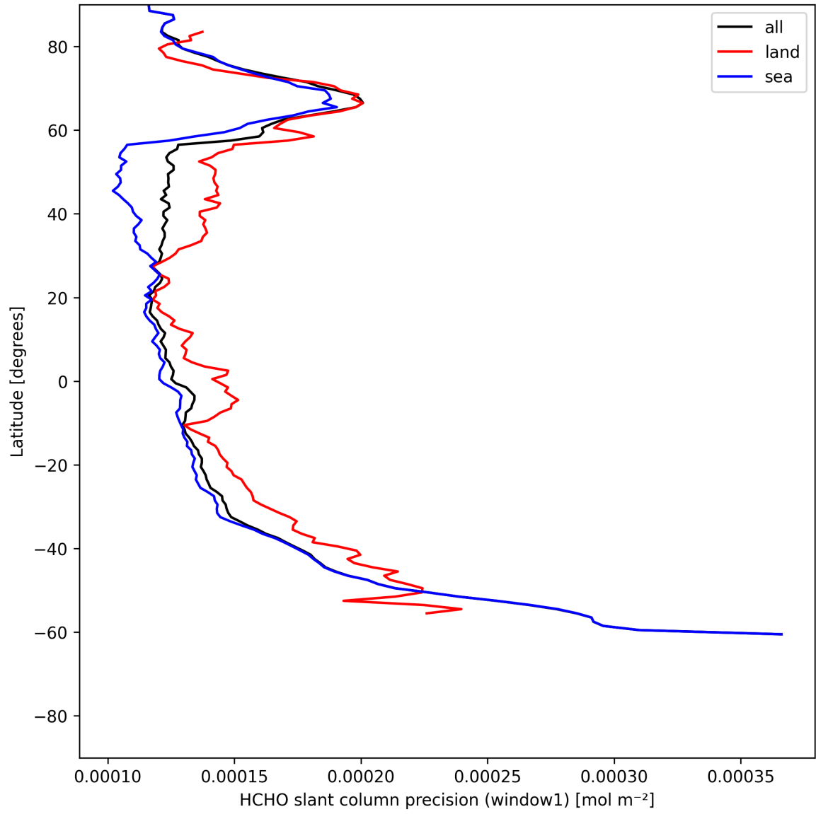
Figure 23: Zonal average of “HCHO slant column precision (window1)” for 2025-06-24 to 2025-06-25.
