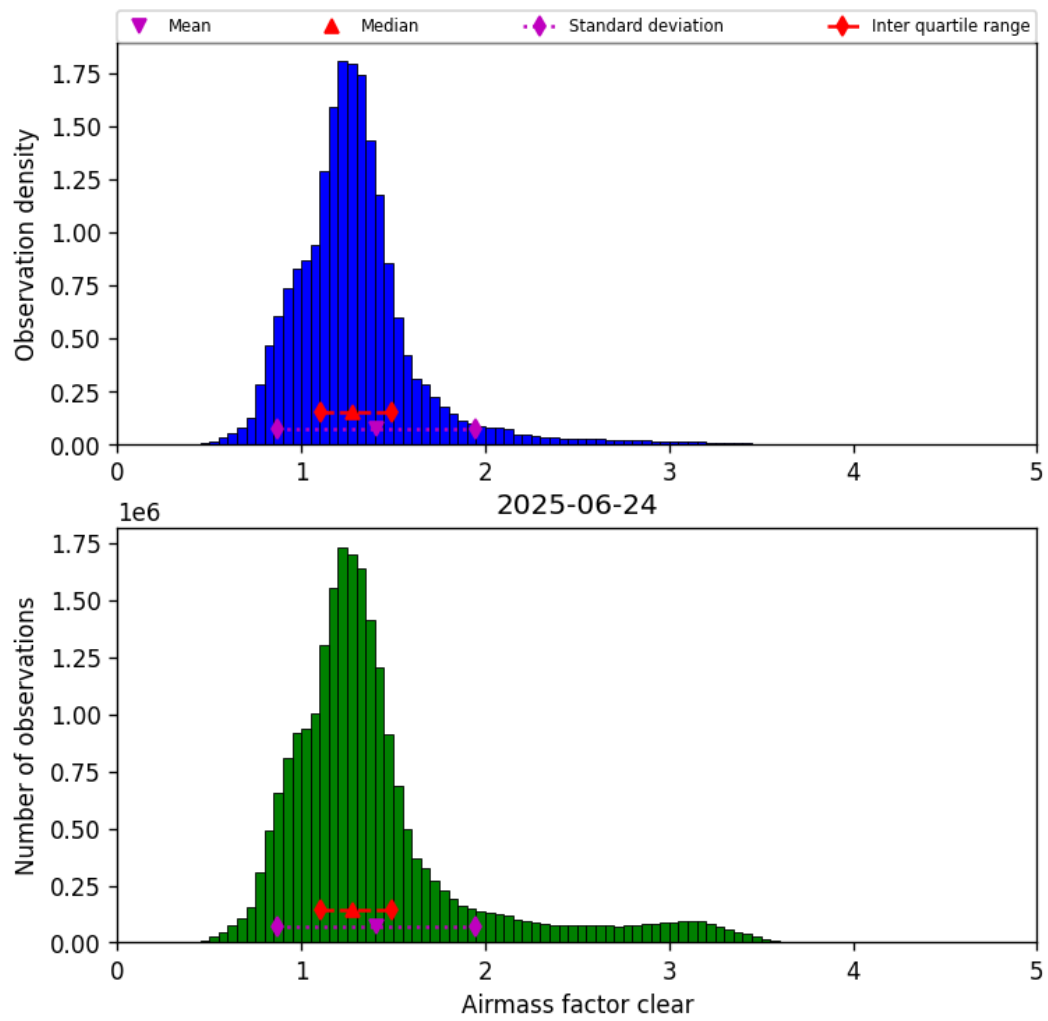
Figure 40: Histogram of “Airmass factor clear” for 2025-06-24 to 2025-06-25
