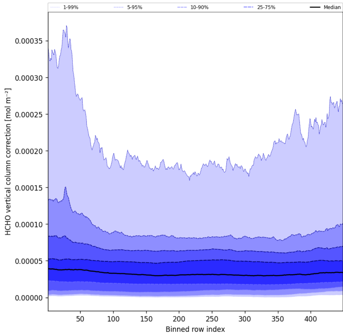
Figure 49: Along track statistics of “HCHO vertical column correction” for 2025-06-24 to 2025-06-25
