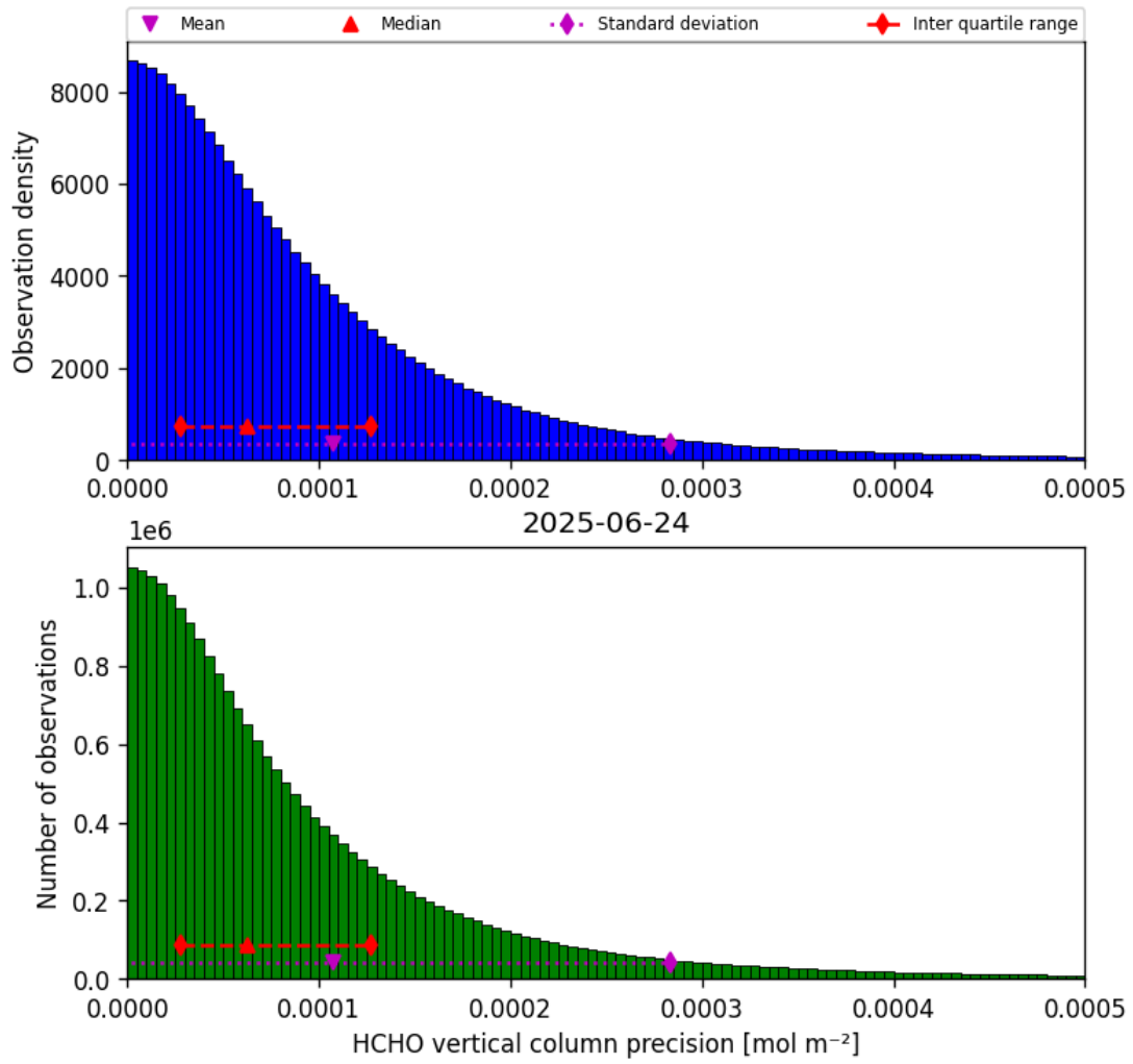
Figure 34: Histogram of “HCHO vertical column precision” for 2025-06-24 to 2025-06-25
