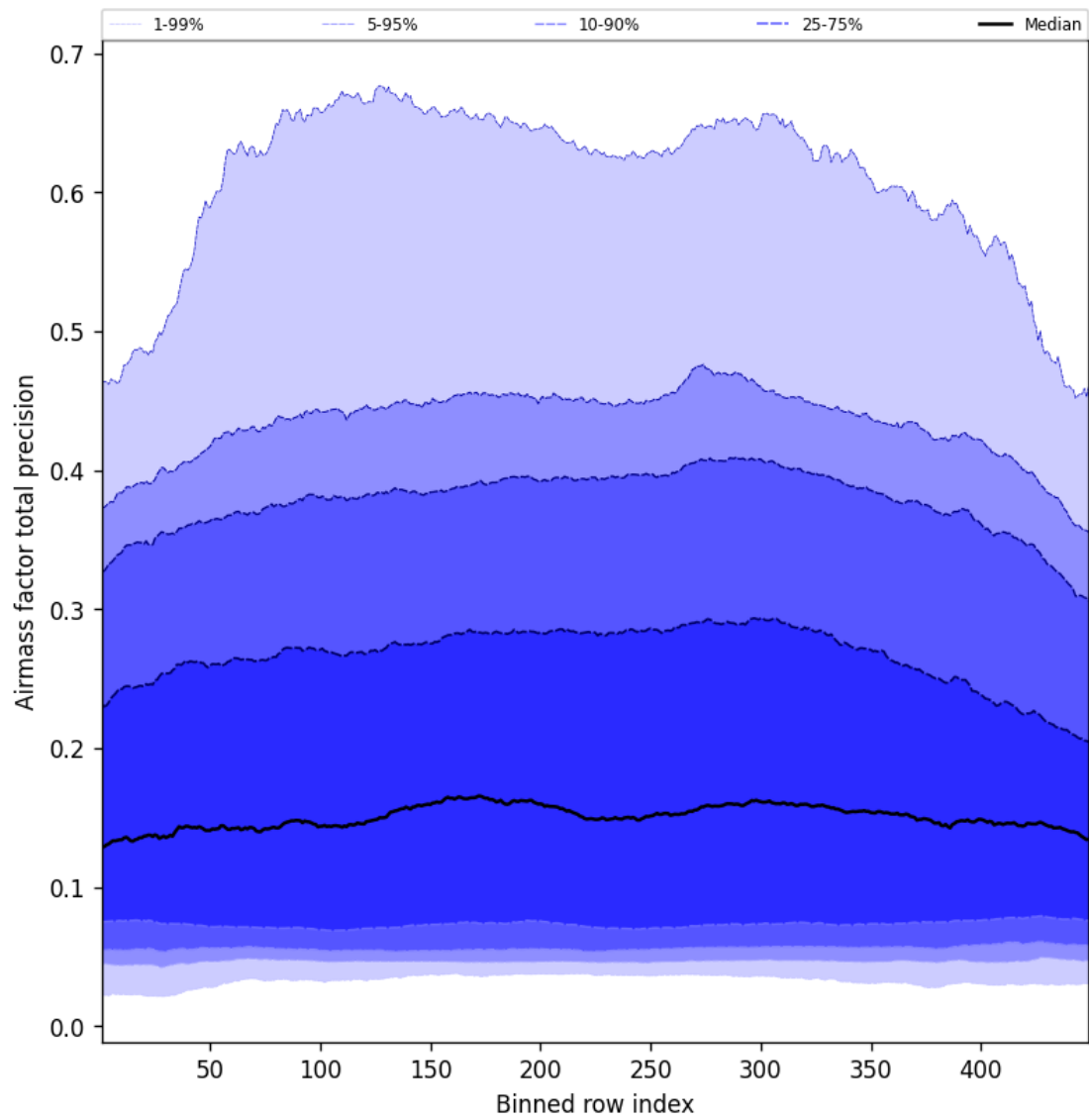
Figure 53: Along track statistics of “Airmass factor total precision” for 2025-06-24 to 2025-06-25
