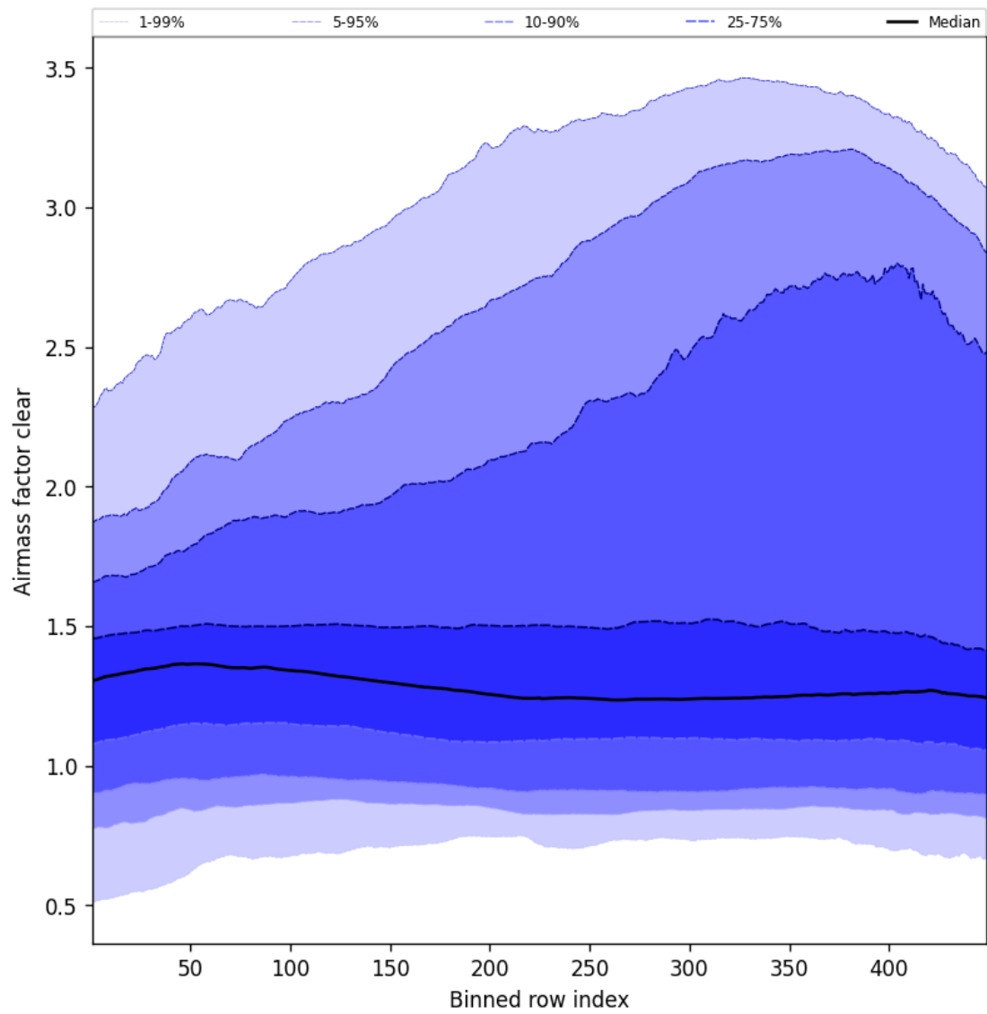
Figure 54: Along track statistics of “Airmass factor clear” for 2025-06-24 to 2025-06-25
