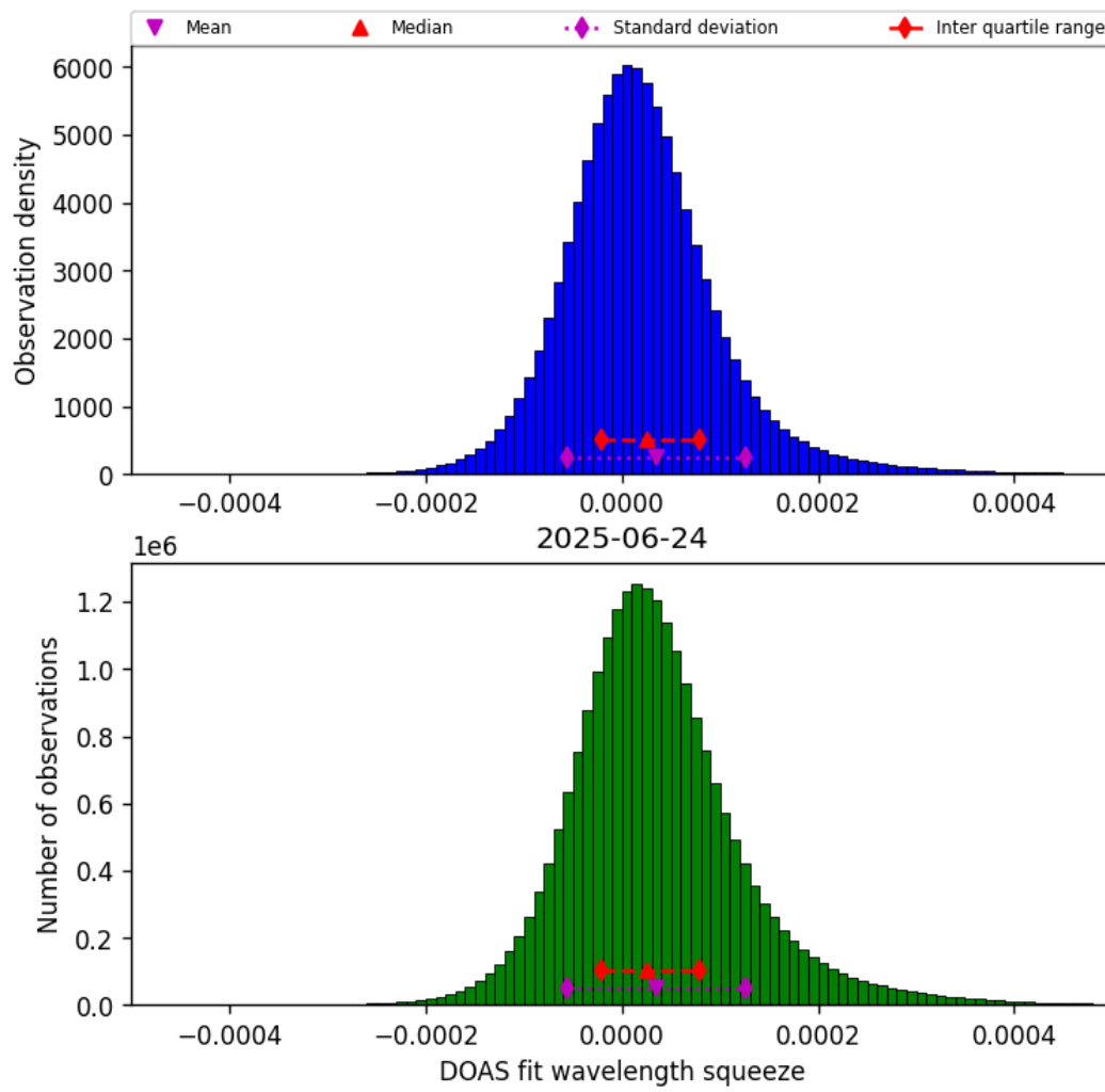
Figure 43: Histogram of “DOAS fit wavelength squeeze” for 2025-06-24 to 2025-06-25
