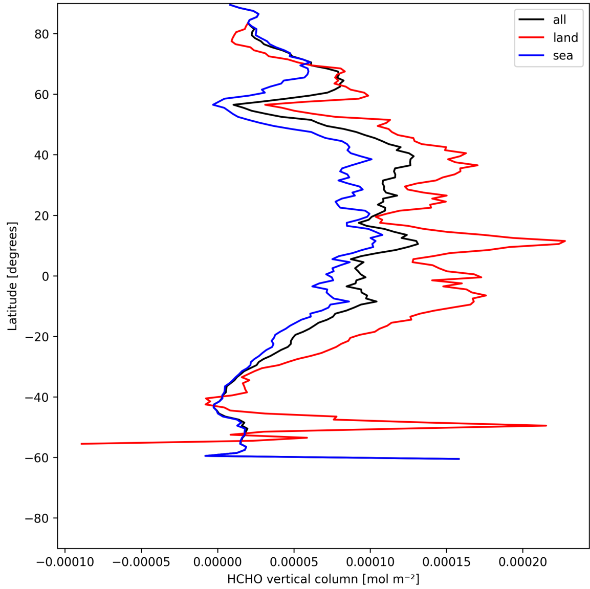
Figure 19: Zonal average of “HCHO vertical column” for 2025-06-24 to 2025-06-25.
