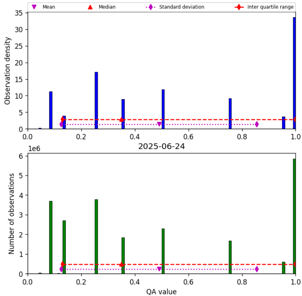
Figure 32: Histogram of “QA value” for 2025-06-24 to 2025-06-25
