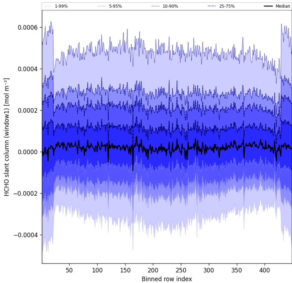
Figure 50: Along track statistics of “HCHO slant column (window1)” for 2025-06-24 to 2025-06-25
