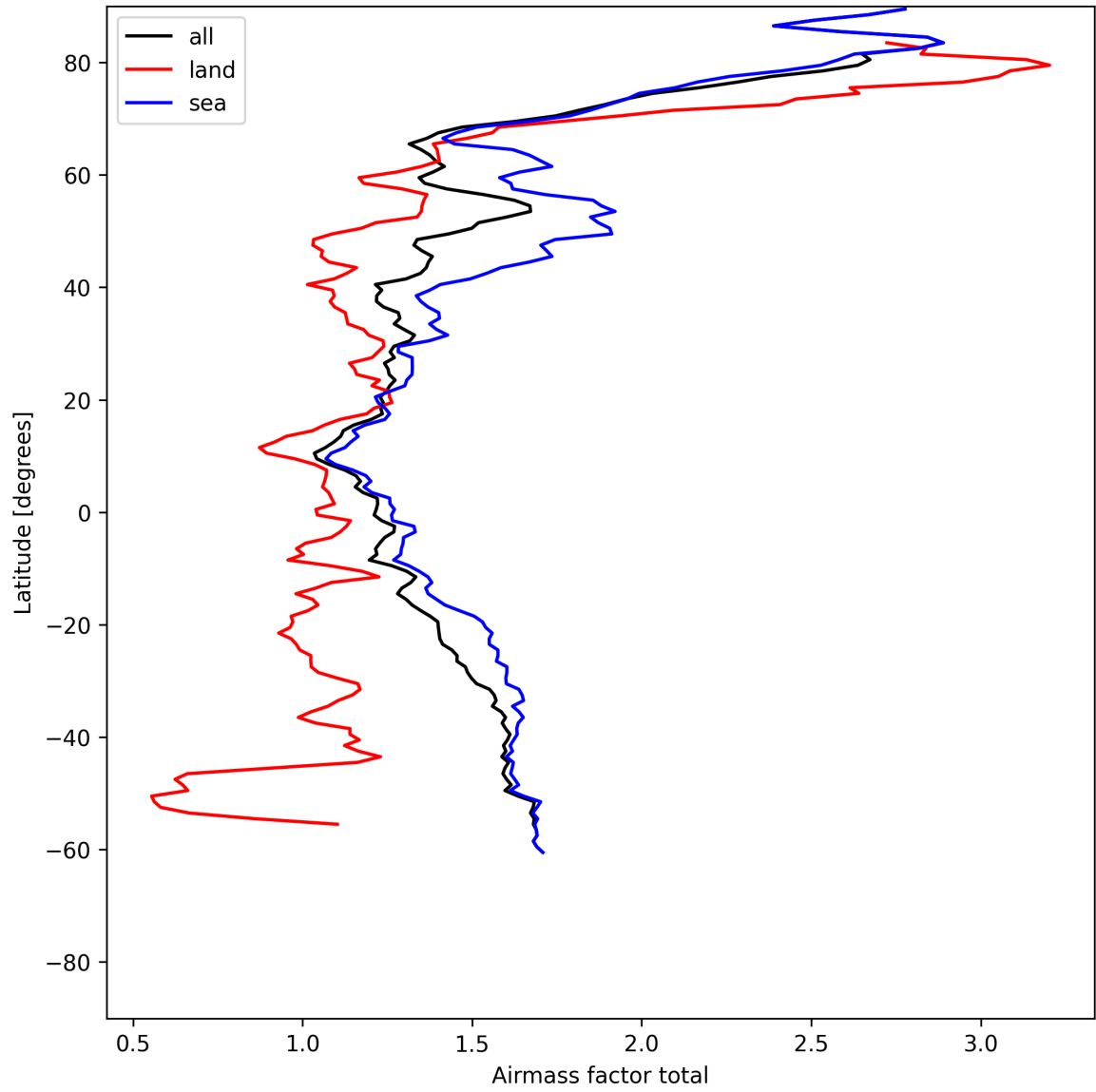
Figure 24: Zonal average of “Airmass factor total” for 2025-06-24 to 2025-06-25.
