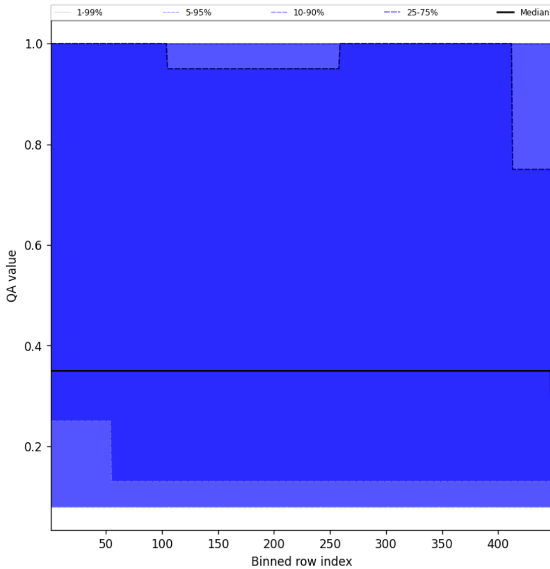
Figure 46: Along track statistics of "QA value" for 2025-06-24 to 2025-06-25
