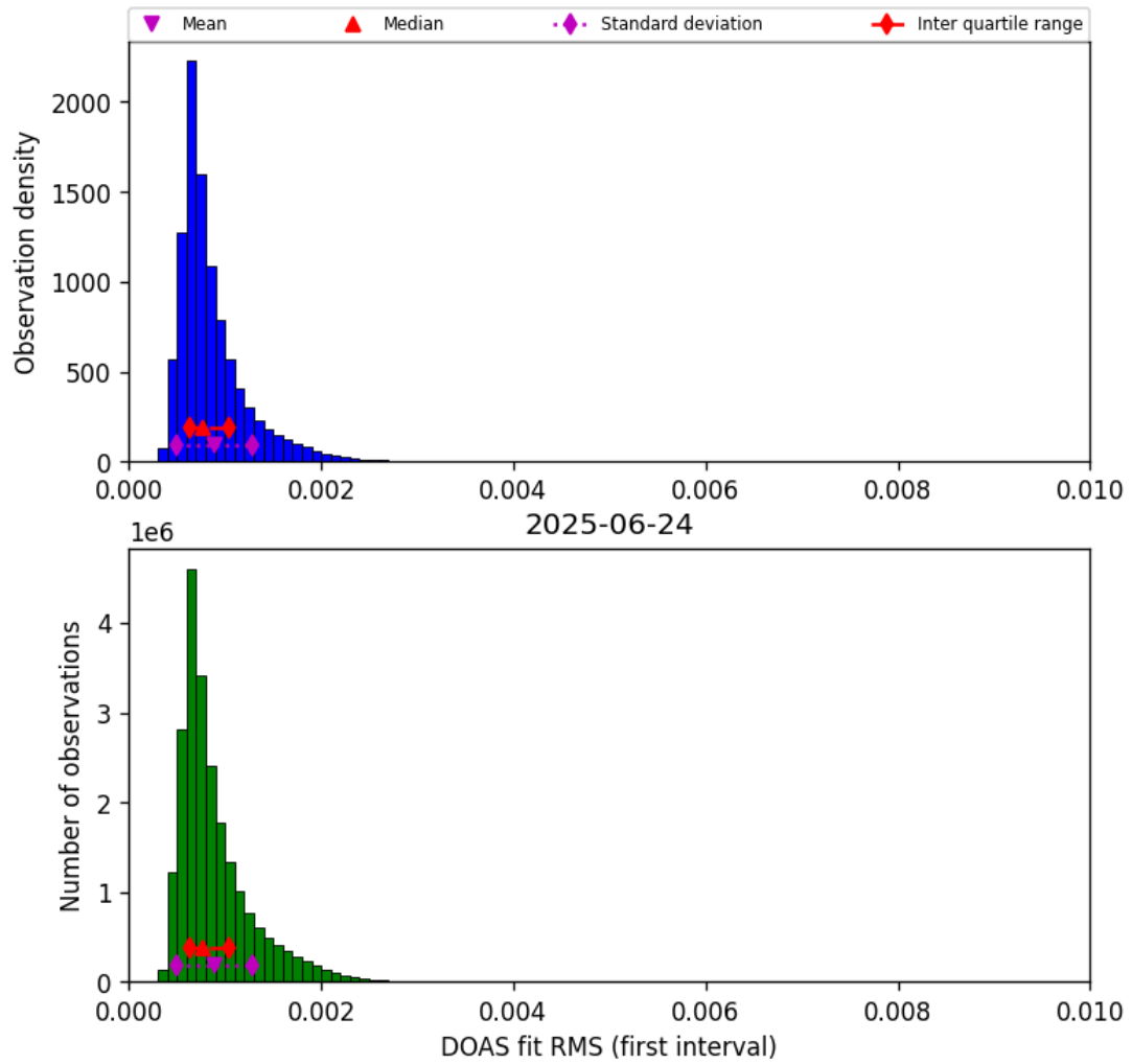
Figure 44: Histogram of “DOAS fit RMS (first interval)” for 2025-06-24 to 2025-06-25
