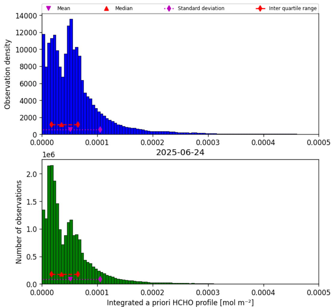
Figure 41: Histogram of “Integrated a priori HCHO profile” for 2025-06-24 to 2025-06-25
