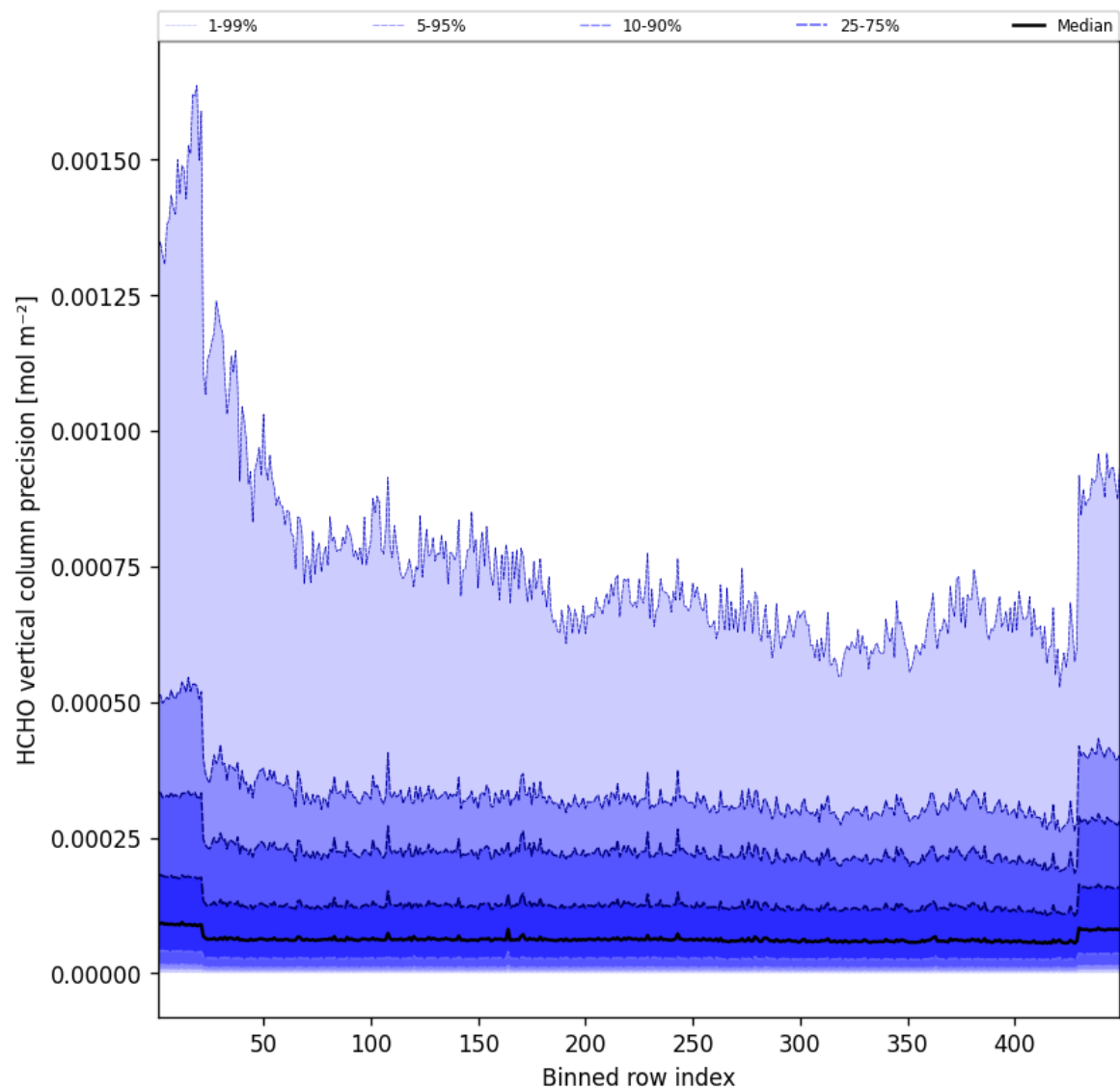
Figure 48: Along track statistics of “HCHO vertical column precision” for 2025-06-24 to 2025-06-25
