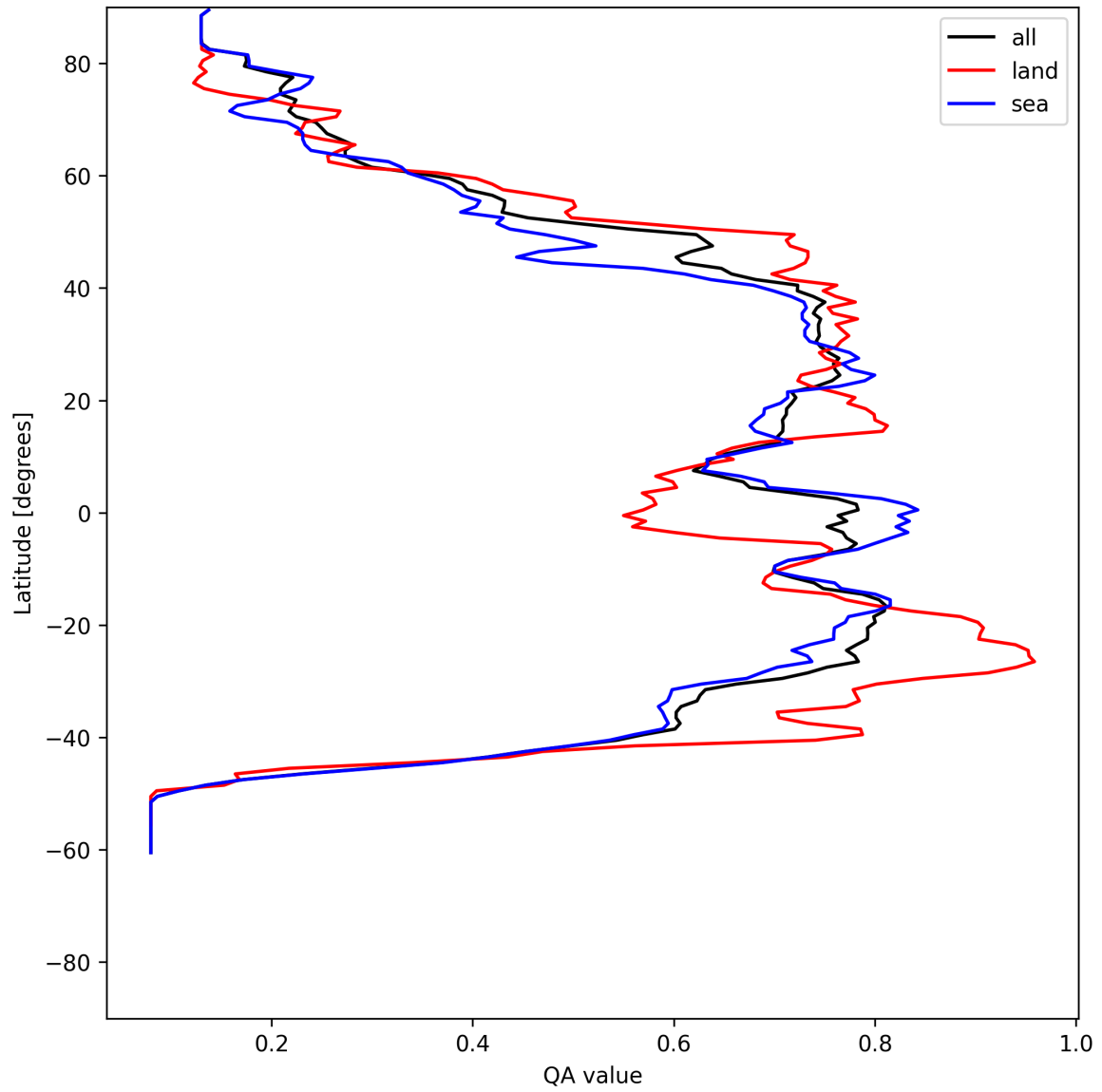
Figure 18: Zonal average of “QA value” for 2025-06-24 to 2025-06-25.
