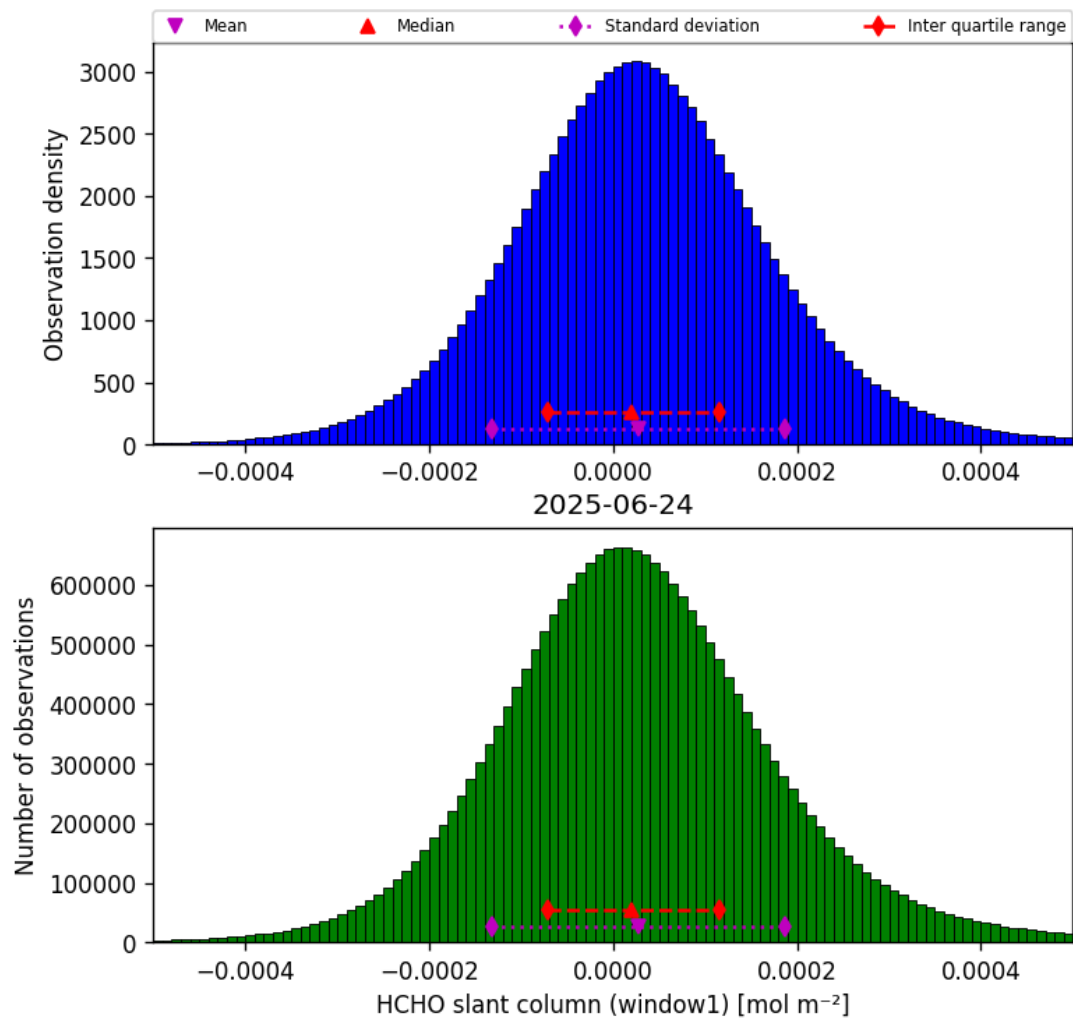
Figure 36: Histogram of “HCHO slant column (window1)” for 2025-06-24 to 2025-06-25
