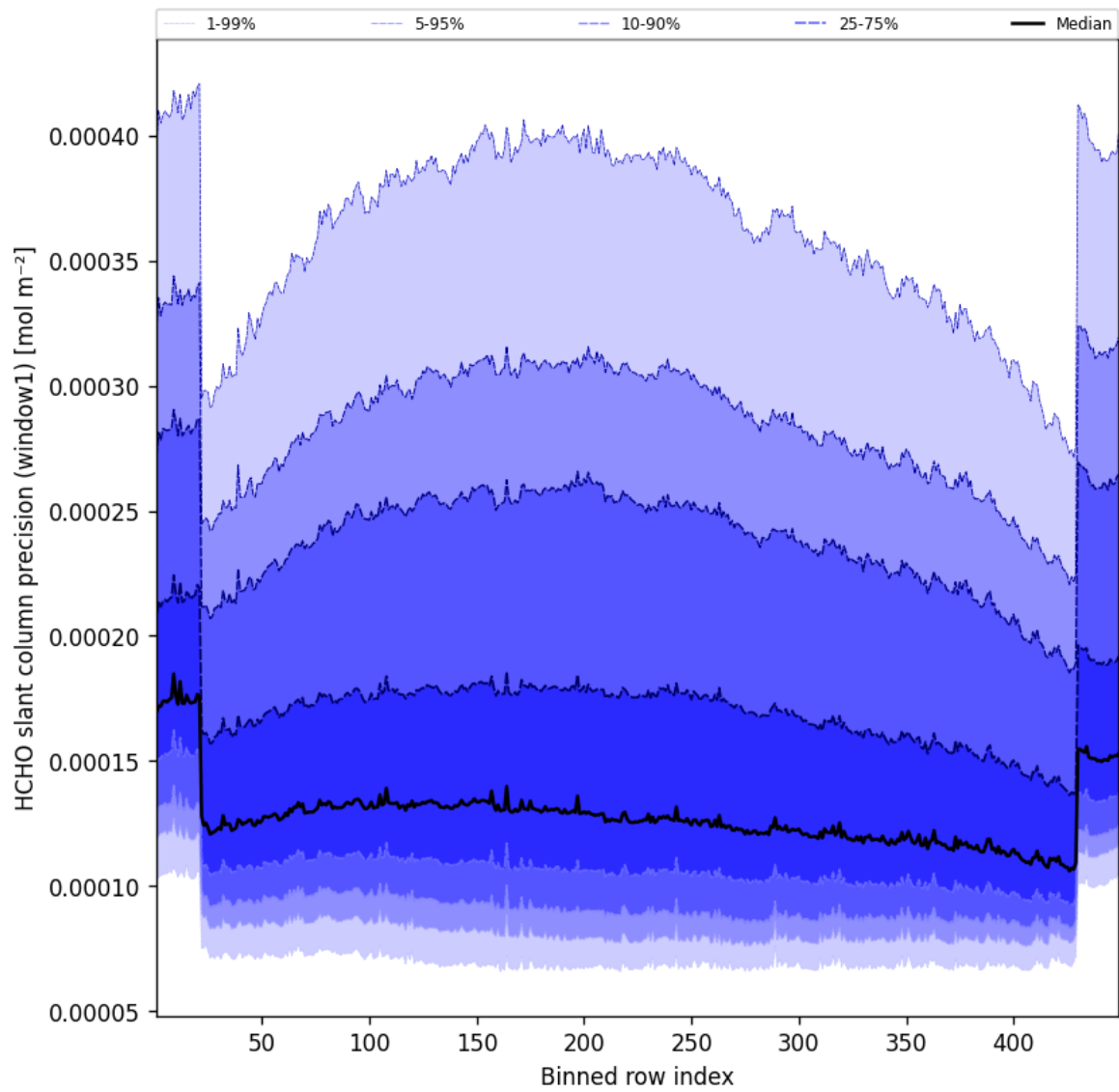
Figure 51: Along track statistics of “HCHO slant column precision (window1)” for 2025-06-24 to 2025-06-25
