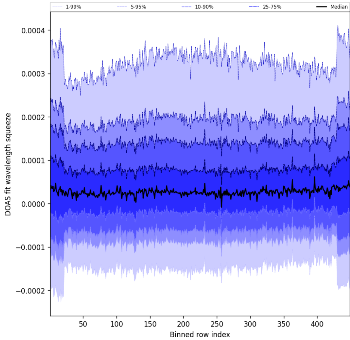
Figure 57: Along track statistics of “DOAS fit wavelength squeeze” for 2025-06-24 to 2025-06-25
