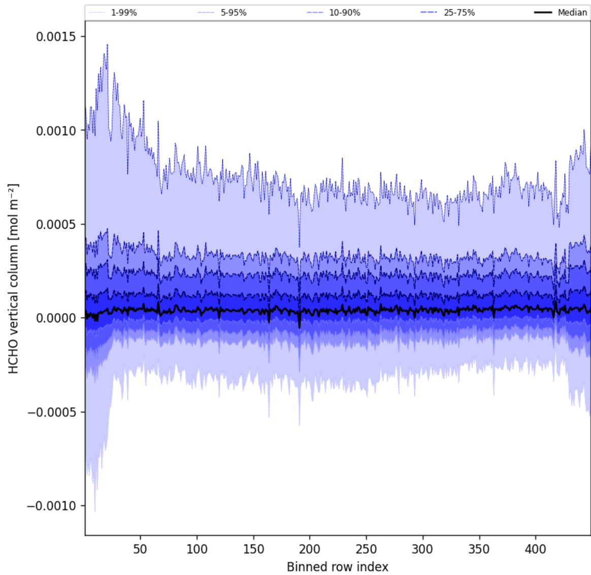
Figure 47: Along track statistics of “HCHO vertical column” for 2025-06-24 to 2025-06-25
