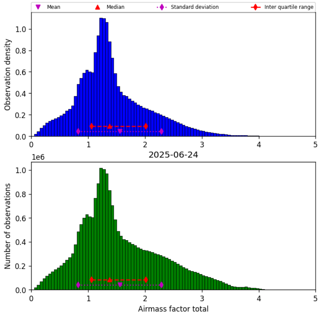
Figure 38: Histogram of “Airmass factor total” for 2025-06-24 to 2025-06-25
