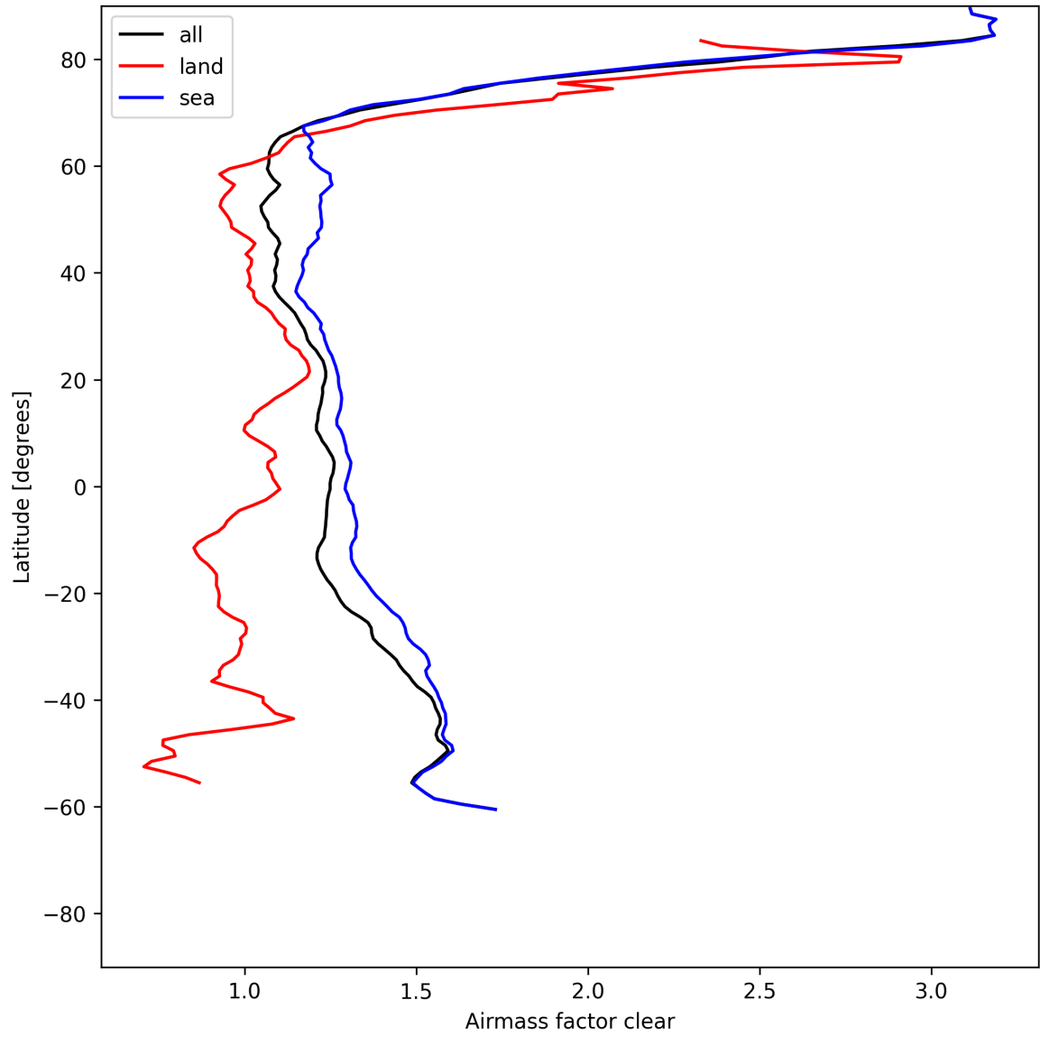
Figure 26: Zonal average of “Airmass factor clear” for 2025-06-24 to 2025-06-25.
