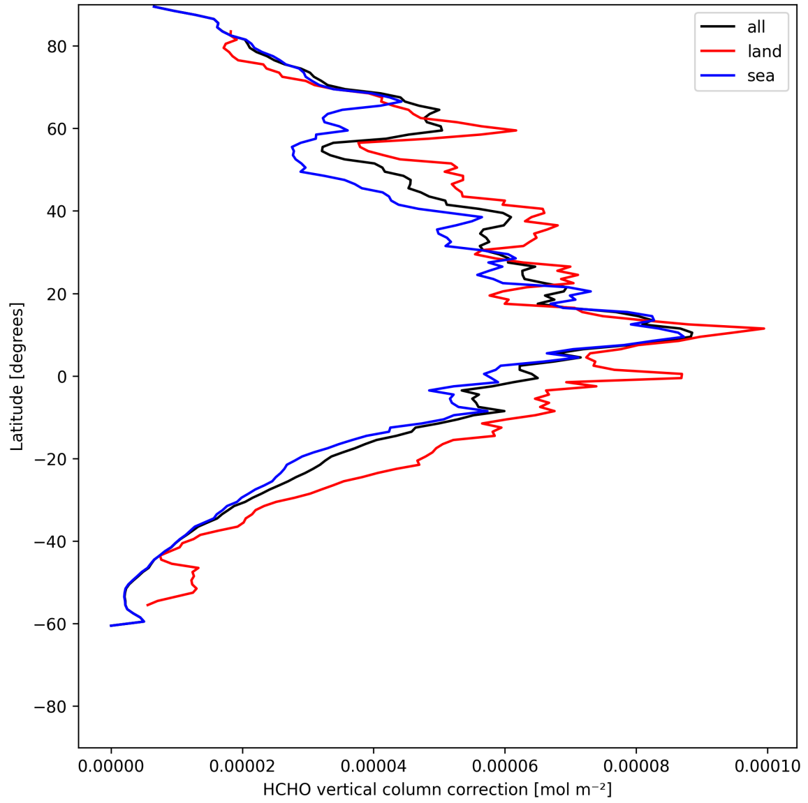
Figure 21: Zonal average of “HCHO vertical column correction” for 2025-06-24 to 2025-06-25.
