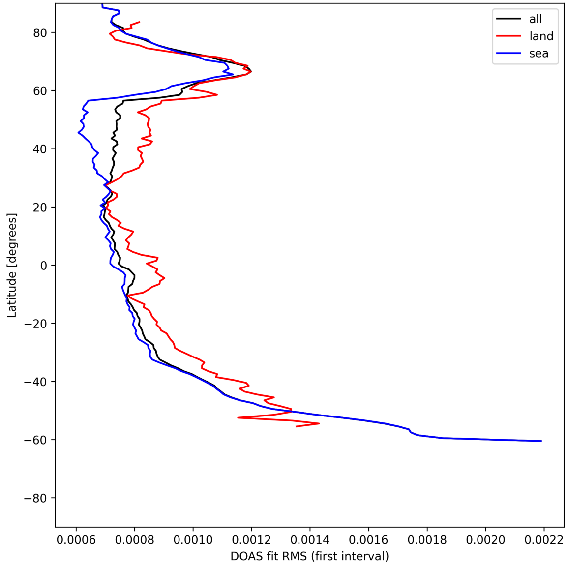
Figure 30: Zonal average of "DOAS fit RMS (first interval)" for 2025-06-24 to 2025-06-25.
