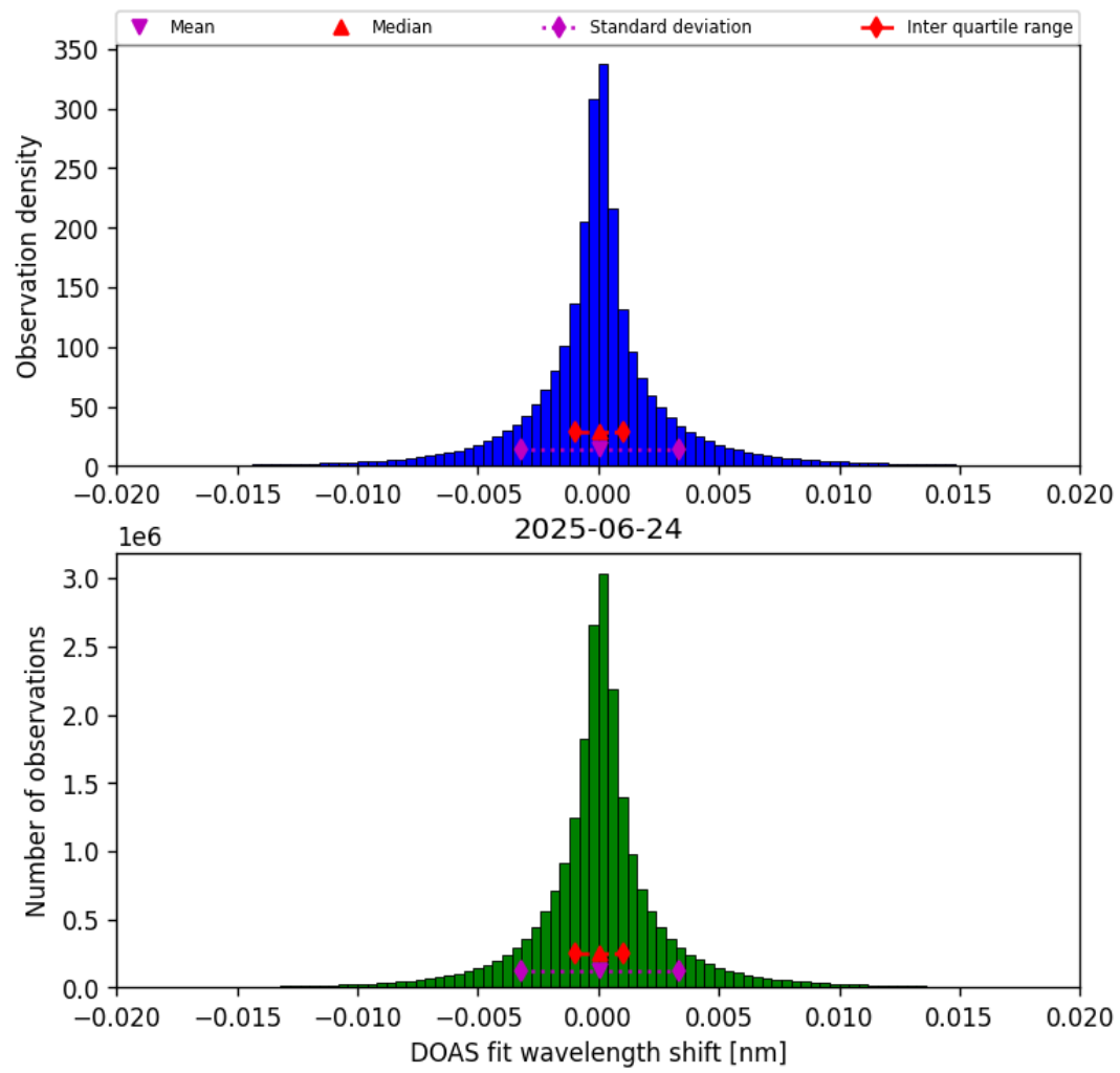
Figure 42: Histogram of “DOAS fit wavelength shift” for 2025-06-24 to 2025-06-25
