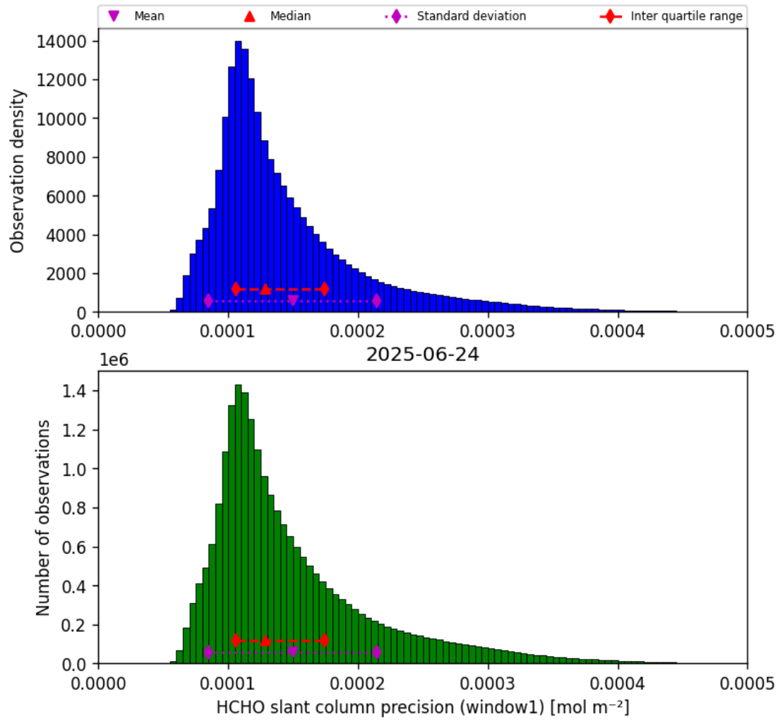
Figure 37: Histogram of “HCHO slant column precision (window1)” for 2025-06-24 to 2025-06-25
