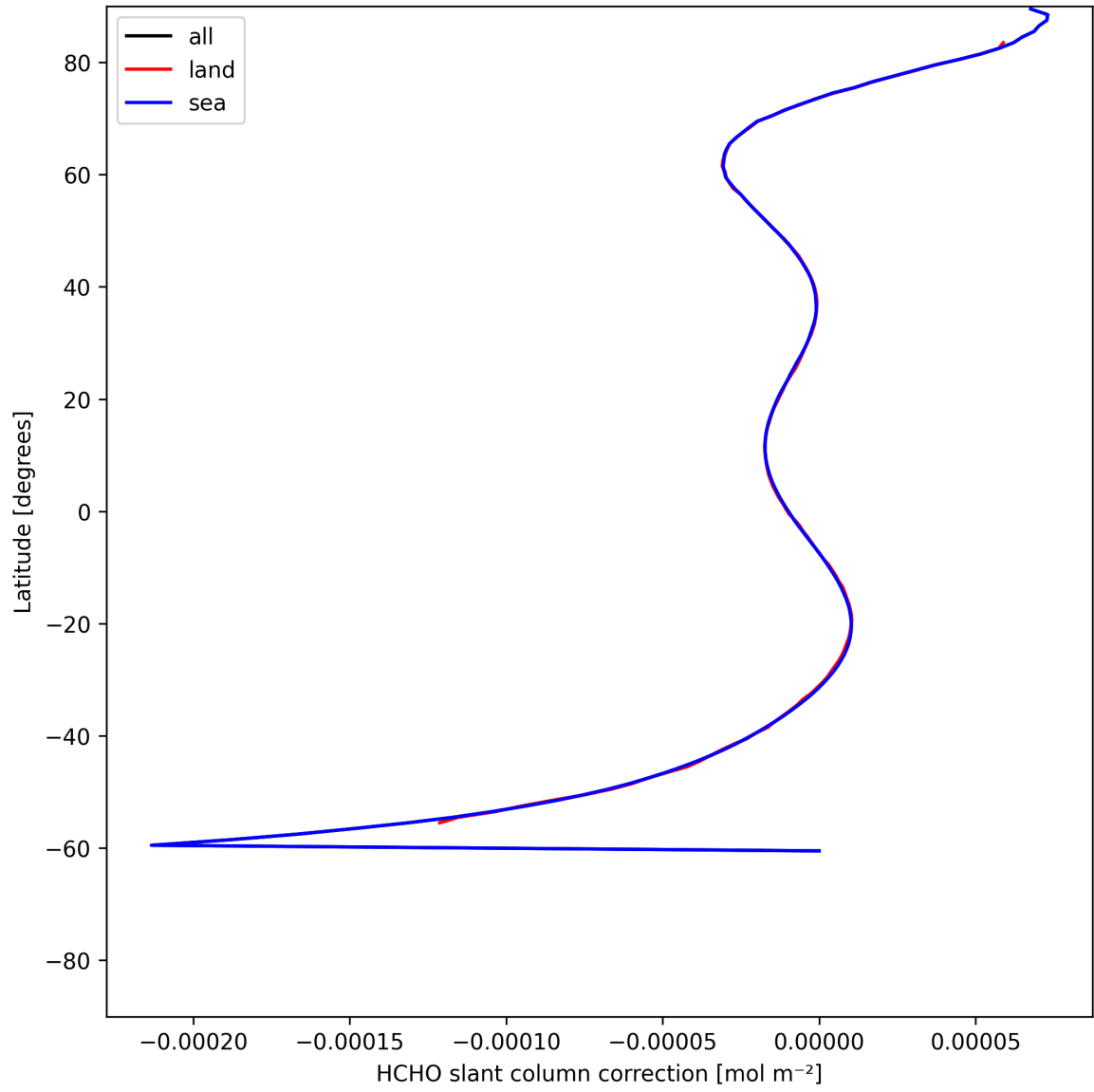
Figure 31: Zonal average of “HCHO slant column correction” for 2025-06-24 to 2025-06-25.
