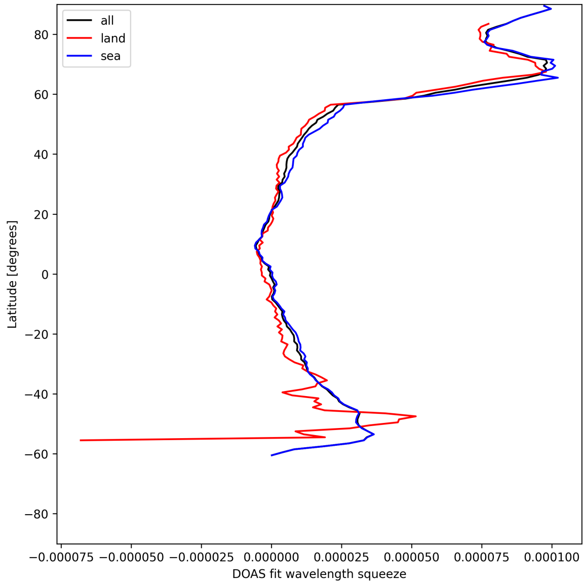
Figure 29: Zonal average of “DOAS fit wavelength squeeze” for 2025-06-24 to 2025-06-25.
