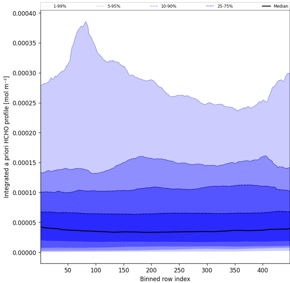
Figure 55: Along track statistics of "Integrated a priori HCHO profile" for 2025-06-24 to 2025-06-25
