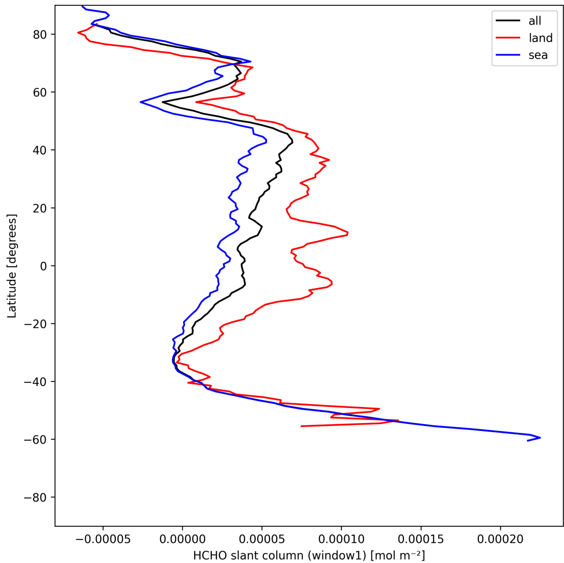
Figure 22: Zonal average of “HCHO slant column (window1)” for 2025-06-24 to 2025-06-25.
