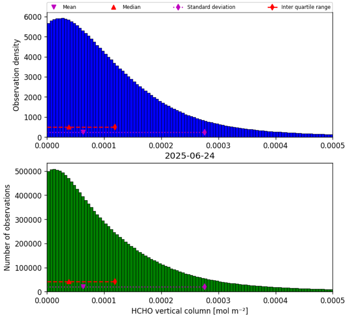
Figure 33: Histogram of “HCHO vertical column” for 2025-06-24 to 2025-06-25
