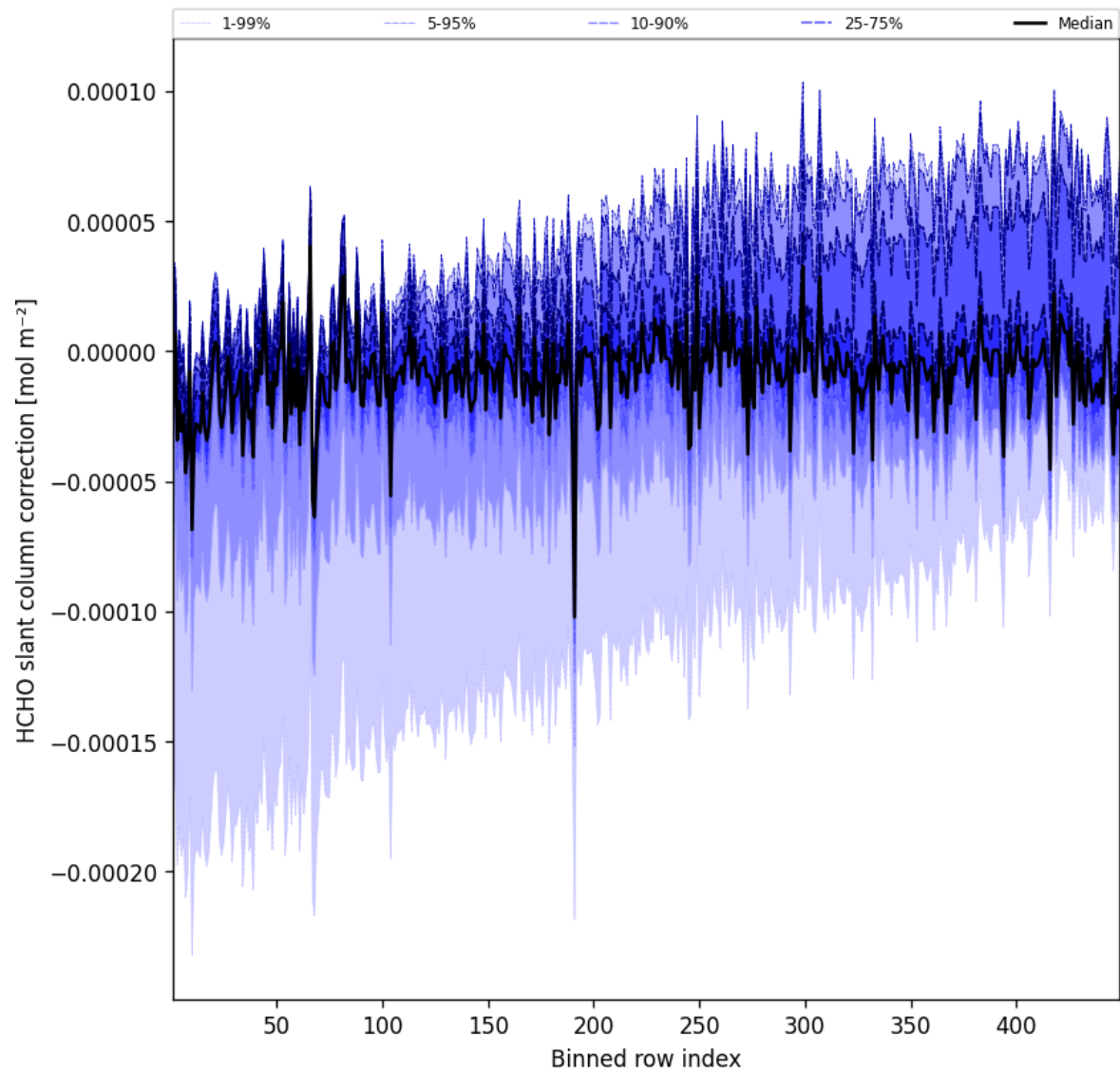
Figure 59: Along track statistics of “HCHO slant column correction” for 2025-06-24 to 2025-06-25
