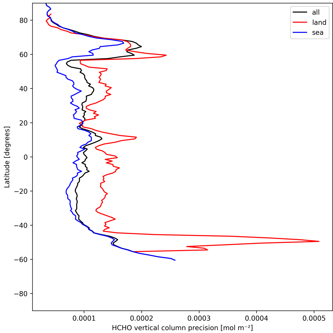
Figure 20: Zonal average of “HCHO vertical column precision” for 2025-06-24 to 2025-06-25.
