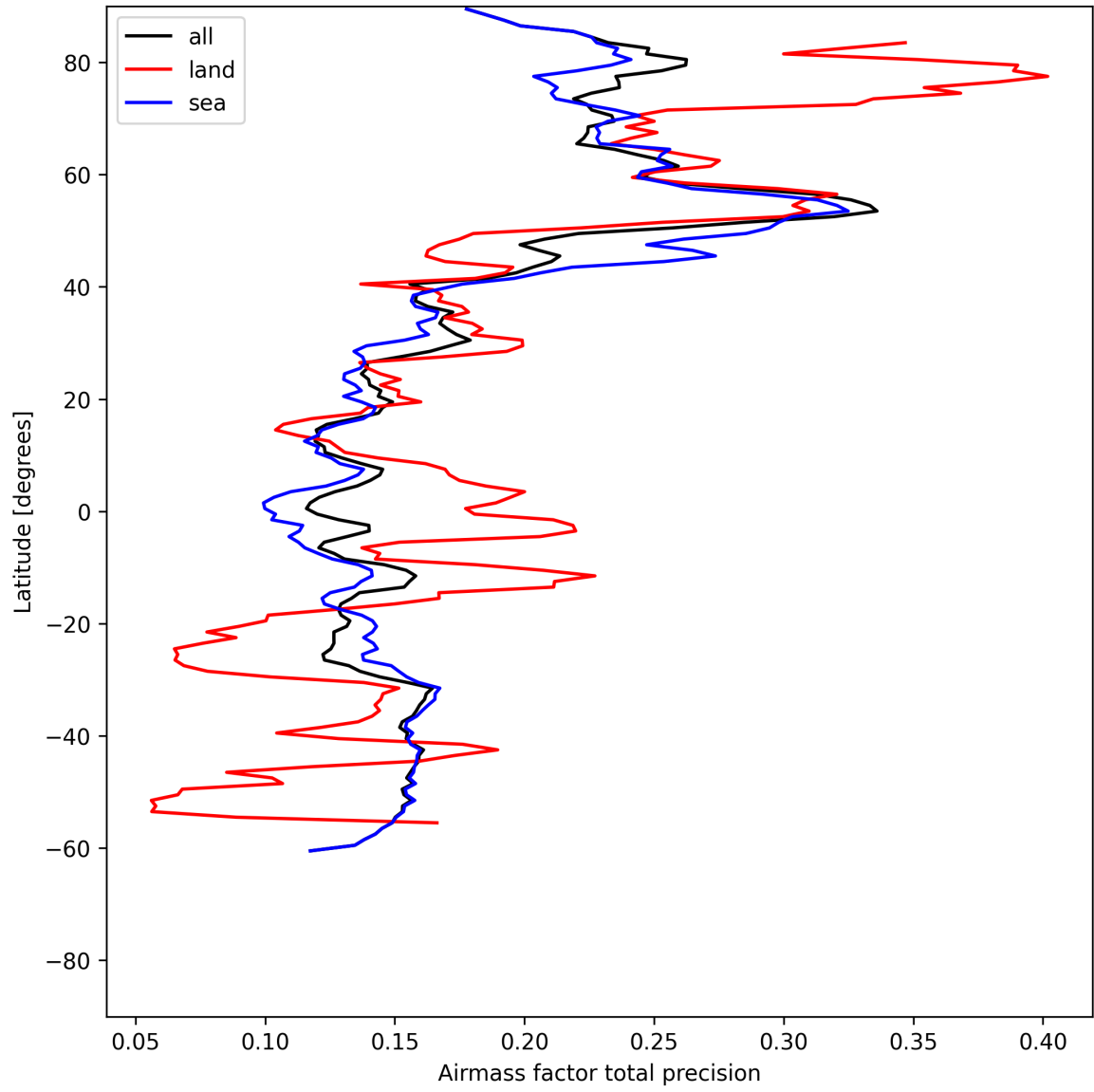
Figure 25: Zonal average of “Airmass factor total precision” for 2025-06-24 to 2025-06-25.
