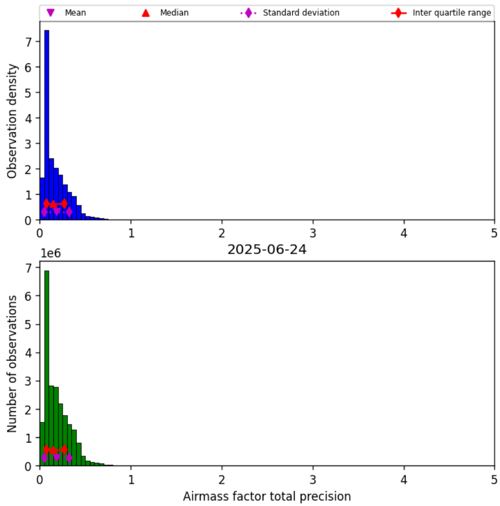
Figure 39: Histogram of “Airmass factor total precision” for 2025-06-24 to 2025-06-25
