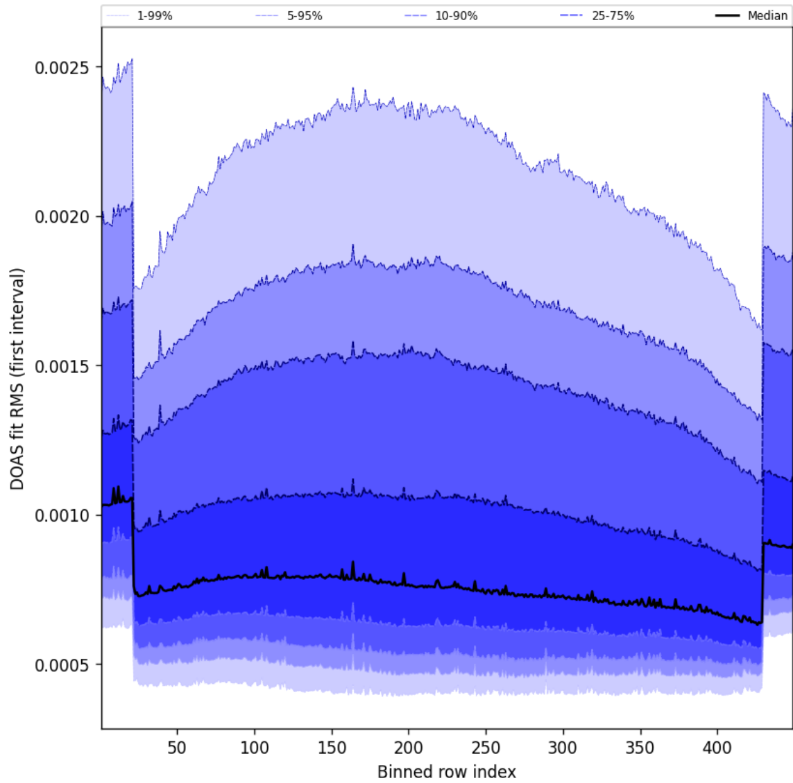
Figure 58: Along track statistics of “DOAS fit RMS (first interval)” for 2025-06-24 to 2025-06-25
