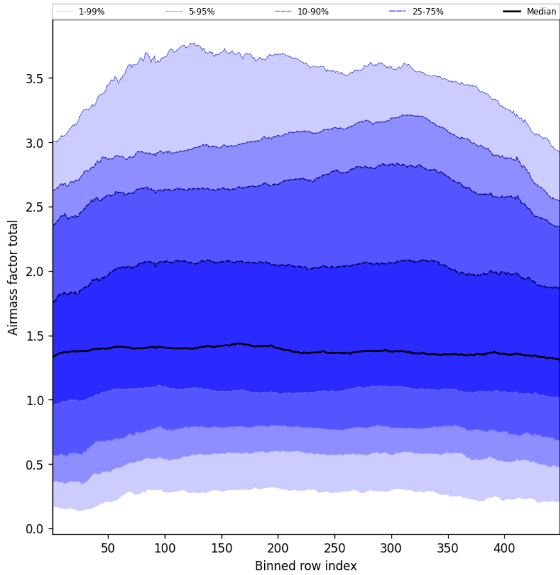
Figure 52: Along track statistics of “Airmass factor total” for 2025-06-24 to 2025-06-25
