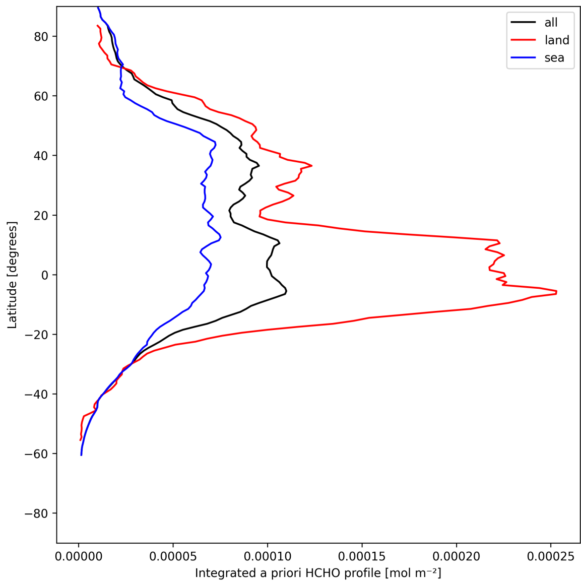
Figure 27: Zonal average of “Integrated a priori HCHO profile” for 2025-06-24 to 2025-06-25.
