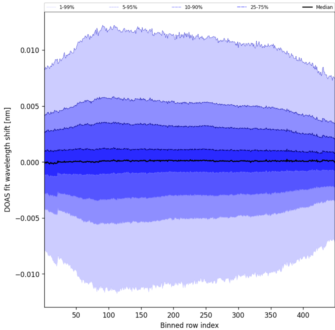
Figure 56: Along track statistics of “DOAS fit wavelength shift” for 2025-06-25 to 2025-06-25
