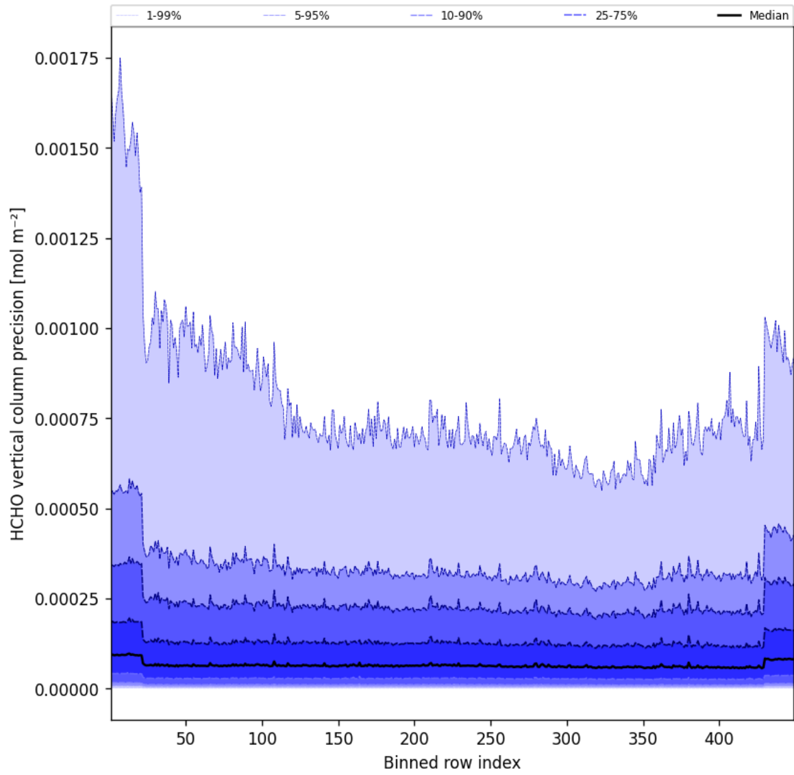
Figure 48: Along track statistics of “HCHO vertical column precision” for 2025-06-25 to 2025-06-25
