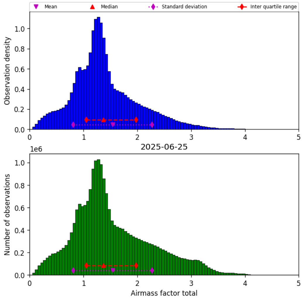
Figure 38: Histogram of “Airmass factor total” for 2025-06-25 to 2025-06-25
