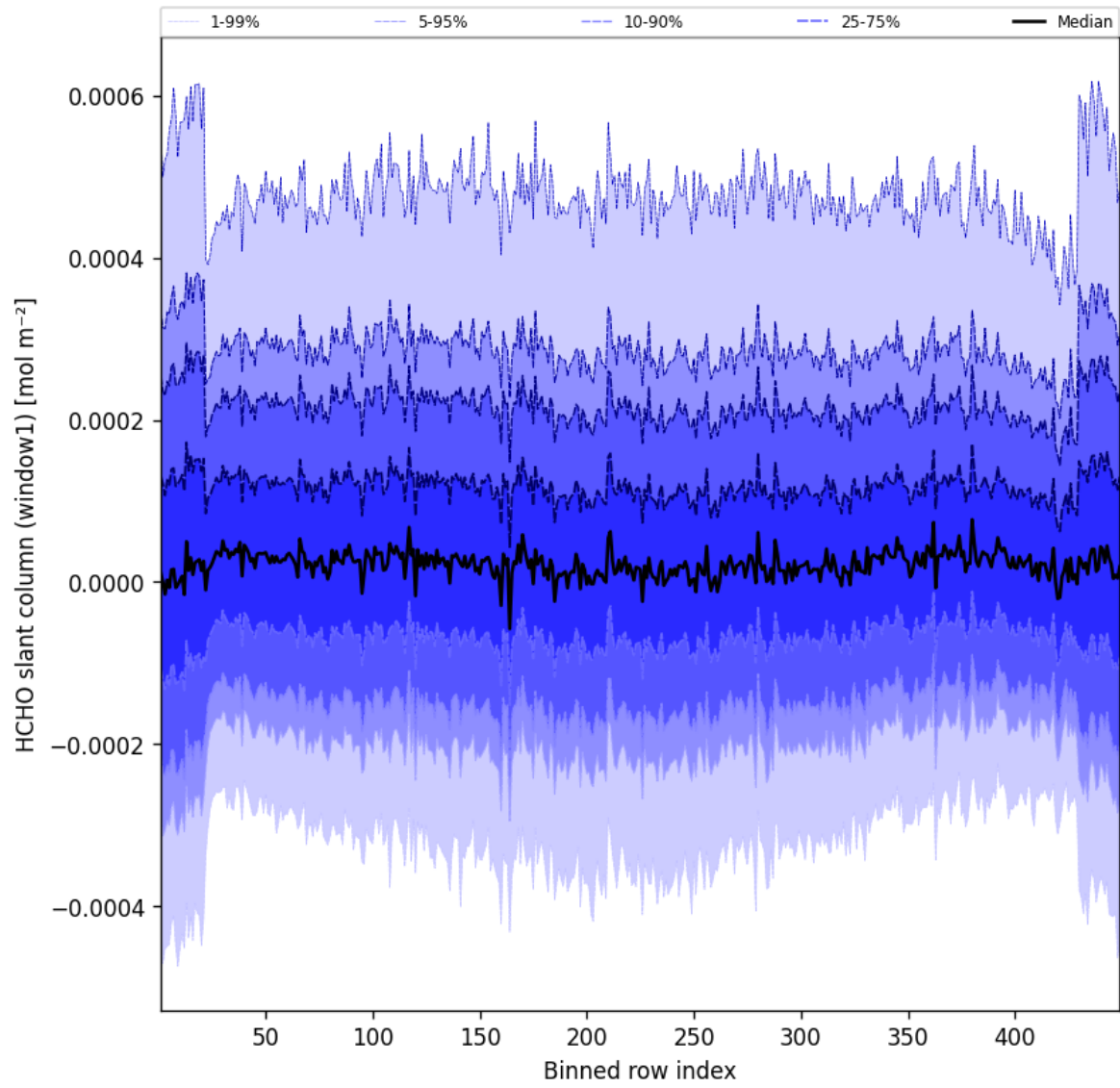
Figure 50: Along track statistics of “HCHO slant column (window1)” for 2025-06-25 to 2025-06-25
