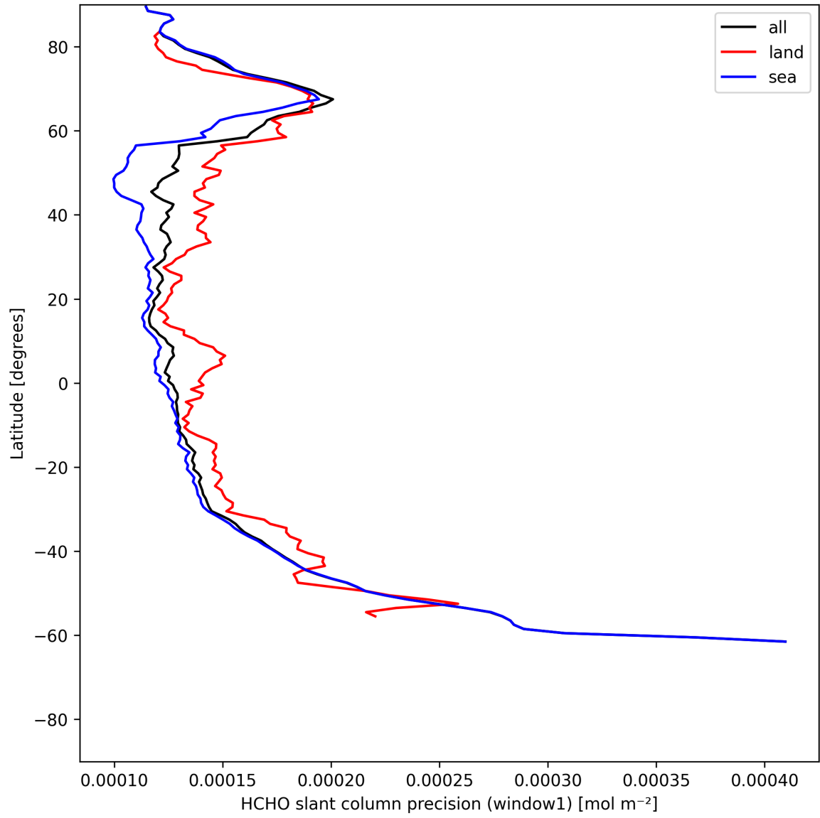
Figure 23: Zonal average of “HCHO slant column precision (window1)” for 2025-06-25 to 2025-06-25.
