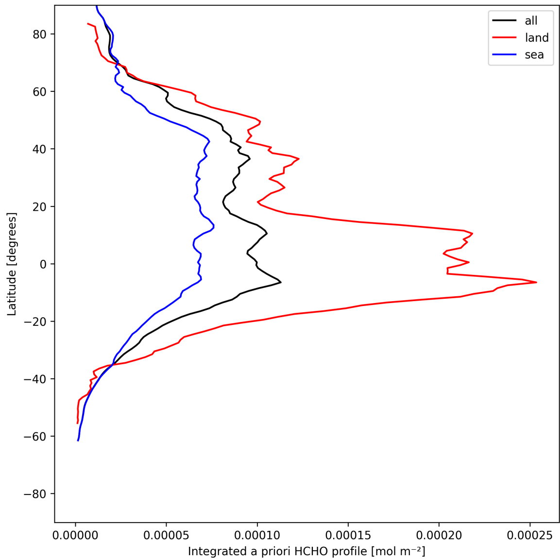
Figure 27: Zonal average of “Integrated a priori HCHO profile” for 2025-06-25 to 2025-06-25.
