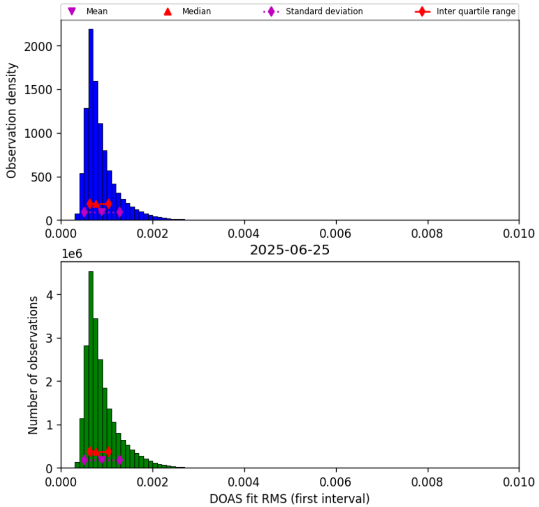
Figure 44: Histogram of “DOAS fit RMS (first interval)” for 2025-06-25 to 2025-06-25
