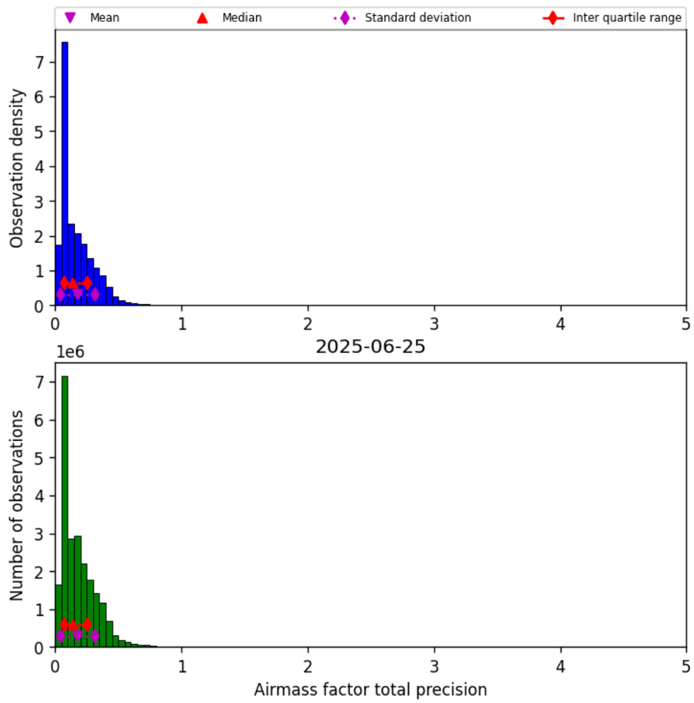
Figure 39: Histogram of “Airmass factor total precision” for 2025-06-25 to 2025-06-25
