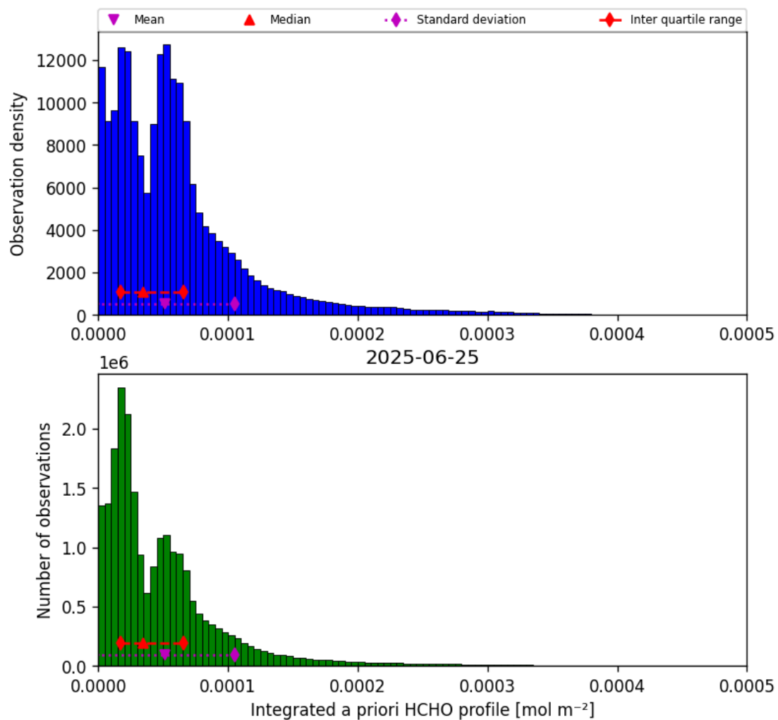
Figure 41: Histogram of “Integrated a priori HCHO profile” for 2025-06-25 to 2025-06-25
