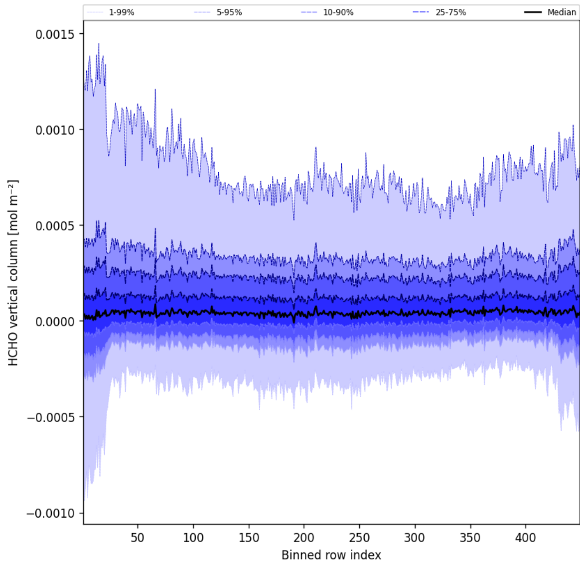
Figure 47: Along track statistics of “HCHO vertical column” for 2025-06-25 to 2025-06-25
