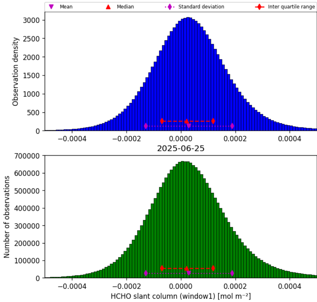
Figure 36: Histogram of “HCHO slant column (window1)” for 2025-06-25 to 2025-06-25
