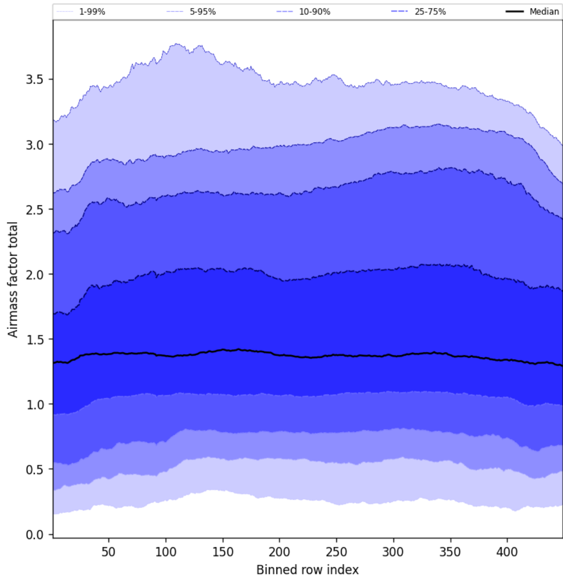
Figure 52: Along track statistics of “Airmass factor total” for 2025-06-25 to 2025-06-25
