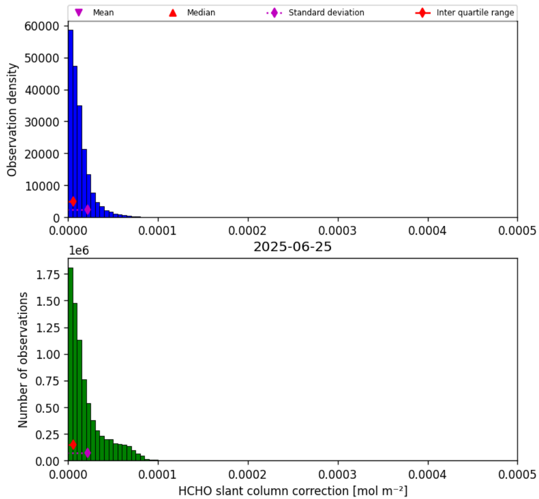
Figure 45: Histogram of “HCHO slant column correction” for 2025-06-25 to 2025-06-25
