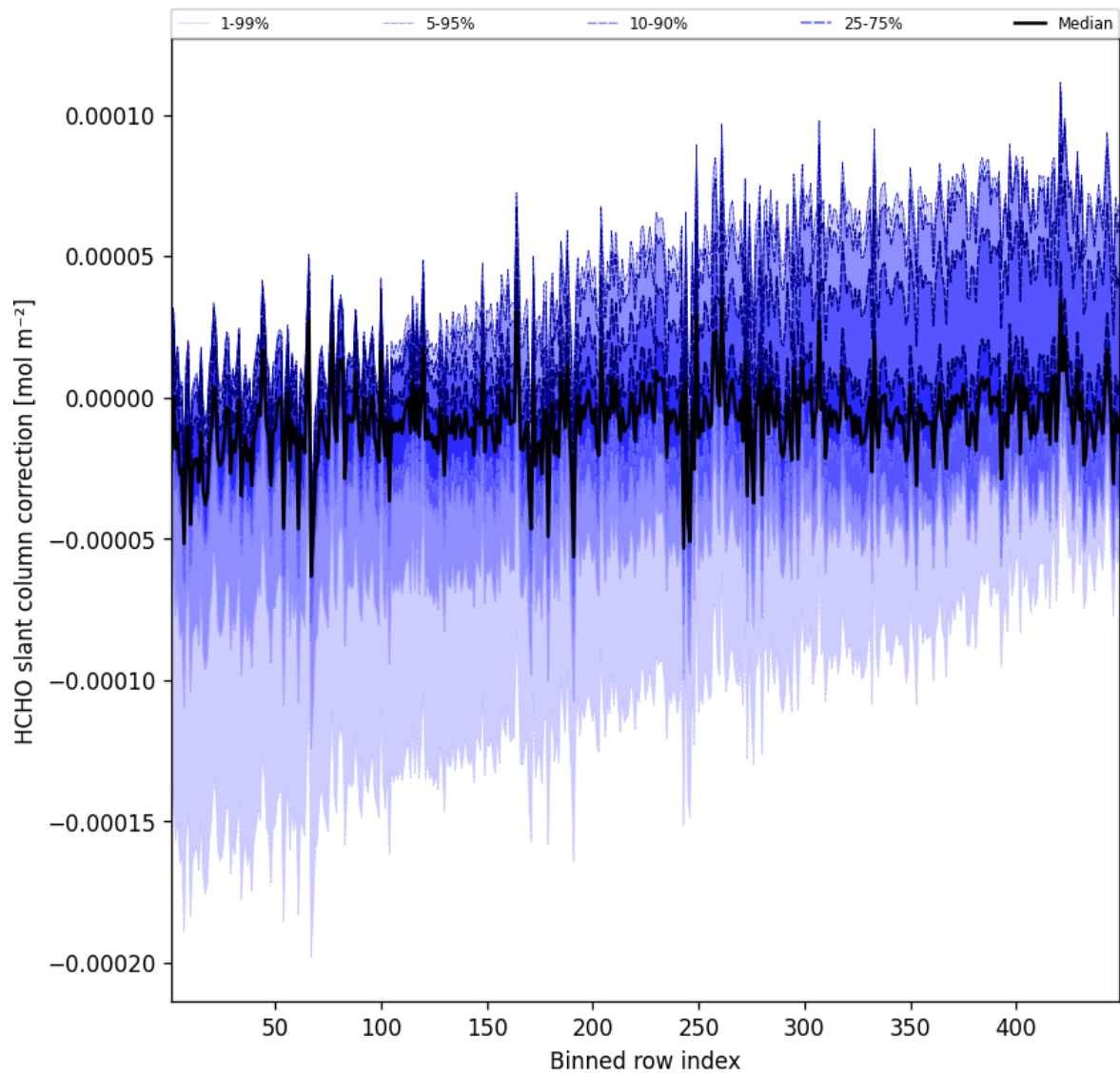
Figure 59: Along track statistics of “HCHO slant column correction” for 2025-06-25 to 2025-06-25
