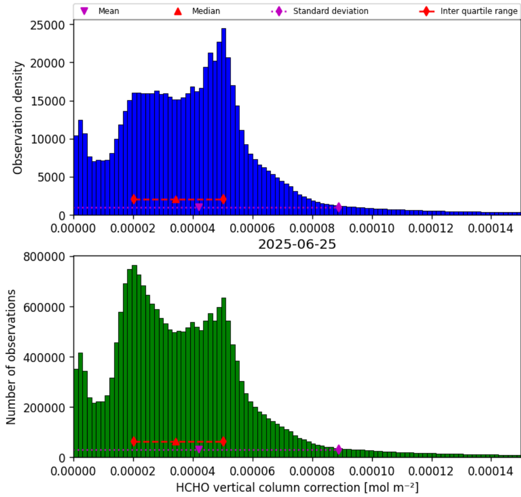
Figure 35: Histogram of “HCHO vertical column correction” for 2025-06-25 to 2025-06-25
