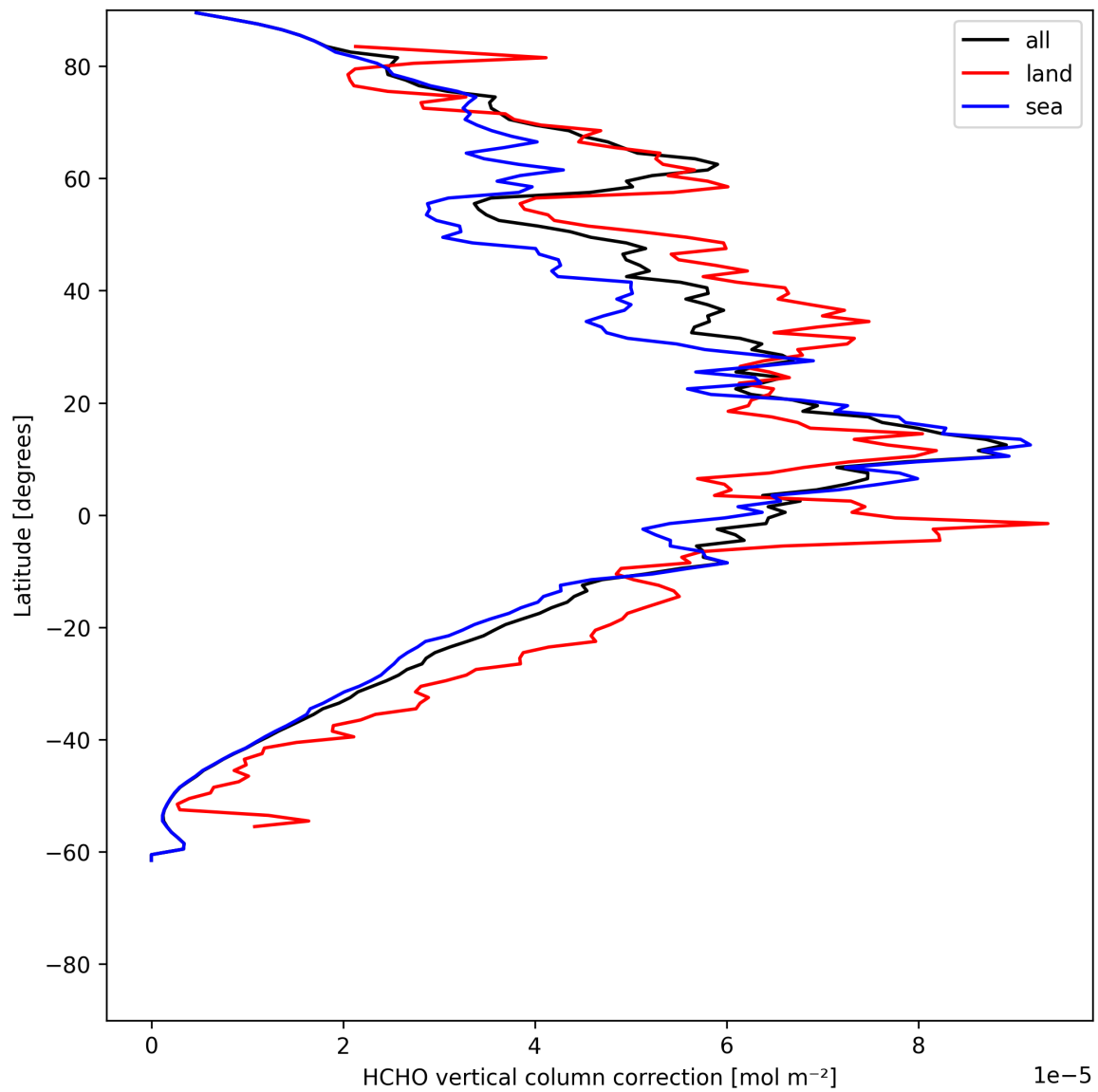
Figure 21: Zonal average of “HCHO vertical column correction” for 2025-06-25 to 2025-06-25.
