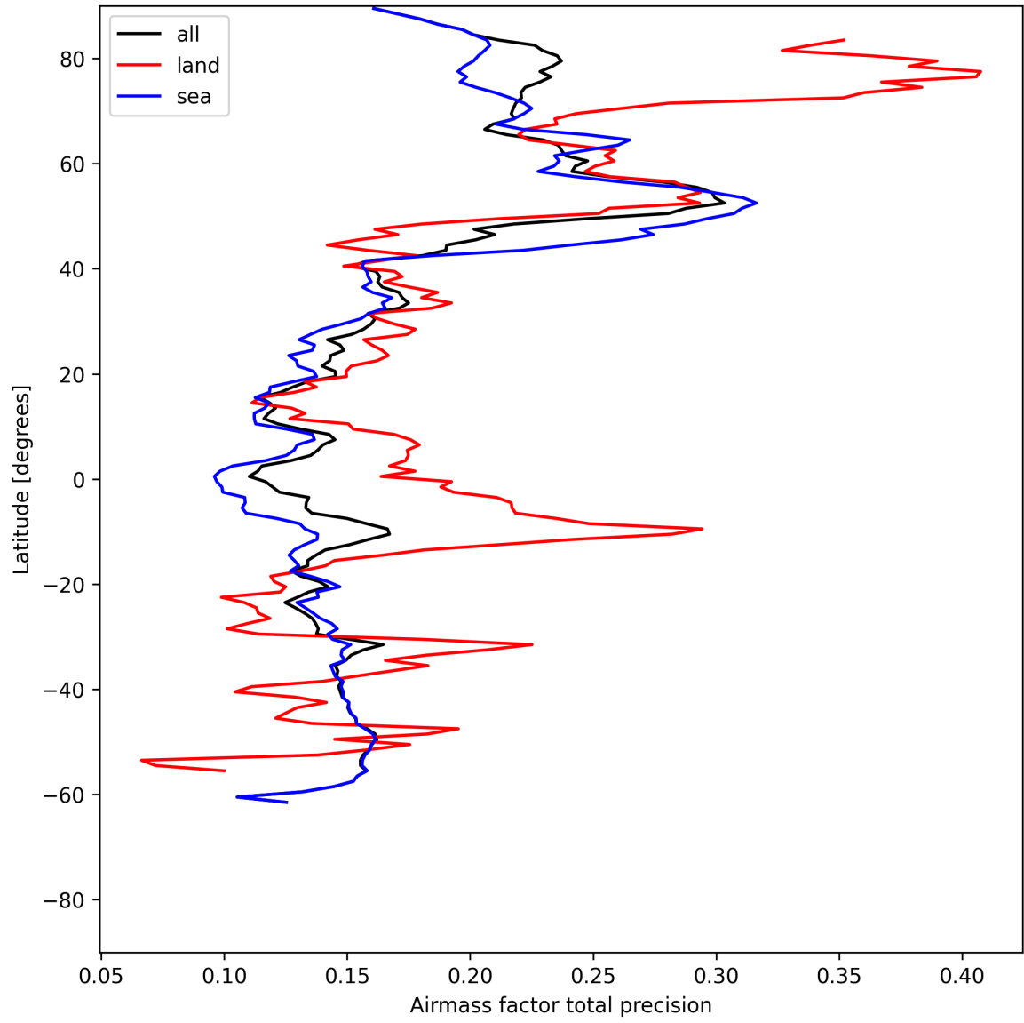
Figure 25: Zonal average of “Airmass factor total precision” for 2025-06-25 to 2025-06-25.
