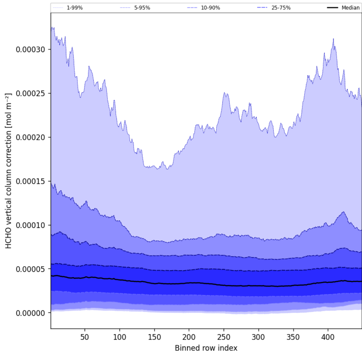
Figure 49: Along track statistics of “HCHO vertical column correction” for 2025-06-25 to 2025-06-25
