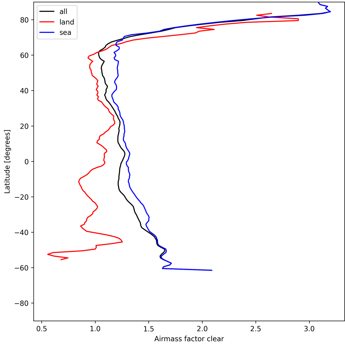
Figure 26: Zonal average of “Airmass factor clear” for 2025-06-25 to 2025-06-25.
