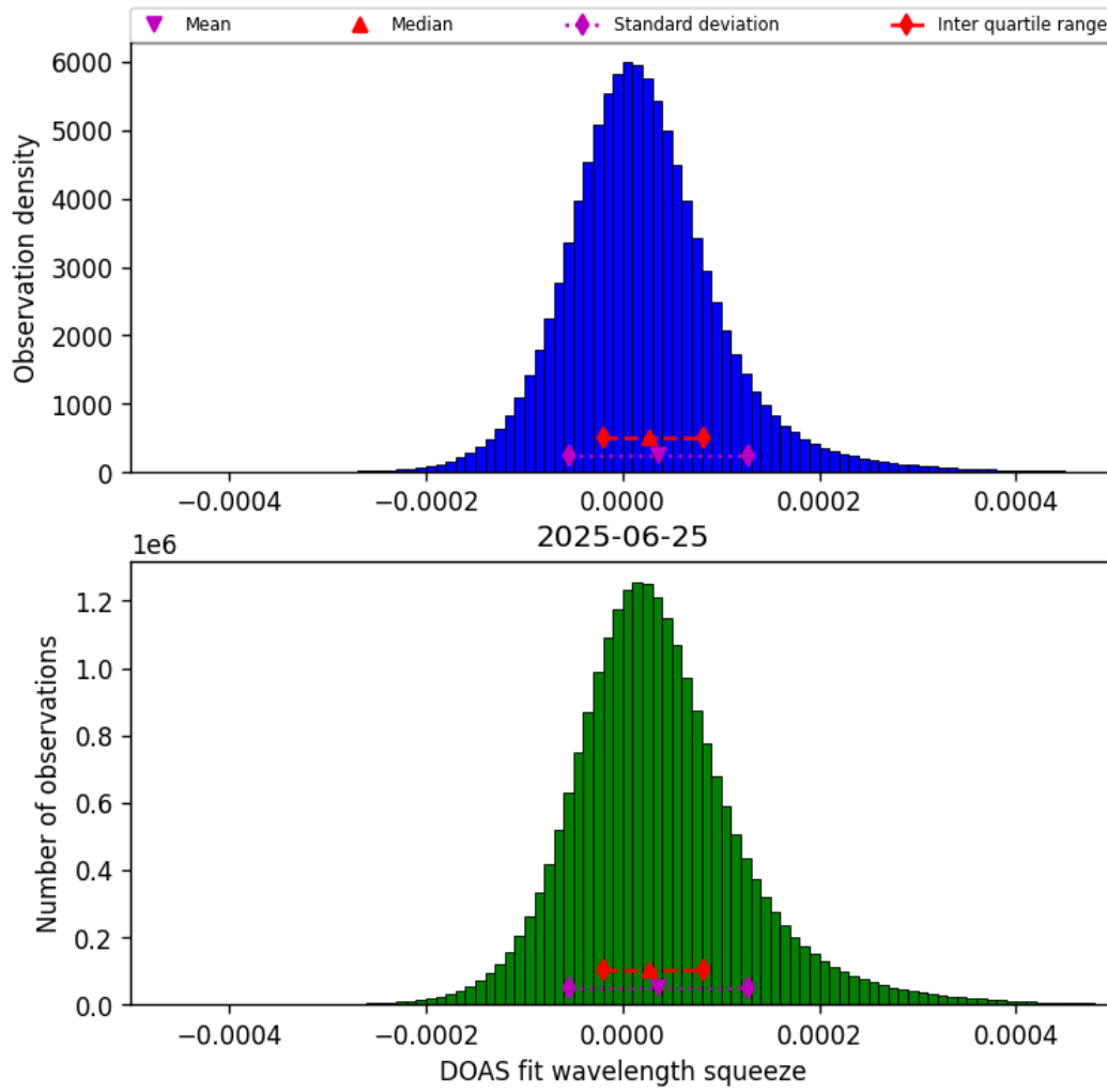
Figure 43: Histogram of “DOAS fit wavelength squeeze” for 2025-06-25 to 2025-06-25
