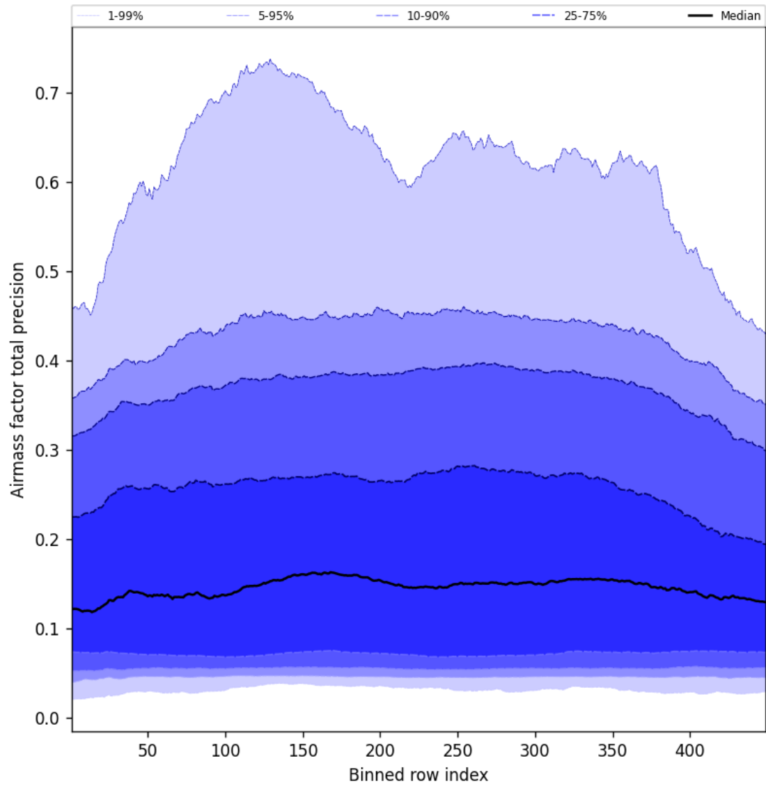
Figure 53: Along track statistics of “Airmass factor total precision” for 2025-06-25 to 2025-06-25
