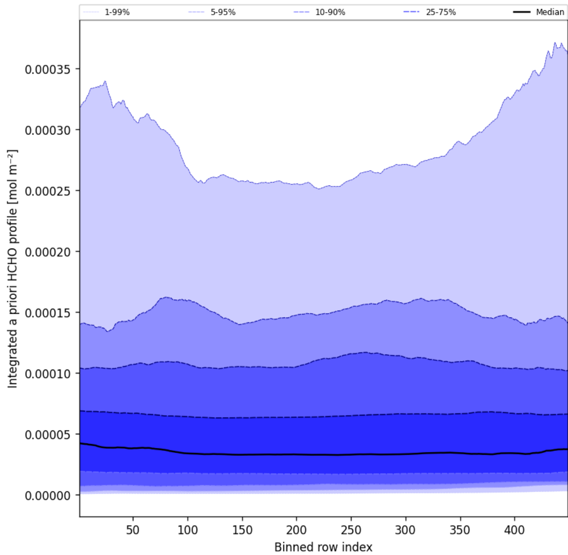
Figure 55: Along track statistics of "Integrated a priori HCHO profile" for 2025-06-25 to 2025-06-25
