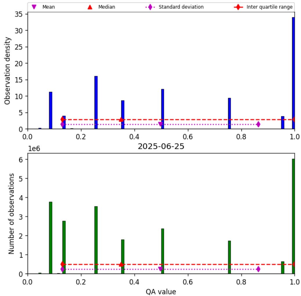
Figure 32: Histogram of “QA value” for 2025-06-25 to 2025-06-25
