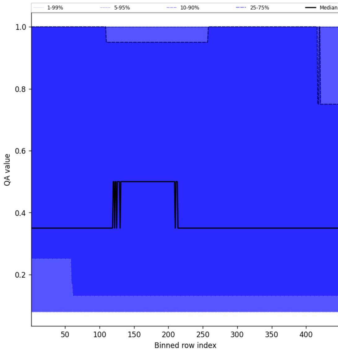
Figure 46: Along track statistics of “QA value” for 2025-06-25 to 2025-06-25
