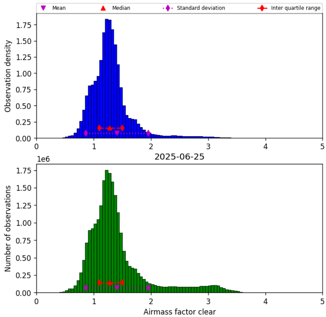
Figure 40: Histogram of “Airmass factor clear” for 2025-06-25 to 2025-06-25
