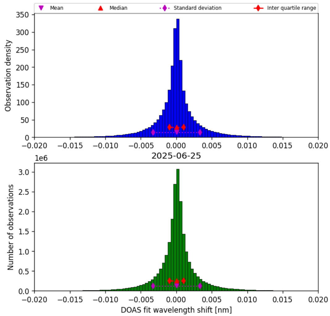
Figure 42: Histogram of “DOAS fit wavelength shift” for 2025-06-25 to 2025-06-25
