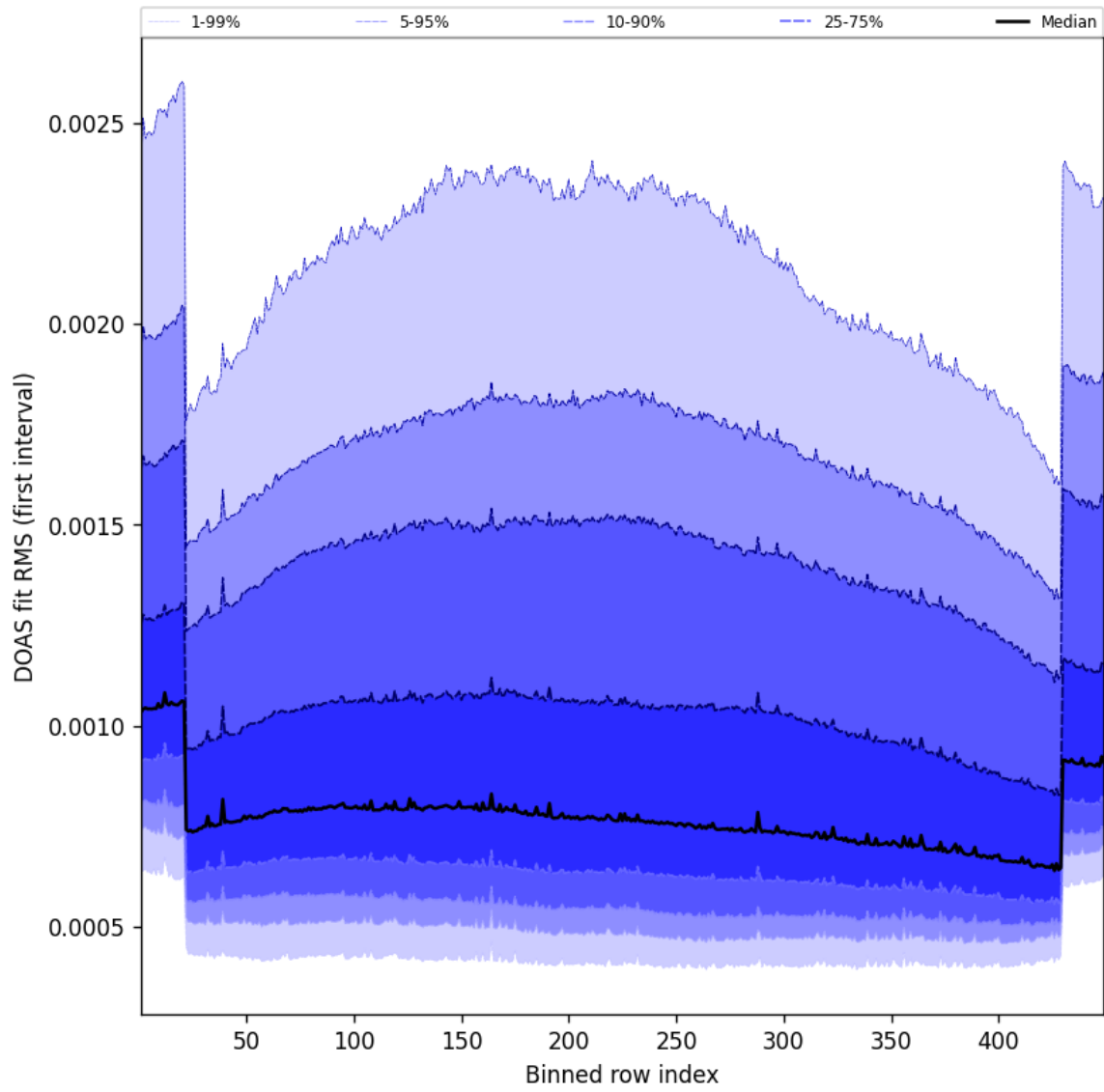
Figure 58: Along track statistics of “DOAS fit RMS (first interval)” for 2025-06-25 to 2025-06-25
