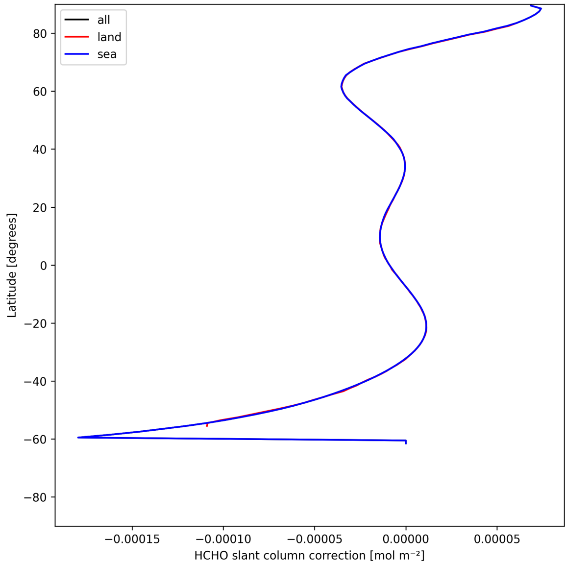
Figure 31: Zonal average of “HCHO slant column correction” for 2025-06-25 to 2025-06-25.
