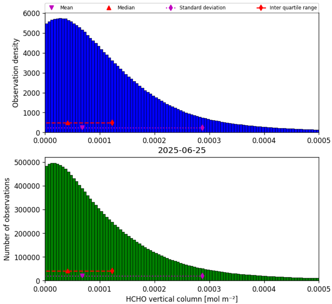
Figure 33: Histogram of “HCHO vertical column” for 2025-06-25 to 2025-06-25
