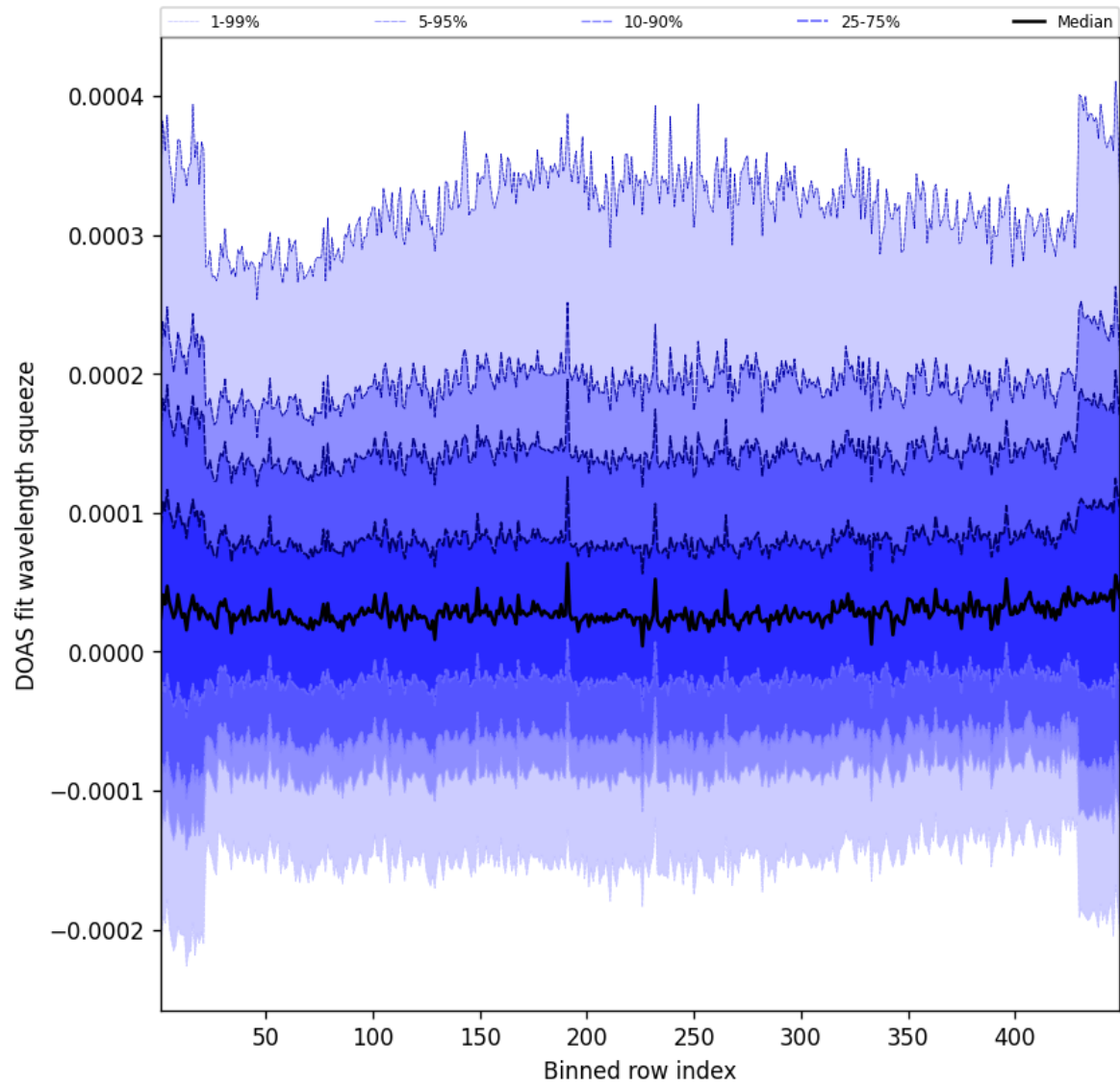
Figure 57: Along track statistics of “DOAS fit wavelength squeeze” for 2025-06-25 to 2025-06-25
