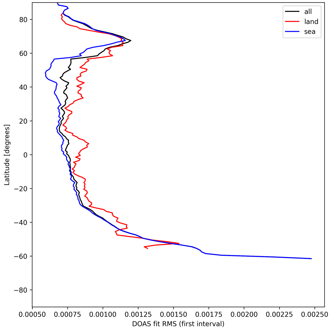
Figure 30: Zonal average of “DOAS fit RMS (first interval)” for 2025-06-25 to 2025-06-25.
