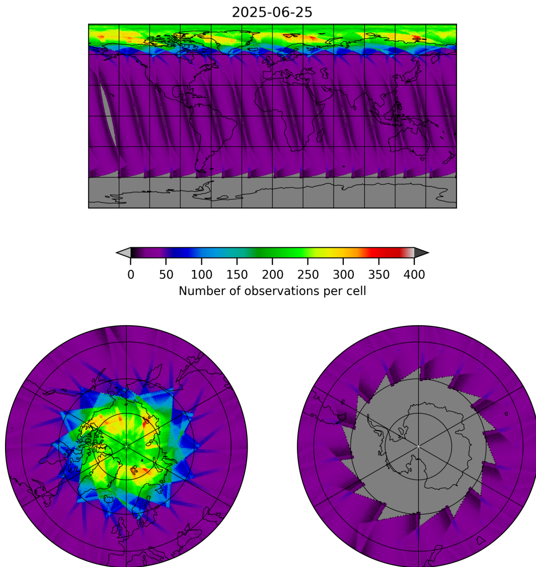
Figure 17: Map of the number of observations for 2025-06-25 to 2025-06-25
