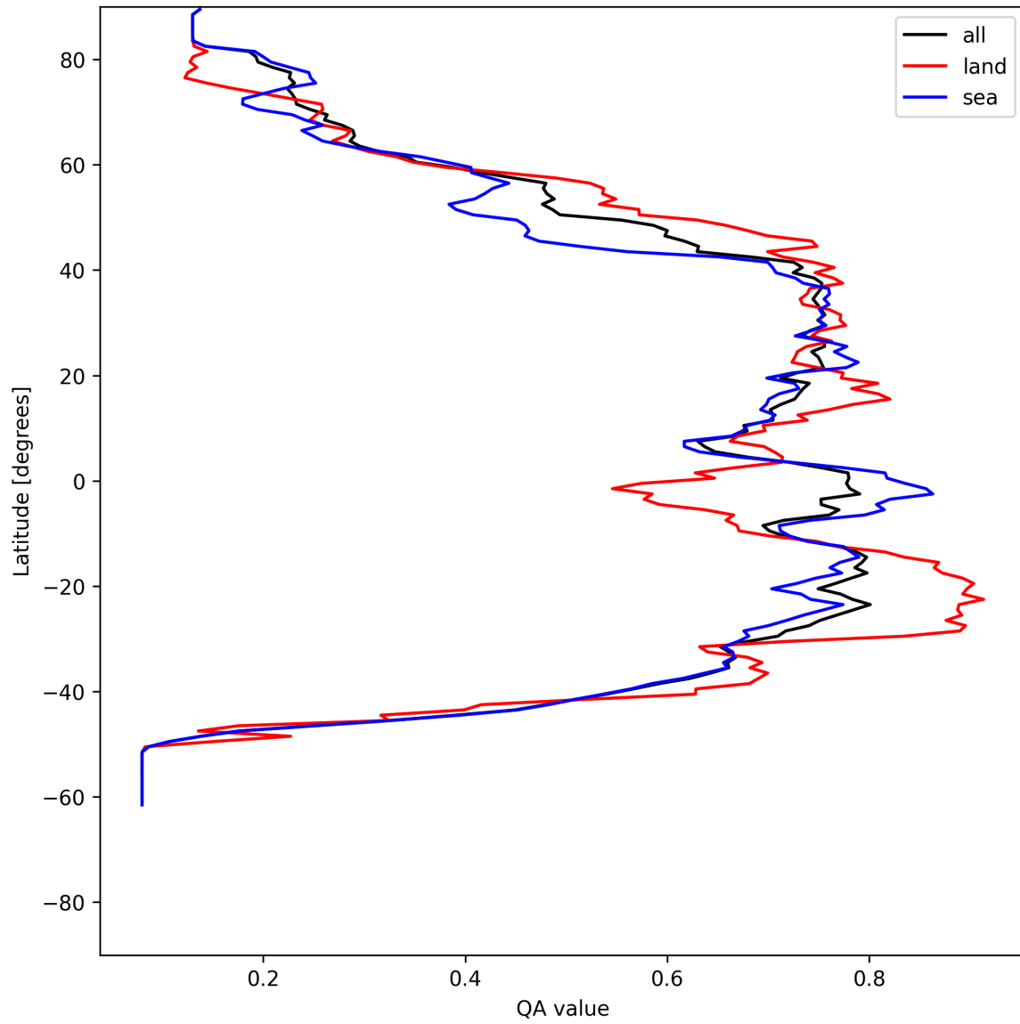
Figure 18: Zonal average of “QA value” for 2025-06-25 to 2025-06-25.
