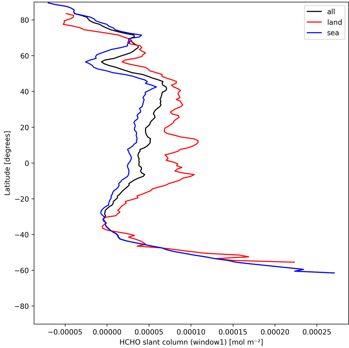
Figure 22: Zonal average of “HCHO slant column (window1)” for 2025-06-25 to 2025-06-25.
