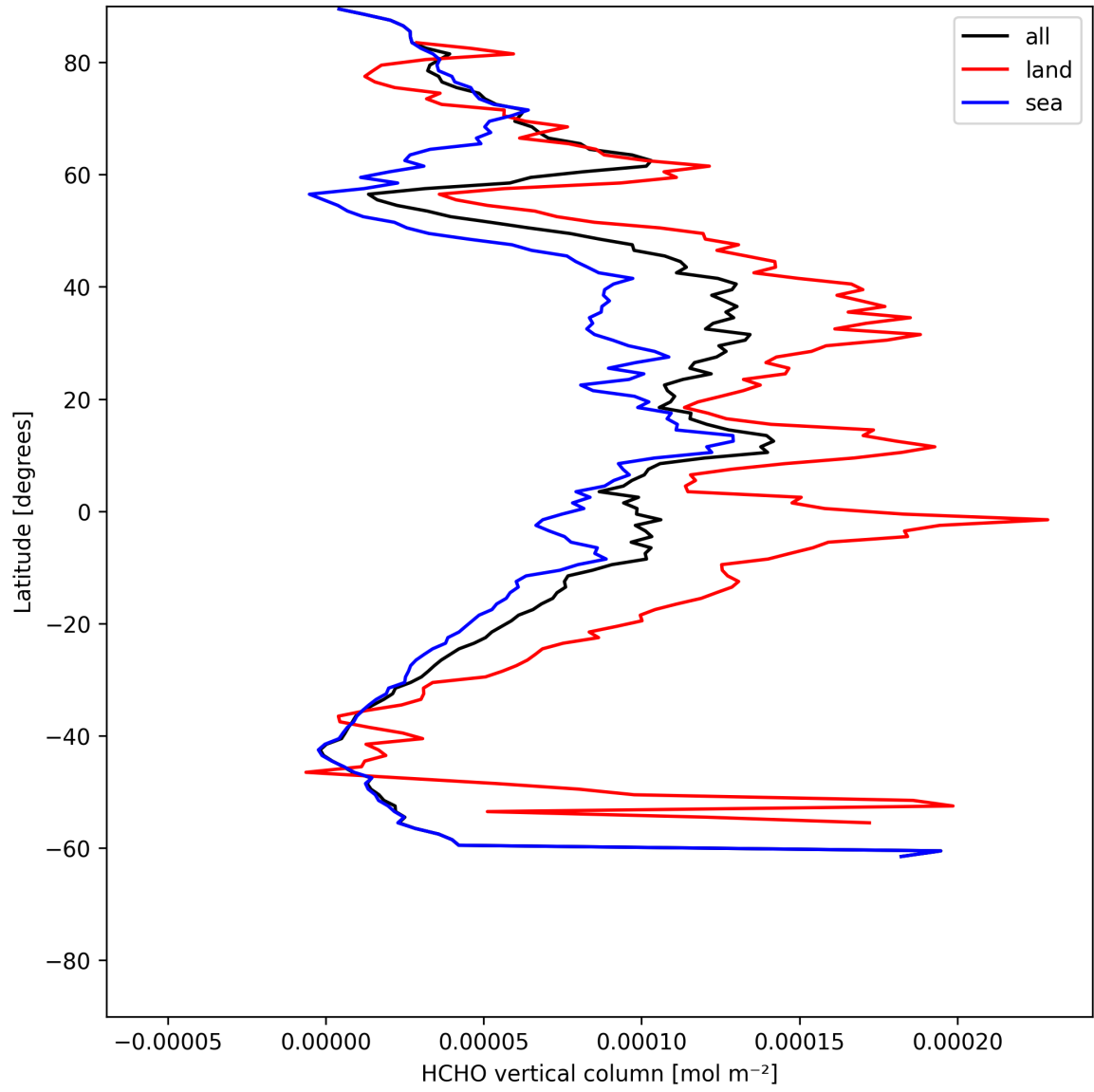
Figure 19: Zonal average of “HCHO vertical column” for 2025-06-25 to 2025-06-25.
