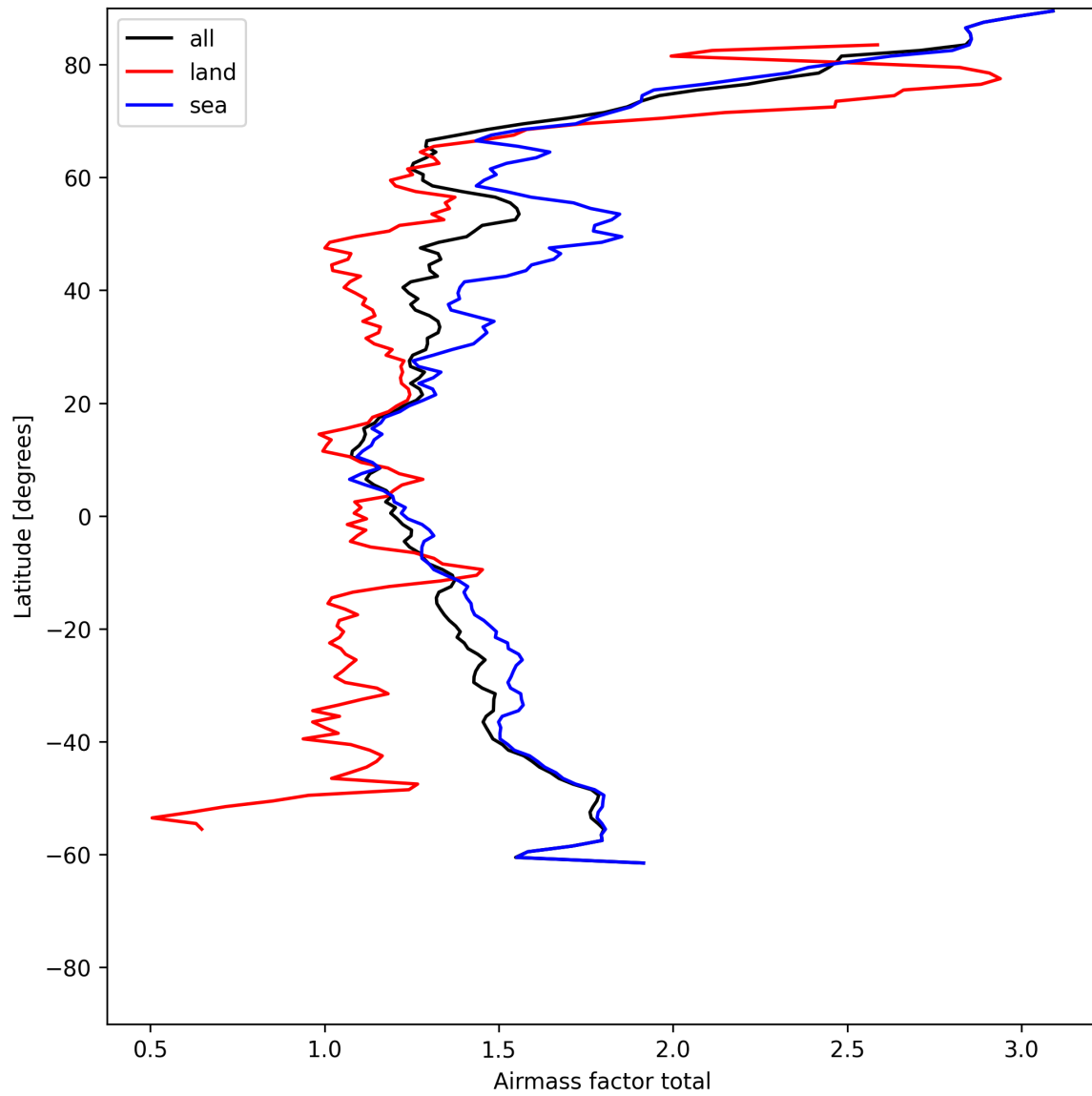
Figure 24: Zonal average of “Airmass factor total” for 2025-06-25 to 2025-06-25.
