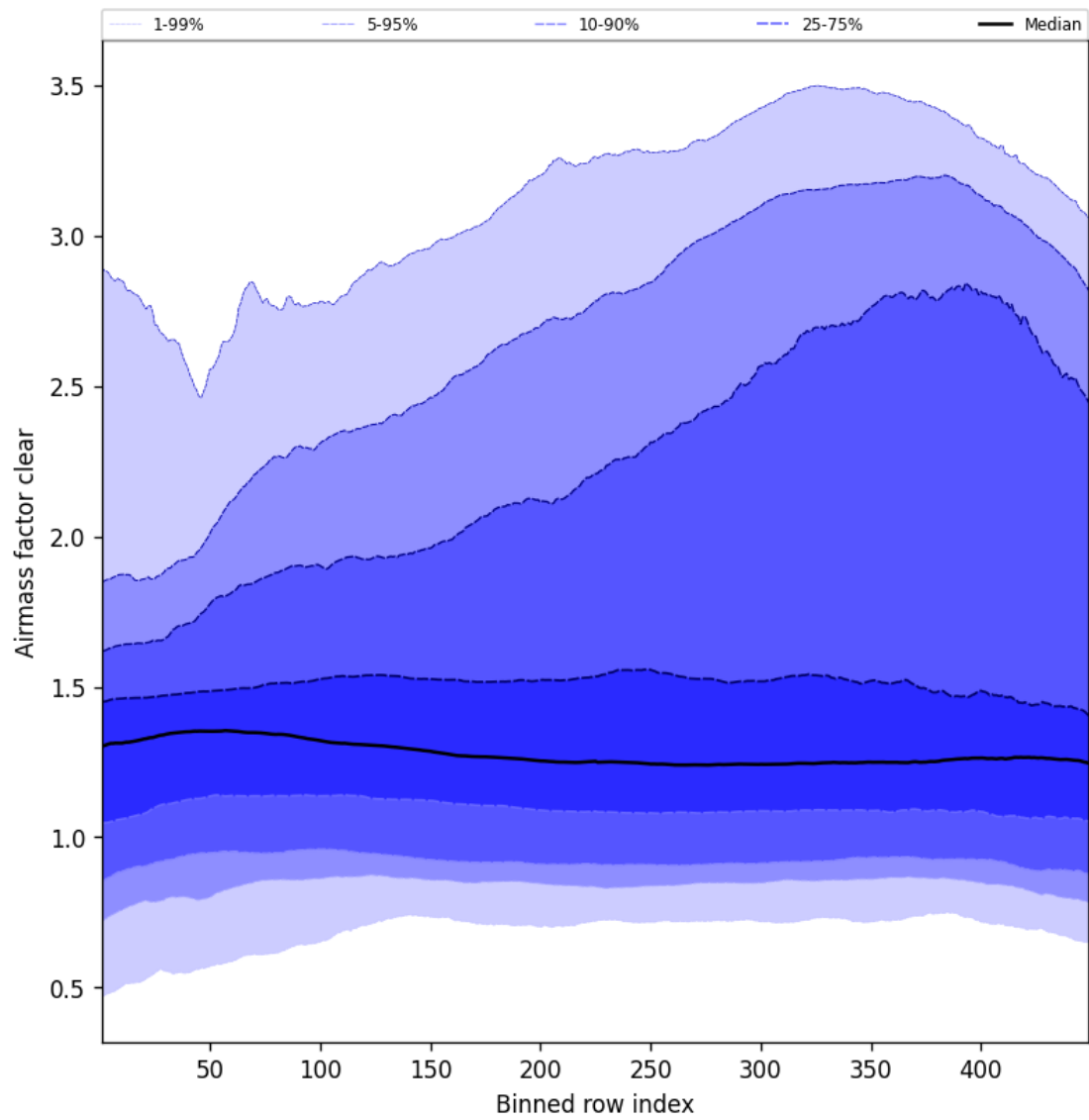
Figure 54: Along track statistics of “Air mass factor clear” for 2025-06-25 to 2025-06-25
