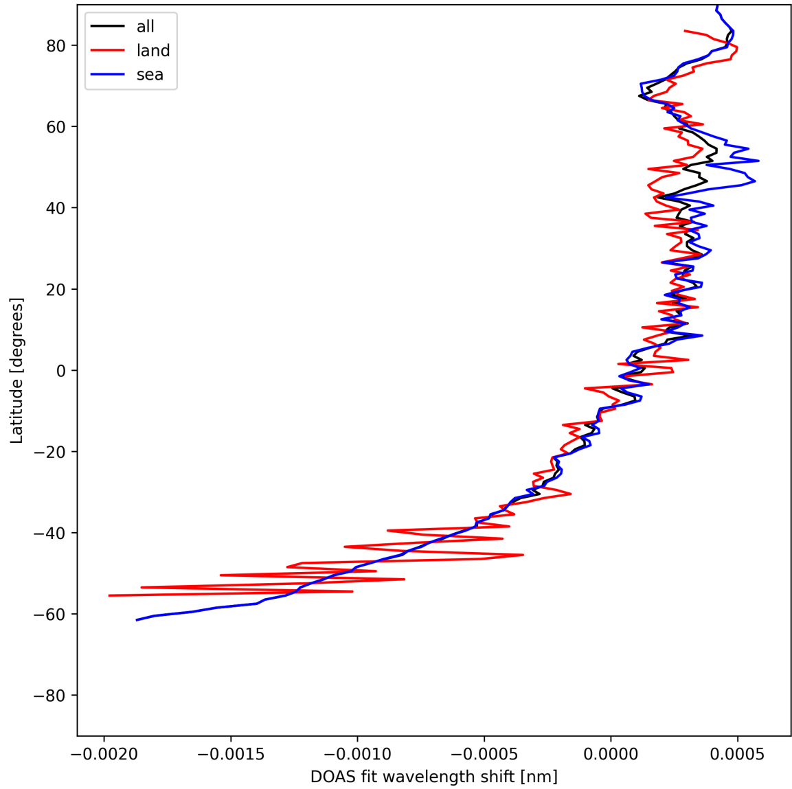
Figure 28: Zonal average of “DOAS fit wavelength shift” for 2025-06-25 to 2025-06-25.
