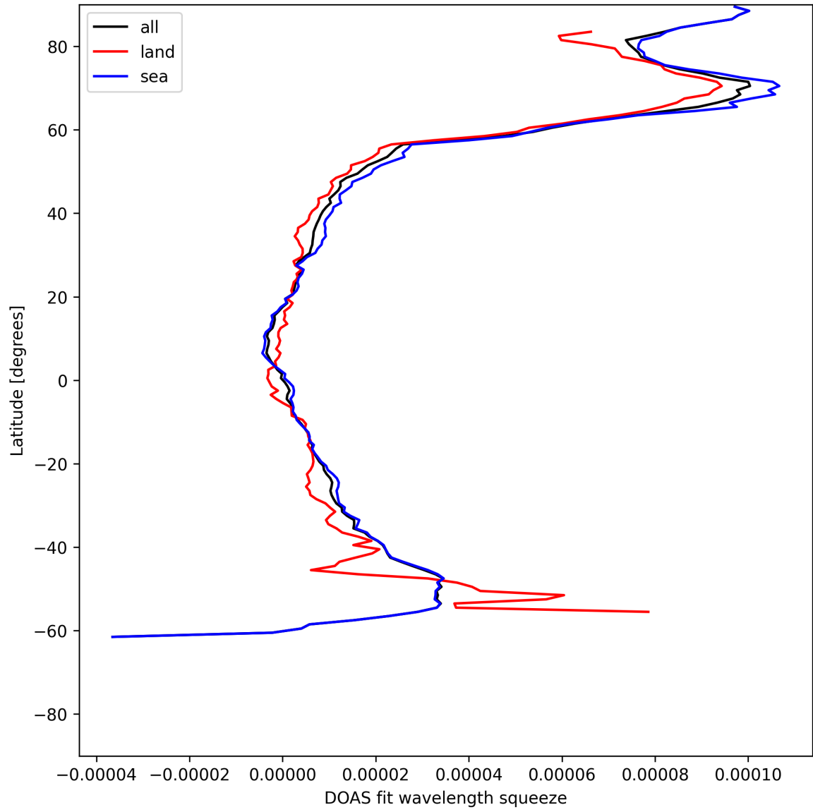
Figure 29: Zonal average of “DOAS fit wavelength squeeze” for 2025-06-25 to 2025-06-25.
