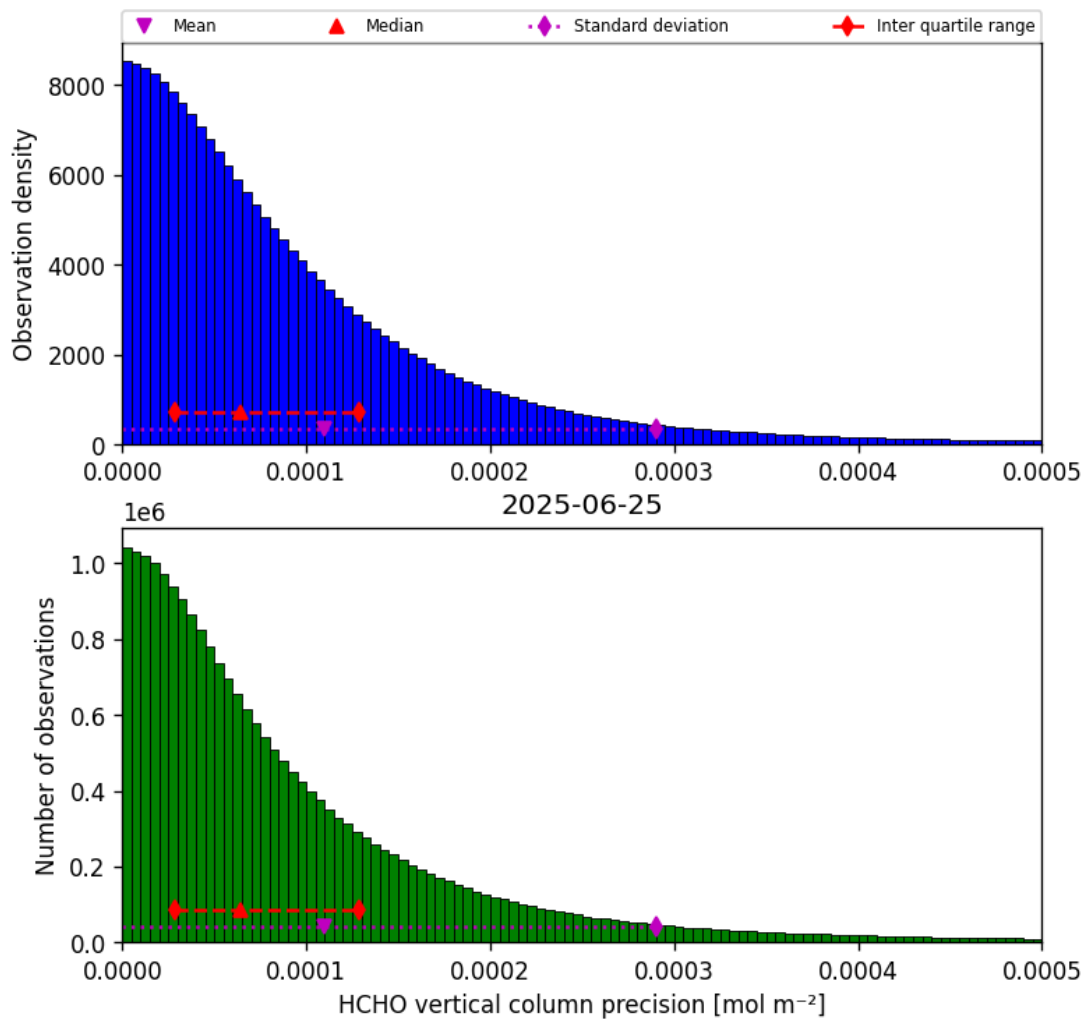
Figure 34: Histogram of “HCHO vertical column precision” for 2025-06-25 to 2025-06-25
