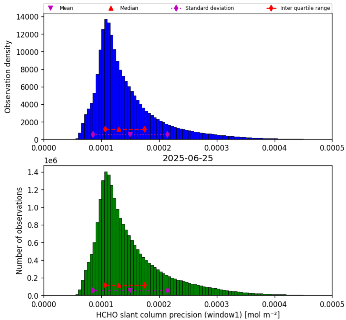
Figure 37: Histogram of “HCHO slant column precision (window1)” for 2025-06-25 to 2025-06-25
