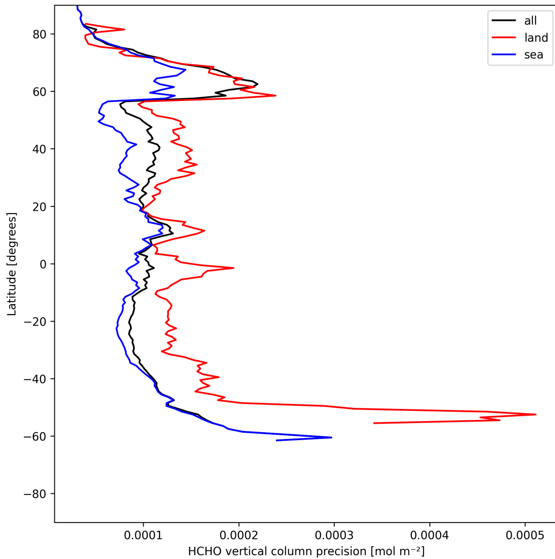
Figure 20: Zonal average of “HCHO vertical column precision” for 2025-06-25 to 2025-06-25.
