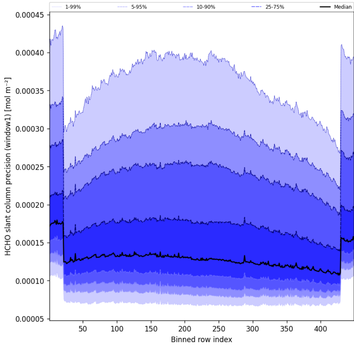
Figure 51: Along track statistics of “HCHO slant column precision (window1)” for 2025-06-25 to 2025-06-25
