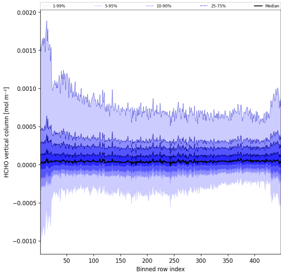
Figure 47: Along track statistics of “HCHO vertical column” for 2025-06-26 to 2025-06-27
