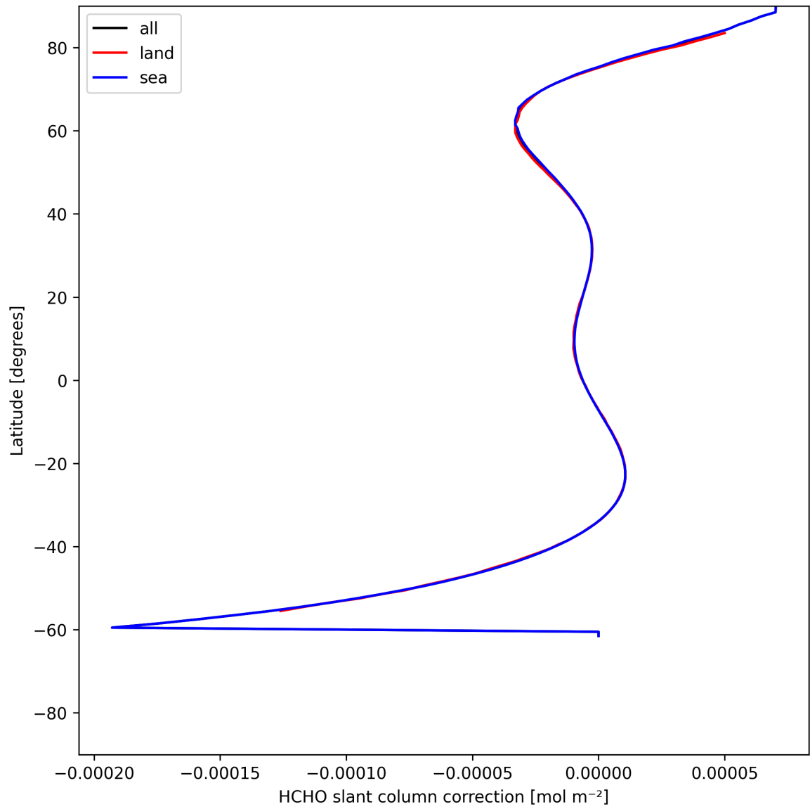
Figure 31: Zonal average of “HCHO slant column correction” for 2025-06-26 to 2025-06-27.
