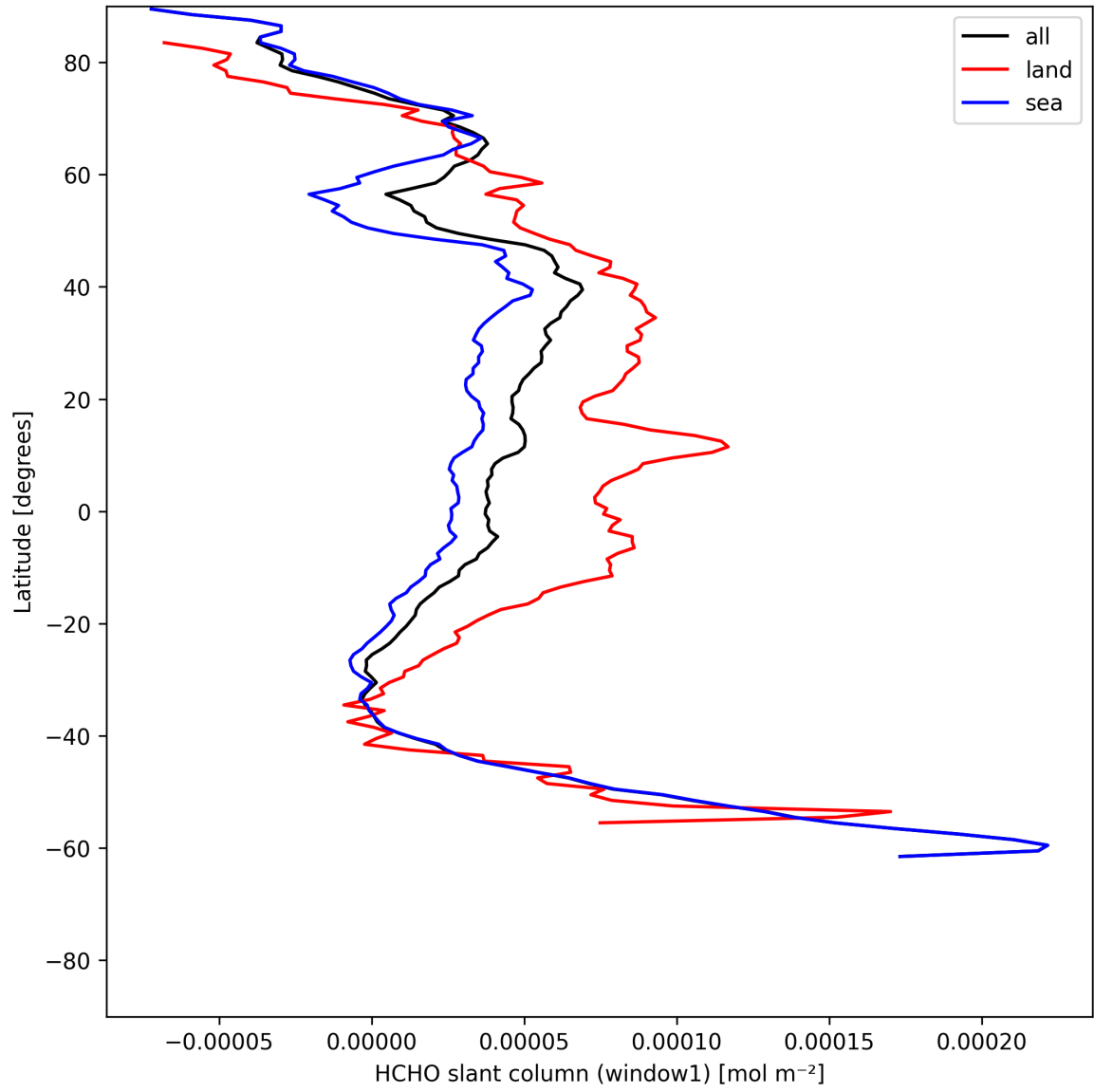
Figure 22: Zonal average of “HCHO slant column (window1)” for 2025-06-26 to 2025-06-27.
