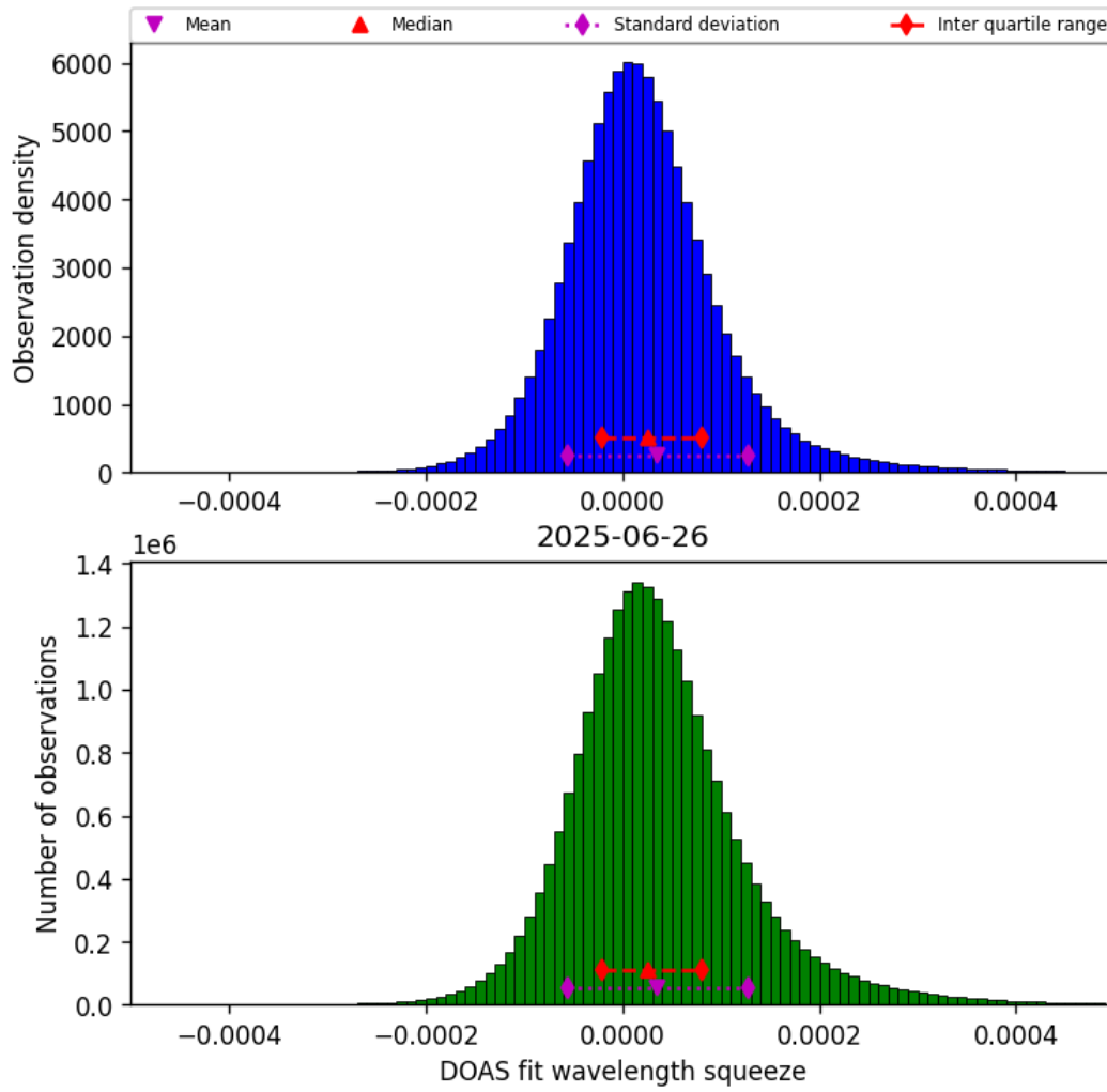
Figure 43: Histogram of “DOAS fit wavelength squeeze” for 2025-06-26 to 2025-06-27
