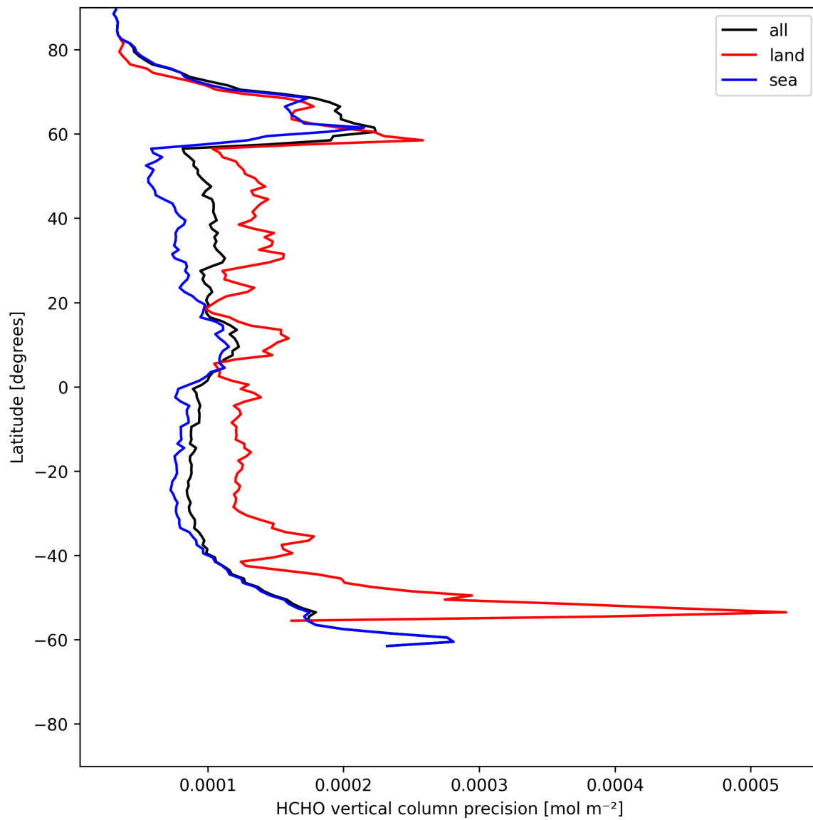
Figure 20: Zonal average of “HCHO vertical column precision” for 2025-06-26 to 2025-06-27.
