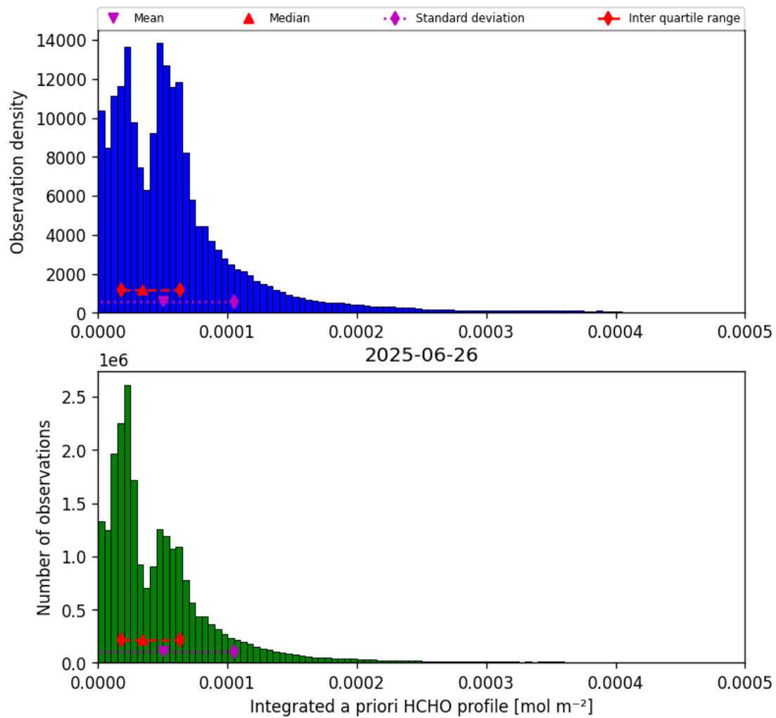
Figure 41: Histogram of “Integrated a priori HCHO profile” for 2025-06-26 to 2025-06-27
