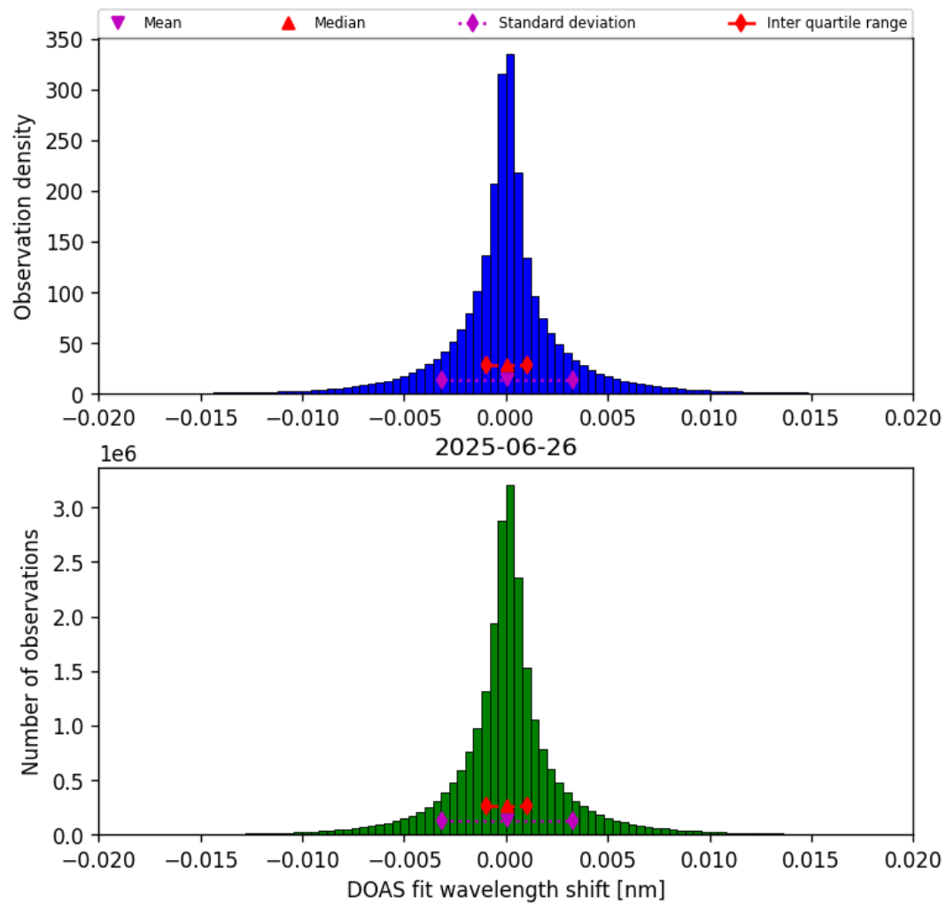
Figure 42: Histogram of “DOAS fit wavelength shift” for 2025-06-26 to 2025-06-27
