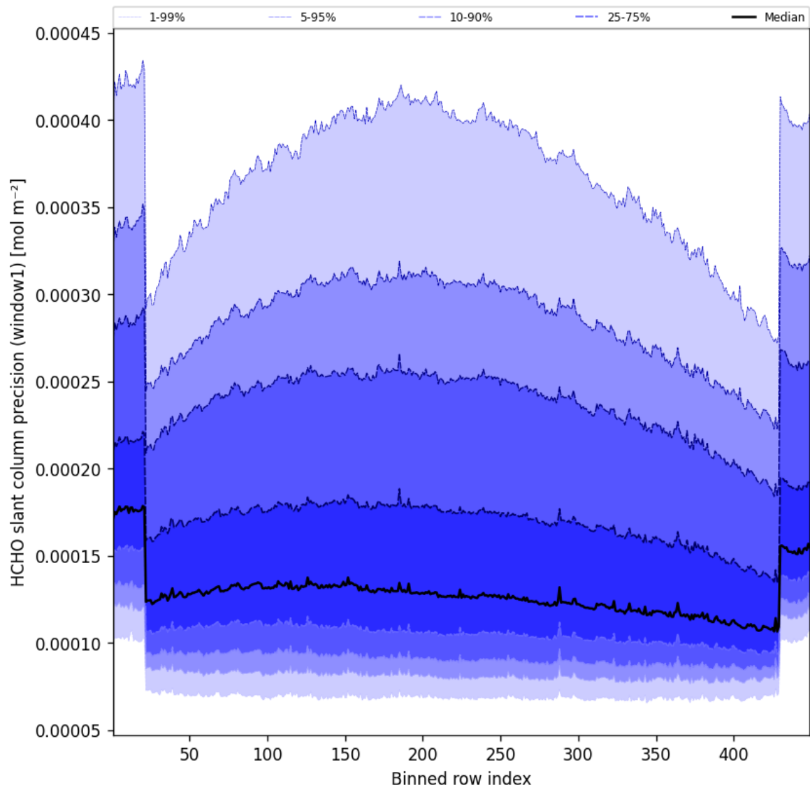
Figure 51: Along track statistics of “HCHO slant column precision (window1)” for 2025-06-26 to 2025-06-27
