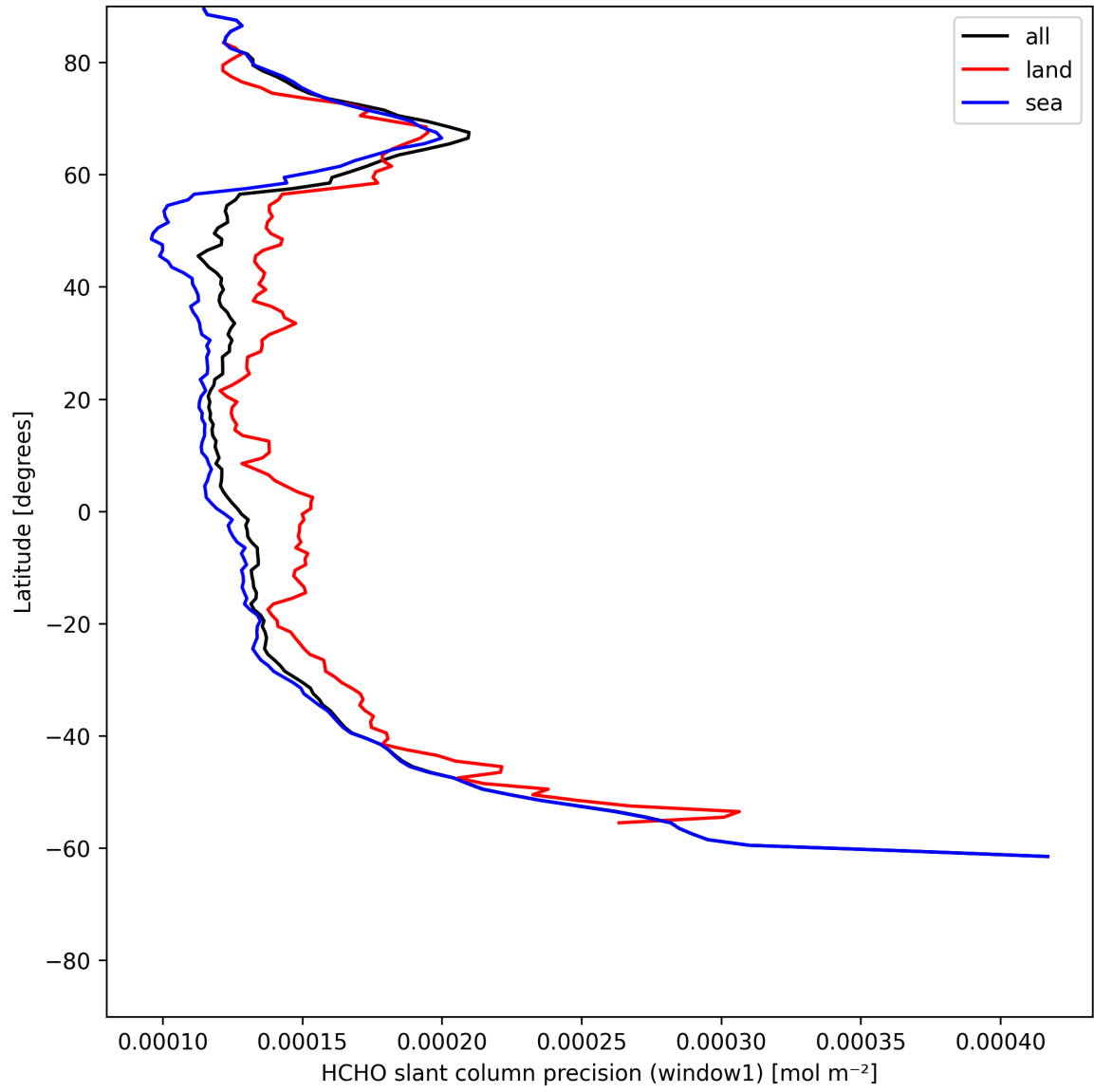
Figure 23: Zonal average of “HCHO slant column precision (window1)” for 2025-06-26 to 2025-06-27.
