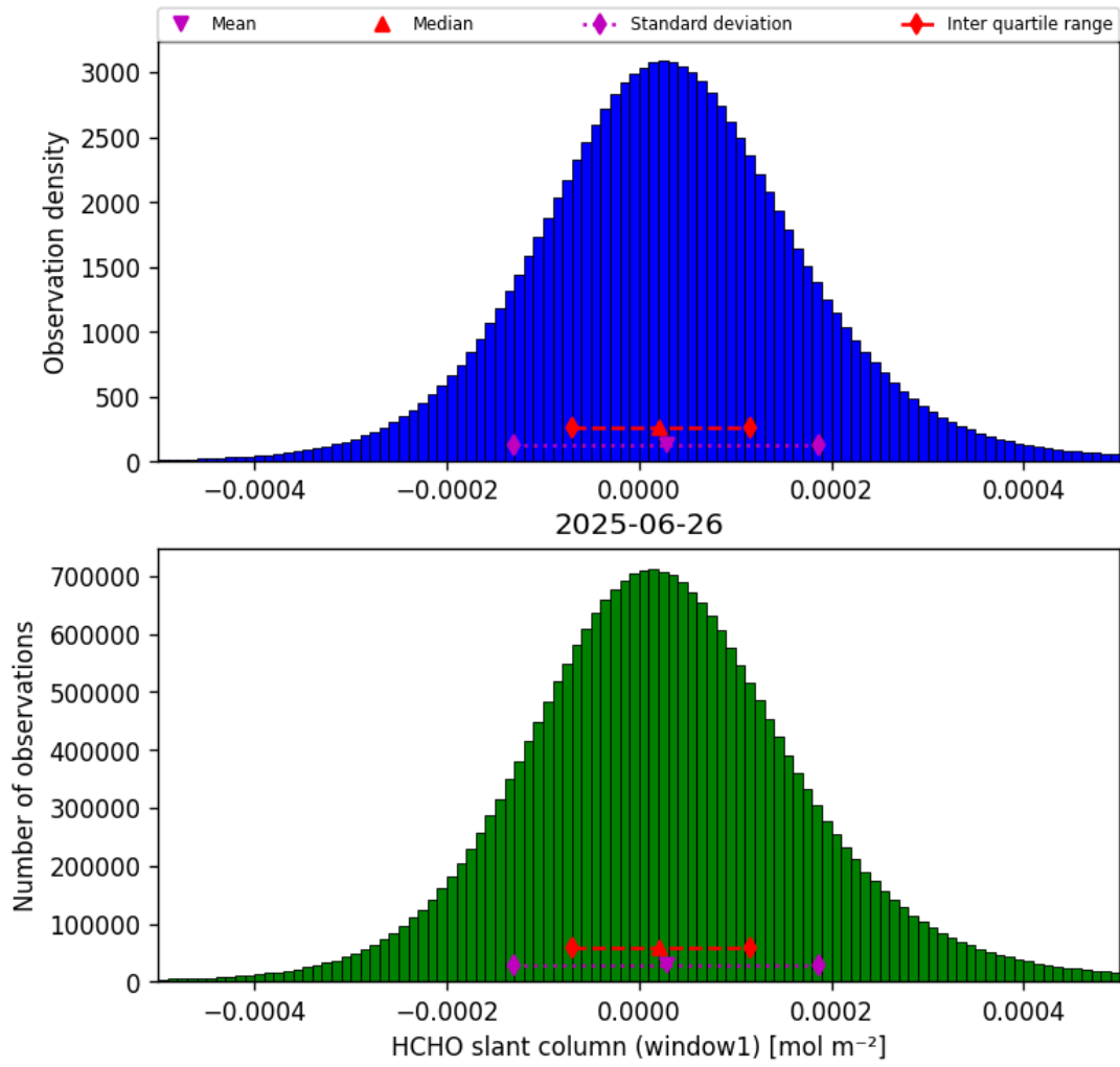
Figure 36: Histogram of “HCHO slant column (window1)” for 2025-06-26 to 2025-06-27
