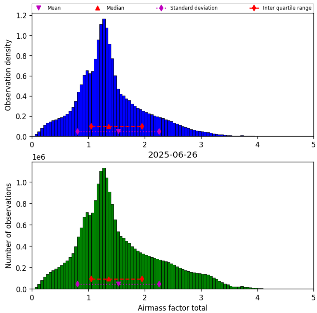
Figure 38: Histogram of “Airmass factor total” for 2025-06-26 to 2025-06-27
