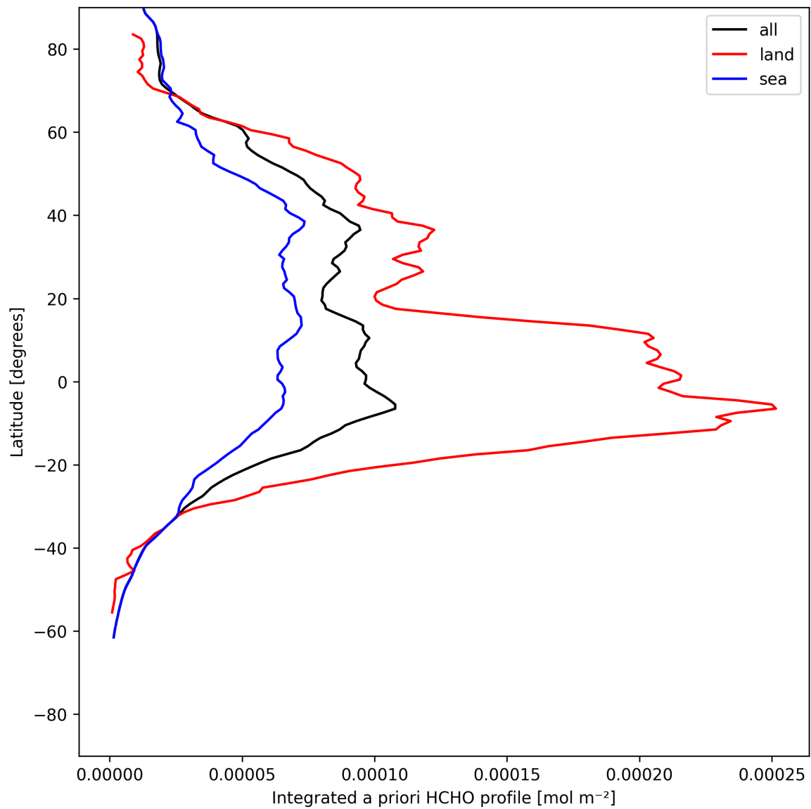
Figure 27: Zonal average of “Integrated a priori HCHO profile” for 2025-06-26 to 2025-06-27.
