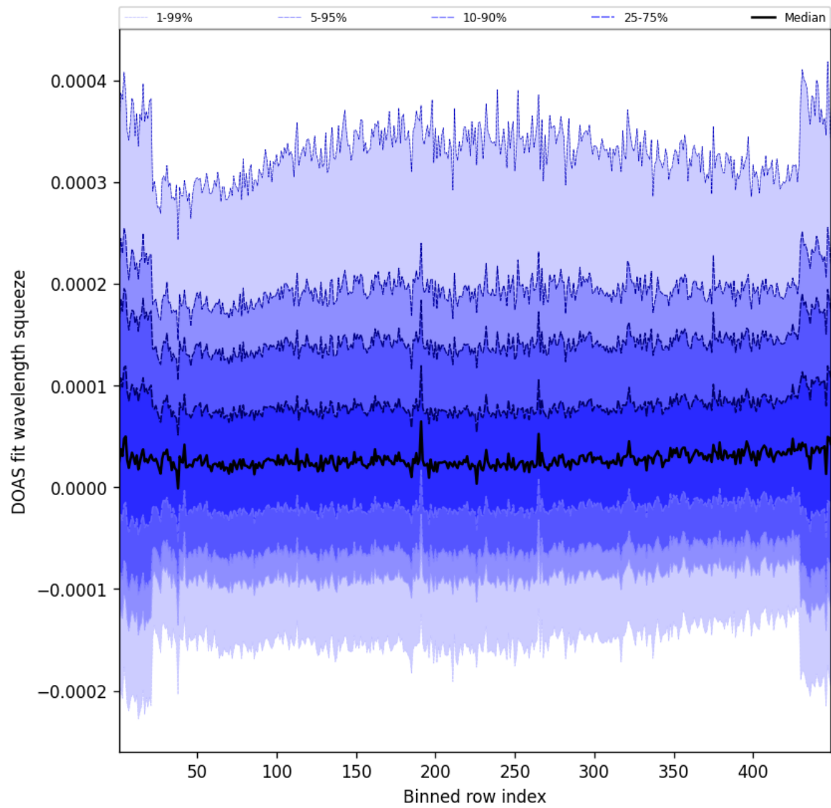
Figure 57: Along track statistics of “DOAS fit wavelength squeeze” for 2025-06-26 to 2025-06-27
