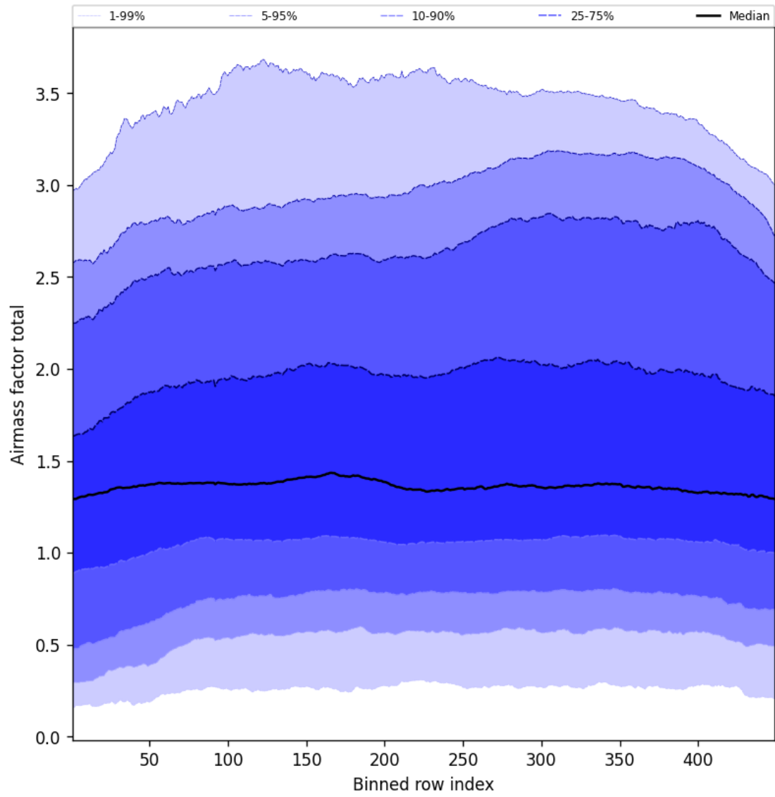
Figure 52: Along track statistics of “Airmass factor total” for 2025-06-26 to 2025-06-27
