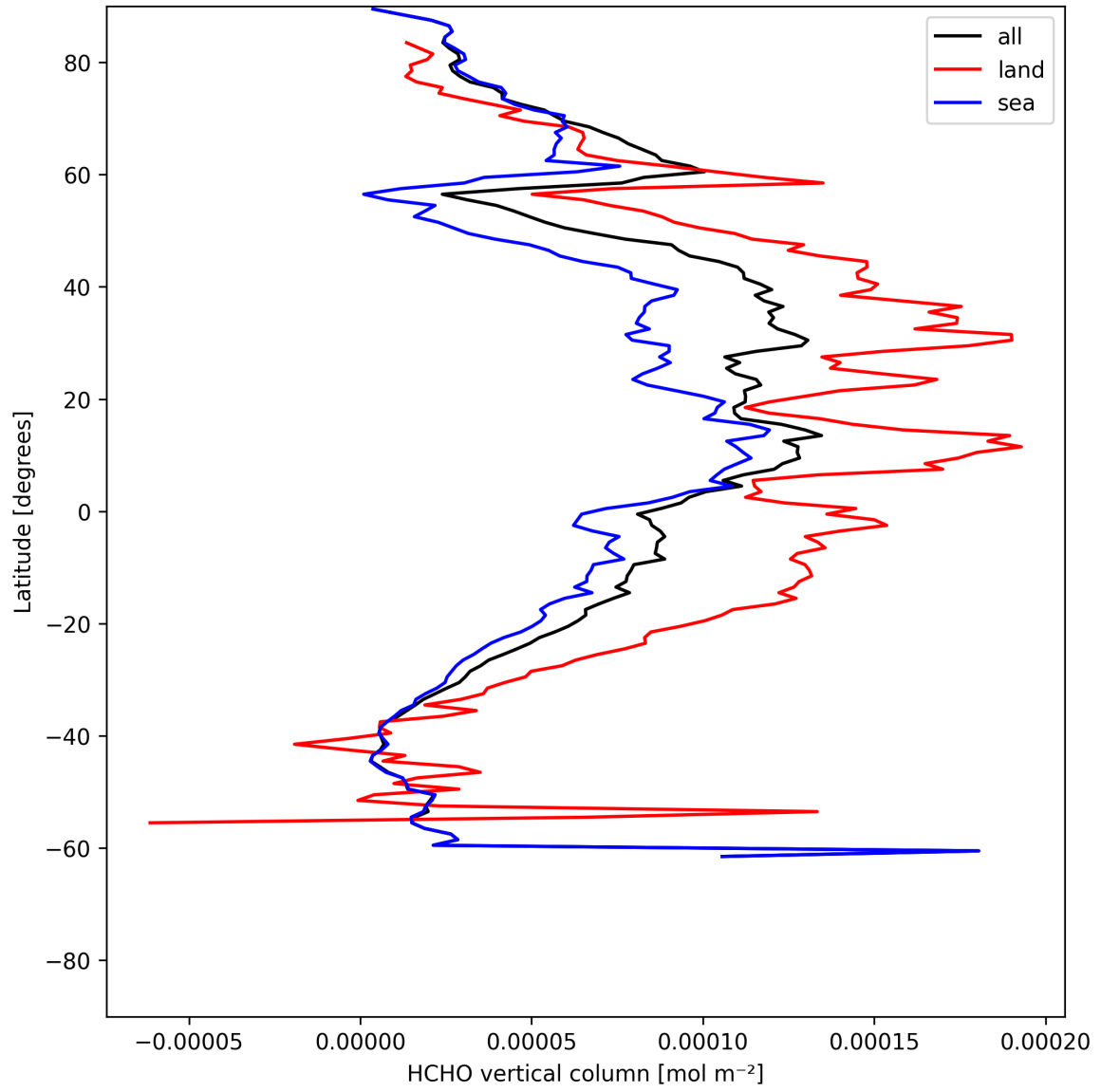
Figure 19: Zonal average of “HCHO vertical column” for 2025-06-26 to 2025-06-27.
