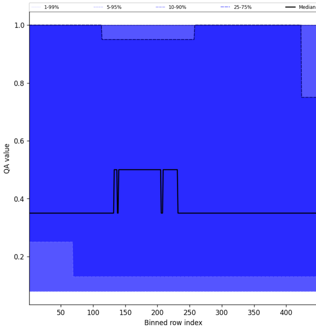
Figure 46: Along track statistics of “QA value” for 2025-06-26 to 2025-06-27
