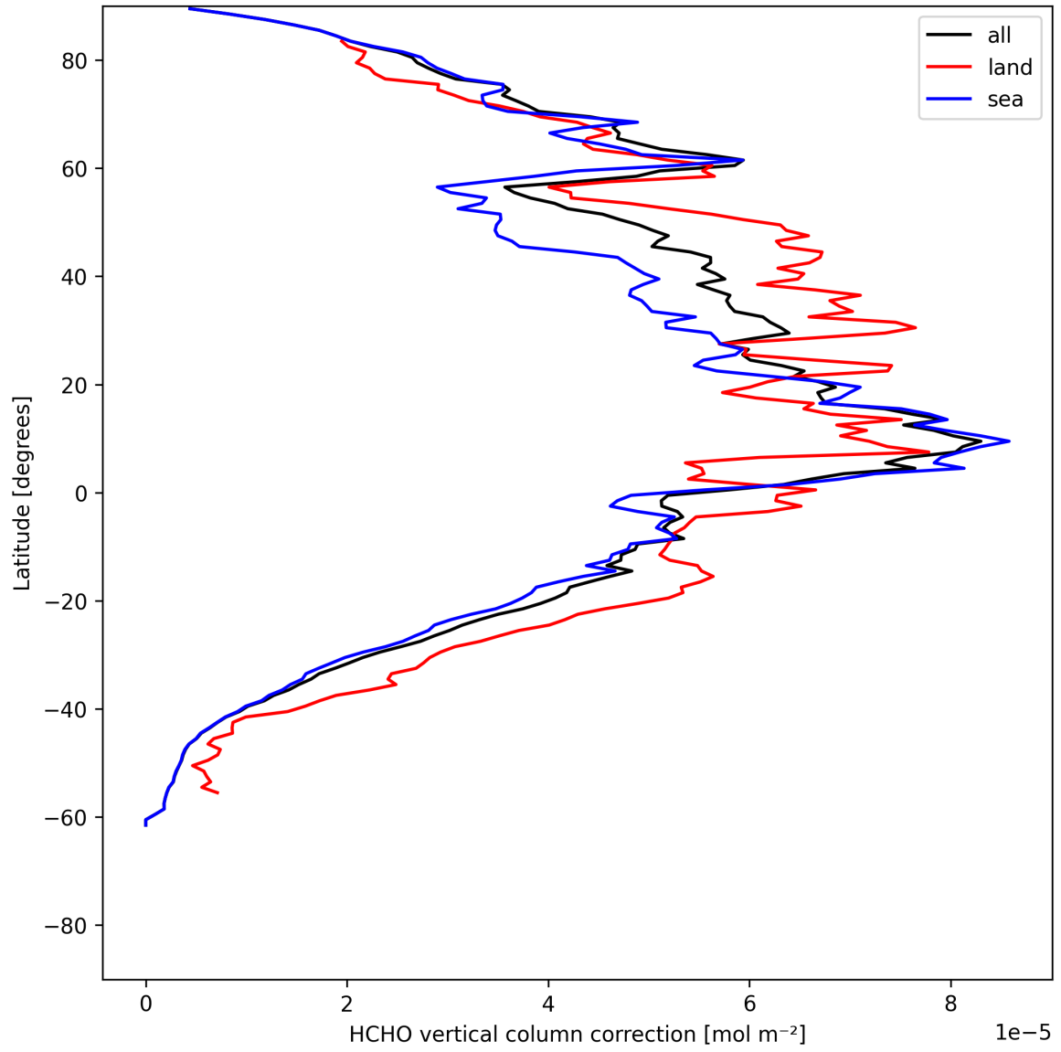
Figure 21: Zonal average of “HCHO vertical column correction” for 2025-06-26 to 2025-06-27.
