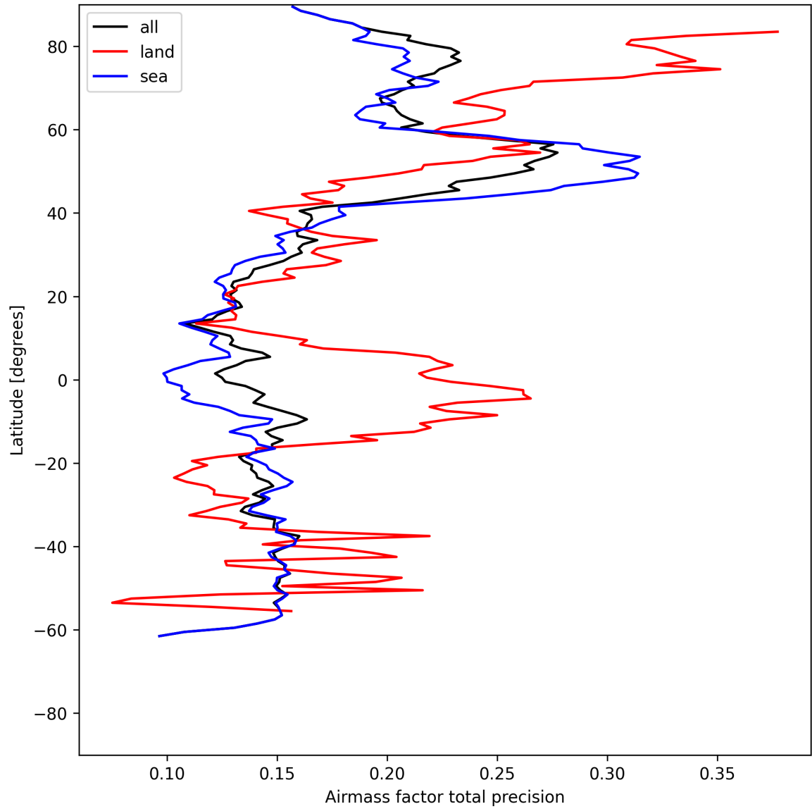
Figure 25: Zonal average of “Airmass factor total precision” for 2025-06-26 to 2025-06-27.
