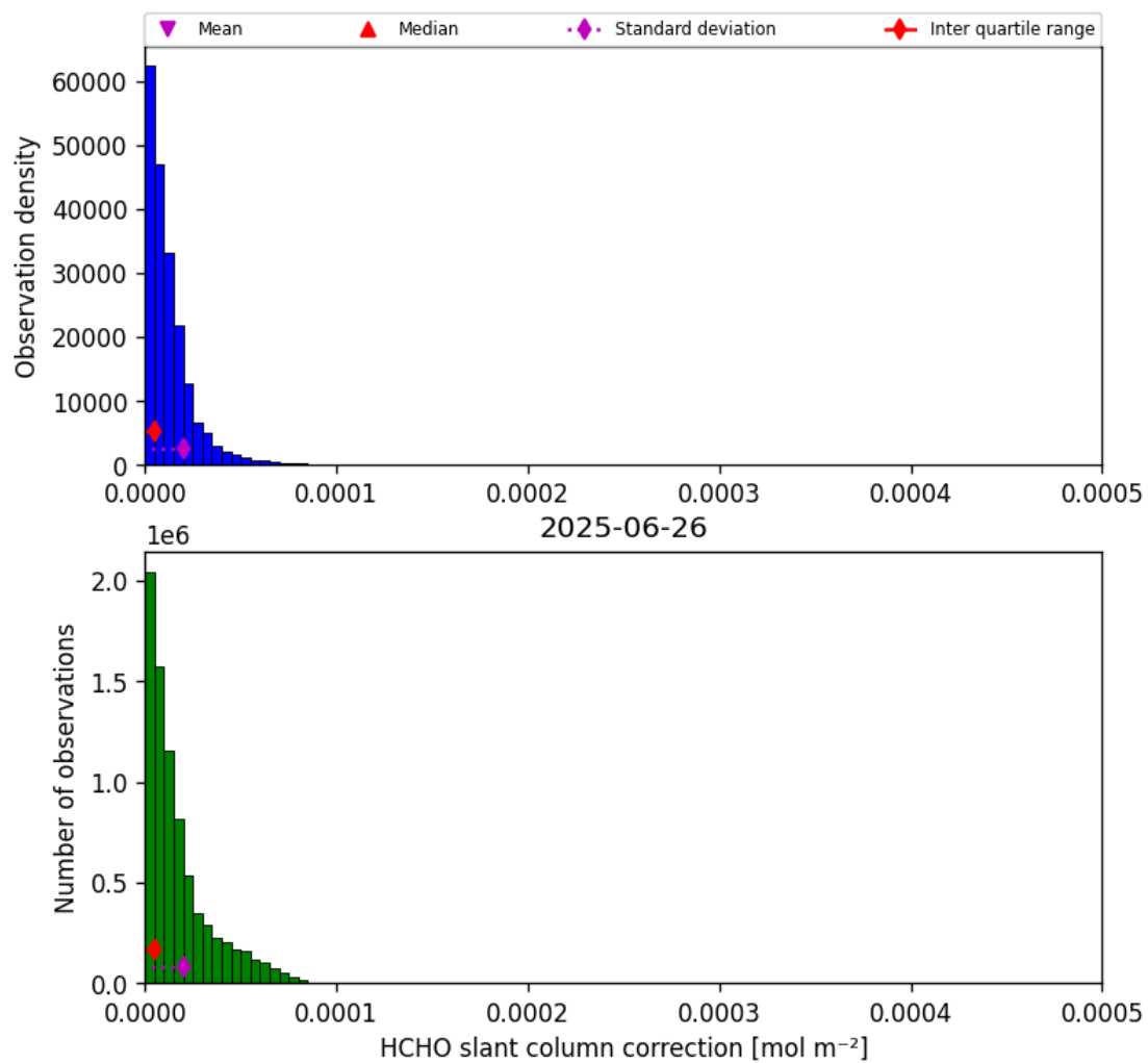
Figure 45: Histogram of “HCHO slant column correction” for 2025-06-26 to 2025-06-27
