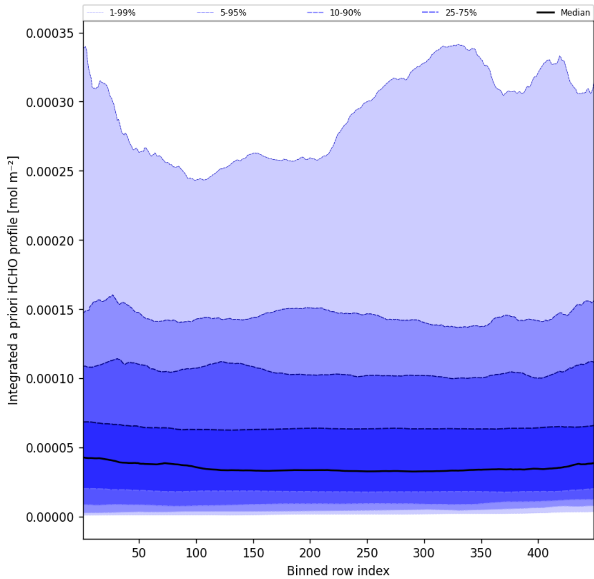
Figure 55: Along track statistics of “Integrated a priori HCHO profile” for 2025-06-26 to 2025-06-27
