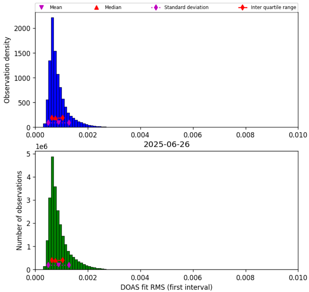
Figure 44: Histogram of “DOAS fit RMS (first interval)” for 2025-06-26 to 2025-06-27
