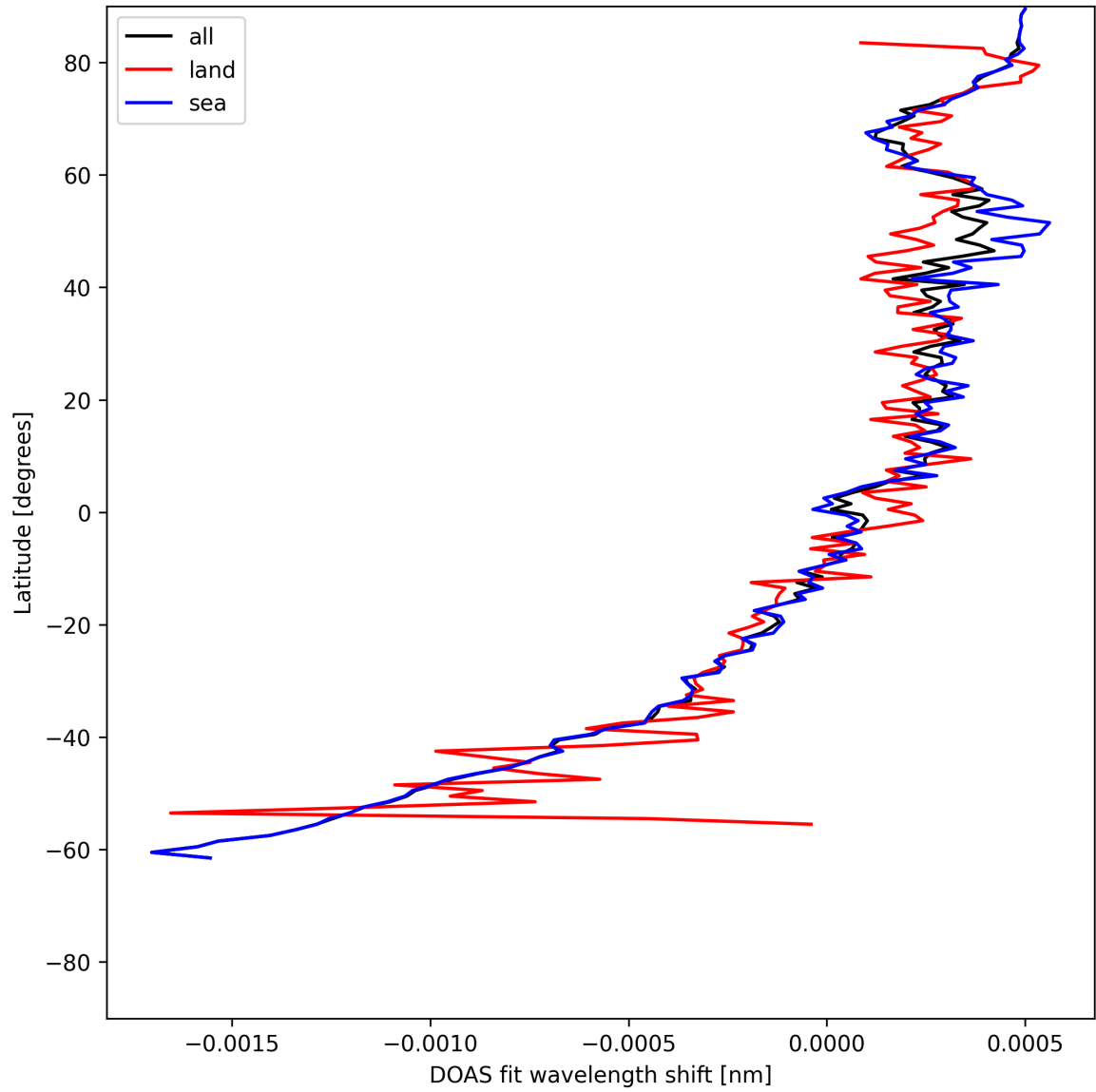
Figure 28: Zonal average of “DOAS fit wavelength shift” for 2025-06-26 to 2025-06-27.
