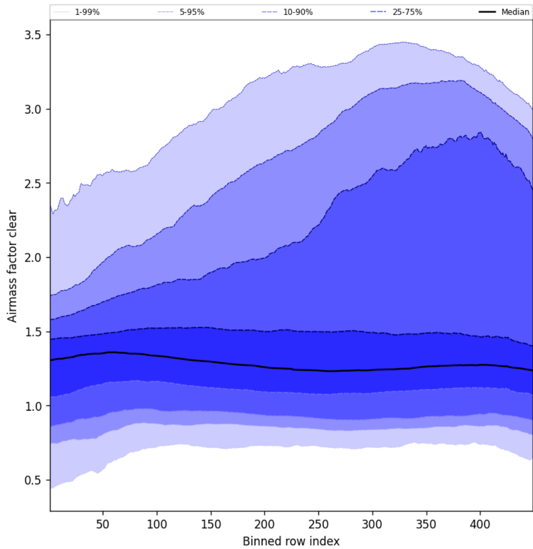
Figure 54: Along track statistics of “Airmass factor clear” for 2025-06-26 to 2025-06-27
