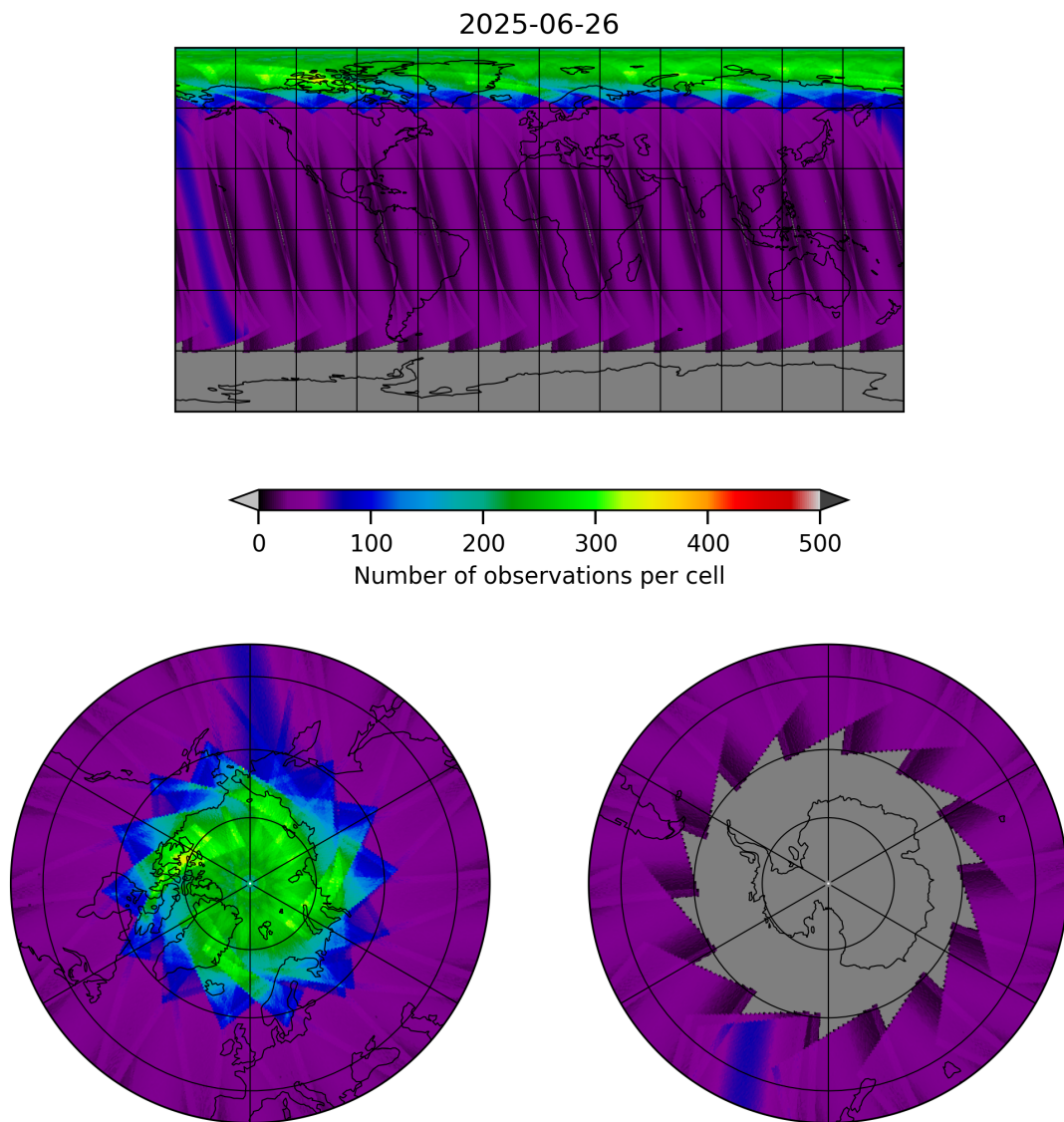
Figure 17: Map of the number of observations for 2025-06-26 to 2025-06-27
