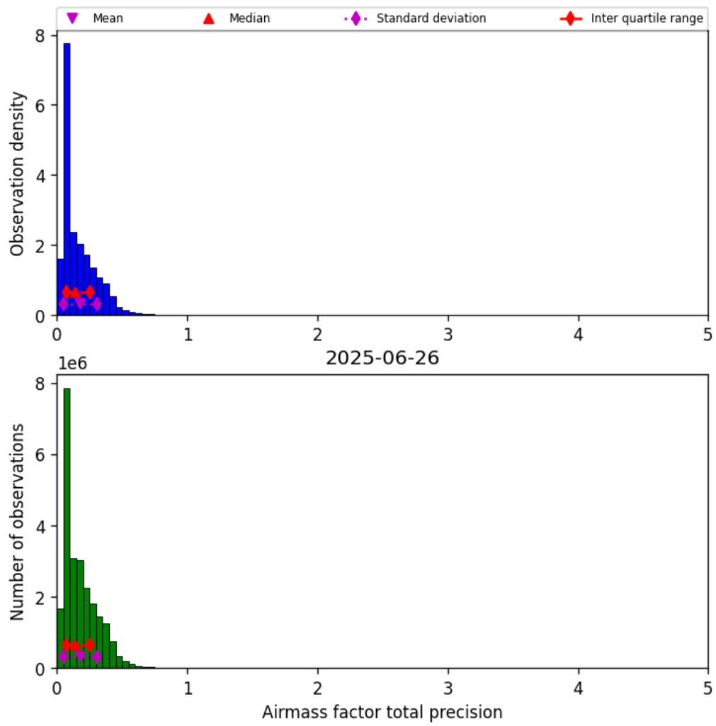
Figure 39: Histogram of “Airmass factor total precision” for 2025-06-26 to 2025-06-27
