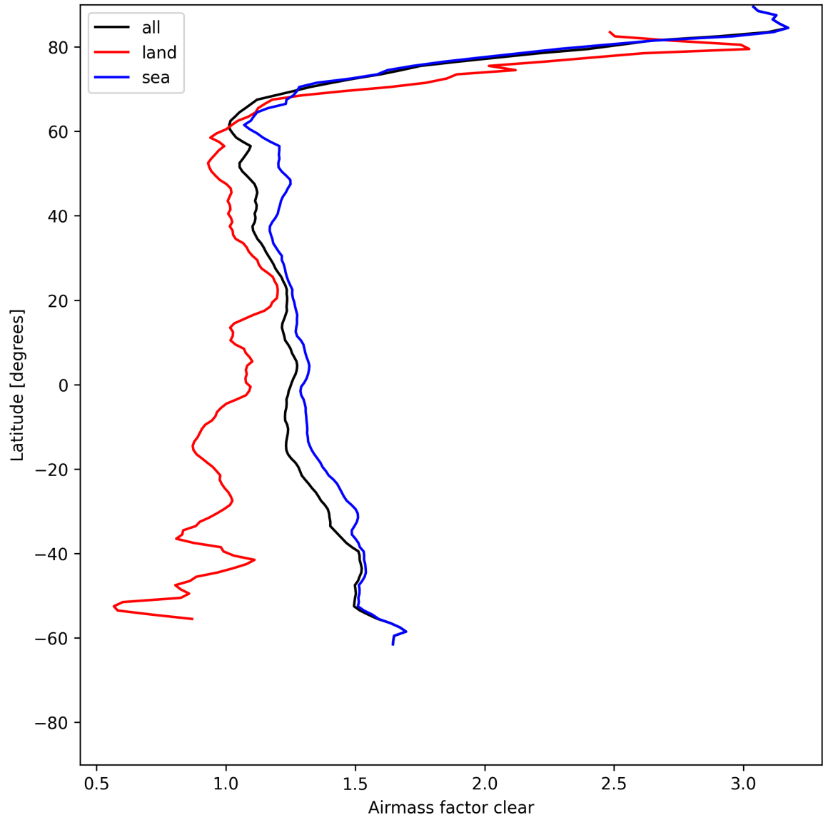
Figure 26: Zonal average of “Airmass factor clear” for 2025-06-26 to 2025-06-27.
