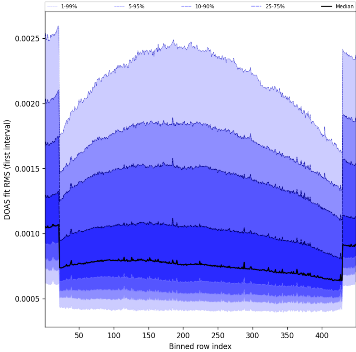
Figure 58: Along track statistics of “DOAS fit RMS (first interval)” for 2025-06-26 to 2025-06-27
