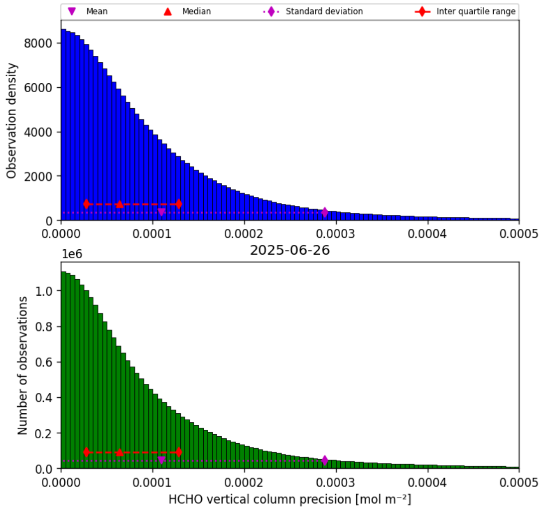
Figure 34: Histogram of “HCHO vertical column precision” for 2025-06-26 to 2025-06-27
