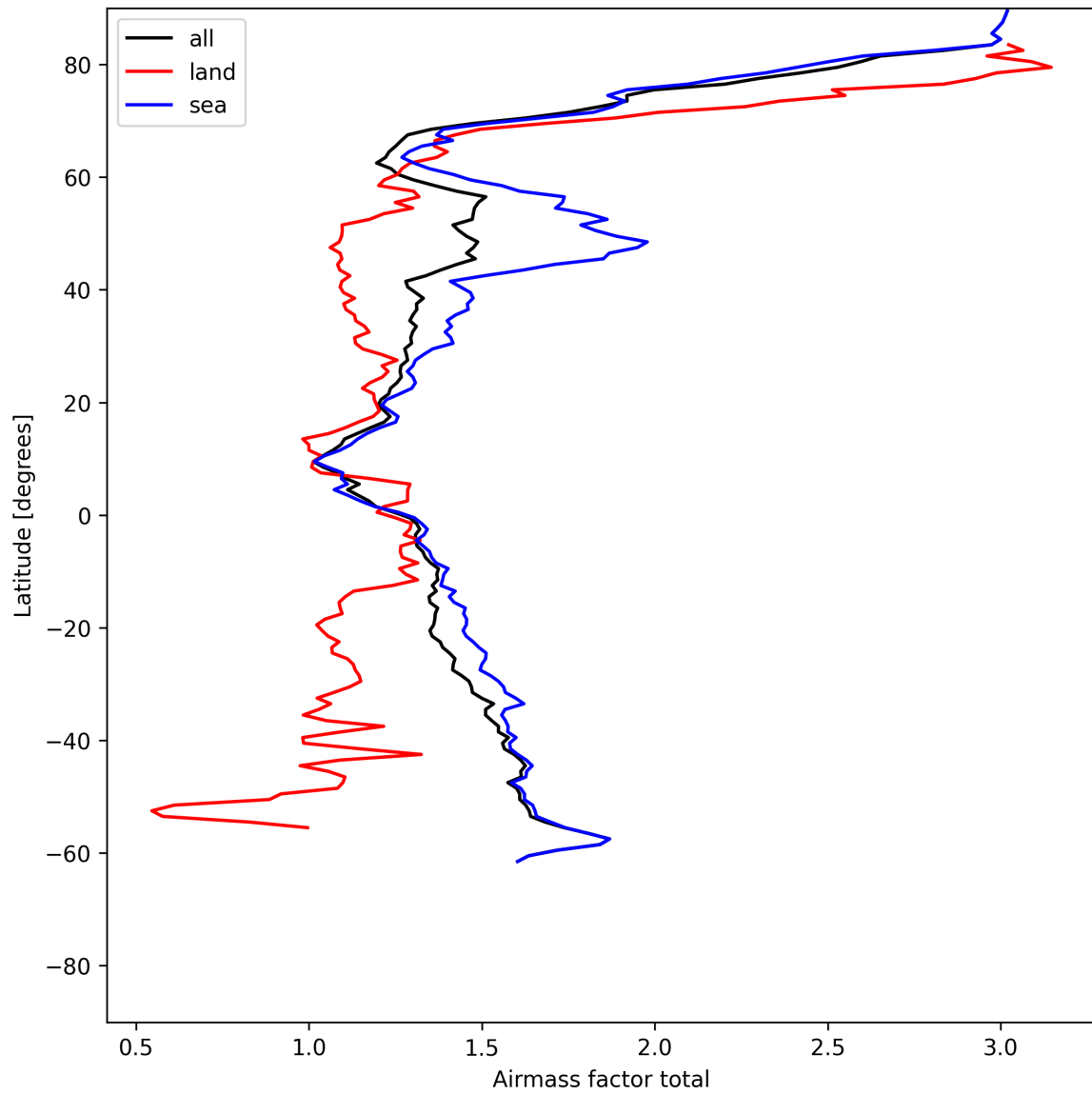
Figure 24: Zonal average of “Airmass factor total” for 2025-06-26 to 2025-06-27.
