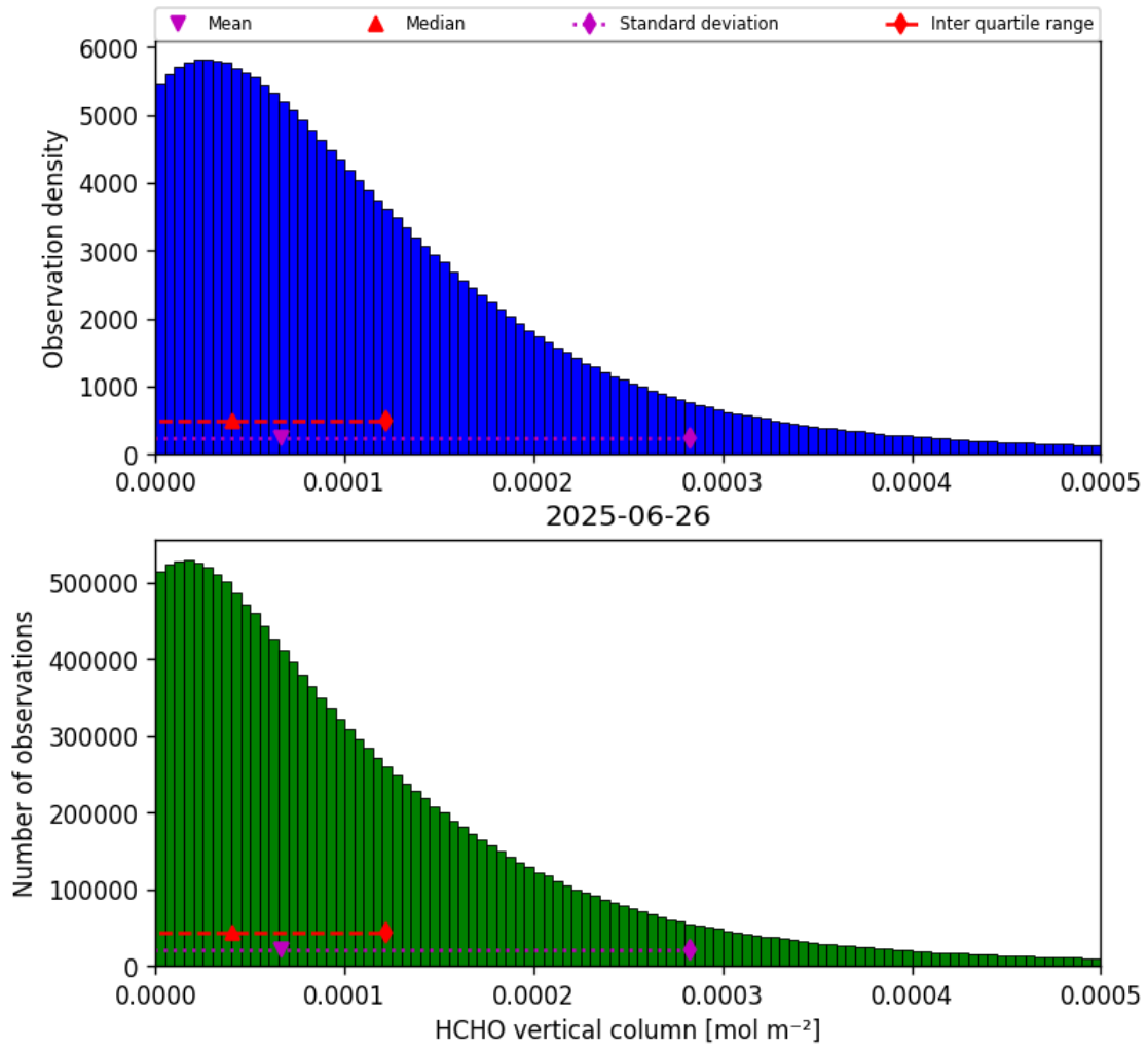
Figure 33: Histogram of “HCHO vertical column” for 2025-06-26 to 2025-06-27
