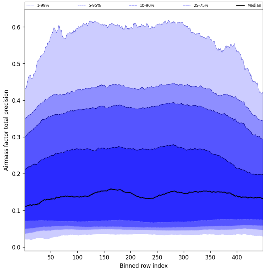
Figure 53: Along track statistics of “Airmass factor total precision” for 2025-06-26 to 2025-06-27
