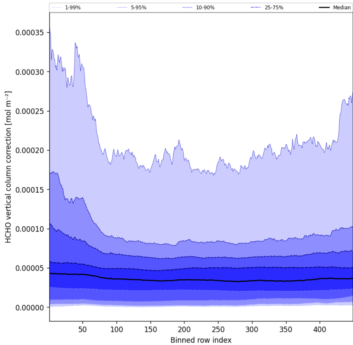
Figure 49: Along track statistics of “HCHO vertical column correction” for 2025-06-26 to 2025-06-27
