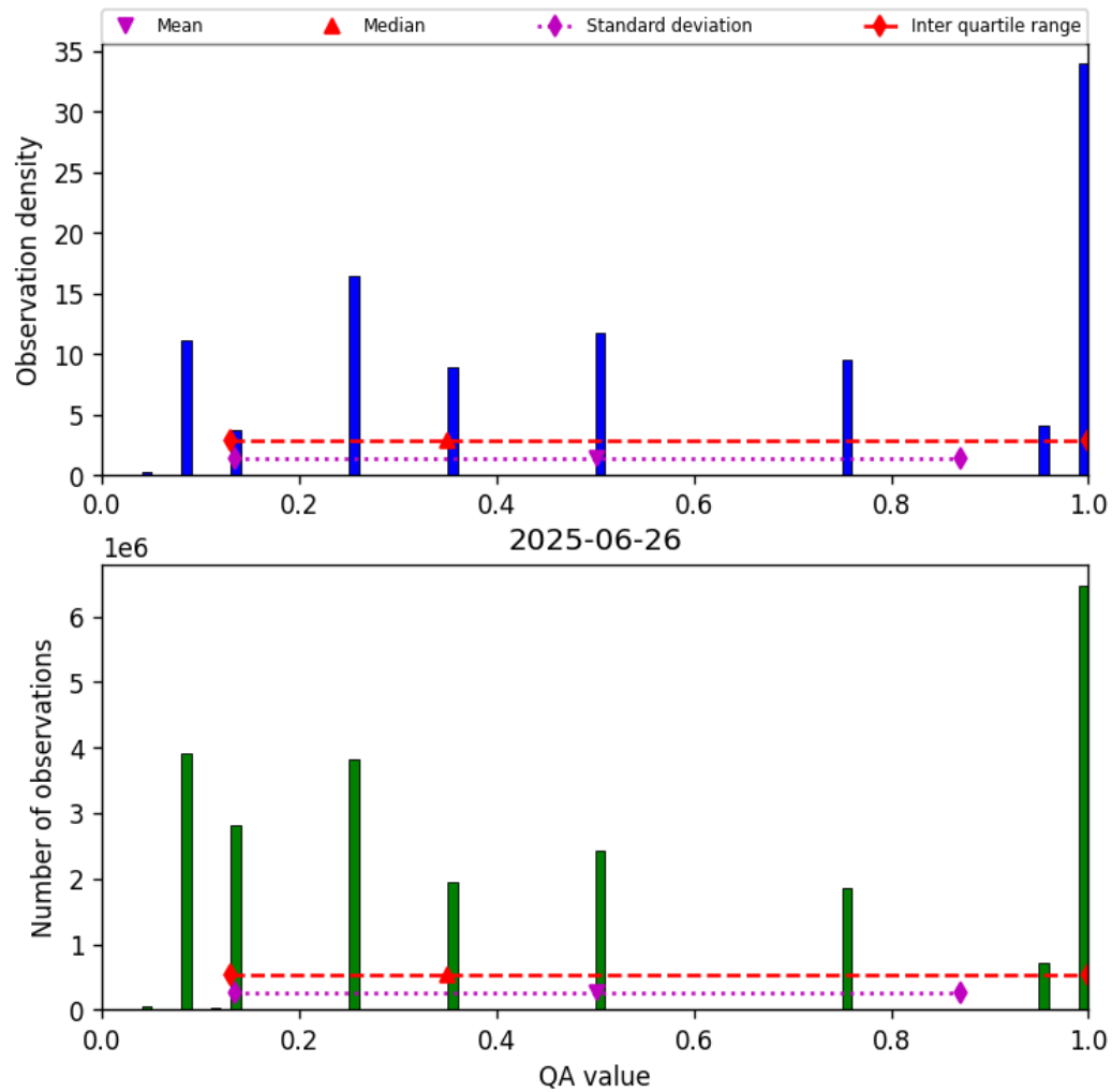
Figure 32: Histogram of “QA value” for 2025-06-26 to 2025-06-27
