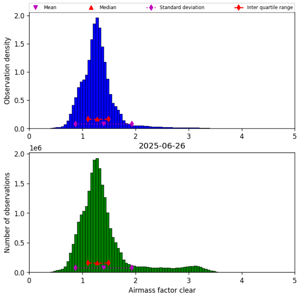
Figure 40: Histogram of “Airmass factor clear” for 2025-06-26 to 2025-06-27
