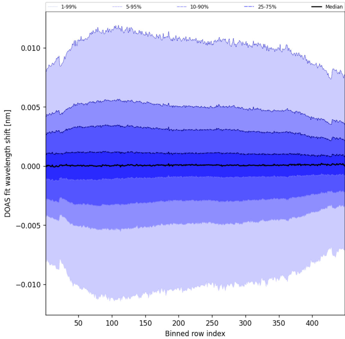
Figure 56: Along track statistics of “DOAS fit wavelength shift” for 2025-06-26 to 2025-06-27
