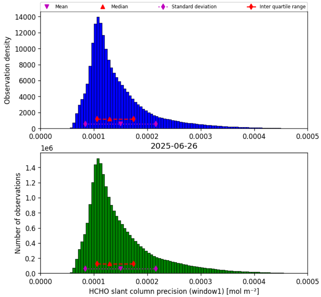
Figure 37: Histogram of “HCHO slant column precision (window1)” for 2025-06-26 to 2025-06-27
