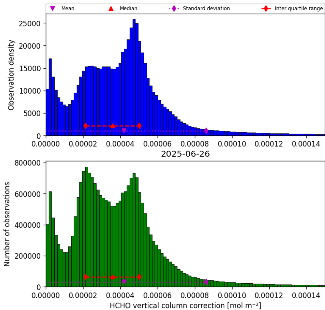
Figure 35: Histogram of “HCHO vertical column correction” for 2025-06-26 to 2025-06-27
