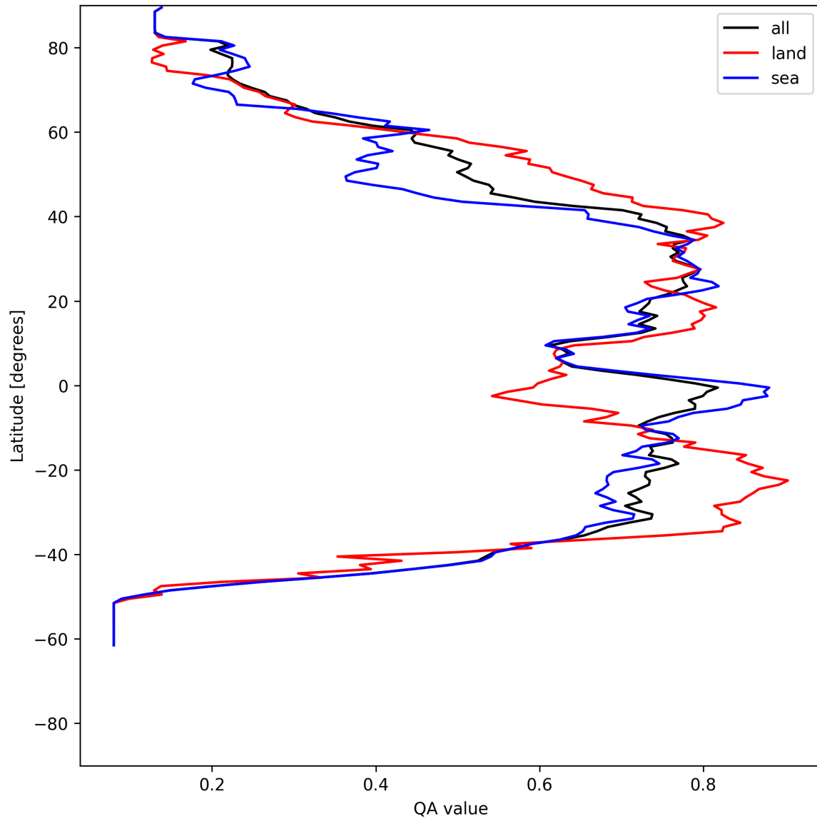
Figure 18: Zonal average of “QA value” for 2025-06-26 to 2025-06-27.
