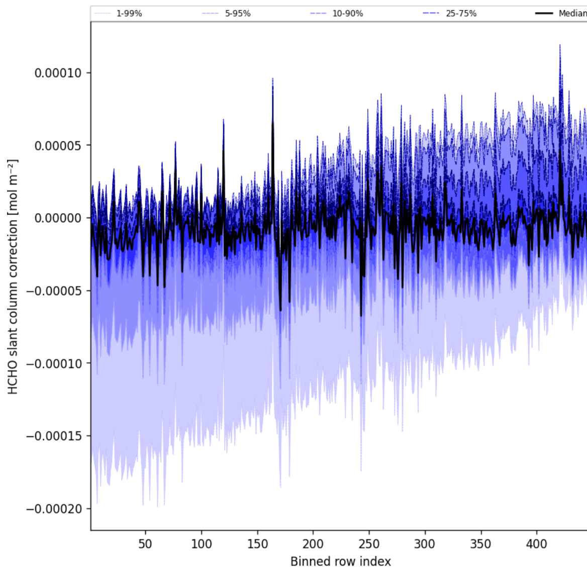
Figure 59: Along track statistics of “HCHO slant column correction” for 2025-06-26 to 2025-06-27
