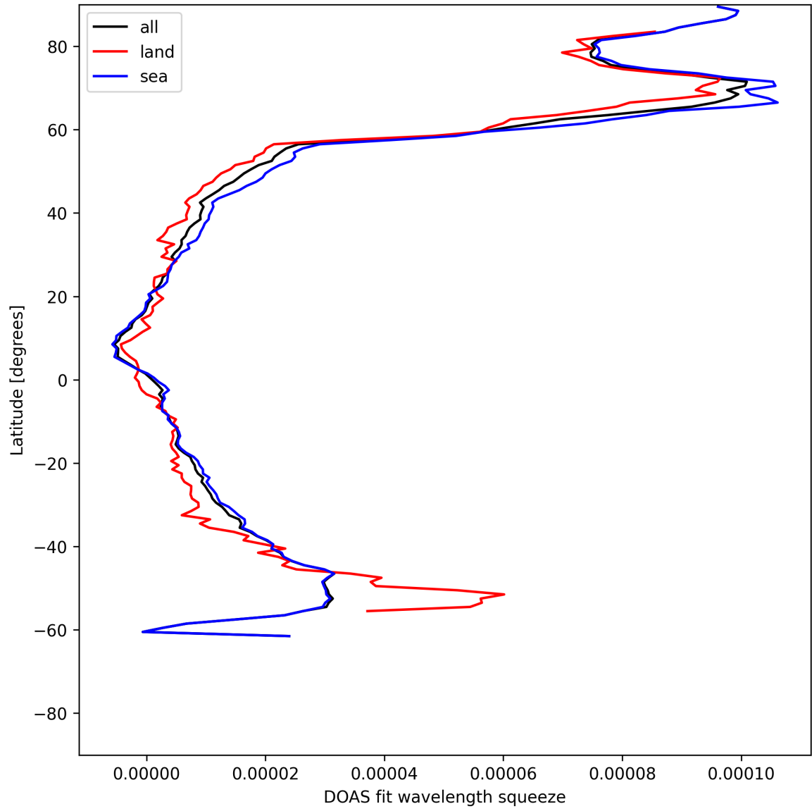
Figure 29: Zonal average of “DOAS fit wavelength squeeze” for 2025-06-26 to 2025-06-27.
