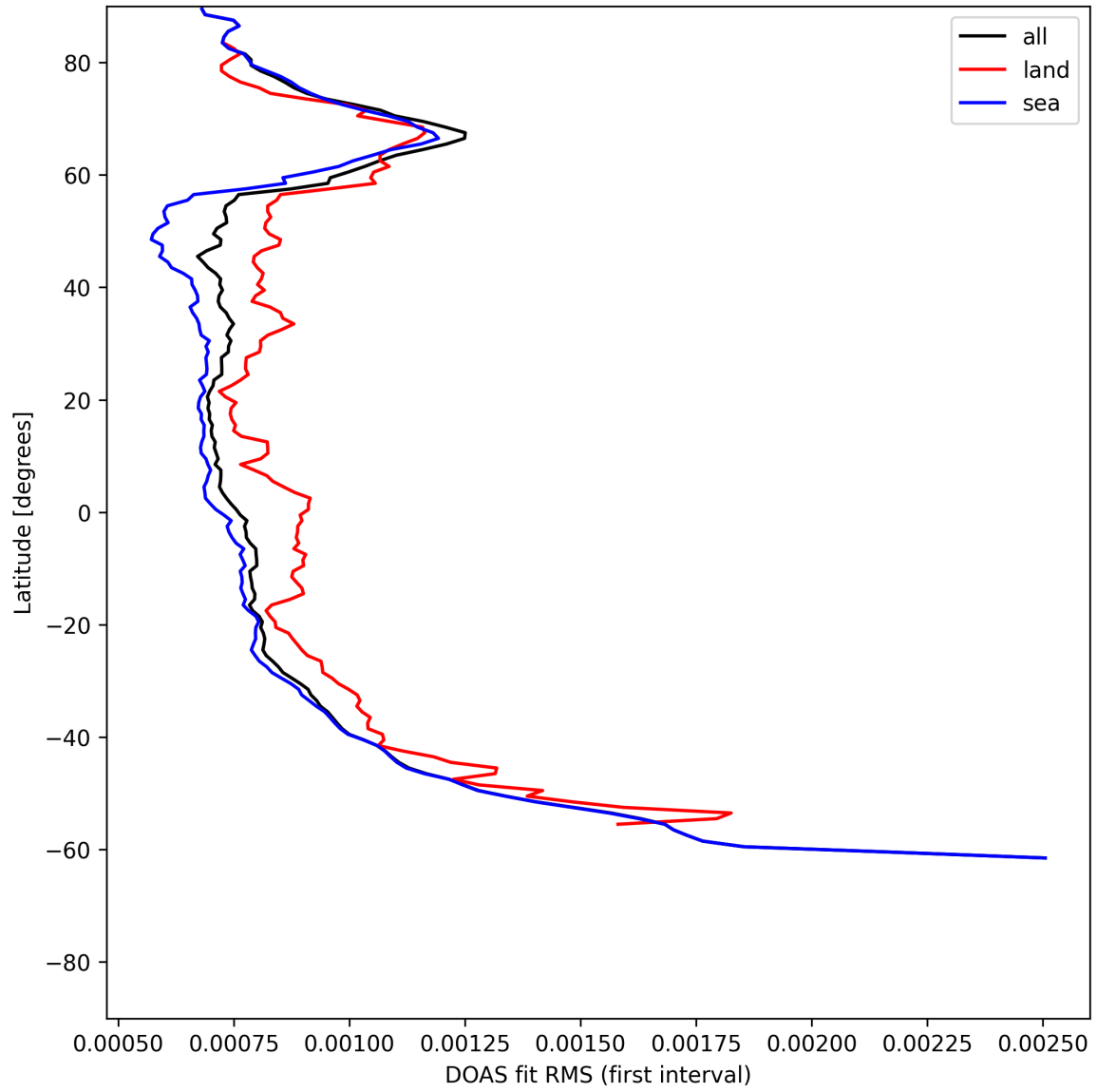
Figure 30: Zonal average of "DOAS fit RMS (first interval)" for 2025-06-26 to 2025-06-27.
