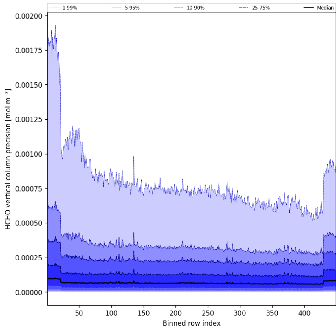
Figure 48: Along track statistics of “HCHO vertical column precision” for 2025-06-26 to 2025-06-27
