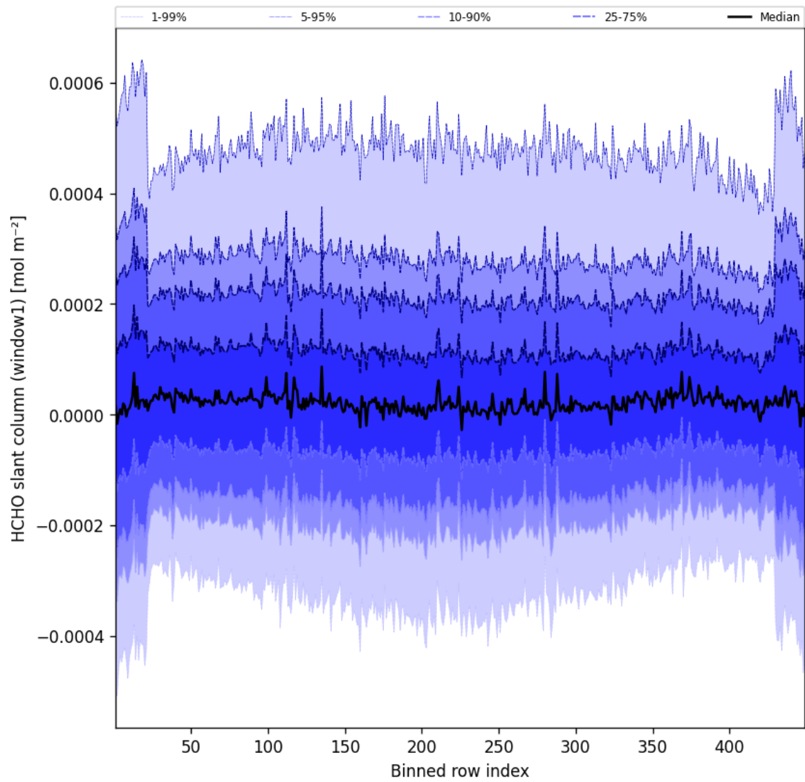
Figure 50: Along track statistics of “HCHO slant column (window1)” for 2025-06-26 to 2025-06-27
