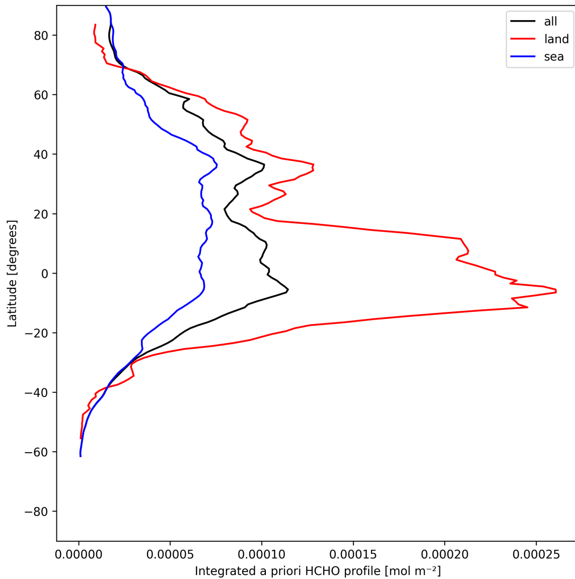
Figure 27: Zonal average of “Integrated a priori HCHO profile” for 2025-06-27 to 2025-06-28.
