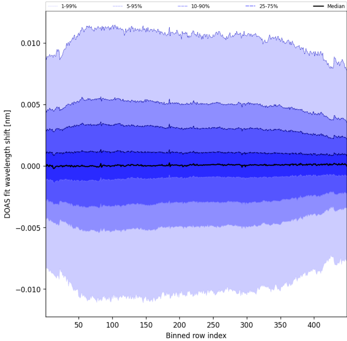
Figure 56: Along track statistics of “DOAS fit wavelength shift” for 2025-06-27 to 2025-06-28
