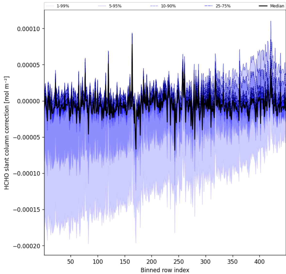
Figure 59: Along track statistics of “HCHO slant column correction” for 2025-06-27 to 2025-06-28
