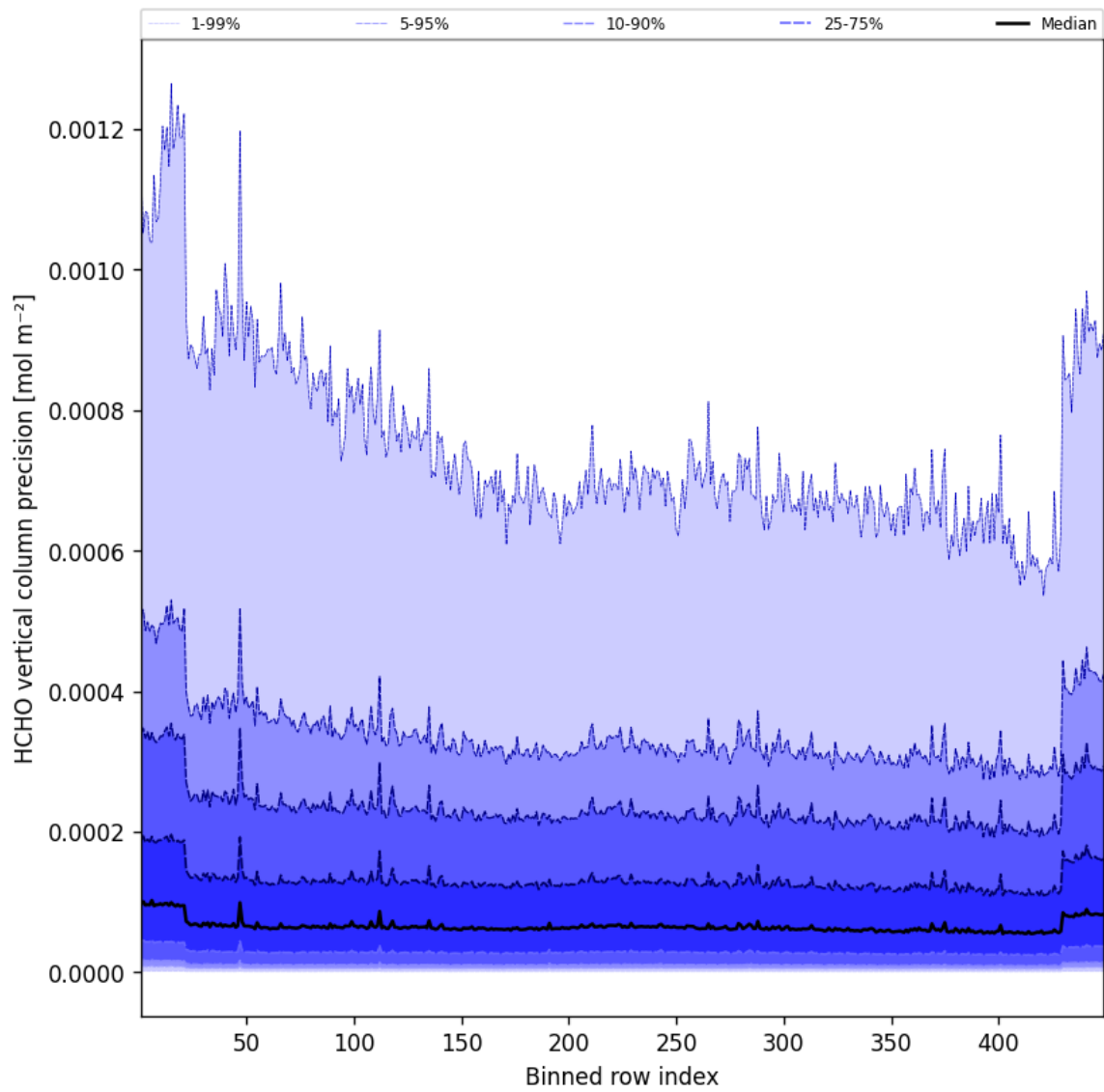
Figure 48: Along track statistics of “HCHO vertical column precision” for 2025-06-27 to 2025-06-28
