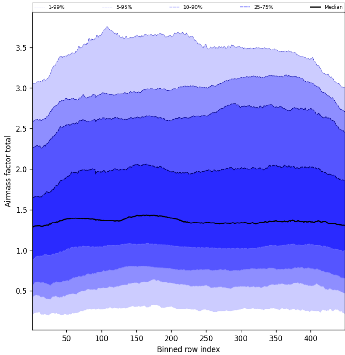
Figure 52: Along track statistics of “Airmass factor total” for 2025-06-27 to 2025-06-28
