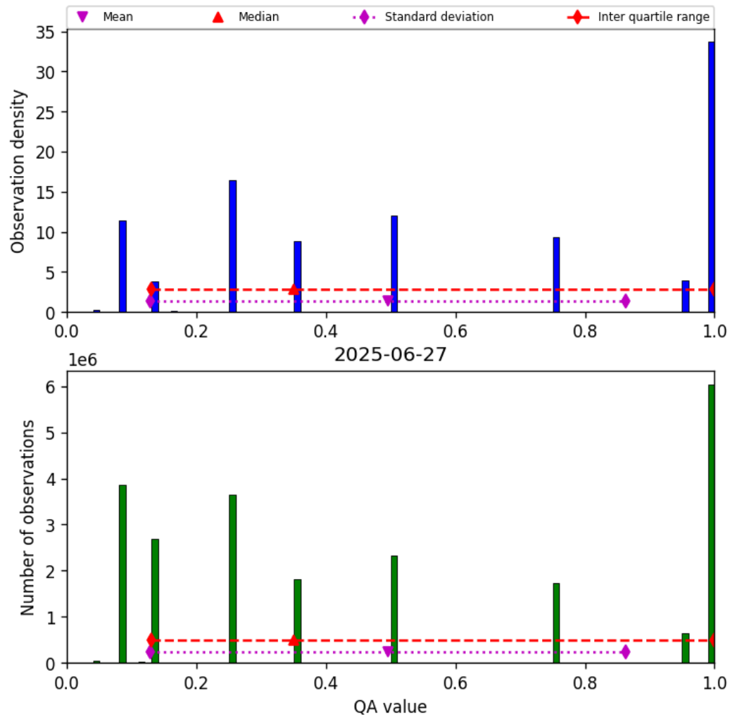
Figure 32: Histogram of “QA value” for 2025-06-27 to 2025-06-28
