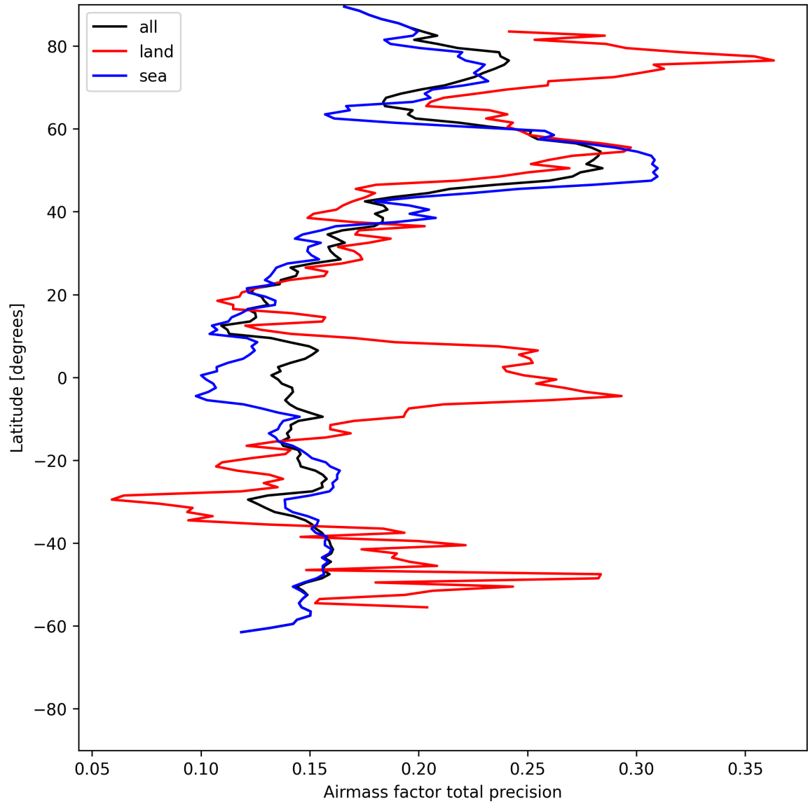
Figure 25: Zonal average of “Airmass factor total precision” for 2025-06-27 to 2025-06-28.
