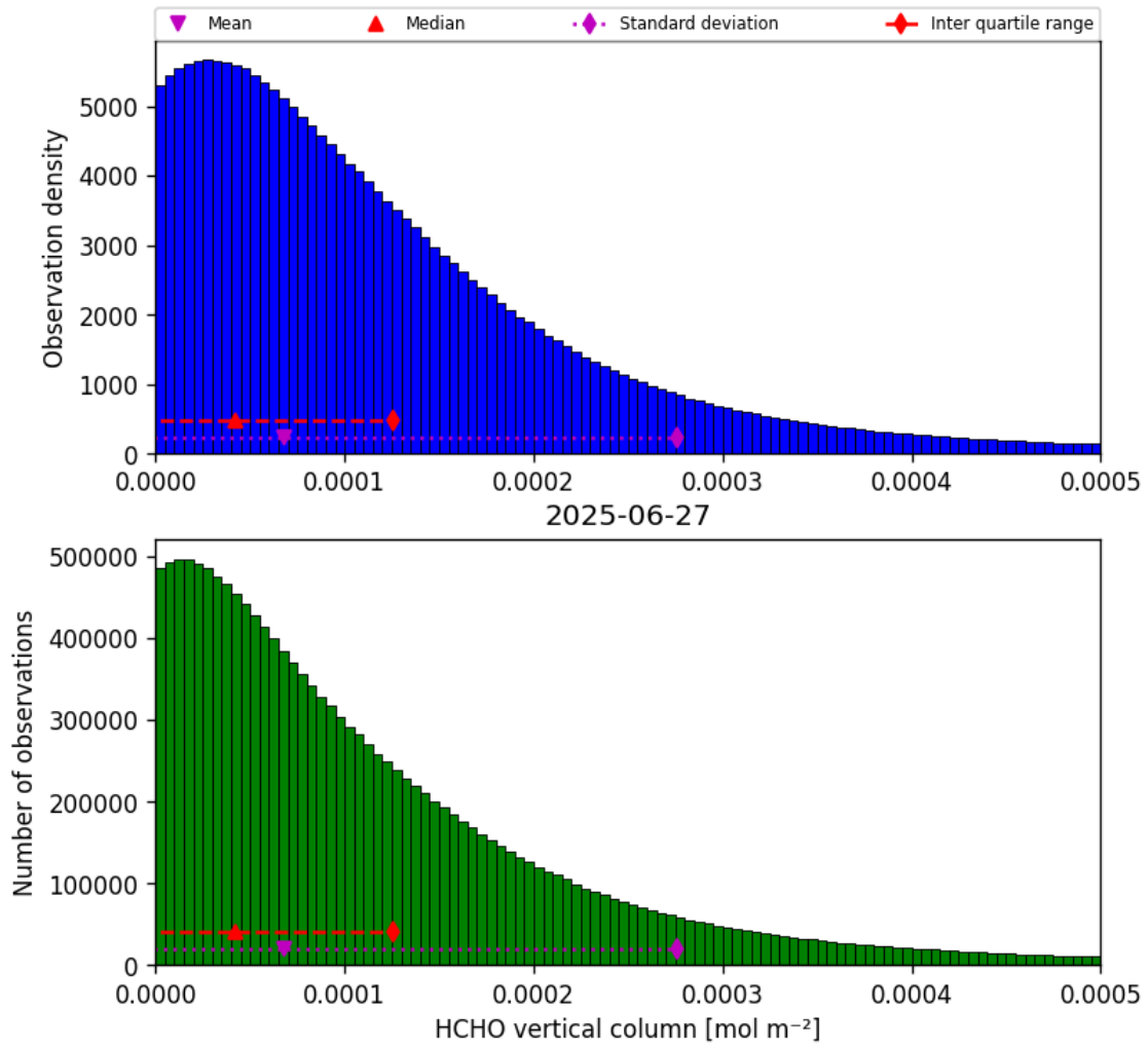
Figure 33: Histogram of “HCHO vertical column” for 2025-06-27 to 2025-06-28
