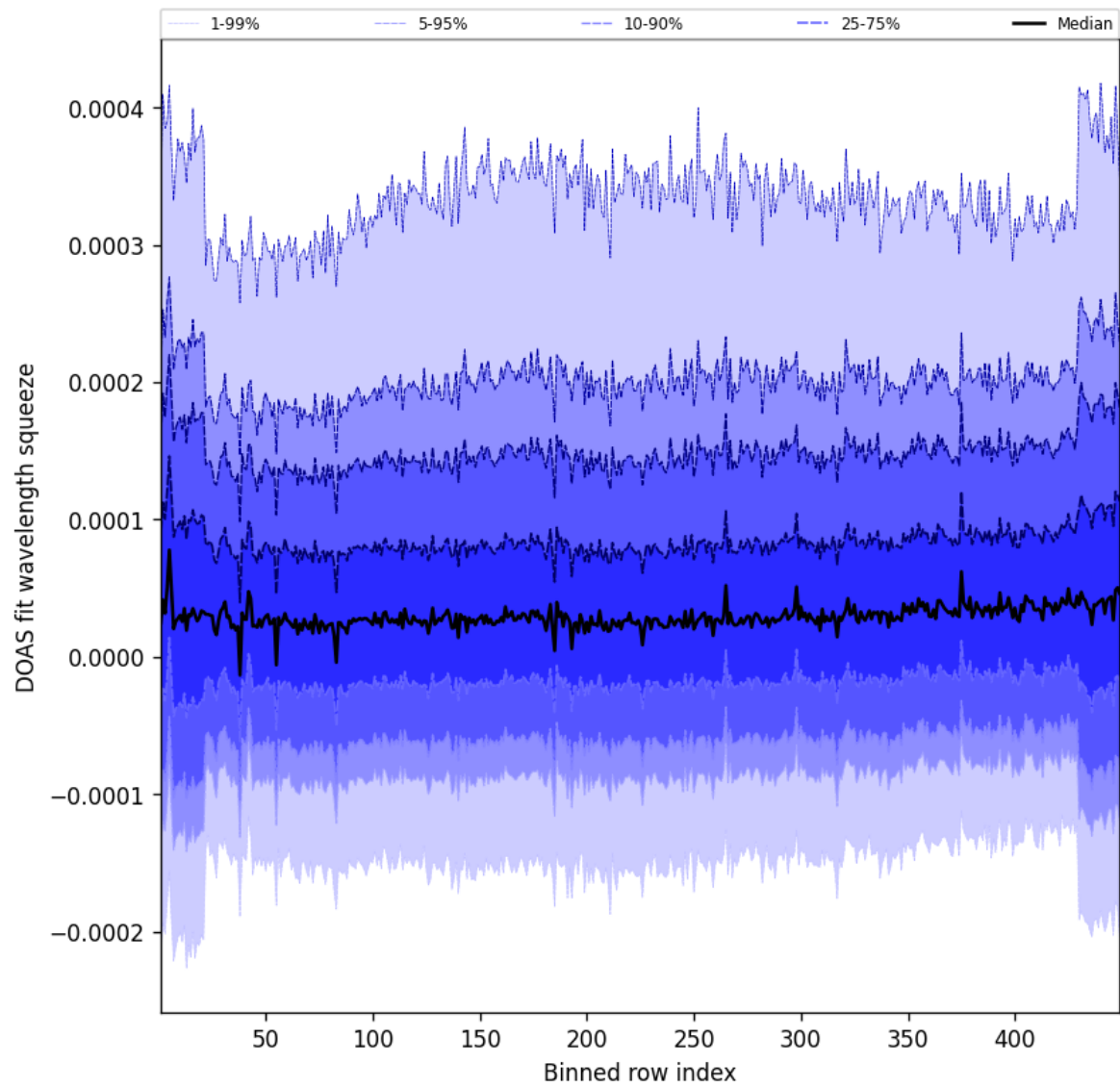
Figure 57: Along track statistics of “DOAS fit wavelength squeeze” for 2025-06-27 to 2025-06-28
