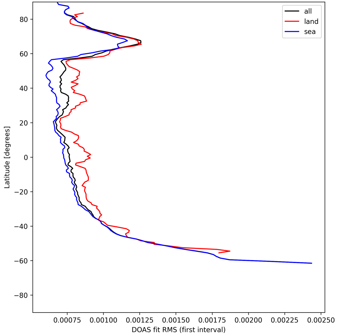
Figure 30: Zonal average of “DOAS fit RMS (first interval)” for 2025-06-27 to 2025-06-28.
