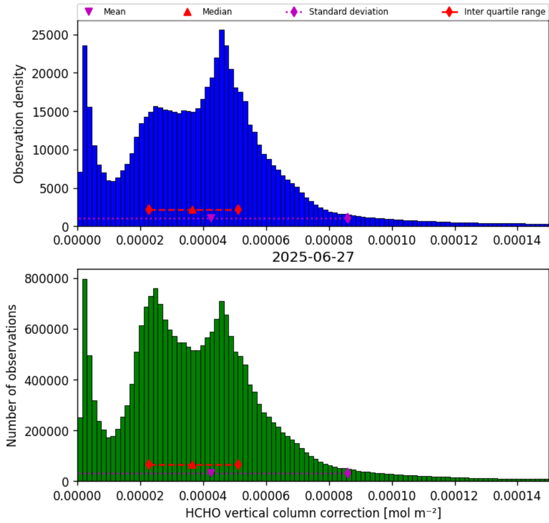
Figure 35: Histogram of “HCHO vertical column correction” for 2025-06-27 to 2025-06-28
