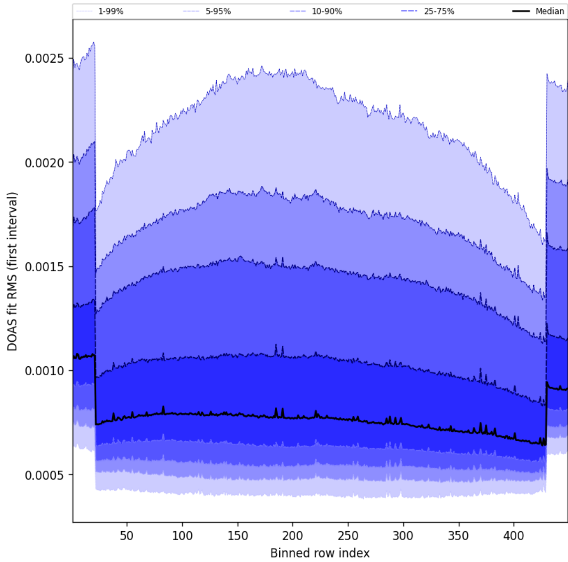
Figure 58: Along track statistics of “DOAS fit RMS (first interval)” for 2025-06-27 to 2025-06-28
