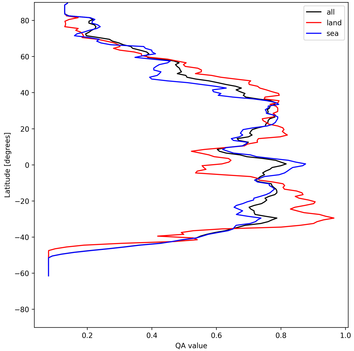
Figure 18: Zonal average of “QA value” for 2025-06-27 to 2025-06-28.
