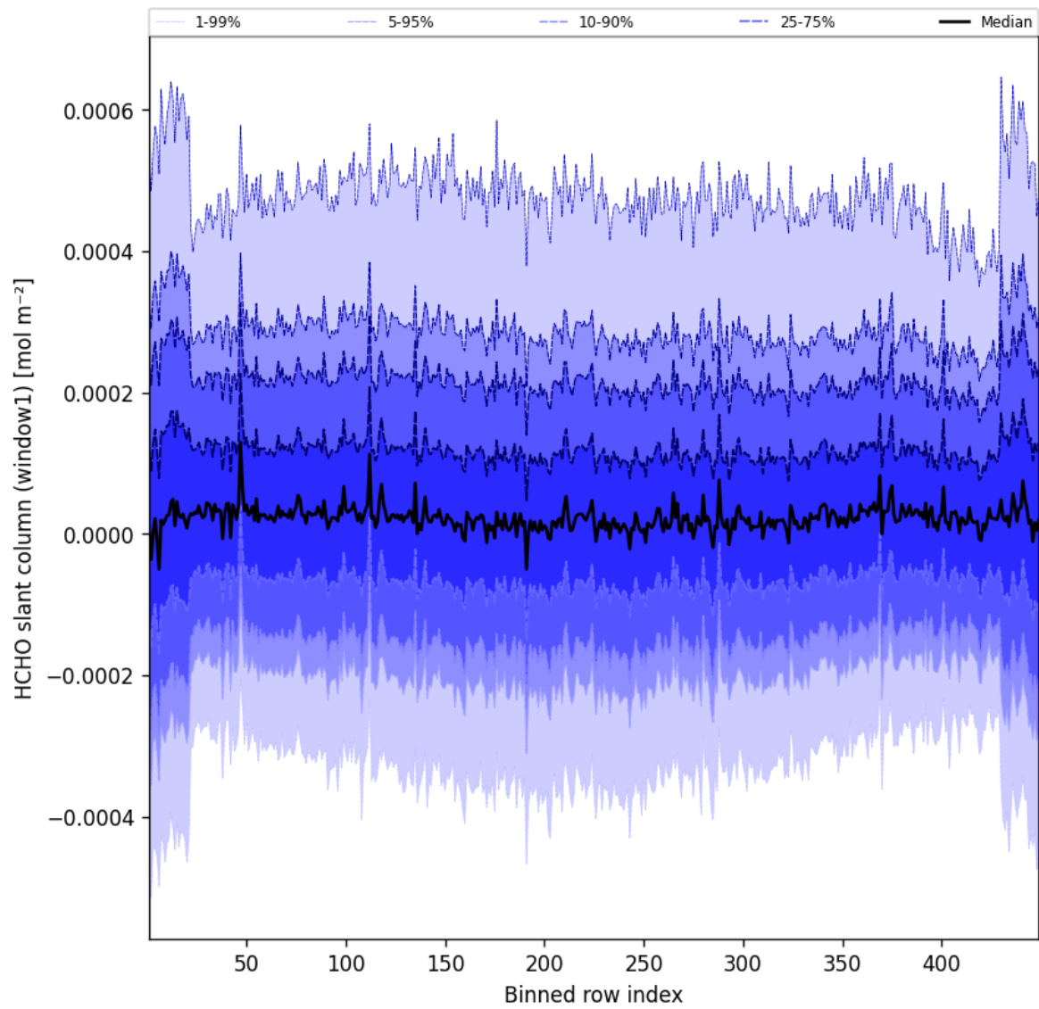
Figure 50: Along track statistics of “HCHO slant column (window1)” for 2025-06-27 to 2025-06-28
