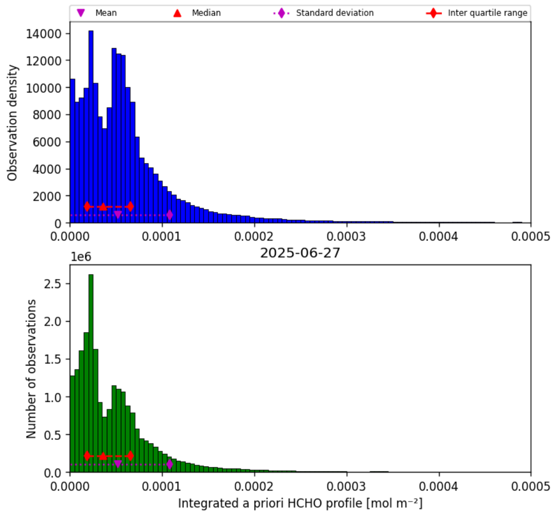
Figure 41: Histogram of “Integrated a priori HCHO profile” for 2025-06-27 to 2025-06-28
