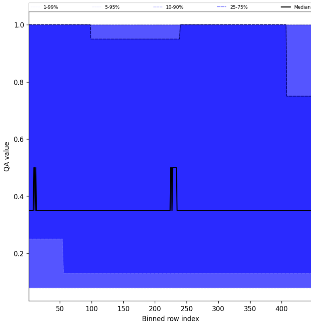
Figure 46: Along track statistics of “QA value” for 2025-06-27 to 2025-06-28
