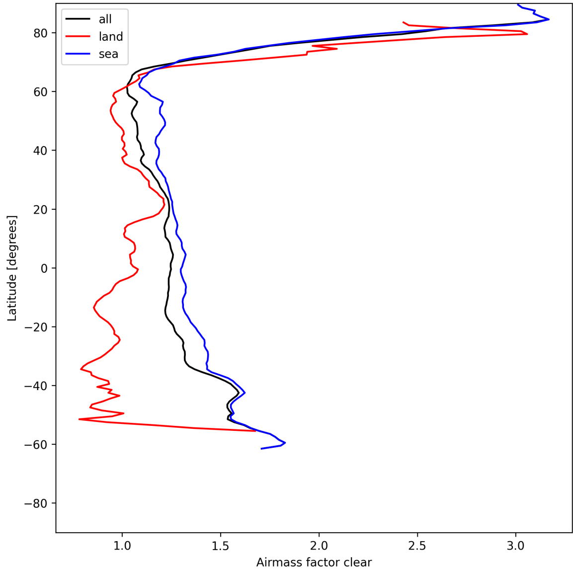
Figure 26: Zonal average of “Airmass factor clear” for 2025-06-27 to 2025-06-28.
