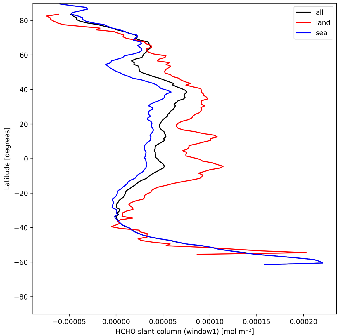
Figure 22: Zonal average of “HCHO slant column (window1)” for 2025-06-27 to 2025-06-28.
