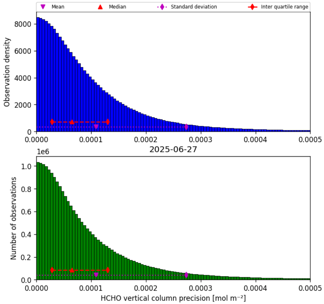
Figure 34: Histogram of “HCHO vertical column precision” for 2025-06-27 to 2025-06-28
