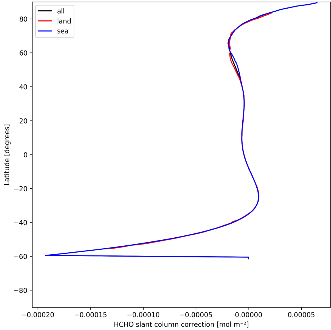
Figure 31: Zonal average of “HCHO slant column correction” for 2025-06-27 to 2025-06-28.
