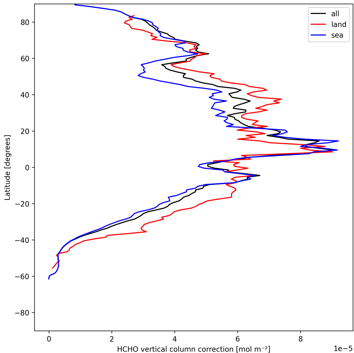
Figure 21: Zonal average of “HCHO vertical column correction” for 2025-06-27 to 2025-06-28.
