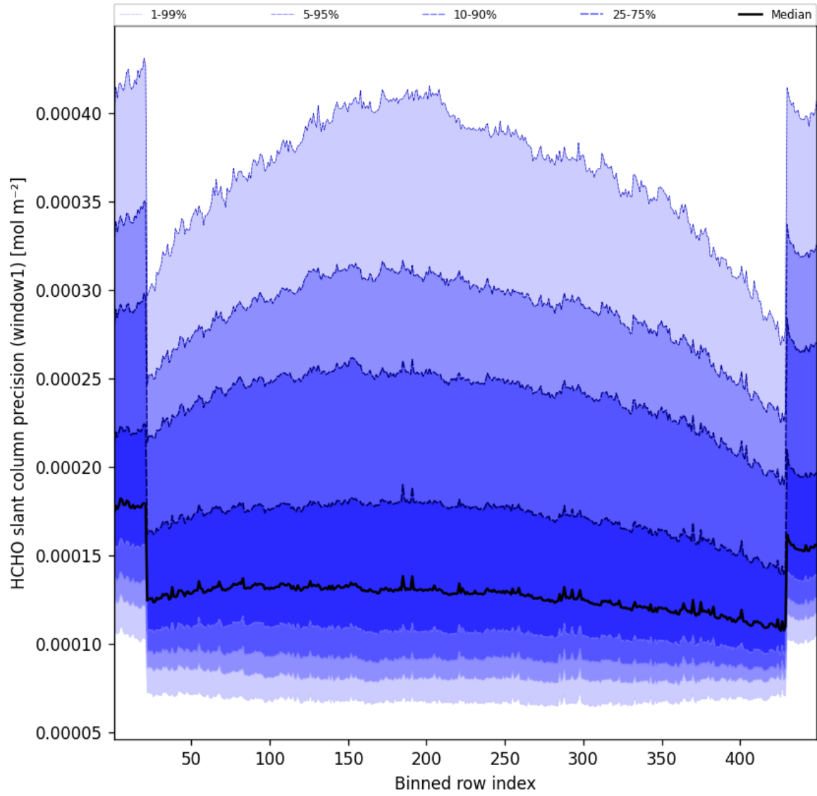
Figure 51: Along track statistics of “HCHO slant column precision (window1)” for 2025-06-27 to 2025-06-28
