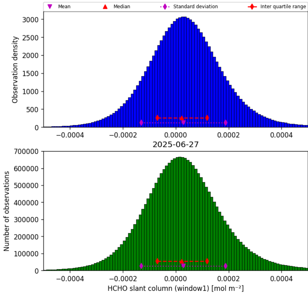
Figure 36: Histogram of “HCHO slant column (window1)” for 2025-06-27 to 2025-06-28
