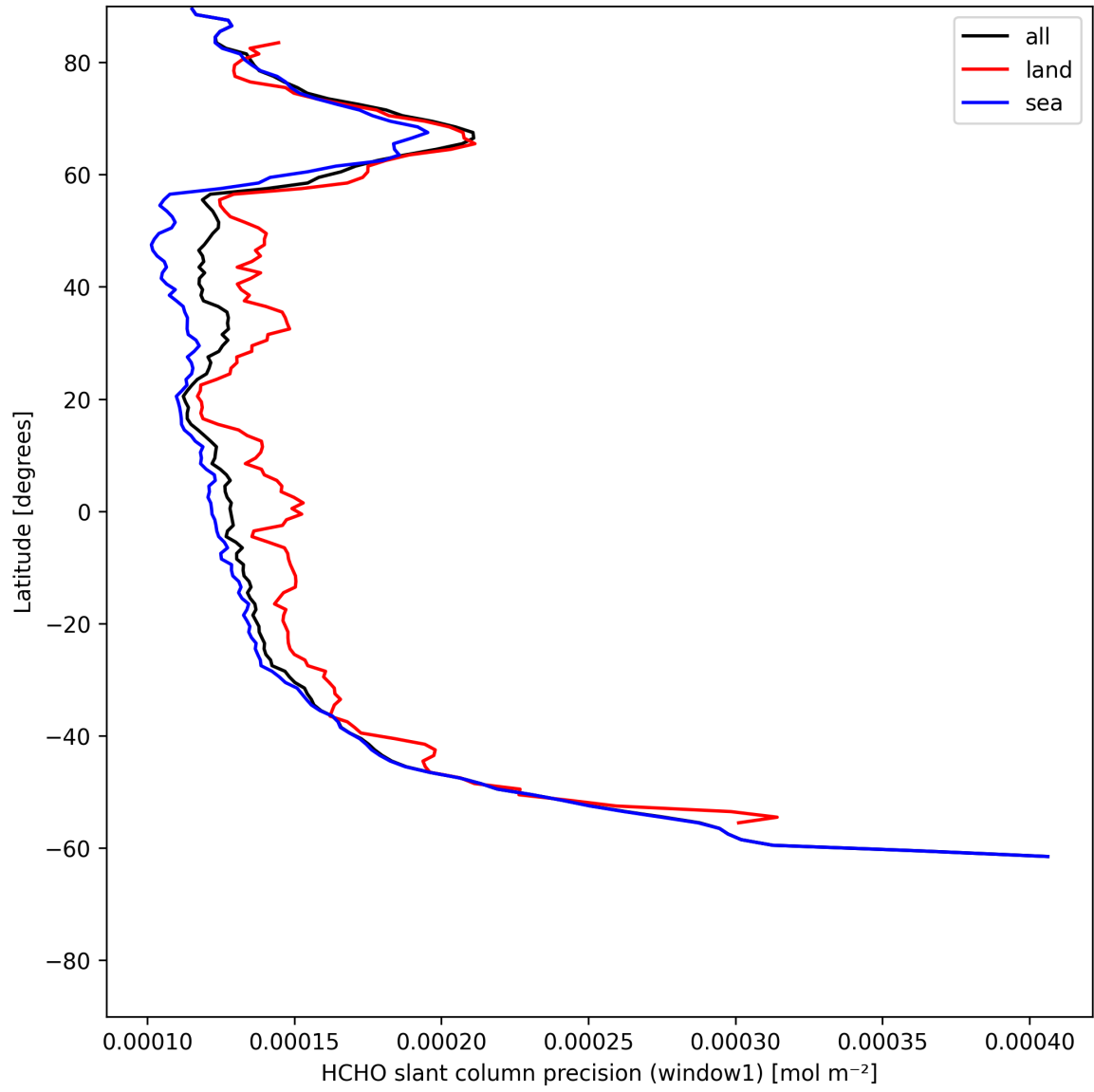
Figure 23: Zonal average of “HCHO slant column precision (window1)” for 2025-06-27 to 2025-06-28.
