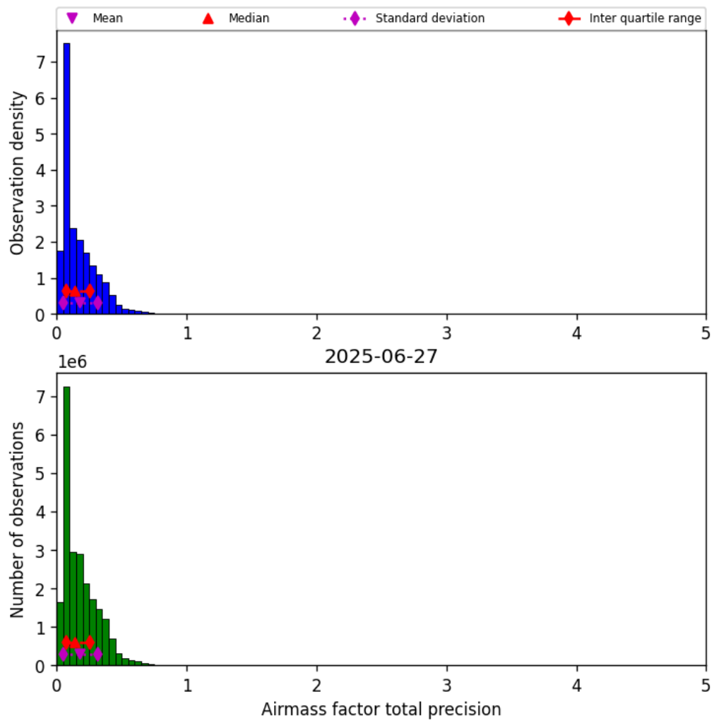
Figure 39: Histogram of “Airmass factor total precision” for 2025-06-27 to 2025-06-28
