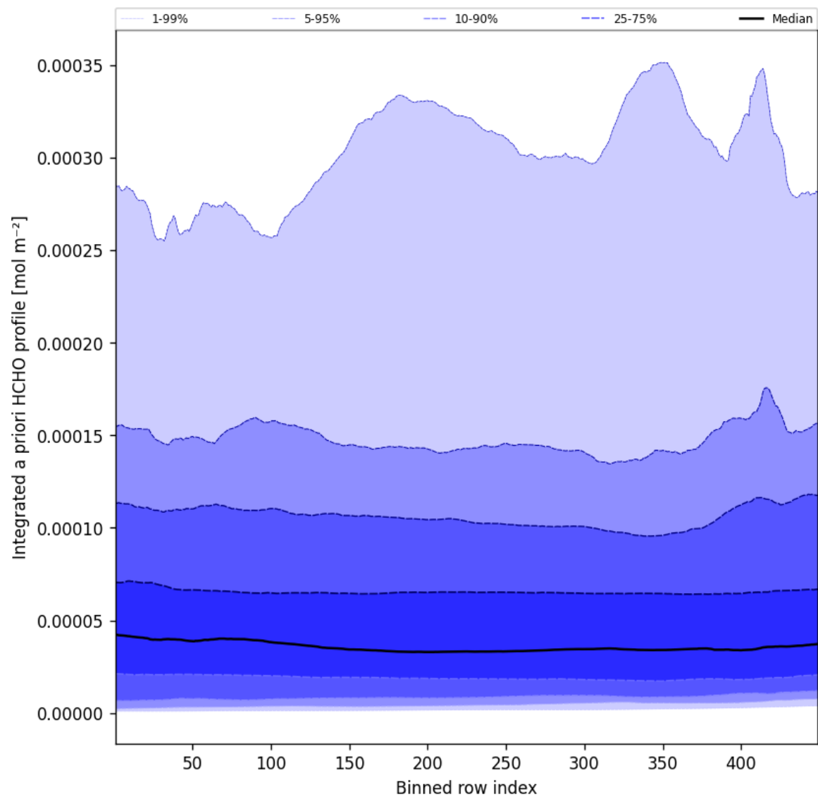
Figure 55: Along track statistics of “Integrated a priori HCHO profile” for 2025-06-27 to 2025-06-28
