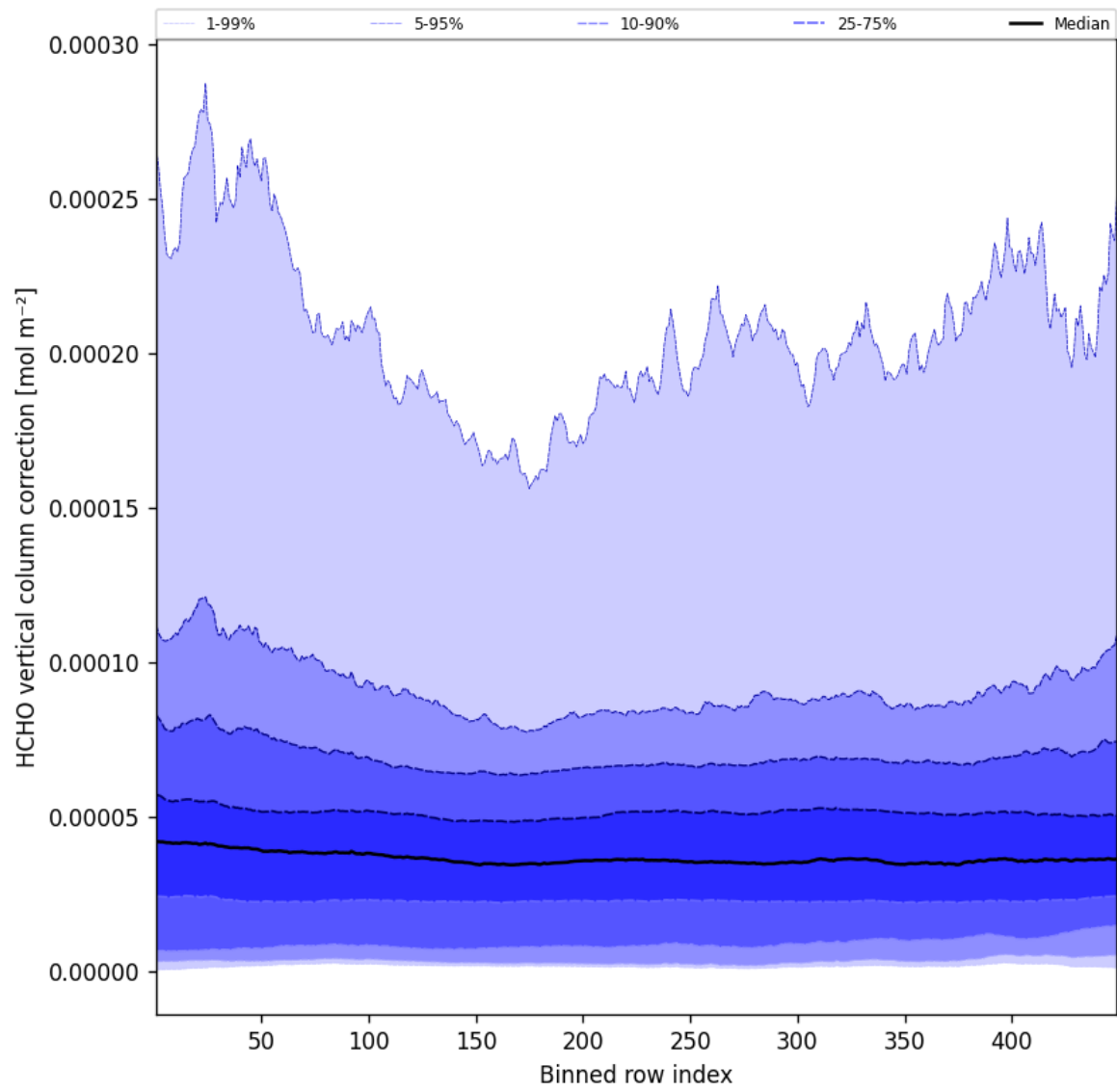
Figure 49: Along track statistics of “HCHO vertical column correction” for 2025-06-27 to 2025-06-28
