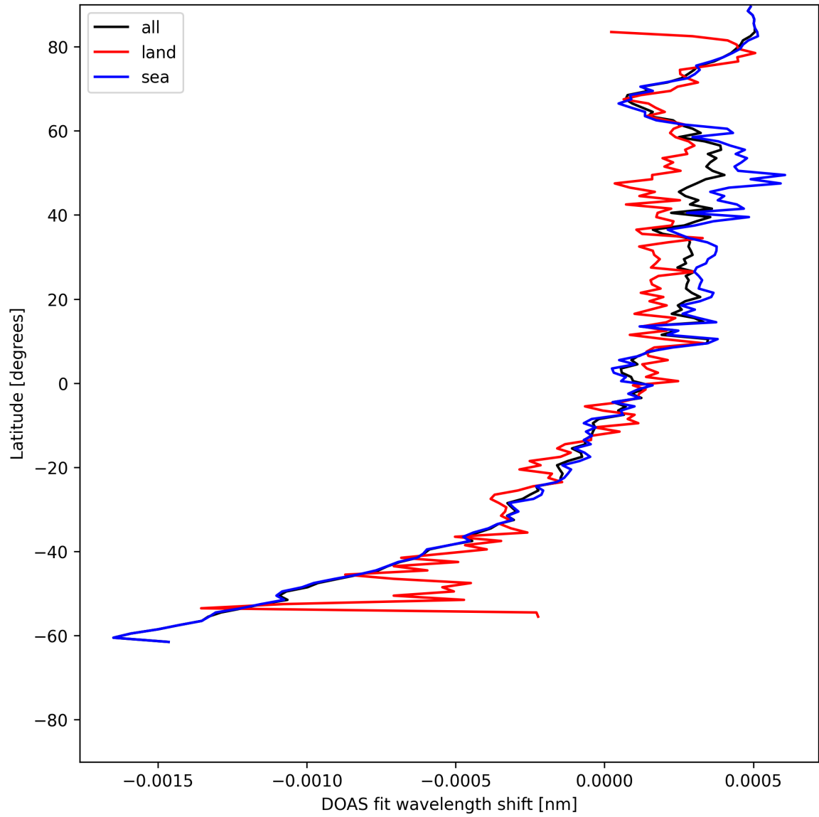
Figure 28: Zonal average of “DOAS fit wavelength shift” for 2025-06-27 to 2025-06-28.
