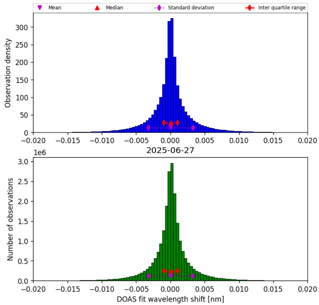
Figure 42: Histogram of “DOAS fit wavelength shift” for 2025-06-27 to 2025-06-28
