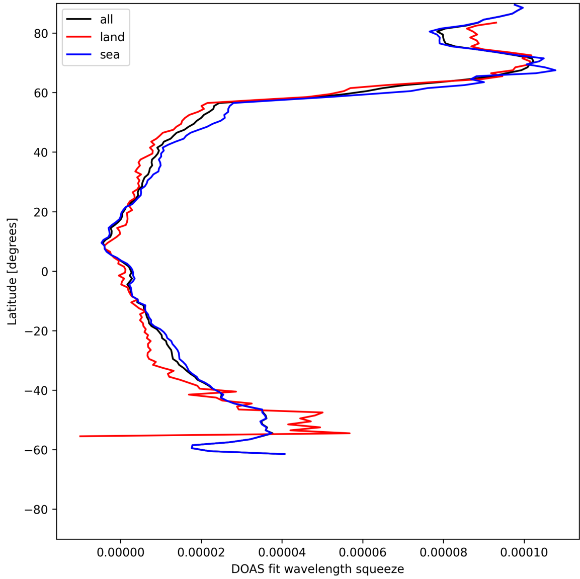
Figure 29: Zonal average of “DOAS fit wavelength squeeze” for 2025-06-27 to 2025-06-28.
