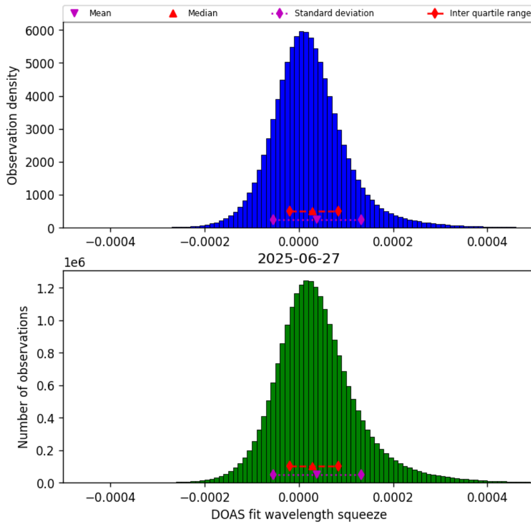
Figure 43: Histogram of “DOAS fit wavelength squeeze” for 2025-06-27 to 2025-06-28
