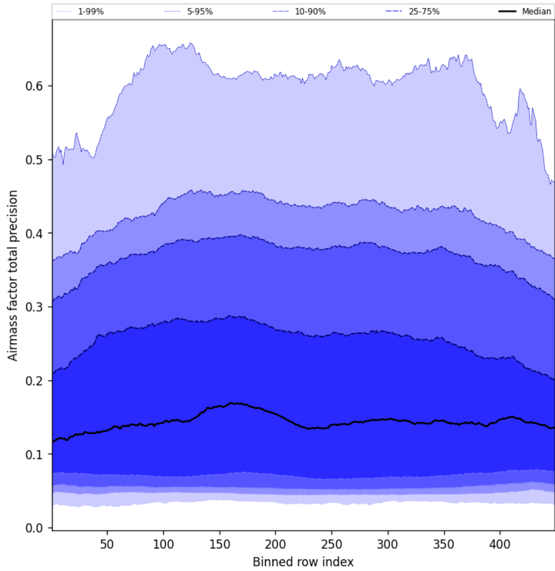
Figure 53: Along track statistics of “Airmass factor total precision” for 2025-06-27 to 2025-06-28
