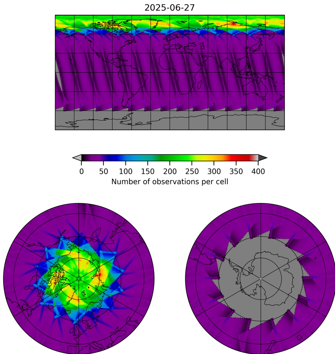
Figure 17: Map of the number of observations for 2025-06-27 to 2025-06-28
