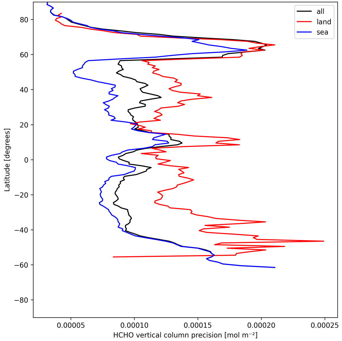
Figure 20: Zonal average of “HCHO vertical column precision” for 2025-06-27 to 2025-06-28.
