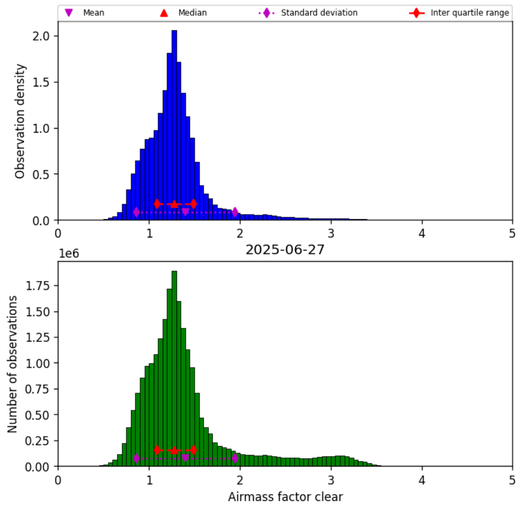
Figure 40: Histogram of “Airmass factor clear” for 2025-06-27 to 2025-06-28
