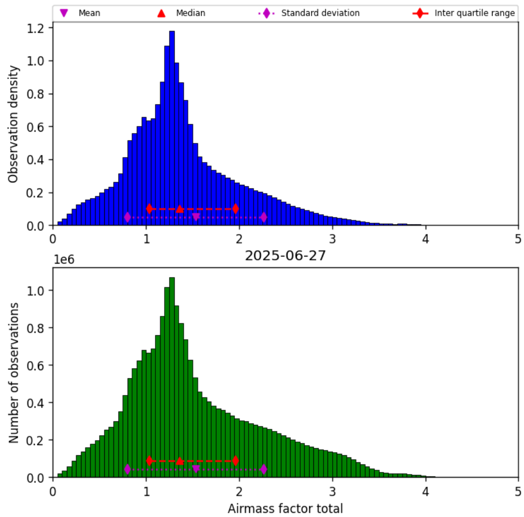
Figure 38: Histogram of “Airmass factor total” for 2025-06-27 to 2025-06-28
