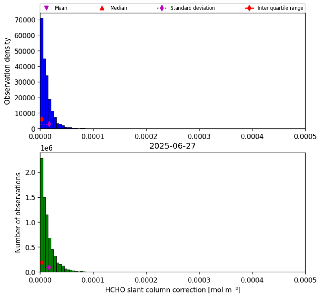
Figure 45: Histogram of “HCHO slant column correction” for 2025-06-27 to 2025-06-28
