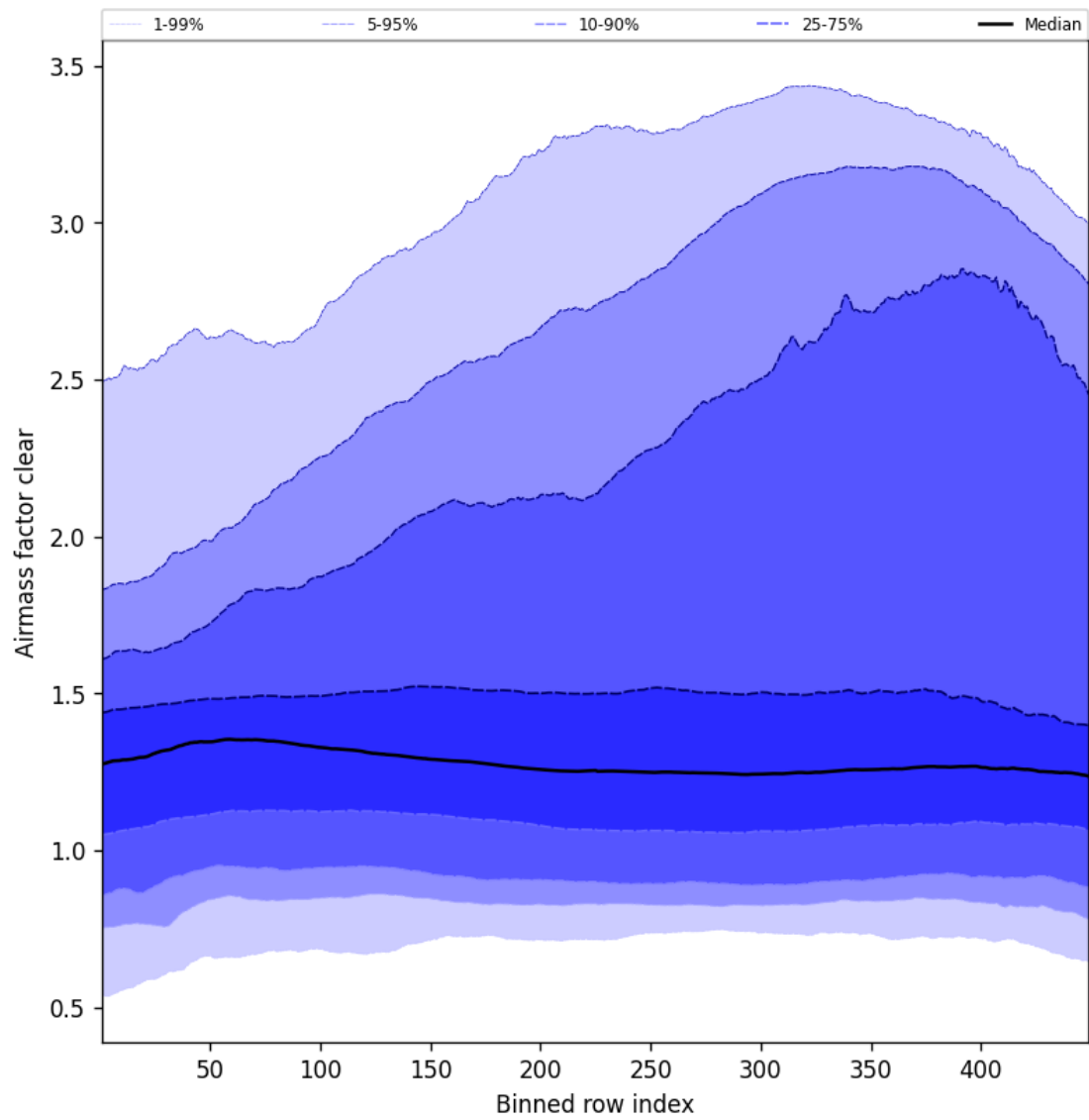
Figure 54: Along track statistics of “Airmass factor clear” for 2025-06-27 to 2025-06-28
