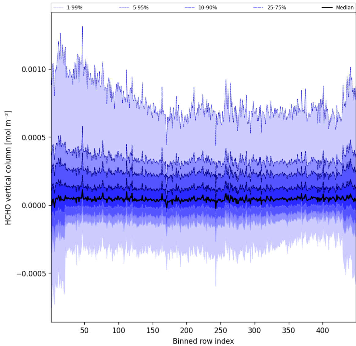
Figure 47: Along track statistics of “HCHO vertical column” for 2025-06-27 to 2025-06-28
