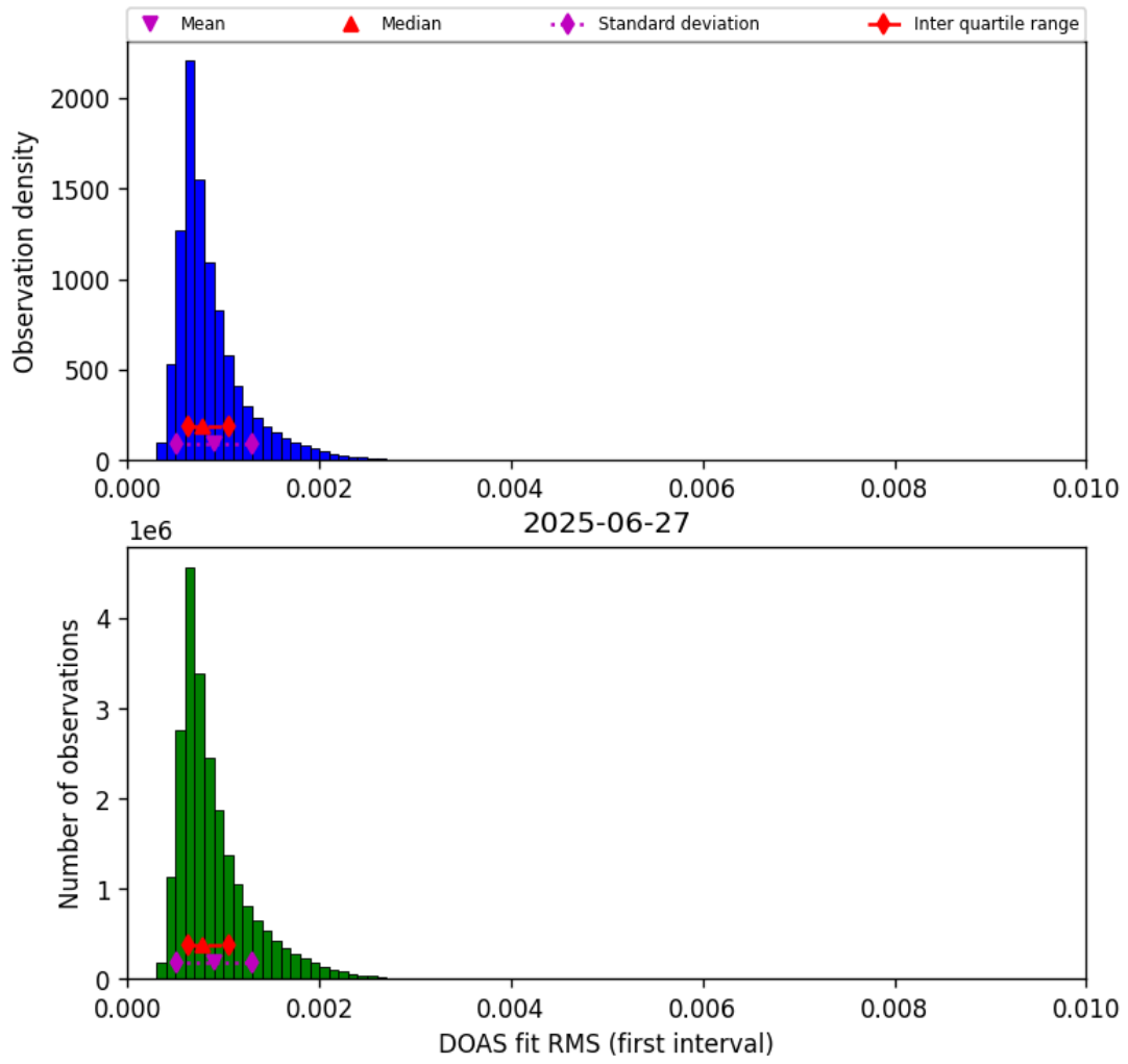
Figure 44: Histogram of “DOAS fit RMS (first interval)” for 2025-06-27 to 2025-06-28
