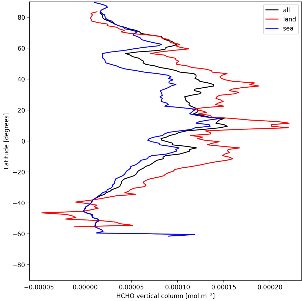
Figure 19: Zonal average of “HCHO vertical column” for 2025-06-27 to 2025-06-28.
