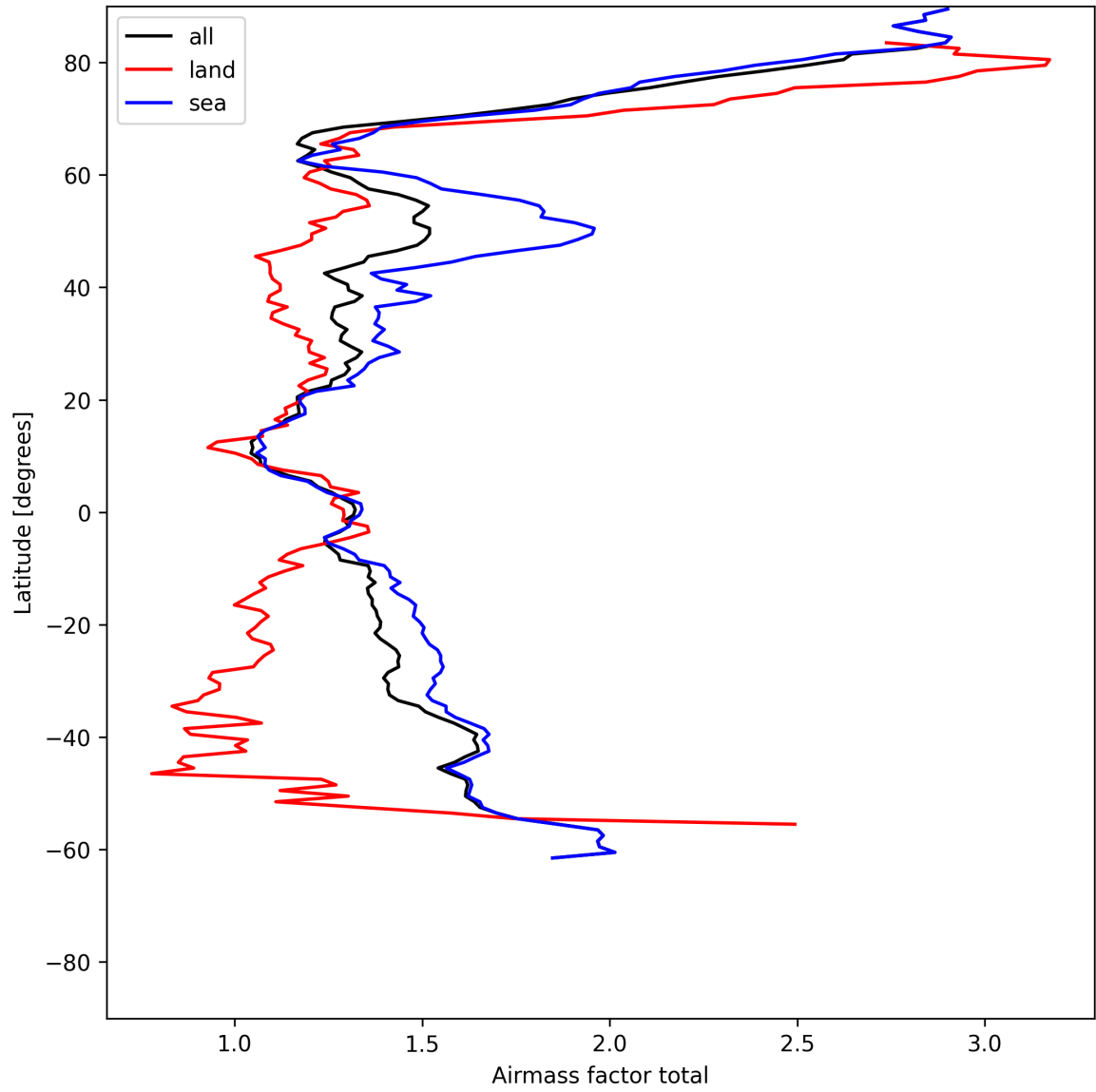
Figure 24: Zonal average of “Airmass factor total” for 2025-06-27 to 2025-06-28.
