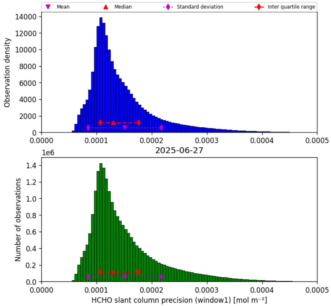
Figure 37: Histogram of “HCHO slant column precision (window1)” for 2025-06-27 to 2025-06-28
