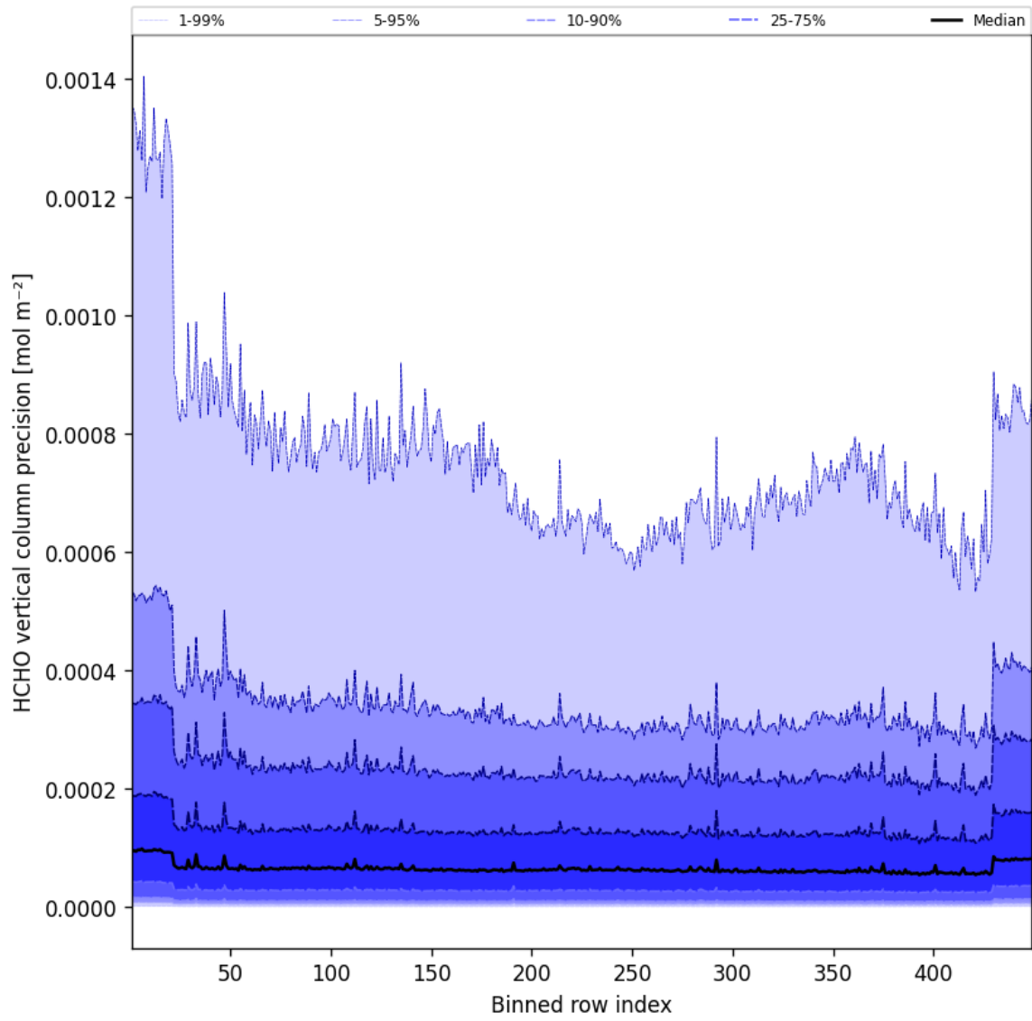
Figure 48: Along track statistics of “HCHO vertical column precision” for 2025-06-28 to 2025-06-29
