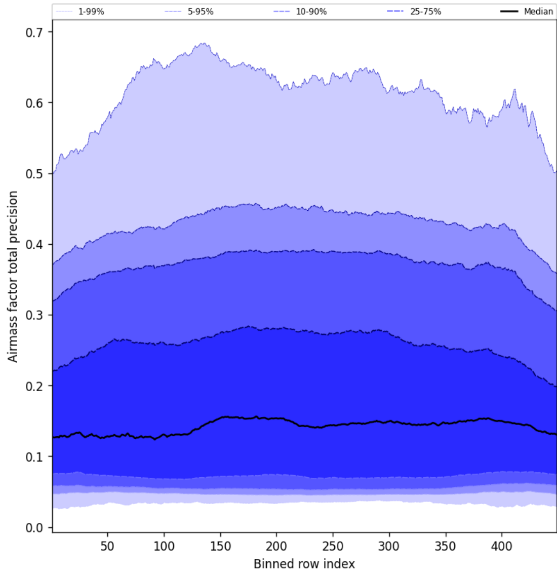
Figure 53: Along track statistics of “Airmass factor total precision” for 2025-06-28 to 2025-06-29
