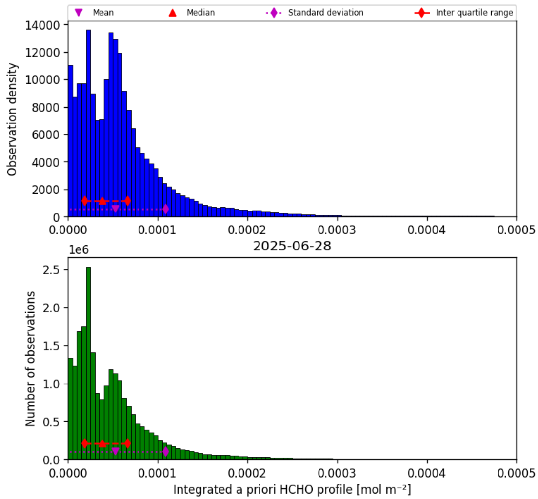
Figure 41: Histogram of “Integrated a priori HCHO profile” for 2025-06-28 to 2025-06-29
