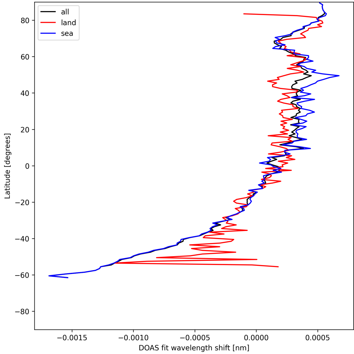
Figure 28: Zonal average of “DOAS fit wavelength shift” for 2025-06-28 to 2025-06-29.
