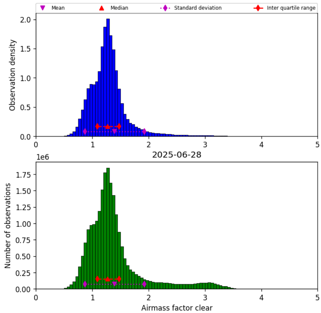
Figure 40: Histogram of “Airmass factor clear” for 2025-06-28 to 2025-06-29
