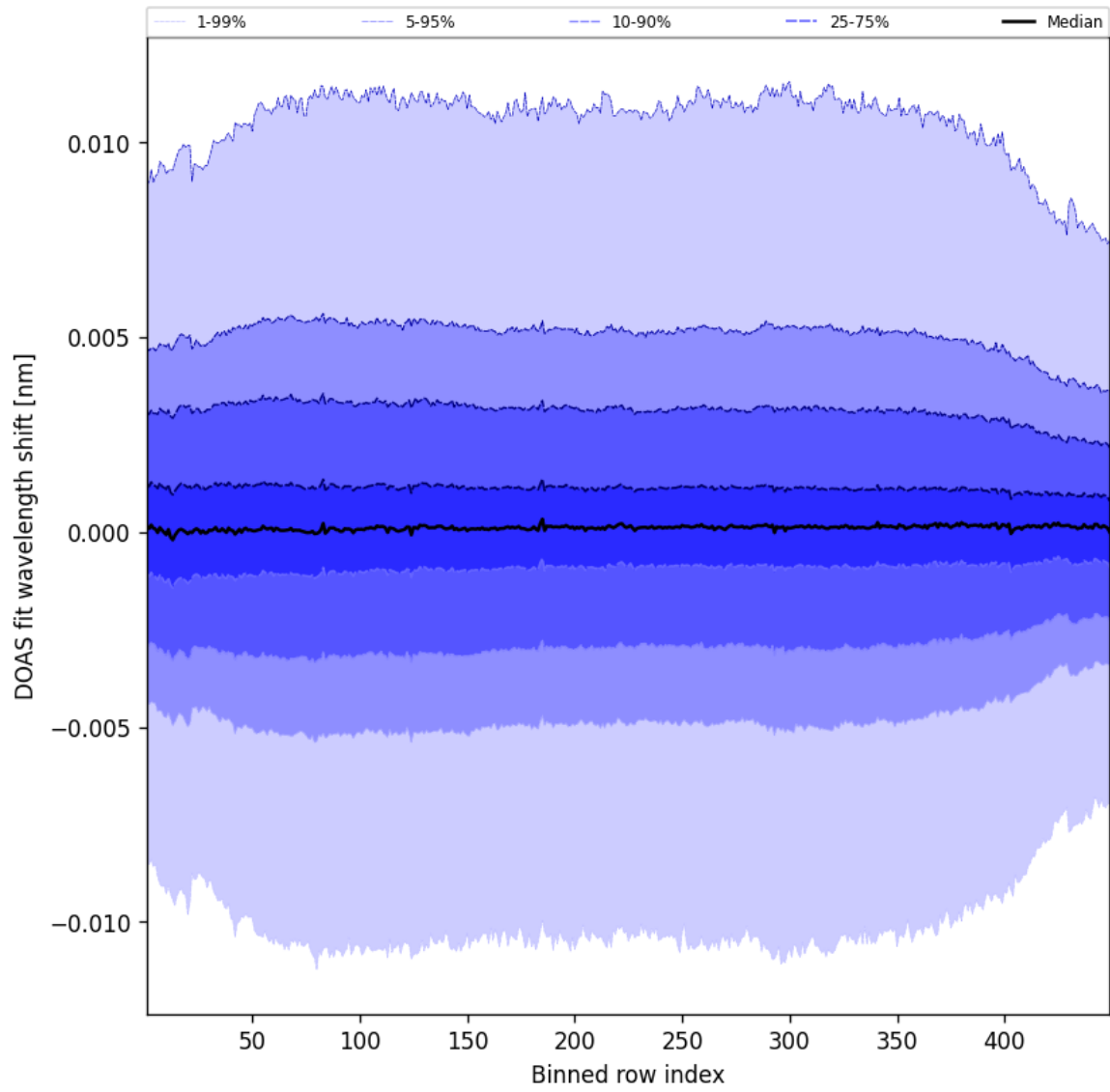
Figure 56: Along track statistics of “DOAS fit wavelength shift” for 2025-06-28 to 2025-06-29
