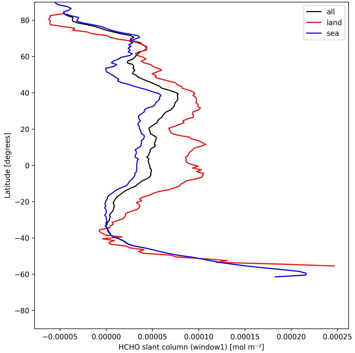
Figure 22: Zonal average of “HCHO slant column (window1)” for 2025-06-28 to 2025-06-29.
