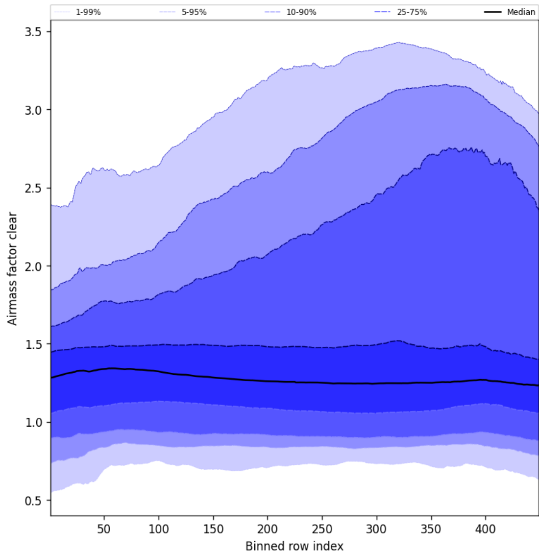
Figure 54: Along track statistics of “Airmass factor clear” for 2025-06-28 to 2025-06-29
