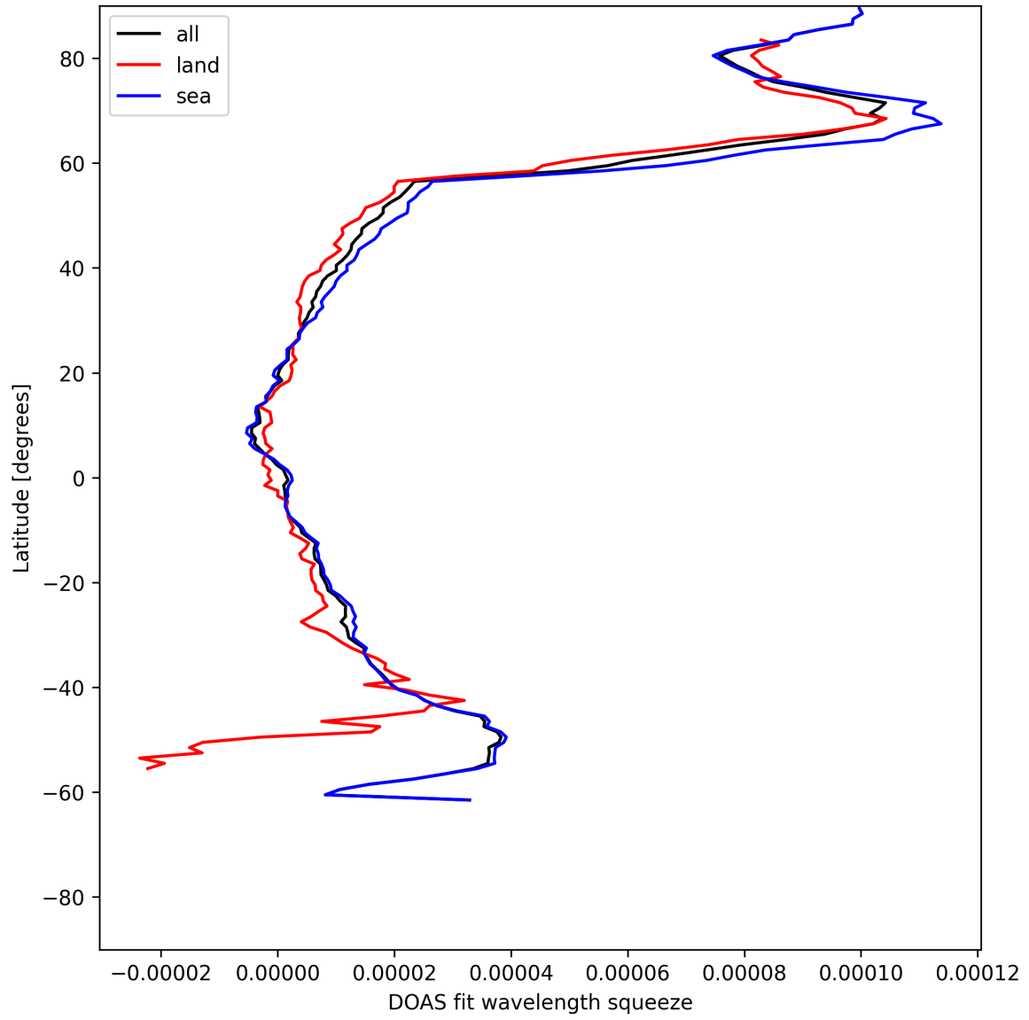
Figure 29: Zonal average of “DOAS fit wavelength squeeze” for 2025-06-28 to 2025-06-29.
