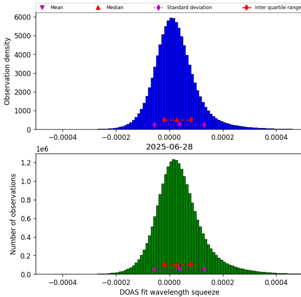
Figure 43: Histogram of “DOAS fit wavelength squeeze” for 2025-06-28 to 2025-06-29
