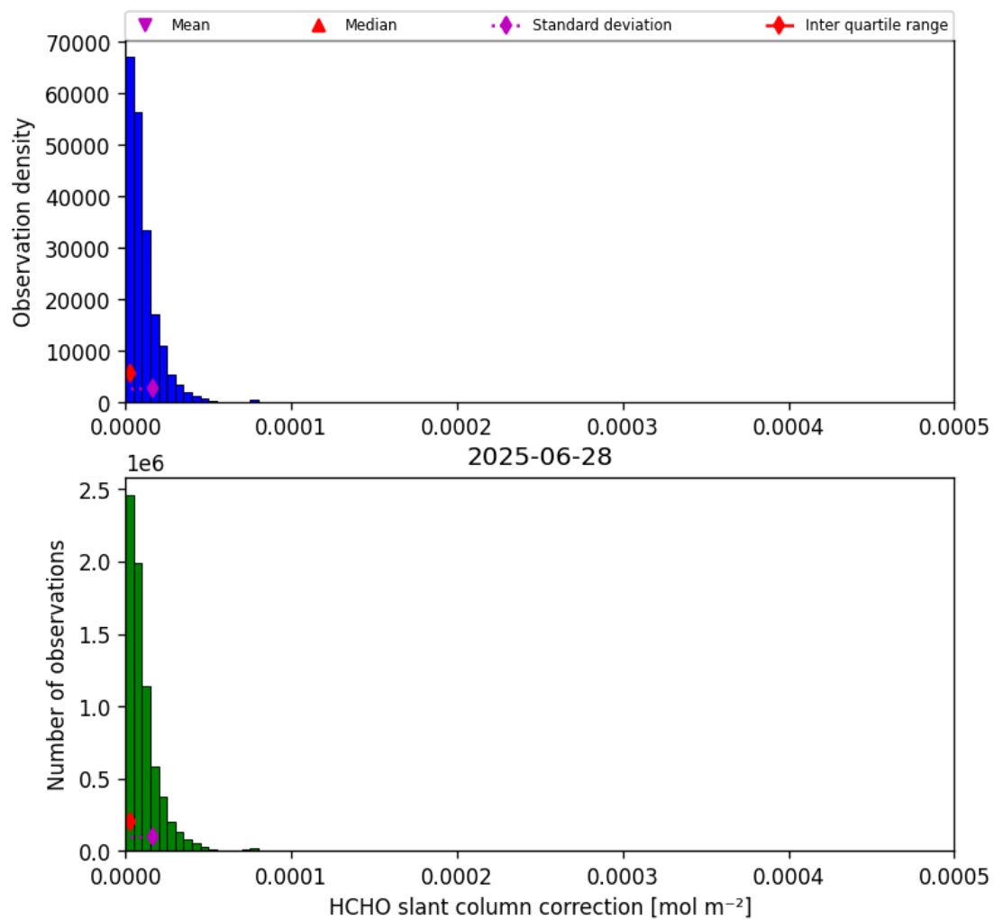
Figure 45: Histogram of "HCHO slant column correction" for 2025-06-28 to 2025-06-29
