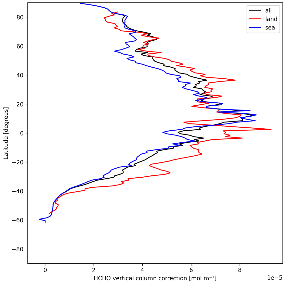
Figure 21: Zonal average of “HCHO vertical column correction” for 2025-06-28 to 2025-06-29.
