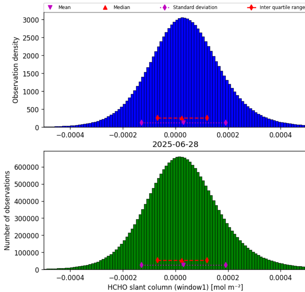
Figure 36: Histogram of “HCHO slant column (window1)” for 2025-06-28 to 2025-06-29
