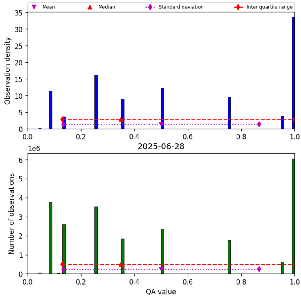
Figure 32: Histogram of “QA value” for 2025-06-28 to 2025-06-29
