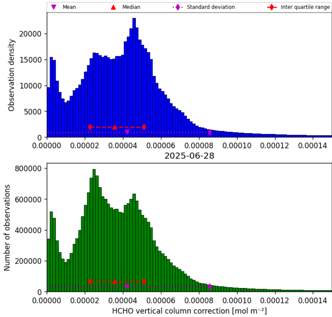
Figure 35: Histogram of “HCHO vertical column correction” for 2025-06-28 to 2025-06-29
