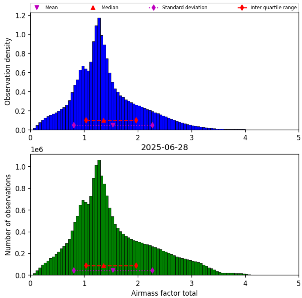
Figure 38: Histogram of “Airmass factor total” for 2025-06-28 to 2025-06-29
