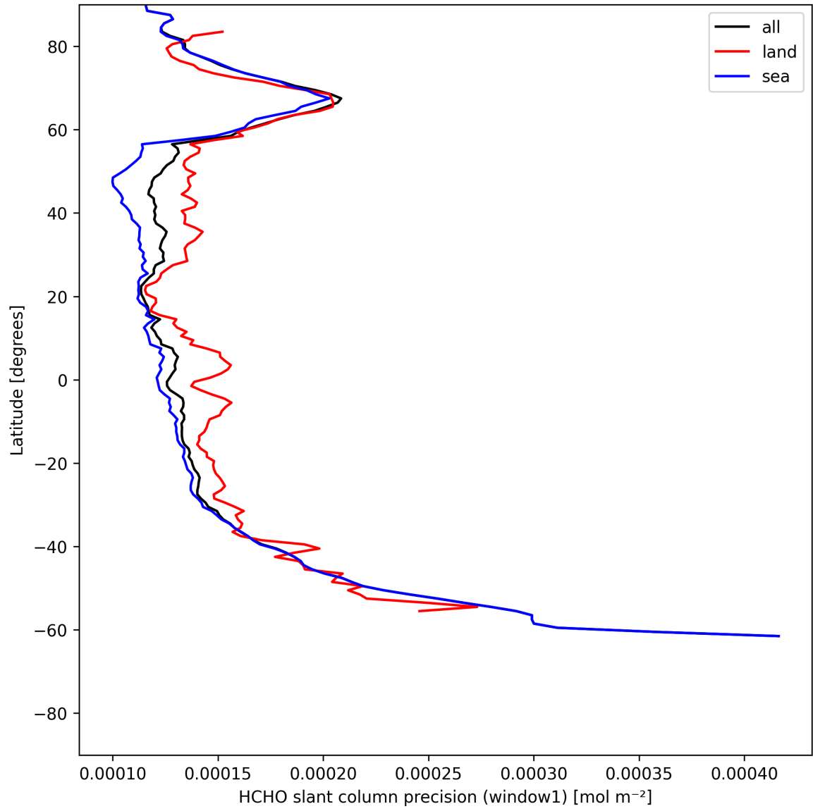
Figure 23: Zonal average of “HCHO slant column precision (window1)” for 2025-06-28 to 2025-06-29.
