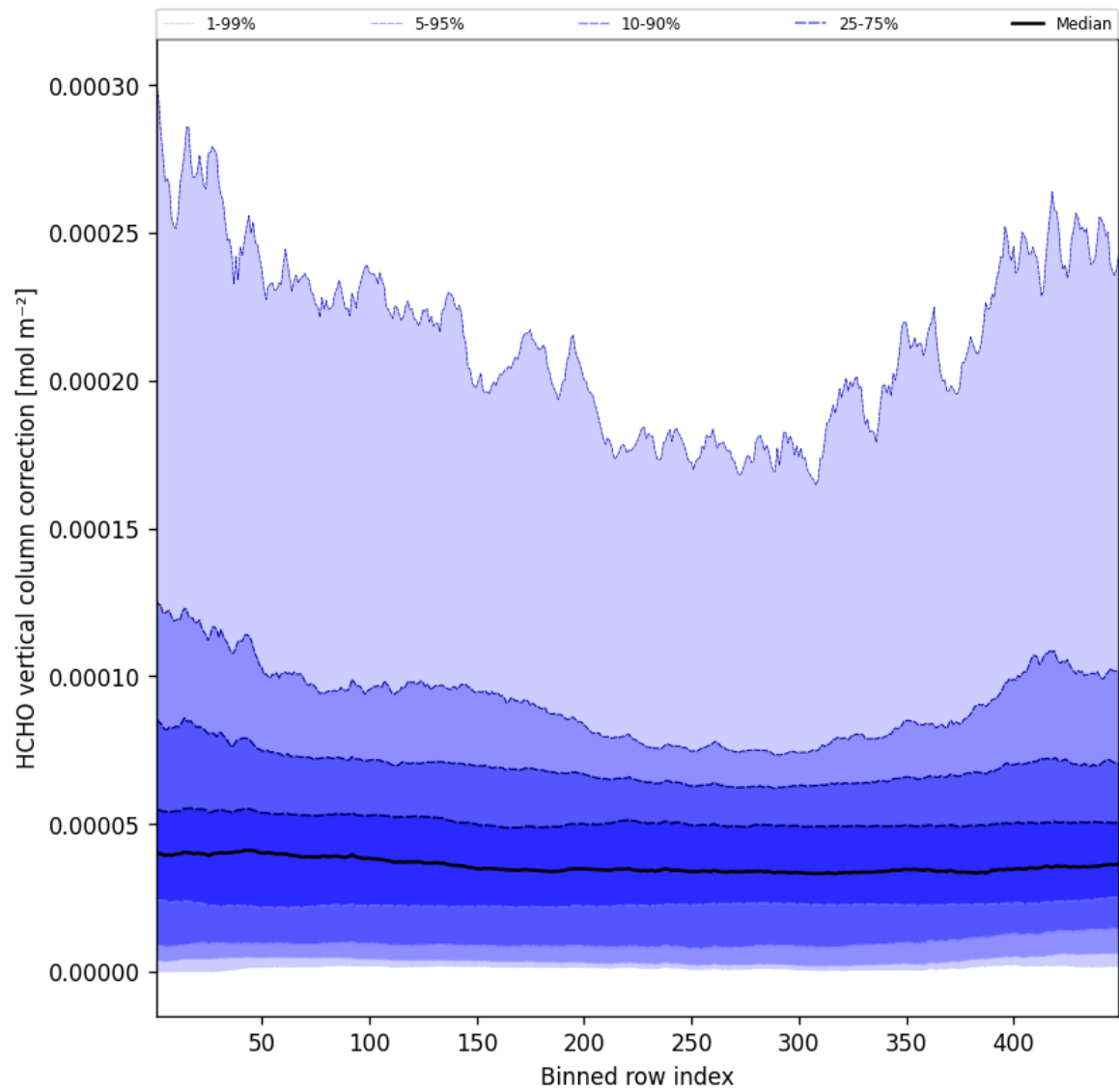
Figure 49: Along track statistics of “HCHO vertical column correction” for 2025-06-28 to 2025-06-29
