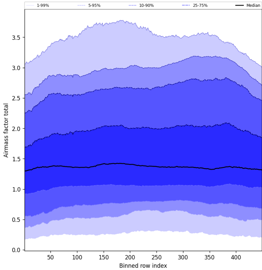
Figure 52: Along track statistics of “Airmass factor total” for 2025-06-28 to 2025-06-29
