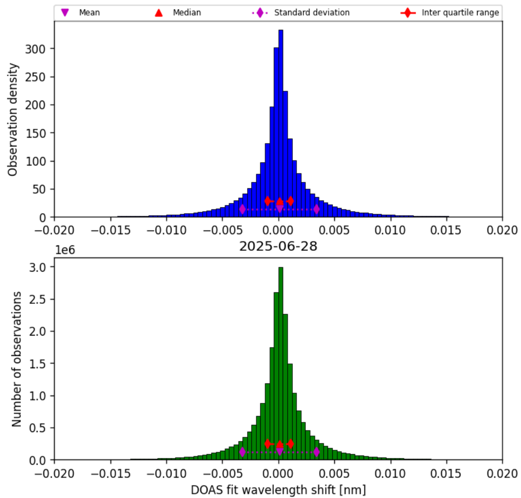
Figure 42: Histogram of “DOAS fit wavelength shift” for 2025-06-28 to 2025-06-29
