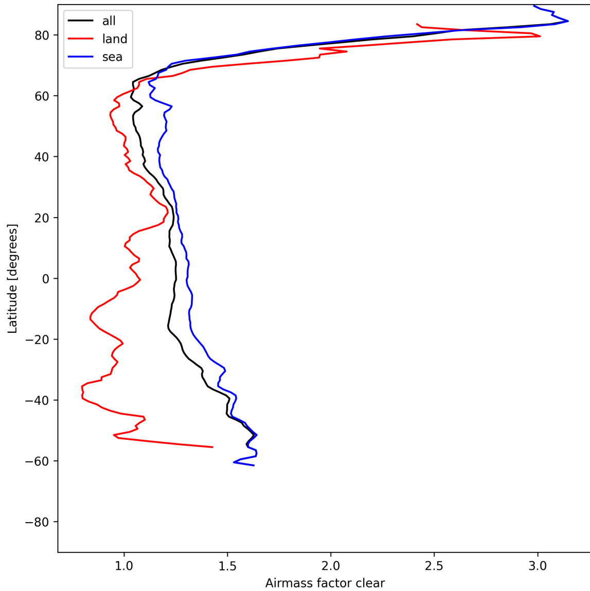
Figure 26: Zonal average of “Airmass factor clear” for 2025-06-28 to 2025-06-29.
