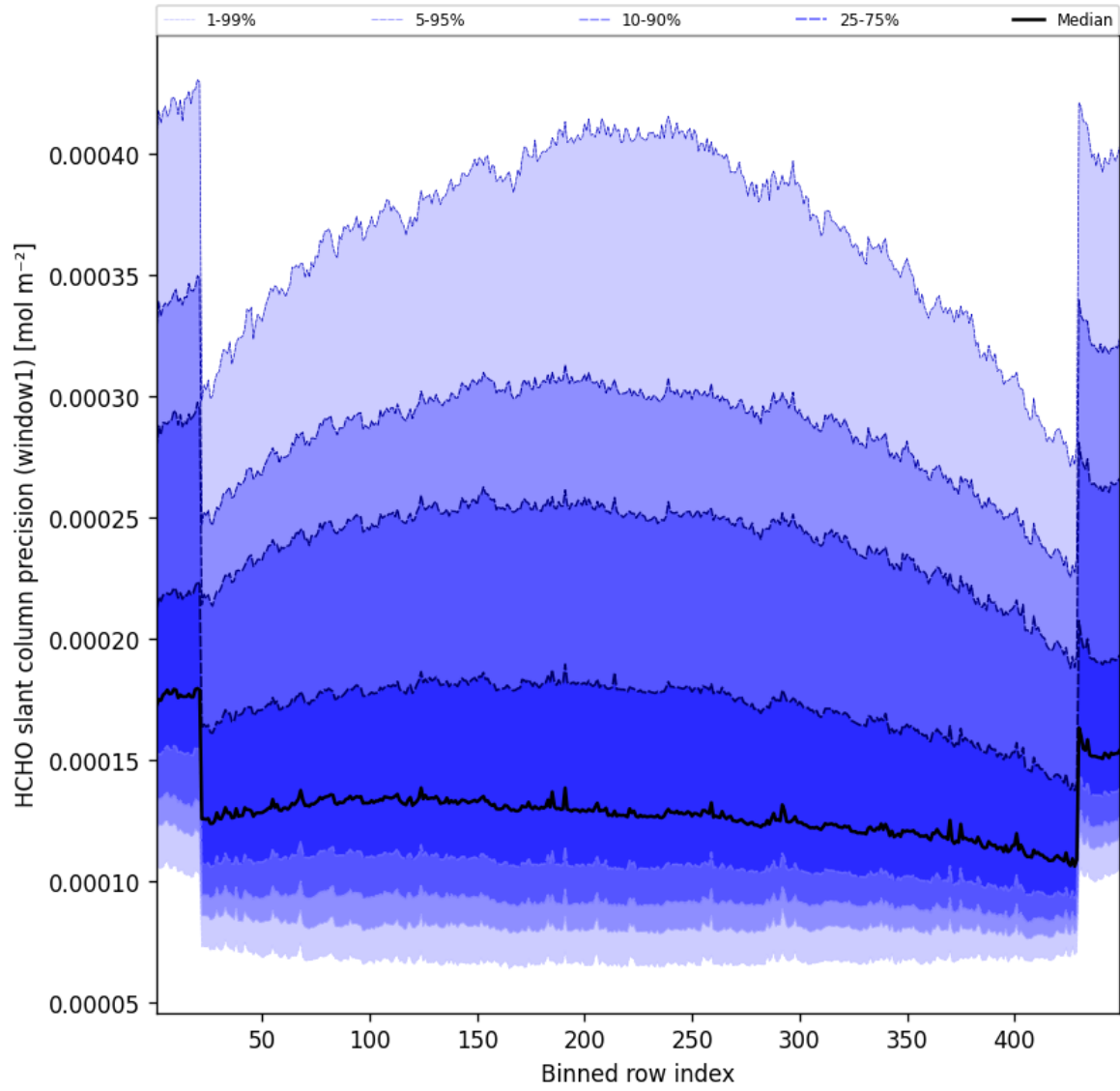
Figure 51: Along track statistics of “HCHO slant column precision (window1)” for 2025-06-28 to 2025-06-29
