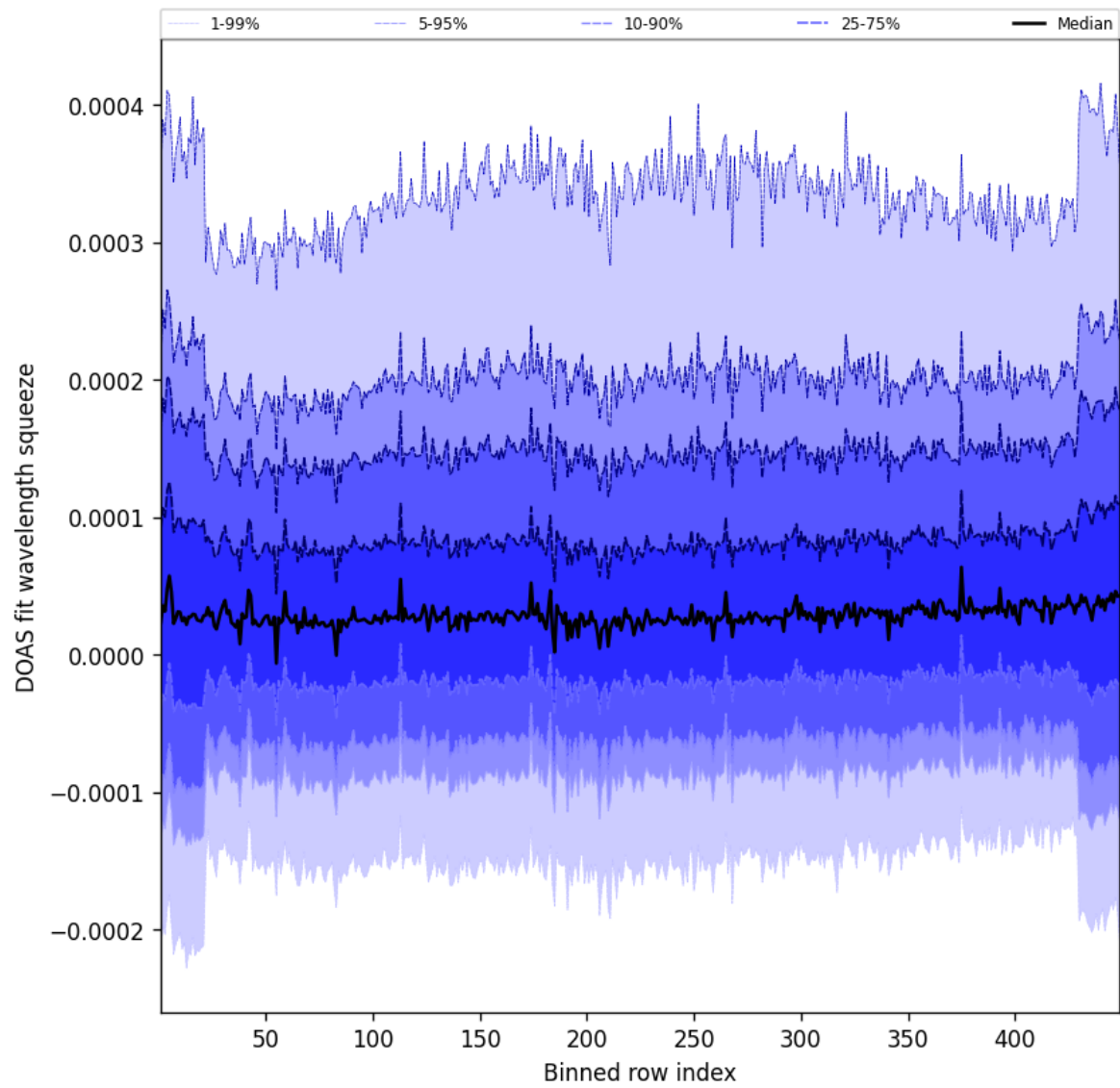
Figure 57: Along track statistics of “DOAS fit wavelength squeeze” for 2025-06-28 to 2025-06-29
