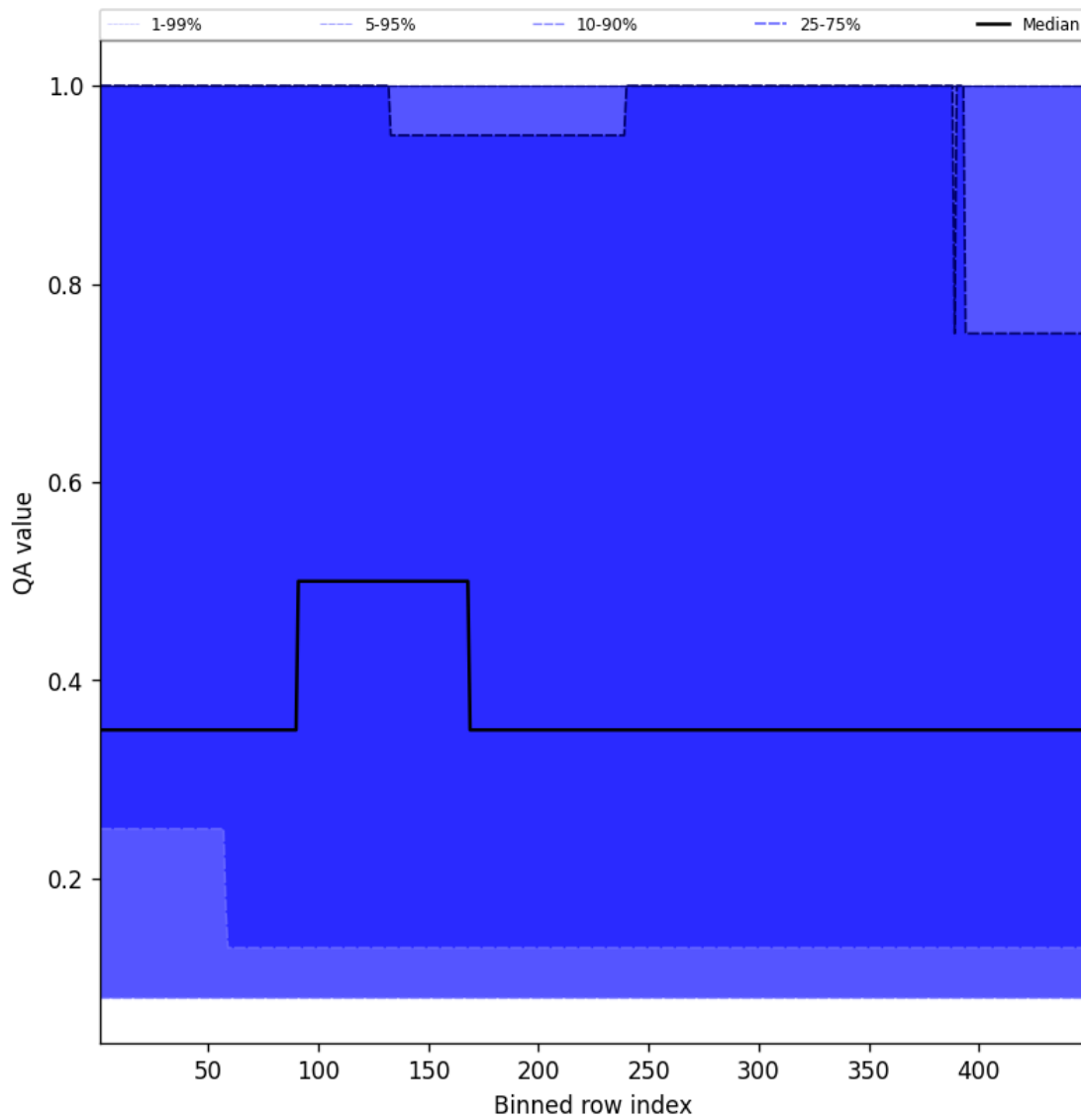
Figure 46: Along track statistics of “QA value” for 2025-06-28 to 2025-06-29
