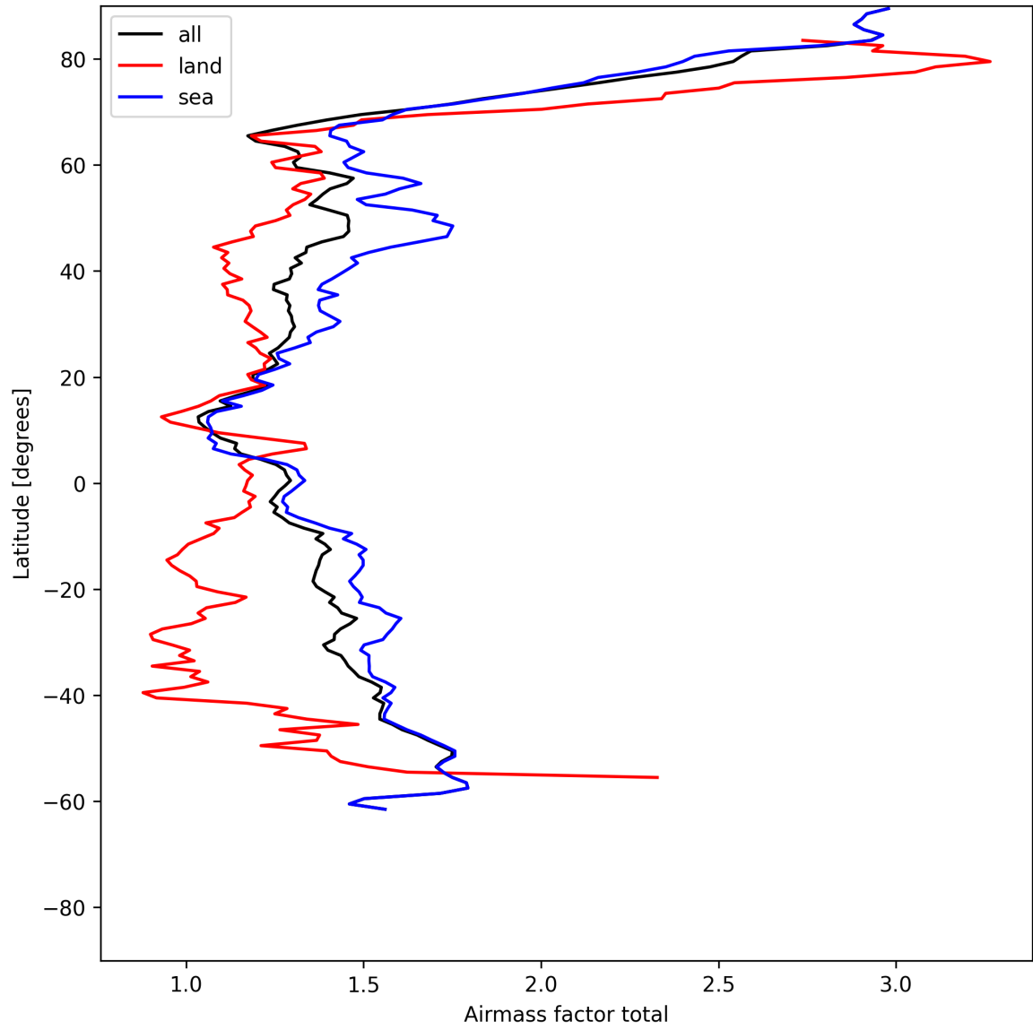
Figure 24: Zonal average of “Airmass factor total” for 2025-06-28 to 2025-06-29.
