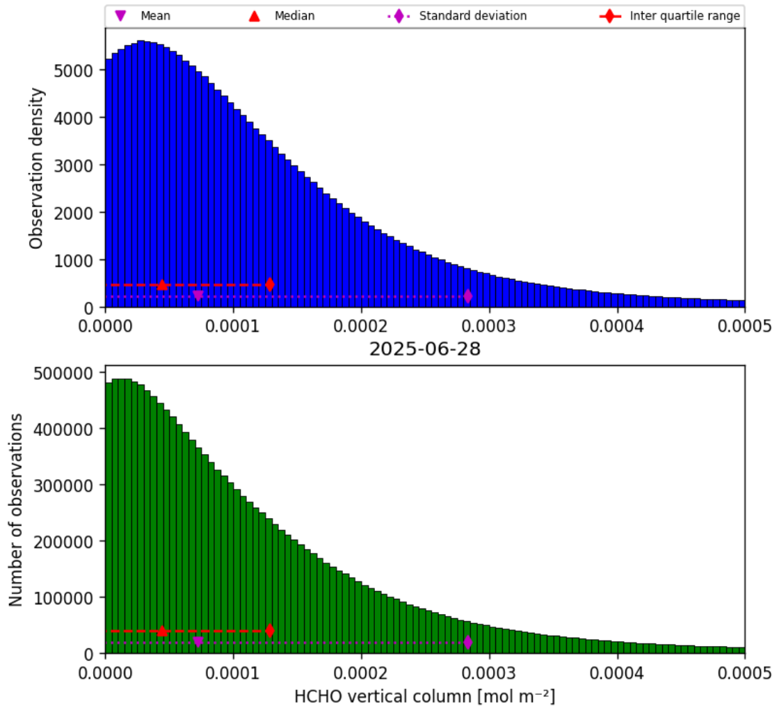
Figure 33: Histogram of “HCHO vertical column” for 2025-06-28 to 2025-06-29
