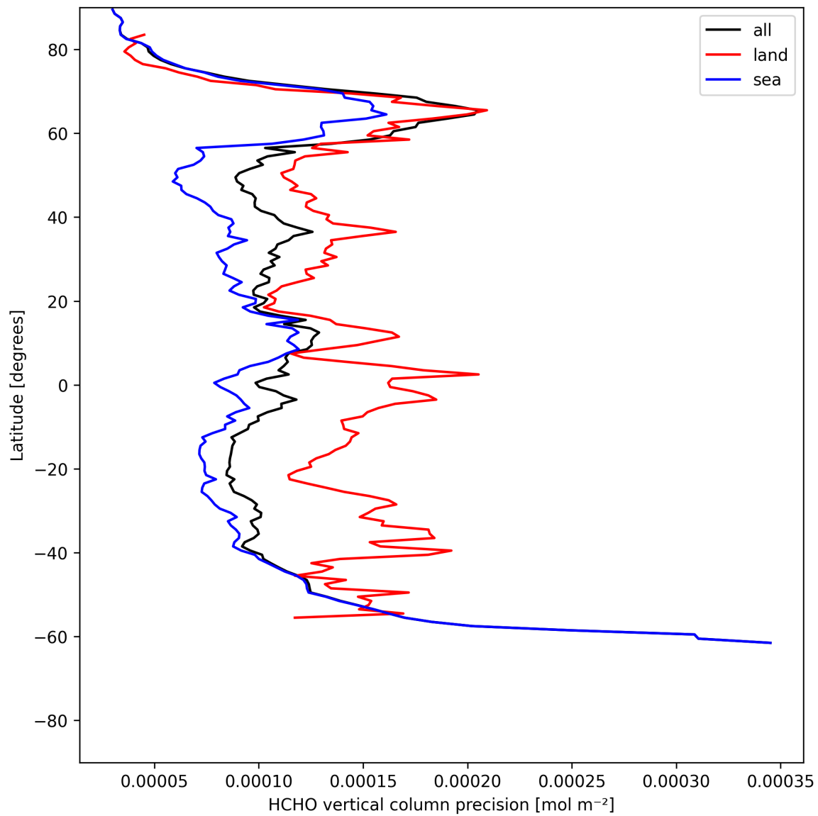
Figure 20: Zonal average of “HCHO vertical column precision” for 2025-06-28 to 2025-06-29.
