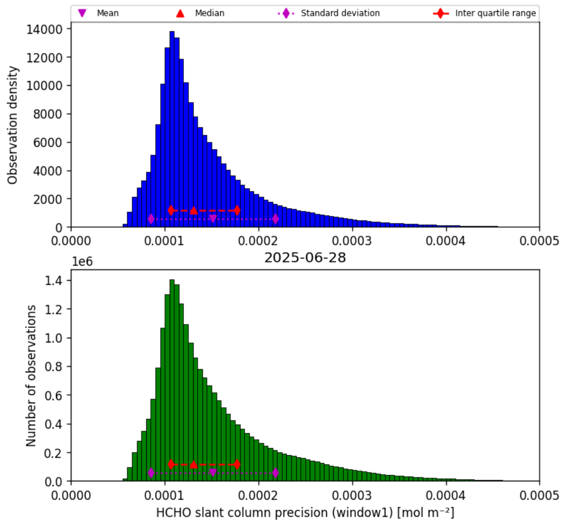
Figure 37: Histogram of “HCHO slant column precision (window1)” for 2025-06-28 to 2025-06-29
