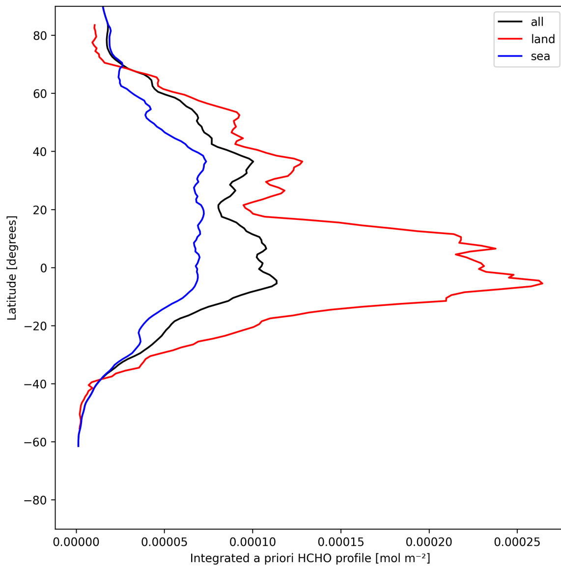
Figure 27: Zonal average of “Integrated a priori HCHO profile” for 2025-06-28 to 2025-06-29.
