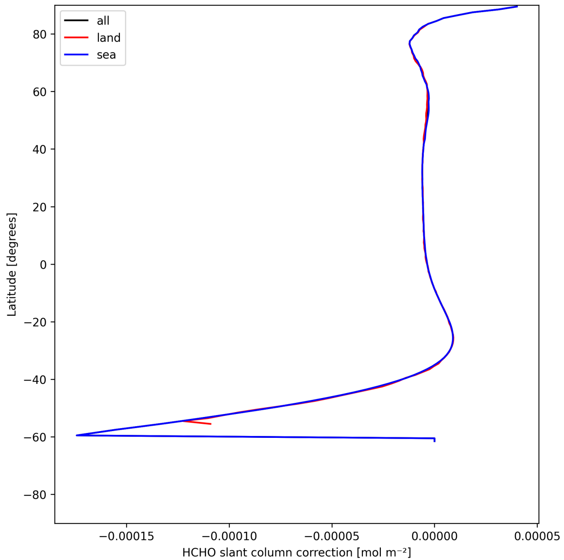
Figure 31: Zonal average of “HCHO slant column correction” for 2025-06-28 to 2025-06-29.
