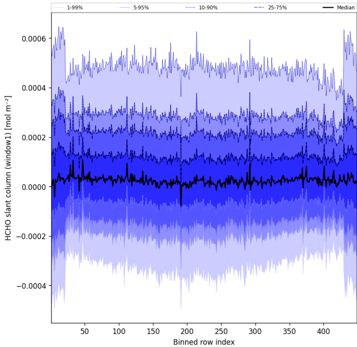
Figure 50: Along track statistics of “HCHO slant column (window1)” for 2025-06-28 to 2025-06-29
