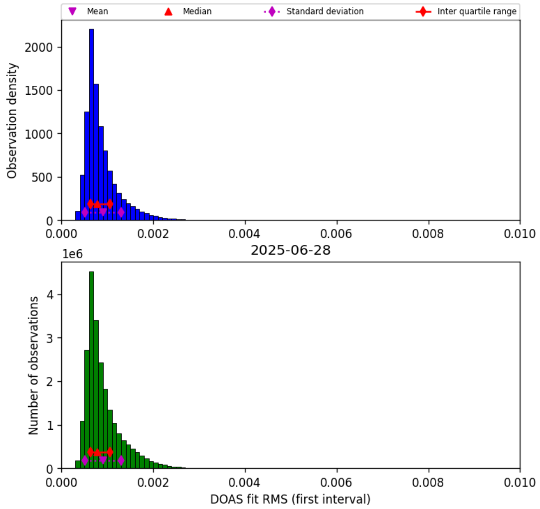
Figure 44: Histogram of “DOAS fit RMS (first interval)” for 2025-06-28 to 2025-06-29
