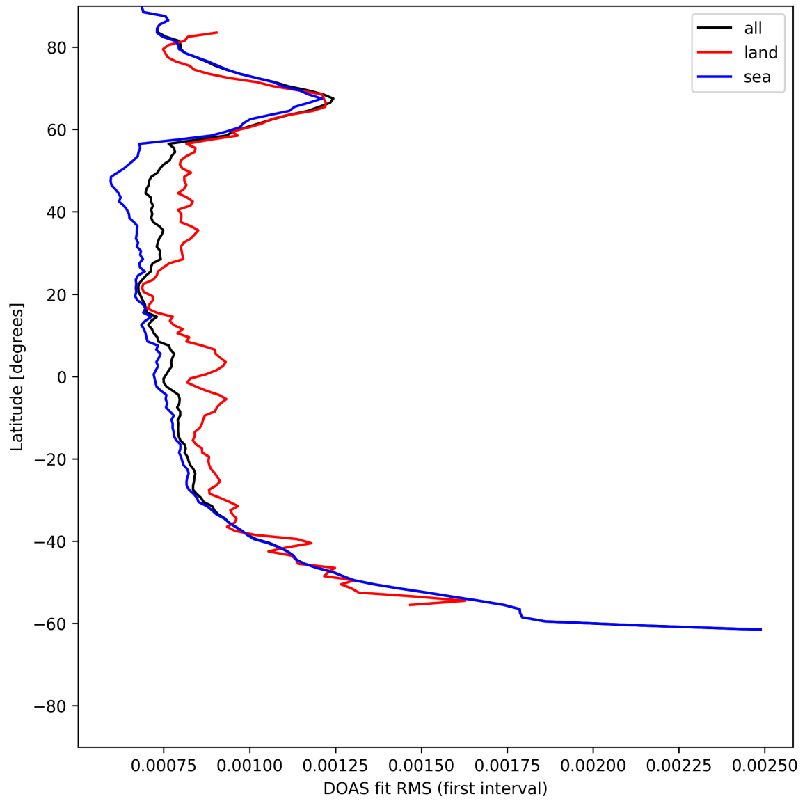
Figure 30: Zonal average of “DOAS fit RMS (first interval)” for 2025-06-28 to 2025-06-29.
