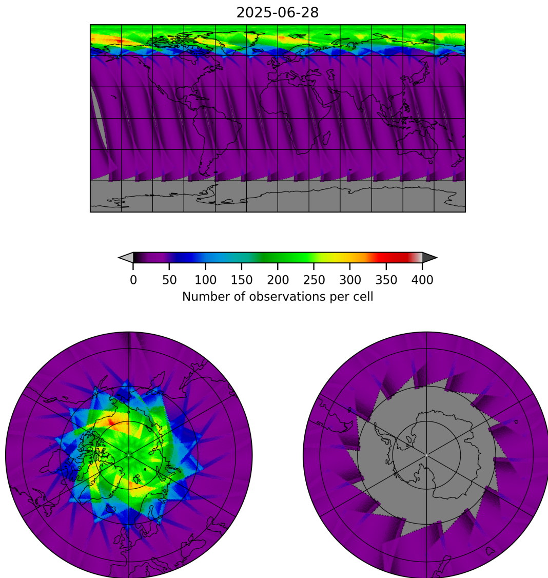
Figure 17: Map of the number of observations for 2025-06-28 to 2025-06-29
