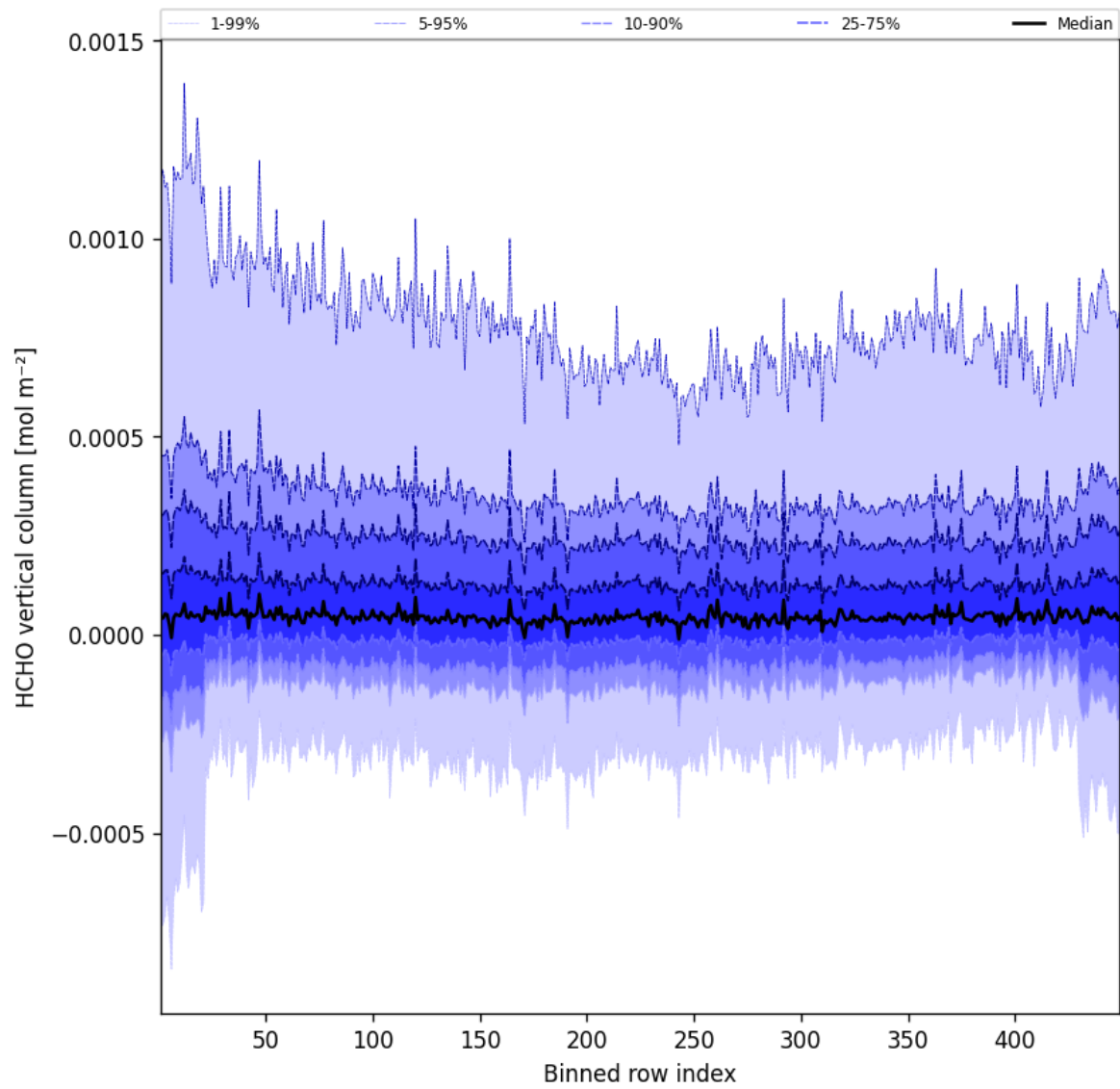
Figure 47: Along track statistics of “HCHO vertical column” for 2025-06-28 to 2025-06-29
