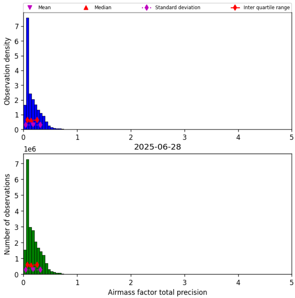
Figure 39: Histogram of “Airmass factor total precision” for 2025-06-28 to 2025-06-29
