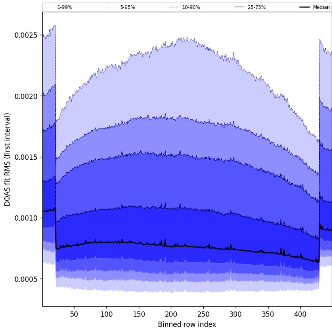
Figure 58: Along track statistics of “DOAS fit RMS (first interval)” for 2025-06-28 to 2025-06-29
