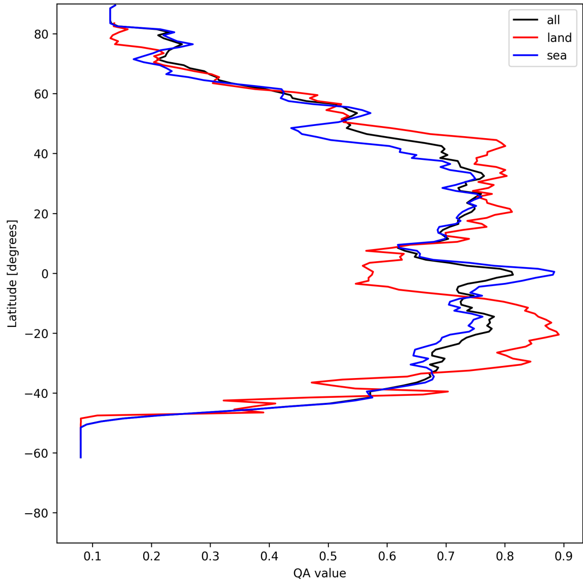
Figure 18: Zonal average of “QA value” for 2025-06-28 to 2025-06-29.
