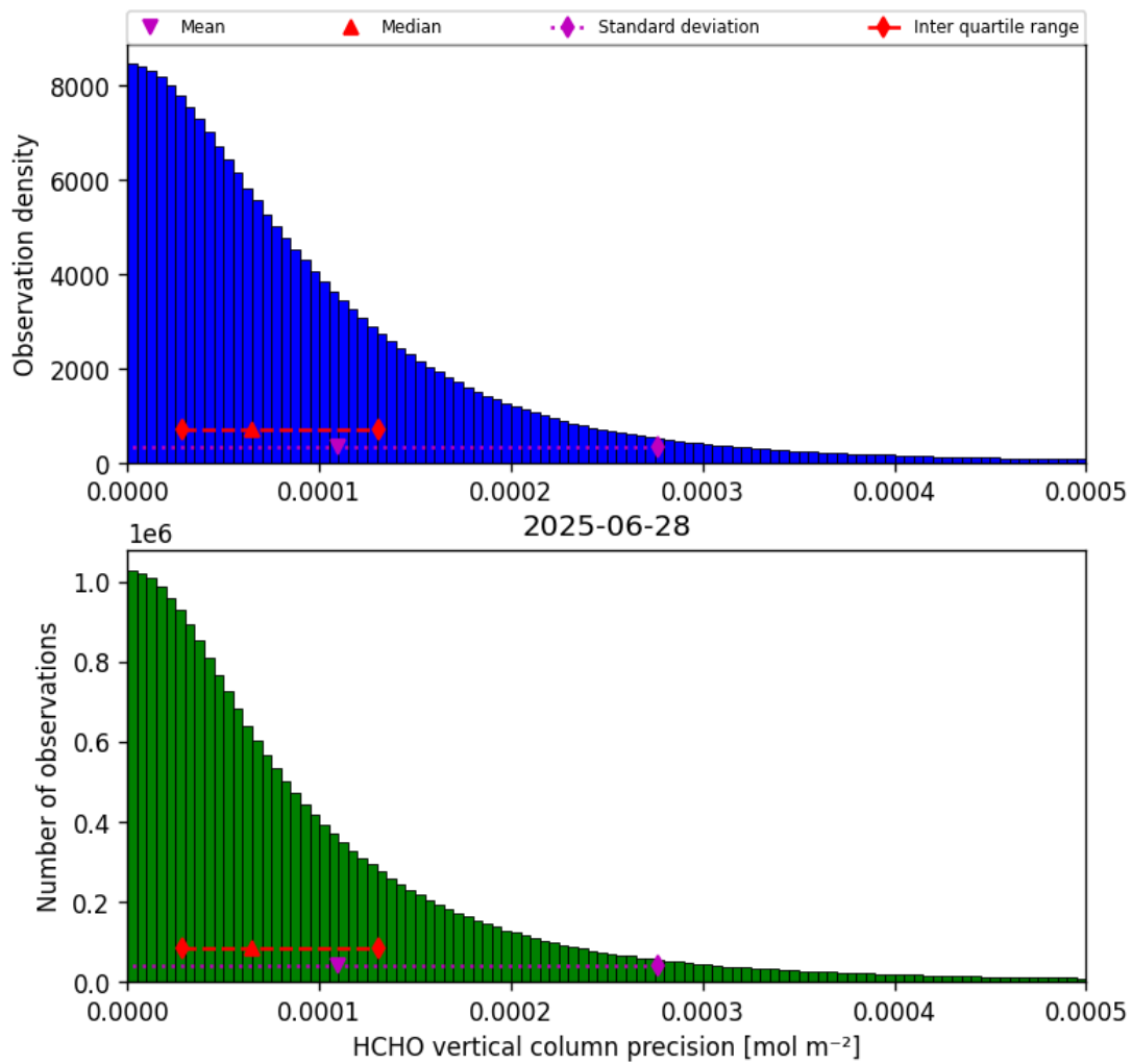
Figure 34: Histogram of “HCHO vertical column precision” for 2025-06-28 to 2025-06-29
