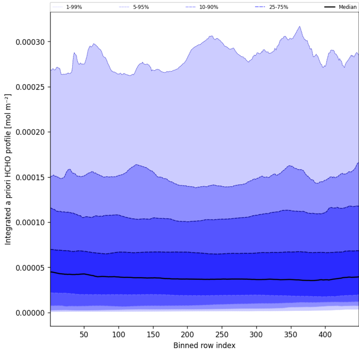
Figure 55: Along track statistics of "Integrated a priori HCHO profile" for 2025-06-28 to 2025-06-29
