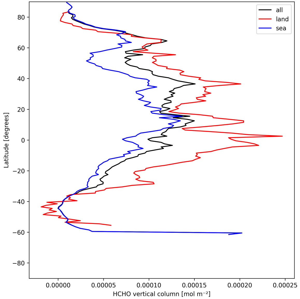
Figure 19: Zonal average of “HCHO vertical column” for 2025-06-28 to 2025-06-29.
