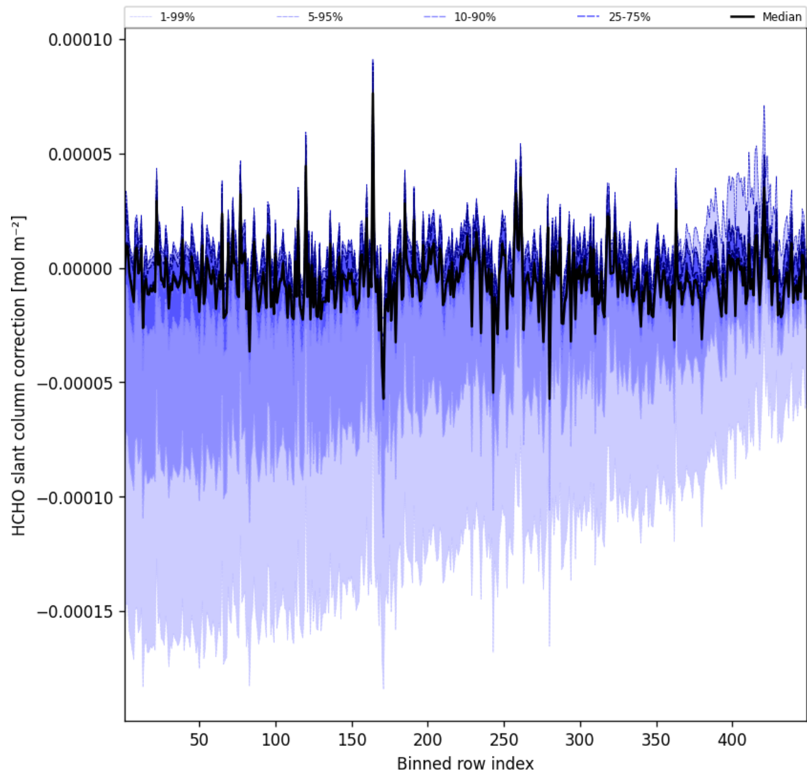
Figure 59: Along track statistics of “HCHO slant column correction” for 2025-06-28 to 2025-06-29
