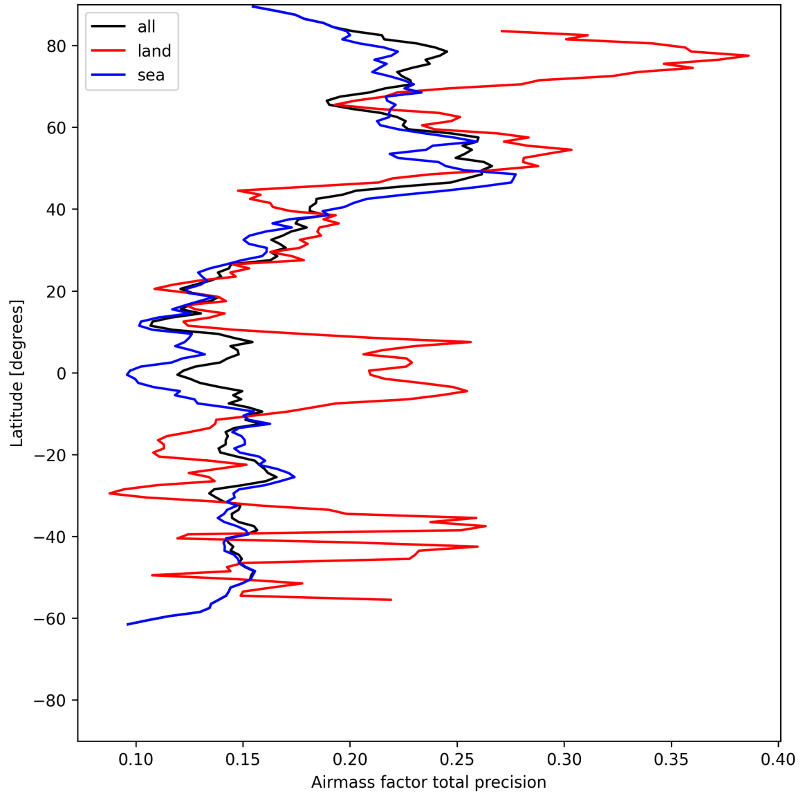
Figure 25: Zonal average of “Airmass factor total precision” for 2025-06-28 to 2025-06-29.
