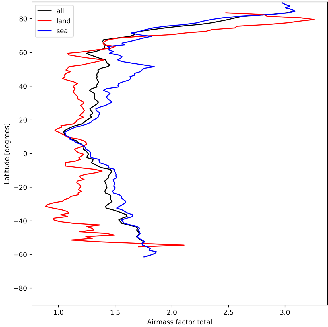
Figure 24: Zonal average of “Airmass factor total” for 2025-06-30 to 2025-06-30.
