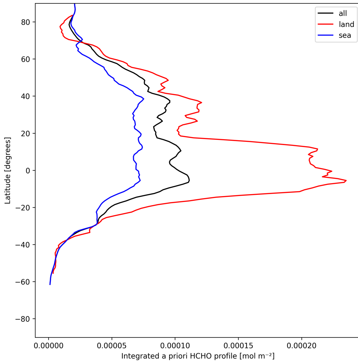
Figure 27: Zonal average of “Integrated a priori HCHO profile” for 2025-06-30 to 2025-06-30.
