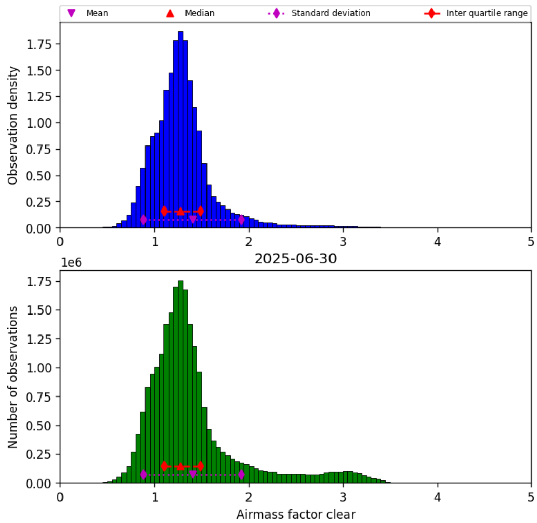
Figure 40: Histogram of “Airmass factor clear” for 2025-06-30 to 2025-06-30
