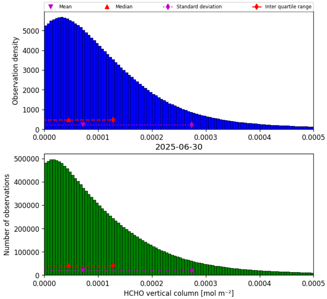
Figure 33: Histogram of “HCHO vertical column” for 2025-06-30 to 2025-06-30
