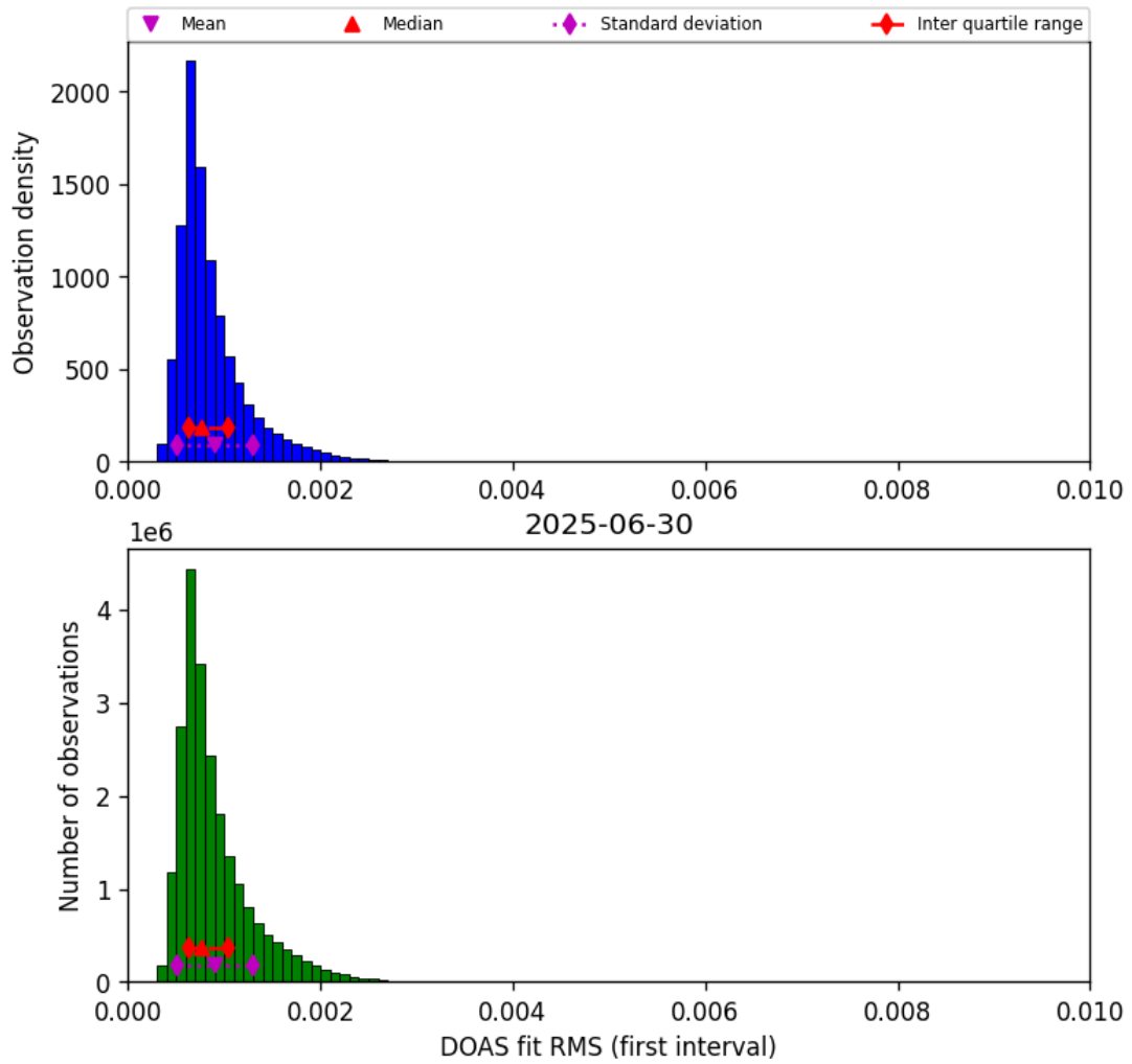
Figure 44: Histogram of “DOAS fit RMS (first interval)” for 2025-06-30 to 2025-06-30
