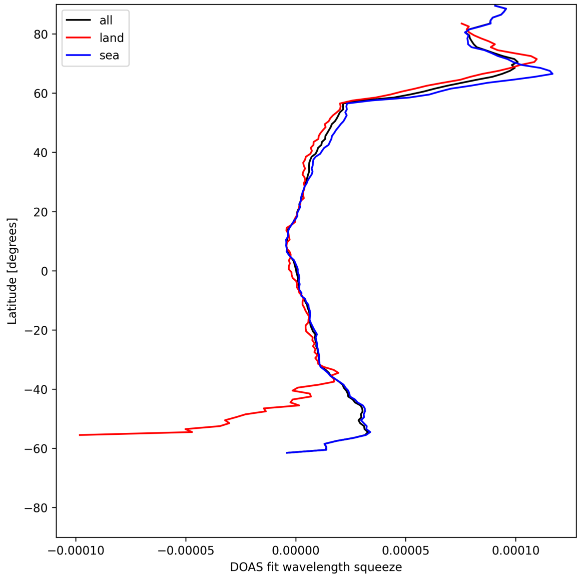
Figure 29: Zonal average of “DOAS fit wavelength squeeze” for 2025-06-30 to 2025-06-30.
