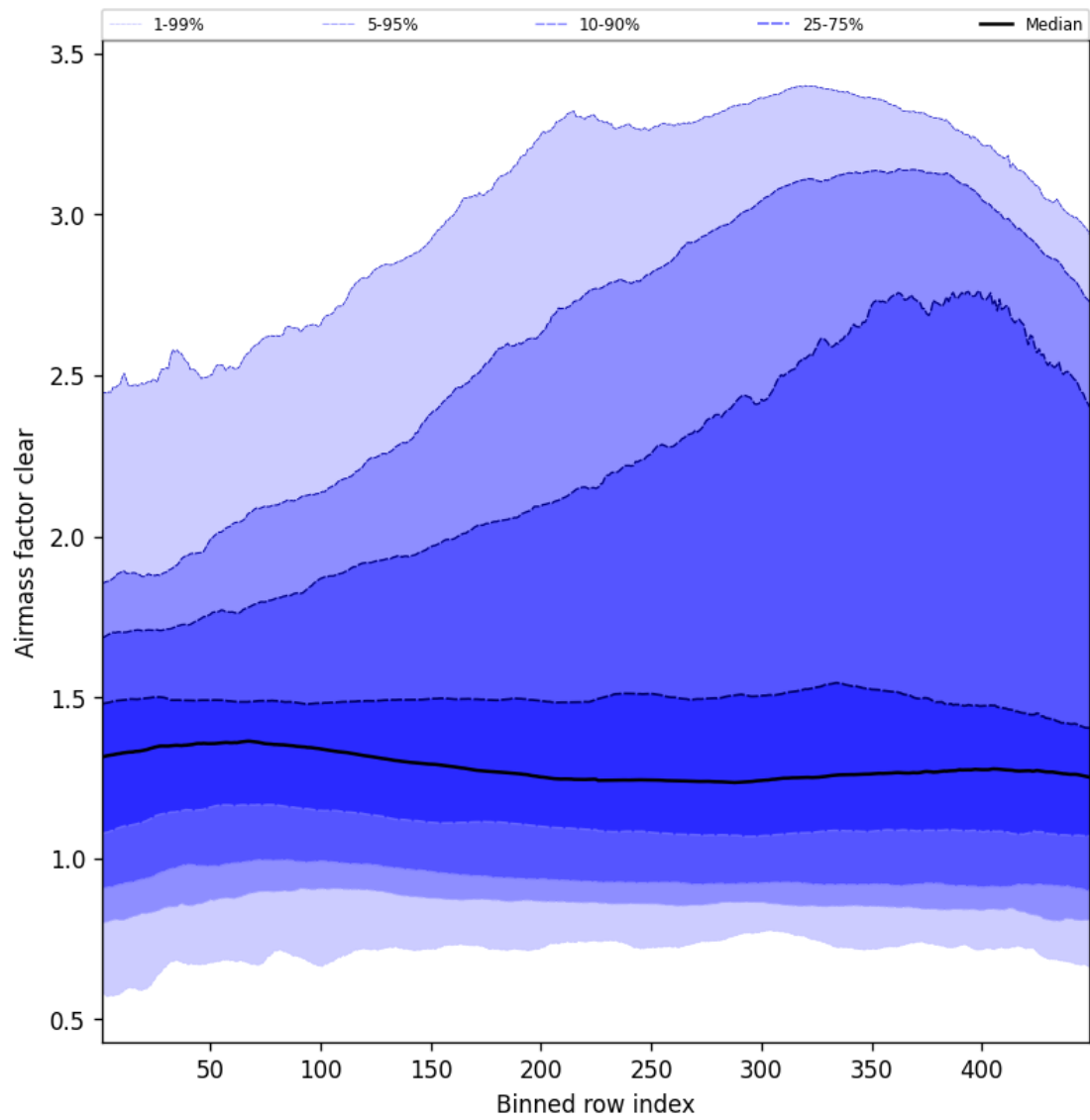
Figure 54: Along track statistics of “Airmass factor clear” for 2025-06-30 to 2025-06-30
