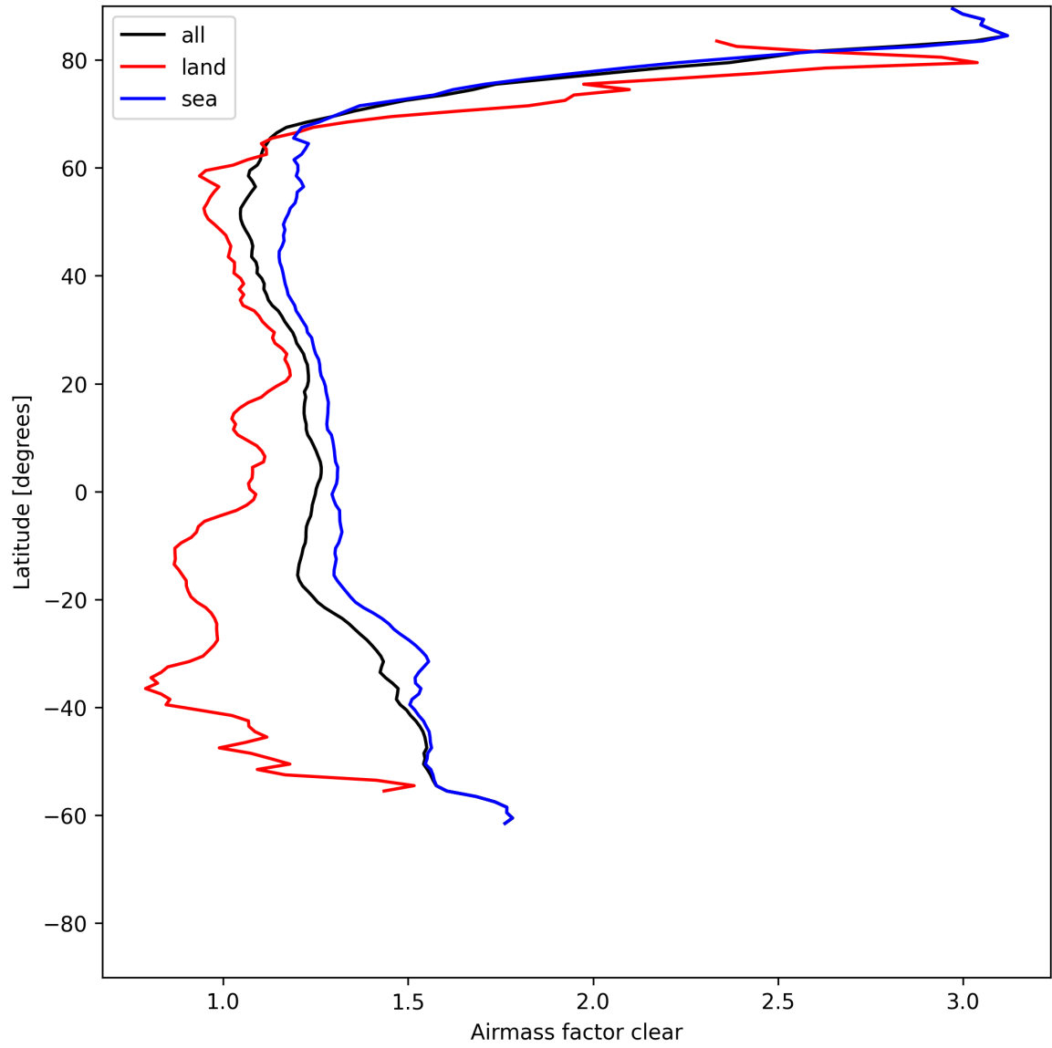
Figure 26: Zonal average of “Airmass factor clear” for 2025-06-30 to 2025-06-30.
