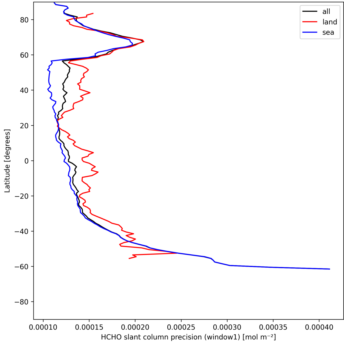
Figure 23: Zonal average of "HCHO slant column precision (window1)" for 2025-06-30 to 2025-06-30.
