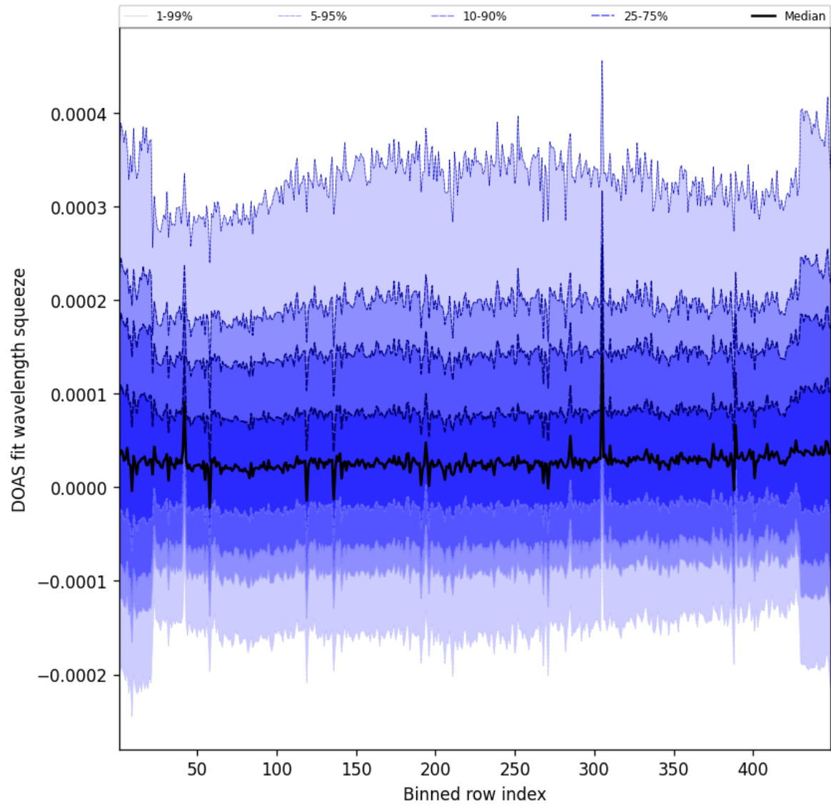
Figure 57: Along track statistics of “DOAS fit wavelength squeeze” for 2025-06-30 to 2025-06-30
