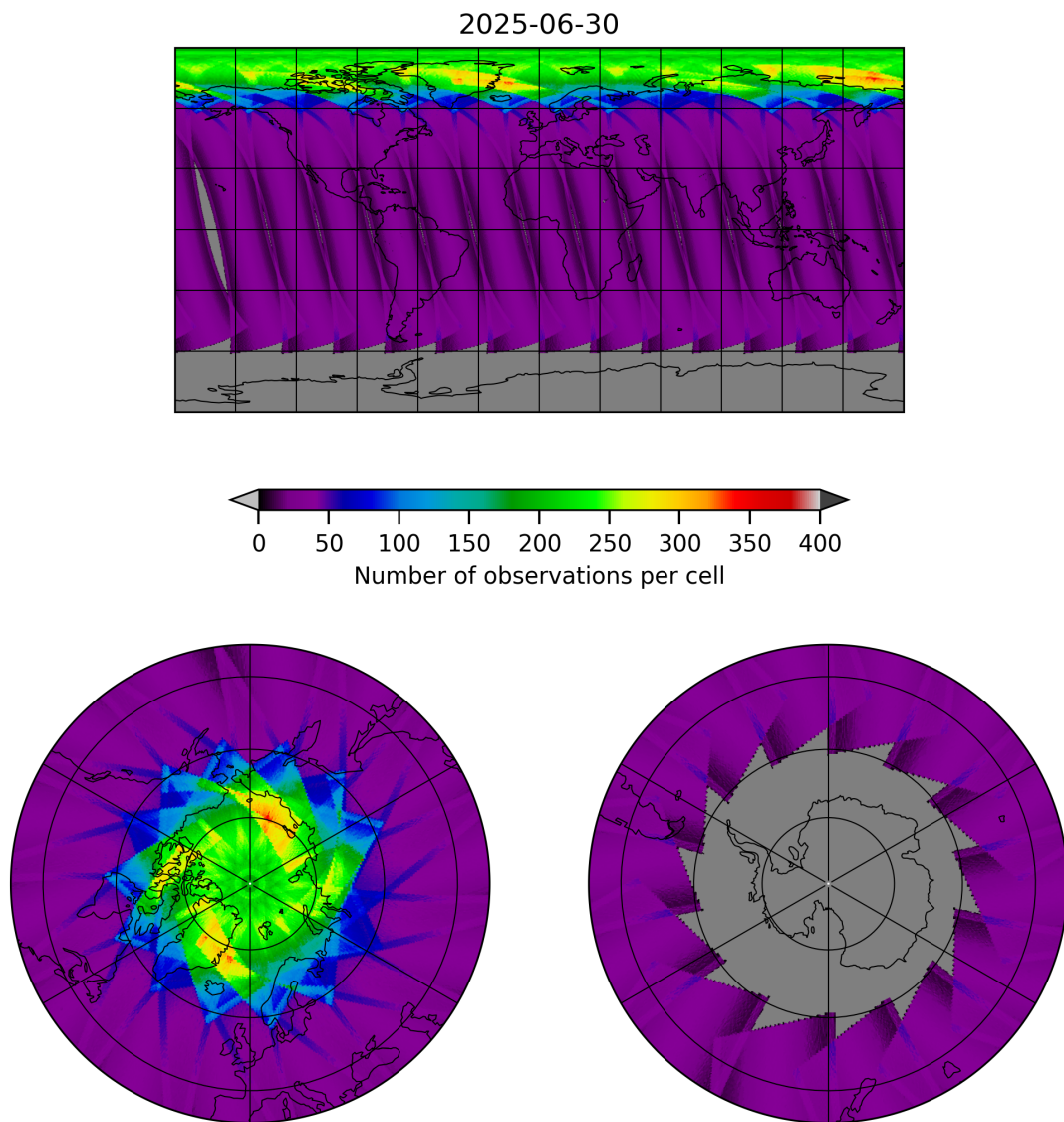
Figure 17: Map of the number of observations for 2025-06-30 to 2025-06-30
