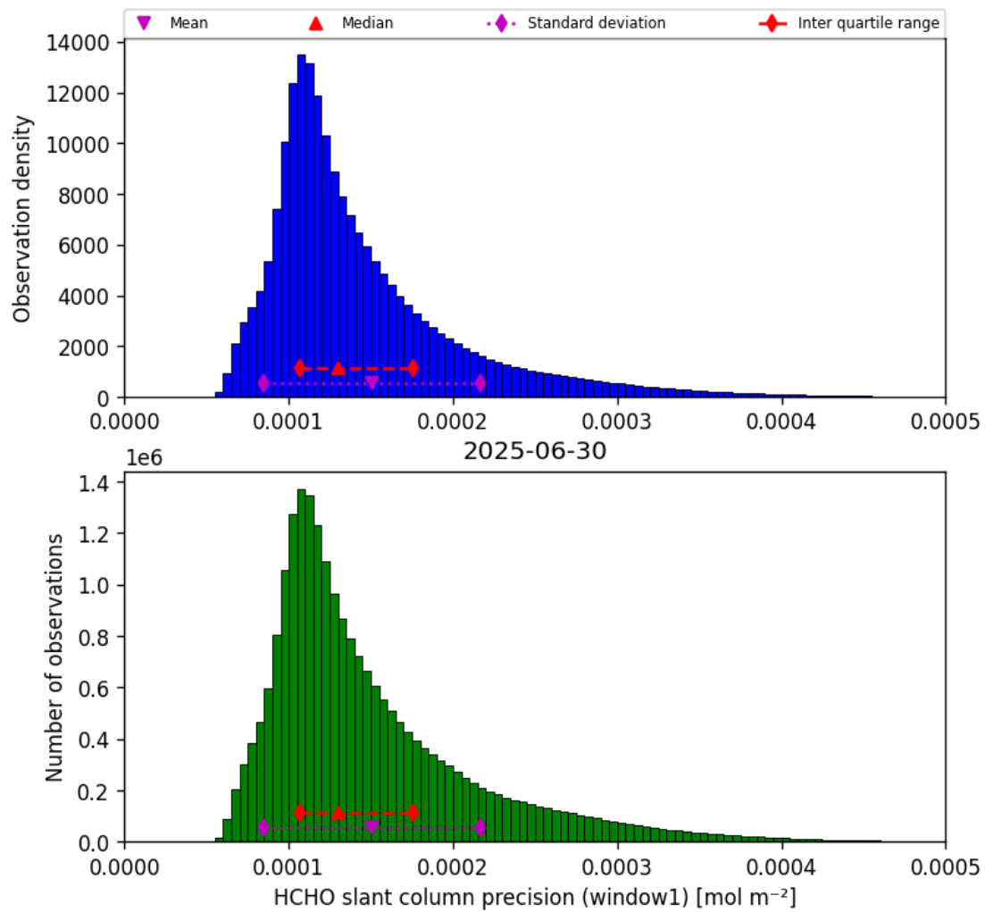
Figure 37: Histogram of “HCHO slant column precision (window1)” for 2025-06-30 to 2025-06-30
