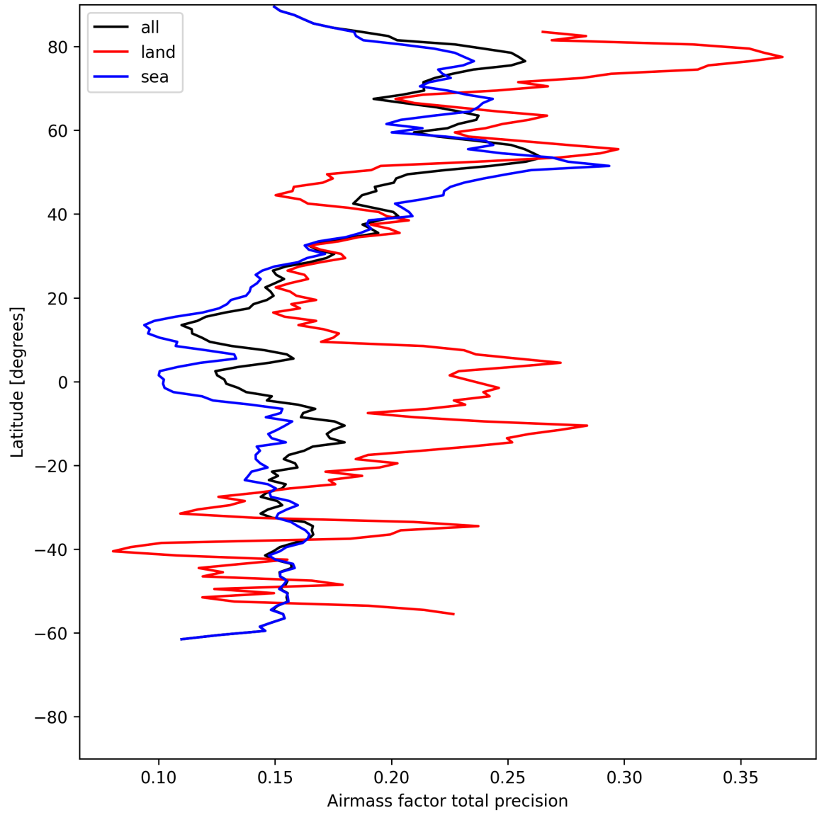
Figure 25: Zonal average of “Airmass factor total precision” for 2025-06-30 to 2025-06-30.
