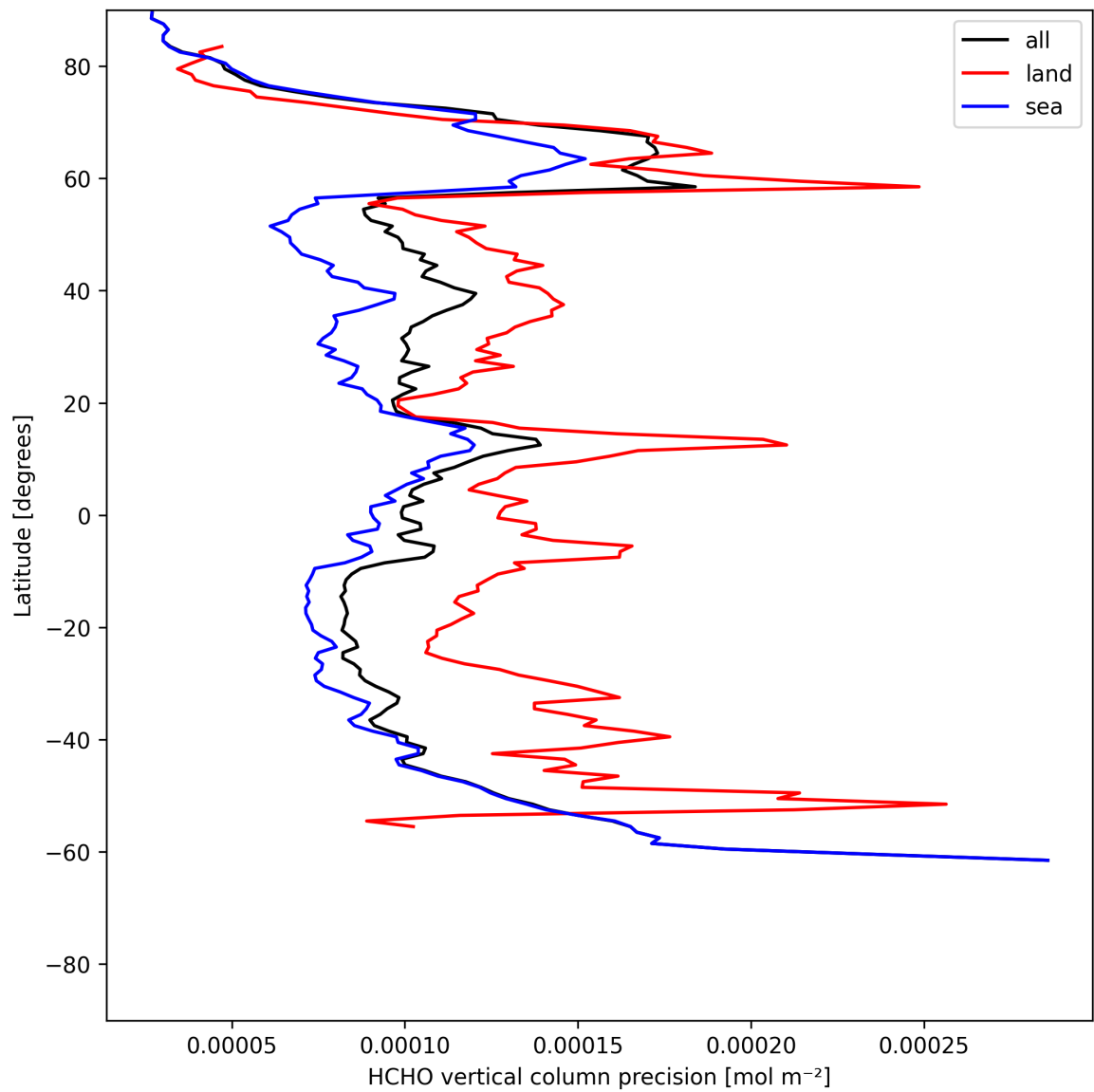
Figure 20: Zonal average of “HCHO vertical column precision” for 2025-06-30 to 2025-06-30.
