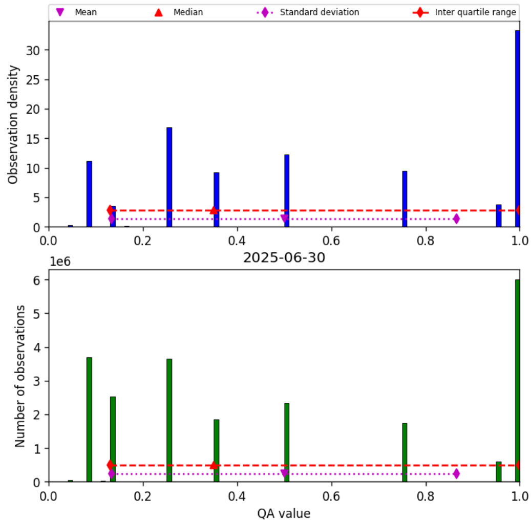
Figure 32: Histogram of “QA value” for 2025-06-30 to 2025-06-30
