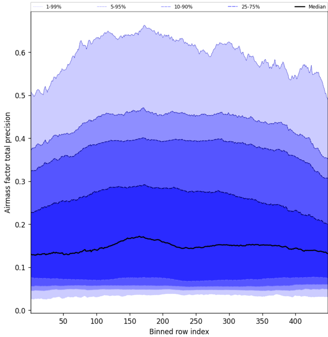
Figure 53: Along track statistics of “Airmass factor total precision” for 2025-06-30 to 2025-06-30
