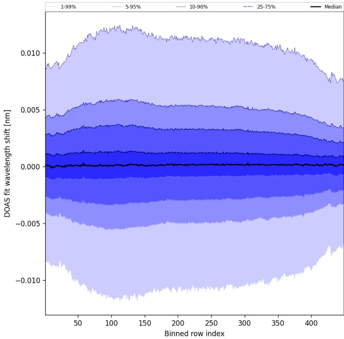
Figure 56: Along track statistics of “DOAS fit wavelength shift” for 2025-06-30 to 2025-06-30
