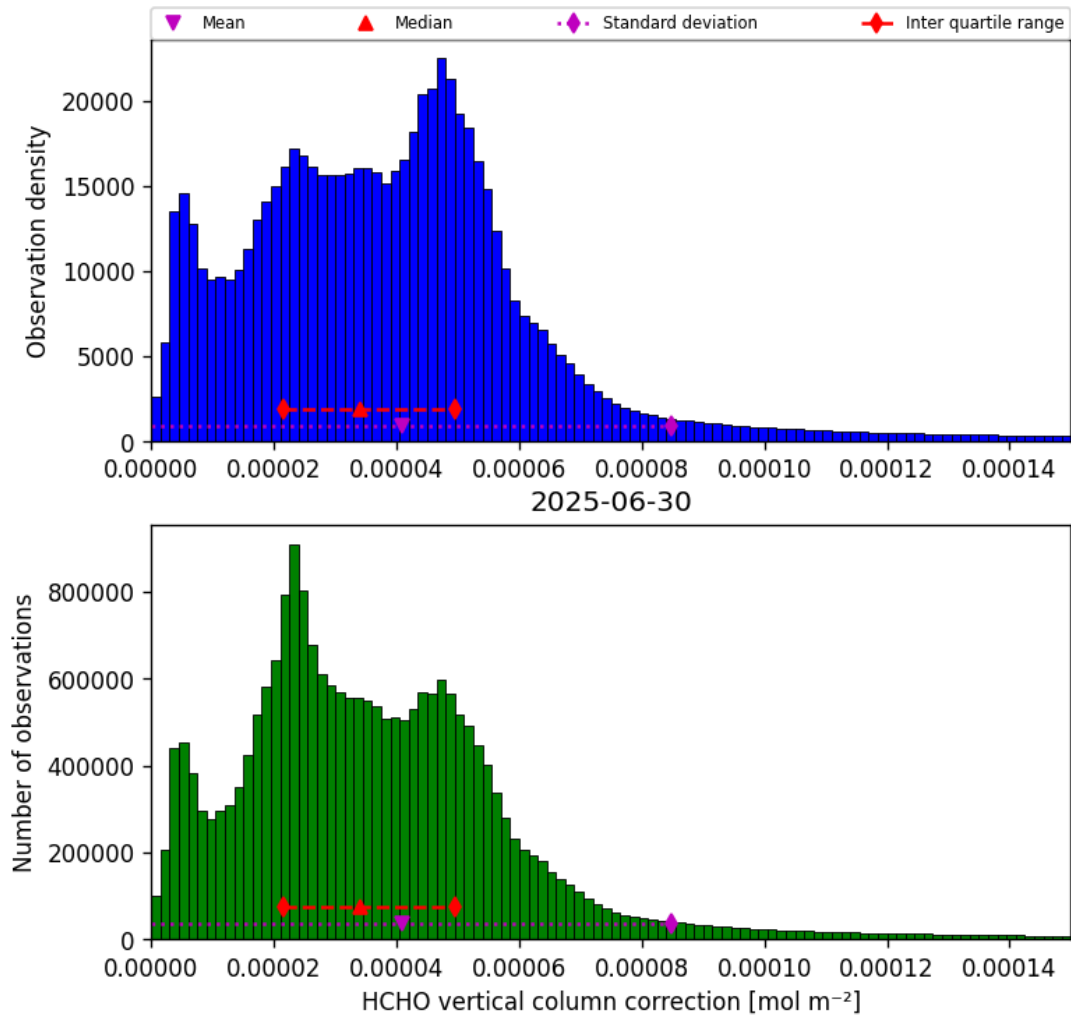
Figure 35: Histogram of “HCHO vertical column correction” for 2025-06-30 to 2025-06-30
