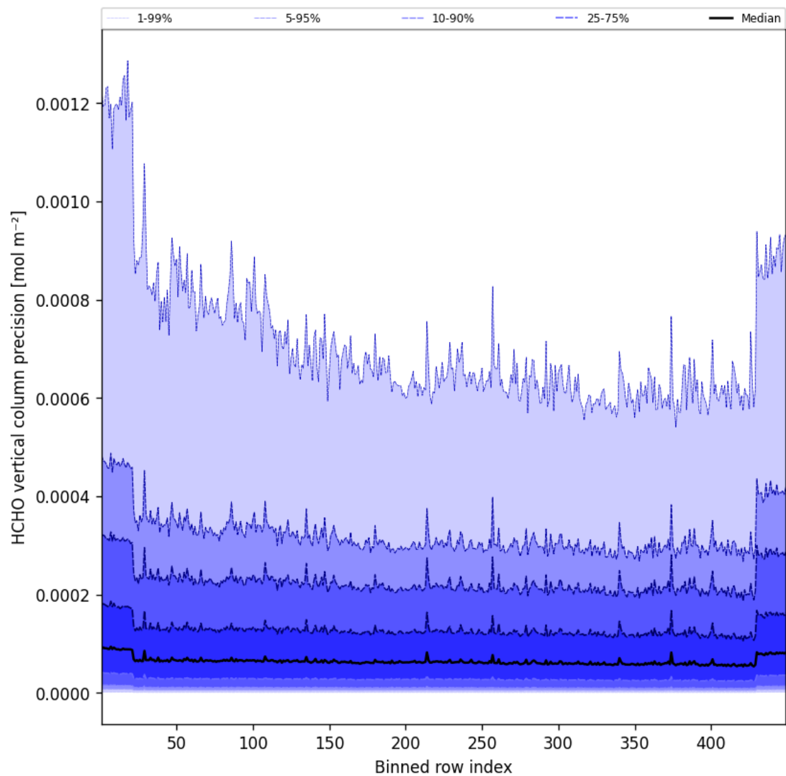
Figure 48: Along track statistics of “HCHO vertical column precision” for 2025-06-30 to 2025-06-30
