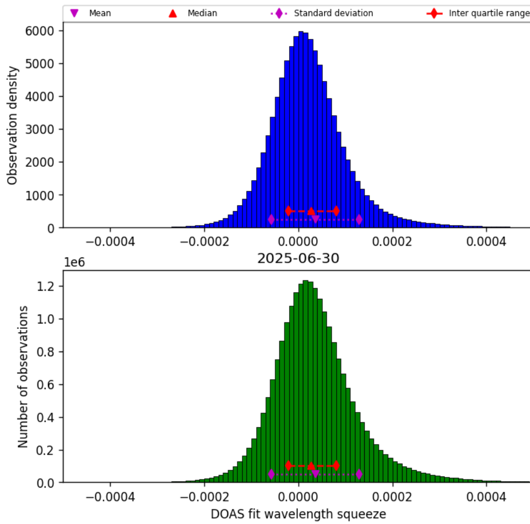
Figure 43: Histogram of “DOAS fit wavelength squeeze” for 2025-06-30 to 2025-06-30
