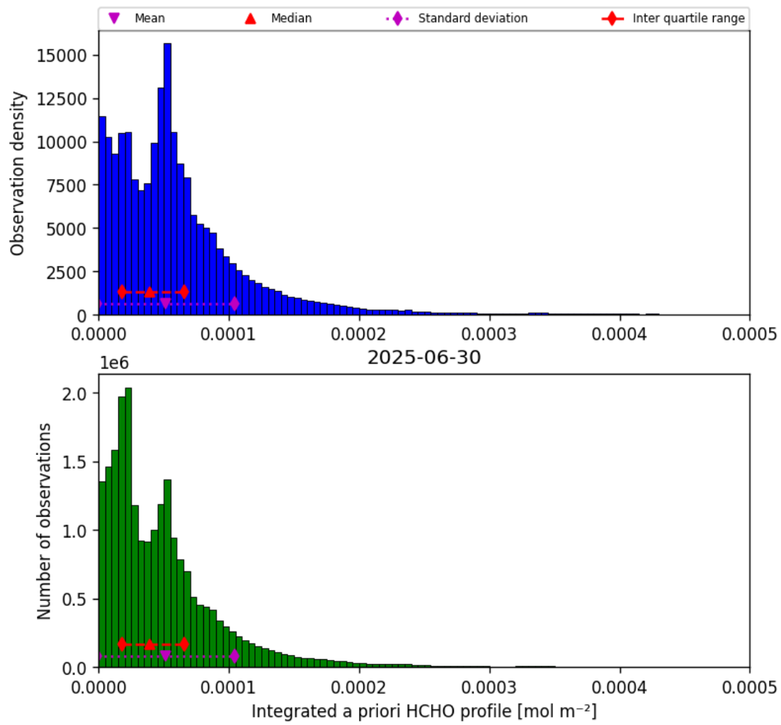
Figure 41: Histogram of “Integrated a priori HCHO profile” for 2025-06-30 to 2025-06-30
