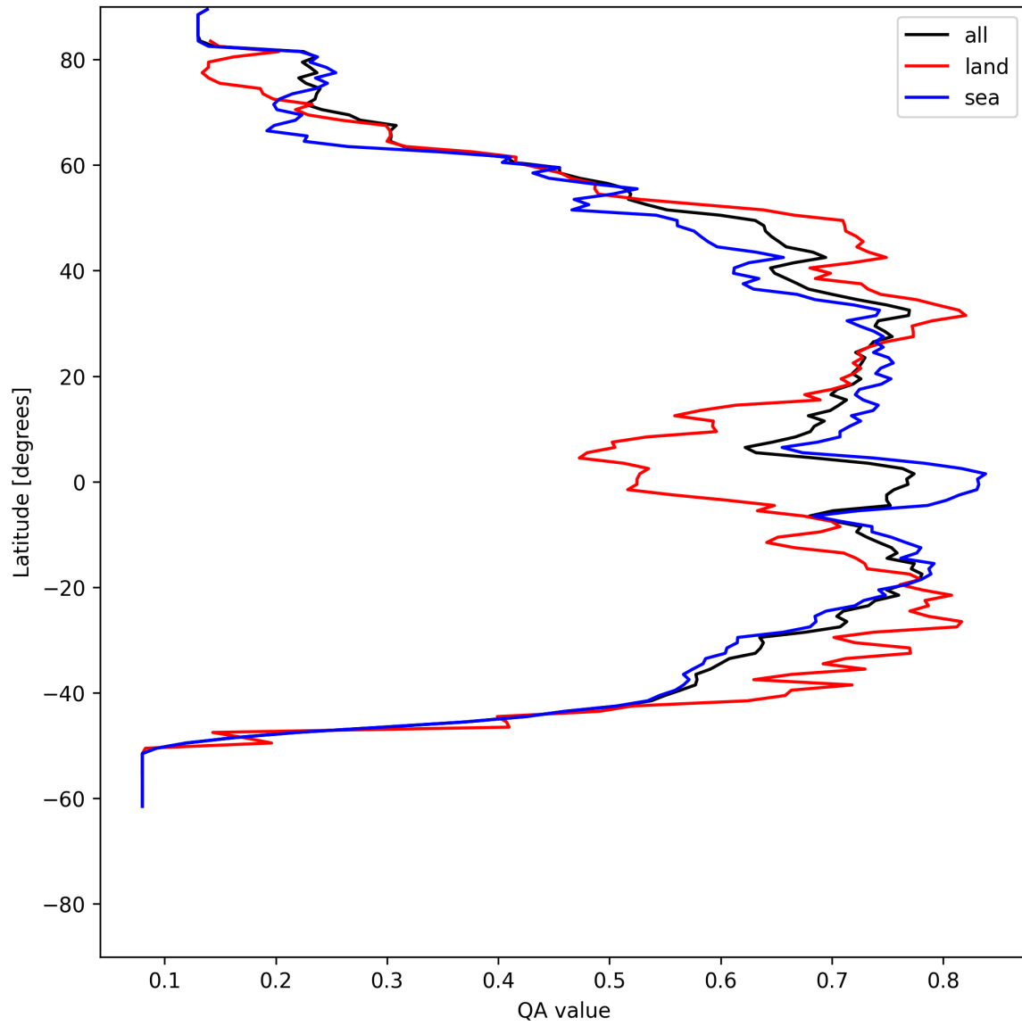
Figure 18: Zonal average of “QA value” for 2025-06-30 to 2025-06-30.
