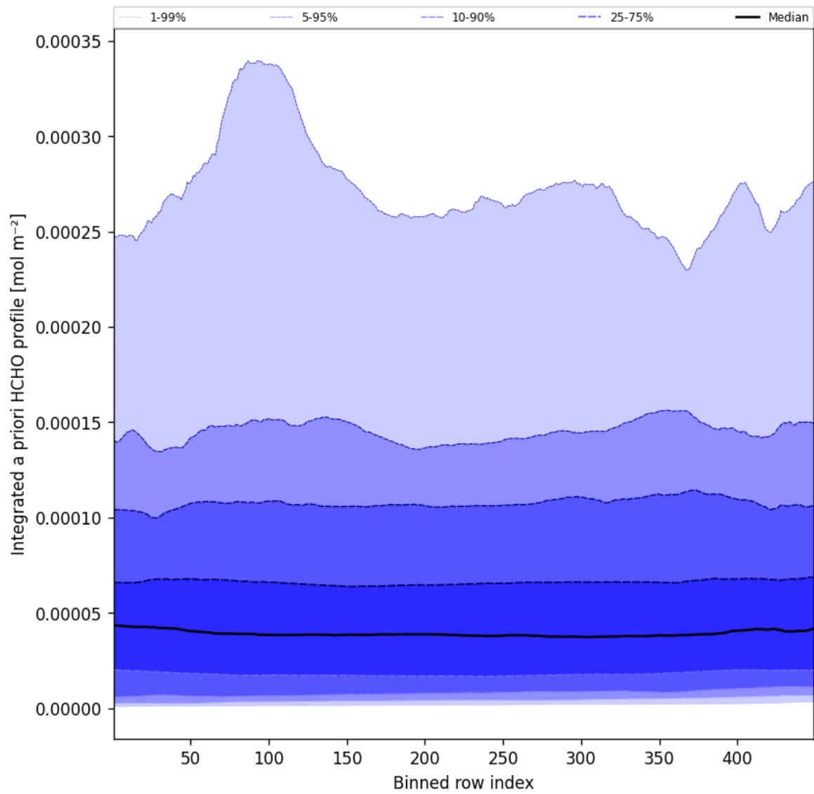
Figure 55: Along track statistics of “Integrated a priori HCHO profile” for 2025-06-30 to 2025-06-30
