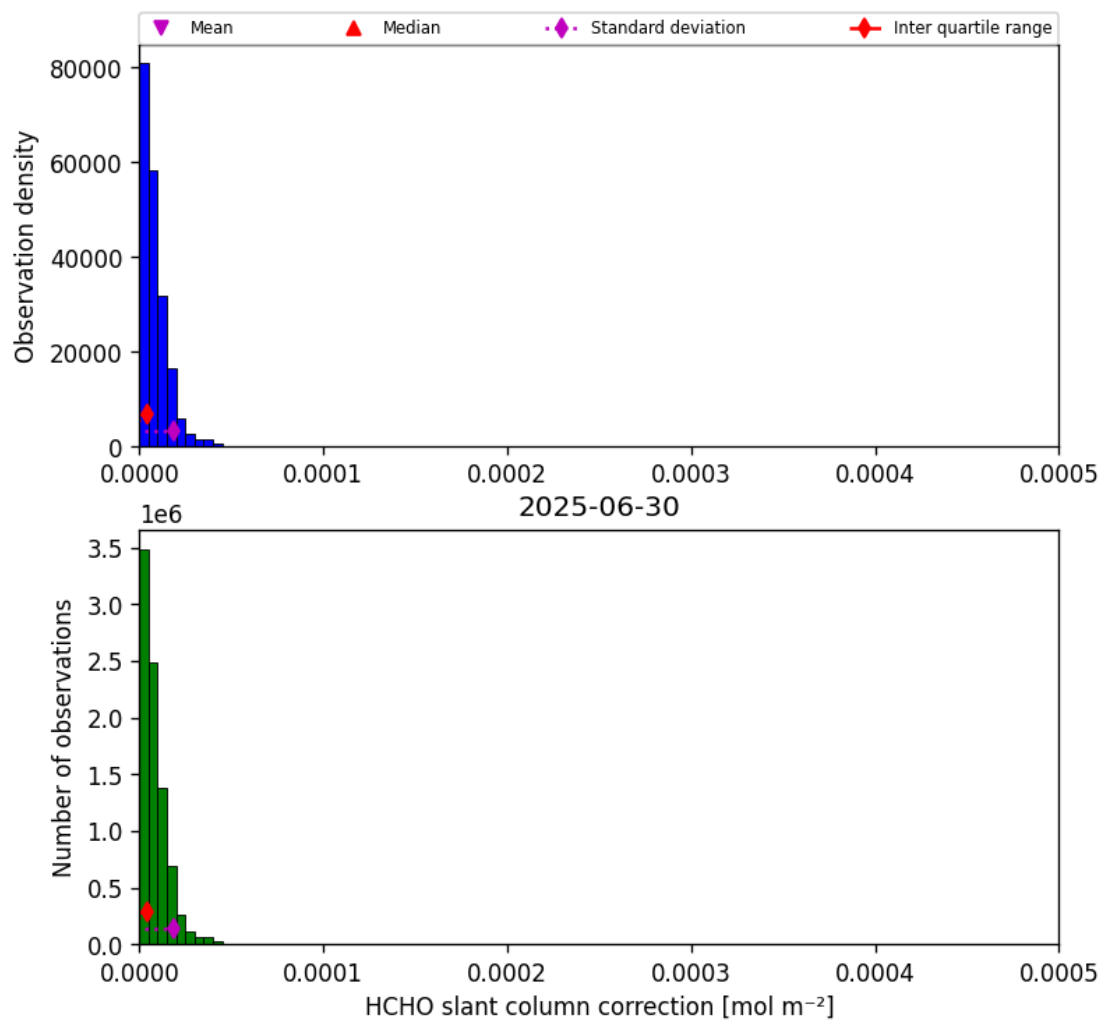
Figure 45: Histogram of “HCHO slant column correction” for 2025-06-30 to 2025-06-30
