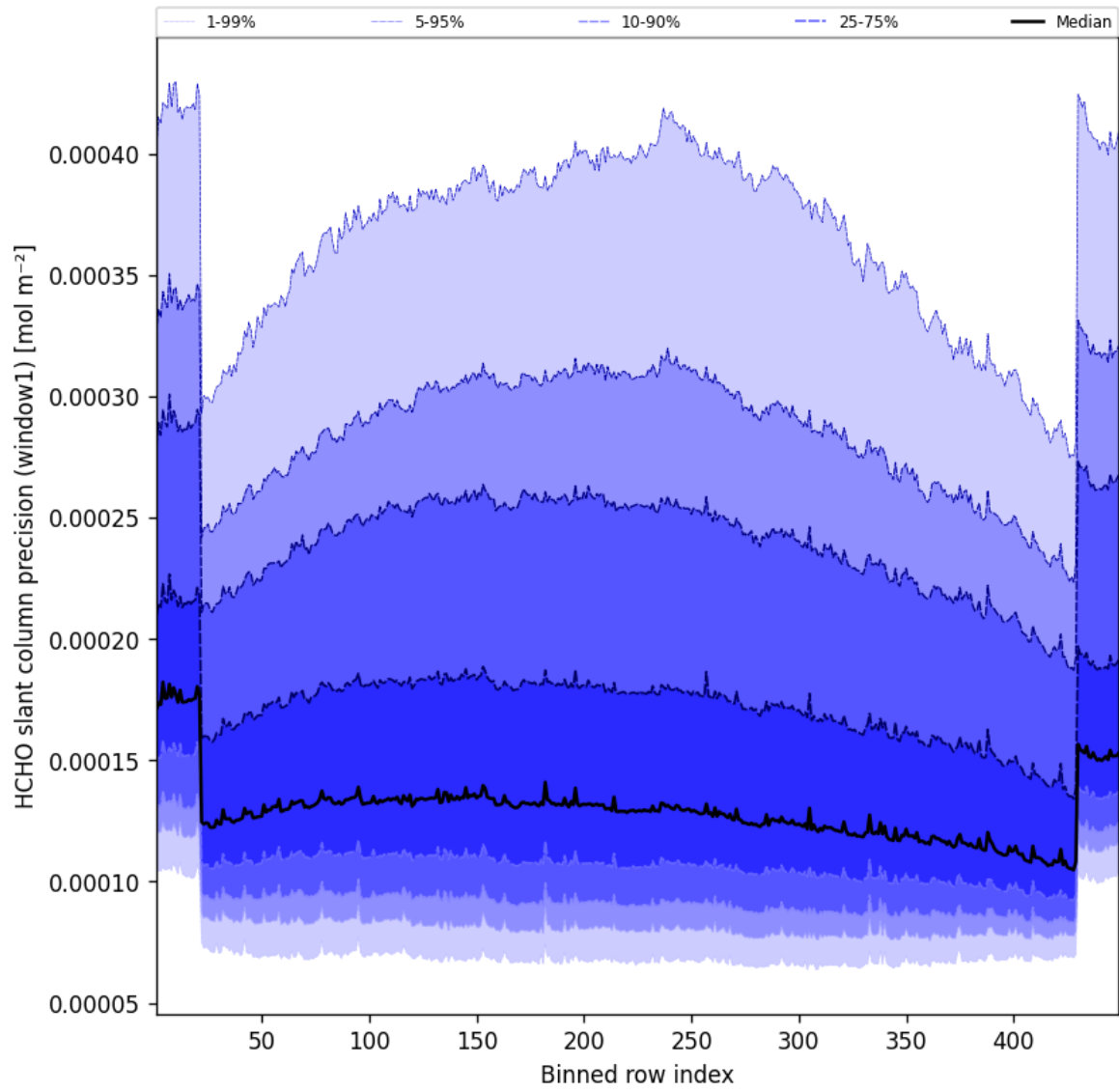
Figure 51: Along track statistics of “HCHO slant column precision (window1)” for 2025-06-30 to 2025-06-30
