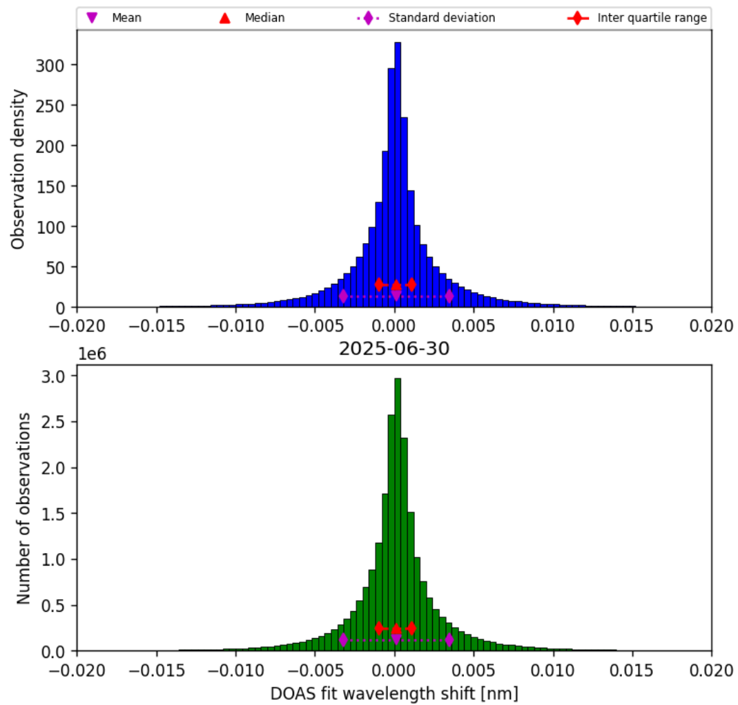
Figure 42: Histogram of “DOAS fit wavelength shift” for 2025-06-30 to 2025-06-30
