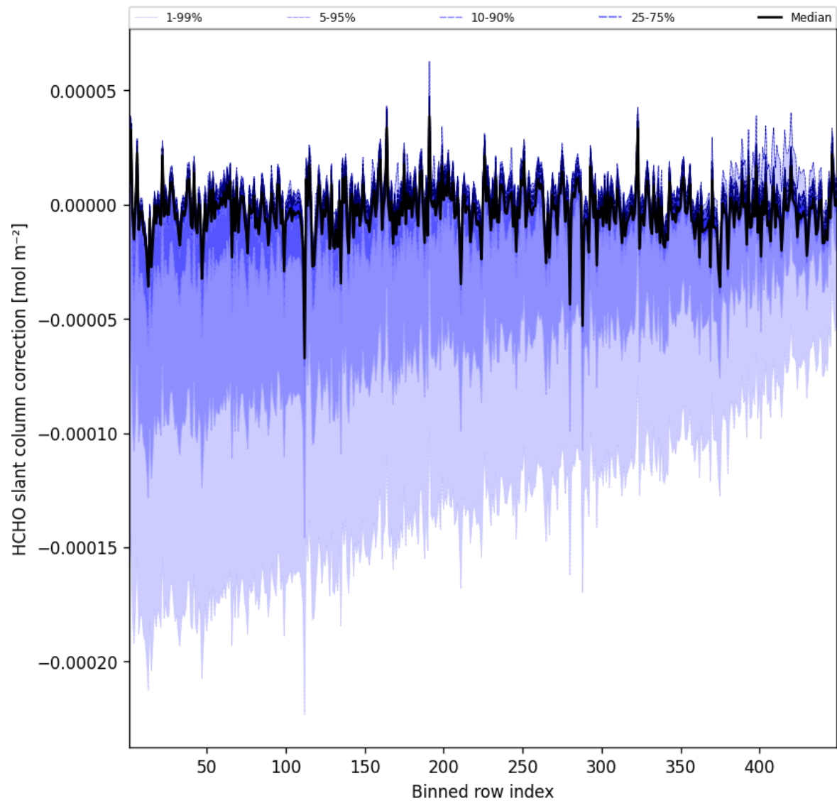
Figure 59: Along track statistics of “HCHO slant column correction” for 2025-06-30 to 2025-06-30
