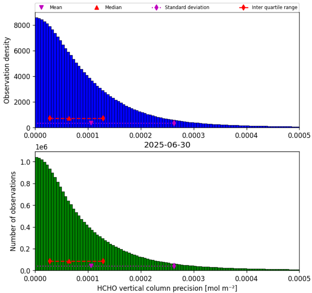
Figure 34: Histogram of “HCHO vertical column precision” for 2025-06-30 to 2025-06-30
