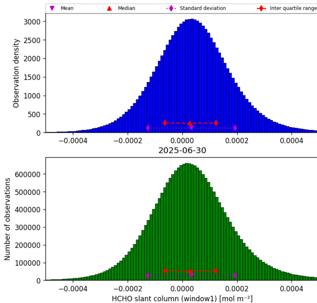
Figure 36: Histogram of "HCHO slant column (window1)" for 2025-06-30 to 2025-06-30
