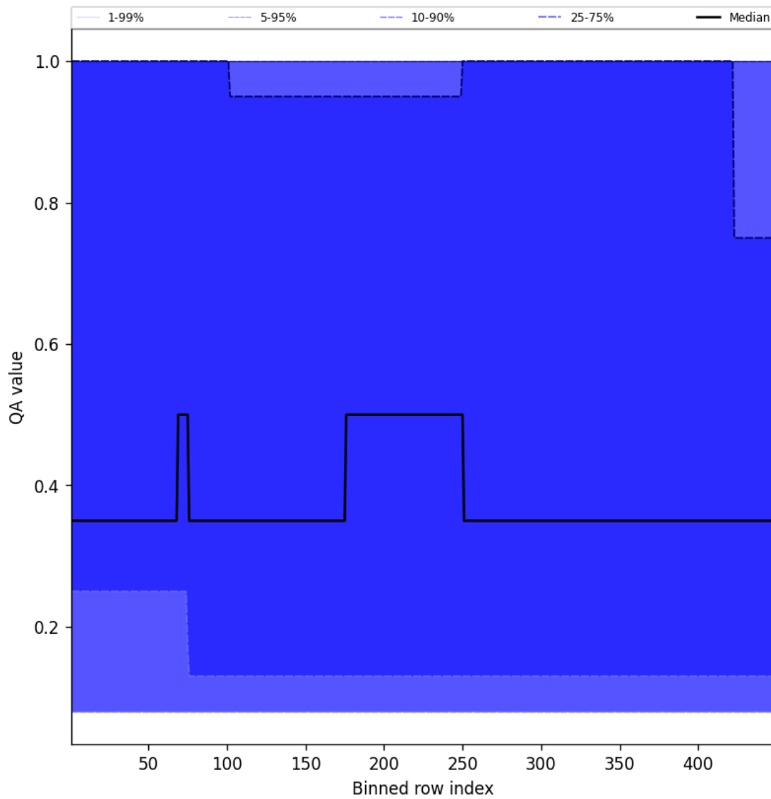
Figure 46: Along track statistics of “QA value” for 2025-06-30 to 2025-06-30
