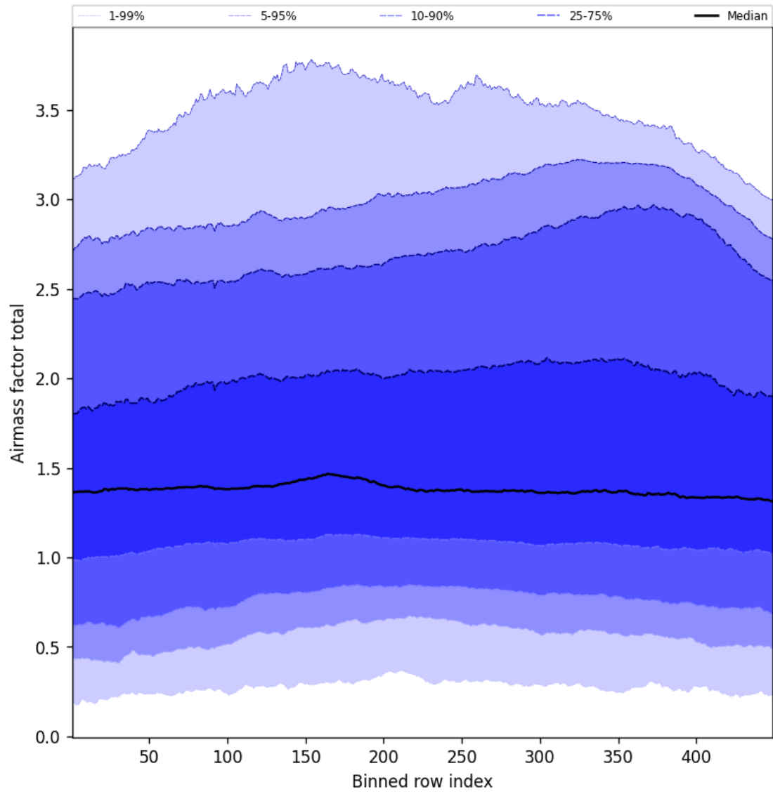
Figure 52: Along track statistics of “Airmass factor total” for 2025-06-30 to 2025-06-30
