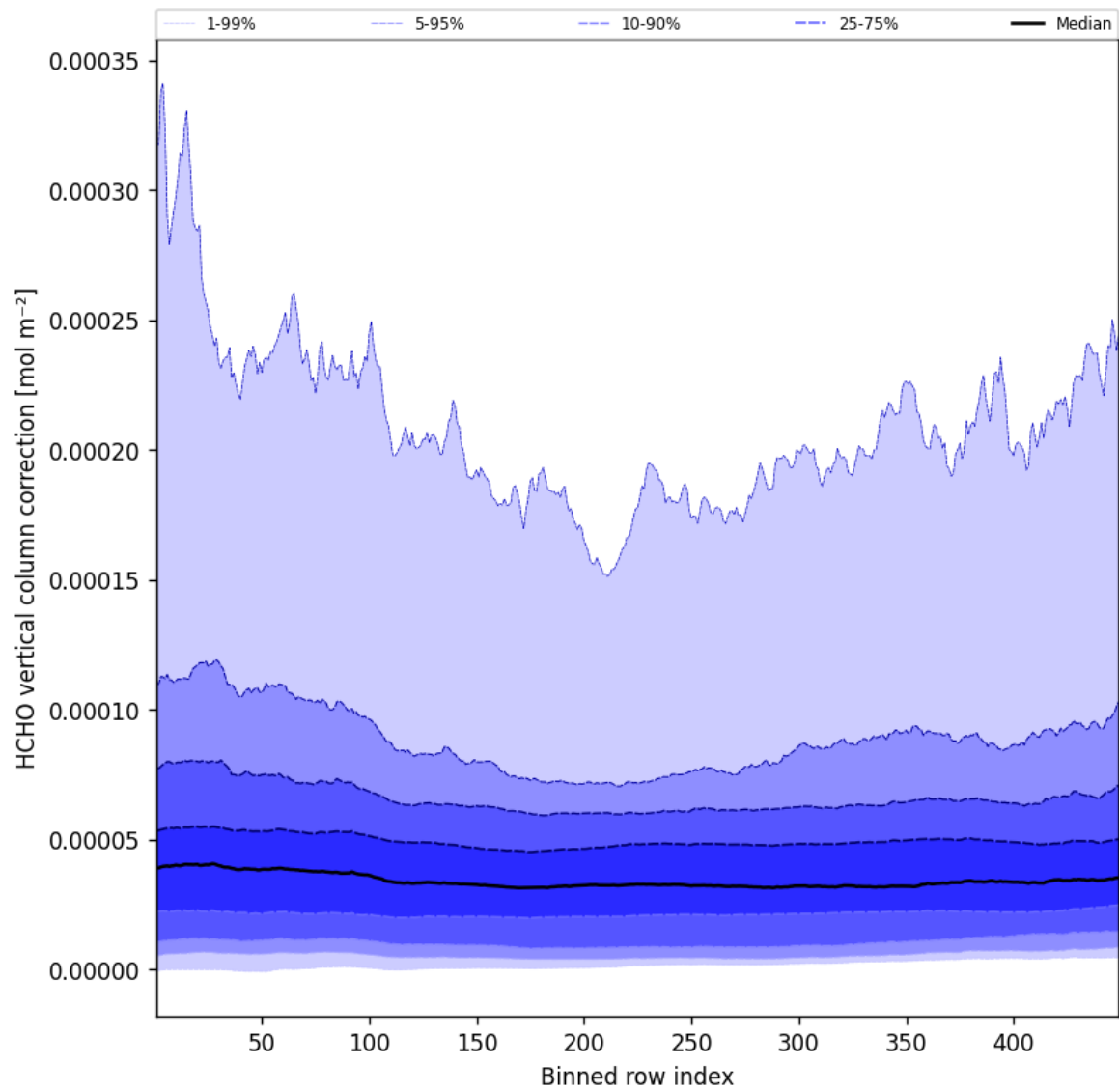
Figure 49: Along track statistics of “HCHO vertical column correction” for 2025-06-30 to 2025-06-30
