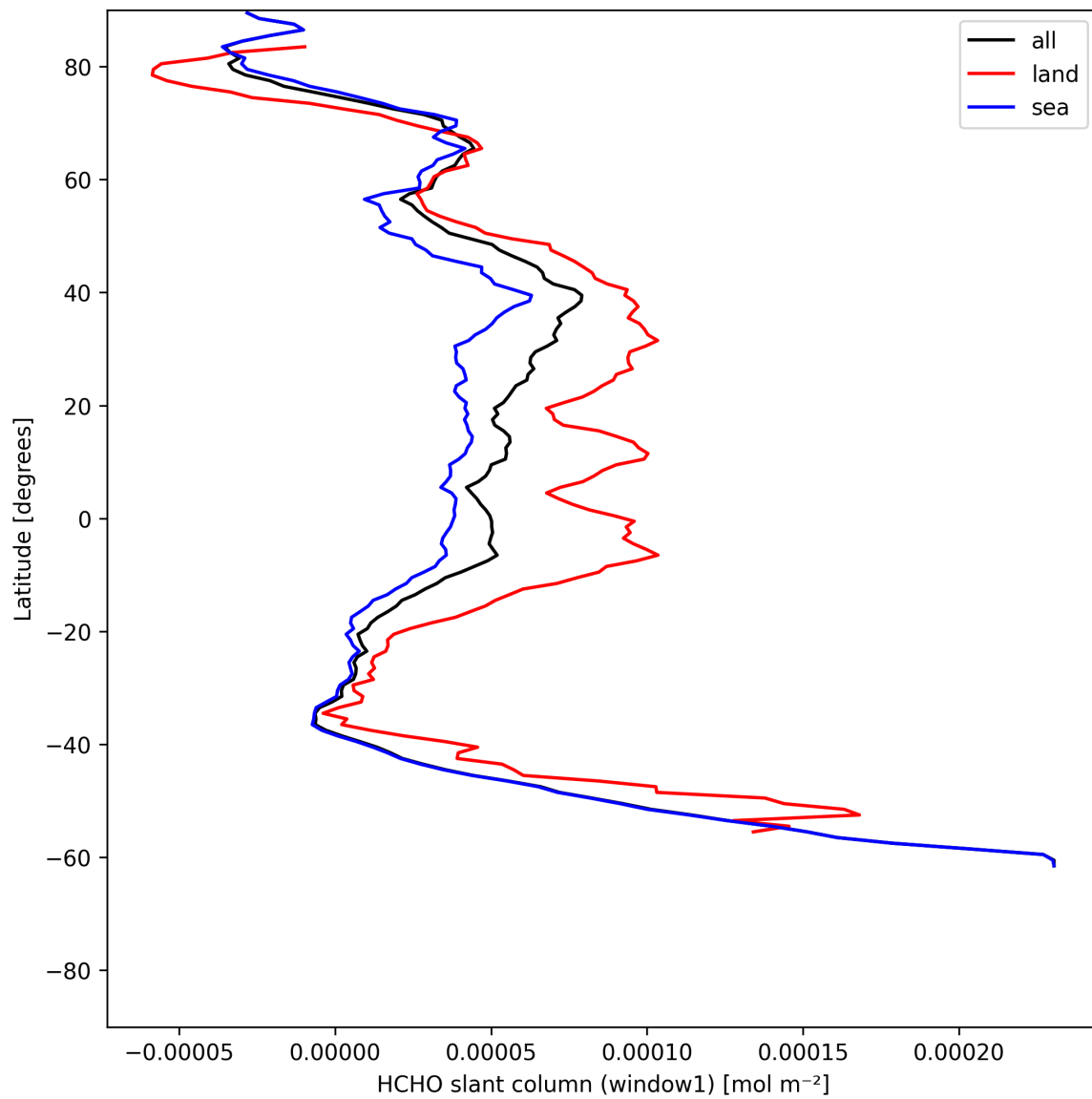
Figure 22: Zonal average of “HCHO slant column (window1)” for 2025-06-30 to 2025-06-30.
