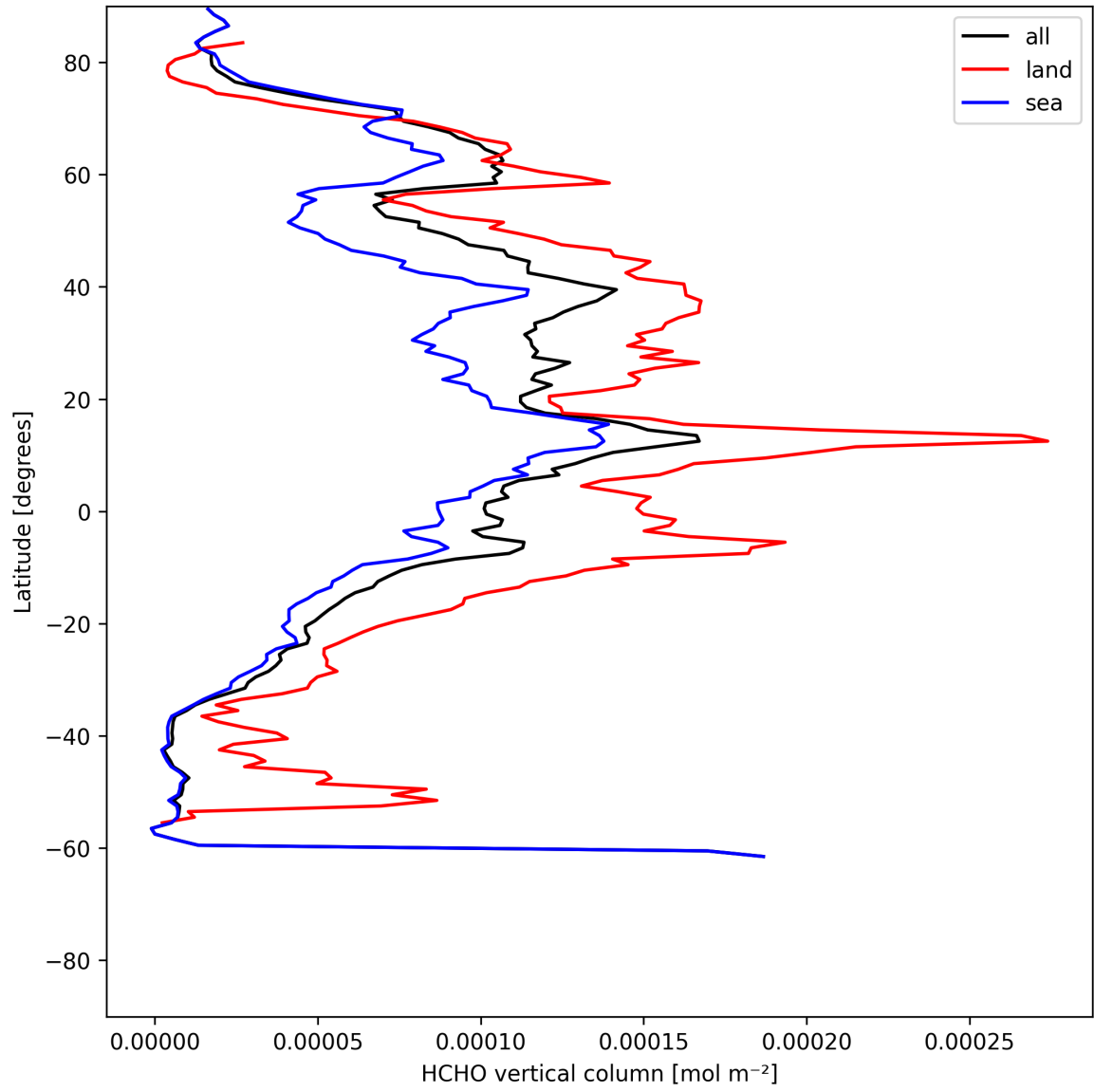
Figure 19: Zonal average of “HCHO vertical column” for 2025-06-30 to 2025-06-30.
