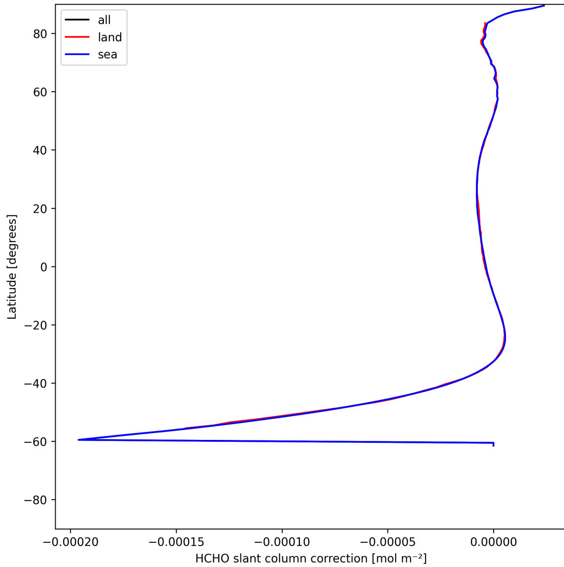
Figure 31: Zonal average of “HCHO slant column correction” for 2025-06-30 to 2025-06-30.
