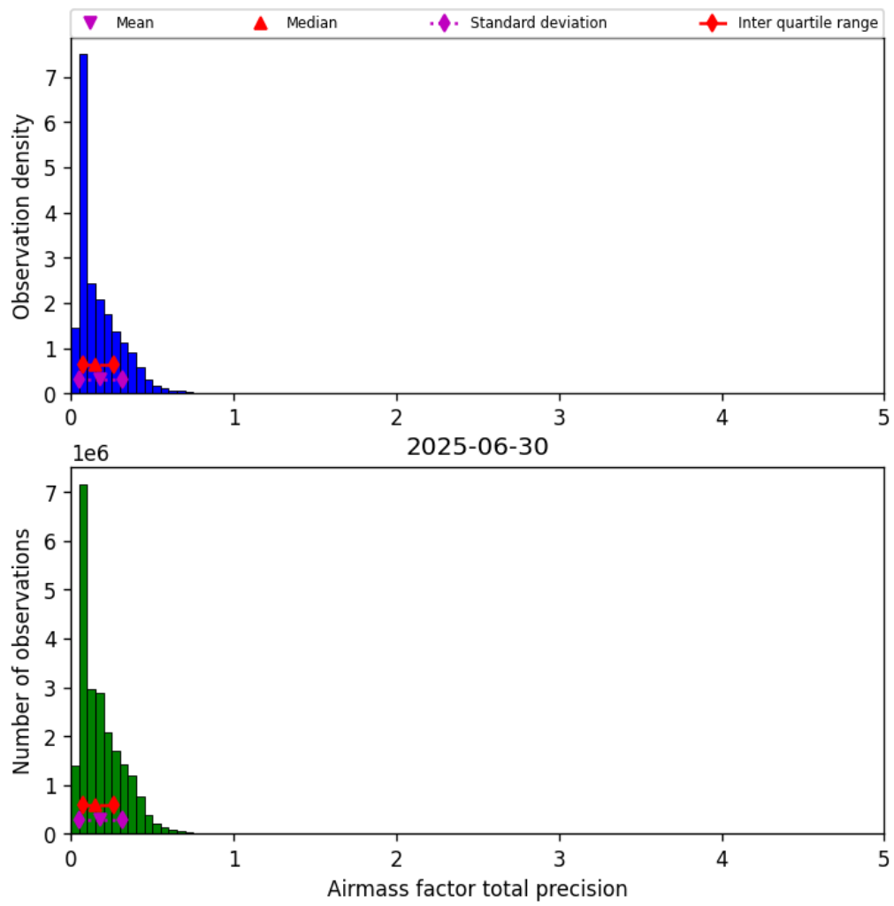
Figure 39: Histogram of “Airmass factor total precision” for 2025-06-30 to 2025-06-30
