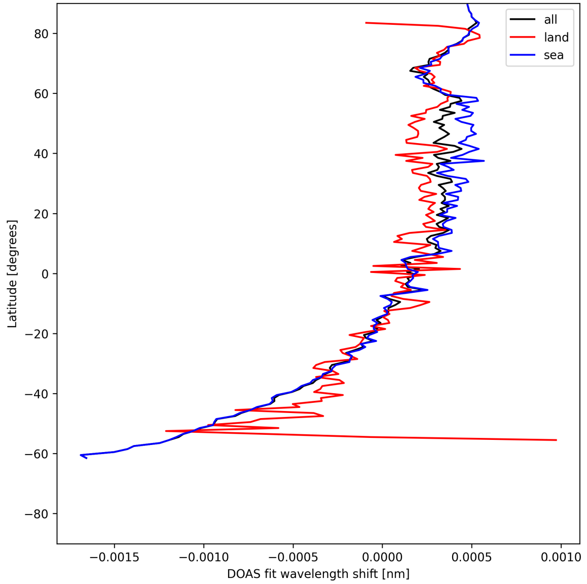
Figure 28: Zonal average of “DOAS fit wavelength shift” for 2025-06-30 to 2025-06-30.
