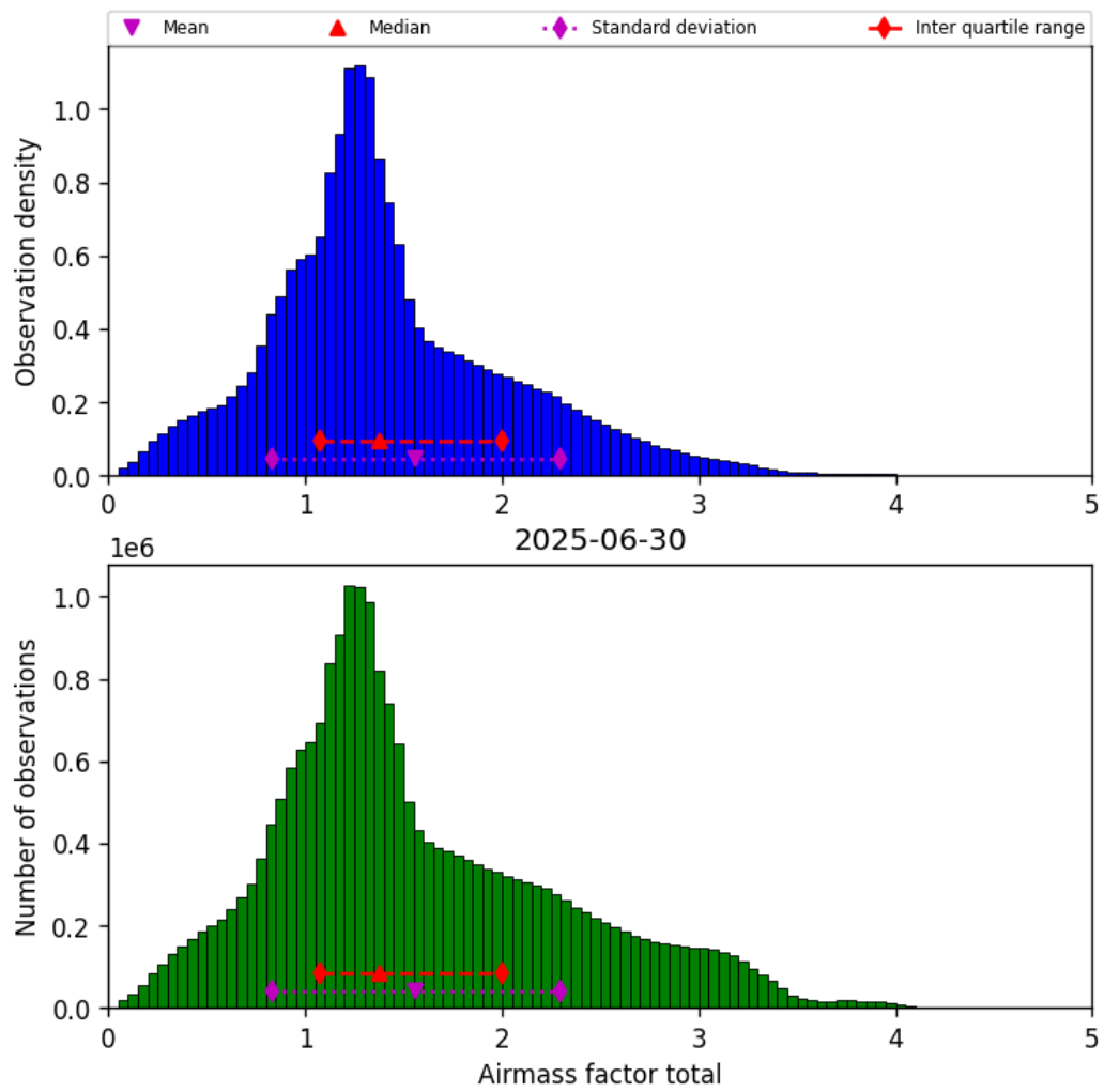
Figure 38: Histogram of “Airmass factor total” for 2025-06-30 to 2025-06-30
