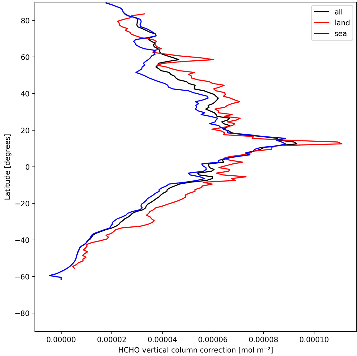
Figure 21: Zonal average of “HCHO vertical column correction” for 2025-06-30 to 2025-06-30.
