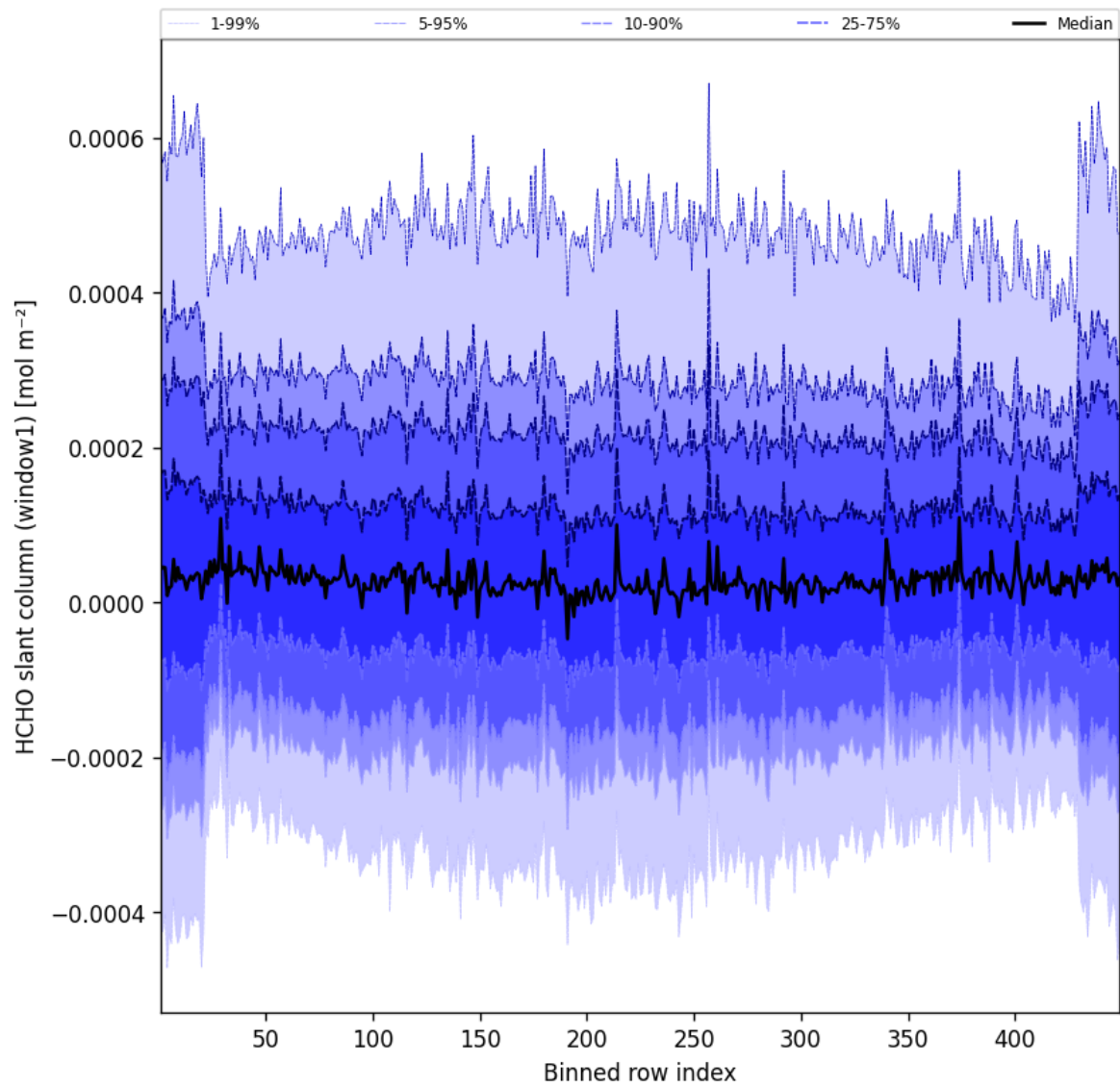
Figure 50: Along track statistics of “HCHO slant column (window1)” for 2025-06-30 to 2025-06-30
