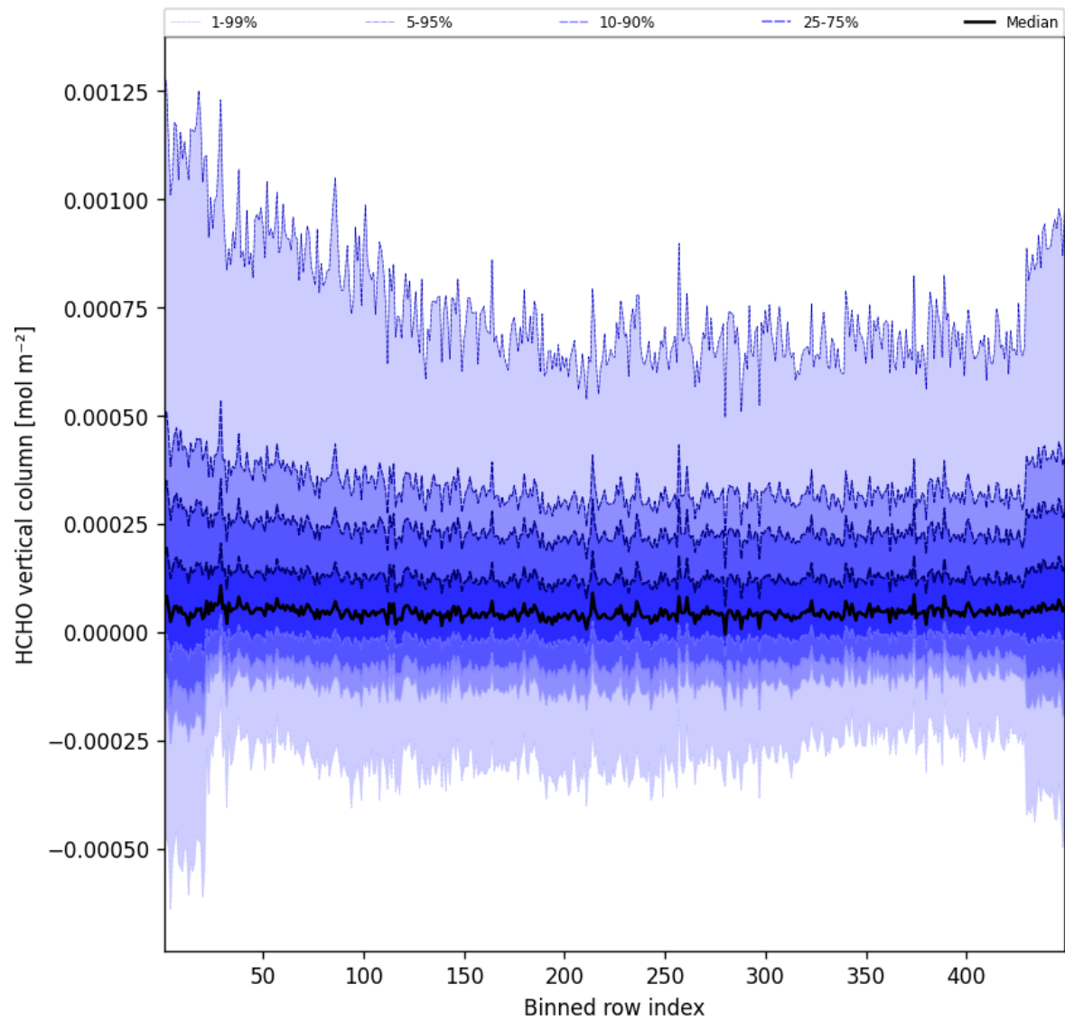
Figure 47: Along track statistics of “HCHO vertical column” for 2025-06-30 to 2025-06-30
