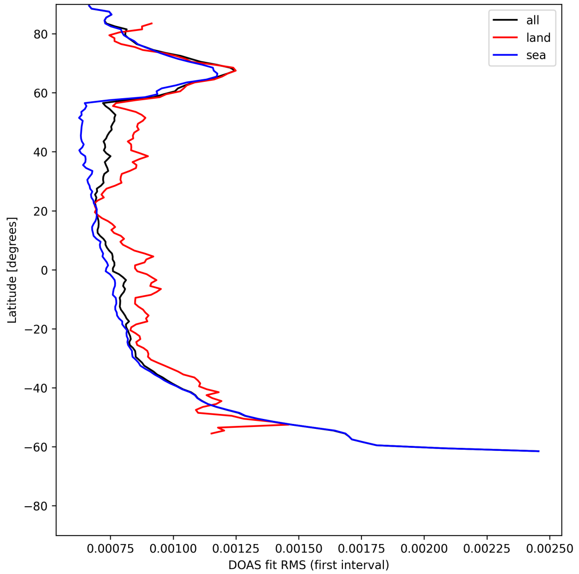
Figure 30: Zonal average of "DOAS fit RMS (first interval)" for 2025-06-30 to 2025-06-30.
