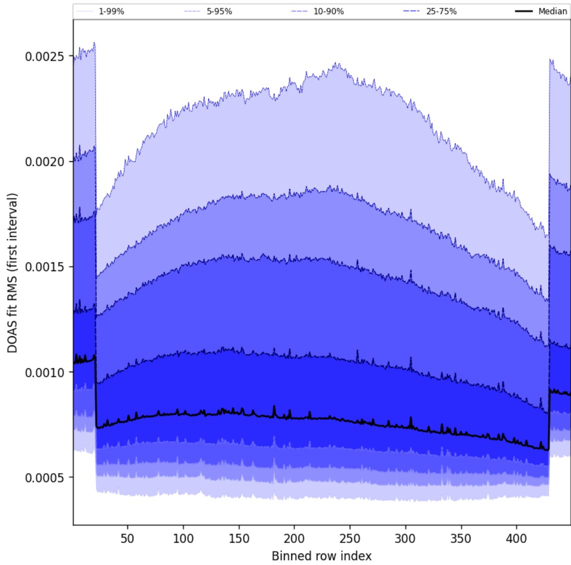
Figure 58: Along track statistics of “DOAS fit RMS (first interval)” for 2025-06-30 to 2025-06-30
