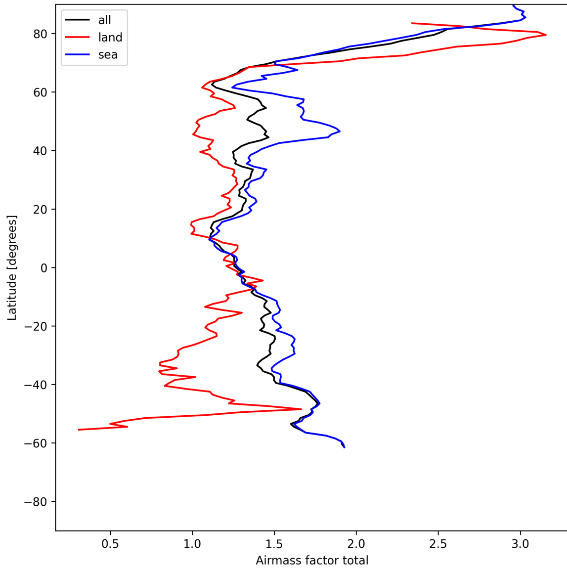
Figure 24: Zonal average of “Airmass factor total” for 2025-07-01 to 2025-07-02.
