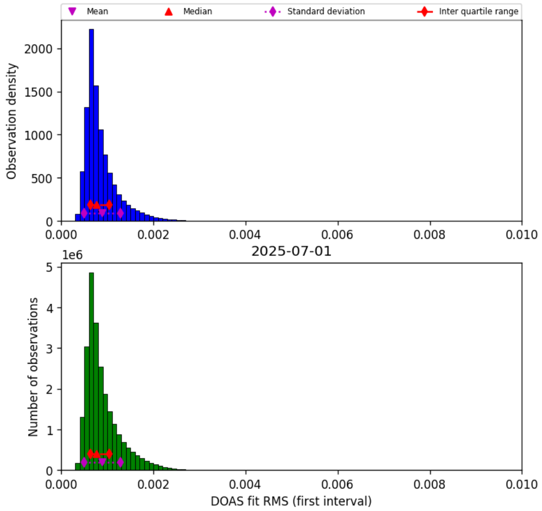
Figure 44: Histogram of “DOAS fit RMS (first interval)” for 2025-07-01 to 2025-07-02
