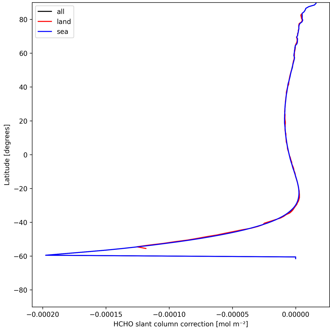
Figure 31: Zonal average of “HCHO slant column correction” for 2025-07-01 to 2025-07-02.
