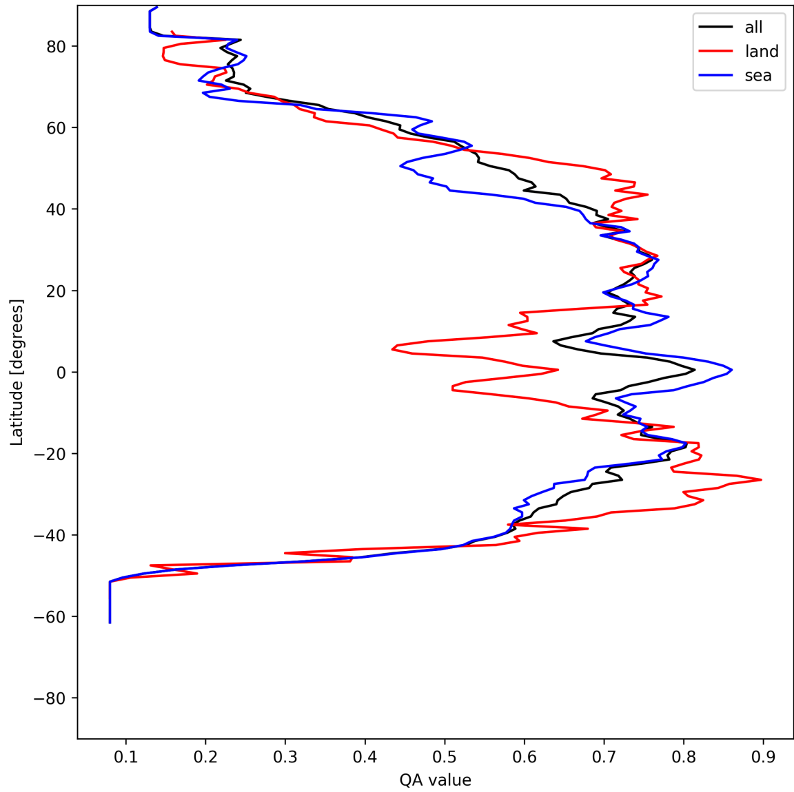
Figure 18: Zonal average of “QA value” for 2025-07-01 to 2025-07-02.
