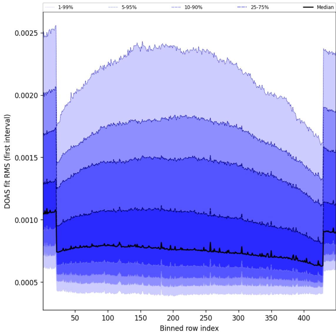
Figure 58: Along track statistics of “DOAS fit RMS (first interval)” for 2025-07-01 to 2025-07-02
