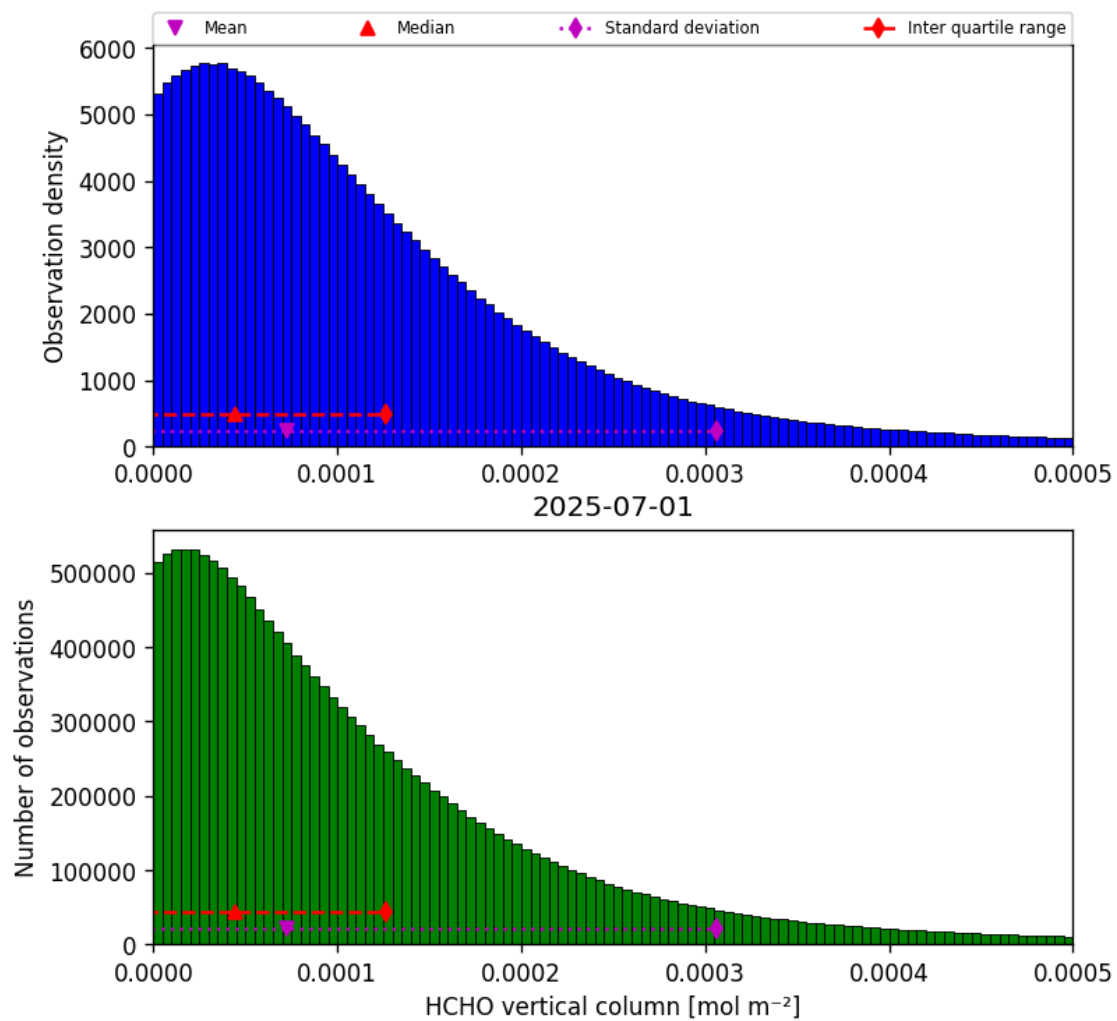
Figure 33: Histogram of “HCHO vertical column” for 2025-07-01 to 2025-07-02
