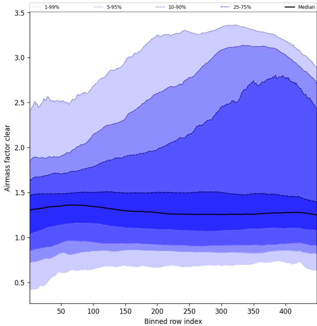
Figure 54: Along track statistics of “Airmass factor clear” for 2025-07-01 to 2025-07-02
