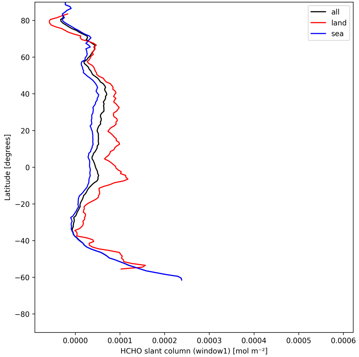
Figure 22: Zonal average of “HCHO slant column (window1)” for 2025-07-01 to 2025-07-02.
