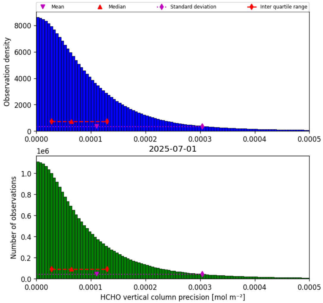
Figure 34: Histogram of “HCHO vertical column precision” for 2025-07-01 to 2025-07-02
