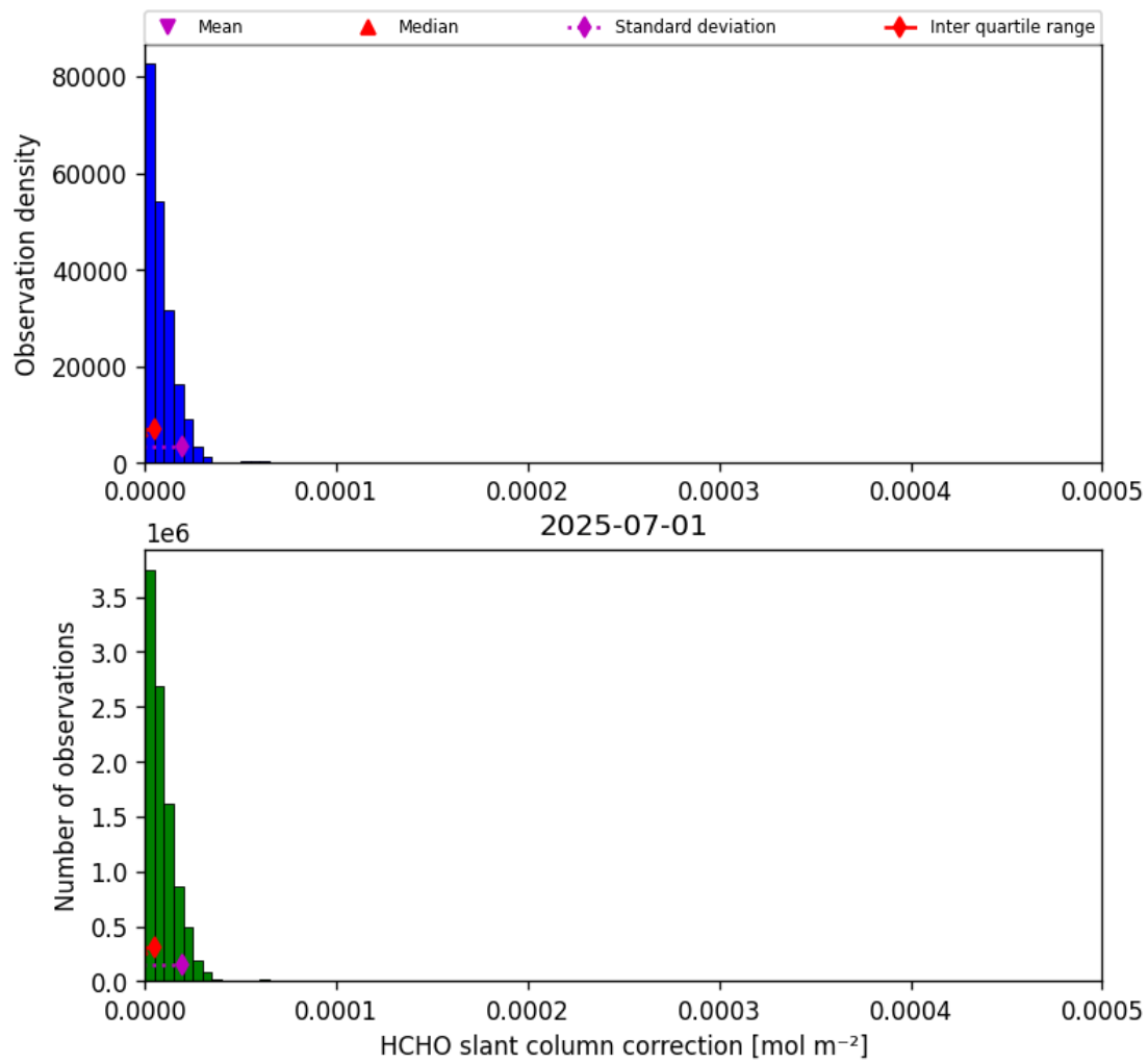
Figure 45: Histogram of “HCHO slant column correction” for 2025-07-01 to 2025-07-02
