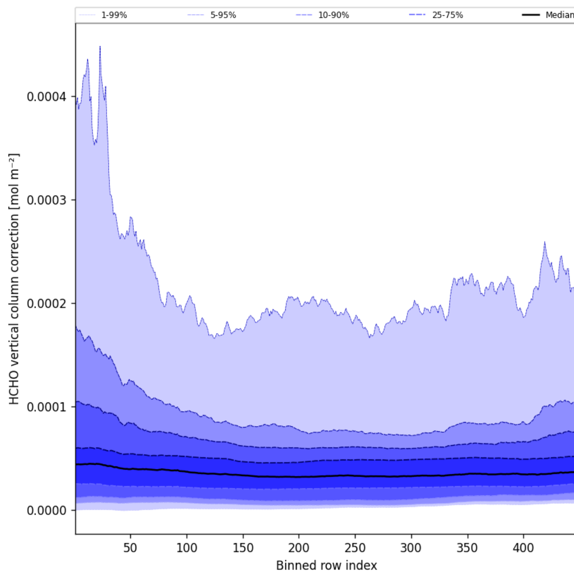
Figure 49: Along track statistics of “HCHO vertical column correction” for 2025-07-01 to 2025-07-02
