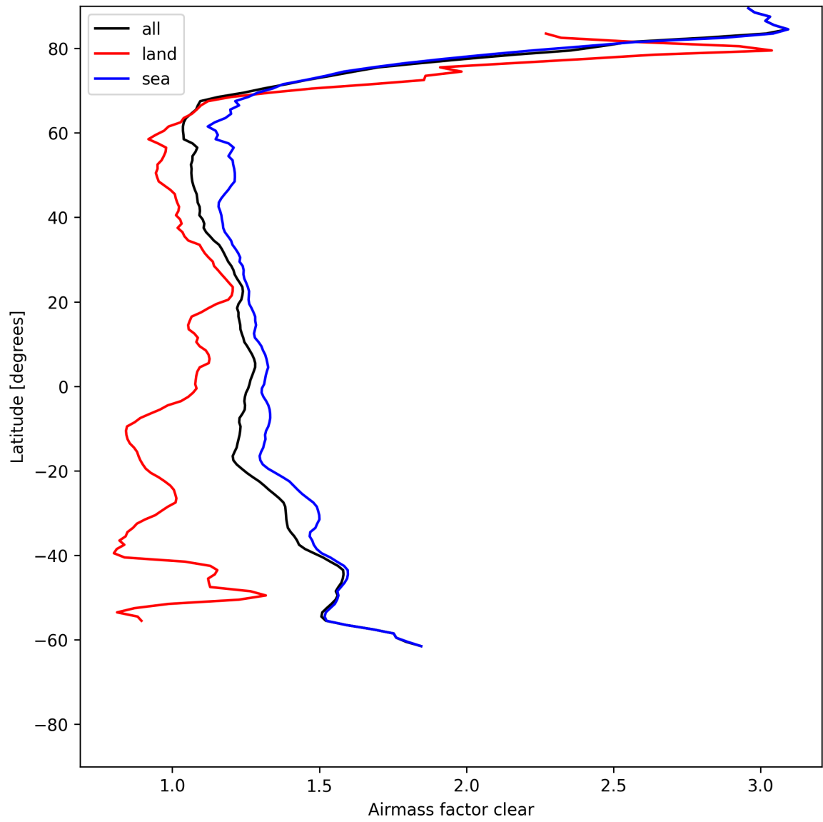
Figure 26: Zonal average of “Airmass factor clear” for 2025-07-01 to 2025-07-02.
