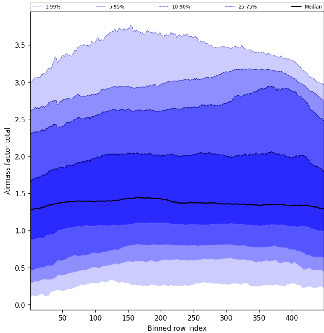
Figure 52: Along track statistics of “Airmass factor total” for 2025-07-01 to 2025-07-02
