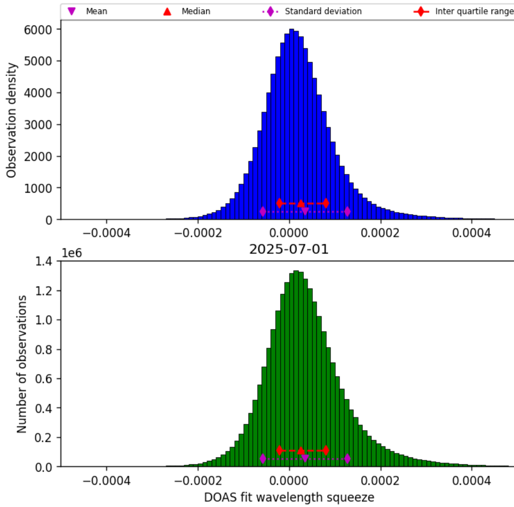
Figure 43: Histogram of “DOAS fit wavelength squeeze” for 2025-07-01 to 2025-07-02
