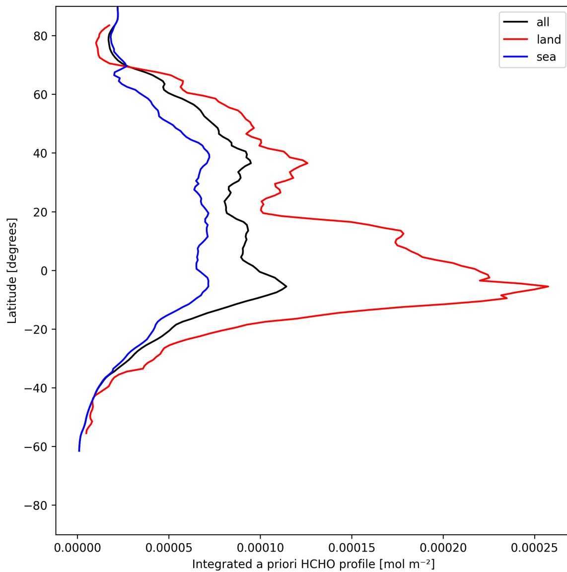
Figure 27: Zonal average of “Integrated a priori HCHO profile” for 2025-07-01 to 2025-07-02.
