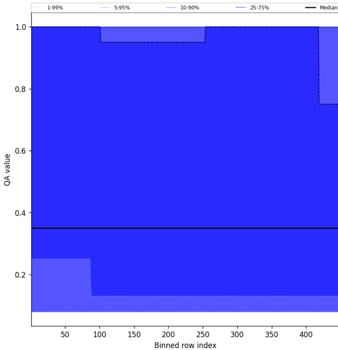
Figure 46: Along track statistics of "QA value" for 2025-07-01 to 2025-07-02
