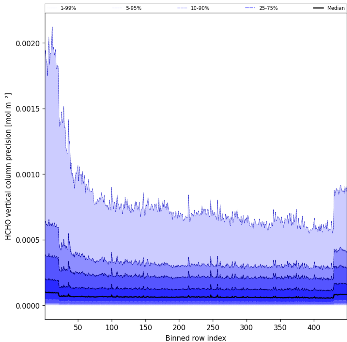
Figure 48: Along track statistics of “HCHO vertical column precision” for 2025-07-01 to 2025-07-02
