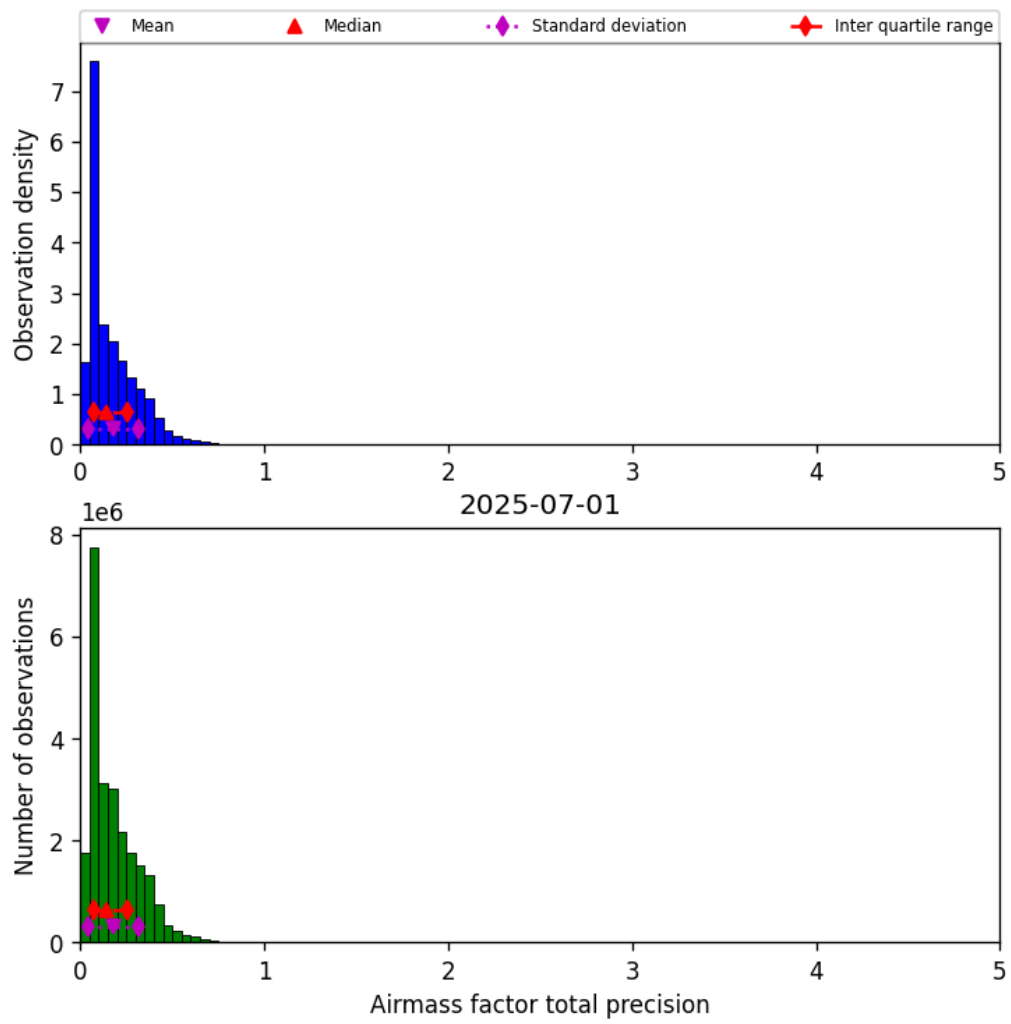
Figure 39: Histogram of “Airmass factor total precision” for 2025-07-01 to 2025-07-02
