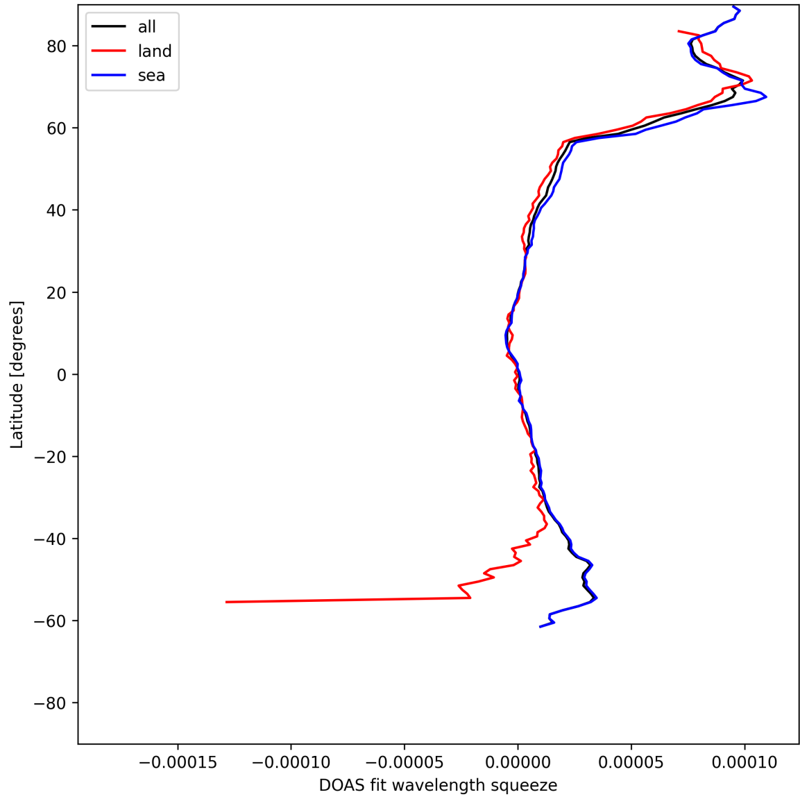
Figure 29: Zonal average of “DOAS fit wavelength squeeze” for 2025-07-01 to 2025-07-02.
