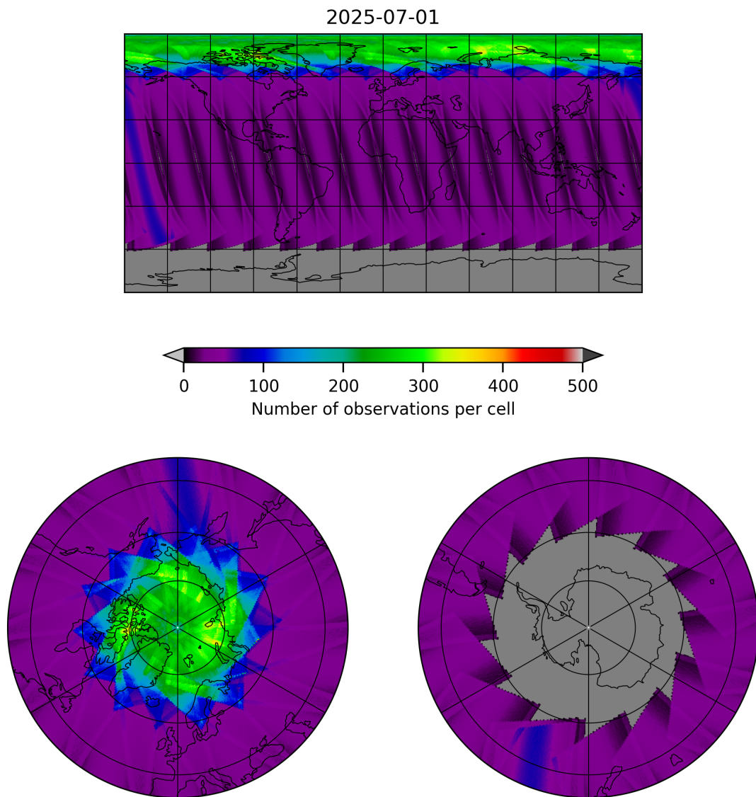
Figure 17: Map of the number of observations for 2025-07-01 to 2025-07-02
