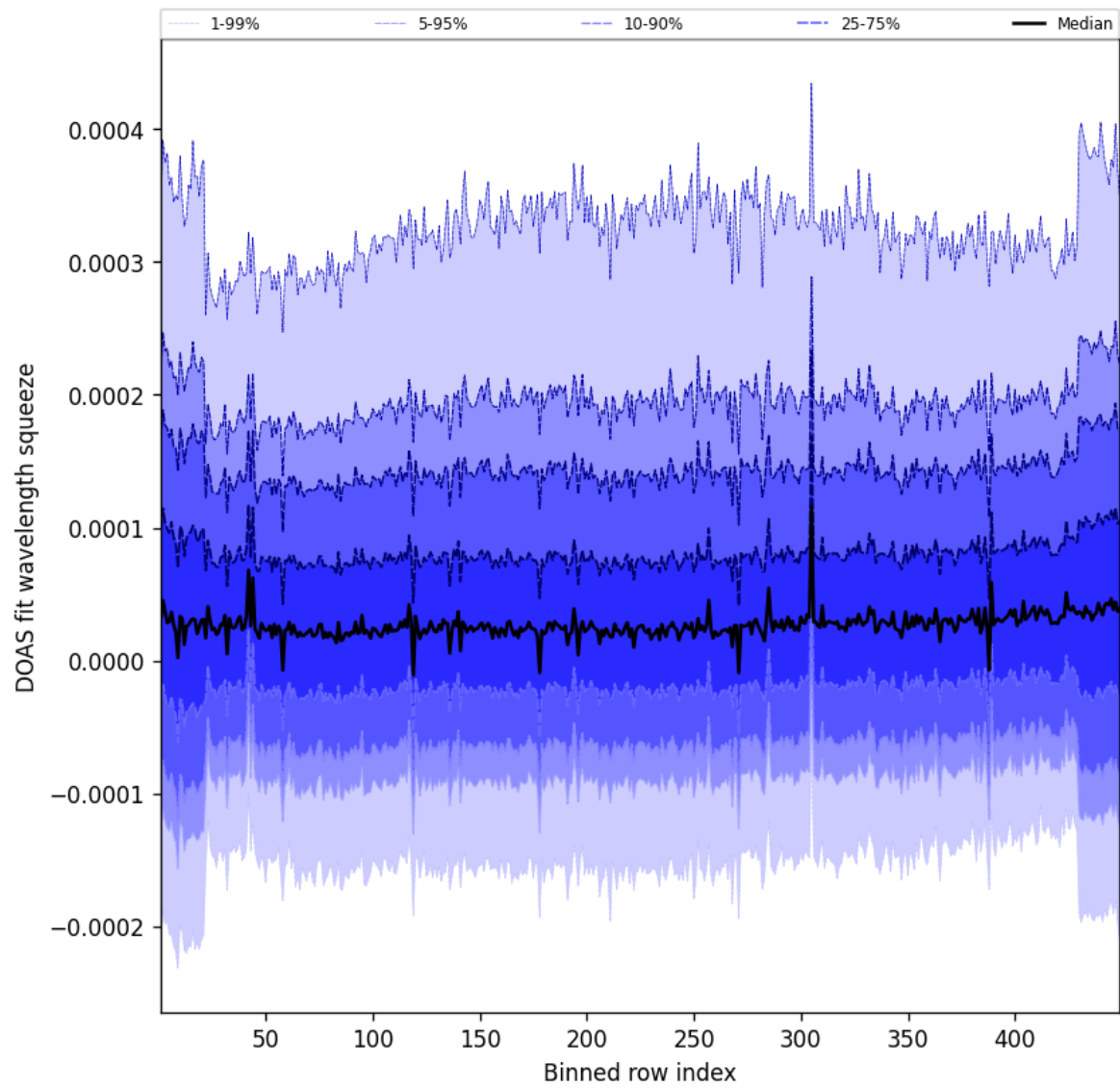
Figure 57: Along track statistics of “DOAS fit wavelength squeeze” for 2025-07-01 to 2025-07-02
