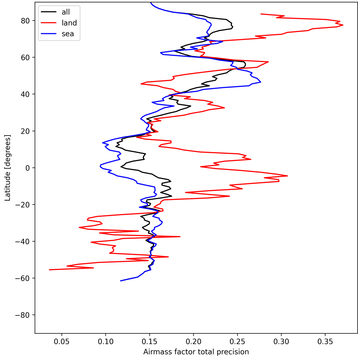
Figure 25: Zonal average of “Airmass factor total precision” for 2025-07-01 to 2025-07-02.
