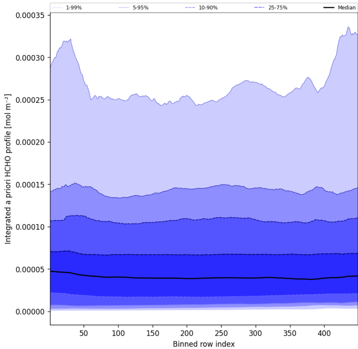
Figure 55: Along track statistics of "Integrated a priori HCHO profile" for 2025-07-01 to 2025-07-02
