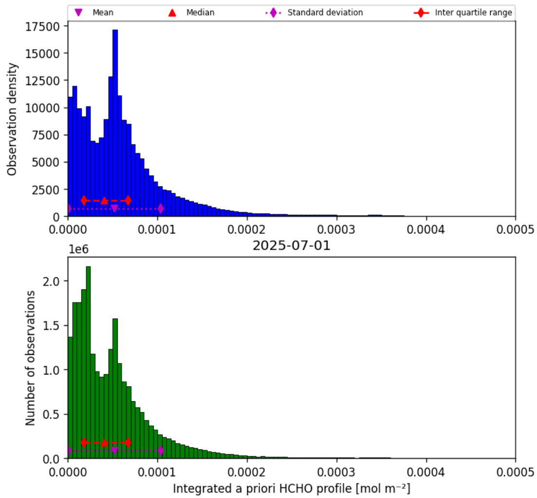
Figure 41: Histogram of “Integrated a priori HCHO profile” for 2025-07-01 to 2025-07-02
