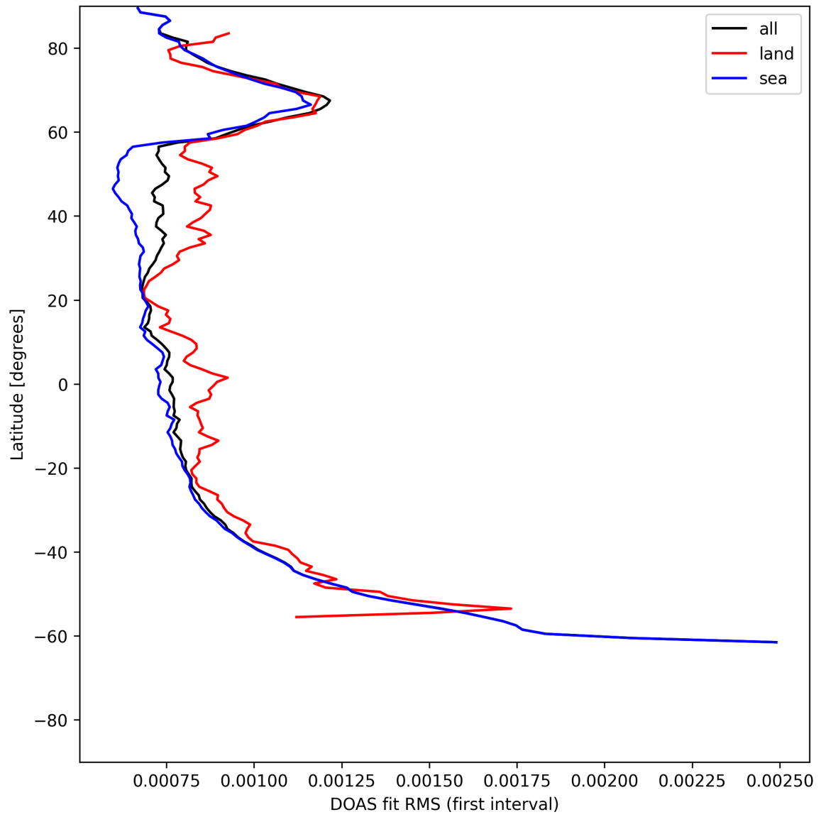
Figure 30: Zonal average of “DOAS fit RMS (first interval)” for 2025-07-01 to 2025-07-02.
