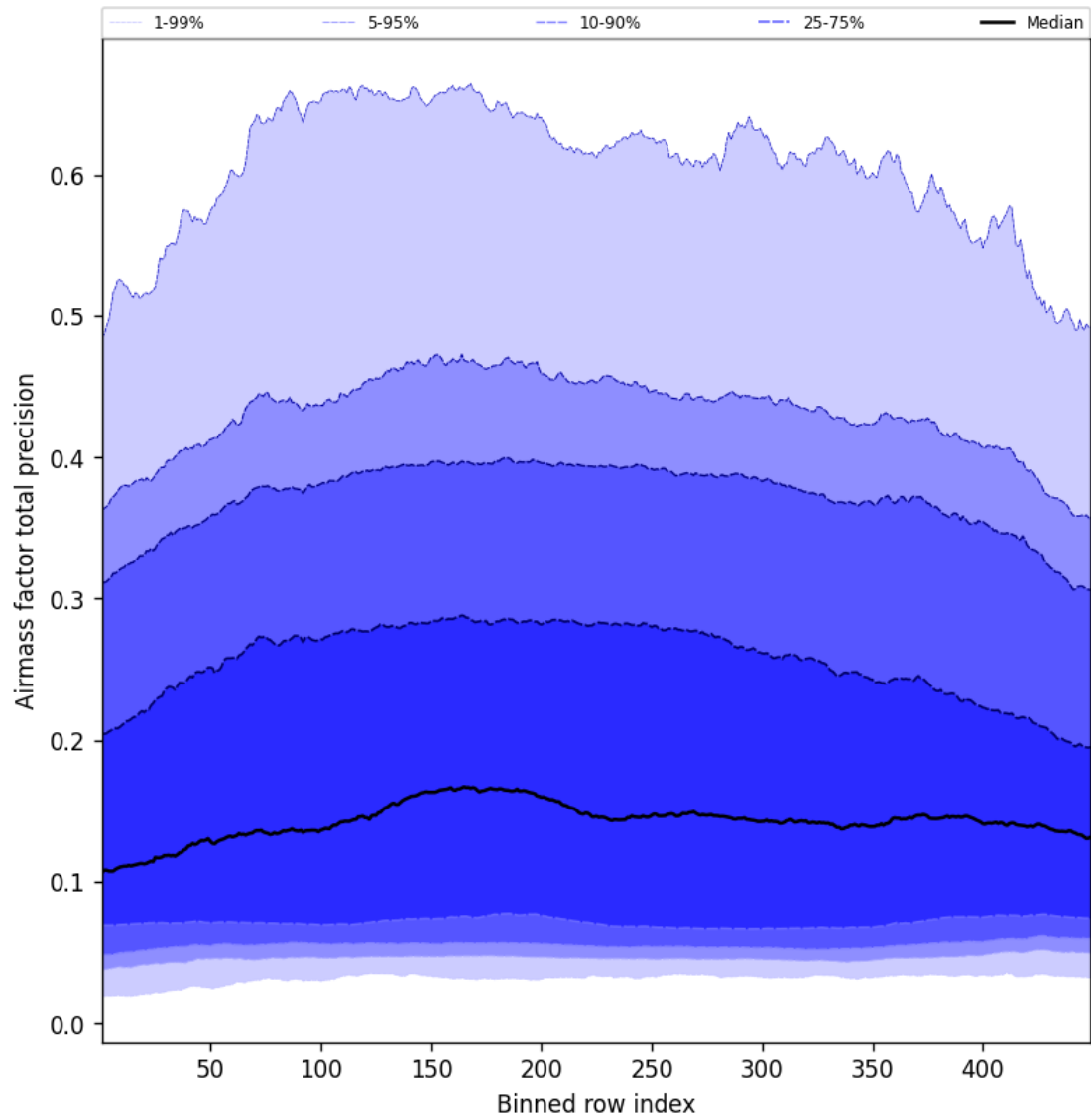
Figure 53: Along track statistics of “Airmass factor total precision” for 2025-07-01 to 2025-07-02
