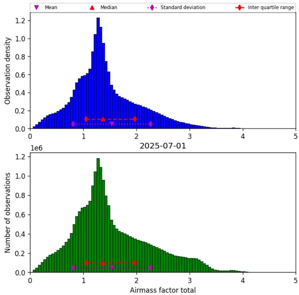
Figure 38: Histogram of “Airmass factor total” for 2025-07-01 to 2025-07-02
