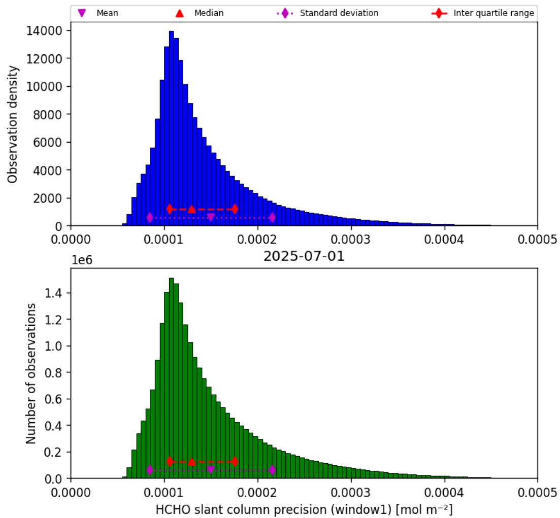
Figure 37: Histogram of “HCHO slant column precision (window1)” for 2025-07-01 to 2025-07-02
