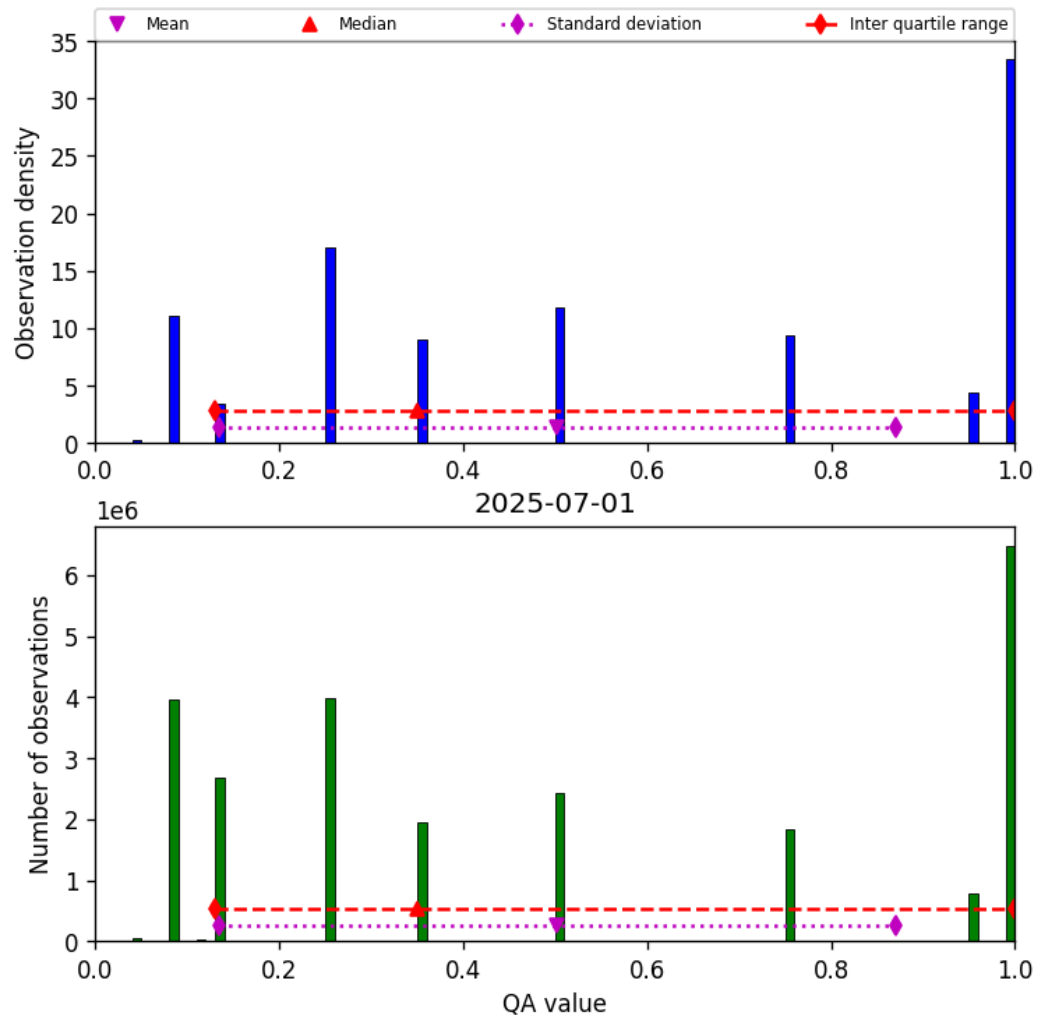
Figure 32: Histogram of “QA value” for 2025-07-01 to 2025-07-02
