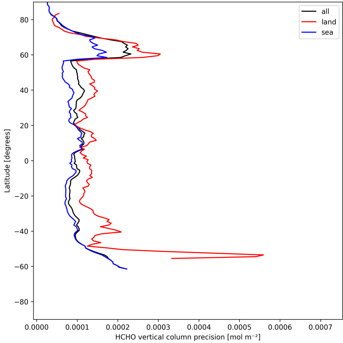
Figure 20: Zonal average of “HCHO vertical column precision” for 2025-07-01 to 2025-07-02.
