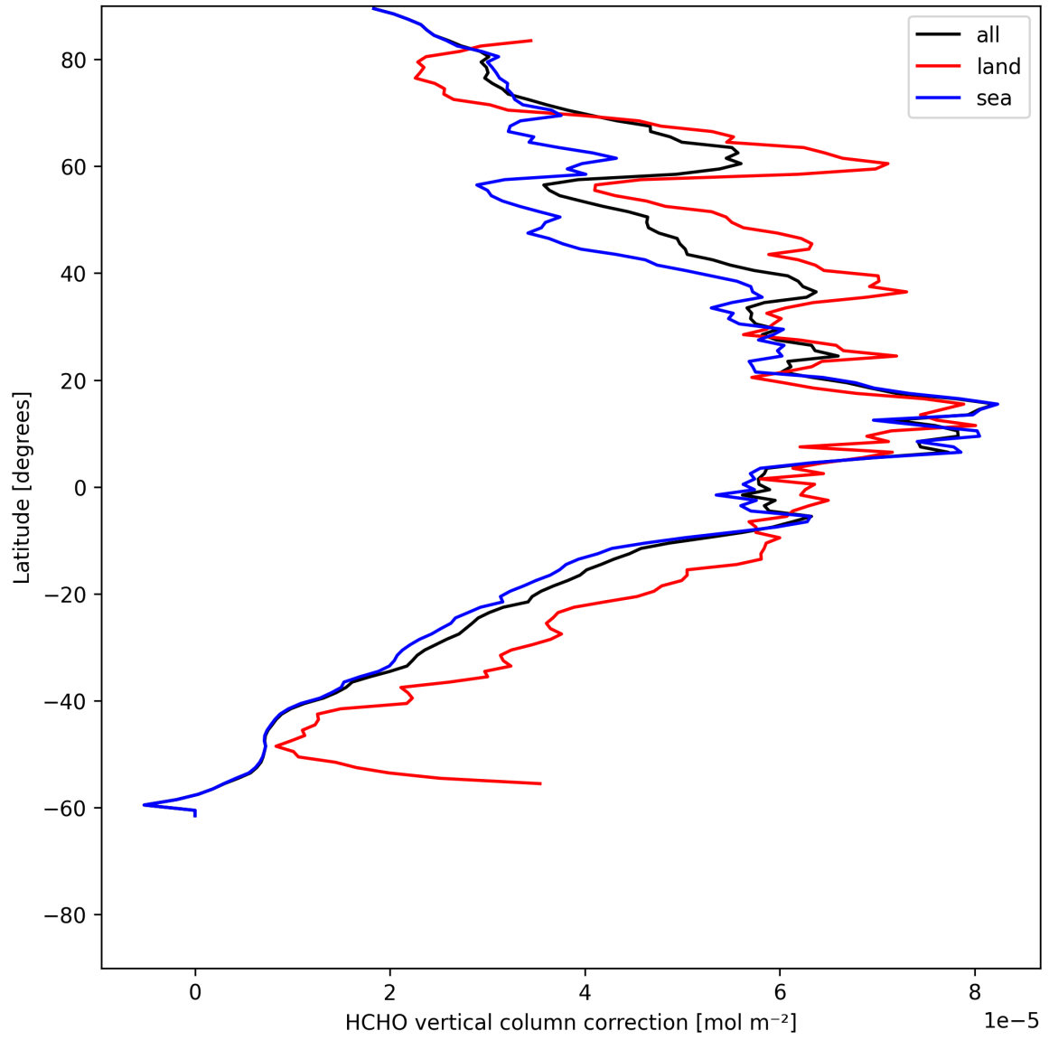
Figure 21: Zonal average of “HCHO vertical column correction” for 2025-07-01 to 2025-07-02.
