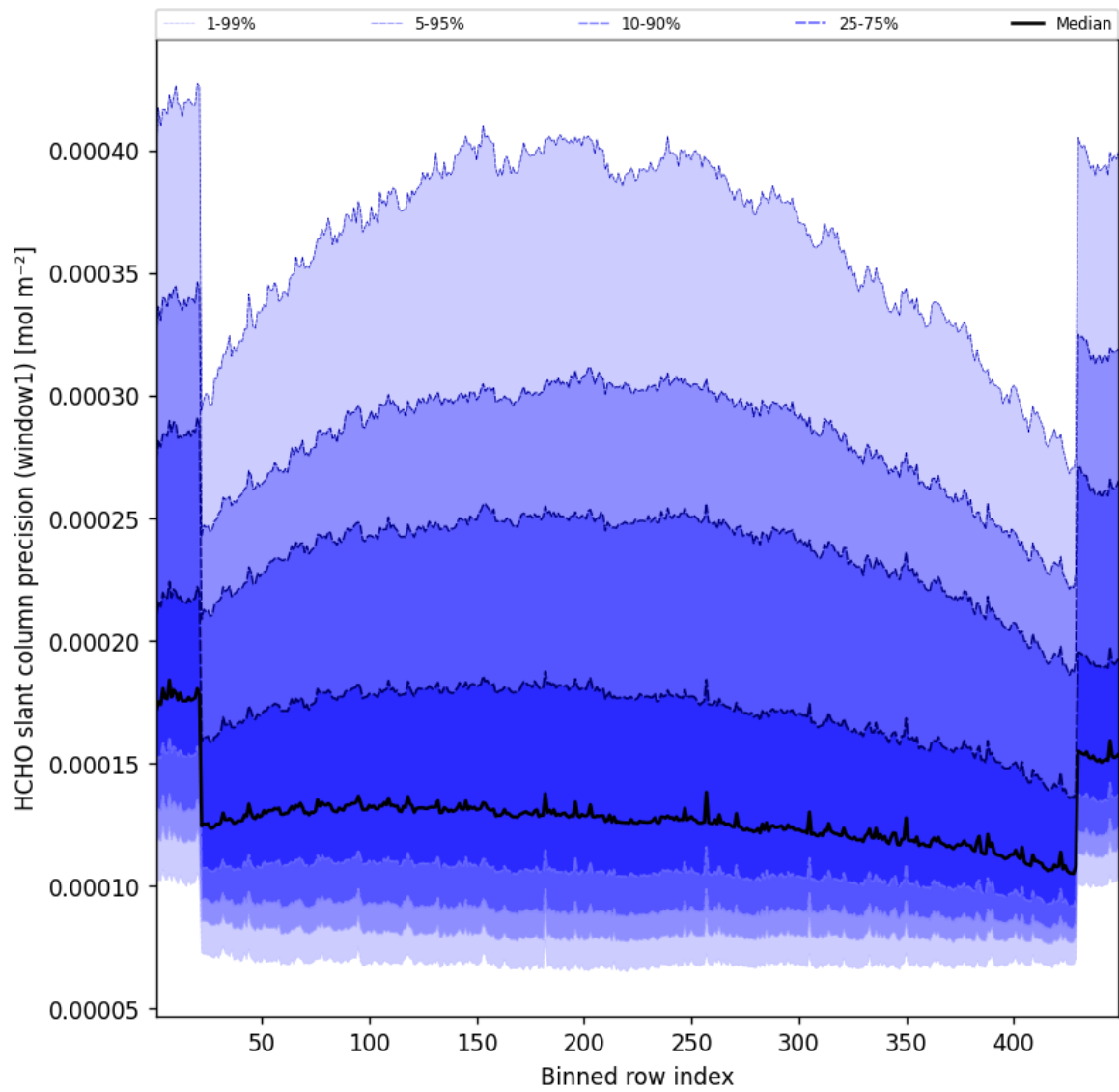
Figure 51: Along track statistics of “HCHO slant column precision (window1)” for 2025-07-01 to 2025-07-02
