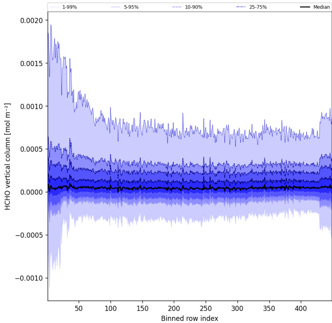
Figure 47: Along track statistics of “HCHO vertical column” for 2025-07-01 to 2025-07-02
