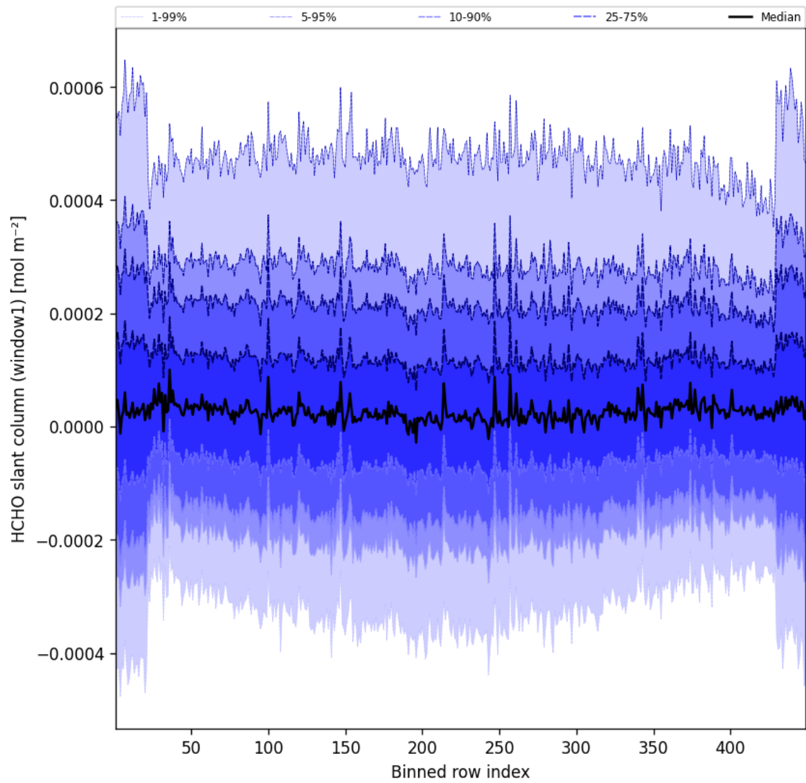
Figure 50: Along track statistics of “HCHO slant column (window1)” for 2025-07-01 to 2025-07-02
