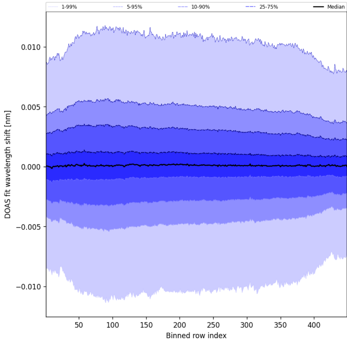
Figure 56: Along track statistics of “DOAS fit wavelength shift” for 2025-07-01 to 2025-07-02
