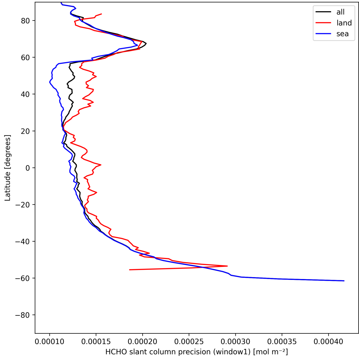
Figure 23: Zonal average of "HCHO slant column precision (window1)" for 2025-07-01 to 2025-07-02.
