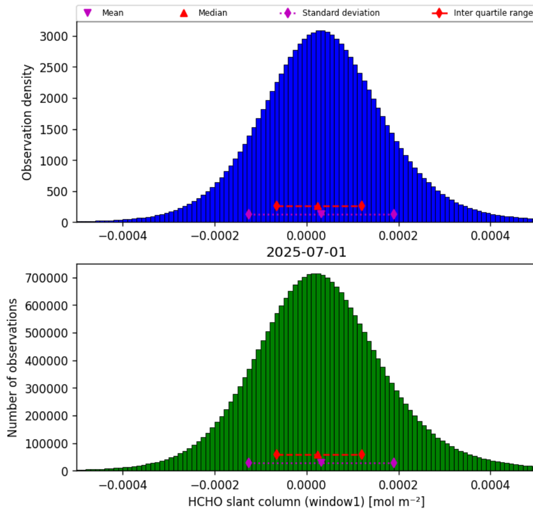
Figure 36: Histogram of “HCHO slant column (window1)” for 2025-07-01 to 2025-07-02
