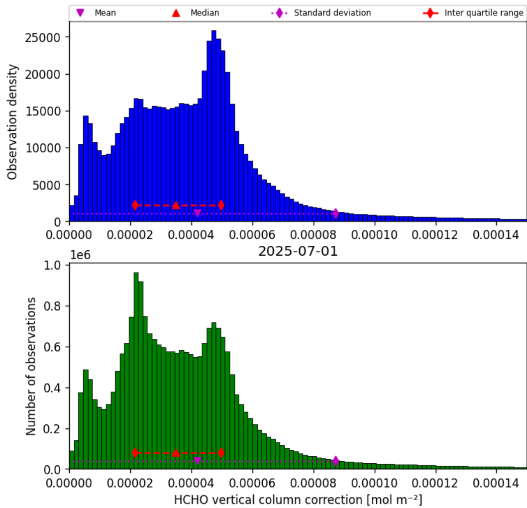
Figure 35: Histogram of “HCHO vertical column correction” for 2025-07-01 to 2025-07-02
