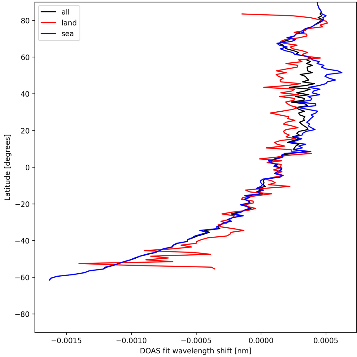
Figure 28: Zonal average of “DOAS fit wavelength shift” for 2025-07-01 to 2025-07-02.
