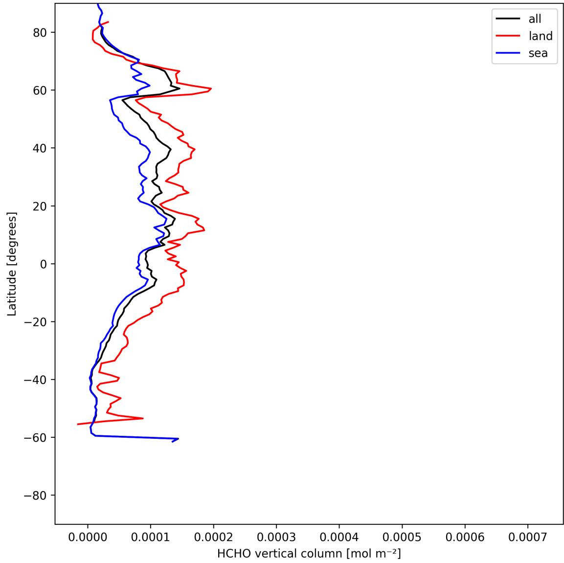
Figure 19: Zonal average of “HCHO vertical column” for 2025-07-01 to 2025-07-02.
