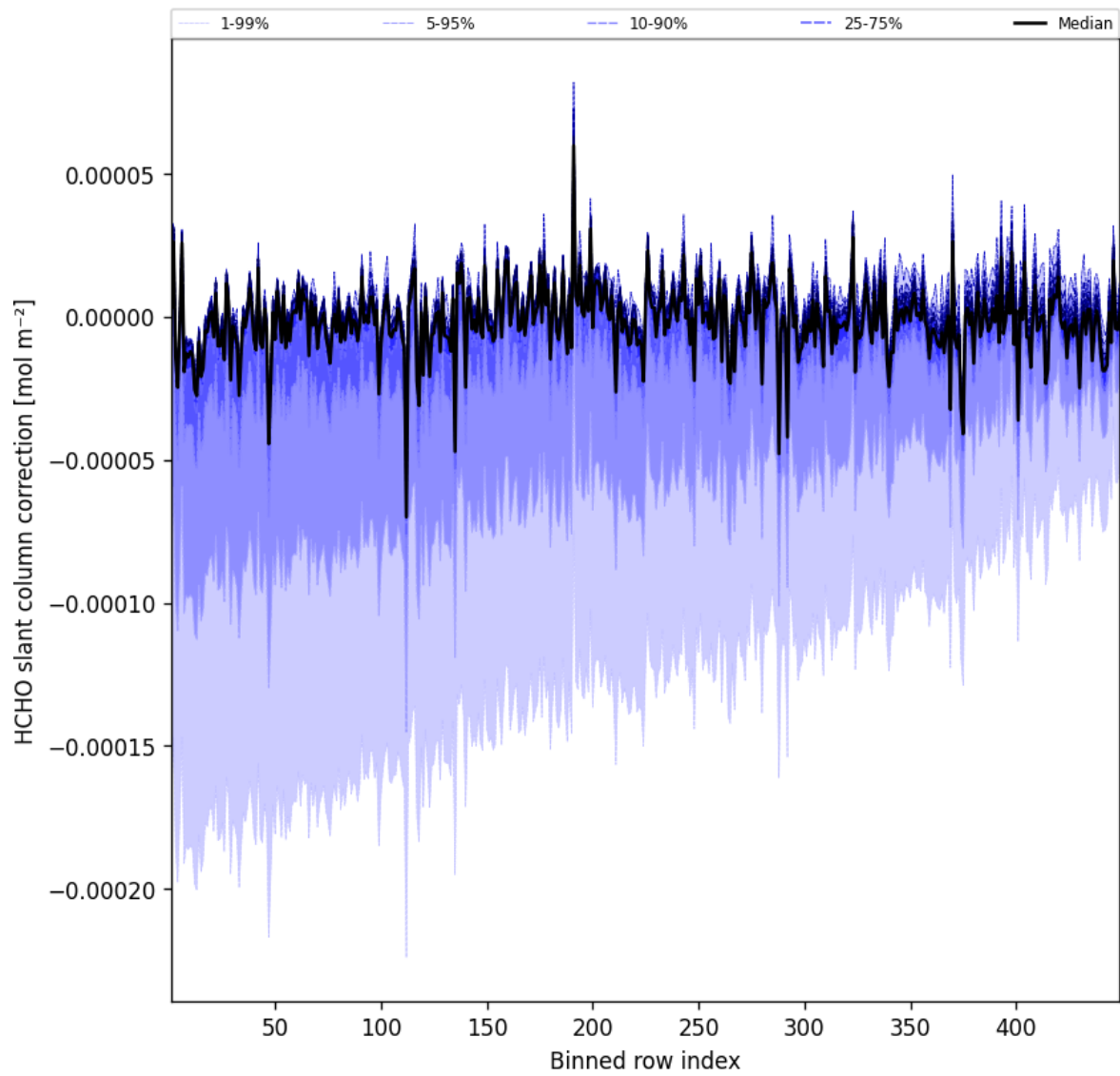
Figure 59: Along track statistics of “HCHO slant column correction” for 2025-07-01 to 2025-07-02
