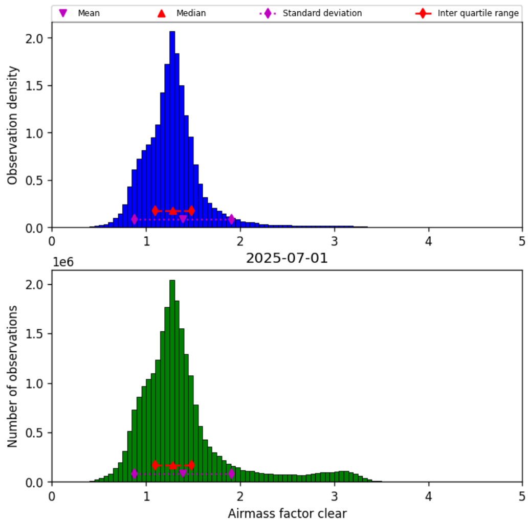
Figure 40: Histogram of “Airmass factor clear” for 2025-07-01 to 2025-07-02
