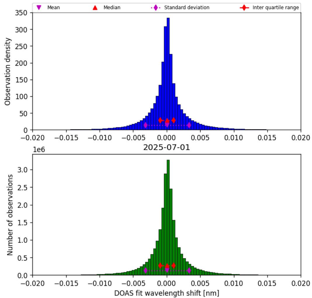
Figure 42: Histogram of “DOAS fit wavelength shift” for 2025-07-01 to 2025-07-02
