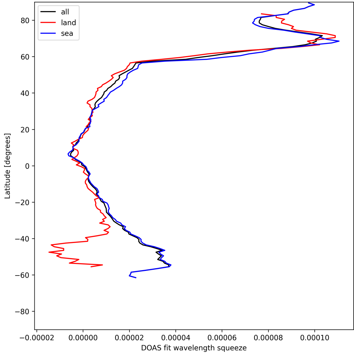
Figure 29: Zonal average of “DOAS fit wavelength squeeze” for 2025-07-02 to 2025-07-03.
