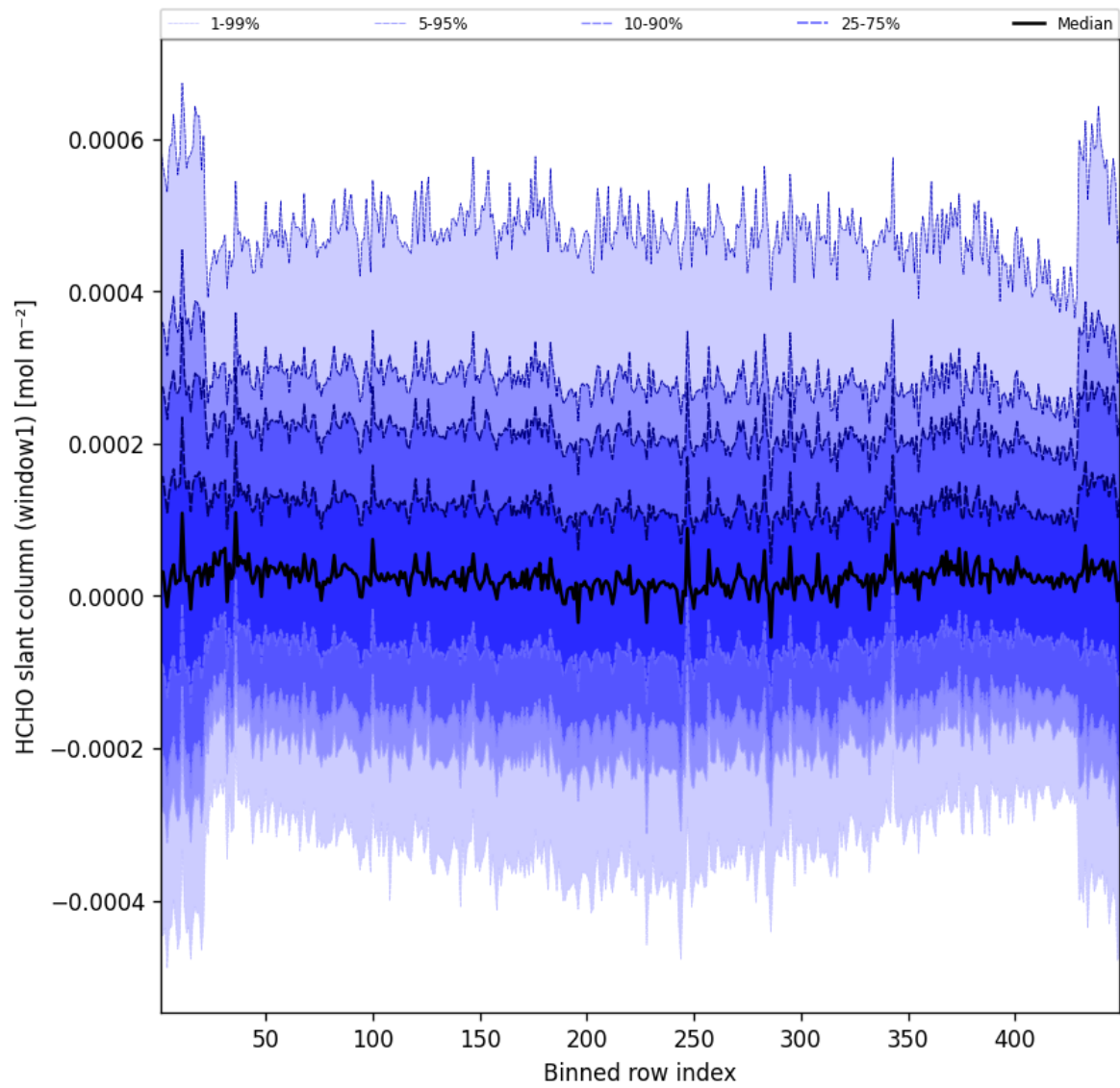
Figure 50: Along track statistics of “HCHO slant column (window1)” for 2025-07-02 to 2025-07-03
