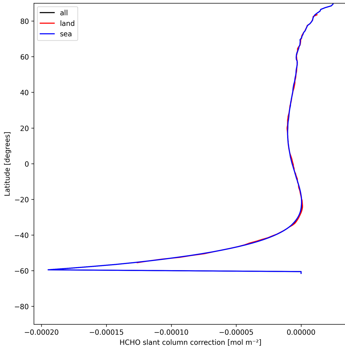
Figure 31: Zonal average of “HCHO slant column correction” for 2025-07-02 to 2025-07-03.
