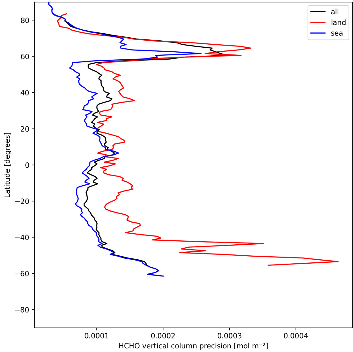
Figure 20: Zonal average of “HCHO vertical column precision” for 2025-07-02 to 2025-07-03.
