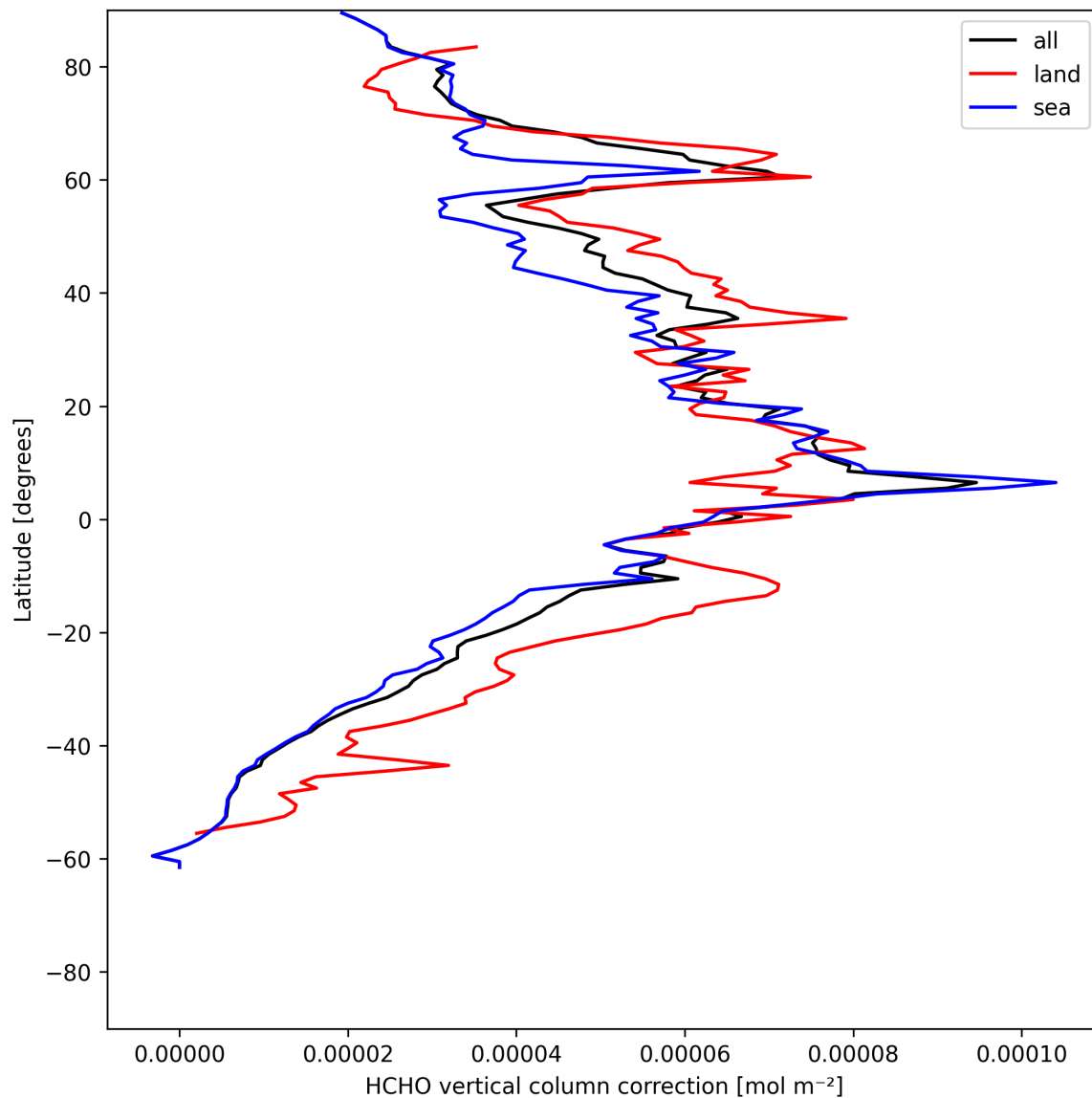
Figure 21: Zonal average of “HCHO vertical column correction” for 2025-07-02 to 2025-07-03.
