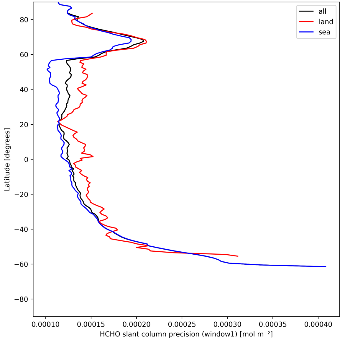
Figure 23: Zonal average of "HCHO slant column precision (window1)" for 2025-07-02 to 2025-07-03.
