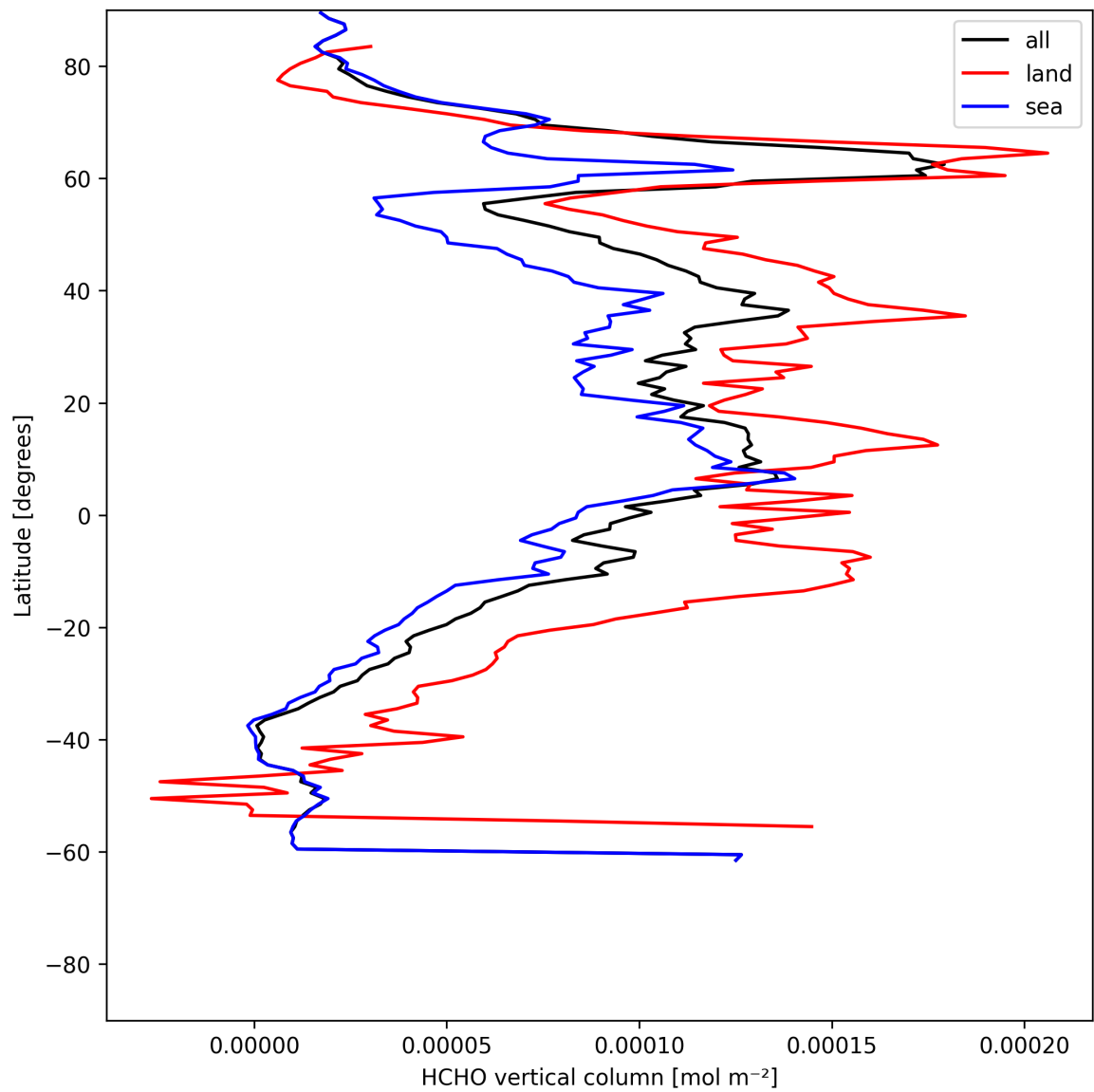
Figure 19: Zonal average of “HCHO vertical column” for 2025-07-02 to 2025-07-03.
