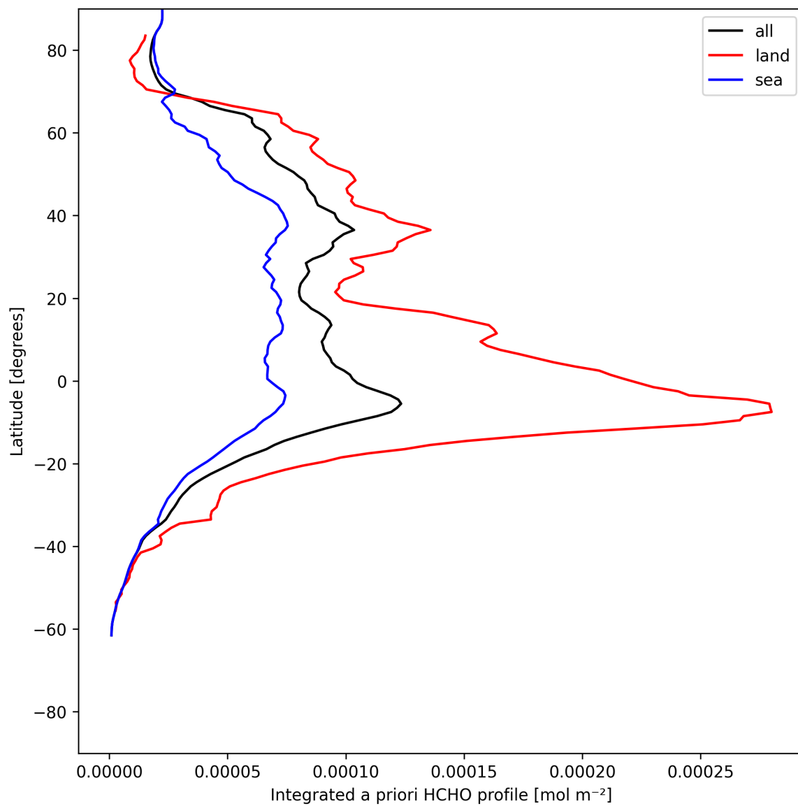
Figure 27: Zonal average of “Integrated a priori HCHO profile” for 2025-07-02 to 2025-07-03.
