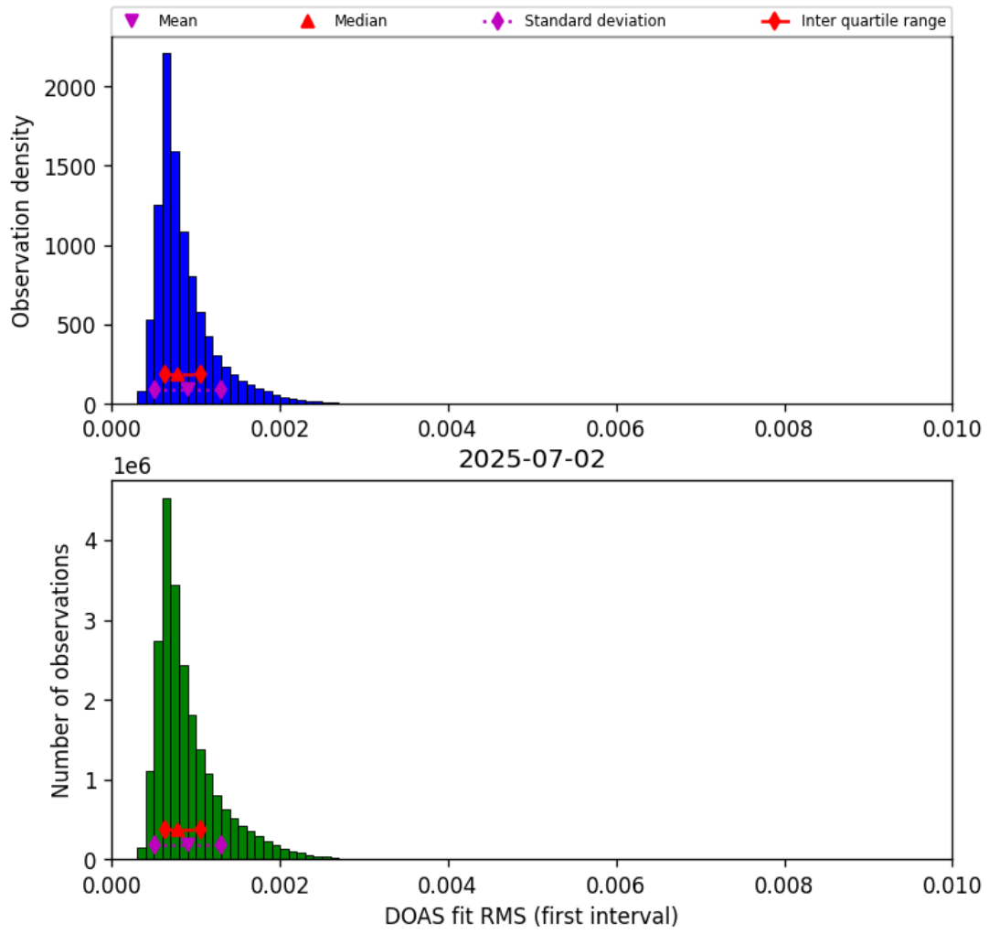
Figure 44: Histogram of “DOAS fit RMS (first interval)” for 2025-07-02 to 2025-07-03
