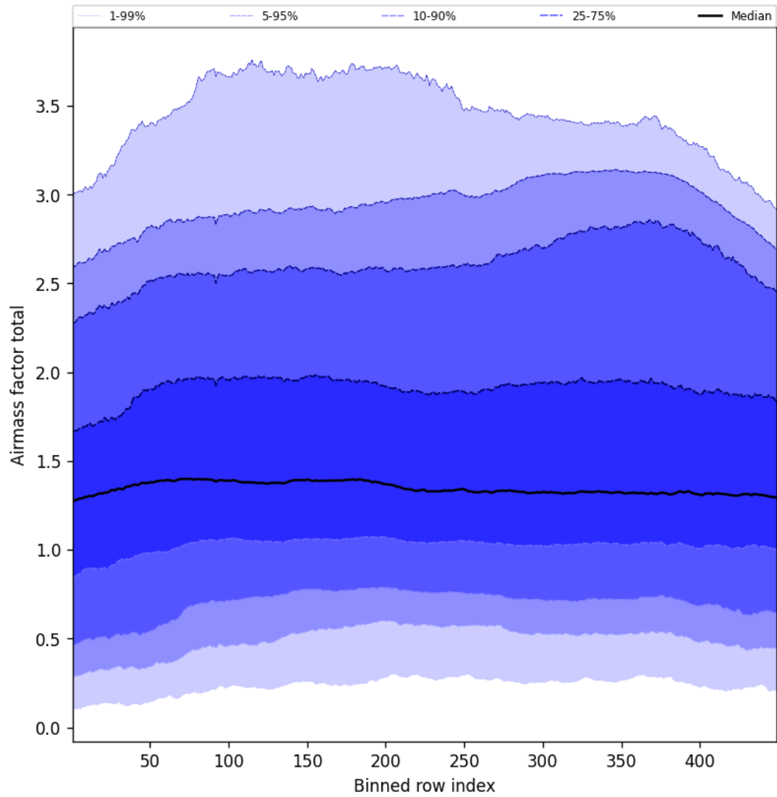
Figure 52: Along track statistics of “Airmass factor total” for 2025-07-02 to 2025-07-03
