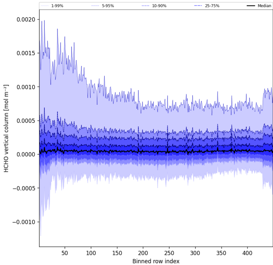
Figure 47: Along track statistics of “HCHO vertical column” for 2025-07-02 to 2025-07-03
