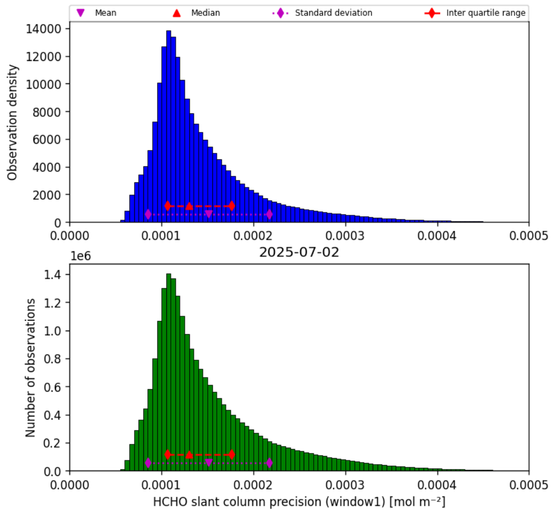
Figure 37: Histogram of “HCHO slant column precision (window1)” for 2025-07-02 to 2025-07-03
