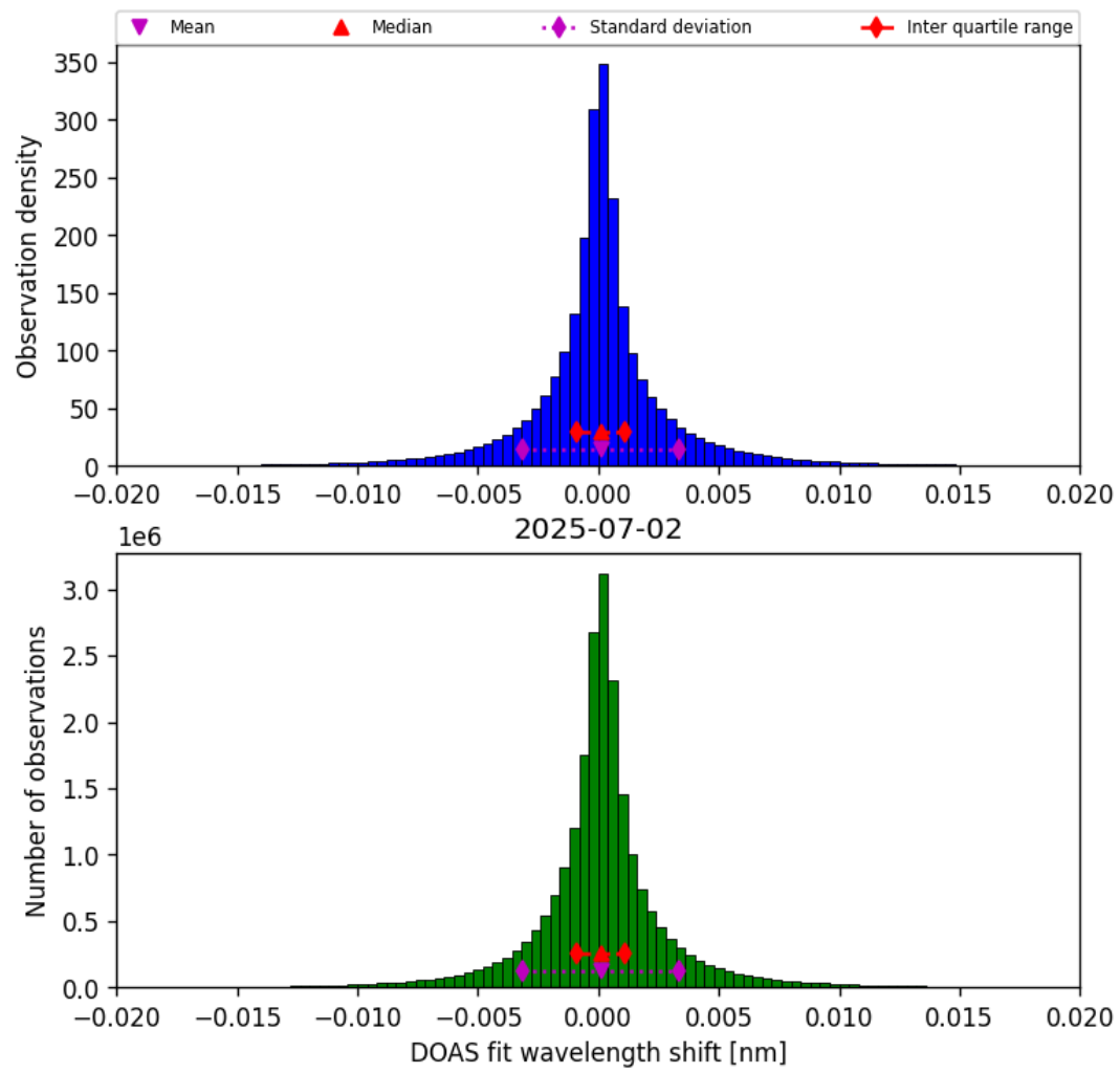
Figure 42: Histogram of “DOAS fit wavelength shift” for 2025-07-02 to 2025-07-03
