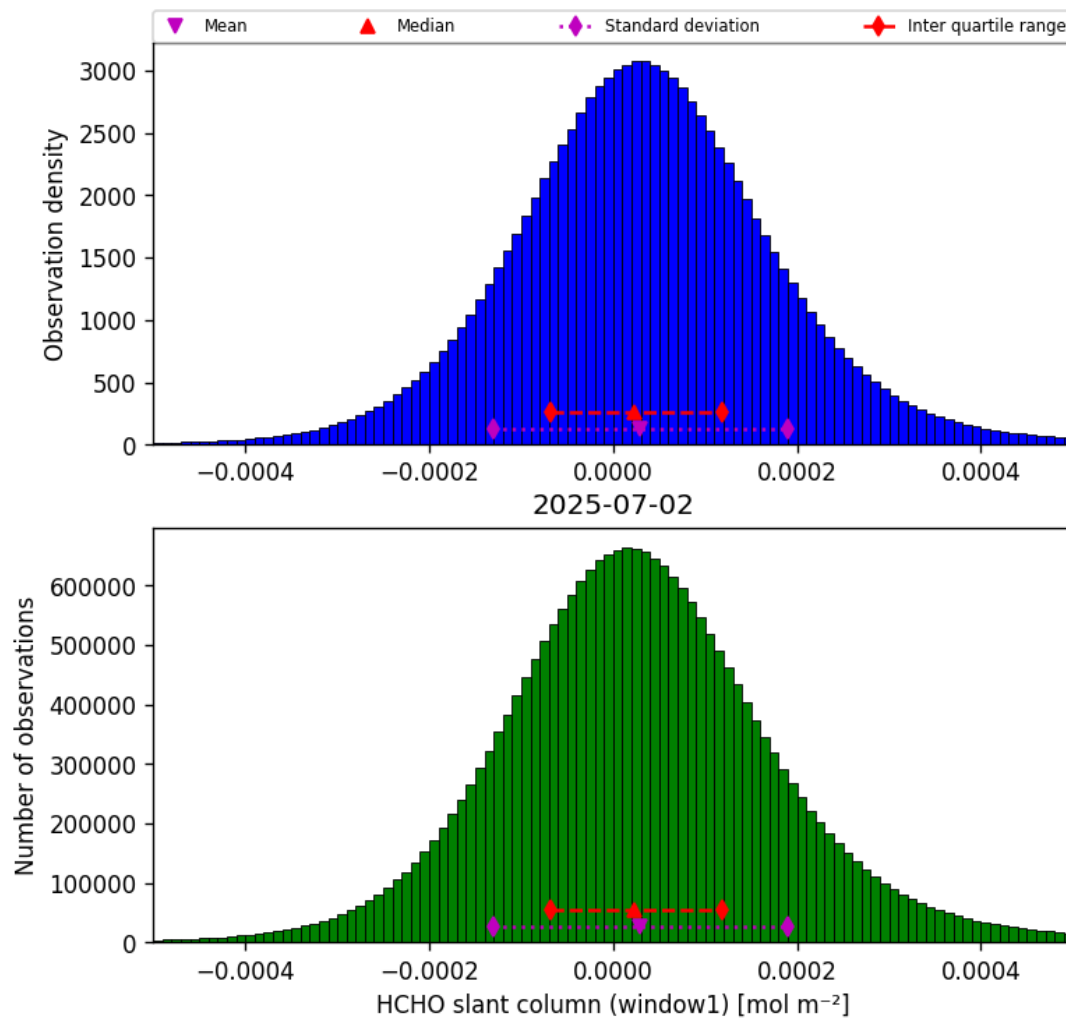
Figure 36: Histogram of “HCHO slant column (window1)” for 2025-07-02 to 2025-07-03
