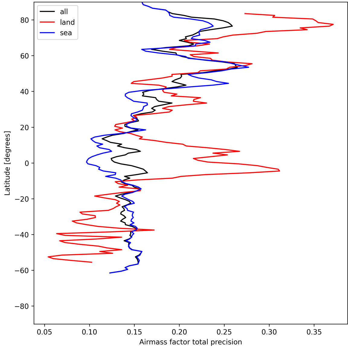
Figure 25: Zonal average of “Airmass factor total precision” for 2025-07-02 to 2025-07-03.
