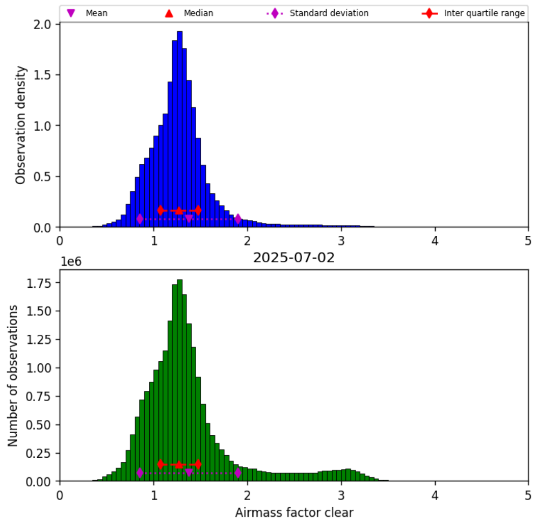
Figure 40: Histogram of “Airmass factor clear” for 2025-07-02 to 2025-07-03
