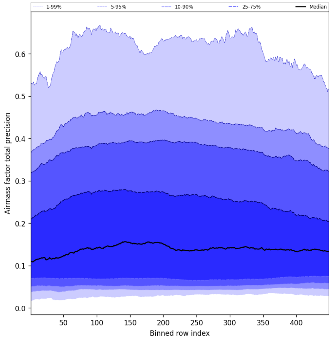
Figure 53: Along track statistics of “Airmass factor total precision” for 2025-07-02 to 2025-07-03
