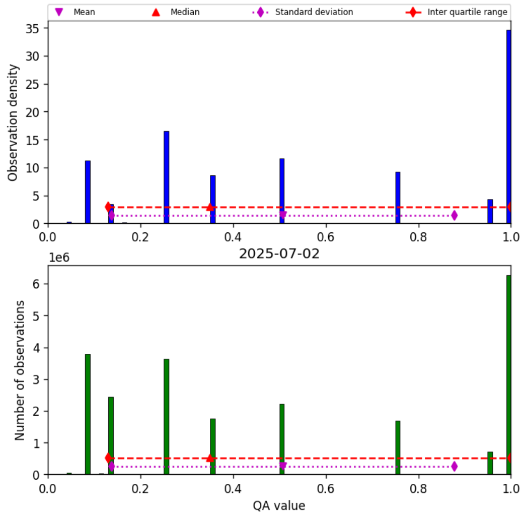
Figure 32: Histogram of “QA value” for 2025-07-02 to 2025-07-03
