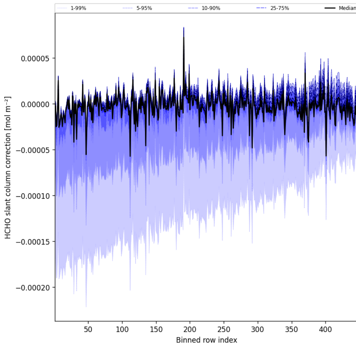
Figure 59: Along track statistics of “HCHO slant column correction” for 2025-07-02 to 2025-07-03
