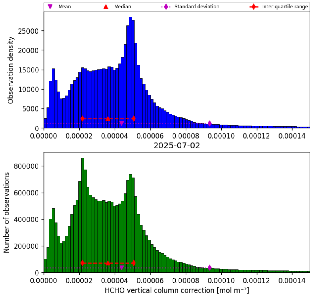
Figure 35: Histogram of “HCHO vertical column correction” for 2025-07-02 to 2025-07-03
