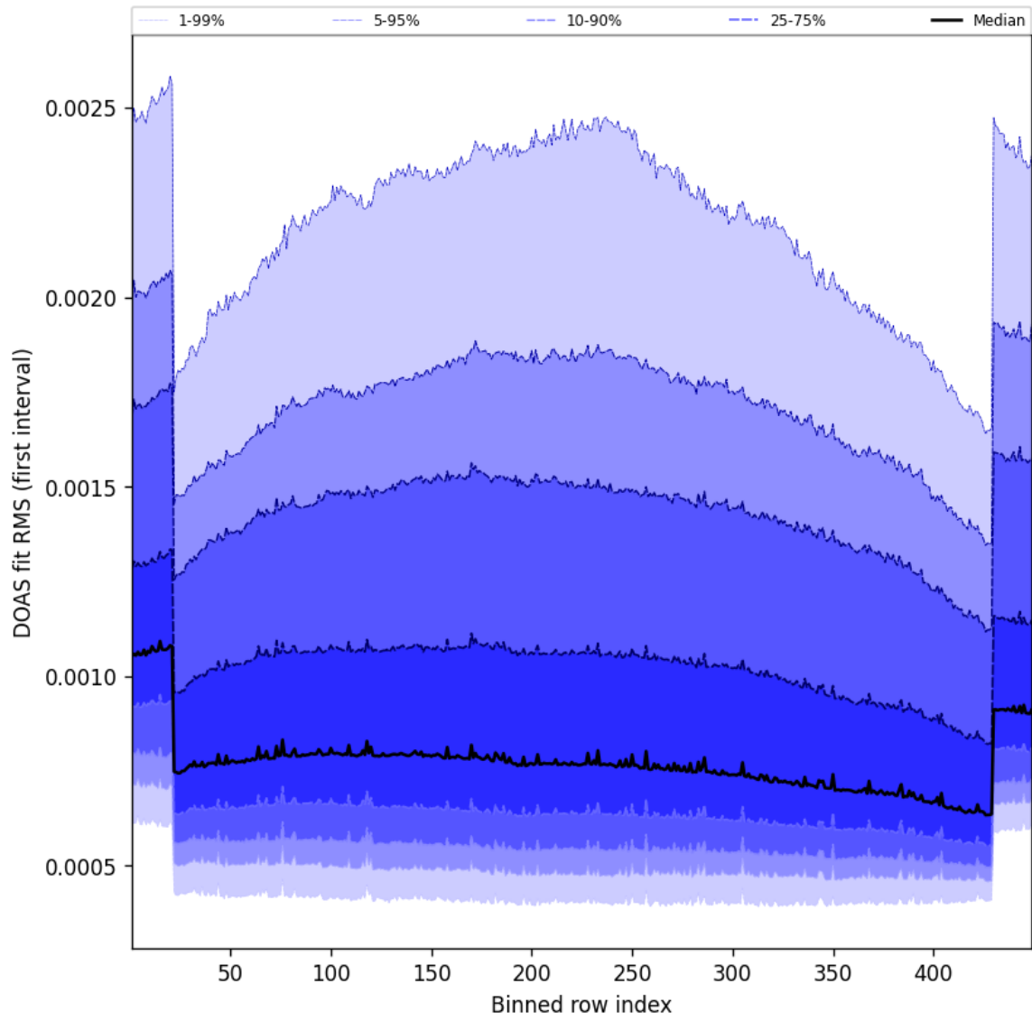
Figure 58: Along track statistics of “DOAS fit RMS (first interval)” for 2025-07-02 to 2025-07-03
