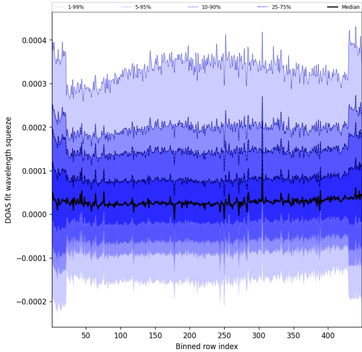
Figure 57: Along track statistics of “DOAS fit wavelength squeeze” for 2025-07-02 to 2025-07-03
