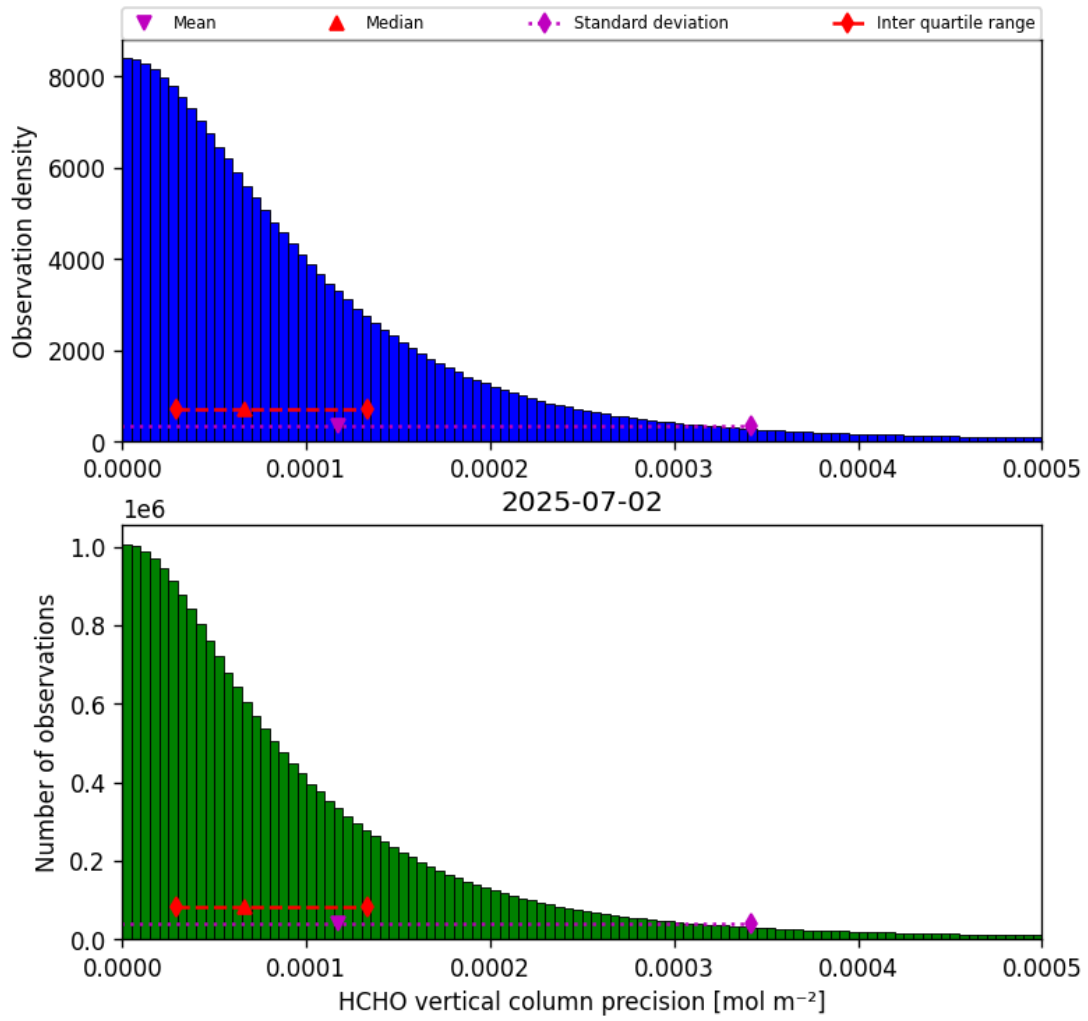
Figure 34: Histogram of “HCHO vertical column precision” for 2025-07-02 to 2025-07-03
