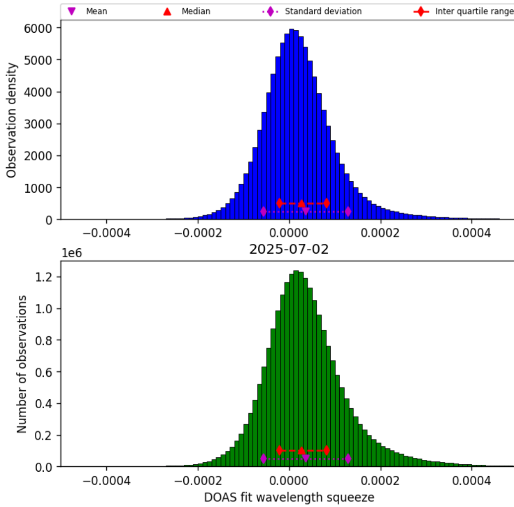
Figure 43: Histogram of “DOAS fit wavelength squeeze” for 2025-07-02 to 2025-07-03
