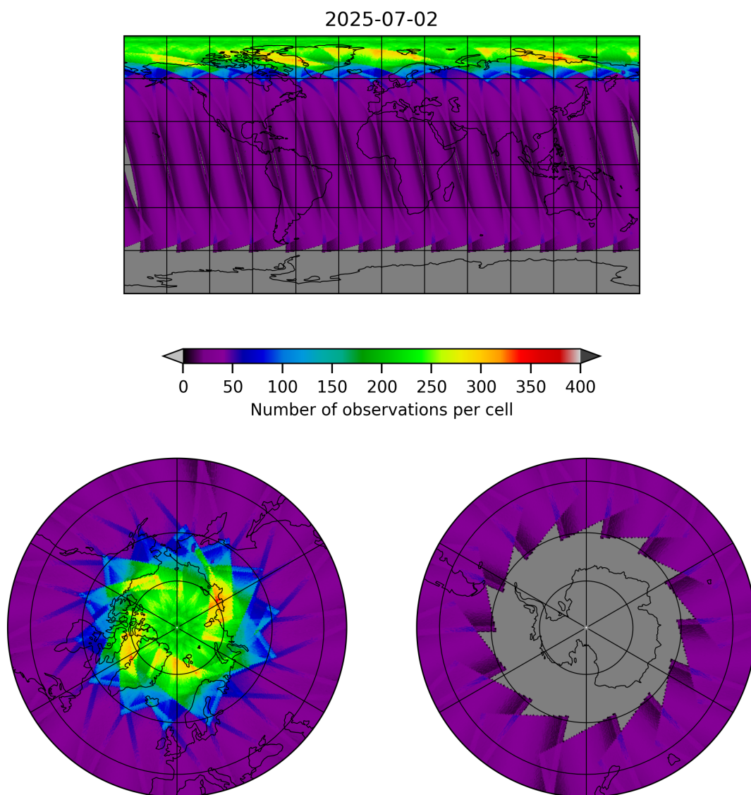
Figure 17: Map of the number of observations for 2025-07-02 to 2025-07-03
