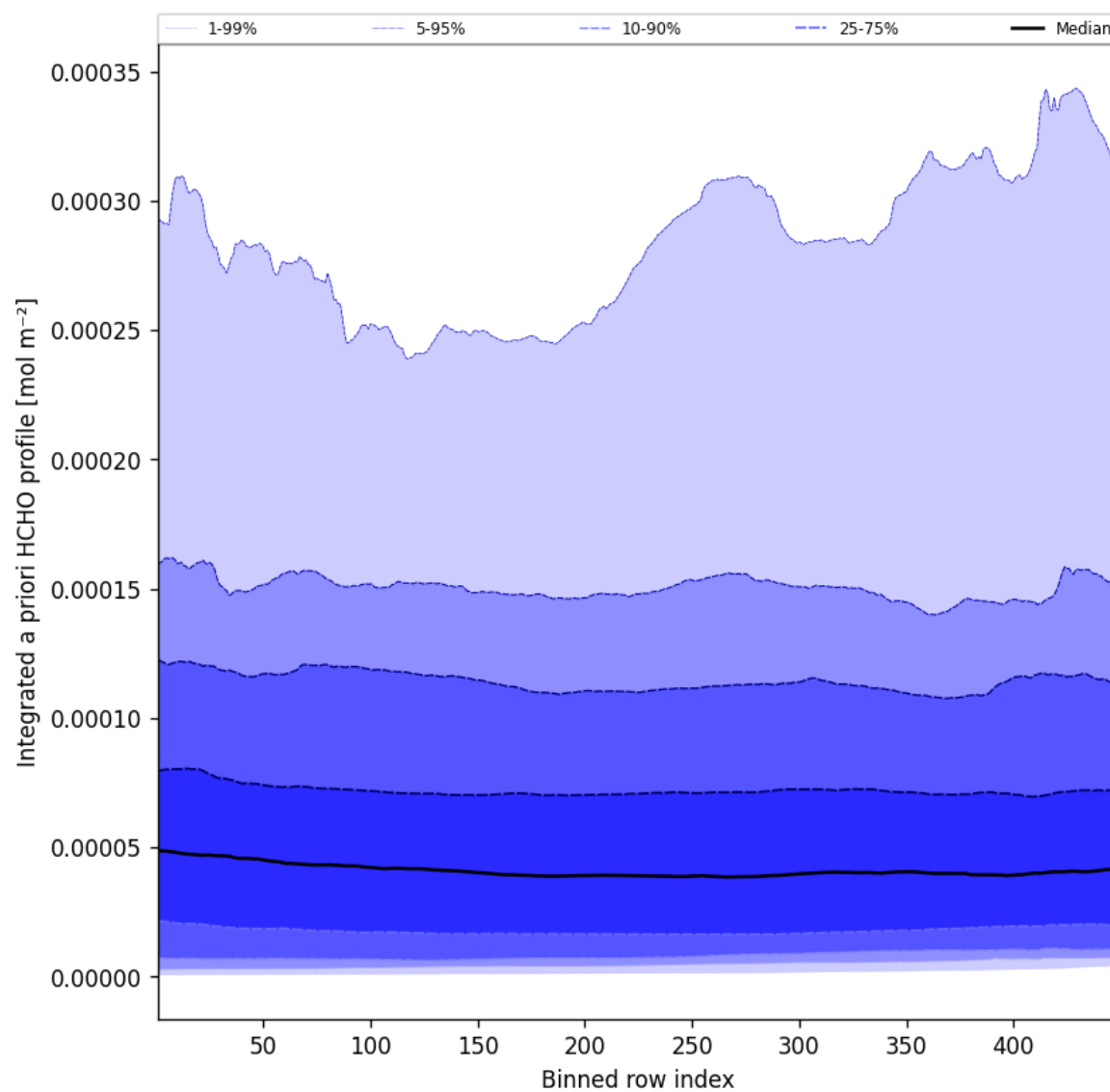
Figure 55: Along track statistics of “Integrated a priori HCHO profile” for 2025-07-02 to 2025-07-03
