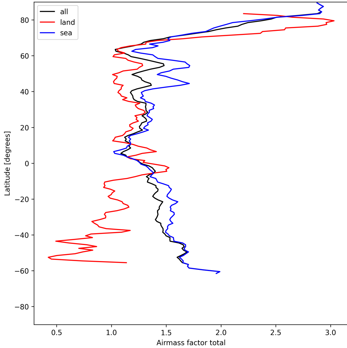
Figure 24: Zonal average of “Airmass factor total” for 2025-07-02 to 2025-07-03.
