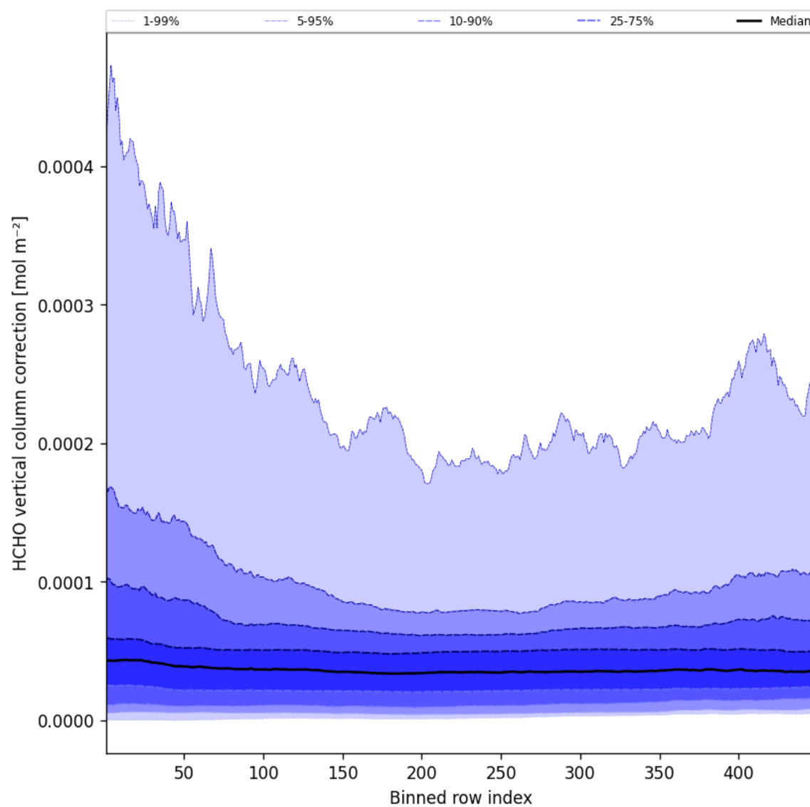
Figure 49: Along track statistics of “HCHO vertical column correction” for 2025-07-02 to 2025-07-03
