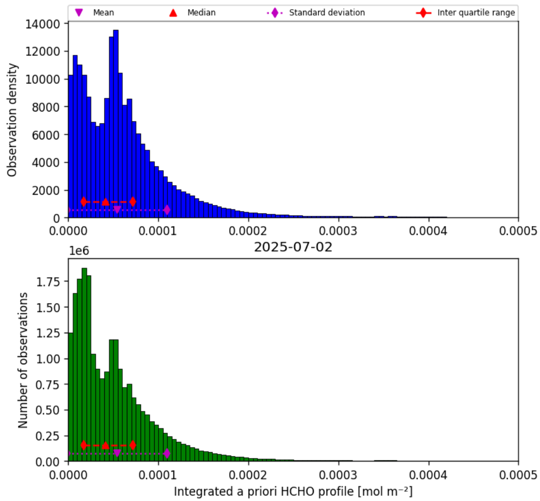
Figure 41: Histogram of “Integrated a priori HCHO profile” for 2025-07-02 to 2025-07-03
