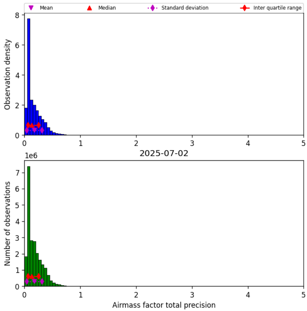
Figure 39: Histogram of “Airmass factor total precision” for 2025-07-02 to 2025-07-03
