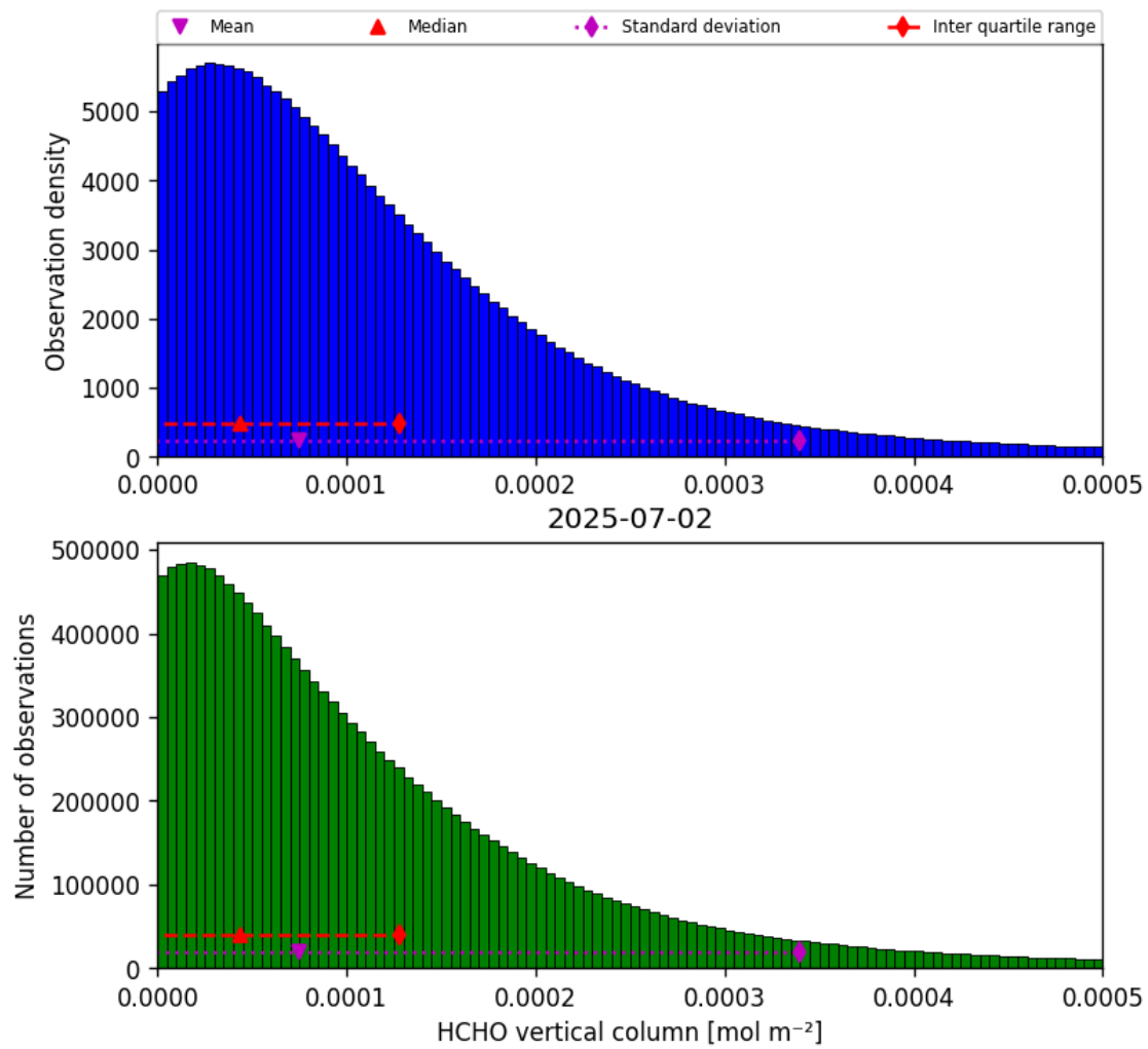
Figure 33: Histogram of “HCHO vertical column” for 2025-07-02 to 2025-07-03
