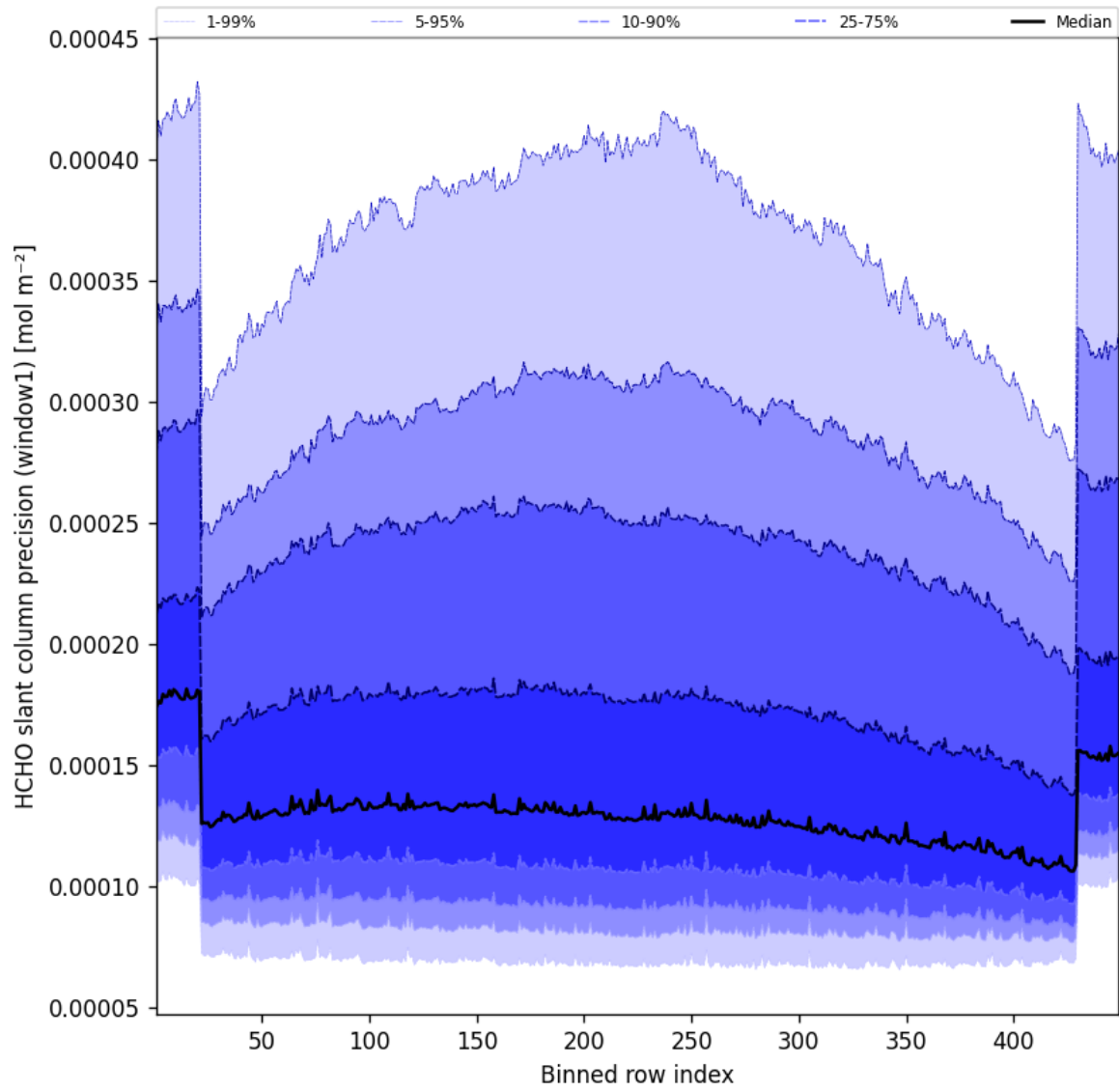
Figure 51: Along track statistics of “HCHO slant column precision (window1)” for 2025-07-02 to 2025-07-03
