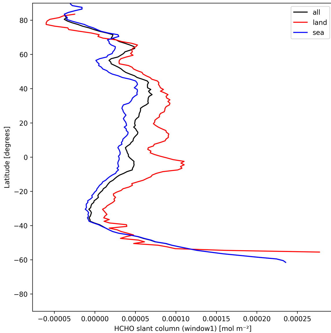
Figure 22: Zonal average of “HCHO slant column (window1)” for 2025-07-02 to 2025-07-03.
