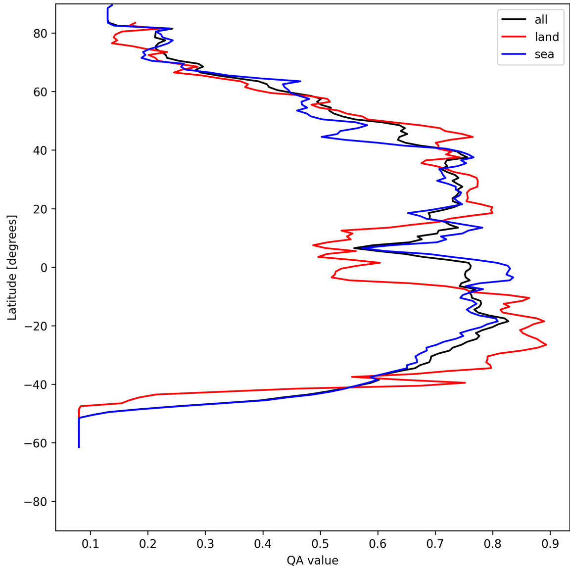
Figure 18: Zonal average of “QA value” for 2025-07-02 to 2025-07-03.
