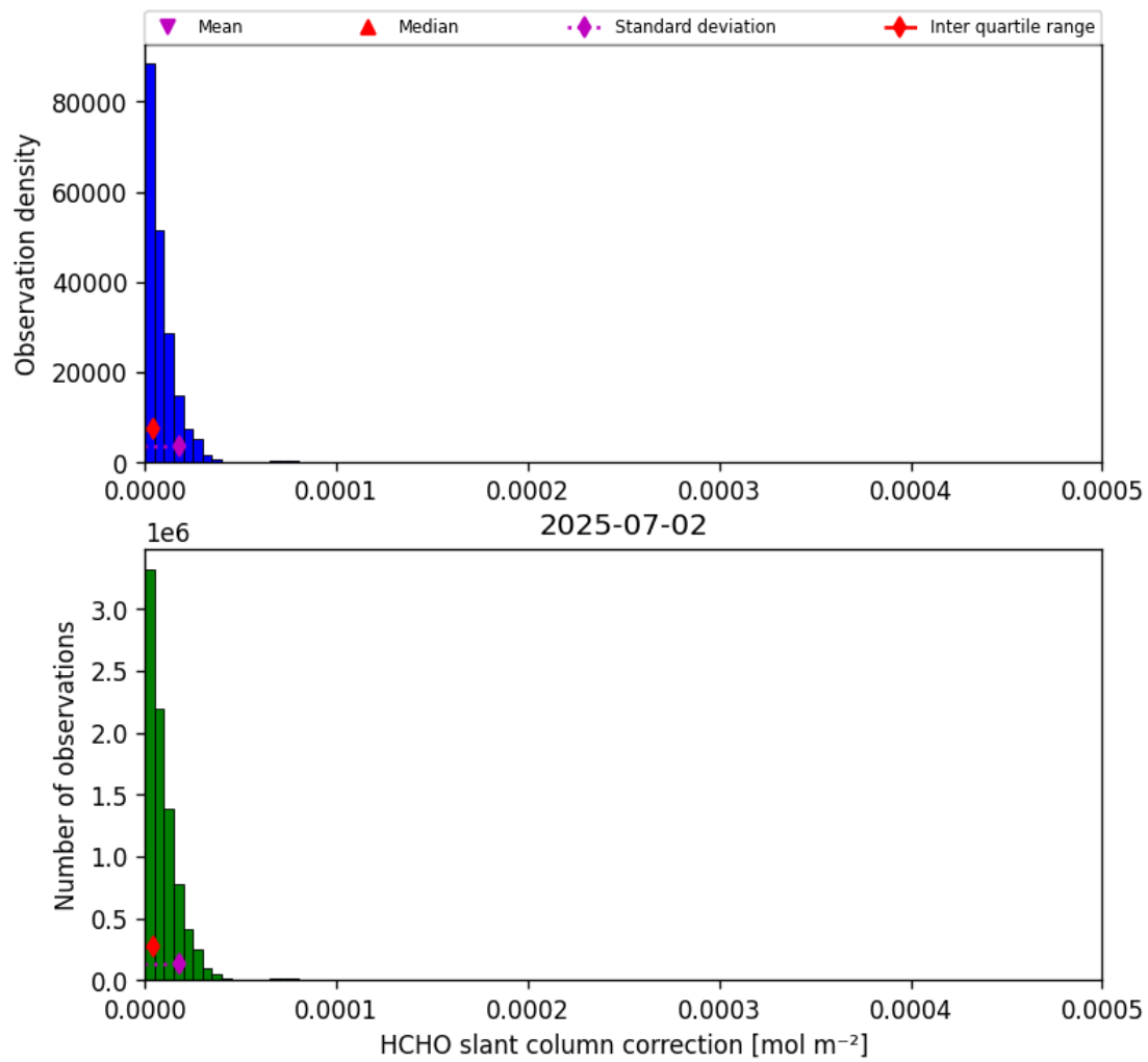
Figure 45: Histogram of “HCHO slant column correction” for 2025-07-02 to 2025-07-03
