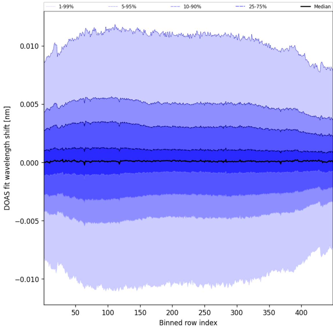
Figure 56: Along track statistics of “DOAS fit wavelength shift” for 2025-07-02 to 2025-07-03
