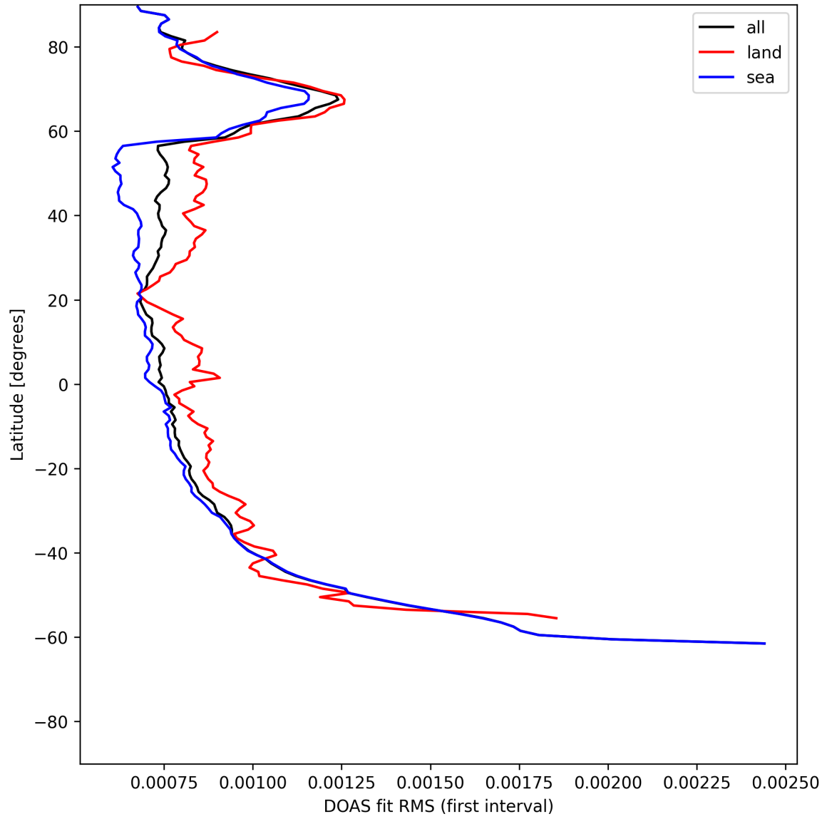
Figure 30: Zonal average of "DOAS fit RMS (first interval)" for 2025-07-02 to 2025-07-03.
