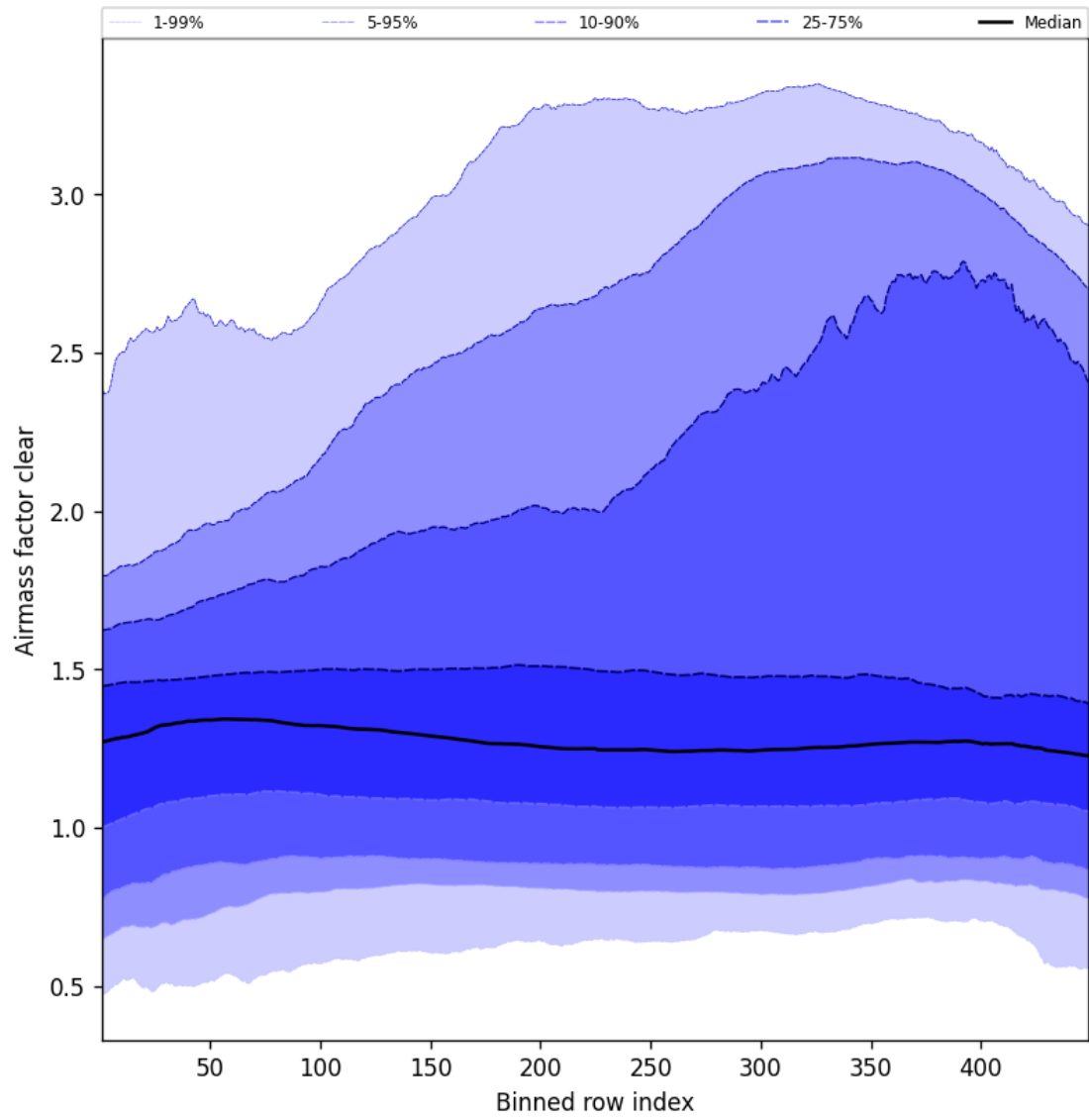
Figure 54: Along track statistics of “Airmass factor clear” for 2025-07-02 to 2025-07-03
