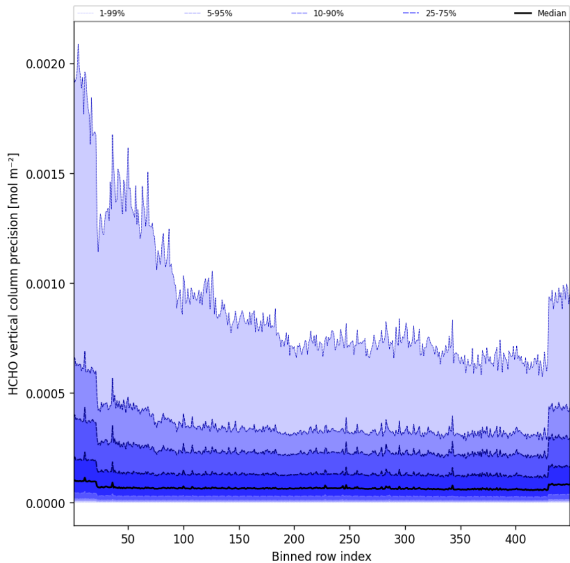
Figure 48: Along track statistics of “HCHO vertical column precision” for 2025-07-02 to 2025-07-03
