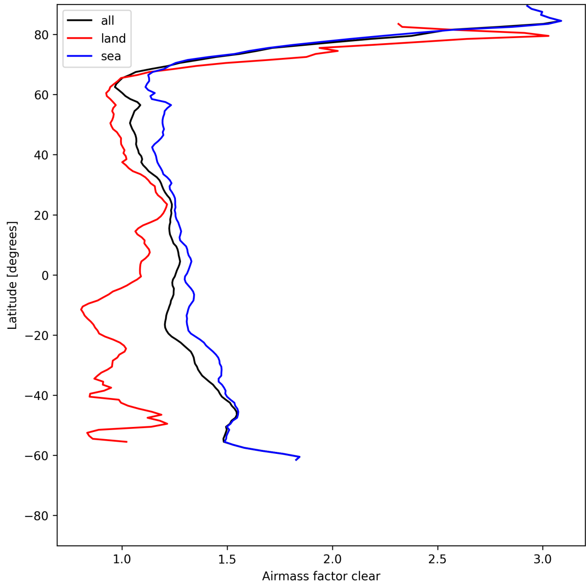
Figure 26: Zonal average of “Airmass factor clear” for 2025-07-02 to 2025-07-03.
