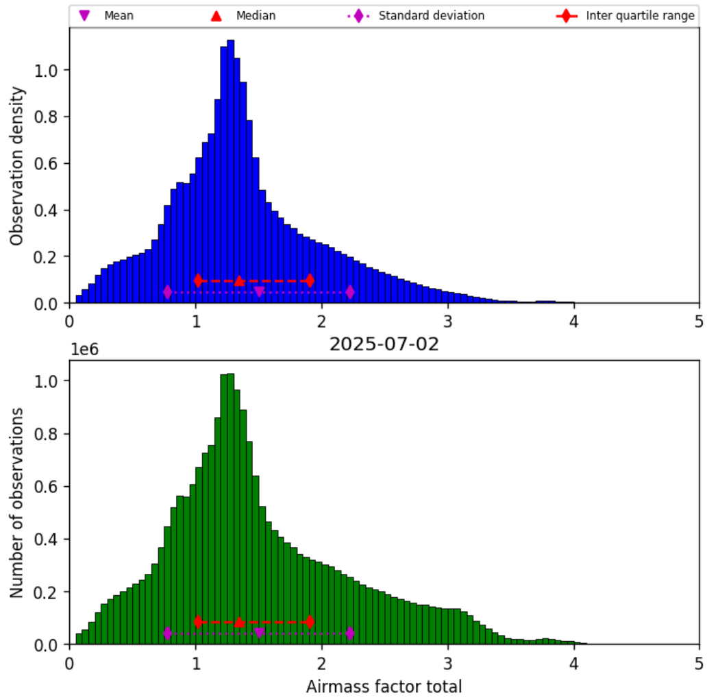
Figure 38: Histogram of “Airmass factor total” for 2025-07-02 to 2025-07-03
