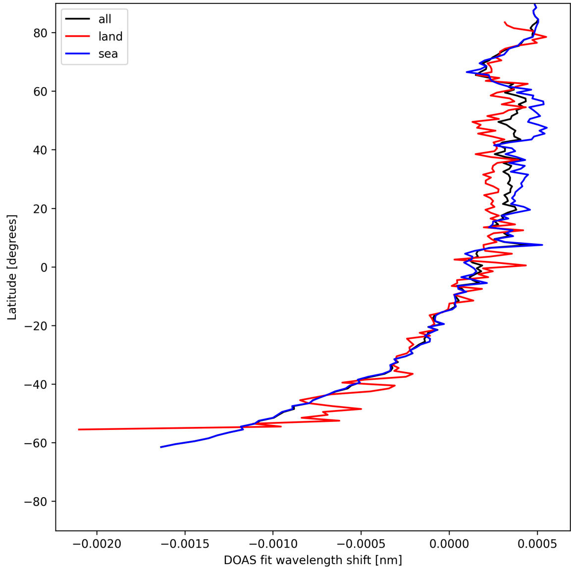
Figure 28: Zonal average of “DOAS fit wavelength shift” for 2025-07-02 to 2025-07-03.
