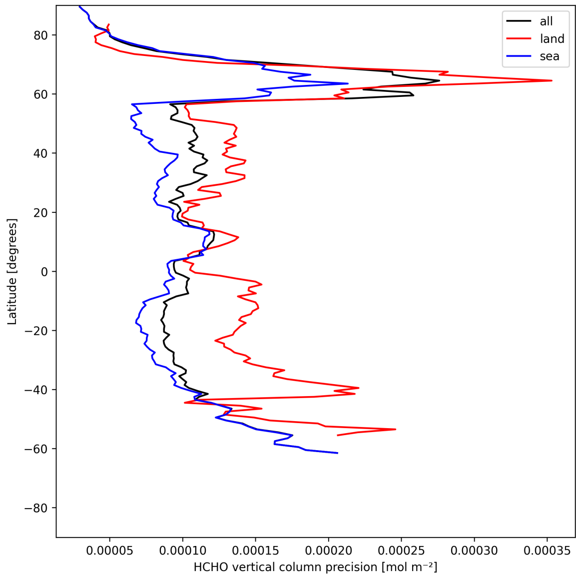
Figure 20: Zonal average of “HCHO vertical column precision” for 2025-07-03 to 2025-07-04.
