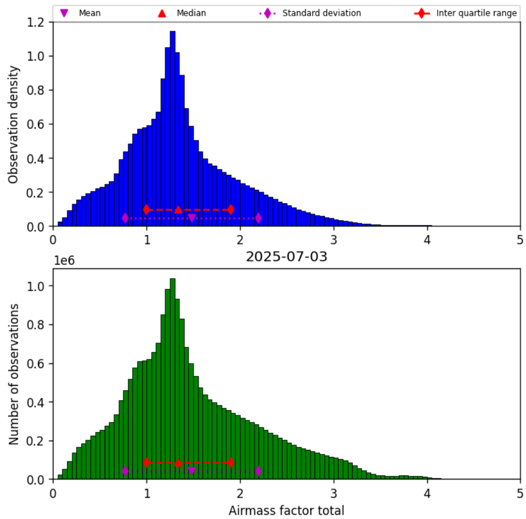
Figure 38: Histogram of “Airmass factor total” for 2025-07-03 to 2025-07-04
