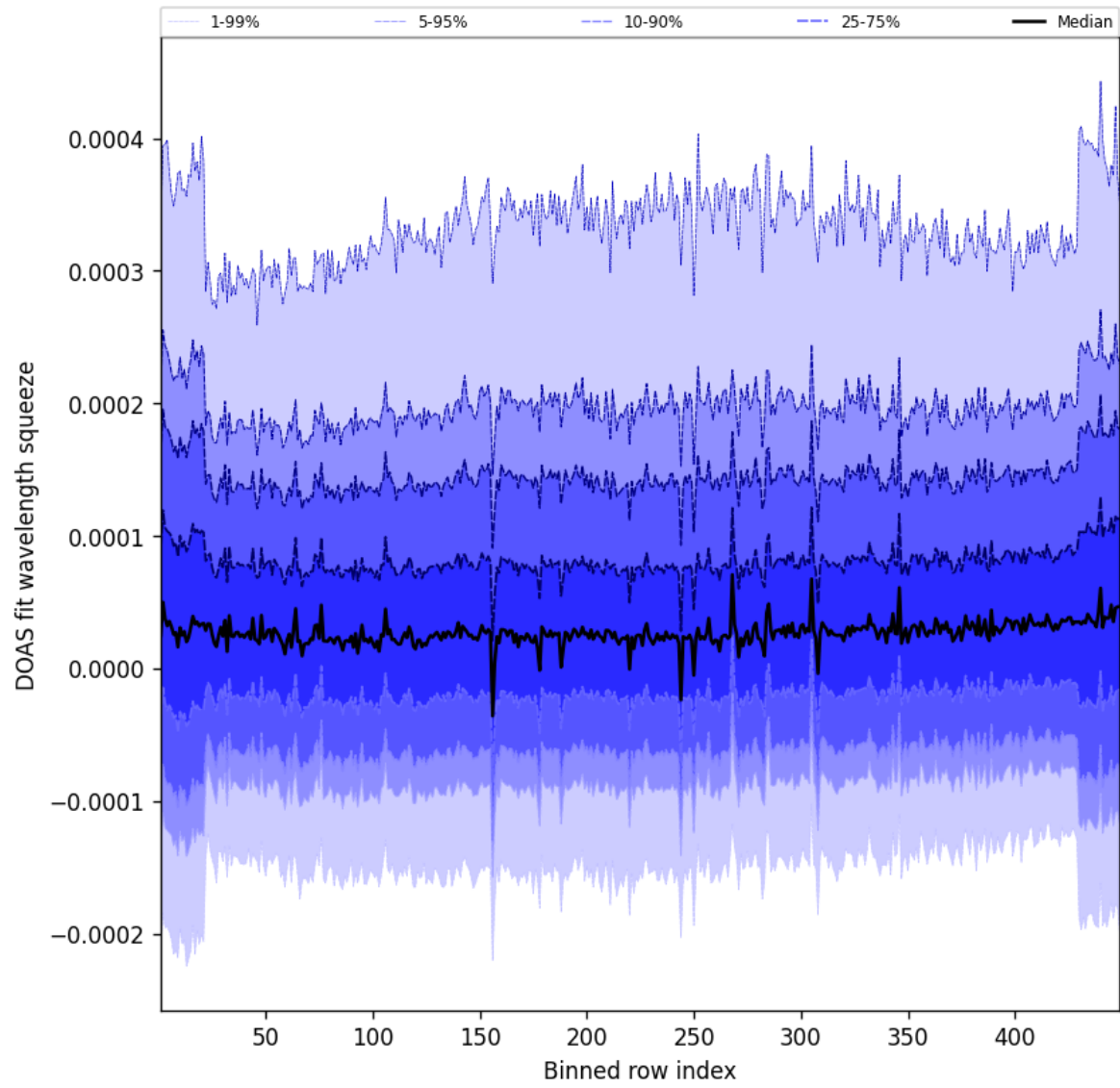
Figure 57: Along track statistics of “DOAS fit wavelength squeeze” for 2025-07-03 to 2025-07-04
