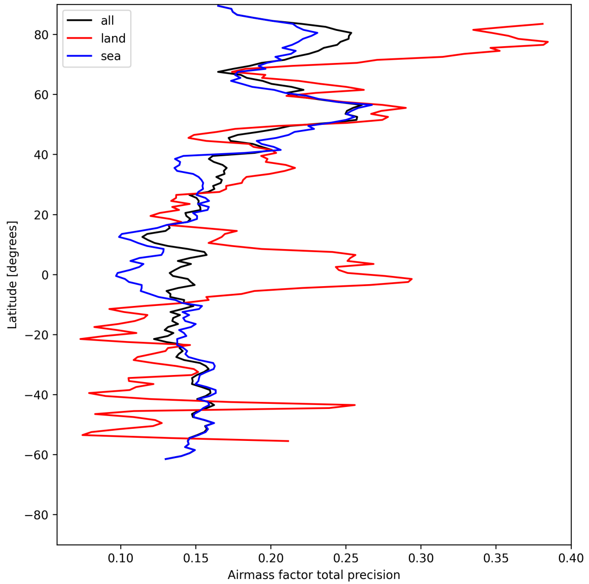
Figure 25: Zonal average of “Airmass factor total precision” for 2025-07-03 to 2025-07-04.
