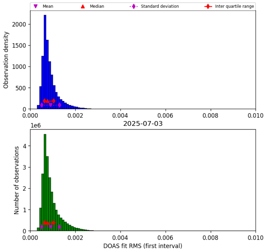
Figure 44: Histogram of “DOAS fit RMS (first interval)” for 2025-07-03 to 2025-07-04
