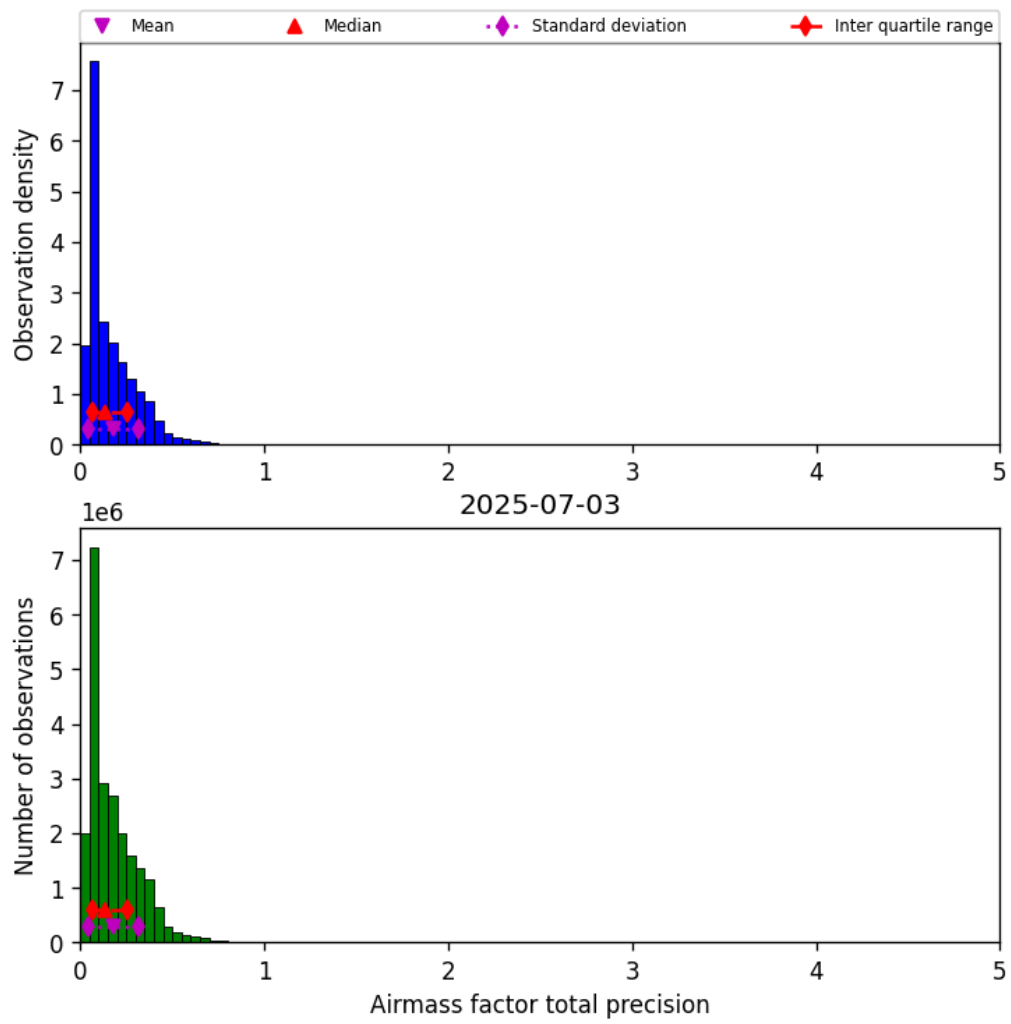
Figure 39: Histogram of “Airmass factor total precision” for 2025-07-03 to 2025-07-04
