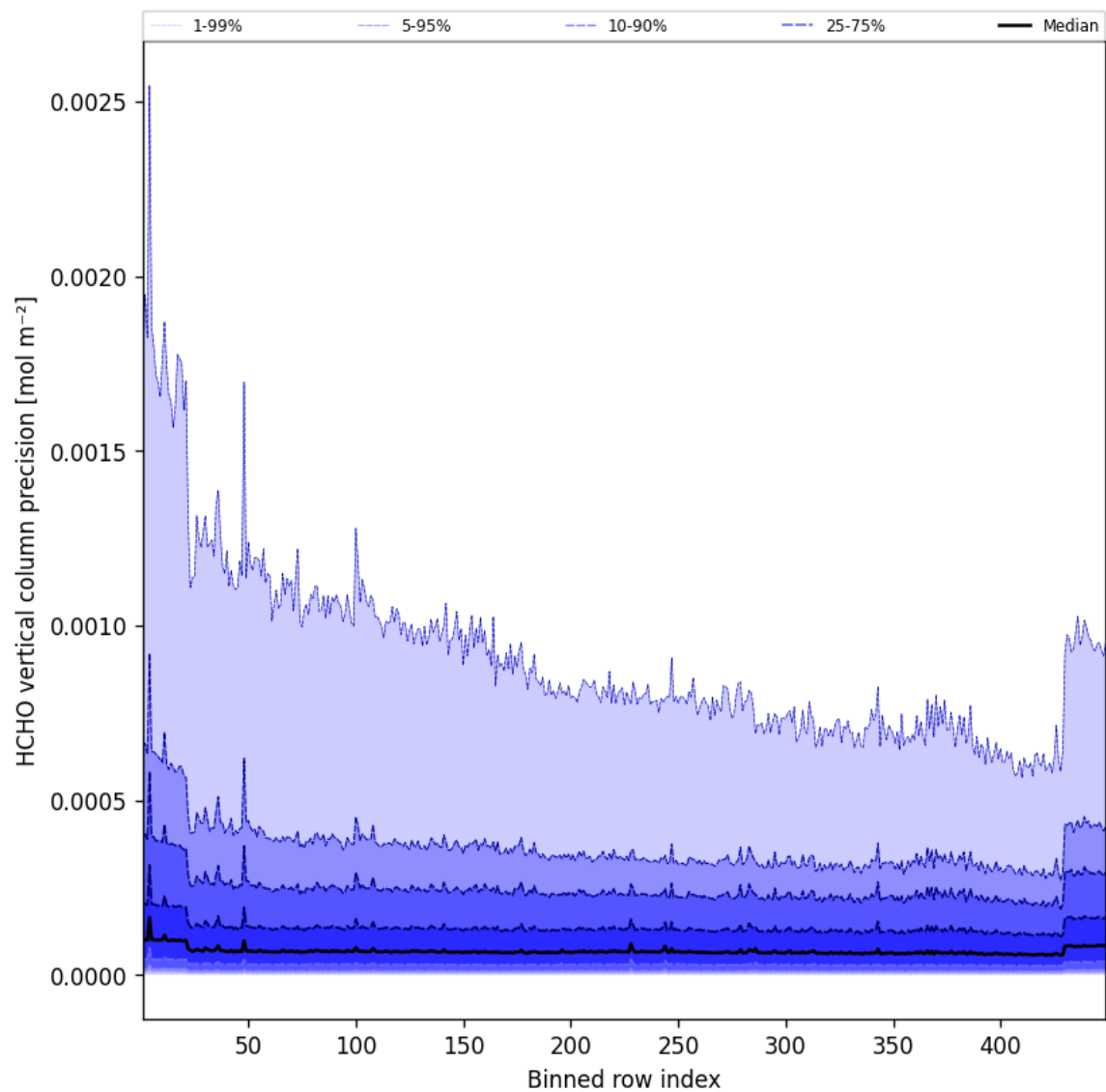
Figure 48: Along track statistics of “HCHO vertical column precision” for 2025-07-03 to 2025-07-04
