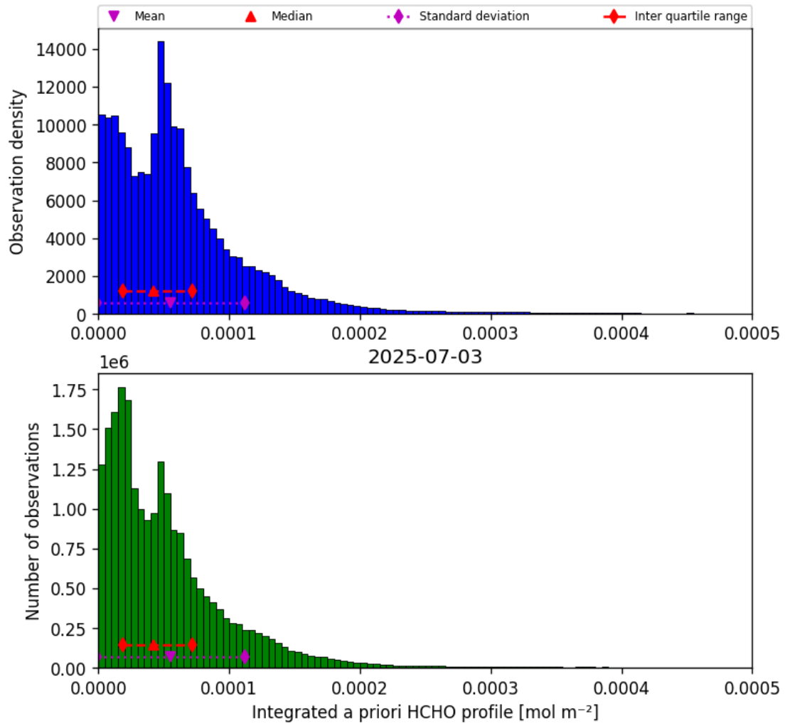
Figure 41: Histogram of “Integrated a priori HCHO profile” for 2025-07-03 to 2025-07-04
