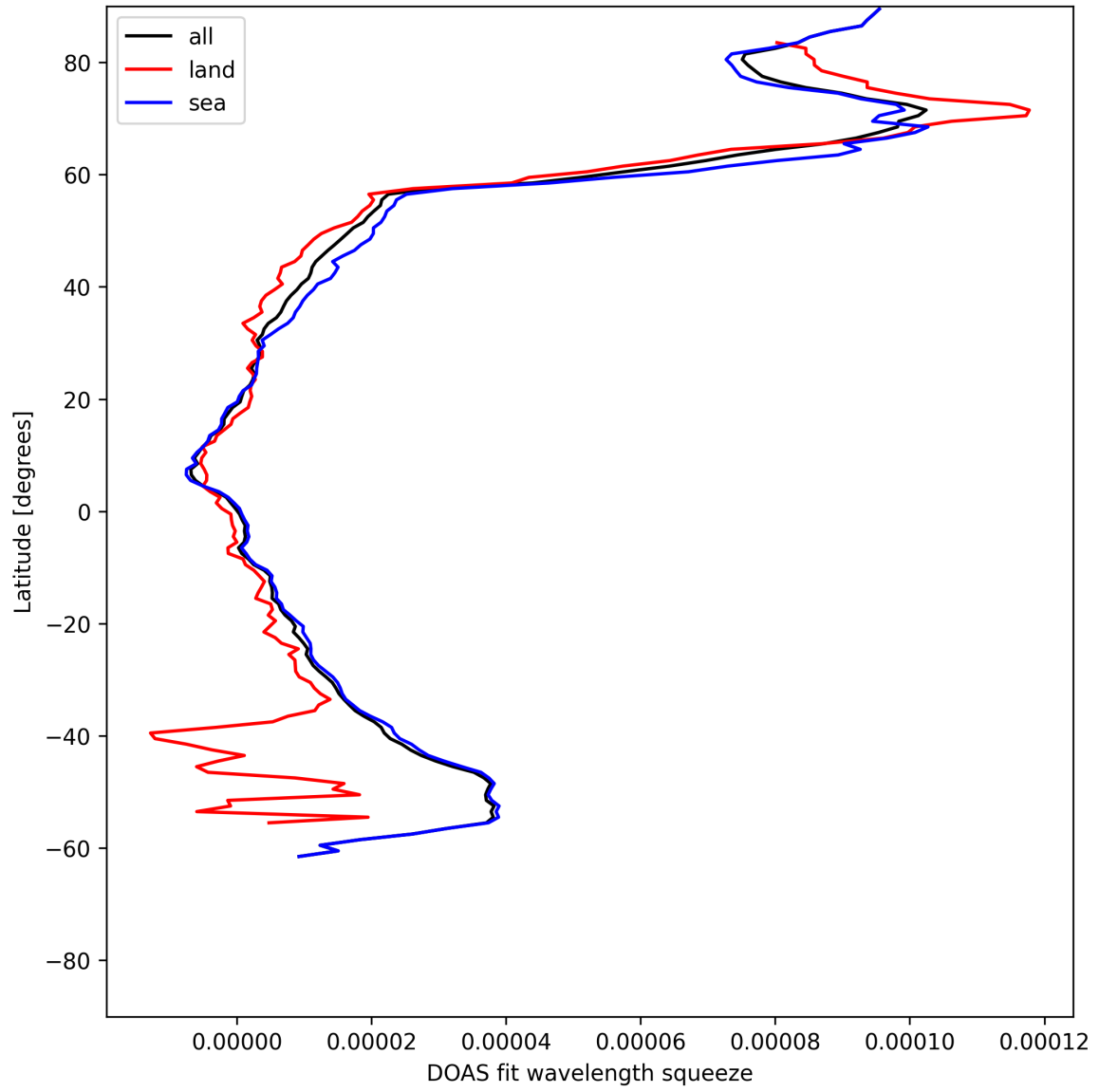
Figure 29: Zonal average of “DOAS fit wavelength squeeze” for 2025-07-03 to 2025-07-04.
