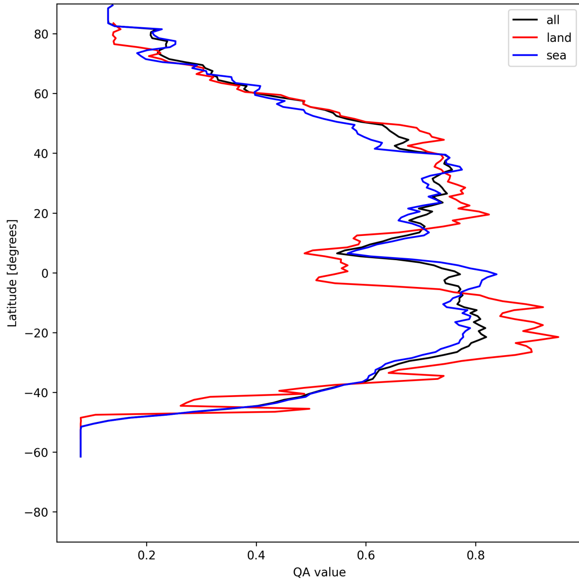
Figure 18: Zonal average of “QA value” for 2025-07-03 to 2025-07-04.
