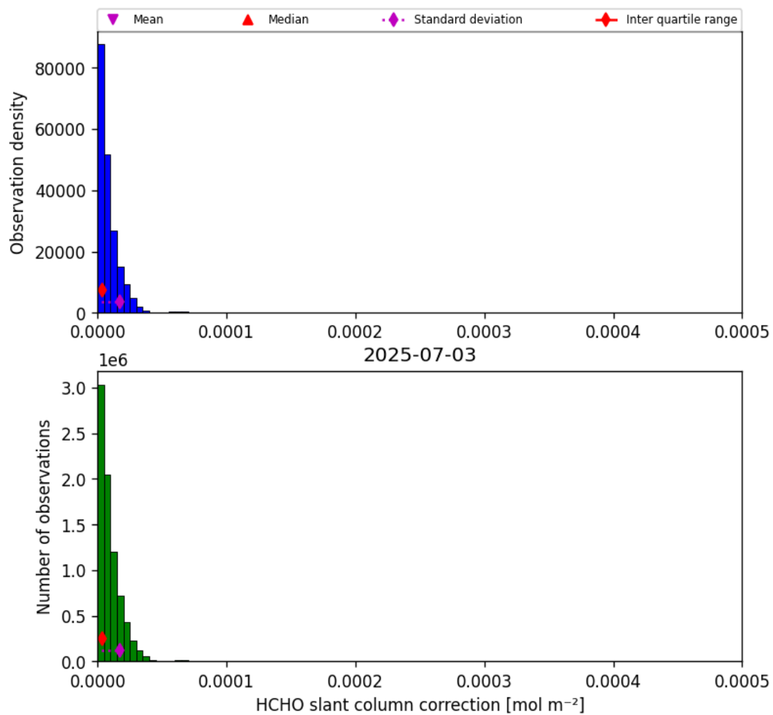
Figure 45: Histogram of “HCHO slant column correction” for 2025-07-03 to 2025-07-04
