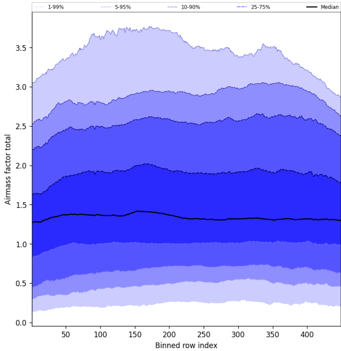
Figure 52: Along track statistics of “Airmass factor total” for 2025-07-03 to 2025-07-04
