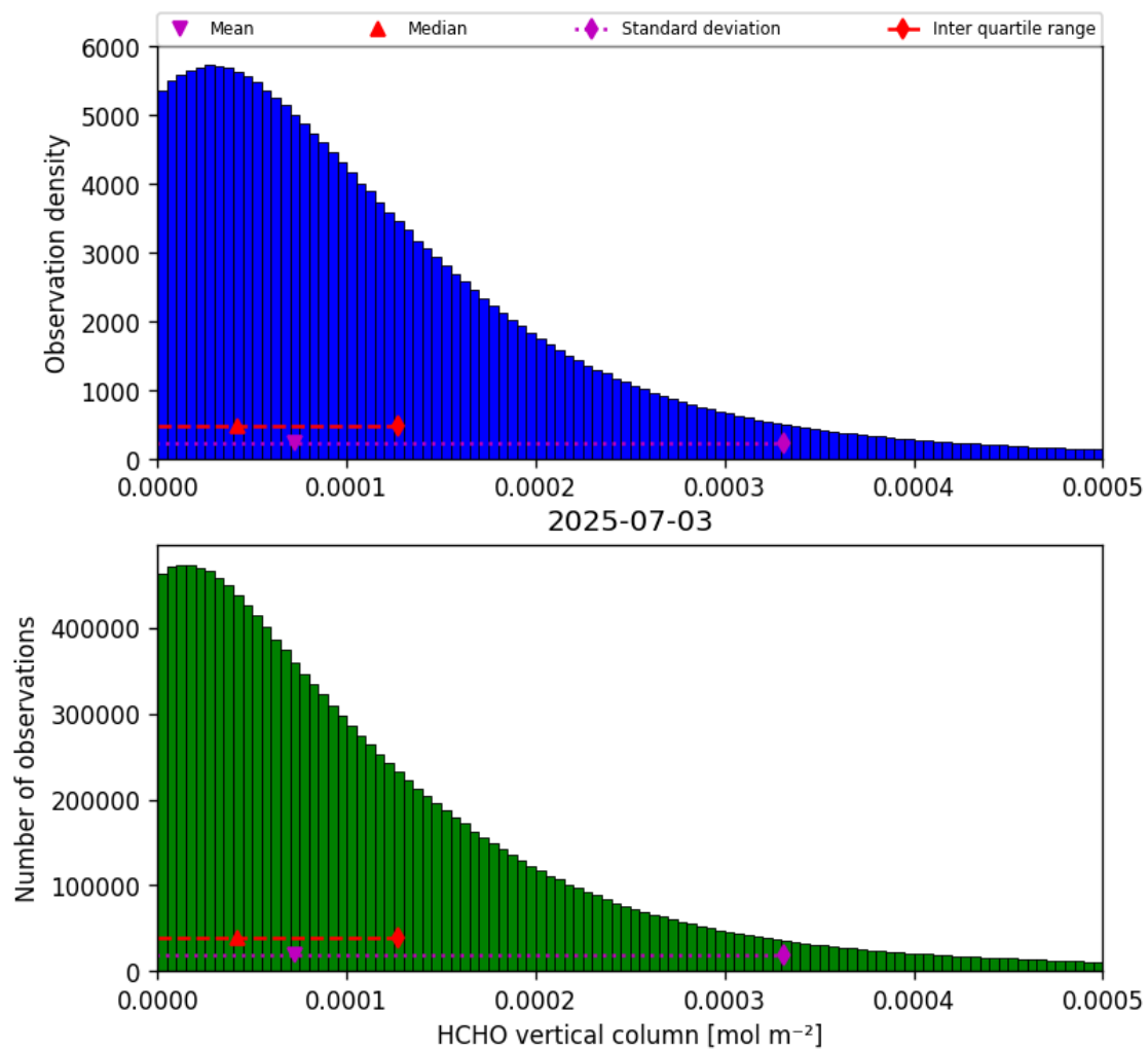
Figure 33: Histogram of “HCHO vertical column” for 2025-07-03 to 2025-07-04
