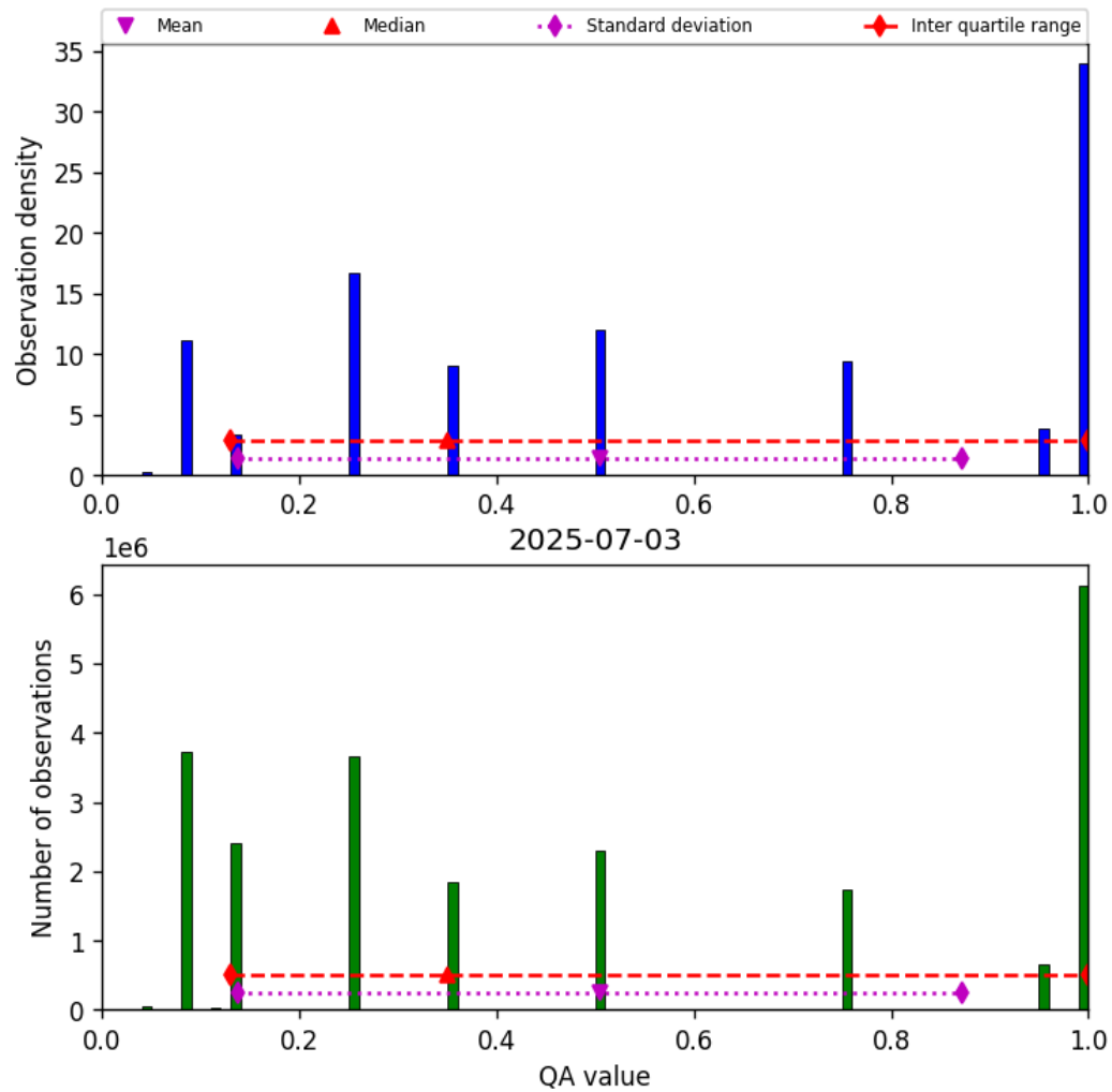
Figure 32: Histogram of “QA value” for 2025-07-03 to 2025-07-04
