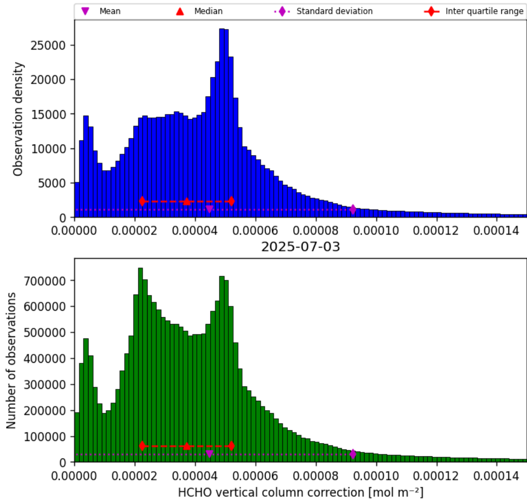
Figure 35: Histogram of “HCHO vertical column correction” for 2025-07-03 to 2025-07-04
