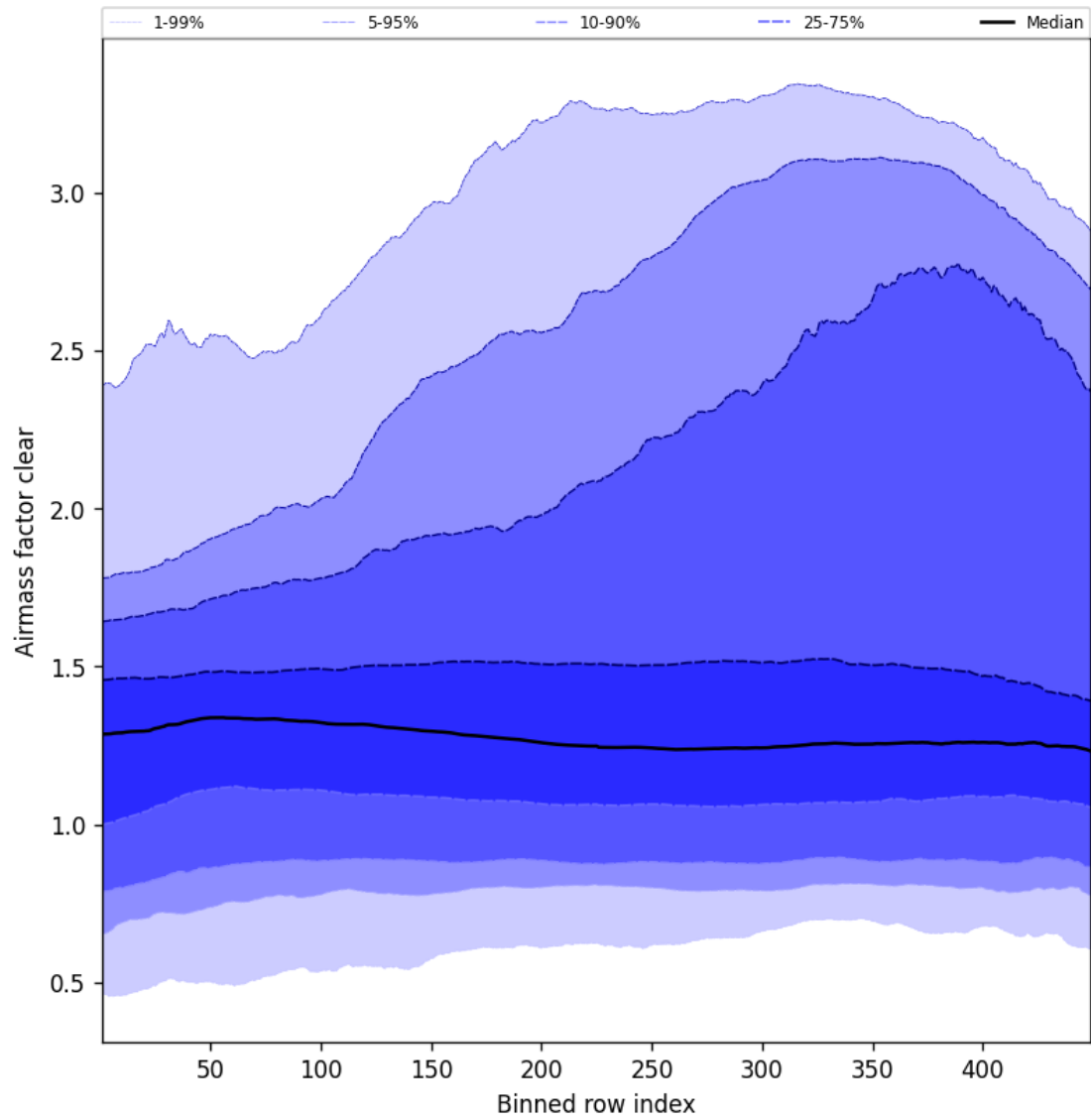
Figure 54: Along track statistics of “Airmass factor clear” for 2025-07-03 to 2025-07-04
