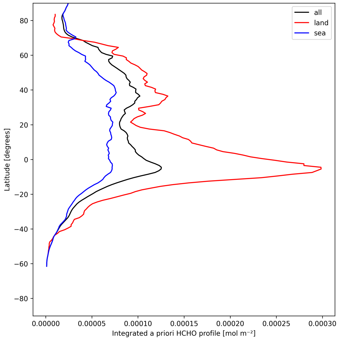
Figure 27: Zonal average of “Integrated a priori HCHO profile” for 2025-07-03 to 2025-07-04.
