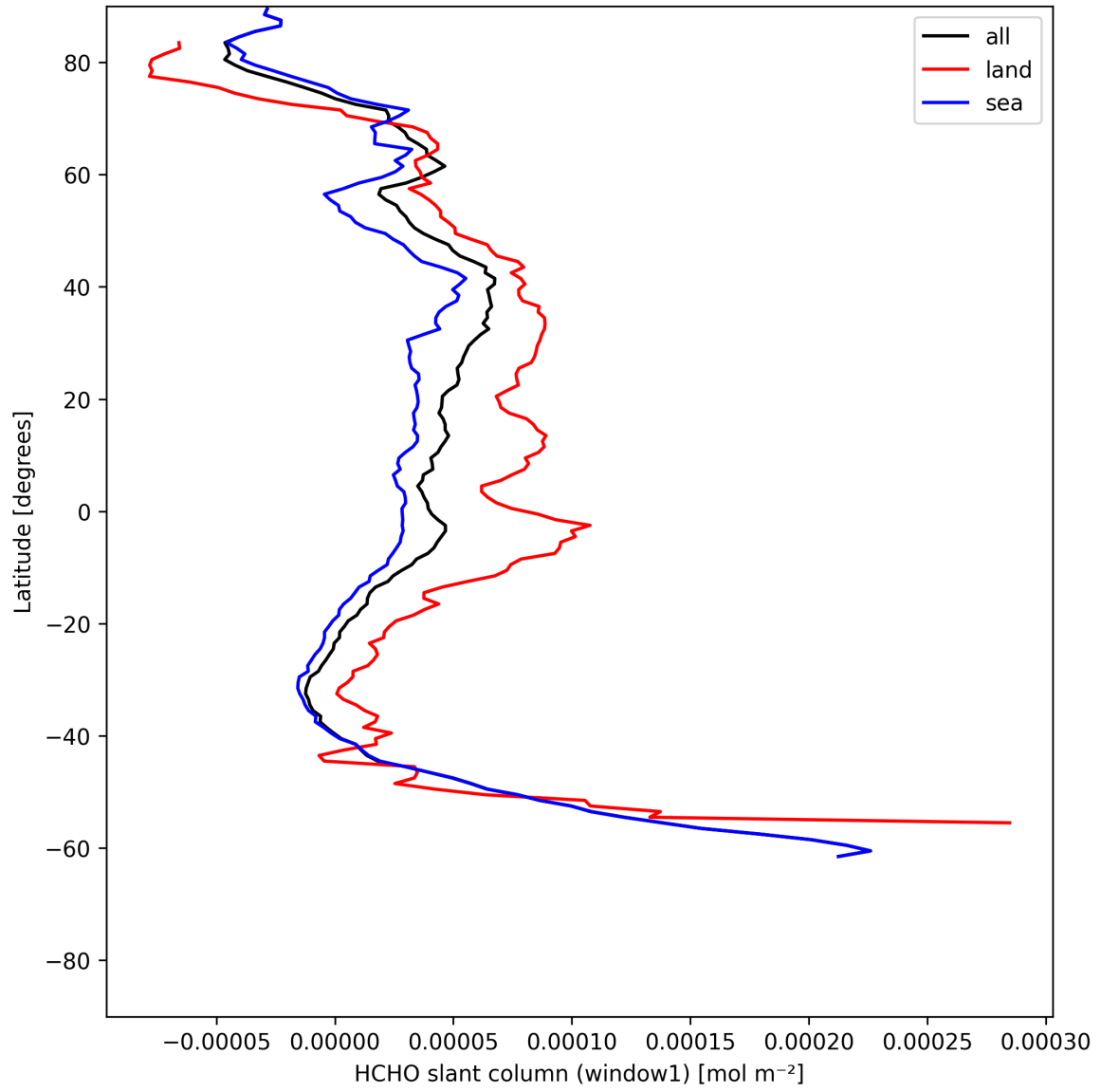
Figure 22: Zonal average of “HCHO slant column (window1)” for 2025-07-03 to 2025-07-04.
