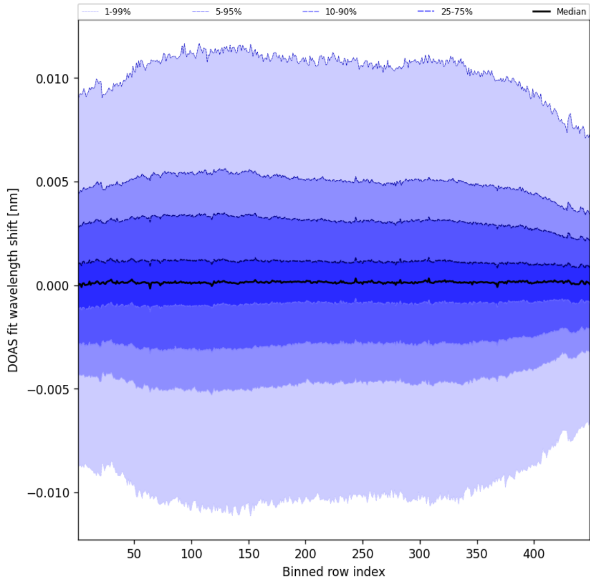
Figure 56: Along track statistics of “DOAS fit wavelength shift” for 2025-07-03 to 2025-07-04
