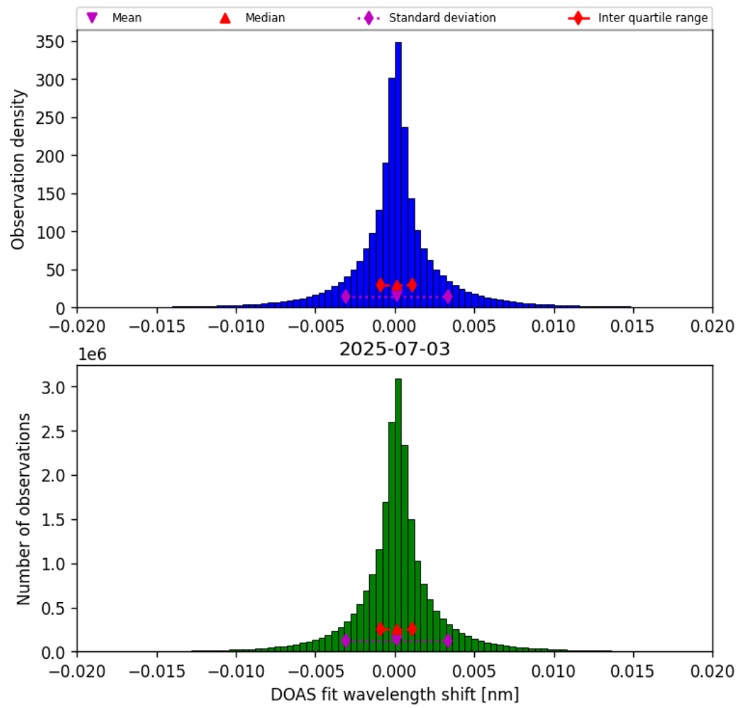
Figure 42: Histogram of “DOAS fit wavelength shift” for 2025-07-03 to 2025-07-04
