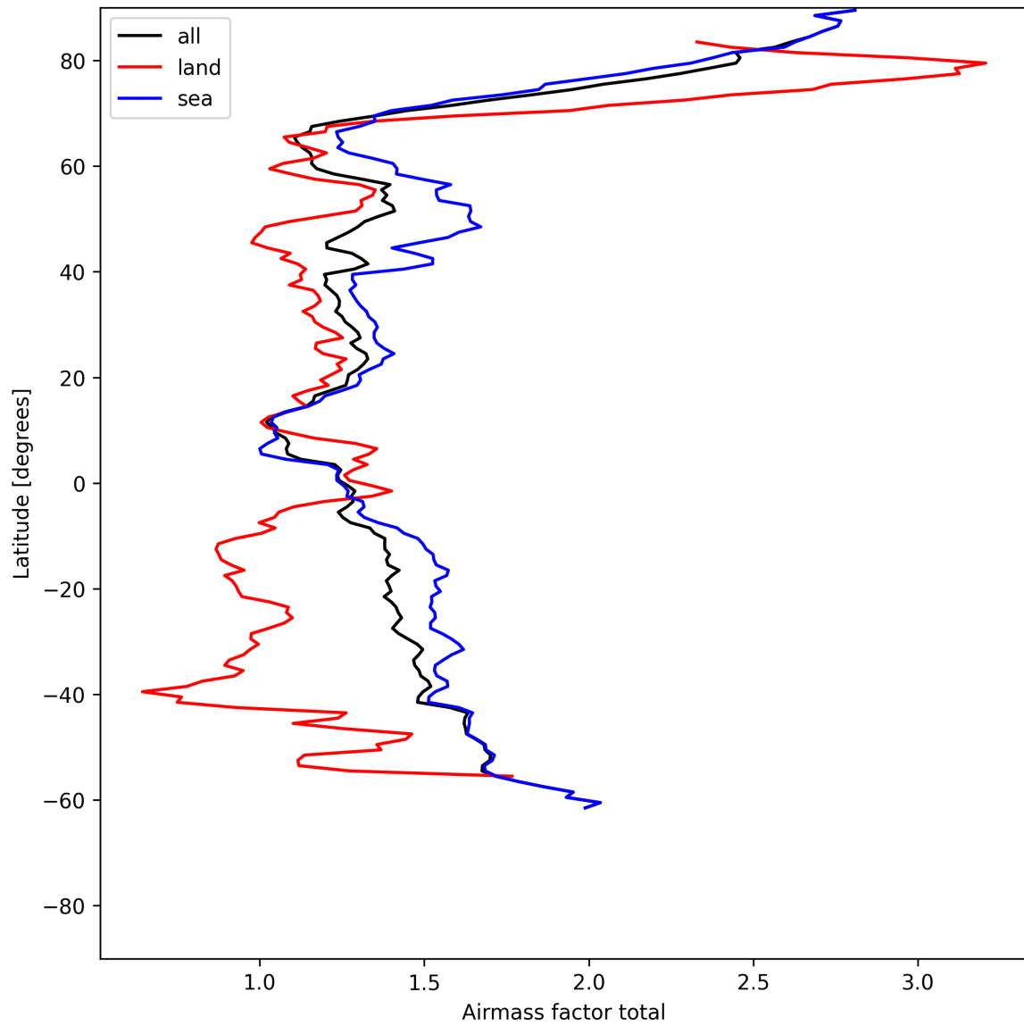
Figure 24: Zonal average of “Airmass factor total” for 2025-07-03 to 2025-07-04.
