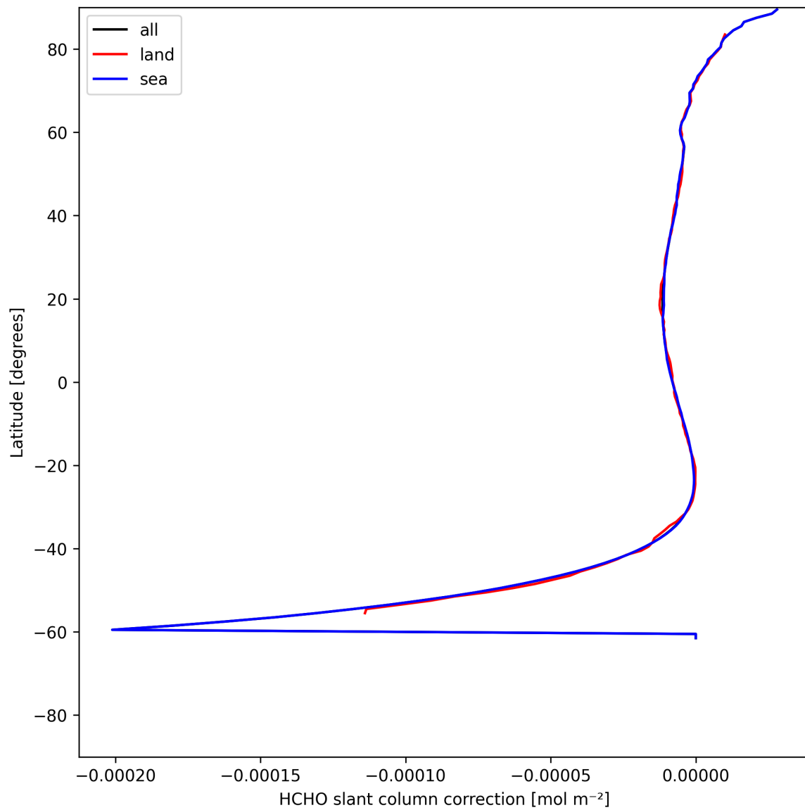
Figure 31: Zonal average of “HCHO slant column correction” for 2025-07-03 to 2025-07-04.
