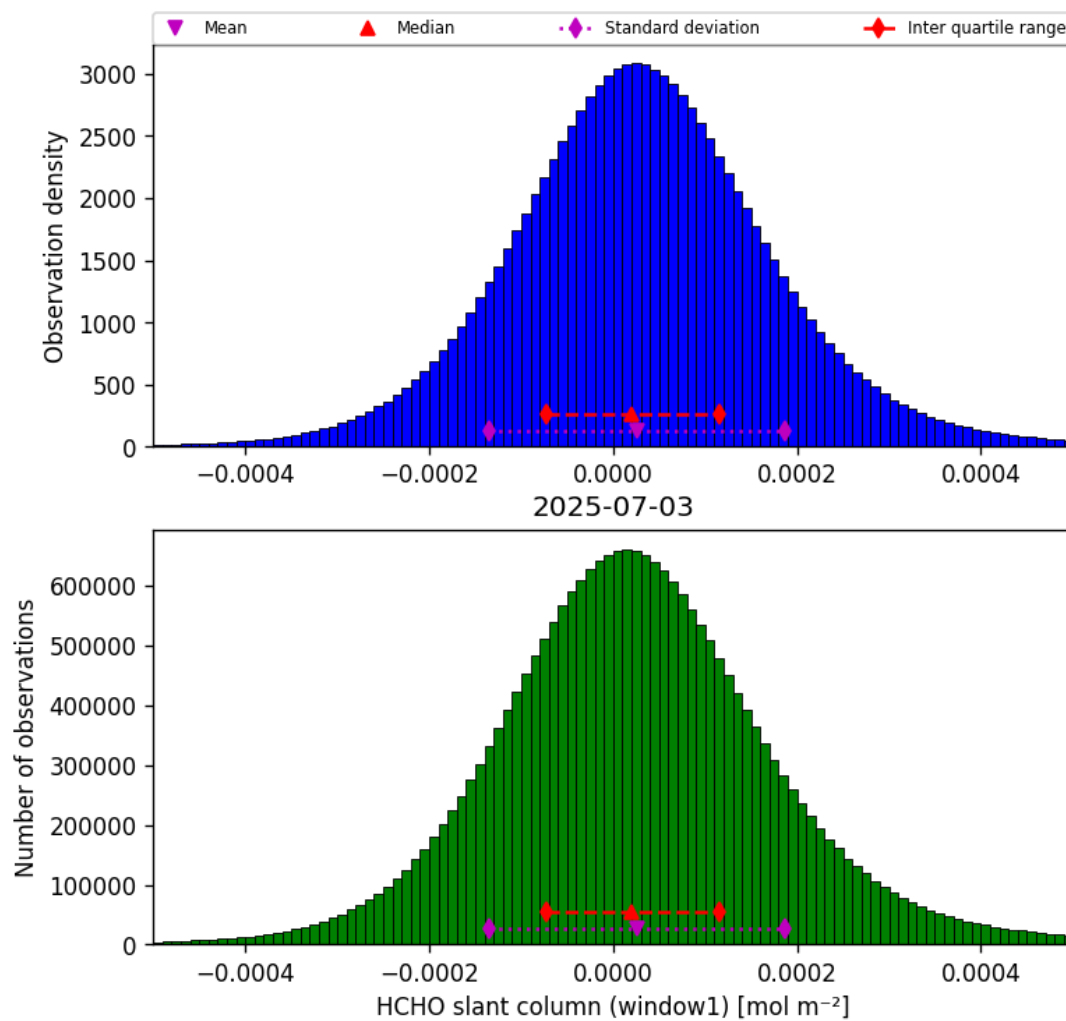
Figure 36: Histogram of “HCHO slant column (window1)” for 2025-07-03 to 2025-07-04
