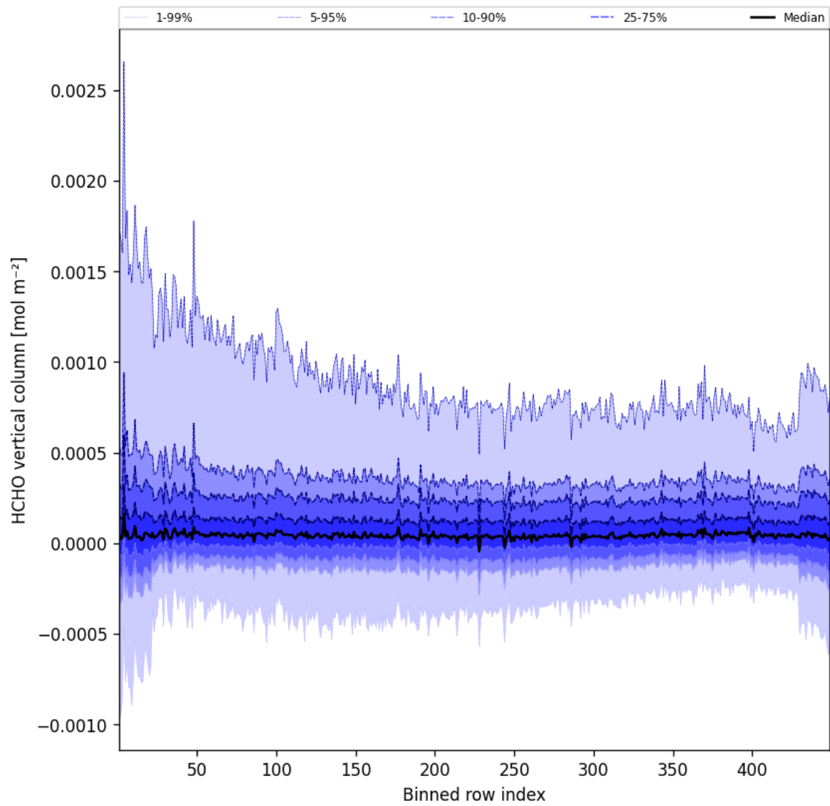
Figure 47: Along track statistics of “HCHO vertical column” for 2025-07-03 to 2025-07-04
