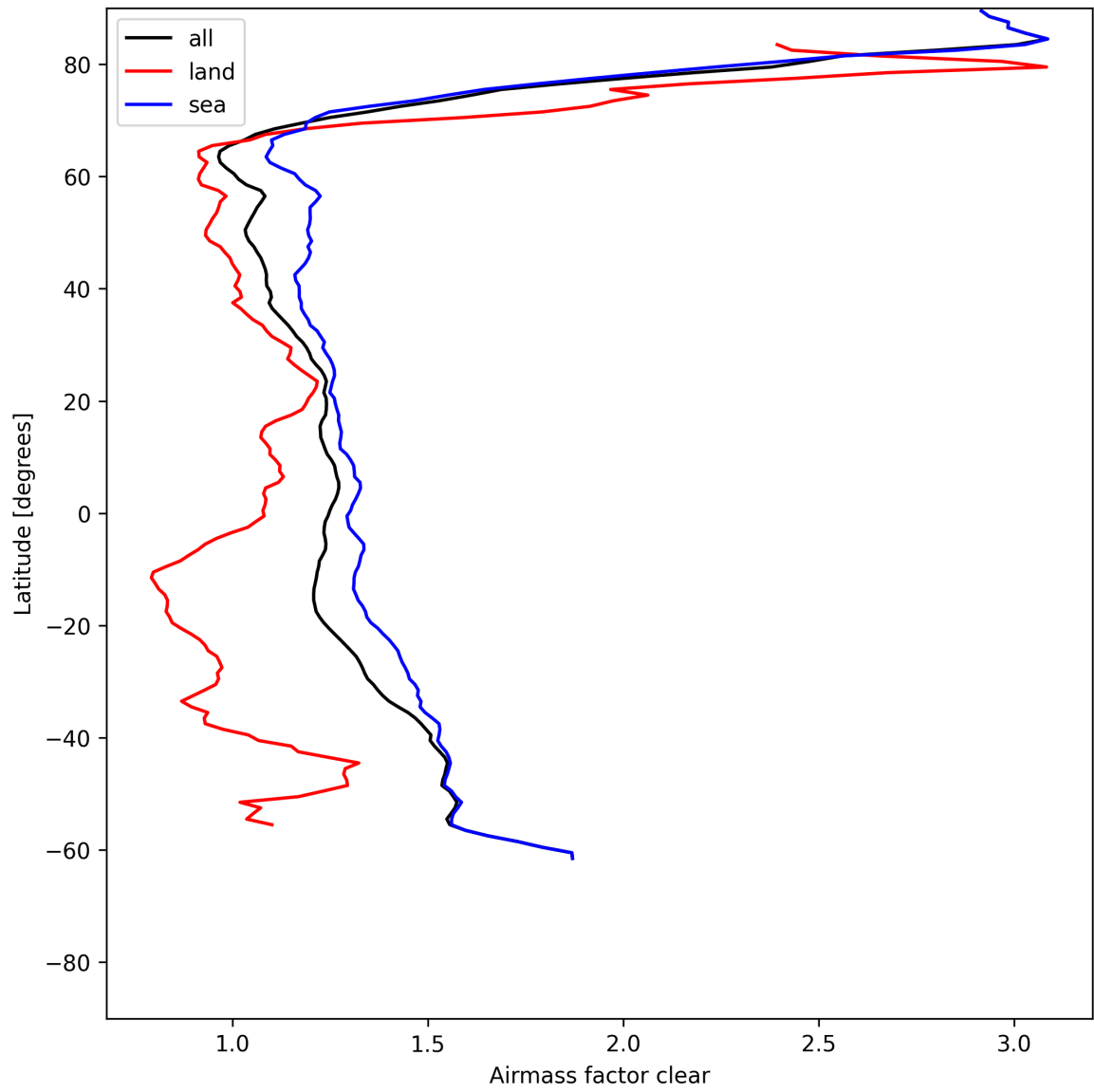
Figure 26: Zonal average of “Airmass factor clear” for 2025-07-03 to 2025-07-04.
