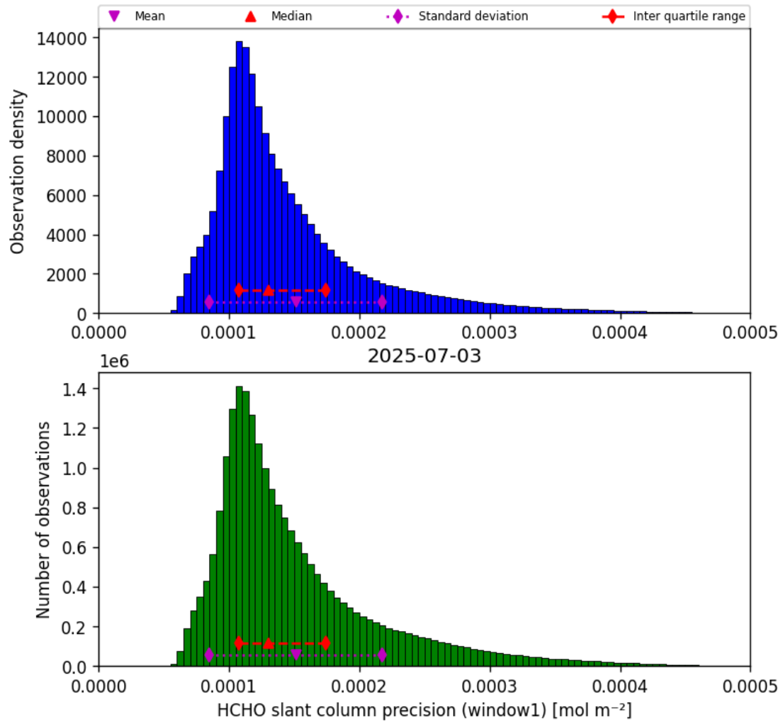
Figure 37: Histogram of “HCHO slant column precision (window1)” for 2025-07-03 to 2025-07-04
