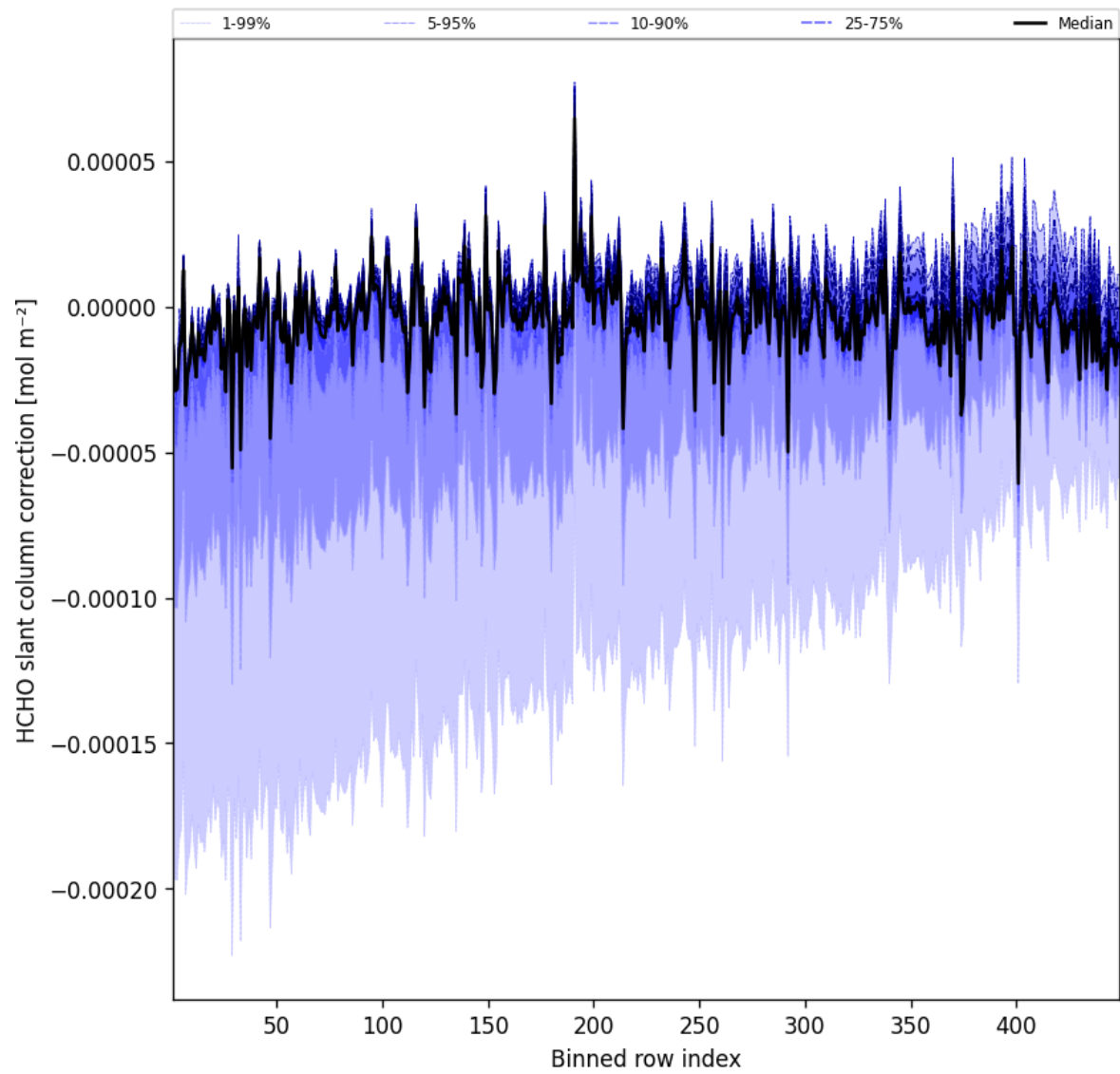
Figure 59: Along track statistics of “HCHO slant column correction” for 2025-07-03 to 2025-07-04
