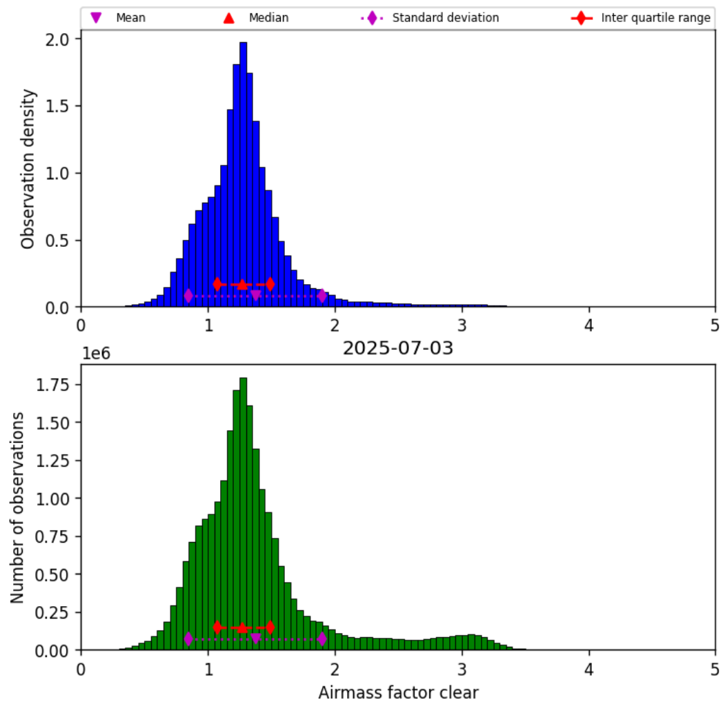
Figure 40: Histogram of “Airmass factor clear” for 2025-07-03 to 2025-07-04
