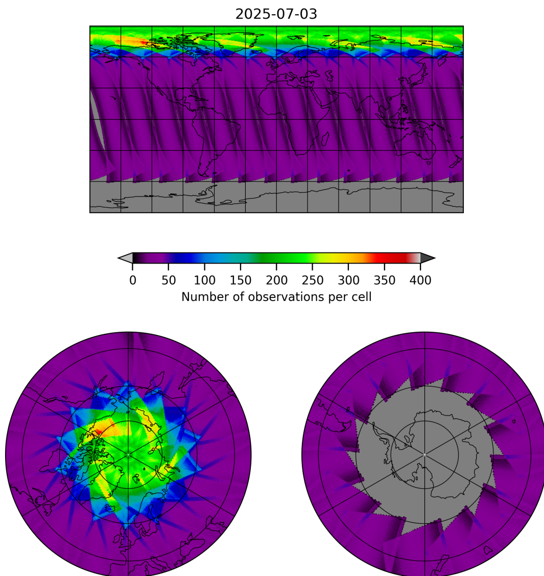
Figure 17: Map of the number of observations for 2025-07-03 to 2025-07-04
