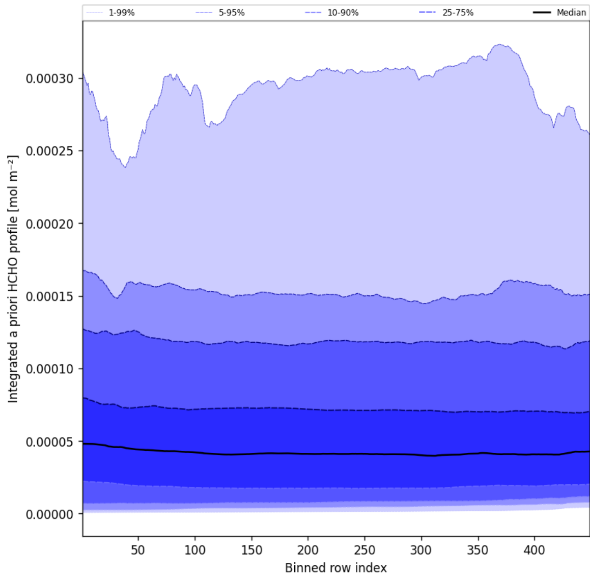
Figure 55: Along track statistics of “Integrated a priori HCHO profile” for 2025-07-03 to 2025-07-04
