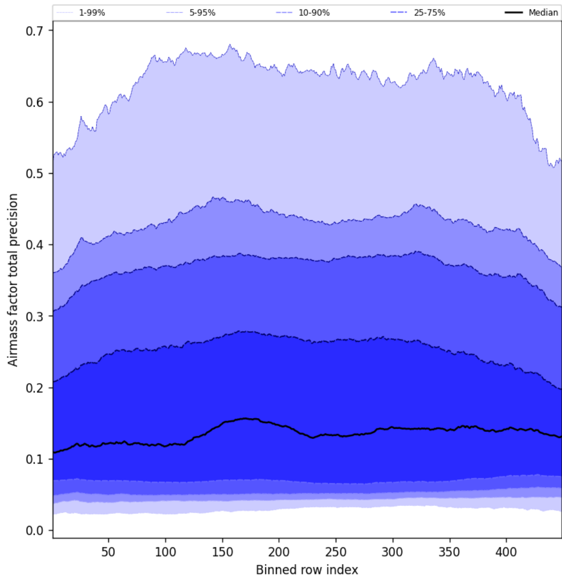
Figure 53: Along track statistics of “Airmass factor total precision” for 2025-07-03 to 2025-07-04
