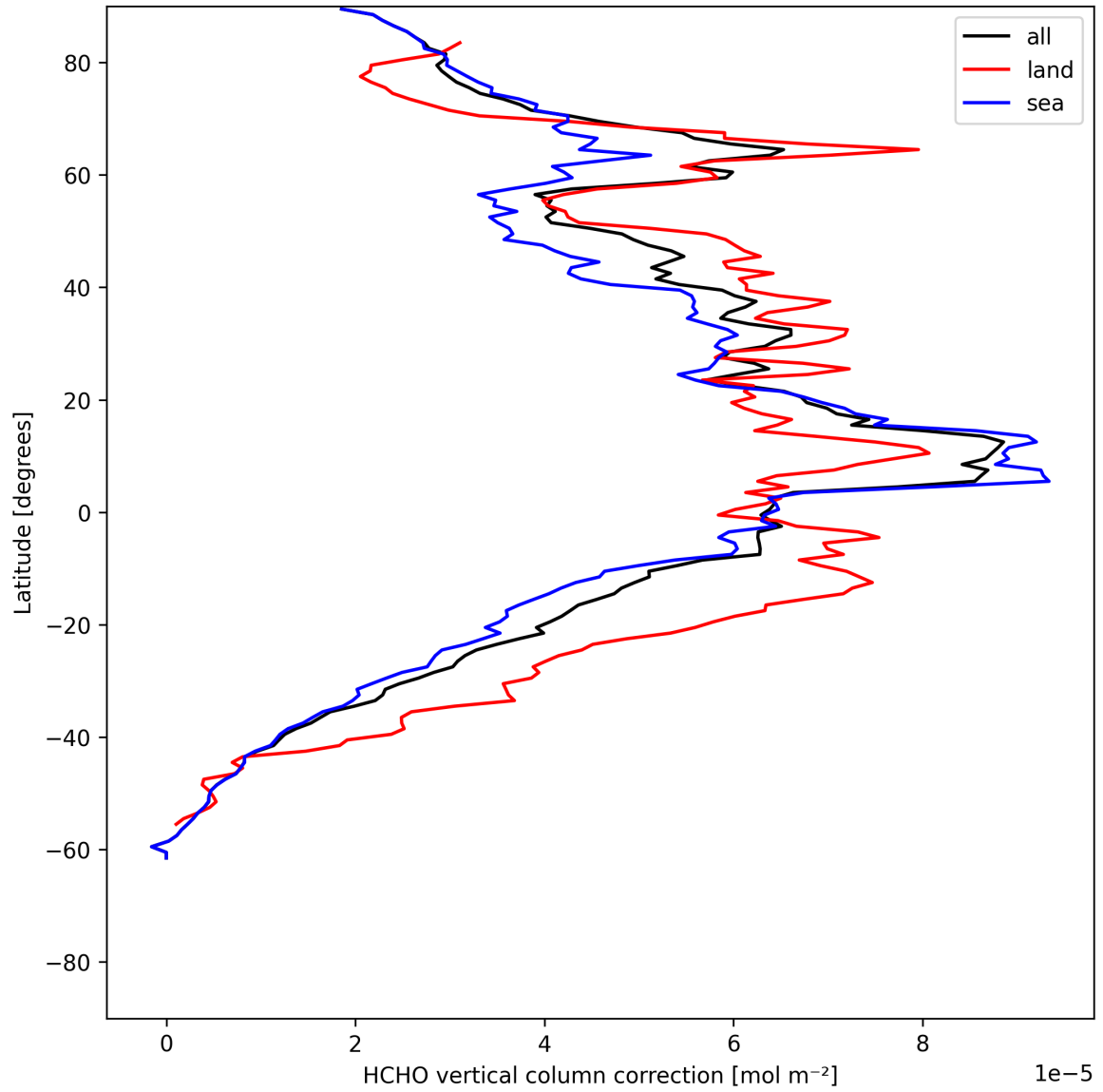
Figure 21: Zonal average of “HCHO vertical column correction” for 2025-07-03 to 2025-07-04.
