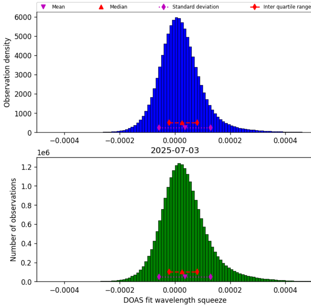
Figure 43: Histogram of “DOAS fit wavelength squeeze” for 2025-07-03 to 2025-07-04
