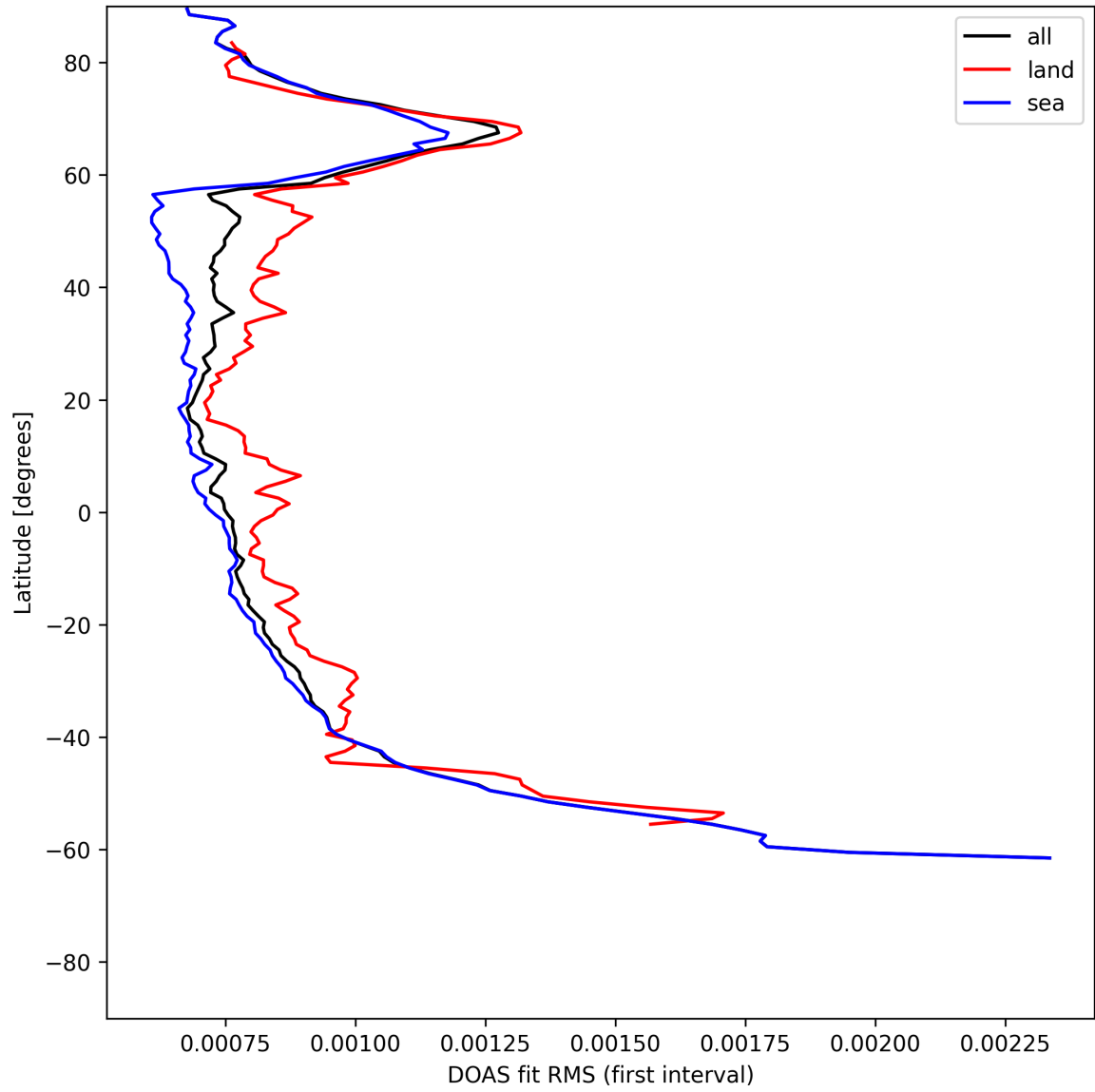
Figure 30: Zonal average of “DOAS fit RMS (first interval)” for 2025-07-03 to 2025-07-04.
