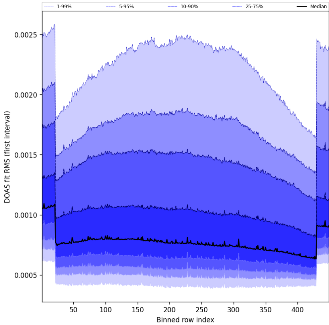
Figure 58: Along track statistics of “DOAS fit RMS (first interval)” for 2025-07-03 to 2025-07-04
