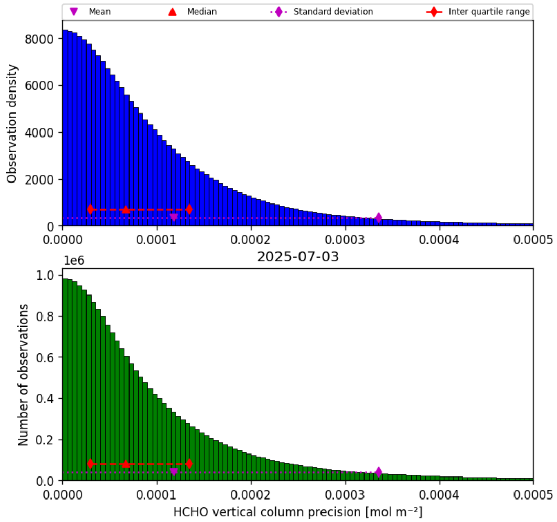
Figure 34: Histogram of “HCHO vertical column precision” for 2025-07-03 to 2025-07-04
