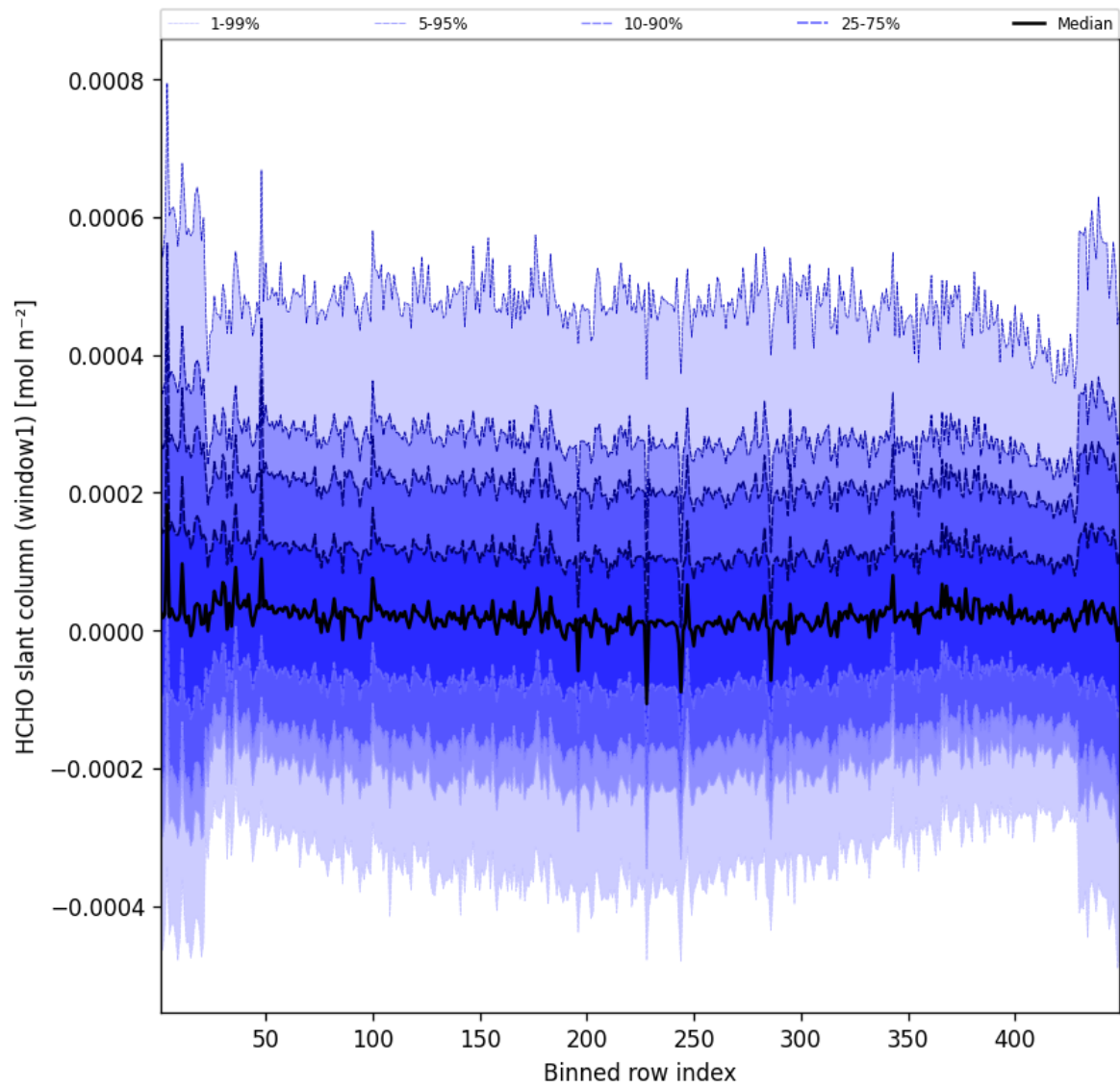
Figure 50: Along track statistics of “HCHO slant column (window1)” for 2025-07-03 to 2025-07-04
