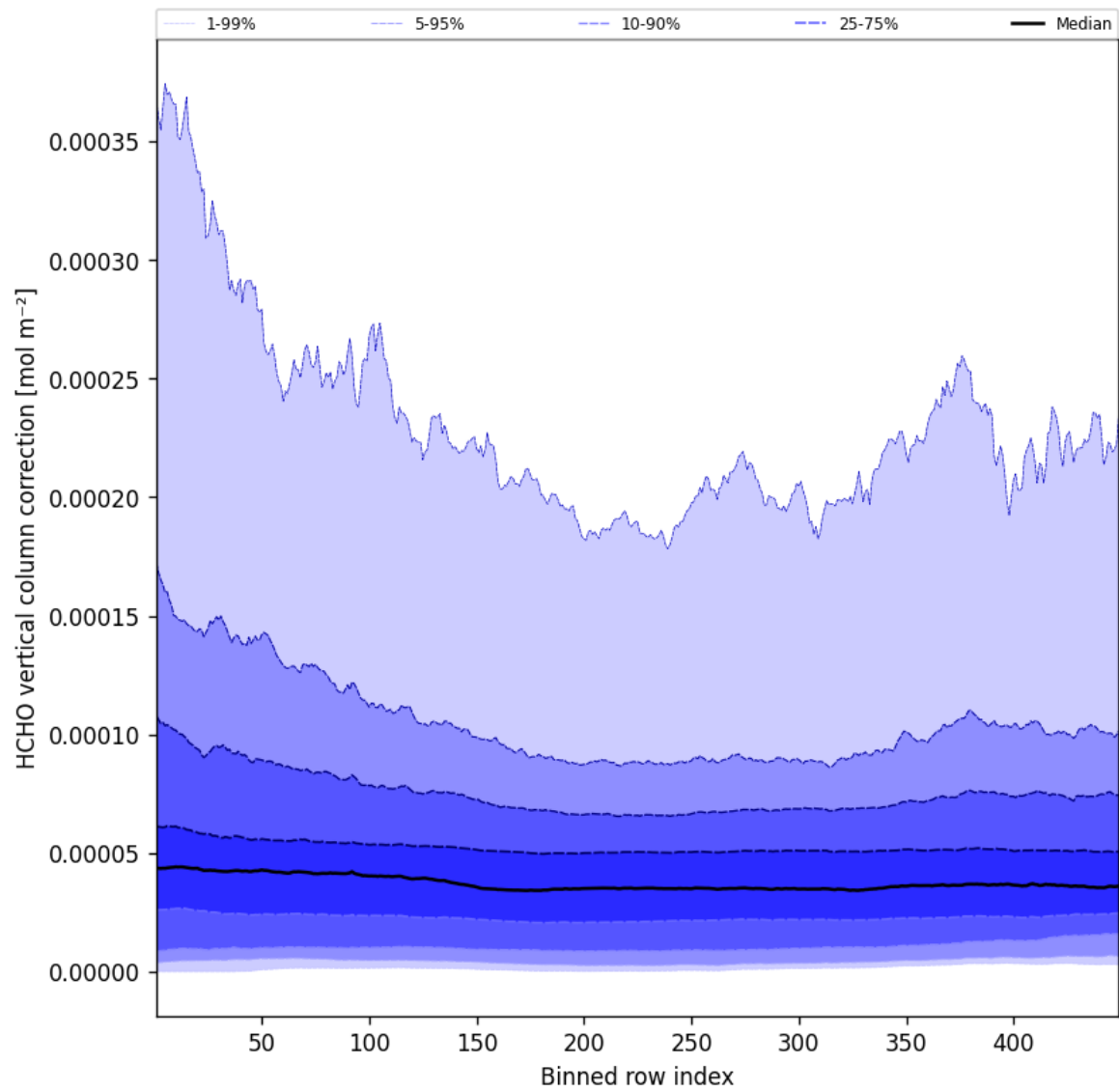
Figure 49: Along track statistics of “HCHO vertical column correction” for 2025-07-03 to 2025-07-04
