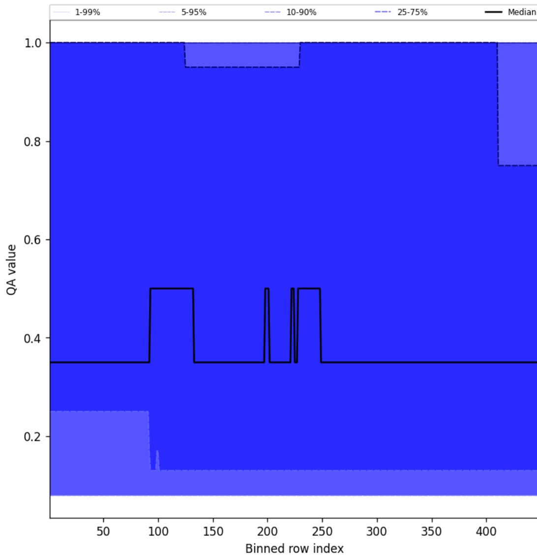
Figure 46: Along track statistics of “QA value” for 2025-07-03 to 2025-07-04
