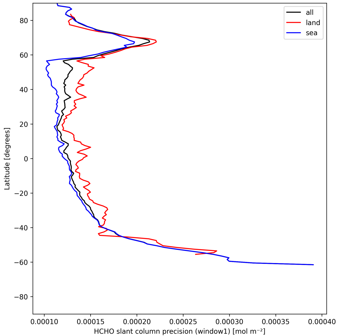
Figure 23: Zonal average of “HCHO slant column precision (window1)” for 2025-07-03 to 2025-07-04.
