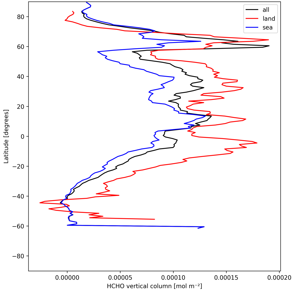
Figure 19: Zonal average of “HCHO vertical column” for 2025-07-03 to 2025-07-04.
