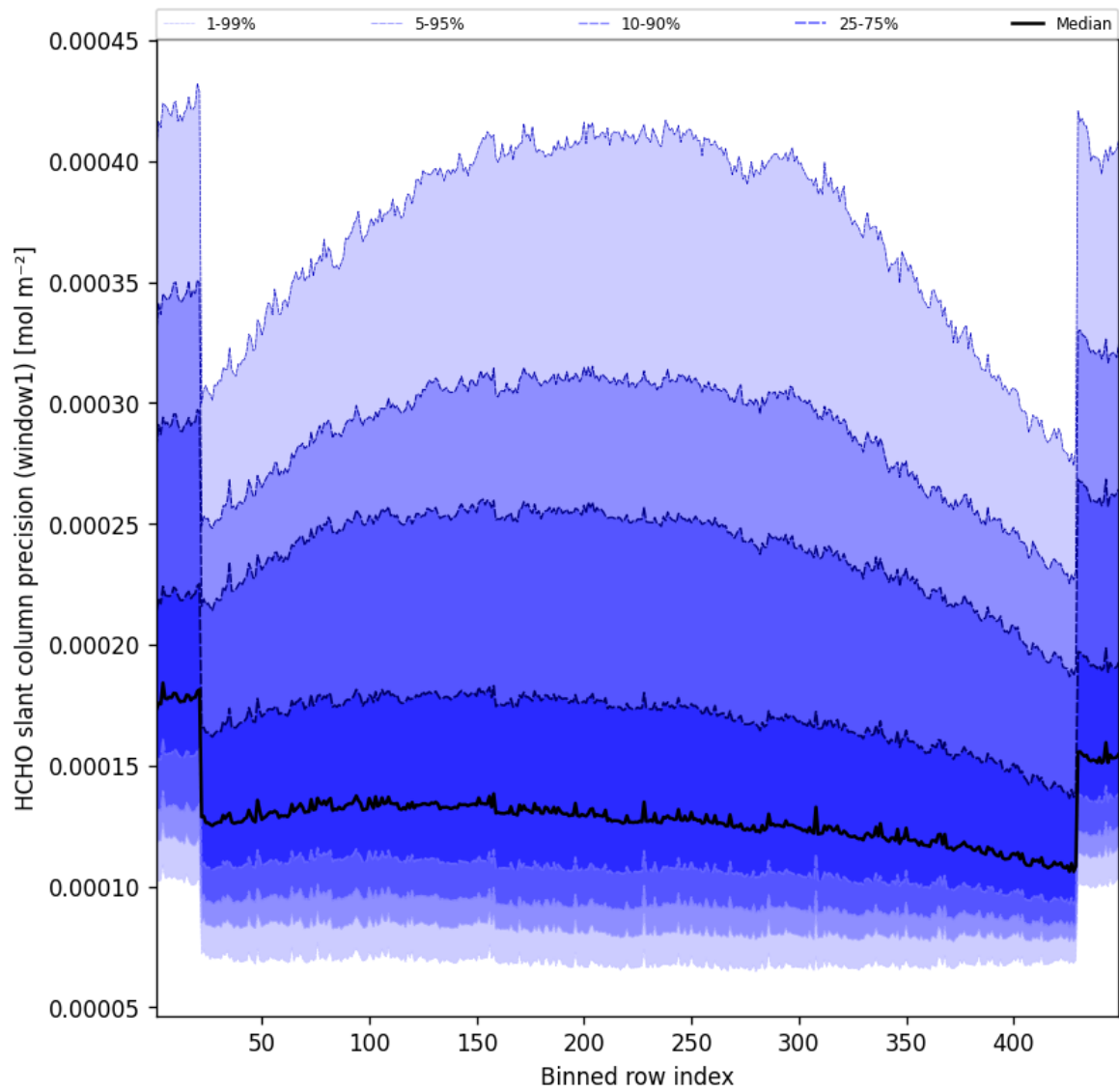
Figure 51: Along track statistics of “HCHO slant column precision (window1)” for 2025-07-03 to 2025-07-04
