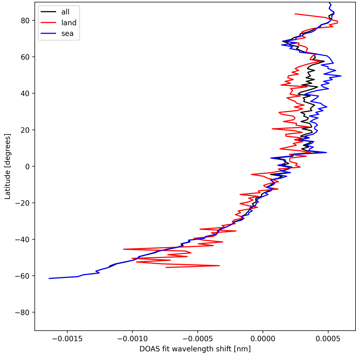
Figure 28: Zonal average of “DOAS fit wavelength shift” for 2025-07-03 to 2025-07-04.
