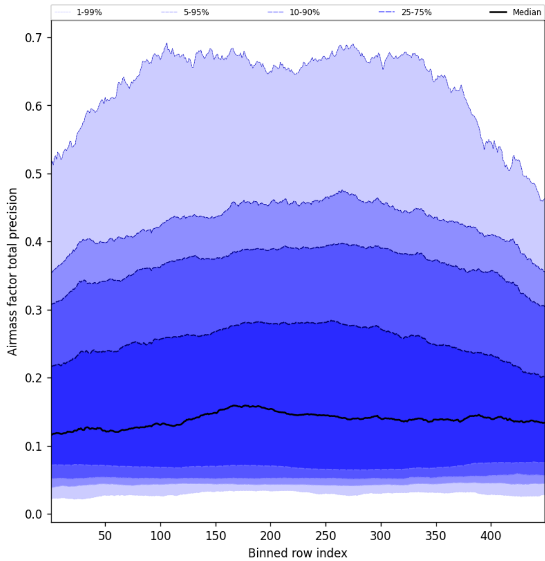
Figure 53: Along track statistics of “Airmass factor total precision” for 2025-07-04 to 2025-07-05
