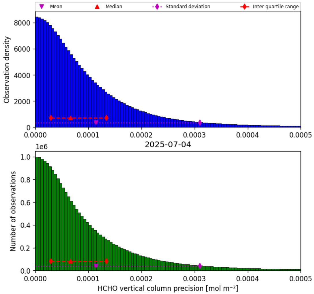
Figure 34: Histogram of “HCHO vertical column precision” for 2025-07-04 to 2025-07-05
