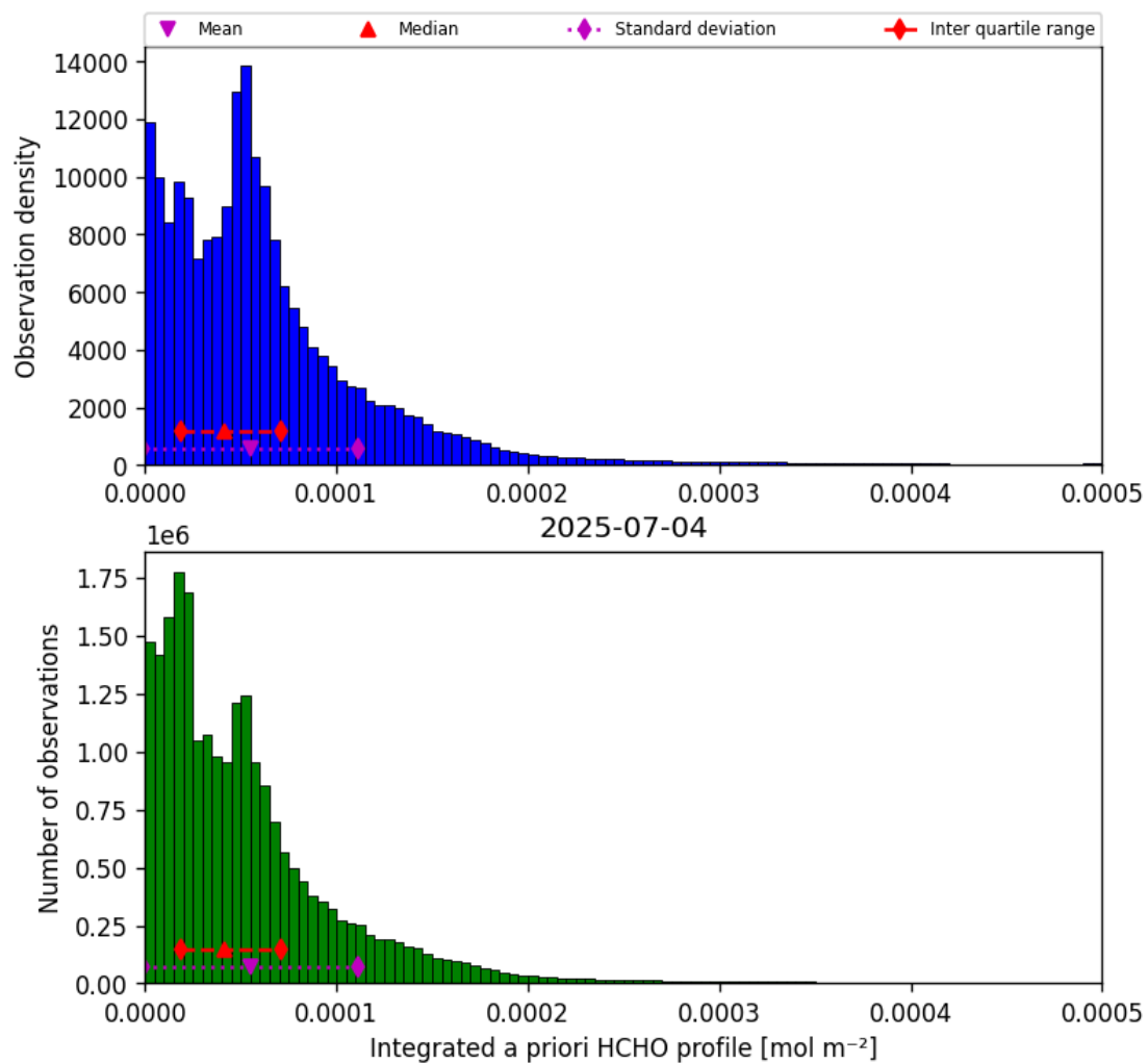
Figure 41: Histogram of “Integrated a priori HCHO profile” for 2025-07-04 to 2025-07-05
