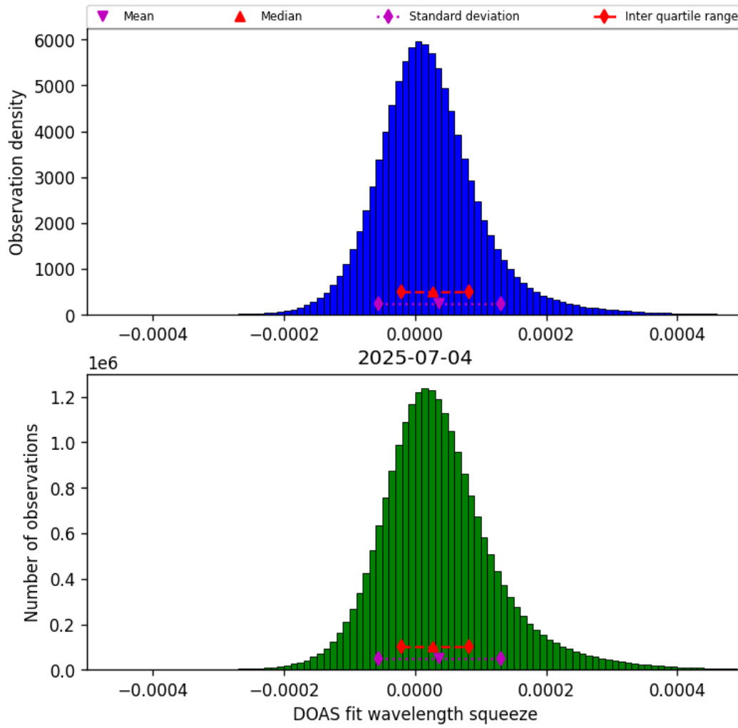
Figure 43: Histogram of “DOAS fit wavelength squeeze” for 2025-07-04 to 2025-07-05
