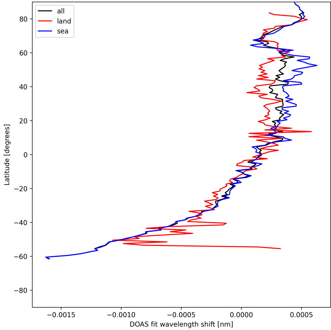
Figure 28: Zonal average of “DOAS fit wavelength shift” for 2025-07-04 to 2025-07-05.
