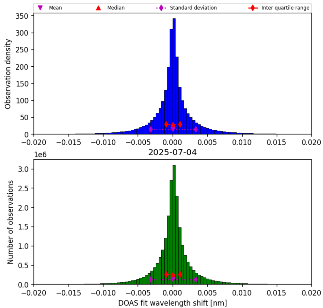
Figure 42: Histogram of “DOAS fit wavelength shift” for 2025-07-04 to 2025-07-05
