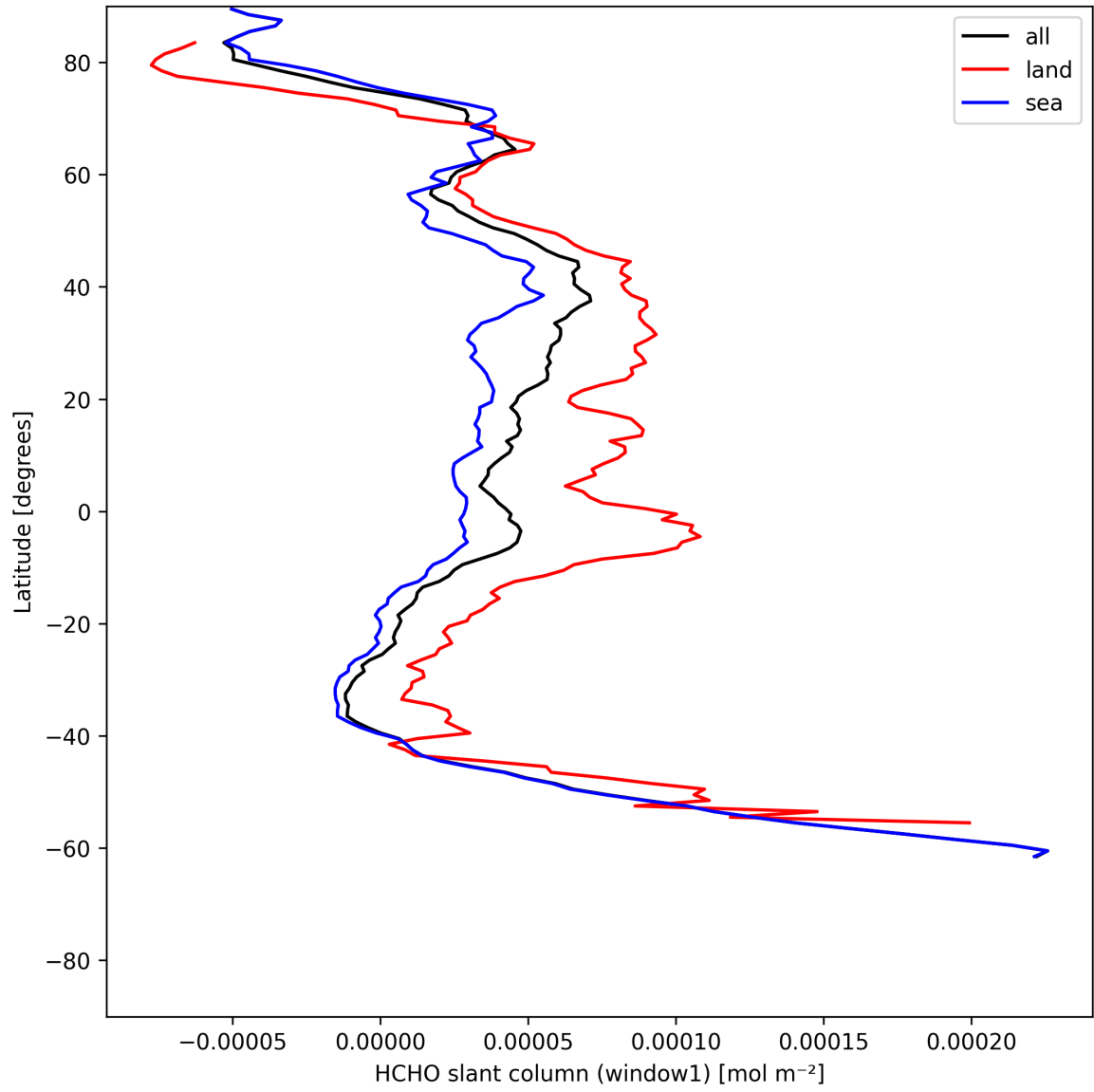
Figure 22: Zonal average of “HCHO slant column (window1)” for 2025-07-04 to 2025-07-05.
