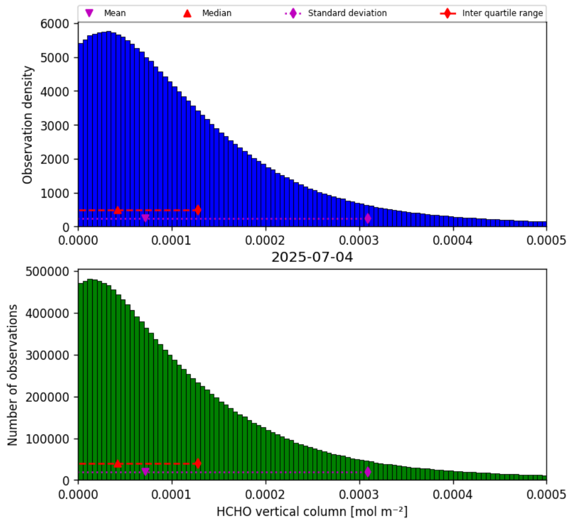
Figure 33: Histogram of “HCHO vertical column” for 2025-07-04 to 2025-07-05
