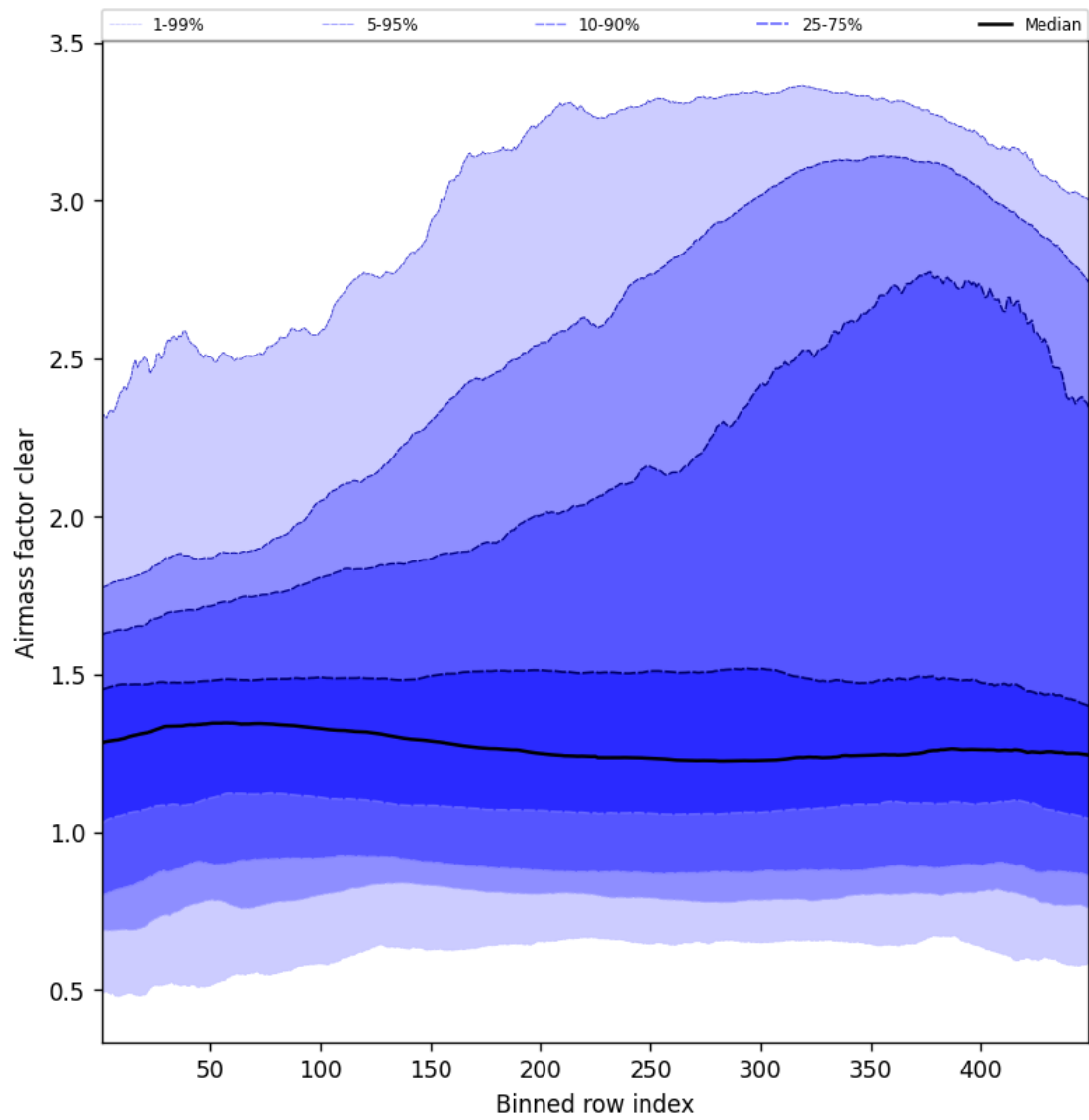
Figure 54: Along track statistics of “Airmass factor clear” for 2025-07-04 to 2025-07-05
