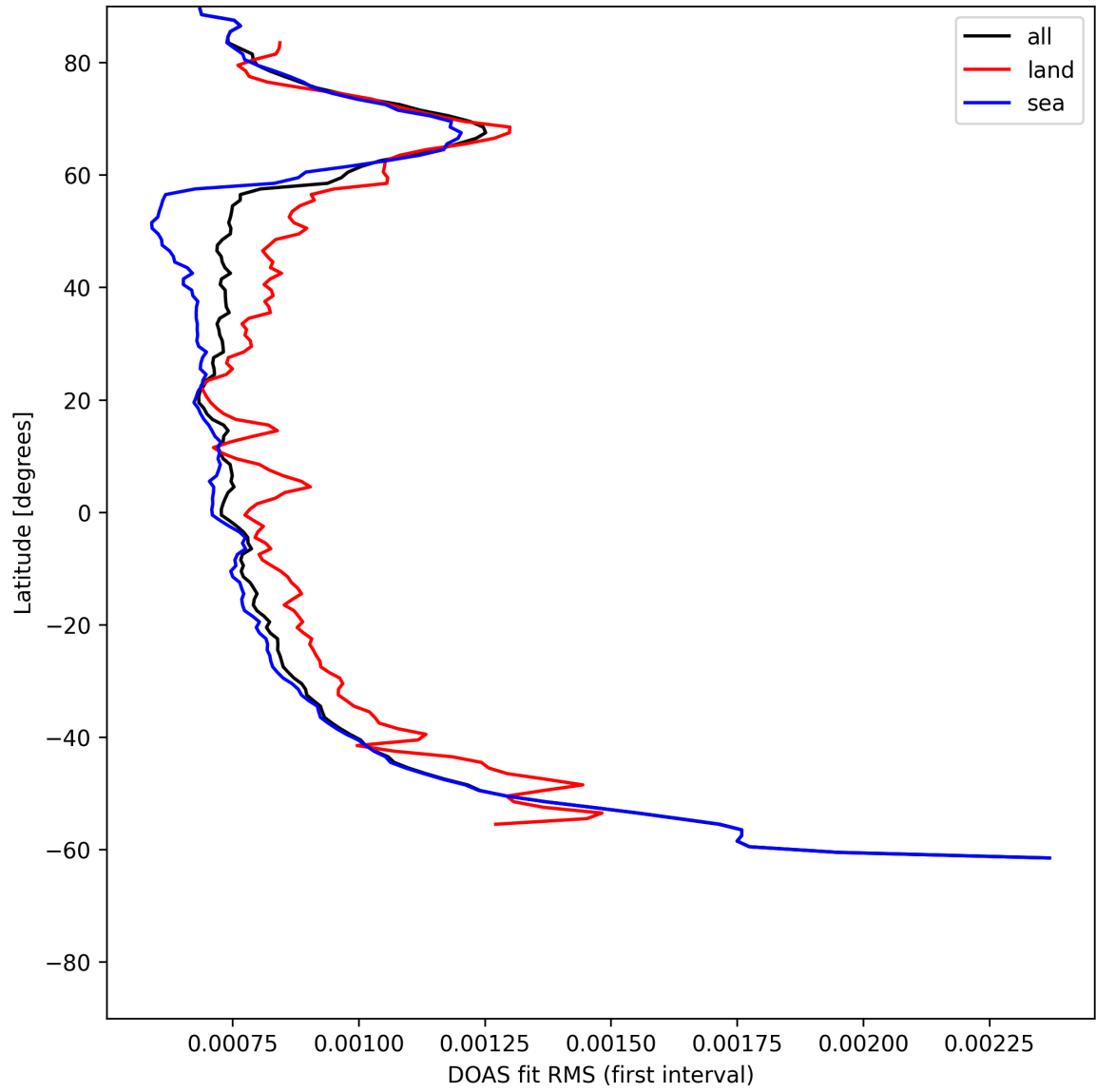
Figure 30: Zonal average of "DOAS fit RMS (first interval)" for 2025-07-04 to 2025-07-05.
