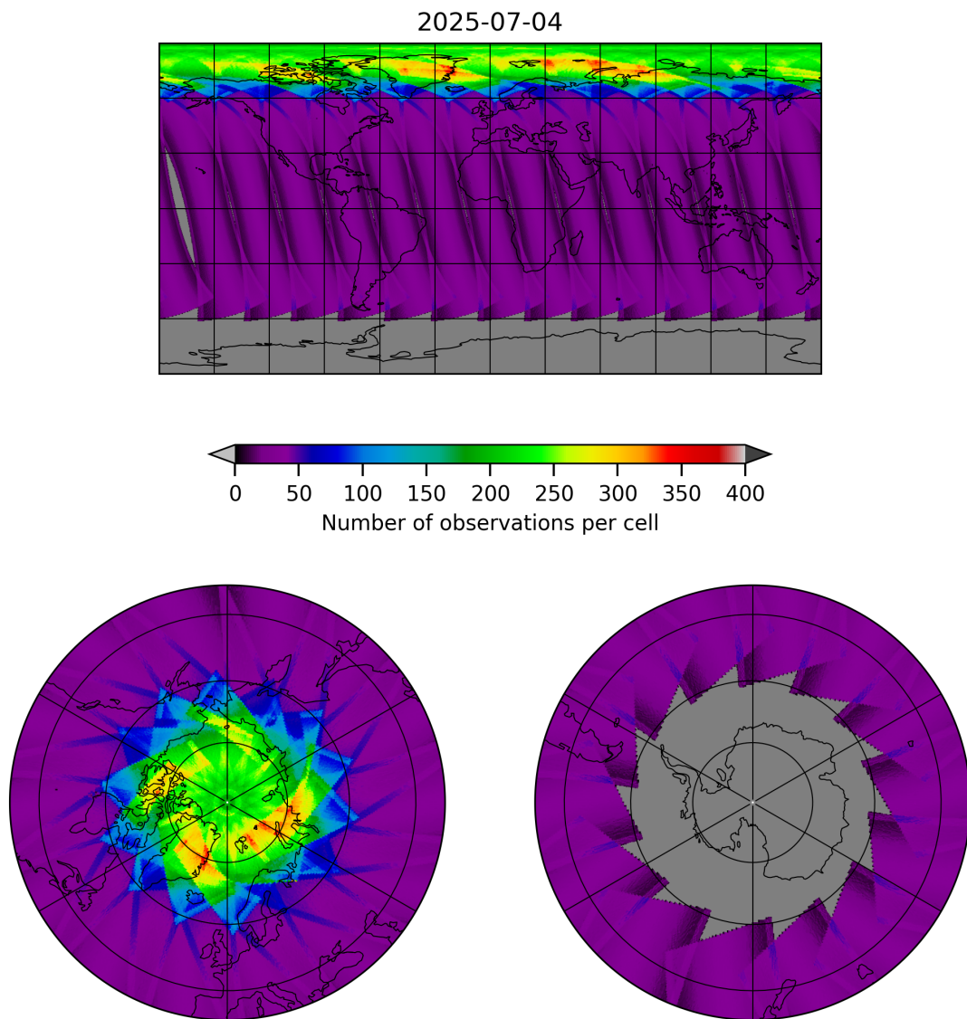
Figure 17: Map of the number of observations for 2025-07-04 to 2025-07-05
