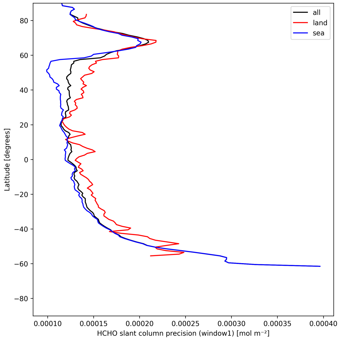
Figure 23: Zonal average of “HCHO slant column precision (window1)” for 2025-07-04 to 2025-07-05.
