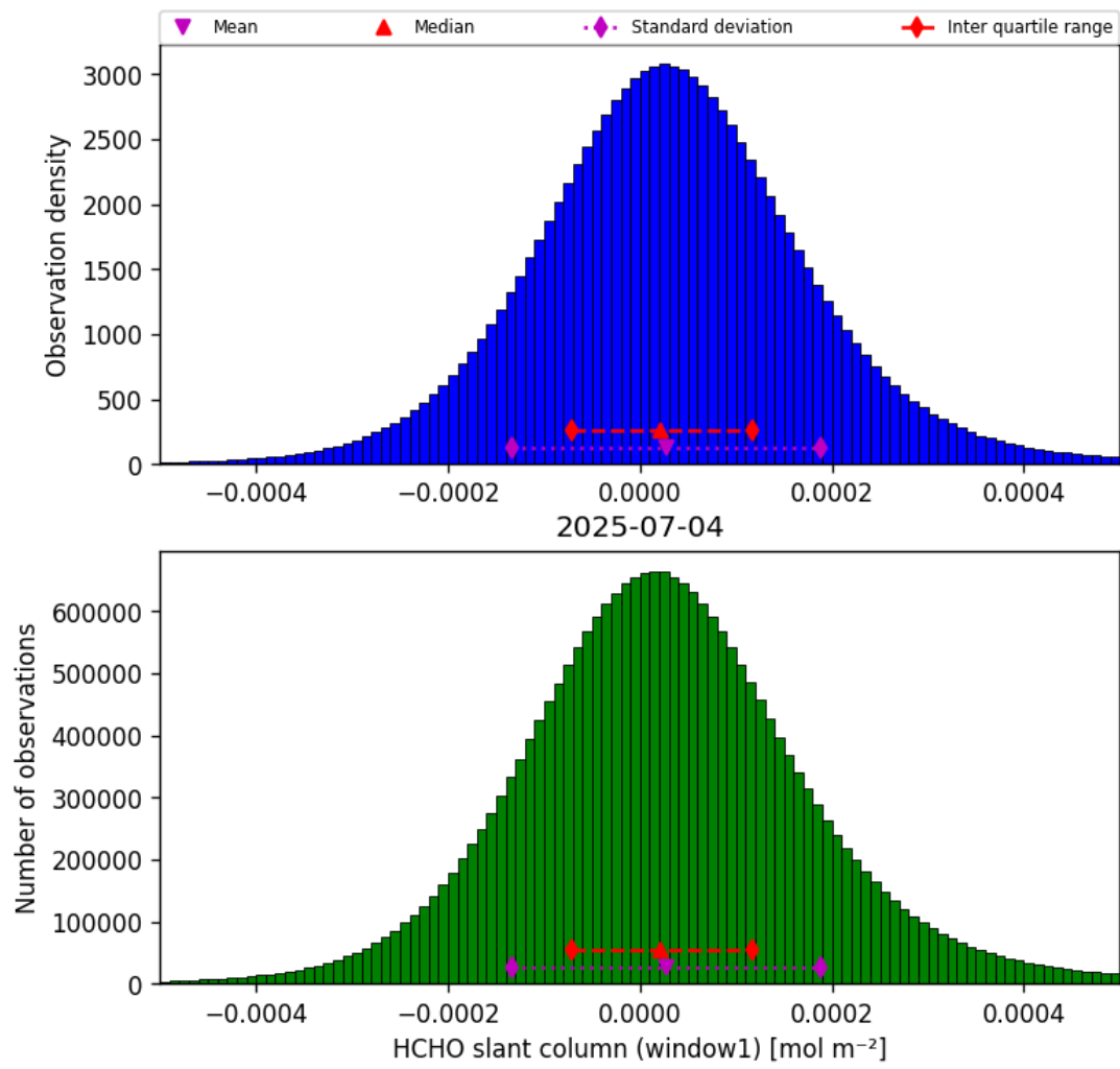
Figure 36: Histogram of “HCHO slant column (window1)” for 2025-07-04 to 2025-07-05
