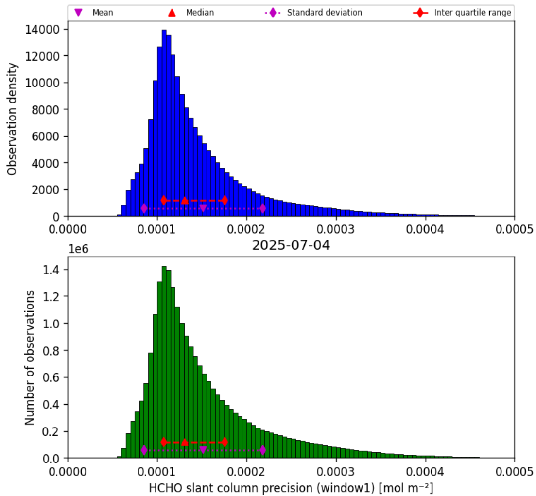
Figure 37: Histogram of “HCHO slant column precision (window1)” for 2025-07-04 to 2025-07-05
