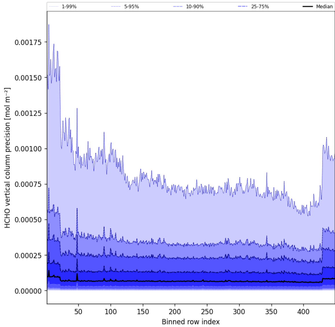
Figure 48: Along track statistics of “HCHO vertical column precision” for 2025-07-04 to 2025-07-05
