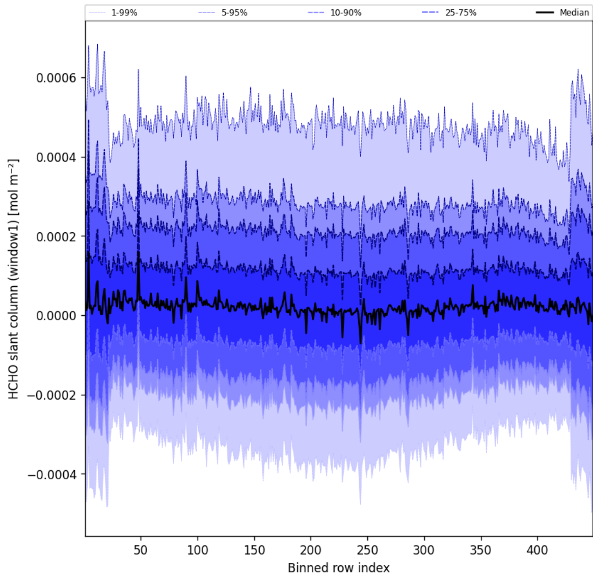
Figure 50: Along track statistics of “HCHO slant column (window1)” for 2025-07-04 to 2025-07-05
