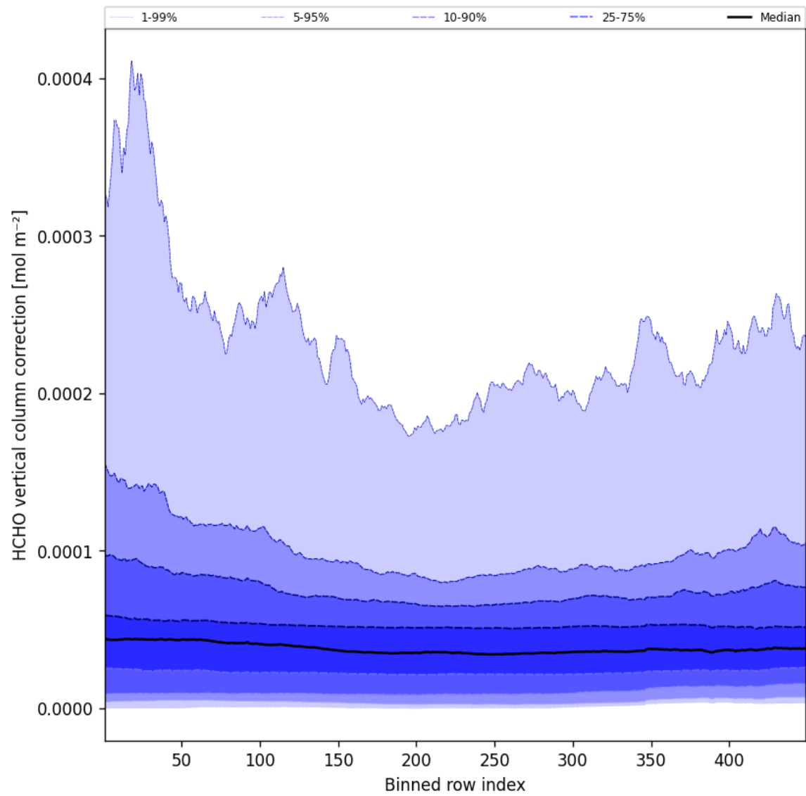
Figure 49: Along track statistics of “HCHO vertical column correction” for 2025-07-04 to 2025-07-05
