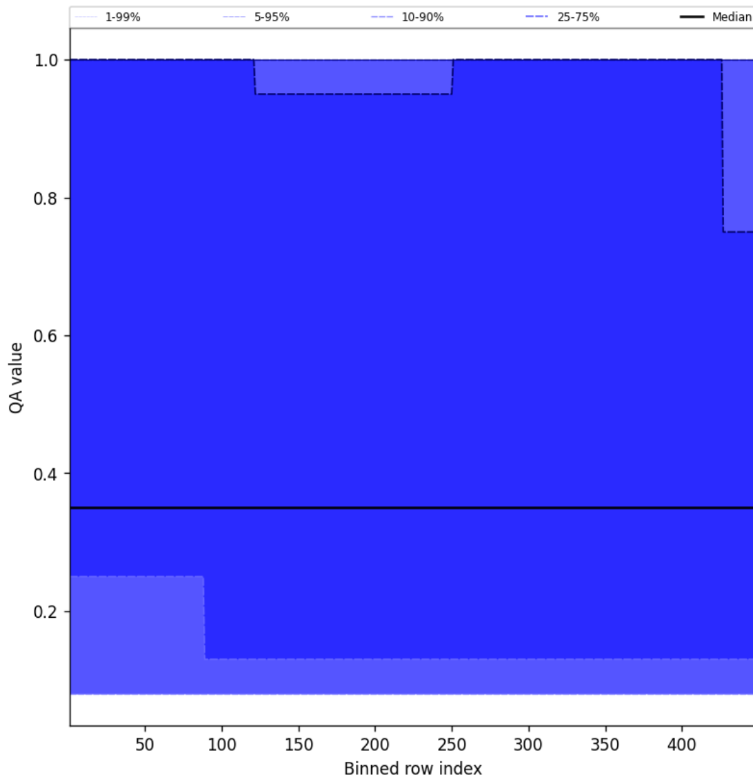
Figure 46: Along track statistics of “QA value” for 2025-07-04 to 2025-07-05
