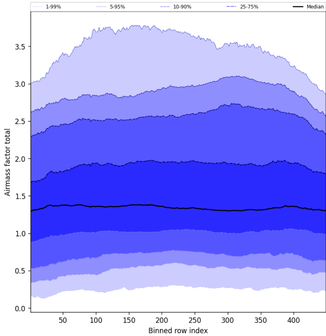
Figure 52: Along track statistics of “Airmass factor total” for 2025-07-04 to 2025-07-05
