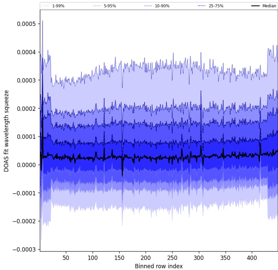
Figure 57: Along track statistics of “DOAS fit wavelength squeeze” for 2025-07-04 to 2025-07-05
