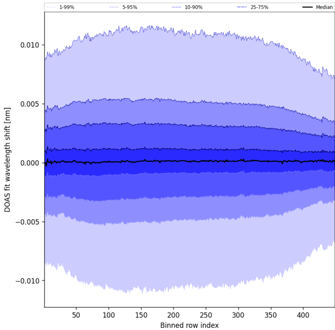
Figure 56: Along track statistics of “DOAS fit wavelength shift” for 2025-07-04 to 2025-07-05
