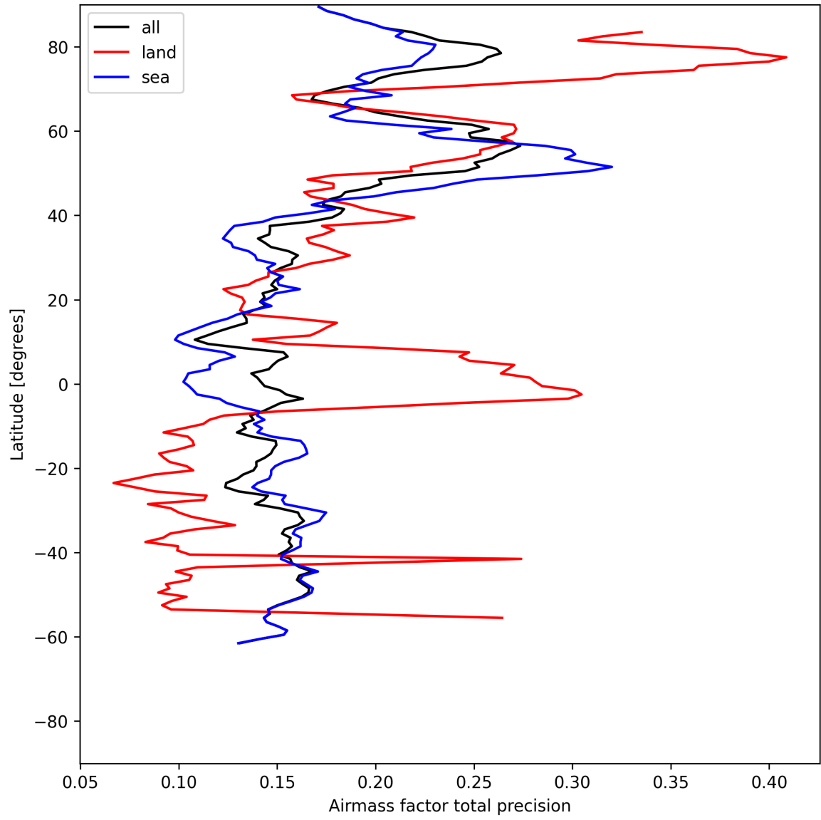
Figure 25: Zonal average of “Airmass factor total precision” for 2025-07-04 to 2025-07-05.
