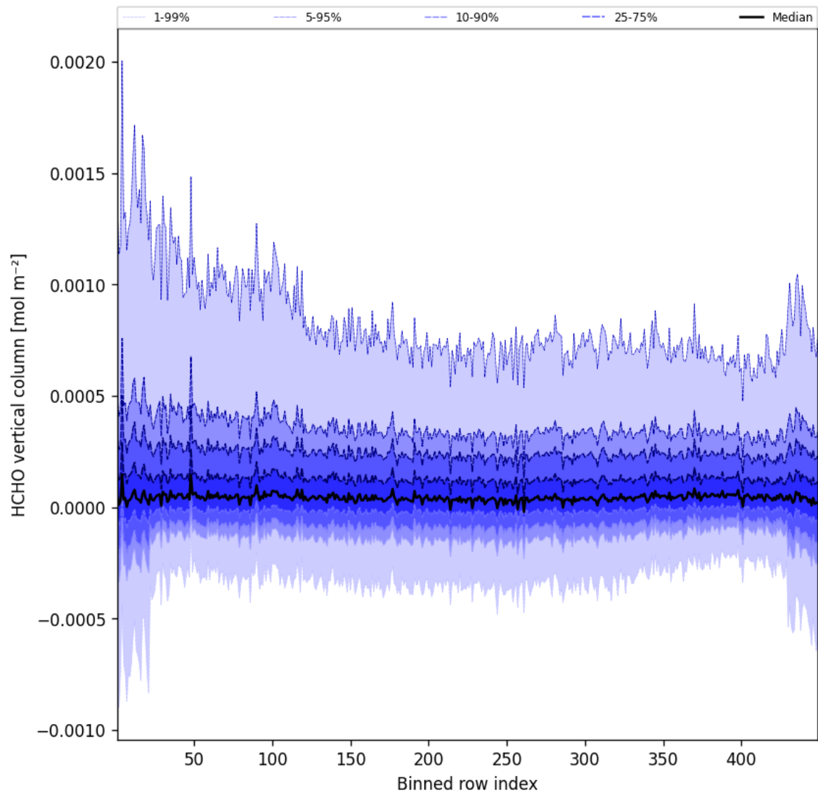
Figure 47: Along track statistics of “HCHO vertical column” for 2025-07-04 to 2025-07-05
