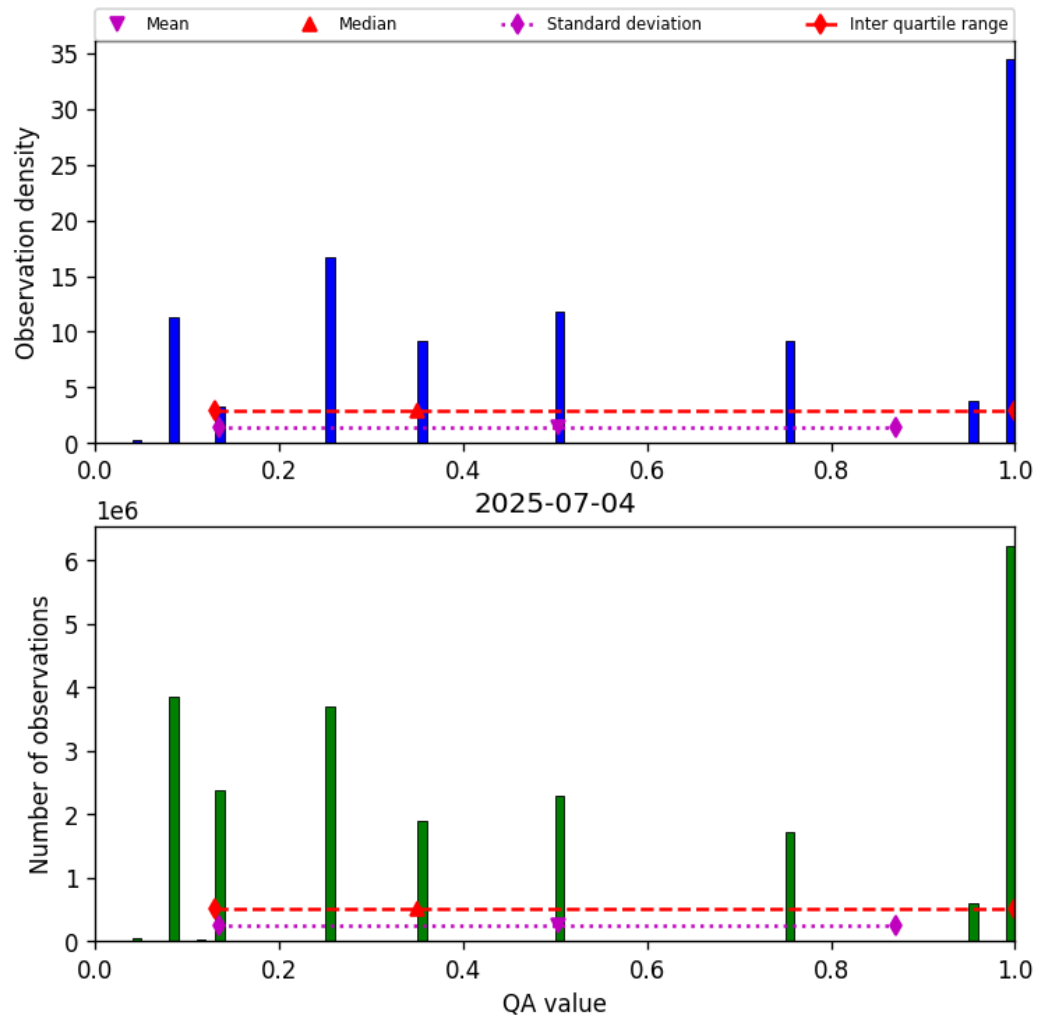
Figure 32: Histogram of “QA value” for 2025-07-04 to 2025-07-05
