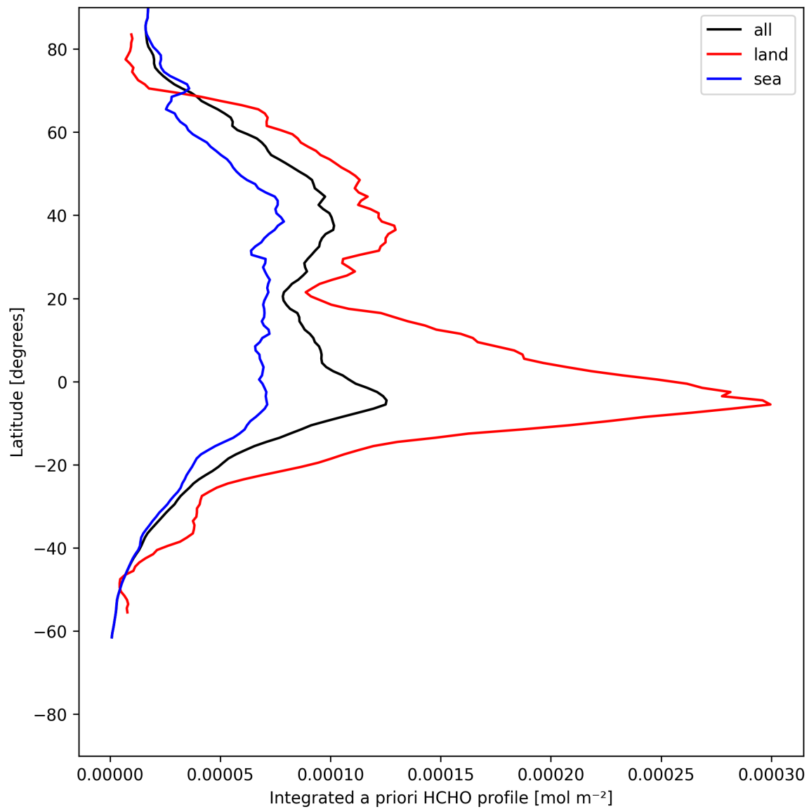
Figure 27: Zonal average of “Integrated a priori HCHO profile” for 2025-07-04 to 2025-07-05.
