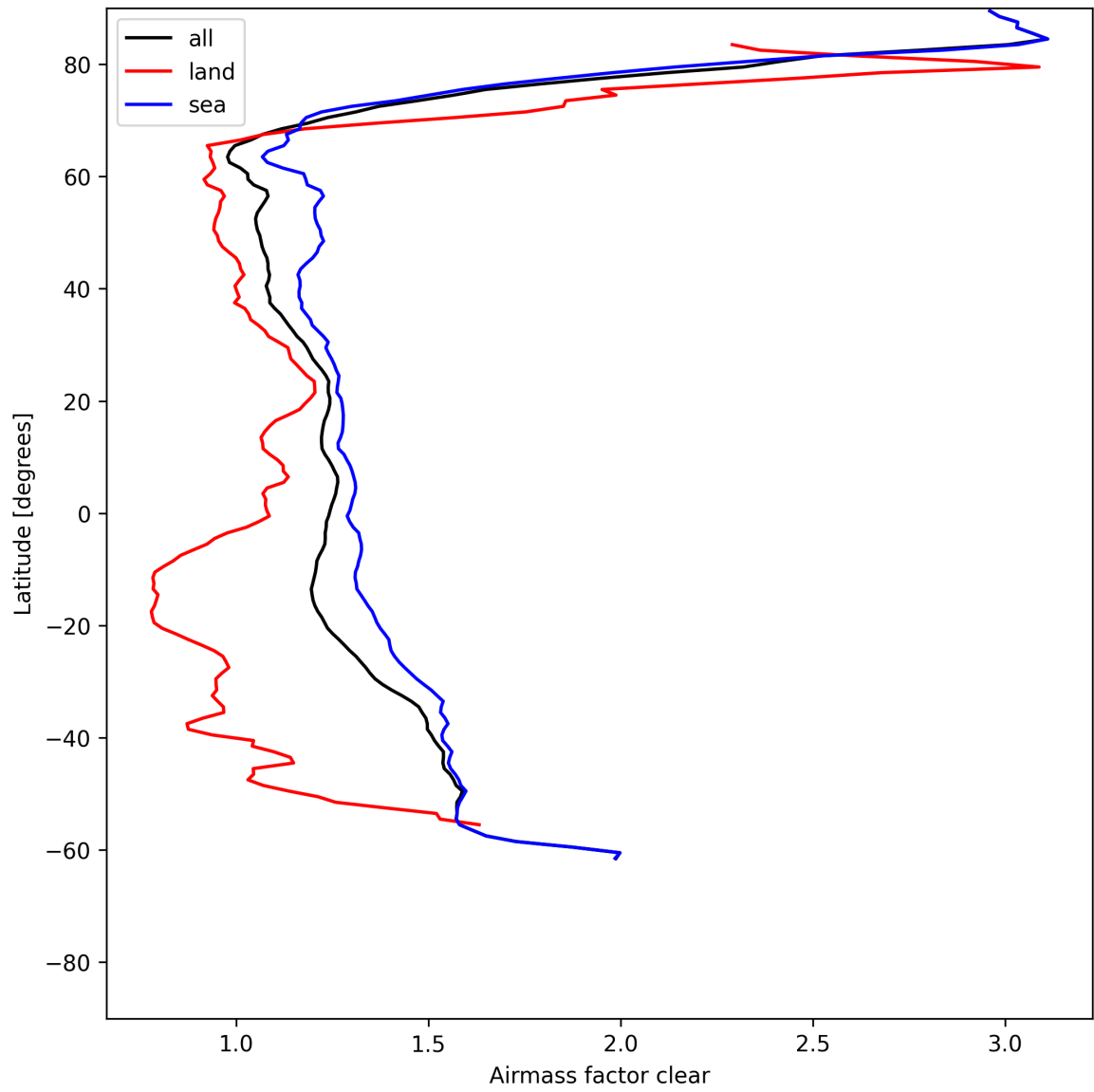
Figure 26: Zonal average of “Airmass factor clear” for 2025-07-04 to 2025-07-05.
