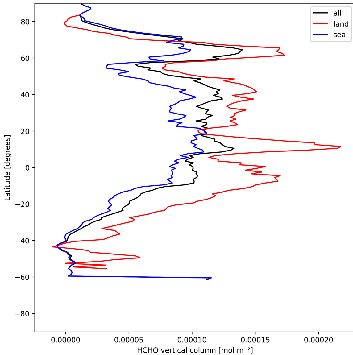
Figure 19: Zonal average of “HCHO vertical column” for 2025-07-04 to 2025-07-05.
