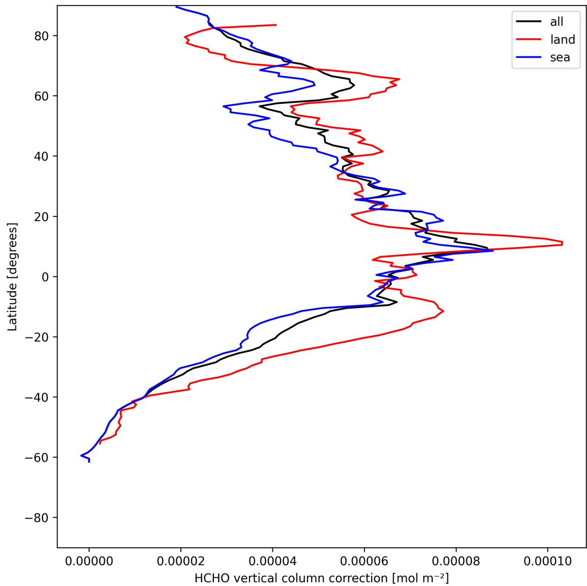
Figure 21: Zonal average of “HCHO vertical column correction” for 2025-07-04 to 2025-07-05.
