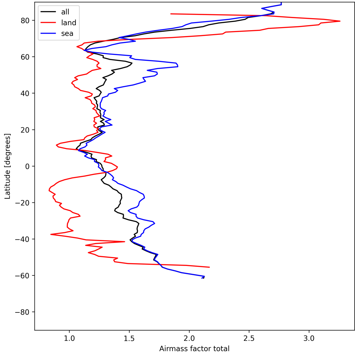
Figure 24: Zonal average of “Airmass factor total” for 2025-07-04 to 2025-07-05.
