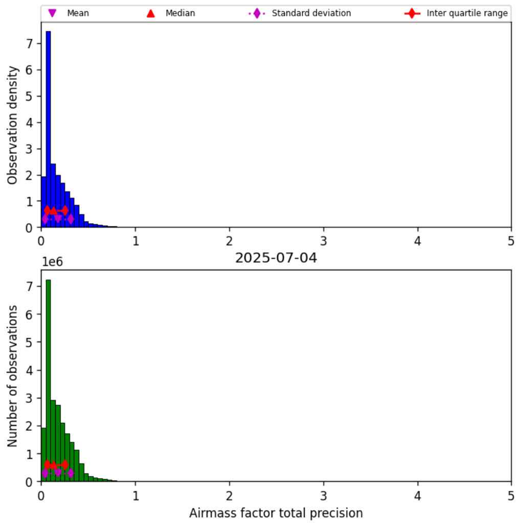
Figure 39: Histogram of “Airmass factor total precision” for 2025-07-04 to 2025-07-05
