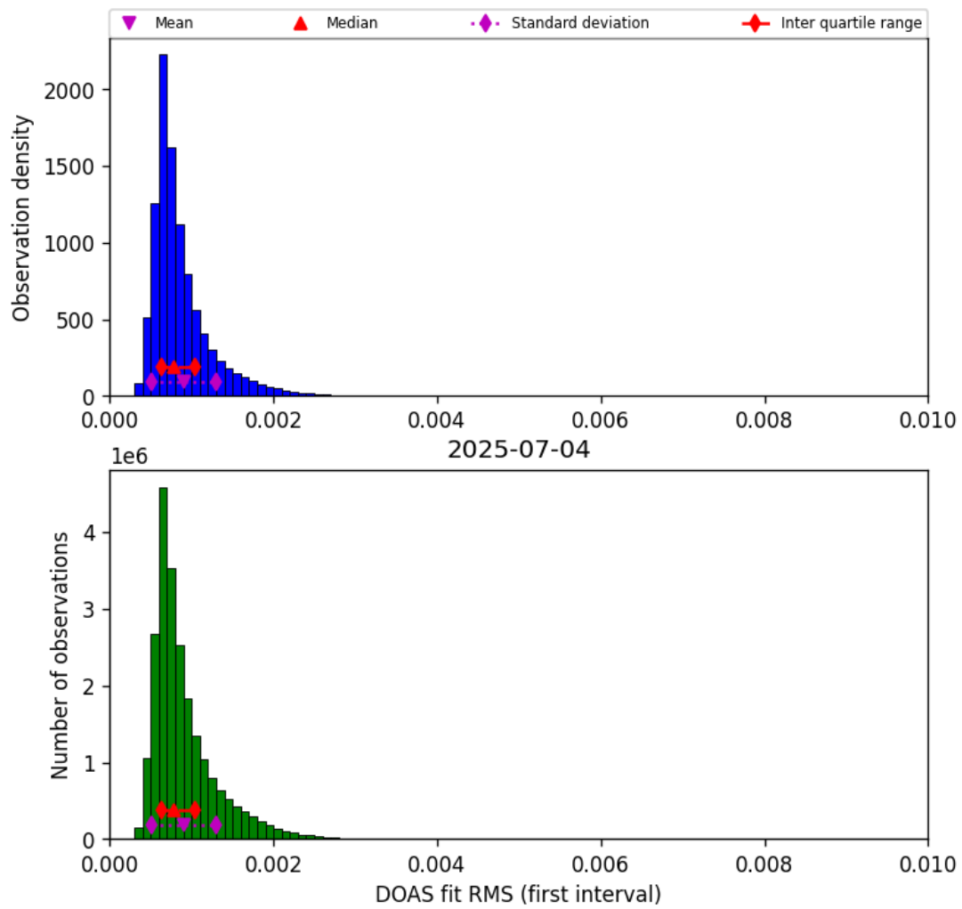
Figure 44: Histogram of “DOAS fit RMS (first interval)” for 2025-07-04 to 2025-07-05
