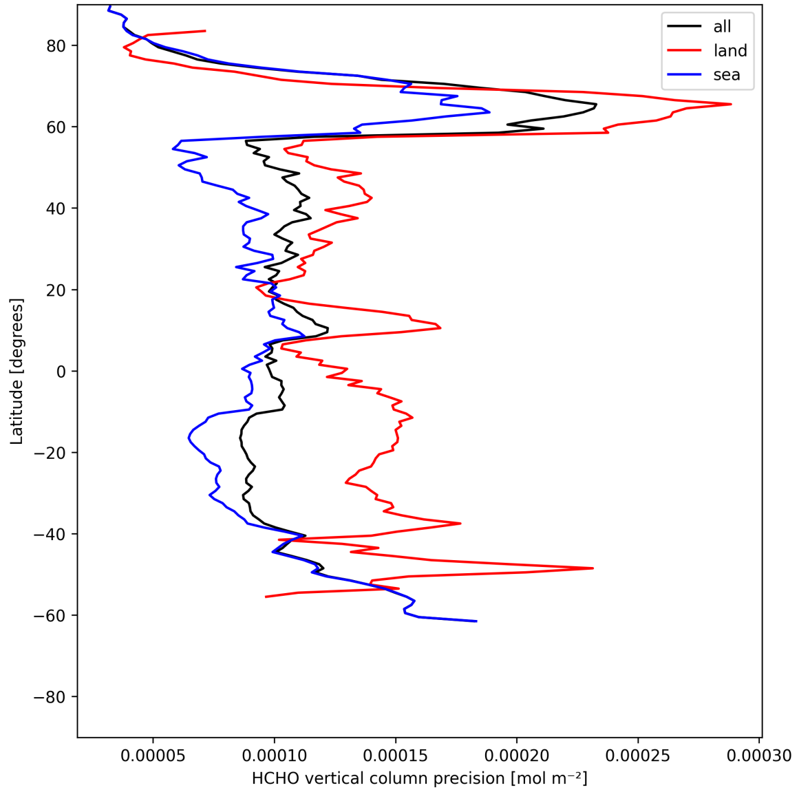
Figure 20: Zonal average of “HCHO vertical column precision” for 2025-07-04 to 2025-07-05.
