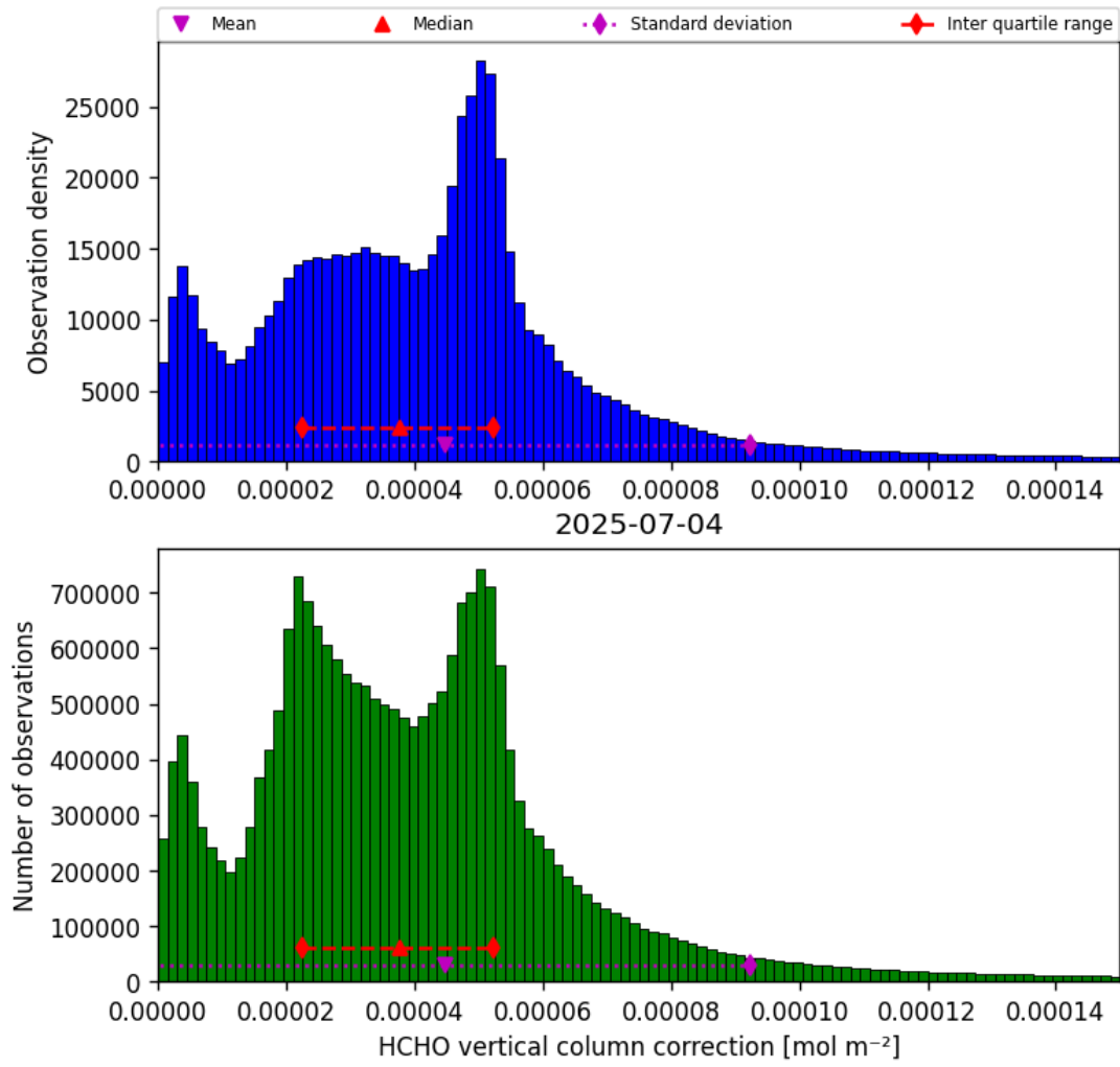
Figure 35: Histogram of “HCHO vertical column correction” for 2025-07-04 to 2025-07-05
