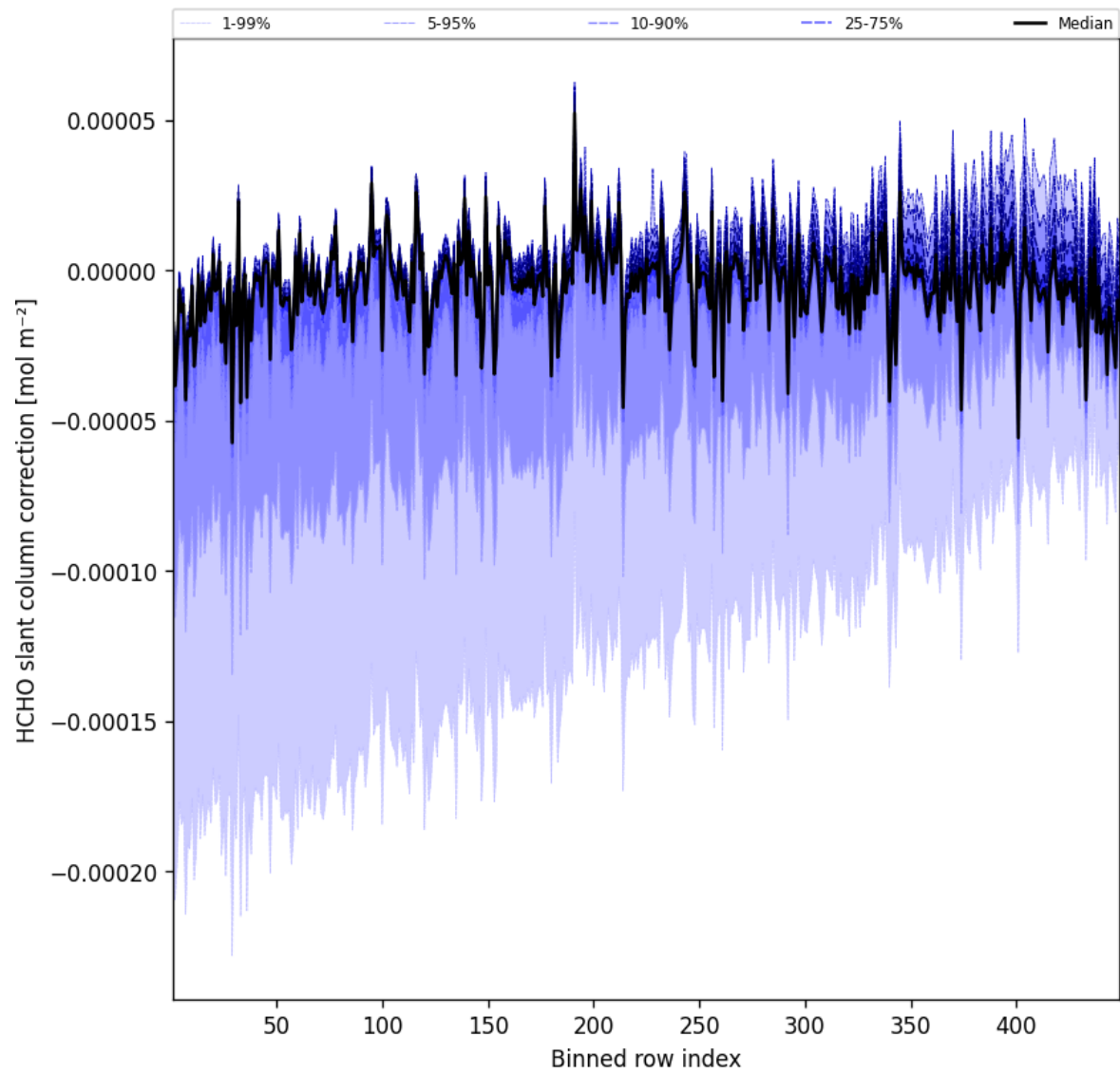
Figure 59: Along track statistics of “HCHO slant column correction” for 2025-07-04 to 2025-07-05
