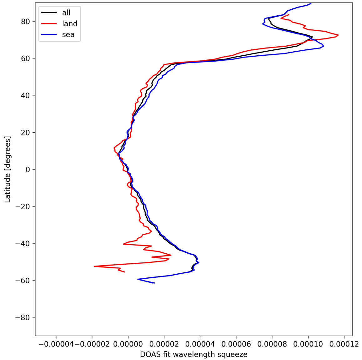
Figure 29: Zonal average of “DOAS fit wavelength squeeze” for 2025-07-04 to 2025-07-05.
