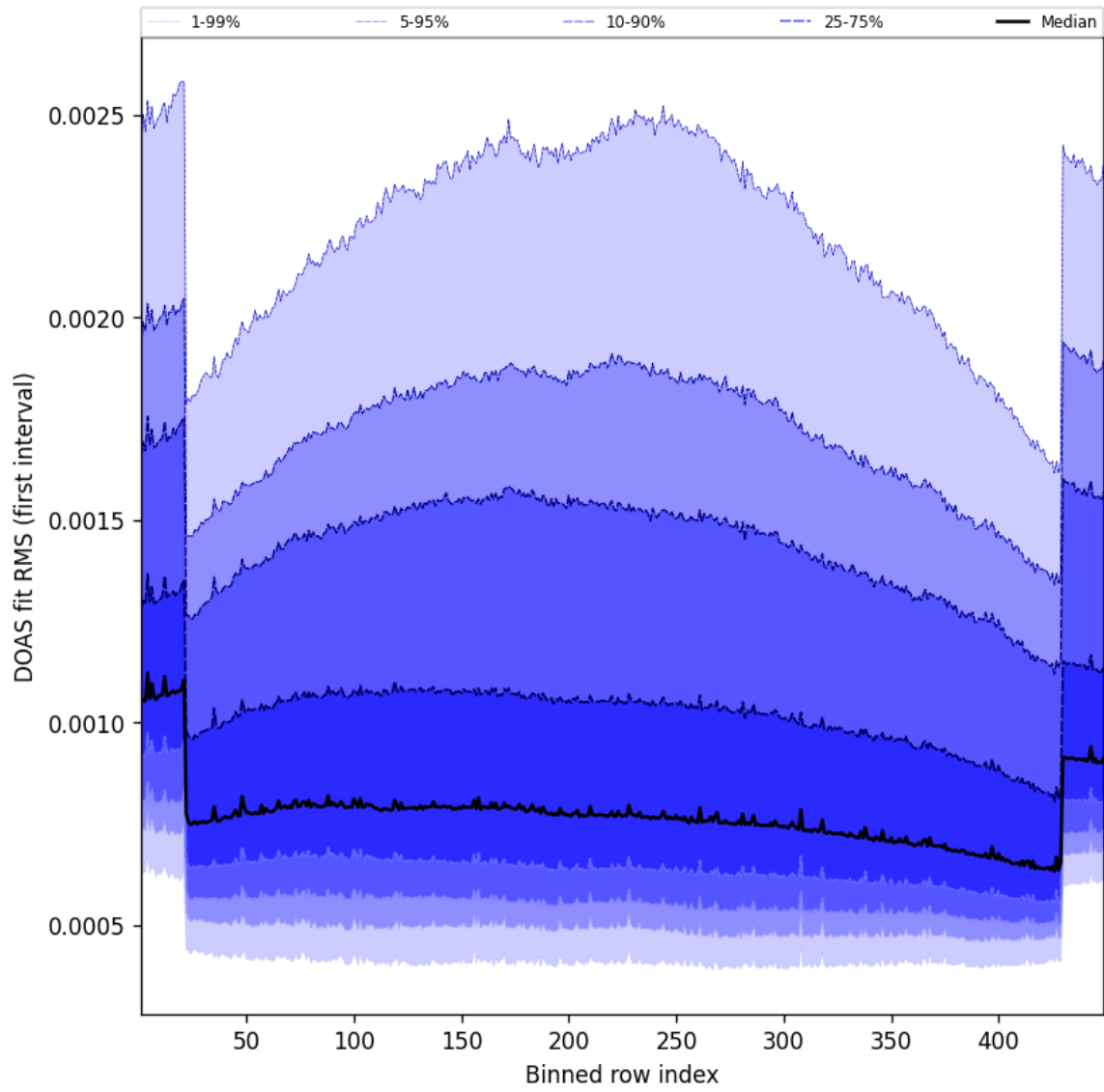
Figure 58: Along track statistics of “DOAS fit RMS (first interval)” for 2025-07-04 to 2025-07-05
