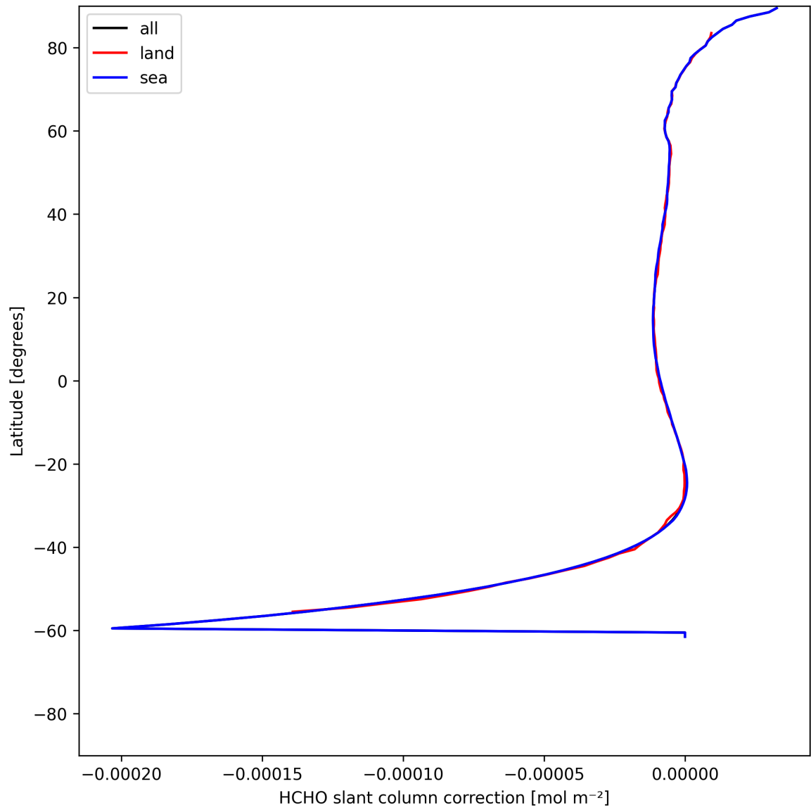
Figure 31: Zonal average of “HCHO slant column correction” for 2025-07-04 to 2025-07-05.
