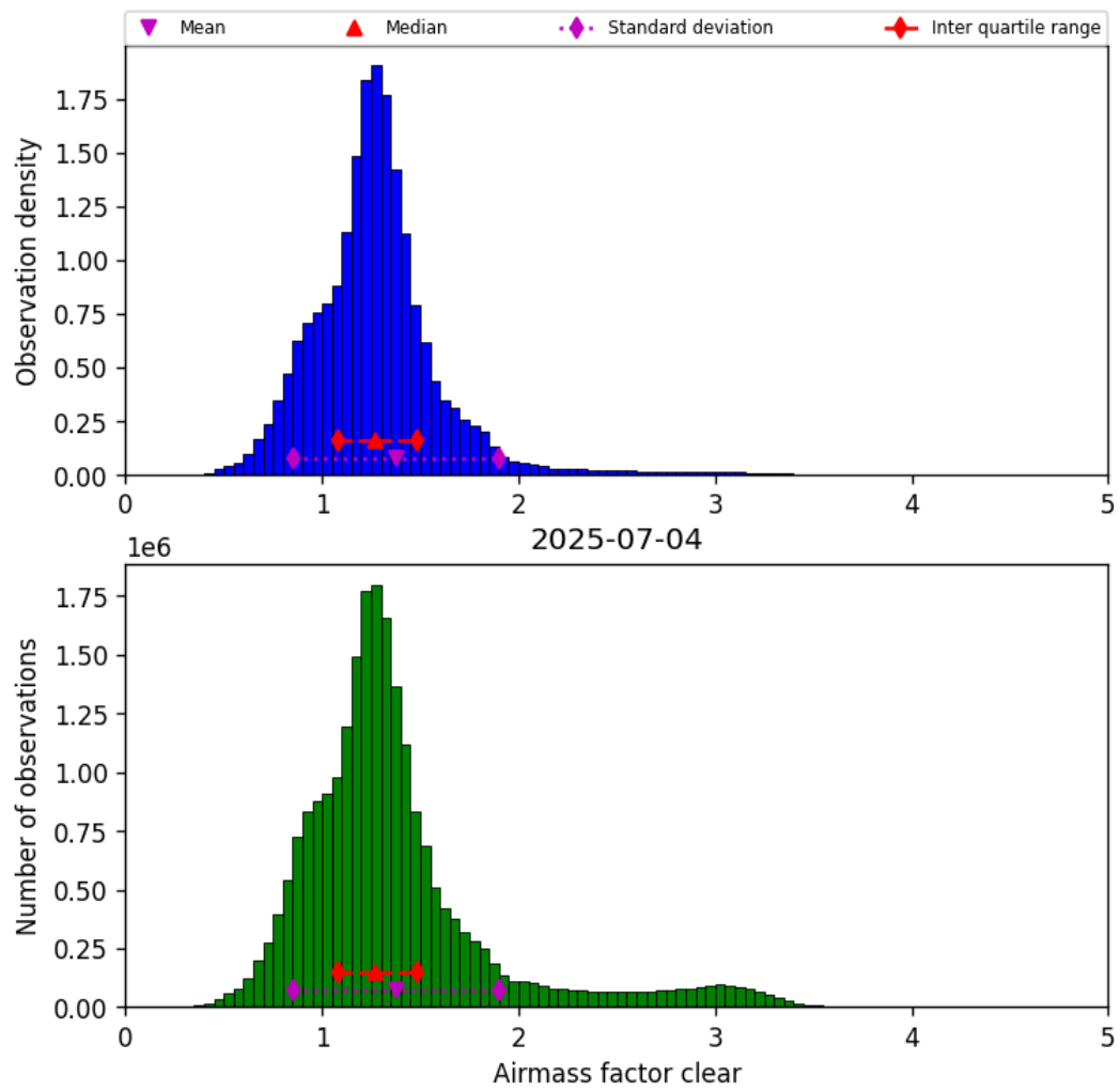
Figure 40: Histogram of “Airmass factor clear” for 2025-07-04 to 2025-07-05
