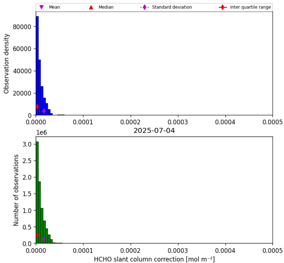
Figure 45: Histogram of “HCHO slant column correction” for 2025-07-04 to 2025-07-05
