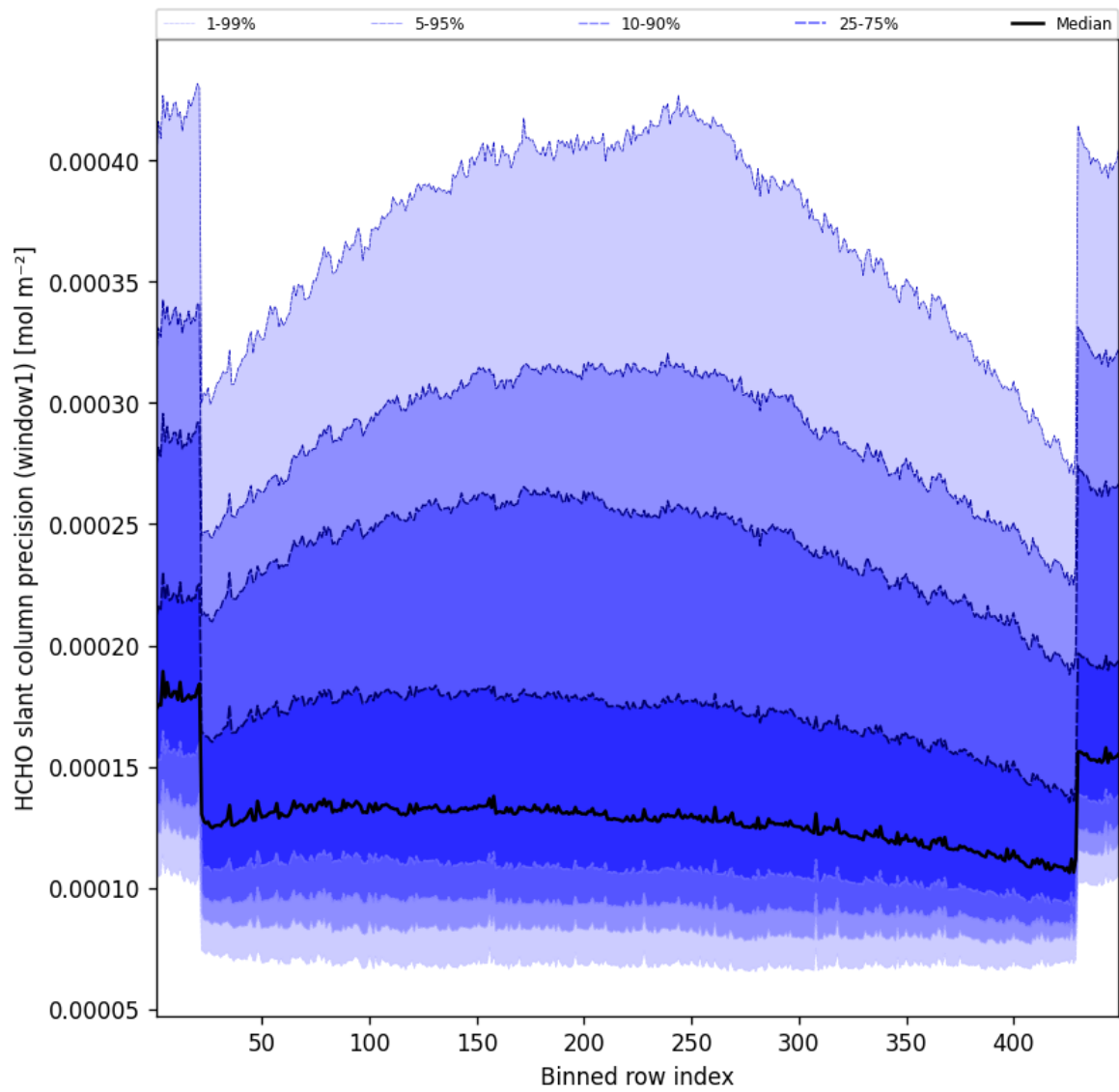
Figure 51: Along track statistics of “HCHO slant column precision (window1)” for 2025-07-04 to 2025-07-05
