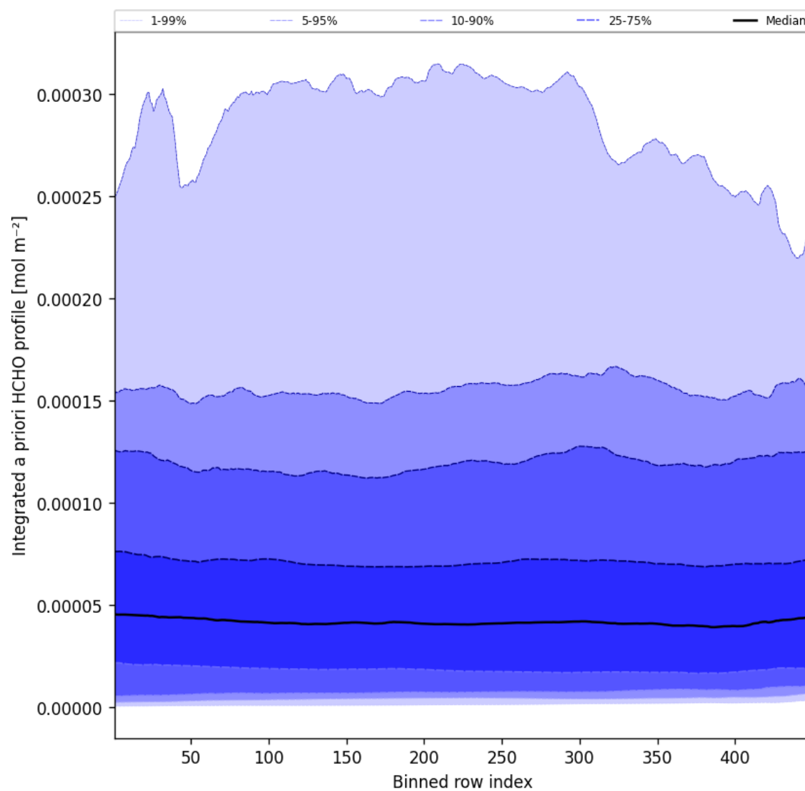
Figure 55: Along track statistics of “Integrated a priori HCHO profile” for 2025-07-04 to 2025-07-05
