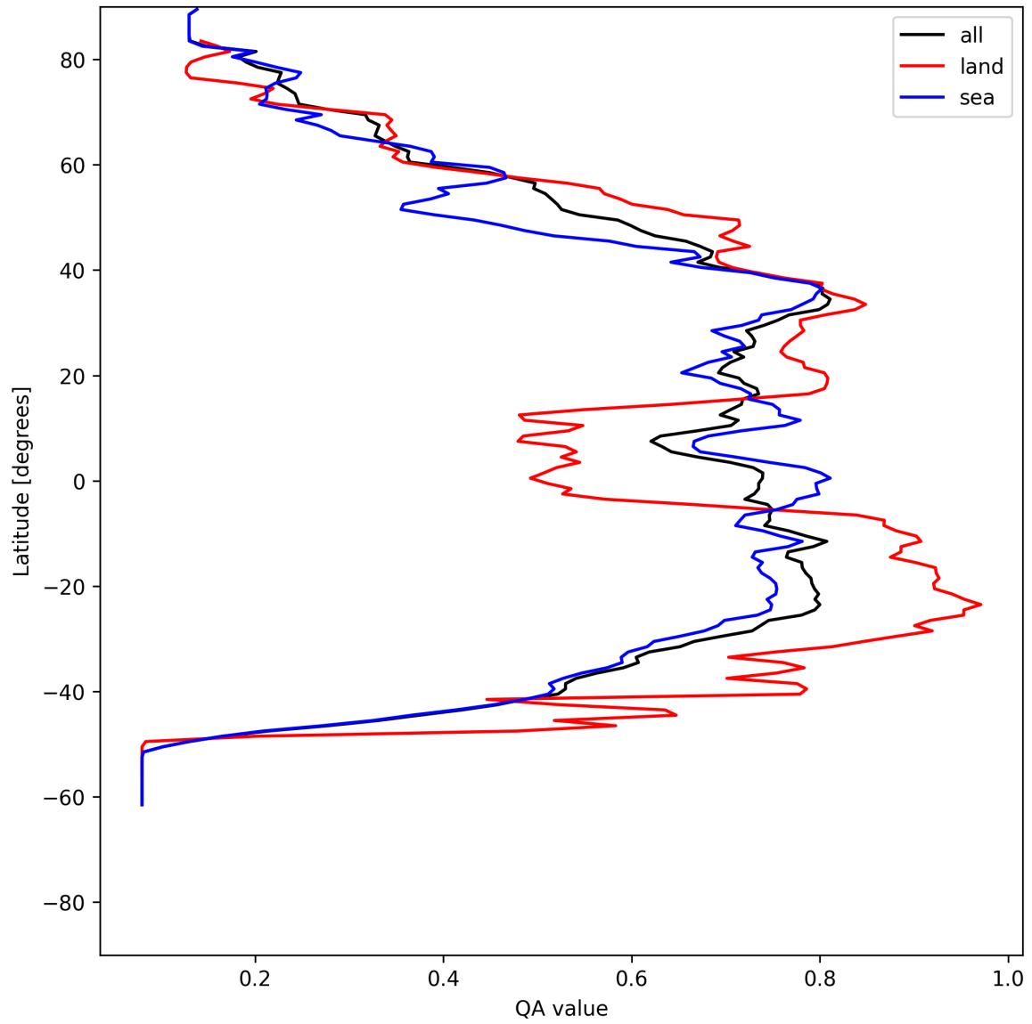
Figure 18: Zonal average of “QA value” for 2025-07-04 to 2025-07-05.
