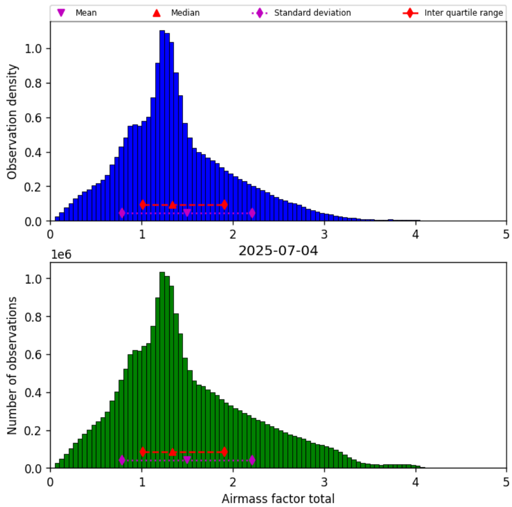
Figure 38: Histogram of “Airmass factor total” for 2025-07-04 to 2025-07-05
