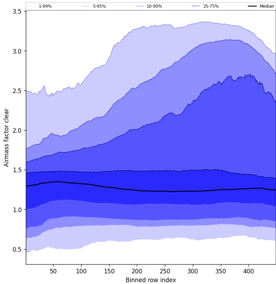
Figure 54: Along track statistics of “Airmass factor clear” for 2025-07-05 to 2025-07-06
