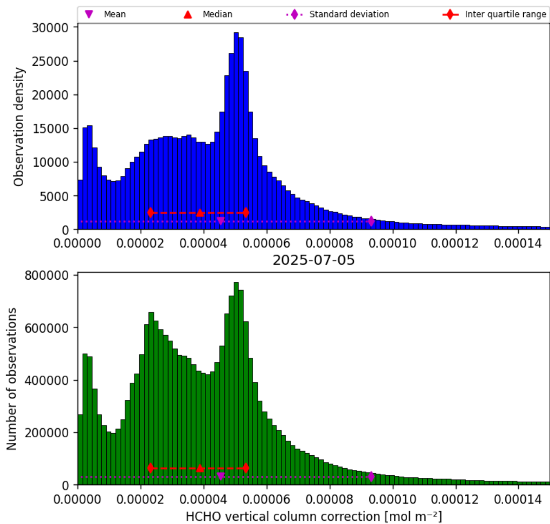
Figure 35: Histogram of “HCHO vertical column correction” for 2025-07-05 to 2025-07-06
