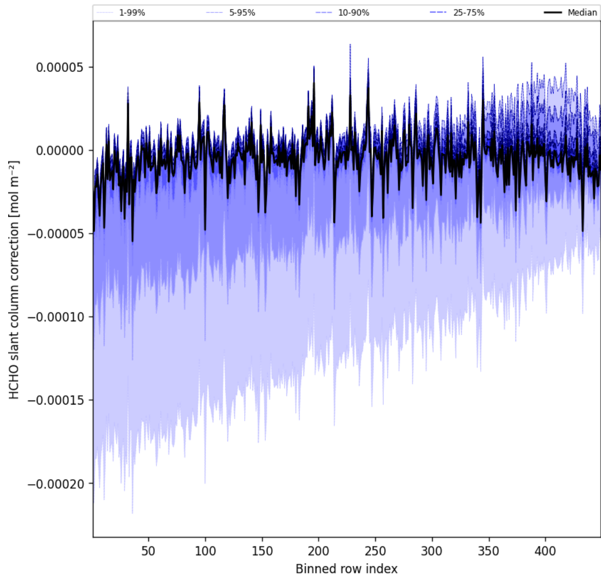
Figure 59: Along track statistics of “HCHO slant column correction” for 2025-07-05 to 2025-07-06
