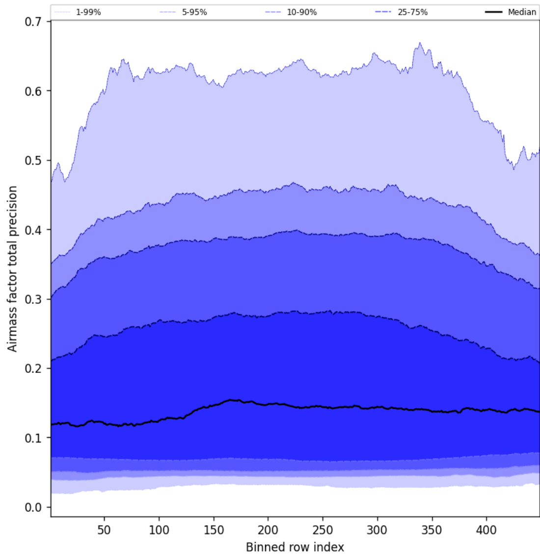
Figure 53: Along track statistics of “Airmass factor total precision” for 2025-07-05 to 2025-07-06
