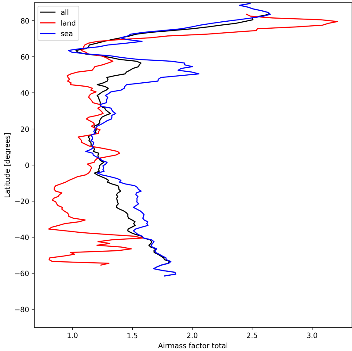
Figure 24: Zonal average of “Airmass factor total” for 2025-07-05 to 2025-07-06.
