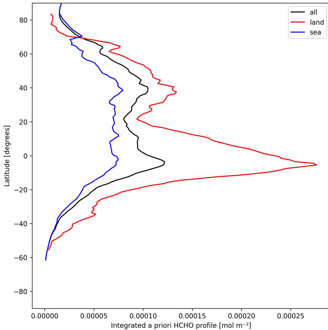
Figure 27: Zonal average of “Integrated a priori HCHO profile” for 2025-07-05 to 2025-07-06.
