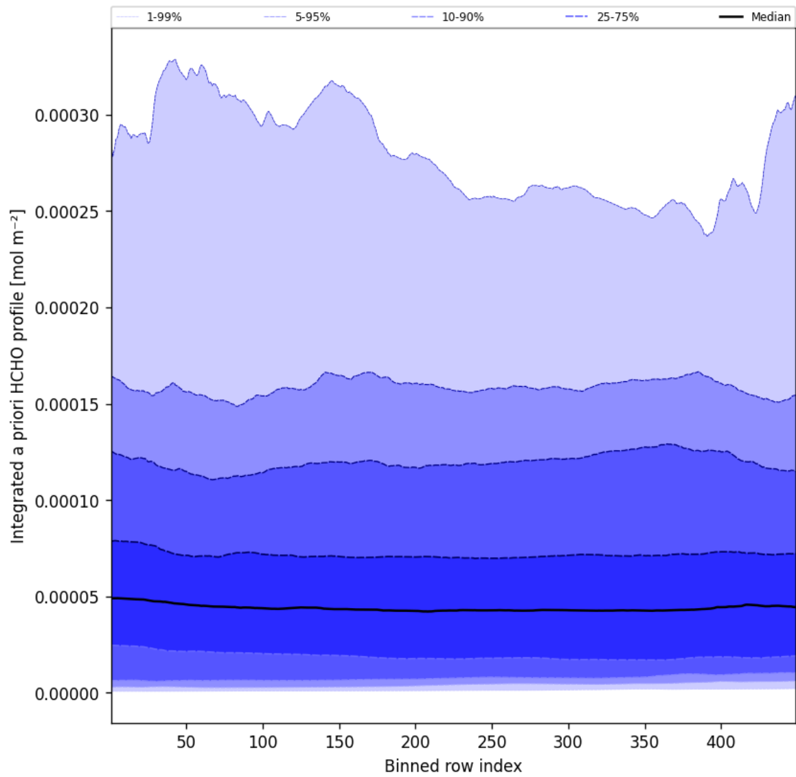
Figure 55: Along track statistics of “Integrated a priori HCHO profile” for 2025-07-05 to 2025-07-06
