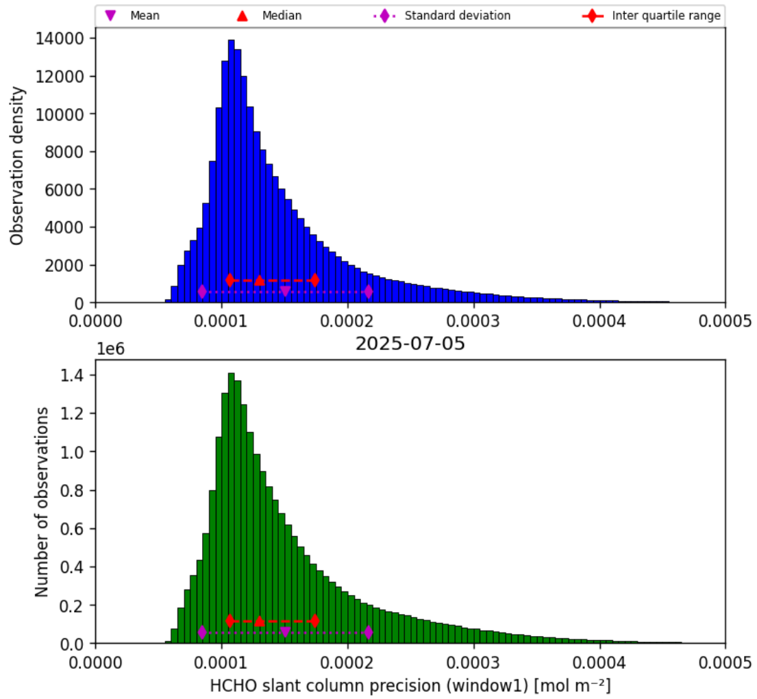
Figure 37: Histogram of “HCHO slant column precision (window1)” for 2025-07-05 to 2025-07-06
