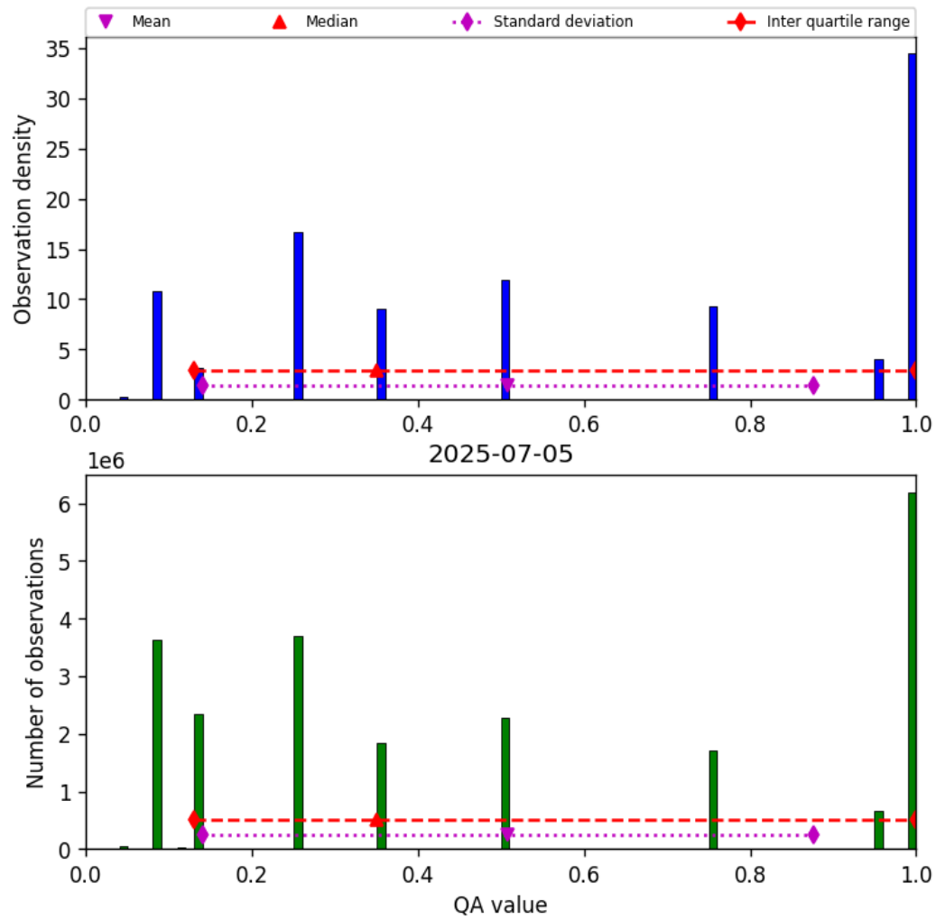
Figure 32: Histogram of “QA value” for 2025-07-05 to 2025-07-06
