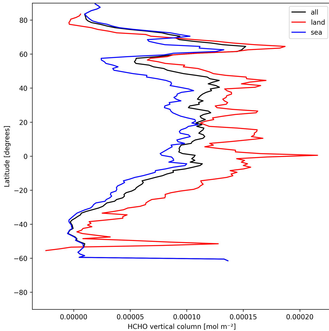
Figure 19: Zonal average of “HCHO vertical column” for 2025-07-05 to 2025-07-06.
