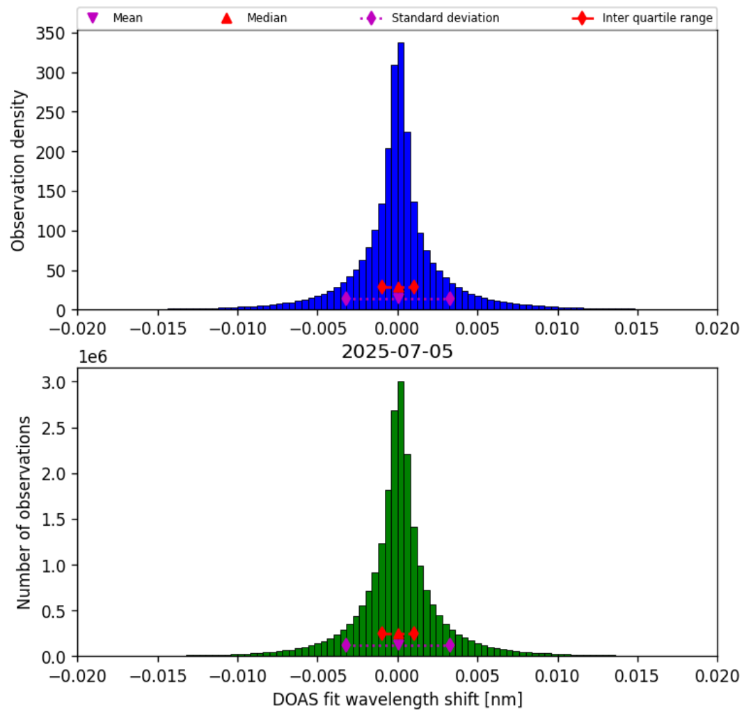
Figure 42: Histogram of “DOAS fit wavelength shift” for 2025-07-05 to 2025-07-06
