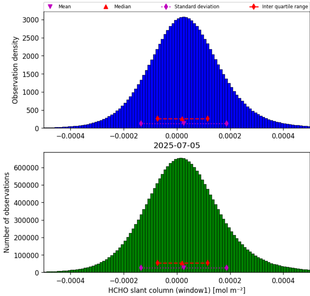
Figure 36: Histogram of “HCHO slant column (window1)” for 2025-07-05 to 2025-07-06
