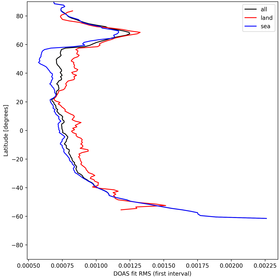
Figure 30: Zonal average of "DOAS fit RMS (first interval)" for 2025-07-05 to 2025-07-06.
