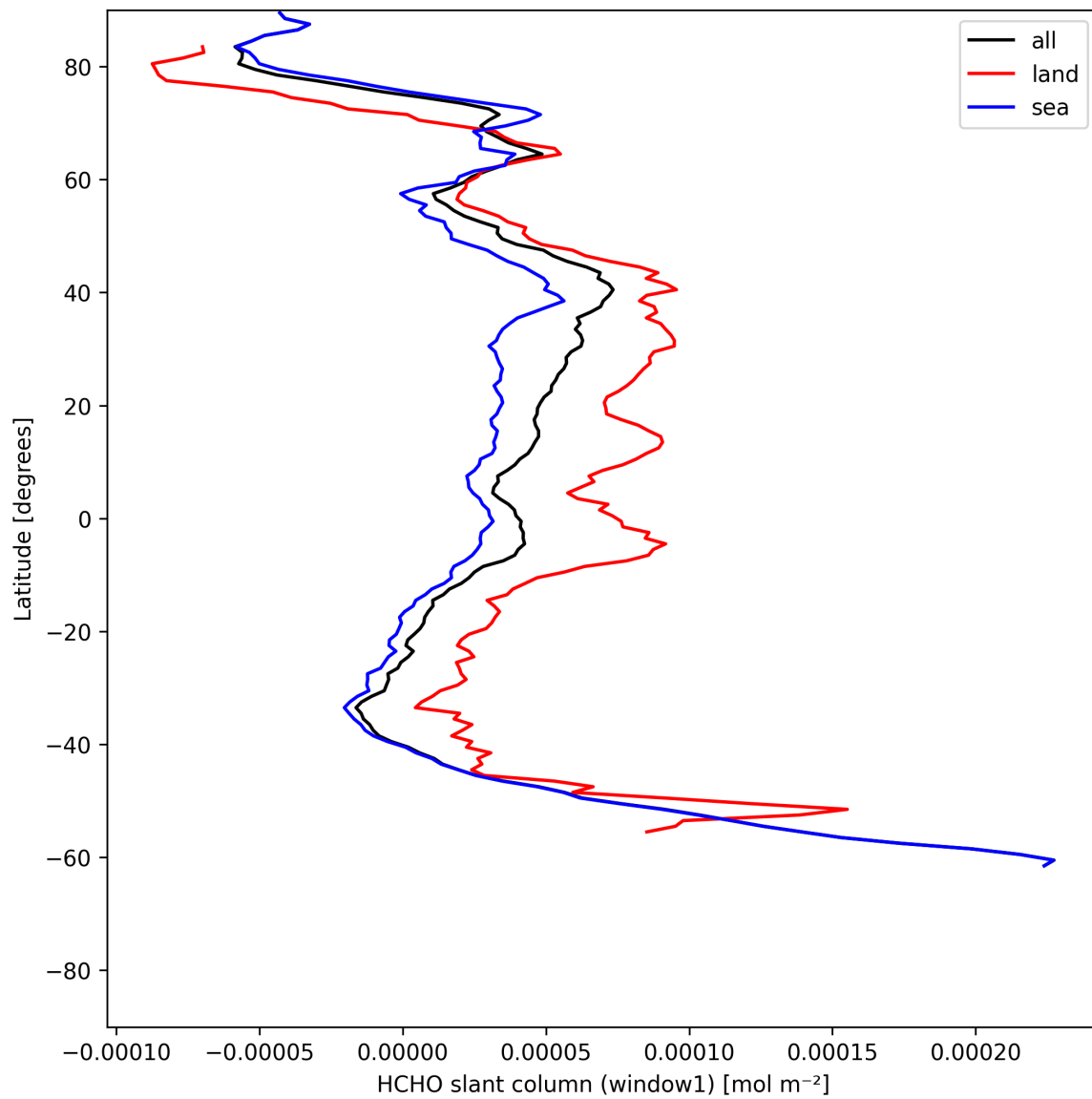
Figure 22: Zonal average of “HCHO slant column (window1)” for 2025-07-05 to 2025-07-06.
