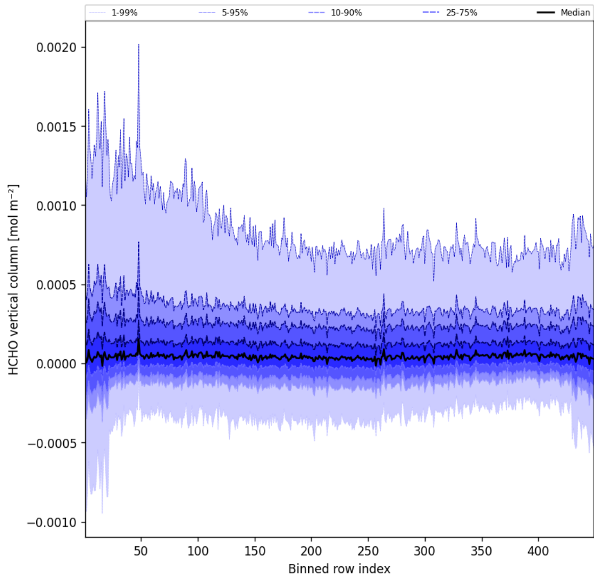
Figure 47: Along track statistics of “HCHO vertical column” for 2025-07-05 to 2025-07-06
