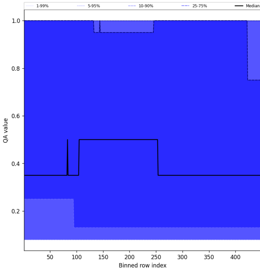
Figure 46: Along track statistics of “QA value” for 2025-07-05 to 2025-07-06
