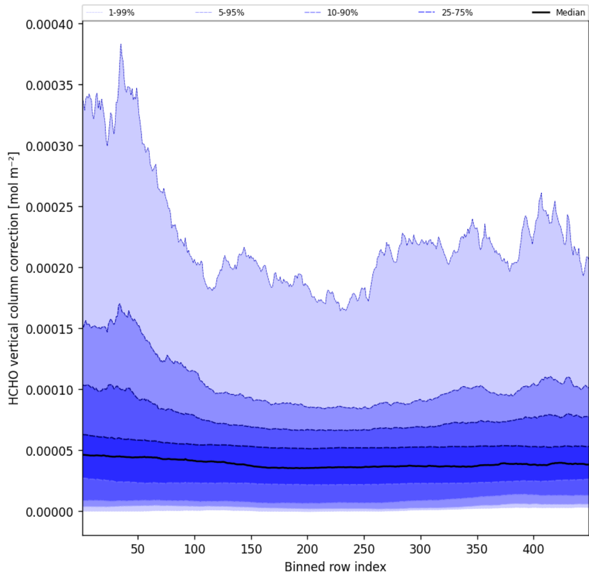
Figure 49: Along track statistics of “HCHO vertical column correction” for 2025-07-05 to 2025-07-06
