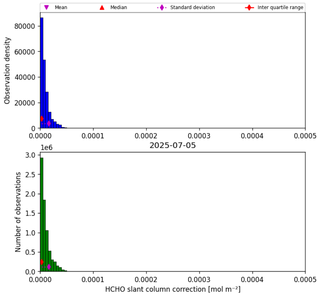
Figure 45: Histogram of “HCHO slant column correction” for 2025-07-05 to 2025-07-06
