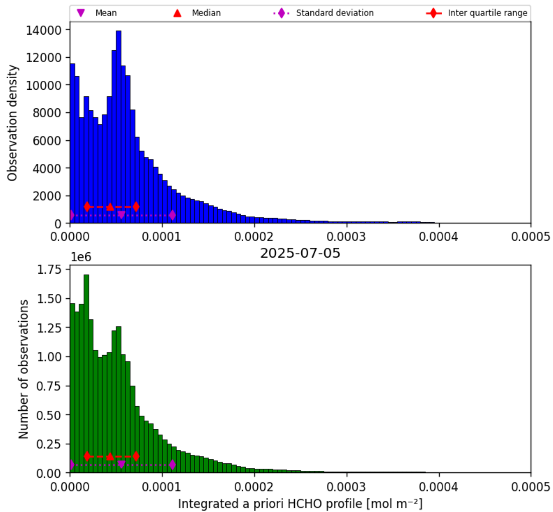
Figure 41: Histogram of “Integrated a priori HCHO profile” for 2025-07-05 to 2025-07-06
