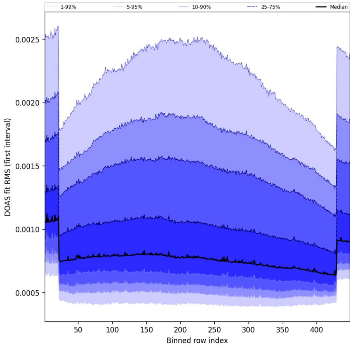
Figure 58: Along track statistics of “DOAS fit RMS (first interval)” for 2025-07-05 to 2025-07-06
