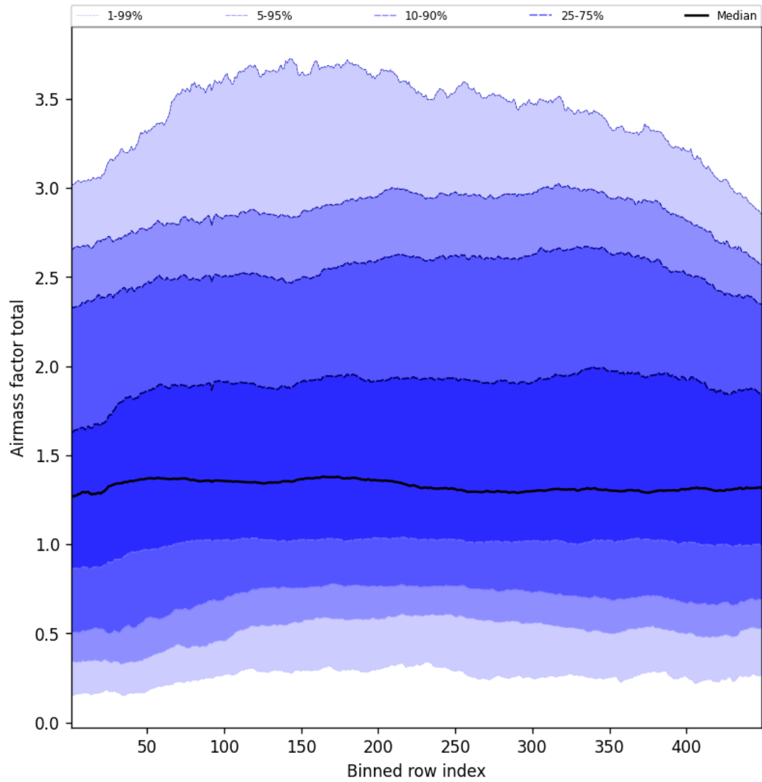
Figure 52: Along track statistics of “Airmass factor total” for 2025-07-05 to 2025-07-06
