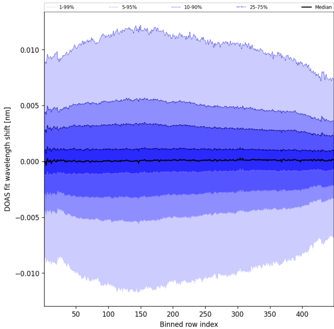
Figure 56: Along track statistics of “DOAS fit wavelength shift” for 2025-07-05 to 2025-07-06
