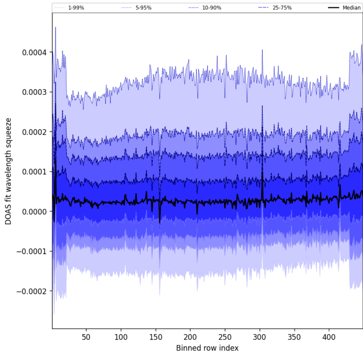
Figure 57: Along track statistics of “DOAS fit wavelength squeeze” for 2025-07-05 to 2025-07-06
