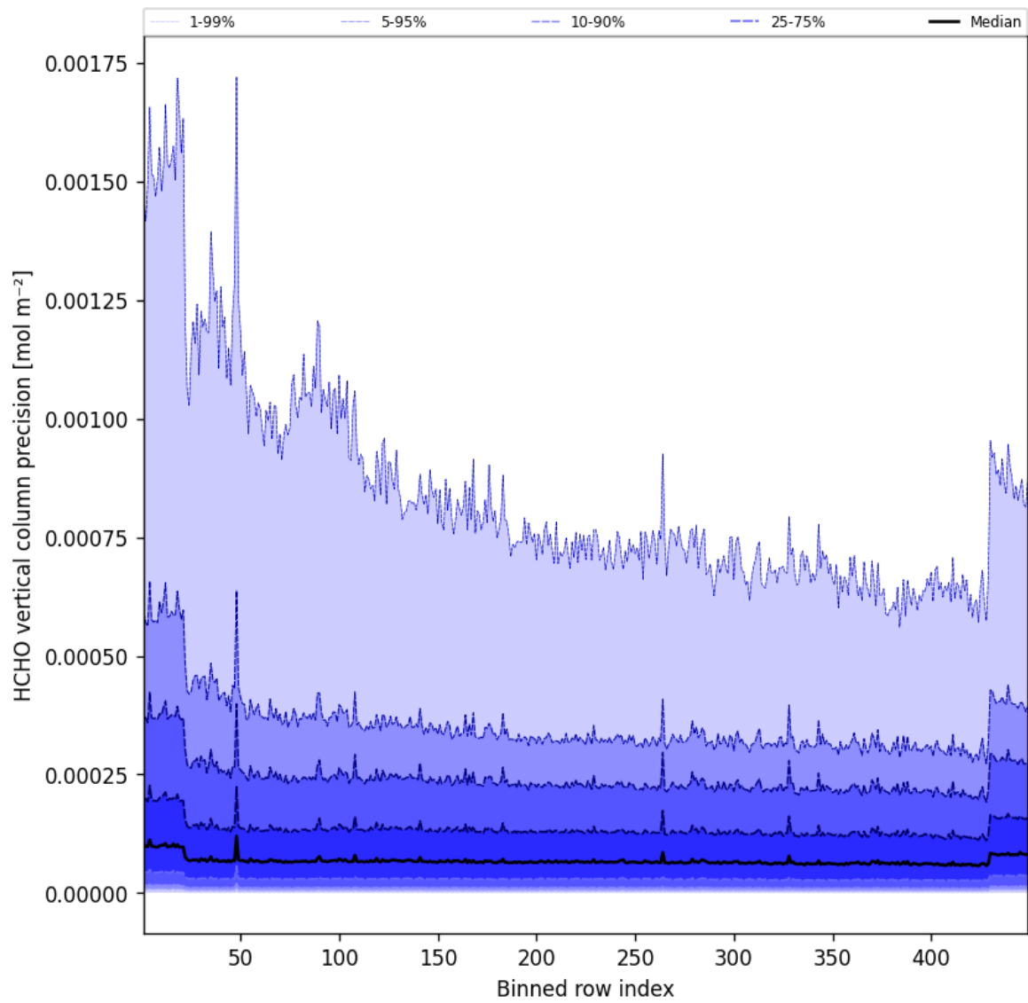
Figure 48: Along track statistics of “HCHO vertical column precision” for 2025-07-05 to 2025-07-06
