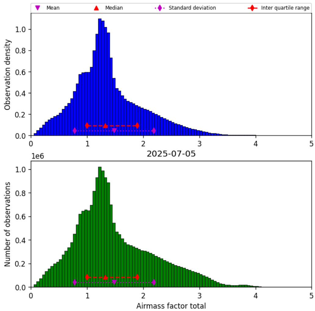
Figure 38: Histogram of “Airmass factor total” for 2025-07-05 to 2025-07-06
