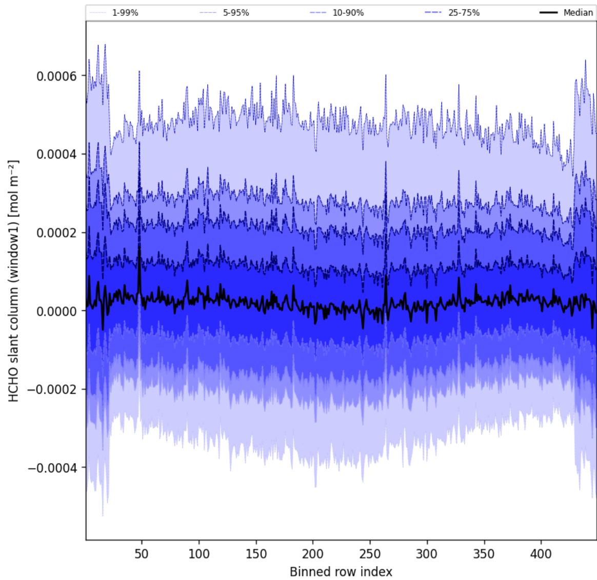
Figure 50: Along track statistics of “HCHO slant column (window1)” for 2025-07-05 to 2025-07-06
