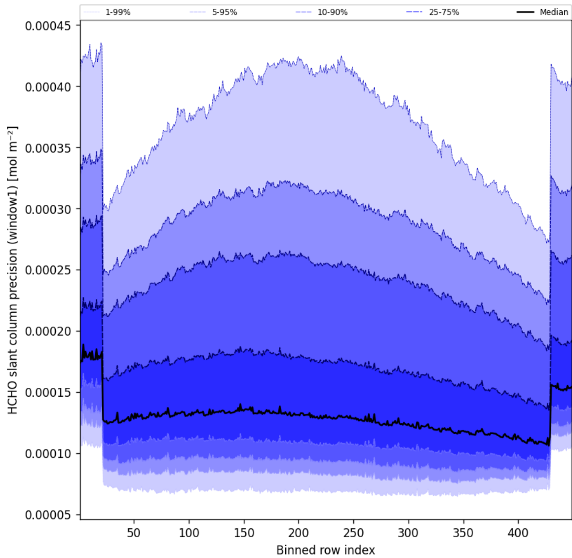
Figure 51: Along track statistics of “HCHO slant column precision (window1)” for 2025-07-05 to 2025-07-06
