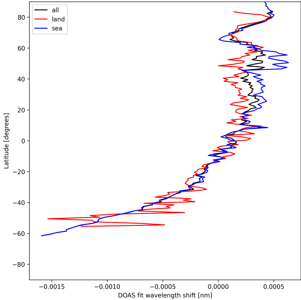
Figure 28: Zonal average of “DOAS fit wavelength shift” for 2025-07-05 to 2025-07-06.
