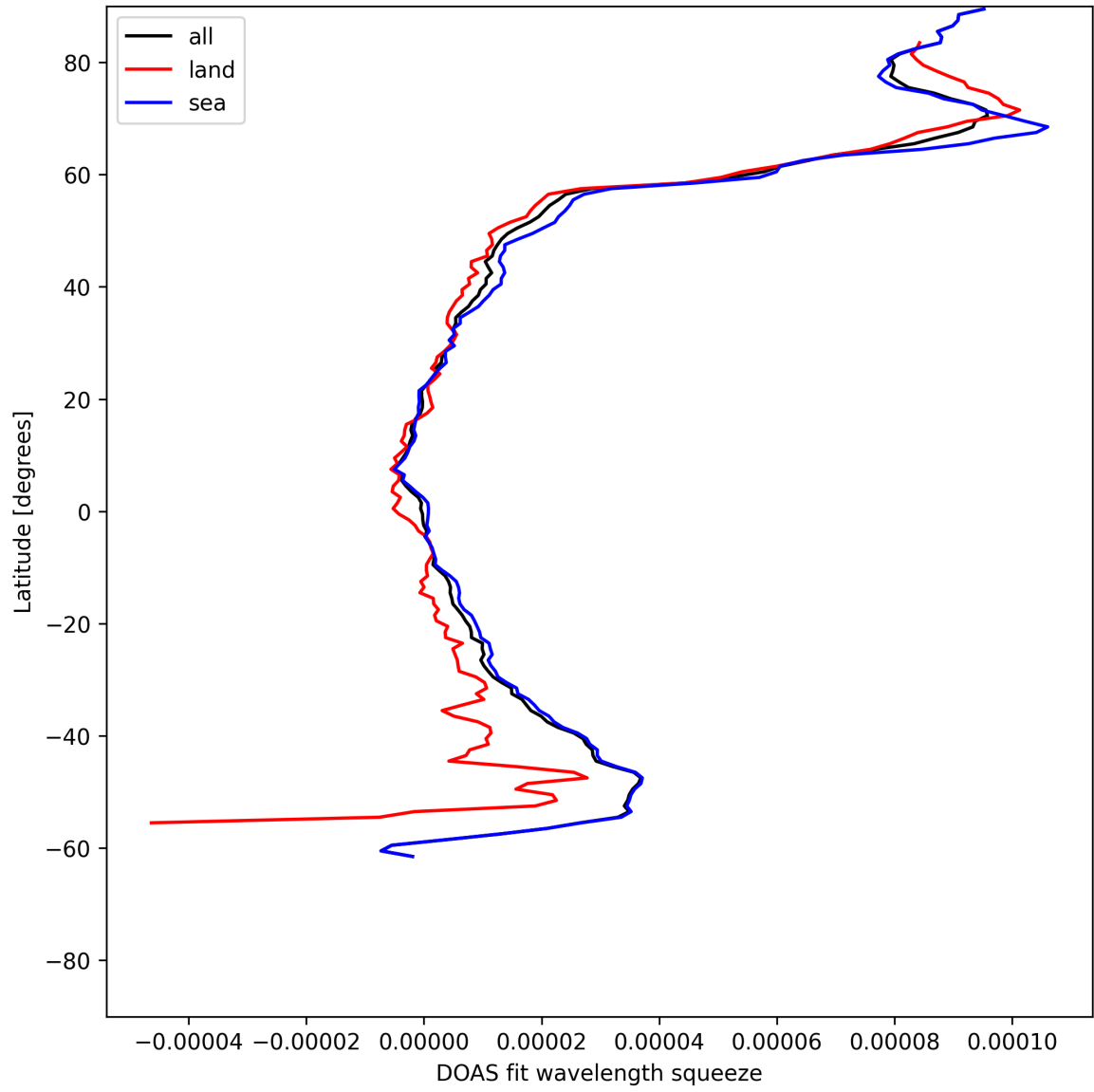
Figure 29: Zonal average of “DOAS fit wavelength squeeze” for 2025-07-05 to 2025-07-06.
