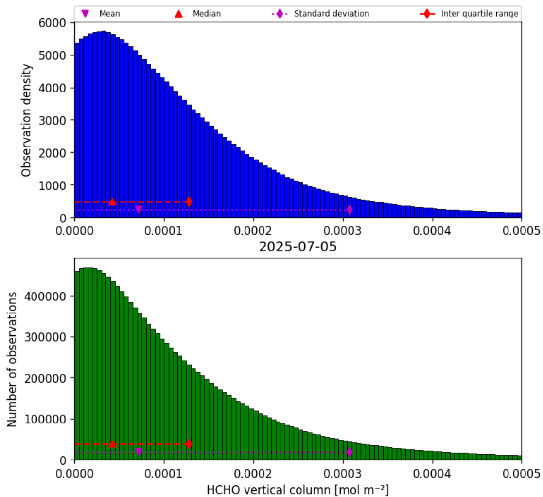
Figure 33: Histogram of “HCHO vertical column” for 2025-07-05 to 2025-07-06
