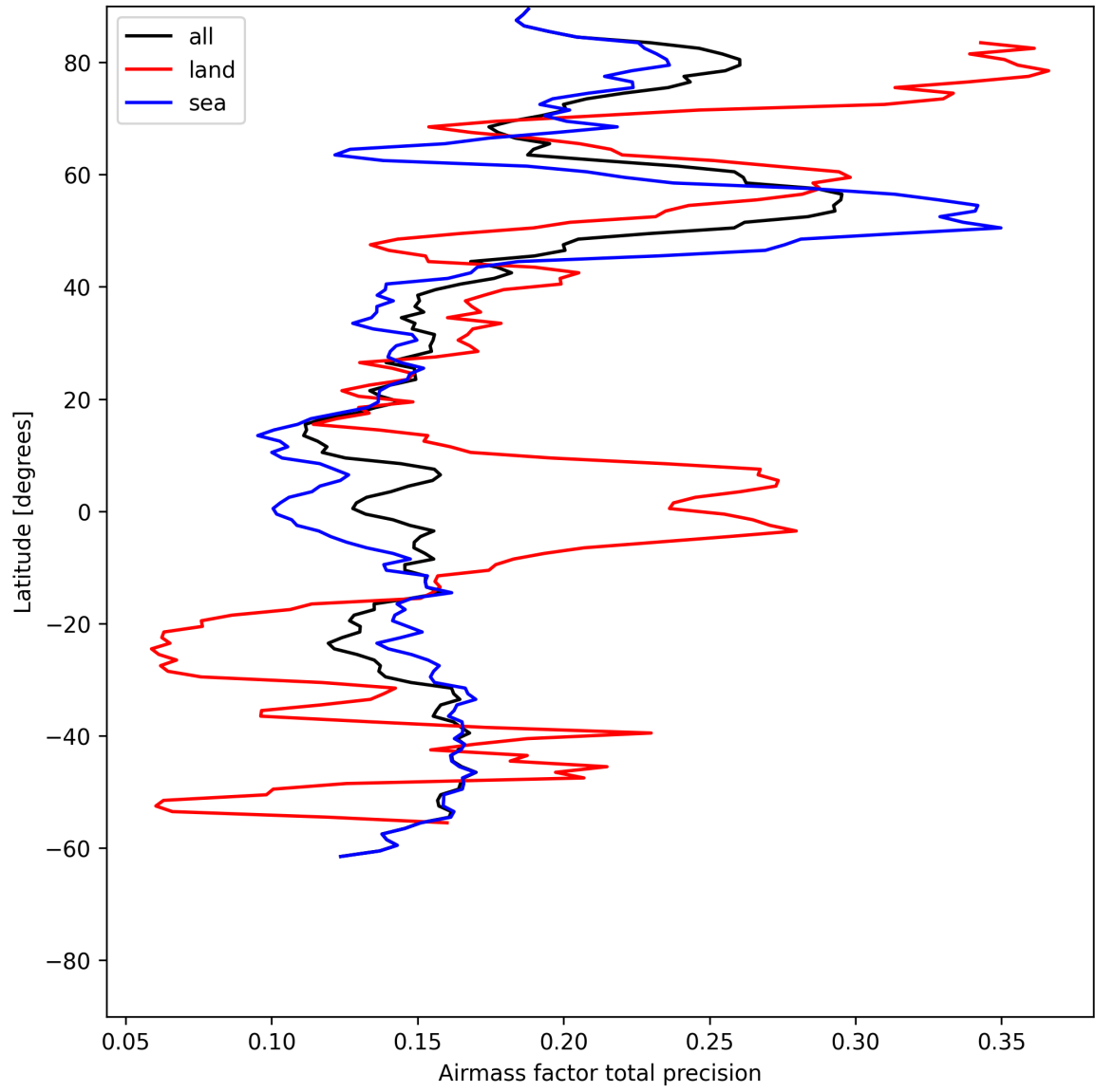
Figure 25: Zonal average of “Airmass factor total precision” for 2025-07-05 to 2025-07-06.
