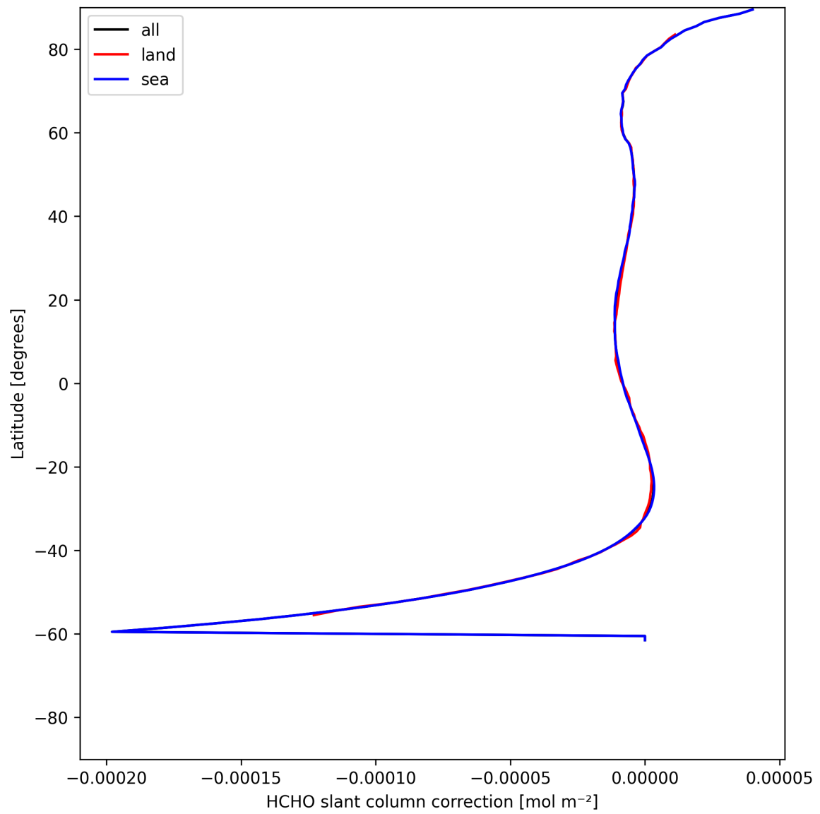
Figure 31: Zonal average of “HCHO slant column correction” for 2025-07-05 to 2025-07-06.
