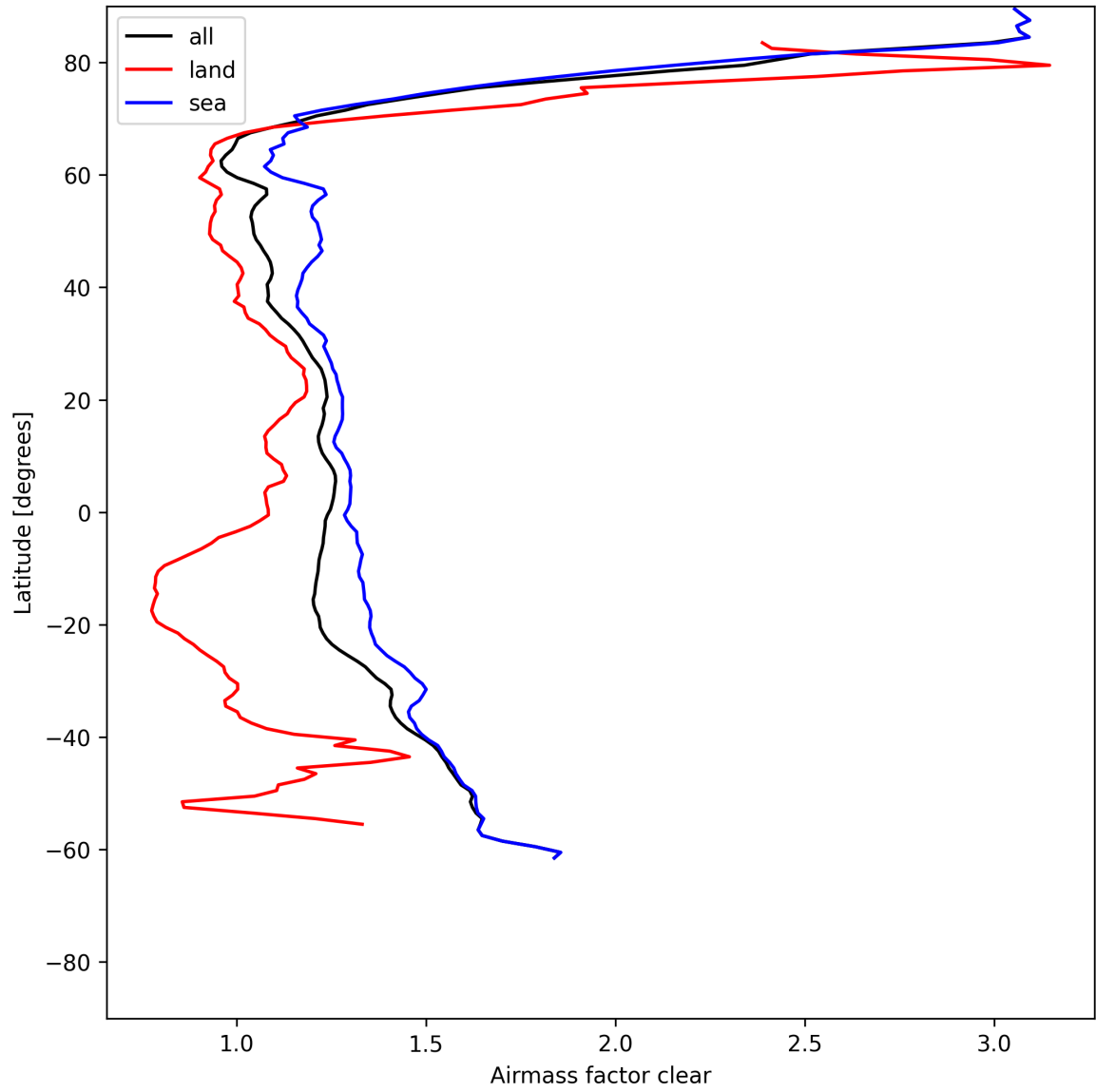
Figure 26: Zonal average of “Airmass factor clear” for 2025-07-05 to 2025-07-06.
