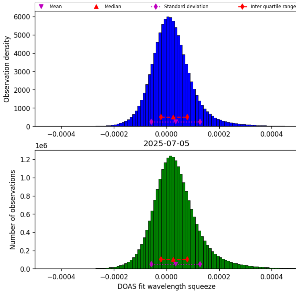
Figure 43: Histogram of “DOAS fit wavelength squeeze” for 2025-07-05 to 2025-07-06
