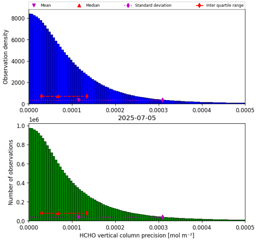
Figure 34: Histogram of “HCHO vertical column precision” for 2025-07-05 to 2025-07-06
