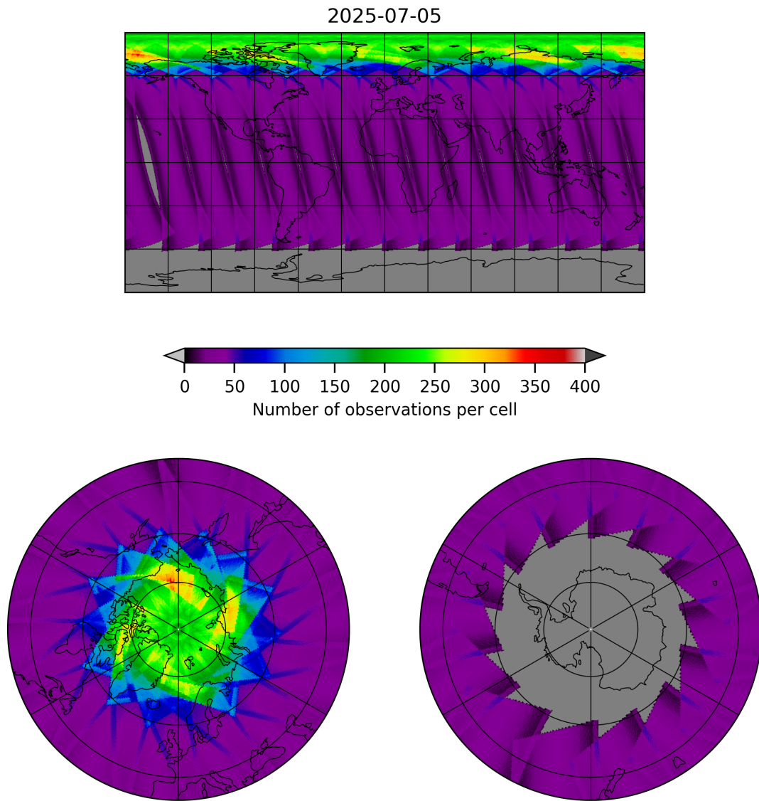
Figure 17: Map of the number of observations for 2025-07-05 to 2025-07-06
