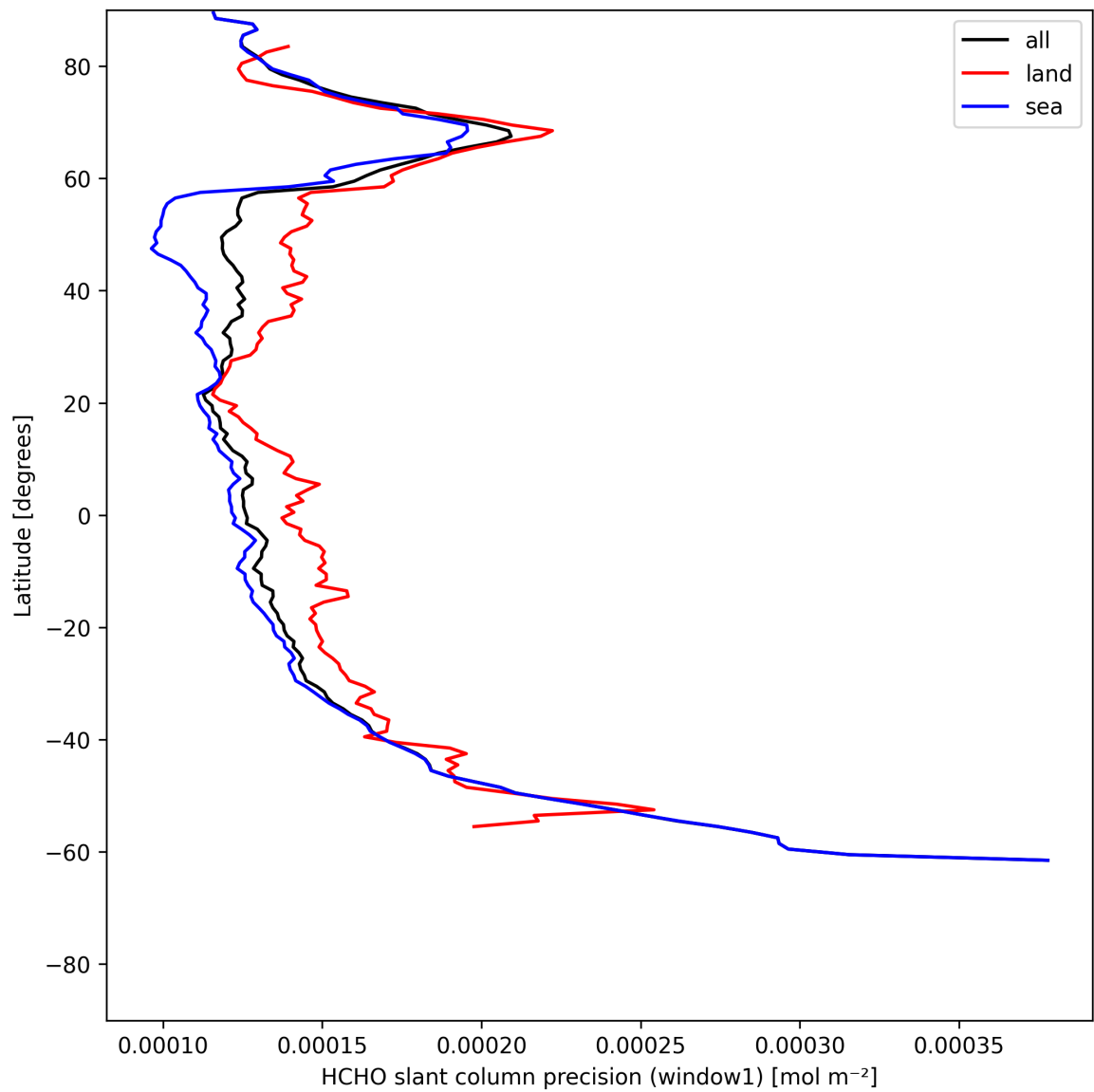
Figure 23: Zonal average of “HCHO slant column precision (window1)” for 2025-07-05 to 2025-07-06.
