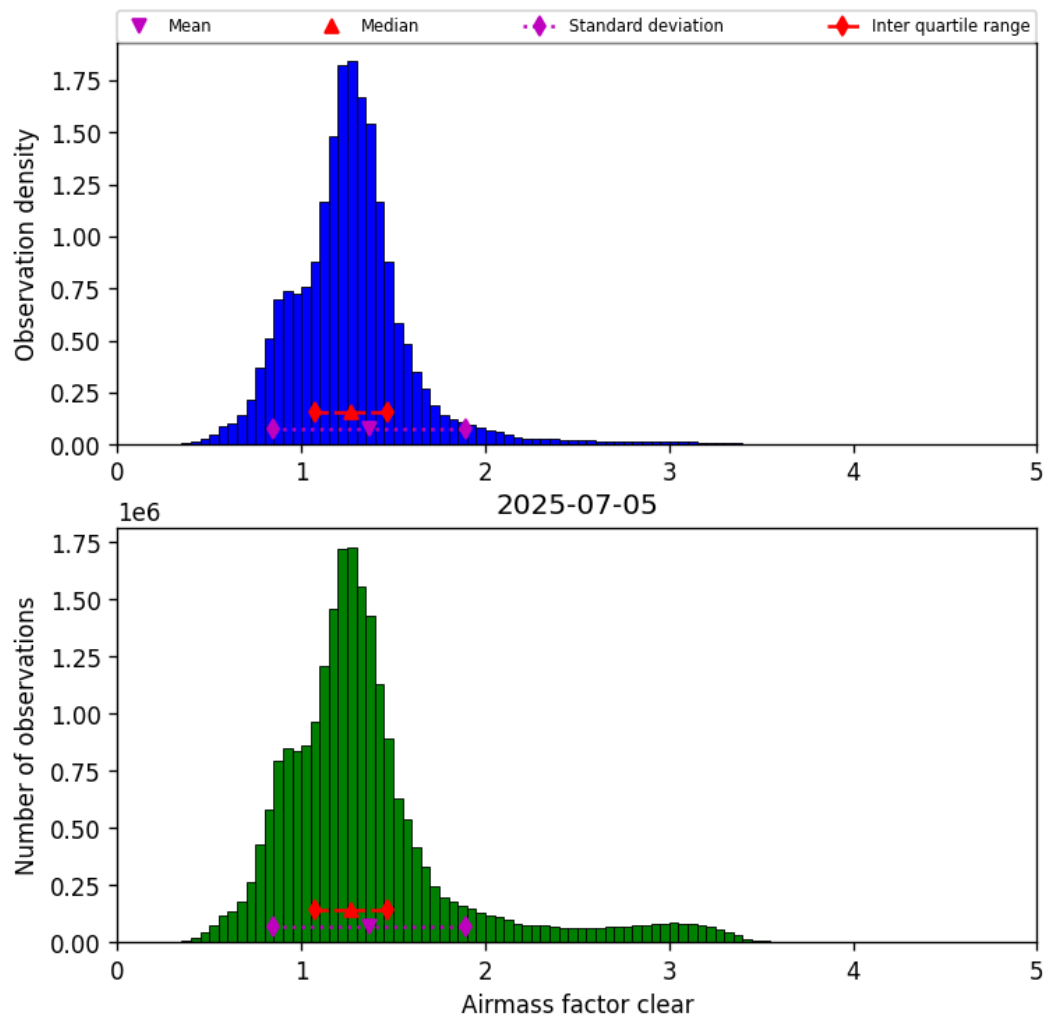
Figure 40: Histogram of “Airmass factor clear” for 2025-07-05 to 2025-07-06
