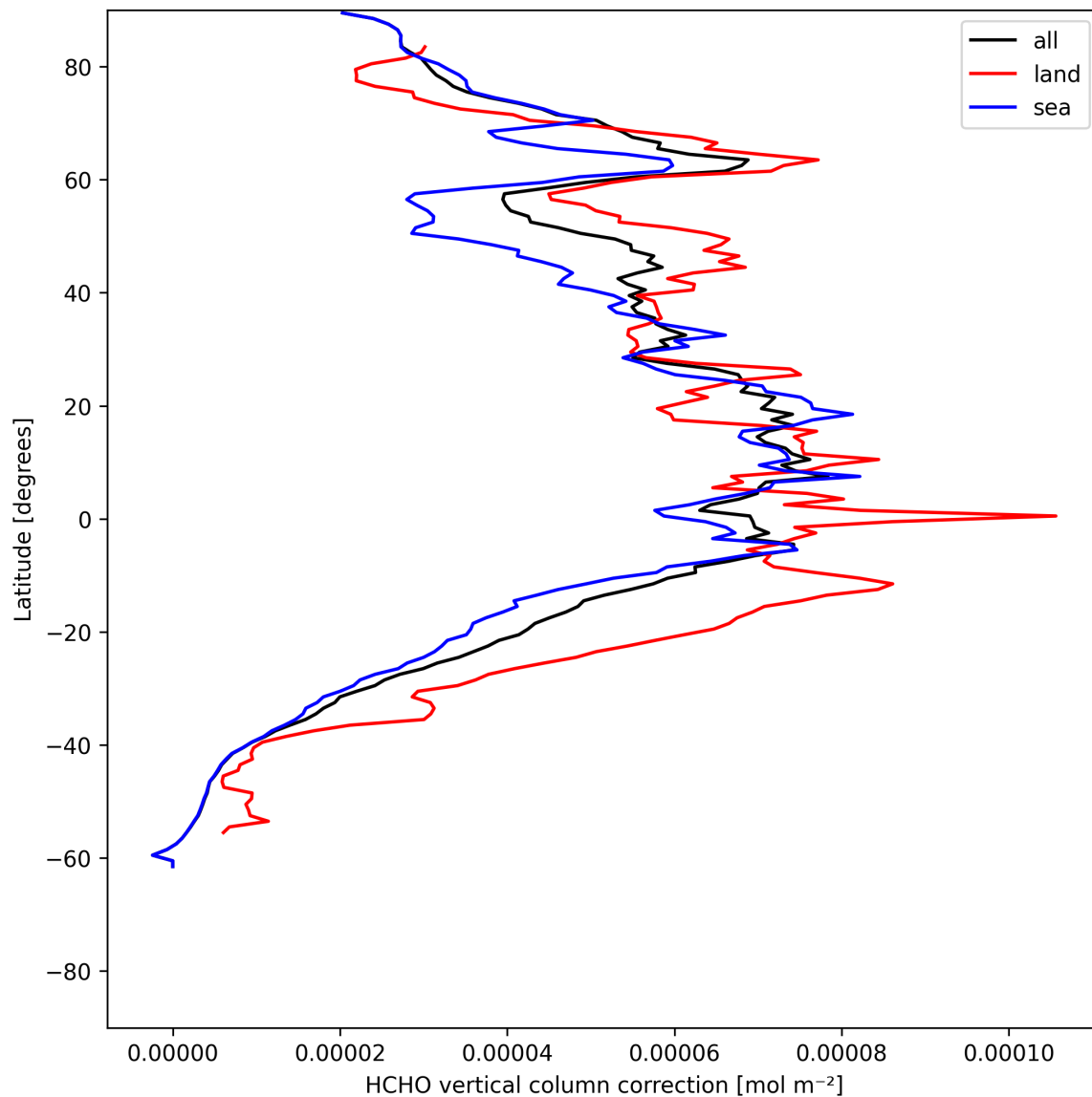
Figure 21: Zonal average of “HCHO vertical column correction” for 2025-07-05 to 2025-07-06.
