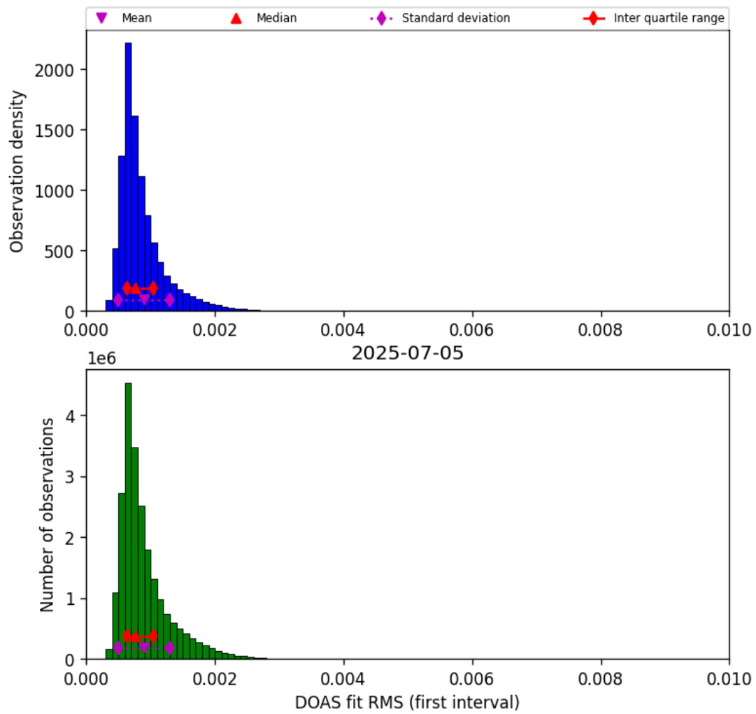
Figure 44: Histogram of “DOAS fit RMS (first interval)” for 2025-07-05 to 2025-07-06
