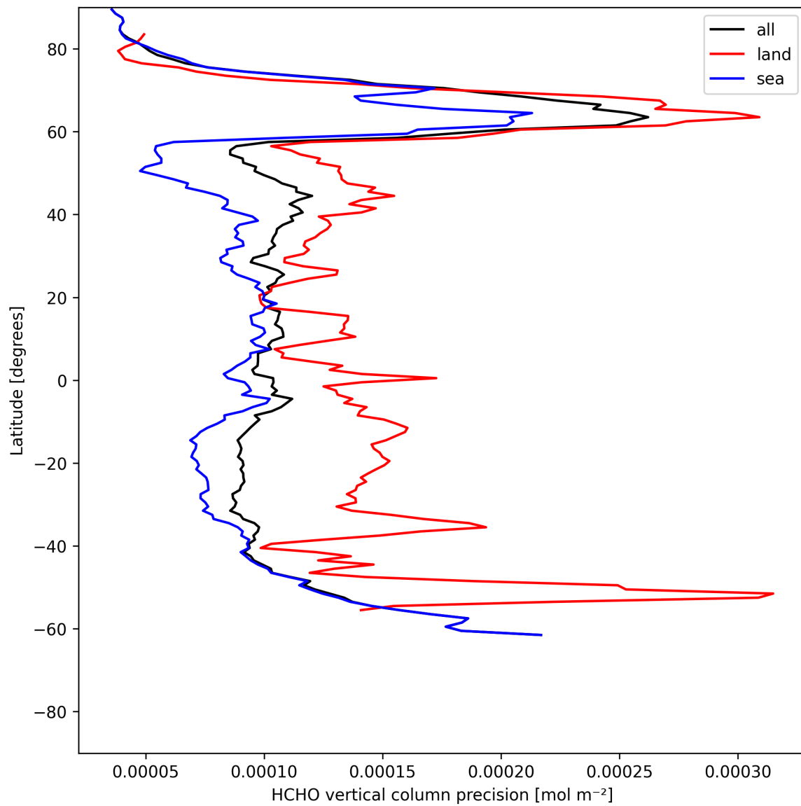
Figure 20: Zonal average of “HCHO vertical column precision” for 2025-07-05 to 2025-07-06.
