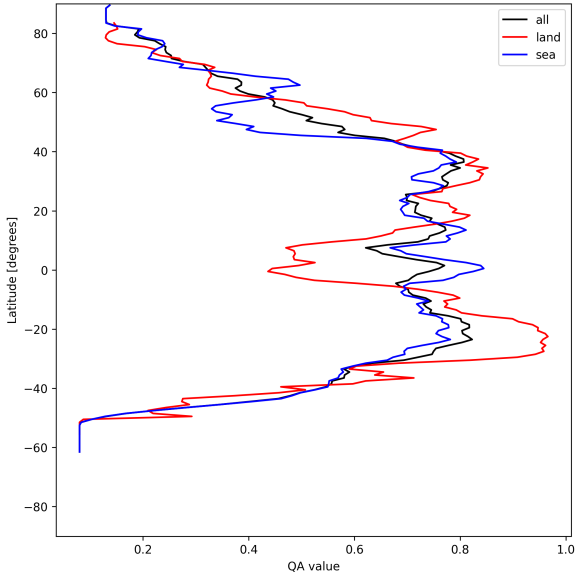
Figure 18: Zonal average of “QA value” for 2025-07-05 to 2025-07-06.
