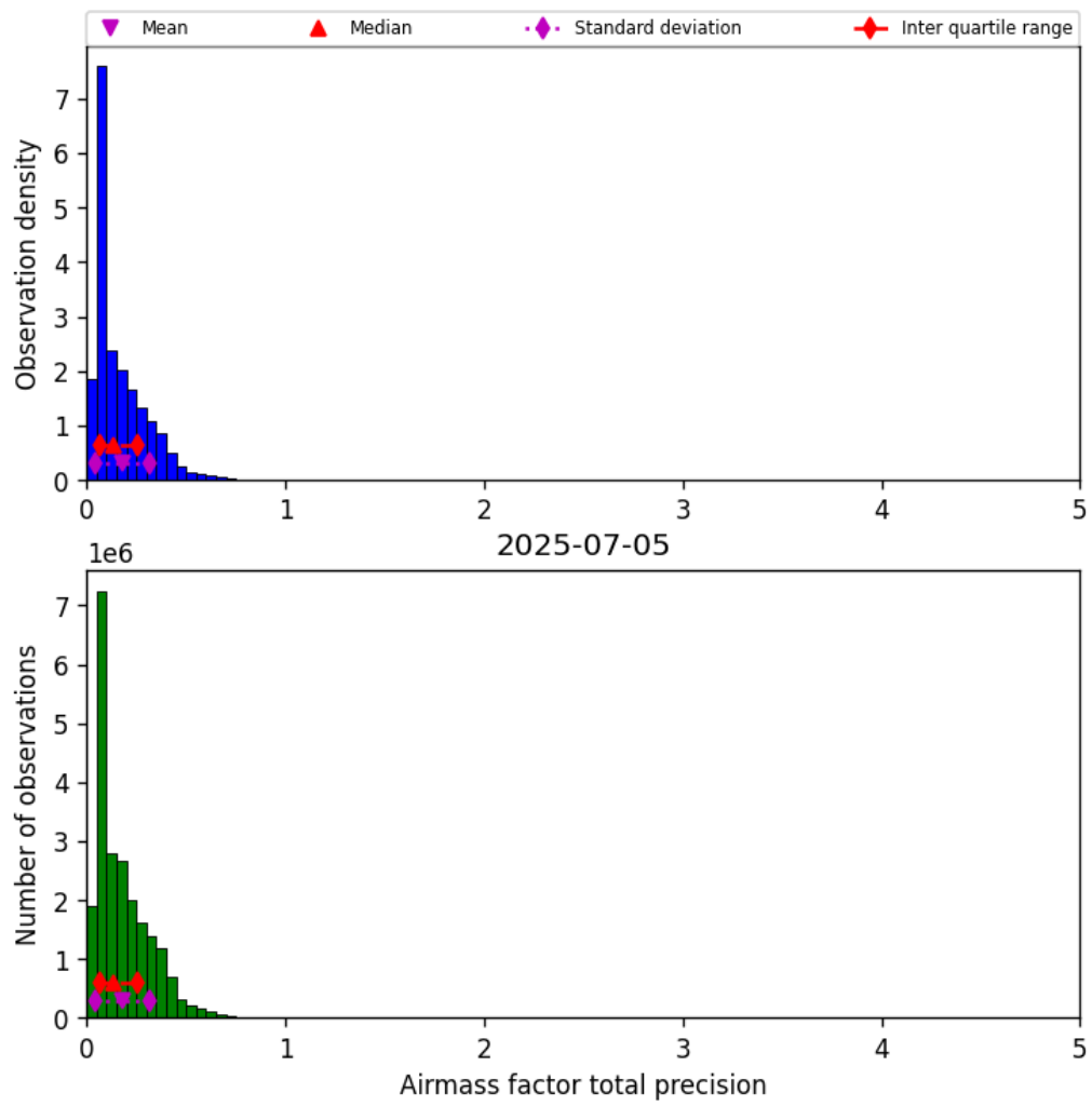
Figure 39: Histogram of “Airmass factor total precision” for 2025-07-05 to 2025-07-06
