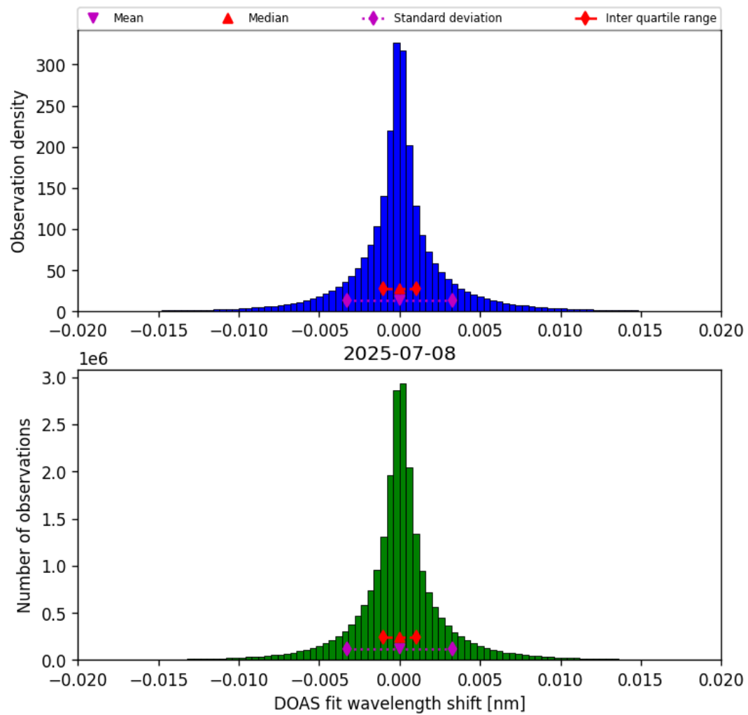
Figure 42: Histogram of “DOAS fit wavelength shift” for 2025-07-08 to 2025-07-09
