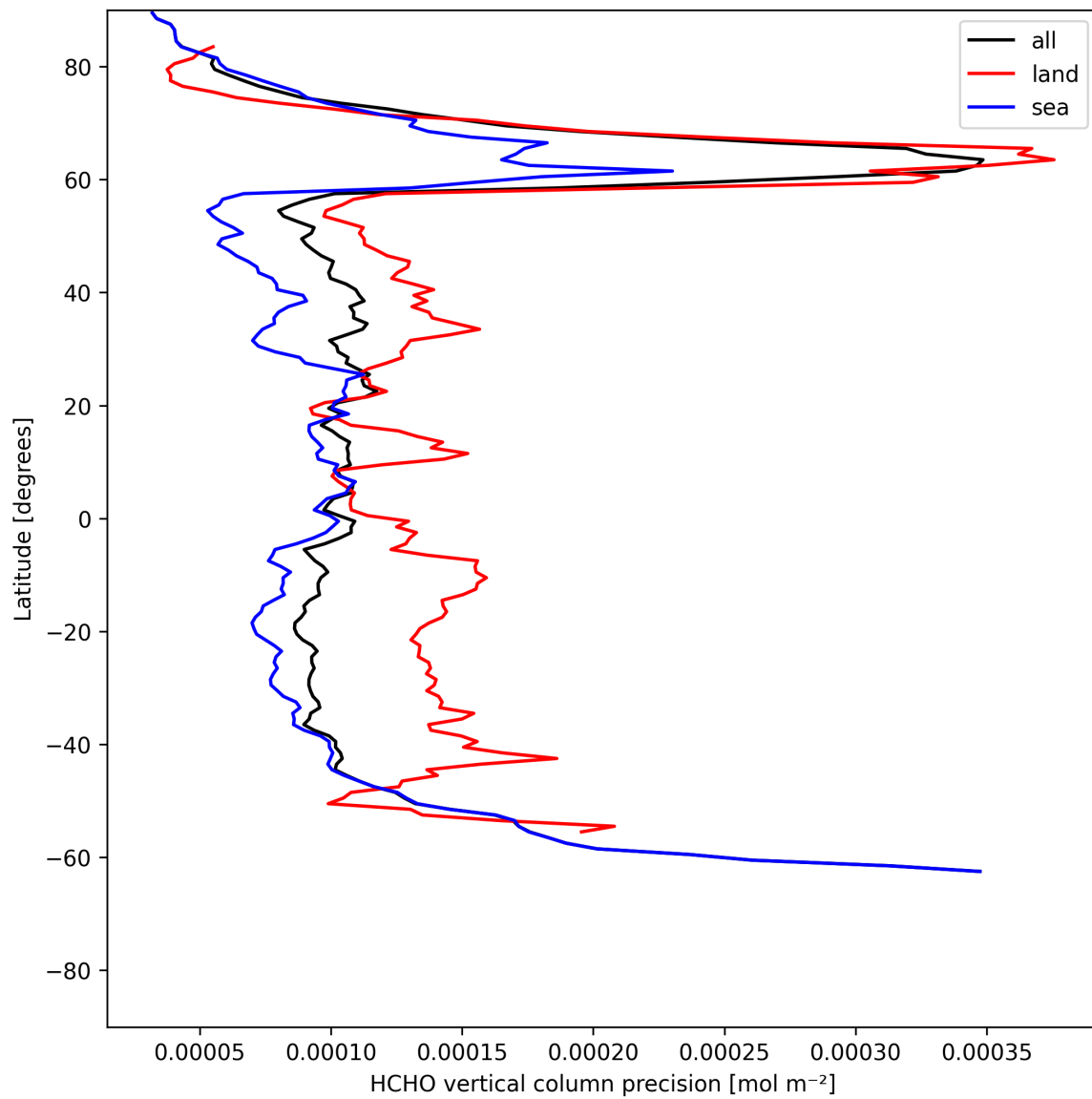
Figure 20: Zonal average of “HCHO vertical column precision” for 2025-07-08 to 2025-07-09.
