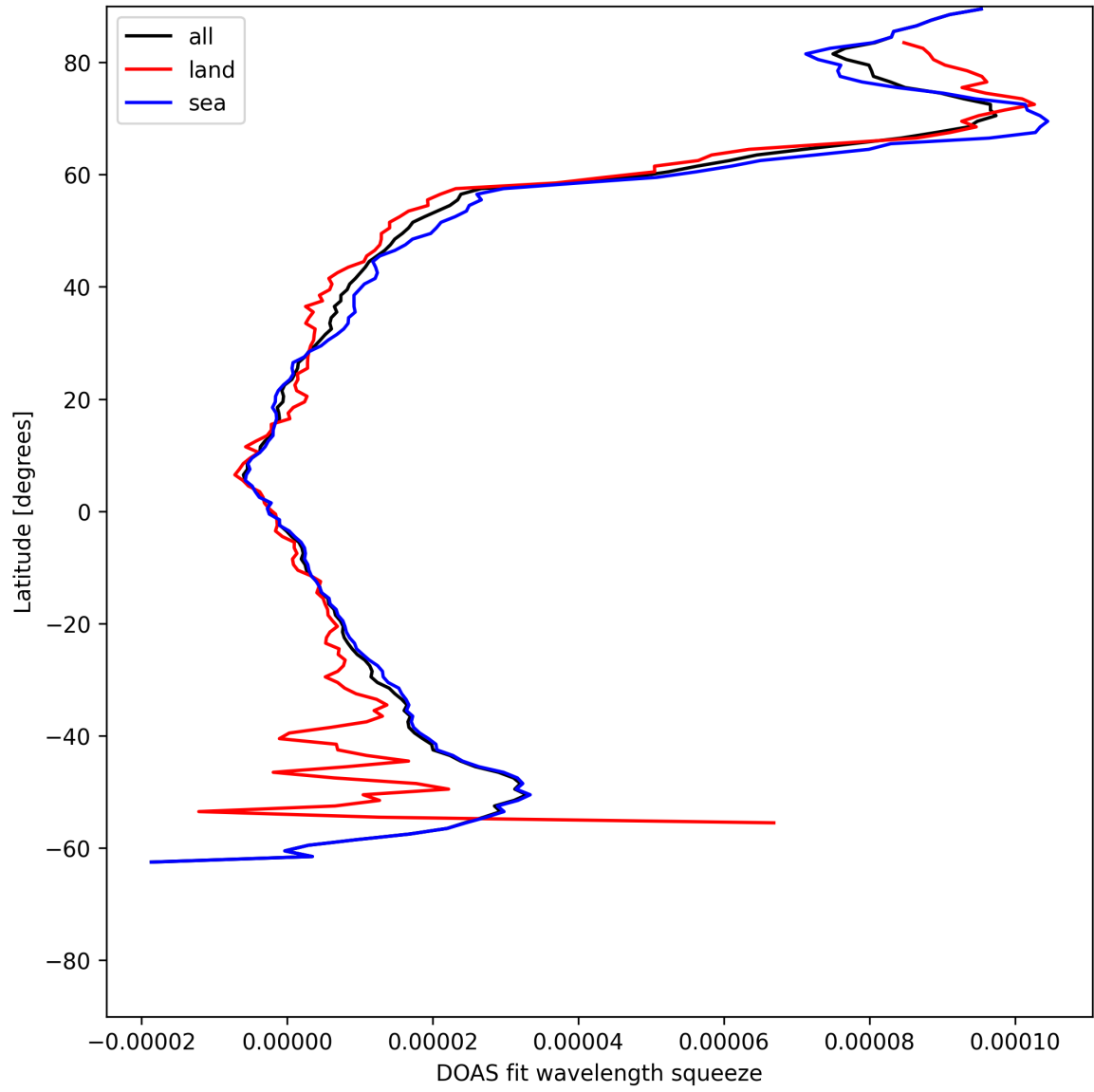
Figure 29: Zonal average of “DOAS fit wavelength squeeze” for 2025-07-08 to 2025-07-09.
