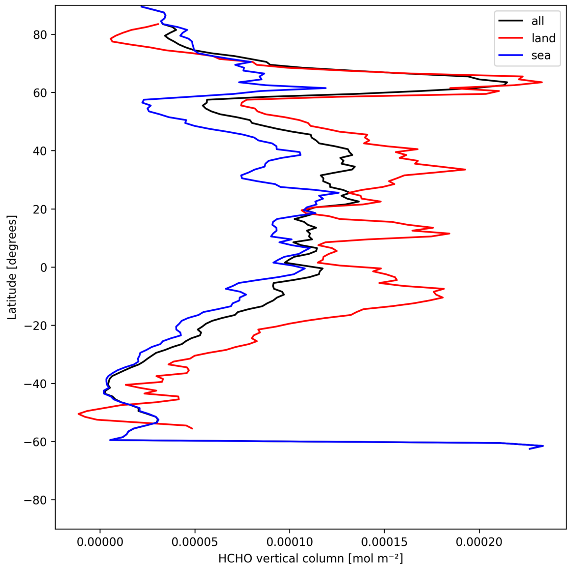
Figure 19: Zonal average of “HCHO vertical column” for 2025-07-08 to 2025-07-09.
