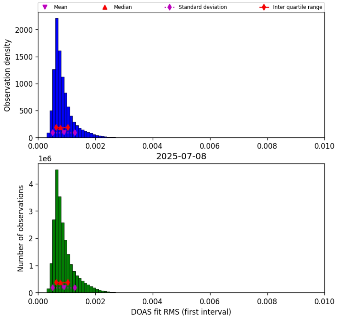
Figure 44: Histogram of “DOAS fit RMS (first interval)” for 2025-07-08 to 2025-07-09
