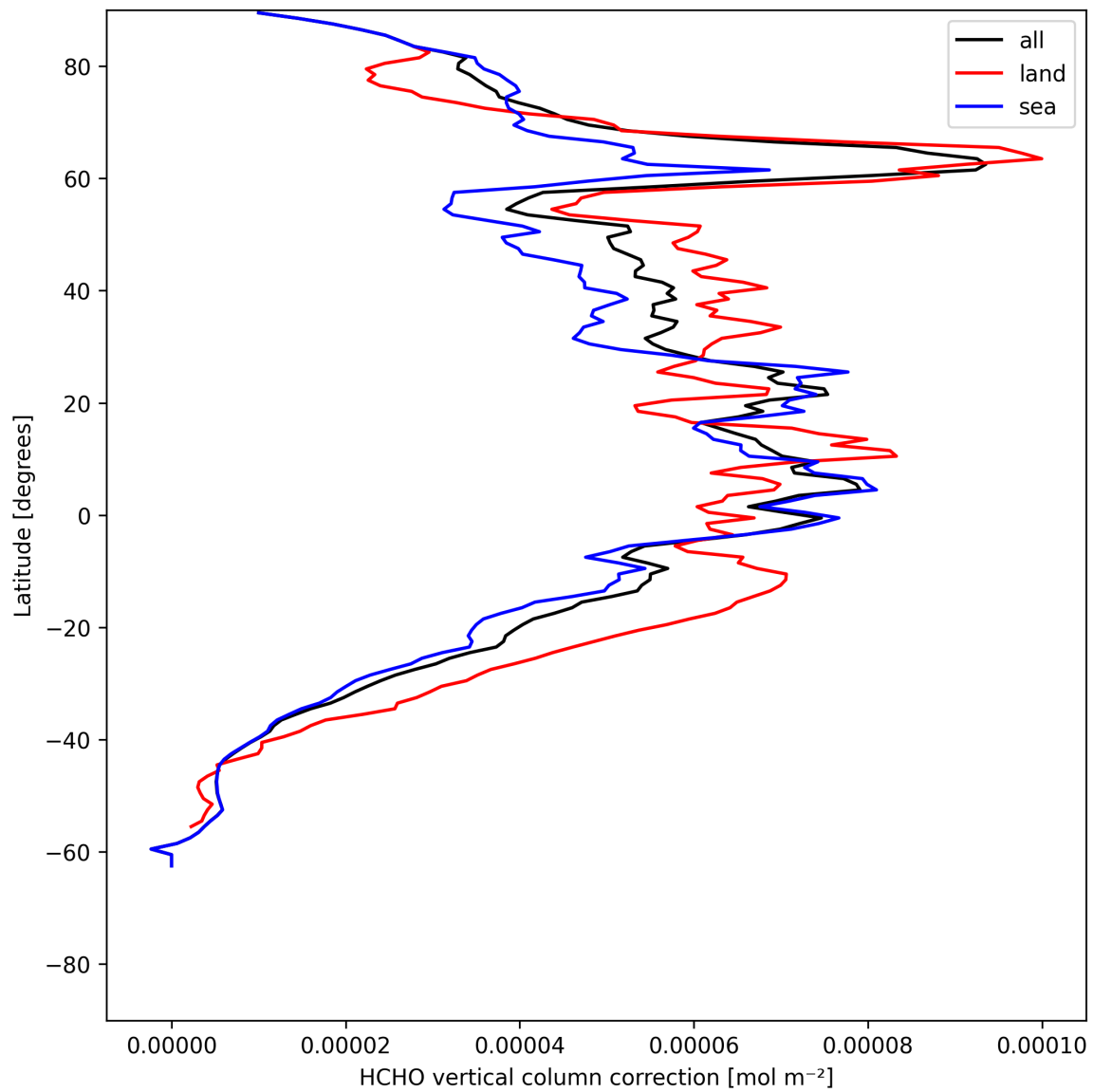
Figure 21: Zonal average of “HCHO vertical column correction” for 2025-07-08 to 2025-07-09.
