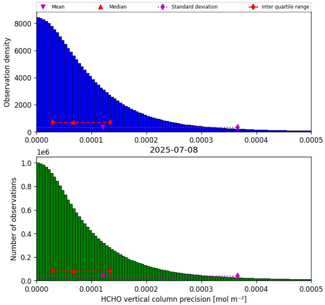
Figure 34: Histogram of “HCHO vertical column precision” for 2025-07-08 to 2025-07-09
