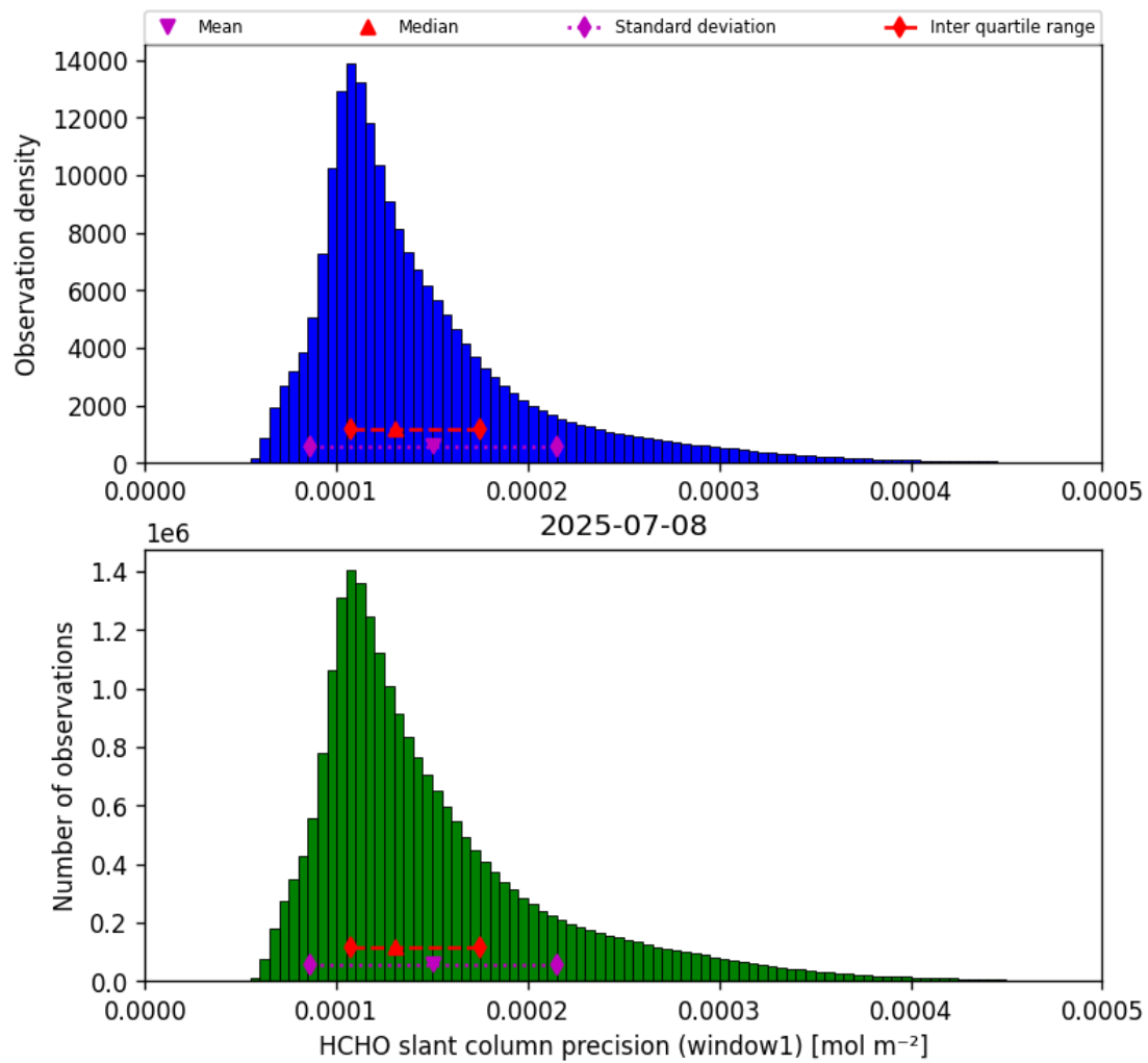
Figure 37: Histogram of “HCHO slant column precision (window1)” for 2025-07-08 to 2025-07-09
