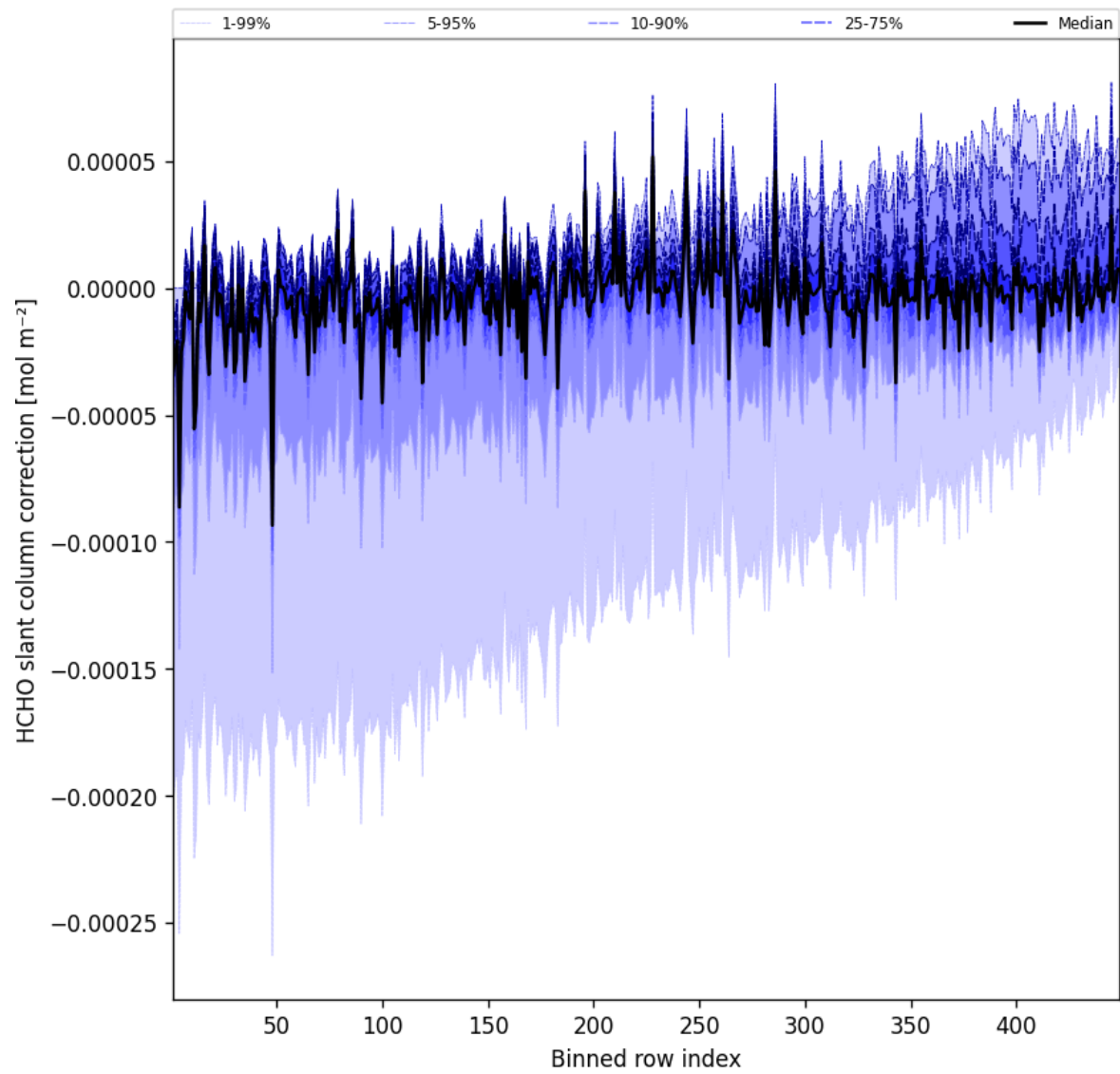
Figure 59: Along track statistics of “HCHO slant column correction” for 2025-07-08 to 2025-07-09
