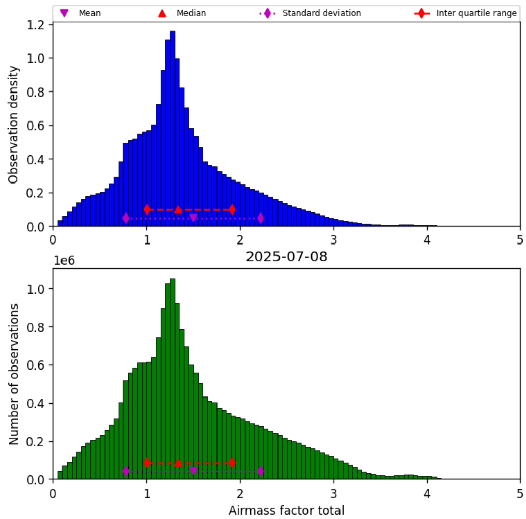
Figure 38: Histogram of “Airmass factor total” for 2025-07-08 to 2025-07-09
