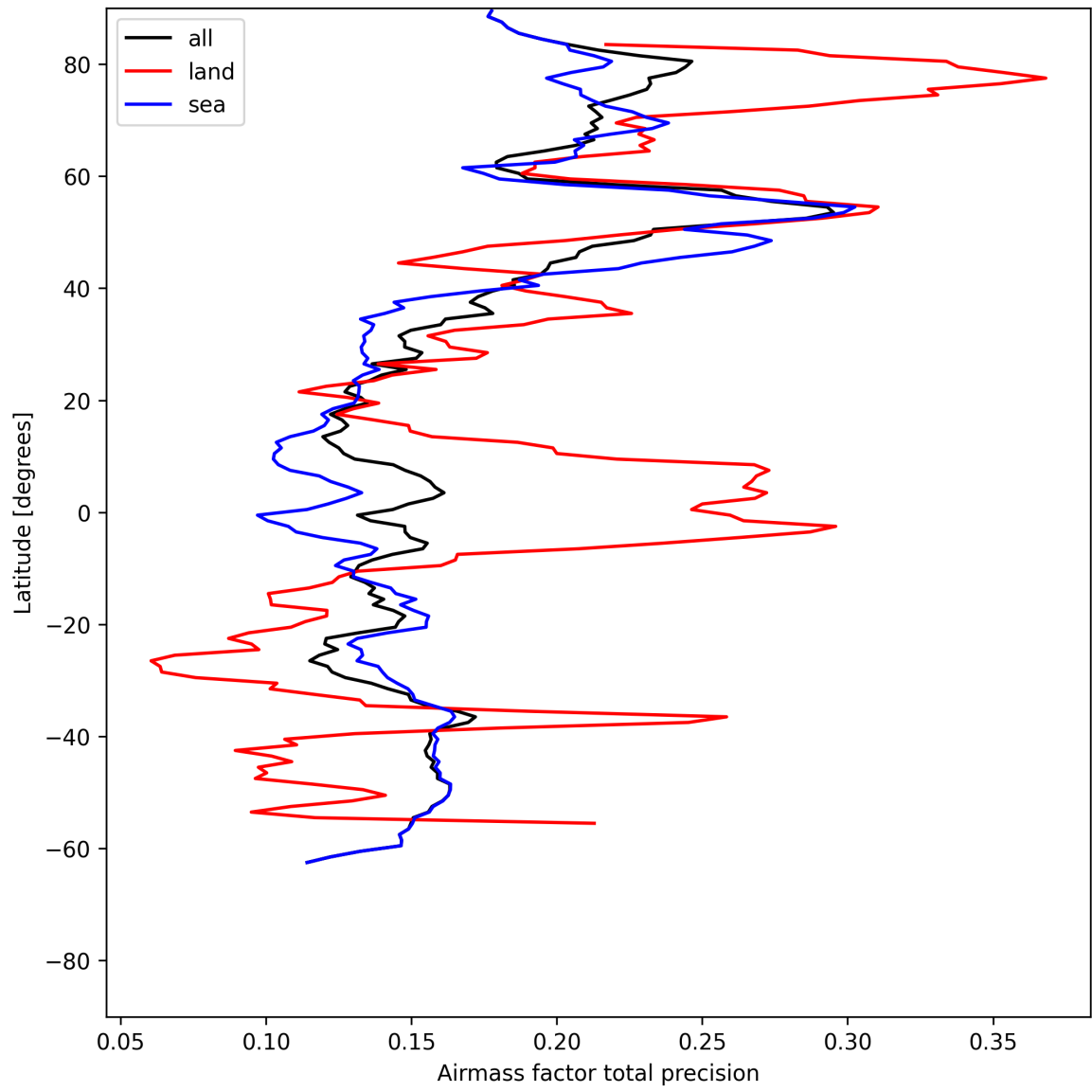
Figure 25: Zonal average of “Airmass factor total precision” for 2025-07-08 to 2025-07-09.
