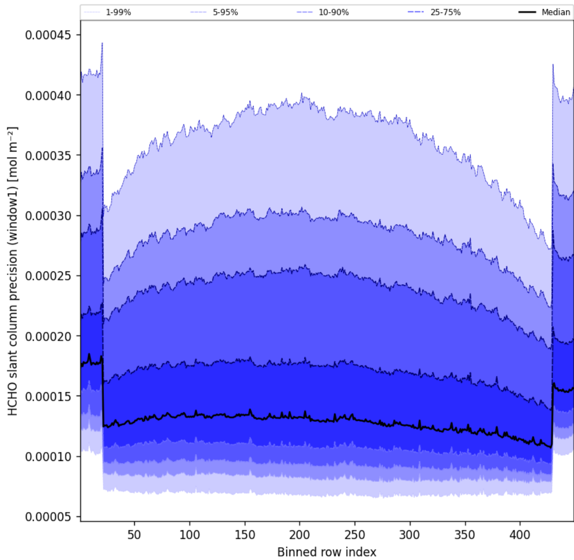
Figure 51: Along track statistics of “HCHO slant column precision (window1)” for 2025-07-08 to 2025-07-09
