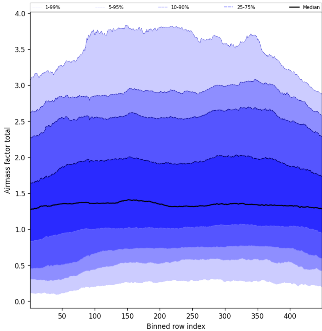
Figure 52: Along track statistics of “Airmass factor total” for 2025-07-08 to 2025-07-09
