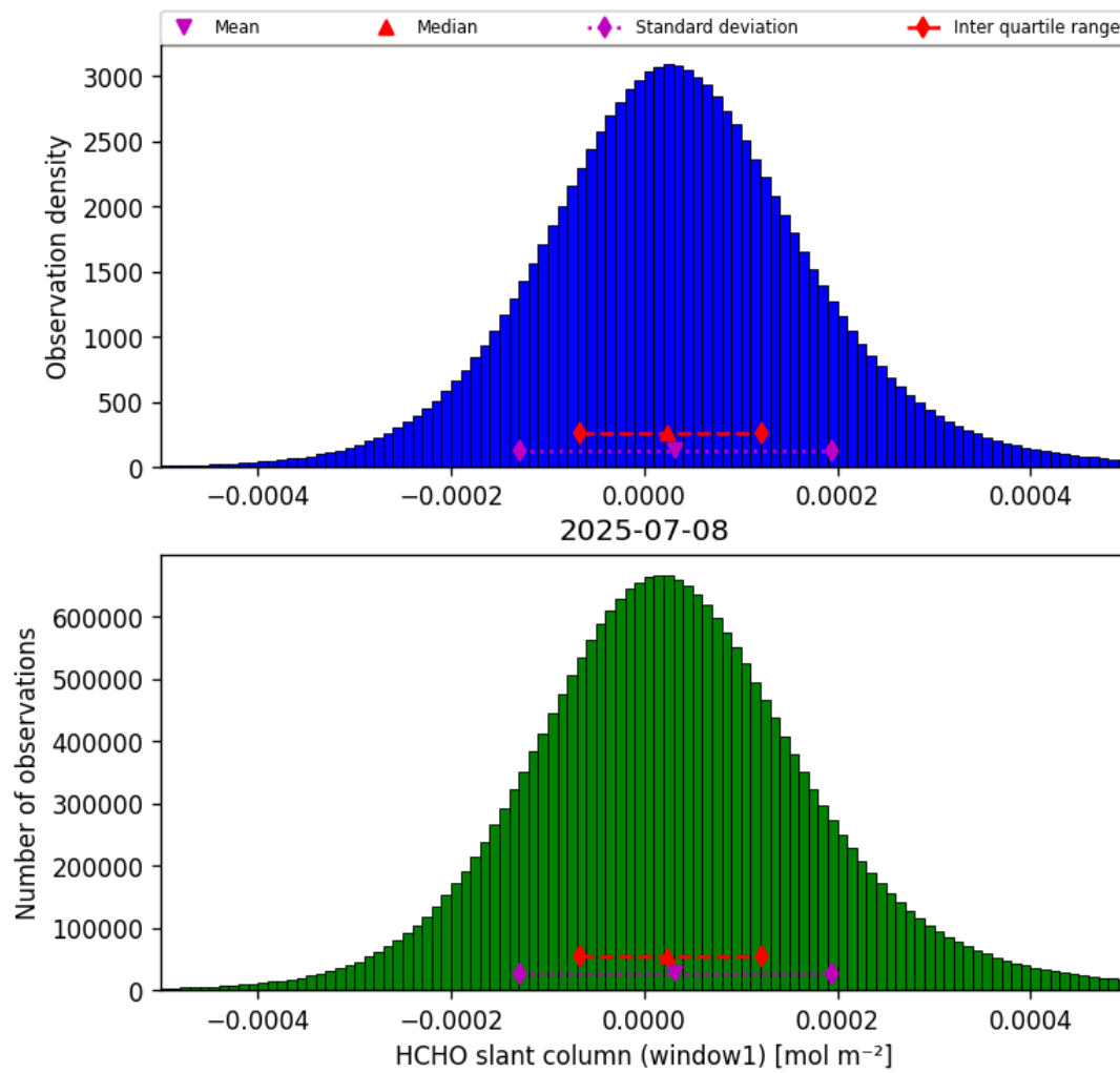
Figure 36: Histogram of “HCHO slant column (window1)” for 2025-07-08 to 2025-07-09
