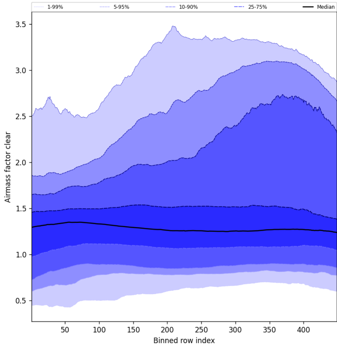
Figure 54: Along track statistics of “Airmass factor clear” for 2025-07-08 to 2025-07-09
