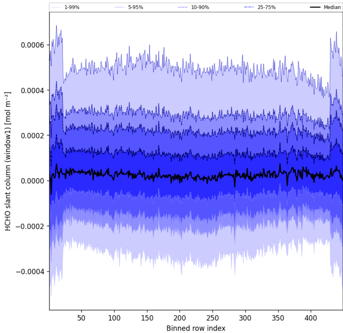
Figure 50: Along track statistics of “HCHO slant column (window1)” for 2025-07-08 to 2025-07-09
