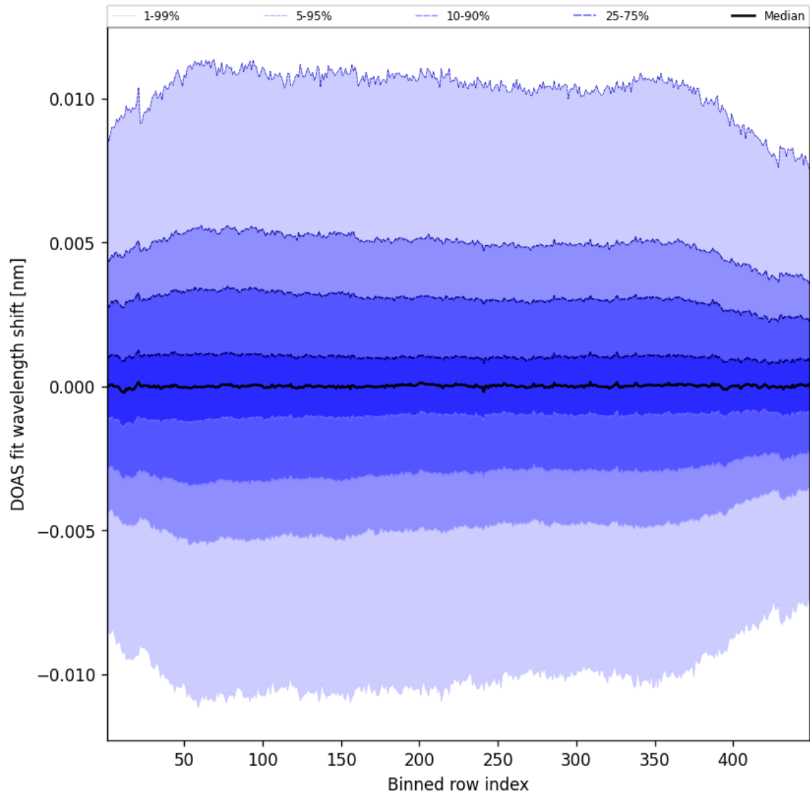
Figure 56: Along track statistics of “DOAS fit wavelength shift” for 2025-07-08 to 2025-07-09
