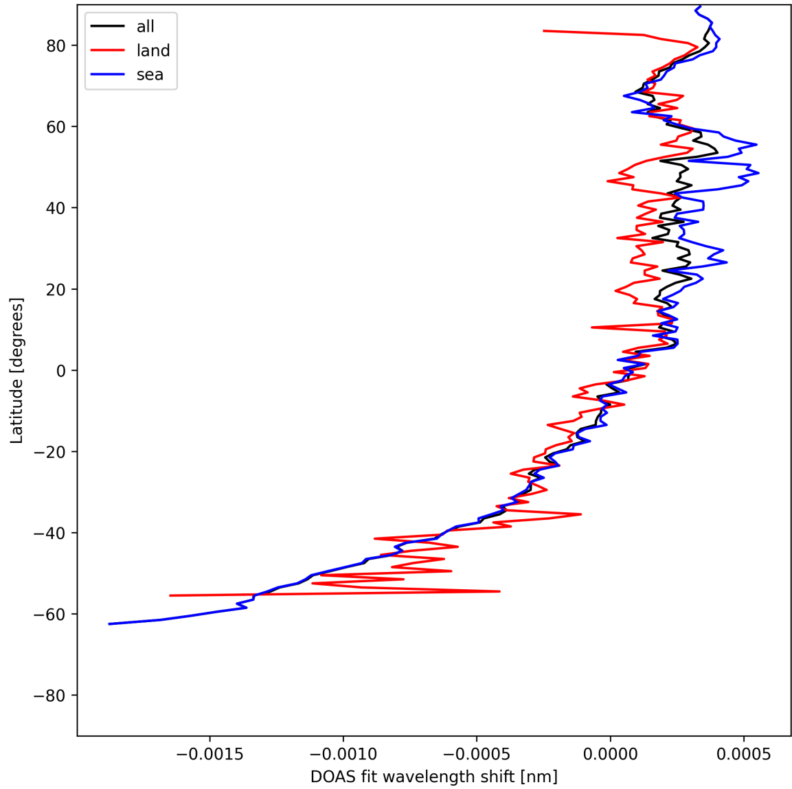
Figure 28: Zonal average of “DOAS fit wavelength shift” for 2025-07-08 to 2025-07-09.
