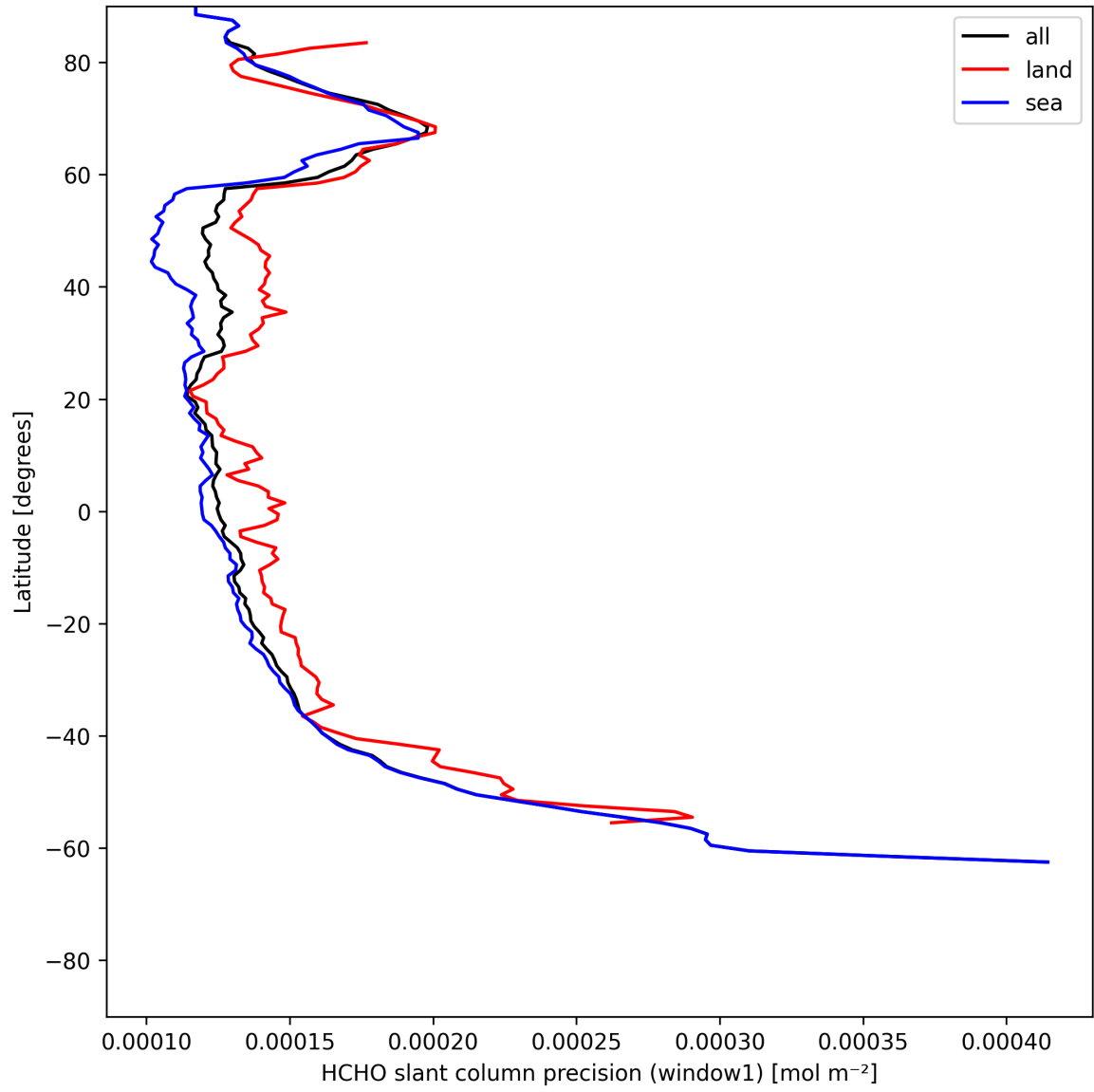
Figure 23: Zonal average of "HCHO slant column precision (window1)" for 2025-07-08 to 2025-07-09.
