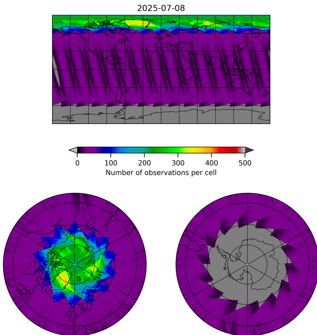
Figure 17: Map of the number of observations for 2025-07-08 to 2025-07-09
