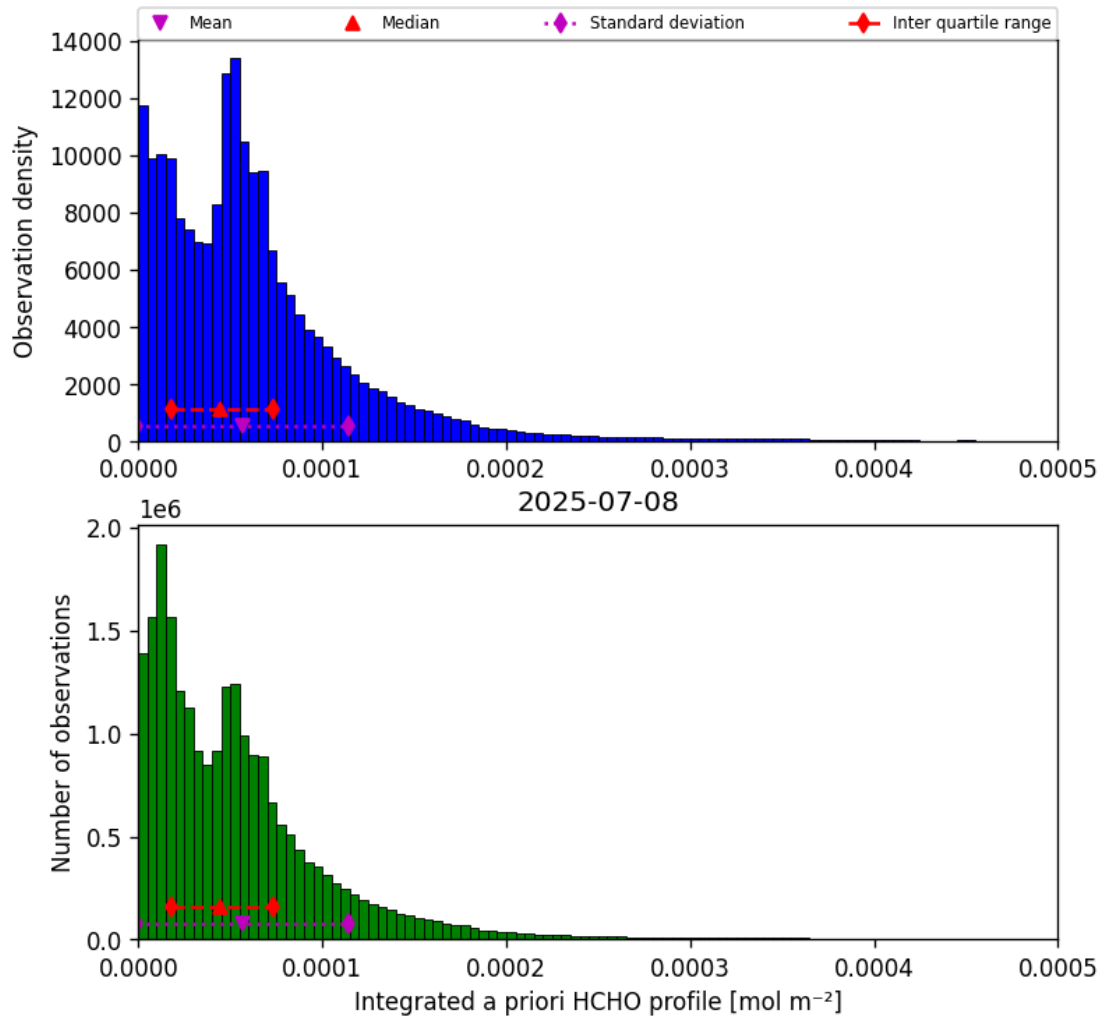
Figure 41: Histogram of “Integrated a priori HCHO profile” for 2025-07-08 to 2025-07-09
