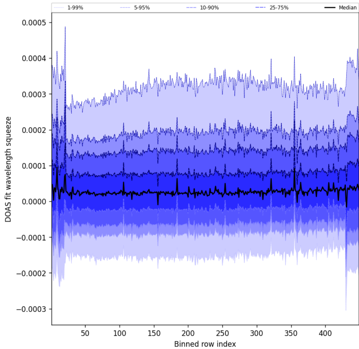
Figure 57: Along track statistics of “DOAS fit wavelength squeeze” for 2025-07-08 to 2025-07-09
