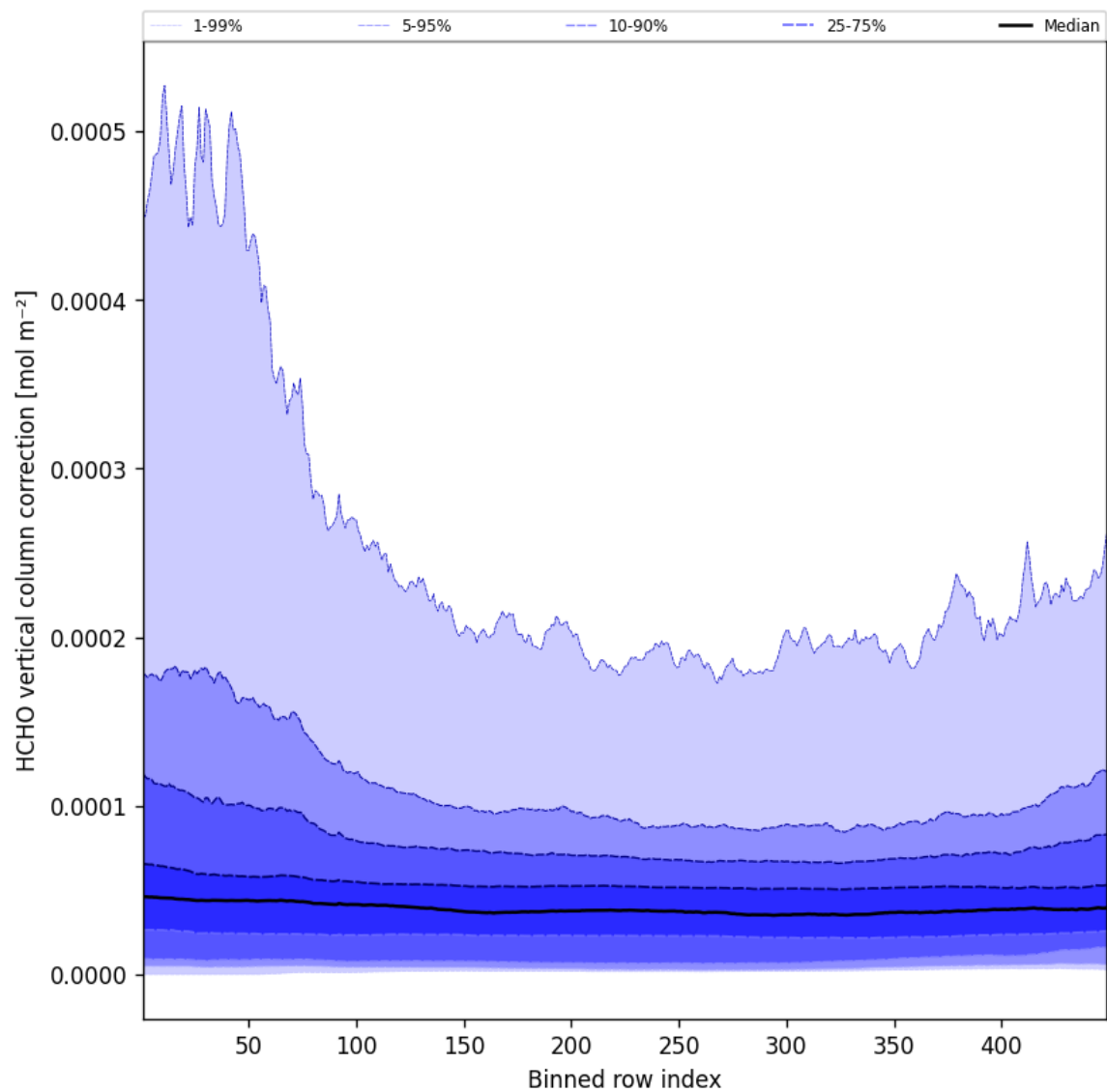
Figure 49: Along track statistics of “HCHO vertical column correction” for 2025-07-08 to 2025-07-09
