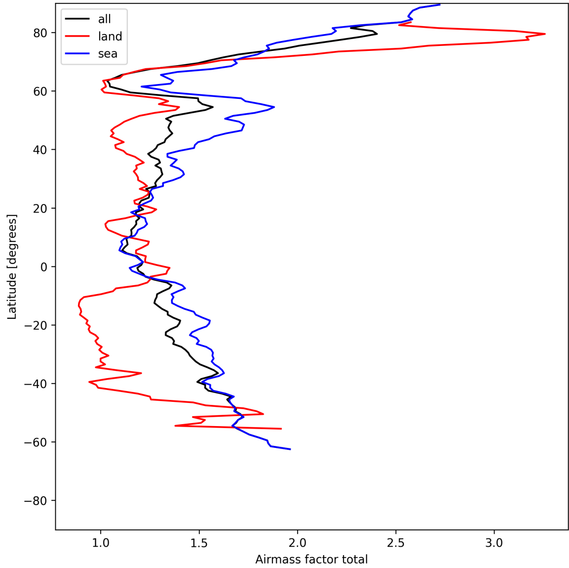
Figure 24: Zonal average of “Airmass factor total” for 2025-07-08 to 2025-07-09.
