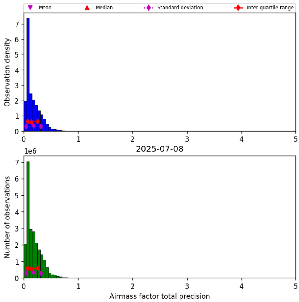
Figure 39: Histogram of “Airmass factor total precision” for 2025-07-08 to 2025-07-09
