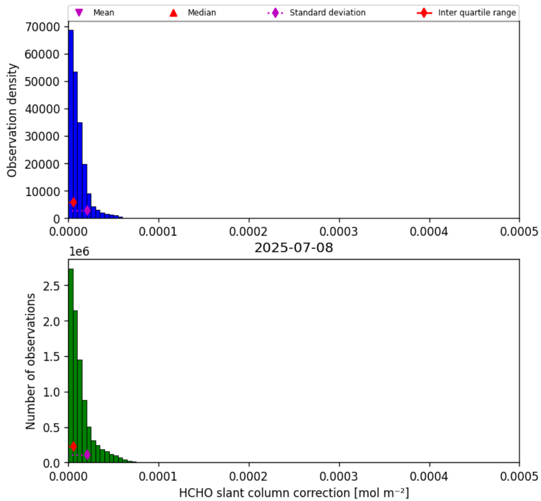
Figure 45: Histogram of “HCHO slant column correction” for 2025-07-08 to 2025-07-09
