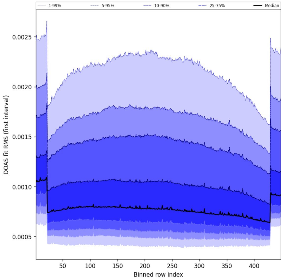
Figure 58: Along track statistics of “DOAS fit RMS (first interval)” for 2025-07-08 to 2025-07-09
