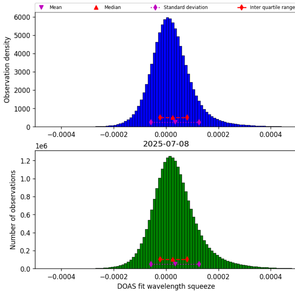
Figure 43: Histogram of “DOAS fit wavelength squeeze” for 2025-07-08 to 2025-07-09
