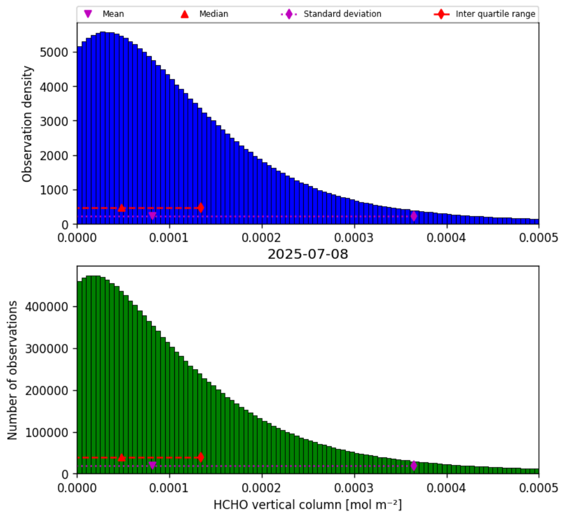
Figure 33: Histogram of “HCHO vertical column” for 2025-07-08 to 2025-07-09
