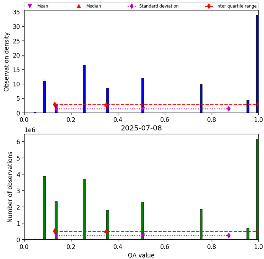
Figure 32: Histogram of “QA value” for 2025-07-08 to 2025-07-09
