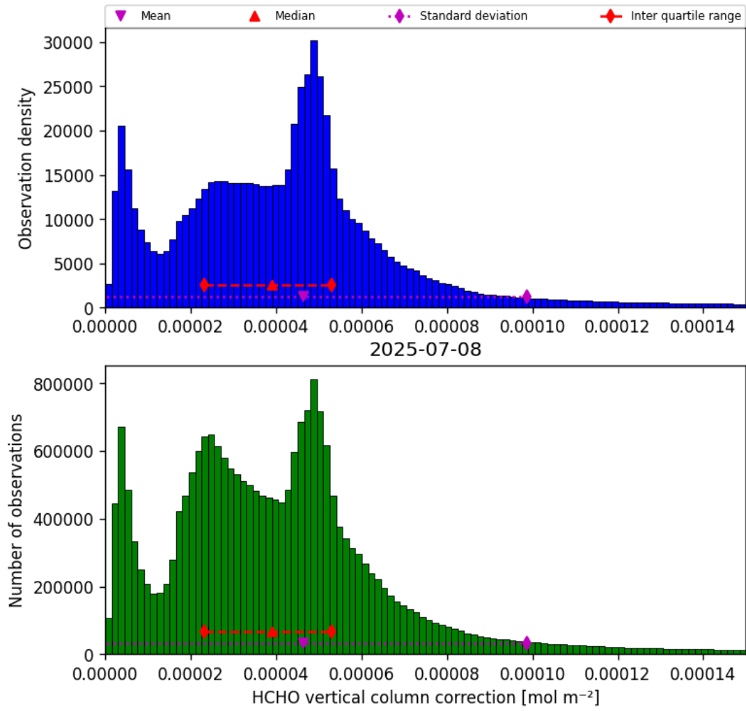
Figure 35: Histogram of “HCHO vertical column correction” for 2025-07-08 to 2025-07-09
