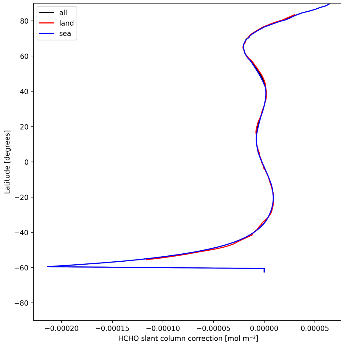
Figure 31: Zonal average of “HCHO slant column correction” for 2025-07-08 to 2025-07-09.
