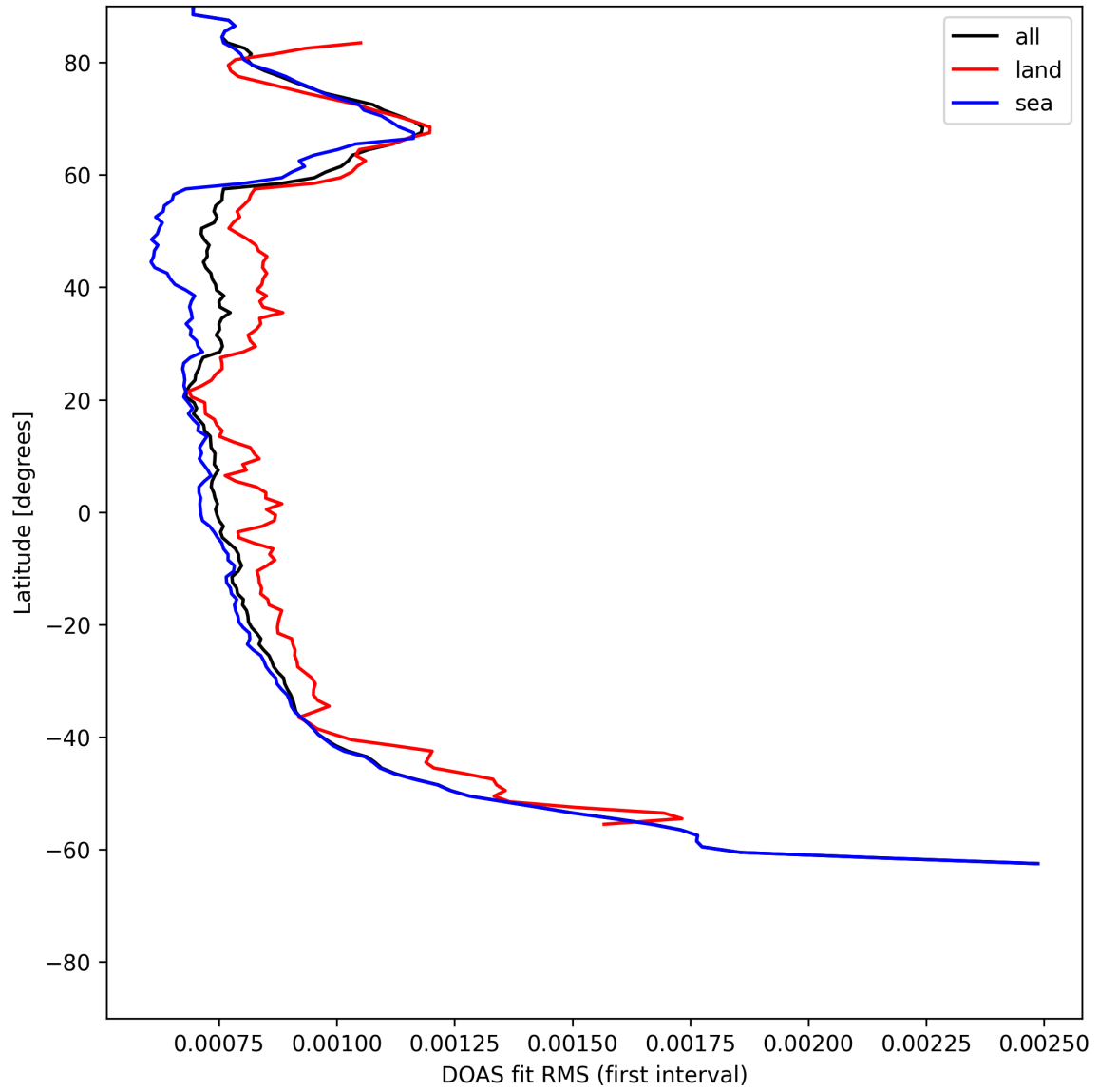
Figure 30: Zonal average of “DOAS fit RMS (first interval)” for 2025-07-08 to 2025-07-09.
