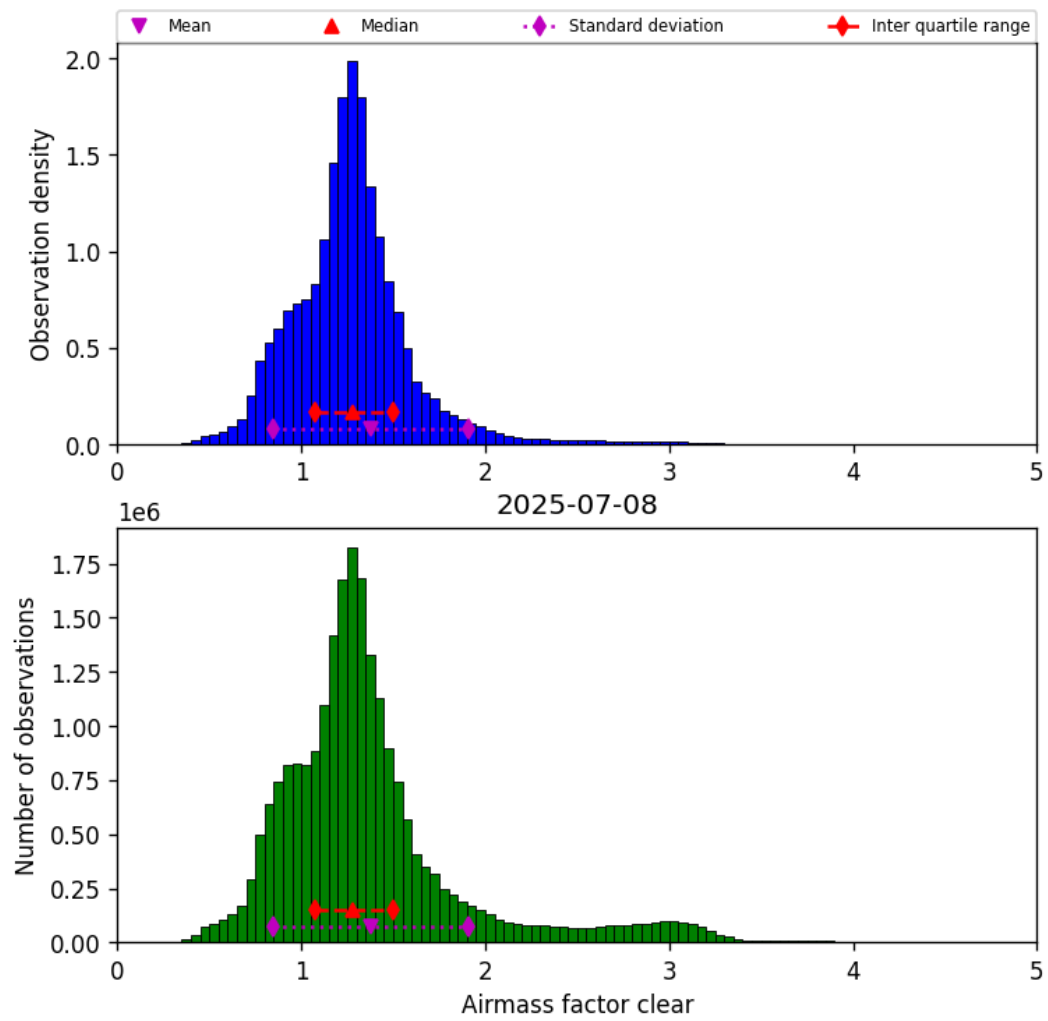
Figure 40: Histogram of “Airmass factor clear” for 2025-07-08 to 2025-07-09
