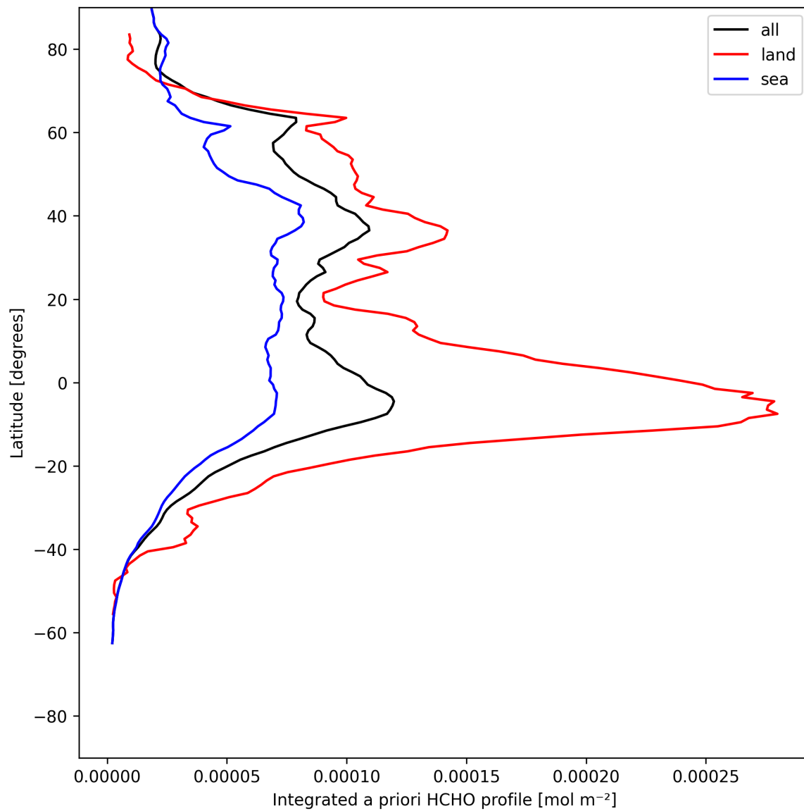
Figure 27: Zonal average of “Integrated a priori HCHO profile” for 2025-07-08 to 2025-07-09.
