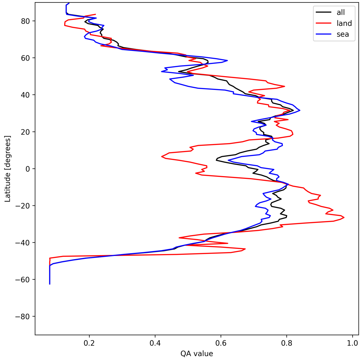
Figure 18: Zonal average of “QA value” for 2025-07-08 to 2025-07-09.
