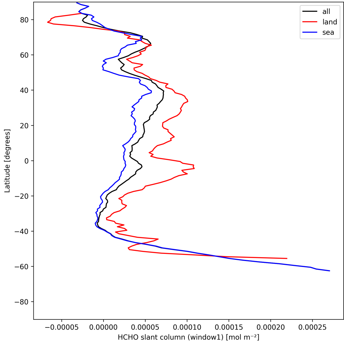
Figure 22: Zonal average of “HCHO slant column (window1)” for 2025-07-08 to 2025-07-09.
