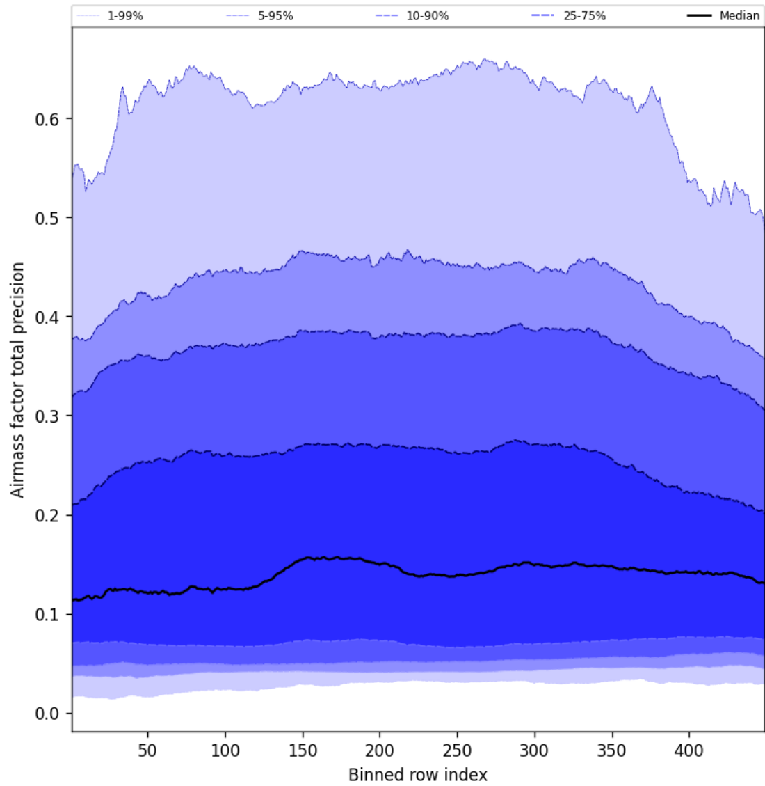
Figure 53: Along track statistics of “Airmass factor total precision” for 2025-07-08 to 2025-07-09
