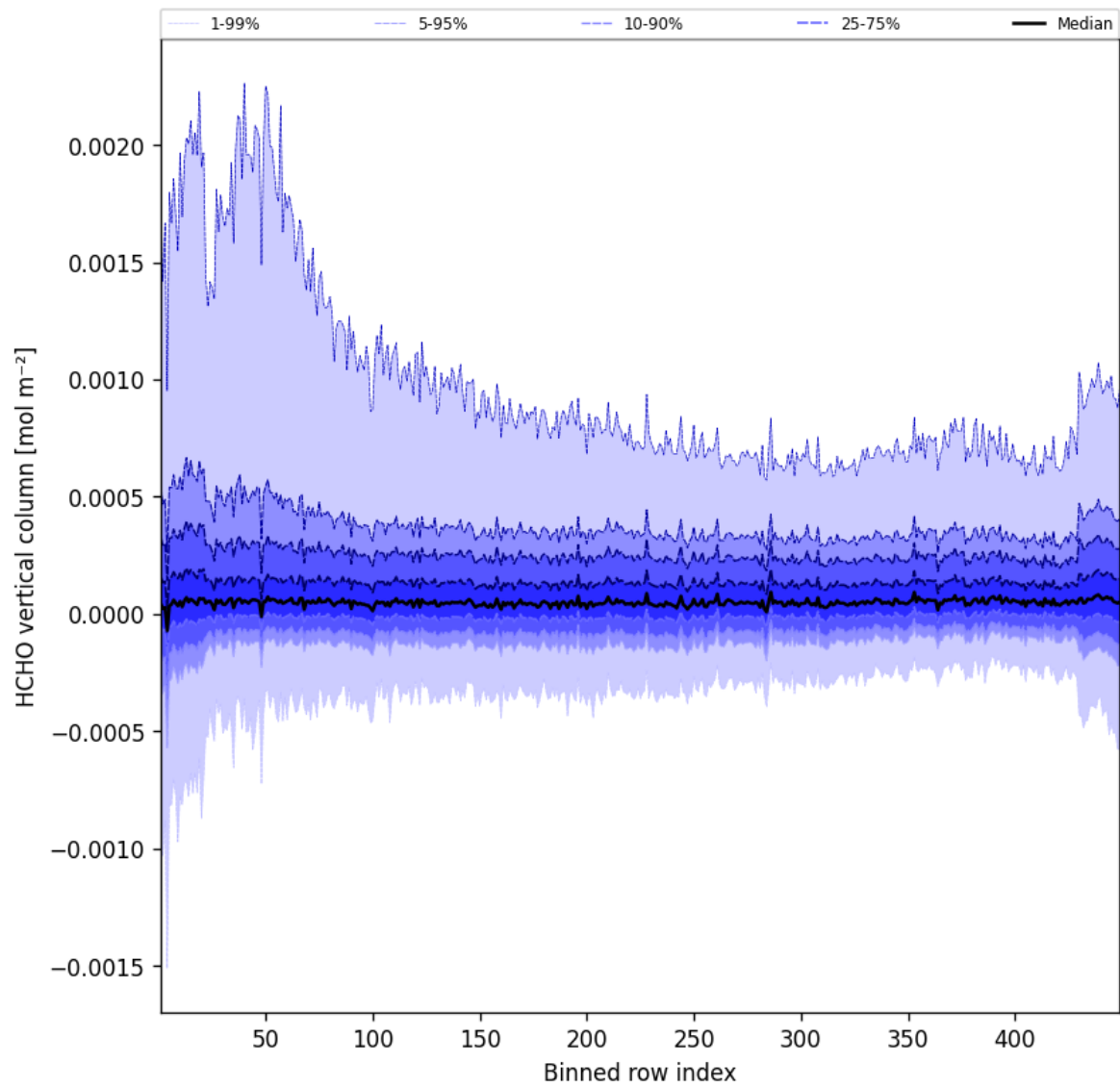
Figure 47: Along track statistics of “HCHO vertical column” for 2025-07-08 to 2025-07-09
