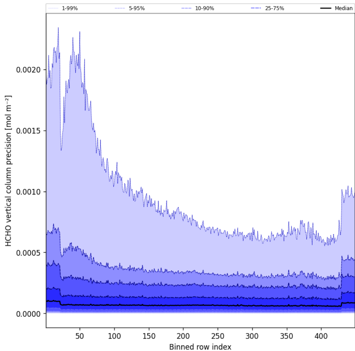
Figure 48: Along track statistics of “HCHO vertical column precision” for 2025-07-08 to 2025-07-09
