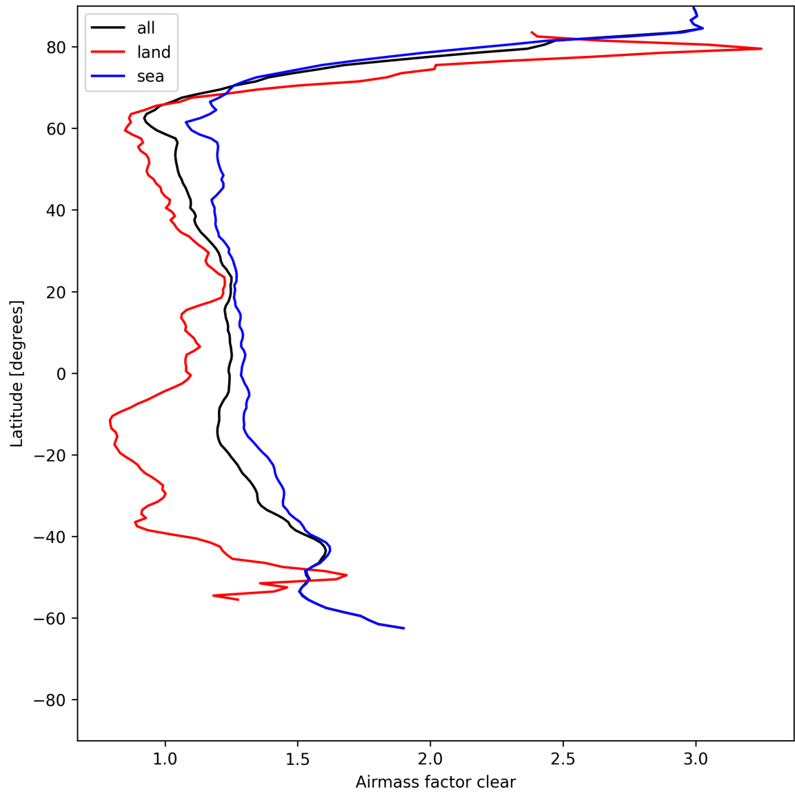
Figure 26: Zonal average of “Airmass factor clear” for 2025-07-08 to 2025-07-09.
