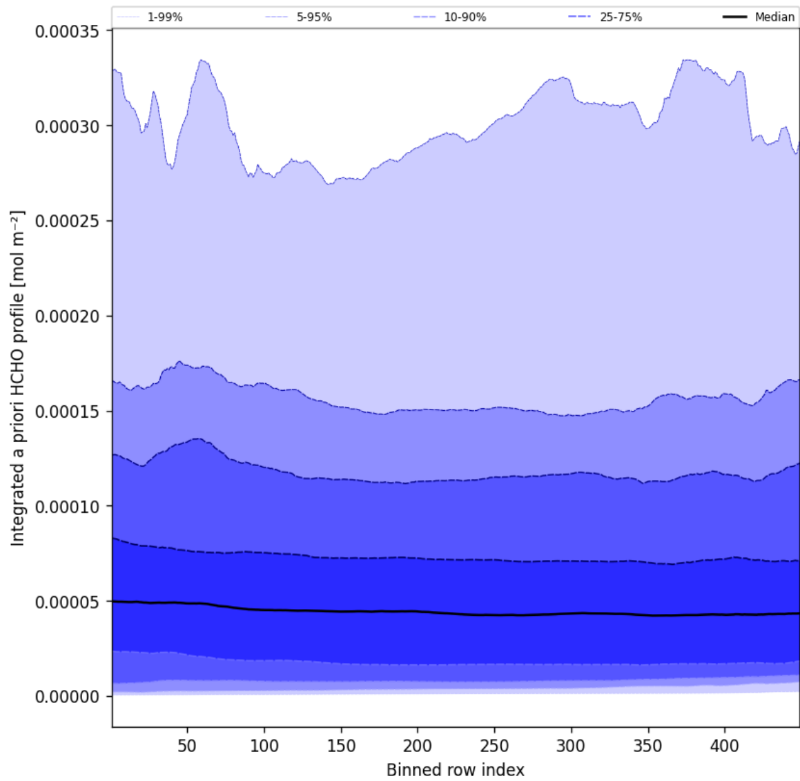
Figure 55: Along track statistics of “Integrated a priori HCHO profile” for 2025-07-08 to 2025-07-09
