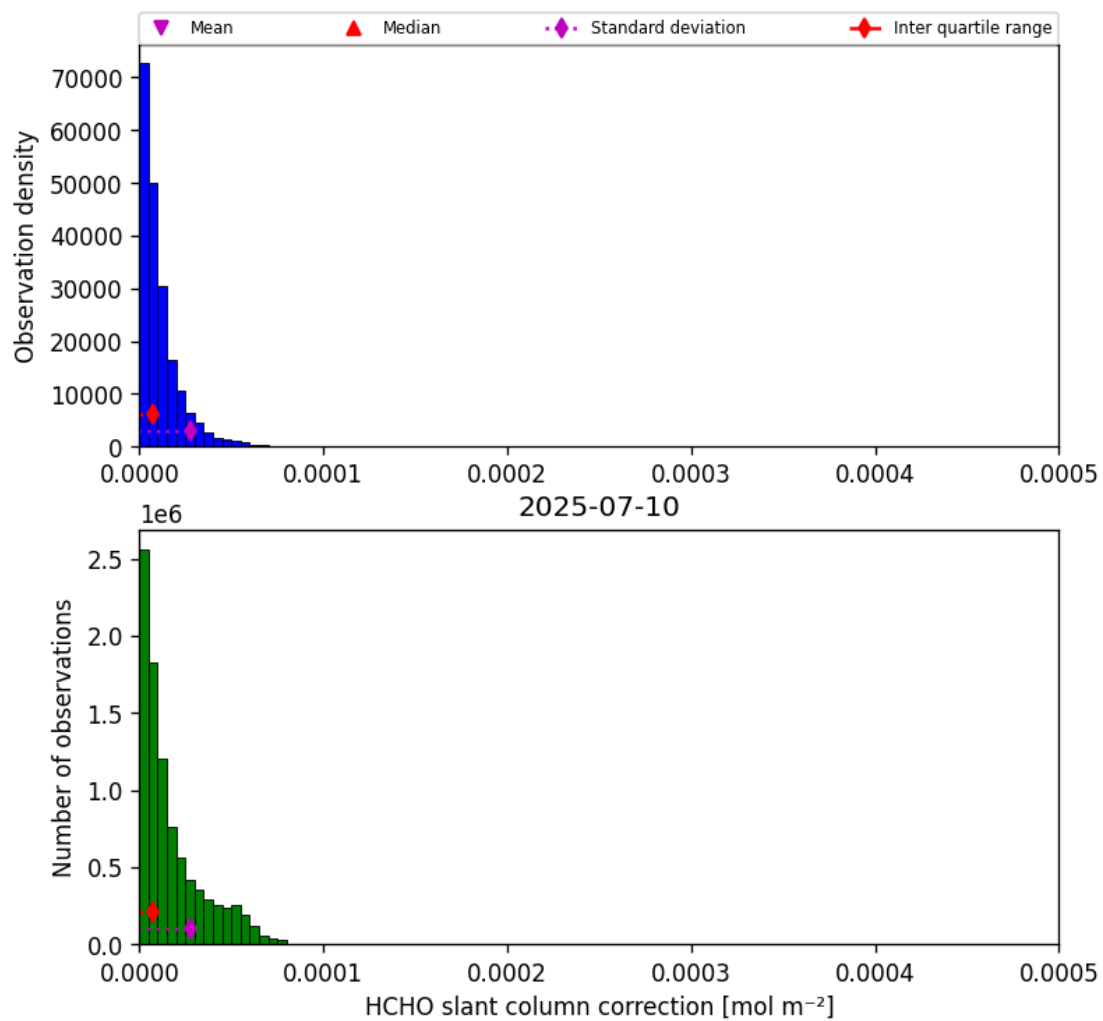
Figure 45: Histogram of “HCHO slant column correction” for 2025-07-10 to 2025-07-11
