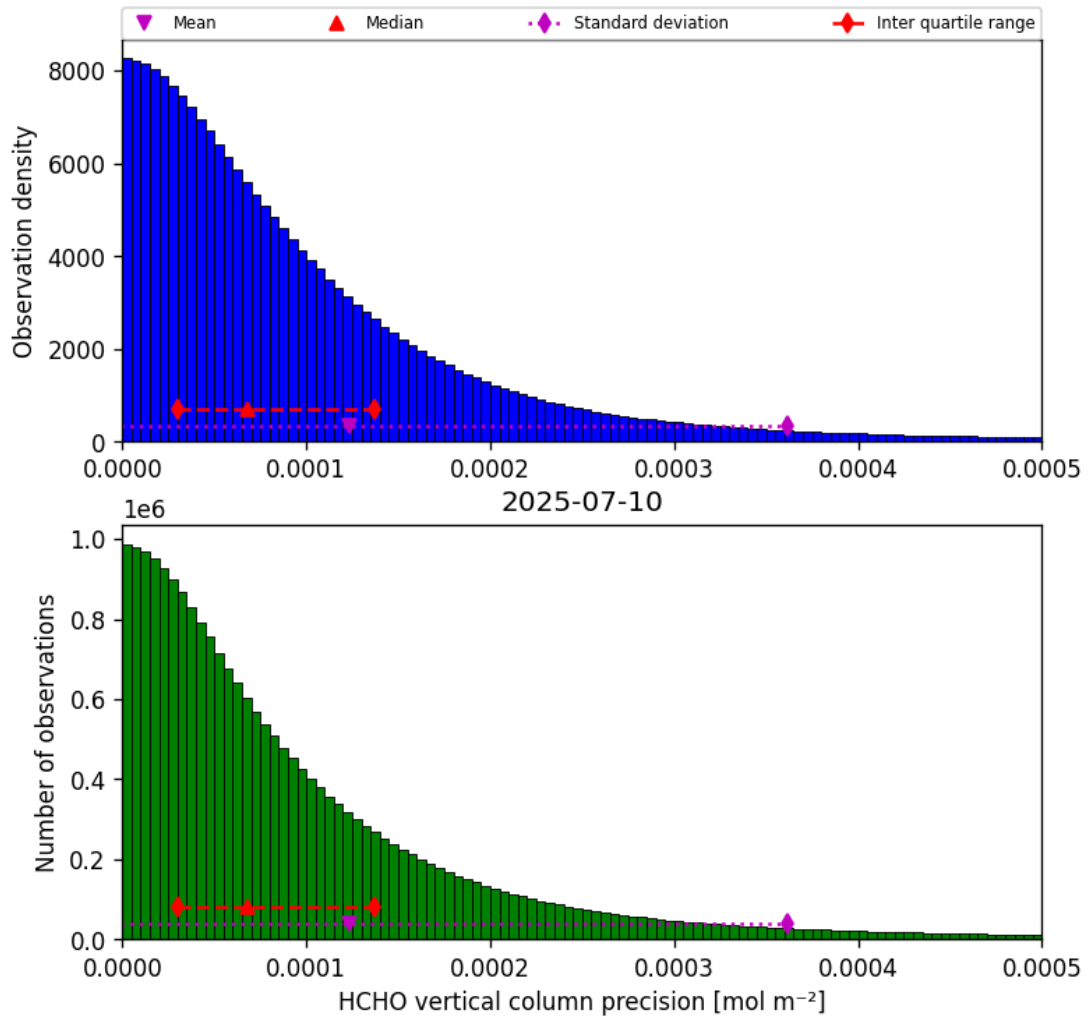
Figure 34: Histogram of “HCHO vertical column precision” for 2025-07-10 to 2025-07-11
