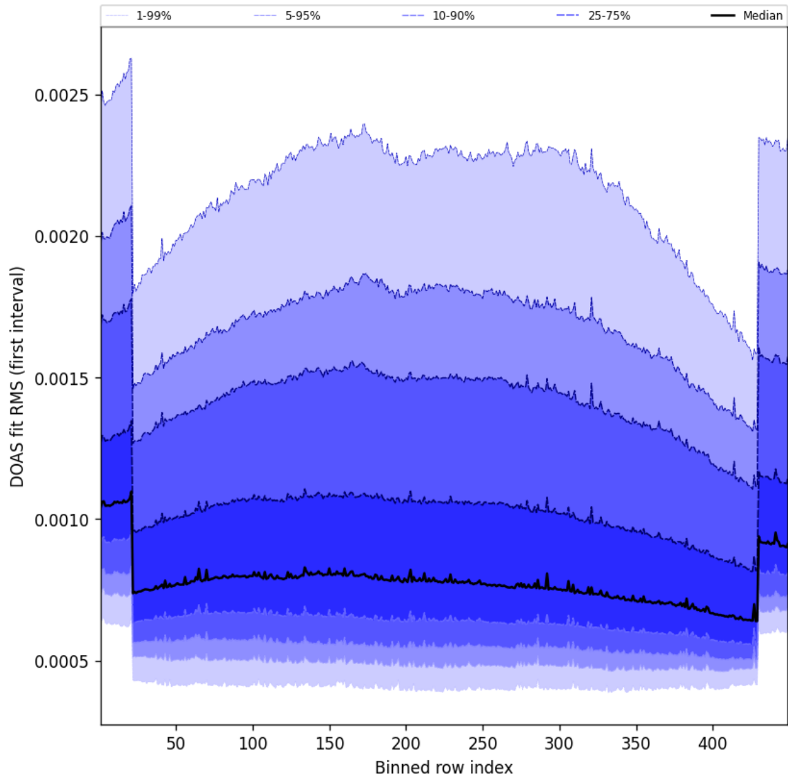
Figure 58: Along track statistics of “DOAS fit RMS (first interval)” for 2025-07-10 to 2025-07-11
