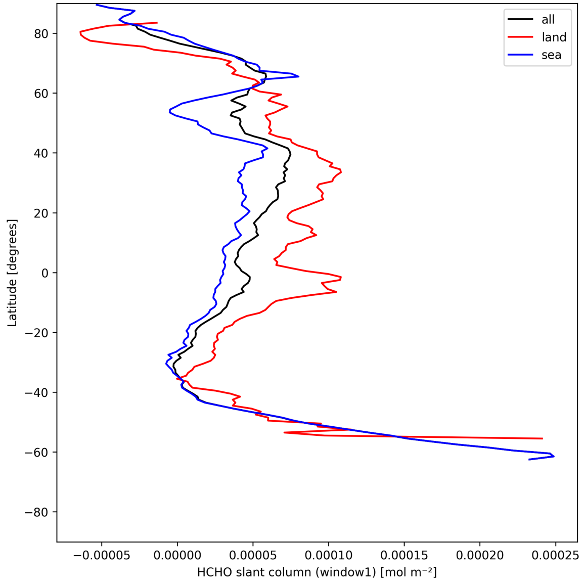
Figure 22: Zonal average of “HCHO slant column (window1)” for 2025-07-10 to 2025-07-11.
