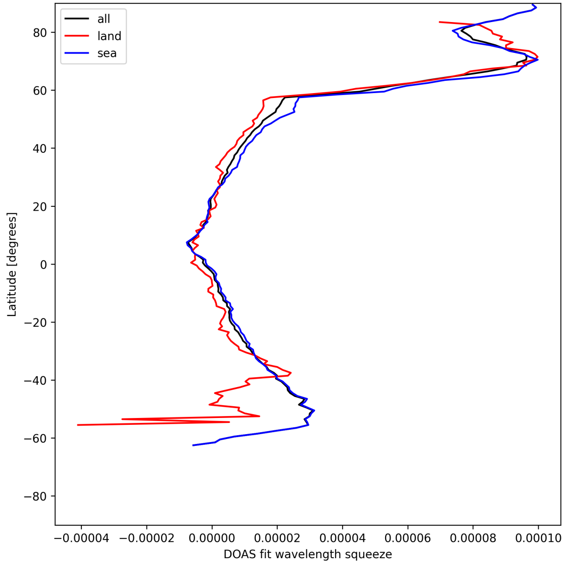
Figure 29: Zonal average of “DOAS fit wavelength squeeze” for 2025-07-10 to 2025-07-11.
