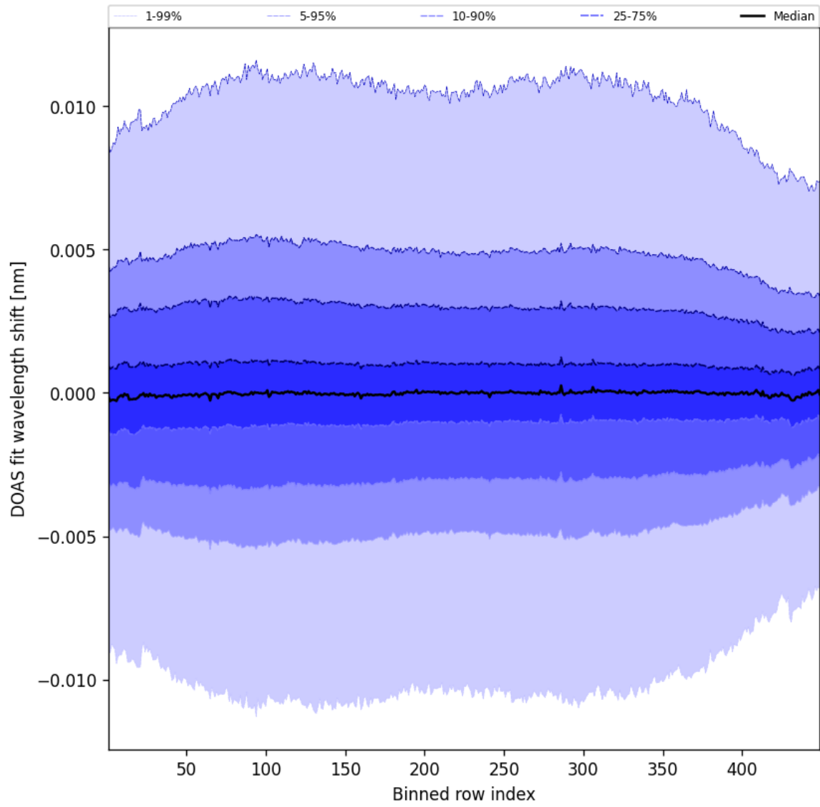
Figure 56: Along track statistics of “DOAS fit wavelength shift” for 2025-07-10 to 2025-07-11
