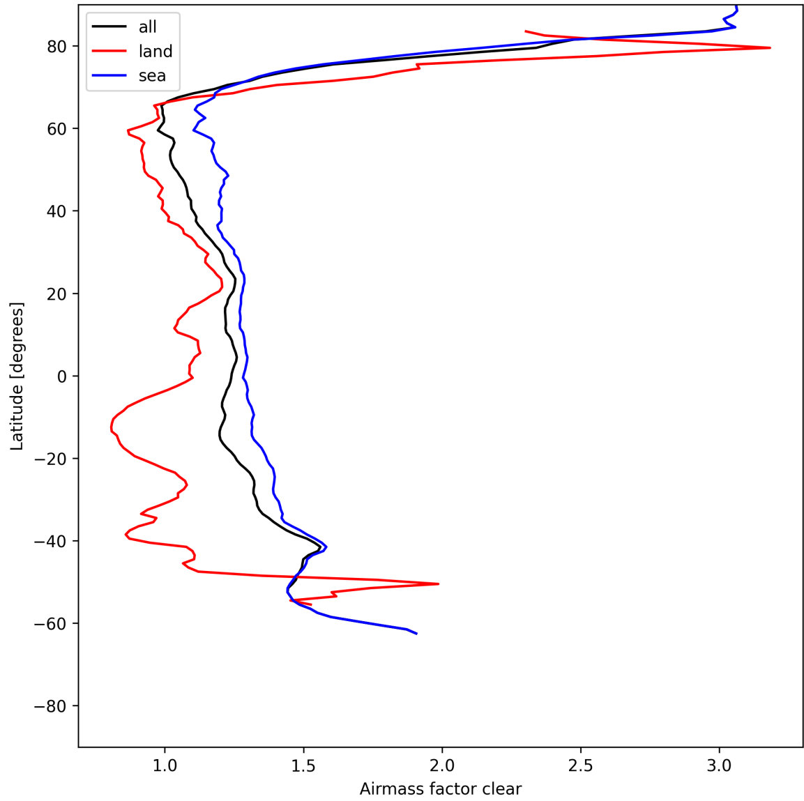
Figure 26: Zonal average of “Airmass factor clear” for 2025-07-10 to 2025-07-11.
