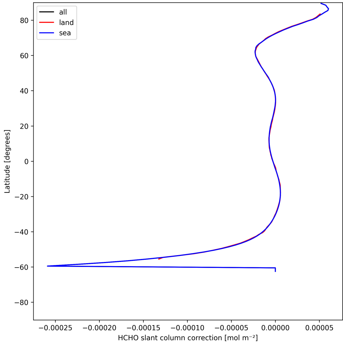
Figure 31: Zonal average of “HCHO slant column correction” for 2025-07-10 to 2025-07-11.
