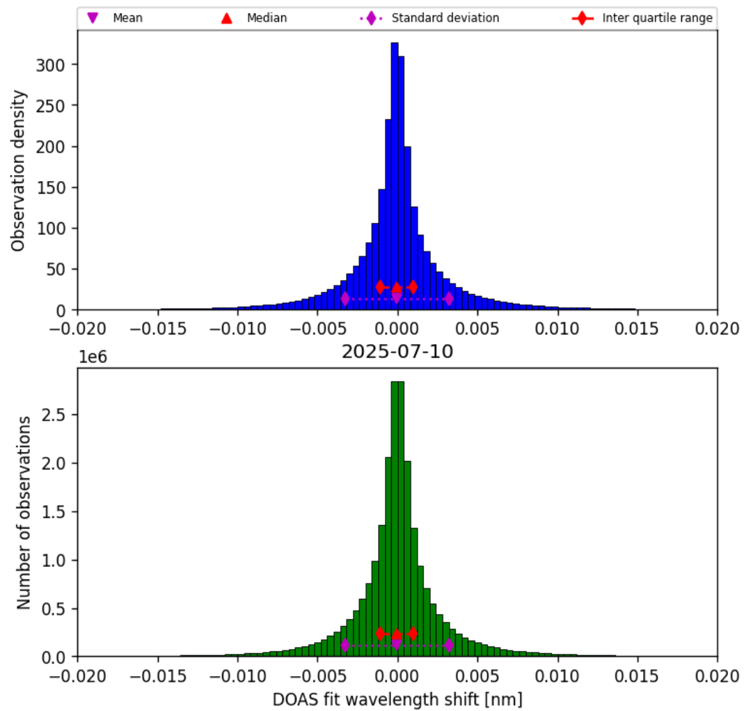
Figure 42: Histogram of “DOAS fit wavelength shift” for 2025-07-10 to 2025-07-11
