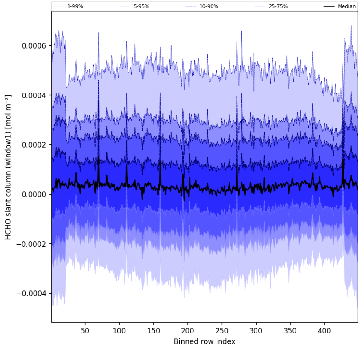
Figure 50: Along track statistics of “HCHO slant column (window1)” for 2025-07-10 to 2025-07-11
