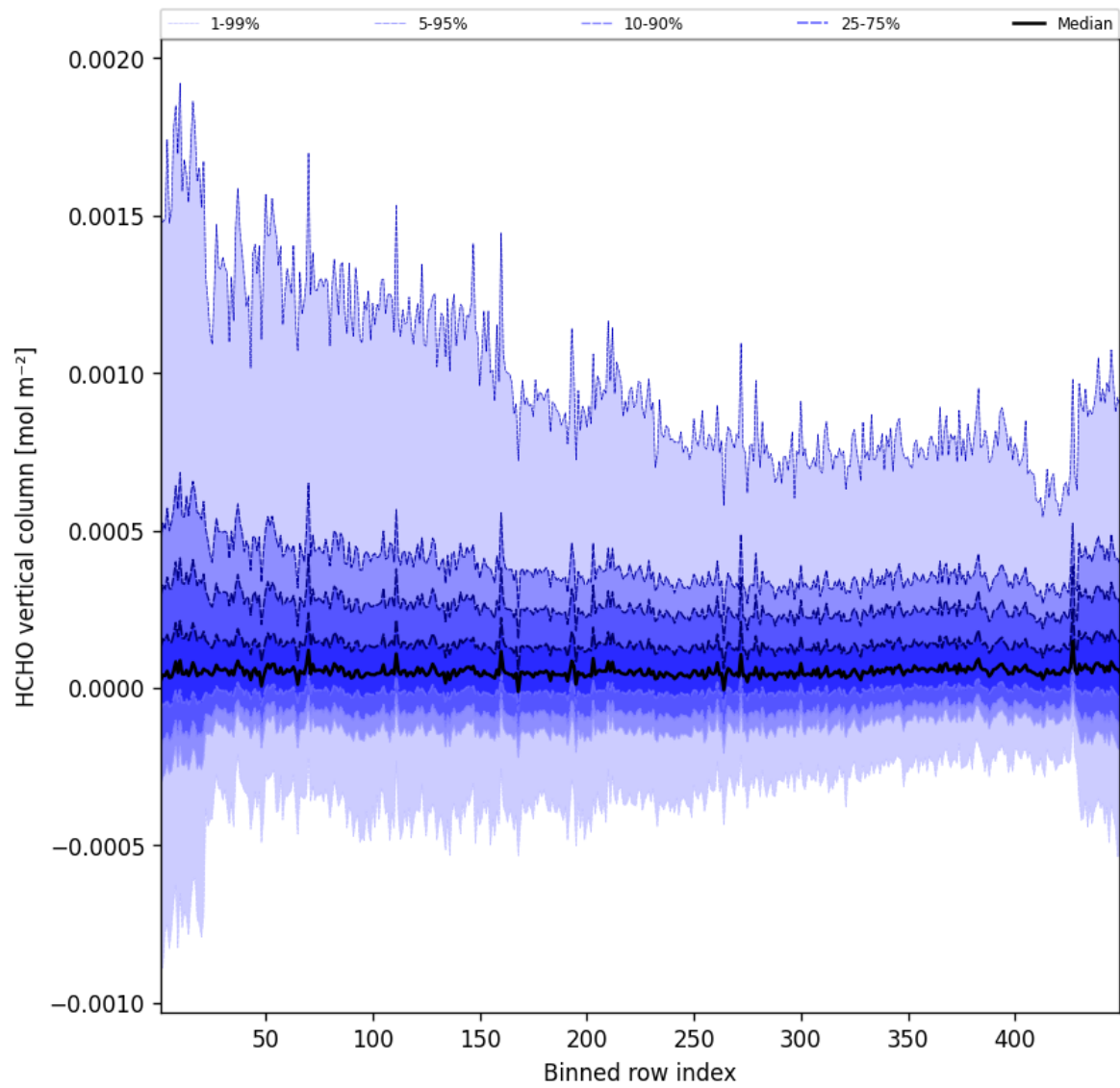
Figure 47: Along track statistics of “HCHO vertical column” for 2025-07-10 to 2025-07-11
