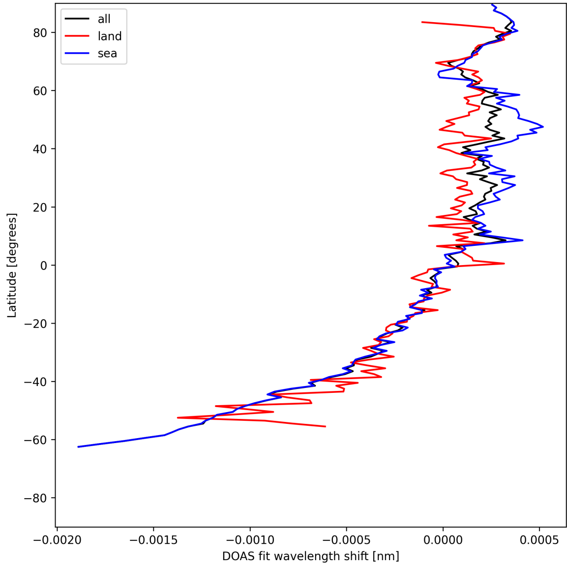
Figure 28: Zonal average of “DOAS fit wavelength shift” for 2025-07-10 to 2025-07-11.
