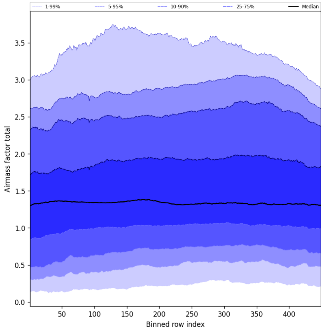
Figure 52: Along track statistics of “Airmass factor total” for 2025-07-10 to 2025-07-11
