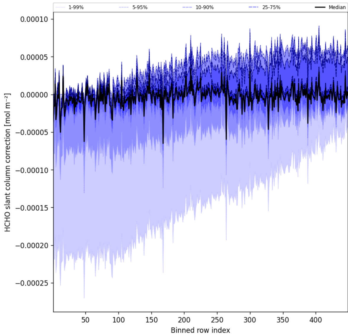
Figure 59: Along track statistics of “HCHO slant column correction” for 2025-07-10 to 2025-07-11
