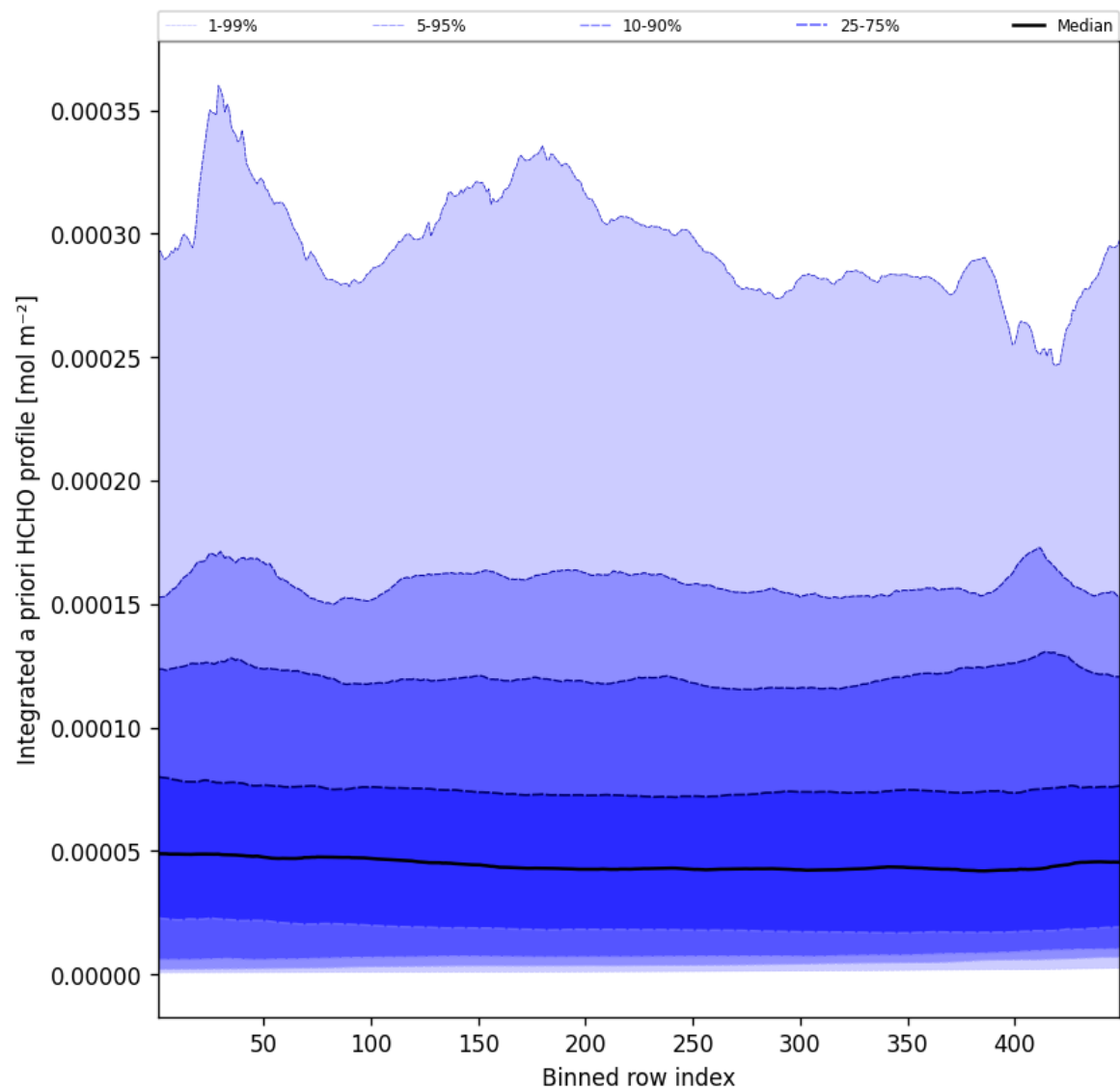
Figure 55: Along track statistics of “Integrated a priori HCHO profile” for 2025-07-10 to 2025-07-11
