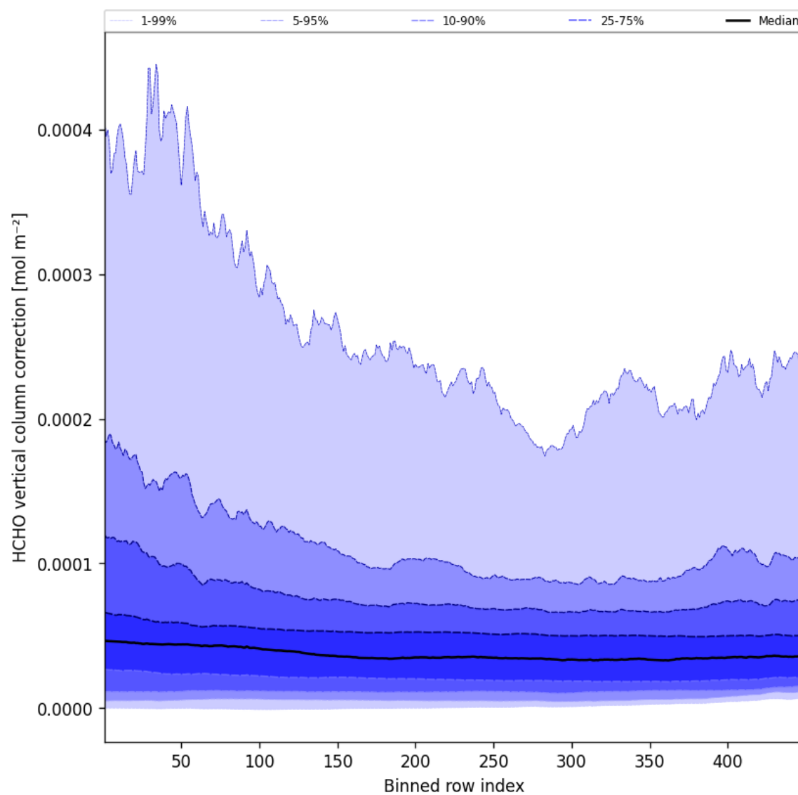
Figure 49: Along track statistics of “HCHO vertical column correction” for 2025-07-10 to 2025-07-11
