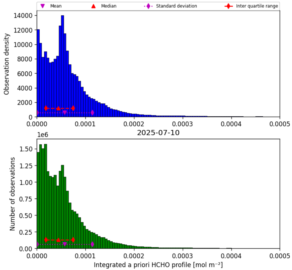
Figure 41: Histogram of “Integrated a priori HCHO profile” for 2025-07-10 to 2025-07-11
