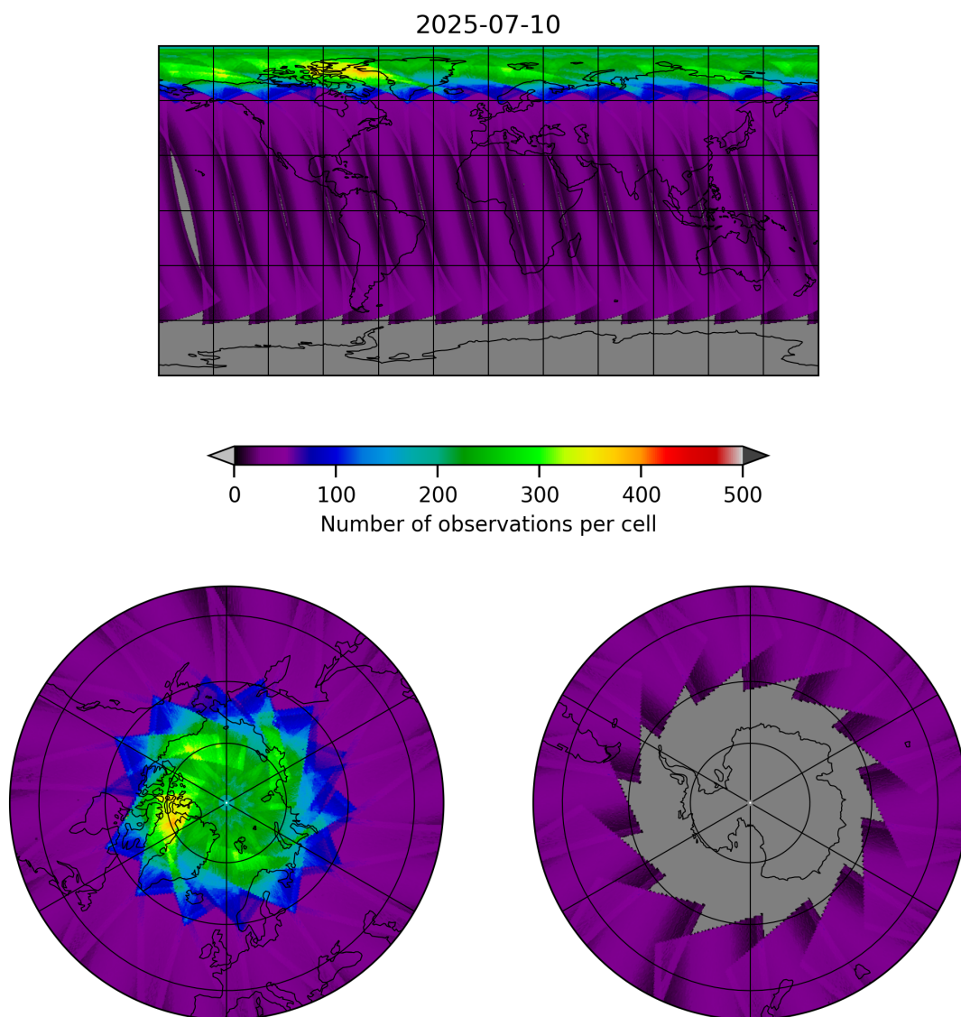
Figure 17: Map of the number of observations for 2025-07-10 to 2025-07-11
