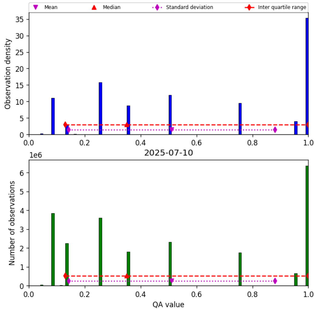
Figure 32: Histogram of “QA value” for 2025-07-10 to 2025-07-11
