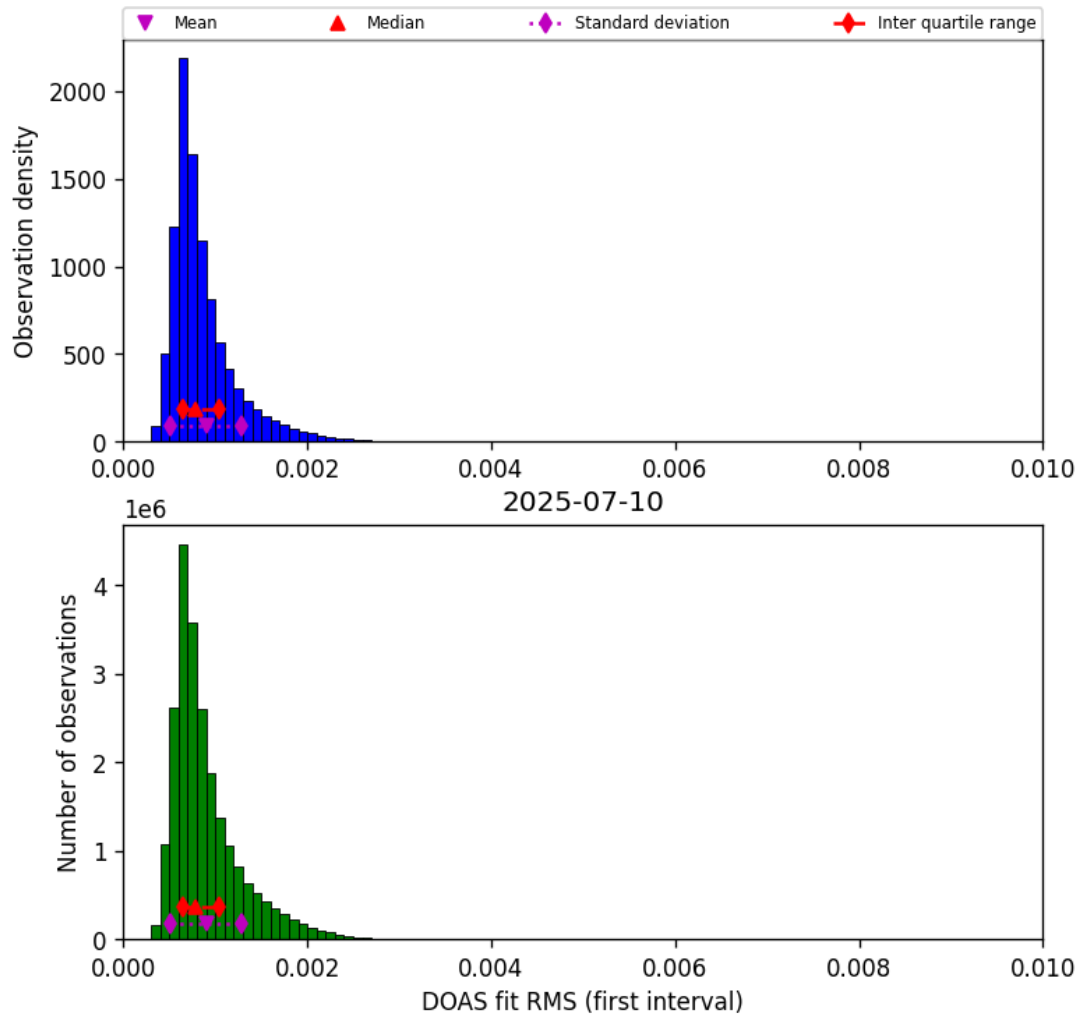
Figure 44: Histogram of "DOAS fit RMS (first interval)" for 2025-07-10 to 2025-07-11
