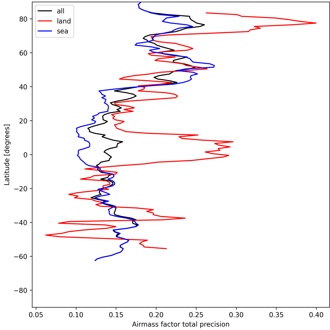
Figure 25: Zonal average of “Airmass factor total precision” for 2025-07-10 to 2025-07-11.
