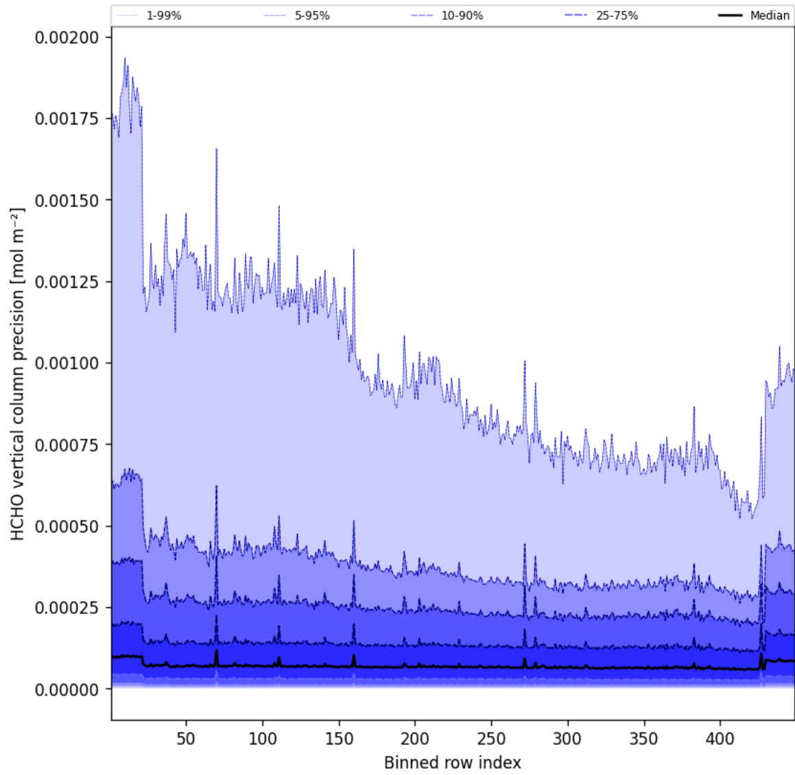
Figure 48: Along track statistics of “HCHO vertical column precision” for 2025-07-10 to 2025-07-11
