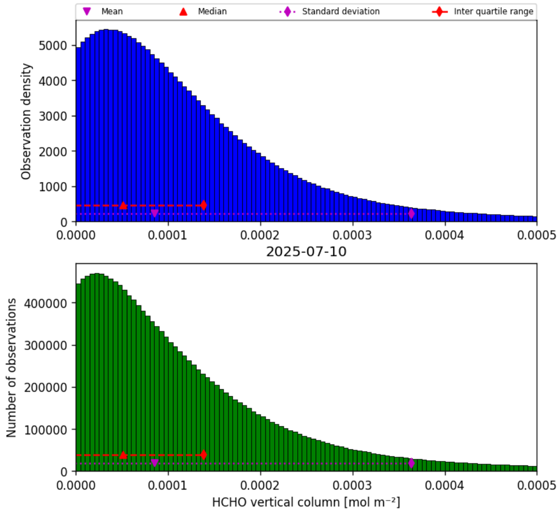
Figure 33: Histogram of “HCHO vertical column” for 2025-07-10 to 2025-07-11
