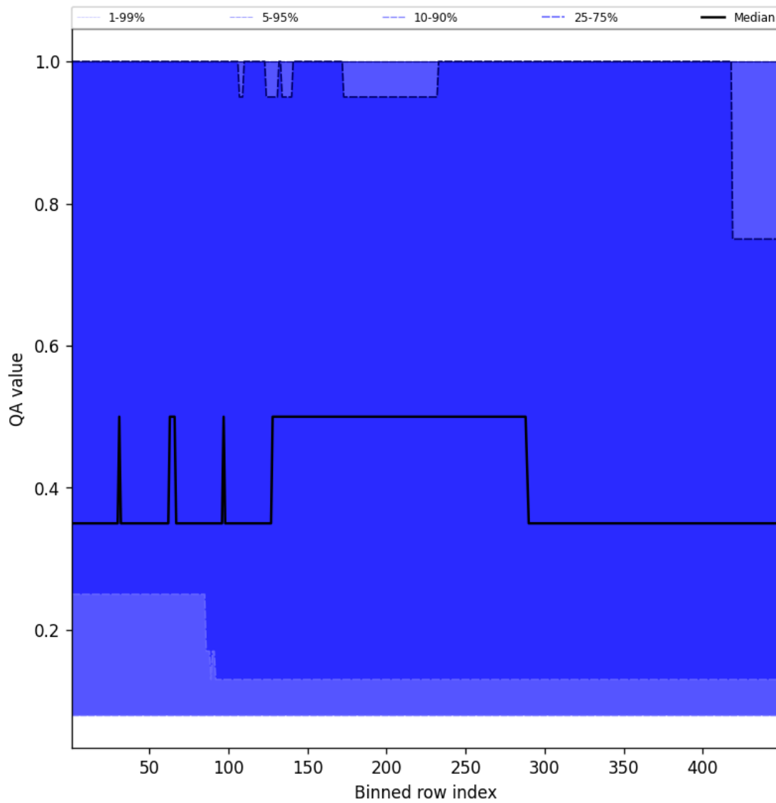
Figure 46: Along track statistics of “QA value” for 2025-07-10 to 2025-07-11
