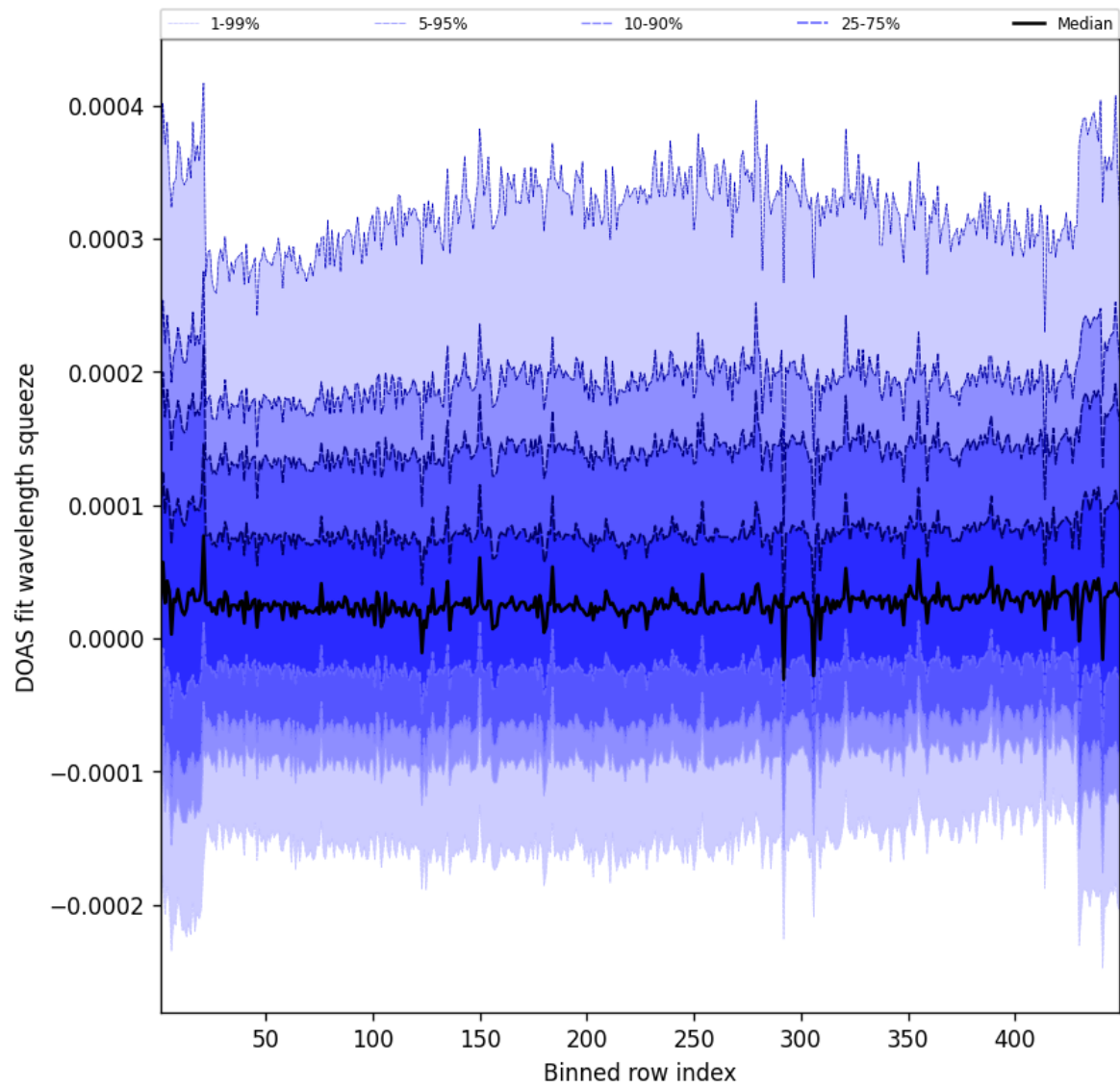
Figure 57: Along track statistics of “DOAS fit wavelength squeeze” for 2025-07-10 to 2025-07-11
