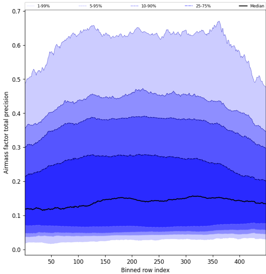
Figure 53: Along track statistics of “Airmass factor total precision” for 2025-07-10 to 2025-07-11
