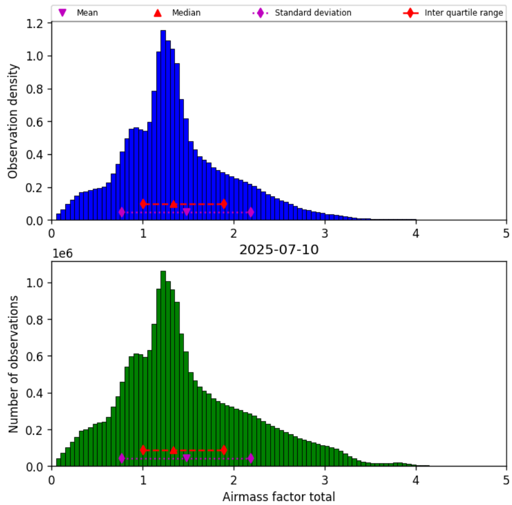
Figure 38: Histogram of “Airmass factor total” for 2025-07-10 to 2025-07-11
