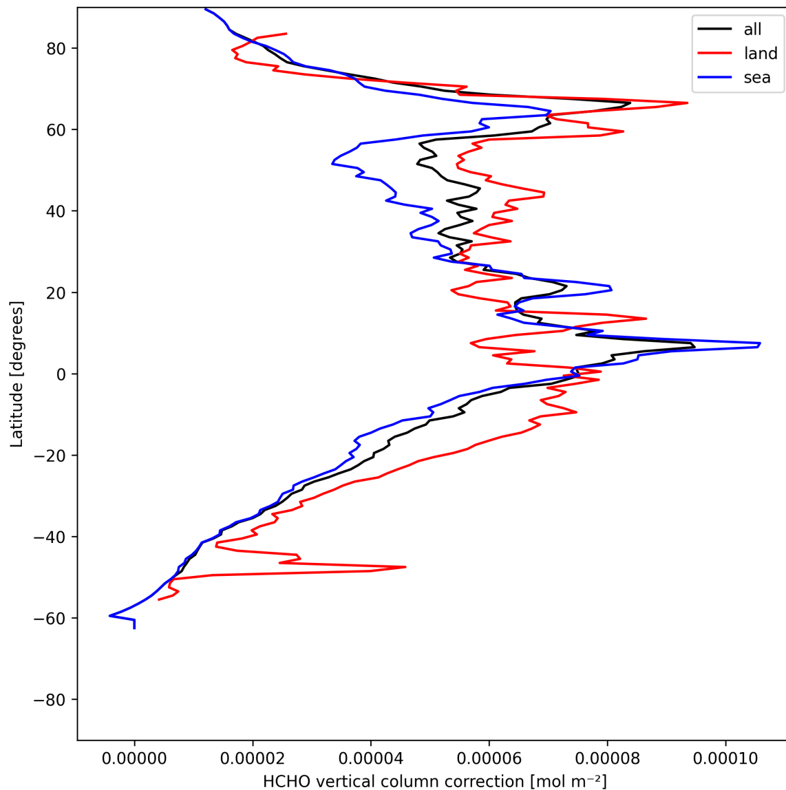
Figure 21: Zonal average of “HCHO vertical column correction” for 2025-07-10 to 2025-07-11.
