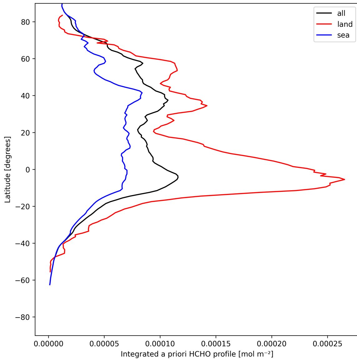
Figure 27: Zonal average of “Integrated a priori HCHO profile” for 2025-07-10 to 2025-07-11.
