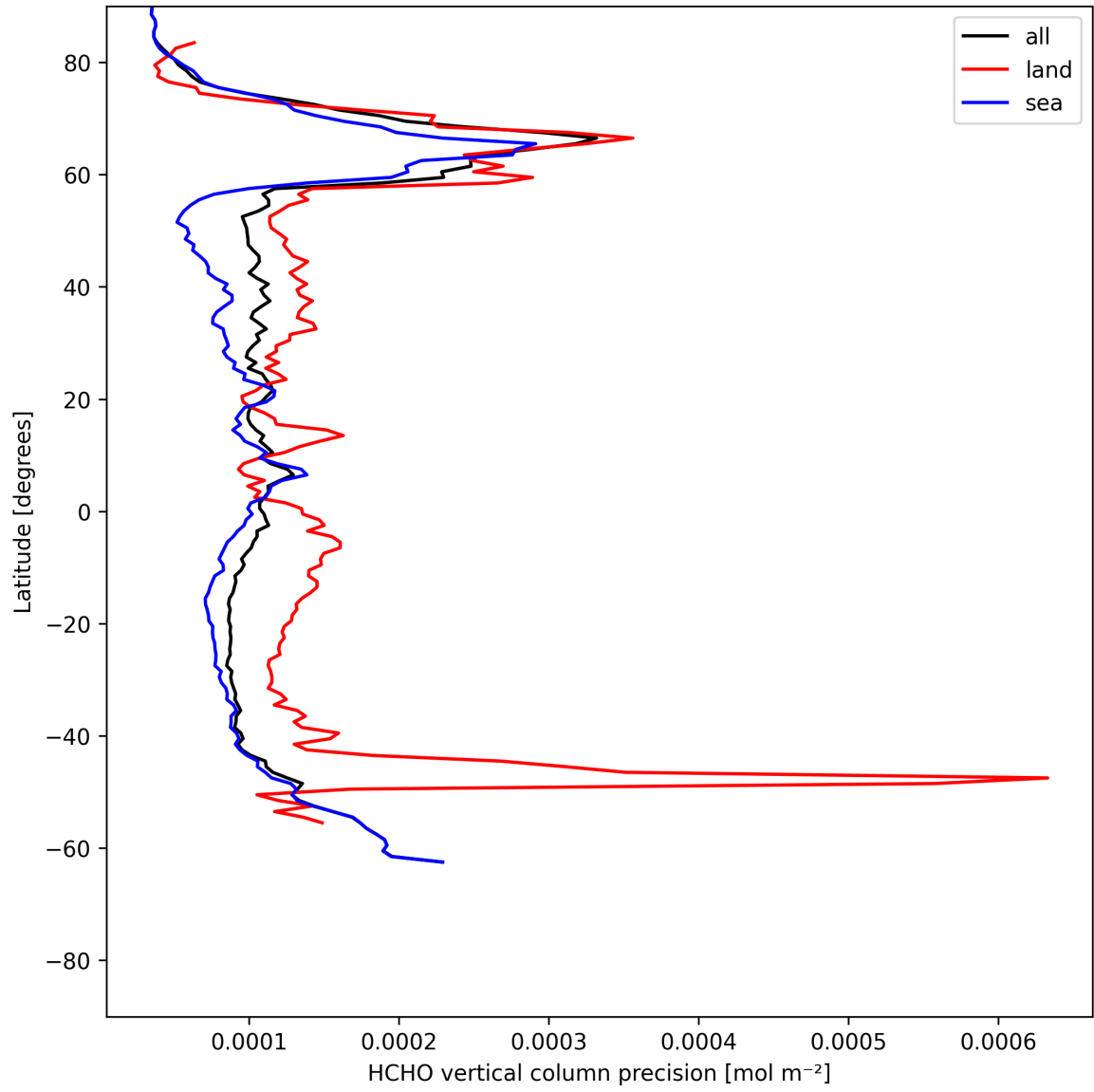
Figure 20: Zonal average of “HCHO vertical column precision” for 2025-07-10 to 2025-07-11.
