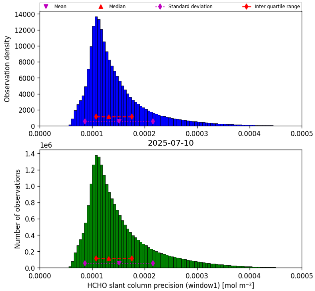
Figure 37: Histogram of “HCHO slant column precision (window1)” for 2025-07-10 to 2025-07-11
