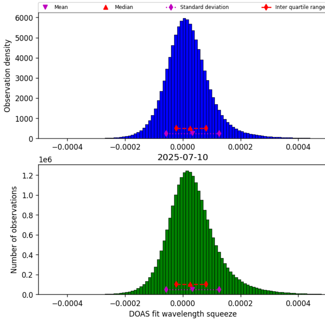
Figure 43: Histogram of “DOAS fit wavelength squeeze” for 2025-07-10 to 2025-07-11
