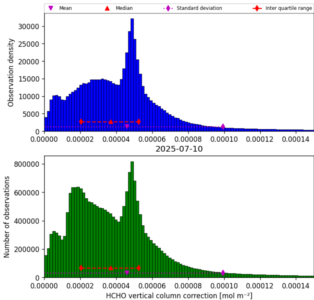
Figure 35: Histogram of “HCHO vertical column correction” for 2025-07-10 to 2025-07-11
