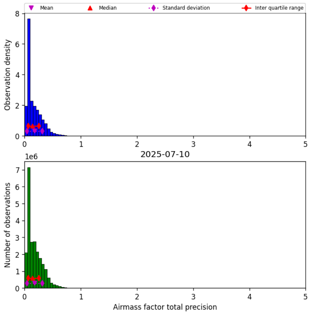
Figure 39: Histogram of “Airmass factor total precision” for 2025-07-10 to 2025-07-11
