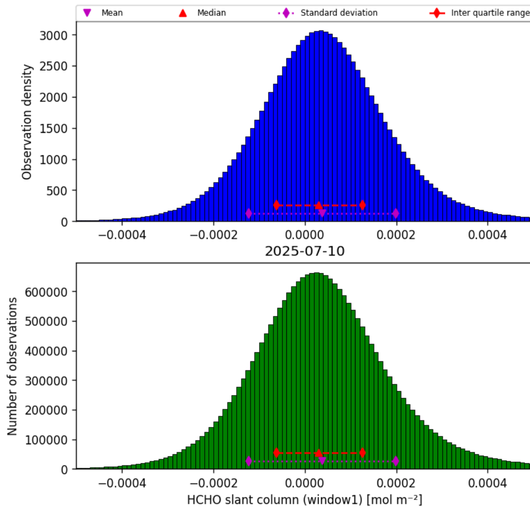
Figure 36: Histogram of “HCHO slant column (window1)” for 2025-07-10 to 2025-07-11
