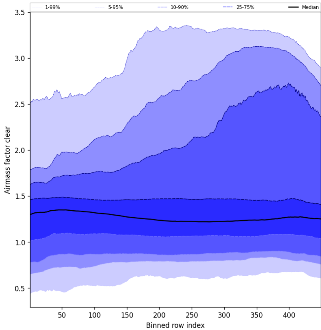
Figure 54: Along track statistics of “Airmass factor clear” for 2025-07-10 to 2025-07-11
