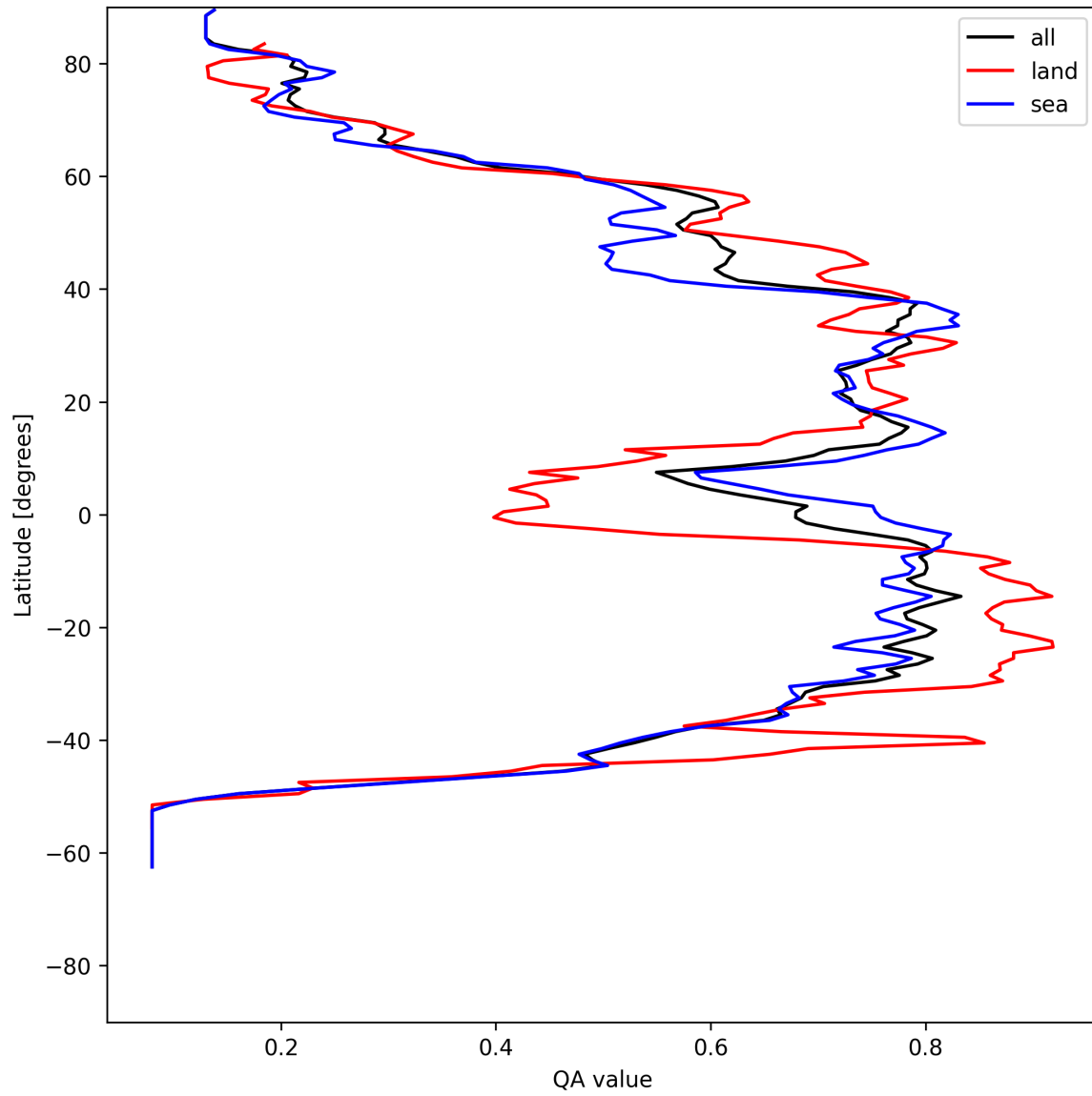
Figure 18: Zonal average of “QA value” for 2025-07-10 to 2025-07-11.
