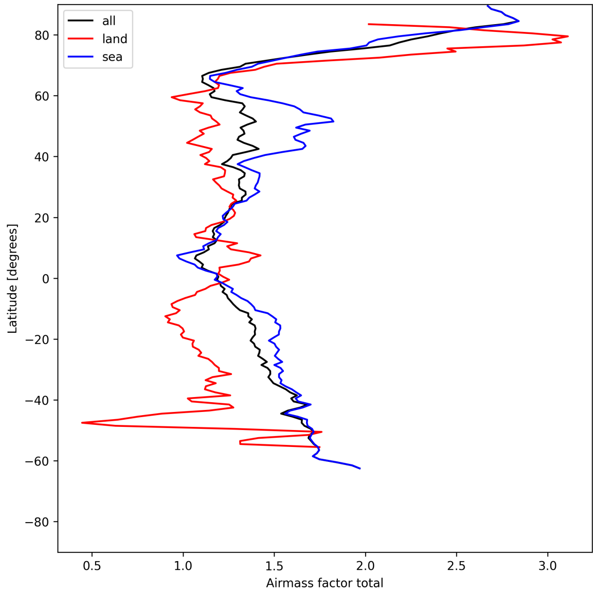
Figure 24: Zonal average of “Airmass factor total” for 2025-07-10 to 2025-07-11.
