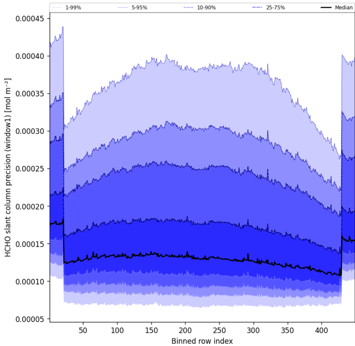
Figure 51: Along track statistics of “HCHO slant column precision (window1)” for 2025-07-10 to 2025-07-11
