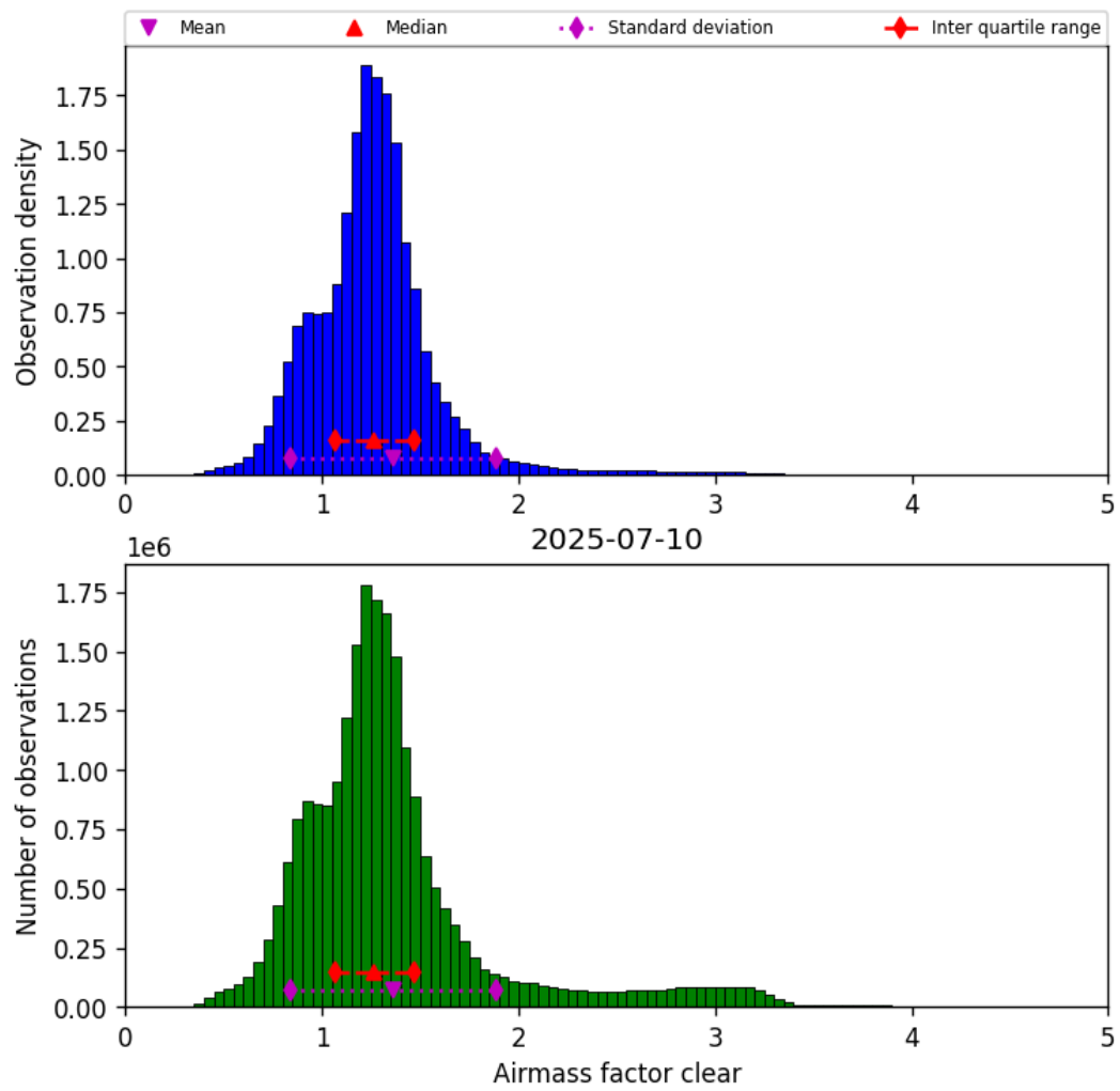
Figure 40: Histogram of “Airmass factor clear” for 2025-07-10 to 2025-07-11
