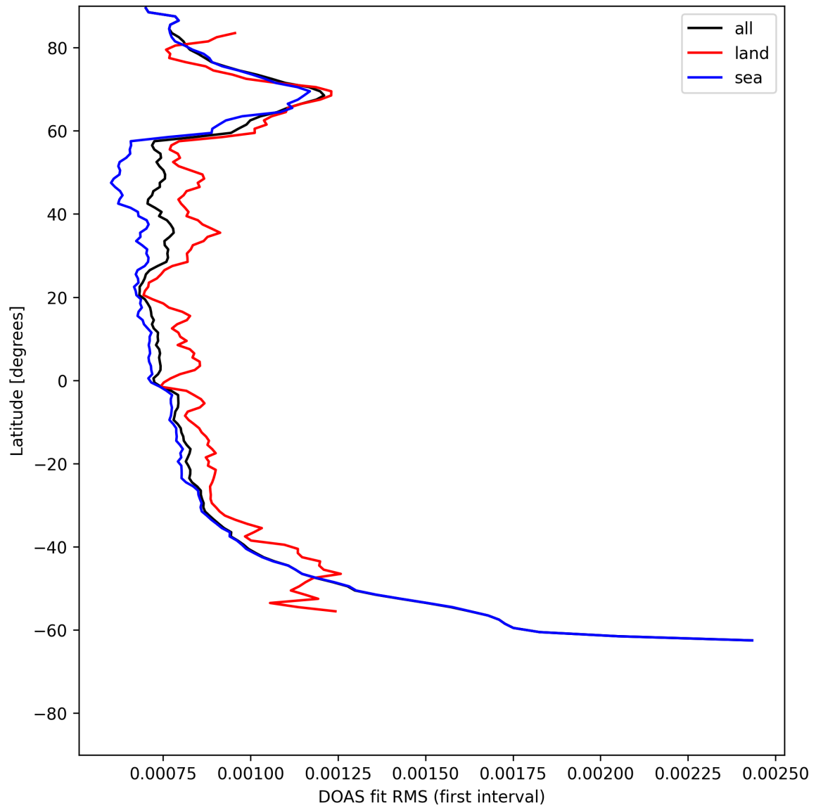
Figure 30: Zonal average of “DOAS fit RMS (first interval)” for 2025-07-10 to 2025-07-11.
