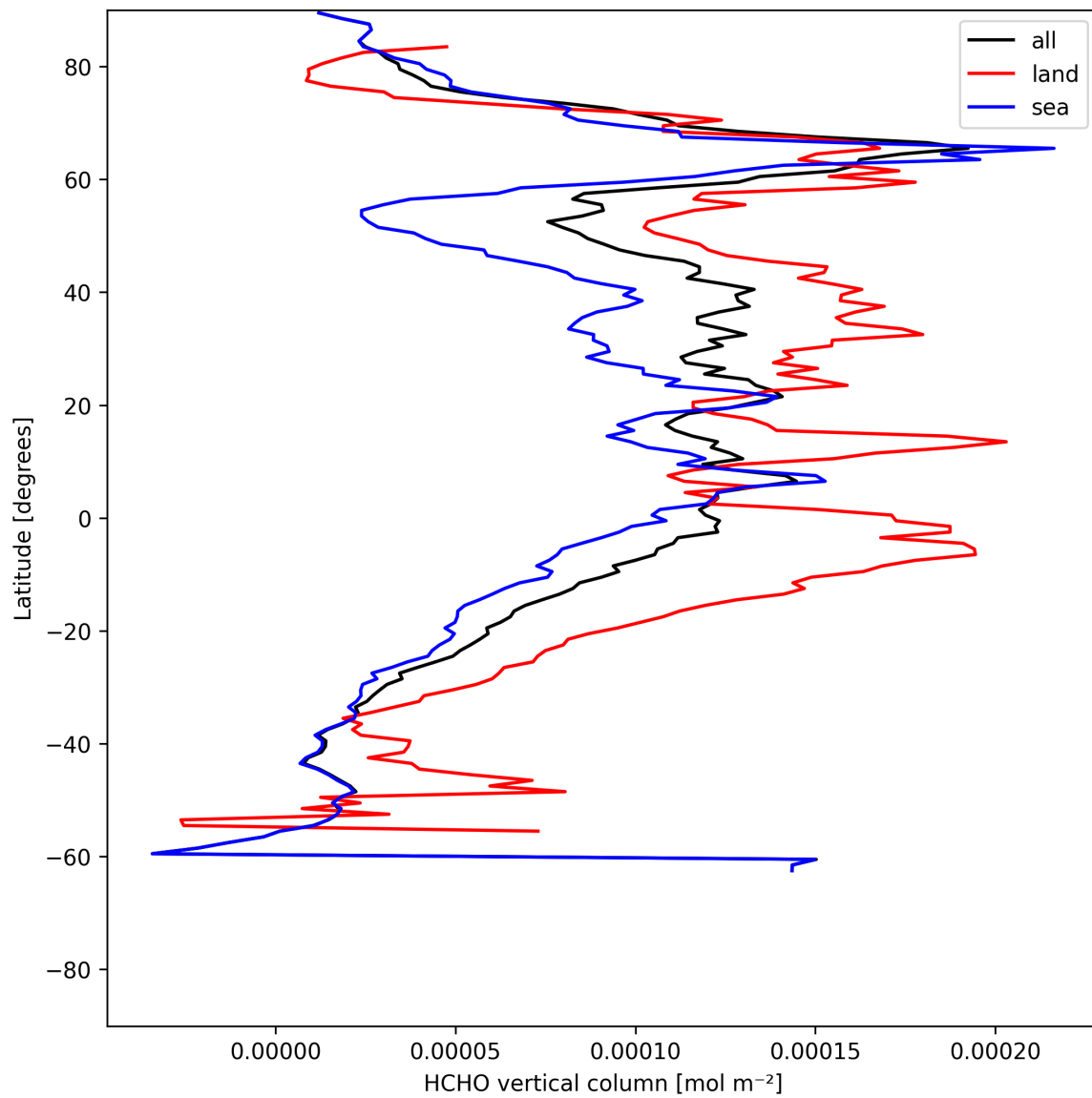
Figure 19: Zonal average of “HCHO vertical column” for 2025-07-10 to 2025-07-11.
