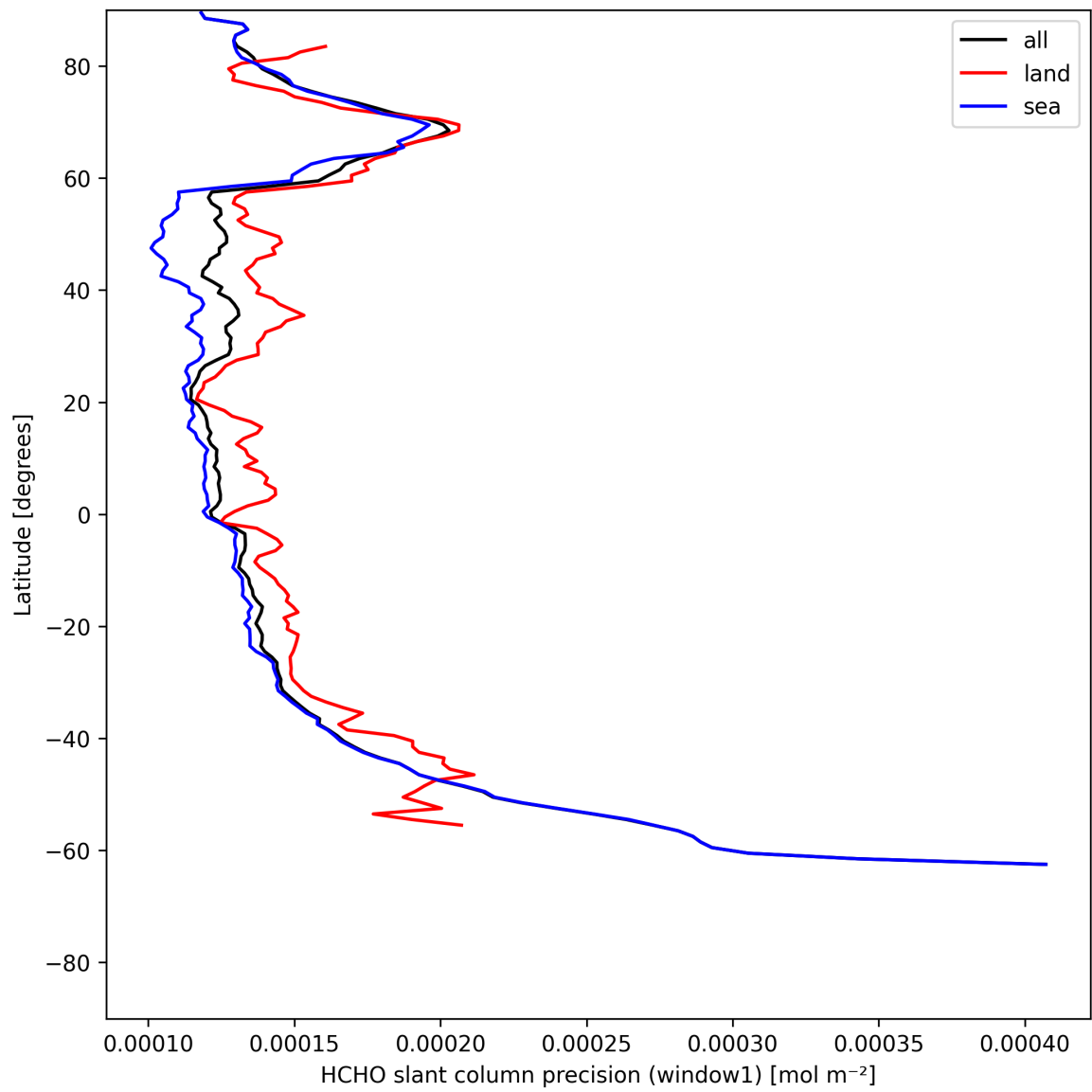
Figure 23: Zonal average of “HCHO slant column precision (window1)” for 2025-07-10 to 2025-07-11.
