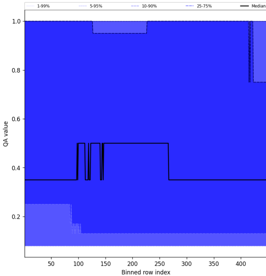
Figure 46: Along track statistics of “QA value” for 2025-07-11 to 2025-07-11
