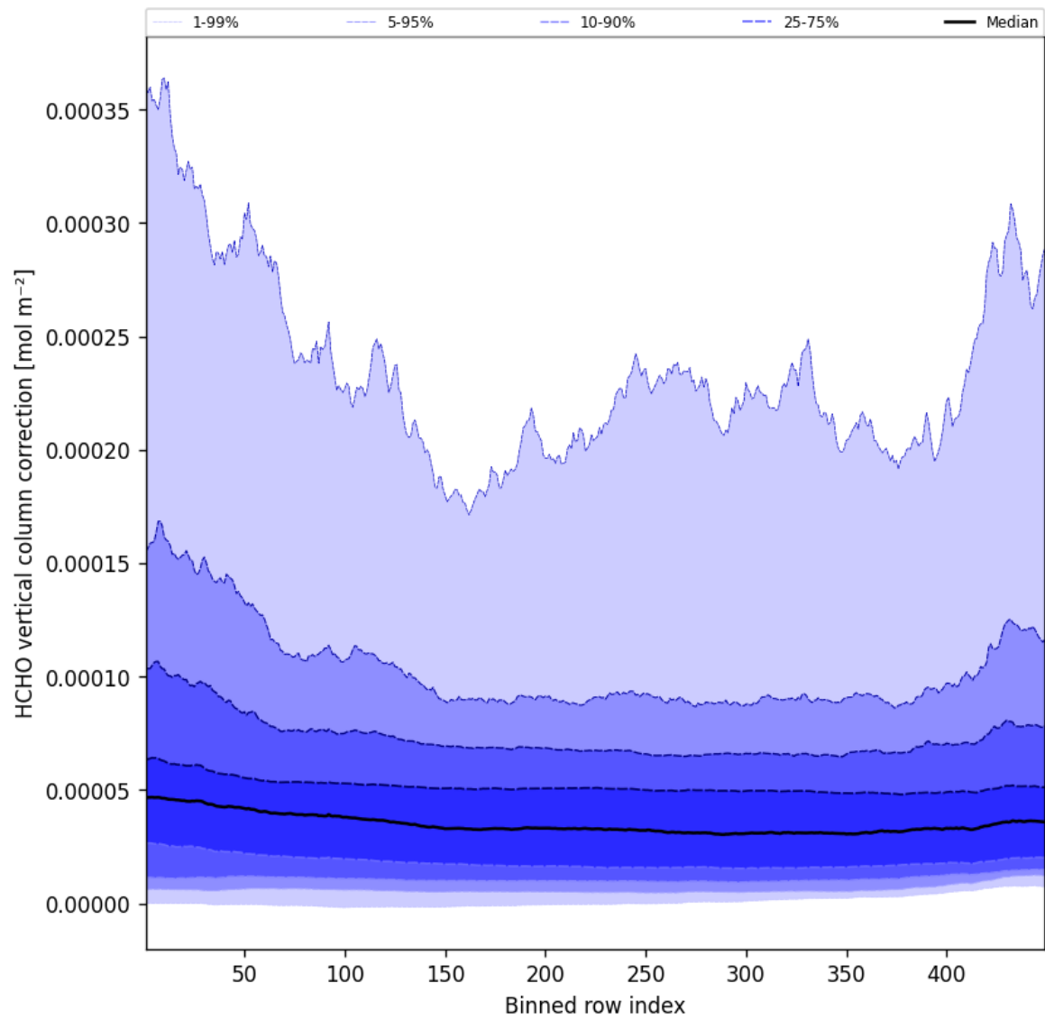
Figure 49: Along track statistics of “HCHO vertical column correction” for 2025-07-11 to 2025-07-11
