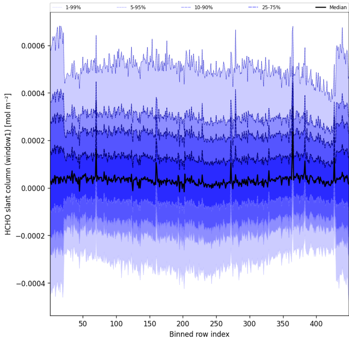
Figure 50: Along track statistics of “HCHO slant column (window1)” for 2025-07-11 to 2025-07-11
