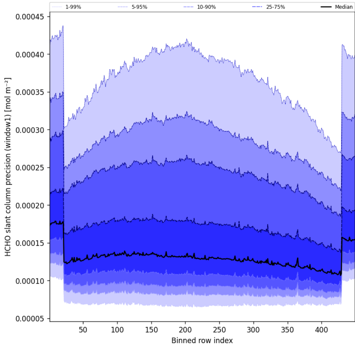
Figure 51: Along track statistics of “HCHO slant column precision (window1)” for 2025-07-11 to 2025-07-11
