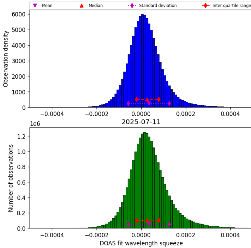
Figure 43: Histogram of “DOAS fit wavelength squeeze” for 2025-07-11 to 2025-07-11
