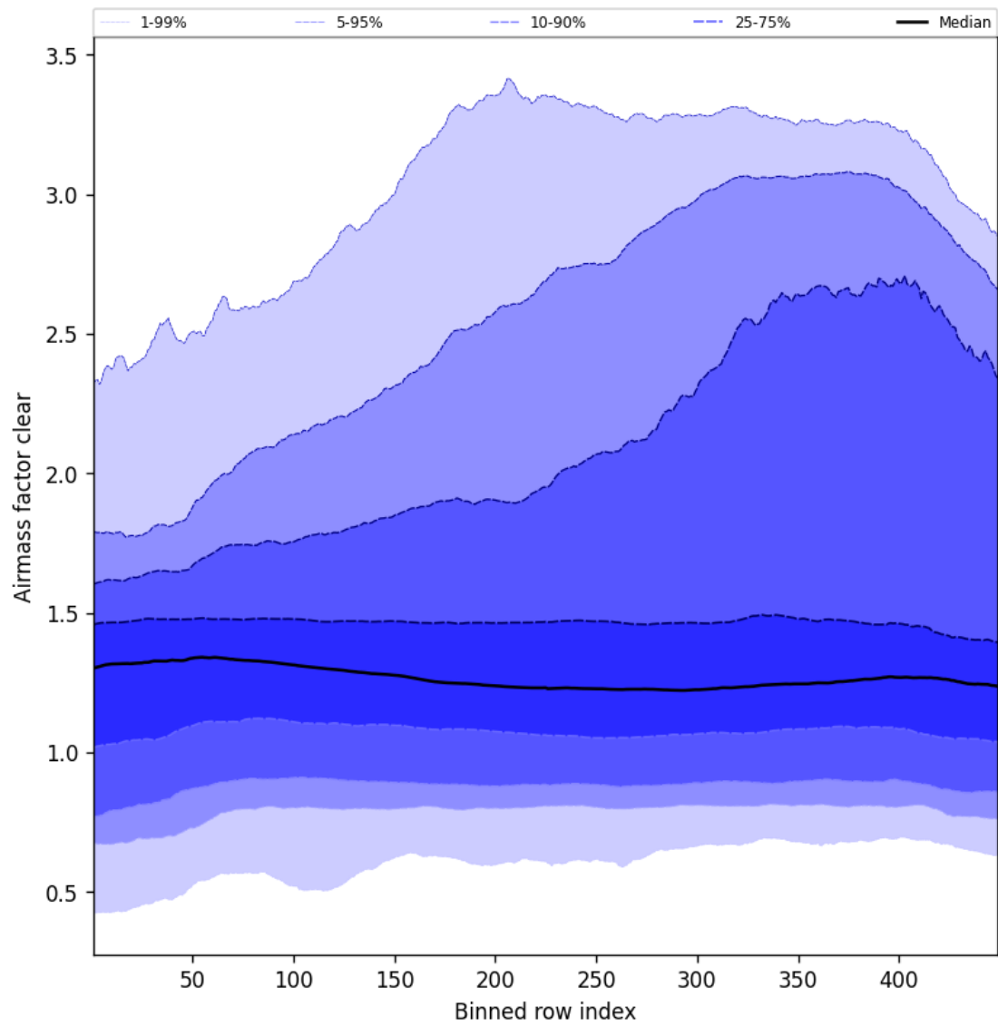
Figure 54: Along track statistics of “Airmass factor clear” for 2025-07-11 to 2025-07-11
