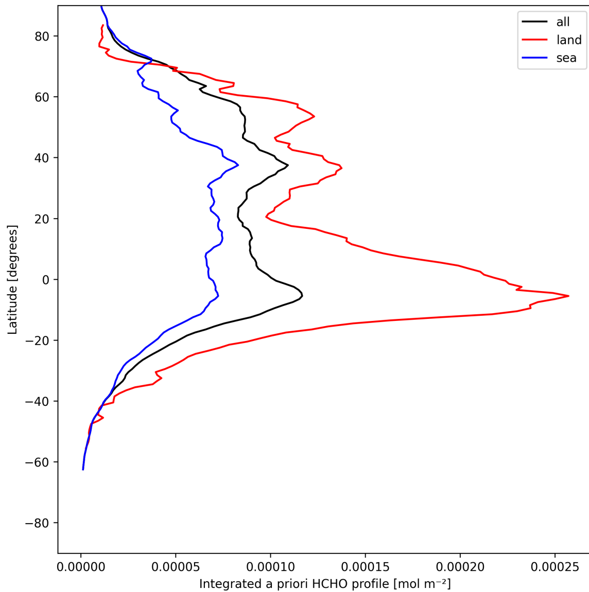
Figure 27: Zonal average of “Integrated a priori HCHO profile” for 2025-07-11 to 2025-07-11.
