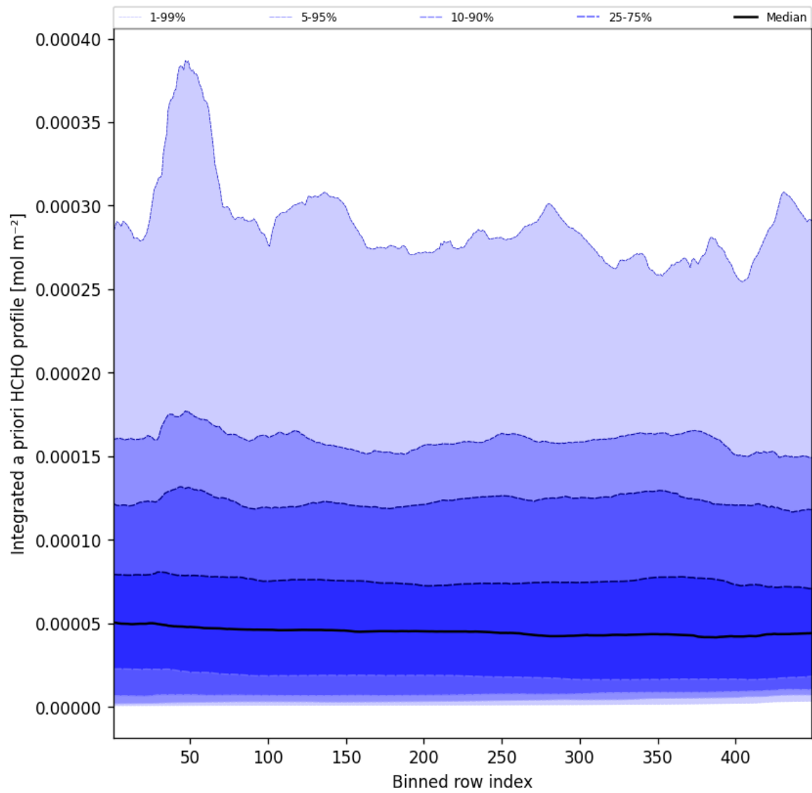
Figure 55: Along track statistics of "Integrated a priori HCHO profile" for 2025-07-11 to 2025-07-11
