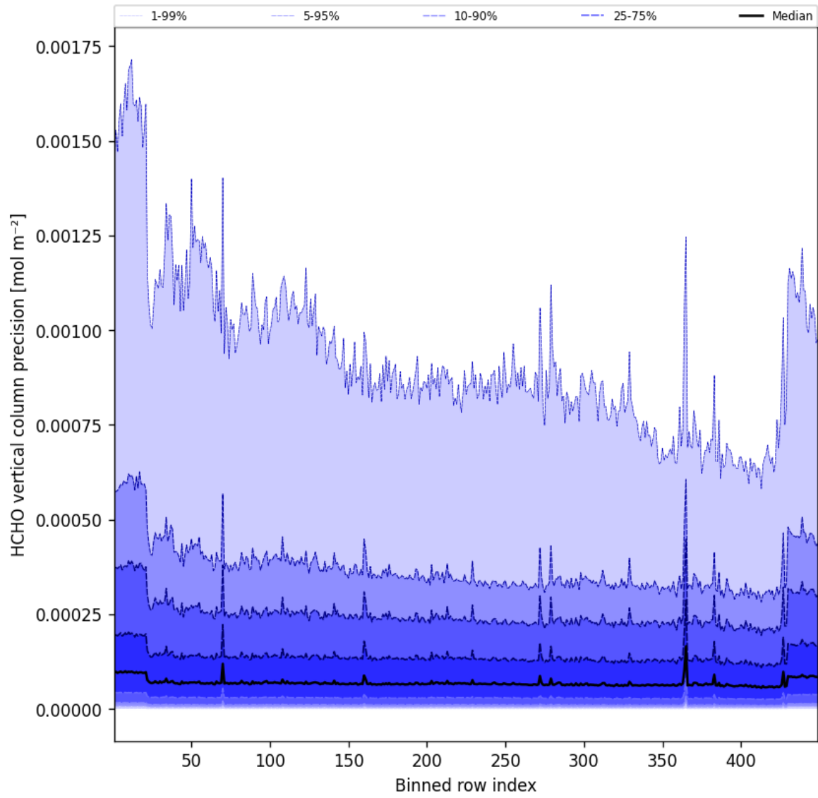
Figure 48: Along track statistics of “HCHO vertical column precision” for 2025-07-11 to 2025-07-11
