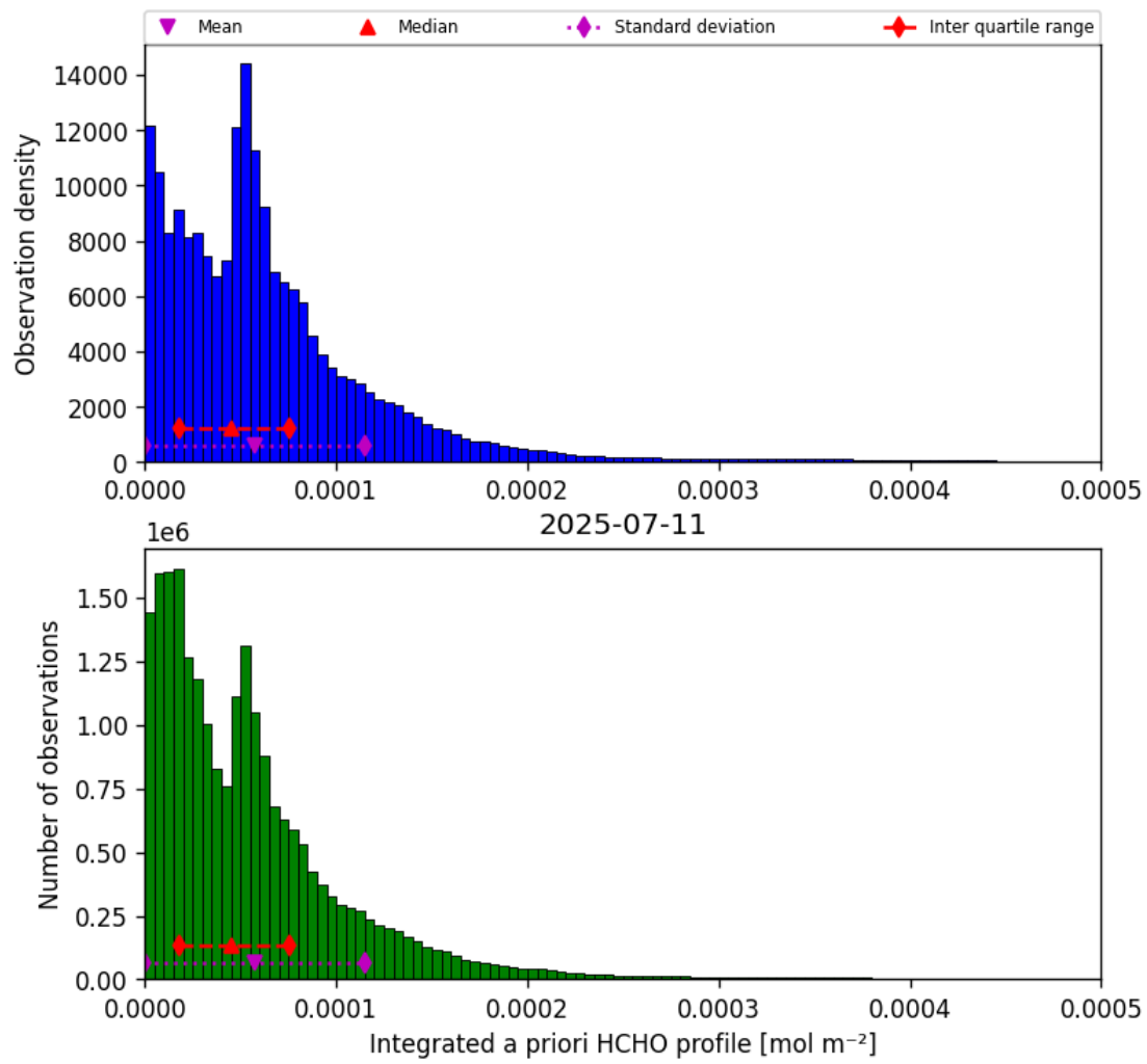
Figure 41: Histogram of “Integrated a priori HCHO profile” for 2025-07-11 to 2025-07-11
