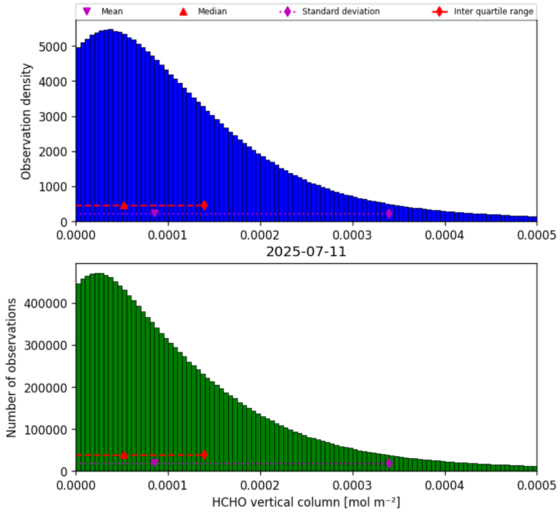
Figure 33: Histogram of “HCHO vertical column” for 2025-07-11 to 2025-07-11
