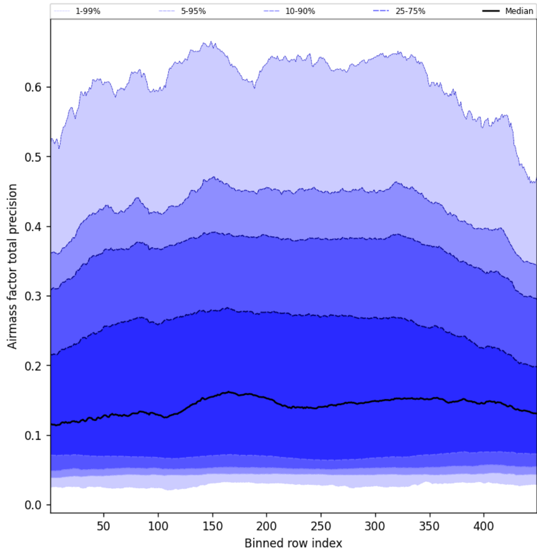
Figure 53: Along track statistics of “Airmass factor total precision” for 2025-07-11 to 2025-07-11
