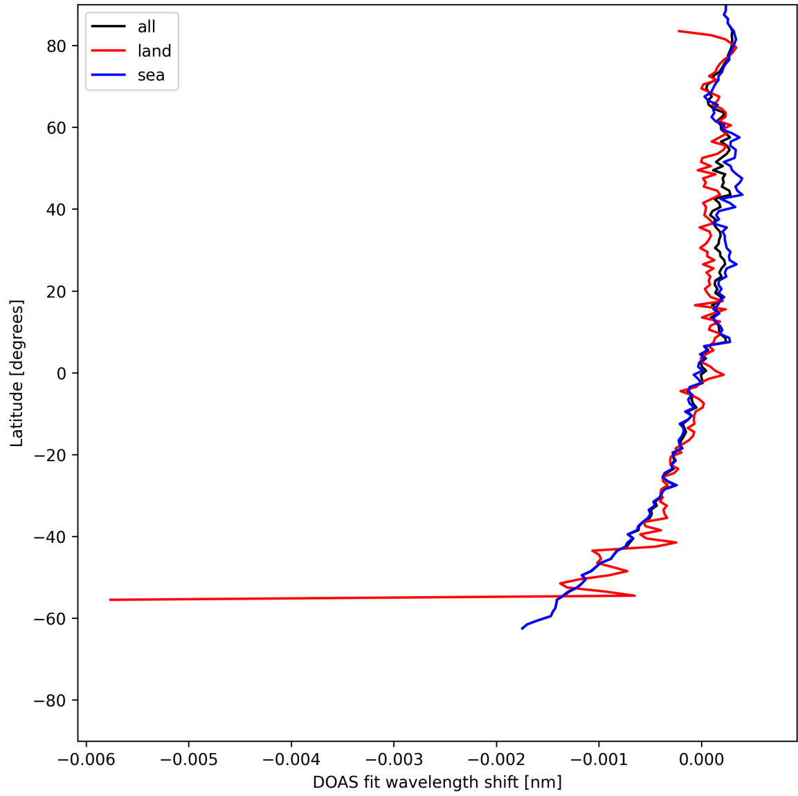
Figure 28: Zonal average of “DOAS fit wavelength shift” for 2025-07-11 to 2025-07-11.
