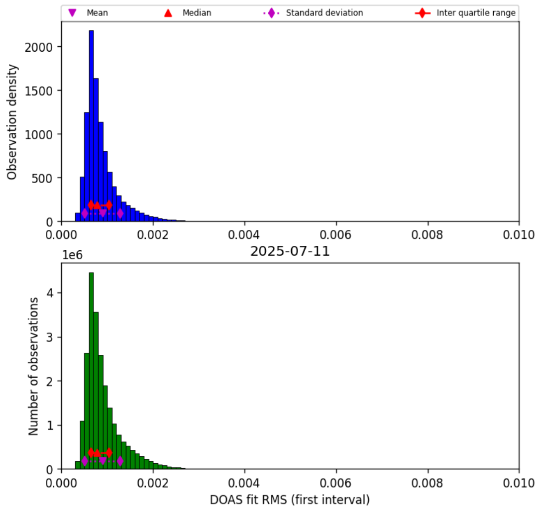
Figure 44: Histogram of “DOAS fit RMS (first interval)” for 2025-07-11 to 2025-07-11
