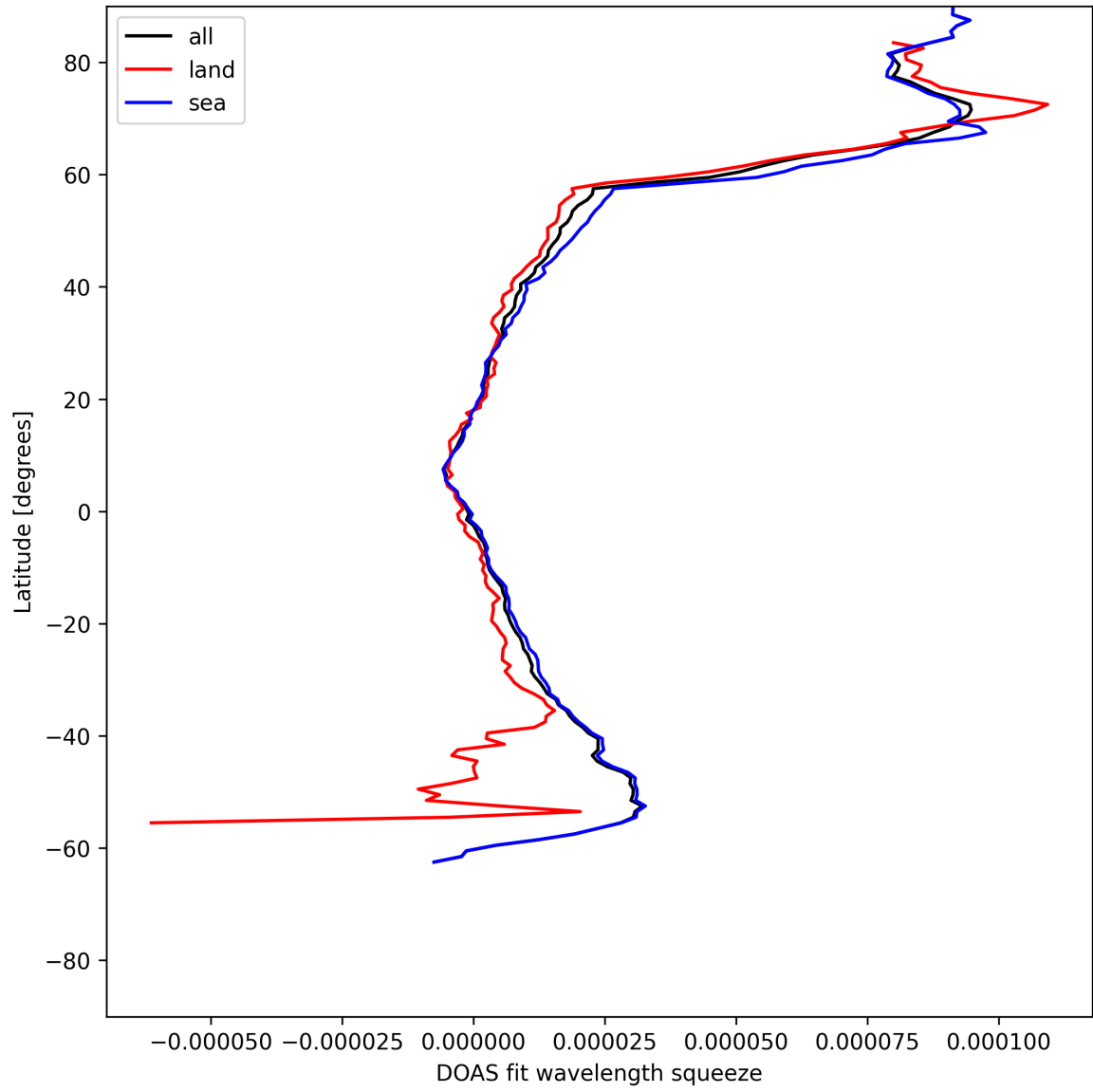
Figure 29: Zonal average of “DOAS fit wavelength squeeze” for 2025-07-11 to 2025-07-11.
