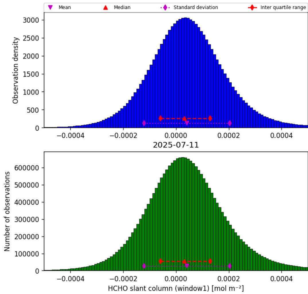
Figure 36: Histogram of "HCHO slant column (window1)" for 2025-07-11 to 2025-07-11
