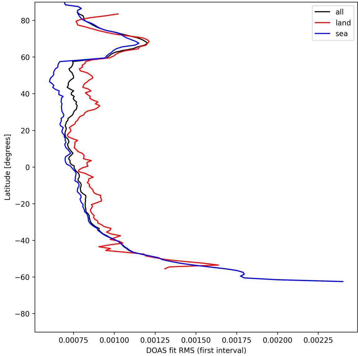
Figure 30: Zonal average of “DOAS fit RMS (first interval)” for 2025-07-11 to 2025-07-11.
