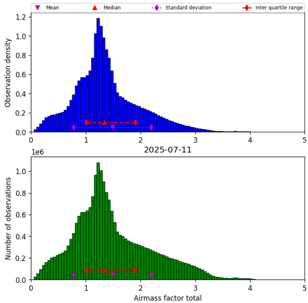
Figure 38: Histogram of “Airmass factor total” for 2025-07-11 to 2025-07-11
