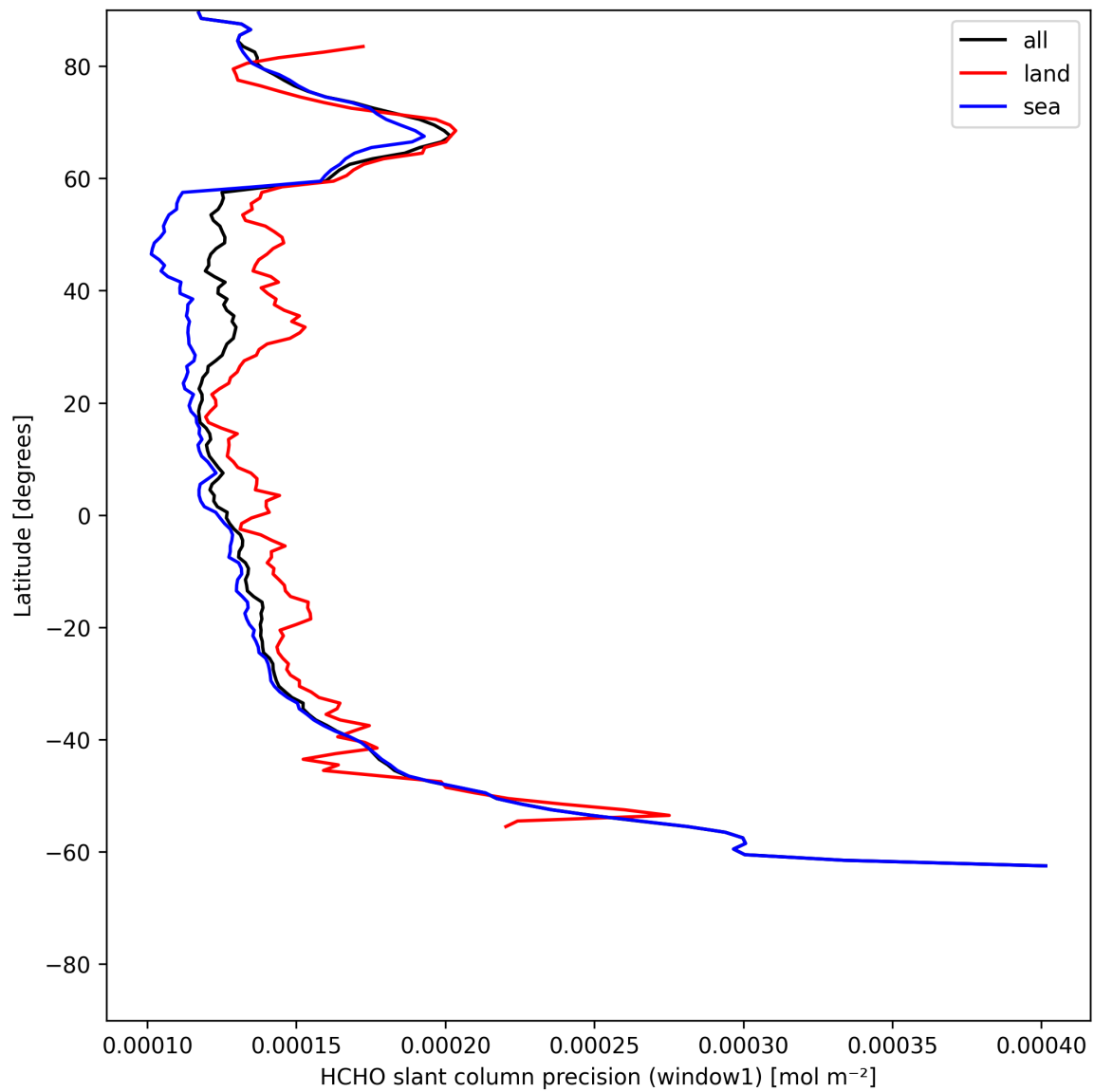
Figure 23: Zonal average of “HCHO slant column precision (window1)” for 2025-07-11 to 2025-07-11.
