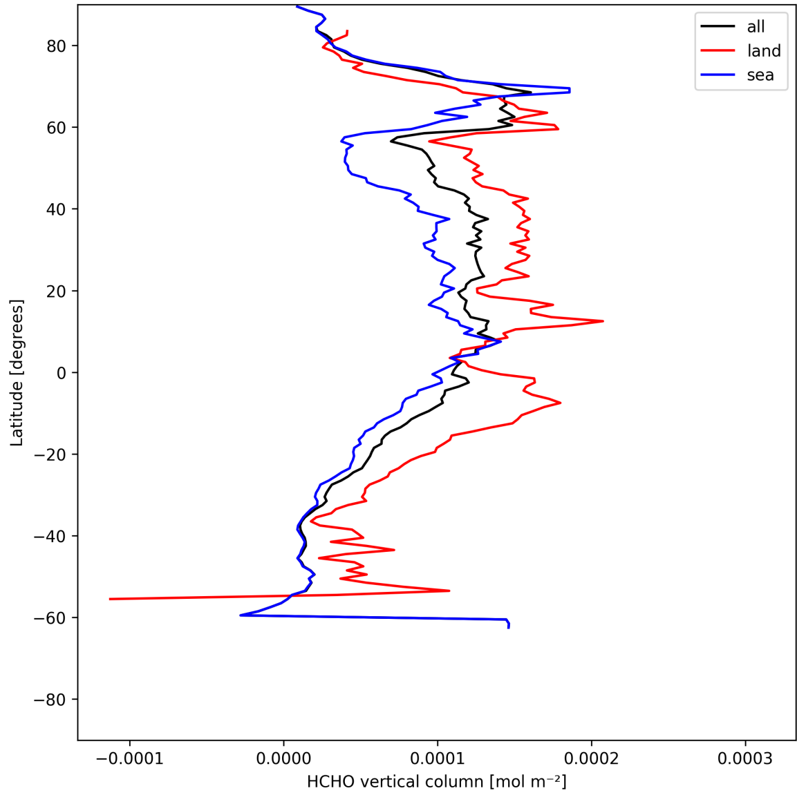
Figure 19: Zonal average of “HCHO vertical column” for 2025-07-11 to 2025-07-11.
