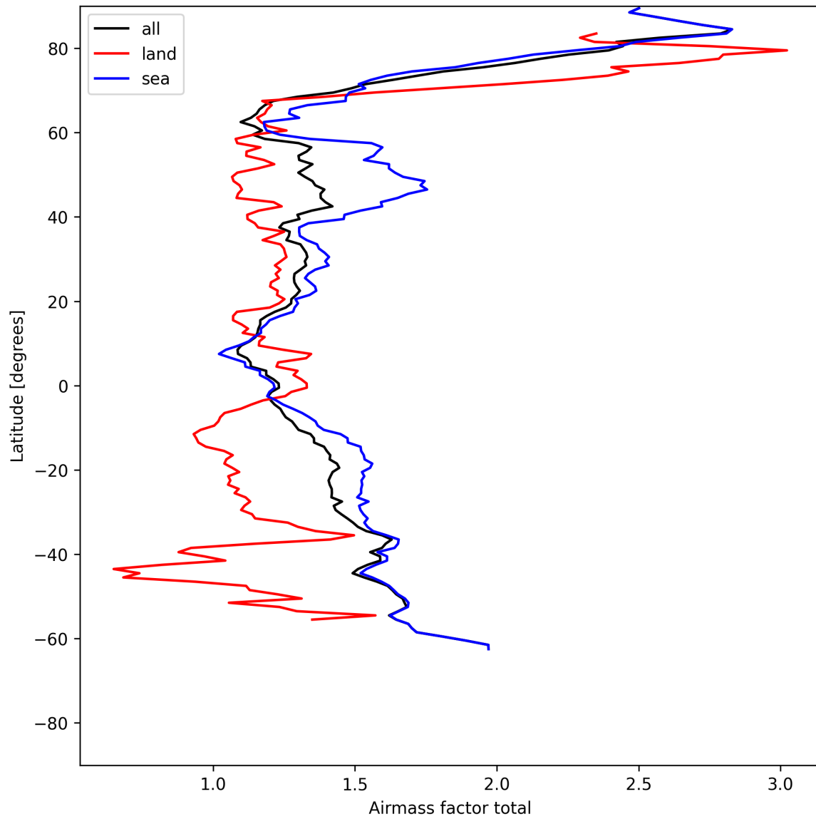
Figure 24: Zonal average of “Airmass factor total” for 2025-07-11 to 2025-07-11.
