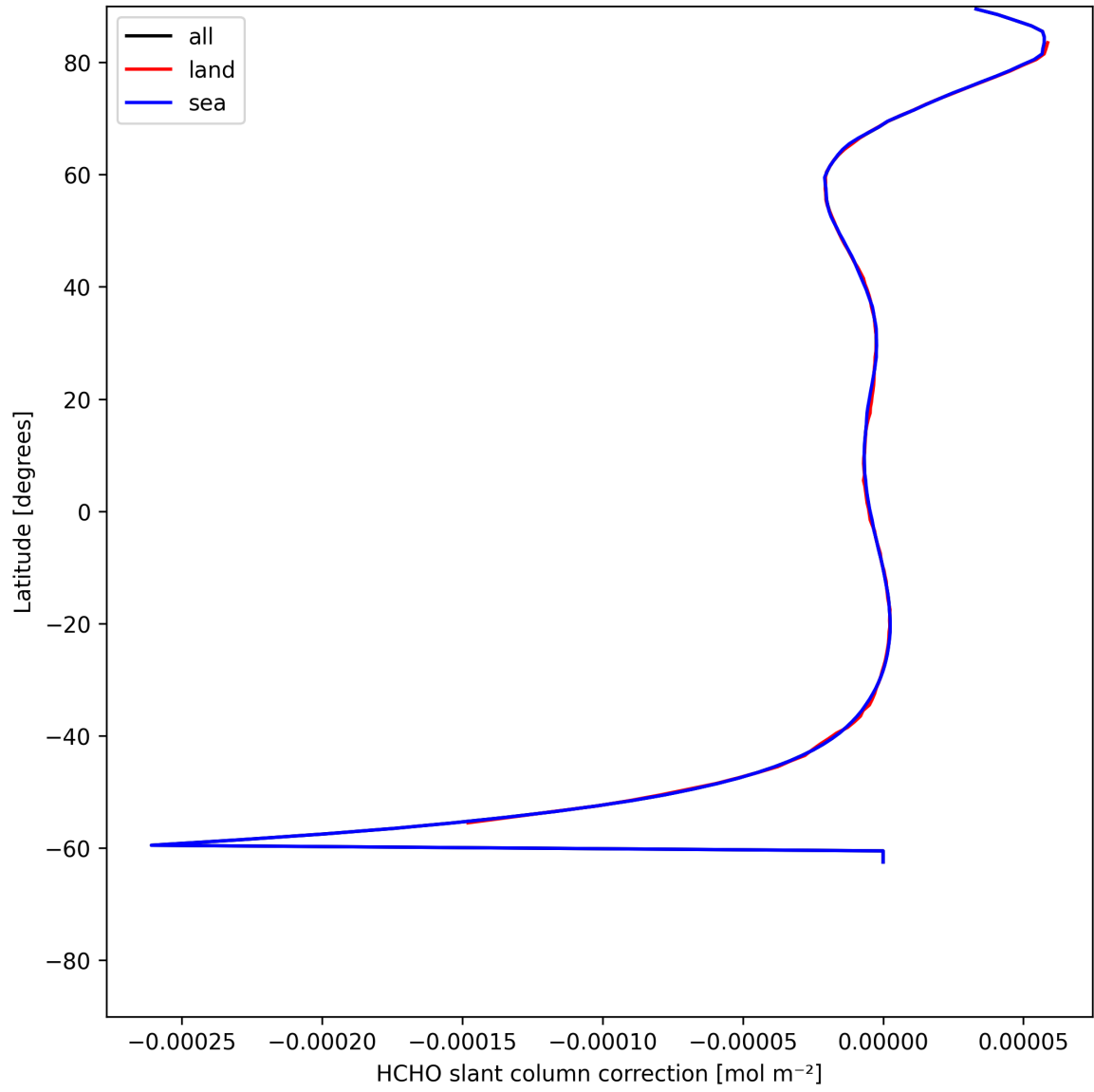
Figure 31: Zonal average of “HCHO slant column correction” for 2025-07-11 to 2025-07-11.
