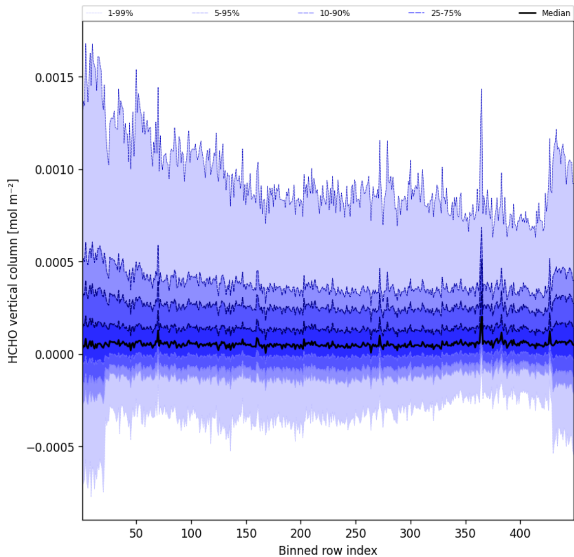
Figure 47: Along track statistics of “HCHO vertical column” for 2025-07-11 to 2025-07-11
