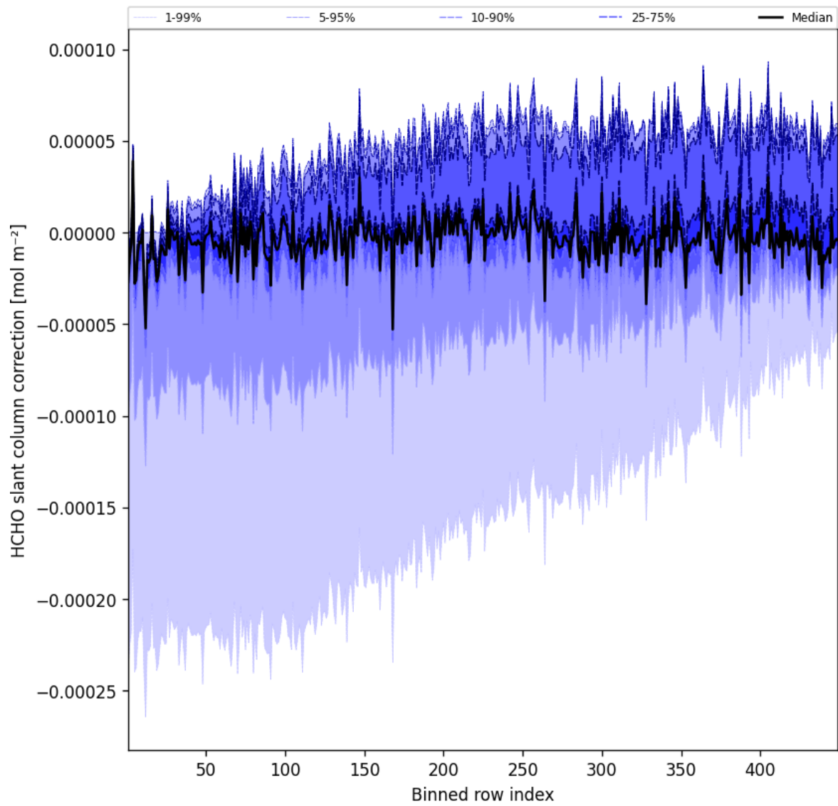
Figure 59: Along track statistics of “HCHO slant column correction” for 2025-07-11 to 2025-07-11
