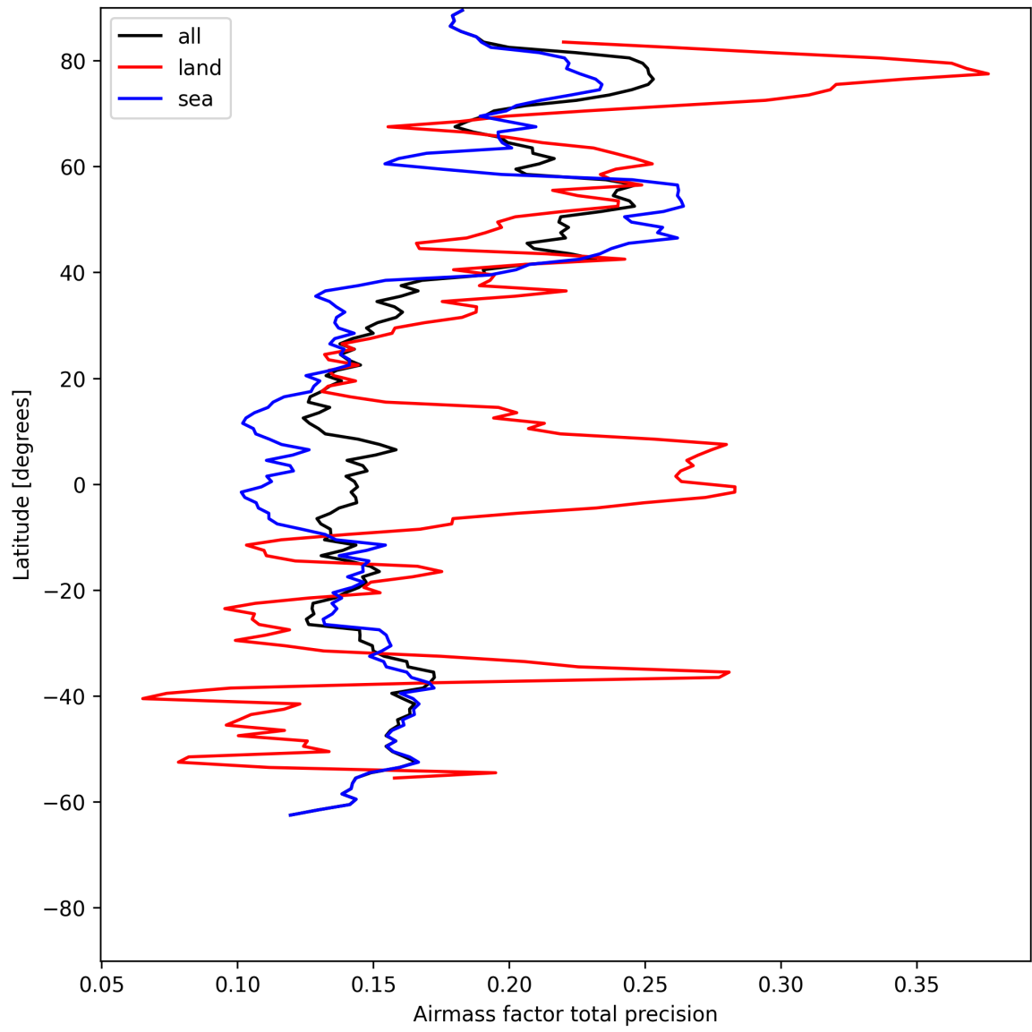
Figure 25: Zonal average of “Airmass factor total precision” for 2025-07-11 to 2025-07-11.
