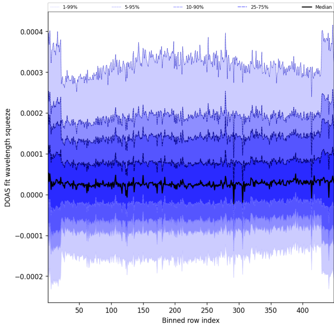
Figure 57: Along track statistics of “DOAS fit wavelength squeeze” for 2025-07-11 to 2025-07-11
