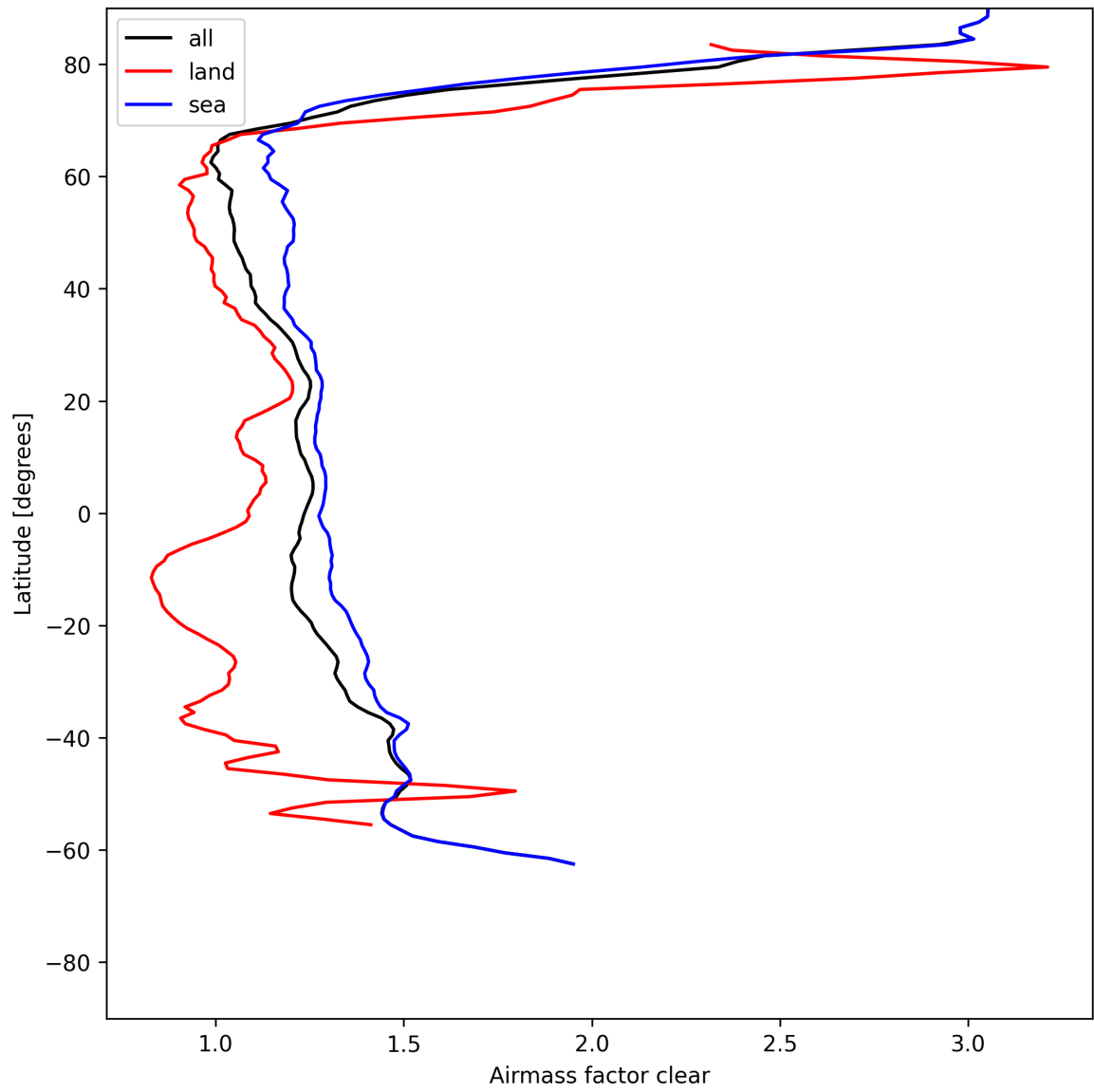
Figure 26: Zonal average of “Airmass factor clear” for 2025-07-11 to 2025-07-11.
