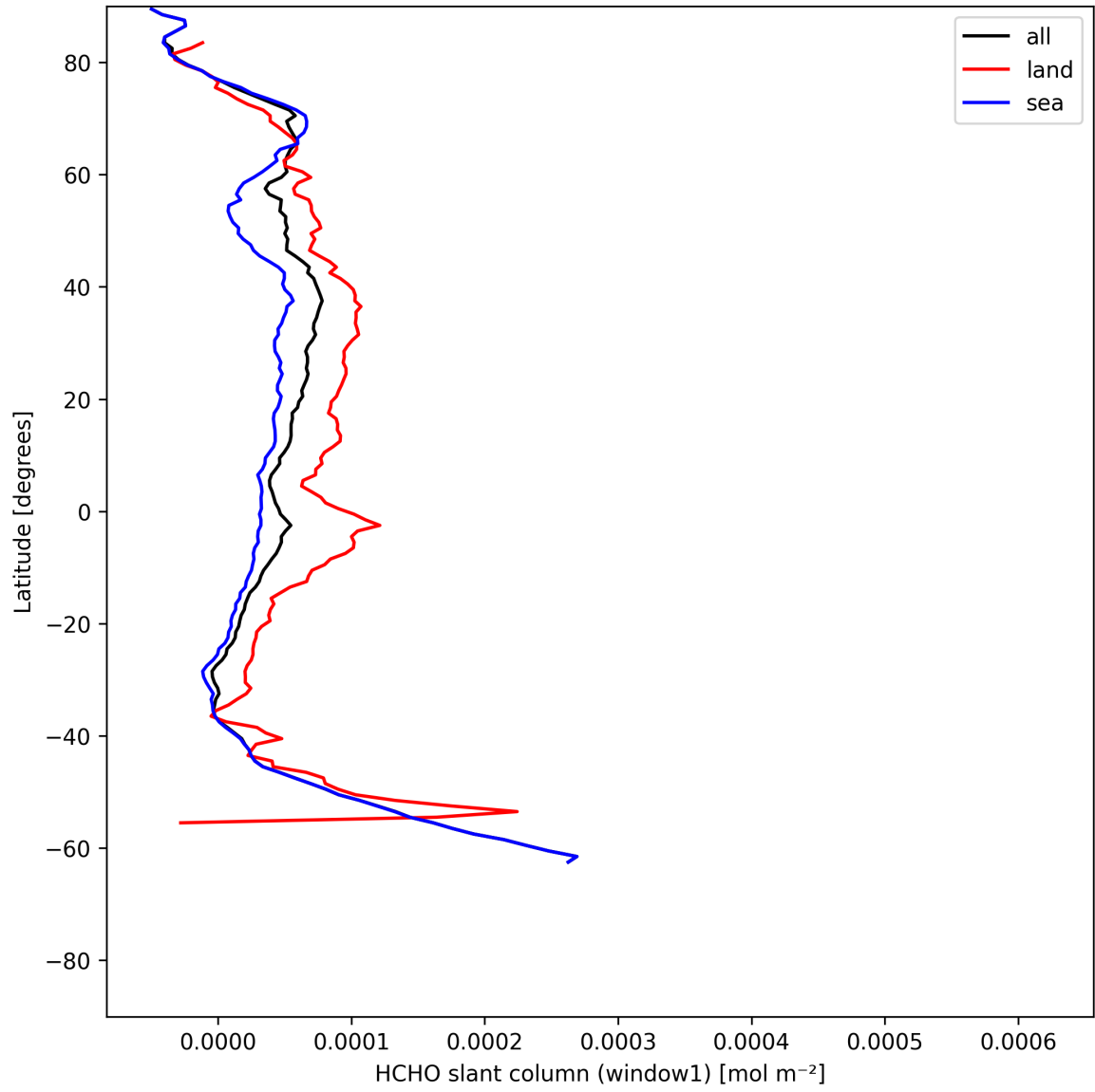
Figure 22: Zonal average of “HCHO slant column (window1)” for 2025-07-11 to 2025-07-11.
