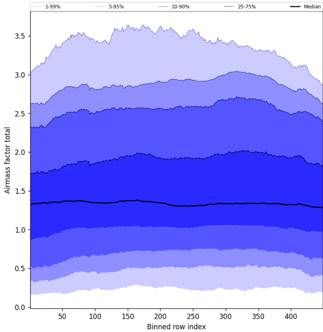
Figure 52: Along track statistics of “Airmass factor total” for 2025-07-11 to 2025-07-11
