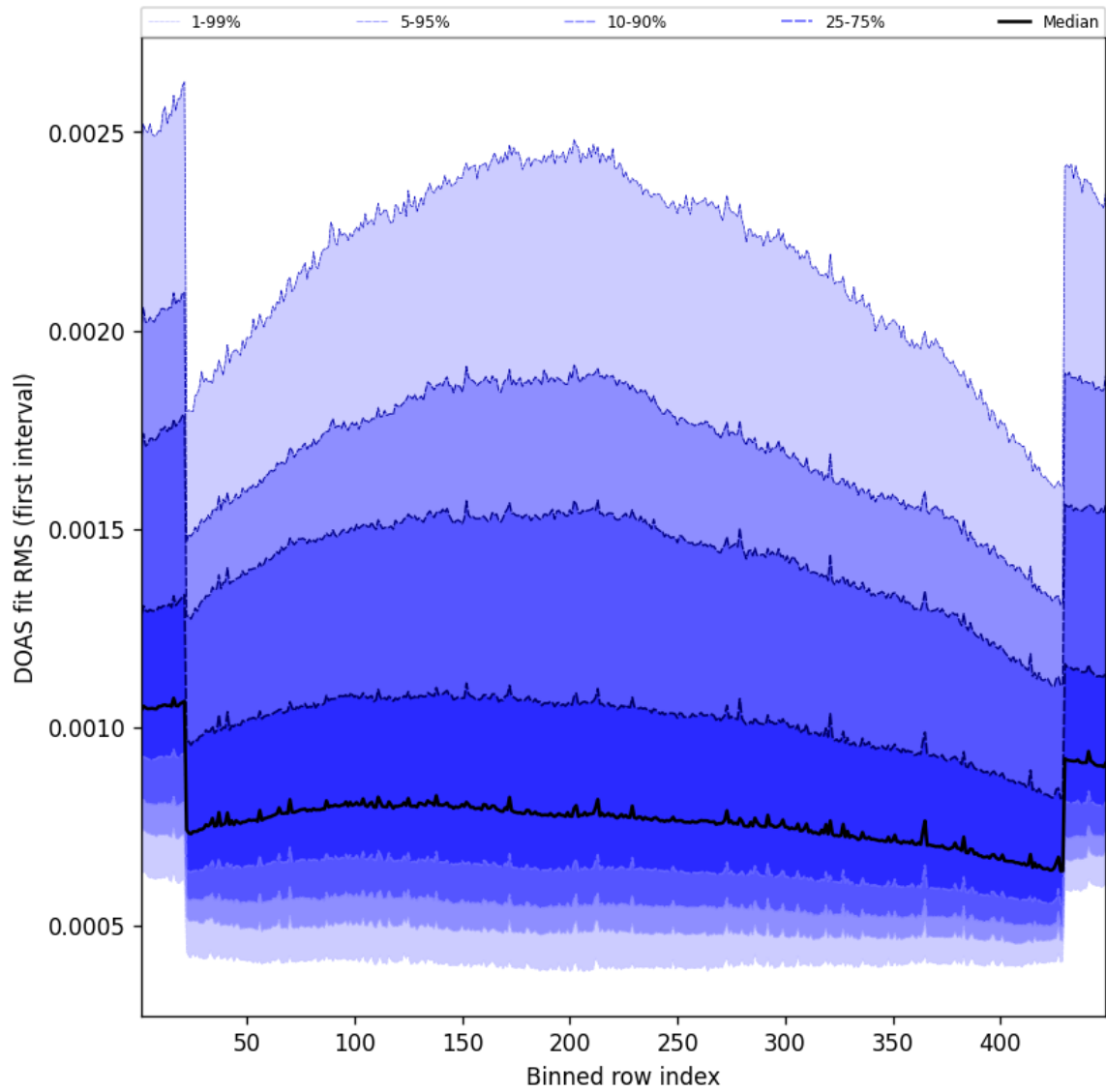
Figure 58: Along track statistics of “DOAS fit RMS (first interval)” for 2025-07-11 to 2025-07-11
