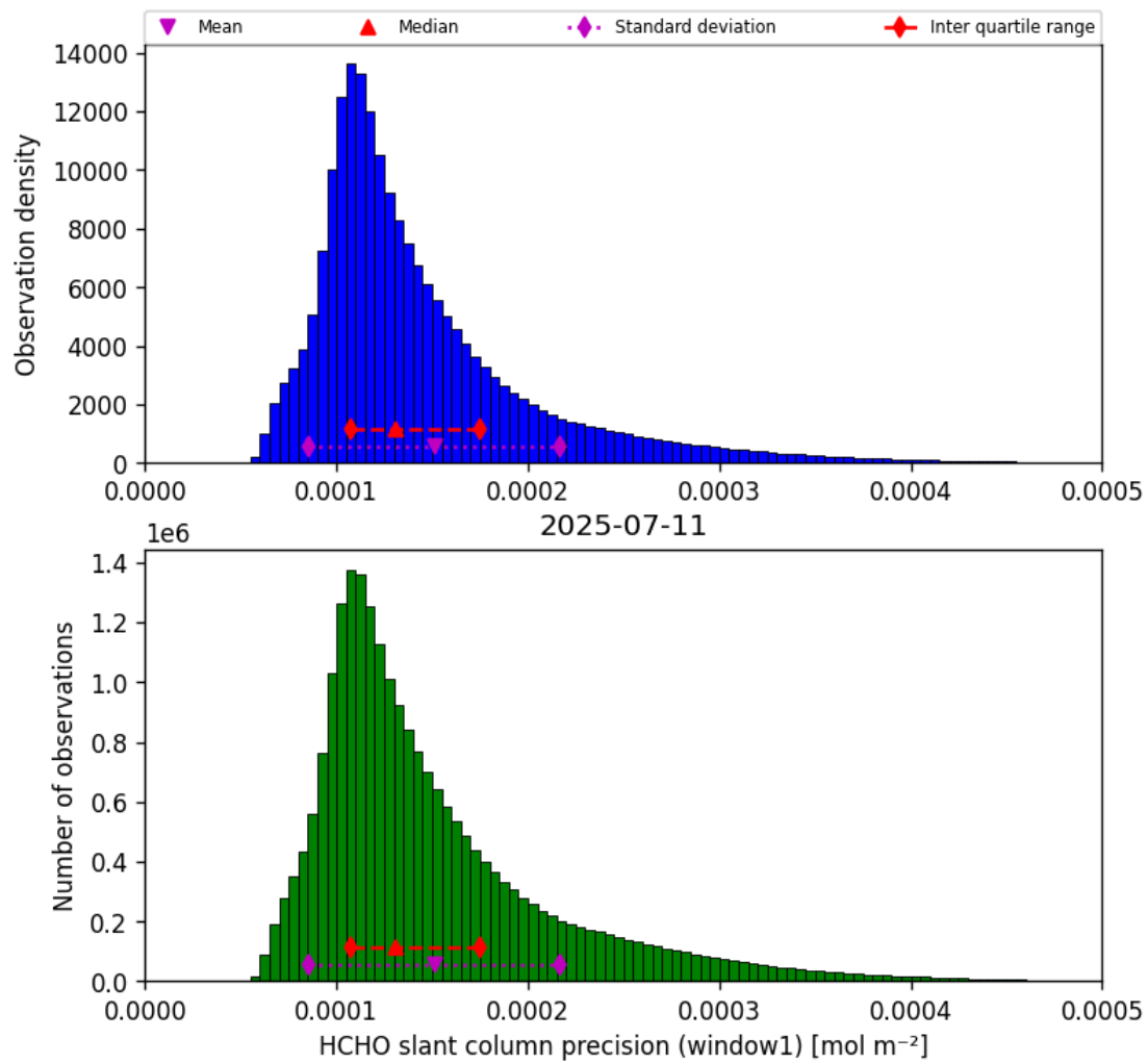
Figure 37: Histogram of “HCHO slant column precision (window1)” for 2025-07-11 to 2025-07-11
