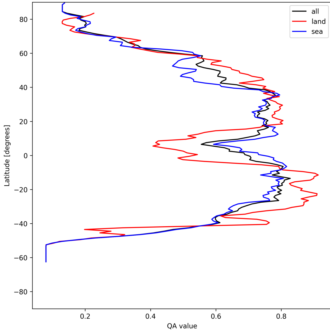
Figure 18: Zonal average of “QA value” for 2025-07-11 to 2025-07-11.
