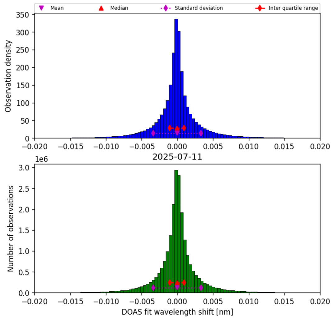
Figure 42: Histogram of “DOAS fit wavelength shift” for 2025-07-11 to 2025-07-11
