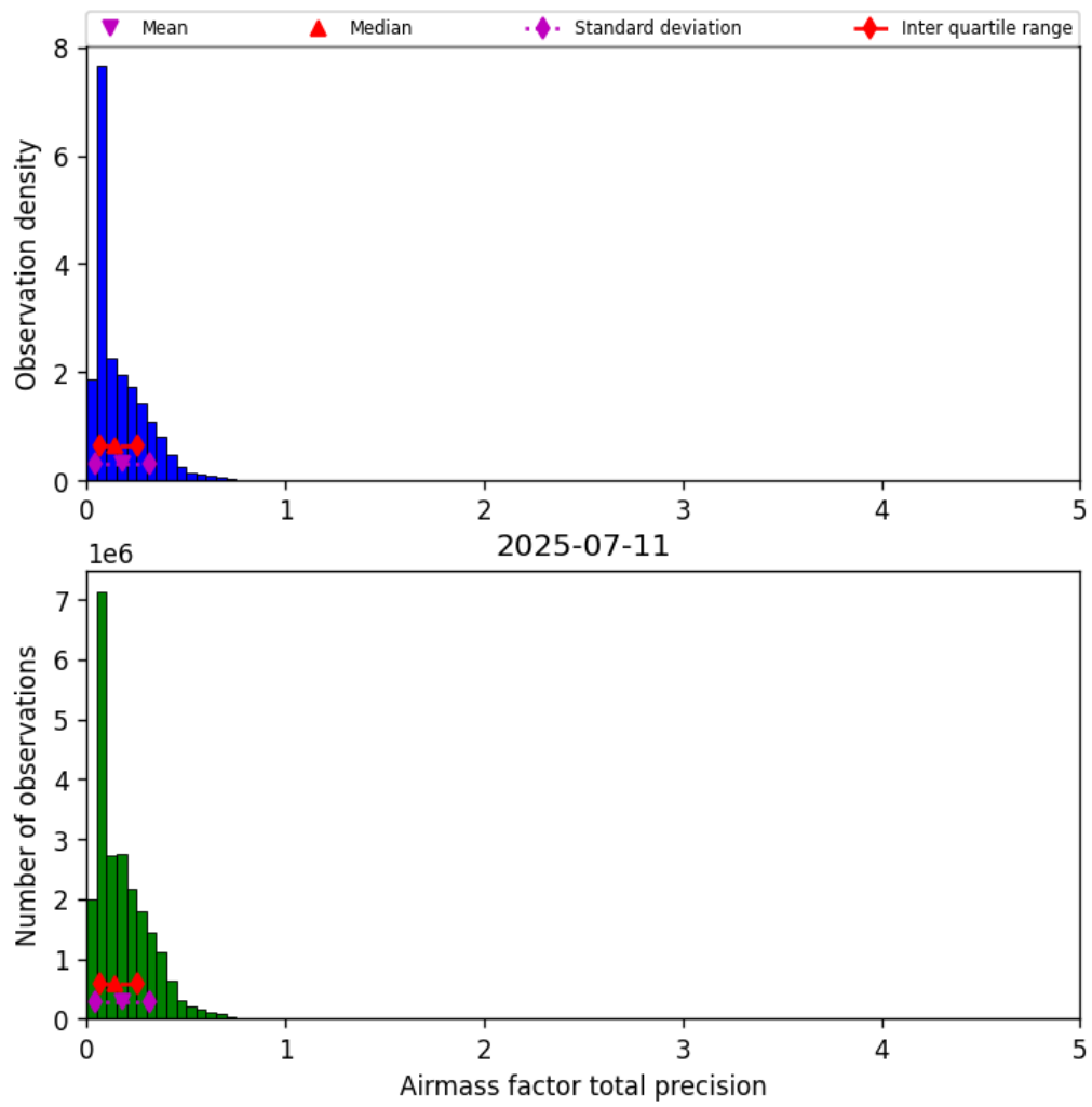
Figure 39: Histogram of “Airmass factor total precision” for 2025-07-11 to 2025-07-11
