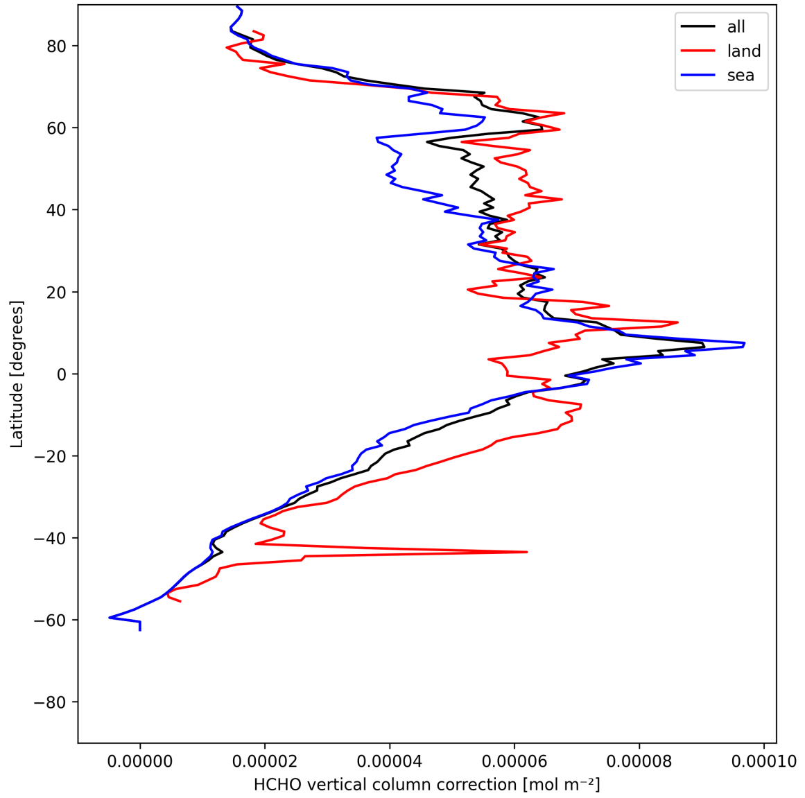
Figure 21: Zonal average of “HCHO vertical column correction” for 2025-07-11 to 2025-07-11.
