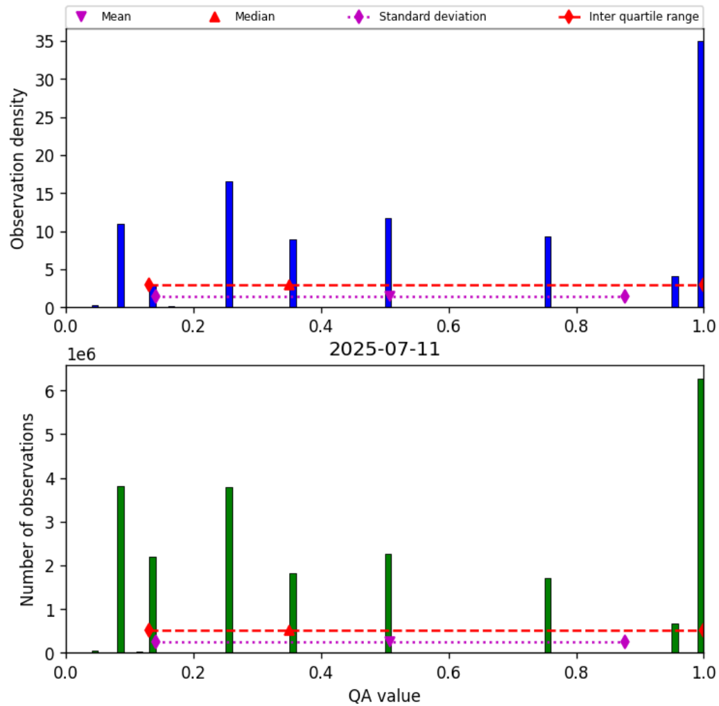
Figure 32: Histogram of “QA value” for 2025-07-11 to 2025-07-11
