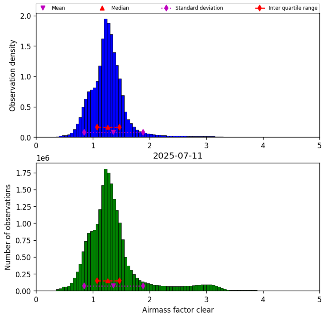
Figure 40: Histogram of “Airmass factor clear” for 2025-07-11 to 2025-07-11
