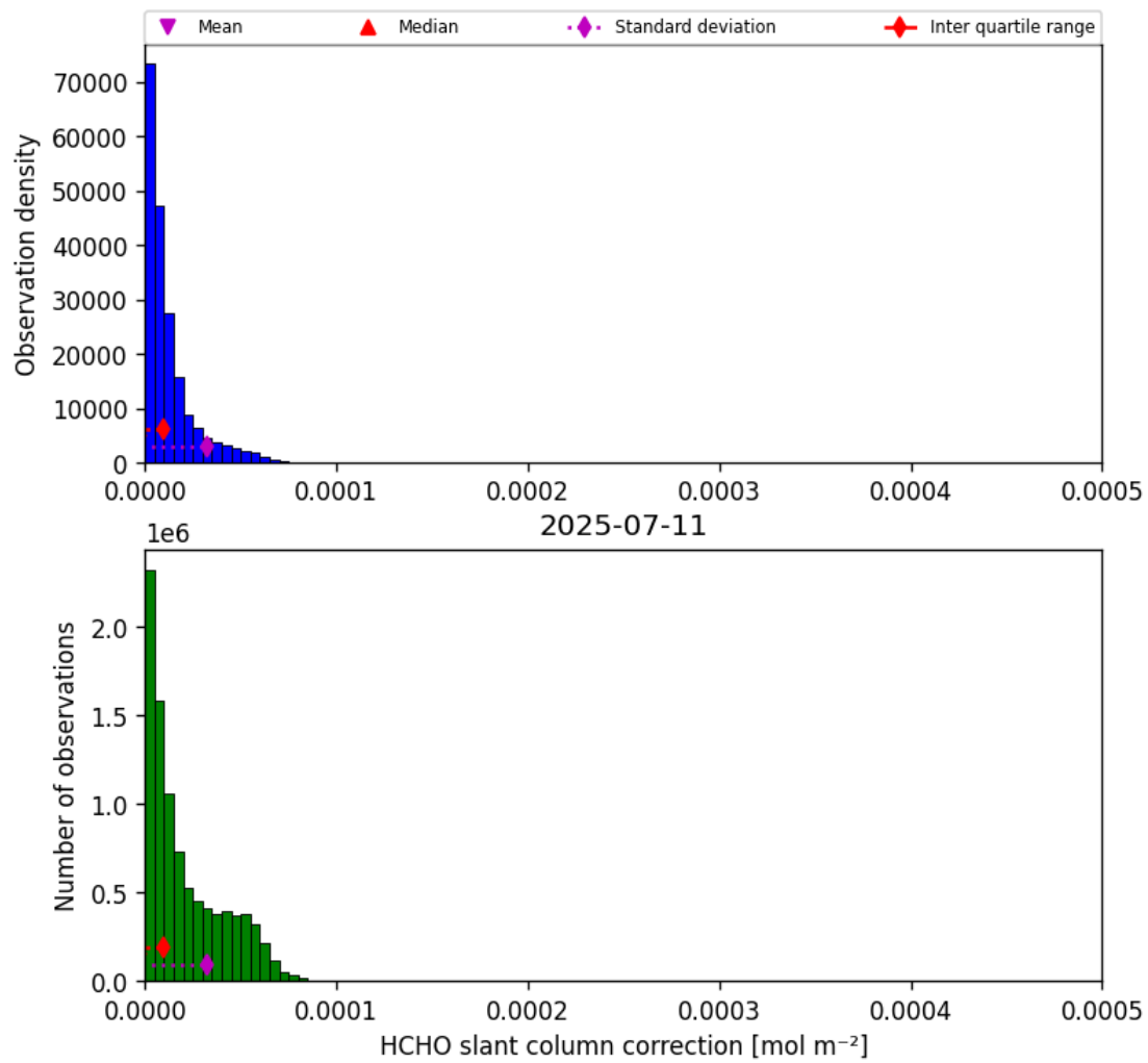
Figure 45: Histogram of “HCHO slant column correction” for 2025-07-11 to 2025-07-11
