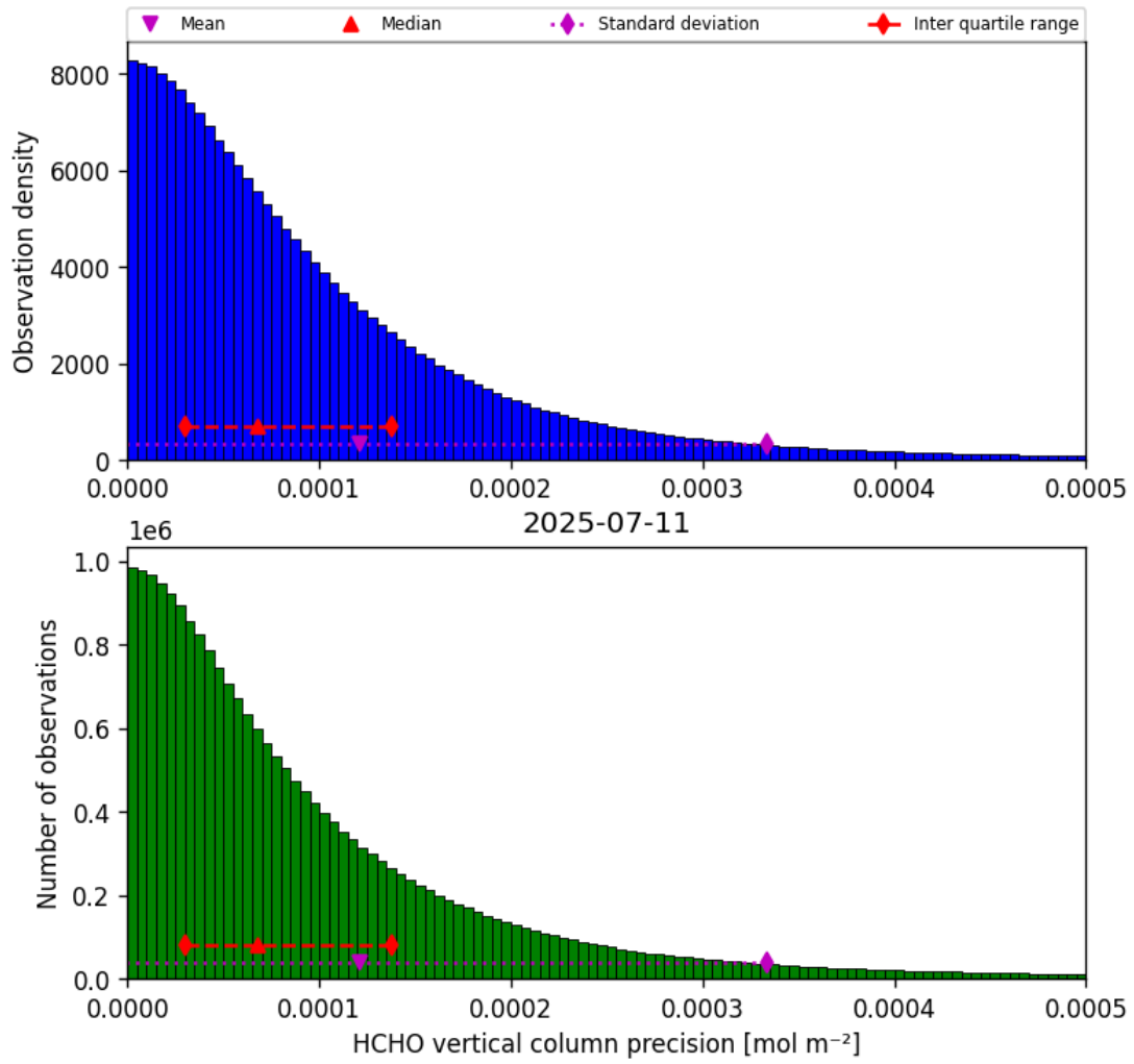
Figure 34: Histogram of “HCHO vertical column precision” for 2025-07-11 to 2025-07-11
