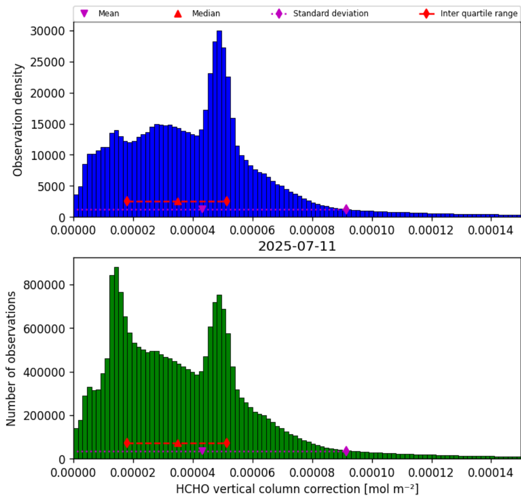
Figure 35: Histogram of “HCHO vertical column correction” for 2025-07-11 to 2025-07-11
