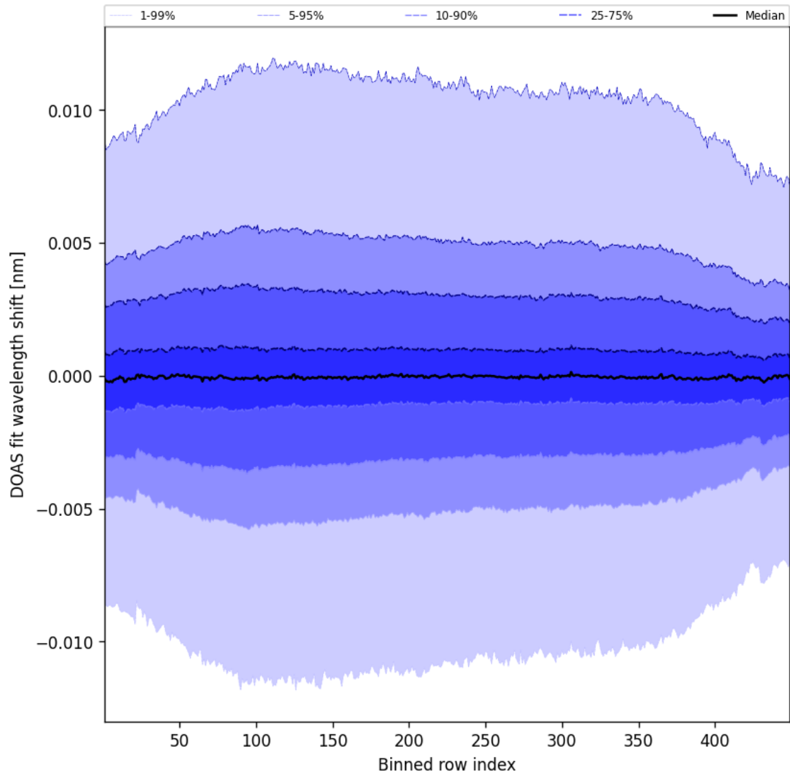
Figure 56: Along track statistics of “DOAS fit wavelength shift” for 2025-07-11 to 2025-07-11
