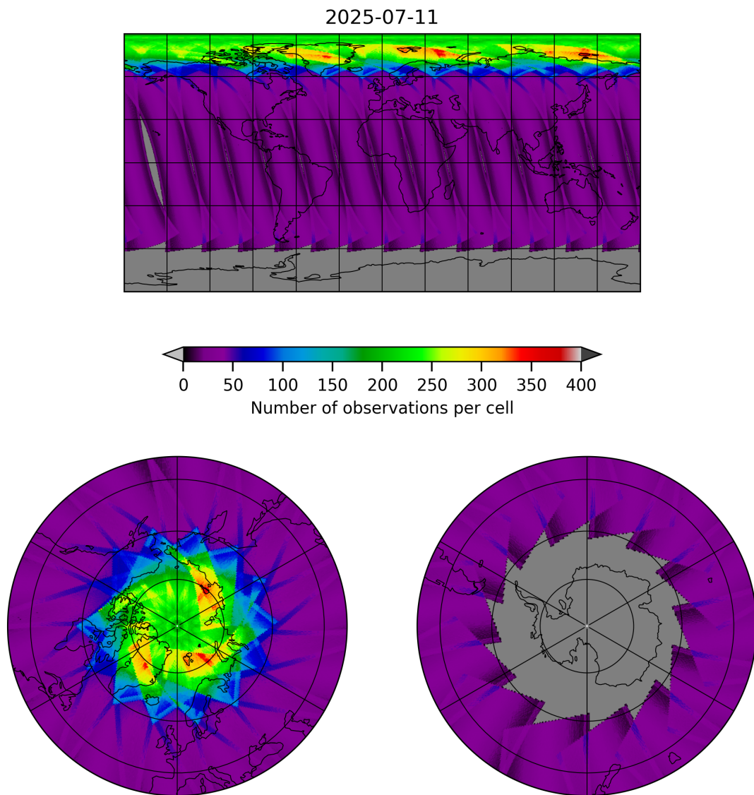
Figure 17: Map of the number of observations for 2025-07-11 to 2025-07-11
