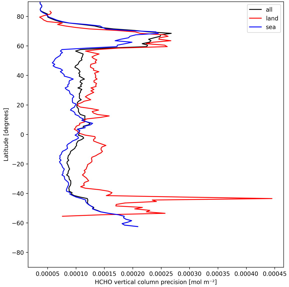
Figure 20: Zonal average of “HCHO vertical column precision” for 2025-07-11 to 2025-07-11.
