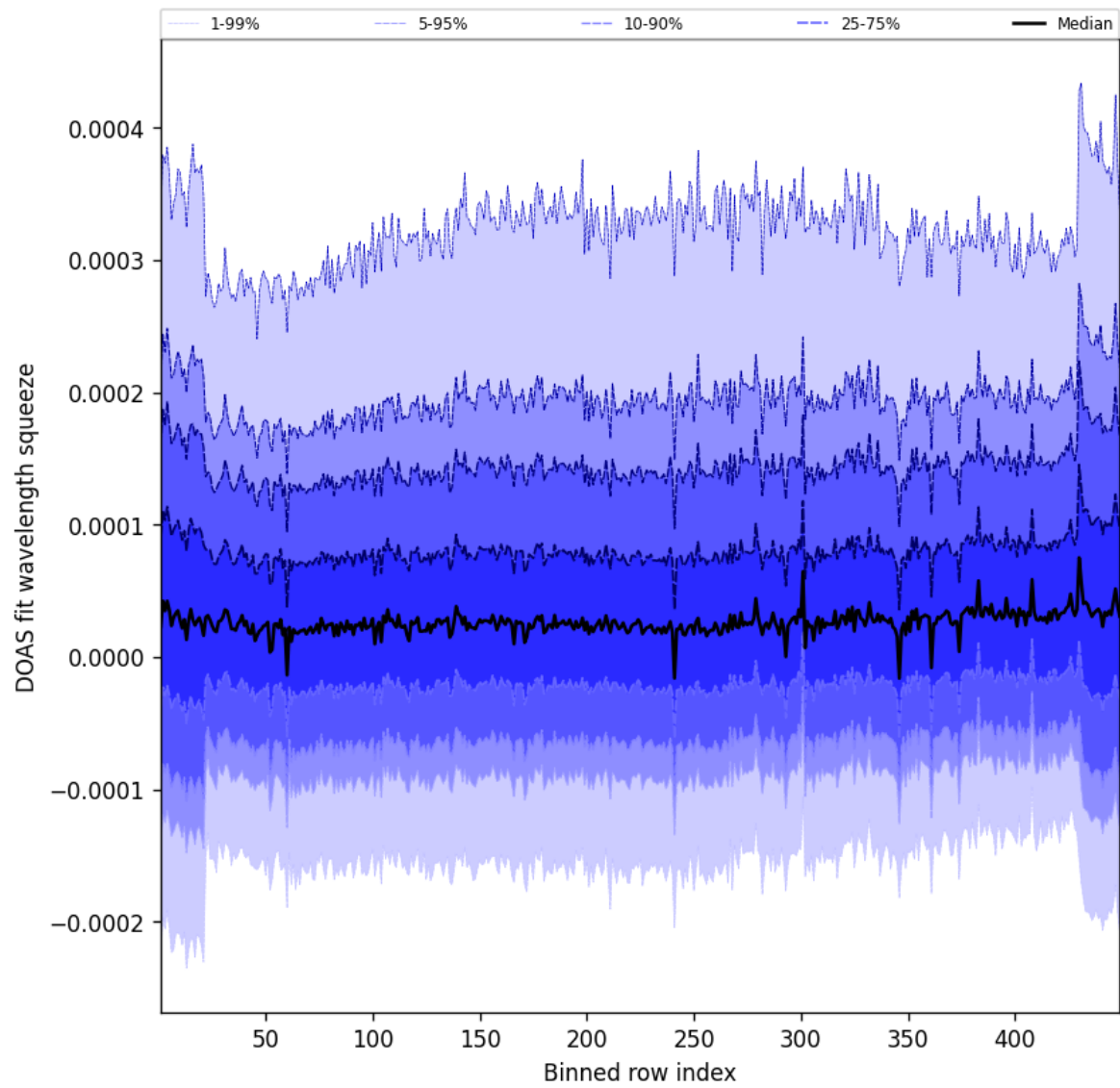
Figure 57: Along track statistics of “DOAS fit wavelength squeeze” for 2025-07-13 to 2025-07-14
