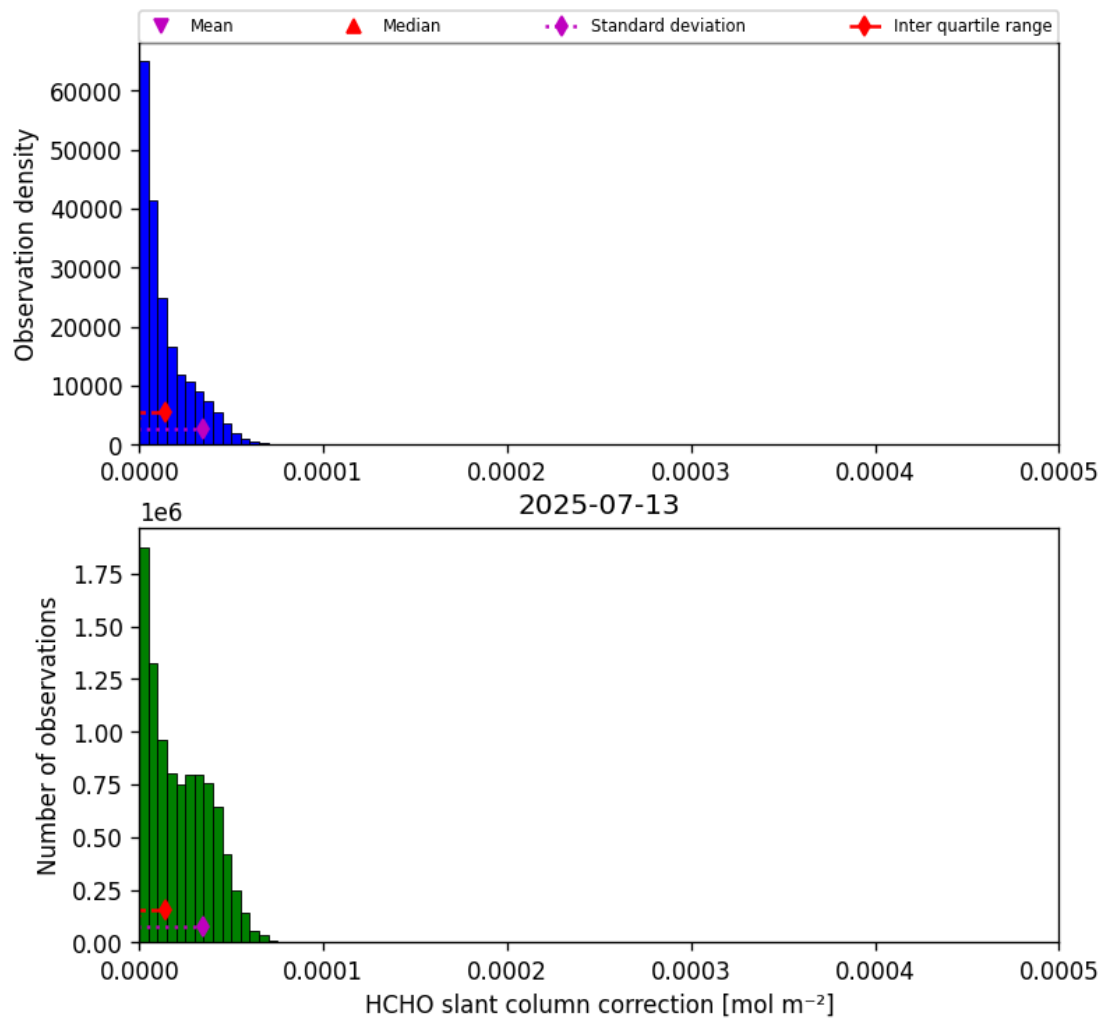
Figure 45: Histogram of “HCHO slant column correction” for 2025-07-13 to 2025-07-14
