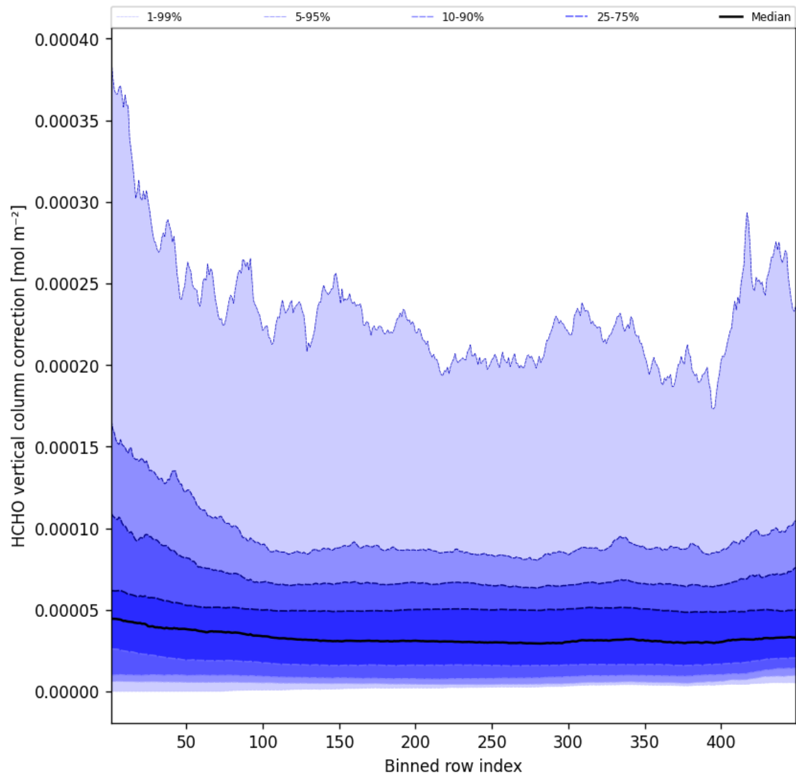
Figure 49: Along track statistics of “HCHO vertical column correction” for 2025-07-13 to 2025-07-14
