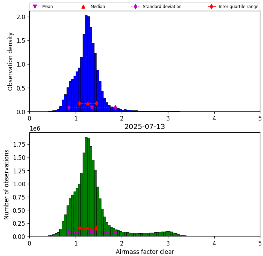
Figure 40: Histogram of “Airmass factor clear” for 2025-07-13 to 2025-07-14
