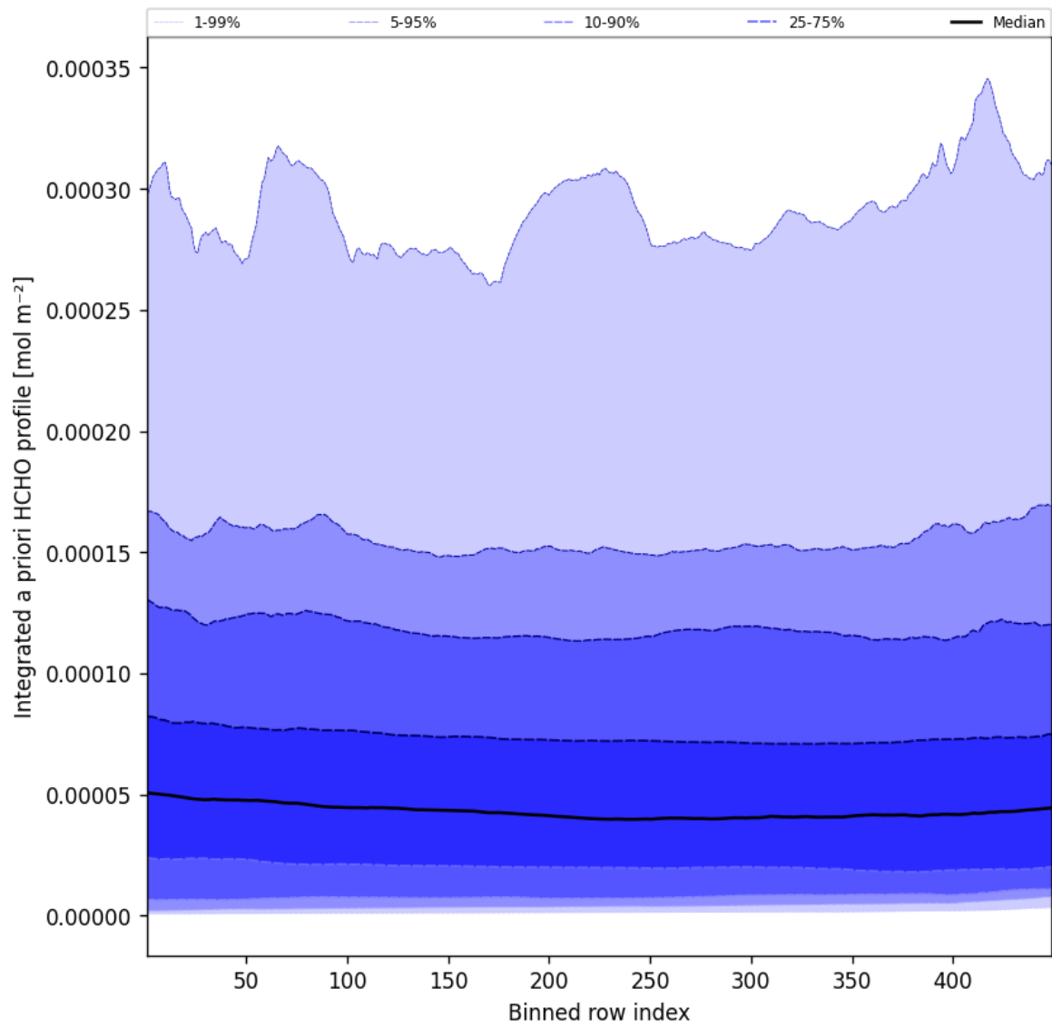
Figure 55: Along track statistics of "Integrated a priori HCHO profile" for 2025-07-13 to 2025-07-14
