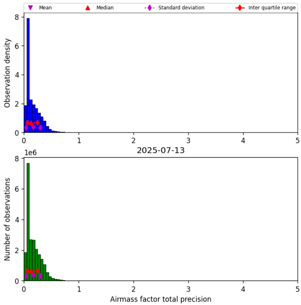
Figure 39: Histogram of “Airmass factor total precision” for 2025-07-13 to 2025-07-14
