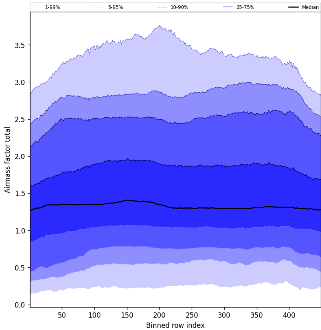
Figure 52: Along track statistics of “Airmass factor total” for 2025-07-13 to 2025-07-14
