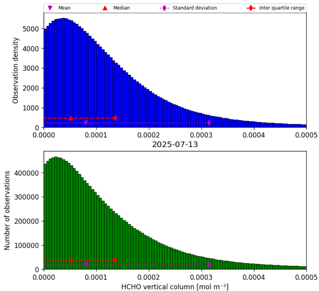
Figure 33: Histogram of “HCHO vertical column” for 2025-07-13 to 2025-07-14
