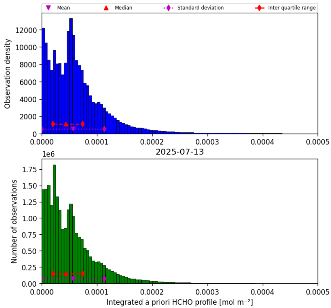
Figure 41: Histogram of “Integrated a priori HCHO profile” for 2025-07-13 to 2025-07-14
