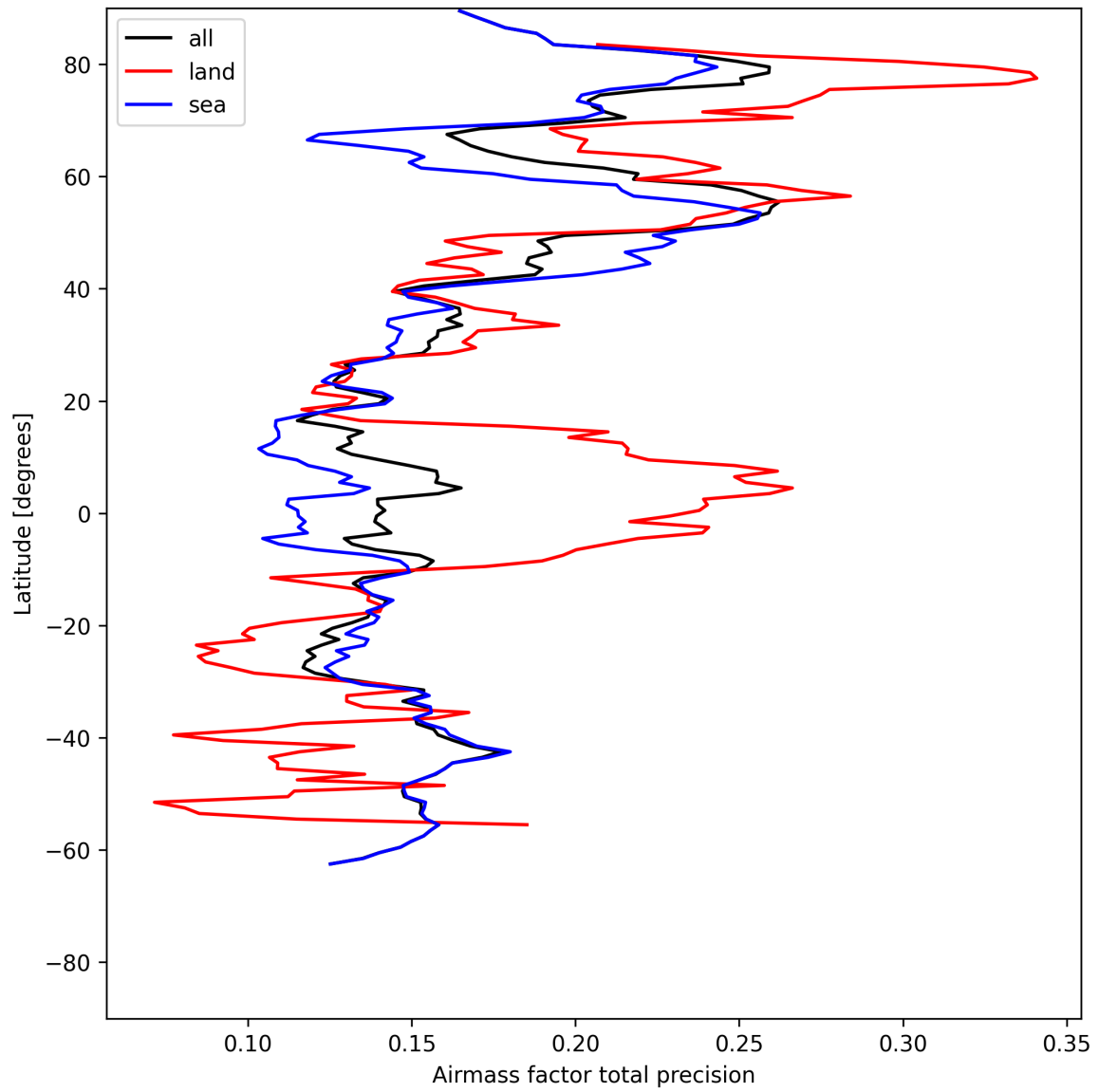
Figure 25: Zonal average of “Airmass factor total precision” for 2025-07-13 to 2025-07-14.
