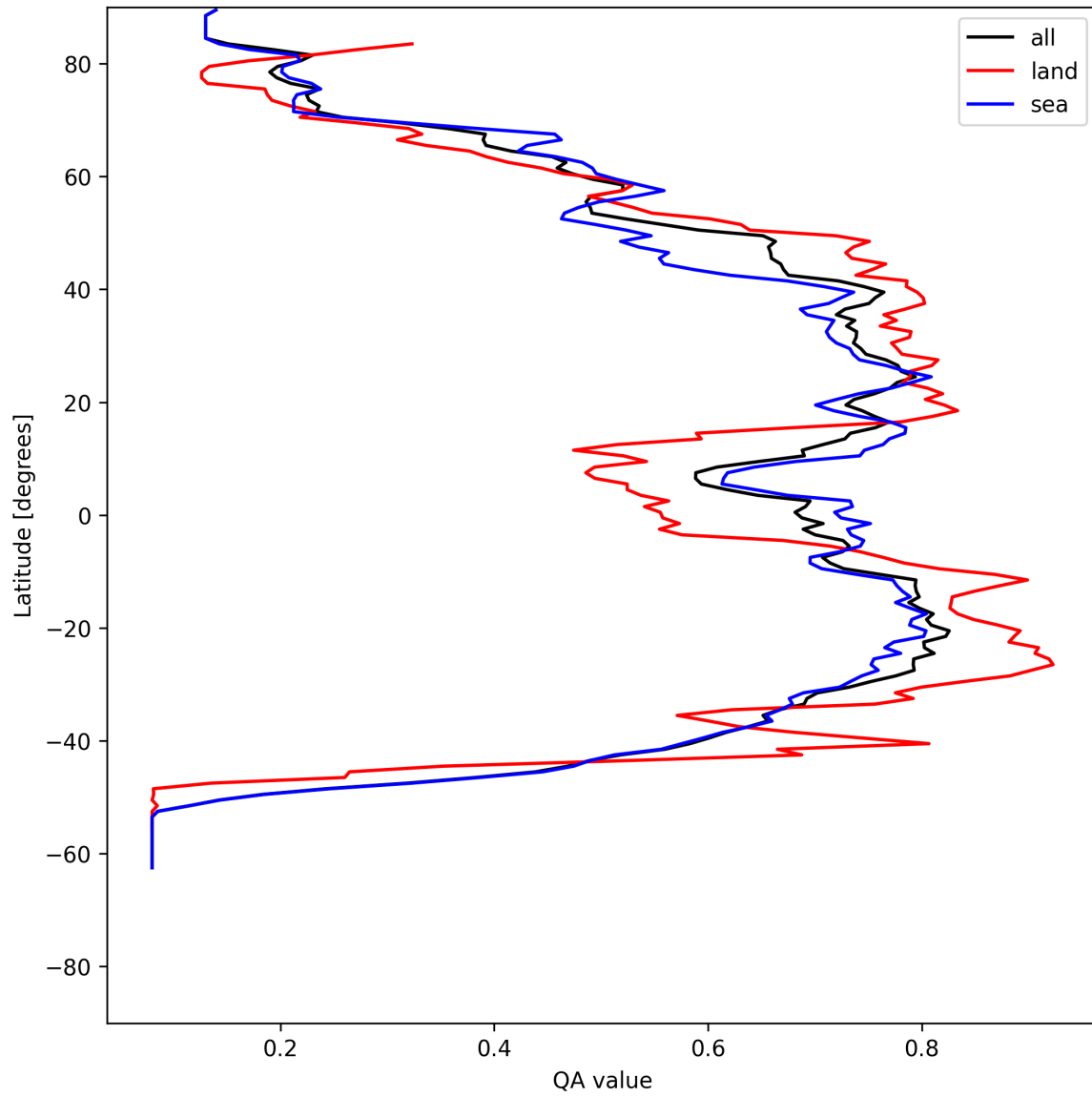
Figure 18: Zonal average of “QA value” for 2025-07-13 to 2025-07-14.
