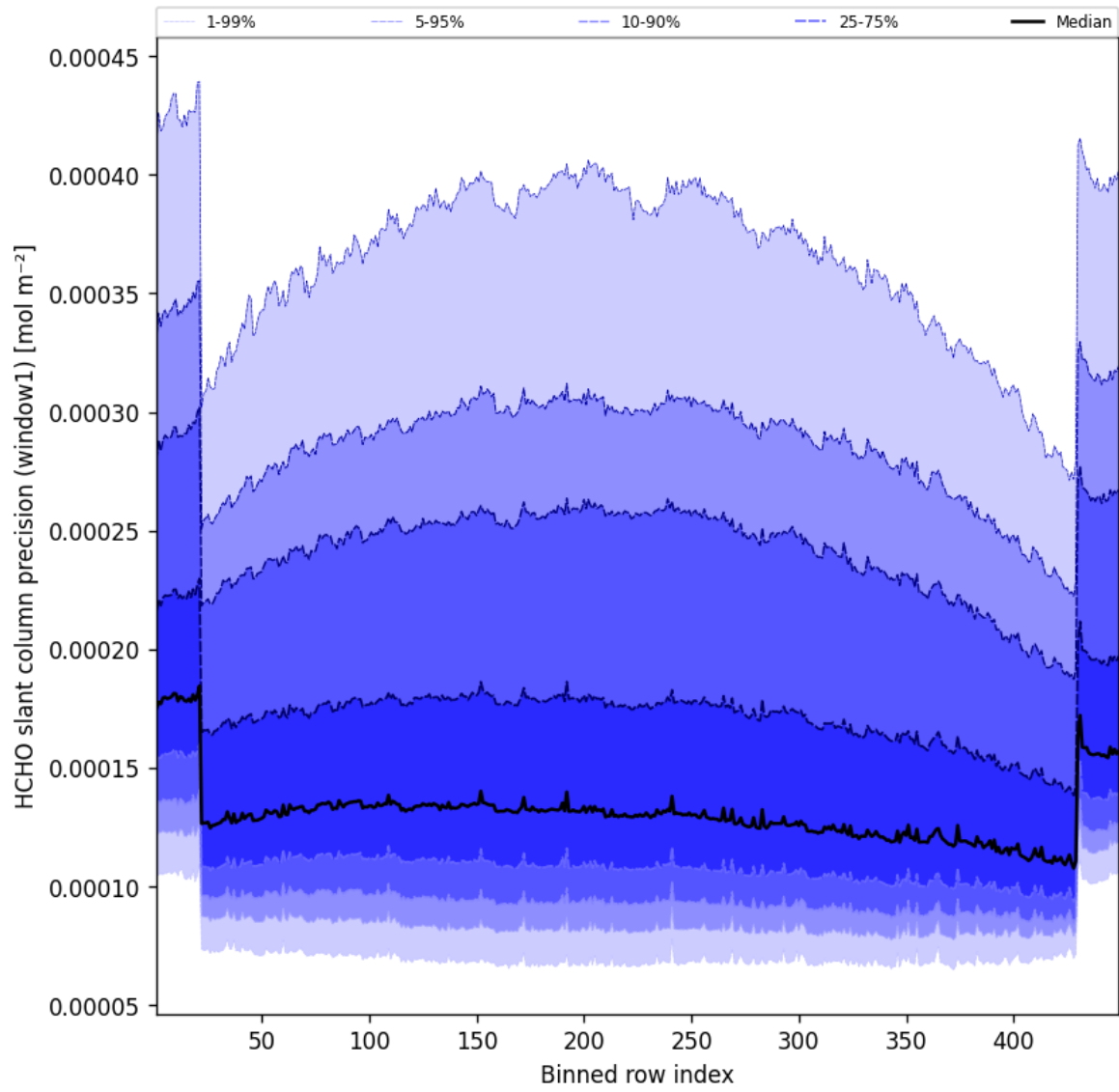
Figure 51: Along track statistics of “HCHO slant column precision (window1)” for 2025-07-13 to 2025-07-14
