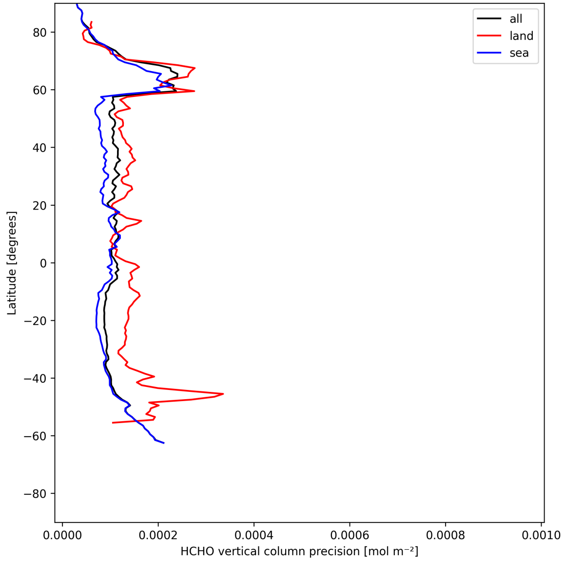
Figure 20: Zonal average of “HCHO vertical column precision” for 2025-07-13 to 2025-07-14.
