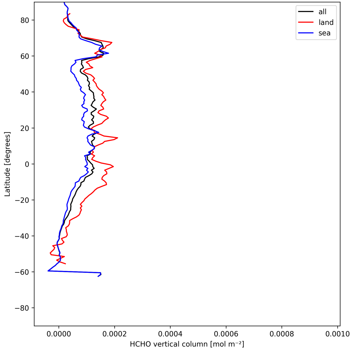
Figure 19: Zonal average of “HCHO vertical column” for 2025-07-13 to 2025-07-14.
