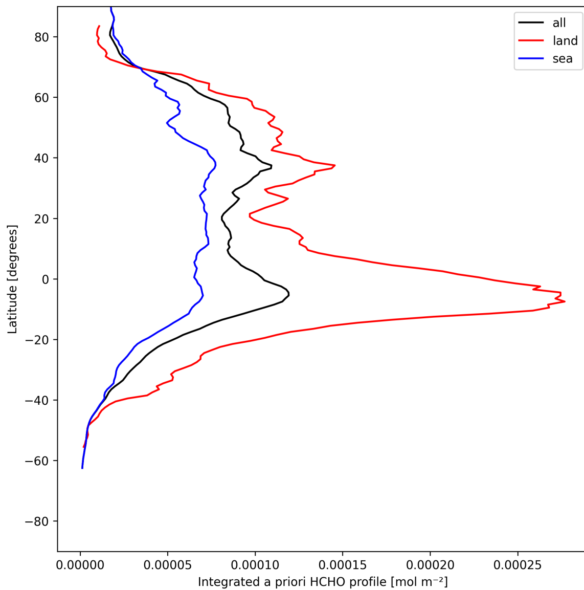
Figure 27: Zonal average of “Integrated a priori HCHO profile” for 2025-07-13 to 2025-07-14.
