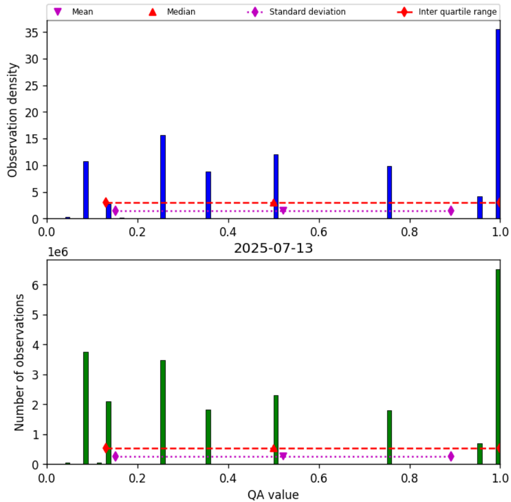
Figure 32: Histogram of “QA value” for 2025-07-13 to 2025-07-14
