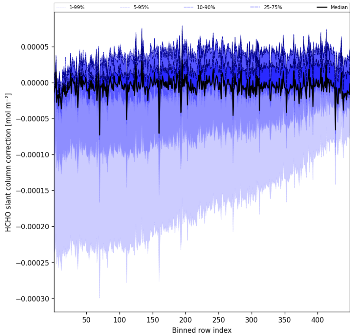
Figure 59: Along track statistics of “HCHO slant column correction” for 2025-07-13 to 2025-07-14
