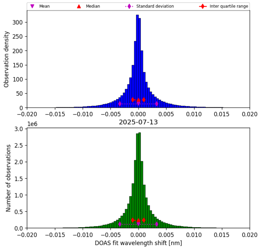
Figure 42: Histogram of “DOAS fit wavelength shift” for 2025-07-13 to 2025-07-14
