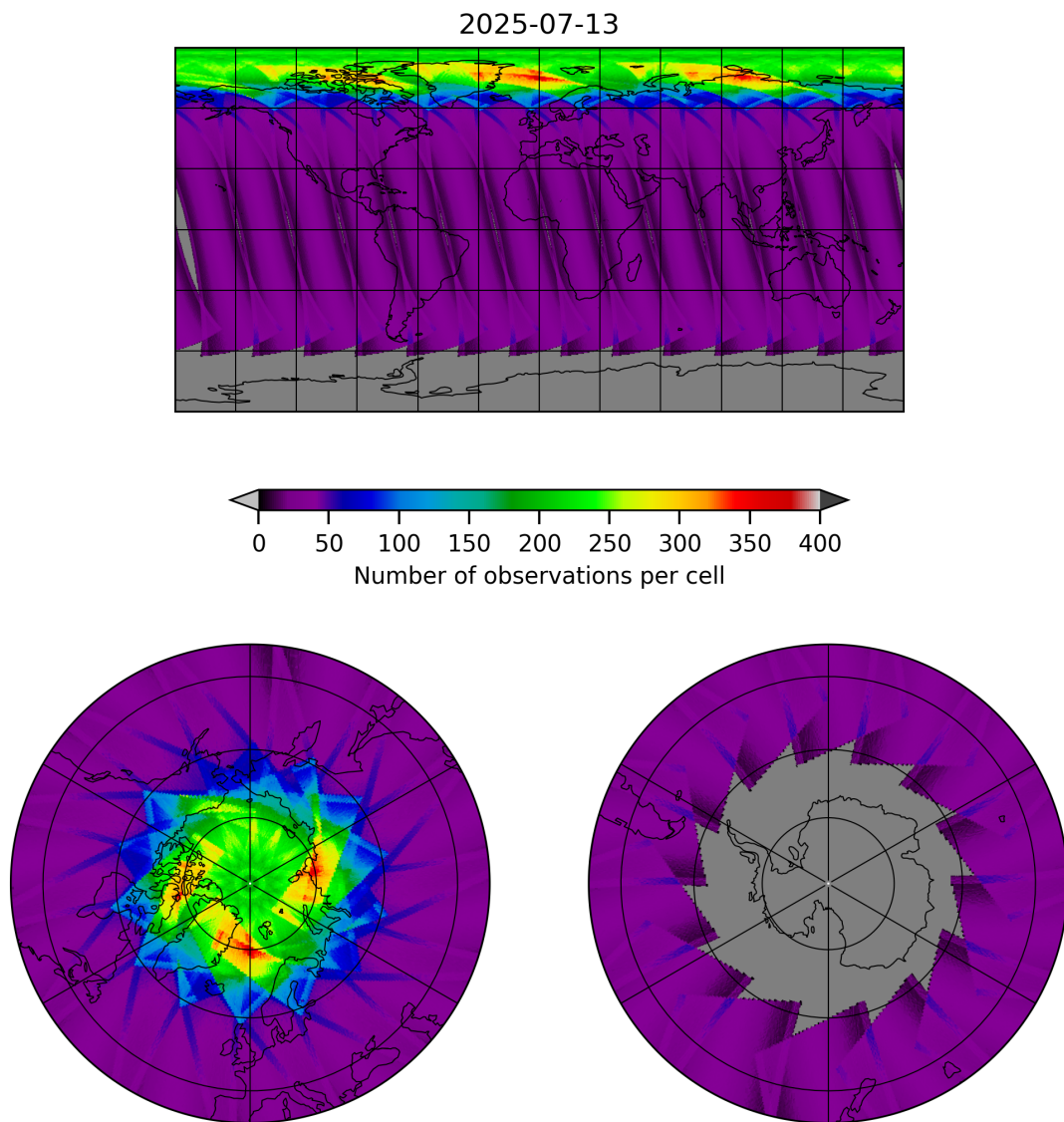
Figure 17: Map of the number of observations for 2025-07-13 to 2025-07-14
