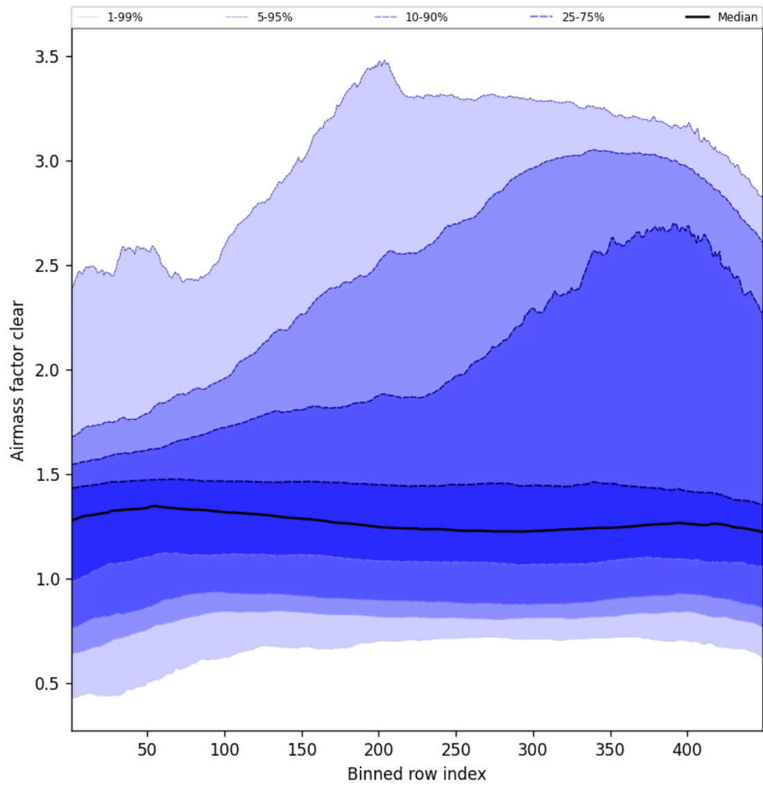
Figure 54: Along track statistics of “Airmass factor clear” for 2025-07-13 to 2025-07-14
