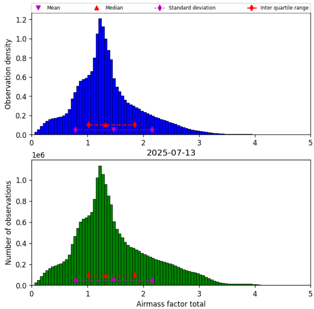
Figure 38: Histogram of “Airmass factor total” for 2025-07-13 to 2025-07-14
