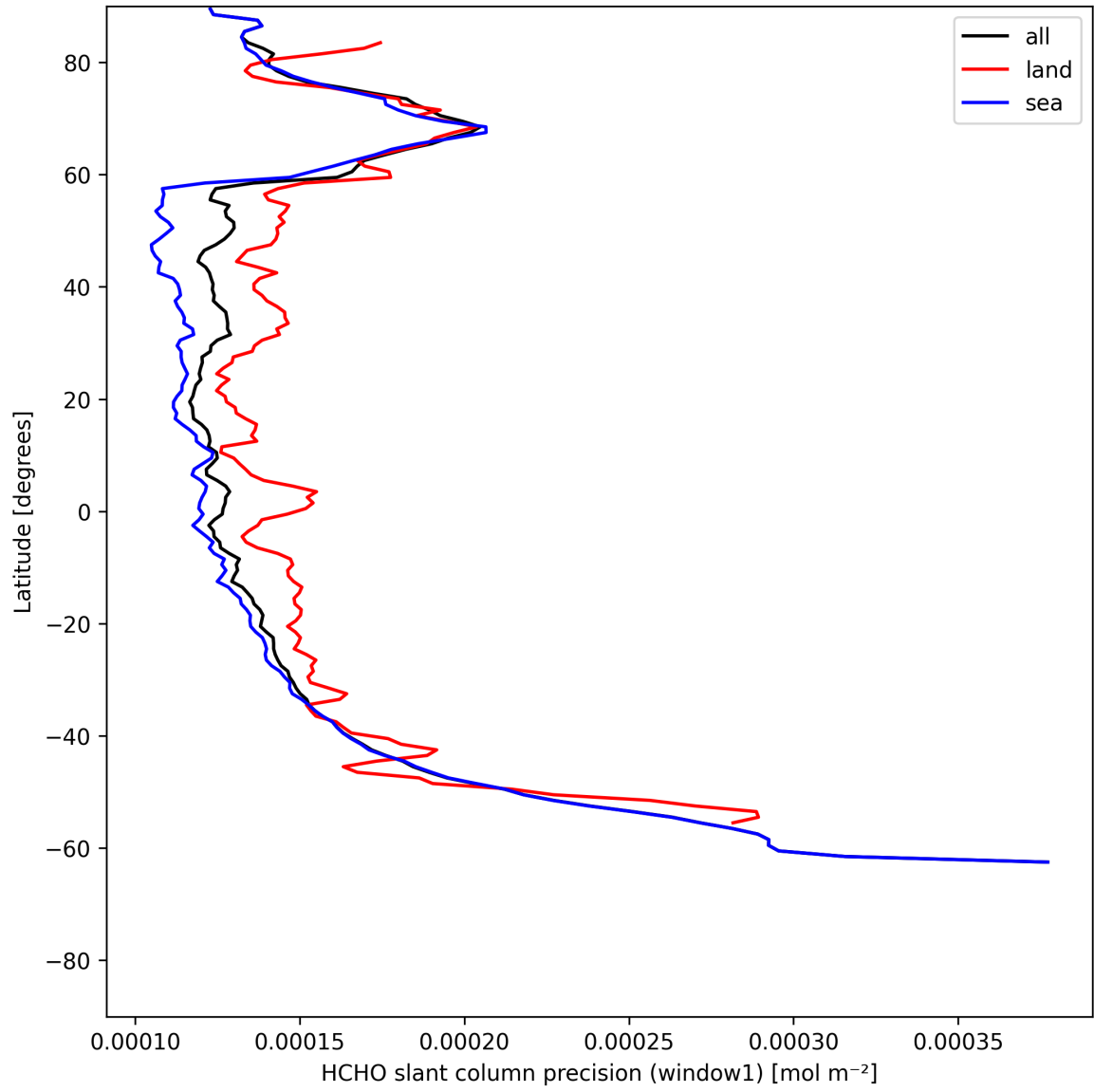
Figure 23: Zonal average of “HCHO slant column precision (window1)” for 2025-07-13 to 2025-07-14.
