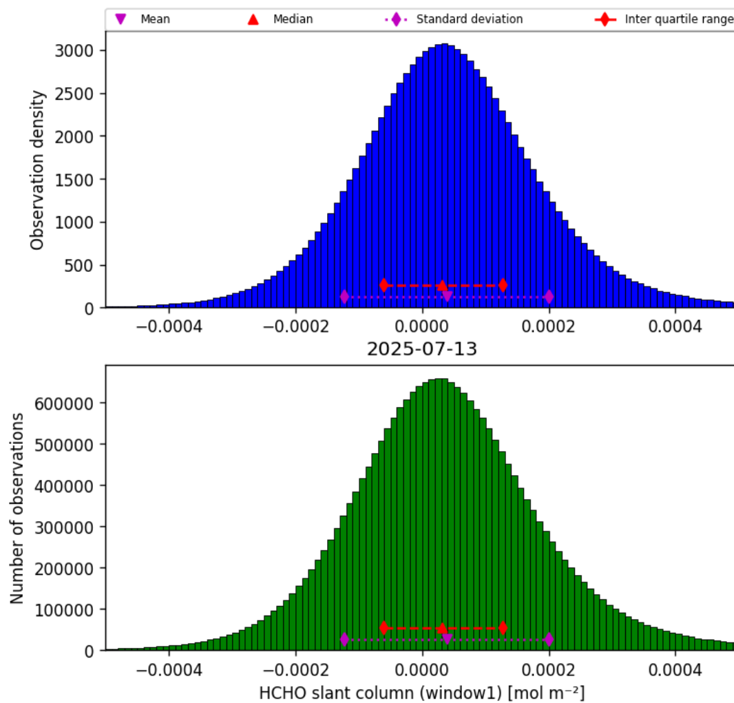
Figure 36: Histogram of “HCHO slant column (window1)” for 2025-07-13 to 2025-07-14
