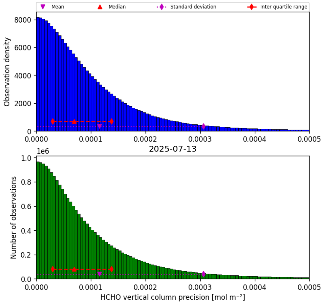
Figure 34: Histogram of “HCHO vertical column precision” for 2025-07-13 to 2025-07-14
