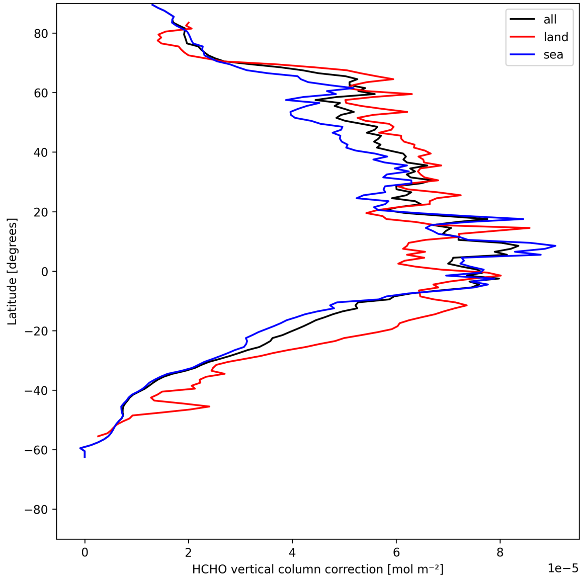
Figure 21: Zonal average of “HCHO vertical column correction” for 2025-07-13 to 2025-07-14.
