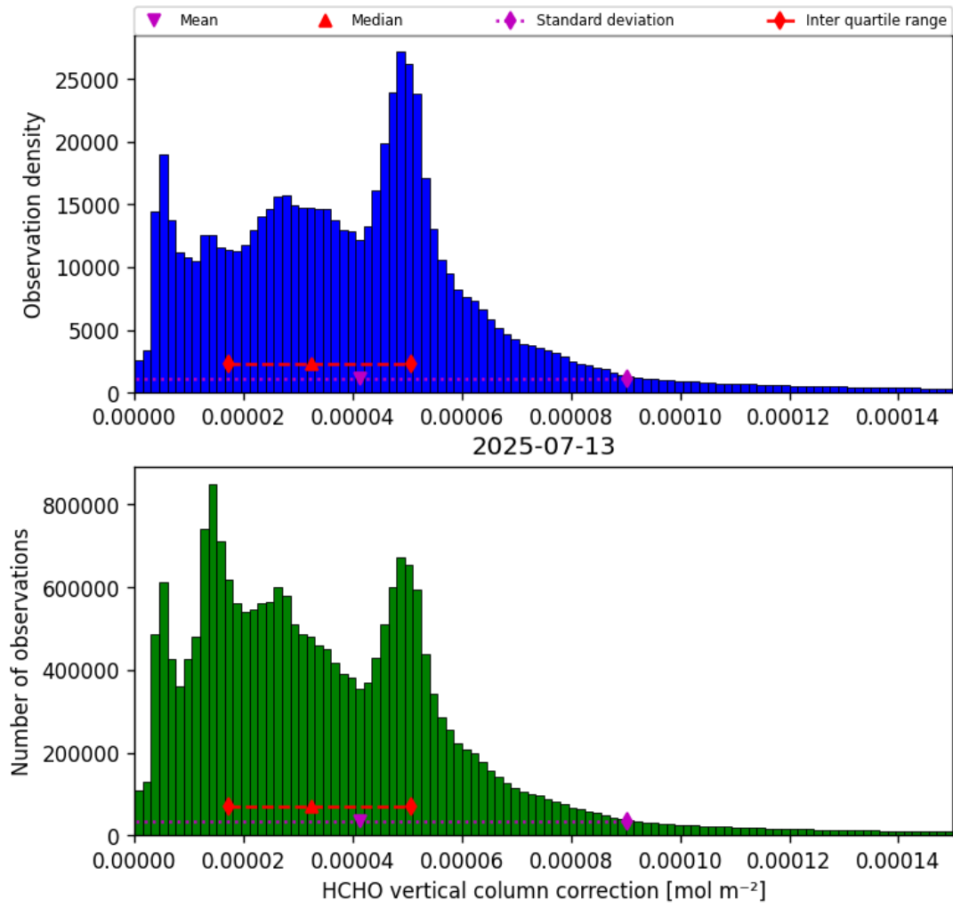
Figure 35: Histogram of “HCHO vertical column correction” for 2025-07-13 to 2025-07-14
