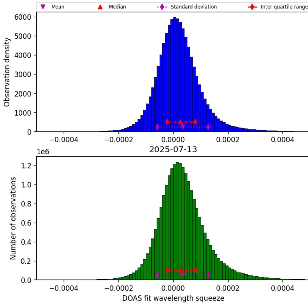
Figure 43: Histogram of “DOAS fit wavelength squeeze” for 2025-07-13 to 2025-07-14
