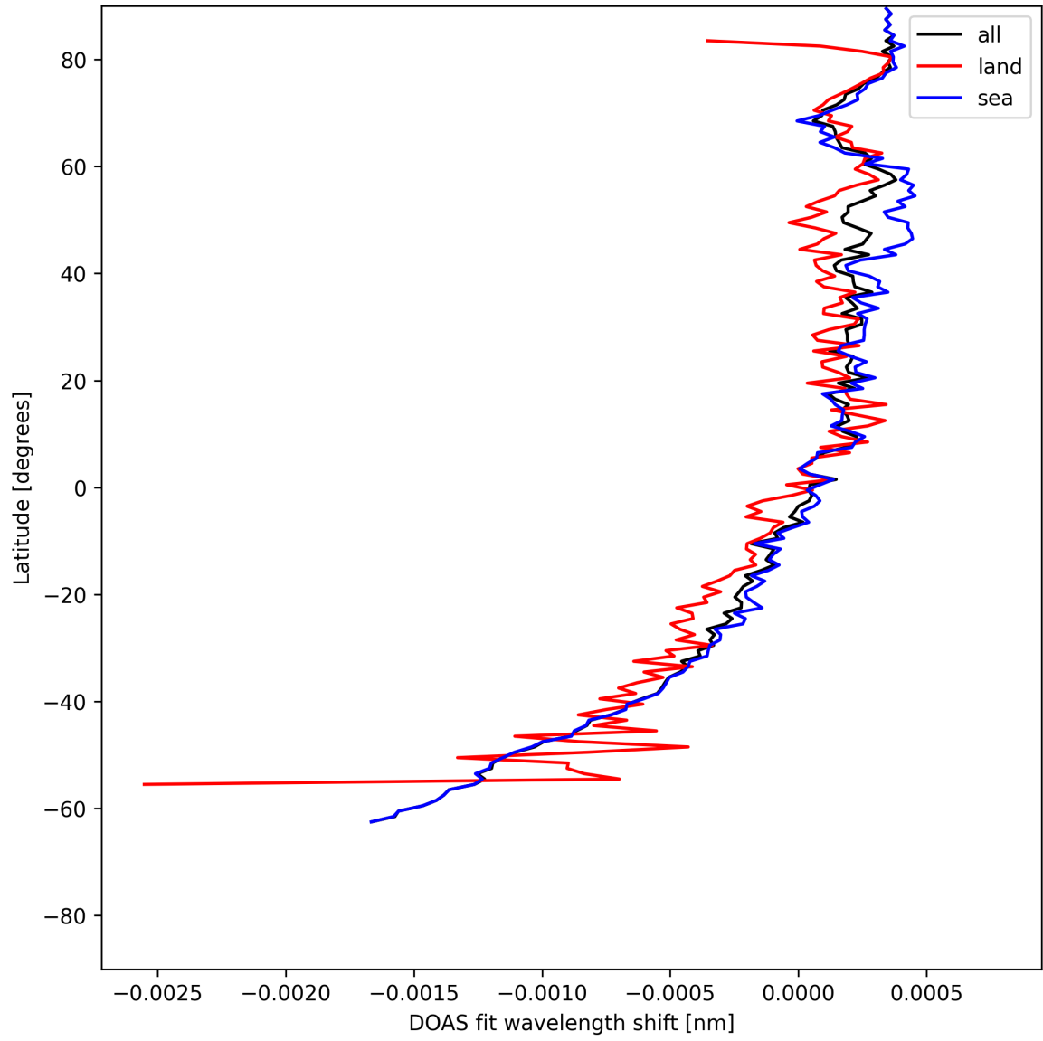
Figure 28: Zonal average of “DOAS fit wavelength shift” for 2025-07-13 to 2025-07-14.
