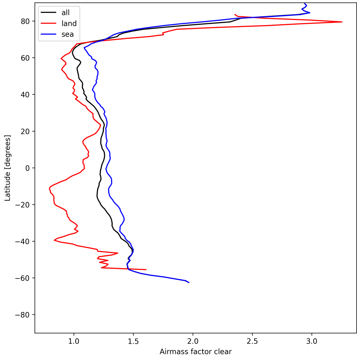
Figure 26: Zonal average of “Airmass factor clear” for 2025-07-13 to 2025-07-14.
