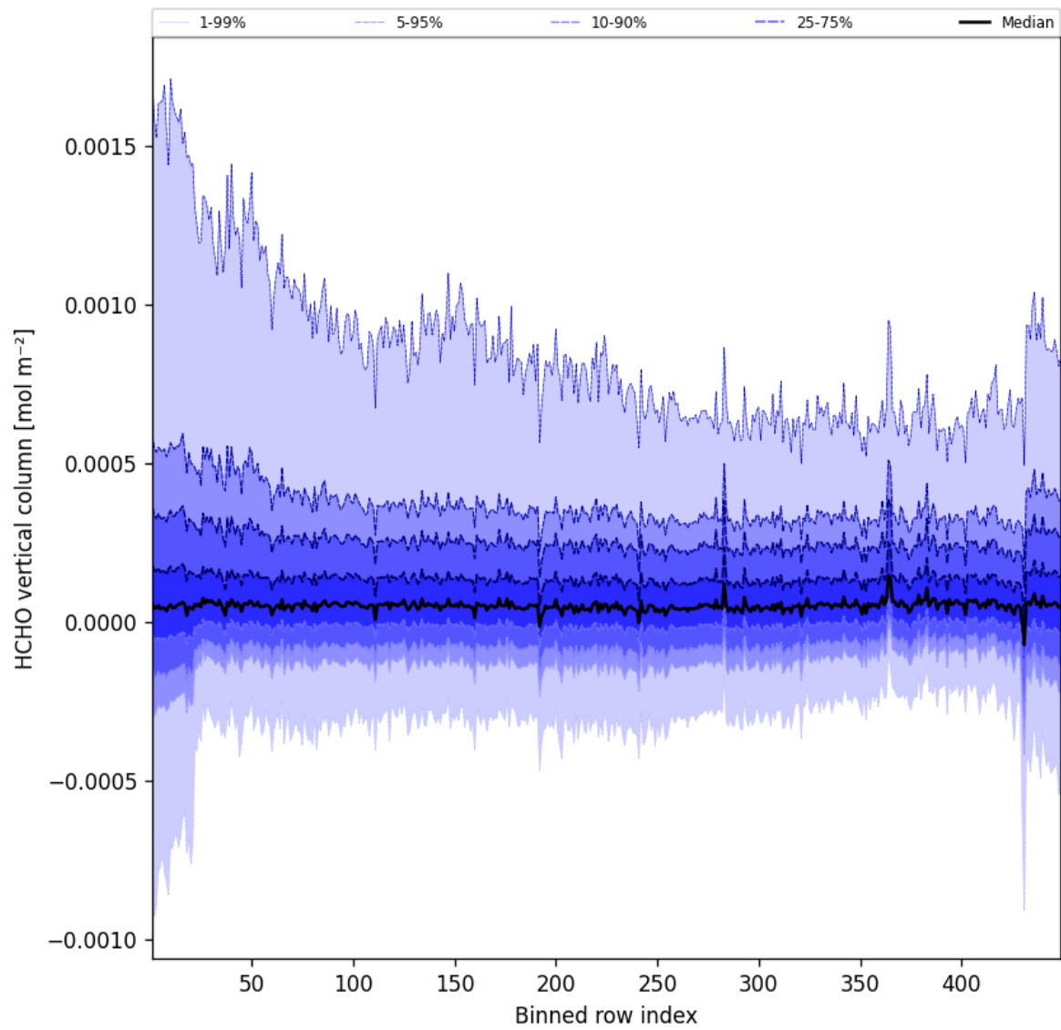
Figure 47: Along track statistics of “HCHO vertical column” for 2025-07-13 to 2025-07-14
