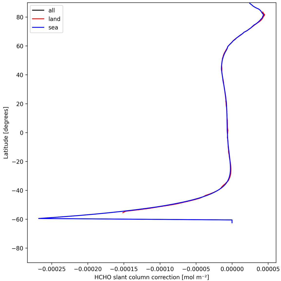
Figure 31: Zonal average of “HCHO slant column correction” for 2025-07-13 to 2025-07-14.
