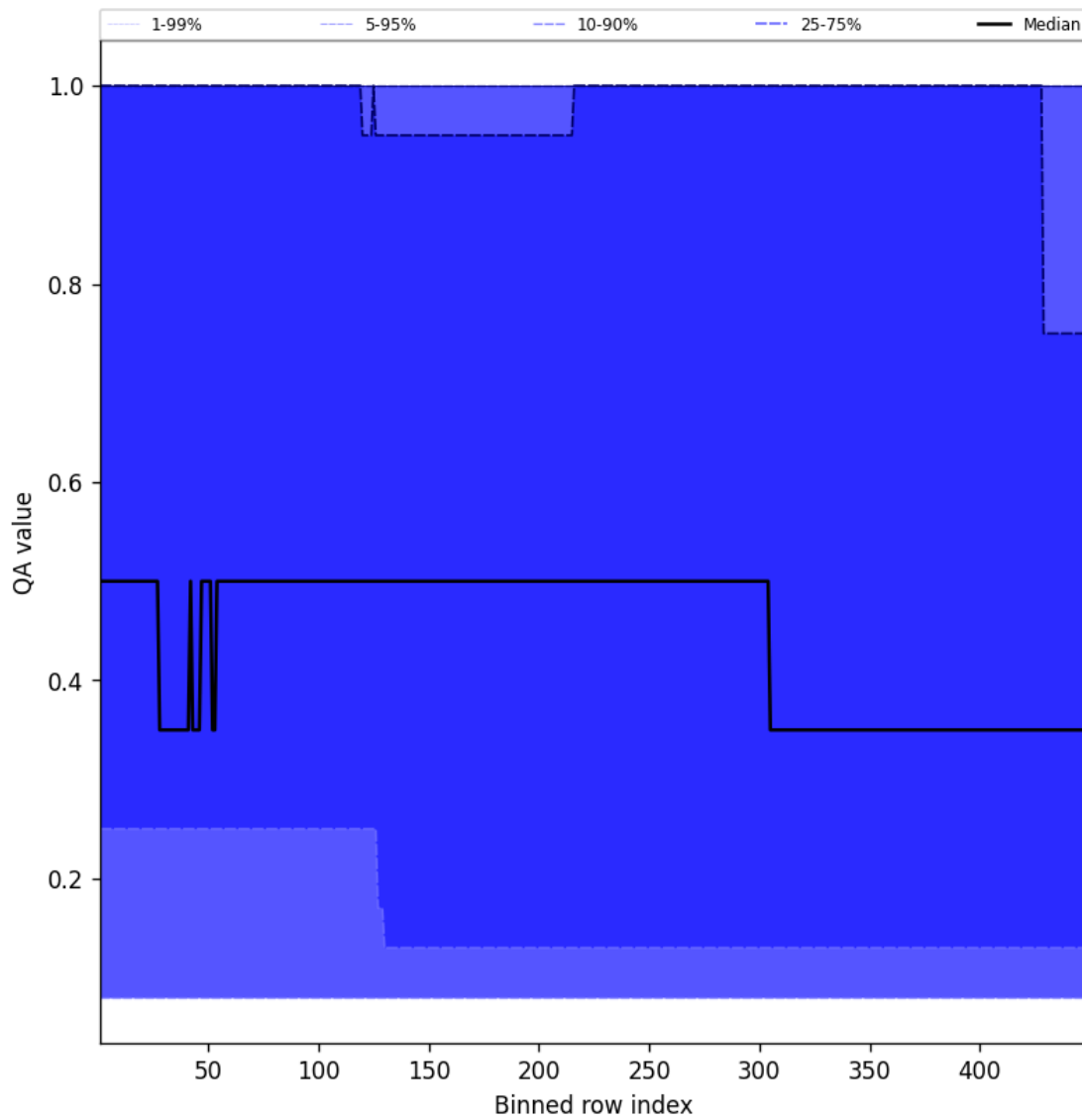
Figure 46: Along track statistics of “QA value” for 2025-07-13 to 2025-07-14
