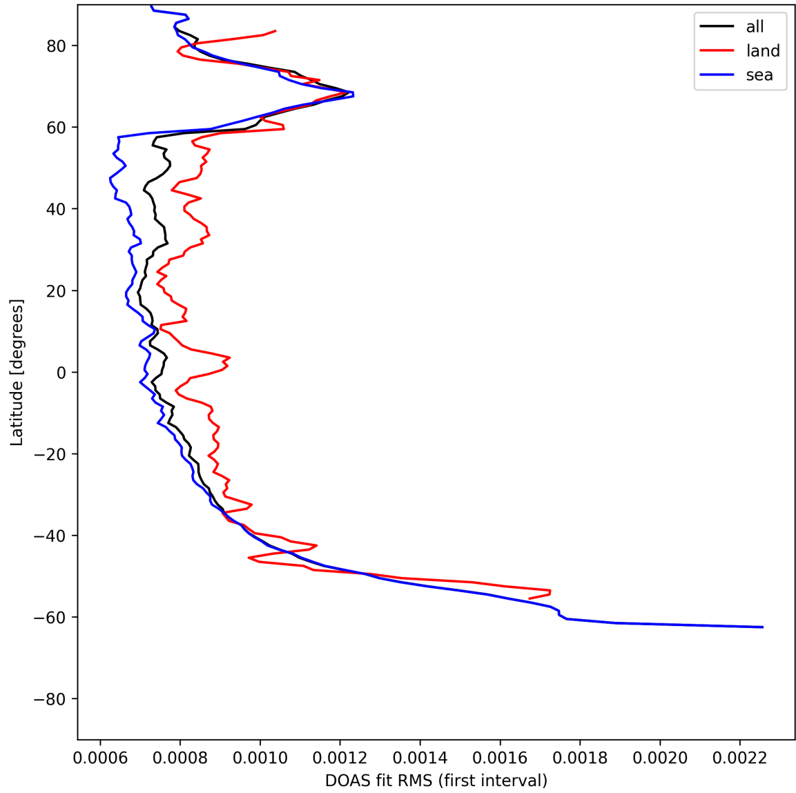
Figure 30: Zonal average of "DOAS fit RMS (first interval)" for 2025-07-13 to 2025-07-14.
