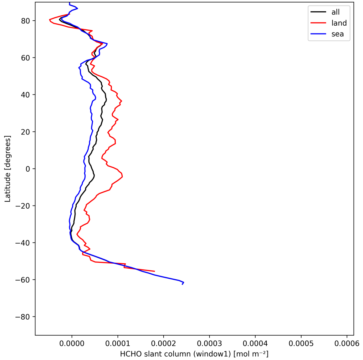
Figure 22: Zonal average of “HCHO slant column (window1)” for 2025-07-13 to 2025-07-14.
