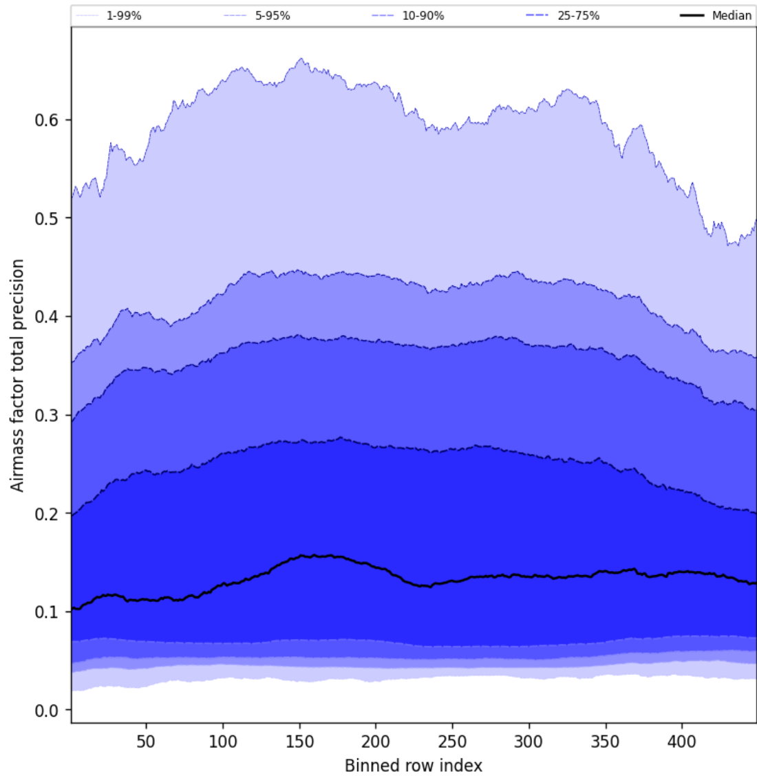
Figure 53: Along track statistics of “Airmass factor total precision” for 2025-07-13 to 2025-07-14
