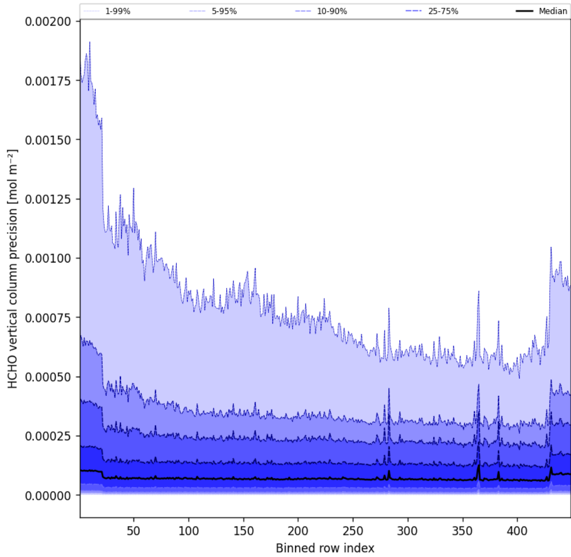
Figure 48: Along track statistics of “HCHO vertical column precision” for 2025-07-13 to 2025-07-14
