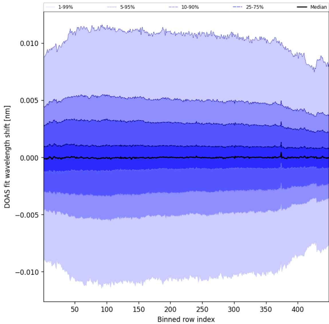
Figure 56: Along track statistics of “DOAS fit wavelength shift” for 2025-07-13 to 2025-07-14
