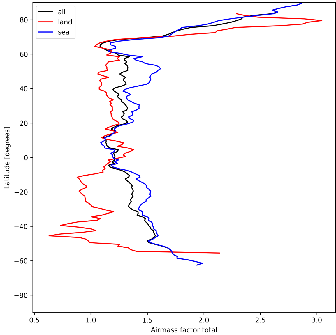
Figure 24: Zonal average of “Airmass factor total” for 2025-07-13 to 2025-07-14.
