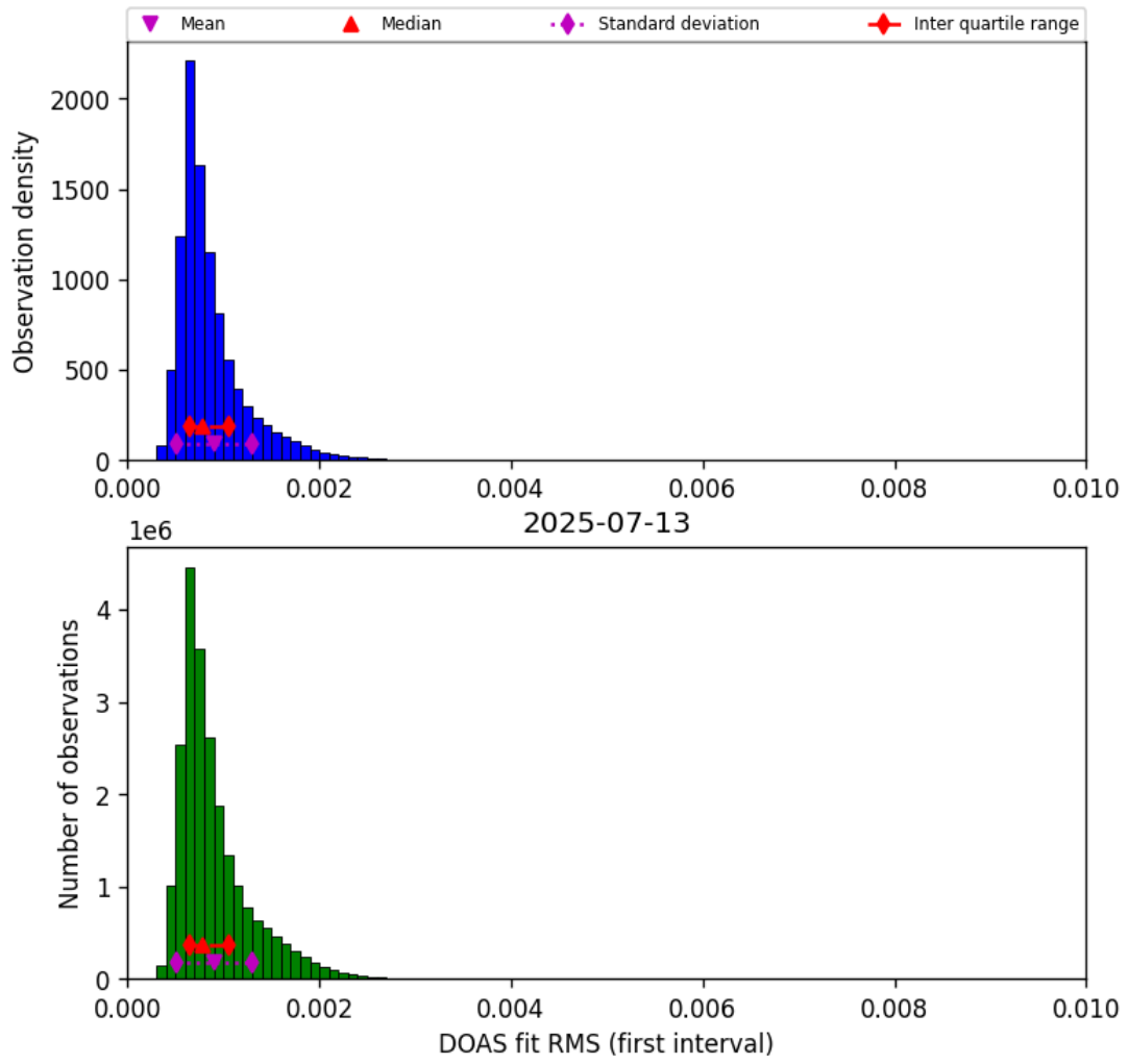
Figure 44: Histogram of “DOAS fit RMS (first interval)” for 2025-07-13 to 2025-07-14
