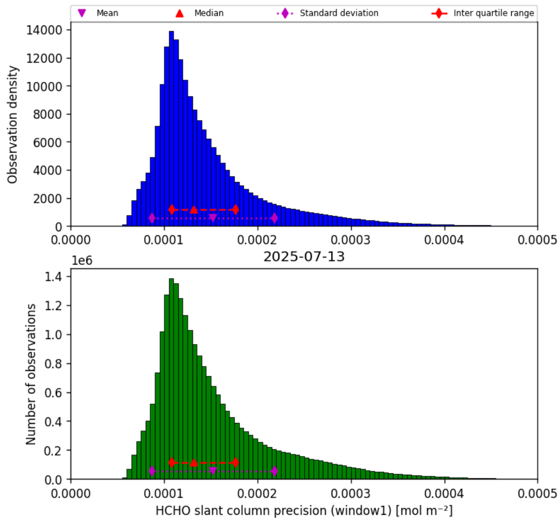
Figure 37: Histogram of “HCHO slant column precision (window1)” for 2025-07-13 to 2025-07-14
