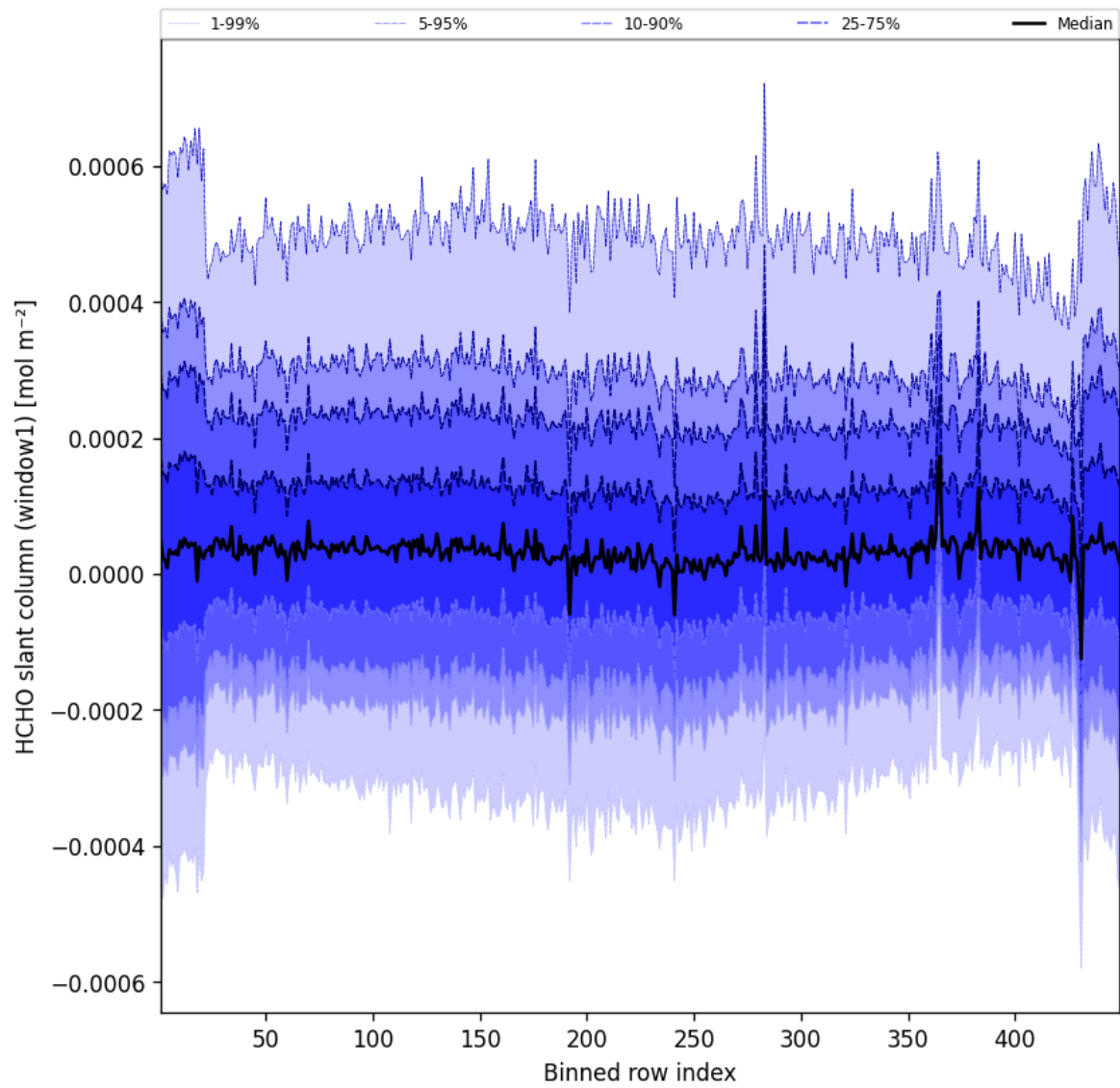
Figure 50: Along track statistics of “HCHO slant column (window1)” for 2025-07-13 to 2025-07-14
