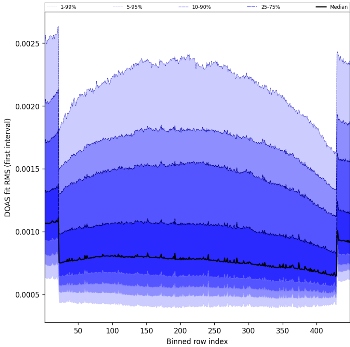
Figure 58: Along track statistics of “DOAS fit RMS (first interval)” for 2025-07-13 to 2025-07-14
