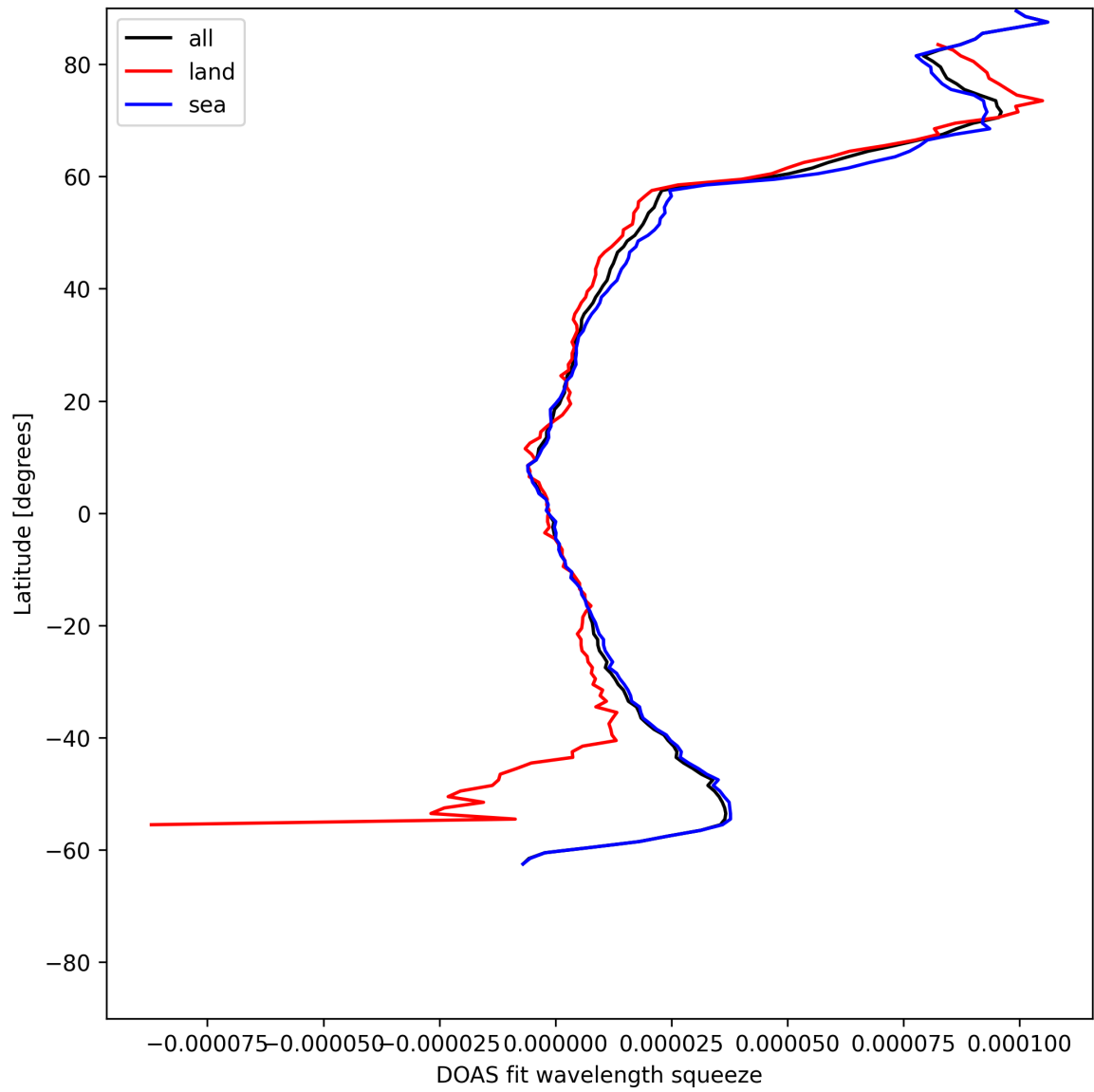
Figure 29: Zonal average of “DOAS fit wavelength squeeze” for 2025-07-13 to 2025-07-14.
