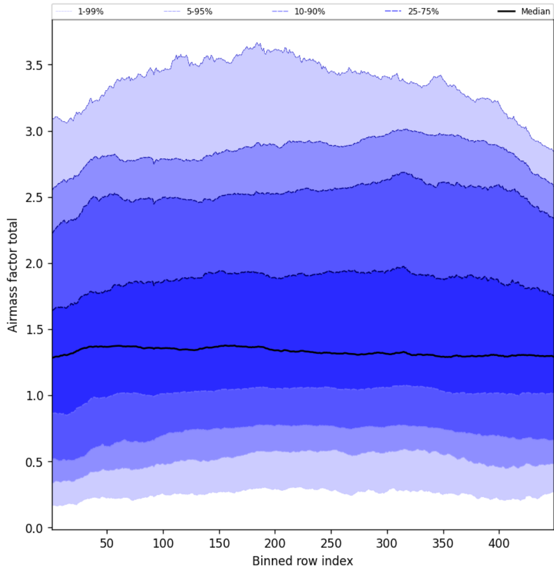
Figure 52: Along track statistics of “Airmass factor total” for 2025-07-14 to 2025-07-15
