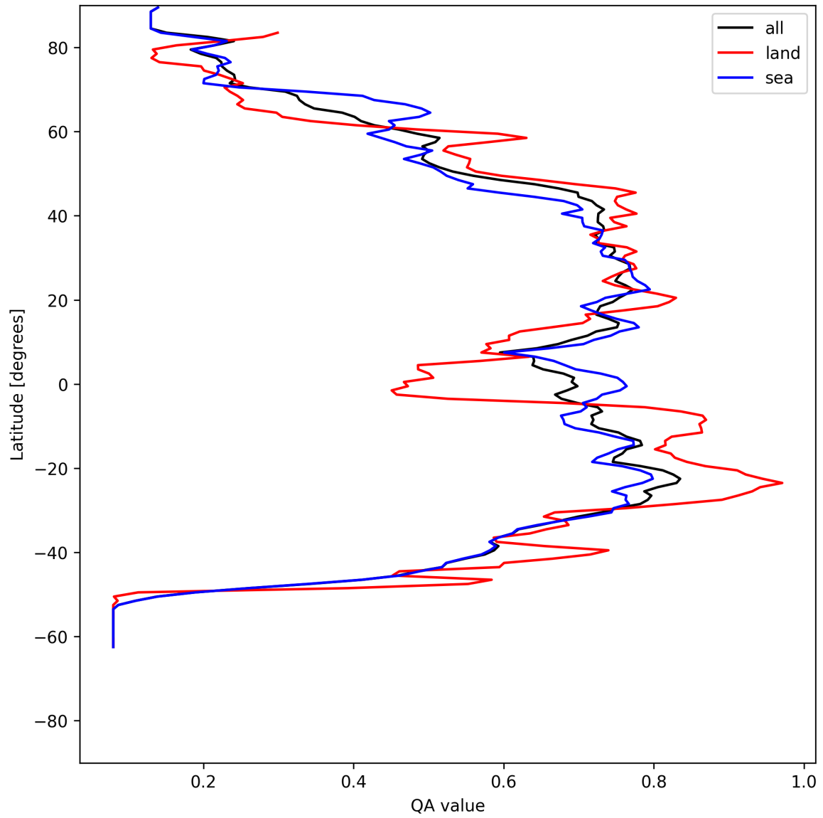
Figure 18: Zonal average of “QA value” for 2025-07-14 to 2025-07-15.
