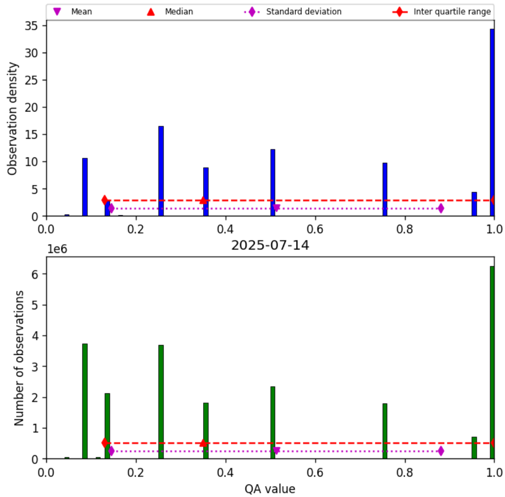
Figure 32: Histogram of “QA value” for 2025-07-14 to 2025-07-15
