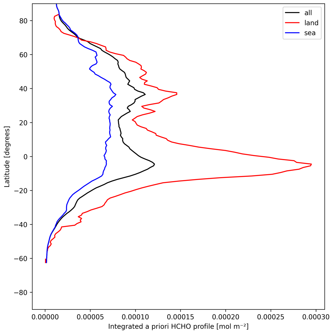
Figure 27: Zonal average of “Integrated a priori HCHO profile” for 2025-07-14 to 2025-07-15.
