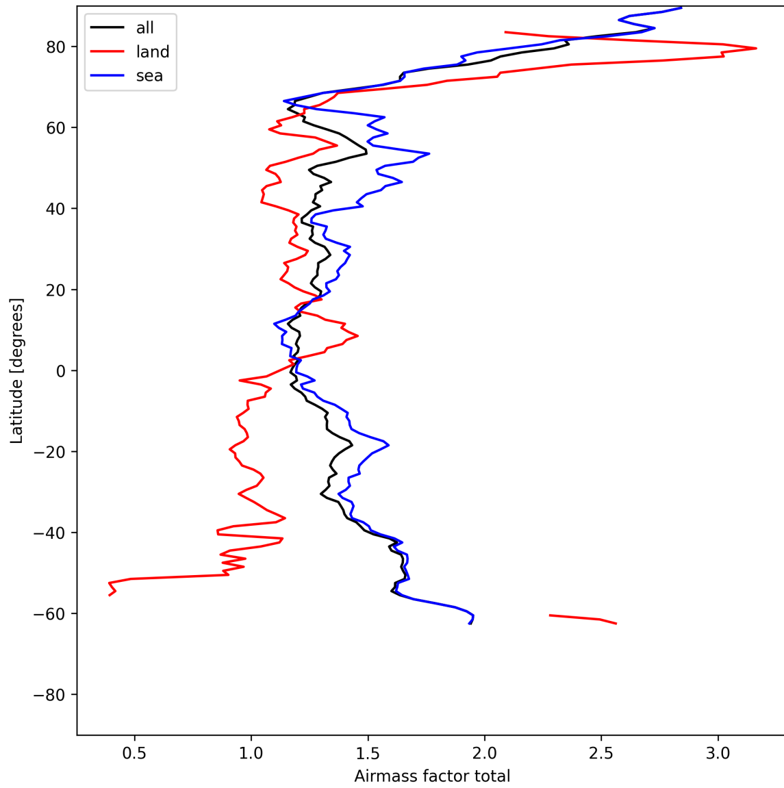
Figure 24: Zonal average of “Airmass factor total” for 2025-07-14 to 2025-07-15.
