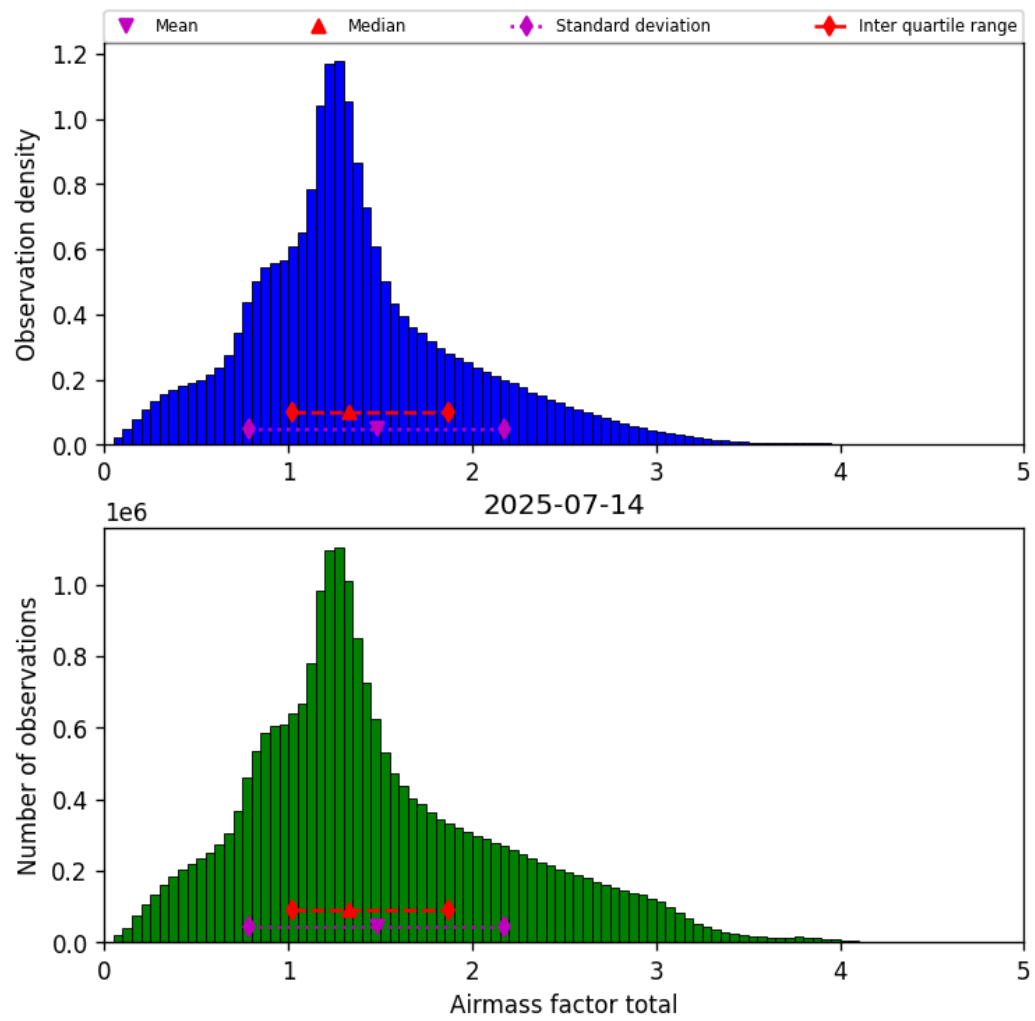
Figure 38: Histogram of “Airmass factor total” for 2025-07-14 to 2025-07-15
