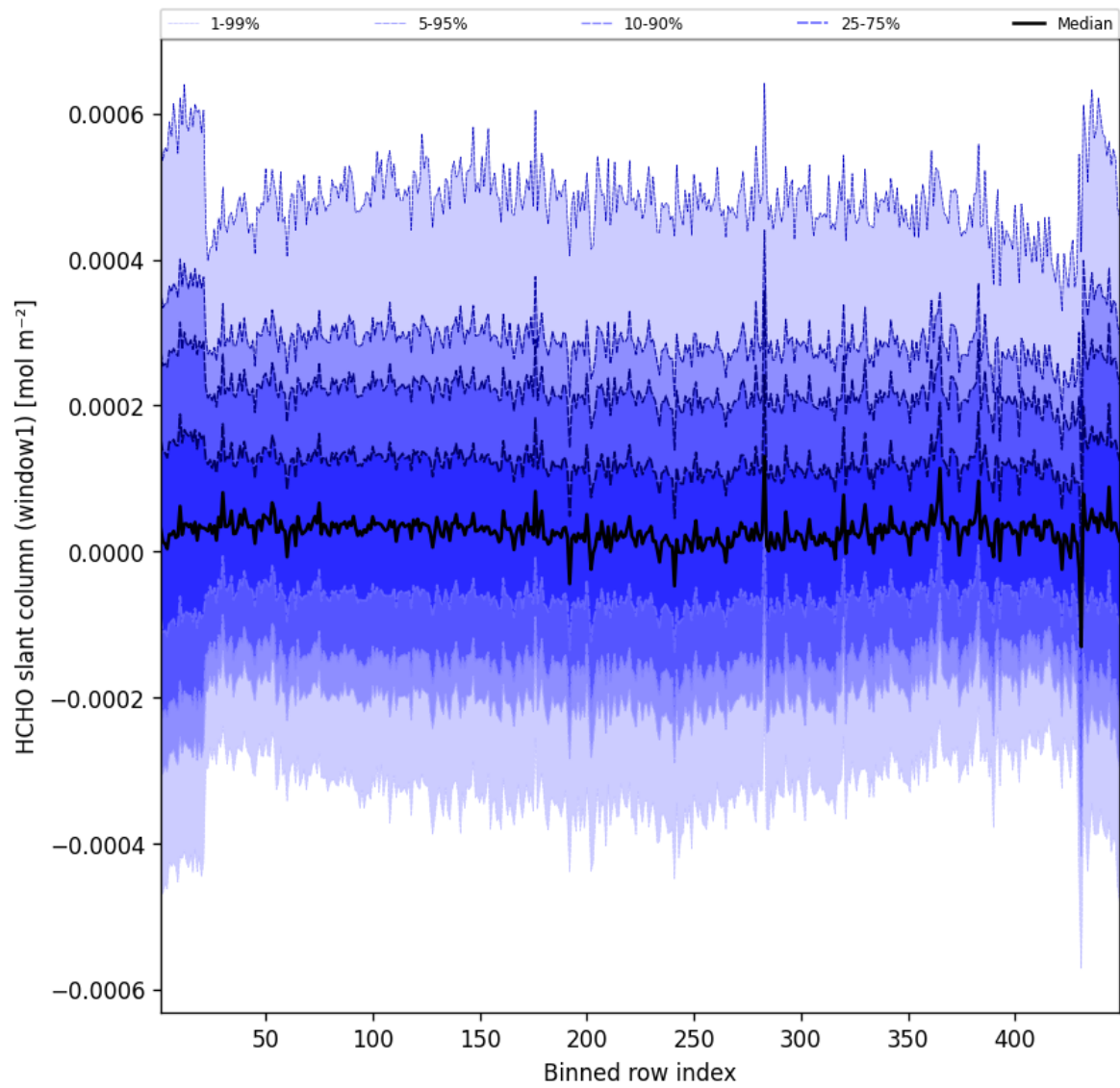
Figure 50: Along track statistics of “HCHO slant column (window1)” for 2025-07-14 to 2025-07-15
