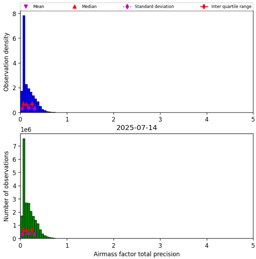
Figure 39: Histogram of “Airmass factor total precision” for 2025-07-14 to 2025-07-15
