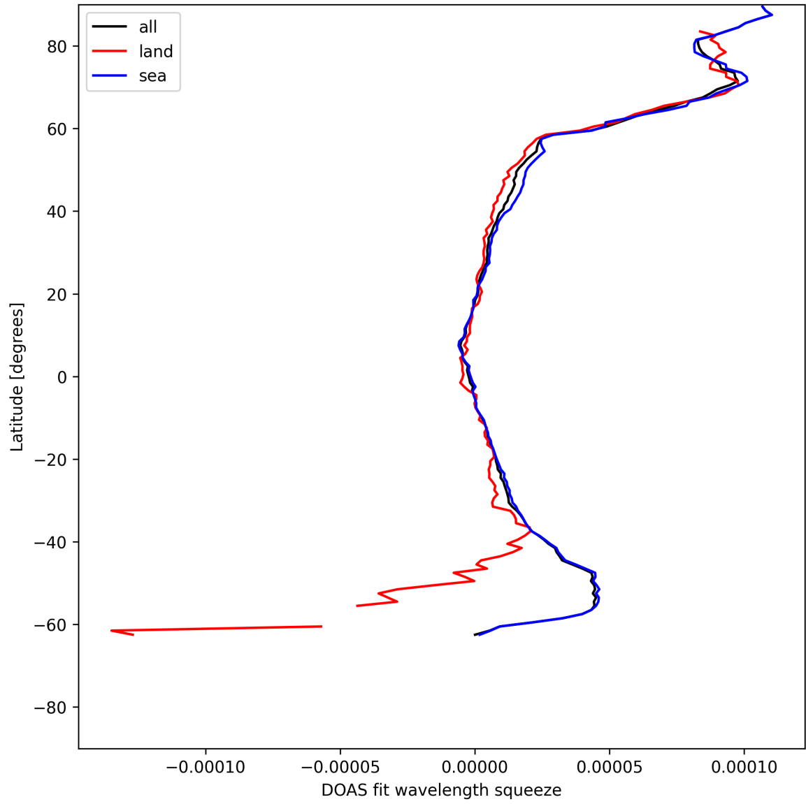
Figure 29: Zonal average of “DOAS fit wavelength squeeze” for 2025-07-14 to 2025-07-15.
