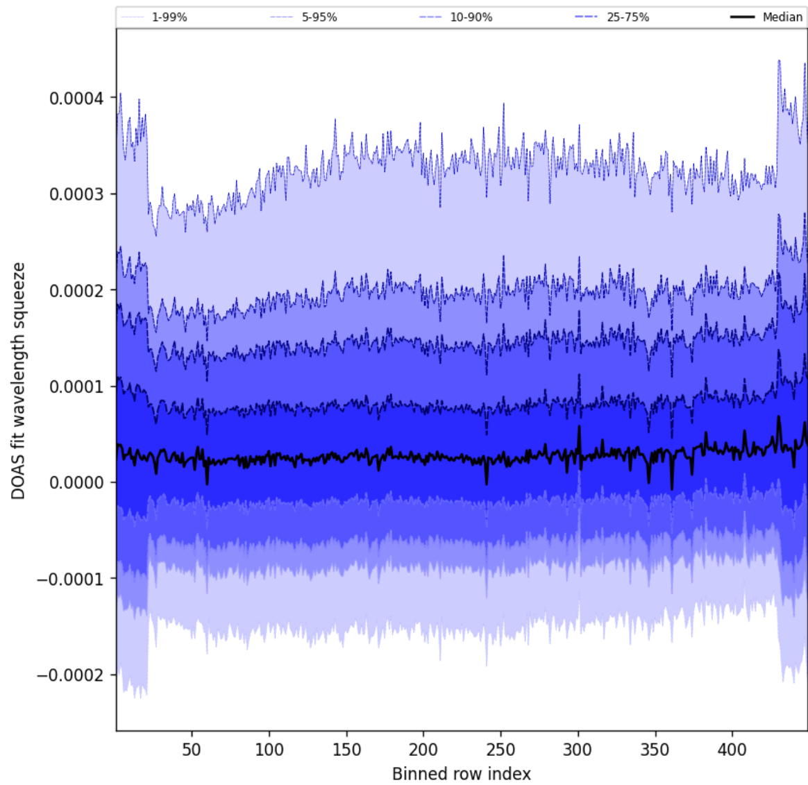
Figure 57: Along track statistics of “DOAS fit wavelength squeeze” for 2025-07-14 to 2025-07-15
