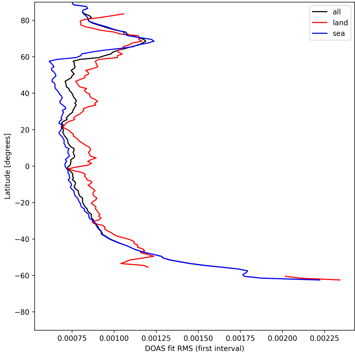
Figure 30: Zonal average of “DOAS fit RMS (first interval)” for 2025-07-14 to 2025-07-15.
