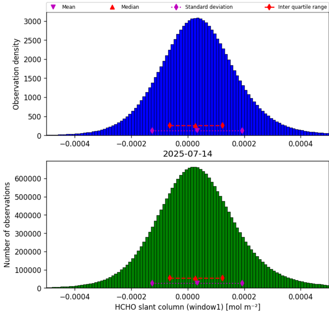
Figure 36: Histogram of “HCHO slant column (window1)” for 2025-07-14 to 2025-07-15
