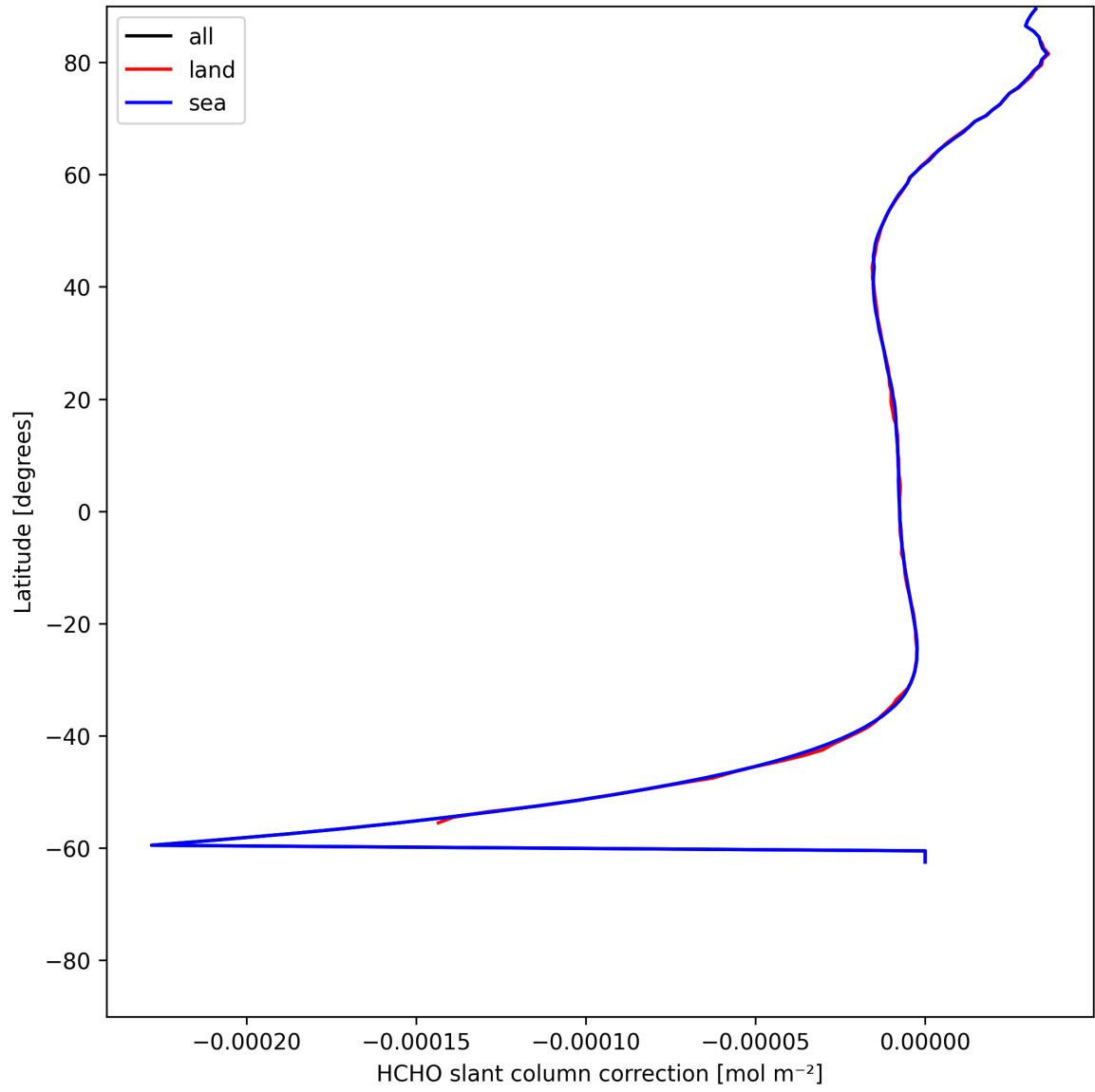
Figure 31: Zonal average of “HCHO slant column correction” for 2025-07-14 to 2025-07-15.
