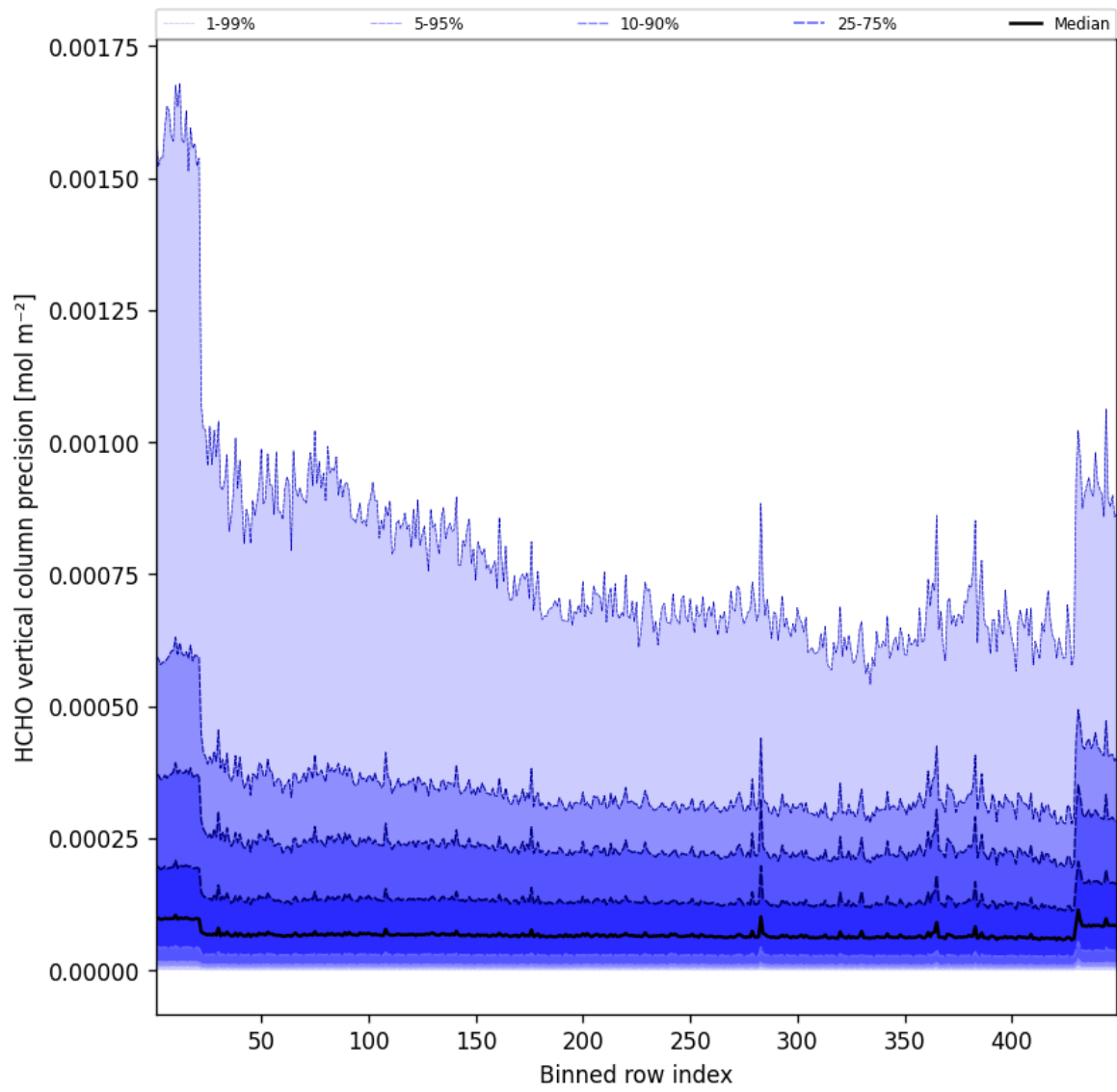
Figure 48: Along track statistics of “HCHO vertical column precision” for 2025-07-14 to 2025-07-15
