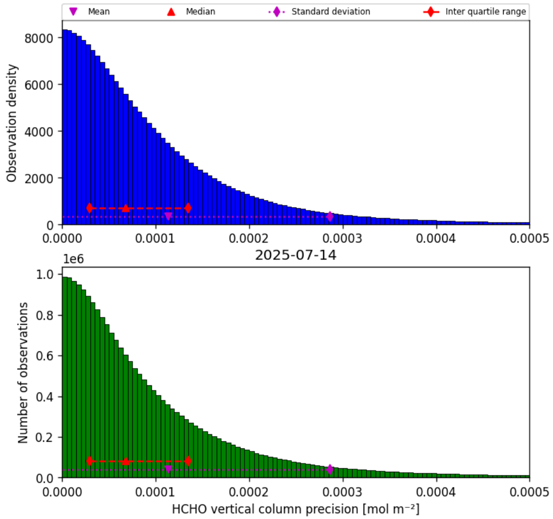
Figure 34: Histogram of “HCHO vertical column precision” for 2025-07-14 to 2025-07-15
