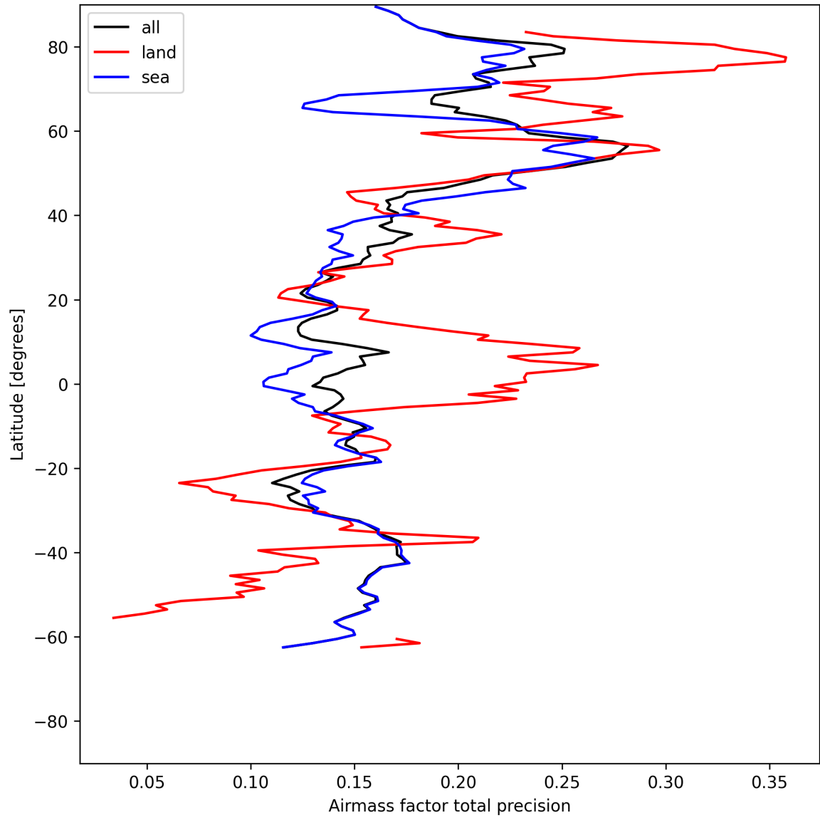
Figure 25: Zonal average of “Airmass factor total precision” for 2025-07-14 to 2025-07-15.
