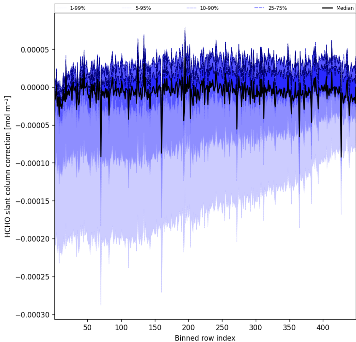
Figure 59: Along track statistics of “HCHO slant column correction” for 2025-07-14 to 2025-07-15
