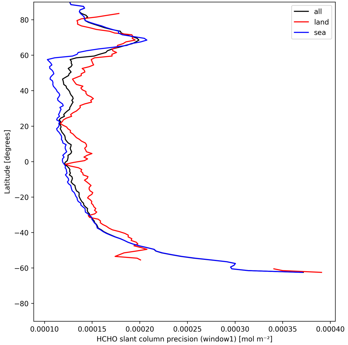
Figure 23: Zonal average of “HCHO slant column precision (window1)” for 2025-07-14 to 2025-07-15.
