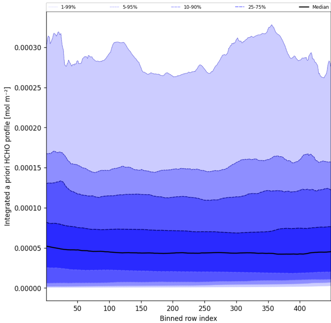
Figure 55: Along track statistics of “Integrated a priori HCHO profile” for 2025-07-14 to 2025-07-15
