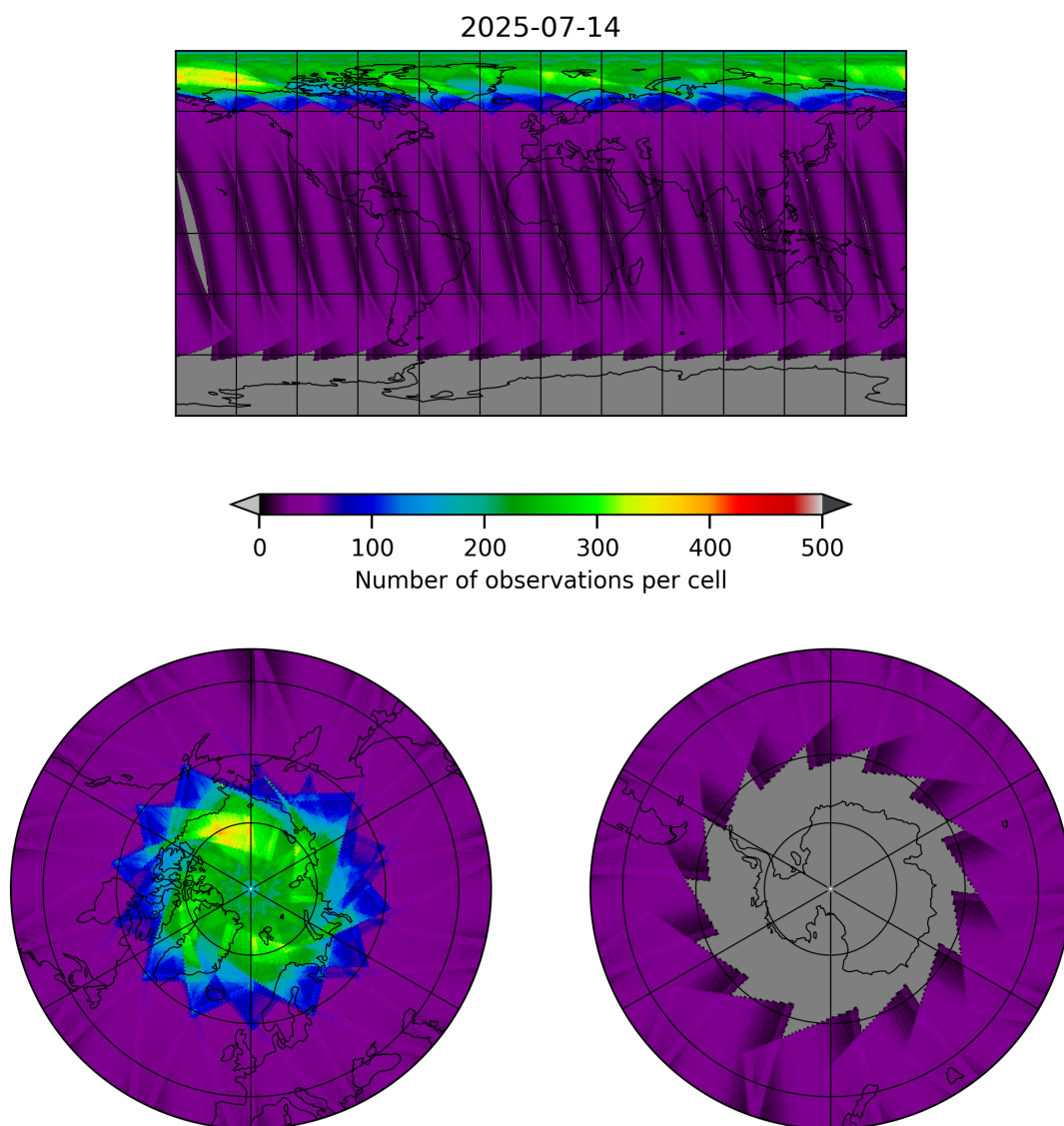
Figure 17: Map of the number of observations for 2025-07-14 to 2025-07-15
