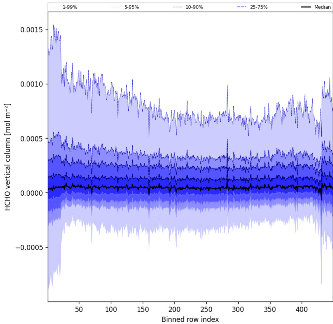
Figure 47: Along track statistics of “HCHO vertical column” for 2025-07-14 to 2025-07-15
