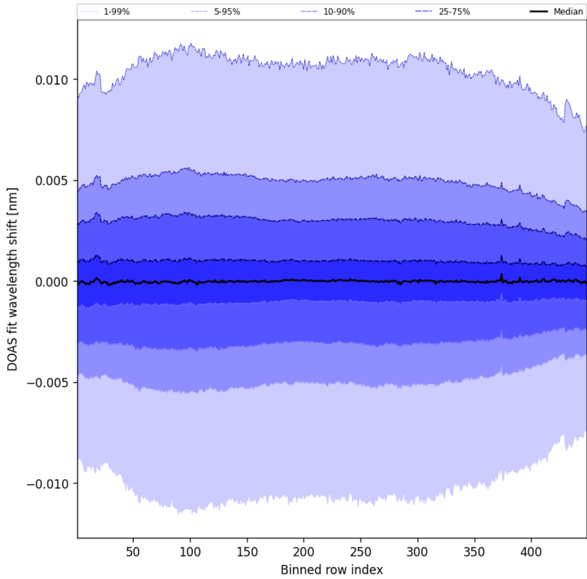
Figure 56: Along track statistics of “DOAS fit wavelength shift” for 2025-07-14 to 2025-07-15
