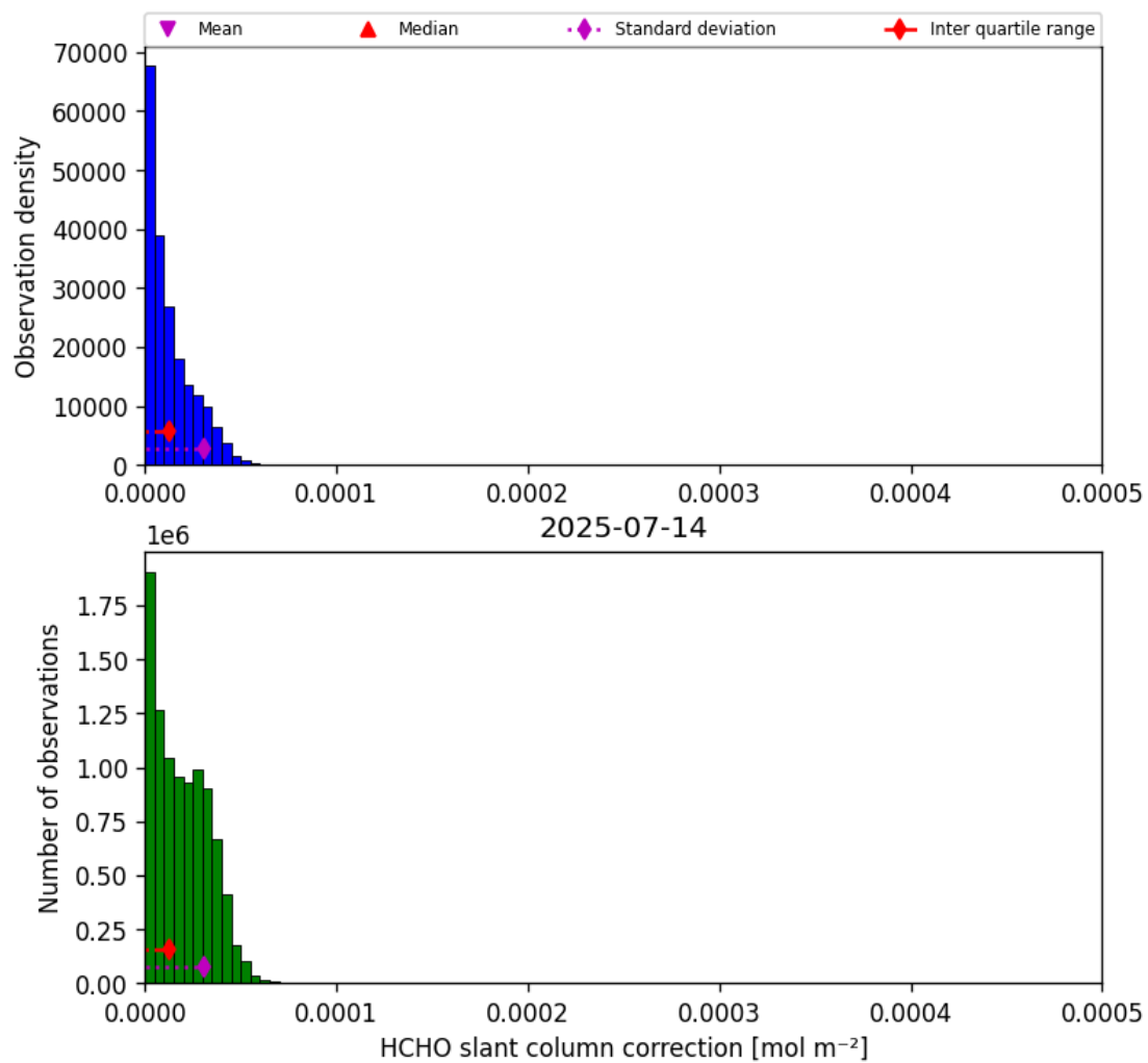
Figure 45: Histogram of “HCHO slant column correction” for 2025-07-14 to 2025-07-15
