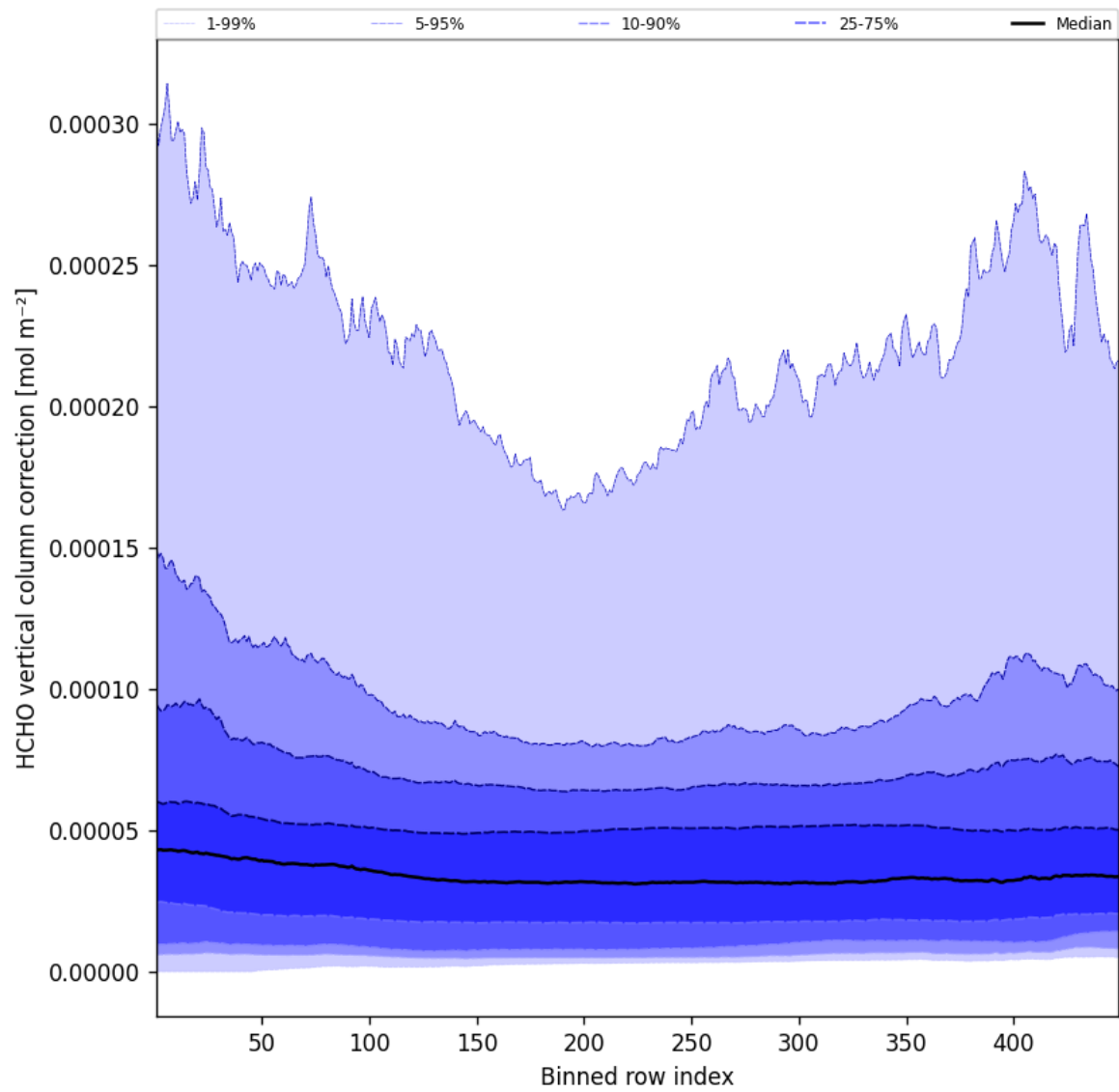
Figure 49: Along track statistics of “HCHO vertical column correction” for 2025-07-14 to 2025-07-15
