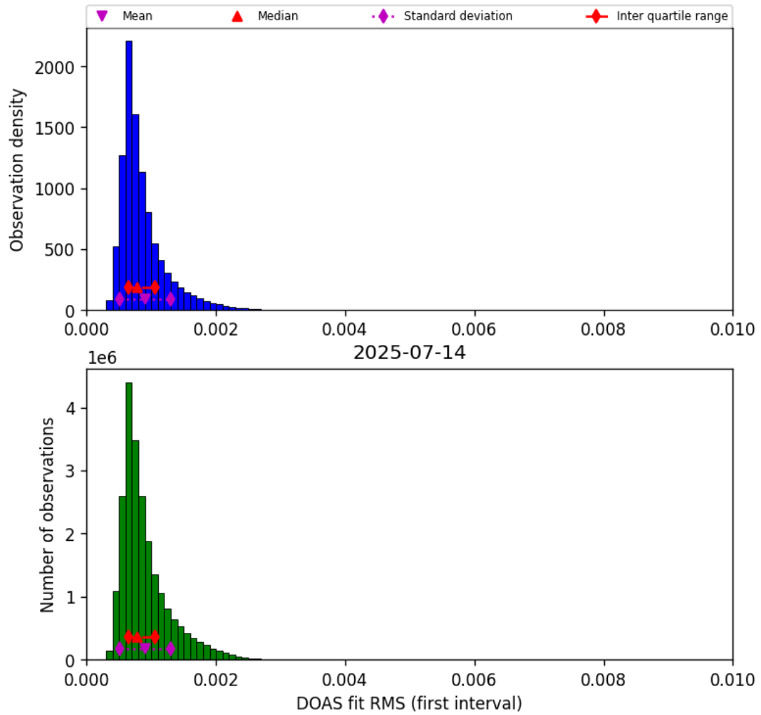
Figure 44: Histogram of “DOAS fit RMS (first interval)” for 2025-07-14 to 2025-07-15
