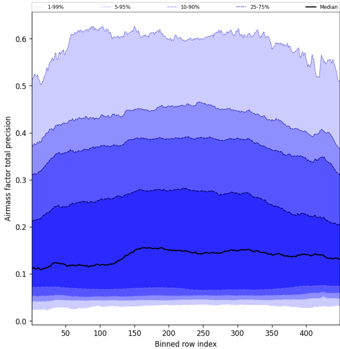
Figure 53: Along track statistics of “Airmass factor total precision” for 2025-07-14 to 2025-07-15
