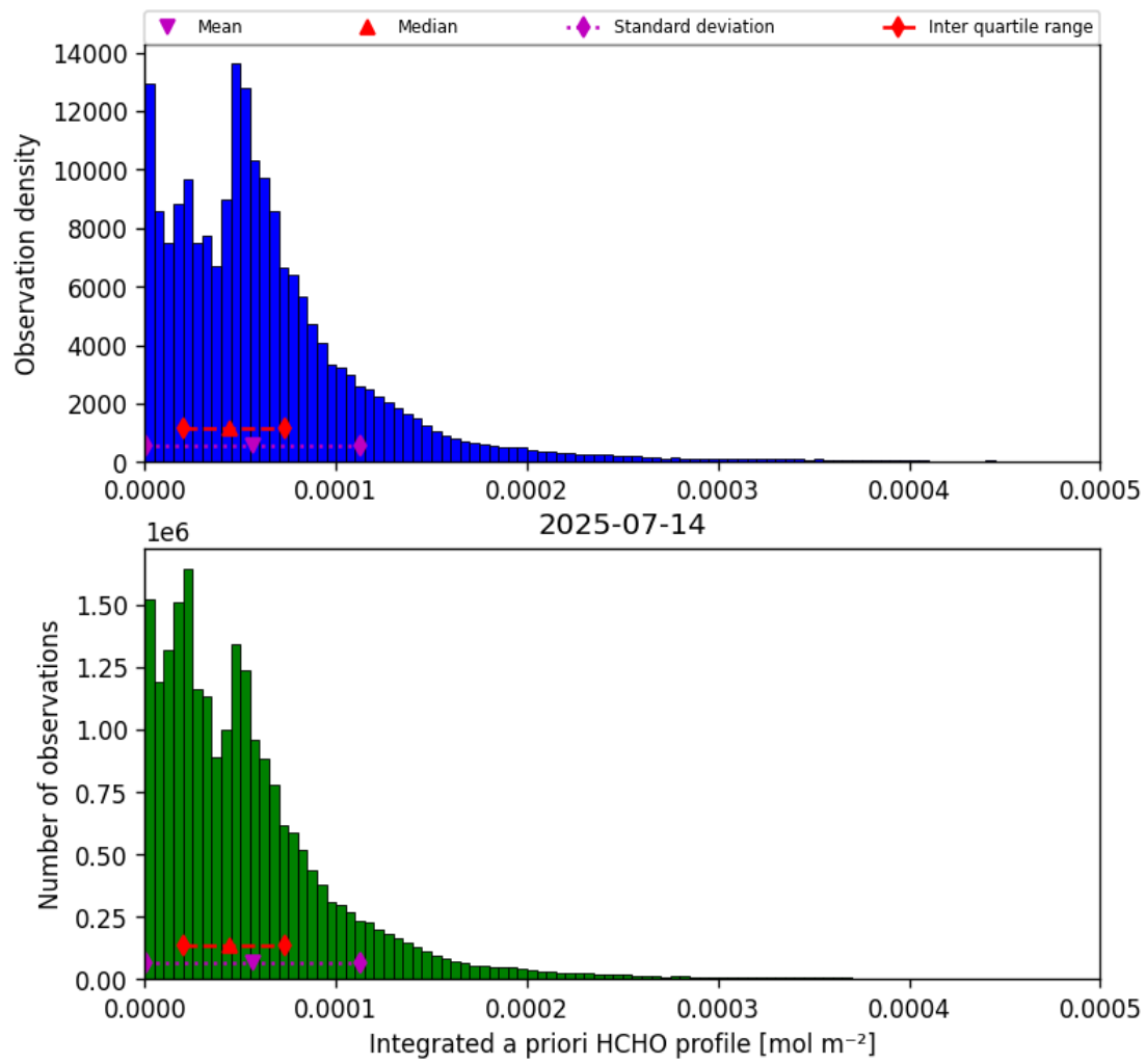
Figure 41: Histogram of “Integrated a priori HCHO profile” for 2025-07-14 to 2025-07-15
