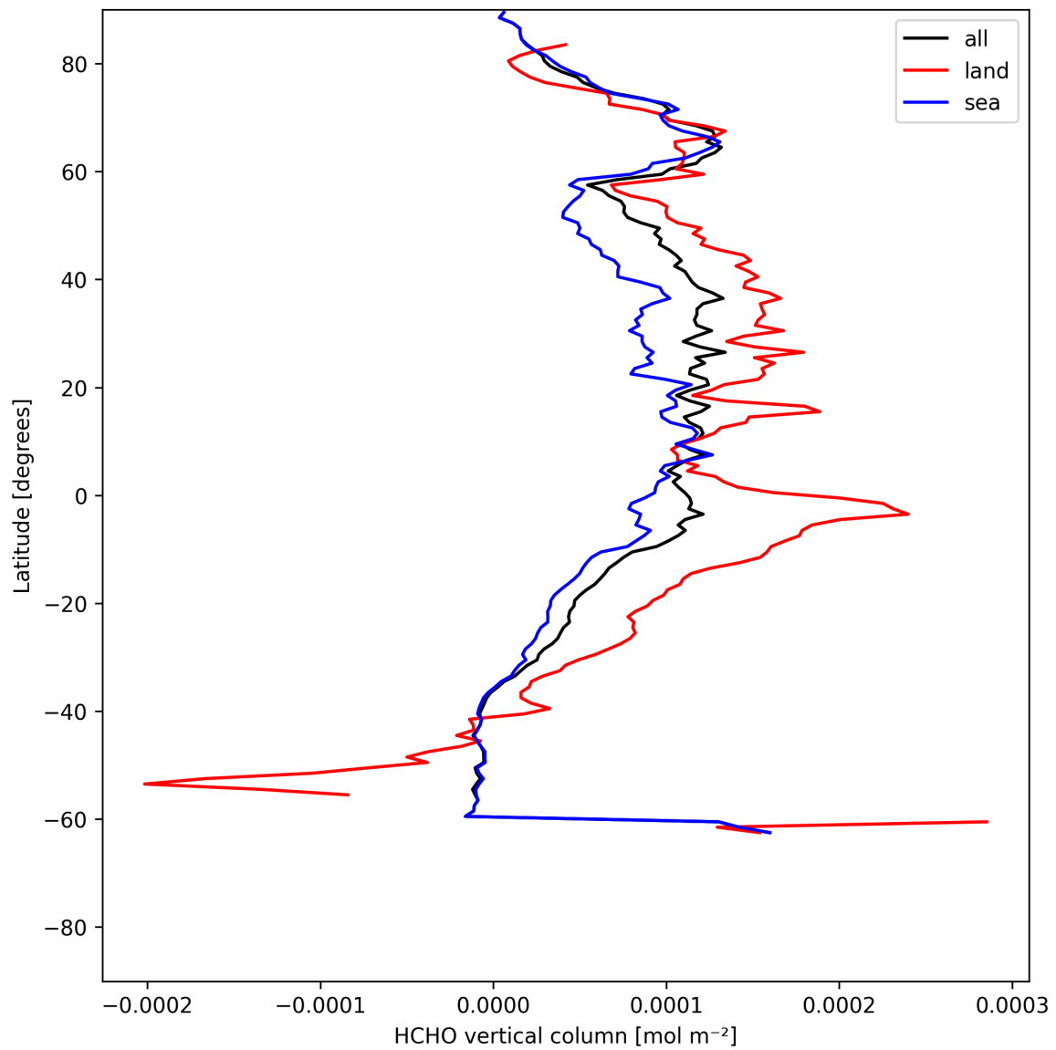
Figure 19: Zonal average of “HCHO vertical column” for 2025-07-14 to 2025-07-15.
