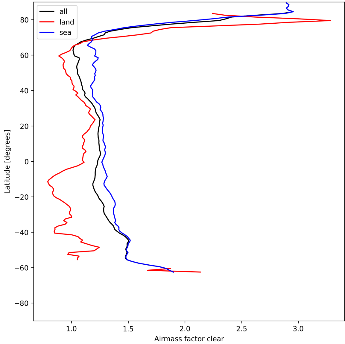
Figure 26: Zonal average of “Airmass factor clear” for 2025-07-14 to 2025-07-15.
