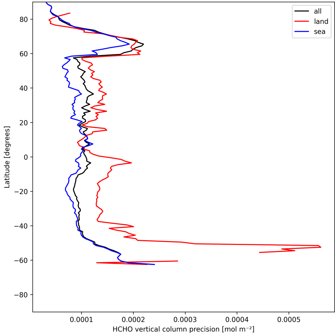
Figure 20: Zonal average of “HCHO vertical column precision” for 2025-07-14 to 2025-07-15.
