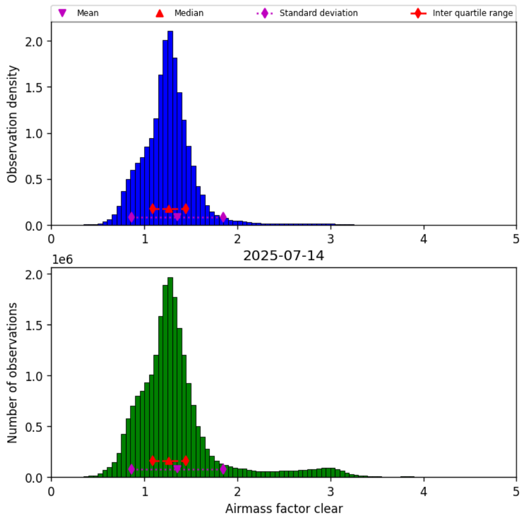
Figure 40: Histogram of “Airmass factor clear” for 2025-07-14 to 2025-07-15
