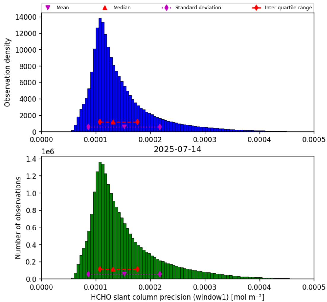
Figure 37: Histogram of “HCHO slant column precision (window1)” for 2025-07-14 to 2025-07-15
