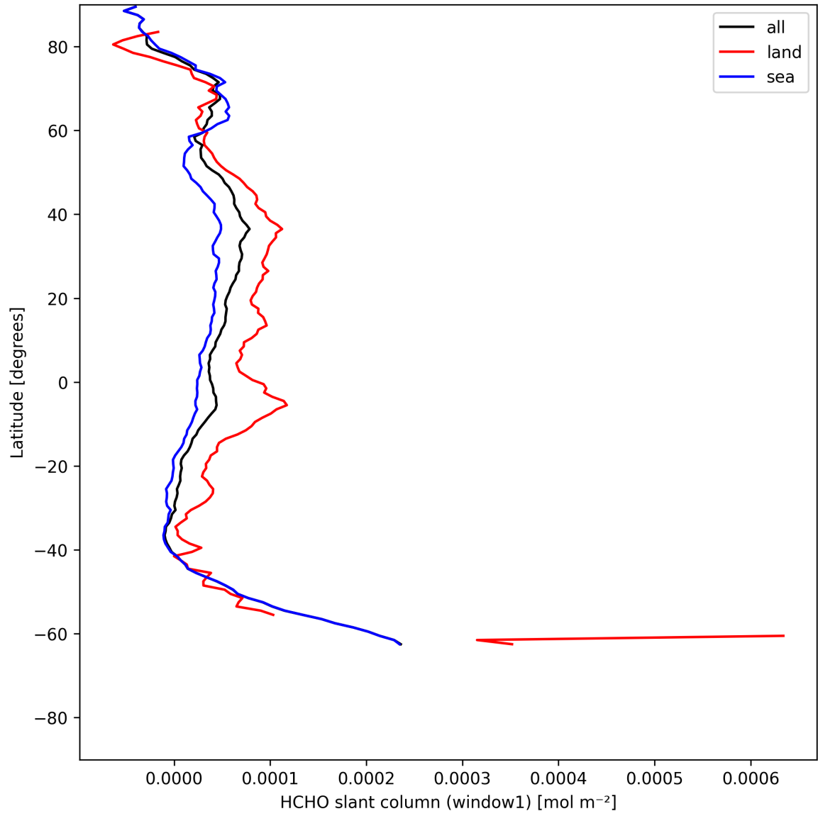
Figure 22: Zonal average of “HCHO slant column (window1)” for 2025-07-14 to 2025-07-15.
