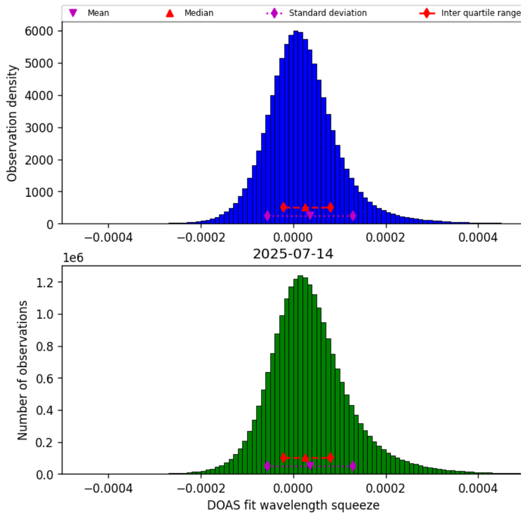
Figure 43: Histogram of “DOAS fit wavelength squeeze” for 2025-07-14 to 2025-07-15
