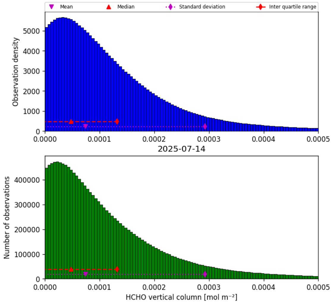
Figure 33: Histogram of “HCHO vertical column” for 2025-07-14 to 2025-07-15
