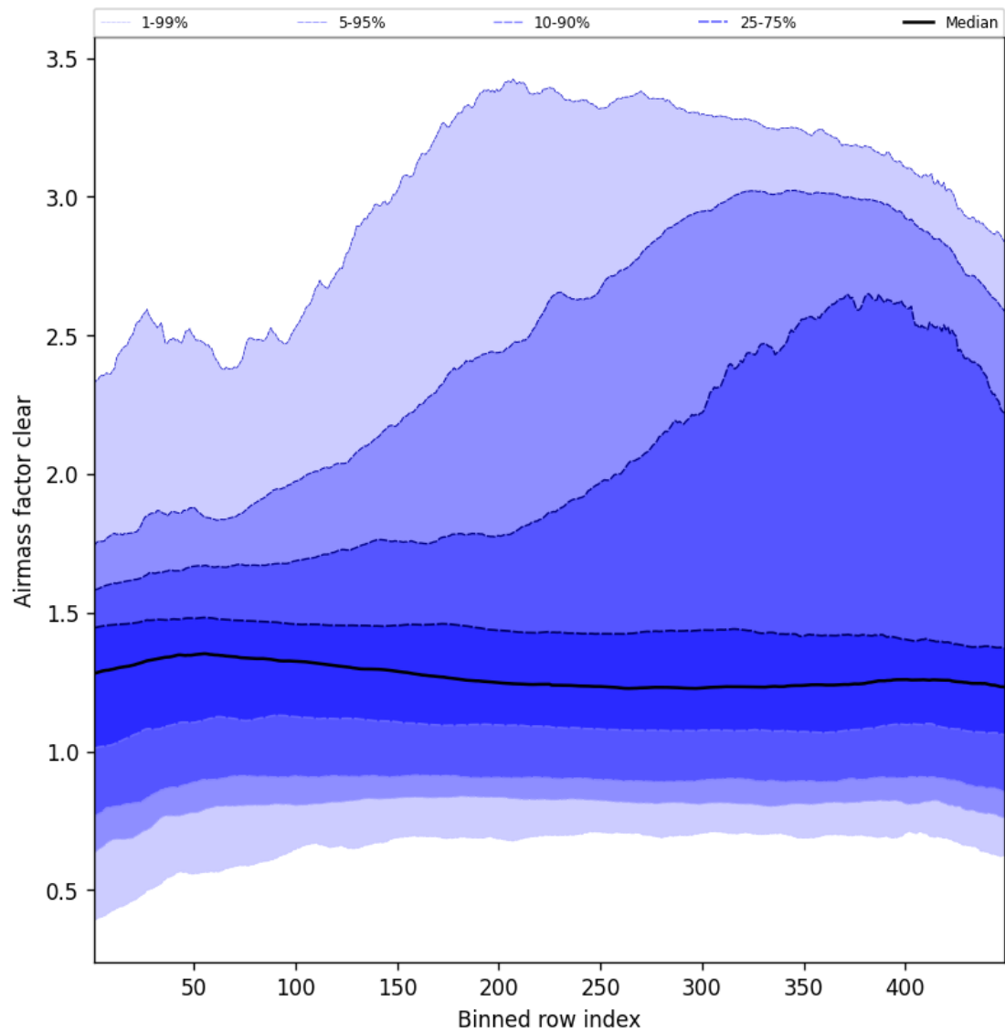
Figure 54: Along track statistics of “Airmass factor clear” for 2025-07-14 to 2025-07-15
