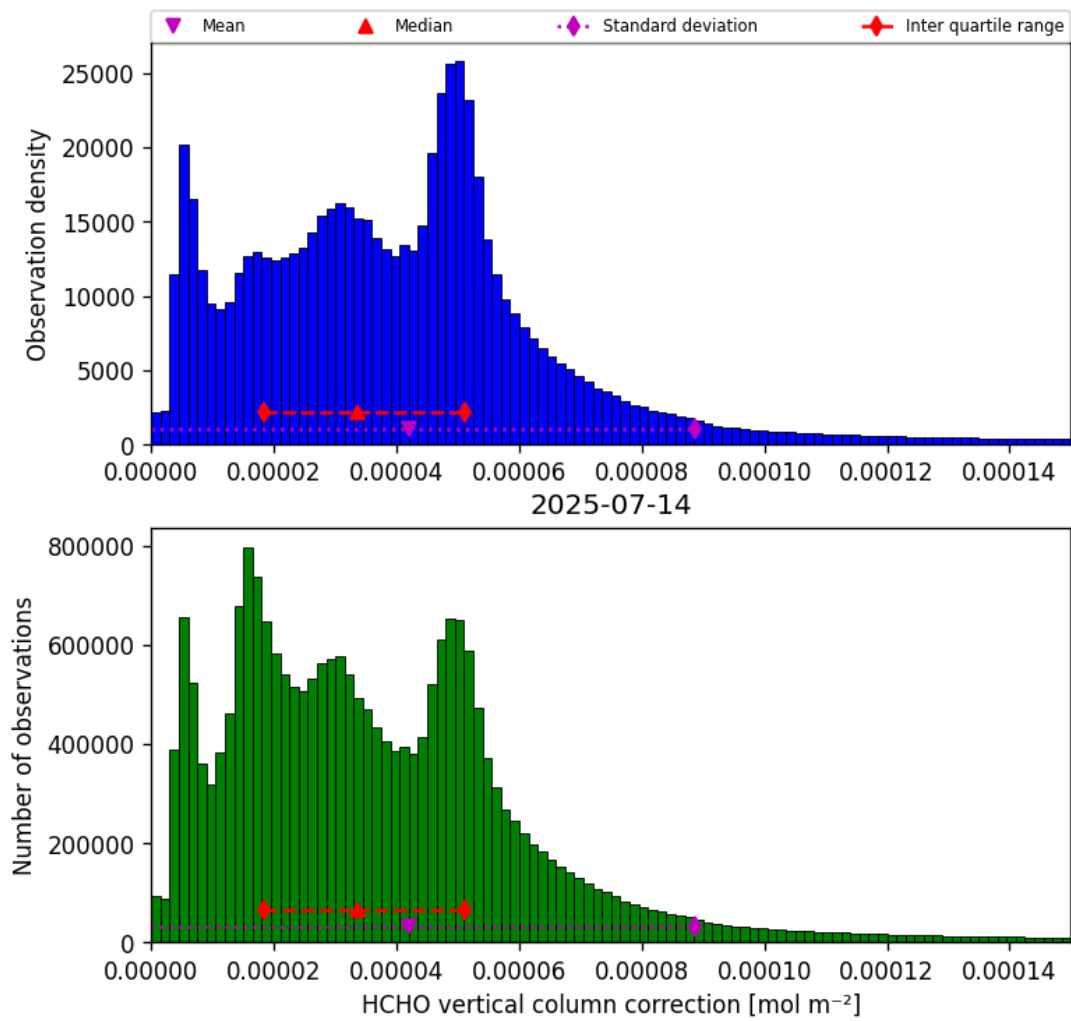
Figure 35: Histogram of “HCHO vertical column correction” for 2025-07-14 to 2025-07-15
