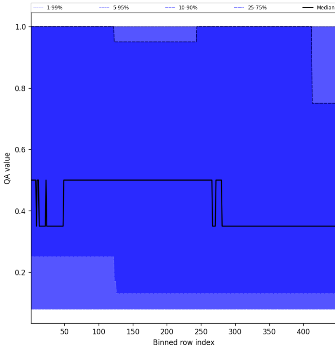
Figure 46: Along track statistics of “QA value” for 2025-07-14 to 2025-07-15
