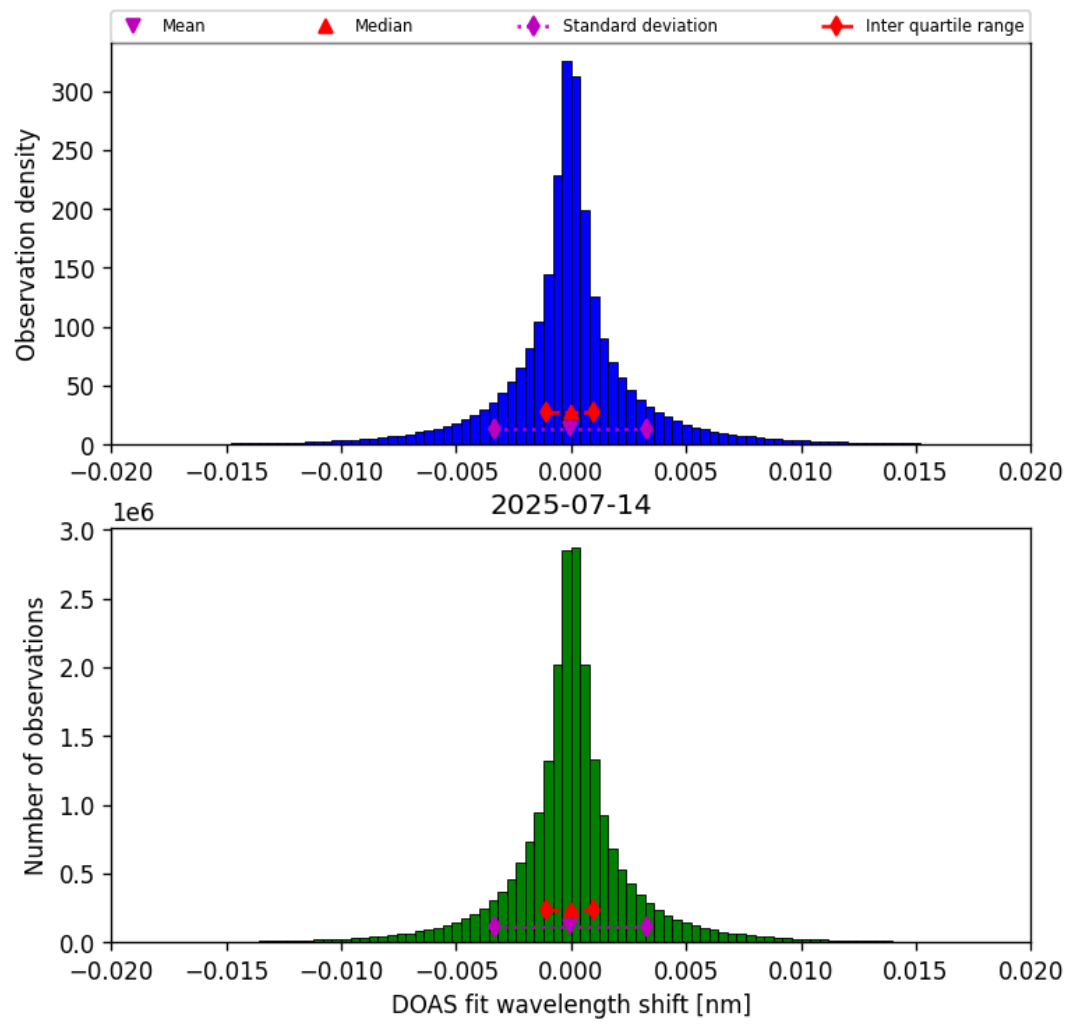
Figure 42: Histogram of “DOAS fit wavelength shift” for 2025-07-14 to 2025-07-15
