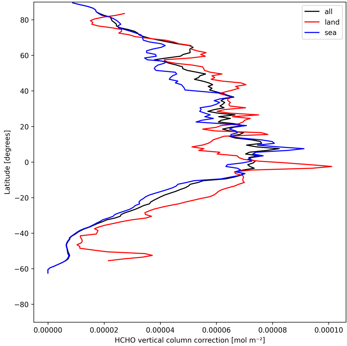
Figure 21: Zonal average of “HCHO vertical column correction” for 2025-07-14 to 2025-07-15.
