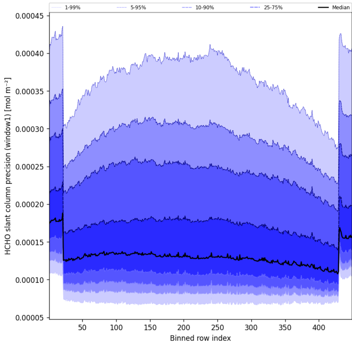
Figure 51: Along track statistics of “HCHO slant column precision (window1)” for 2025-07-14 to 2025-07-15
