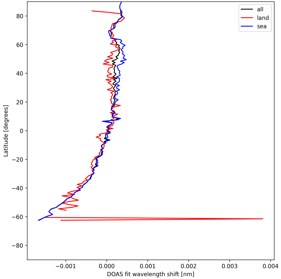
Figure 28: Zonal average of “DOAS fit wavelength shift” for 2025-07-14 to 2025-07-15.
