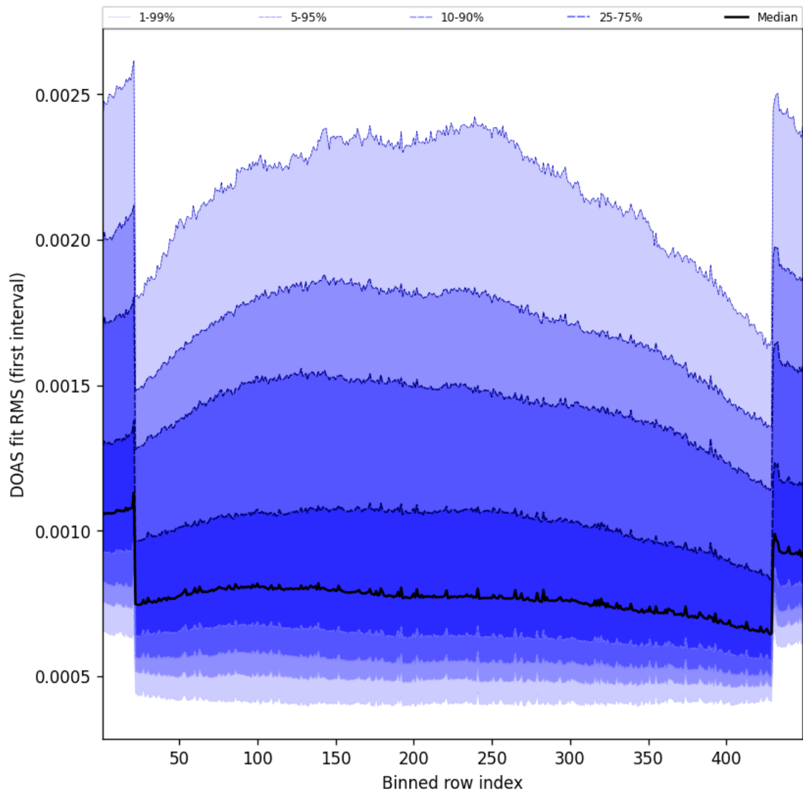
Figure 58: Along track statistics of “DOAS fit RMS (first interval)” for 2025-07-14 to 2025-07-15
