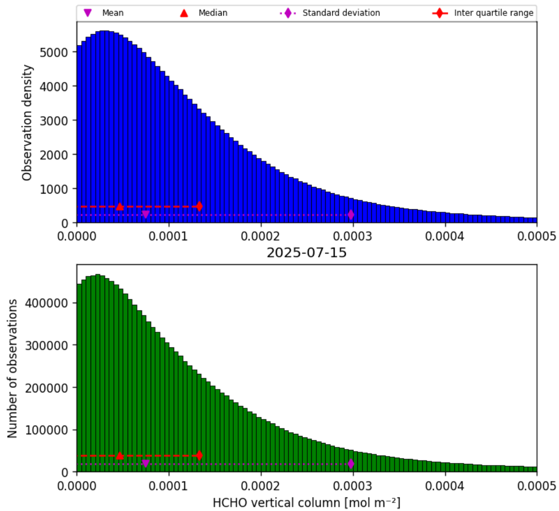
Figure 33: Histogram of “HCHO vertical column” for 2025-07-15 to 2025-07-16
