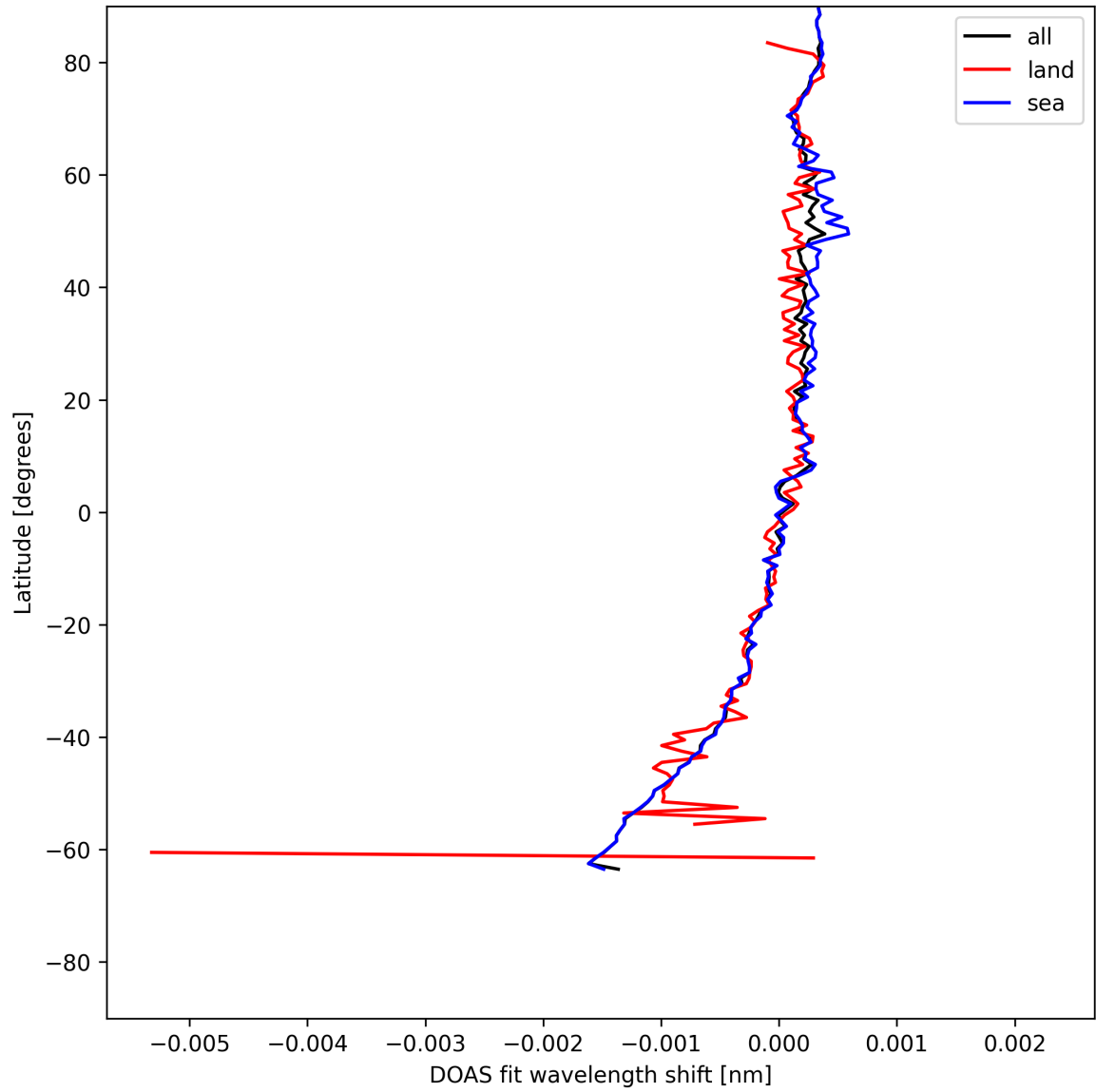
Figure 28: Zonal average of “DOAS fit wavelength shift” for 2025-07-15 to 2025-07-16.
