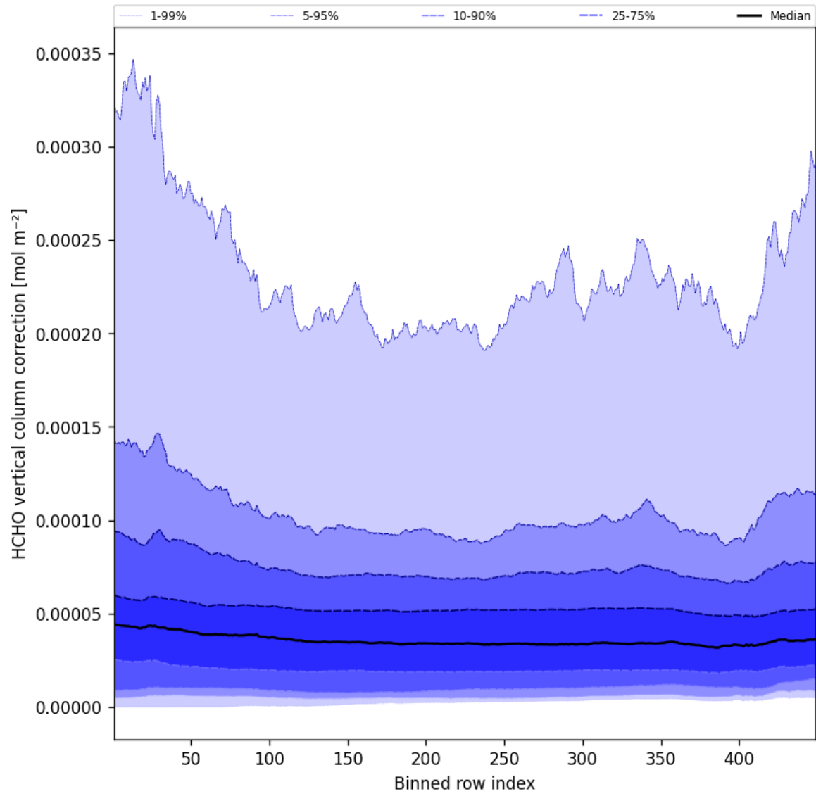
Figure 49: Along track statistics of “HCHO vertical column correction” for 2025-07-15 to 2025-07-16
