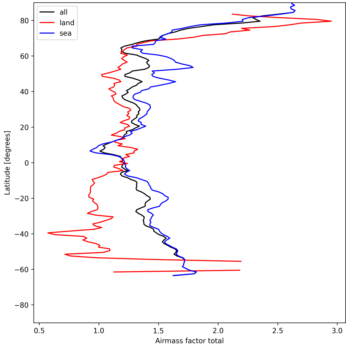
Figure 24: Zonal average of “Airmass factor total” for 2025-07-15 to 2025-07-16.
