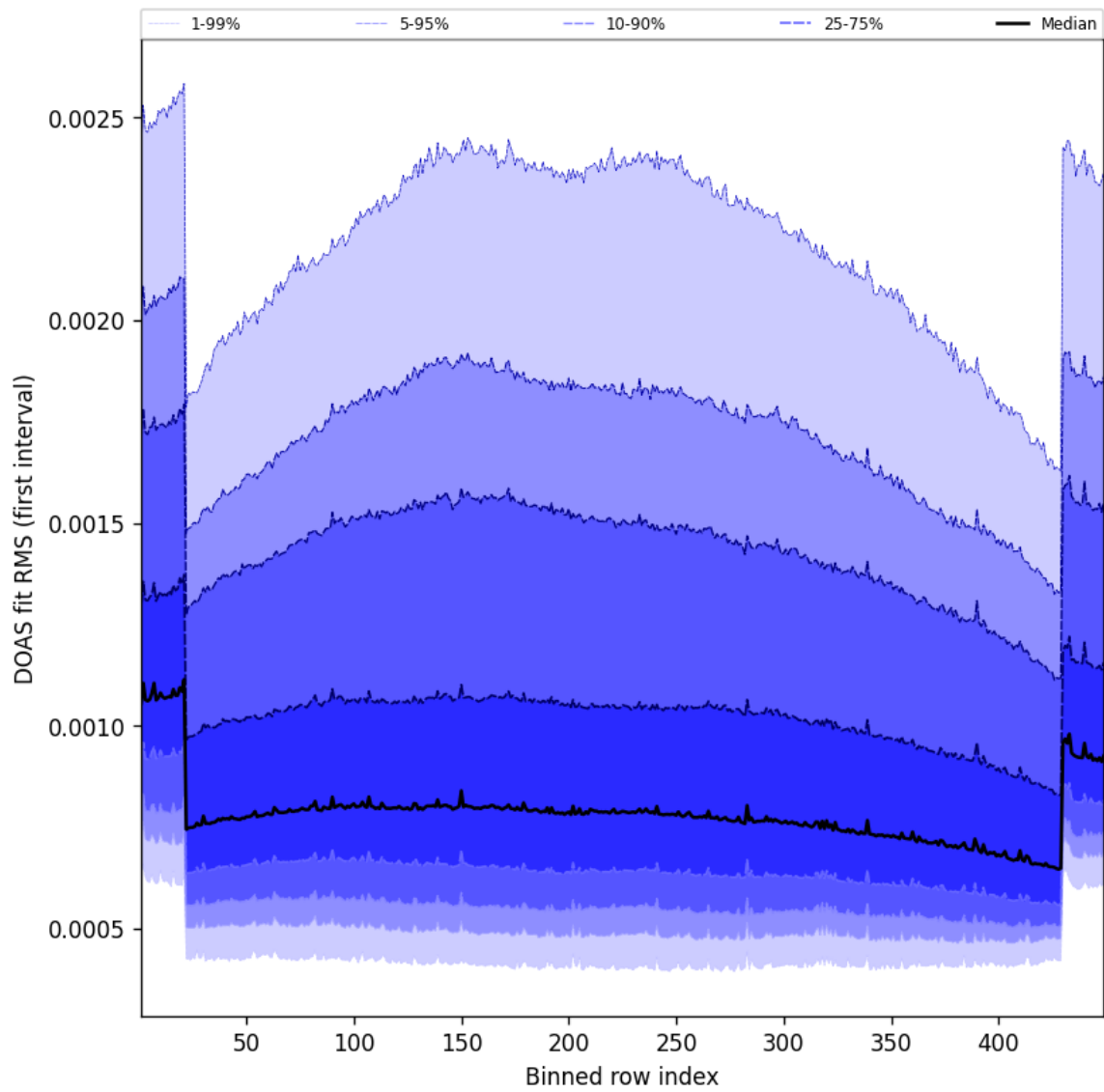
Figure 58: Along track statistics of “DOAS fit RMS (first interval)” for 2025-07-15 to 2025-07-16
