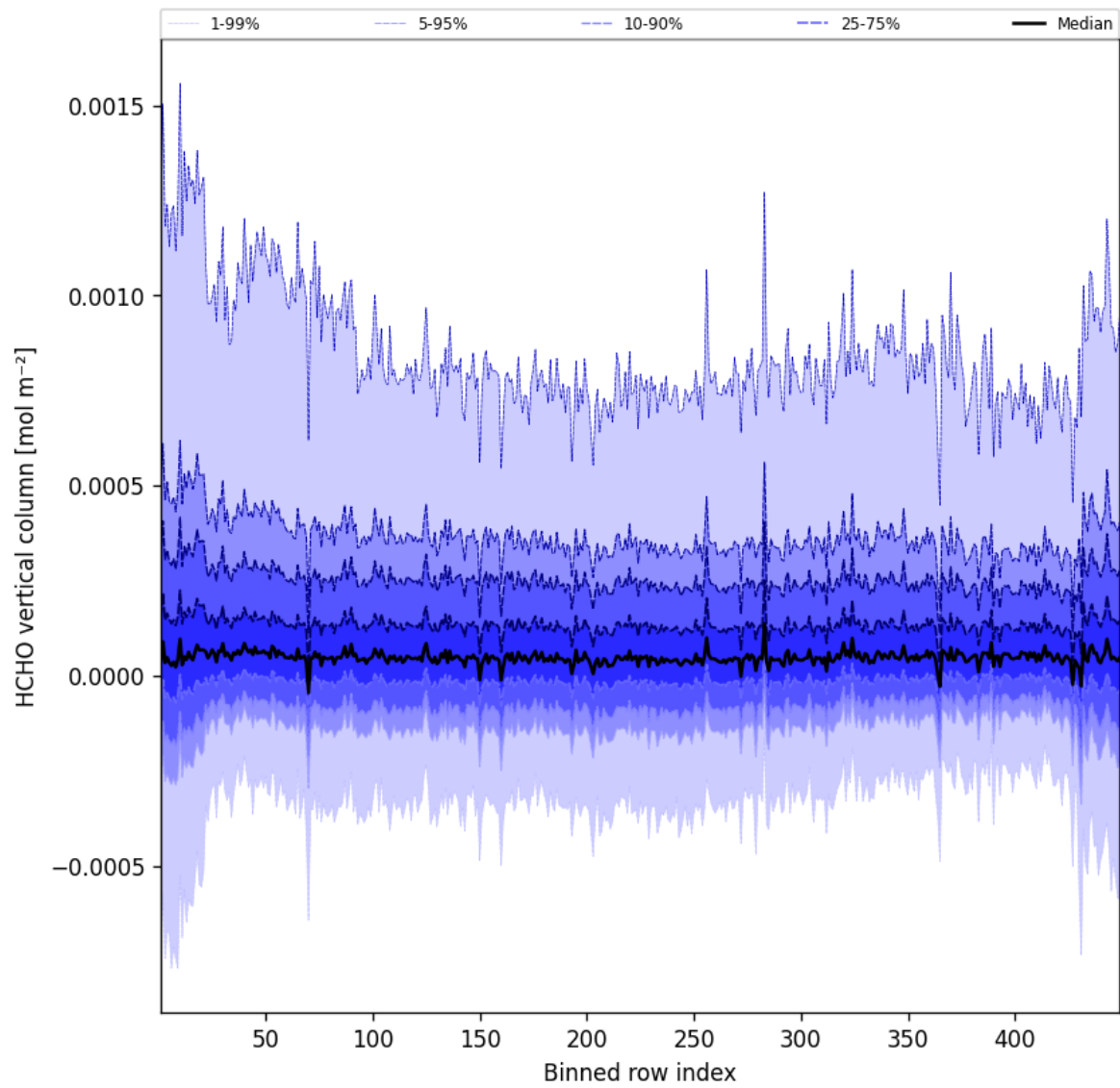
Figure 47: Along track statistics of “HCHO vertical column” for 2025-07-15 to 2025-07-16
