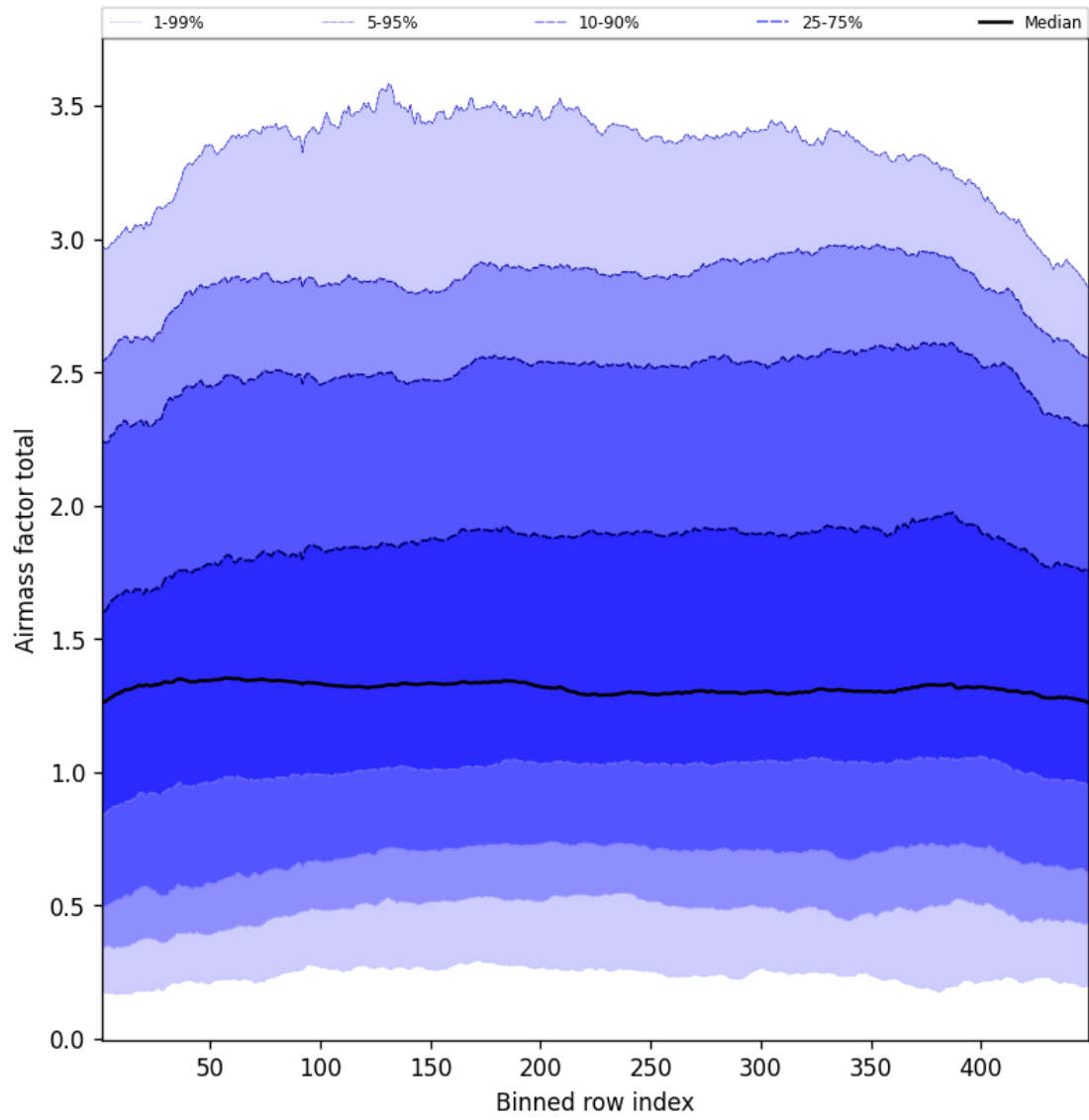
Figure 52: Along track statistics of “Airmass factor total” for 2025-07-15 to 2025-07-16
