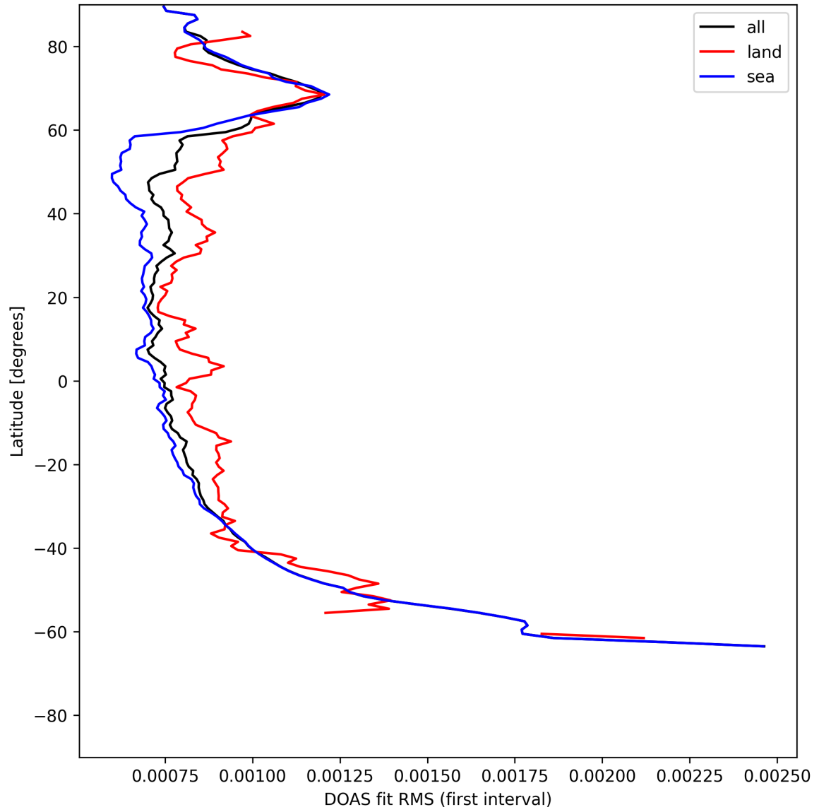
Figure 30: Zonal average of “DOAS fit RMS (first interval)” for 2025-07-15 to 2025-07-16.
