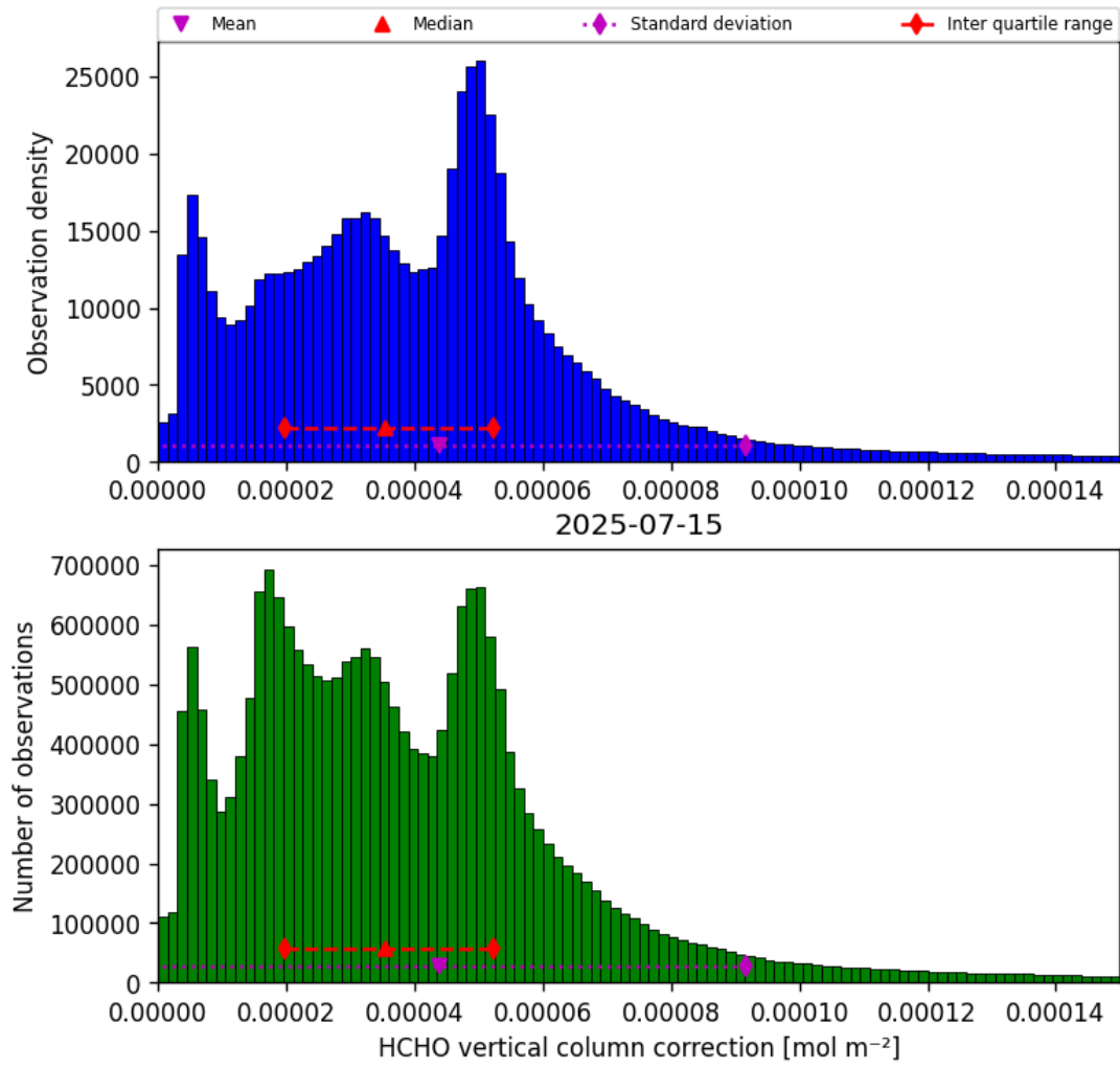
Figure 35: Histogram of “HCHO vertical column correction” for 2025-07-15 to 2025-07-16
