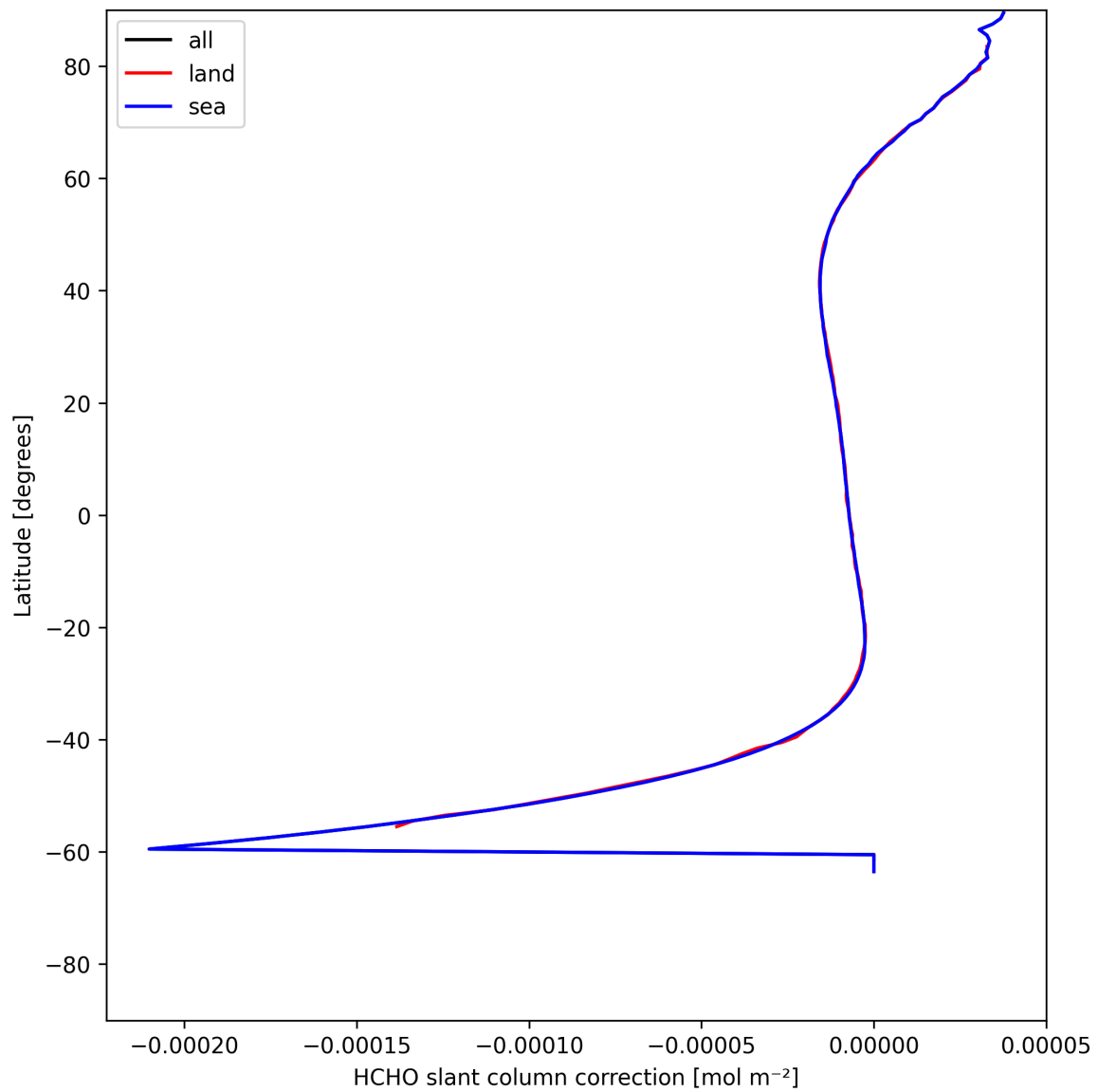
Figure 31: Zonal average of “HCHO slant column correction” for 2025-07-15 to 2025-07-16.
