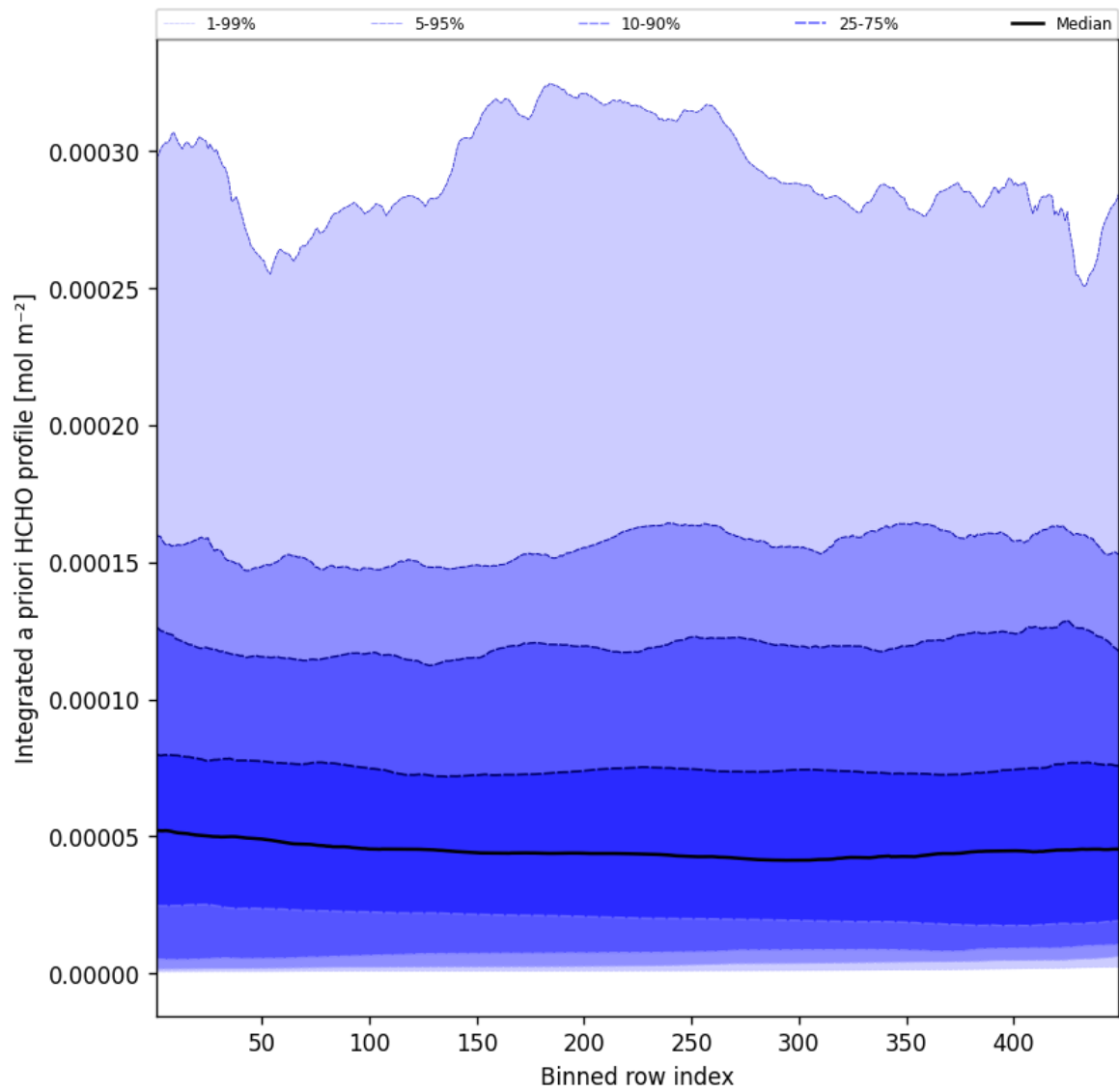
Figure 55: Along track statistics of “Integrated a priori HCHO profile” for 2025-07-15 to 2025-07-16
