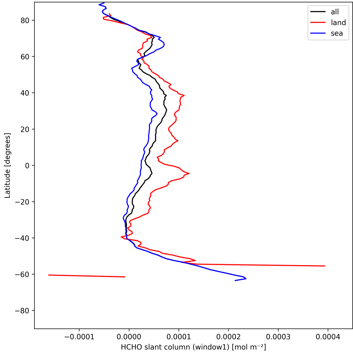
Figure 22: Zonal average of “HCHO slant column (window1)” for 2025-07-15 to 2025-07-16.
