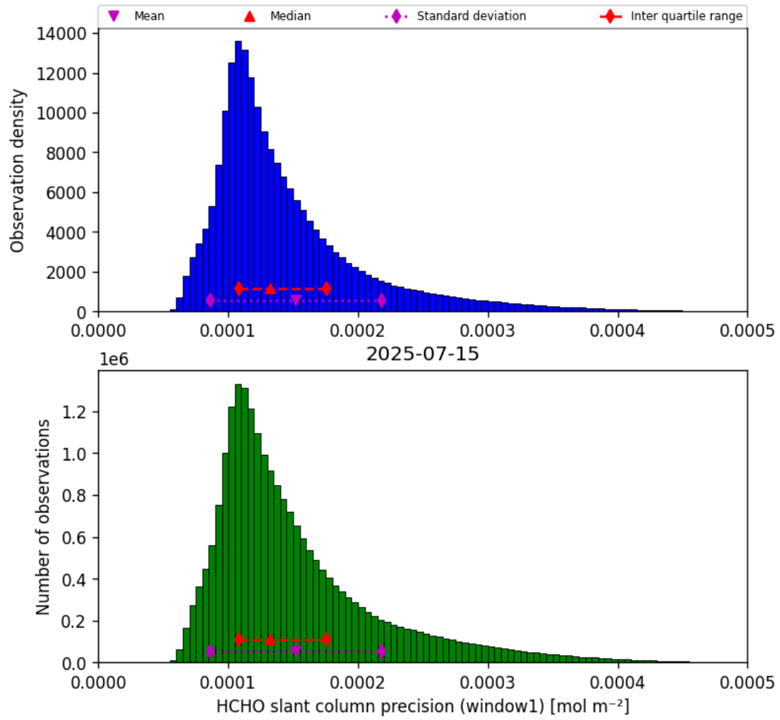
Figure 37: Histogram of “HCHO slant column precision (window1)” for 2025-07-15 to 2025-07-16
