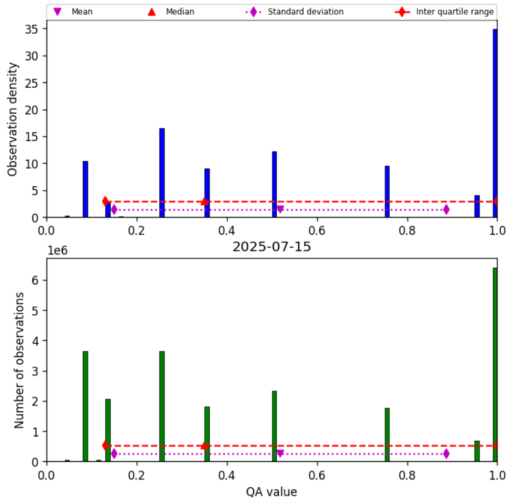
Figure 32: Histogram of “QA value” for 2025-07-15 to 2025-07-16
