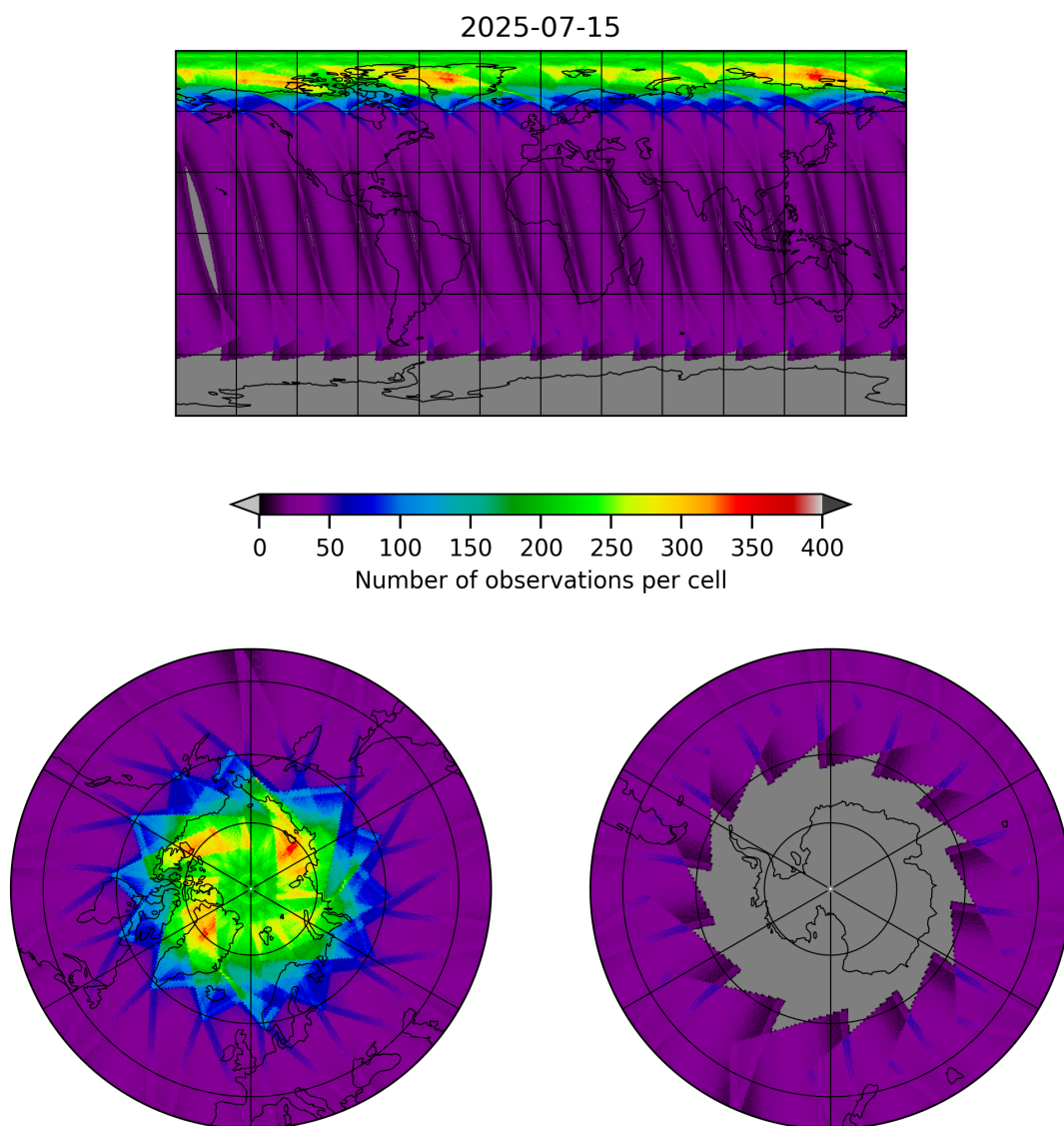
Figure 17: Map of the number of observations for 2025-07-15 to 2025-07-16
