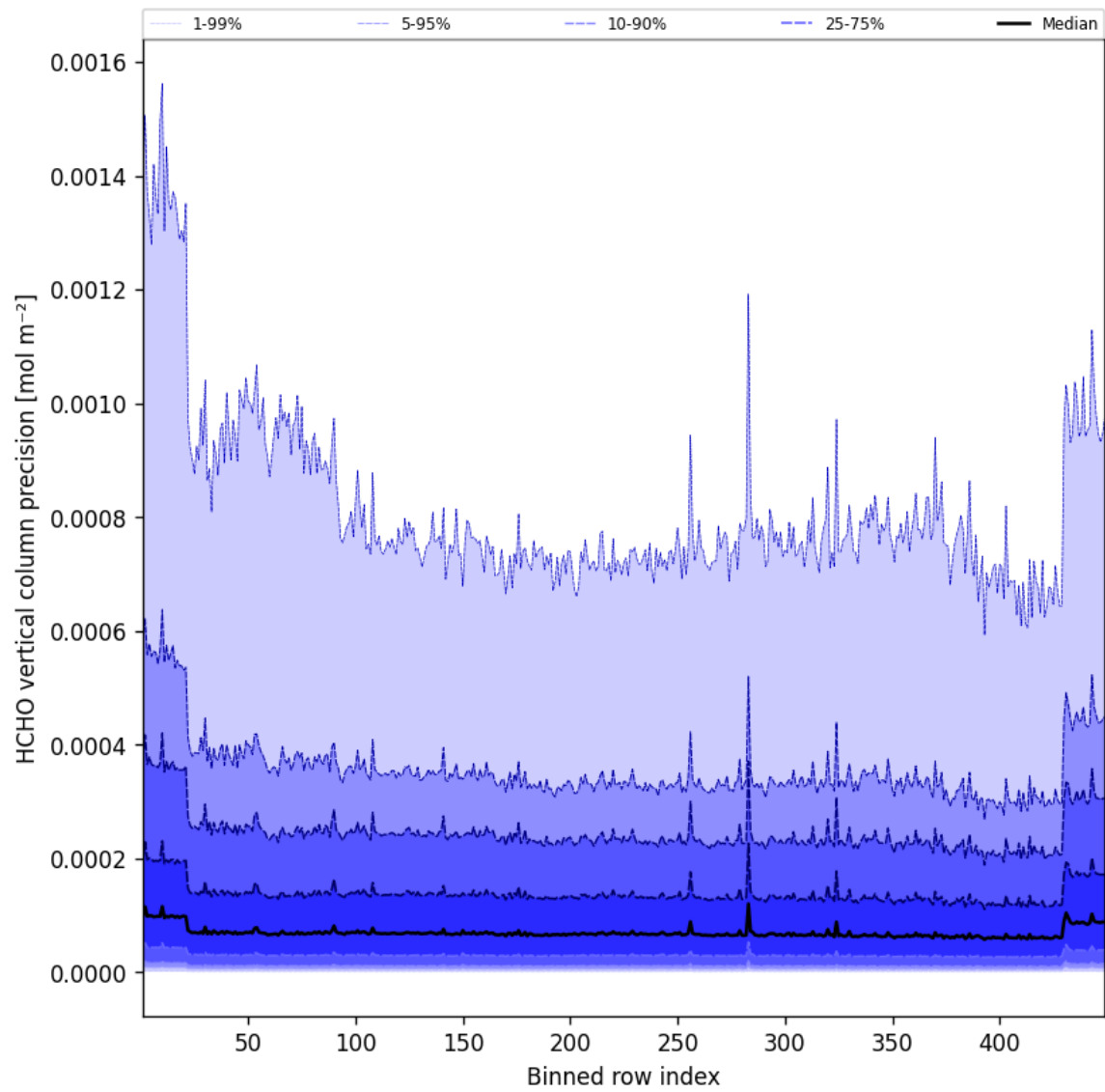
Figure 48: Along track statistics of “HCHO vertical column precision” for 2025-07-15 to 2025-07-16
