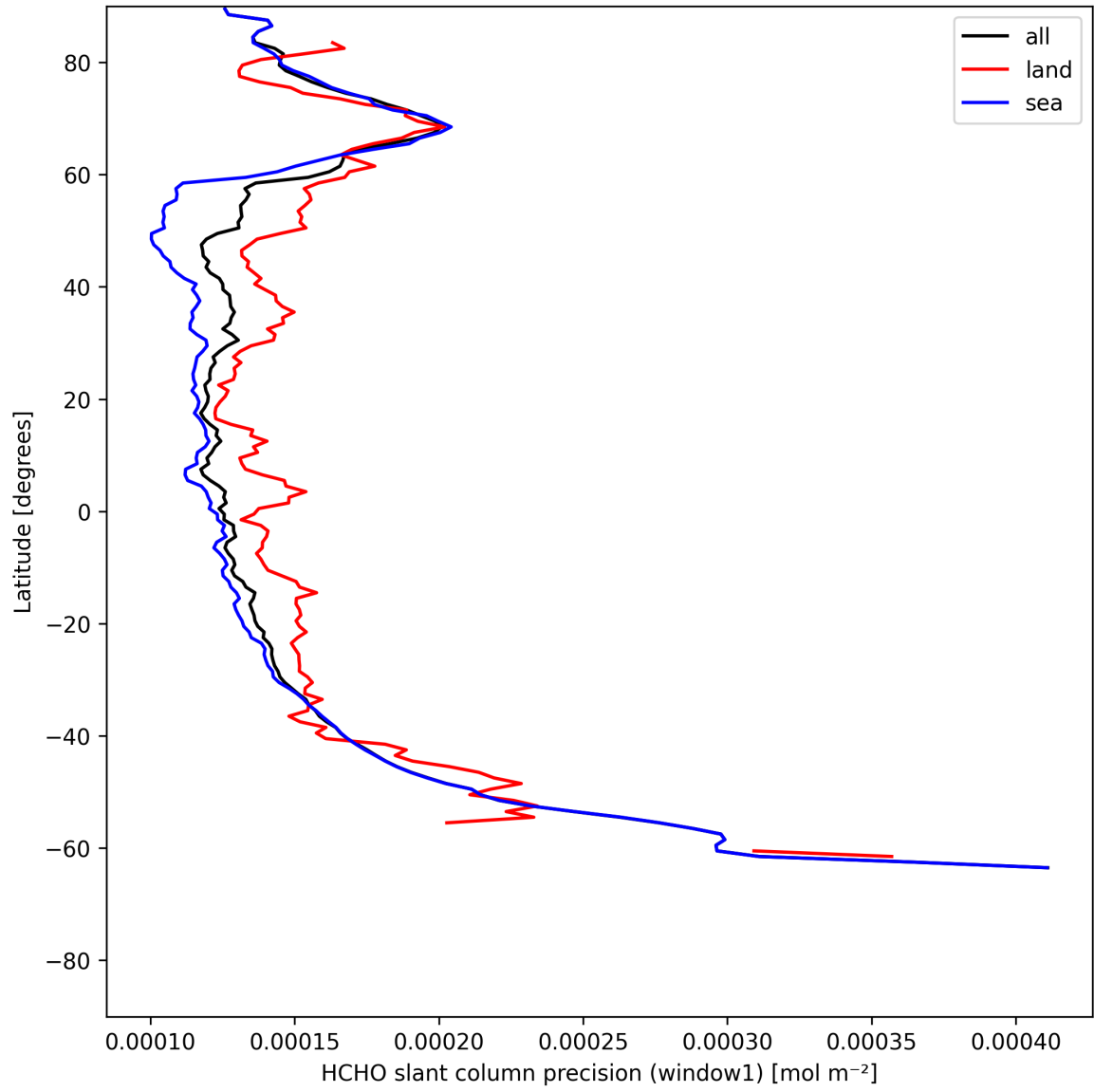
Figure 23: Zonal average of “HCHO slant column precision (window1)” for 2025-07-15 to 2025-07-16.
