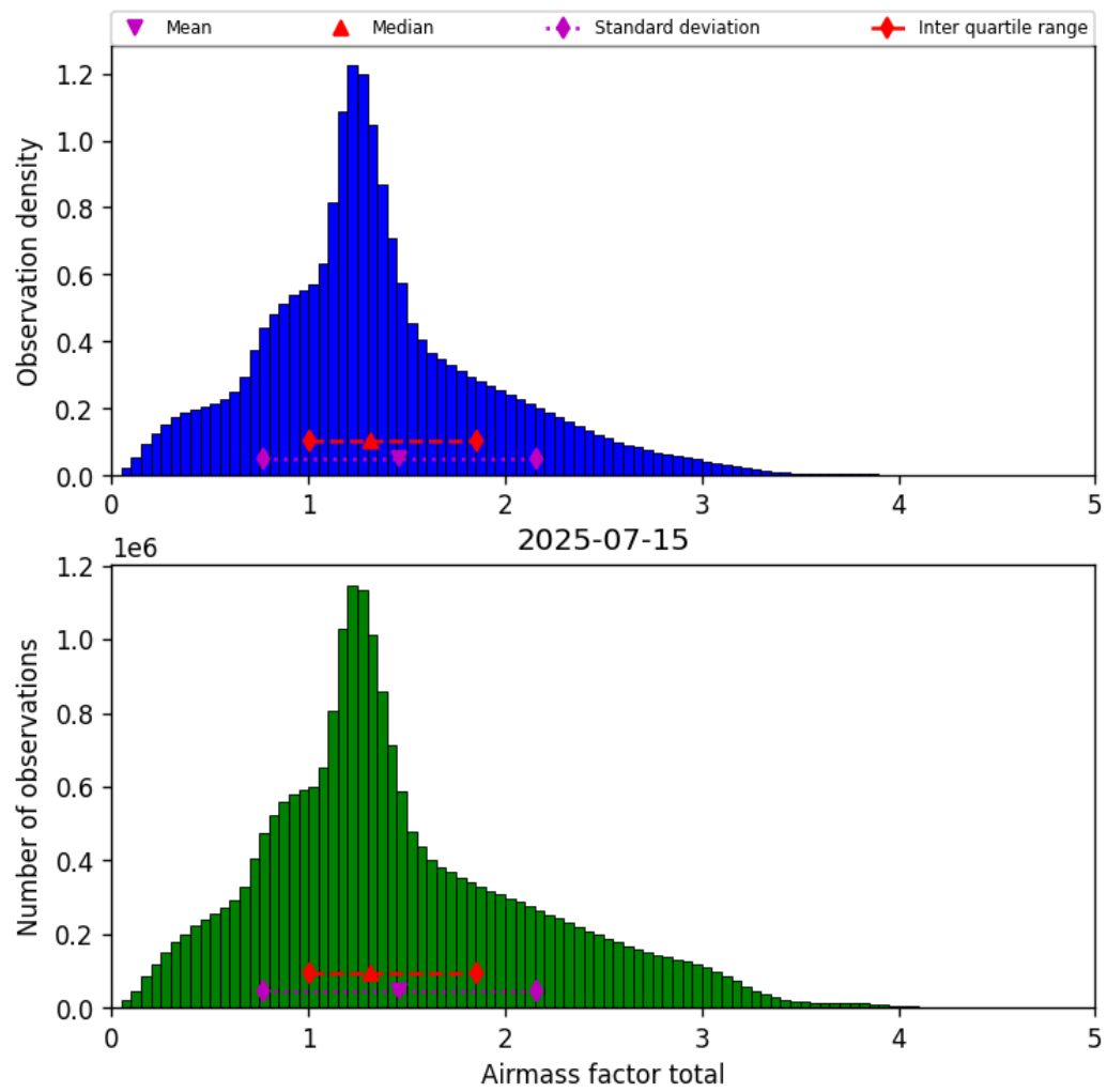
Figure 38: Histogram of “Airmass factor total” for 2025-07-15 to 2025-07-16
