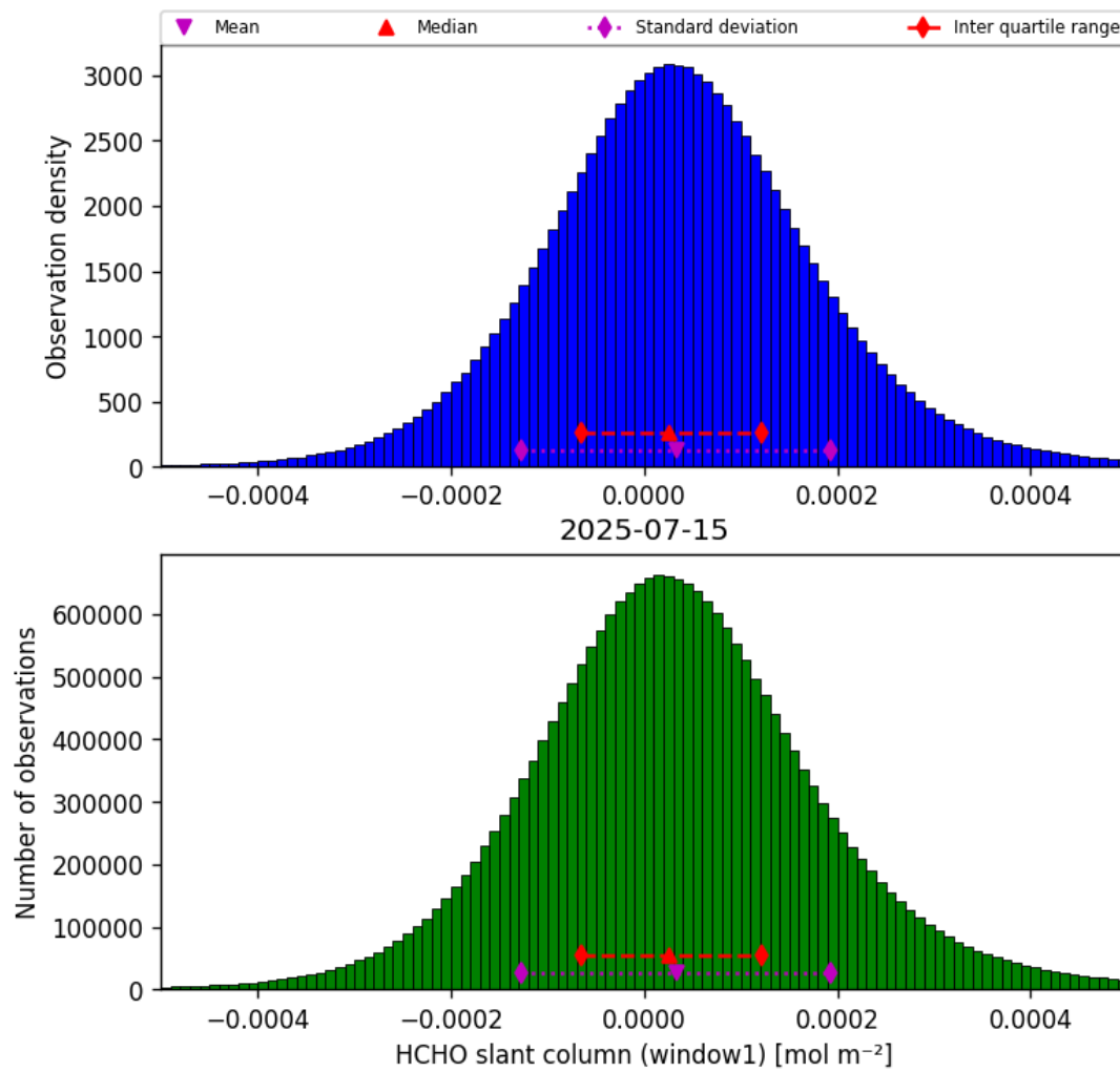
Figure 36: Histogram of “HCHO slant column (window1)” for 2025-07-15 to 2025-07-16
