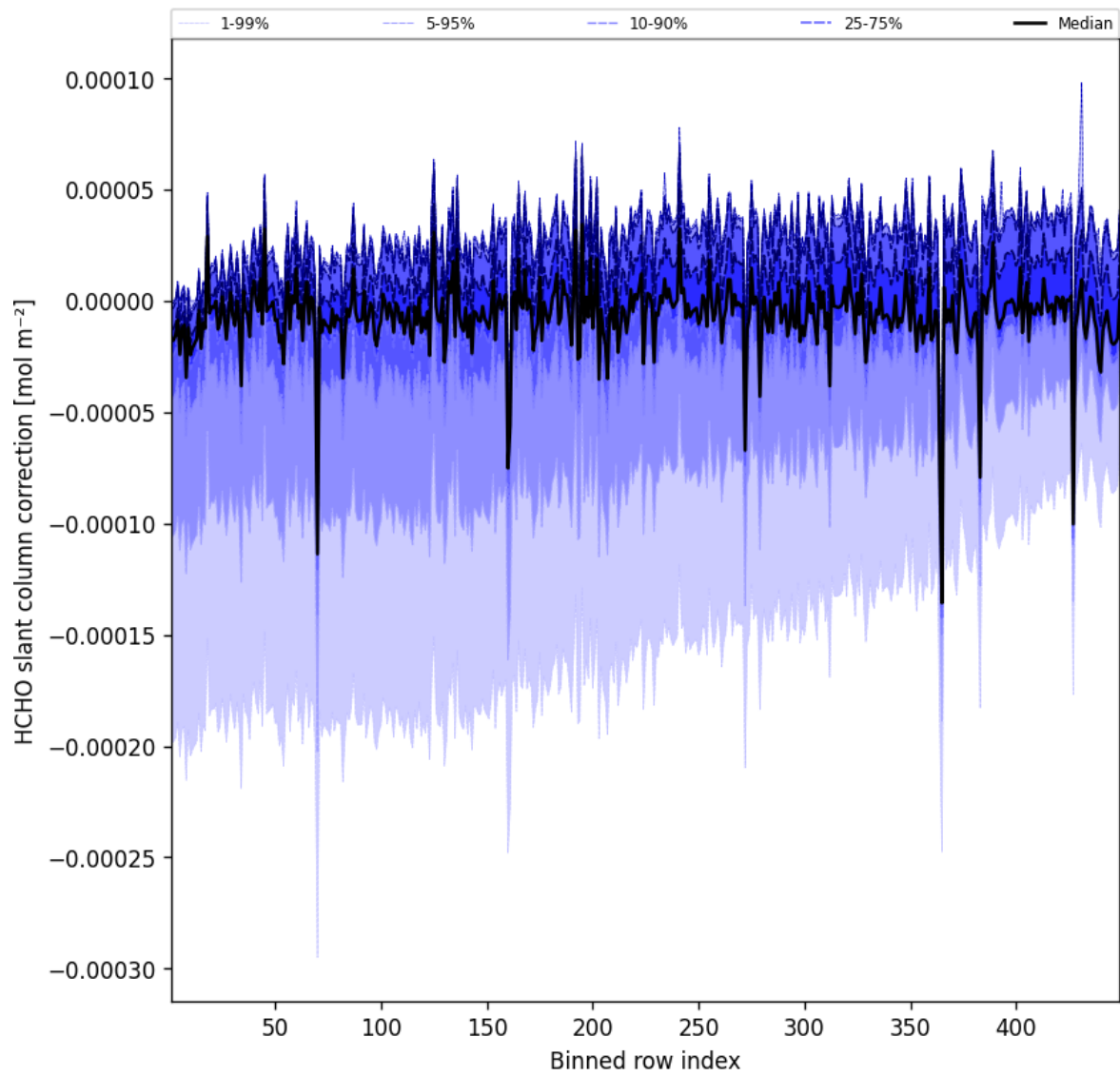
Figure 59: Along track statistics of “HCHO slant column correction” for 2025-07-15 to 2025-07-16
