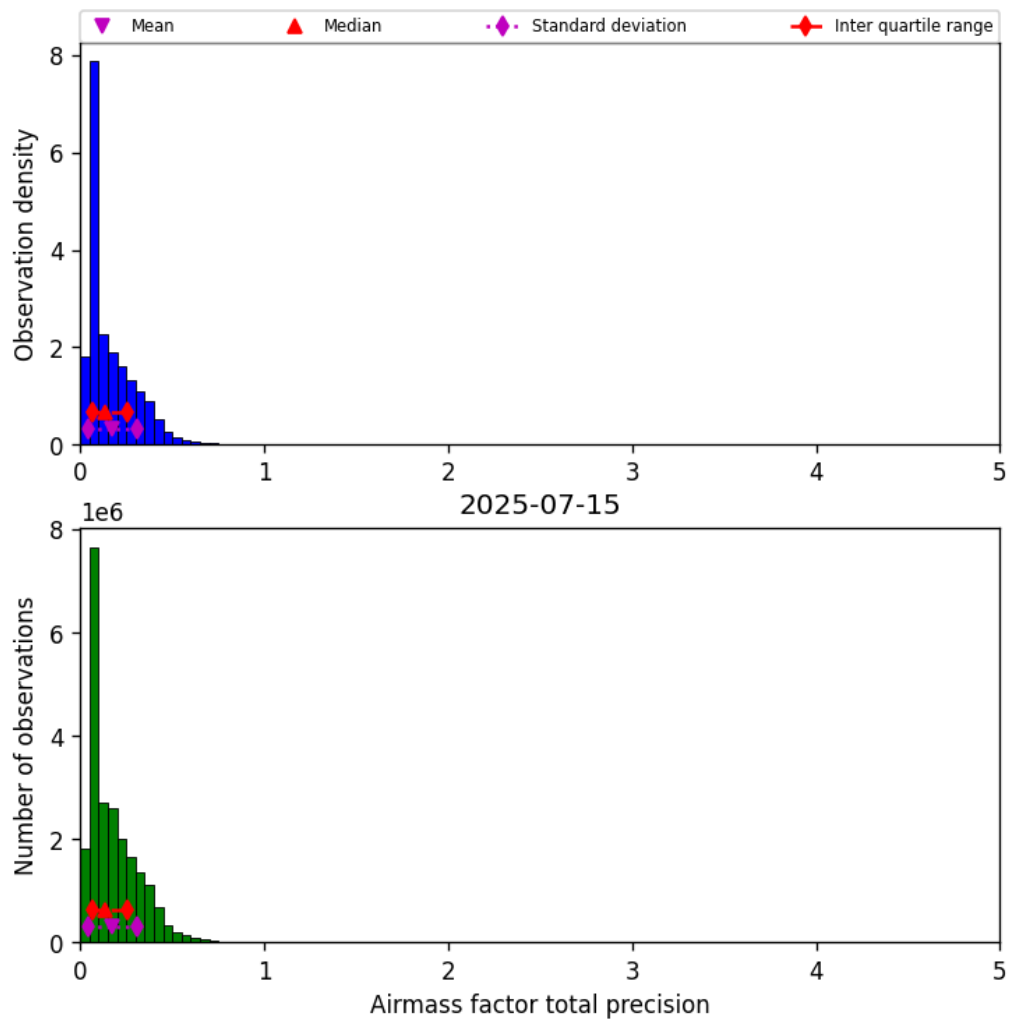
Figure 39: Histogram of “Airmass factor total precision” for 2025-07-15 to 2025-07-16
