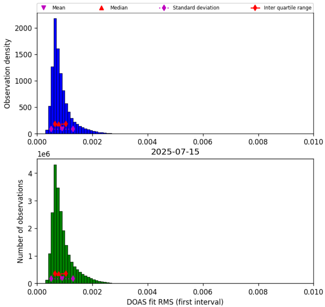
Figure 44: Histogram of “DOAS fit RMS (first interval)” for 2025-07-15 to 2025-07-16
