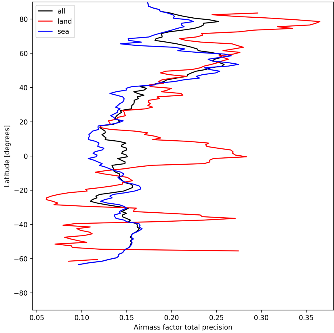
Figure 25: Zonal average of “Airmass factor total precision” for 2025-07-15 to 2025-07-16.
