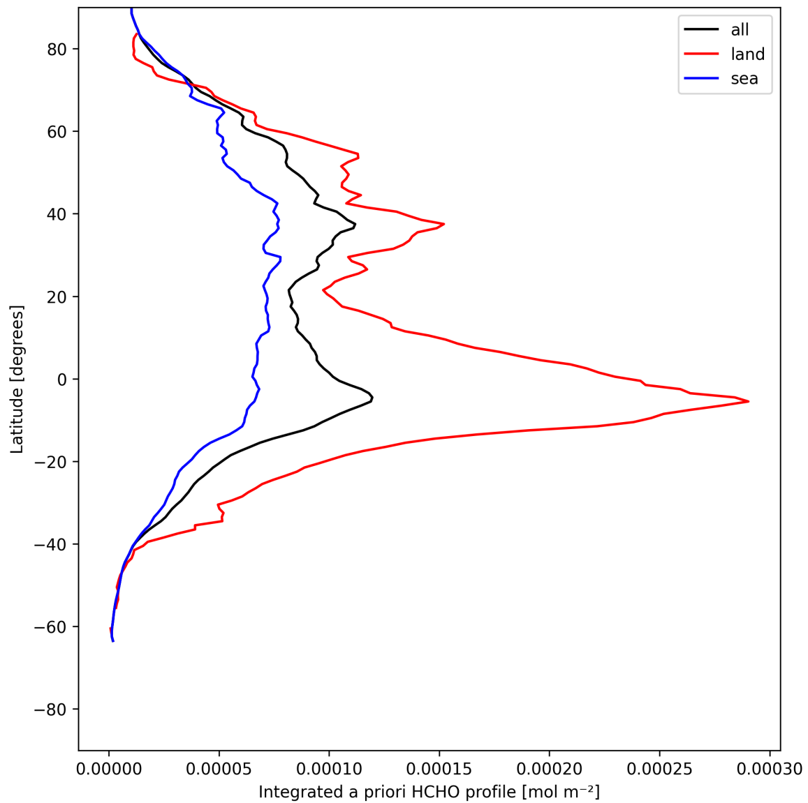
Figure 27: Zonal average of “Integrated a priori HCHO profile” for 2025-07-15 to 2025-07-16.
