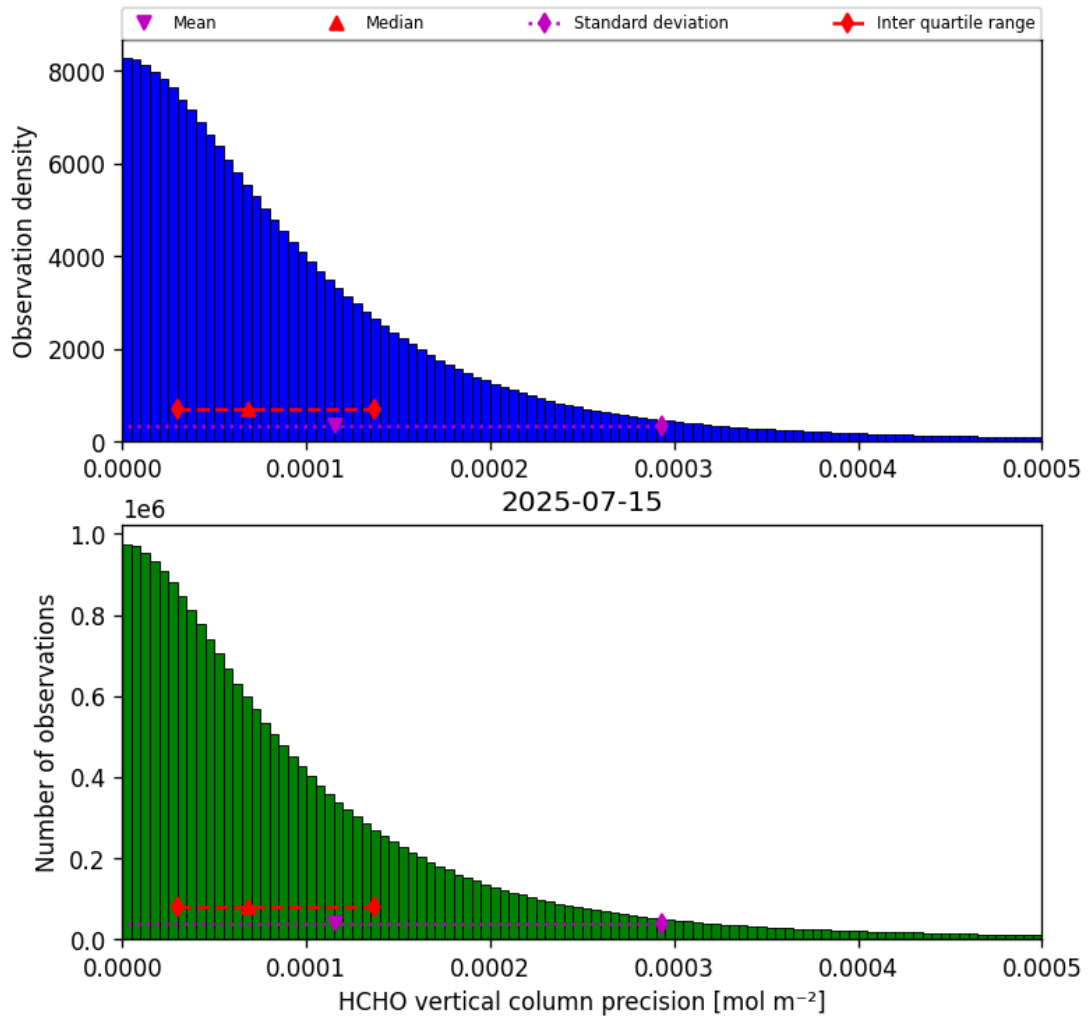
Figure 34: Histogram of “HCHO vertical column precision” for 2025-07-15 to 2025-07-16
