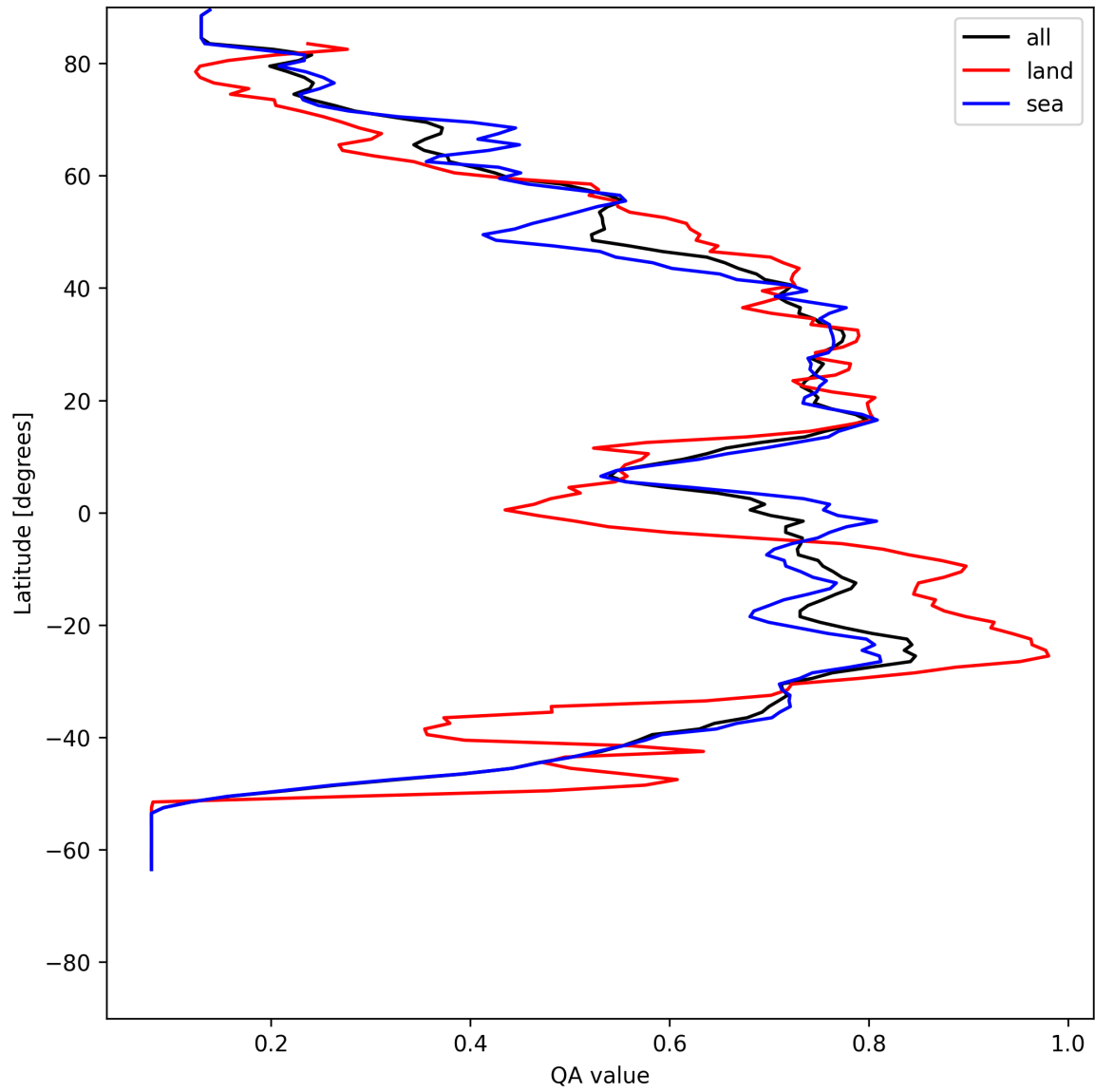
Figure 18: Zonal average of “QA value” for 2025-07-15 to 2025-07-16.
