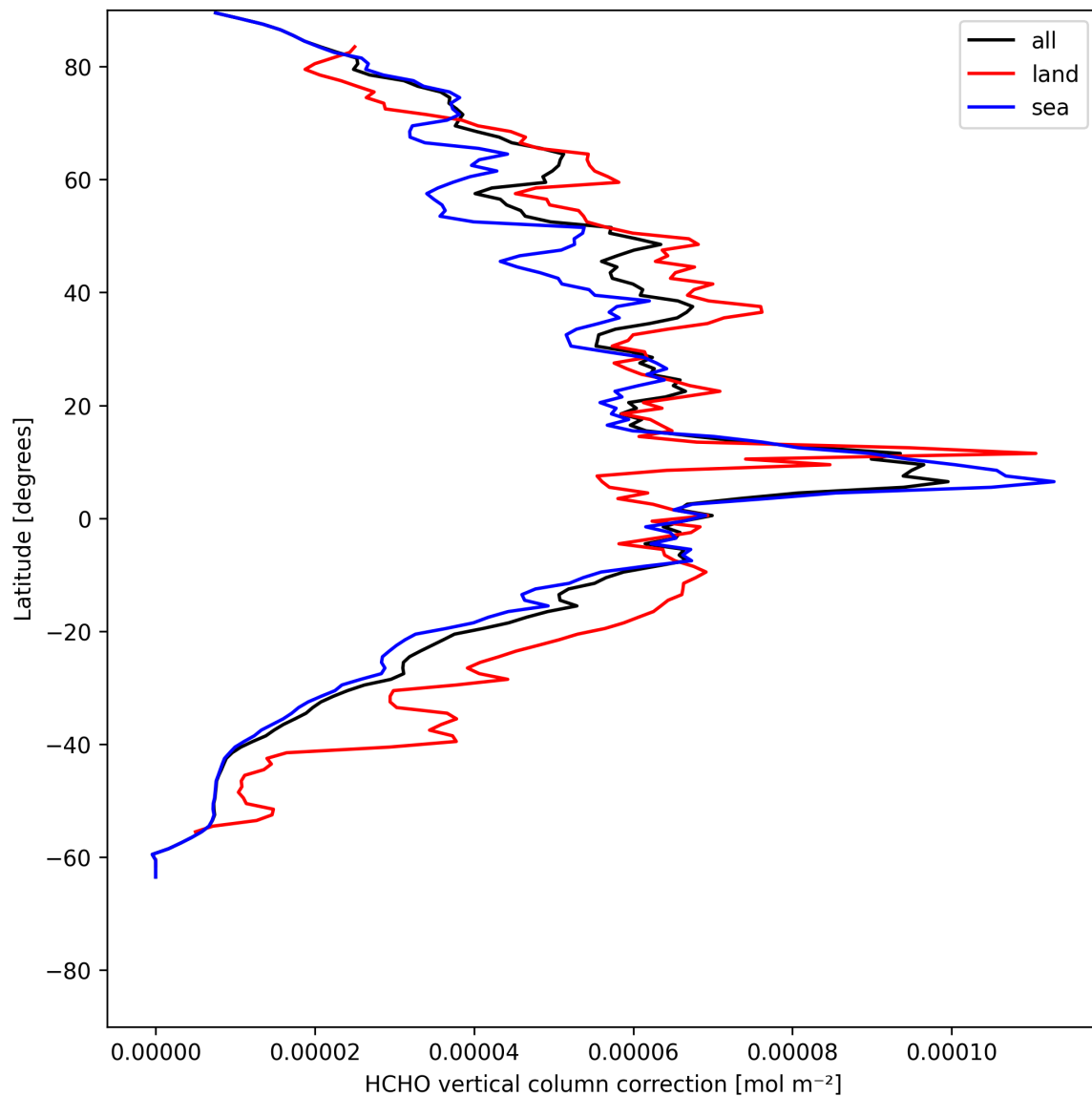
Figure 21: Zonal average of “HCHO vertical column correction” for 2025-07-15 to 2025-07-16.
