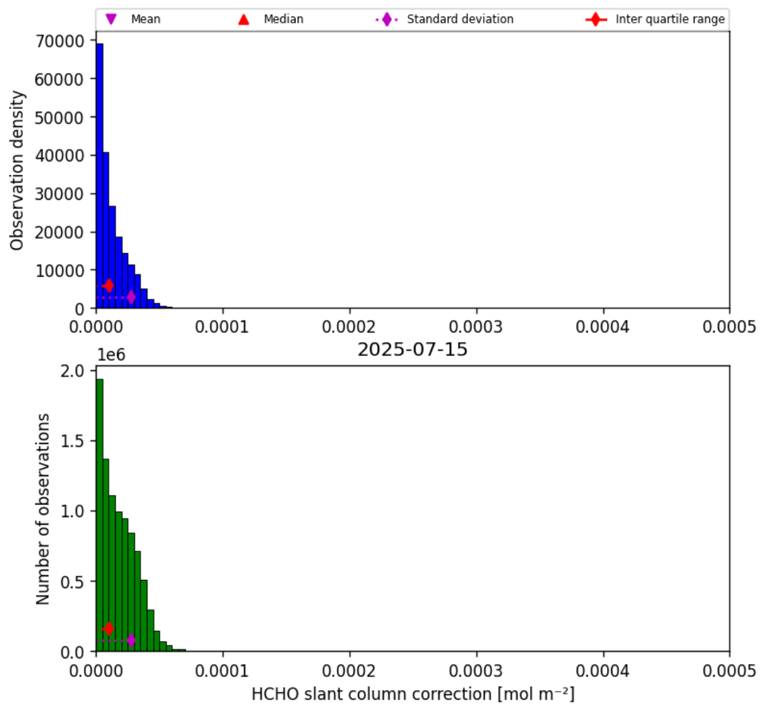
Figure 45: Histogram of “HCHO slant column correction” for 2025-07-15 to 2025-07-16
