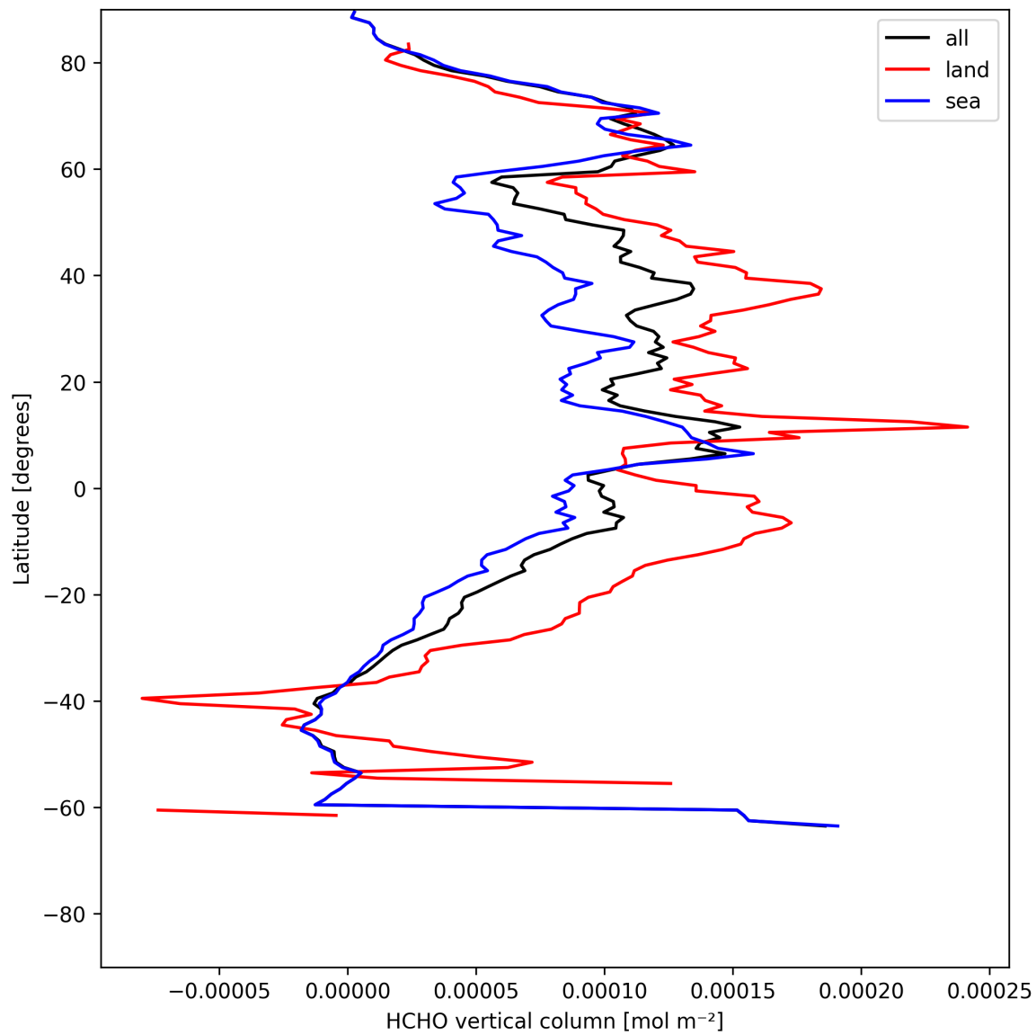
Figure 19: Zonal average of “HCHO vertical column” for 2025-07-15 to 2025-07-16.
