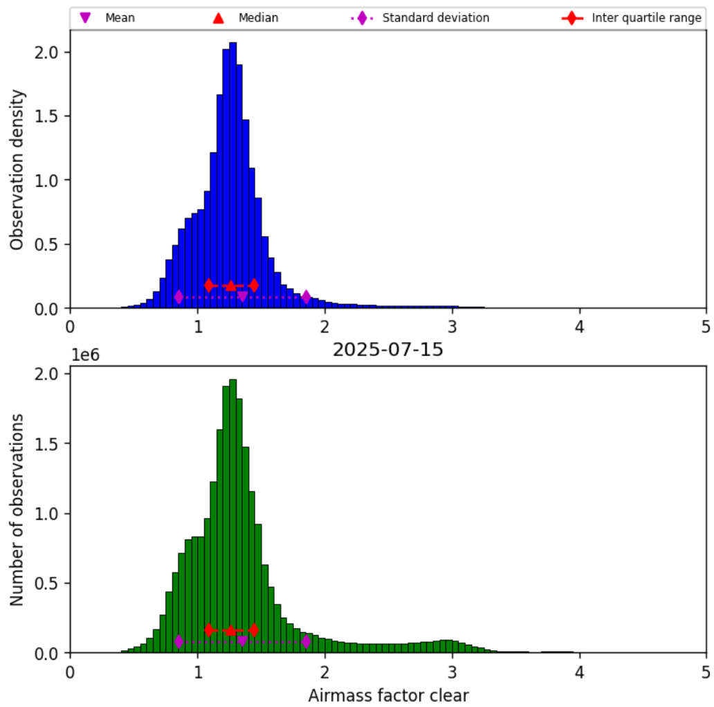
Figure 40: Histogram of “Airmass factor clear” for 2025-07-15 to 2025-07-16
