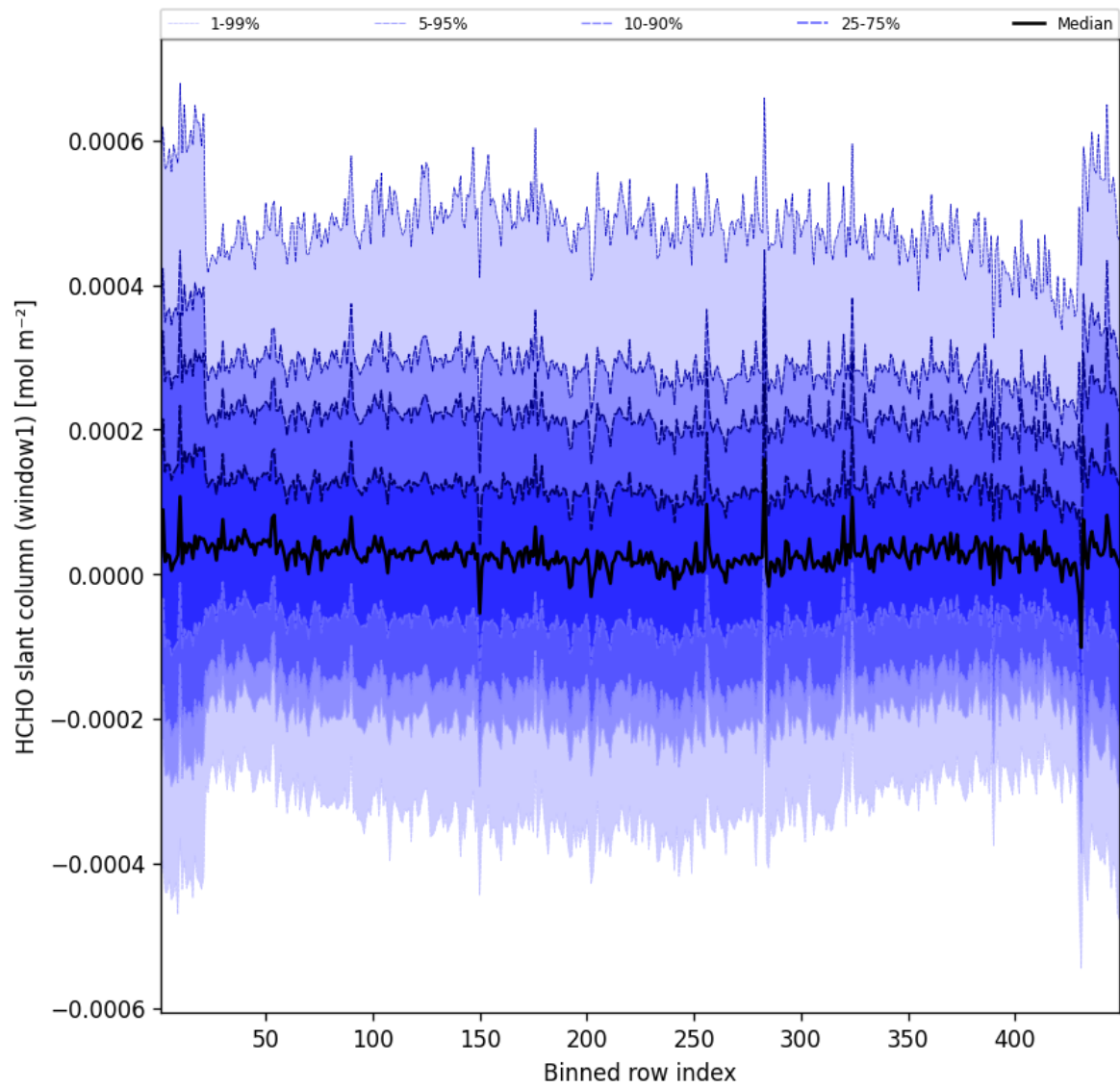
Figure 50: Along track statistics of “HCHO slant column (window1)” for 2025-07-15 to 2025-07-16
