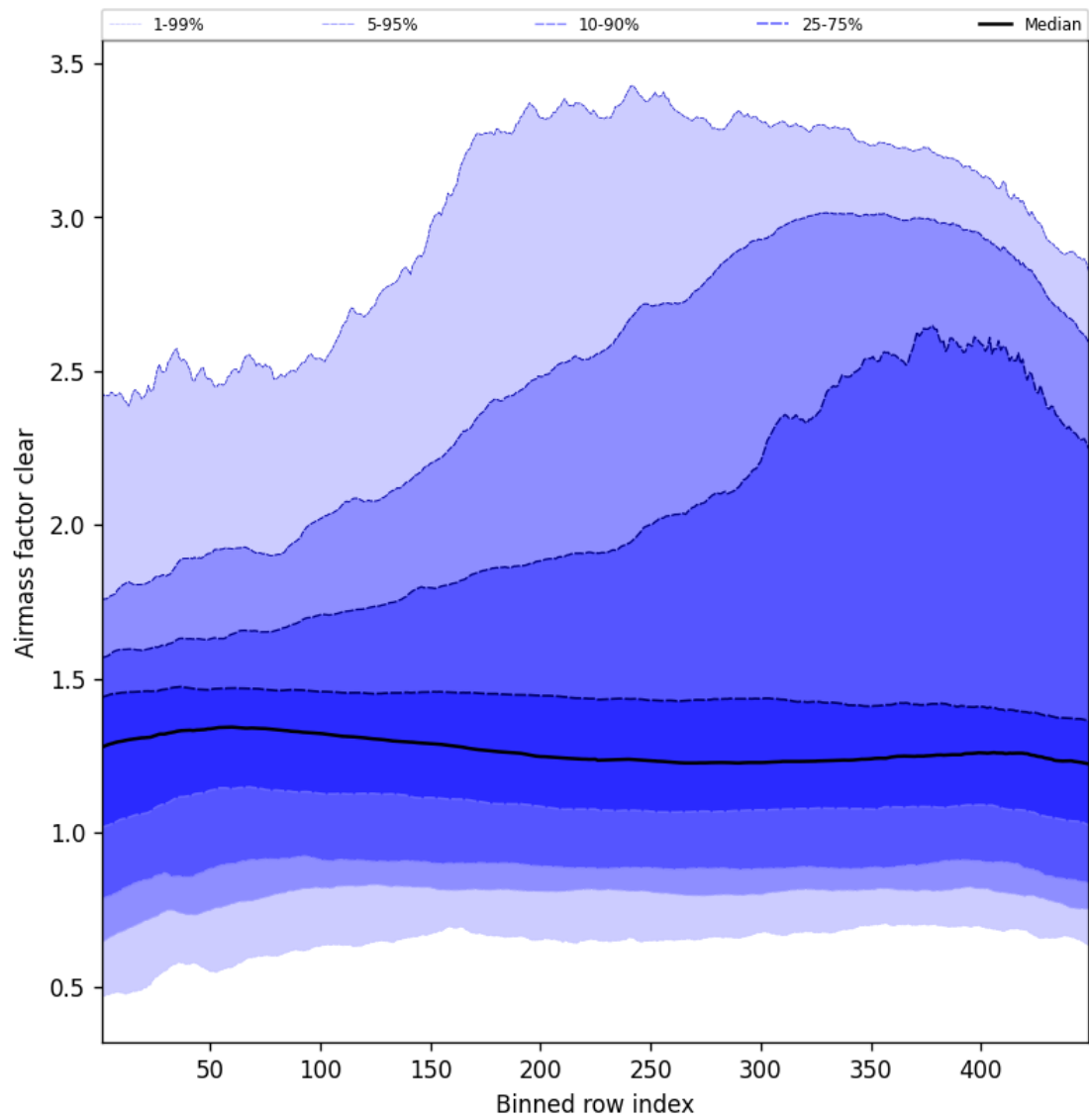
Figure 54: Along track statistics of “Airmass factor clear” for 2025-07-15 to 2025-07-16
