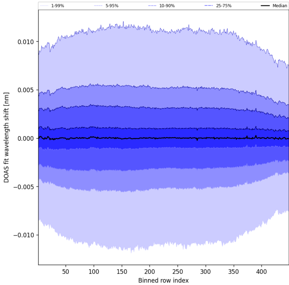
Figure 56: Along track statistics of “DOAS fit wavelength shift” for 2025-07-15 to 2025-07-16
