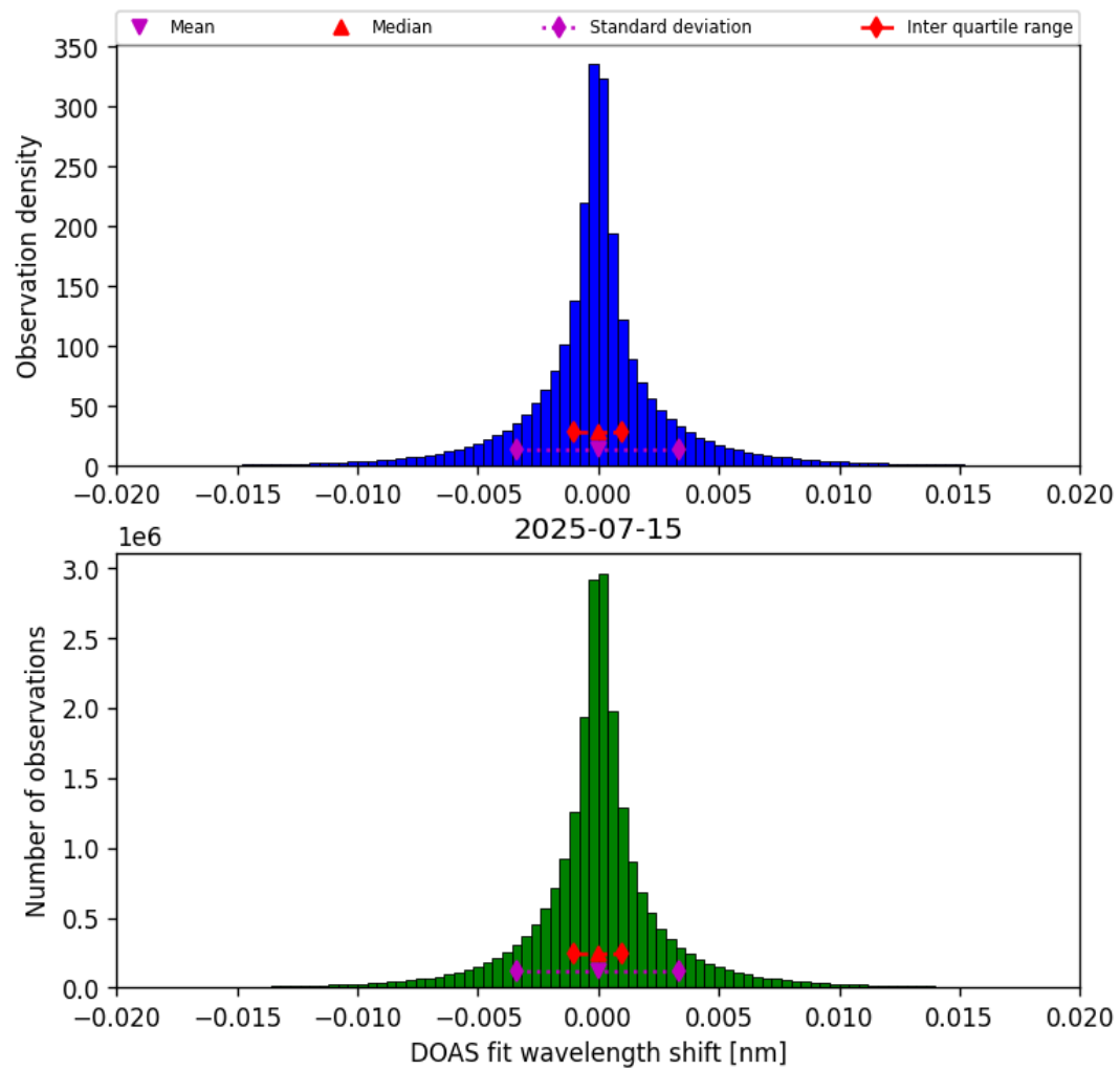
Figure 42: Histogram of “DOAS fit wavelength shift” for 2025-07-15 to 2025-07-16
