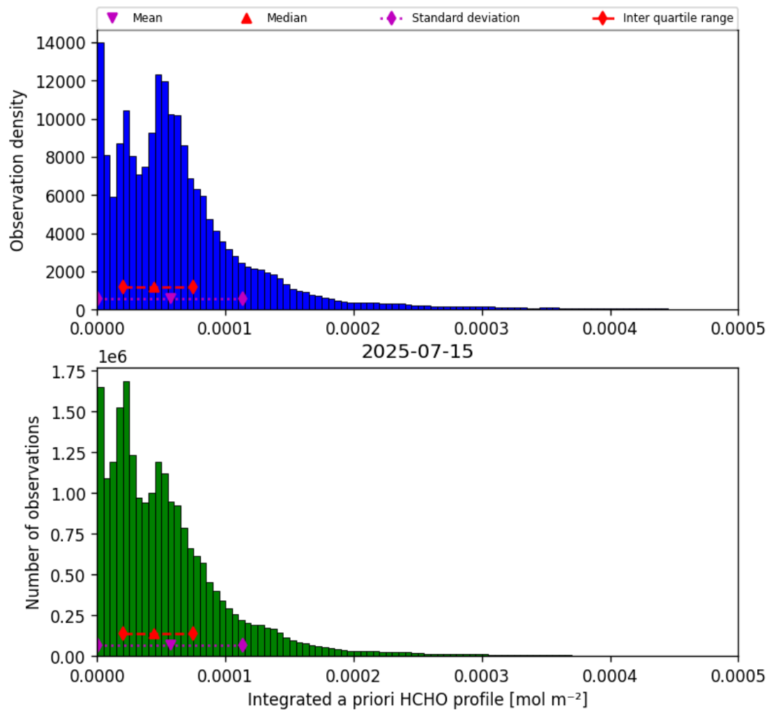
Figure 41: Histogram of “Integrated a priori HCHO profile” for 2025-07-15 to 2025-07-16
