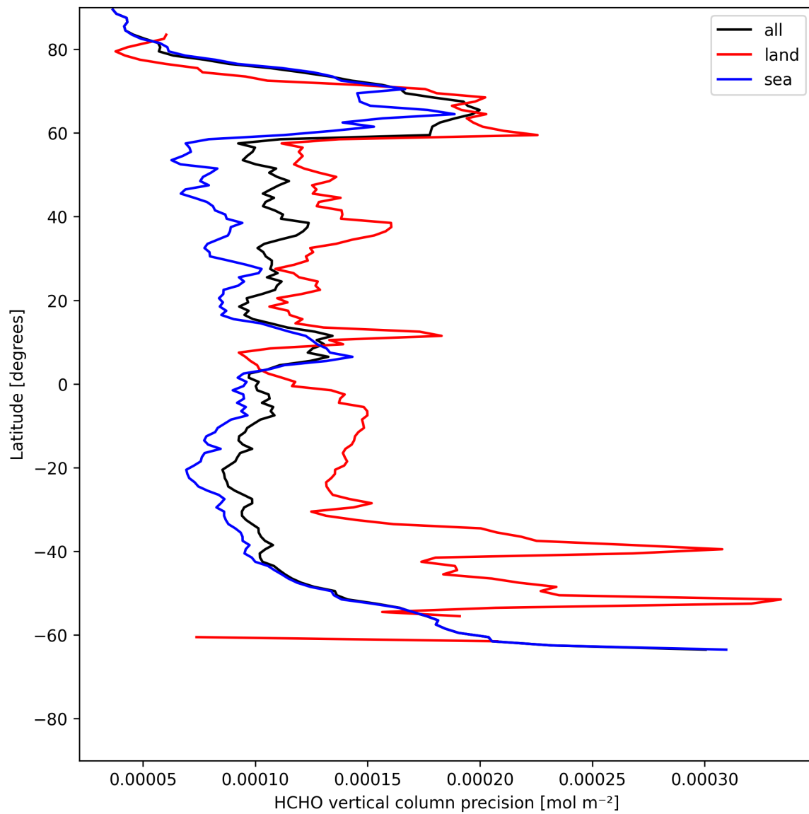
Figure 20: Zonal average of “HCHO vertical column precision” for 2025-07-15 to 2025-07-16.
