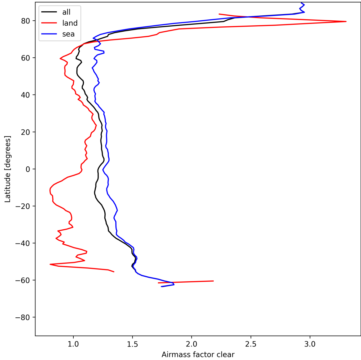
Figure 26: Zonal average of “Airmass factor clear” for 2025-07-15 to 2025-07-16.
