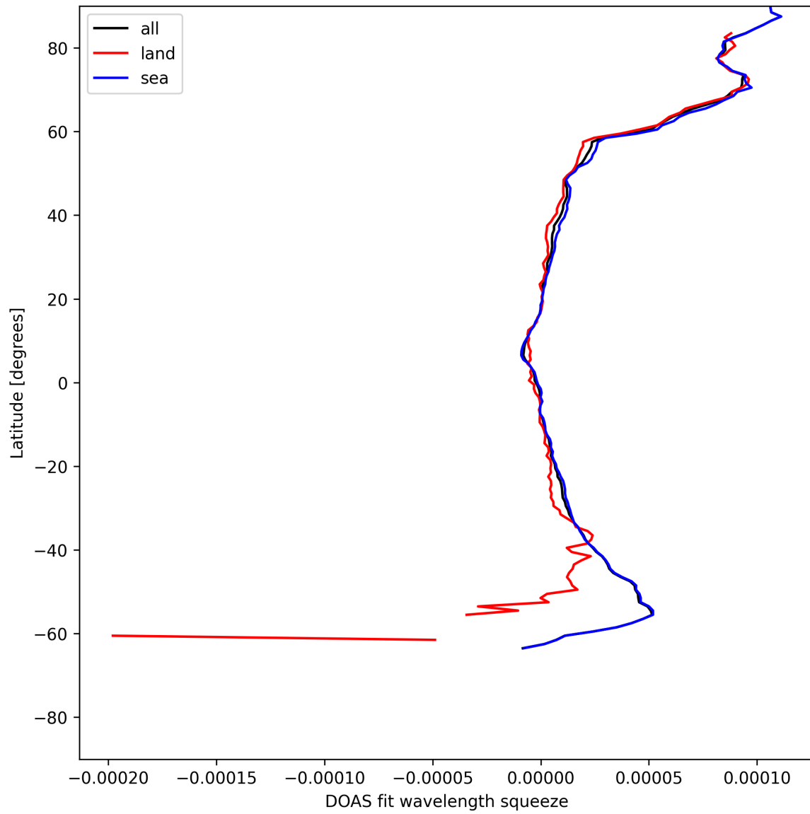
Figure 29: Zonal average of “DOAS fit wavelength squeeze” for 2025-07-15 to 2025-07-16.
