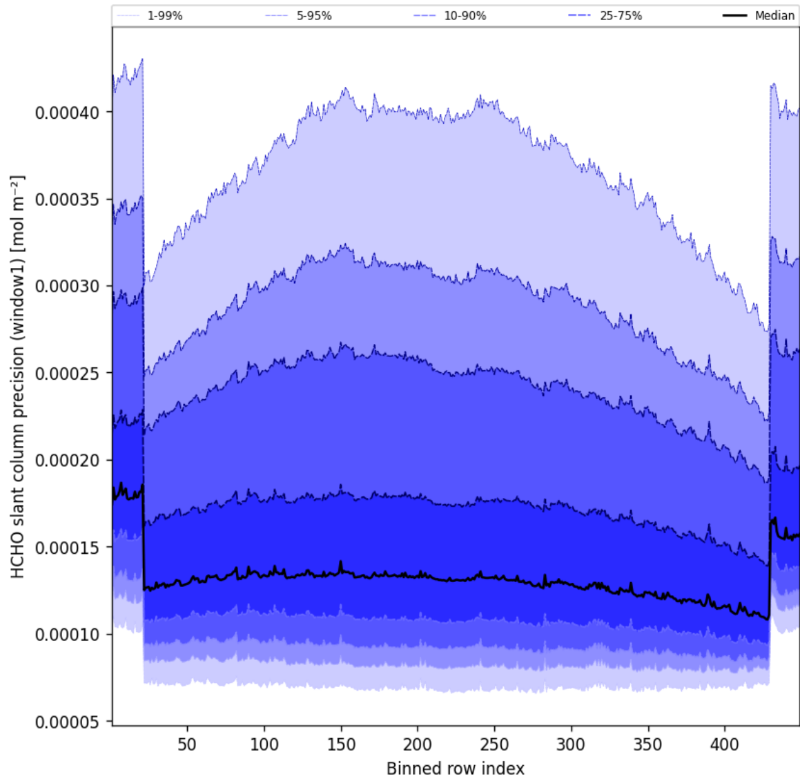
Figure 51: Along track statistics of “HCHO slant column precision (window1)” for 2025-07-15 to 2025-07-16
