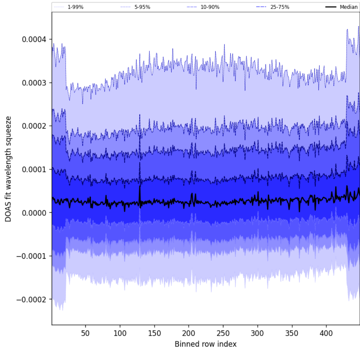
Figure 57: Along track statistics of “DOAS fit wavelength squeeze” for 2025-07-15 to 2025-07-16
