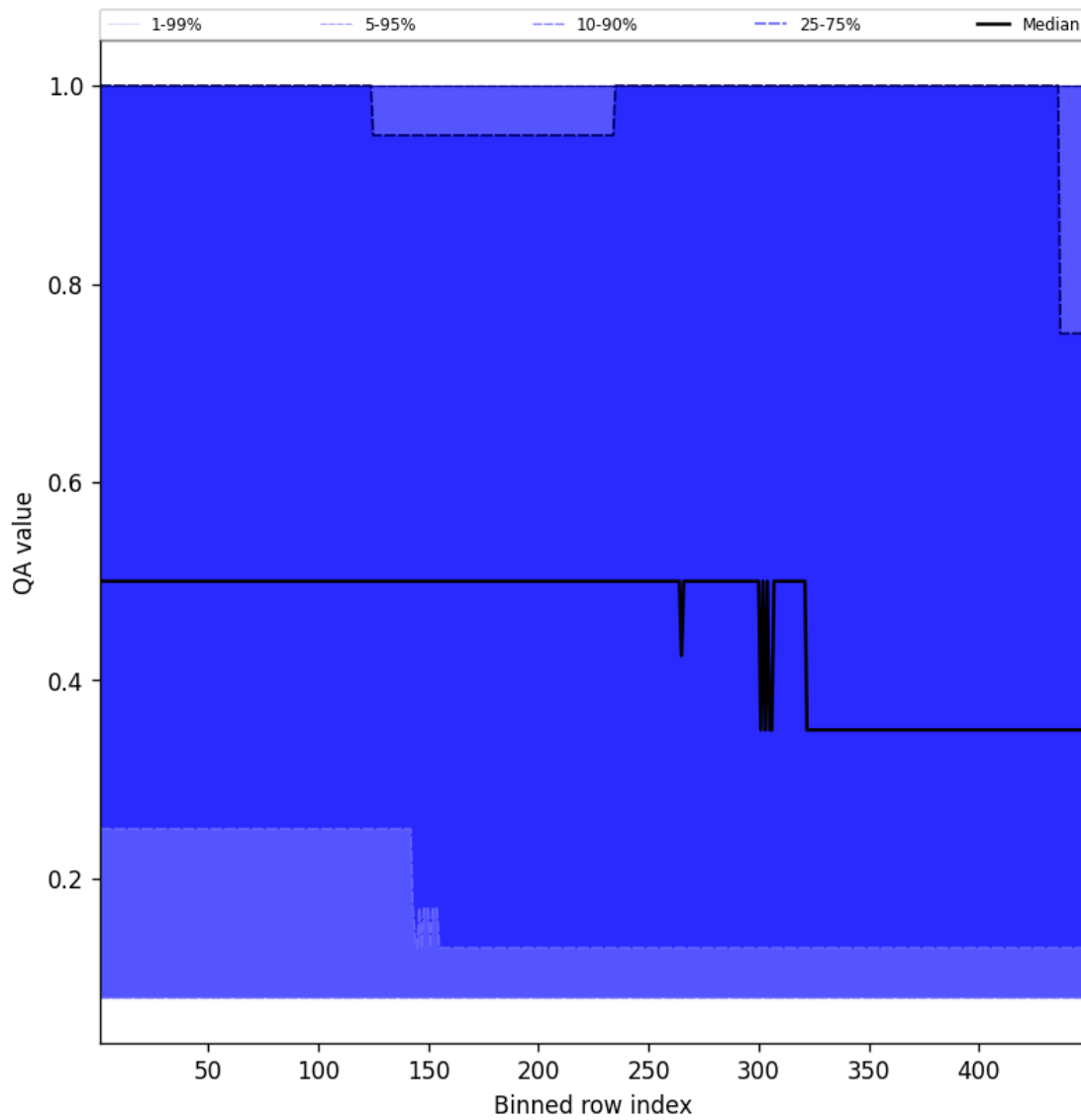
Figure 46: Along track statistics of “QA value” for 2025-07-15 to 2025-07-16
