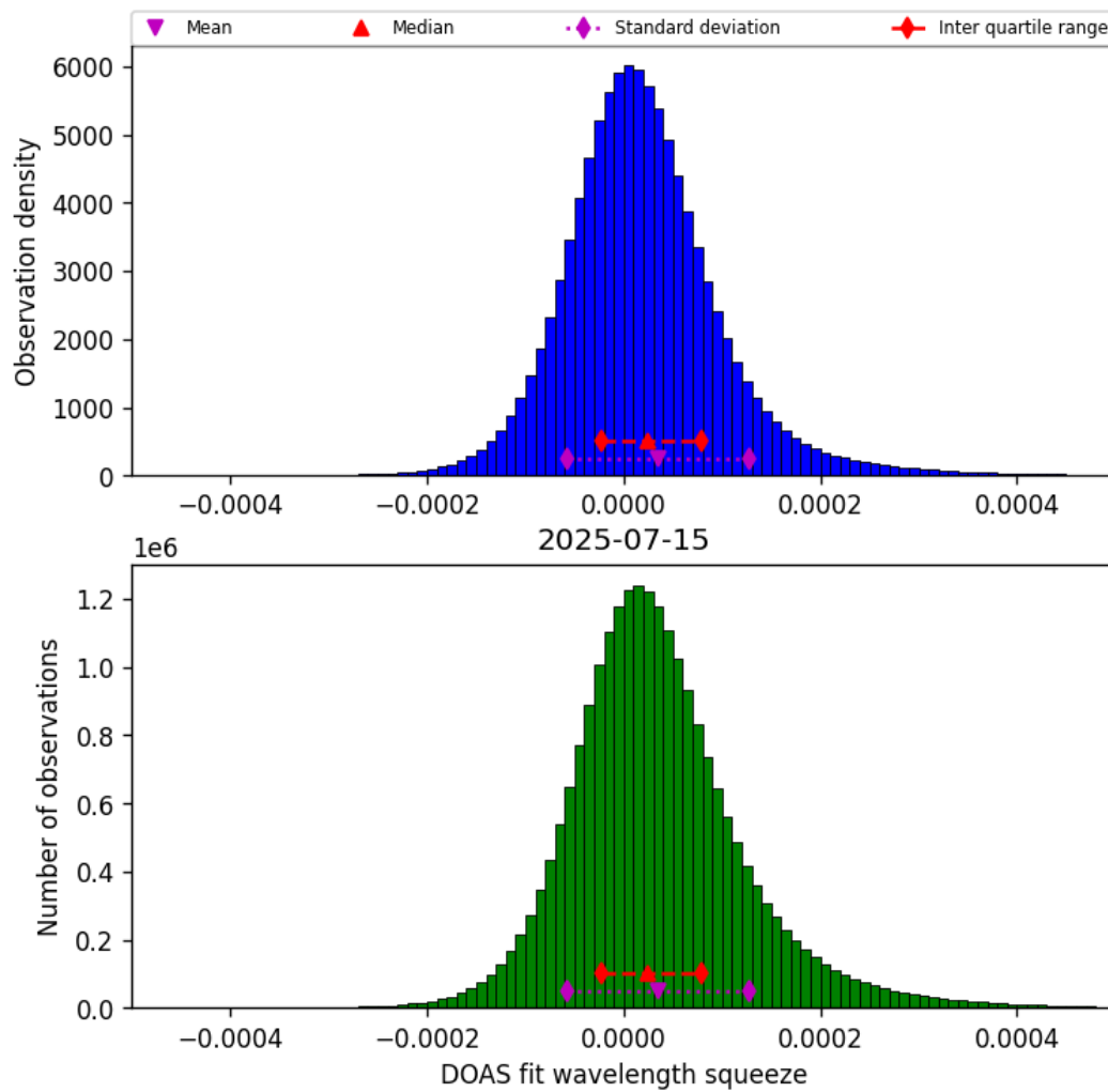
Figure 43: Histogram of “DOAS fit wavelength squeeze” for 2025-07-15 to 2025-07-16
