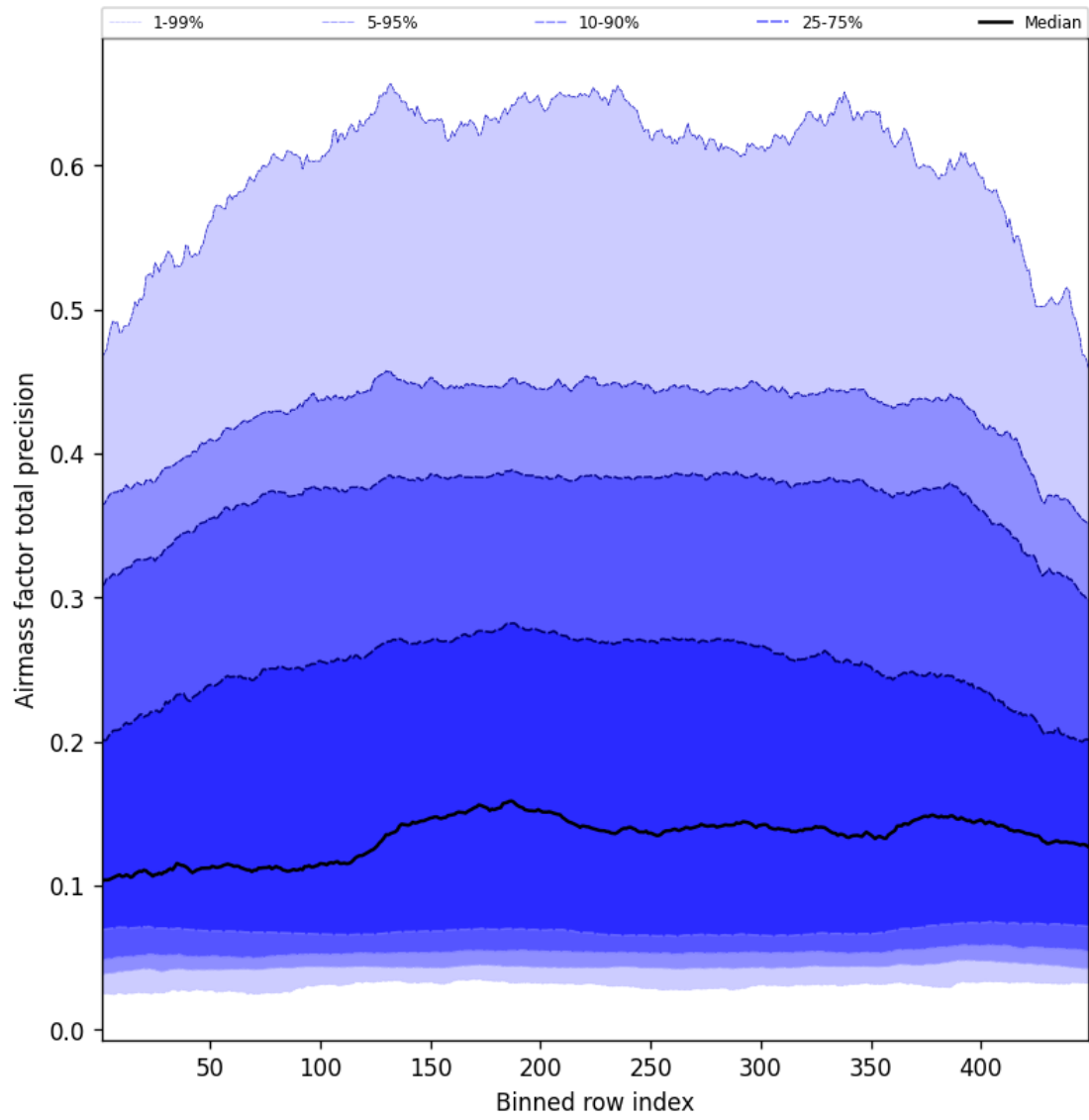
Figure 53: Along track statistics of “Airmass factor total precision” for 2025-07-15 to 2025-07-16
