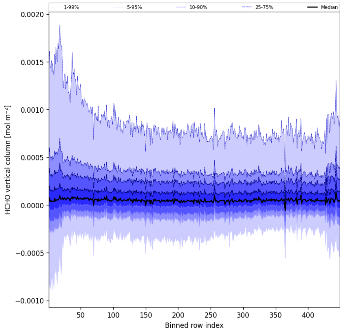
Figure 47: Along track statistics of “HCHO vertical column” for 2025-07-16 to 2025-07-16
