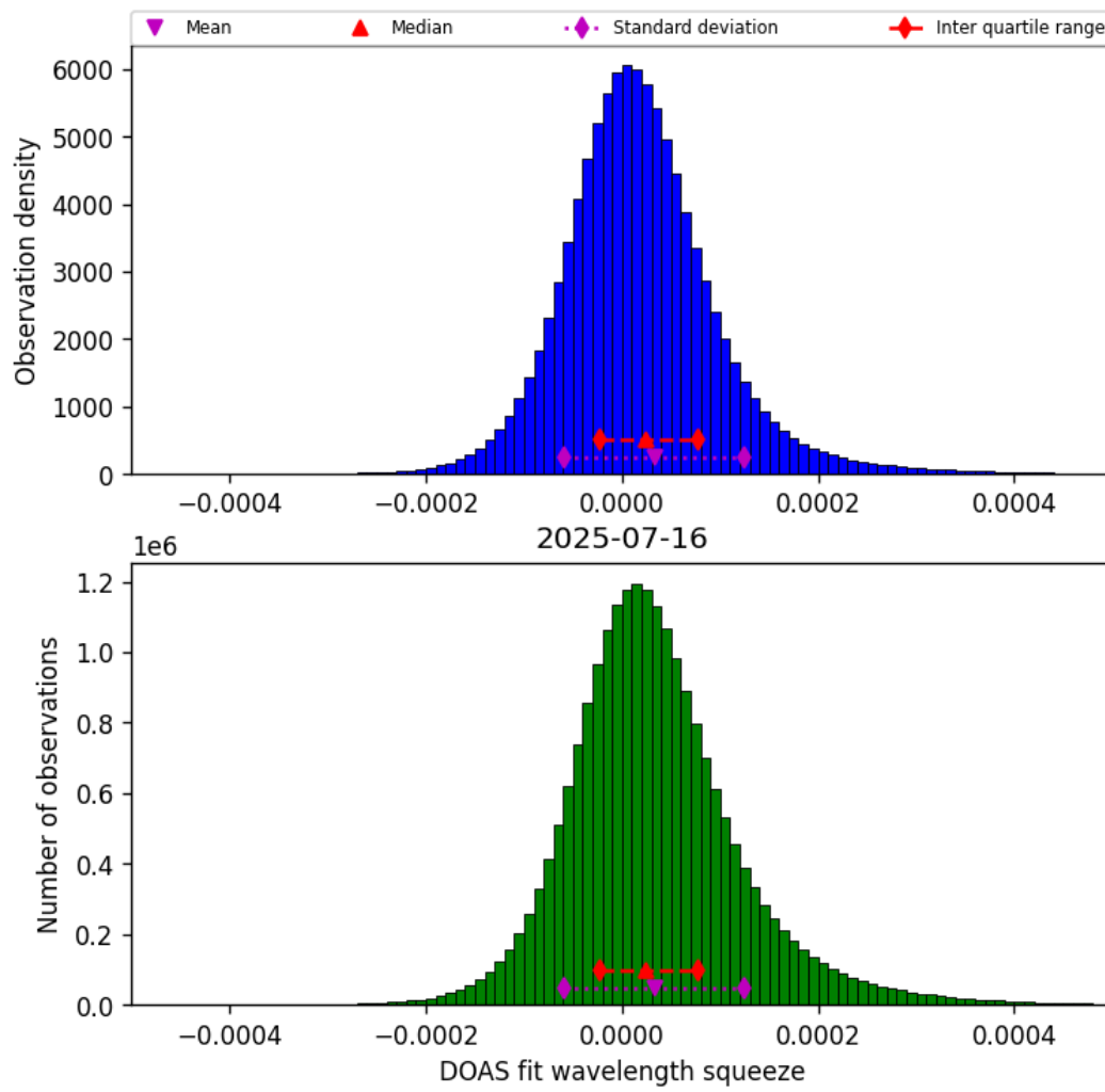
Figure 43: Histogram of “DOAS fit wavelength squeeze” for 2025-07-16 to 2025-07-16
