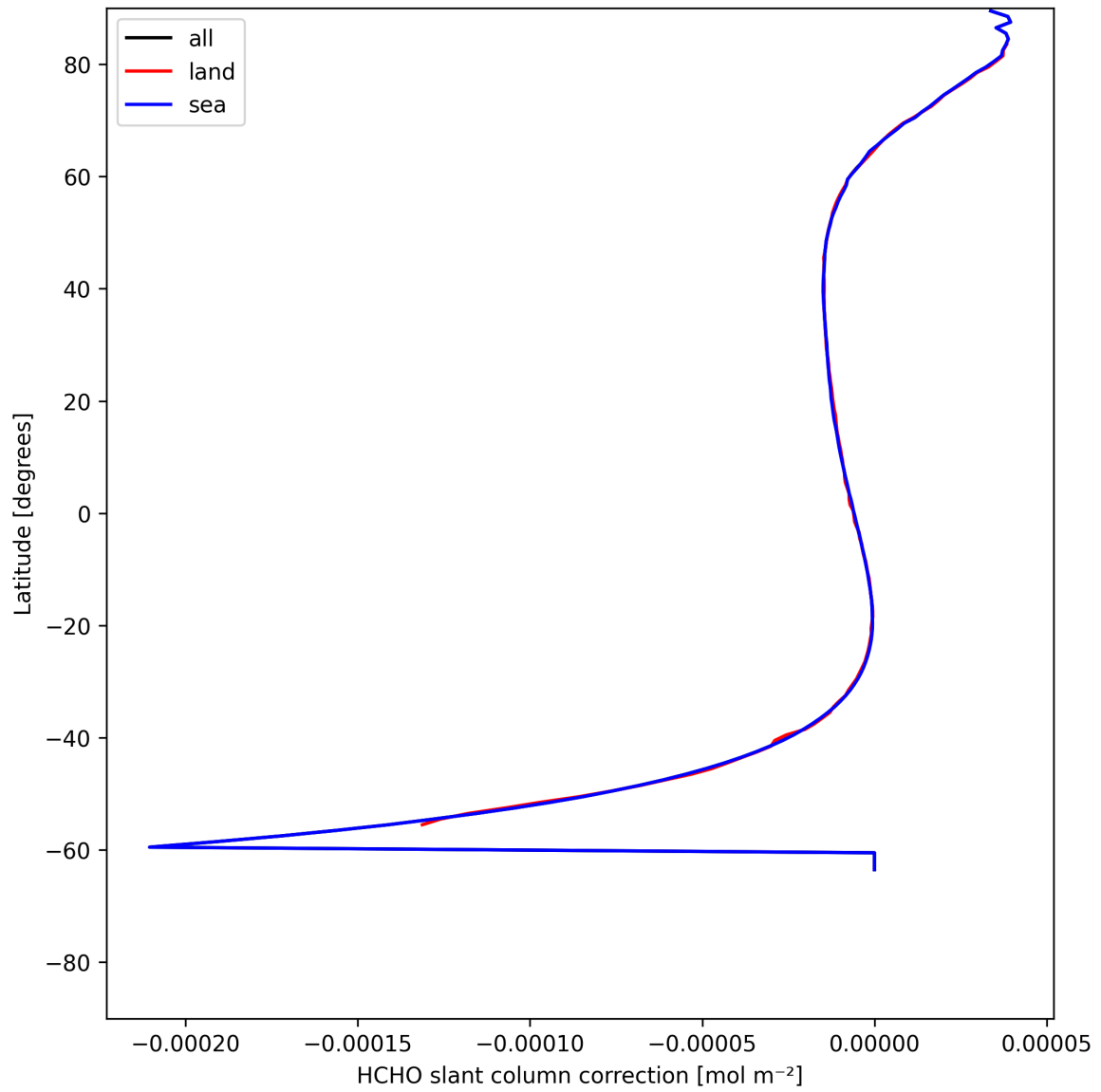
Figure 31: Zonal average of “HCHO slant column correction” for 2025-07-16 to 2025-07-16.
