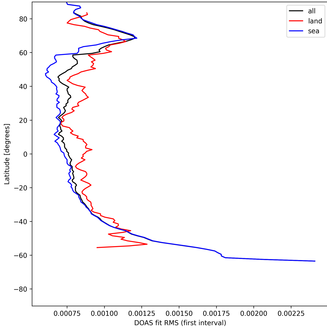
Figure 30: Zonal average of "DOAS fit RMS (first interval)" for 2025-07-16 to 2025-07-16.
