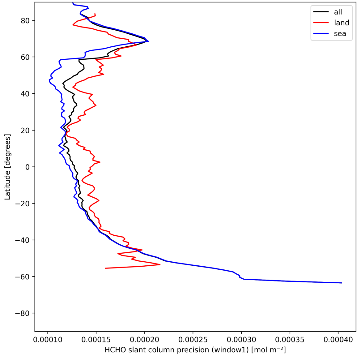
Figure 23: Zonal average of "HCHO slant column precision (window1)" for 2025-07-16 to 2025-07-16.
