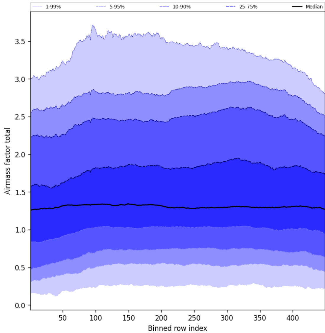
Figure 52: Along track statistics of “Airmass factor total” for 2025-07-16 to 2025-07-16
