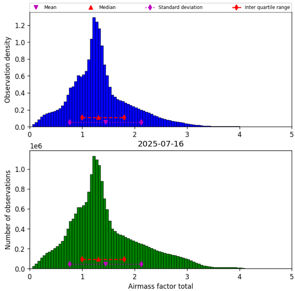
Figure 38: Histogram of “Airmass factor total” for 2025-07-16 to 2025-07-16
