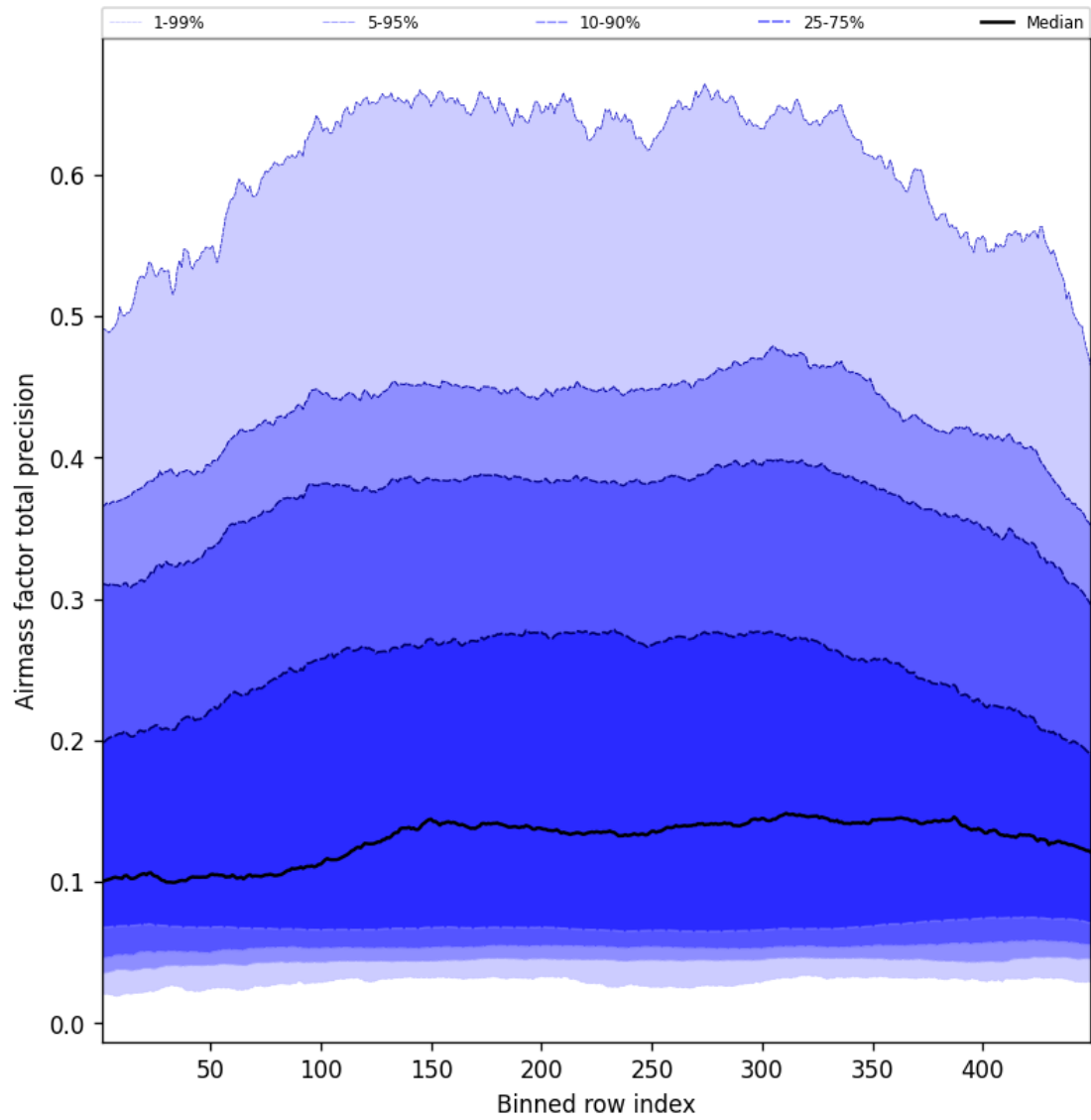
Figure 53: Along track statistics of “Airmass factor total precision” for 2025-07-16 to 2025-07-16
