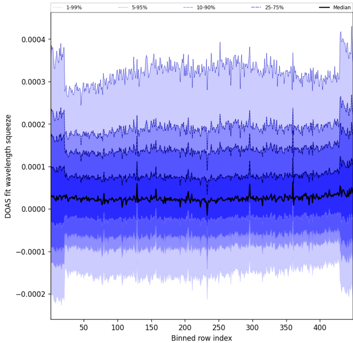
Figure 57: Along track statistics of “DOAS fit wavelength squeeze” for 2025-07-16 to 2025-07-16
