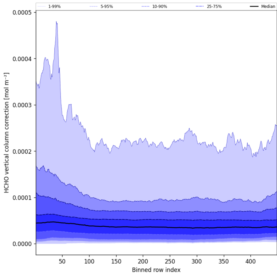
Figure 49: Along track statistics of “HCHO vertical column correction” for 2025-07-16 to 2025-07-16
