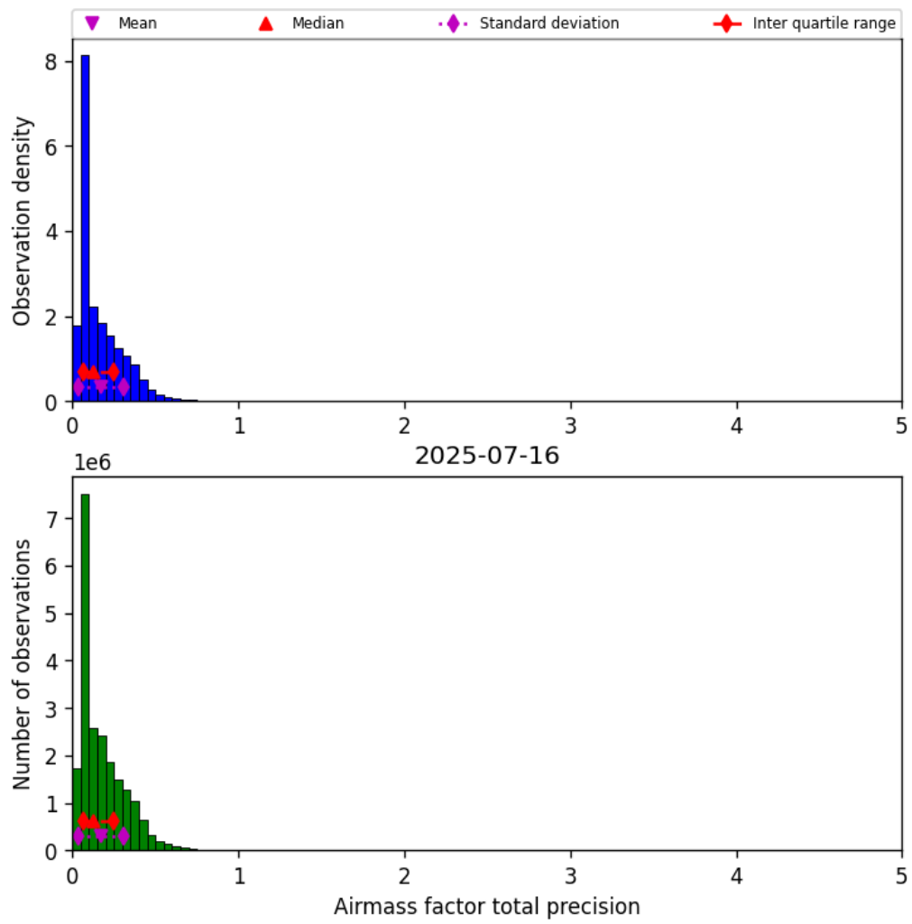
Figure 39: Histogram of “Airmass factor total precision” for 2025-07-16 to 2025-07-16
