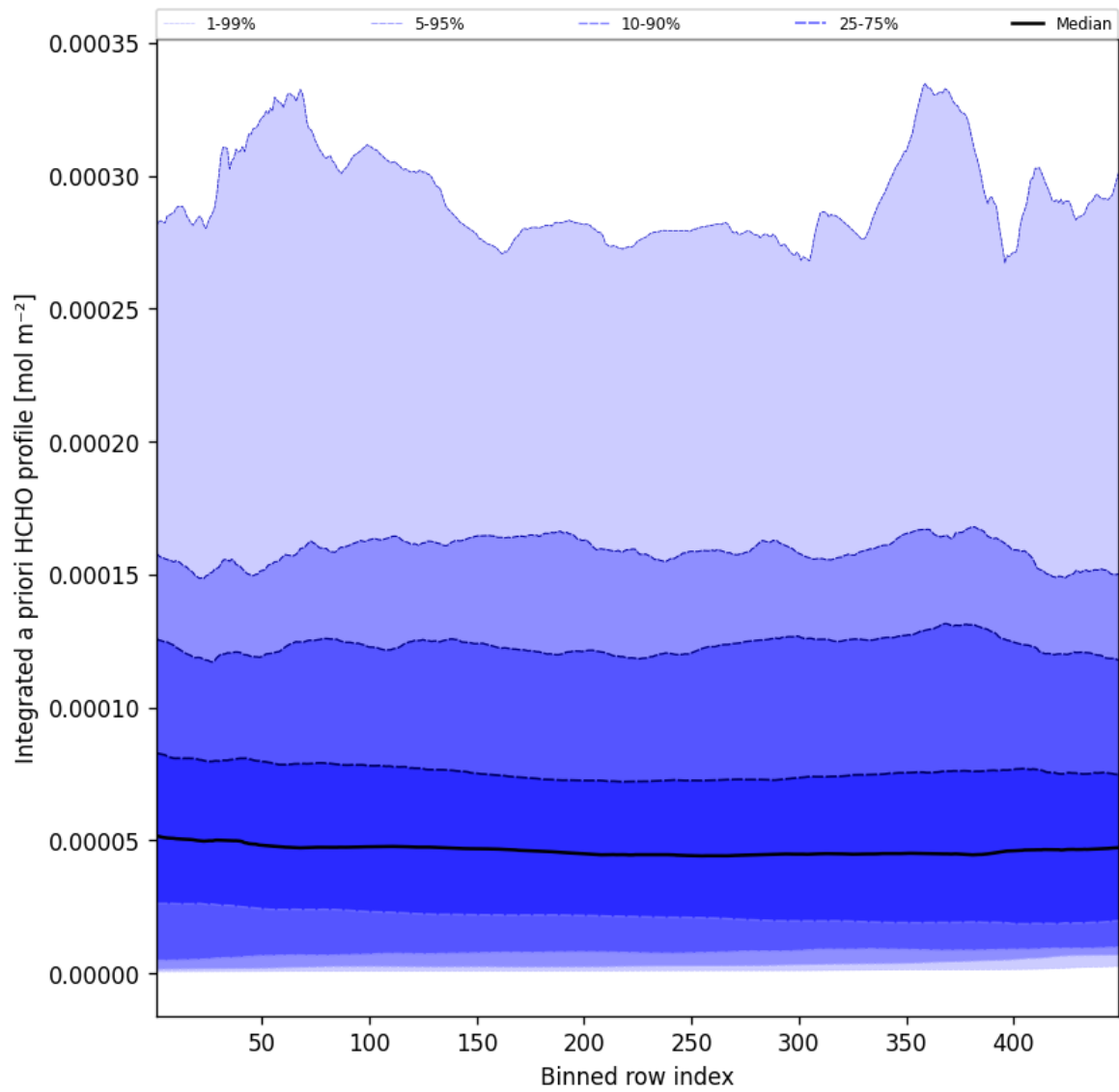
Figure 55: Along track statistics of “Integrated a priori HCHO profile” for 2025-07-16 to 2025-07-16
