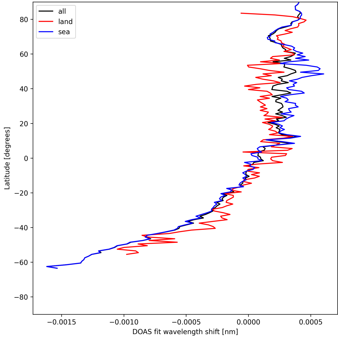
Figure 28: Zonal average of “DOAS fit wavelength shift” for 2025-07-16 to 2025-07-16.
