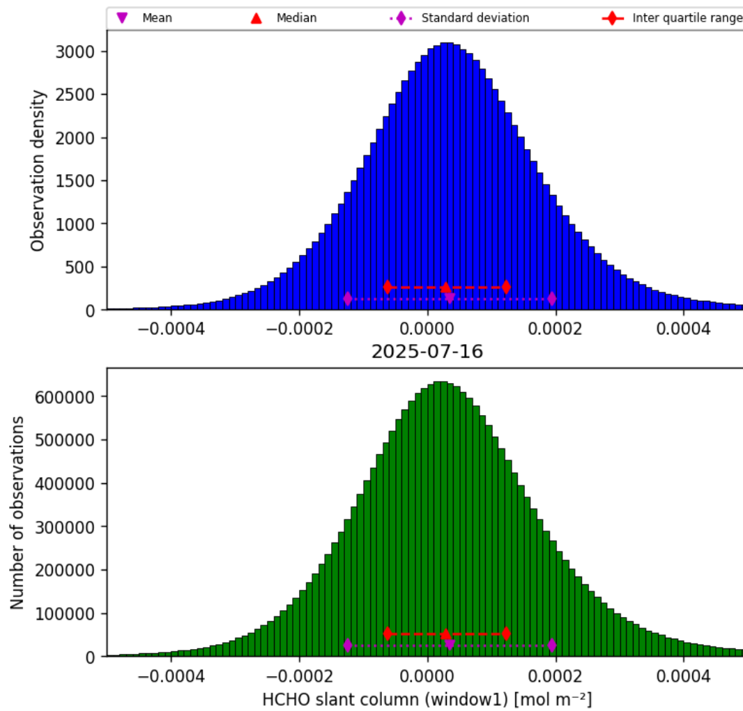
Figure 36: Histogram of “HCHO slant column (window1)” for 2025-07-16 to 2025-07-16
