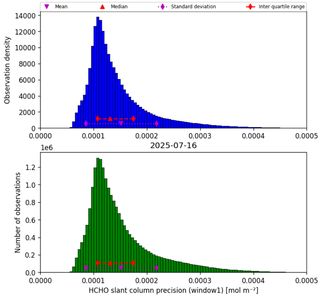
Figure 37: Histogram of “HCHO slant column precision (window1)” for 2025-07-16 to 2025-07-16
