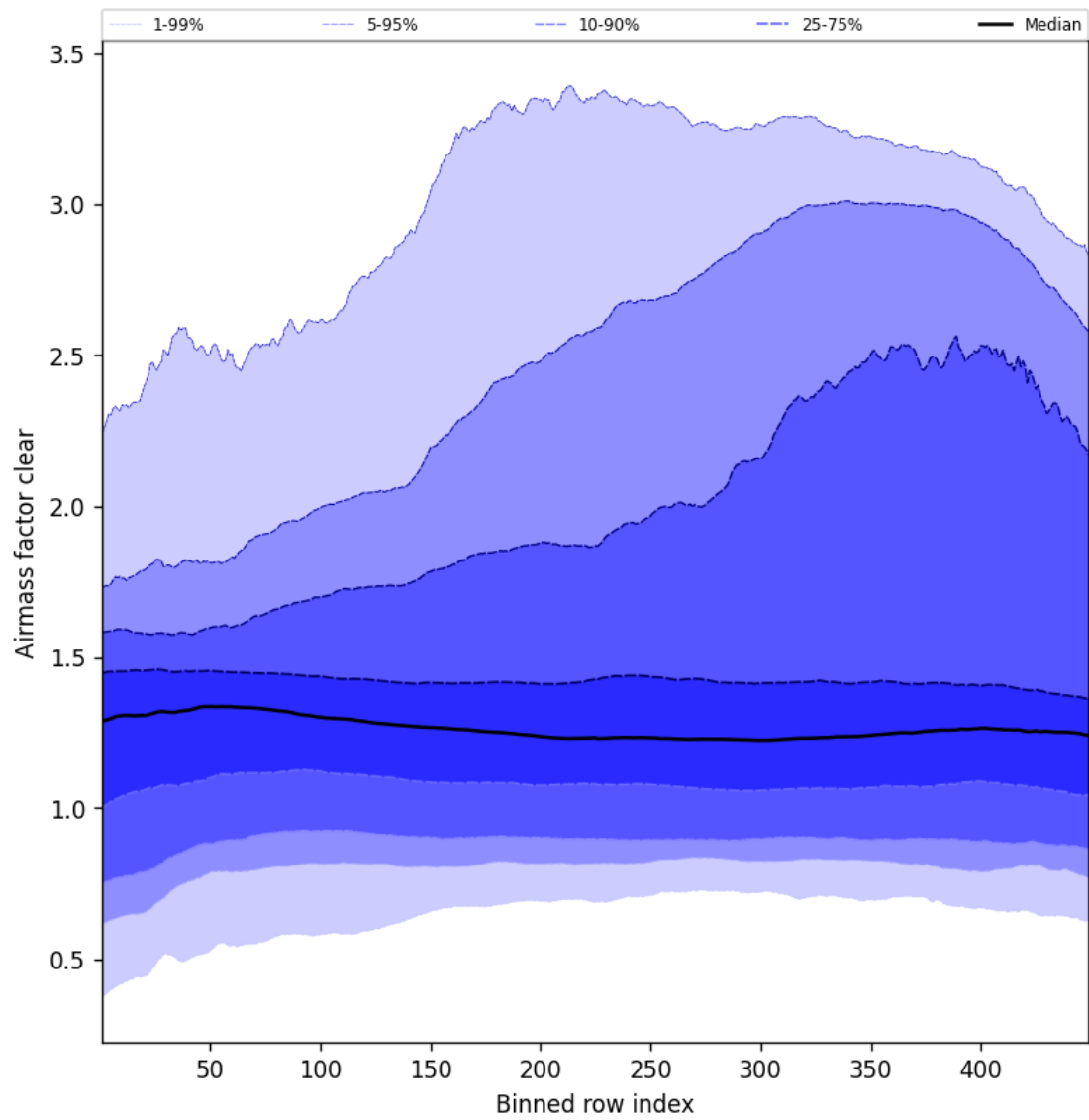
Figure 54: Along track statistics of “Airmass factor clear” for 2025-07-16 to 2025-07-16
