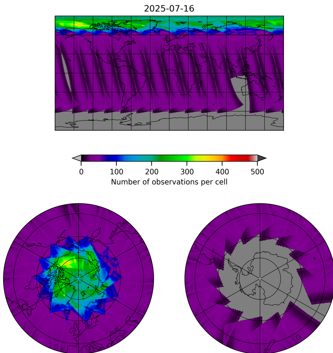
Figure 17: Map of the number of observations for 2025-07-16 to 2025-07-16
