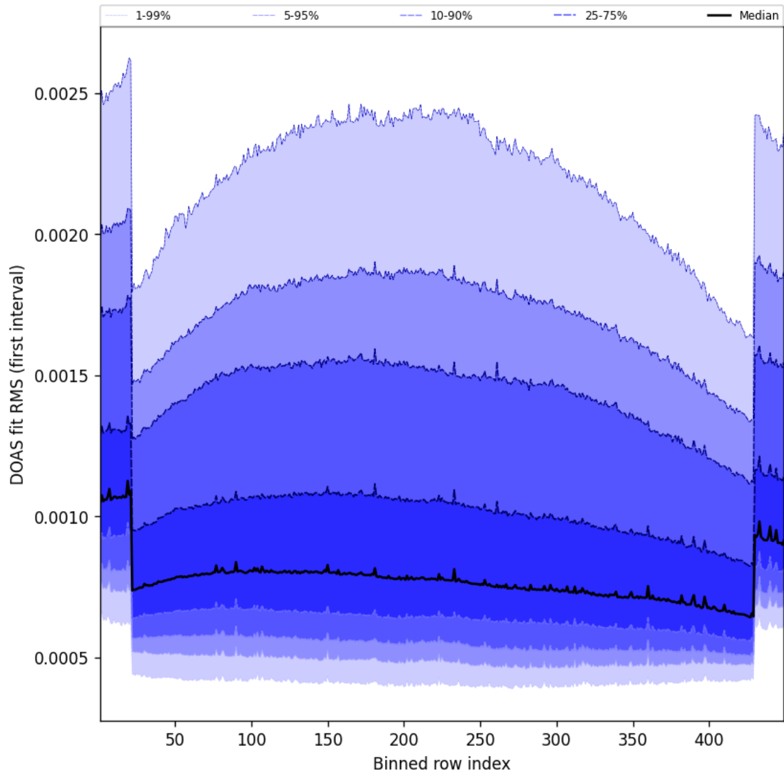
Figure 58: Along track statistics of “DOAS fit RMS (first interval)” for 2025-07-16 to 2025-07-16
