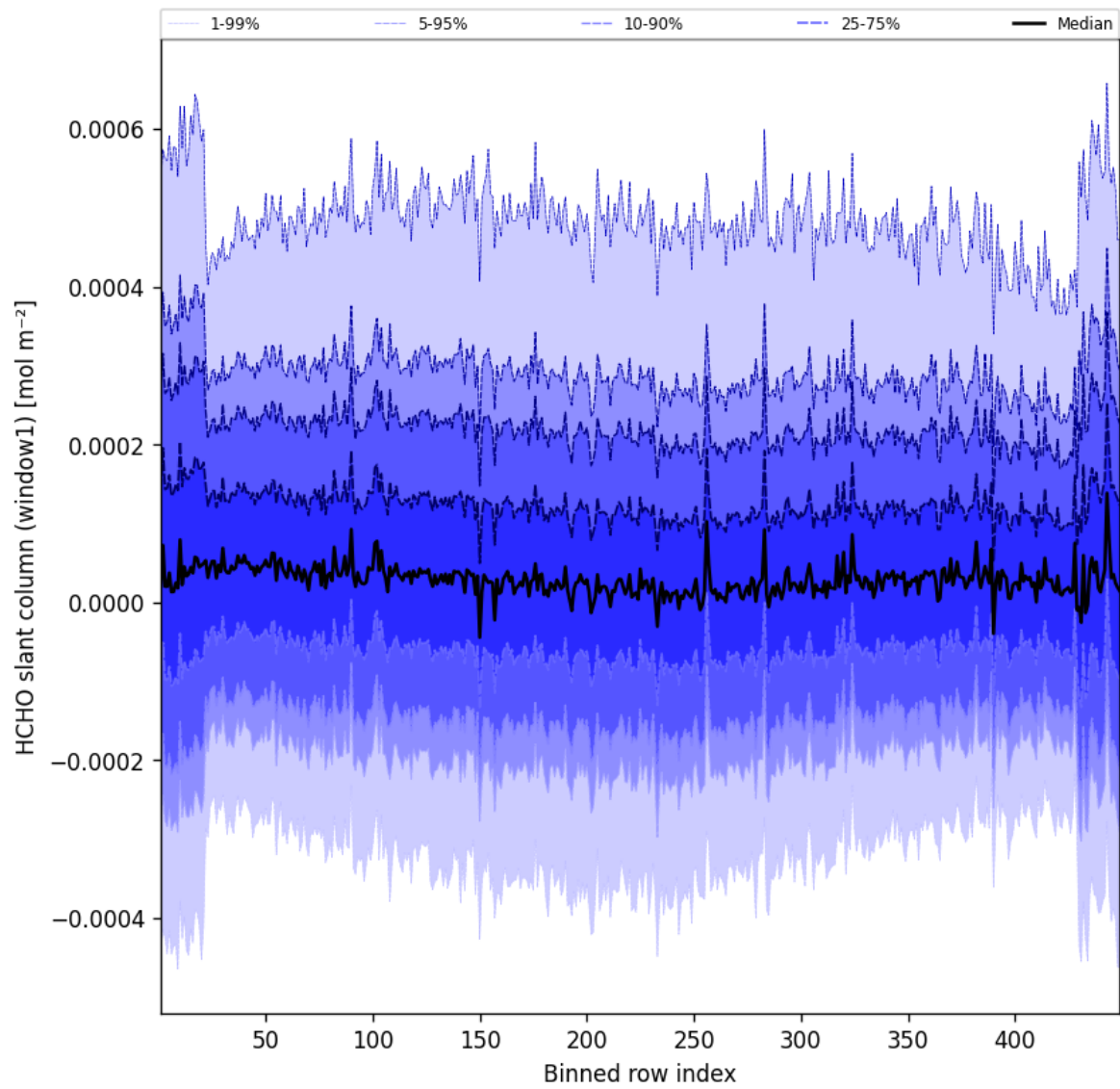
Figure 50: Along track statistics of “HCHO slant column (window1)” for 2025-07-16 to 2025-07-16
