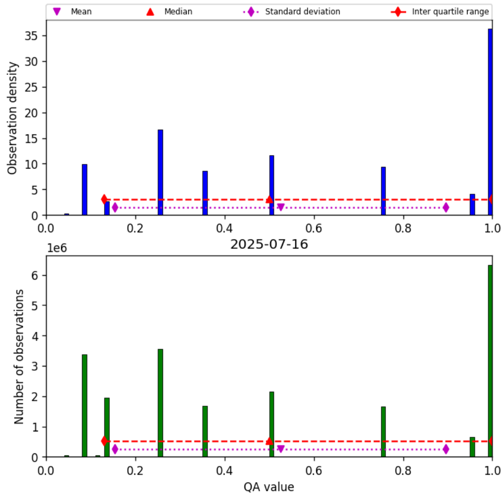
Figure 32: Histogram of “QA value” for 2025-07-16 to 2025-07-16
