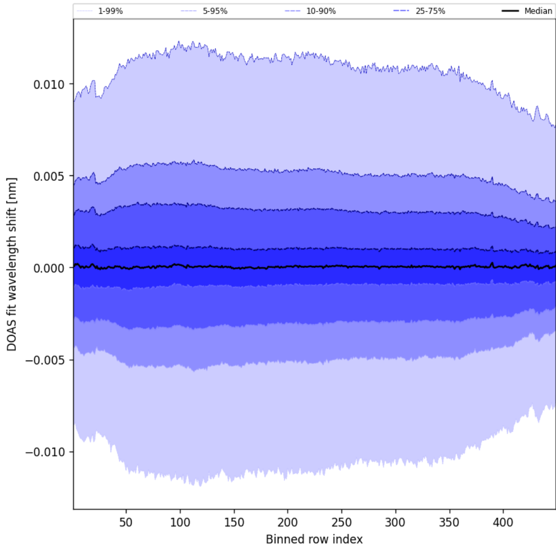
Figure 56: Along track statistics of “DOAS fit wavelength shift” for 2025-07-16 to 2025-07-16
