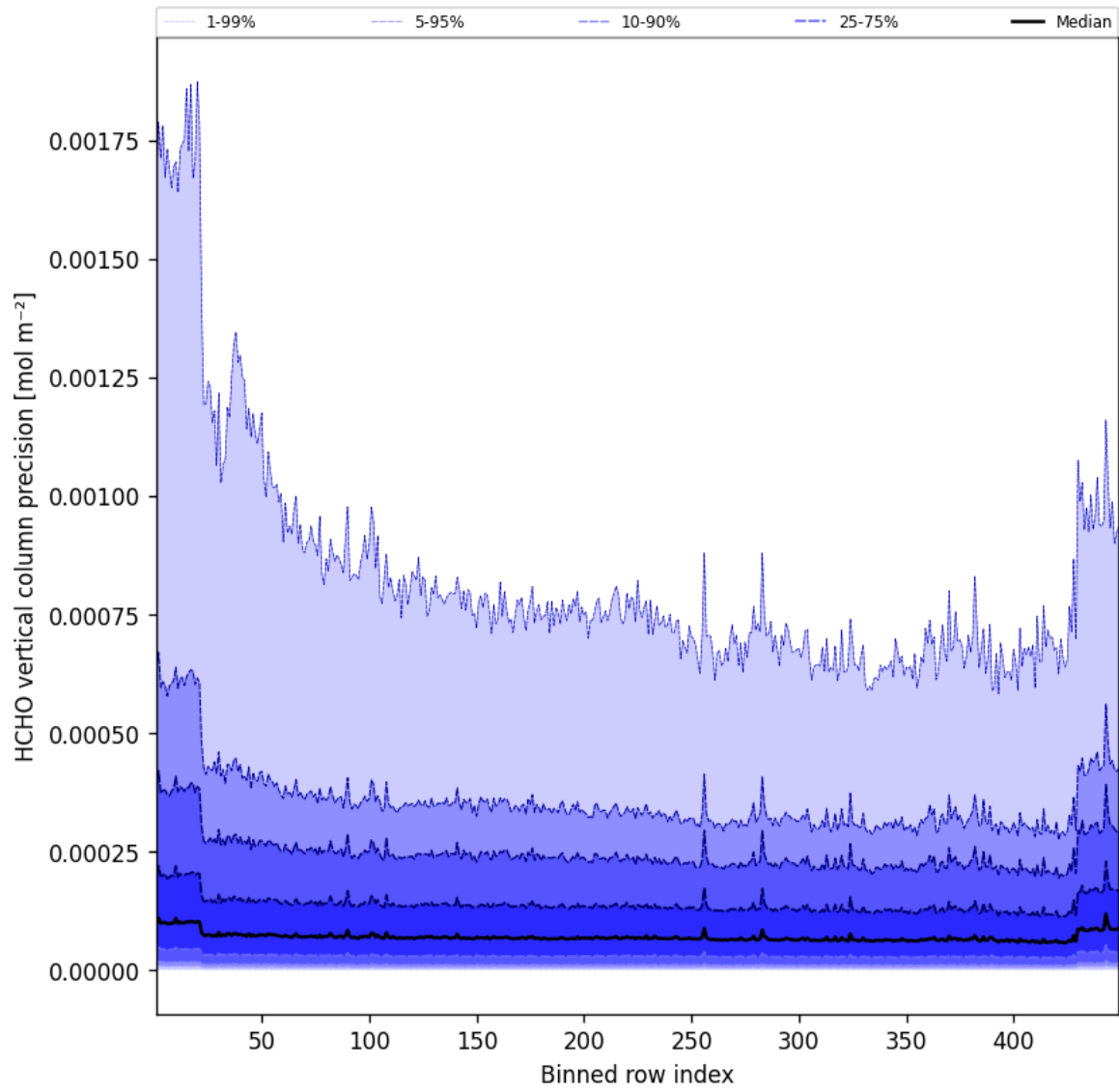
Figure 48: Along track statistics of “HCHO vertical column precision” for 2025-07-16 to 2025-07-16
