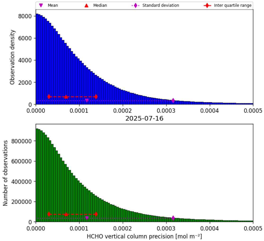
Figure 34: Histogram of “HCHO vertical column precision” for 2025-07-16 to 2025-07-16
