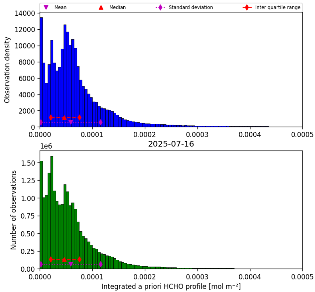
Figure 41: Histogram of “Integrated a priori HCHO profile” for 2025-07-16 to 2025-07-16
