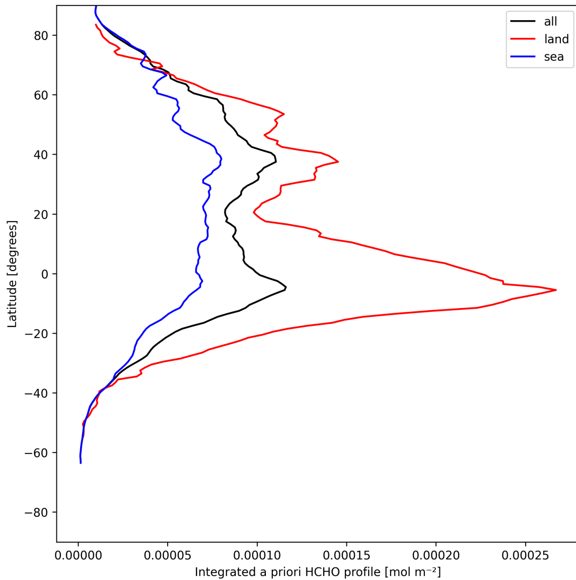
Figure 27: Zonal average of “Integrated a priori HCHO profile” for 2025-07-16 to 2025-07-16.
