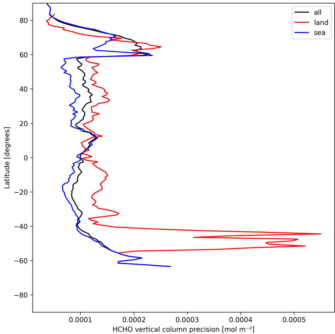
Figure 20: Zonal average of “HCHO vertical column precision” for 2025-07-16 to 2025-07-16.
