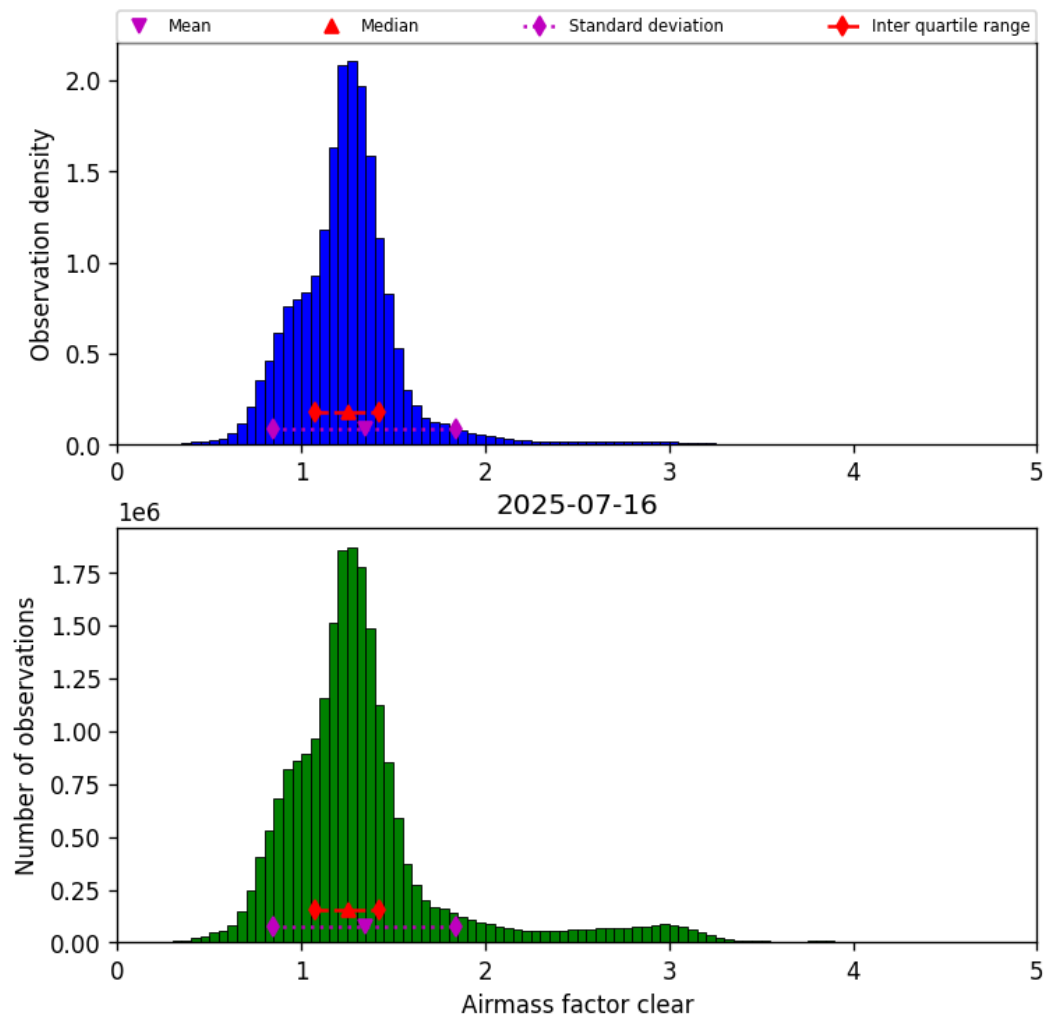
Figure 40: Histogram of “Airmass factor clear” for 2025-07-16 to 2025-07-16
