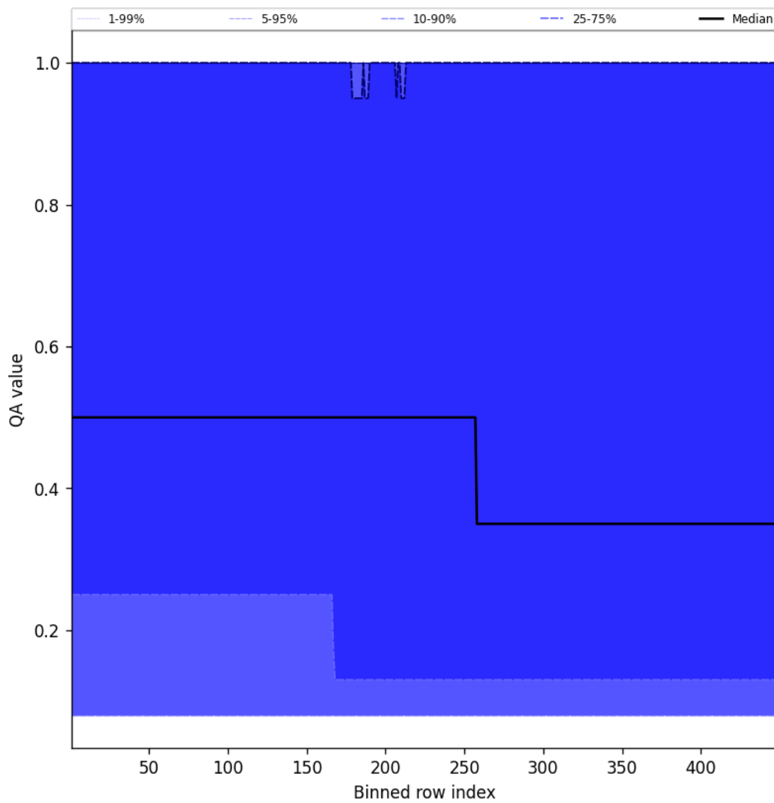
Figure 46: Along track statistics of “QA value” for 2025-07-16 to 2025-07-16
