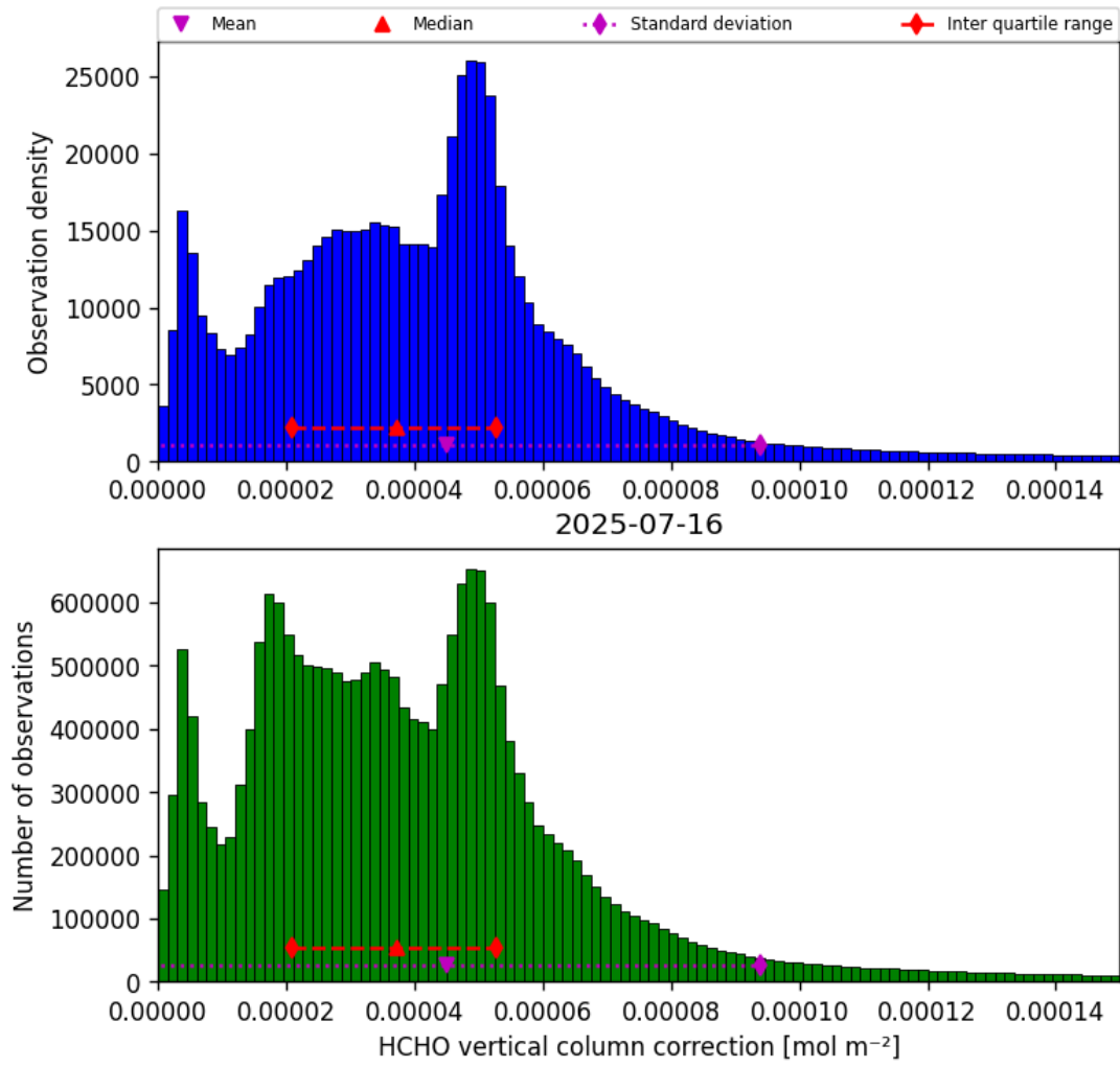
Figure 35: Histogram of “HCHO vertical column correction” for 2025-07-16 to 2025-07-16
