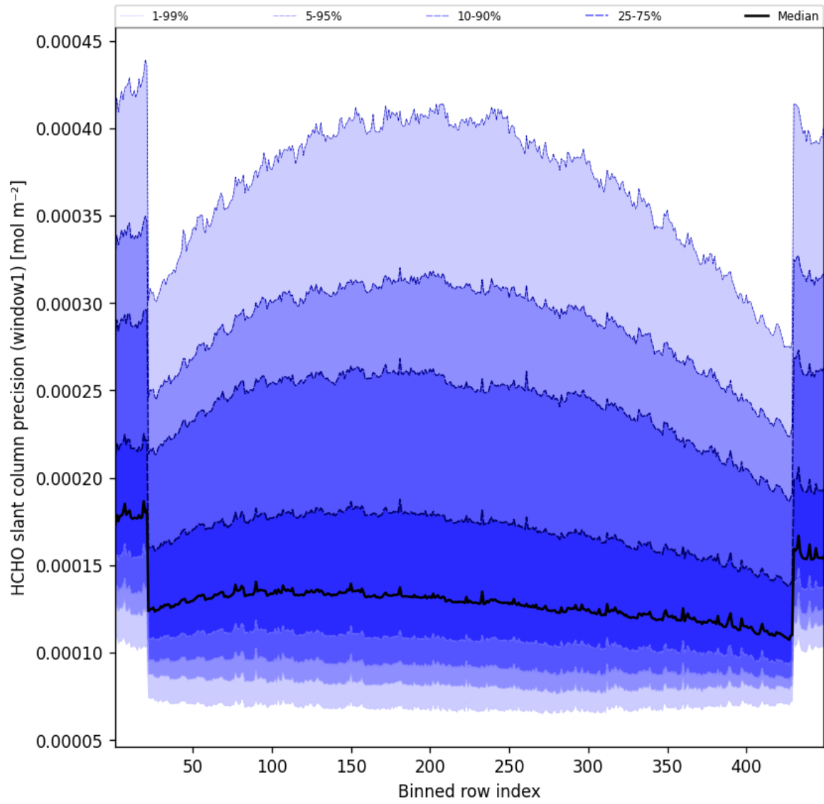
Figure 51: Along track statistics of “HCHO slant column precision (window1)” for 2025-07-16 to 2025-07-16
