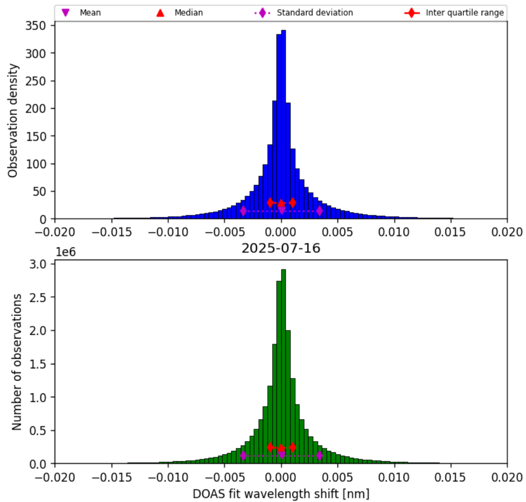
Figure 42: Histogram of “DOAS fit wavelength shift” for 2025-07-16 to 2025-07-16
