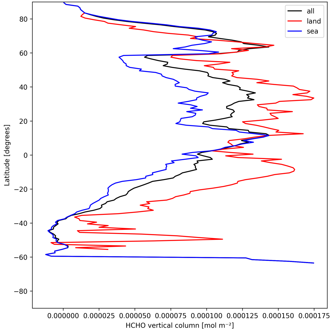
Figure 19: Zonal average of “HCHO vertical column” for 2025-07-16 to 2025-07-16.
