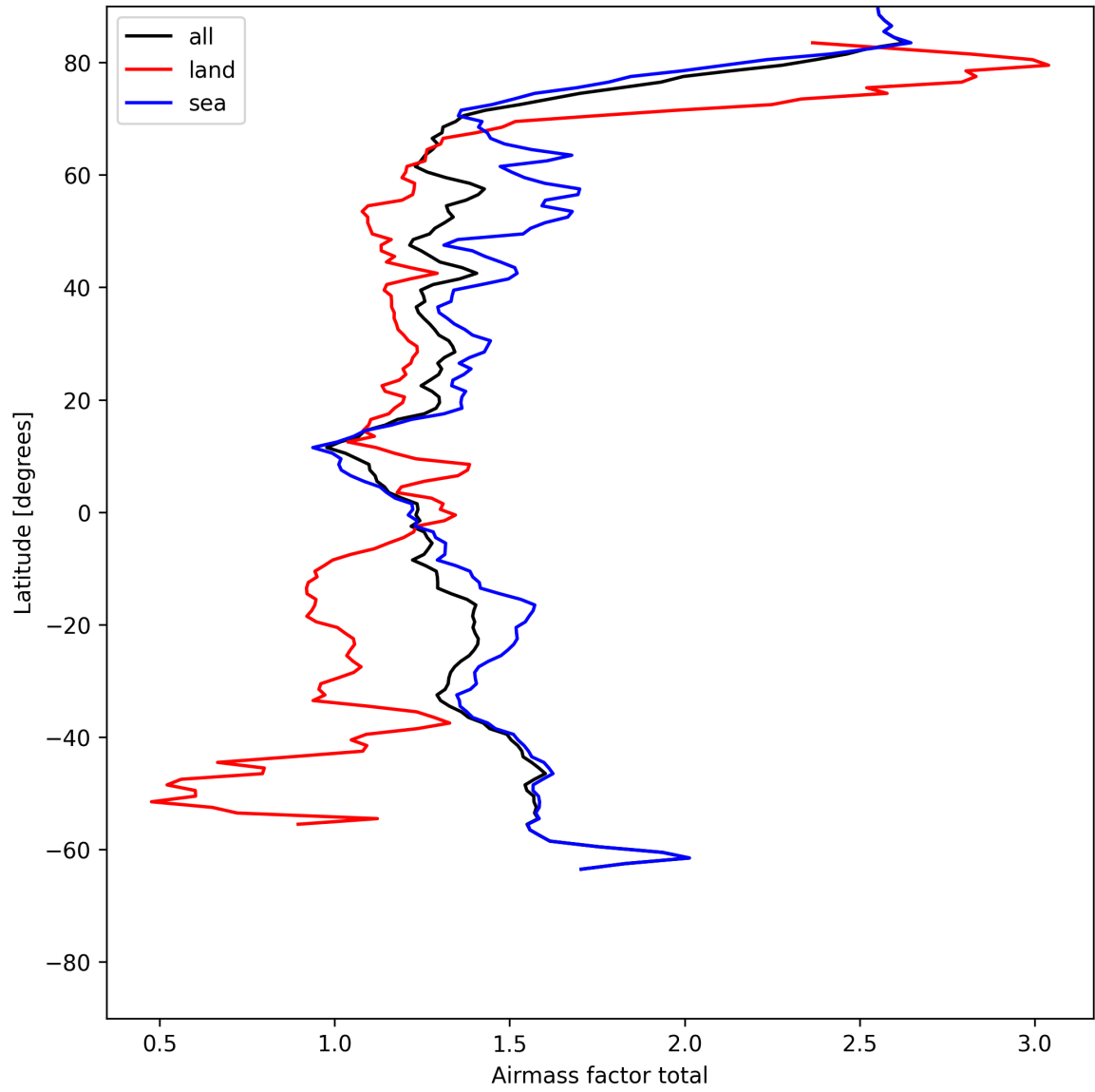
Figure 24: Zonal average of “Airmass factor total” for 2025-07-16 to 2025-07-16.
