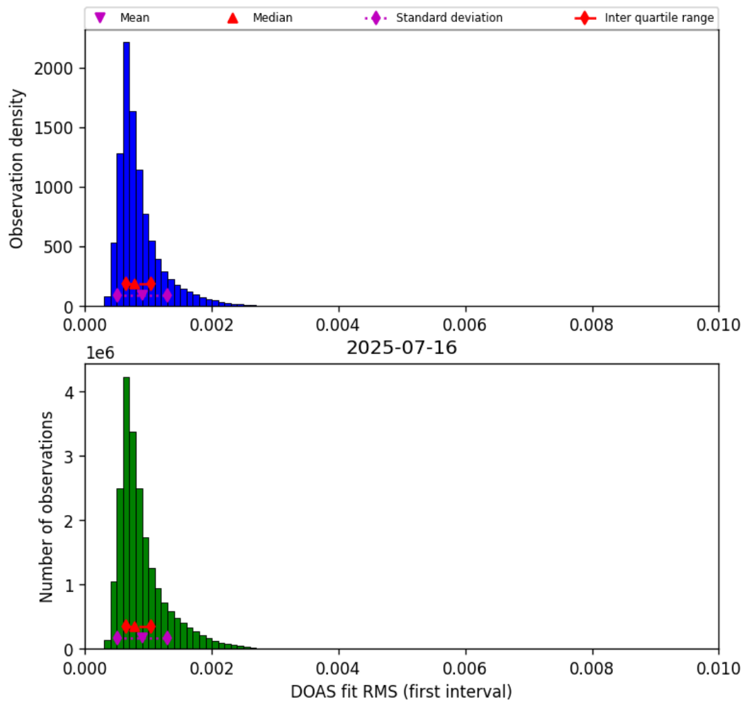
Figure 44: Histogram of “DOAS fit RMS (first interval)” for 2025-07-16 to 2025-07-16
