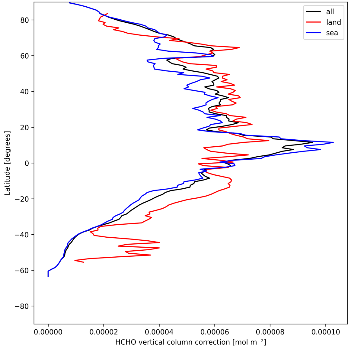
Figure 21: Zonal average of “HCHO vertical column correction” for 2025-07-16 to 2025-07-16.
