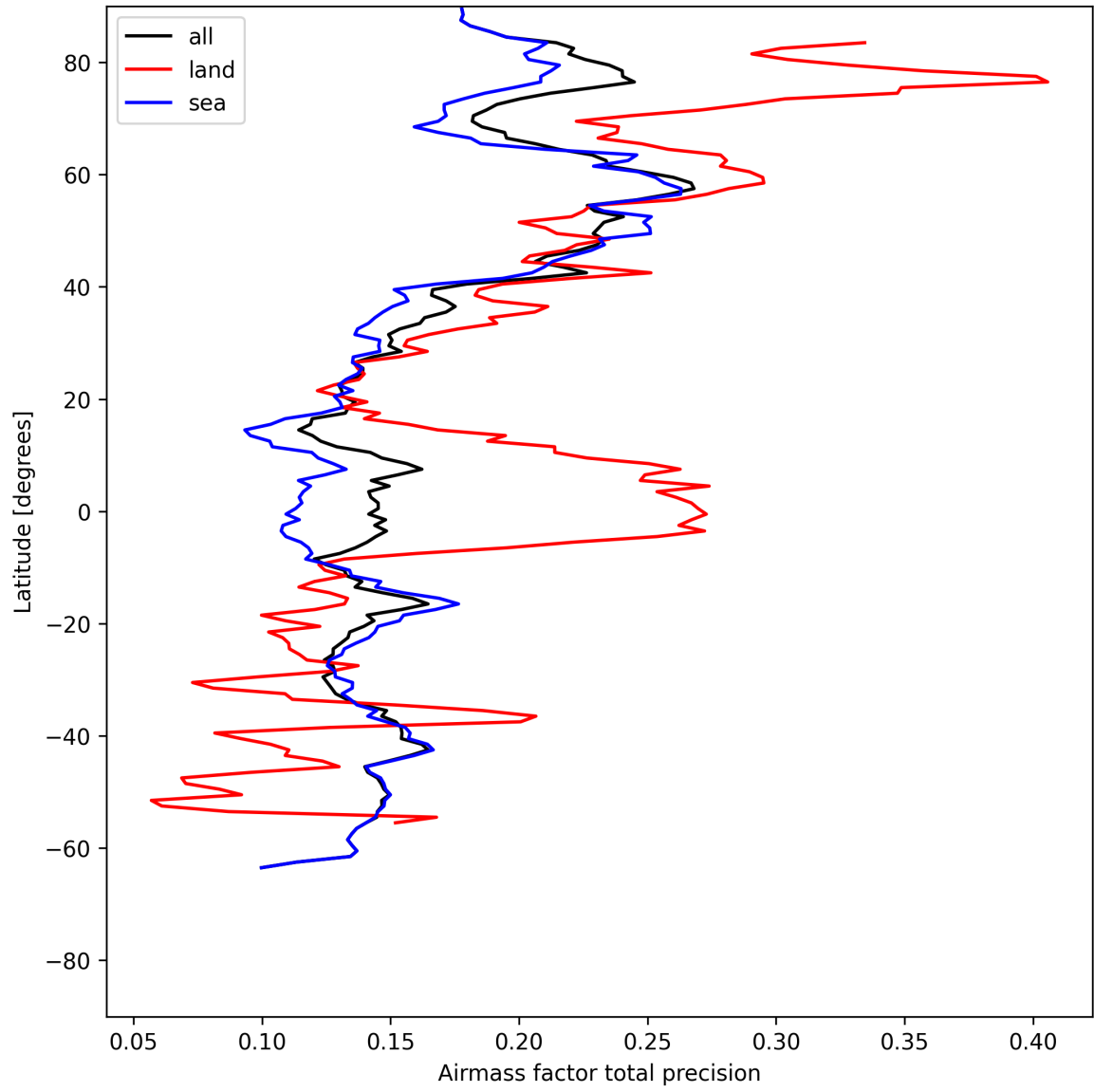
Figure 25: Zonal average of “Airmass factor total precision” for 2025-07-16 to 2025-07-16.
