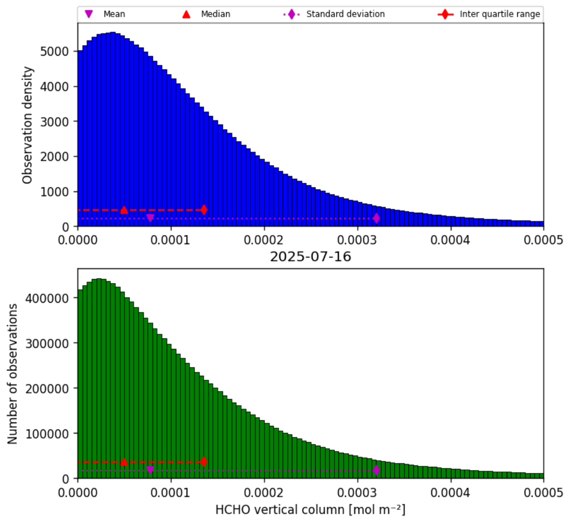
Figure 33: Histogram of “HCHO vertical column” for 2025-07-16 to 2025-07-16
