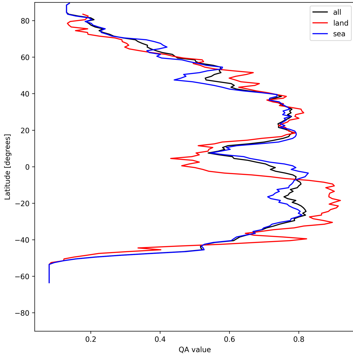
Figure 18: Zonal average of “QA value” for 2025-07-16 to 2025-07-16.
