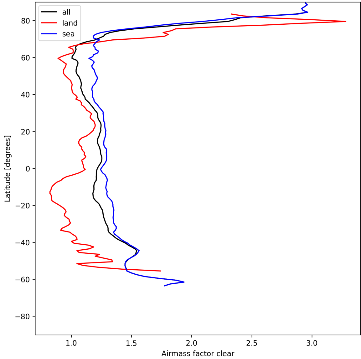
Figure 26: Zonal average of “Airmass factor clear” for 2025-07-16 to 2025-07-16.
