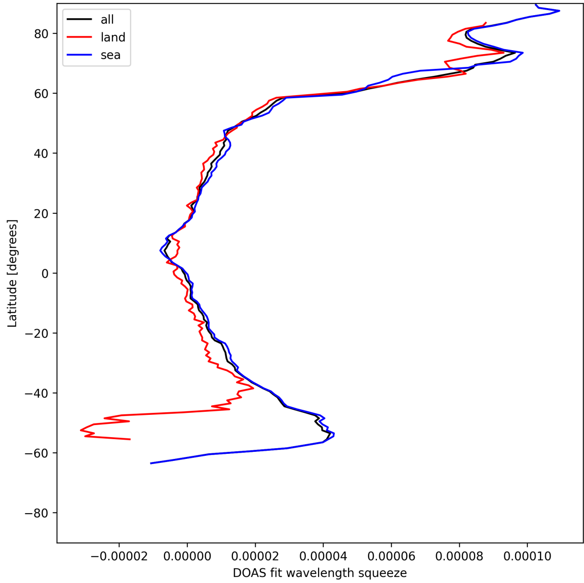
Figure 29: Zonal average of “DOAS fit wavelength squeeze” for 2025-07-16 to 2025-07-16.
