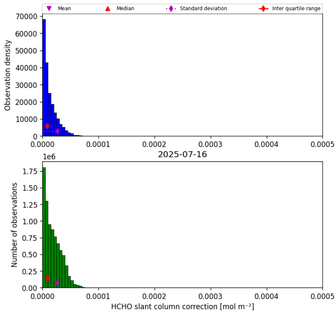
Figure 45: Histogram of “HCHO slant column correction” for 2025-07-16 to 2025-07-16
