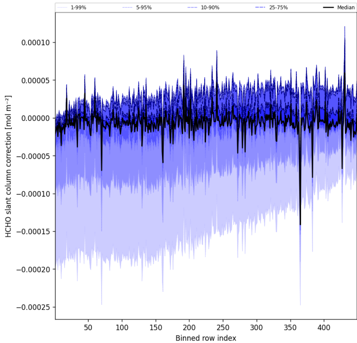
Figure 59: Along track statistics of “HCHO slant column correction” for 2025-07-16 to 2025-07-16
