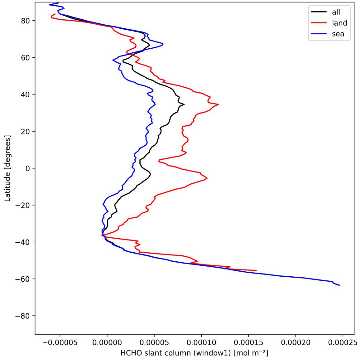
Figure 22: Zonal average of “HCHO slant column (window1)” for 2025-07-16 to 2025-07-16.
