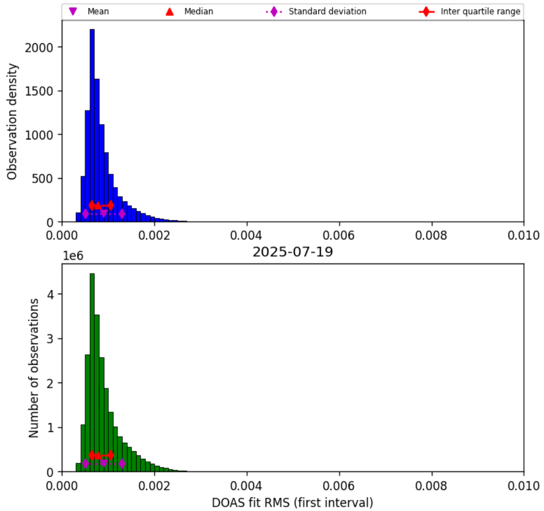
Figure 44: Histogram of “DOAS fit RMS (first interval)” for 2025-07-19 to 2025-07-20
