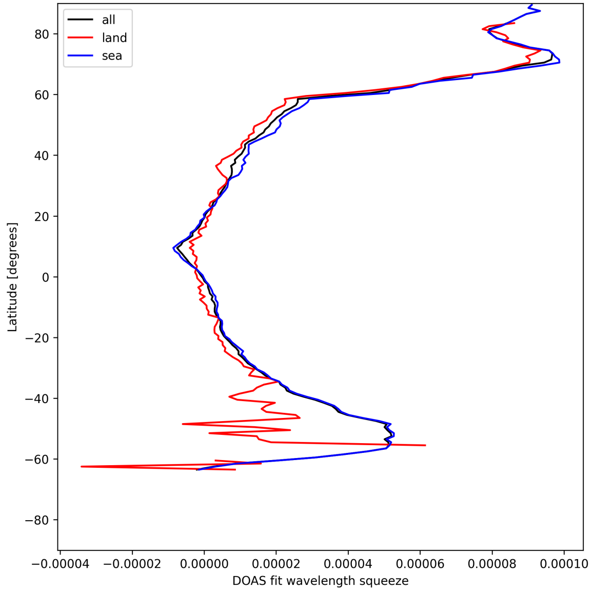
Figure 29: Zonal average of “DOAS fit wavelength squeeze” for 2025-07-19 to 2025-07-20.
