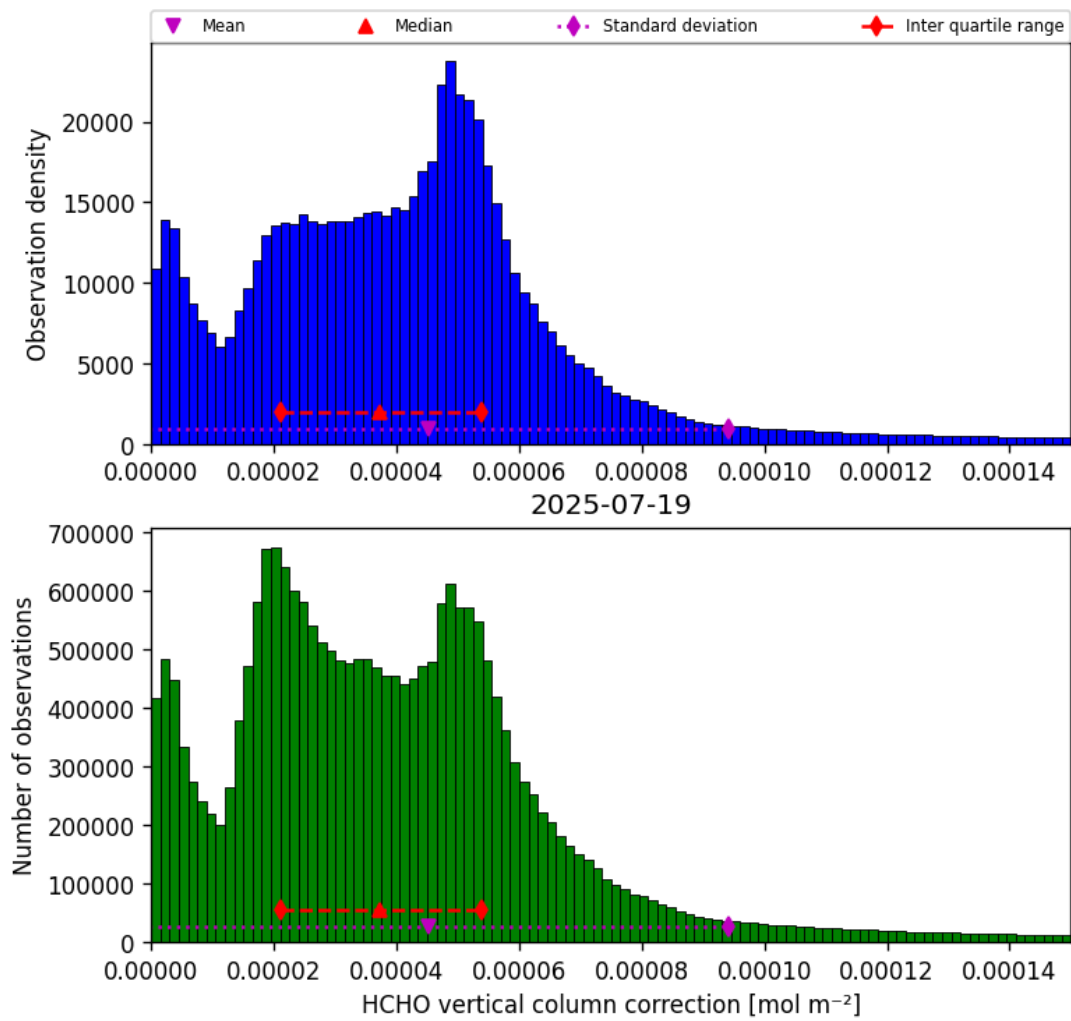
Figure 35: Histogram of “HCHO vertical column correction” for 2025-07-19 to 2025-07-20
