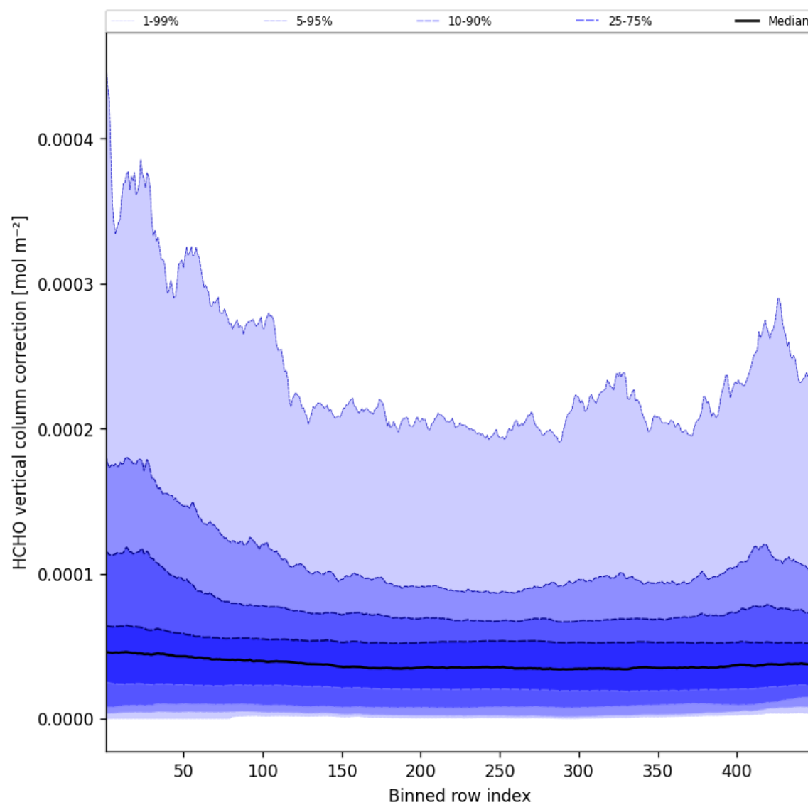
Figure 49: Along track statistics of “HCHO vertical column correction” for 2025-07-19 to 2025-07-20
