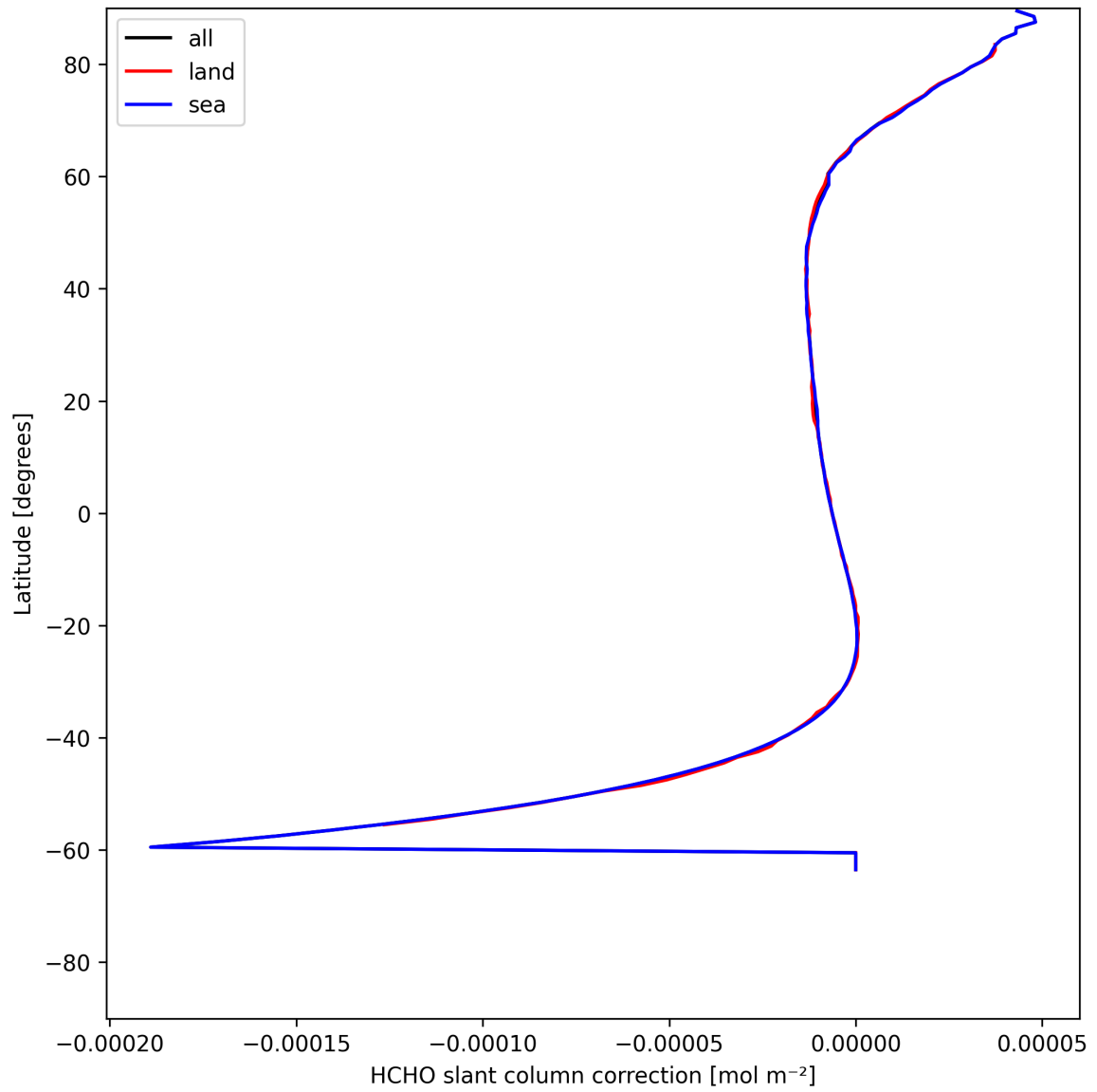
Figure 31: Zonal average of “HCHO slant column correction” for 2025-07-19 to 2025-07-20.
