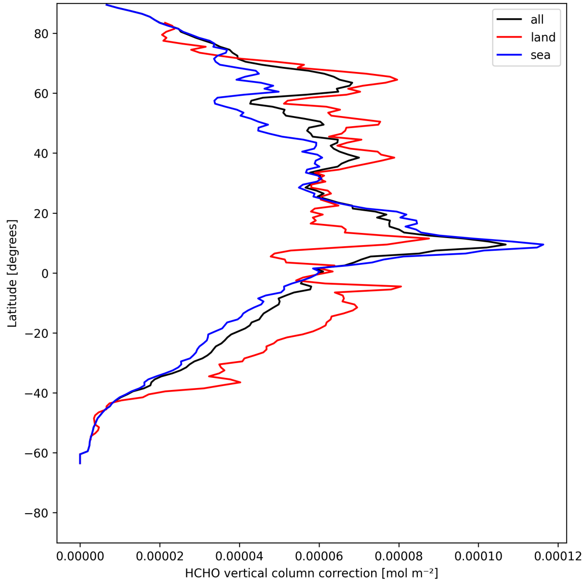
Figure 21: Zonal average of “HCHO vertical column correction” for 2025-07-19 to 2025-07-20.
