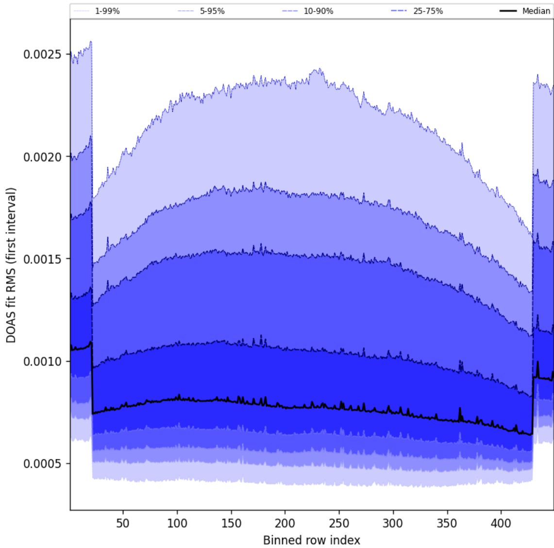
Figure 58: Along track statistics of “DOAS fit RMS (first interval)” for 2025-07-19 to 2025-07-20
