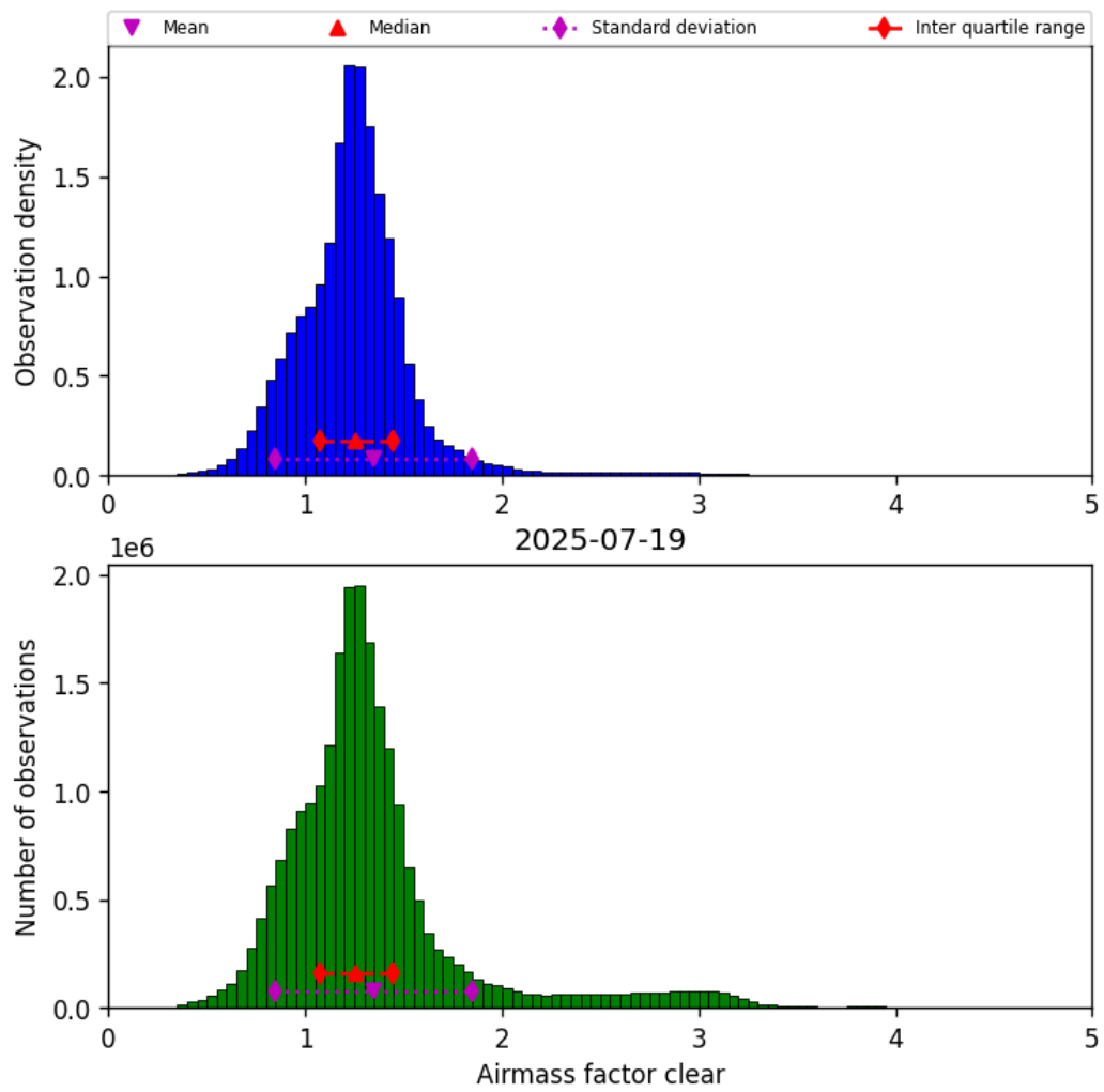
Figure 40: Histogram of “Airmass factor clear” for 2025-07-19 to 2025-07-20
