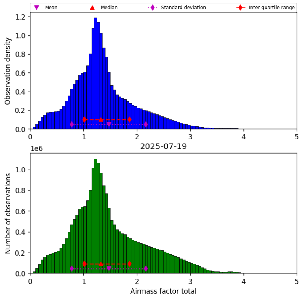
Figure 38: Histogram of “Airmass factor total” for 2025-07-19 to 2025-07-20
