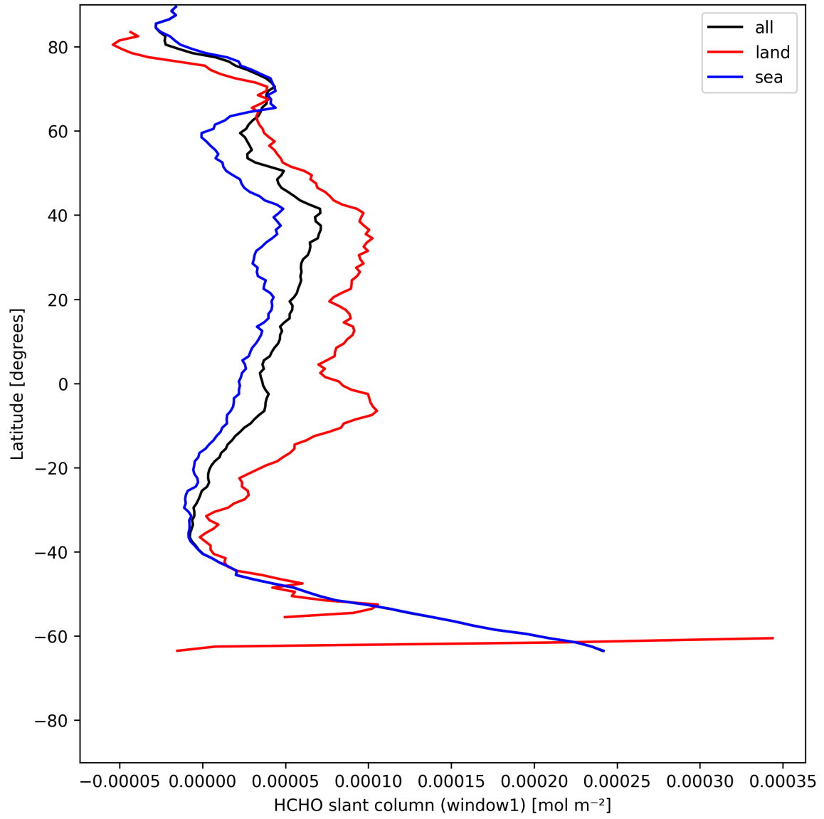
Figure 22: Zonal average of “HCHO slant column (window1)” for 2025-07-19 to 2025-07-20.
