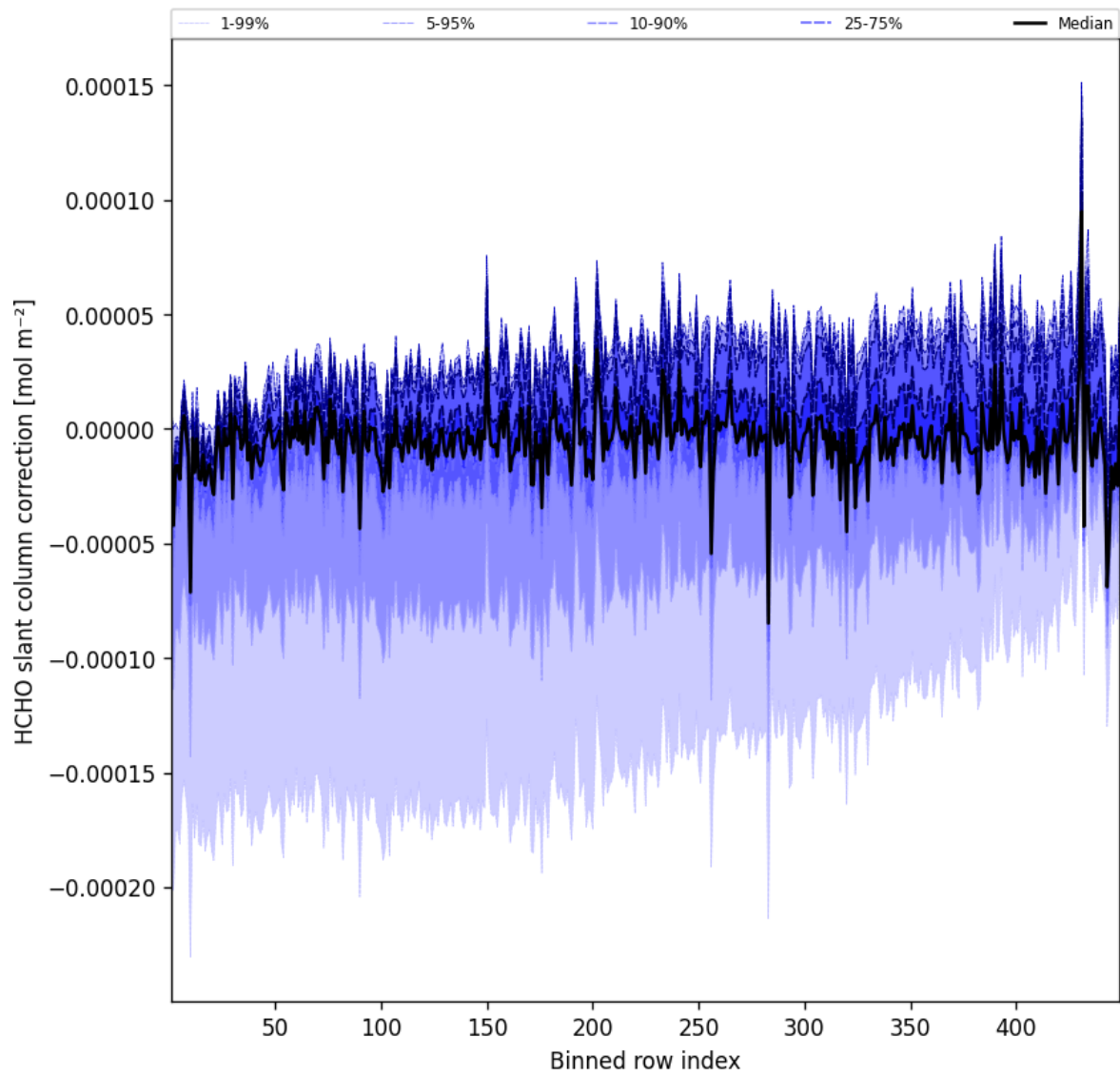
Figure 59: Along track statistics of “HCHO slant column correction” for 2025-07-19 to 2025-07-20
