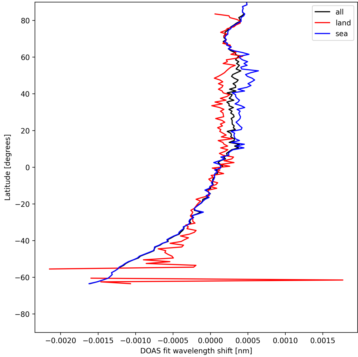
Figure 28: Zonal average of “DOAS fit wavelength shift” for 2025-07-19 to 2025-07-20.
