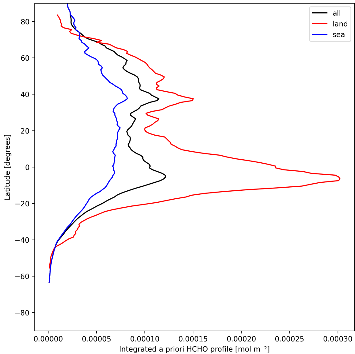
Figure 27: Zonal average of “Integrated a priori HCHO profile” for 2025-07-19 to 2025-07-20.
