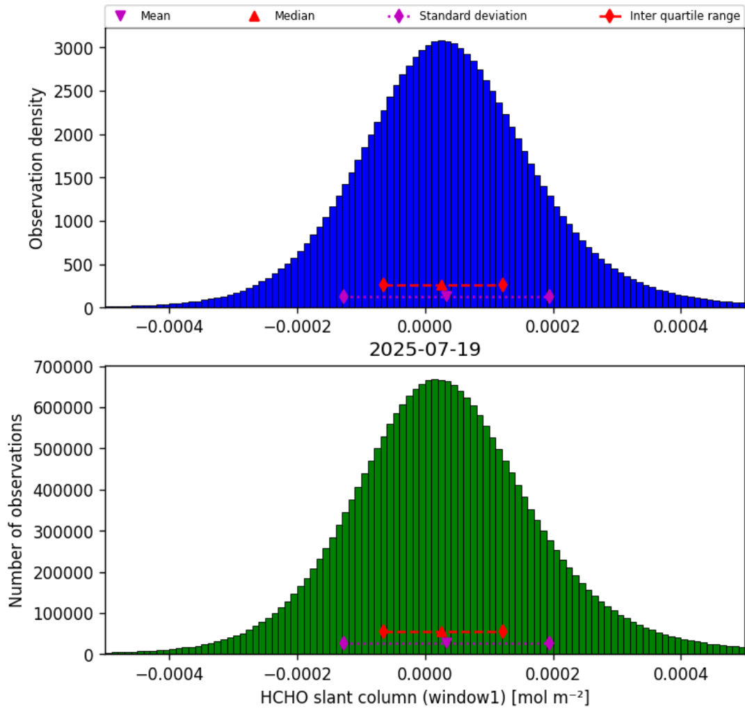
Figure 36: Histogram of “HCHO slant column (window1)” for 2025-07-19 to 2025-07-20
