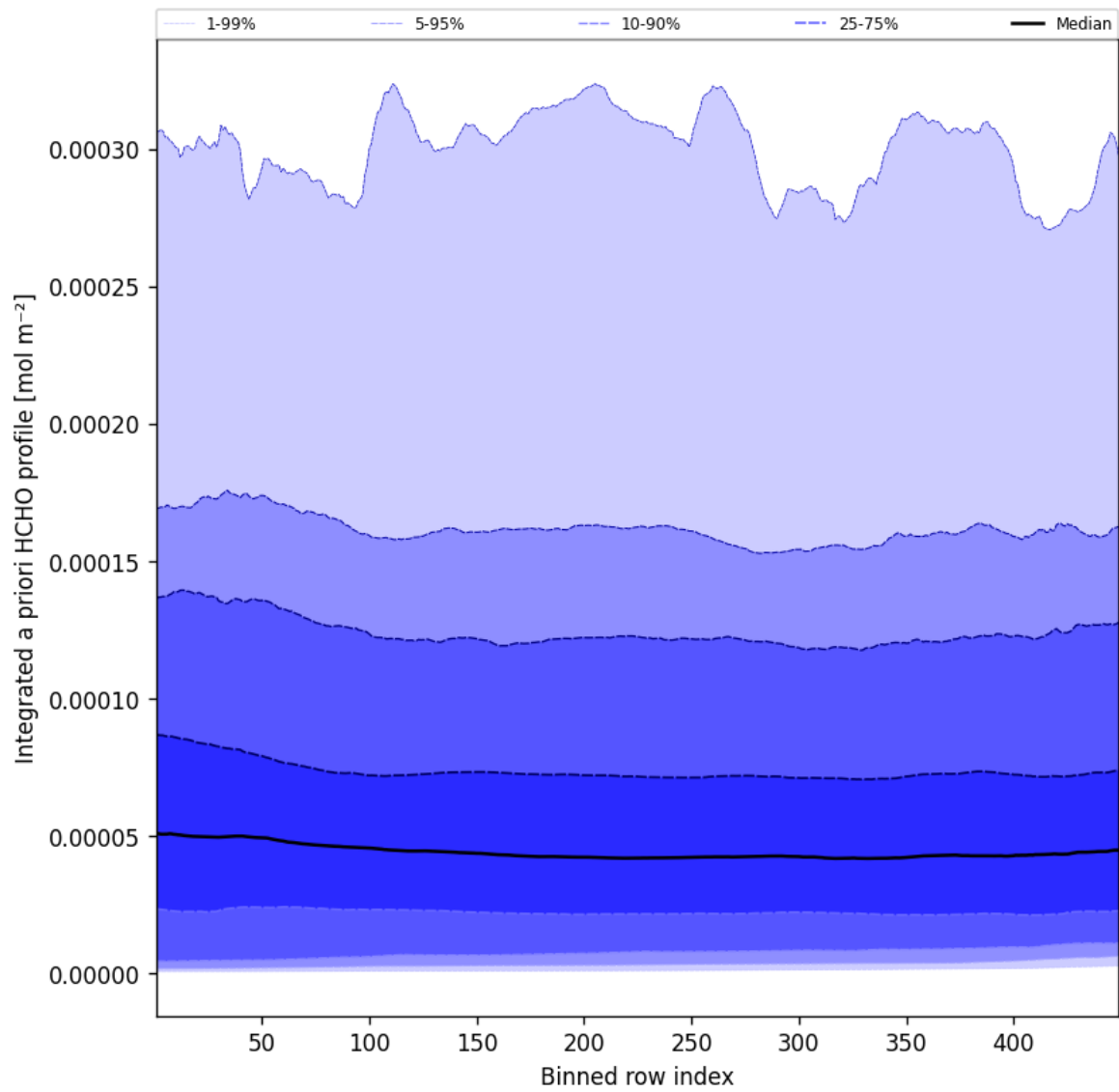
Figure 55: Along track statistics of “Integrated a priori HCHO profile” for 2025-07-19 to 2025-07-20
