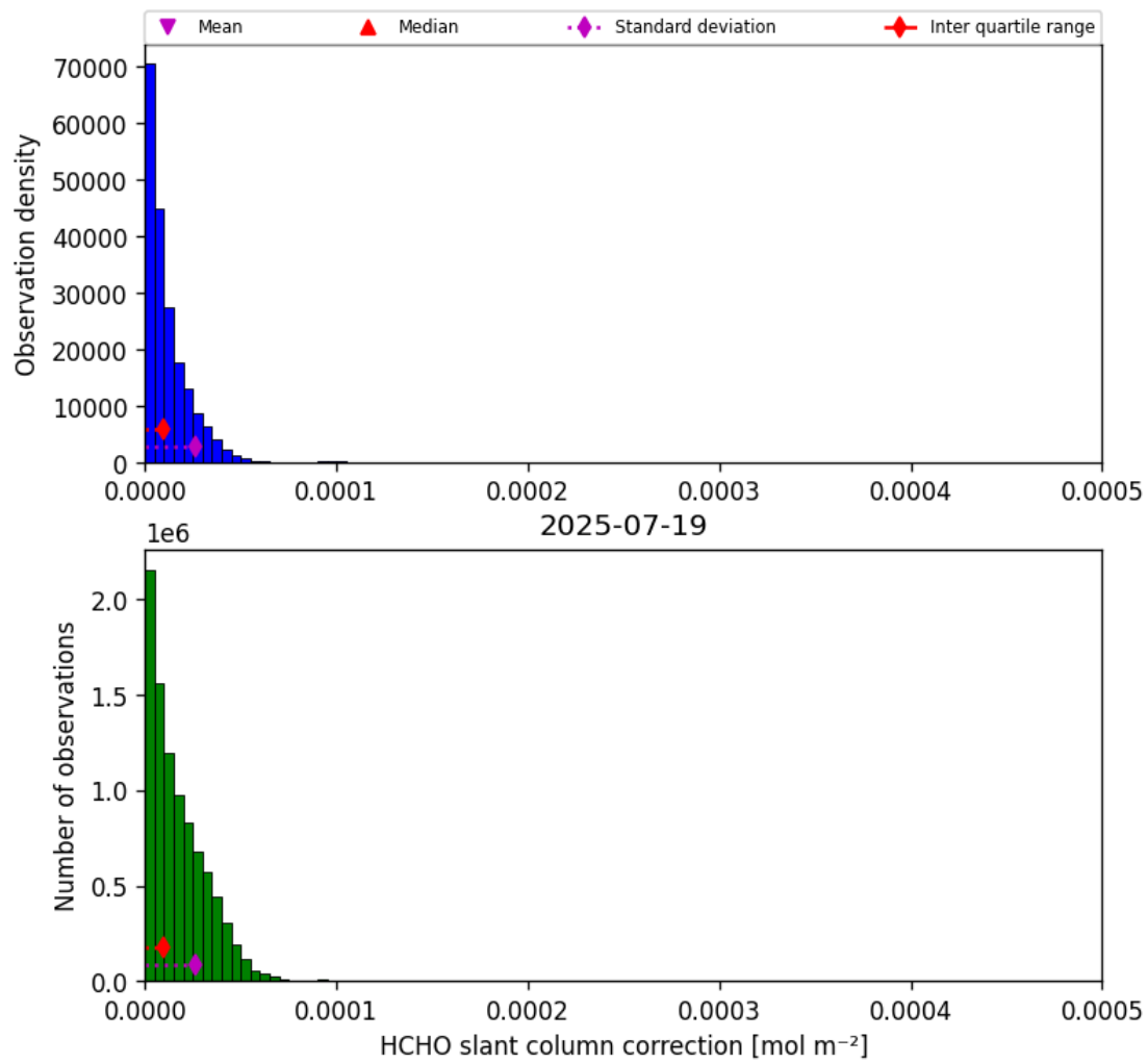
Figure 45: Histogram of “HCHO slant column correction” for 2025-07-19 to 2025-07-20
