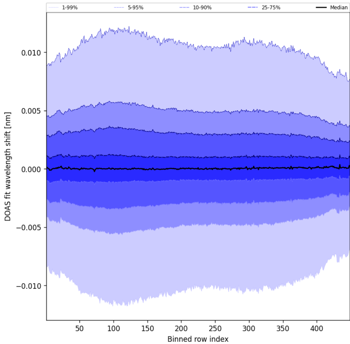
Figure 56: Along track statistics of “DOAS fit wavelength shift” for 2025-07-19 to 2025-07-20
