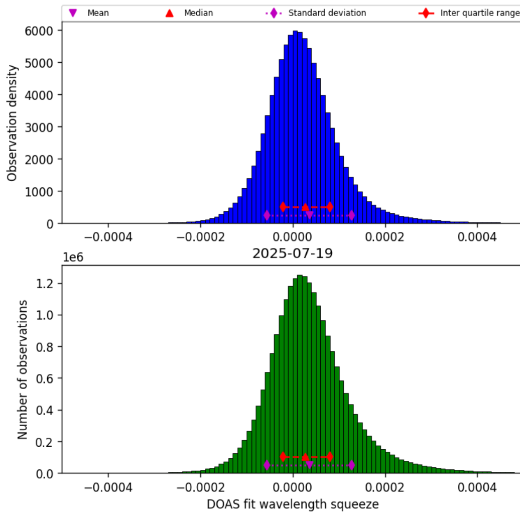
Figure 43: Histogram of “DOAS fit wavelength squeeze” for 2025-07-19 to 2025-07-20
