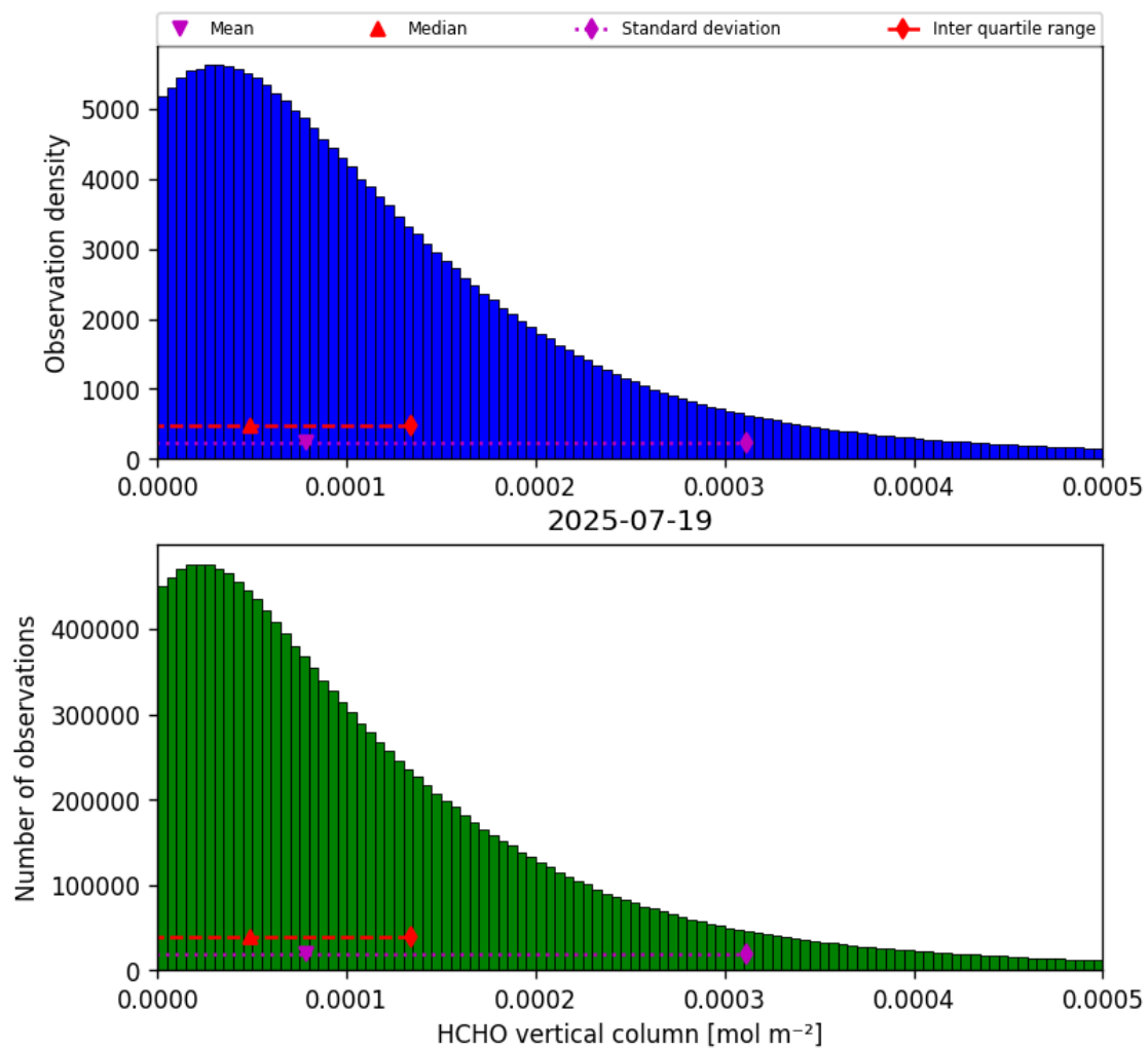
Figure 33: Histogram of “HCHO vertical column” for 2025-07-19 to 2025-07-20
