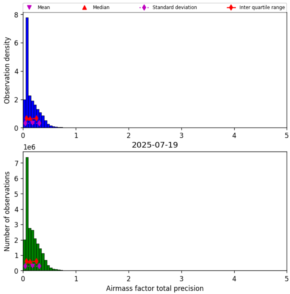
Figure 39: Histogram of “Airmass factor total precision” for 2025-07-19 to 2025-07-20
