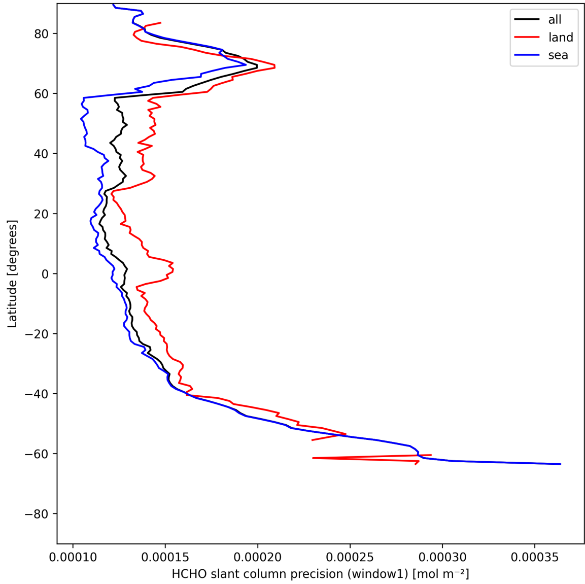
Figure 23: Zonal average of “HCHO slant column precision (window1)” for 2025-07-19 to 2025-07-20.
