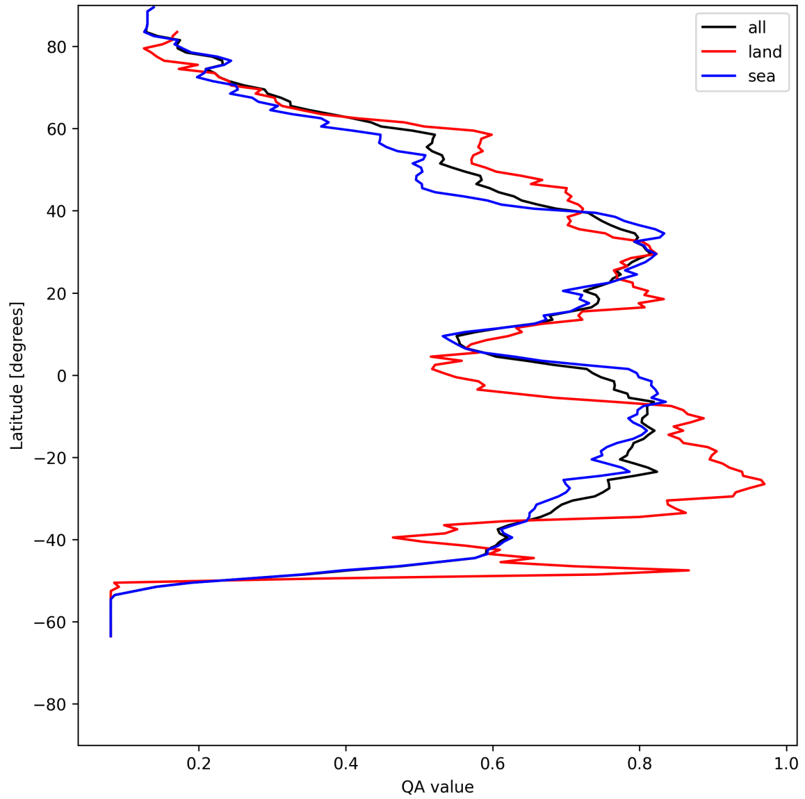
Figure 18: Zonal average of “QA value” for 2025-07-19 to 2025-07-20.
