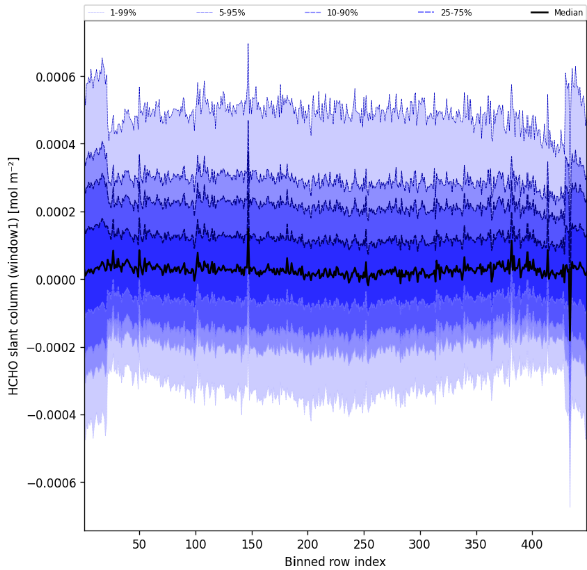
Figure 50: Along track statistics of “HCHO slant column (window1)” for 2025-07-19 to 2025-07-20
