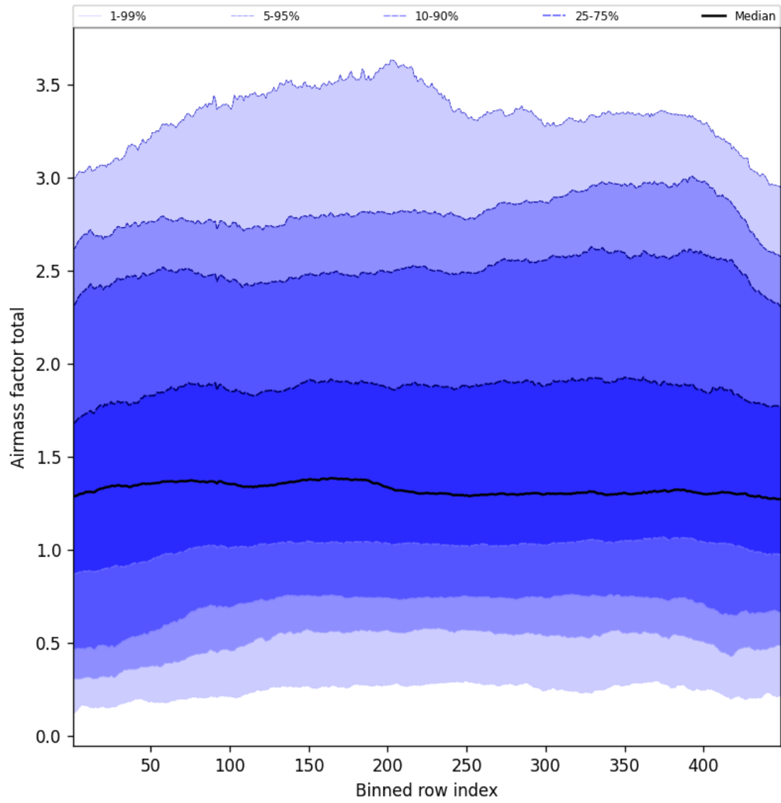
Figure 52: Along track statistics of “Airmass factor total” for 2025-07-19 to 2025-07-20
