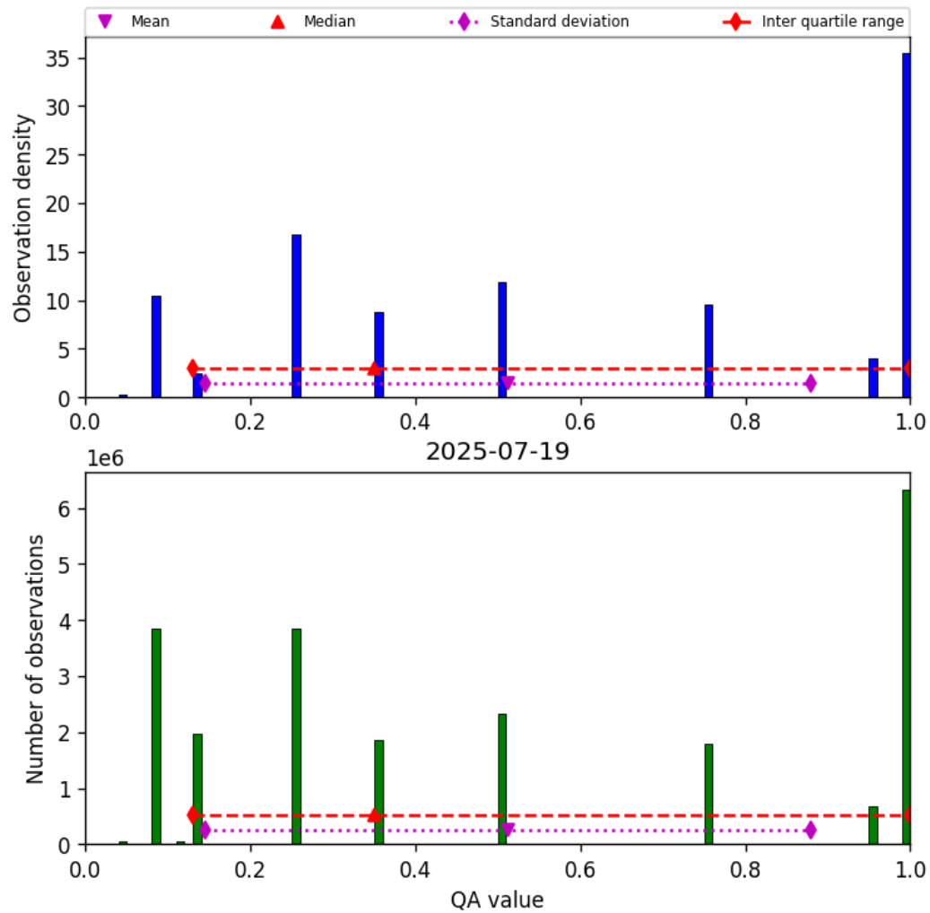
Figure 32: Histogram of “QA value” for 2025-07-19 to 2025-07-20
