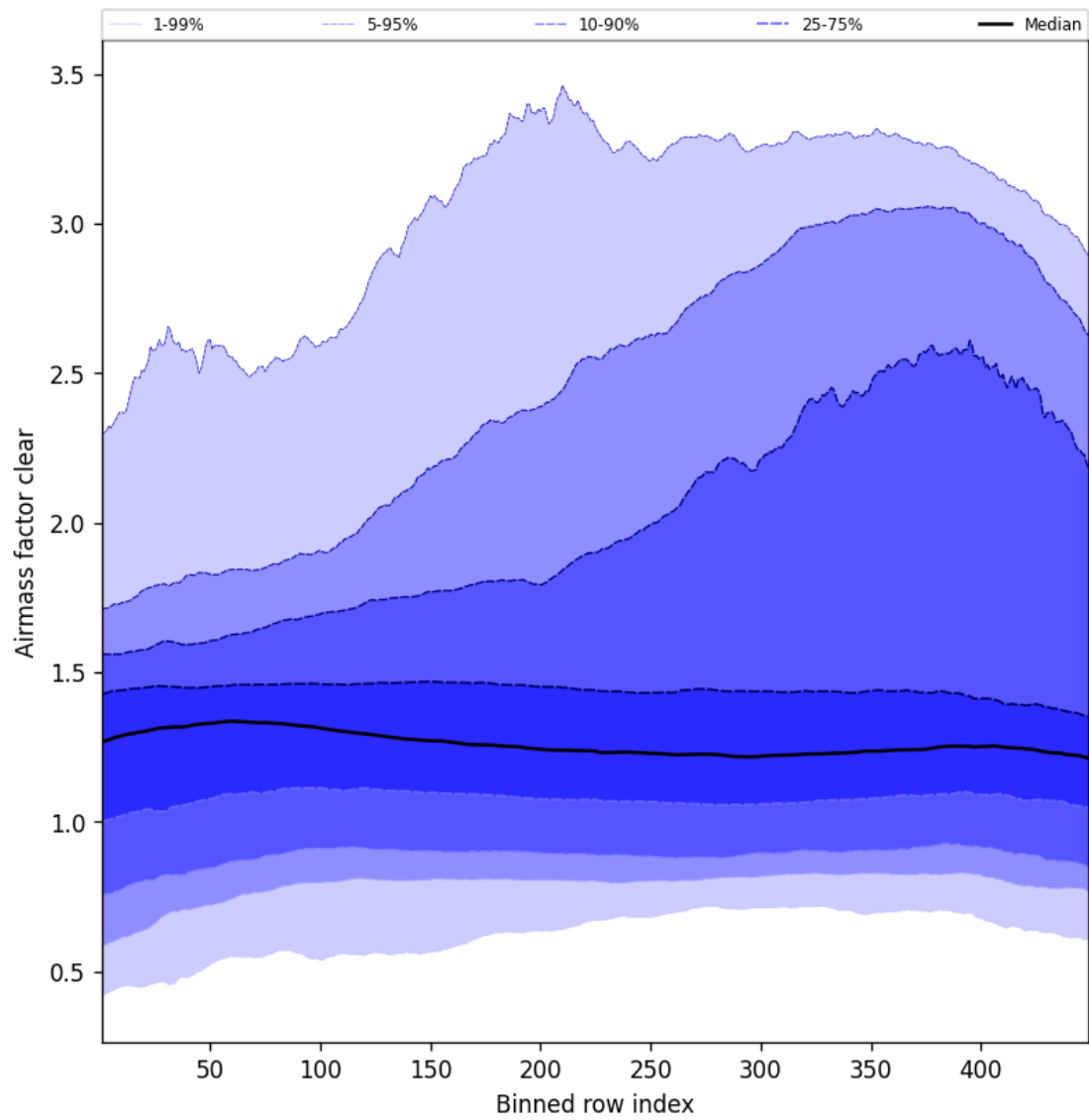
Figure 54: Along track statistics of “Airmass factor clear” for 2025-07-19 to 2025-07-20
