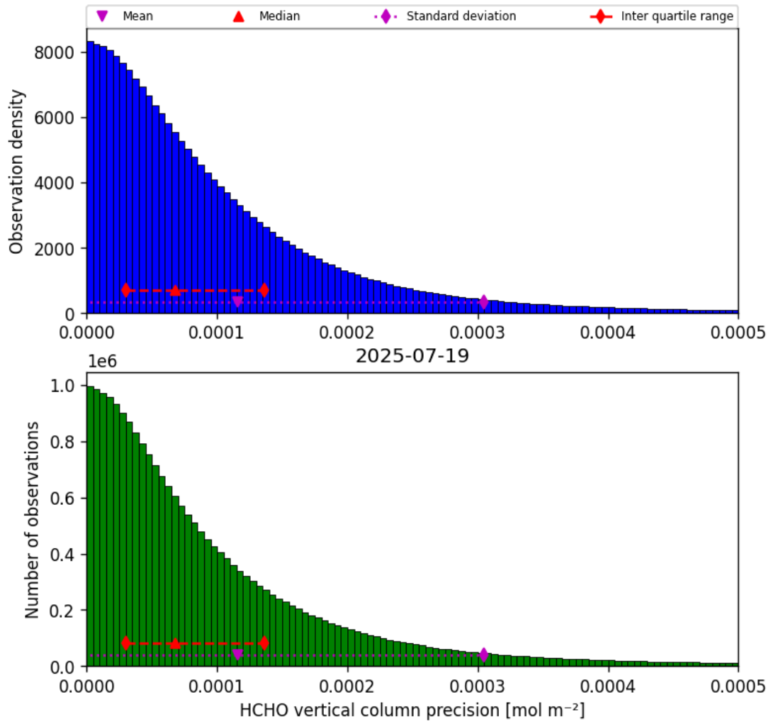
Figure 34: Histogram of “HCHO vertical column precision” for 2025-07-19 to 2025-07-20
