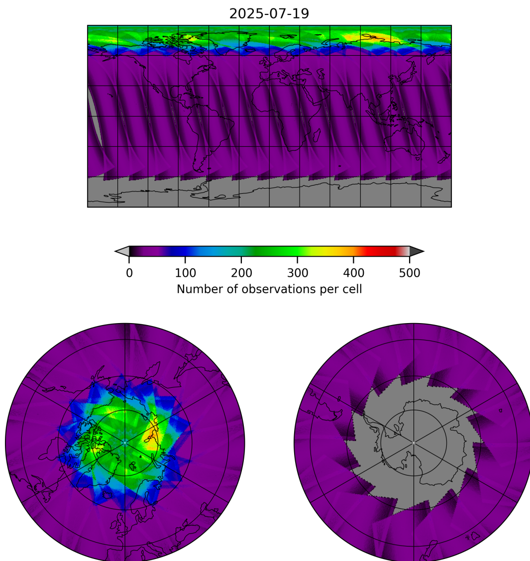
Figure 17: Map of the number of observations for 2025-07-19 to 2025-07-20
