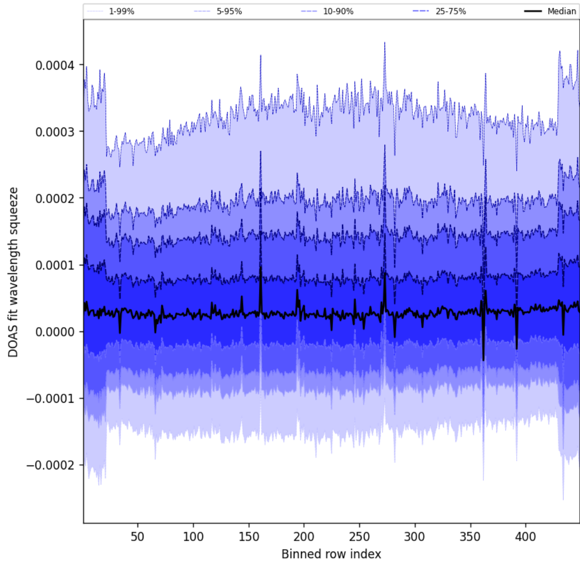
Figure 57: Along track statistics of “DOAS fit wavelength squeeze” for 2025-07-19 to 2025-07-20
