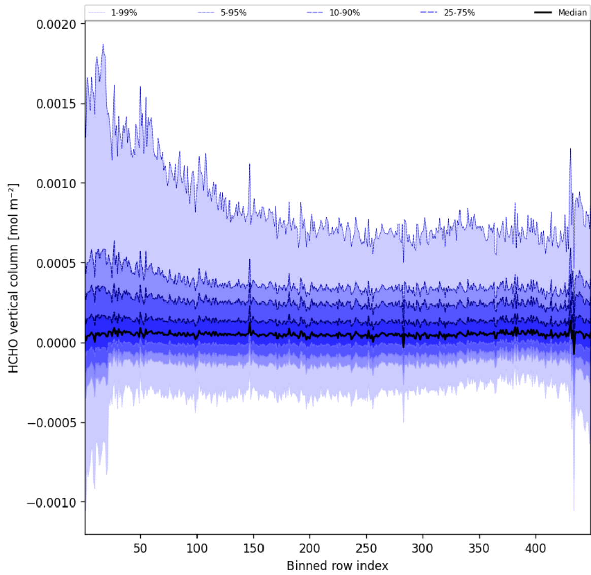
Figure 47: Along track statistics of “HCHO vertical column” for 2025-07-19 to 2025-07-20
