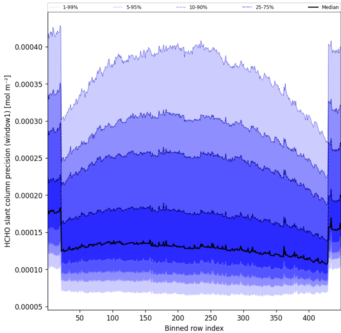
Figure 51: Along track statistics of “HCHO slant column precision (window1)” for 2025-07-19 to 2025-07-20
