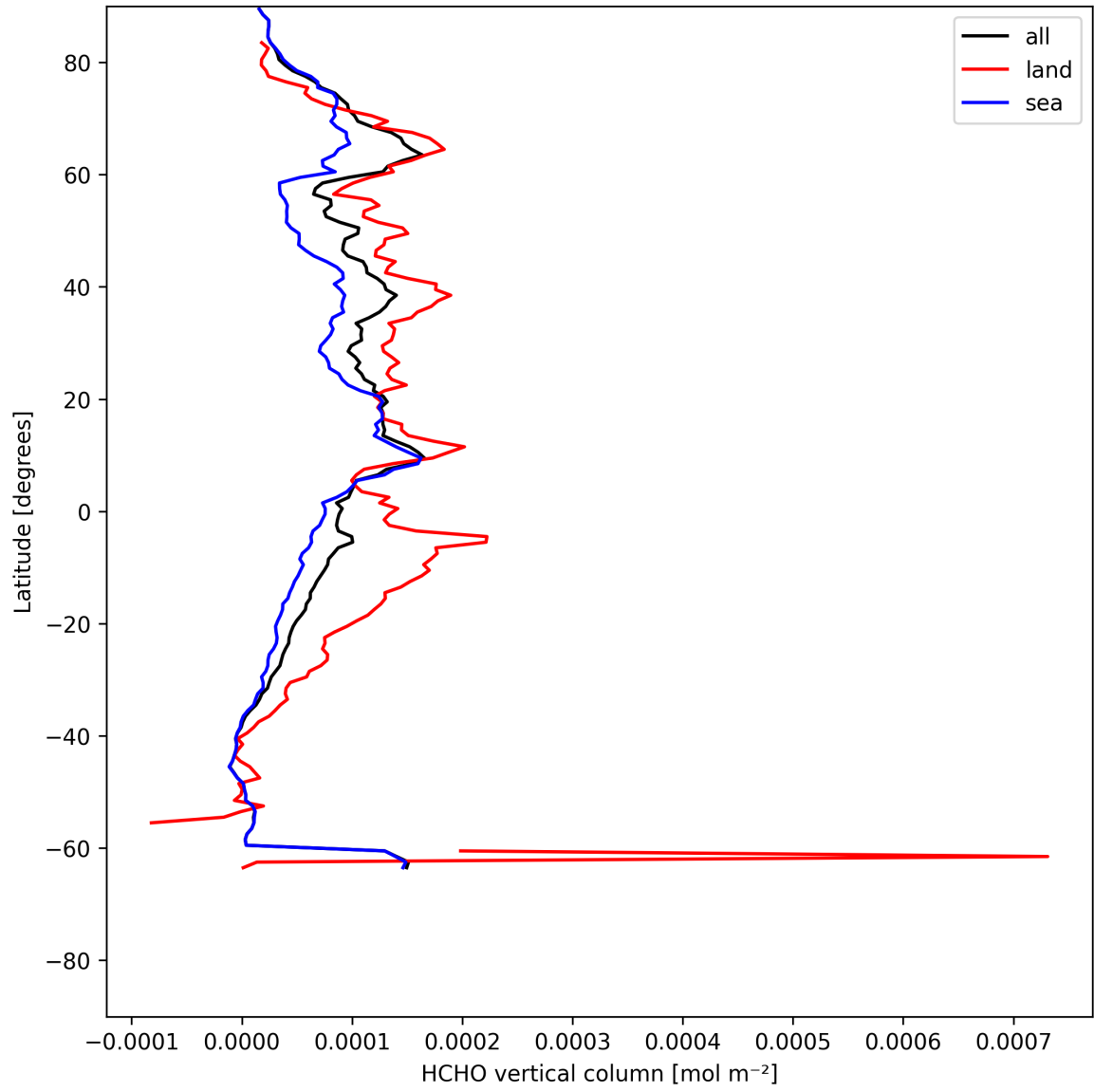
Figure 19: Zonal average of “HCHO vertical column” for 2025-07-19 to 2025-07-20.
