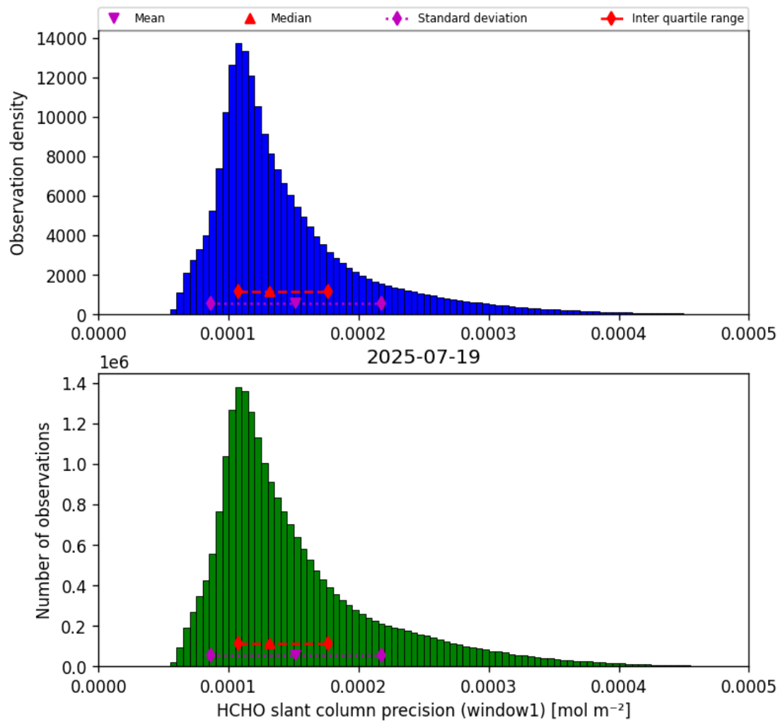
Figure 37: Histogram of “HCHO slant column precision (window1)” for 2025-07-19 to 2025-07-20
