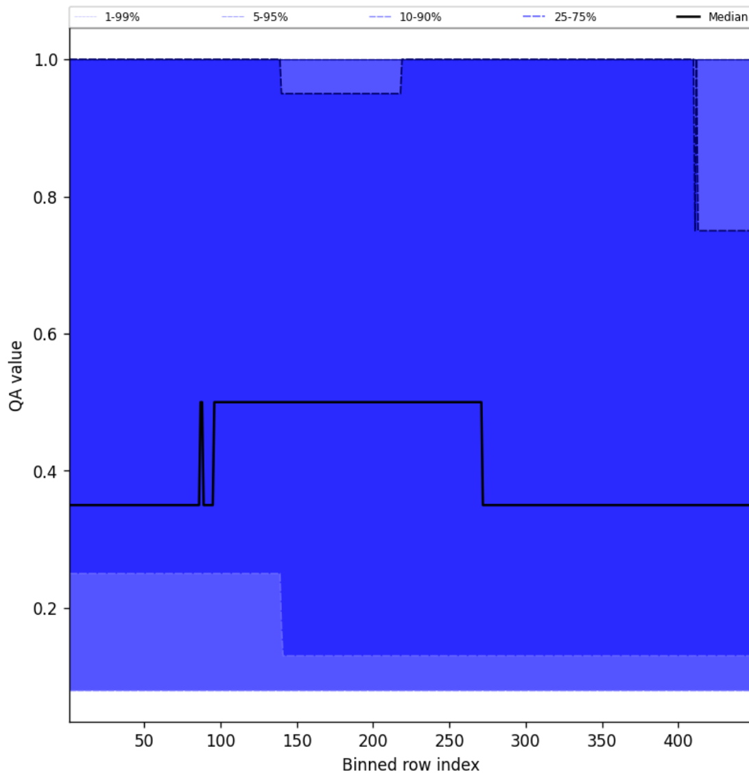
Figure 46: Along track statistics of “QA value” for 2025-07-19 to 2025-07-20
