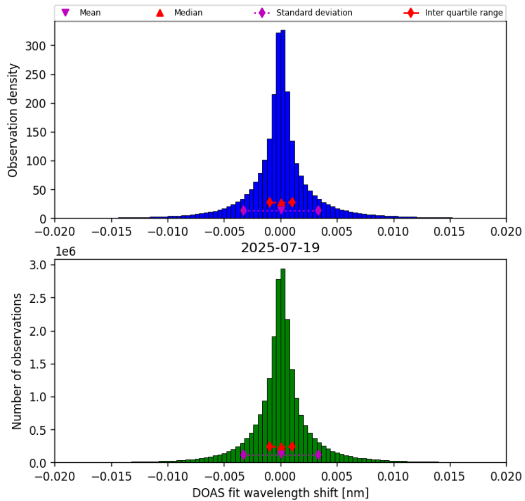
Figure 42: Histogram of “DOAS fit wavelength shift” for 2025-07-19 to 2025-07-20
