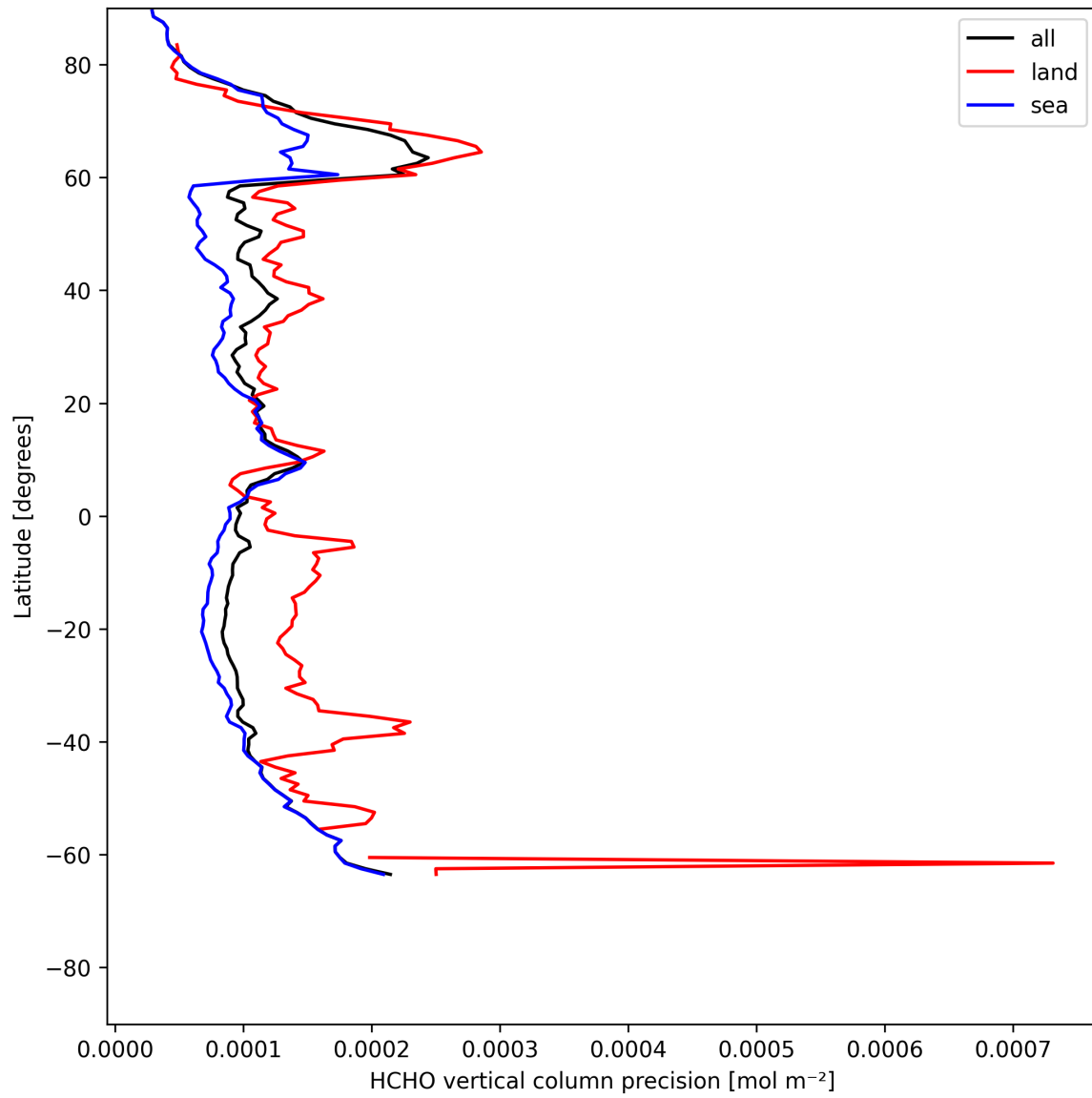
Figure 20: Zonal average of “HCHO vertical column precision” for 2025-07-19 to 2025-07-20.
