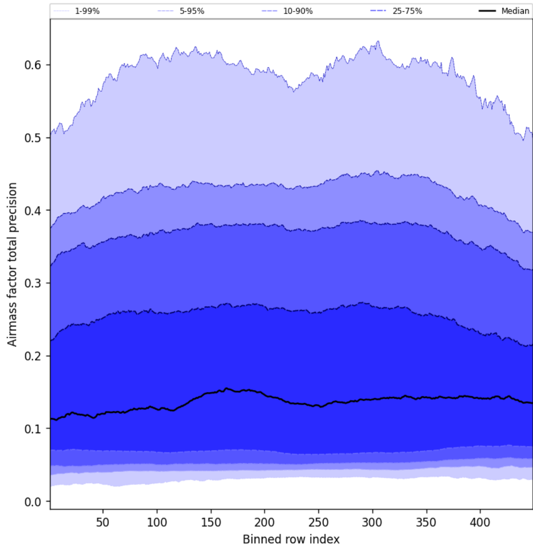
Figure 53: Along track statistics of “Airmass factor total precision” for 2025-07-19 to 2025-07-20
