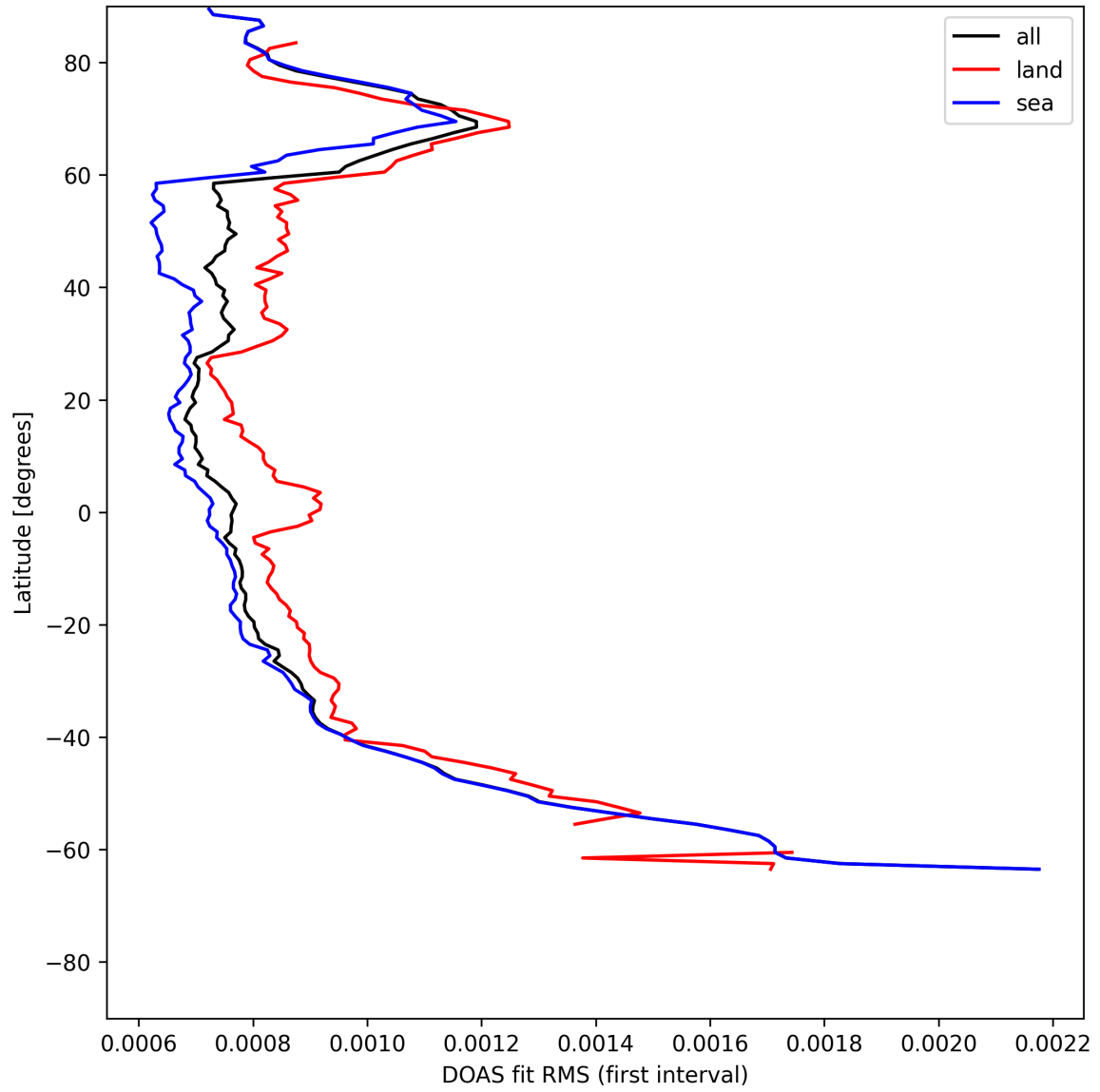
Figure 30: Zonal average of "DOAS fit RMS (first interval)" for 2025-07-19 to 2025-07-20.
