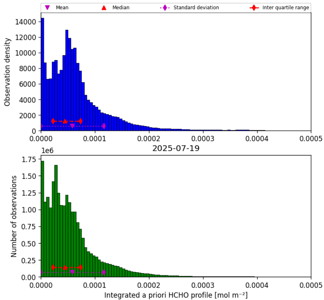
Figure 41: Histogram of “Integrated a priori HCHO profile” for 2025-07-19 to 2025-07-20
