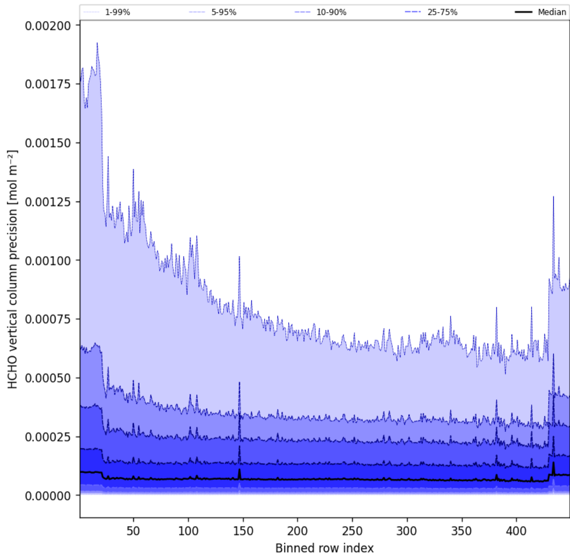
Figure 48: Along track statistics of “HCHO vertical column precision” for 2025-07-19 to 2025-07-20
