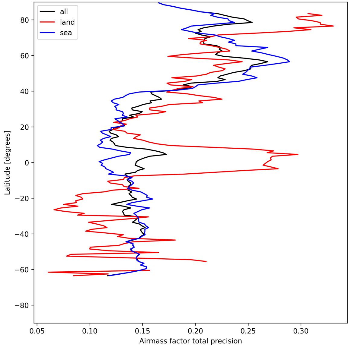
Figure 25: Zonal average of “Airmass factor total precision” for 2025-07-19 to 2025-07-20.
