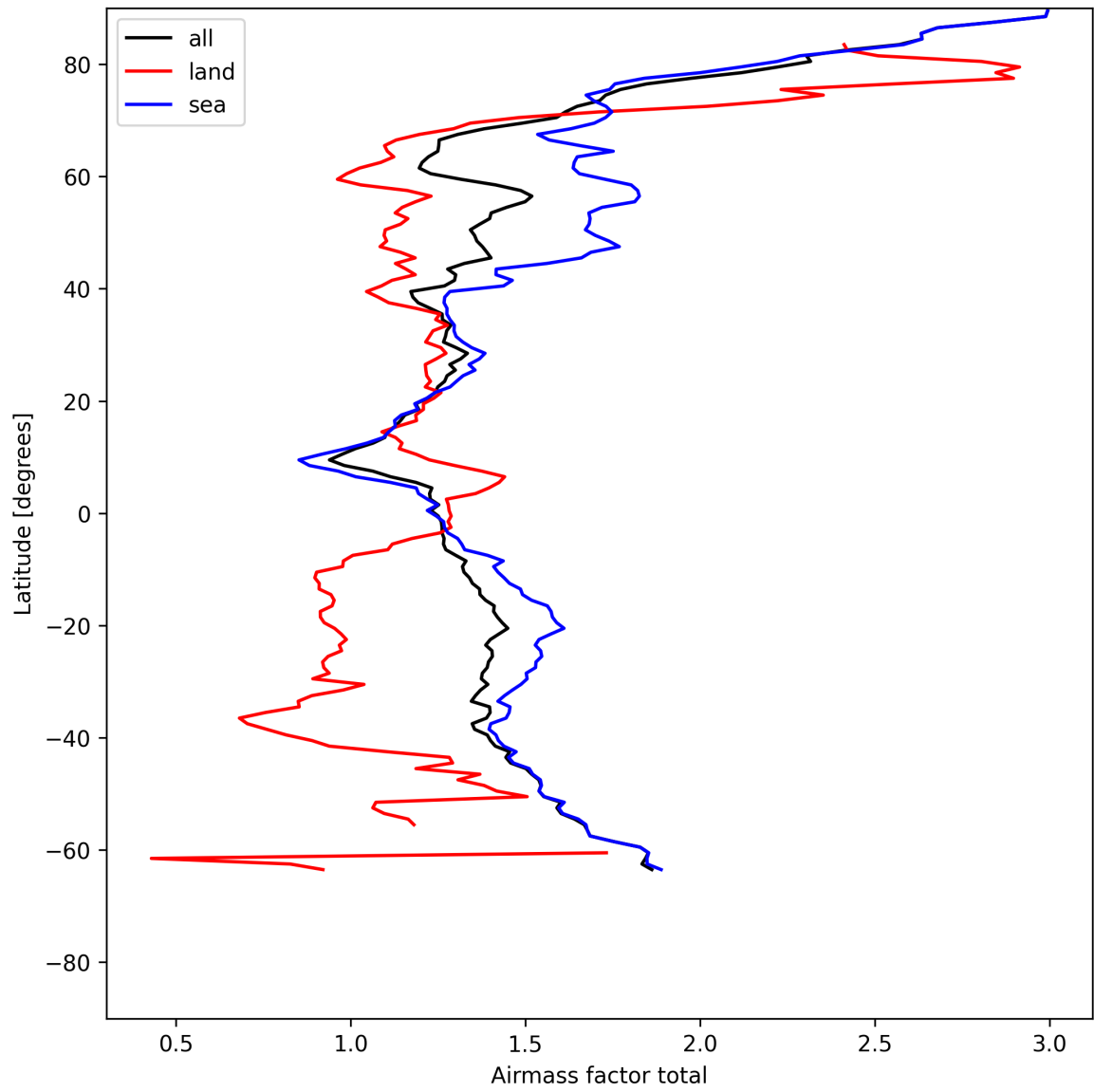
Figure 24: Zonal average of “Airmass factor total” for 2025-07-19 to 2025-07-20.
