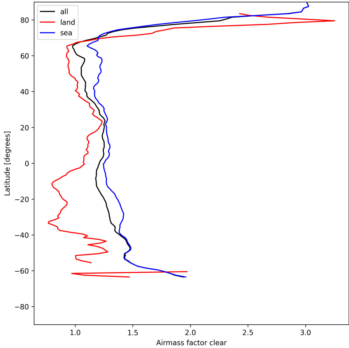
Figure 26: Zonal average of “Airmass factor clear” for 2025-07-19 to 2025-07-20.
