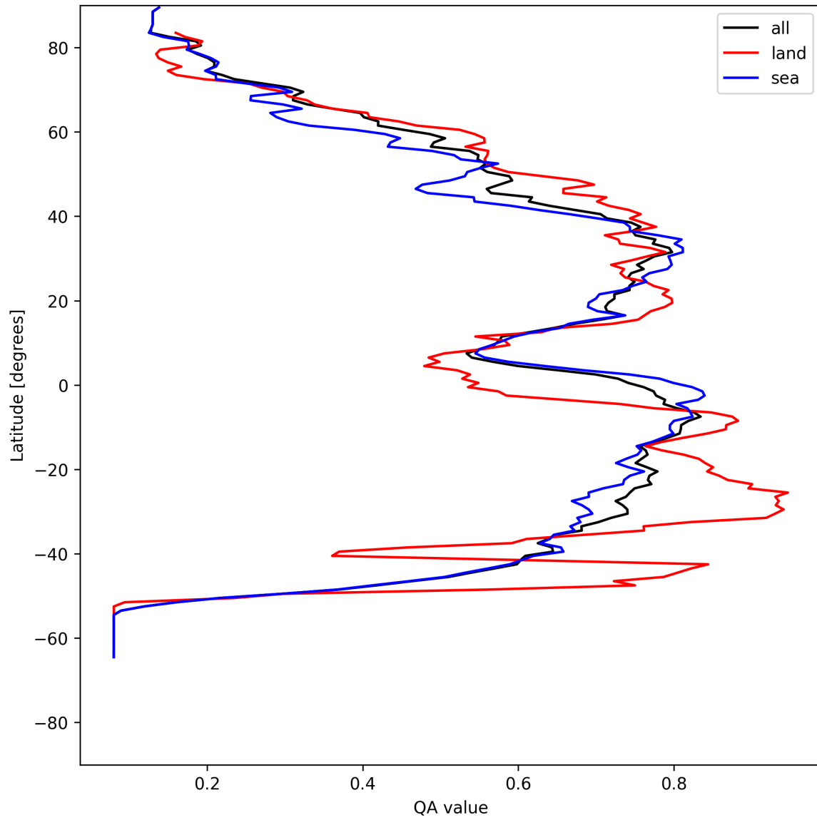
Figure 18: Zonal average of “QA value” for 2025-07-20 to 2025-07-21.
