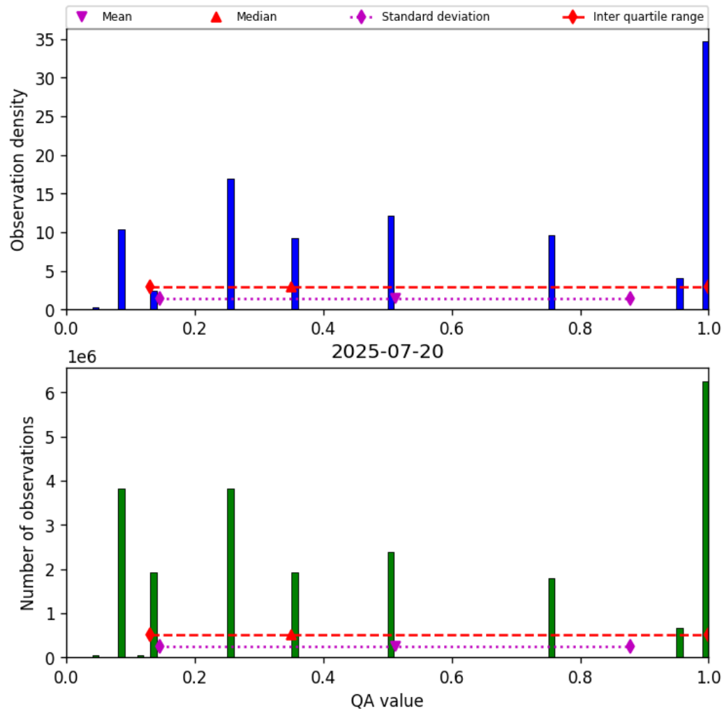
Figure 32: Histogram of “QA value” for 2025-07-20 to 2025-07-21
