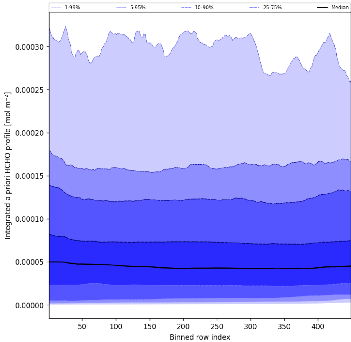
Figure 55: Along track statistics of “Integrated a priori HCHO profile” for 2025-07-20 to 2025-07-21
