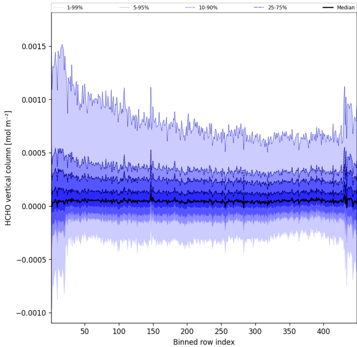
Figure 47: Along track statistics of “HCHO vertical column” for 2025-07-20 to 2025-07-21
