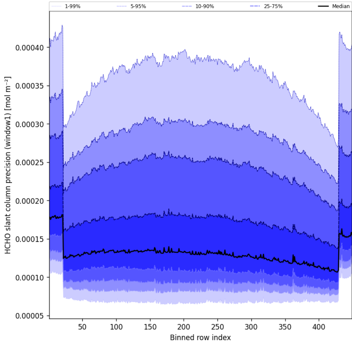
Figure 51: Along track statistics of “HCHO slant column precision (window1)” for 2025-07-20 to 2025-07-21
