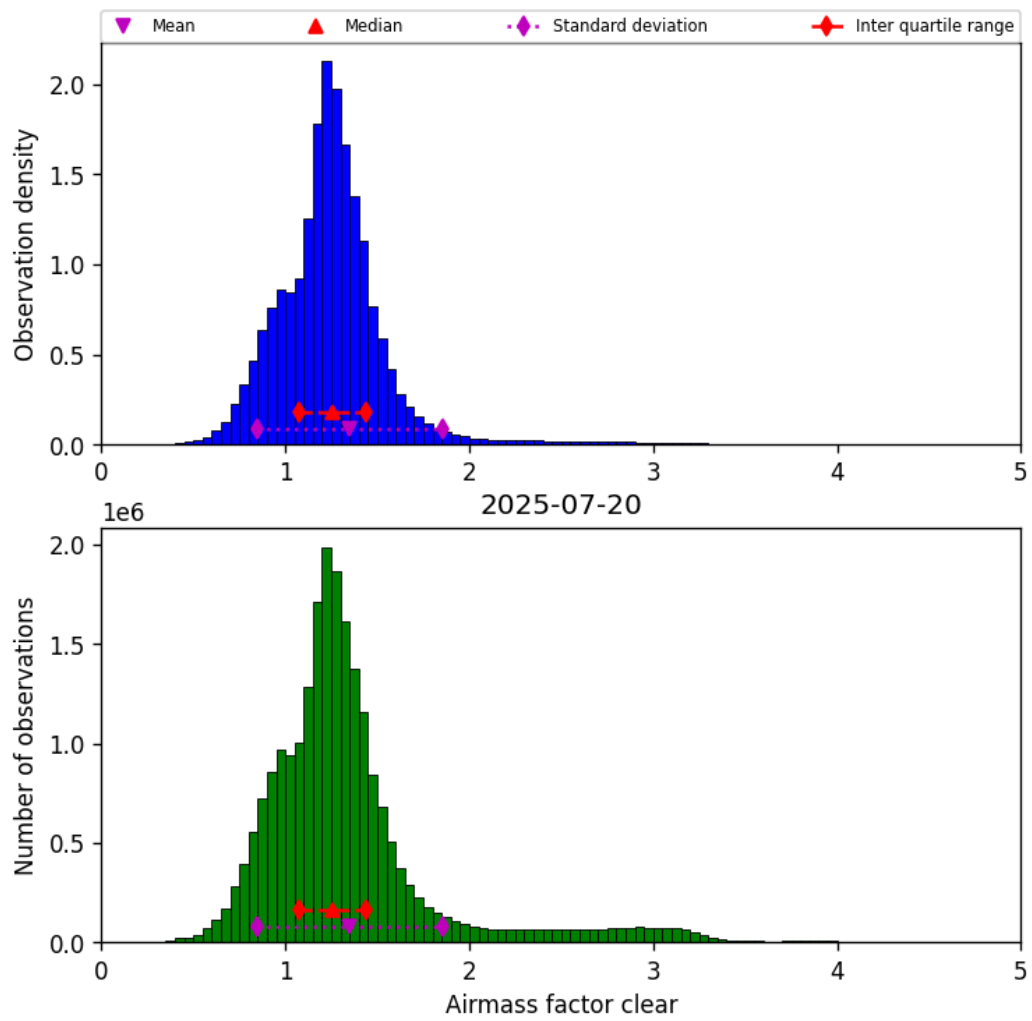
Figure 40: Histogram of “Airmass factor clear” for 2025-07-20 to 2025-07-21
