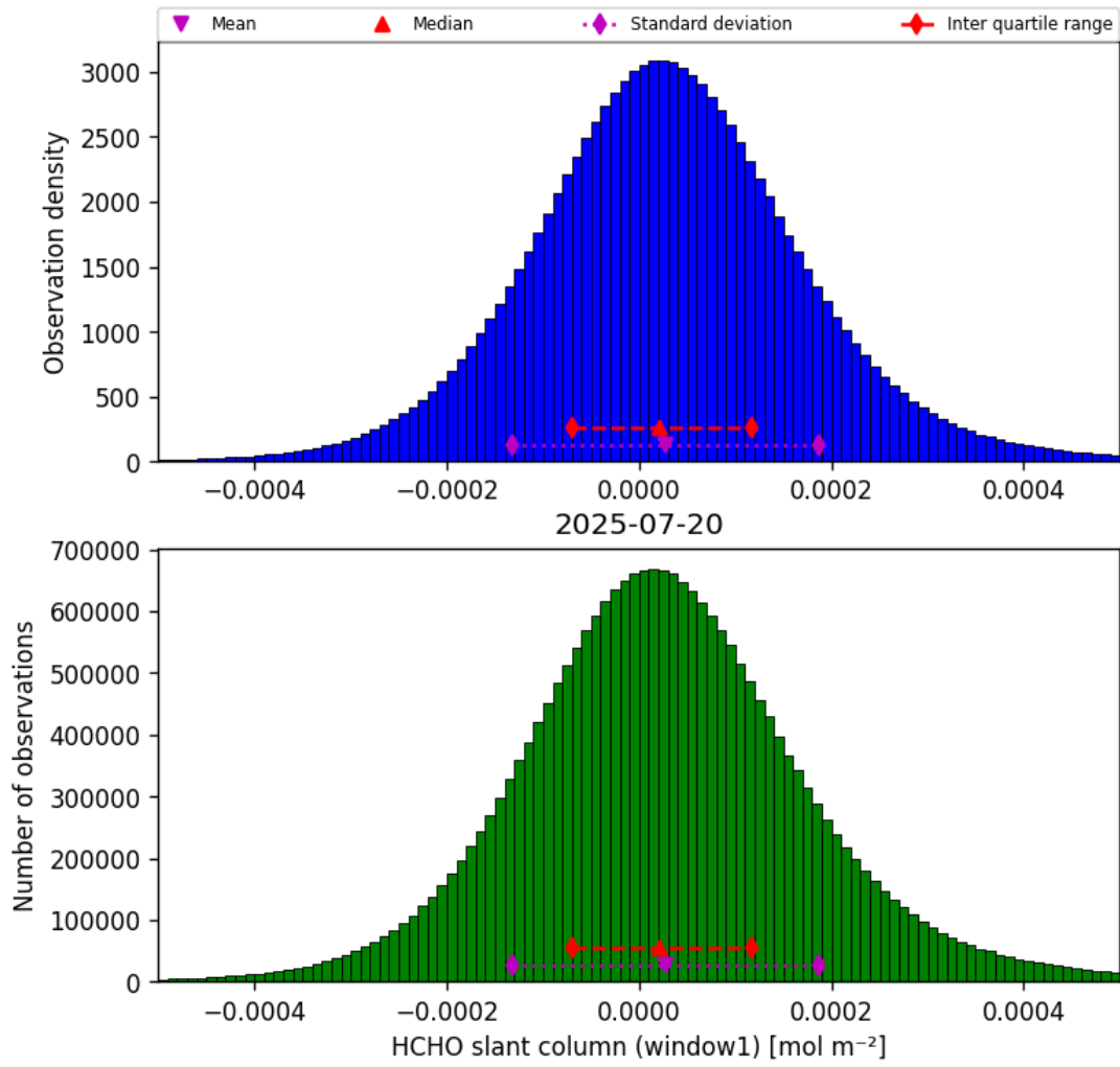
Figure 36: Histogram of “HCHO slant column (window1)” for 2025-07-20 to 2025-07-21
