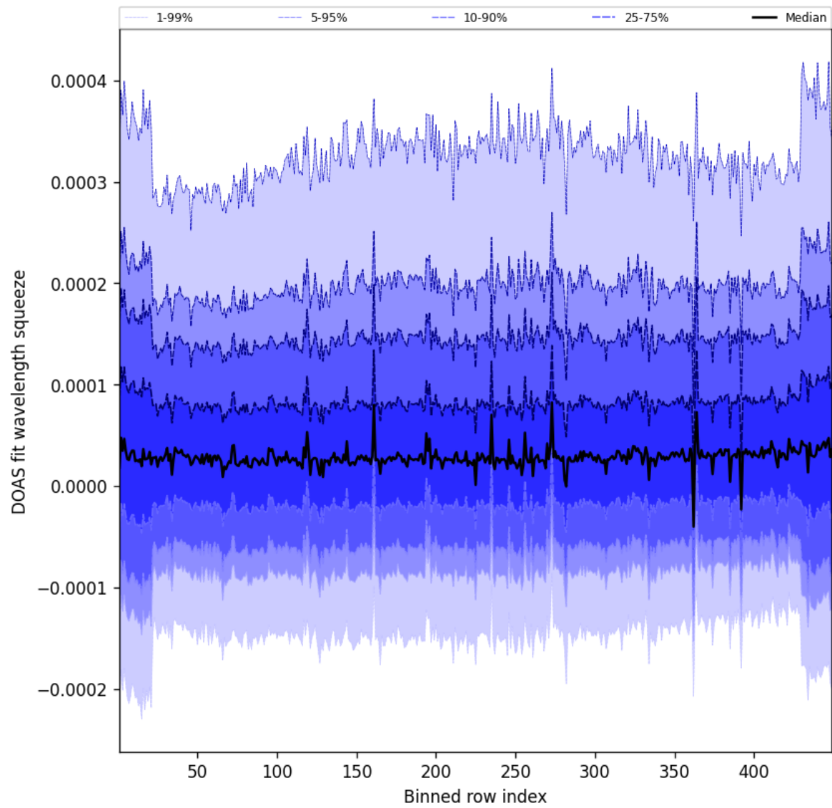
Figure 57: Along track statistics of “DOAS fit wavelength squeeze” for 2025-07-20 to 2025-07-21
