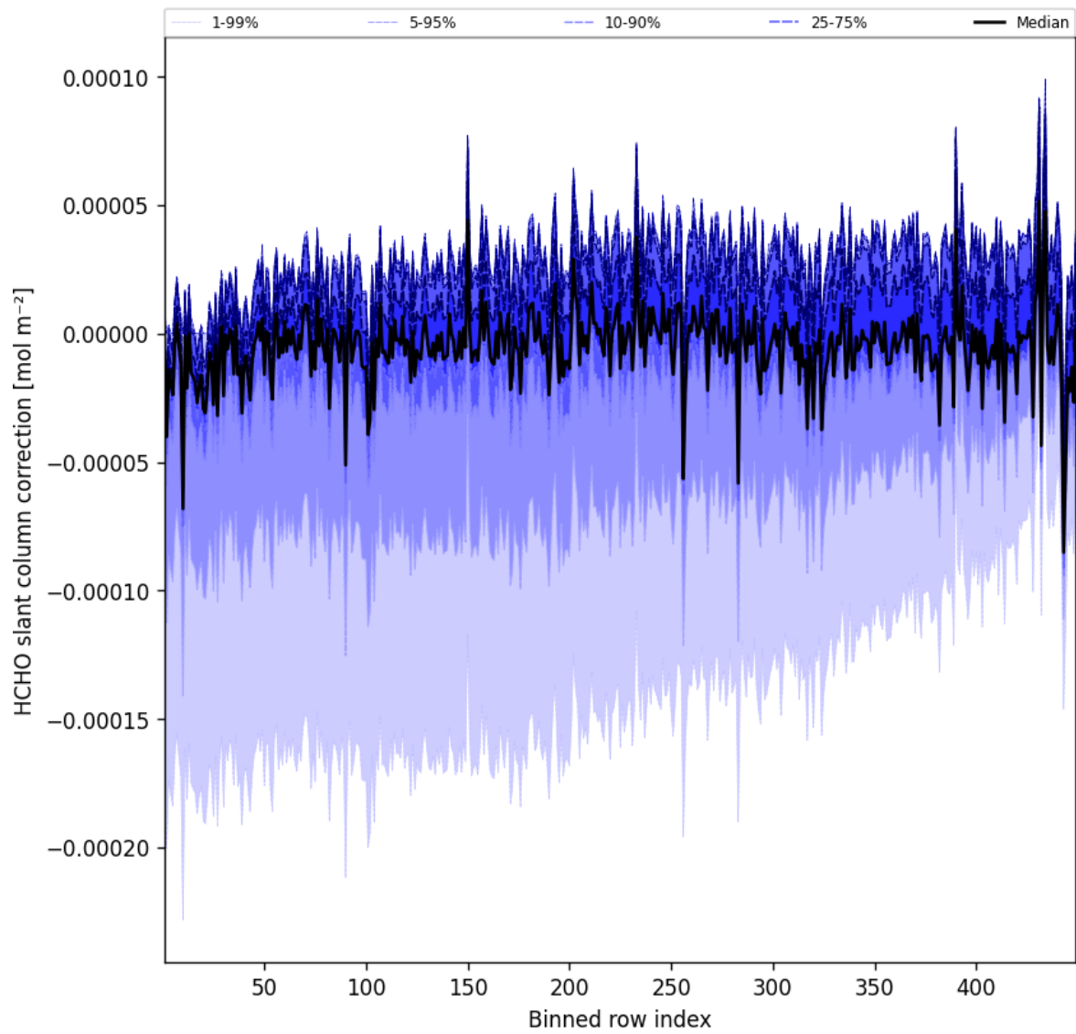
Figure 59: Along track statistics of “HCHO slant column correction” for 2025-07-20 to 2025-07-21
