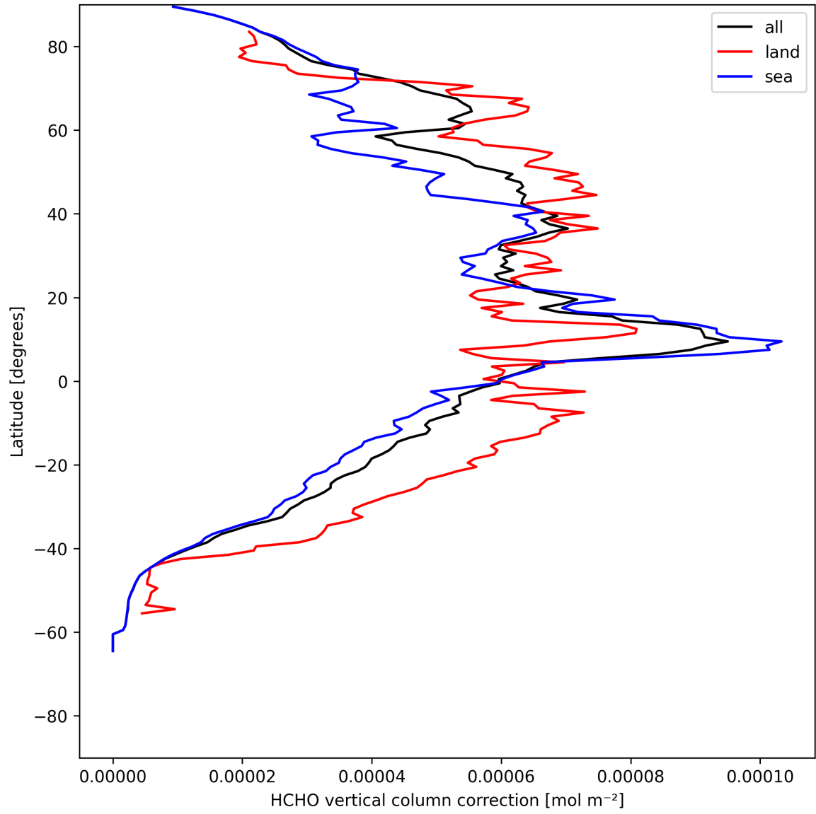
Figure 21: Zonal average of “HCHO vertical column correction” for 2025-07-20 to 2025-07-21.
