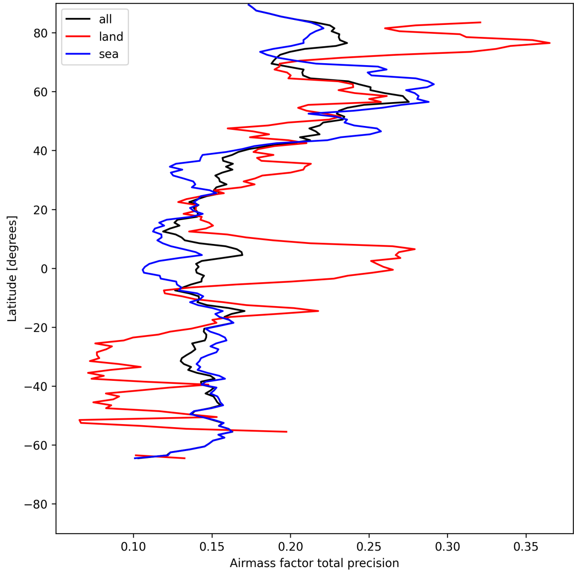
Figure 25: Zonal average of “Airmass factor total precision” for 2025-07-20 to 2025-07-21.
