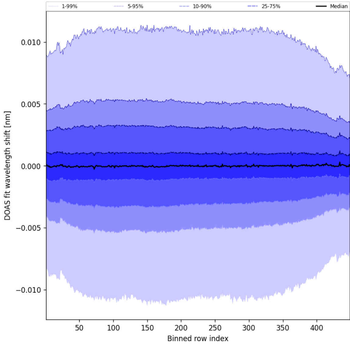
Figure 56: Along track statistics of “DOAS fit wavelength shift” for 2025-07-20 to 2025-07-21
