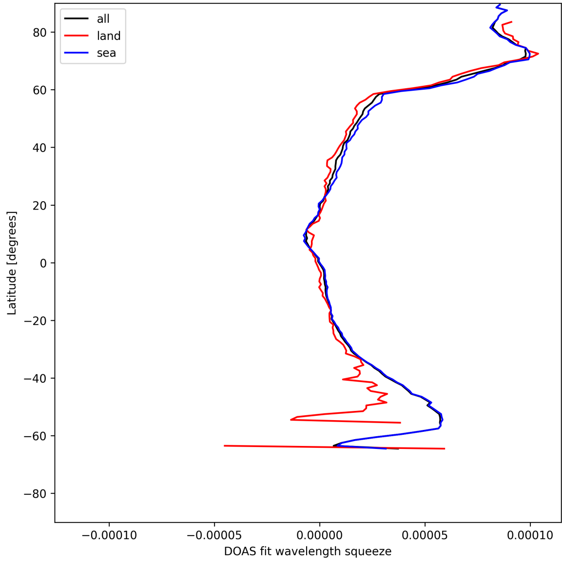
Figure 29: Zonal average of “DOAS fit wavelength squeeze” for 2025-07-20 to 2025-07-21.
