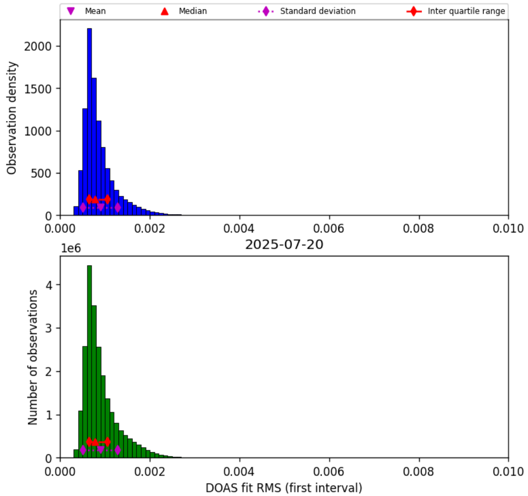
Figure 44: Histogram of “DOAS fit RMS (first interval)” for 2025-07-20 to 2025-07-21
