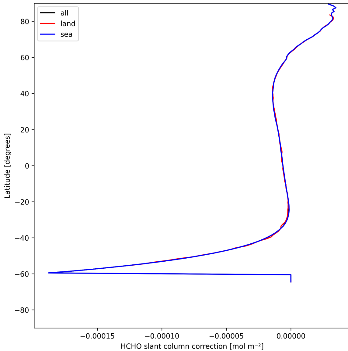
Figure 31: Zonal average of “HCHO slant column correction” for 2025-07-20 to 2025-07-21.
