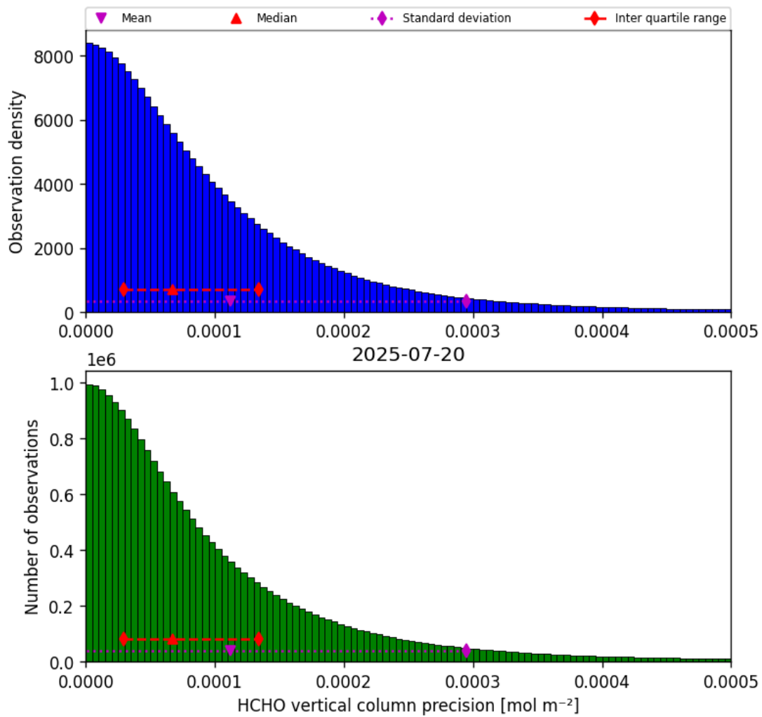
Figure 34: Histogram of “HCHO vertical column precision” for 2025-07-20 to 2025-07-21
