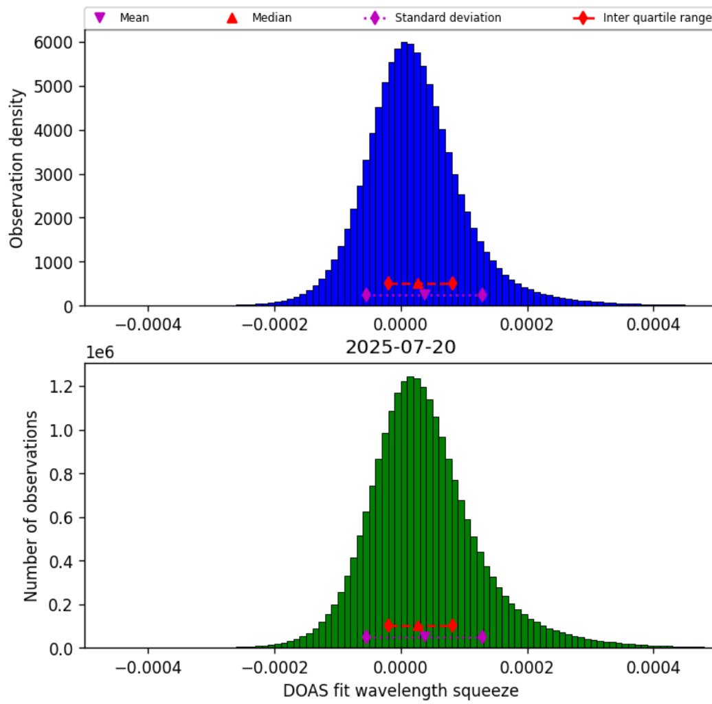
Figure 43: Histogram of “DOAS fit wavelength squeeze” for 2025-07-20 to 2025-07-21
