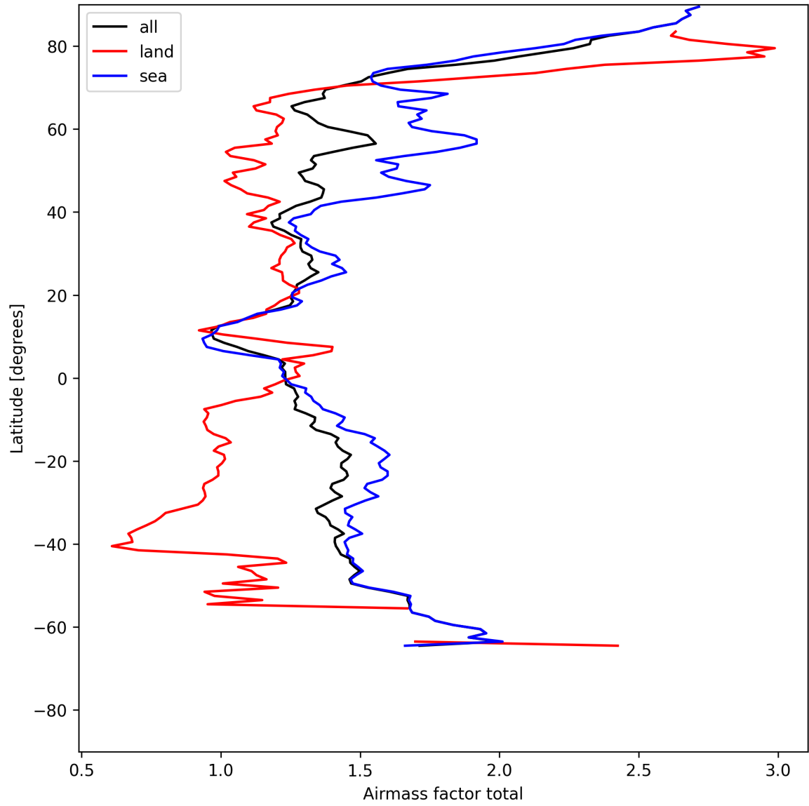
Figure 24: Zonal average of “Airmass factor total” for 2025-07-20 to 2025-07-21.
