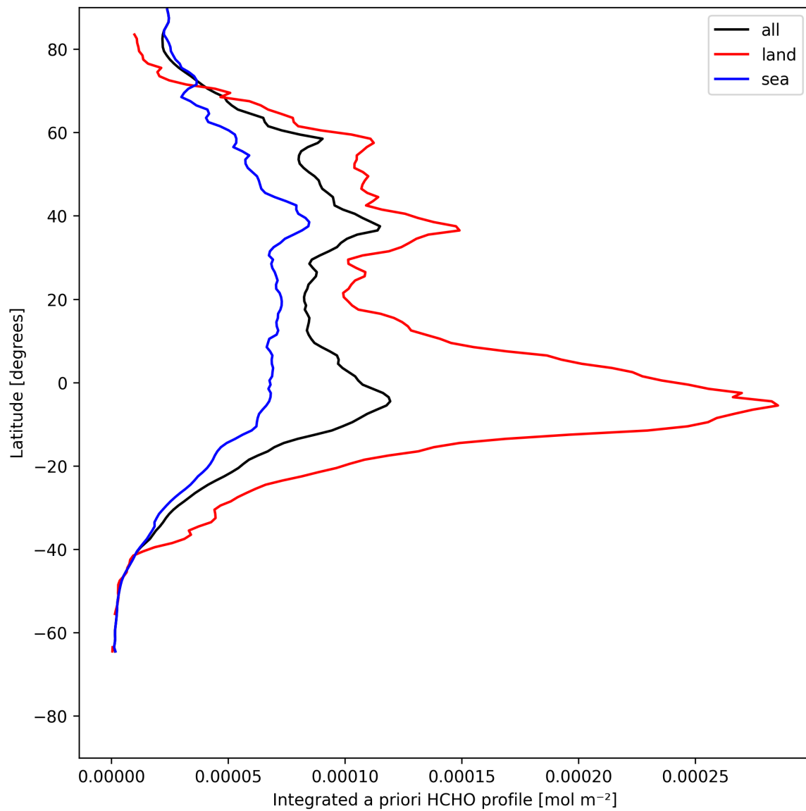
Figure 27: Zonal average of “Integrated a priori HCHO profile” for 2025-07-20 to 2025-07-21.
