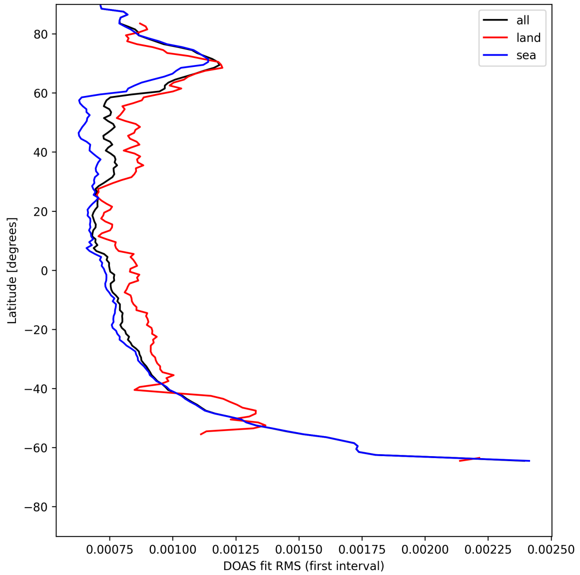
Figure 30: Zonal average of “DOAS fit RMS (first interval)” for 2025-07-20 to 2025-07-21.
