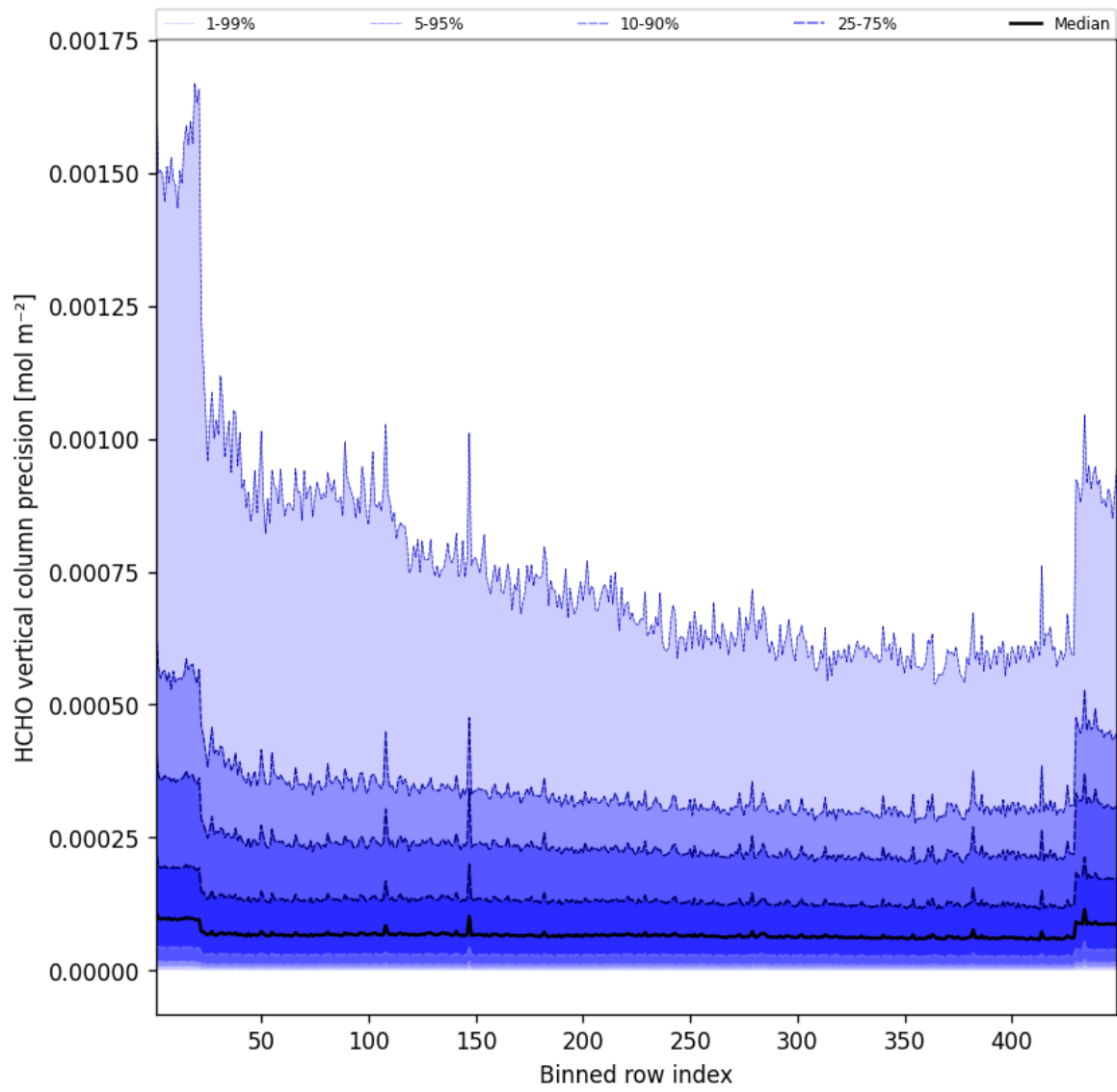
Figure 48: Along track statistics of “HCHO vertical column precision” for 2025-07-20 to 2025-07-21
