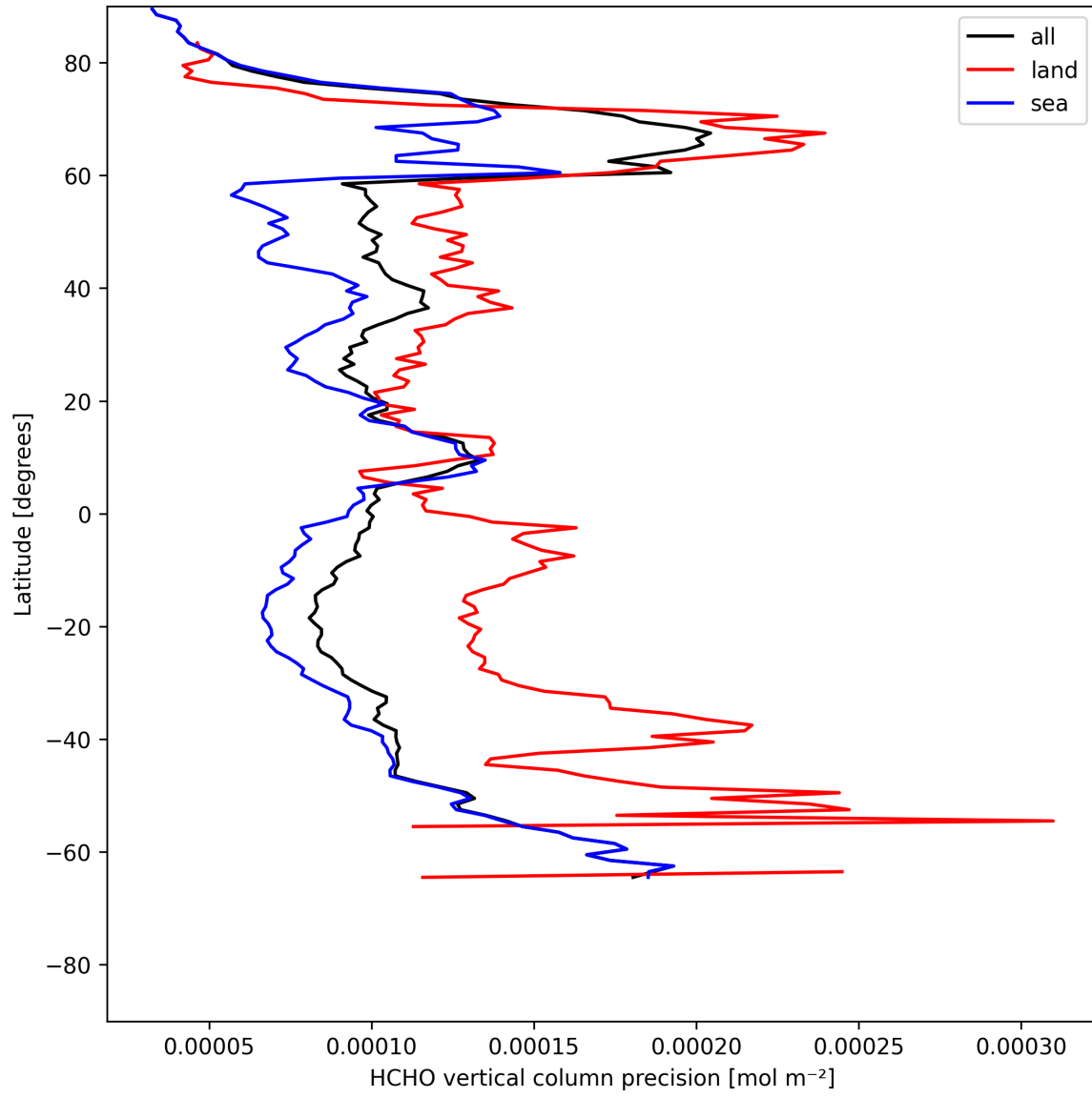
Figure 20: Zonal average of “HCHO vertical column precision” for 2025-07-20 to 2025-07-21.
