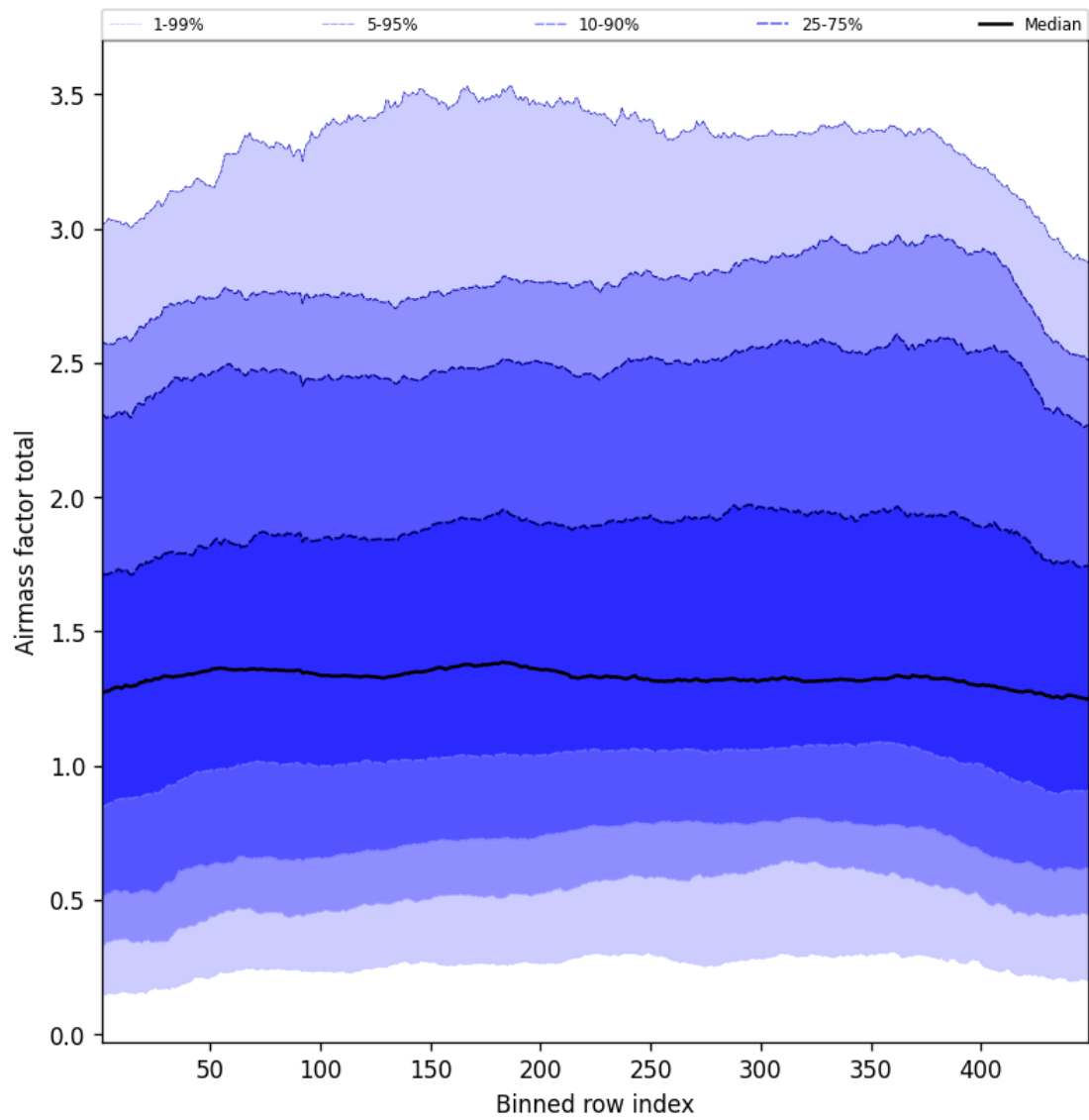
Figure 52: Along track statistics of “Airmass factor total” for 2025-07-20 to 2025-07-21
