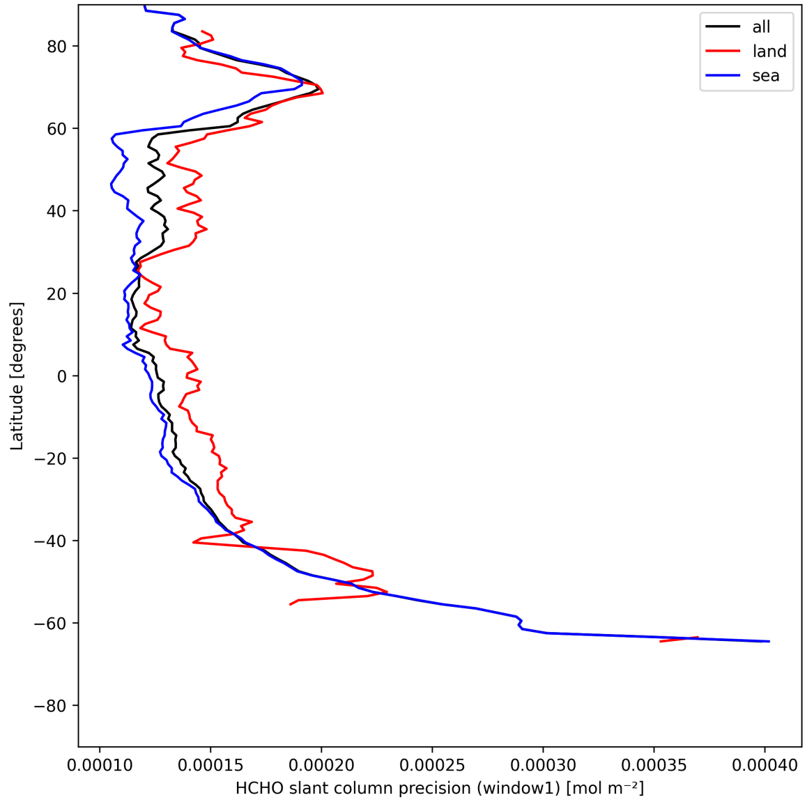
Figure 23: Zonal average of “HCHO slant column precision (window1)” for 2025-07-20 to 2025-07-21.
