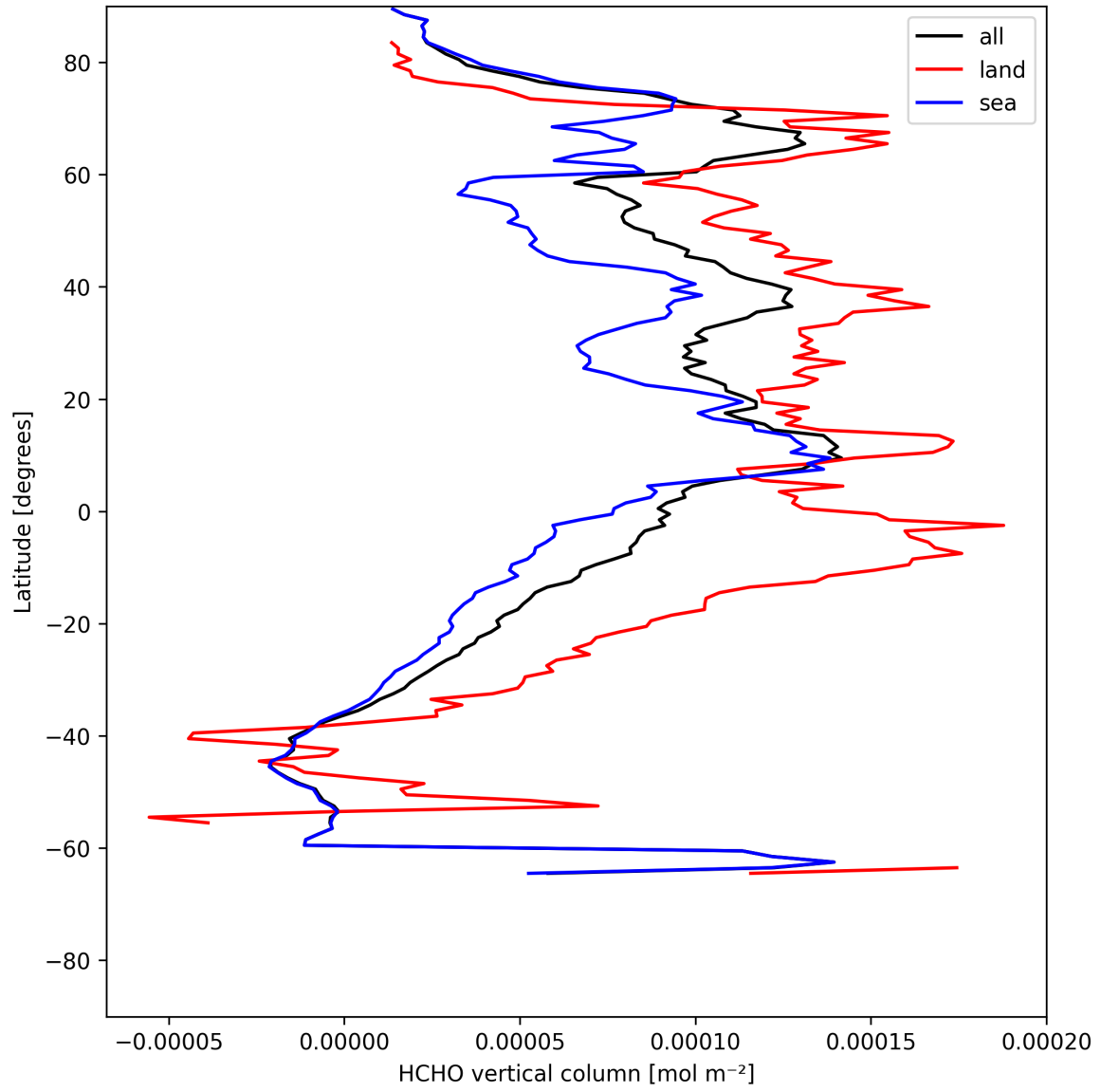
Figure 19: Zonal average of “HCHO vertical column” for 2025-07-20 to 2025-07-21.
