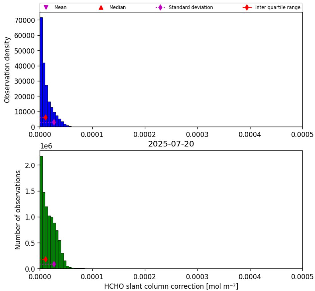
Figure 45: Histogram of “HCHO slant column correction” for 2025-07-20 to 2025-07-21
