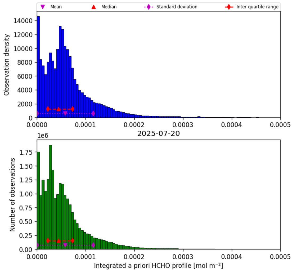
Figure 41: Histogram of “Integrated a priori HCHO profile” for 2025-07-20 to 2025-07-21
