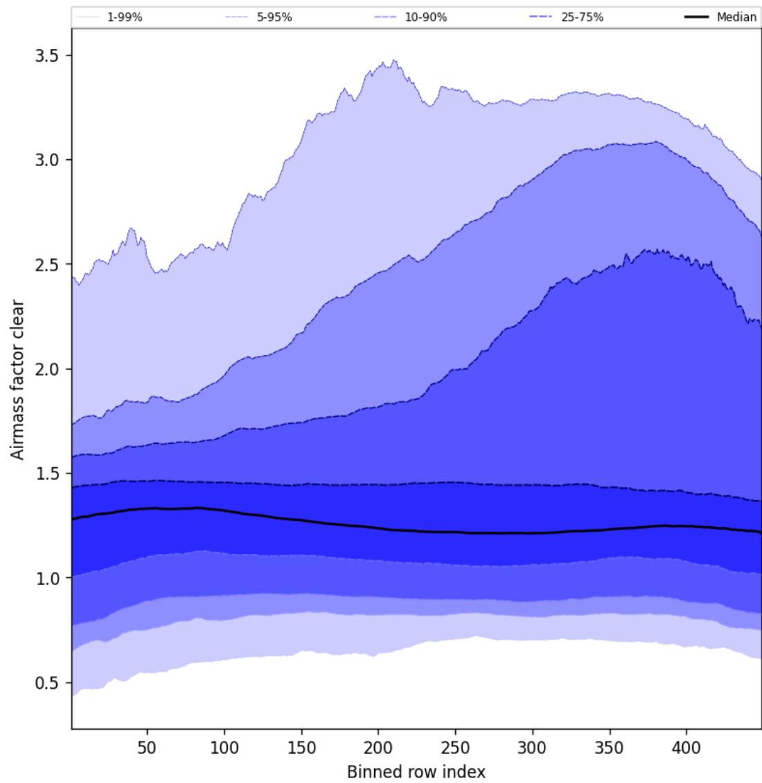
Figure 54: Along track statistics of “Airmass factor clear” for 2025-07-20 to 2025-07-21
