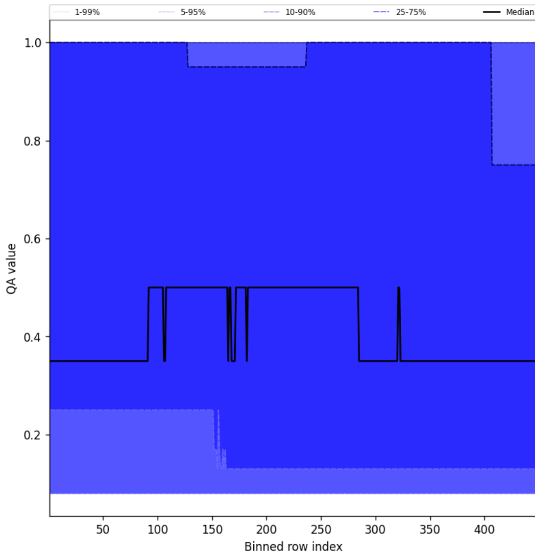
Figure 46: Along track statistics of “QA value” for 2025-07-20 to 2025-07-21
