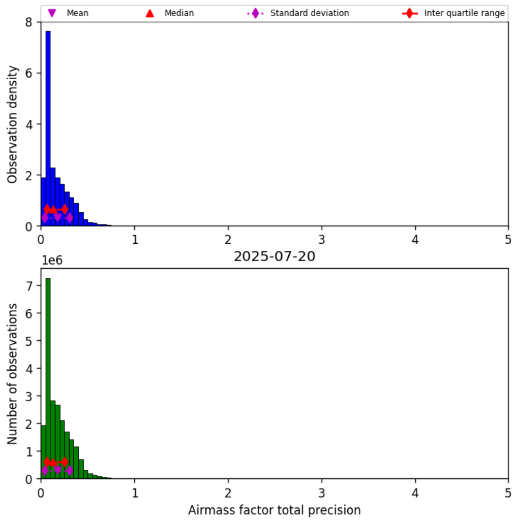
Figure 39: Histogram of “Airmass factor total precision” for 2025-07-20 to 2025-07-21
