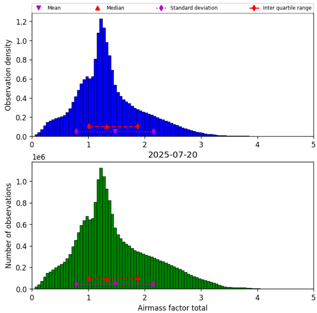
Figure 38: Histogram of “Airmass factor total” for 2025-07-20 to 2025-07-21
