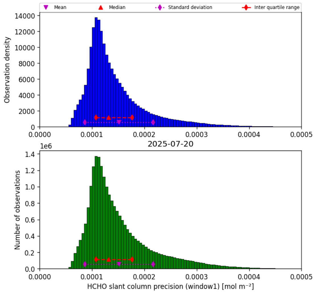
Figure 37: Histogram of “HCHO slant column precision (window1)” for 2025-07-20 to 2025-07-21
