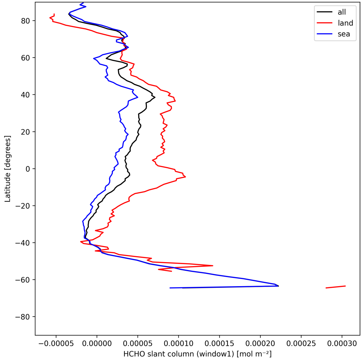
Figure 22: Zonal average of “HCHO slant column (window1)” for 2025-07-20 to 2025-07-21.
