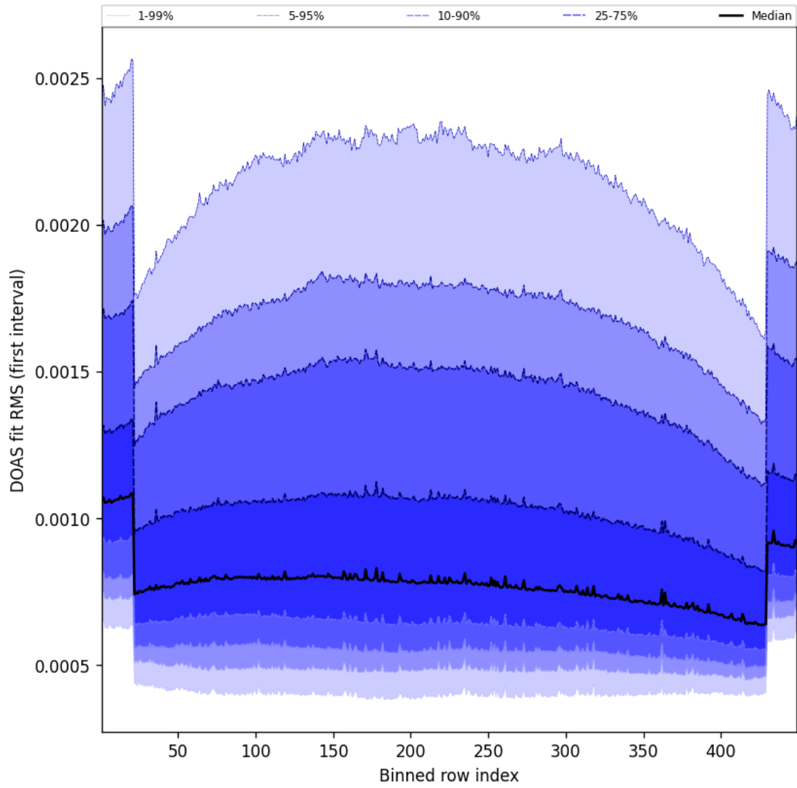
Figure 58: Along track statistics of “DOAS fit RMS (first interval)” for 2025-07-20 to 2025-07-21
