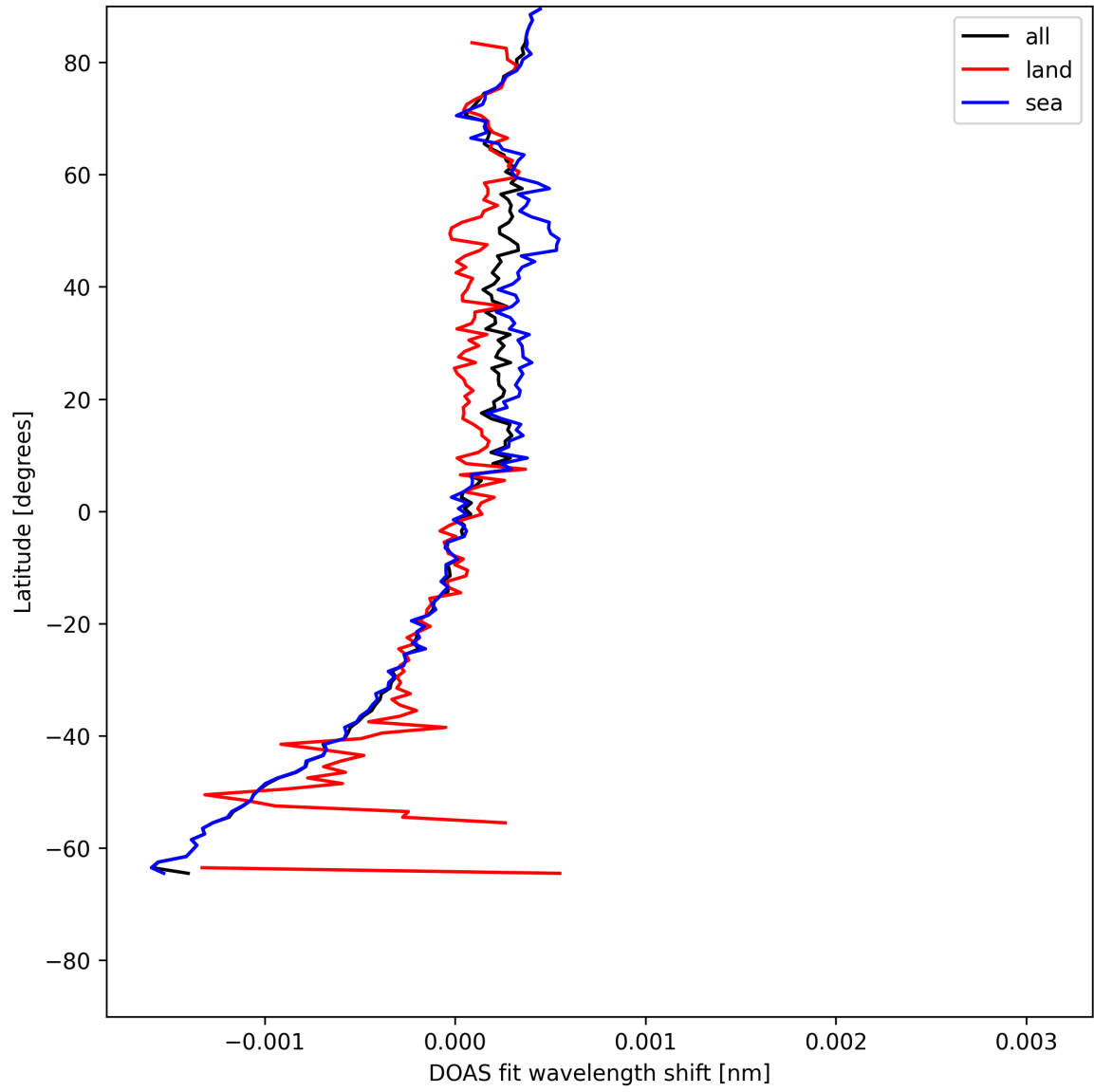
Figure 28: Zonal average of "DOAS fit wavelength shift" for 2025-07-20 to 2025-07-21.
