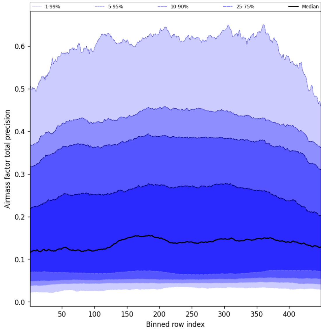
Figure 53: Along track statistics of “Airmass factor total precision” for 2025-07-20 to 2025-07-21
