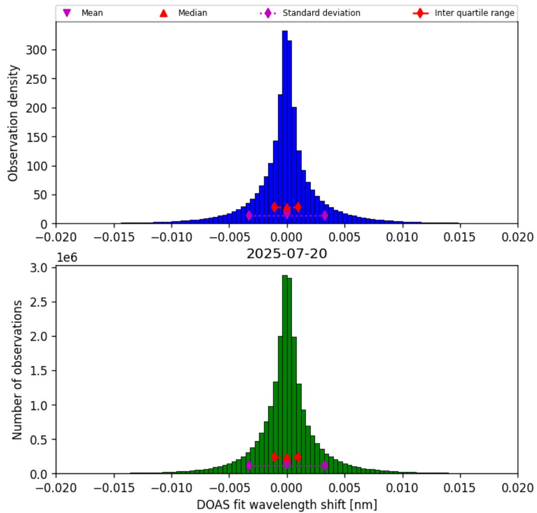
Figure 42: Histogram of “DOAS fit wavelength shift” for 2025-07-20 to 2025-07-21
