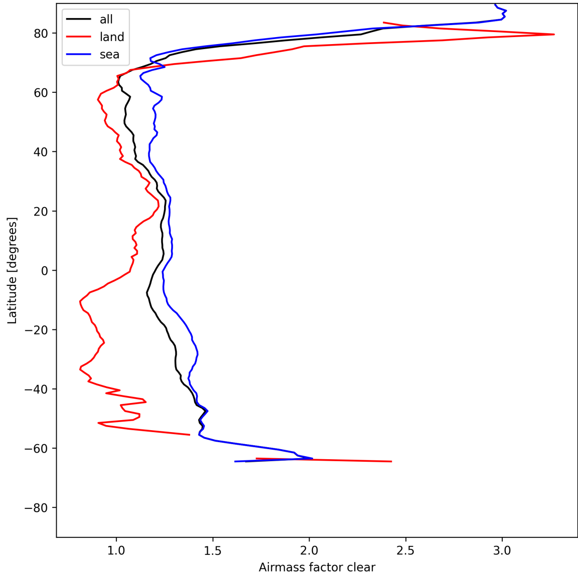
Figure 26: Zonal average of “Airmass factor clear” for 2025-07-20 to 2025-07-21.
