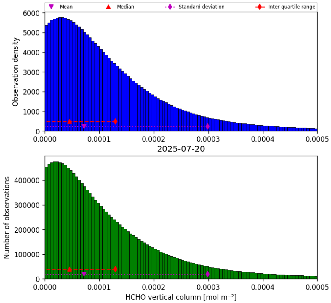
Figure 33: Histogram of “HCHO vertical column” for 2025-07-20 to 2025-07-21
