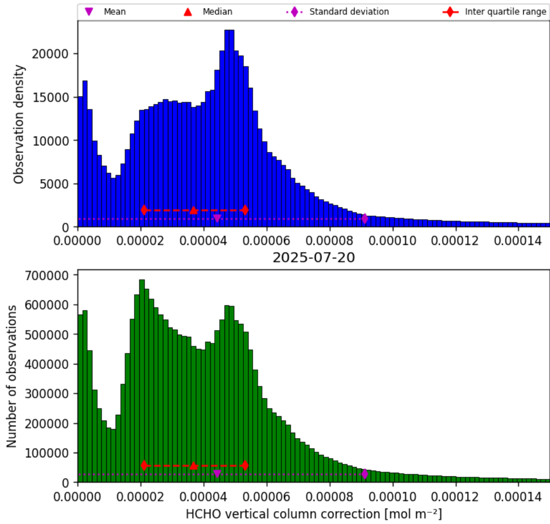
Figure 35: Histogram of “HCHO vertical column correction” for 2025-07-20 to 2025-07-21
