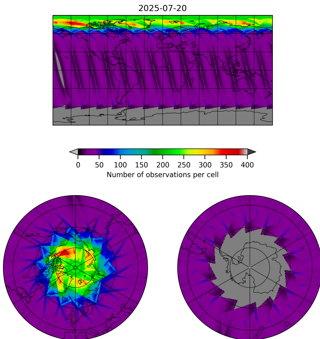
Figure 17: Map of the number of observations for 2025-07-20 to 2025-07-21
