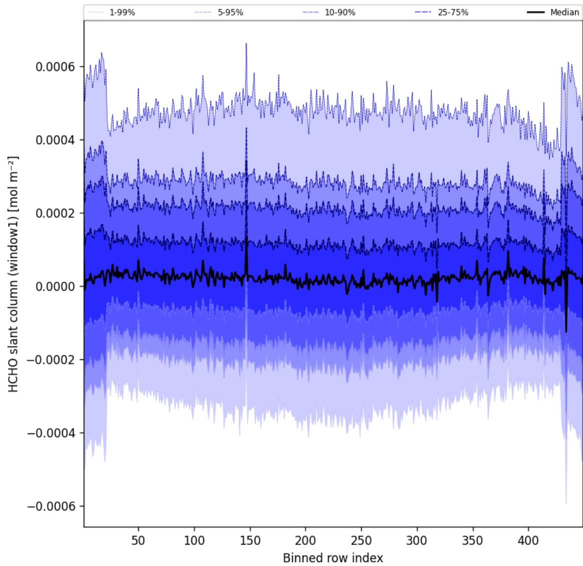
Figure 50: Along track statistics of “HCHO slant column (window1)” for 2025-07-20 to 2025-07-21
