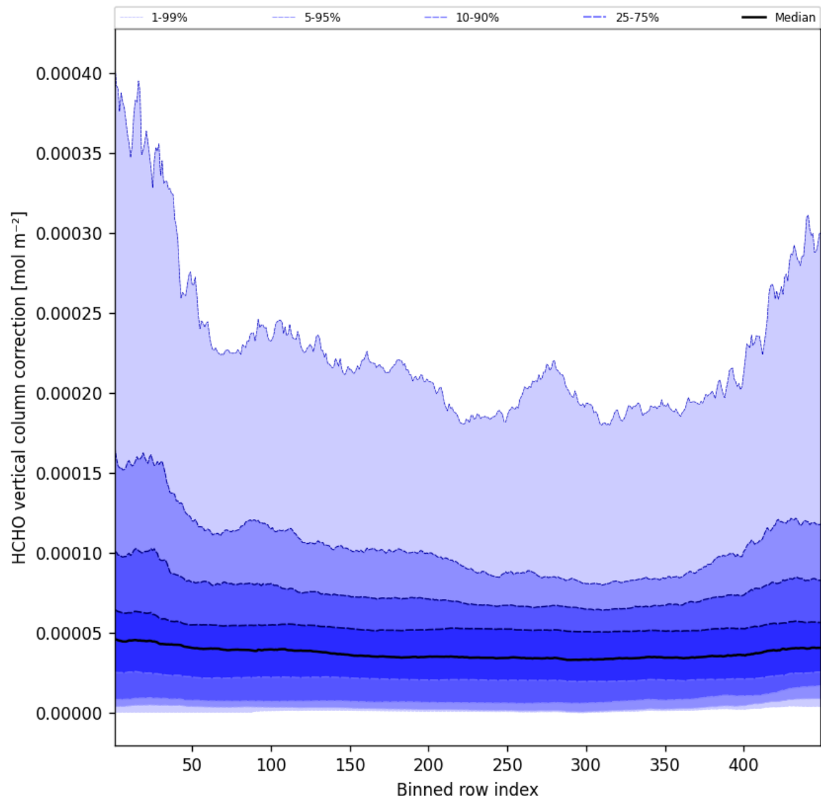
Figure 49: Along track statistics of “HCHO vertical column correction” for 2025-07-20 to 2025-07-21
