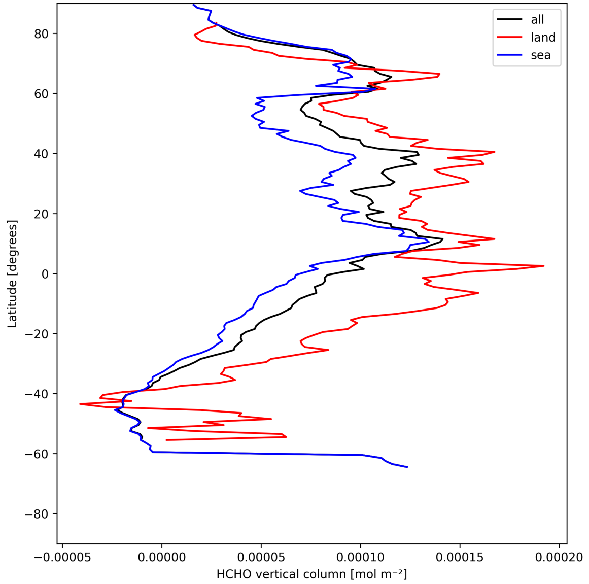
Figure 19: Zonal average of “HCHO vertical column” for 2025-07-21 to 2025-07-22.
