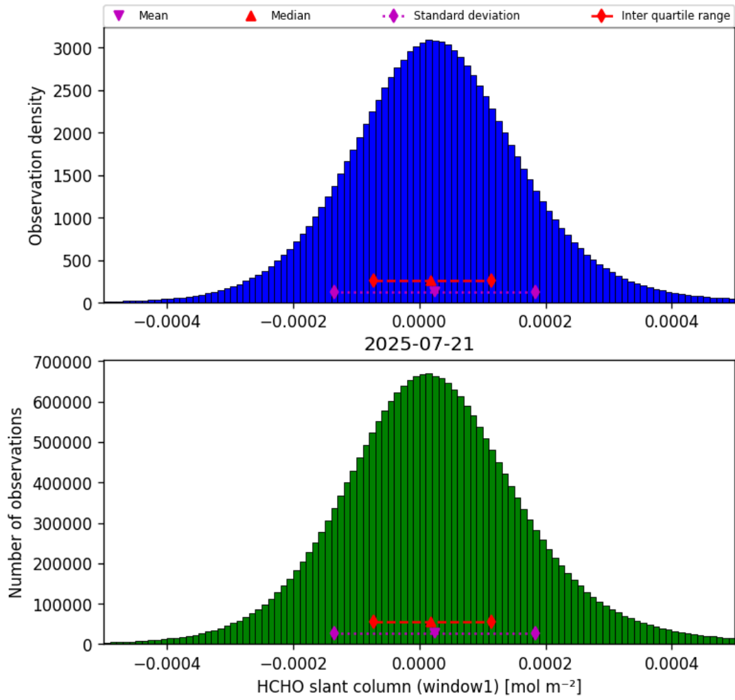
Figure 36: Histogram of “HCHO slant column (window1)” for 2025-07-21 to 2025-07-22
