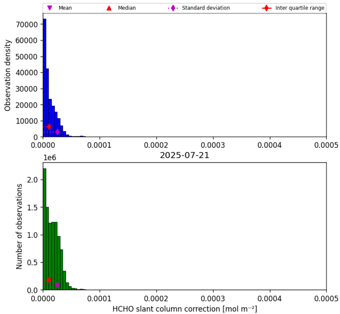
Figure 45: Histogram of “HCHO slant column correction” for 2025-07-21 to 2025-07-22
