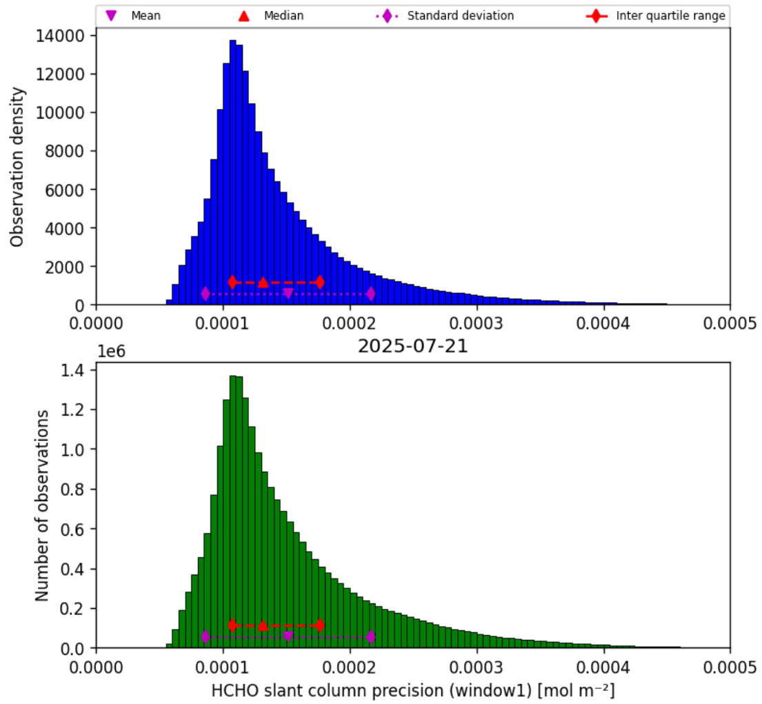
Figure 37: Histogram of “HCHO slant column precision (window1)” for 2025-07-21 to 2025-07-22
