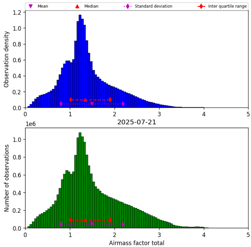
Figure 38: Histogram of “Airmass factor total” for 2025-07-21 to 2025-07-22
