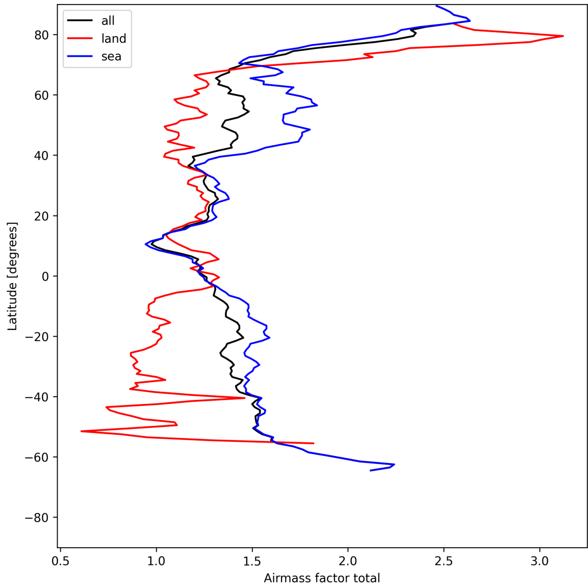
Figure 24: Zonal average of “Airmass factor total” for 2025-07-21 to 2025-07-22.
