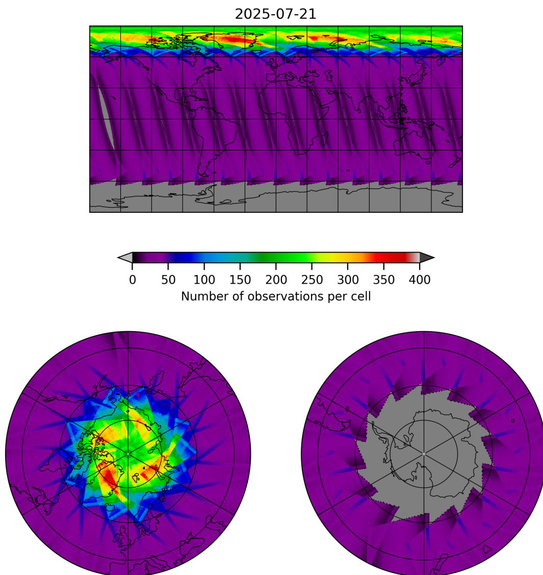
Figure 17: Map of the number of observations for 2025-07-21 to 2025-07-22
