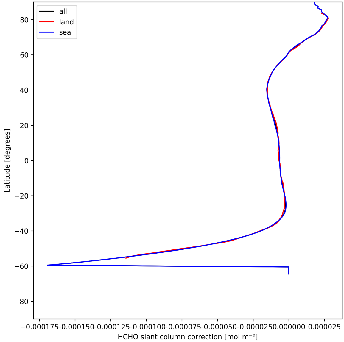
Figure 31: Zonal average of “HCHO slant column correction” for 2025-07-21 to 2025-07-22.
