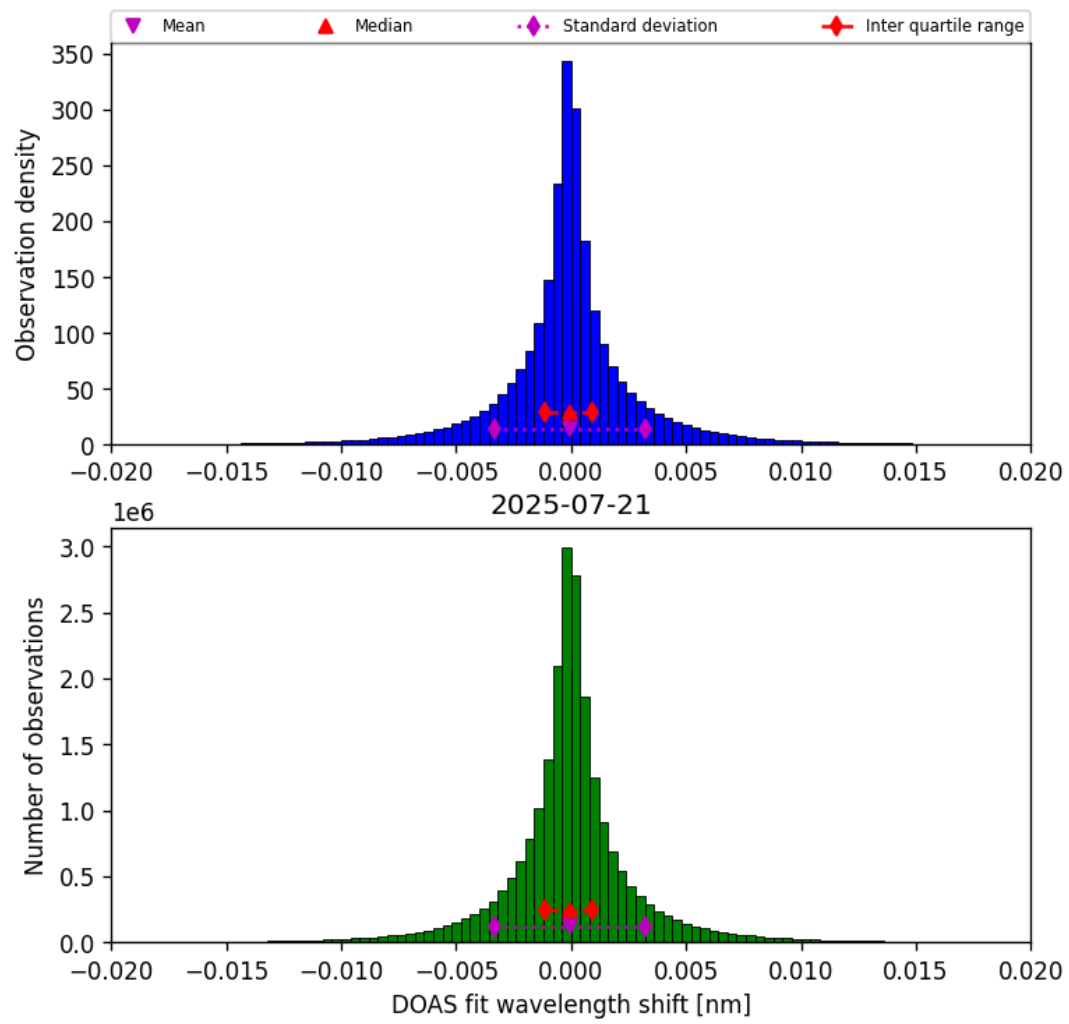
Figure 42: Histogram of “DOAS fit wavelength shift” for 2025-07-21 to 2025-07-22
