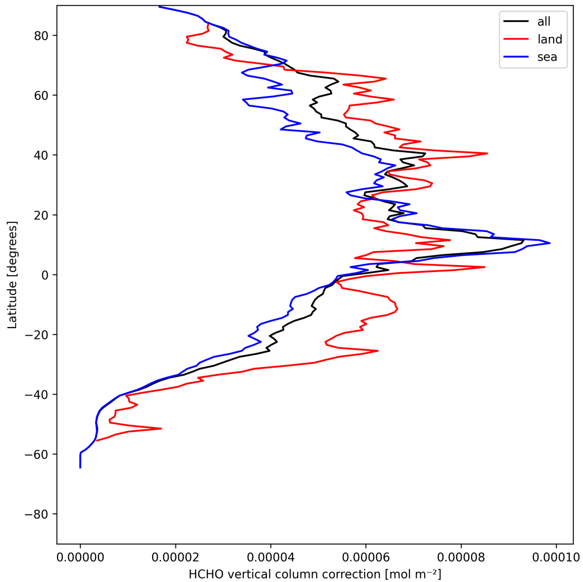
Figure 21: Zonal average of “HCHO vertical column correction” for 2025-07-21 to 2025-07-22.
