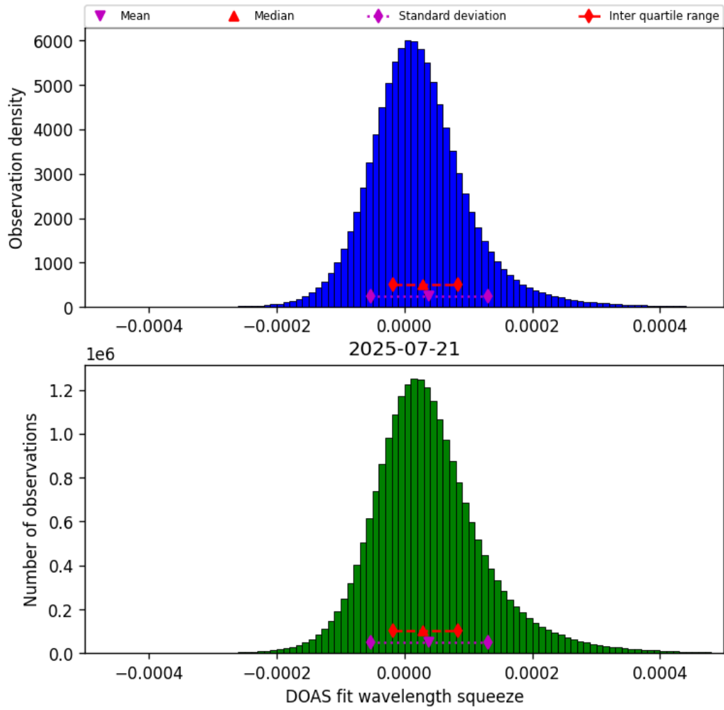
Figure 43: Histogram of “DOAS fit wavelength squeeze” for 2025-07-21 to 2025-07-22
