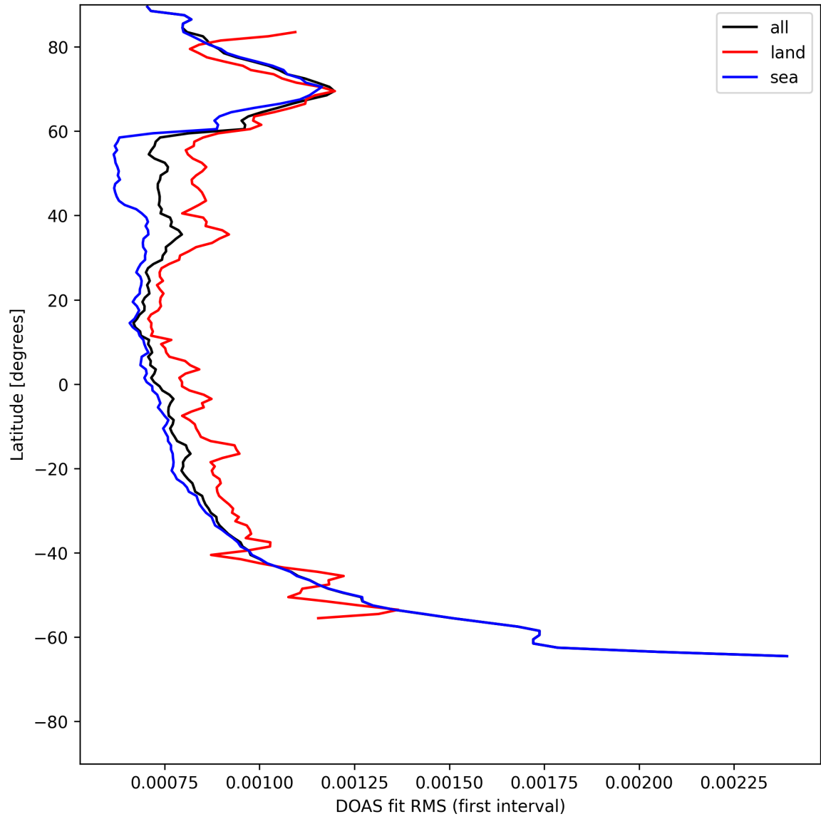
Figure 30: Zonal average of “DOAS fit RMS (first interval)” for 2025-07-21 to 2025-07-22.
