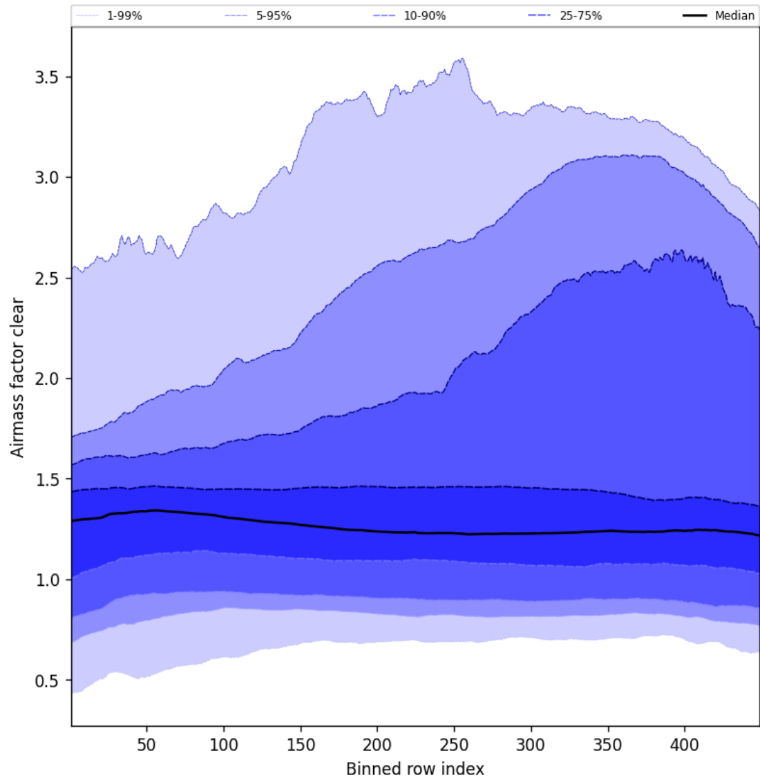
Figure 54: Along track statistics of “Airmass factor clear” for 2025-07-21 to 2025-07-22
