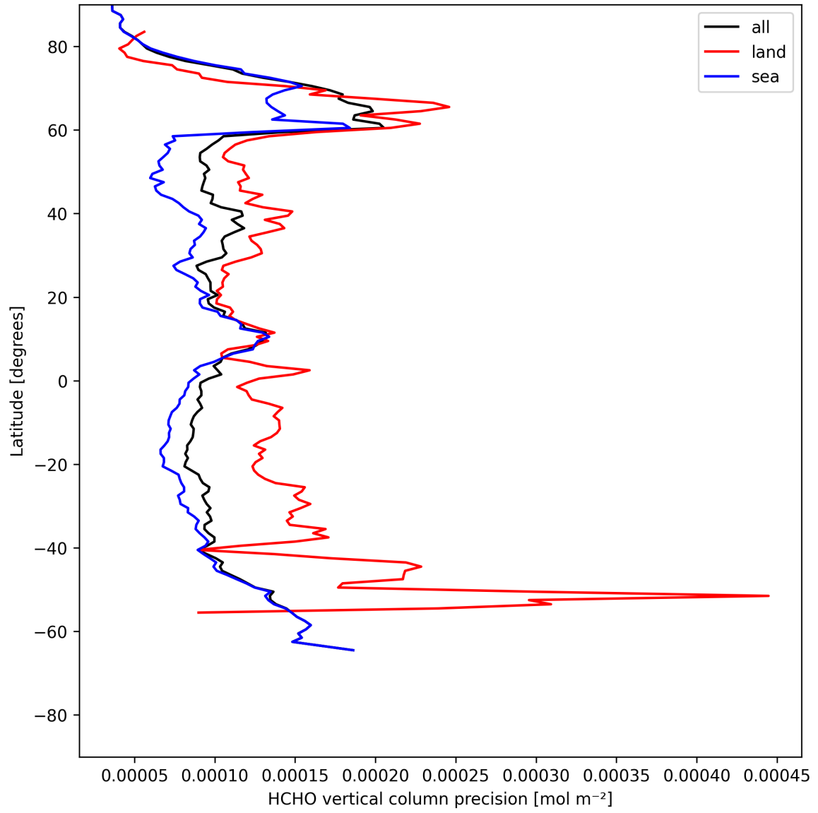
Figure 20: Zonal average of “HCHO vertical column precision” for 2025-07-21 to 2025-07-22.
