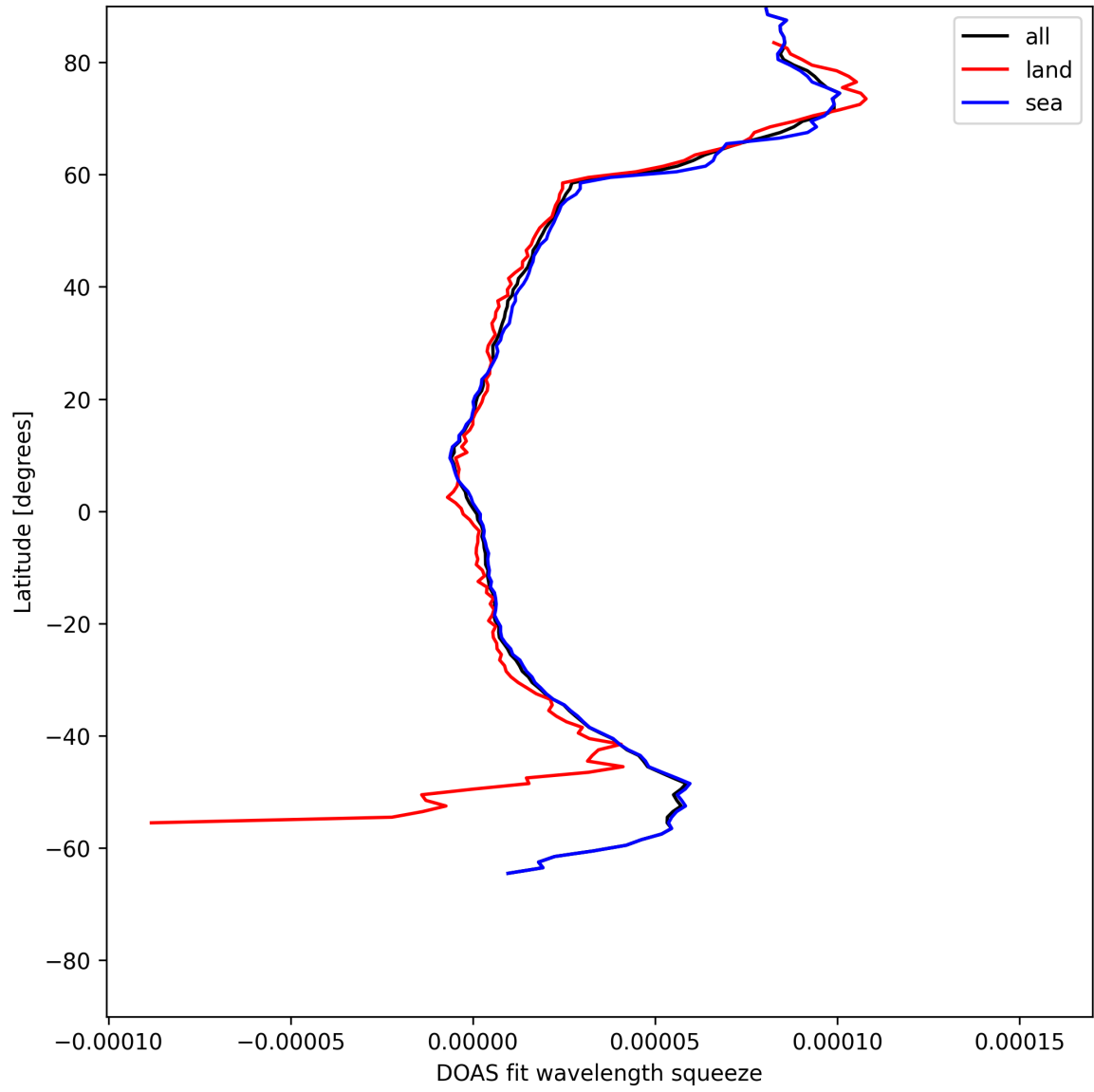
Figure 29: Zonal average of “DOAS fit wavelength squeeze” for 2025-07-21 to 2025-07-22.
