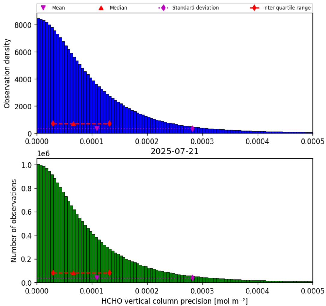
Figure 34: Histogram of “HCHO vertical column precision” for 2025-07-21 to 2025-07-22
