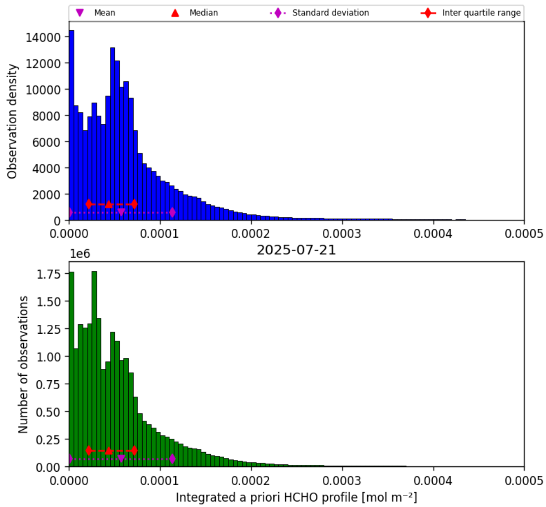
Figure 41: Histogram of “Integrated a priori HCHO profile” for 2025-07-21 to 2025-07-22
