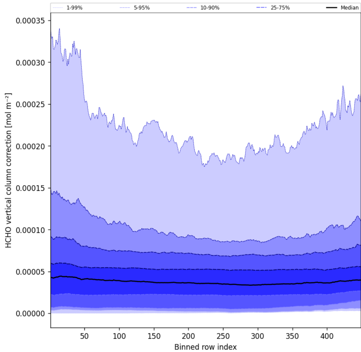
Figure 49: Along track statistics of “HCHO vertical column correction” for 2025-07-21 to 2025-07-22
