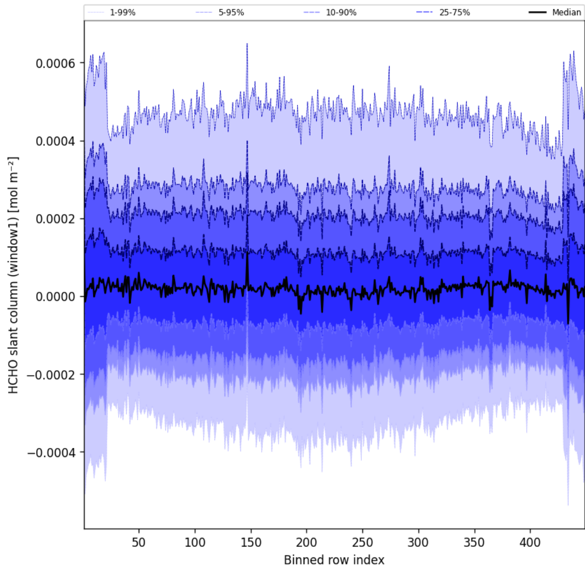
Figure 50: Along track statistics of “HCHO slant column (window1)” for 2025-07-21 to 2025-07-22
