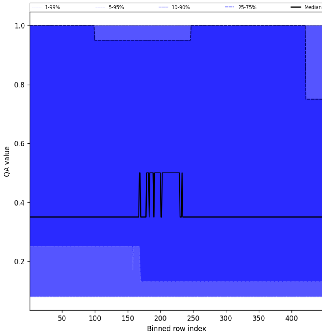
Figure 46: Along track statistics of “QA value” for 2025-07-21 to 2025-07-22
