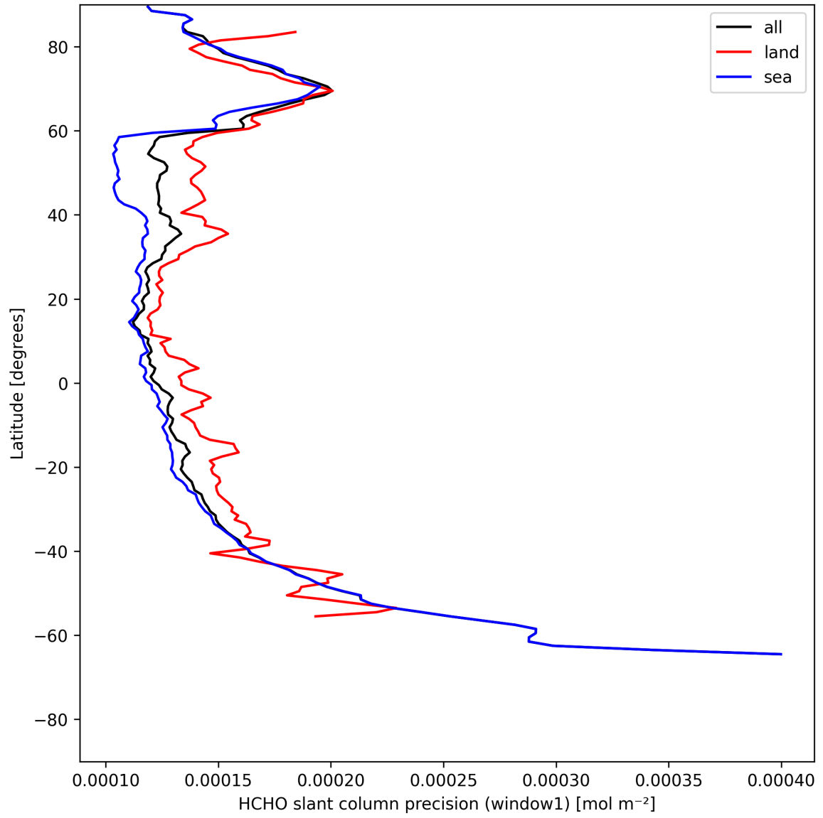
Figure 23: Zonal average of "HCHO slant column precision (window1)" for 2025-07-21 to 2025-07-22.
