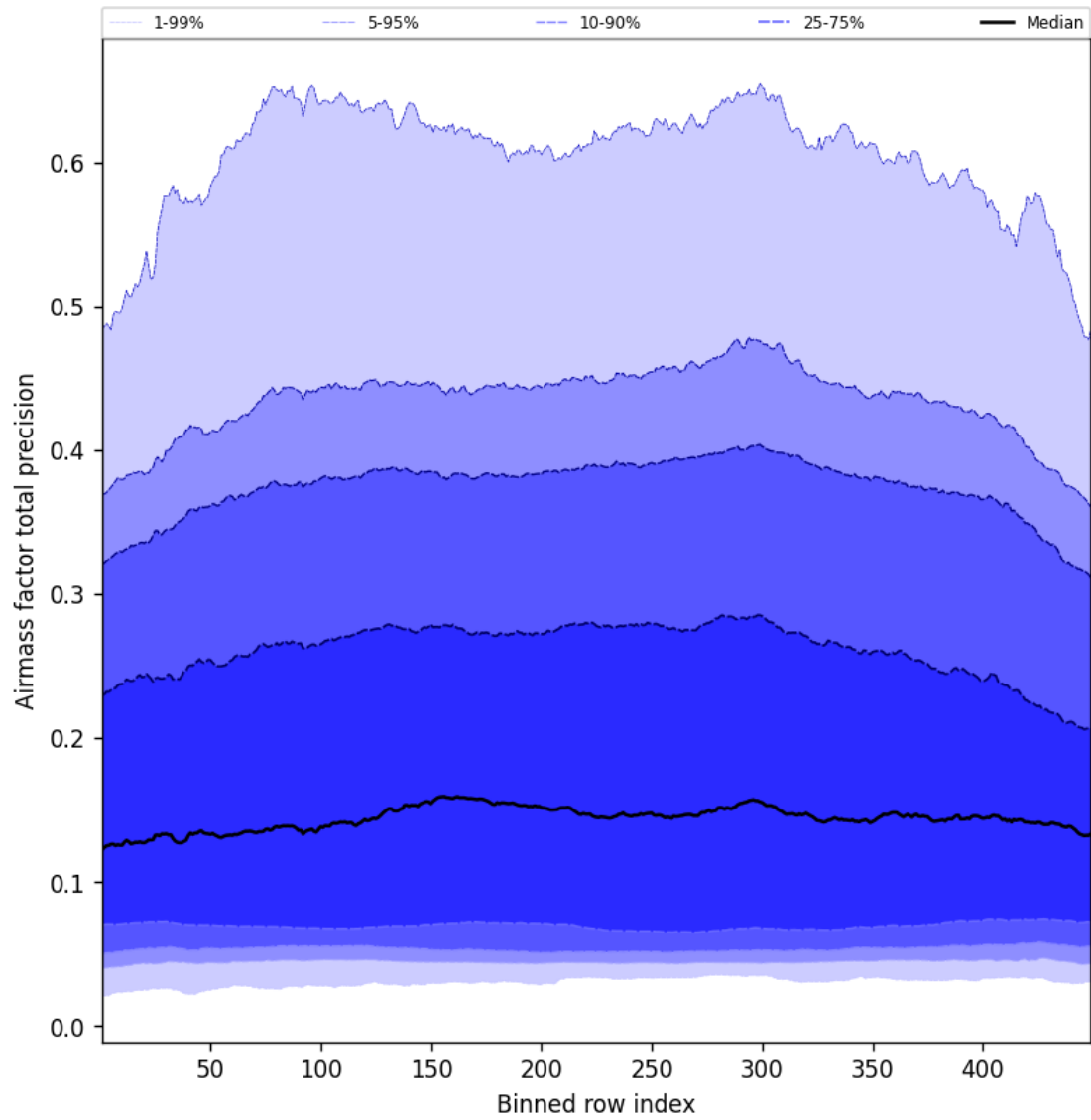
Figure 53: Along track statistics of “Airmass factor total precision” for 2025-07-21 to 2025-07-22
