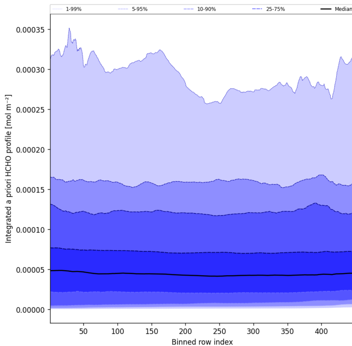
Figure 55: Along track statistics of “Integrated a priori HCHO profile” for 2025-07-21 to 2025-07-22
