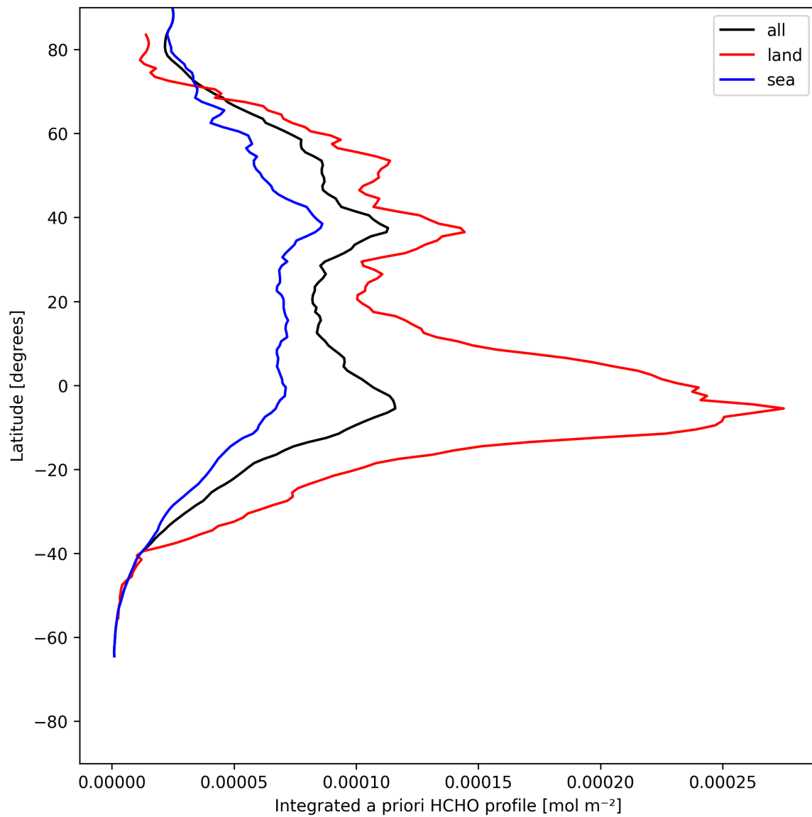
Figure 27: Zonal average of “Integrated a priori HCHO profile” for 2025-07-21 to 2025-07-22.
