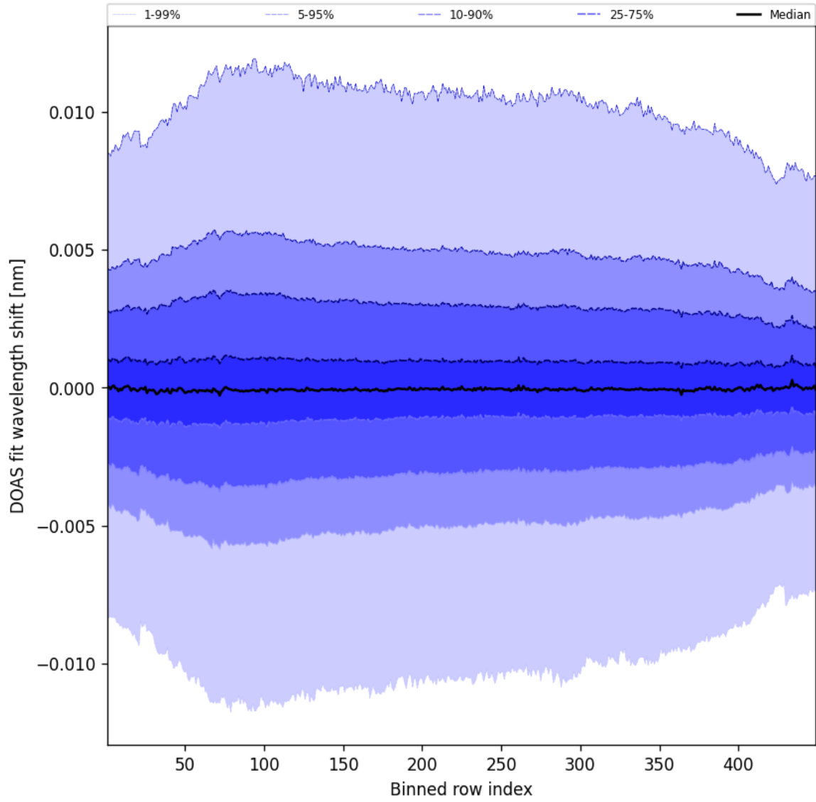
Figure 56: Along track statistics of “DOAS fit wavelength shift” for 2025-07-21 to 2025-07-22
