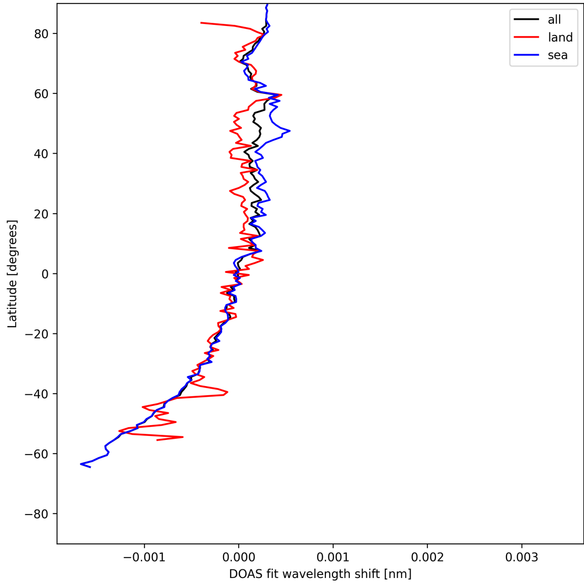
Figure 28: Zonal average of "DOAS fit wavelength shift" for 2025-07-21 to 2025-07-22.
