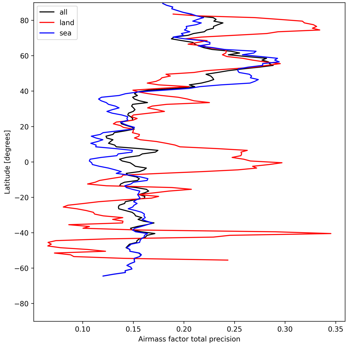
Figure 25: Zonal average of “Airmass factor total precision” for 2025-07-21 to 2025-07-22.
