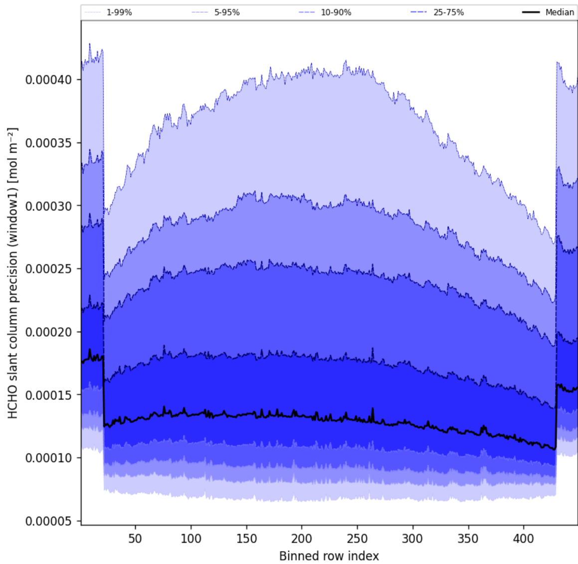
Figure 51: Along track statistics of “HCHO slant column precision (window1)” for 2025-07-21 to 2025-07-22
