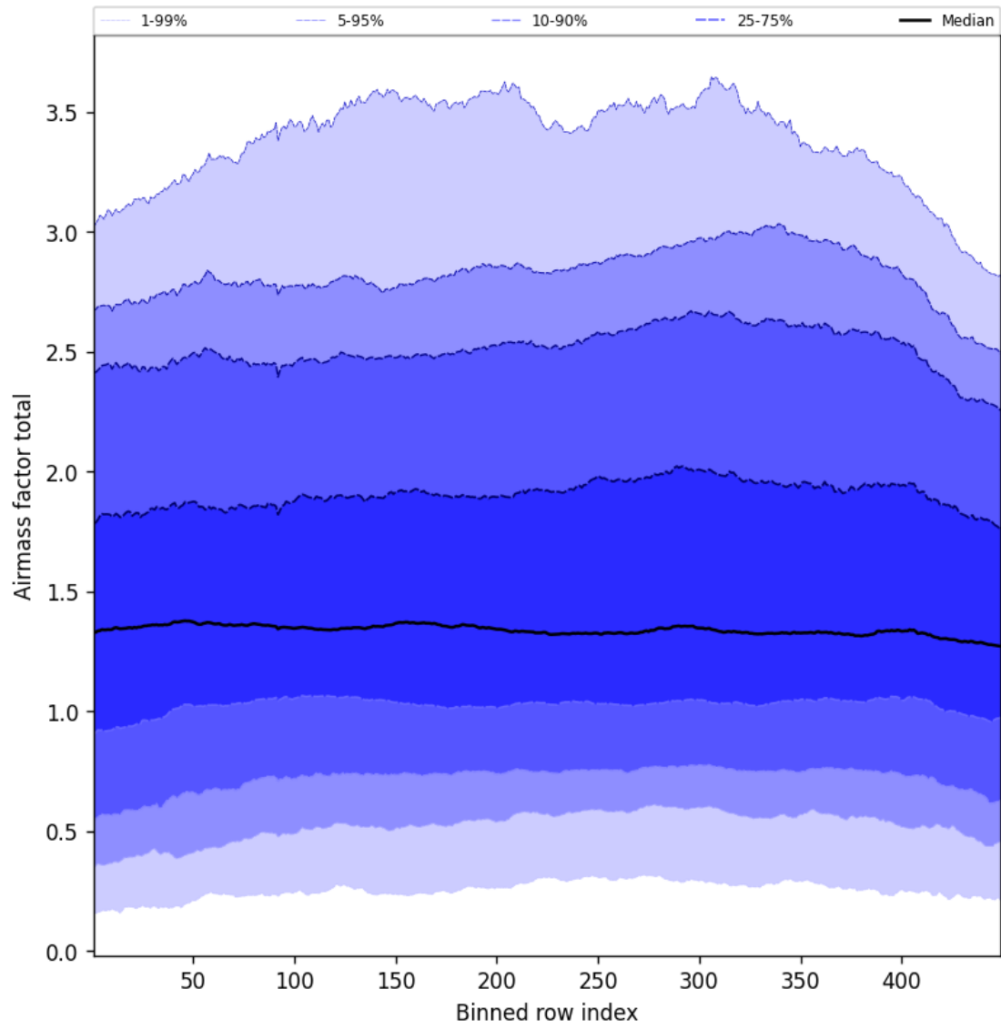
Figure 52: Along track statistics of “Airmass factor total” for 2025-07-21 to 2025-07-22
