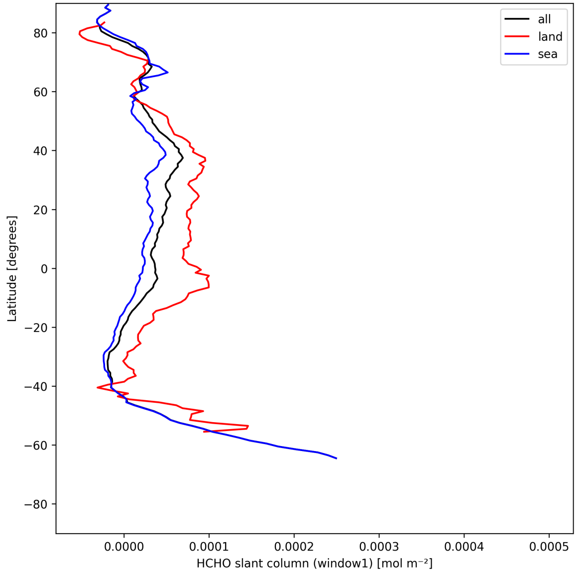
Figure 22: Zonal average of “HCHO slant column (window1)” for 2025-07-21 to 2025-07-22.
