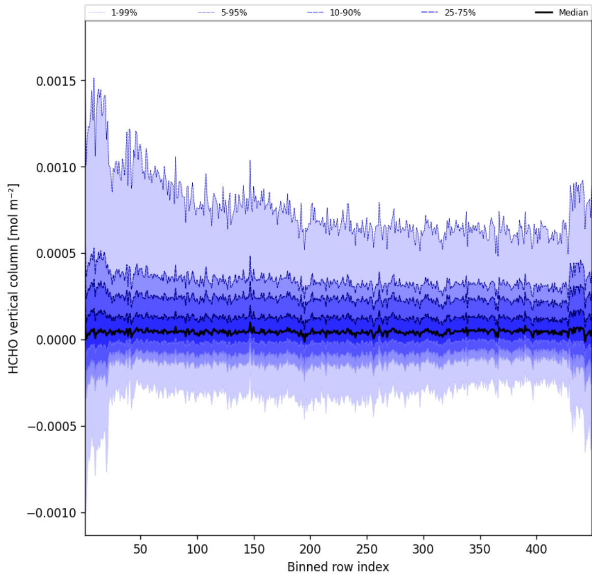
Figure 47: Along track statistics of “HCHO vertical column” for 2025-07-21 to 2025-07-22
