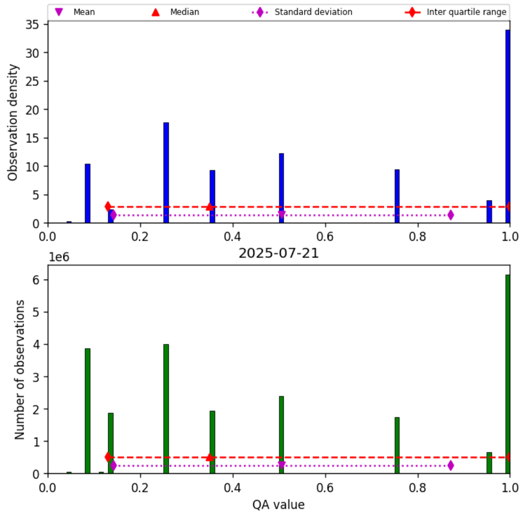
Figure 32: Histogram of “QA value” for 2025-07-21 to 2025-07-22
