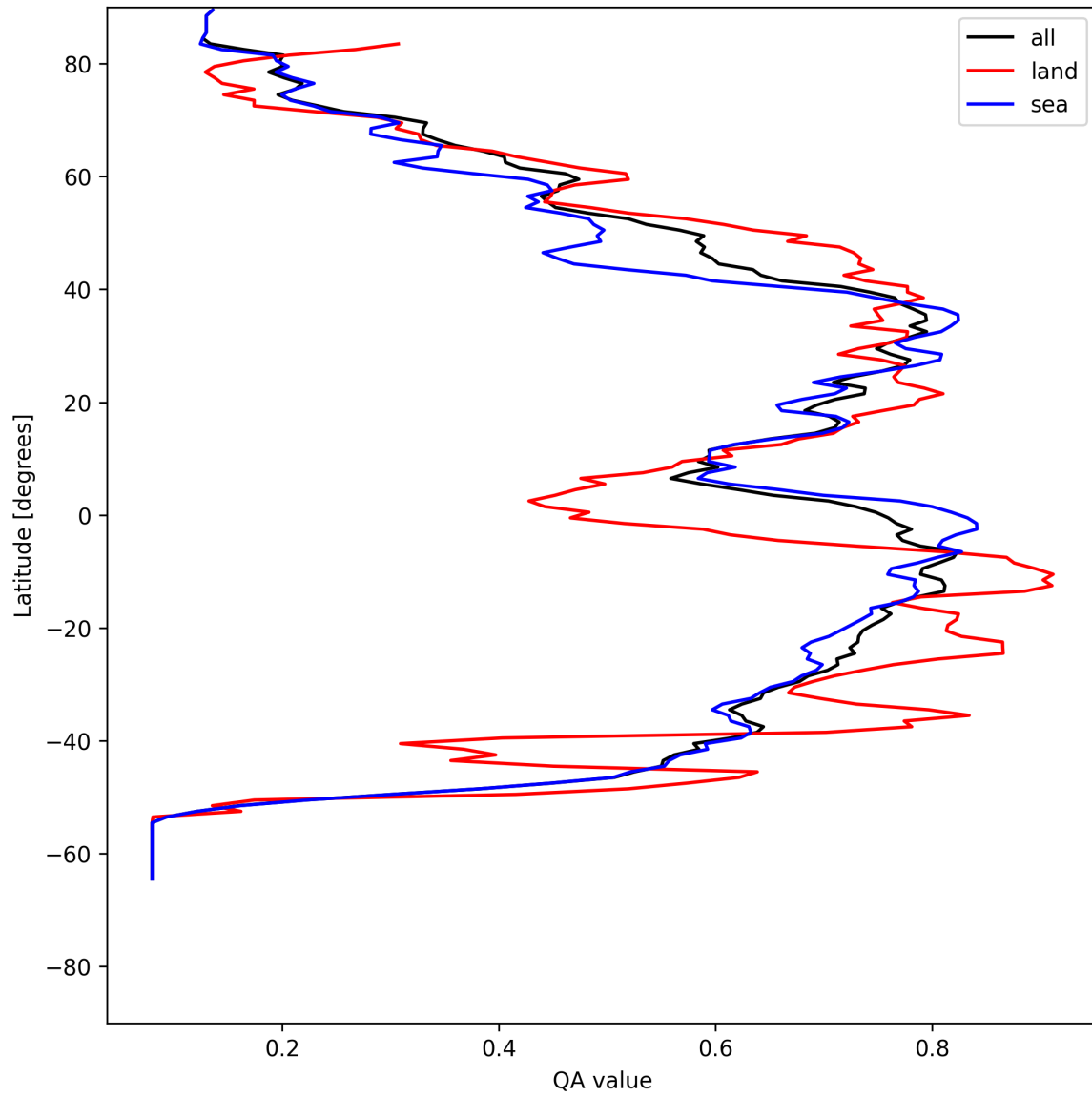
Figure 18: Zonal average of “QA value” for 2025-07-21 to 2025-07-22.
