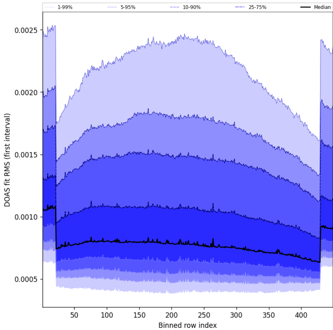
Figure 58: Along track statistics of “DOAS fit RMS (first interval)” for 2025-07-21 to 2025-07-22
