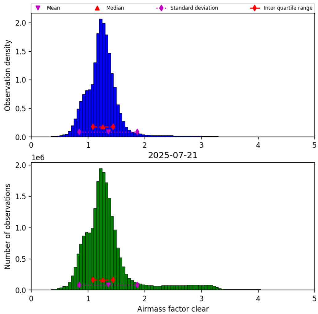
Figure 40: Histogram of “Airmass factor clear” for 2025-07-21 to 2025-07-22
