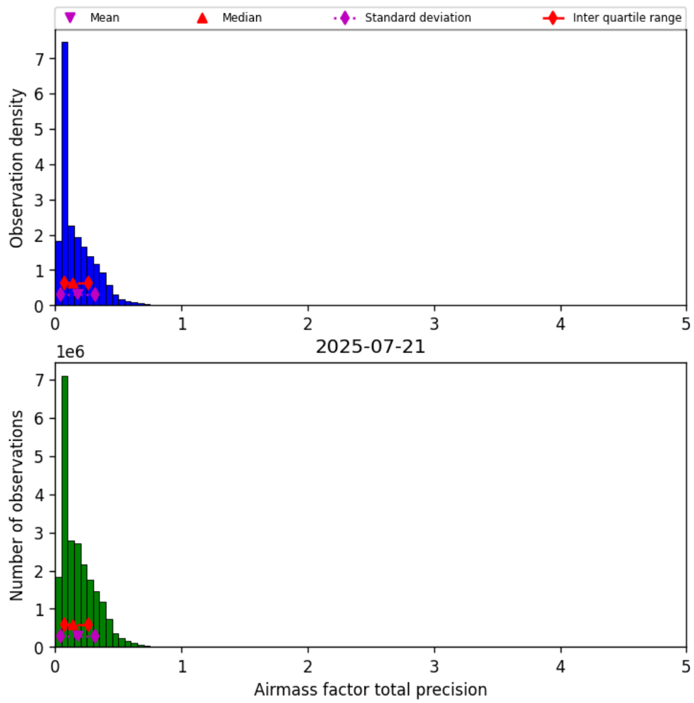
Figure 39: Histogram of “Airmass factor total precision” for 2025-07-21 to 2025-07-22
