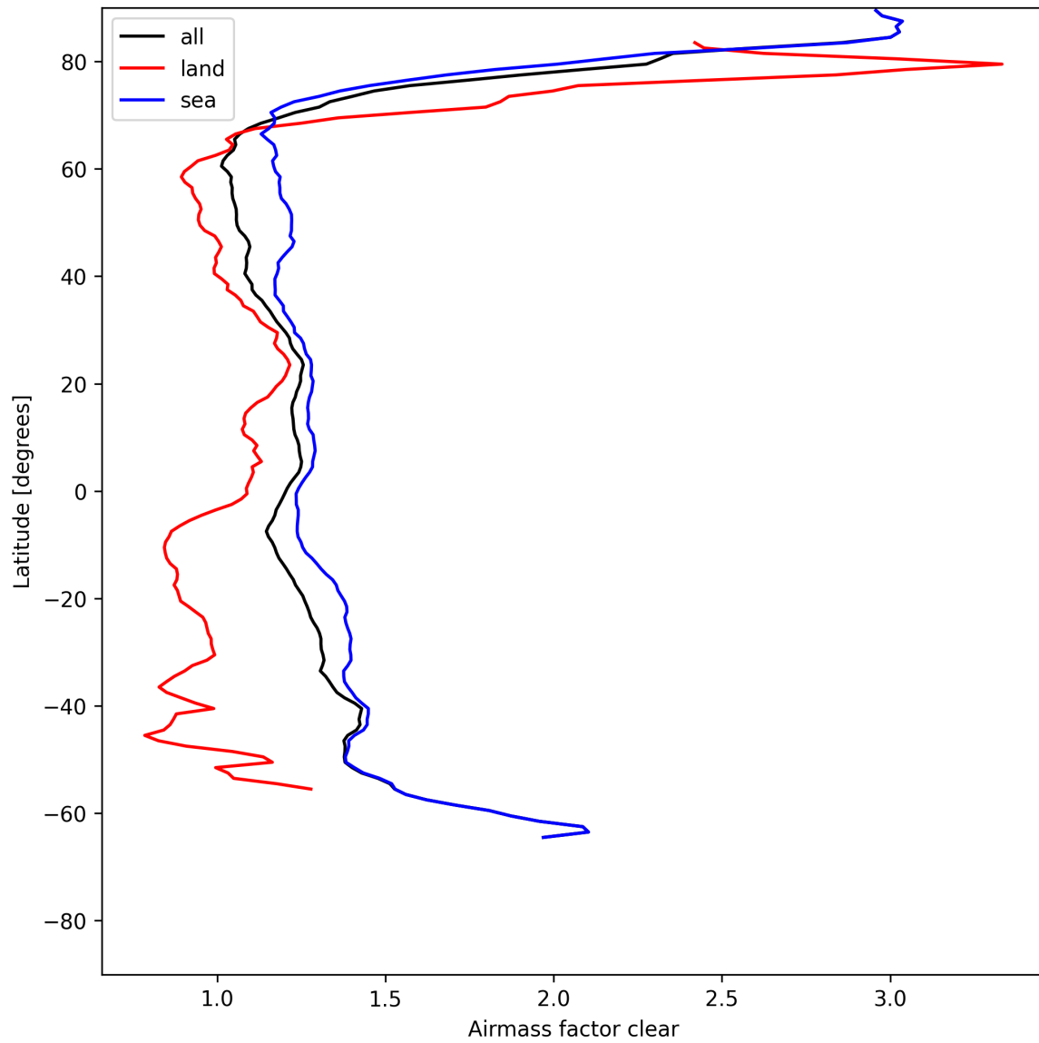
Figure 26: Zonal average of “Airmass factor clear” for 2025-07-21 to 2025-07-22.
