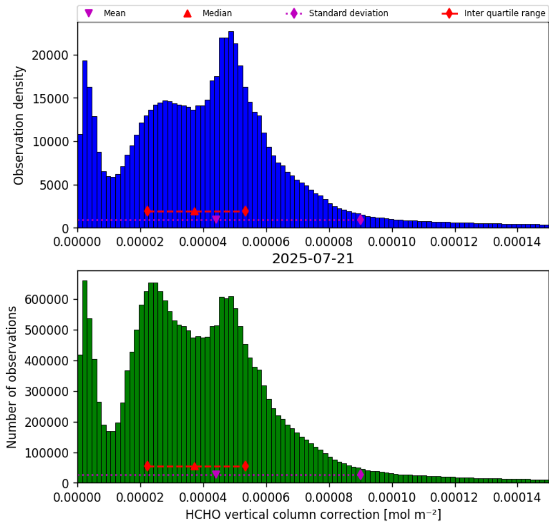
Figure 35: Histogram of “HCHO vertical column correction” for 2025-07-21 to 2025-07-22
