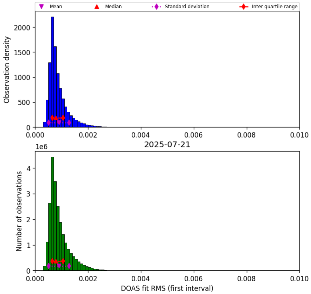
Figure 44: Histogram of "DOAS fit RMS (first interval)" for 2025-07-21 to 2025-07-22
