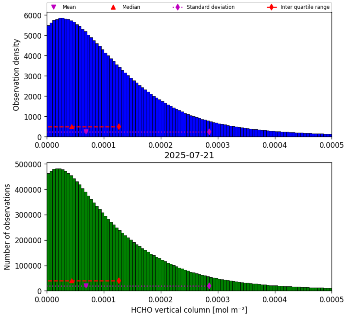
Figure 33: Histogram of “HCHO vertical column” for 2025-07-21 to 2025-07-22
