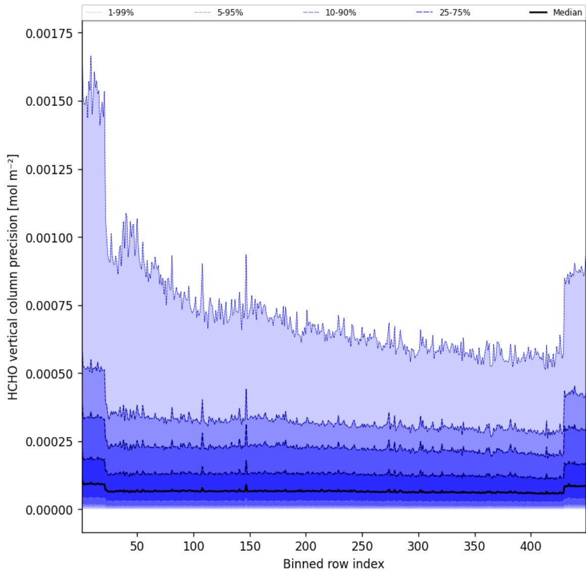
Figure 48: Along track statistics of “HCHO vertical column precision” for 2025-07-21 to 2025-07-22
