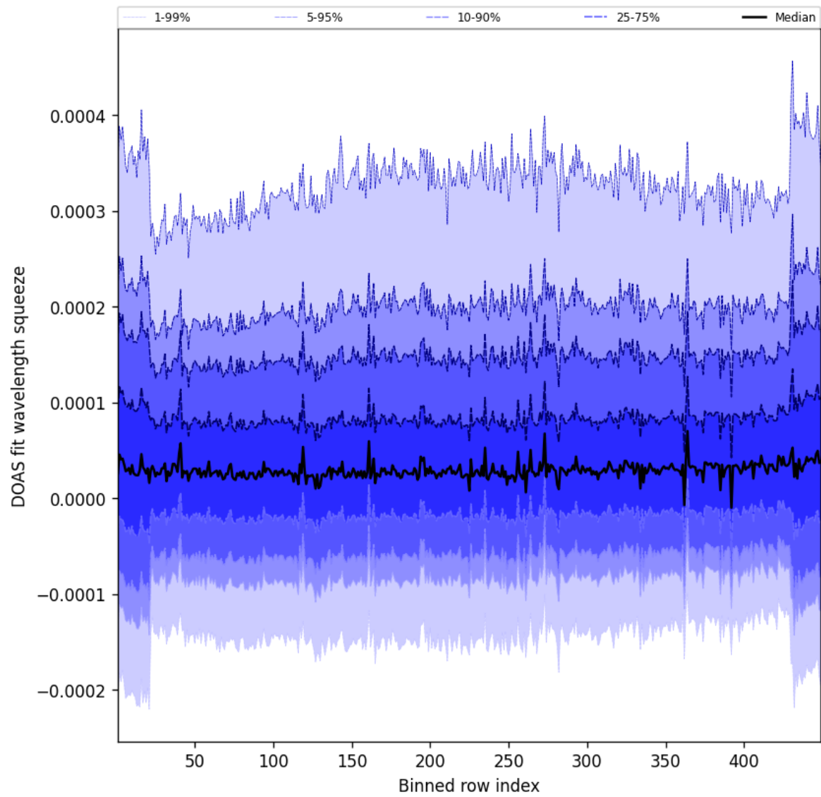
Figure 57: Along track statistics of “DOAS fit wavelength squeeze” for 2025-07-21 to 2025-07-22
