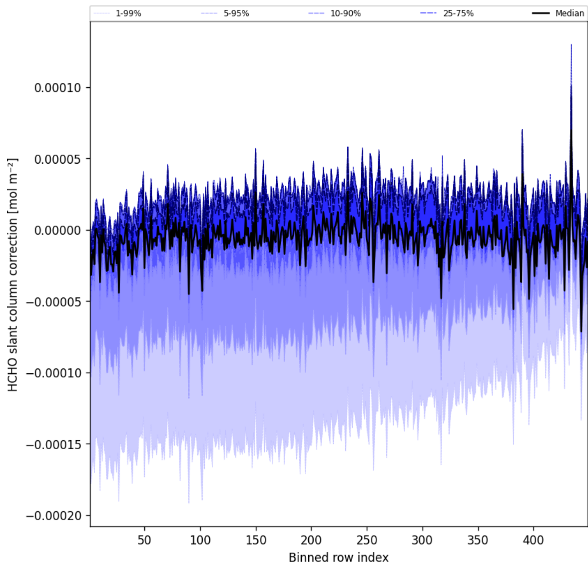
Figure 59: Along track statistics of “HCHO slant column correction” for 2025-07-21 to 2025-07-22
