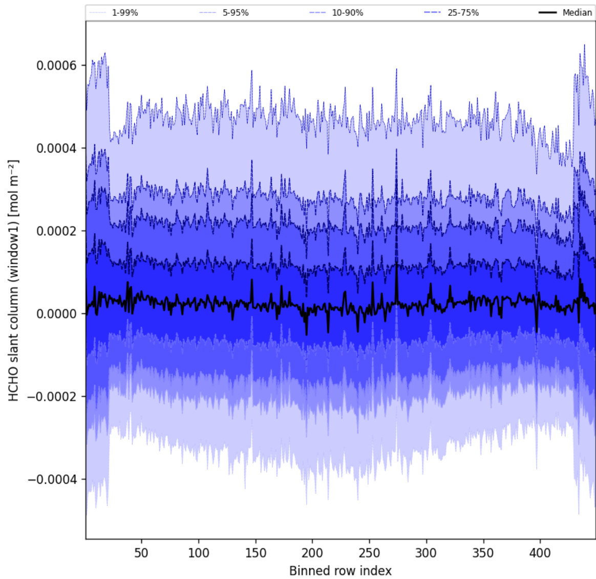
Figure 50: Along track statistics of “HCHO slant column (window1)” for 2025-07-22 to 2025-07-22
