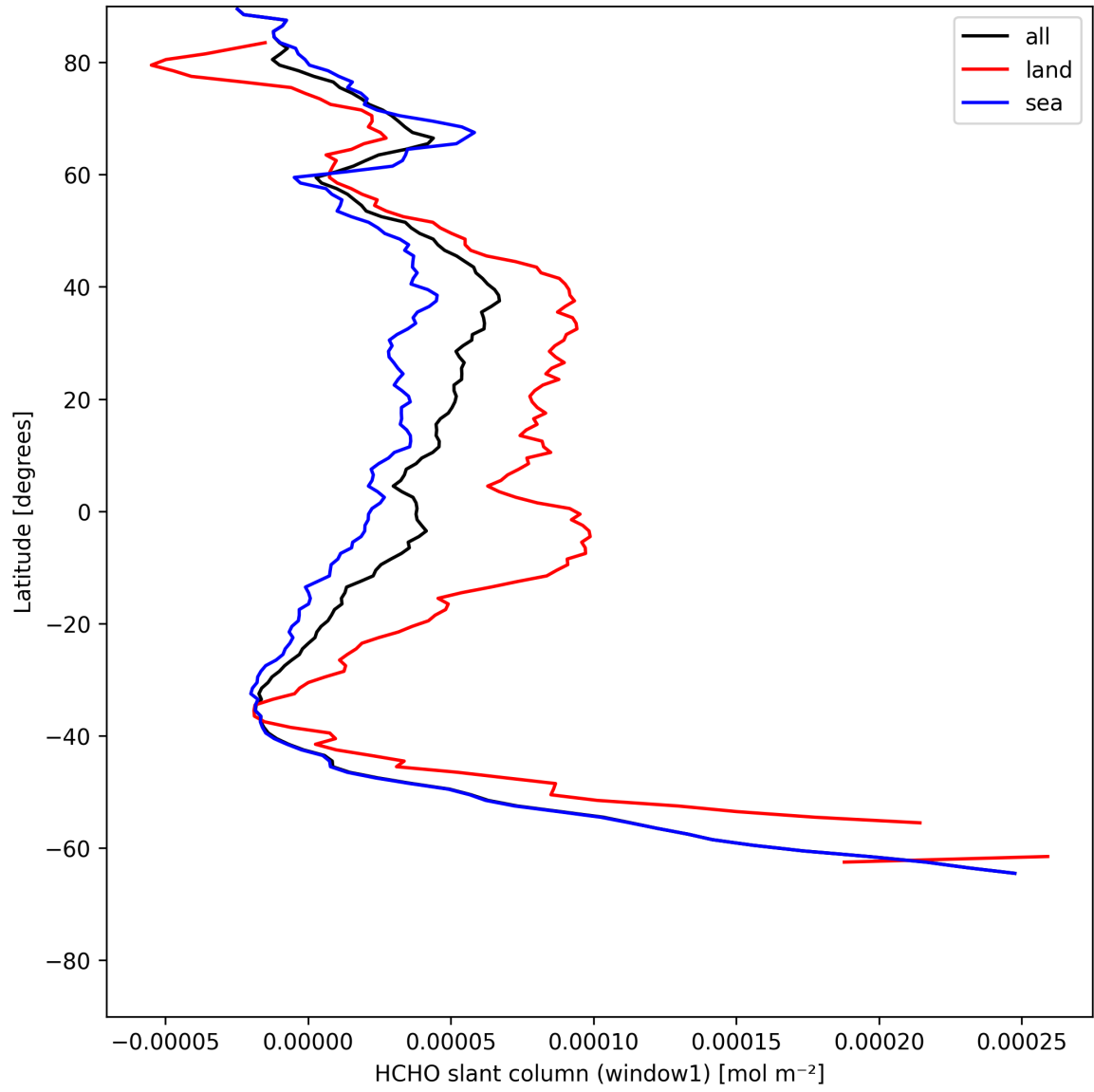
Figure 22: Zonal average of “HCHO slant column (window1)” for 2025-07-22 to 2025-07-22.
