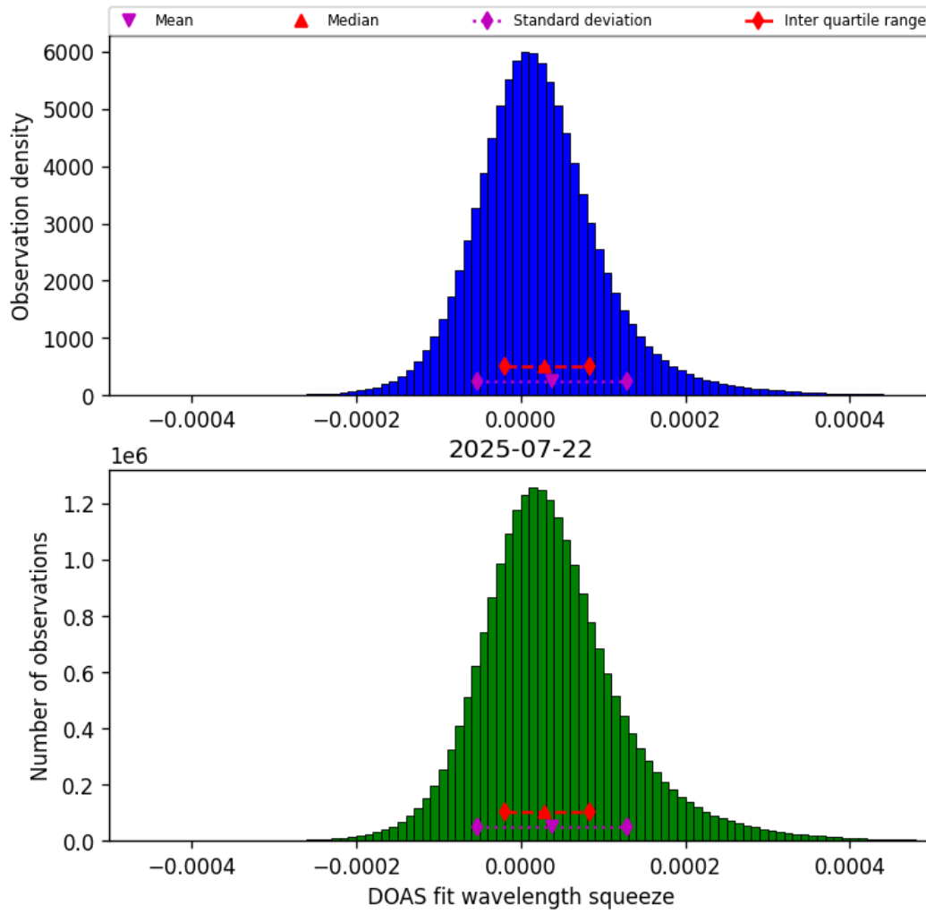
Figure 43: Histogram of “DOAS fit wavelength squeeze” for 2025-07-22 to 2025-07-22
