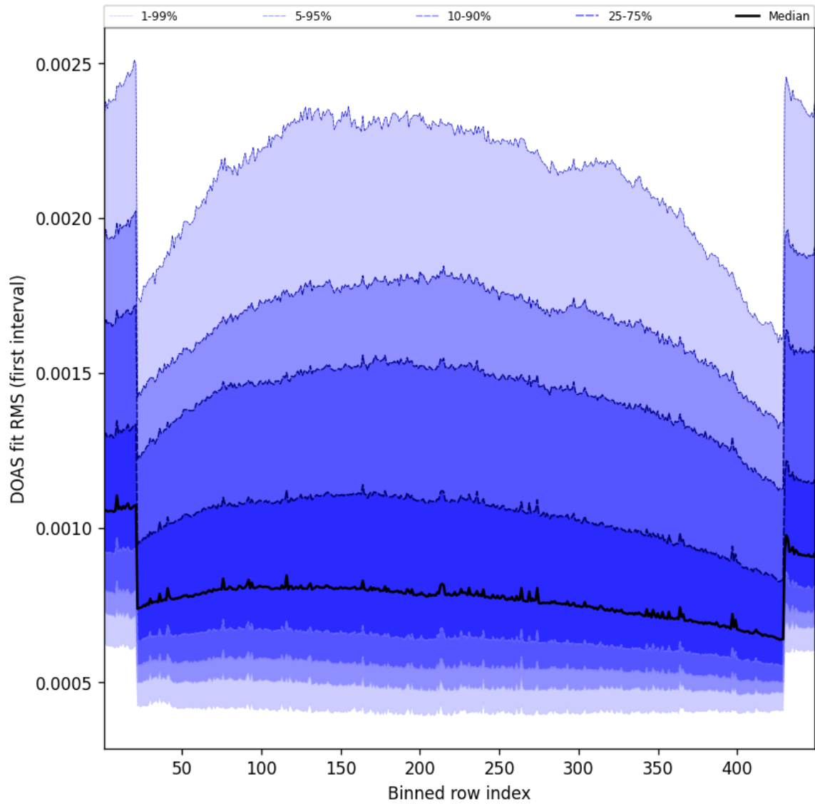
Figure 58: Along track statistics of “DOAS fit RMS (first interval)” for 2025-07-22 to 2025-07-22
