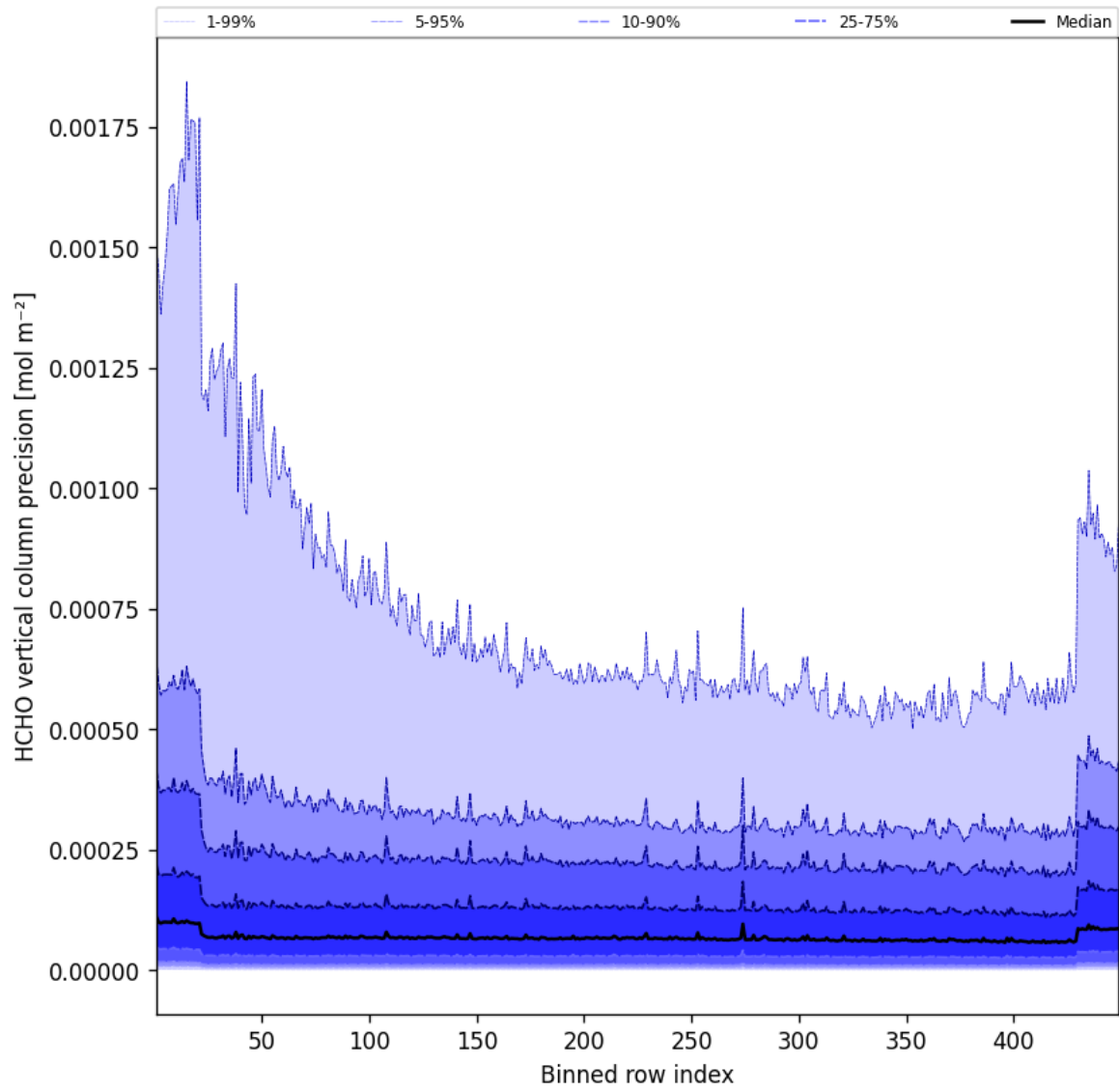
Figure 48: Along track statistics of “HCHO vertical column precision” for 2025-07-22 to 2025-07-22
