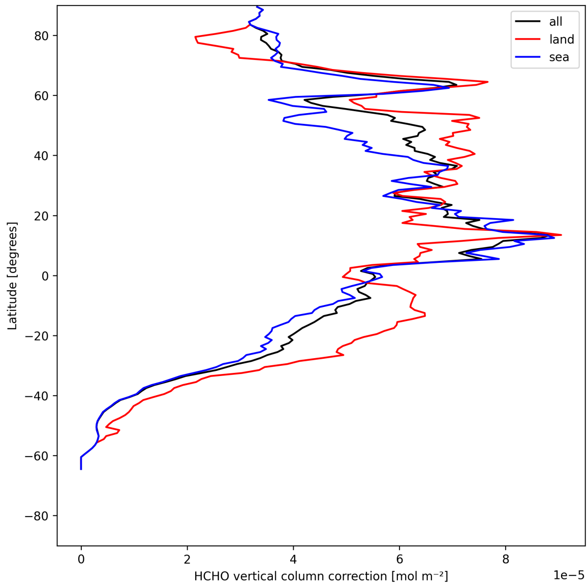
Figure 21: Zonal average of “HCHO vertical column correction” for 2025-07-22 to 2025-07-22.
