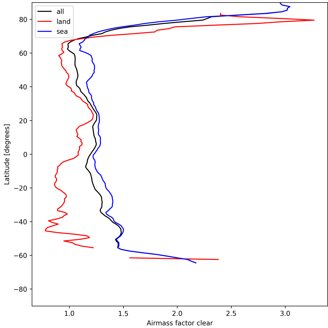
Figure 26: Zonal average of “Airmass factor clear” for 2025-07-22 to 2025-07-22.
