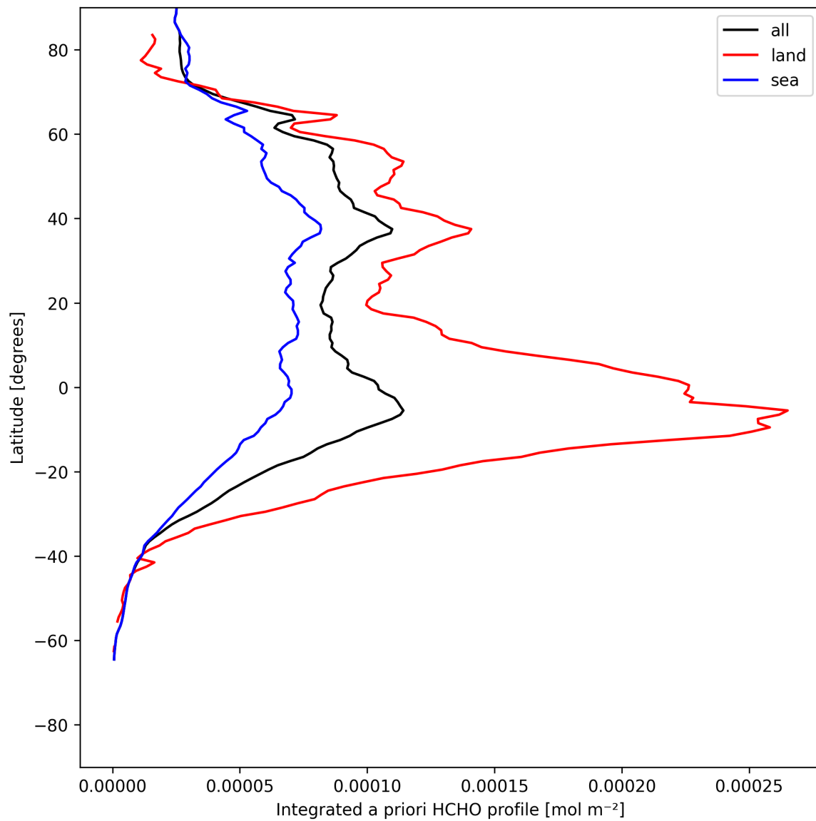
Figure 27: Zonal average of “Integrated a priori HCHO profile” for 2025-07-22 to 2025-07-22.
