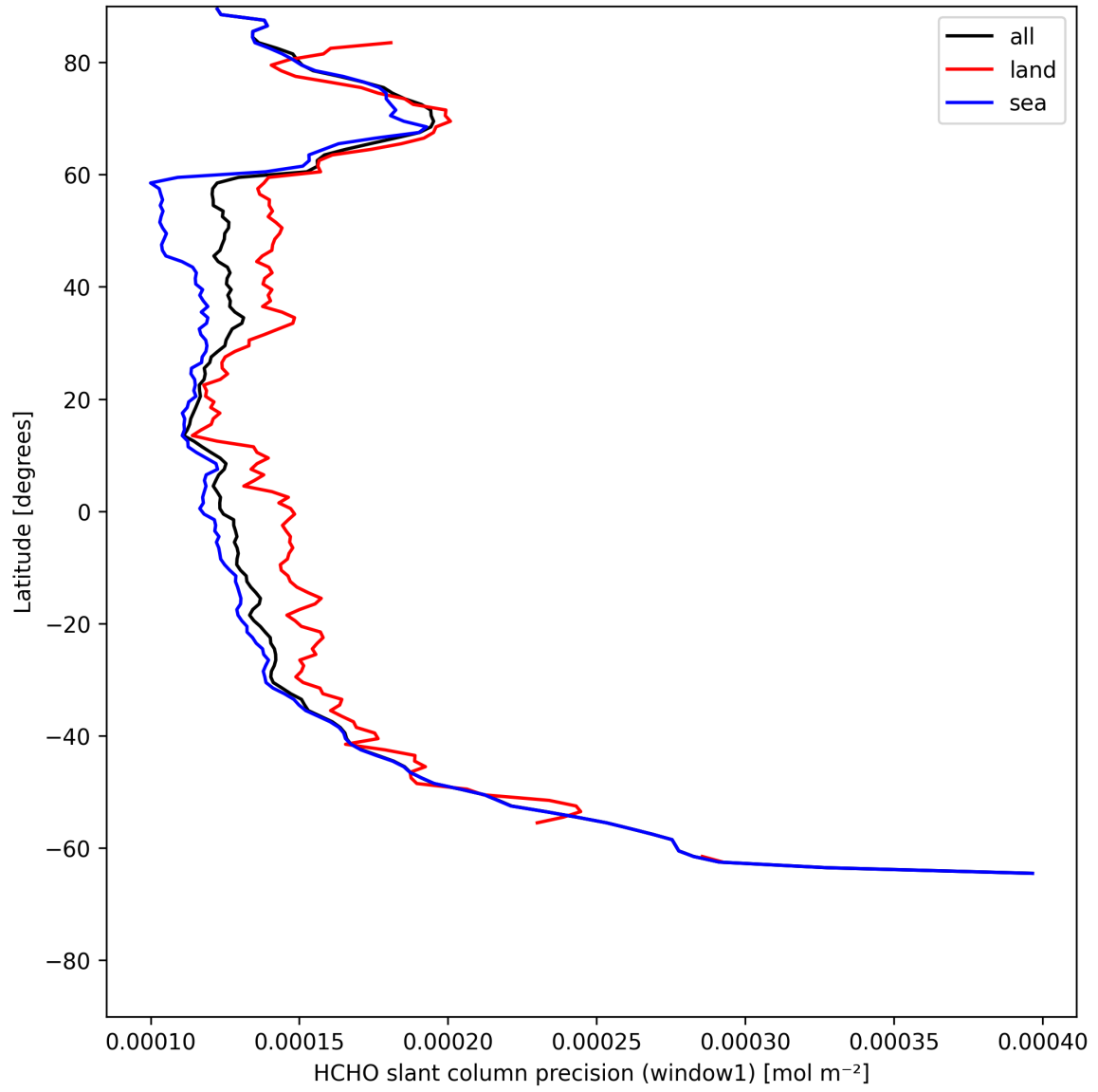
Figure 23: Zonal average of "HCHO slant column precision (window1)" for 2025-07-22 to 2025-07-22.
