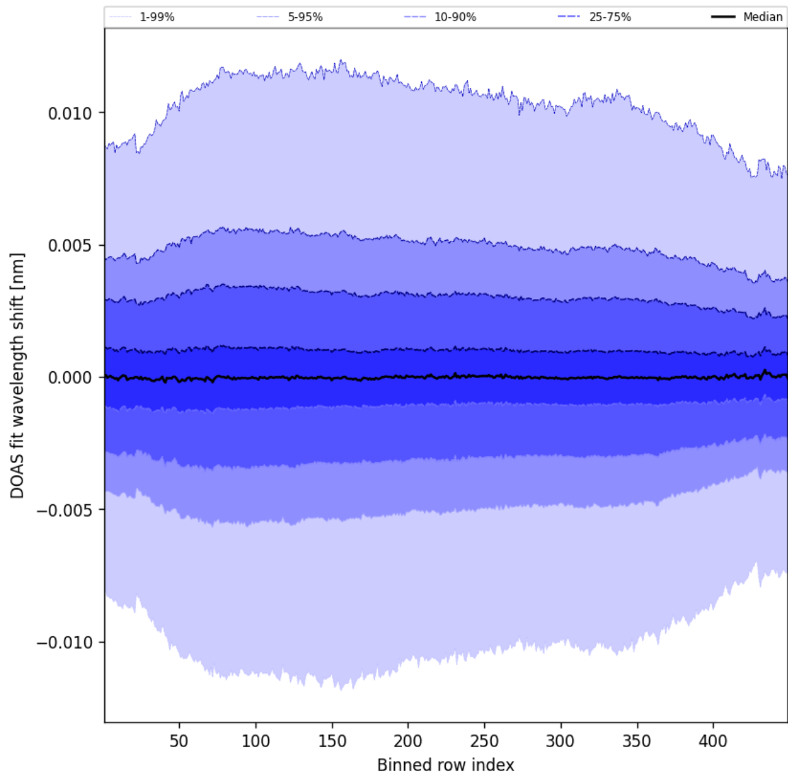
Figure 56: Along track statistics of “DOAS fit wavelength shift” for 2025-07-22 to 2025-07-22
