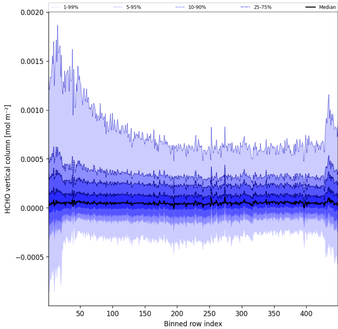
Figure 47: Along track statistics of “HCHO vertical column” for 2025-07-22 to 2025-07-22
