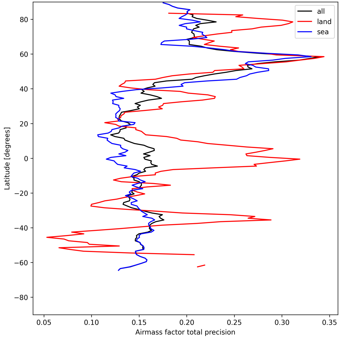
Figure 25: Zonal average of “Airmass factor total precision” for 2025-07-22 to 2025-07-22.
