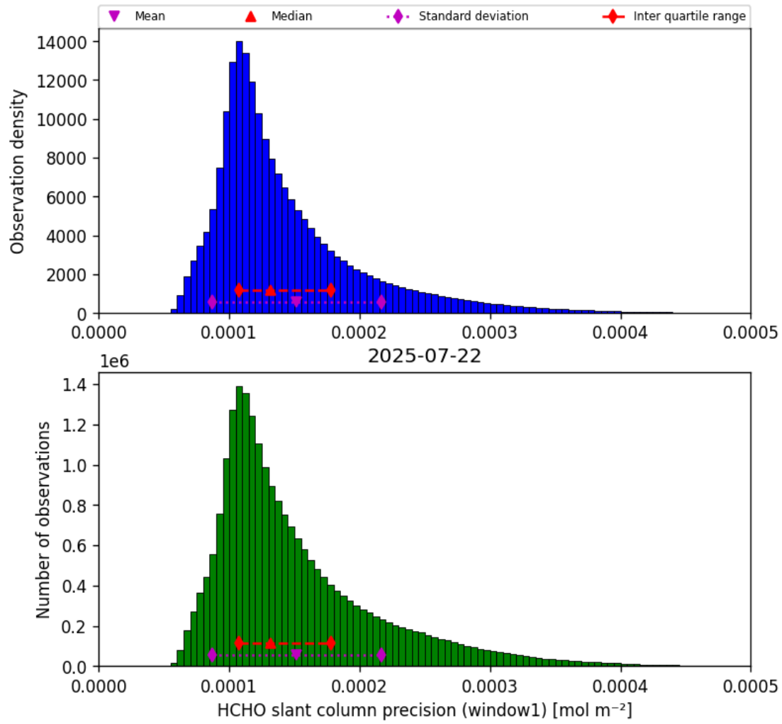
Figure 37: Histogram of “HCHO slant column precision (window1)” for 2025-07-22 to 2025-07-22
