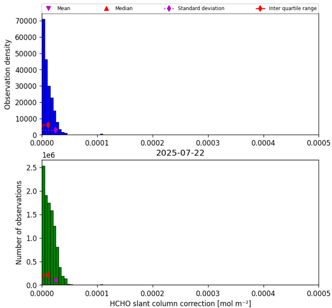
Figure 45: Histogram of “HCHO slant column correction” for 2025-07-22 to 2025-07-22
