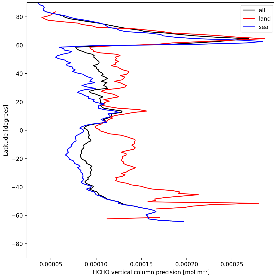
Figure 20: Zonal average of “HCHO vertical column precision” for 2025-07-22 to 2025-07-22.
