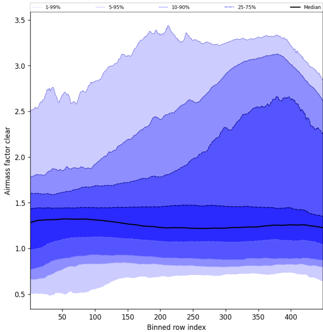
Figure 54: Along track statistics of “Airmass factor clear” for 2025-07-22 to 2025-07-22
