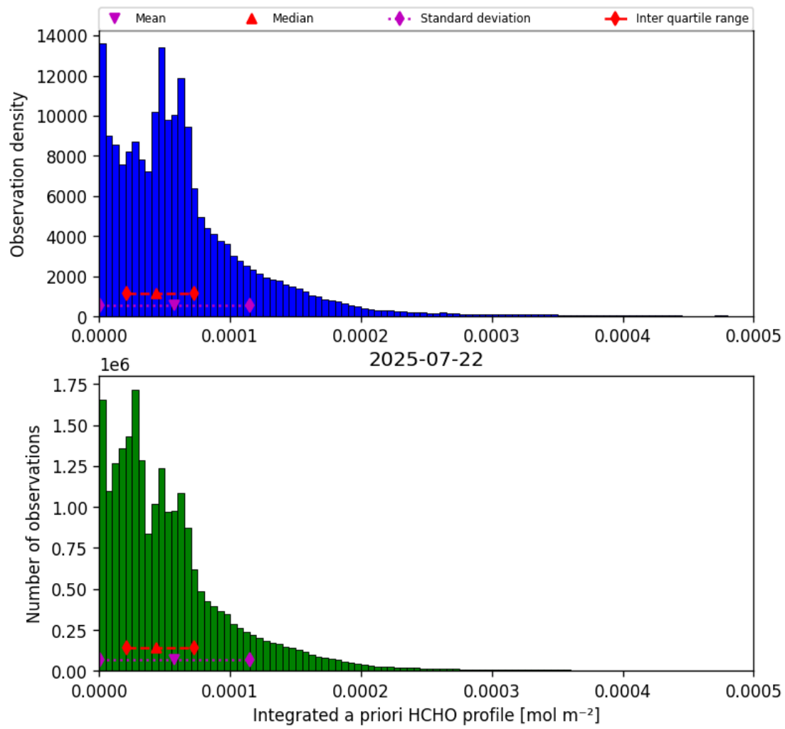
Figure 41: Histogram of “Integrated a priori HCHO profile” for 2025-07-22 to 2025-07-22
