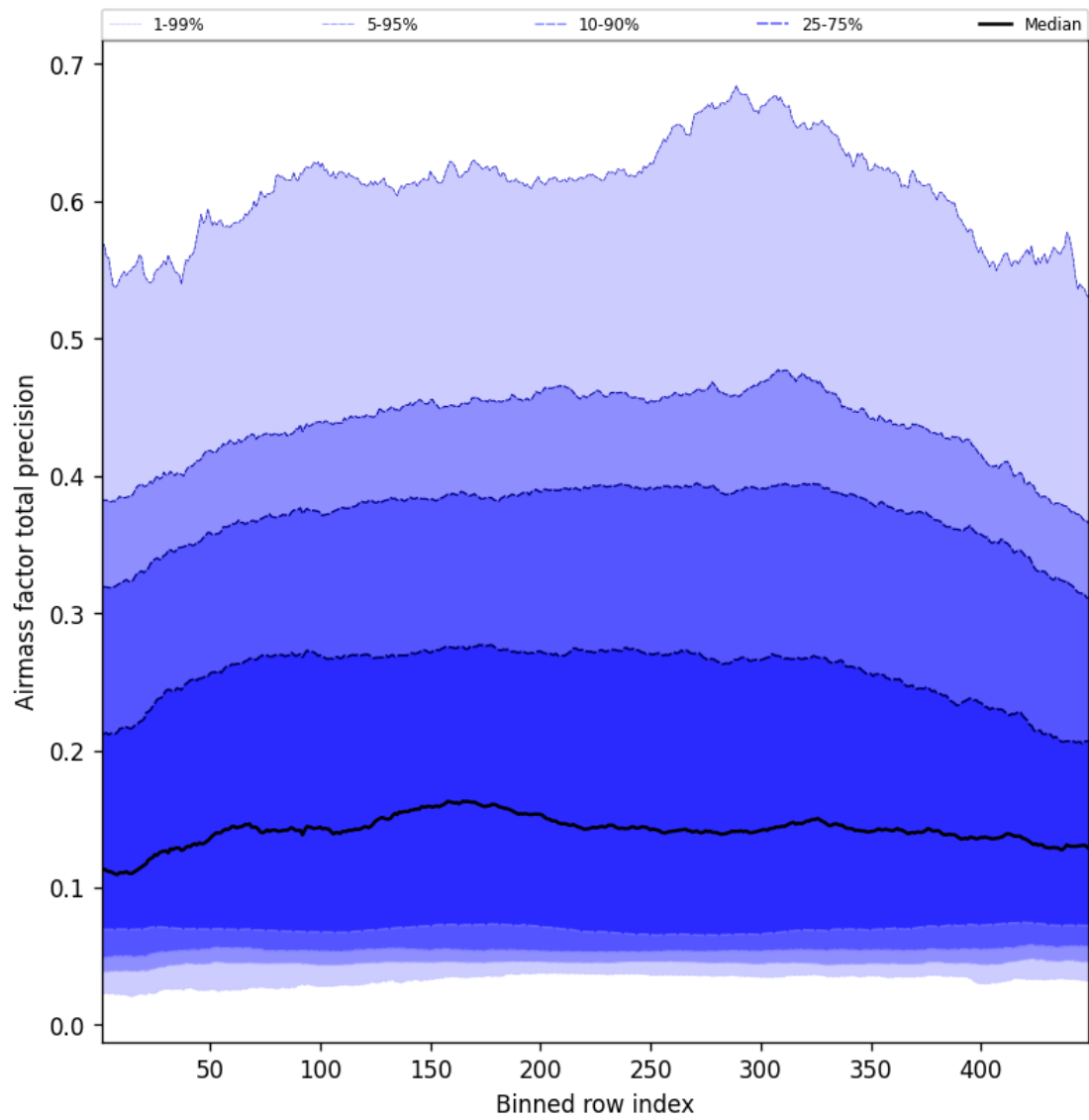
Figure 53: Along track statistics of “Airmass factor total precision” for 2025-07-22 to 2025-07-22
