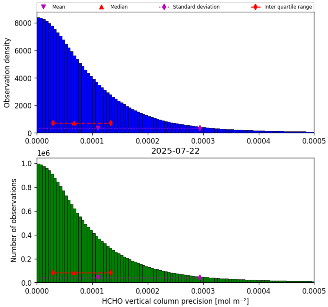
Figure 34: Histogram of “HCHO vertical column precision” for 2025-07-22 to 2025-07-22
