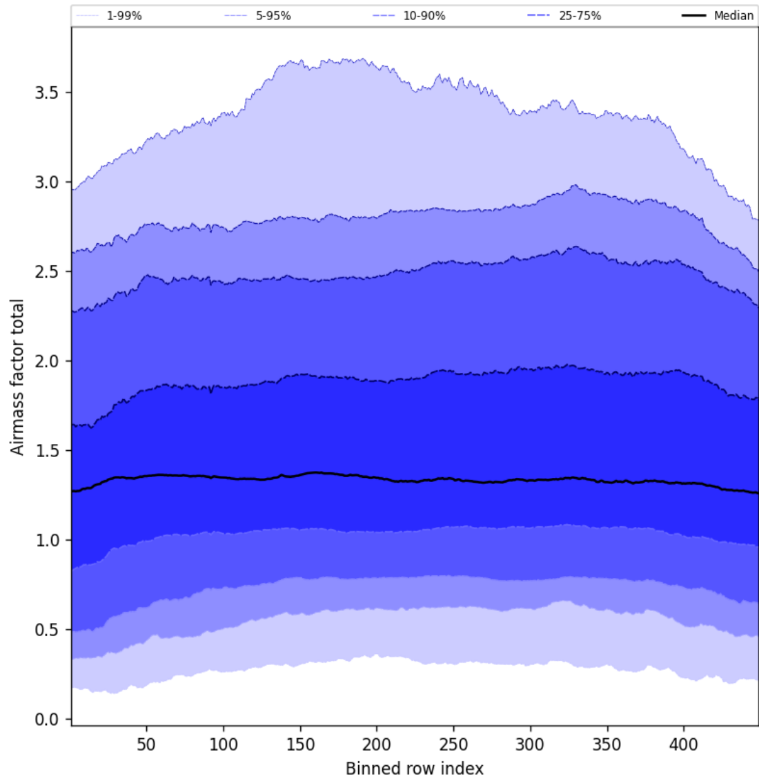
Figure 52: Along track statistics of “Airmass factor total” for 2025-07-22 to 2025-07-22
