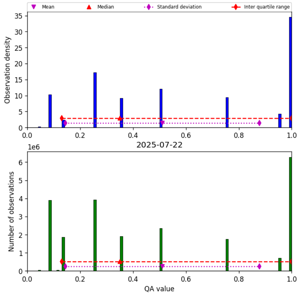
Figure 32: Histogram of “QA value” for 2025-07-22 to 2025-07-22
