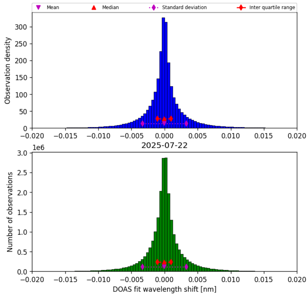
Figure 42: Histogram of “DOAS fit wavelength shift” for 2025-07-22 to 2025-07-22
