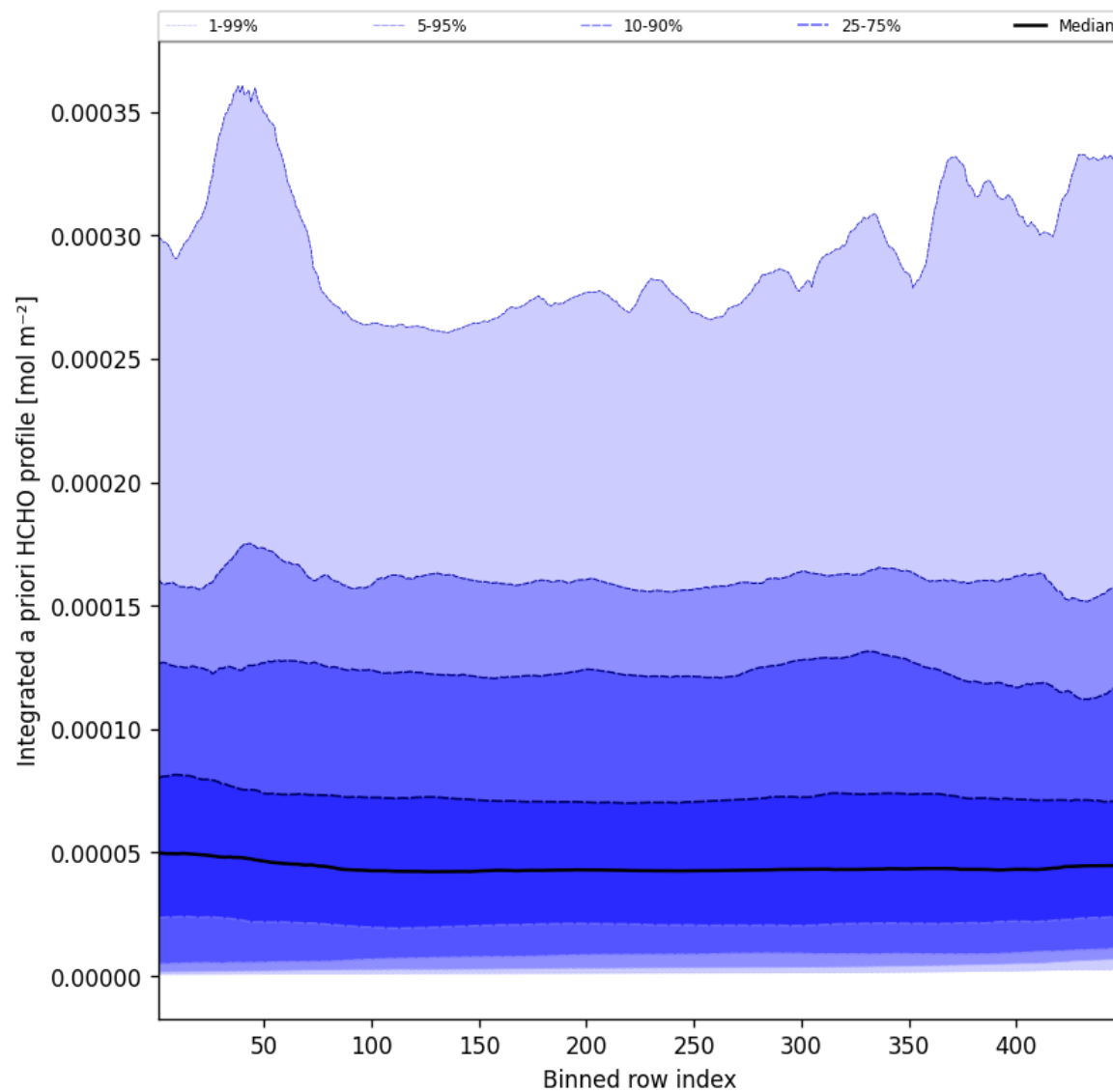
Figure 55: Along track statistics of "Integrated a priori HCHO profile" for 2025-07-22 to 2025-07-22
