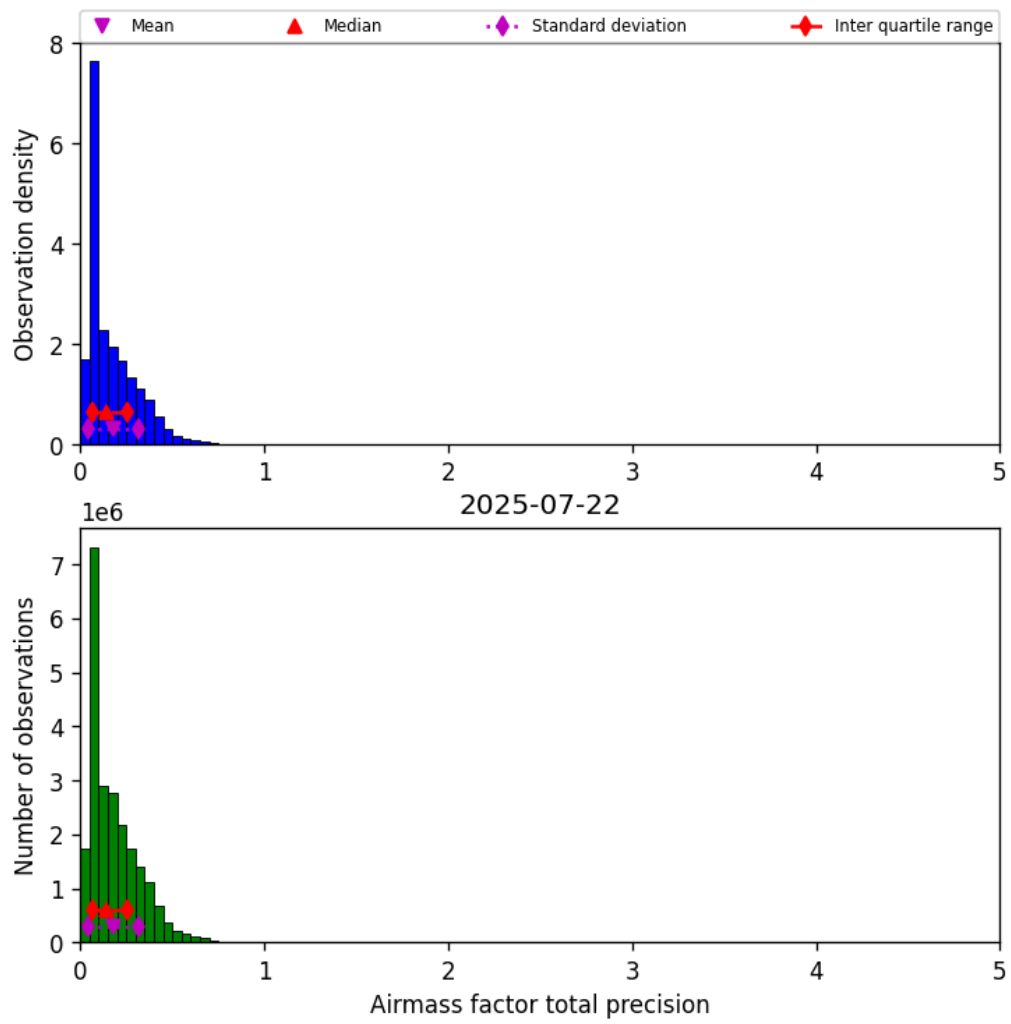
Figure 39: Histogram of “Airmass factor total precision” for 2025-07-22 to 2025-07-22
