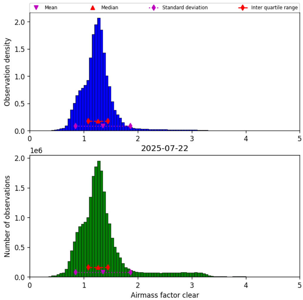
Figure 40: Histogram of “Airmass factor clear” for 2025-07-22 to 2025-07-22
