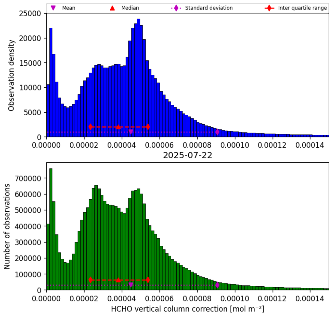
Figure 35: Histogram of “HCHO vertical column correction” for 2025-07-22 to 2025-07-22
