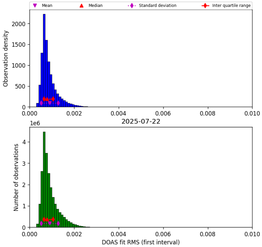
Figure 44: Histogram of “DOAS fit RMS (first interval)” for 2025-07-22 to 2025-07-22
