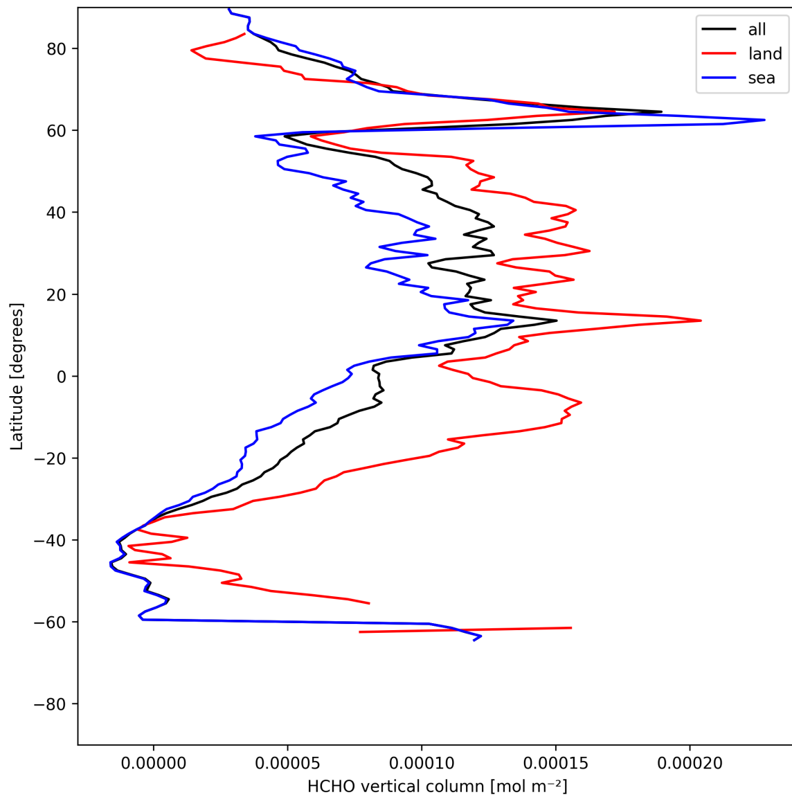
Figure 19: Zonal average of “HCHO vertical column” for 2025-07-22 to 2025-07-22.
