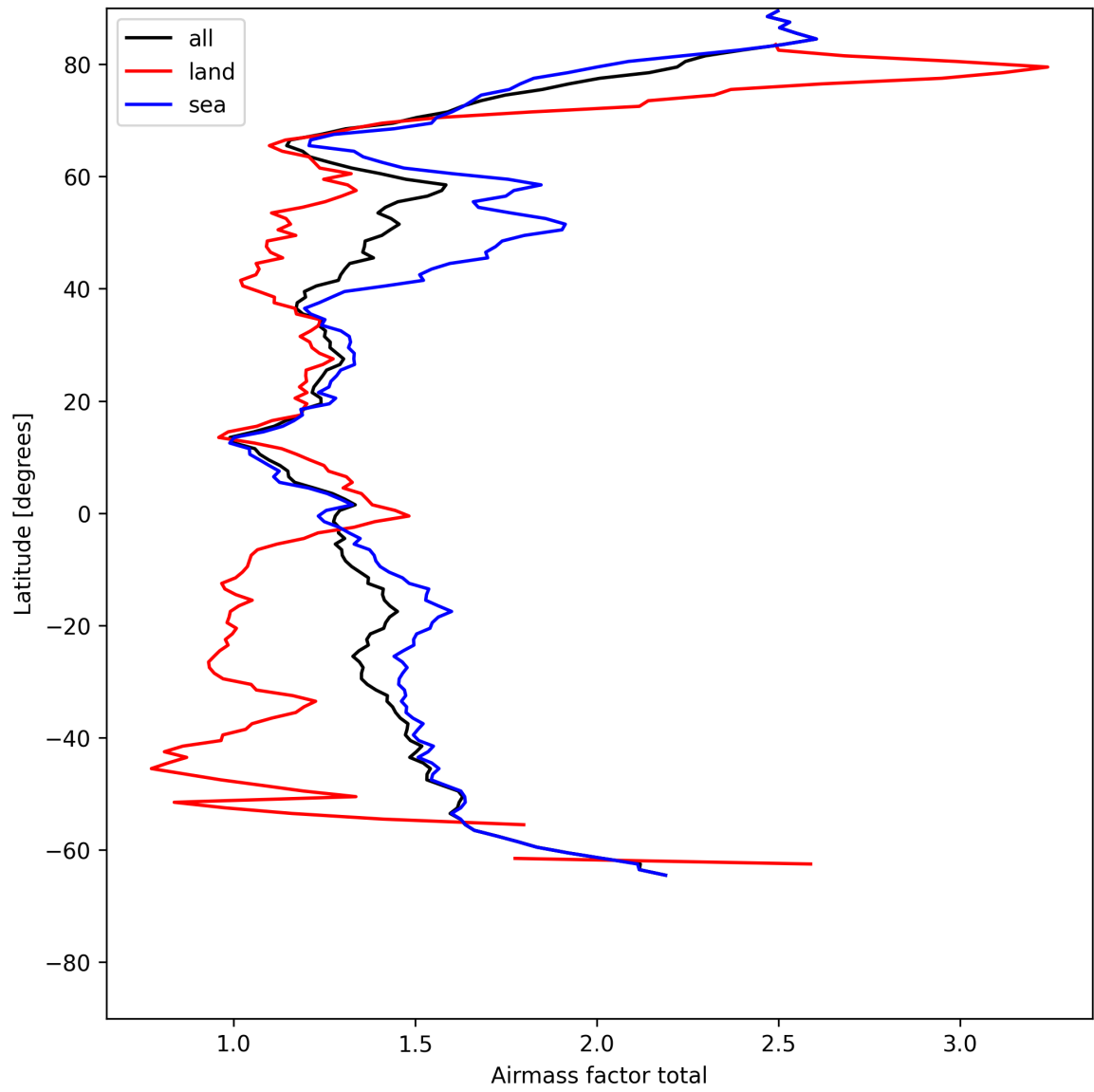
Figure 24: Zonal average of “Airmass factor total” for 2025-07-22 to 2025-07-22.
