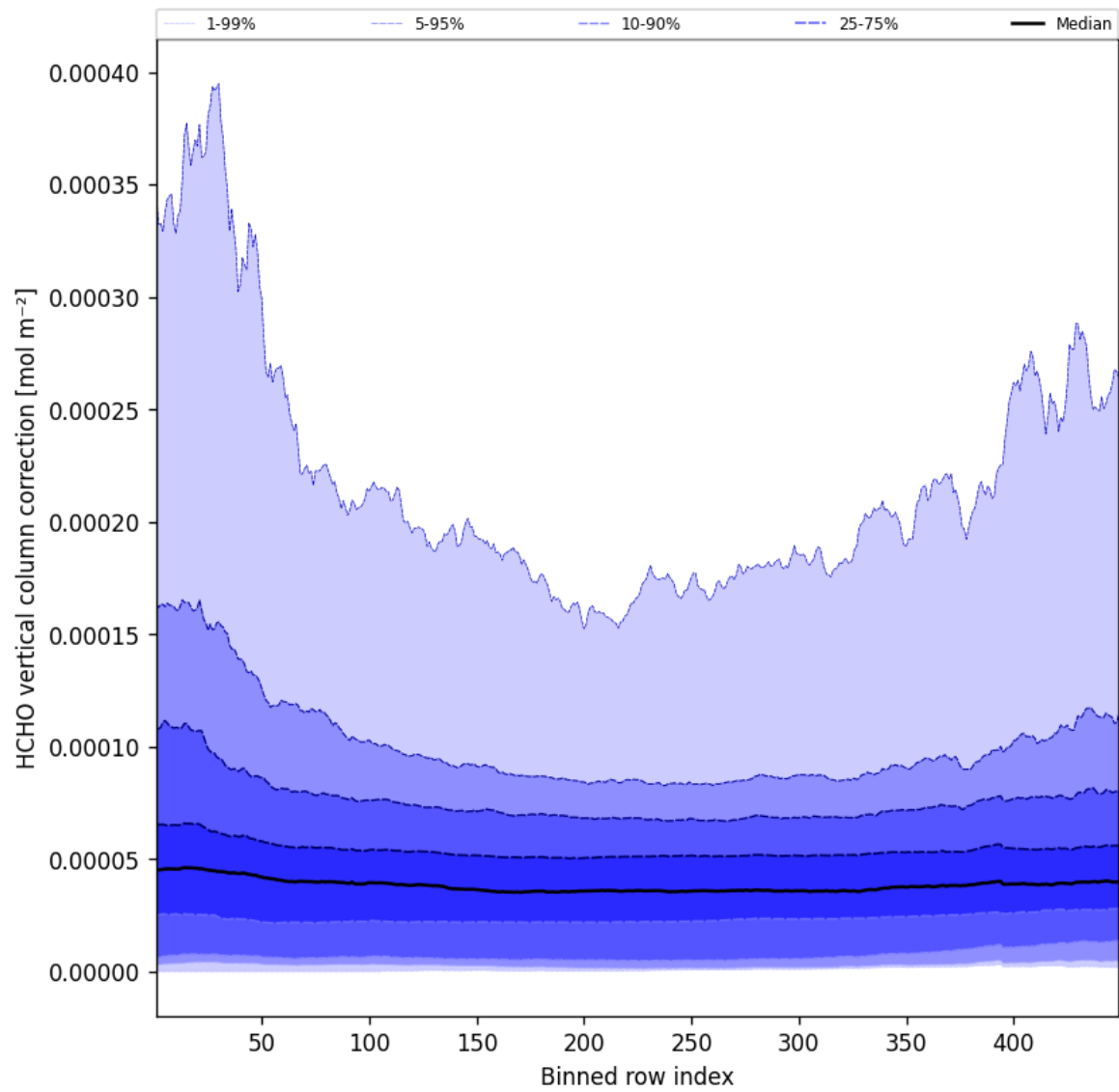
Figure 49: Along track statistics of “HCHO vertical column correction” for 2025-07-22 to 2025-07-22
