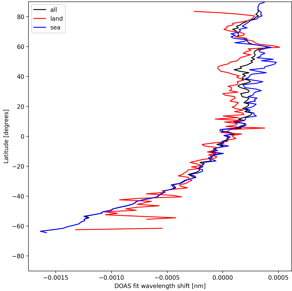
Figure 28: Zonal average of “DOAS fit wavelength shift” for 2025-07-22 to 2025-07-22.
