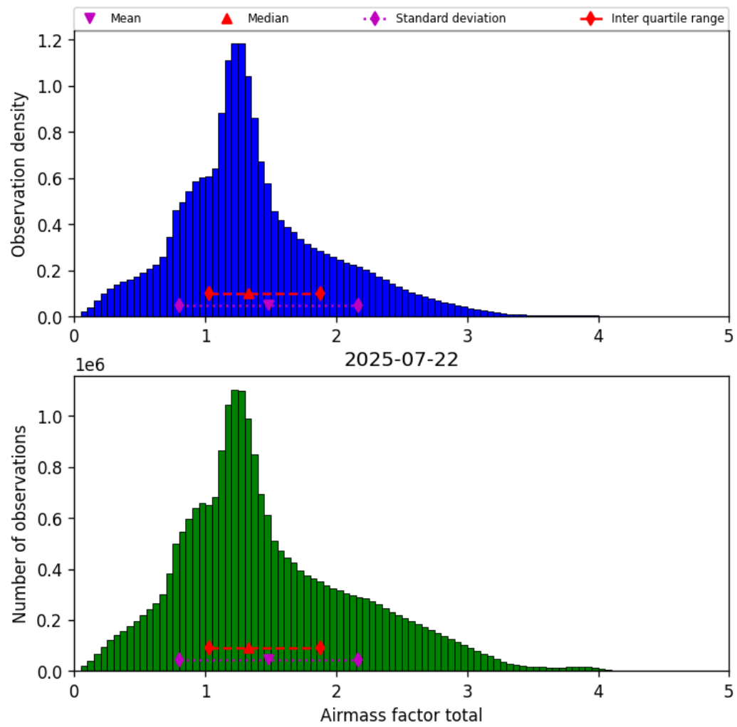
Figure 38: Histogram of “Airmass factor total” for 2025-07-22 to 2025-07-22
