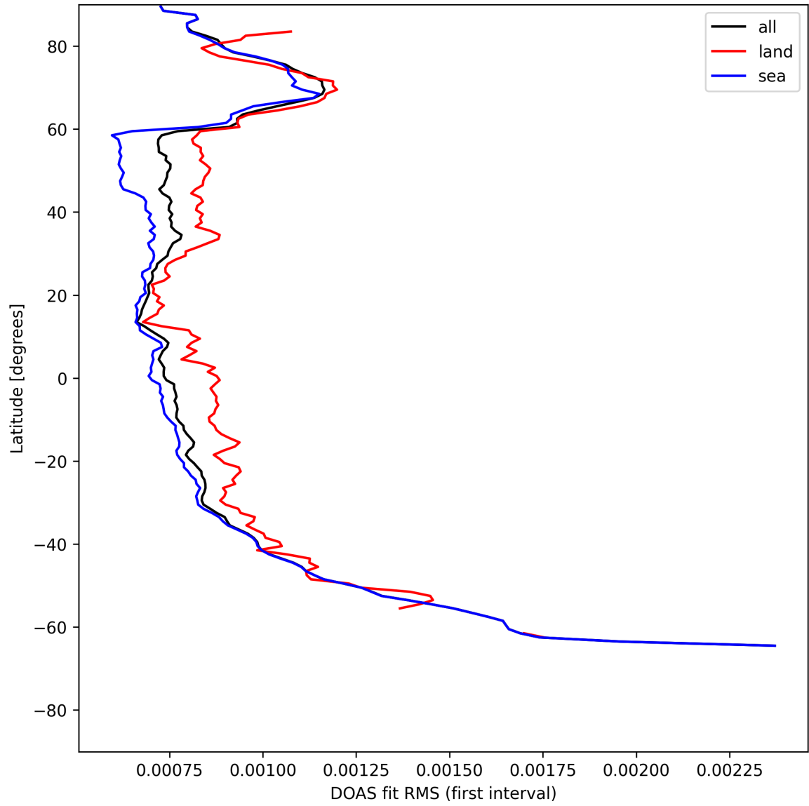
Figure 30: Zonal average of “DOAS fit RMS (first interval)” for 2025-07-22 to 2025-07-22.
