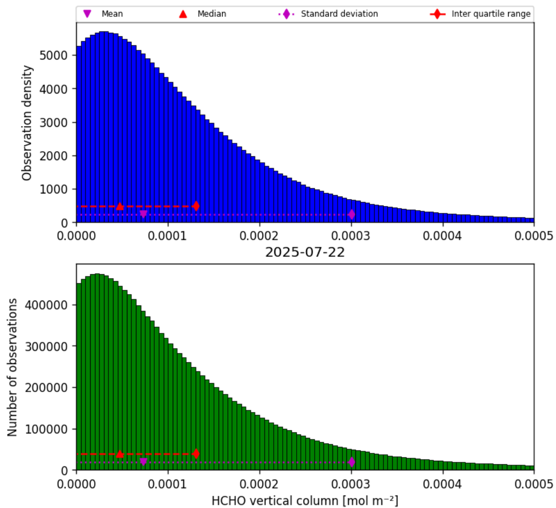
Figure 33: Histogram of “HCHO vertical column” for 2025-07-22 to 2025-07-22
