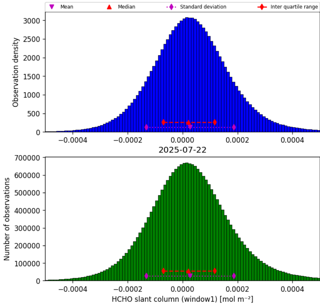
Figure 36: Histogram of “HCHO slant column (window1)” for 2025-07-22 to 2025-07-22
