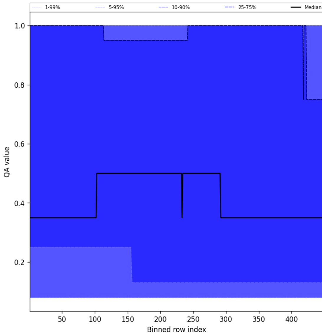
Figure 46: Along track statistics of “QA value” for 2025-07-22 to 2025-07-22
