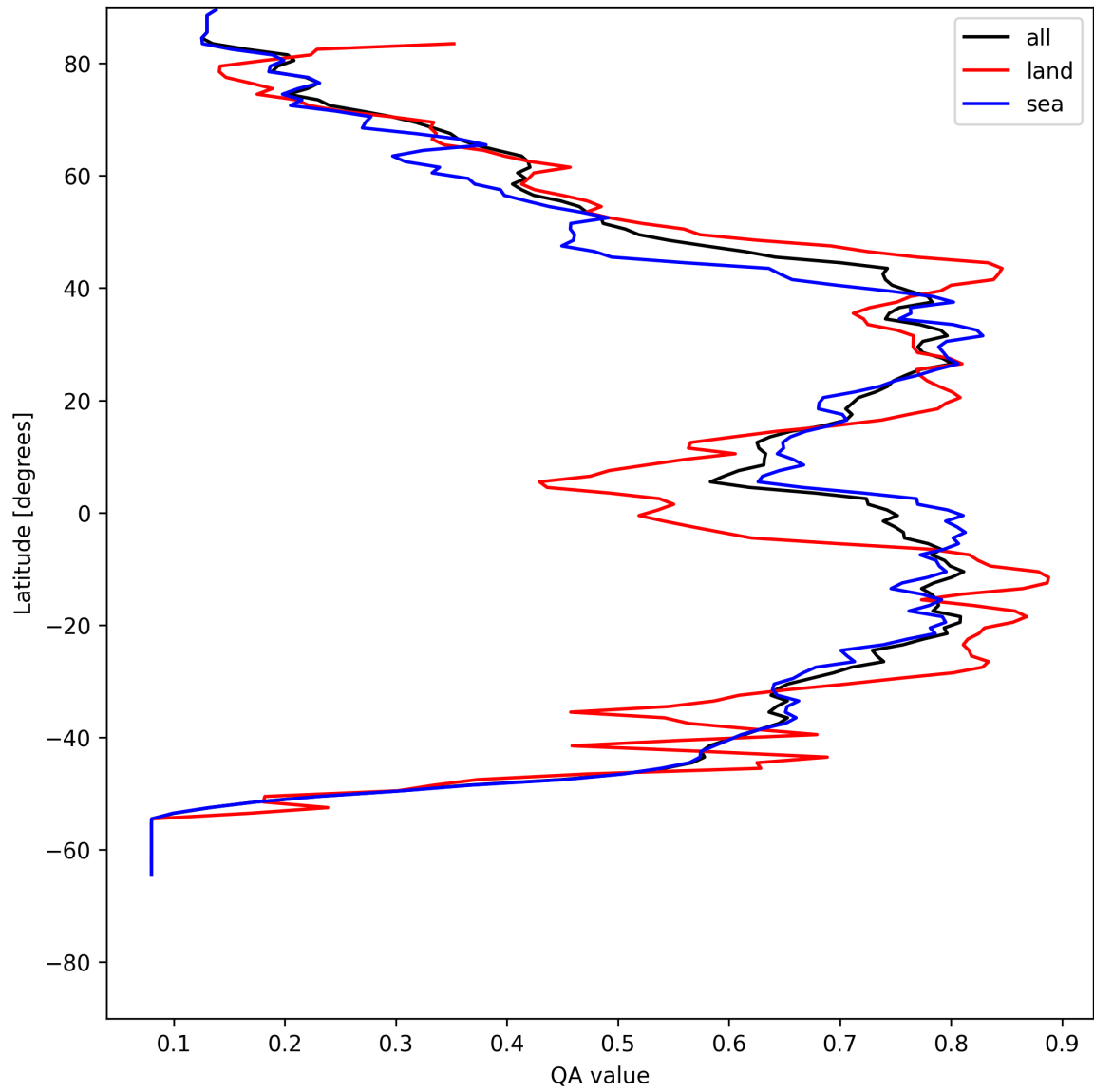
Figure 18: Zonal average of “QA value” for 2025-07-22 to 2025-07-22.
