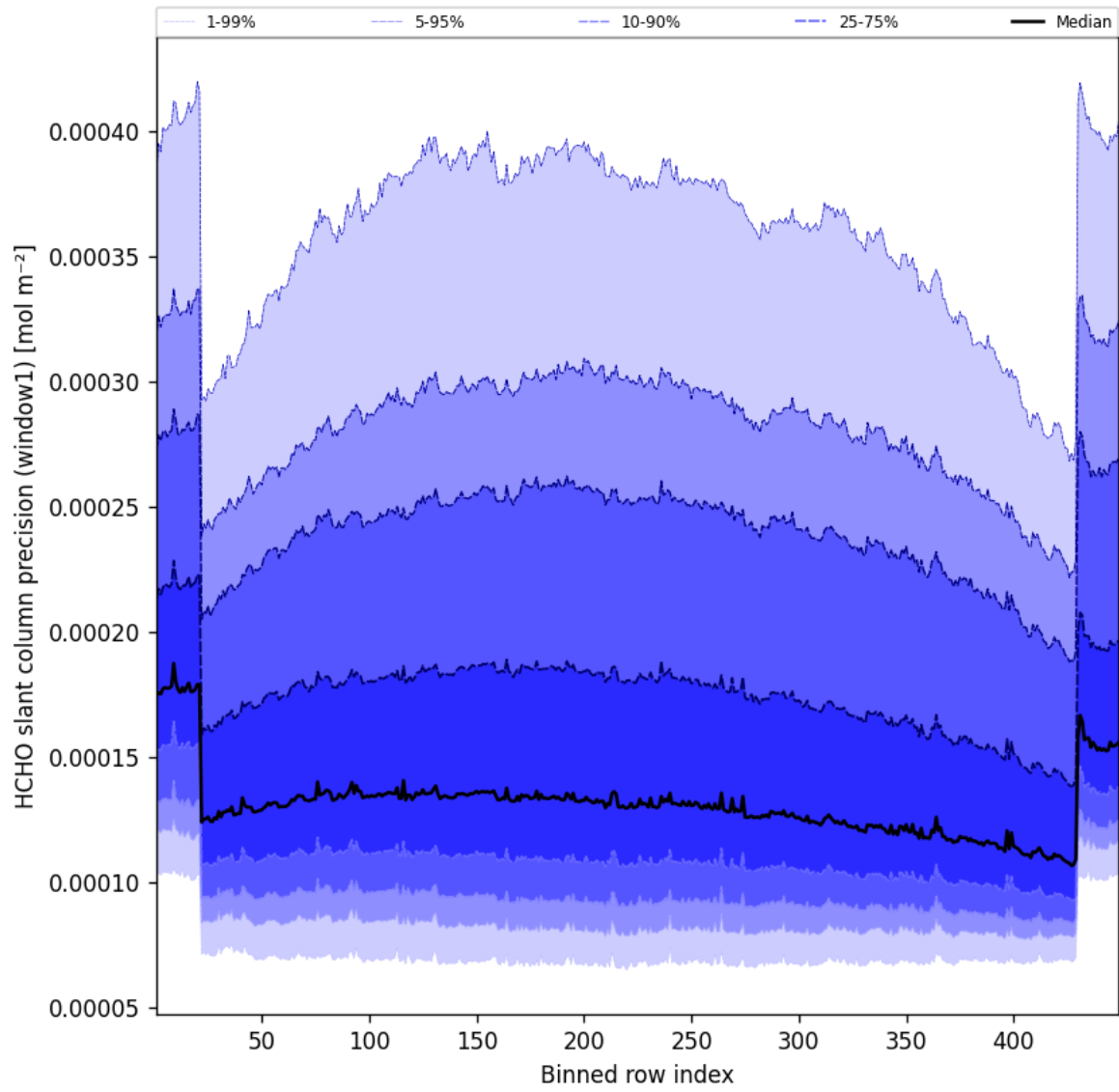
Figure 51: Along track statistics of "HCHO slant column precision (window1)" for 2025-07-22 to 2025-07-22
