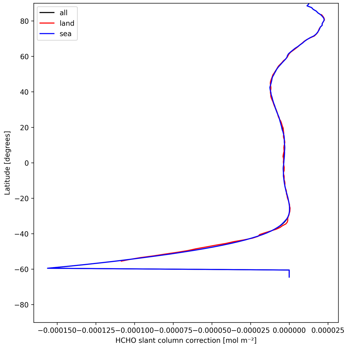
Figure 31: Zonal average of “HCHO slant column correction” for 2025-07-22 to 2025-07-22.
