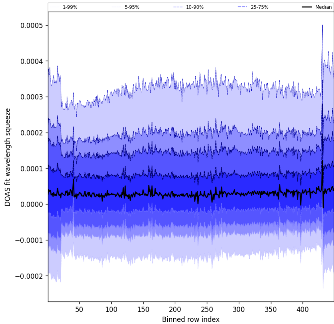
Figure 57: Along track statistics of “DOAS fit wavelength squeeze” for 2025-07-22 to 2025-07-22
