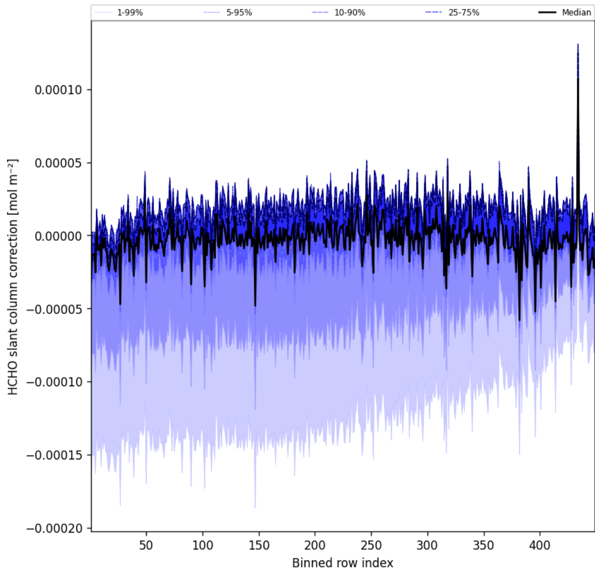
Figure 59: Along track statistics of “HCHO slant column correction” for 2025-07-22 to 2025-07-22
