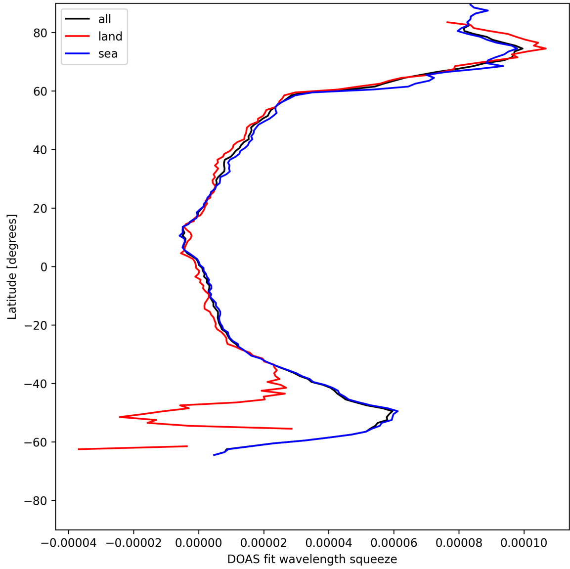
Figure 29: Zonal average of “DOAS fit wavelength squeeze” for 2025-07-22 to 2025-07-22.
