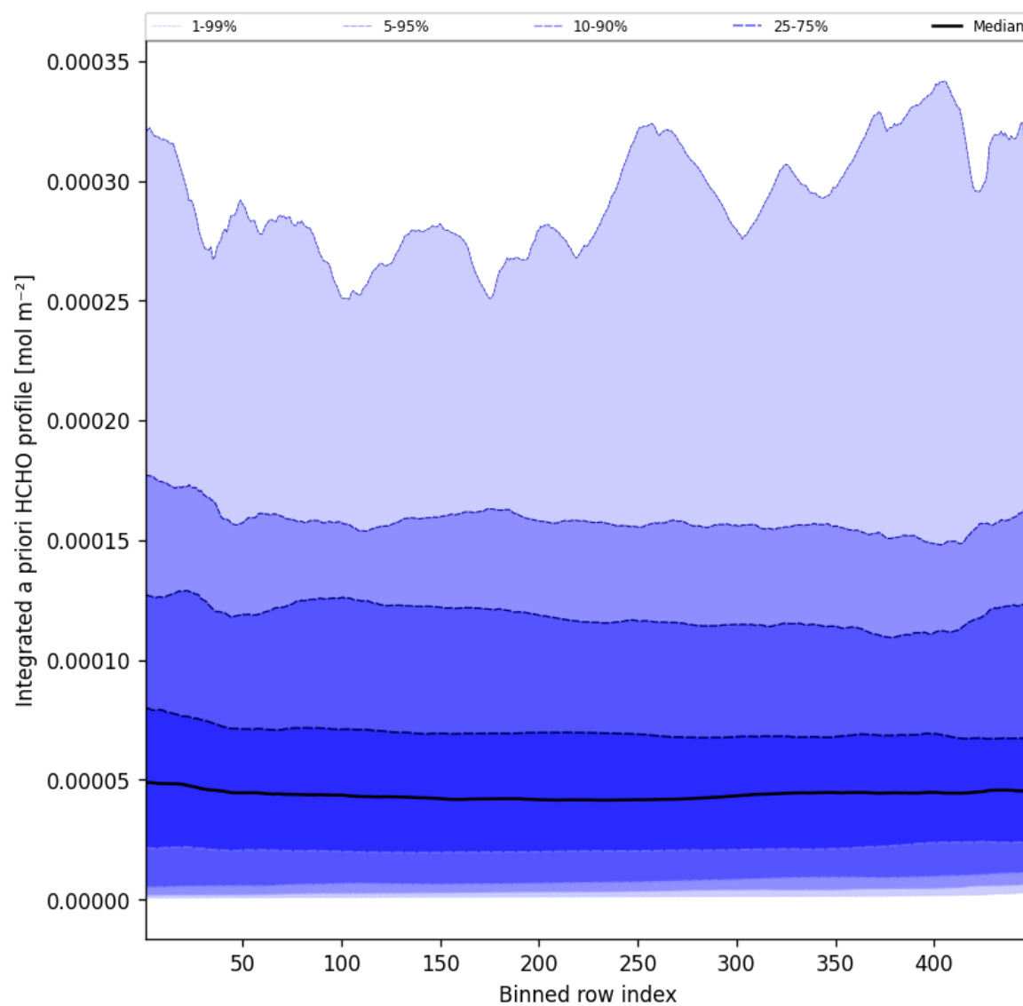
Figure 55: Along track statistics of “Integrated a priori HCHO profile” for 2025-07-23 to 2025-07-24
