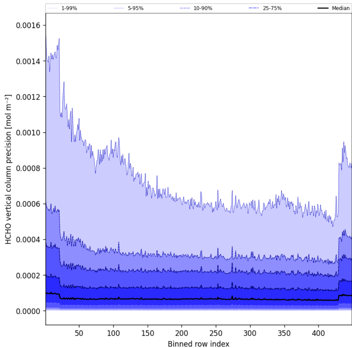
Figure 48: Along track statistics of “HCHO vertical column precision” for 2025-07-23 to 2025-07-24
