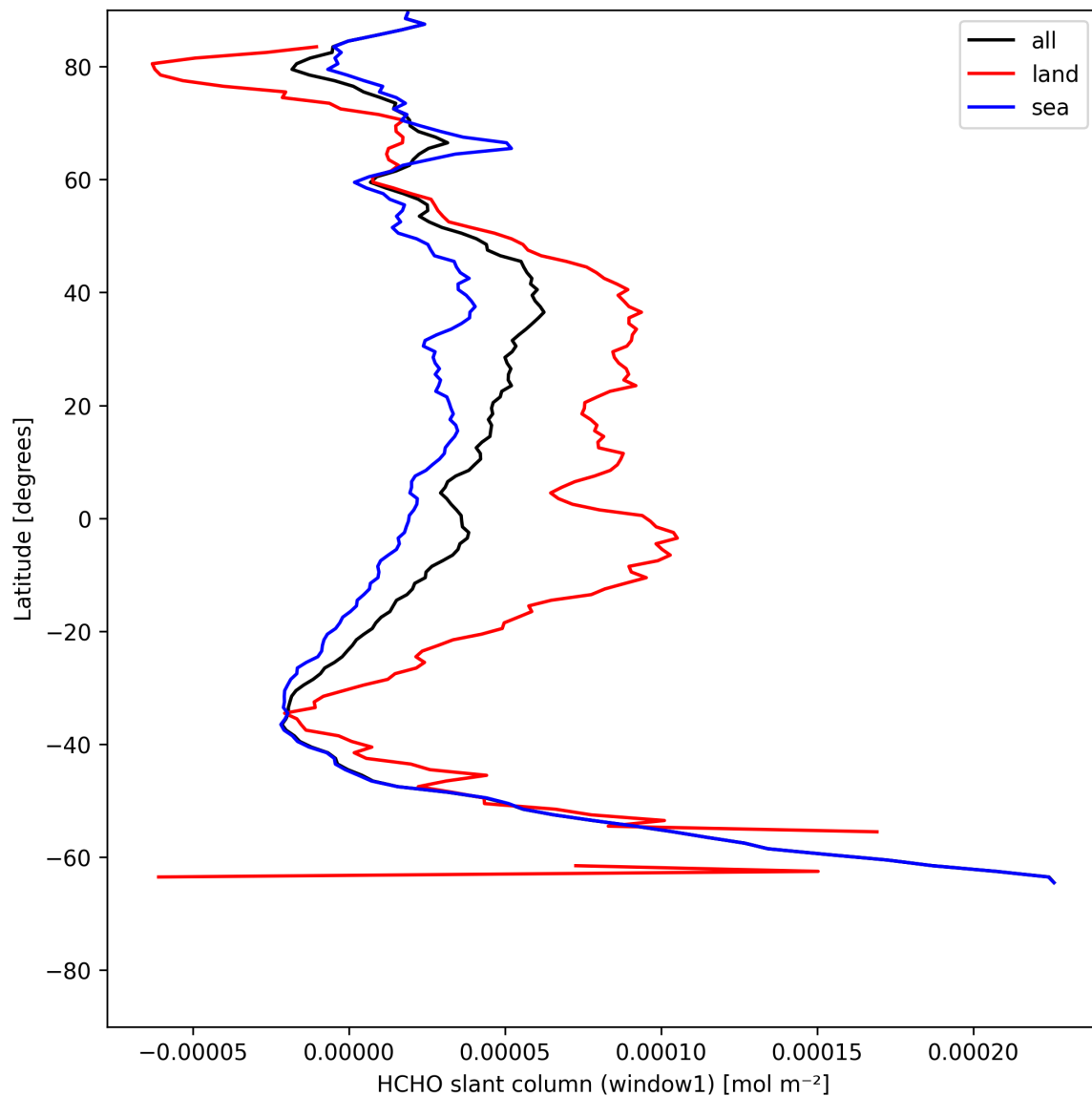
Figure 22: Zonal average of “HCHO slant column (window1)” for 2025-07-23 to 2025-07-24.
