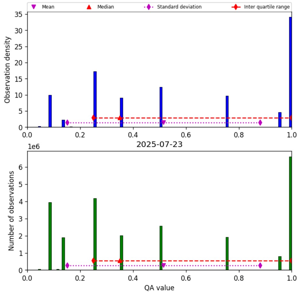
Figure 32: Histogram of “QA value” for 2025-07-23 to 2025-07-24
