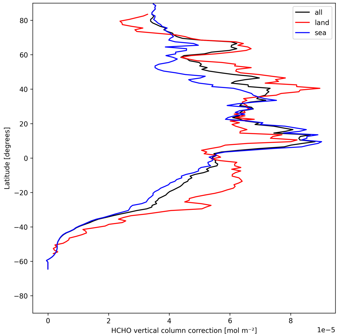
Figure 21: Zonal average of “HCHO vertical column correction” for 2025-07-23 to 2025-07-24.
