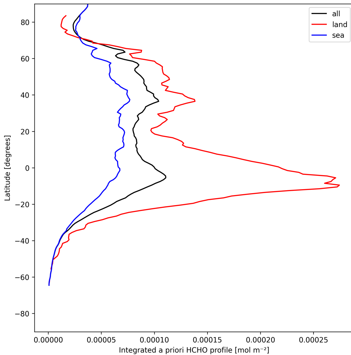
Figure 27: Zonal average of “Integrated a priori HCHO profile” for 2025-07-23 to 2025-07-24.
