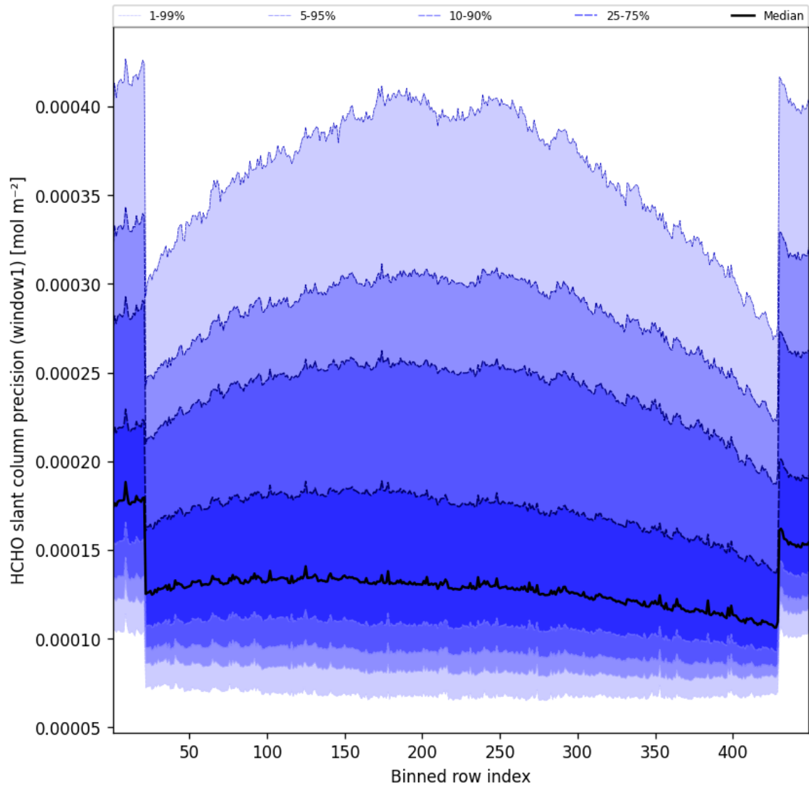
Figure 51: Along track statistics of “HCHO slant column precision (window1)” for 2025-07-23 to 2025-07-24
