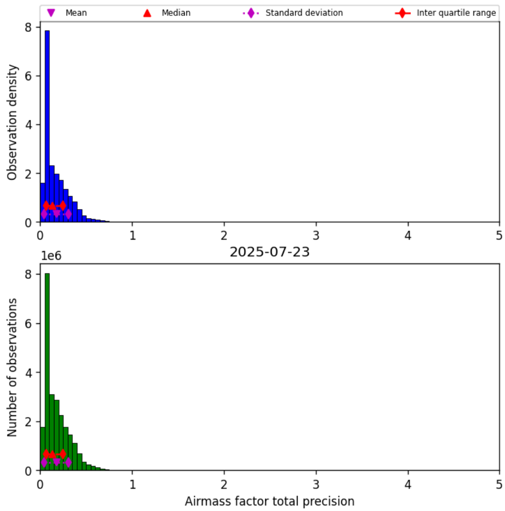
Figure 39: Histogram of “Airmass factor total precision” for 2025-07-23 to 2025-07-24
