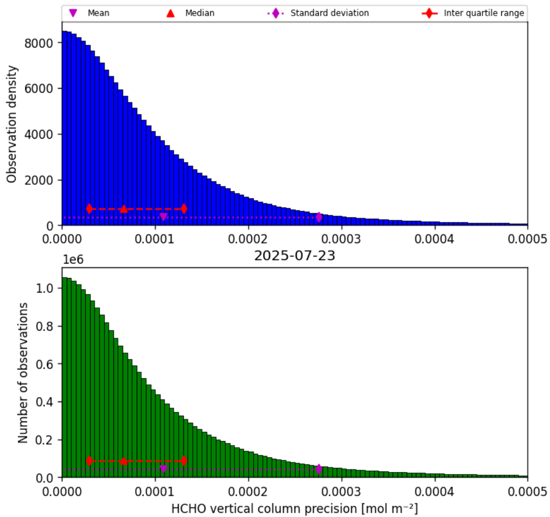
Figure 34: Histogram of “HCHO vertical column precision” for 2025-07-23 to 2025-07-24
