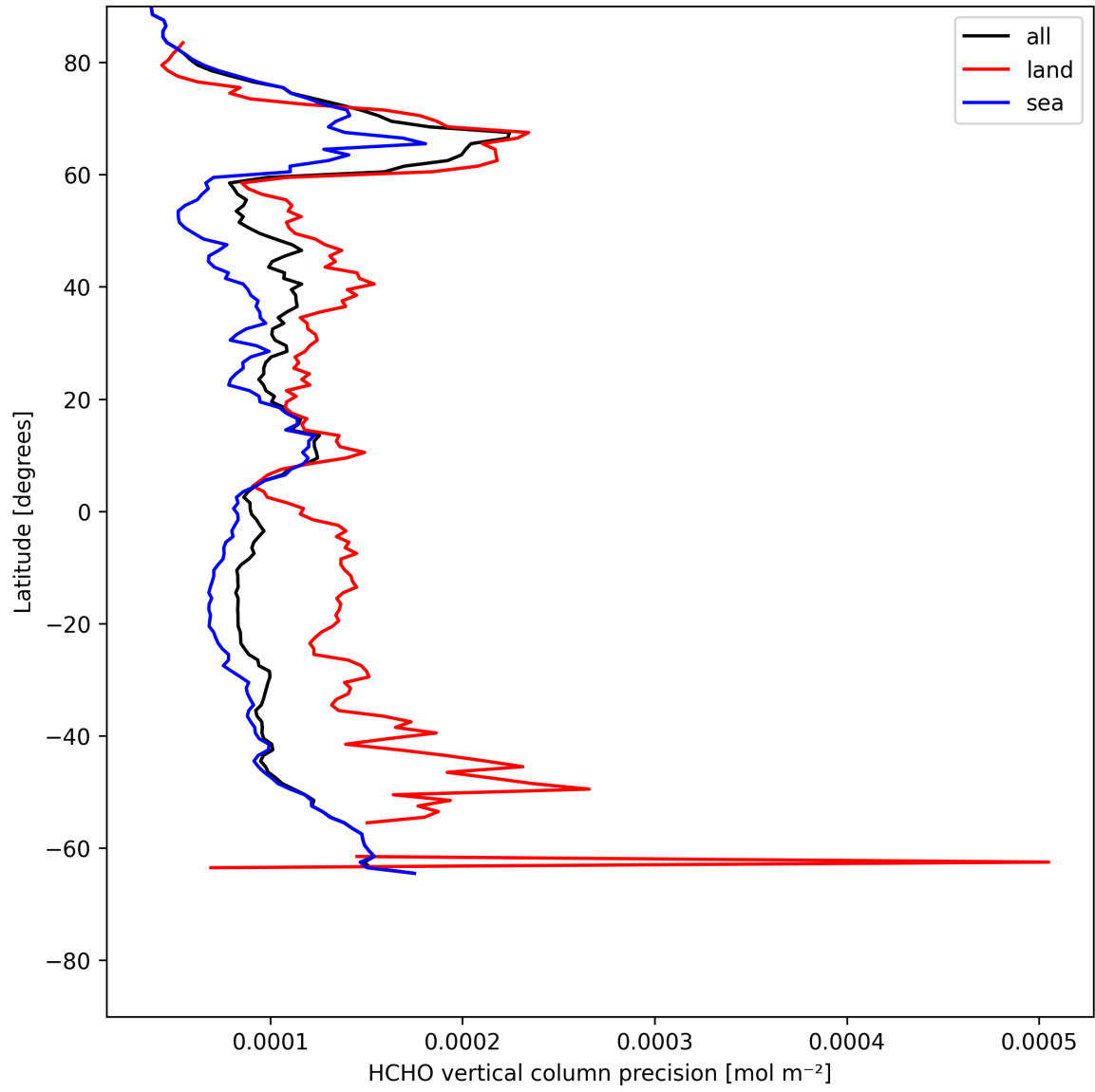
Figure 20: Zonal average of “HCHO vertical column precision” for 2025-07-23 to 2025-07-24.
