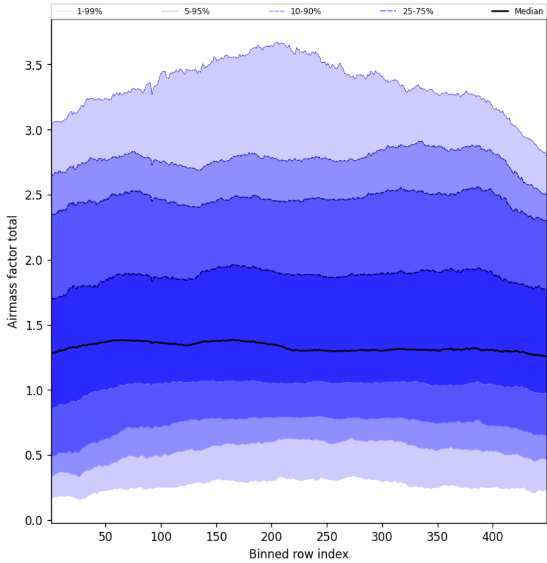
Figure 52: Along track statistics of “Airmass factor total” for 2025-07-23 to 2025-07-24
