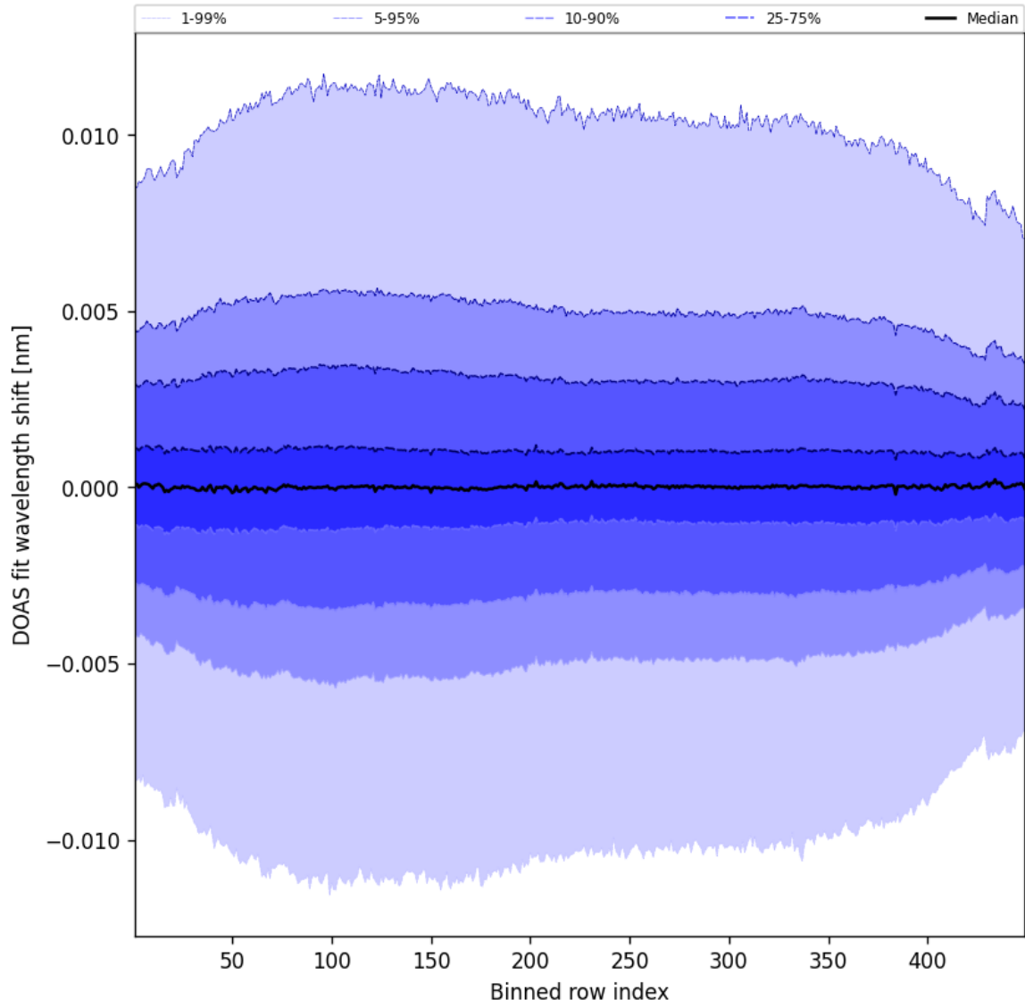
Figure 56: Along track statistics of “DOAS fit wavelength shift” for 2025-07-23 to 2025-07-24
