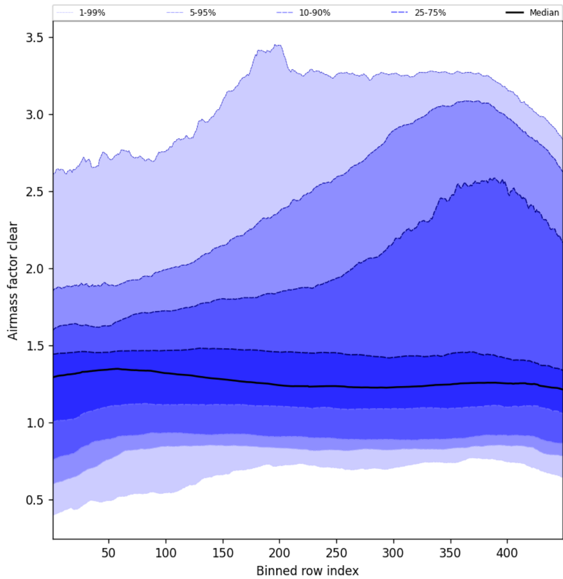
Figure 54: Along track statistics of “Airmass factor clear” for 2025-07-23 to 2025-07-24
