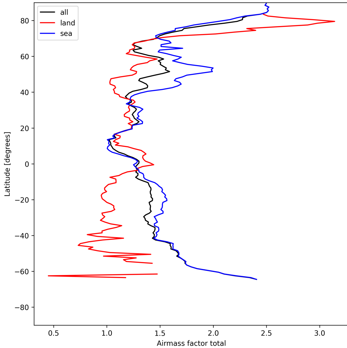
Figure 24: Zonal average of "Airmass factor total" for 2025-07-23 to 2025-07-24.
