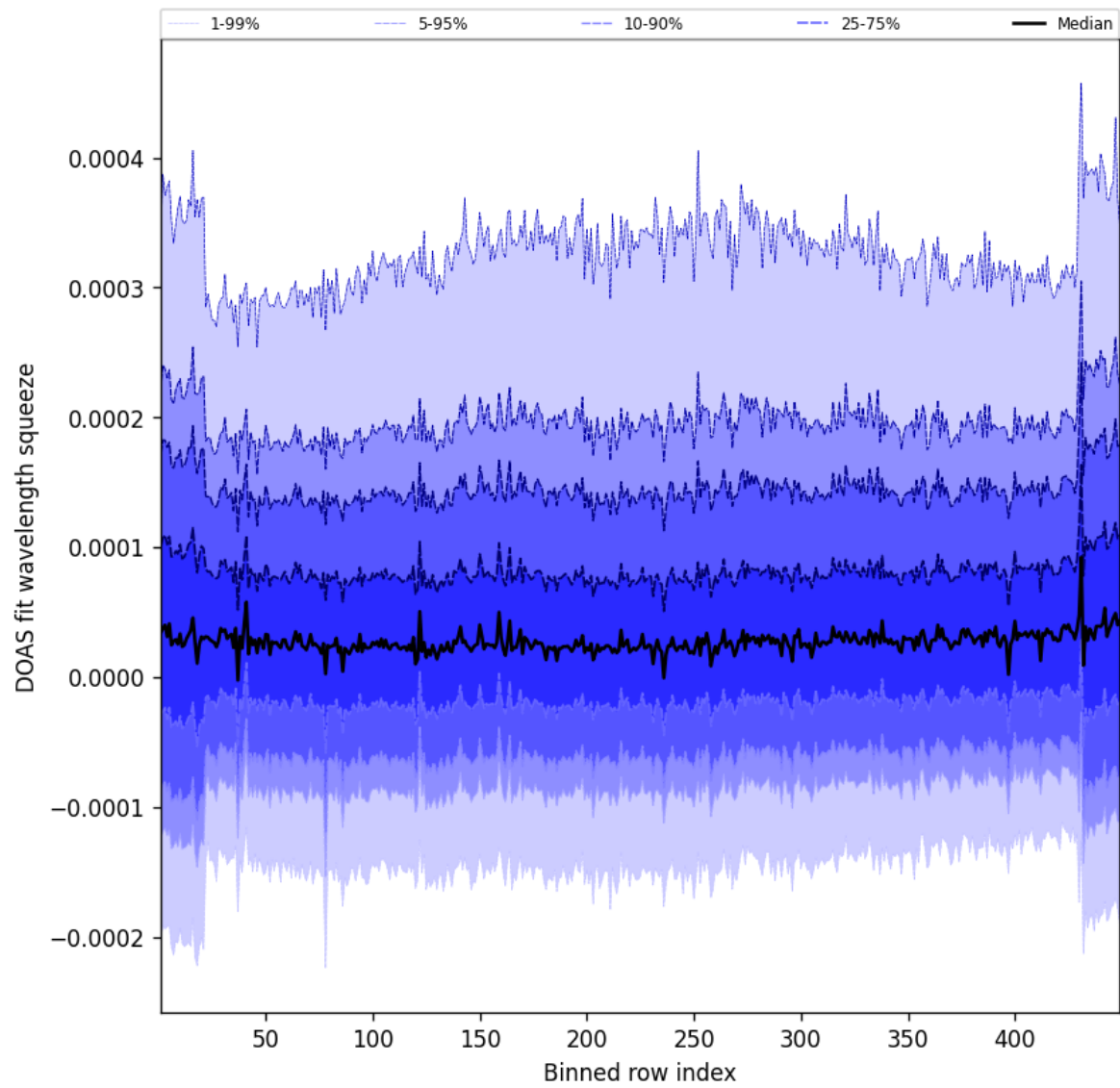
Figure 57: Along track statistics of “DOAS fit wavelength squeeze” for 2025-07-23 to 2025-07-24
