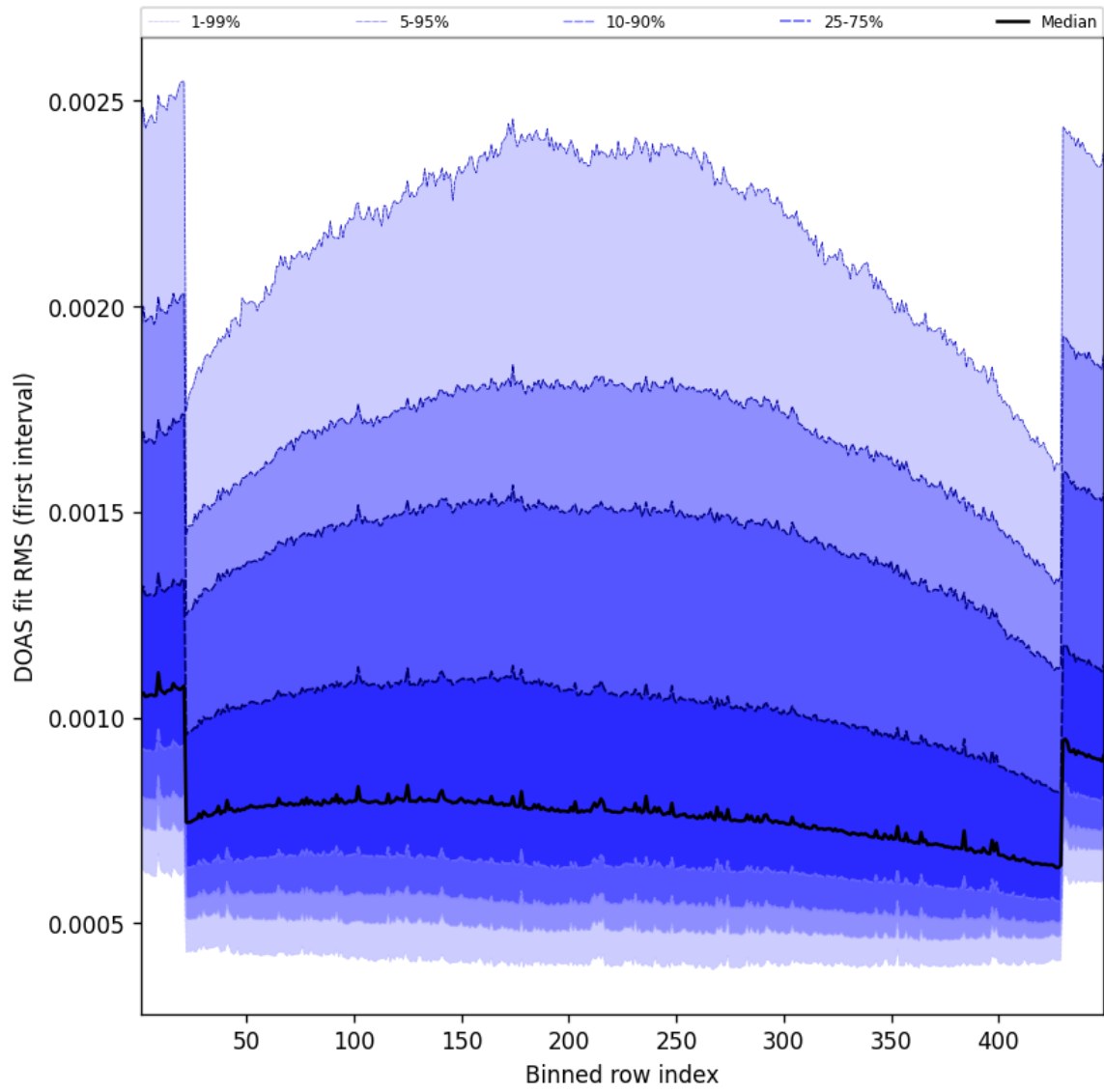
Figure 58: Along track statistics of “DOAS fit RMS (first interval)” for 2025-07-23 to 2025-07-24
