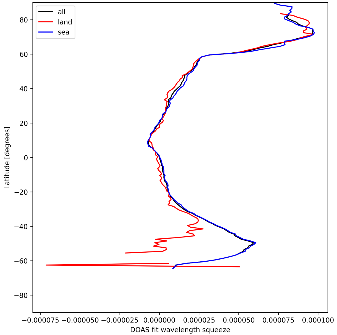
Figure 29: Zonal average of “DOAS fit wavelength squeeze” for 2025-07-23 to 2025-07-24.
