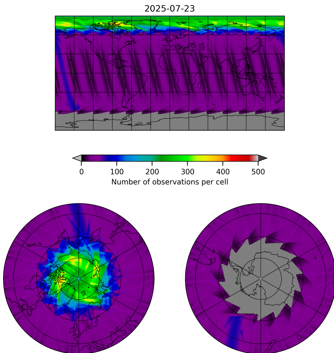
Figure 17: Map of the number of observations for 2025-07-23 to 2025-07-24
