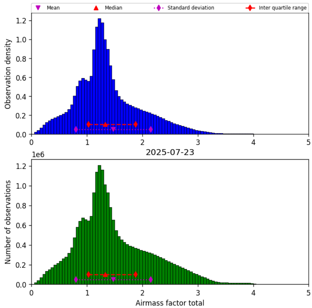
Figure 38: Histogram of “Airmass factor total” for 2025-07-23 to 2025-07-24
