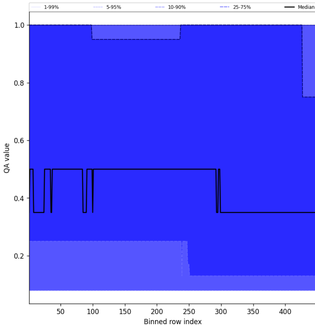
Figure 46: Along track statistics of “QA value” for 2025-07-23 to 2025-07-24
