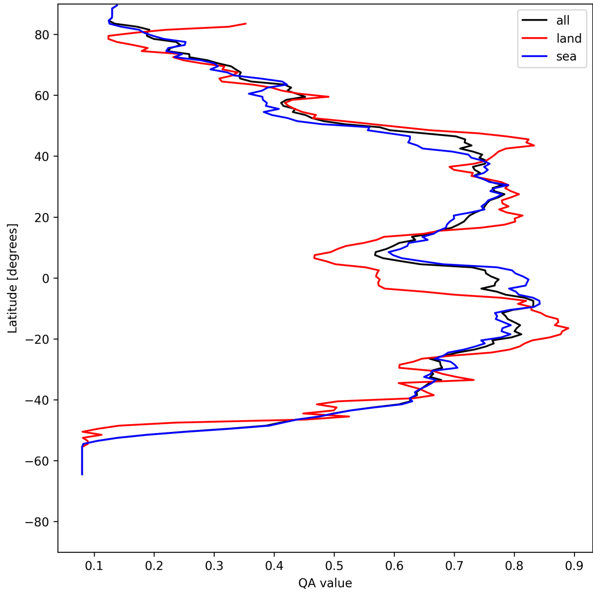
Figure 18: Zonal average of “QA value” for 2025-07-23 to 2025-07-24.
