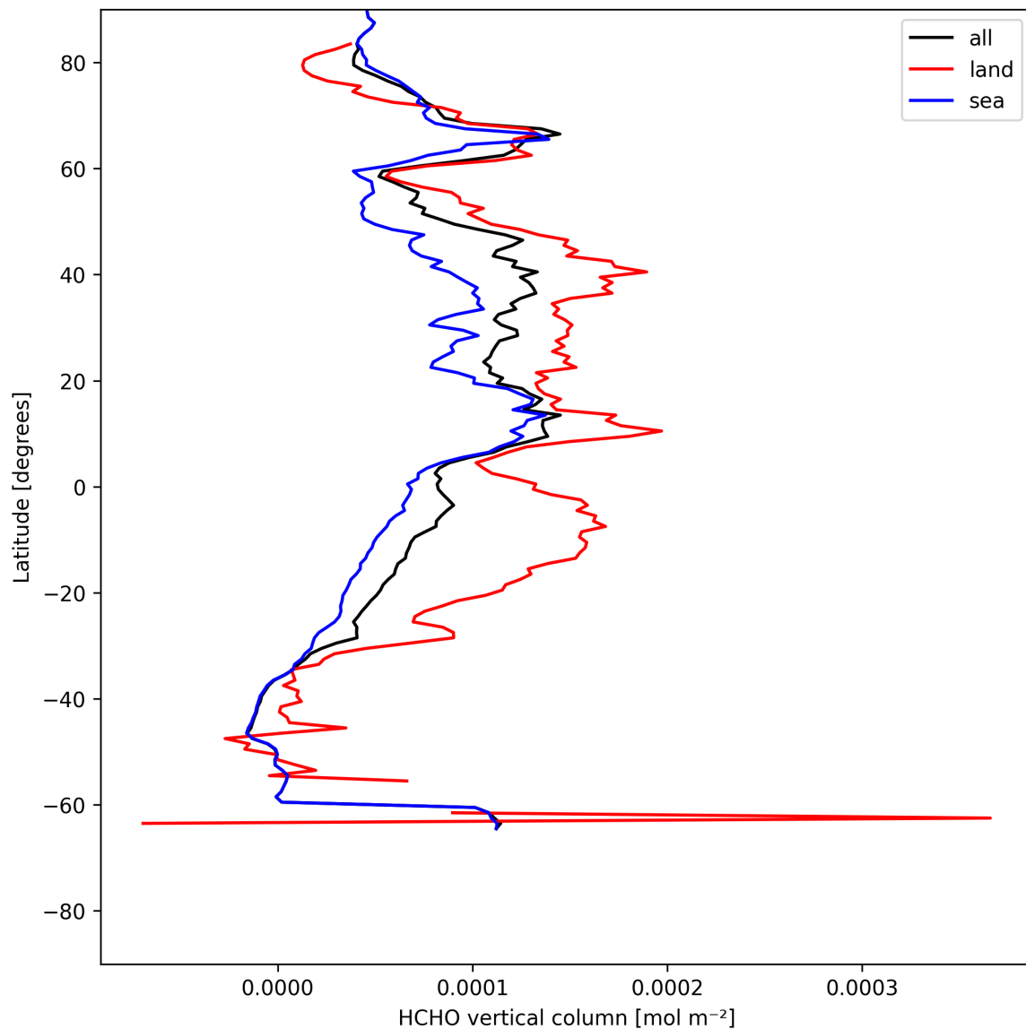
Figure 19: Zonal average of “HCHO vertical column” for 2025-07-23 to 2025-07-24.
