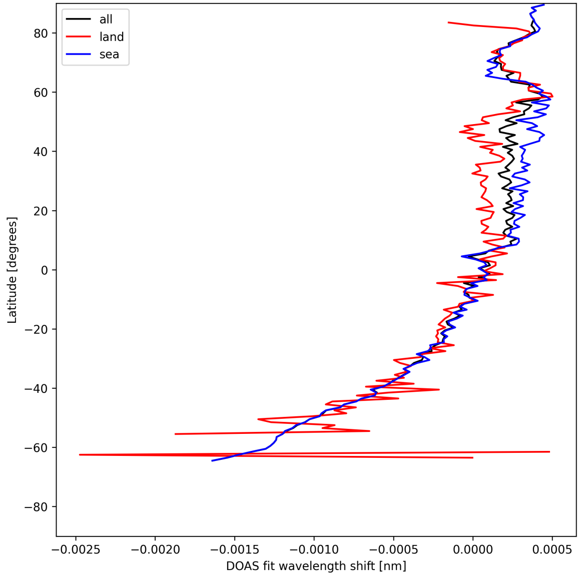
Figure 28: Zonal average of “DOAS fit wavelength shift” for 2025-07-23 to 2025-07-24.
