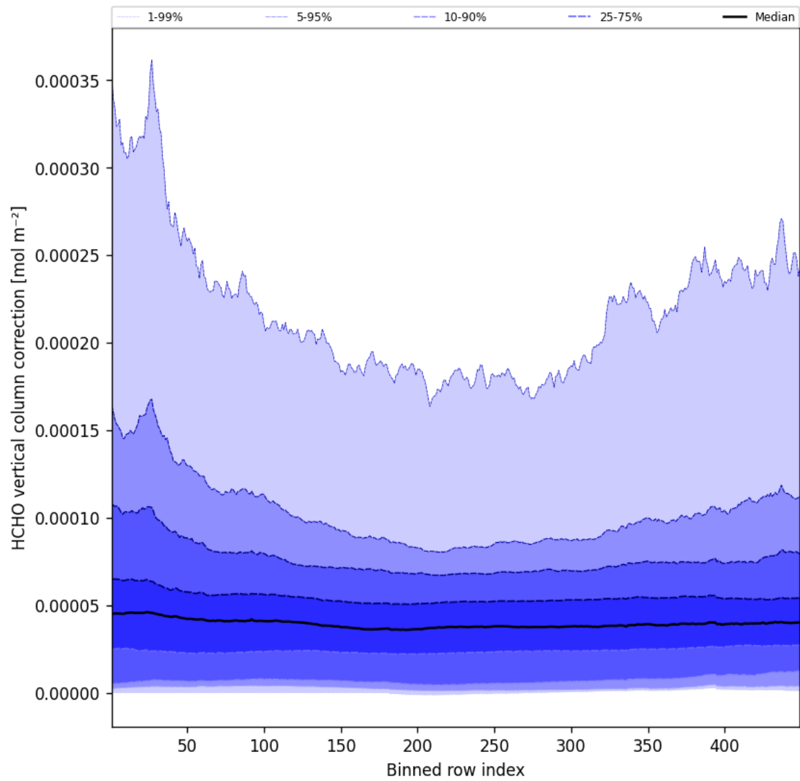
Figure 49: Along track statistics of “HCHO vertical column correction” for 2025-07-23 to 2025-07-24
