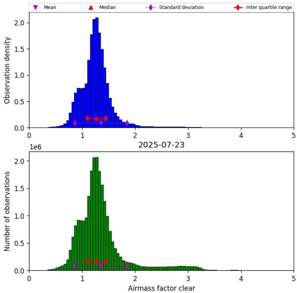
Figure 40: Histogram of “Airmass factor clear” for 2025-07-23 to 2025-07-24
