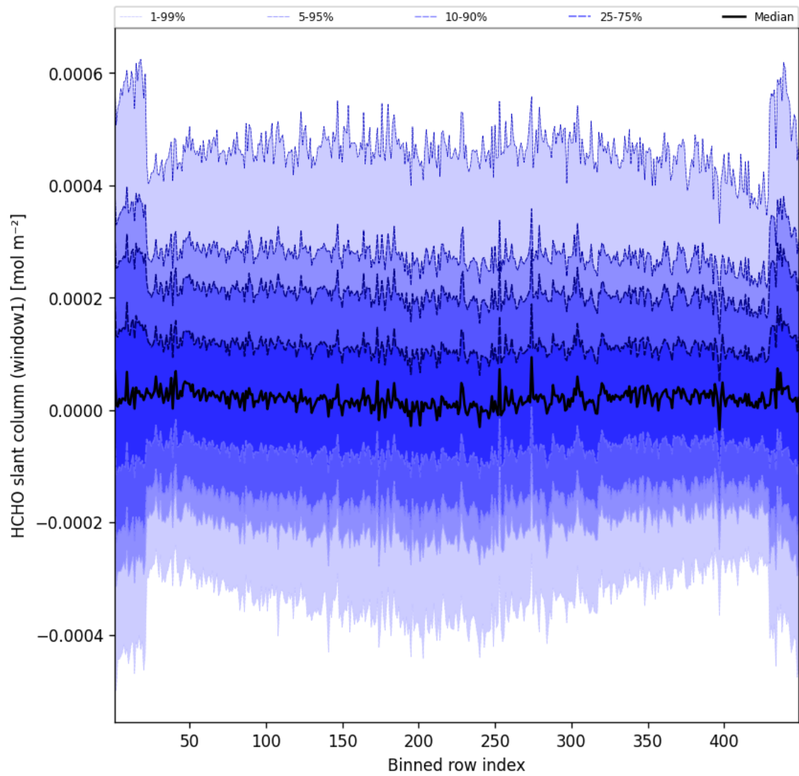
Figure 50: Along track statistics of “HCHO slant column (window1)” for 2025-07-23 to 2025-07-24
