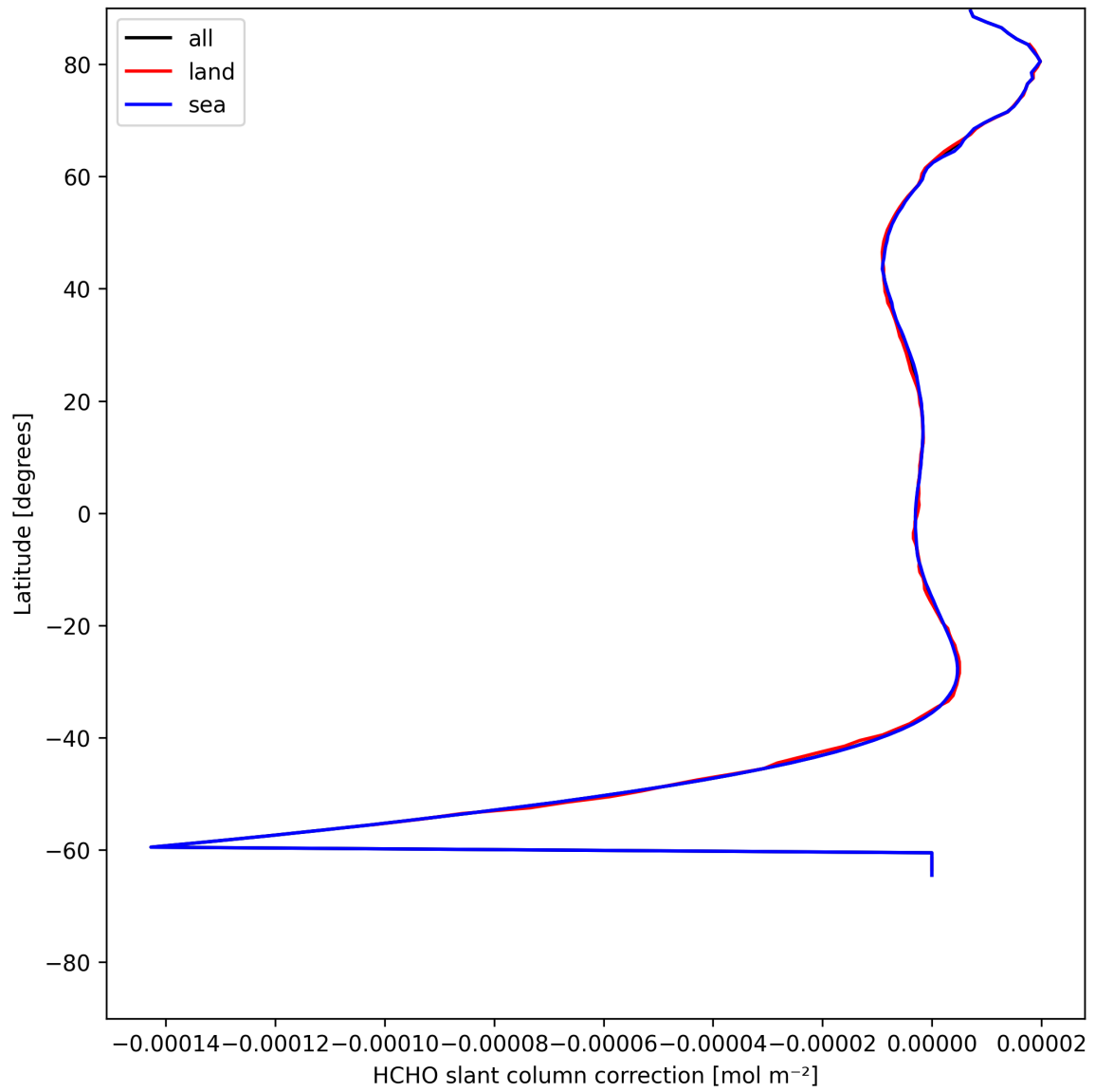
Figure 31: Zonal average of “HCHO slant column correction” for 2025-07-23 to 2025-07-24.
