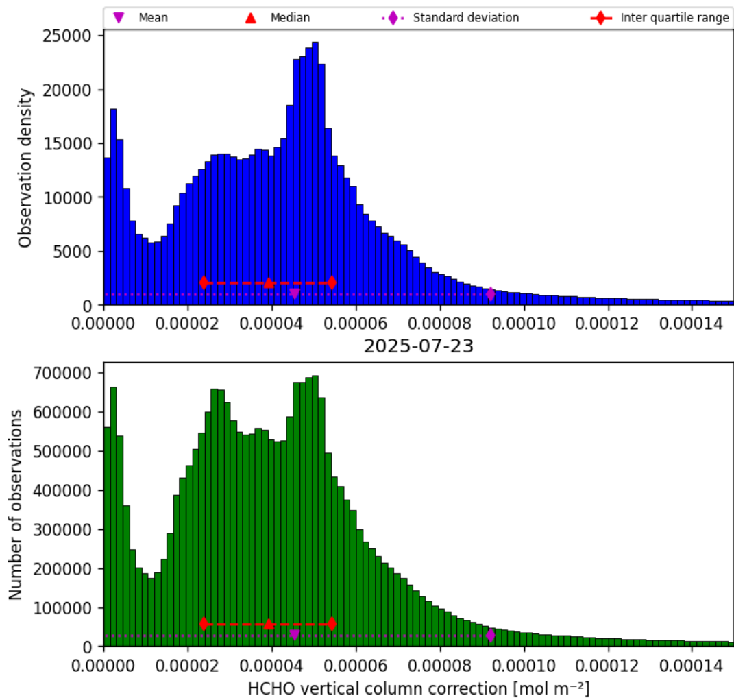
Figure 35: Histogram of “HCHO vertical column correction” for 2025-07-23 to 2025-07-24
