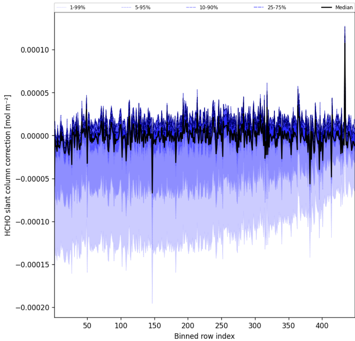
Figure 59: Along track statistics of “HCHO slant column correction” for 2025-07-23 to 2025-07-24
