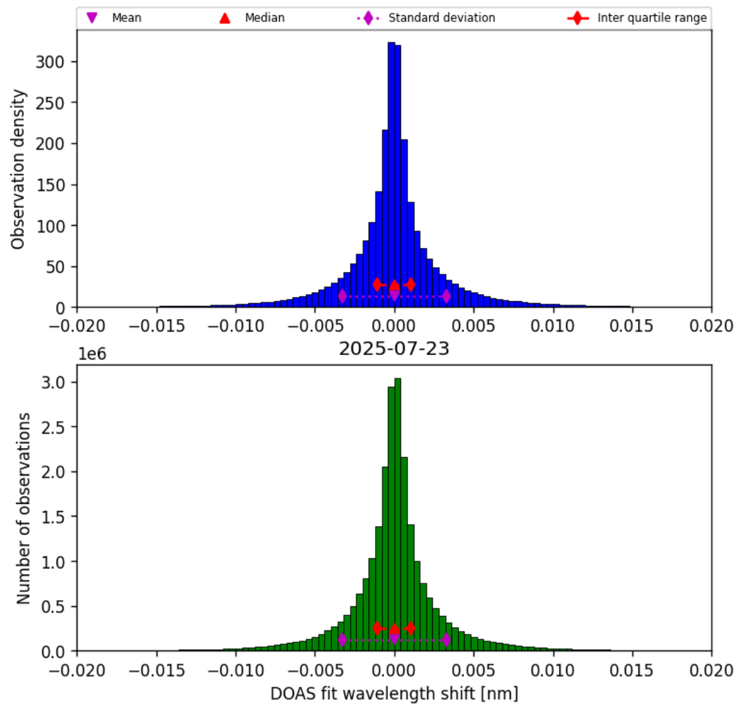
Figure 42: Histogram of “DOAS fit wavelength shift” for 2025-07-23 to 2025-07-24
