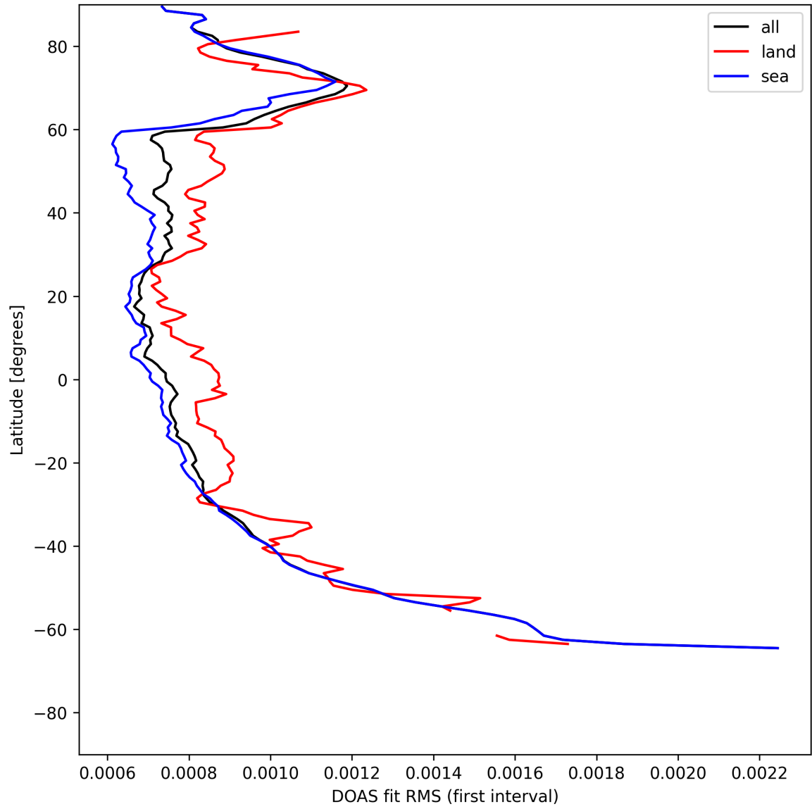
Figure 30: Zonal average of "DOAS fit RMS (first interval)" for 2025-07-23 to 2025-07-24.
