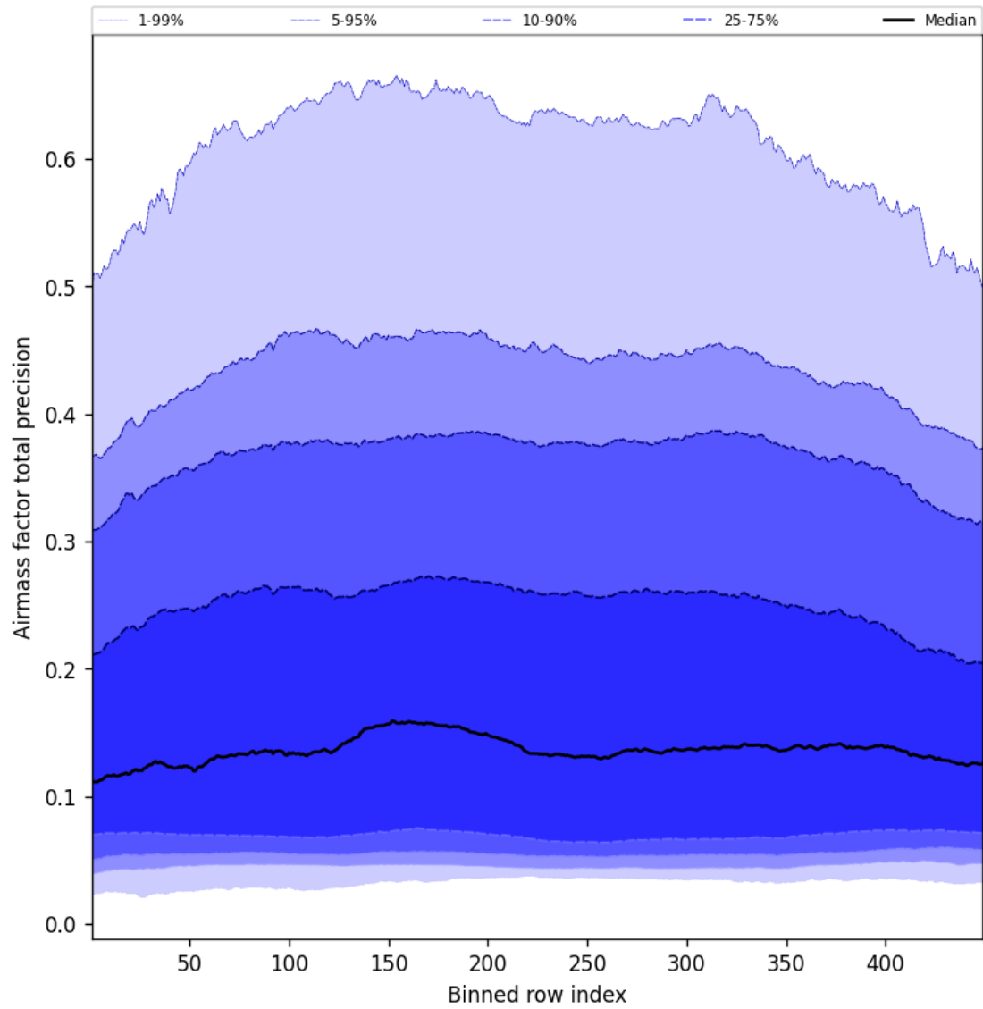
Figure 53: Along track statistics of “Airmass factor total precision” for 2025-07-23 to 2025-07-24
