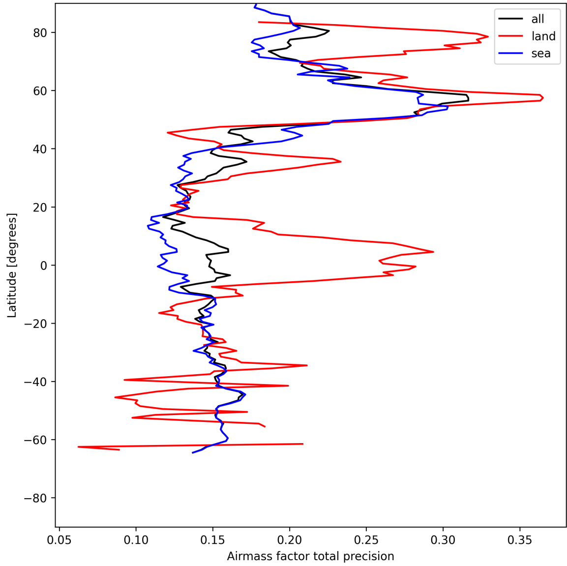
Figure 25: Zonal average of “Airmass factor total precision” for 2025-07-23 to 2025-07-24.
