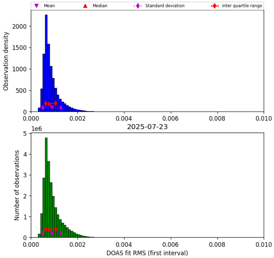
Figure 44: Histogram of “DOAS fit RMS (first interval)” for 2025-07-23 to 2025-07-24
