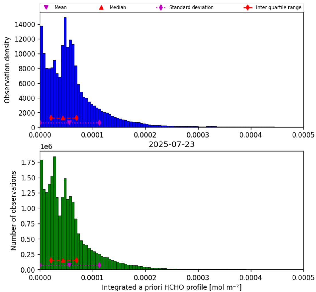
Figure 41: Histogram of “Integrated a priori HCHO profile” for 2025-07-23 to 2025-07-24
