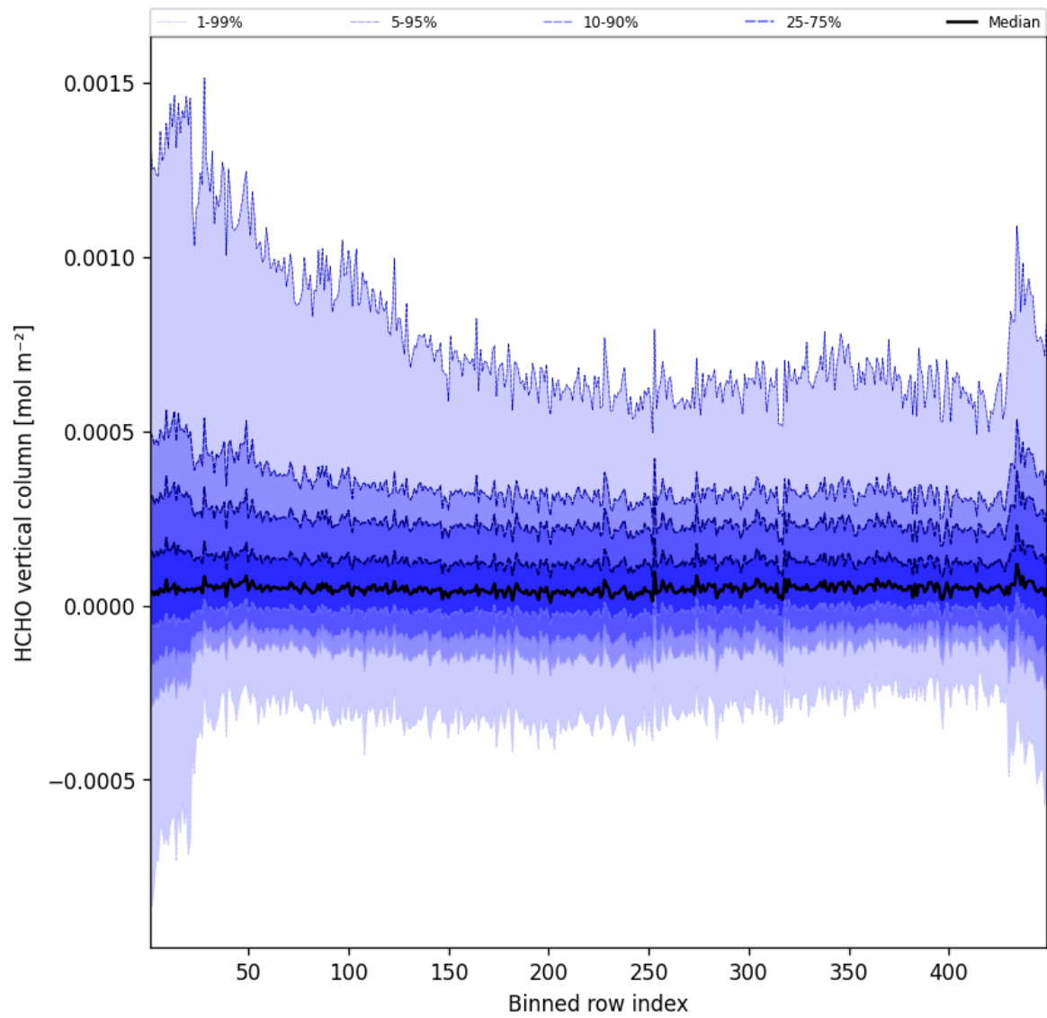
Figure 47: Along track statistics of “HCHO vertical column” for 2025-07-23 to 2025-07-24
