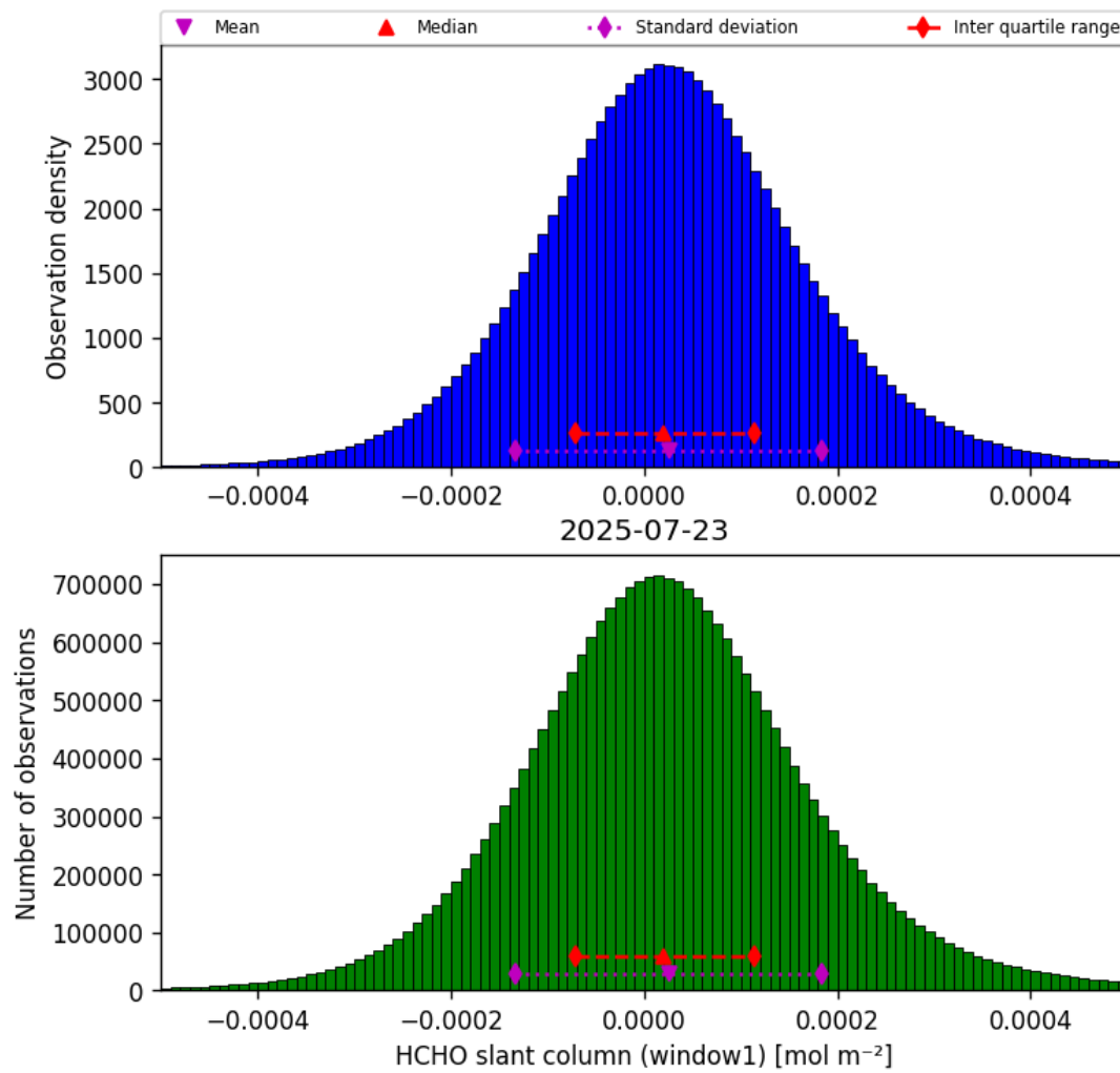
Figure 36: Histogram of “HCHO slant column (window1)” for 2025-07-23 to 2025-07-24
