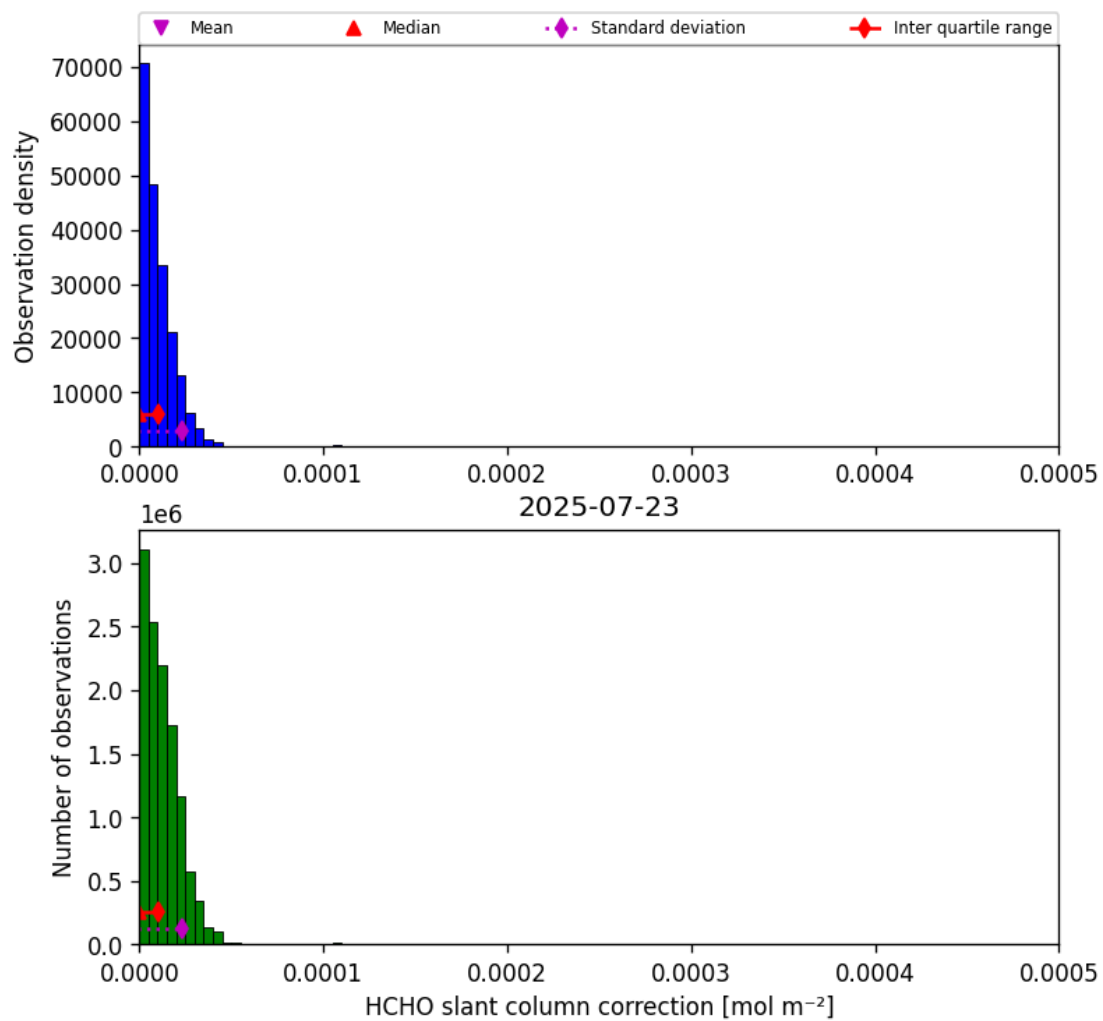
Figure 45: Histogram of “HCHO slant column correction” for 2025-07-23 to 2025-07-24
