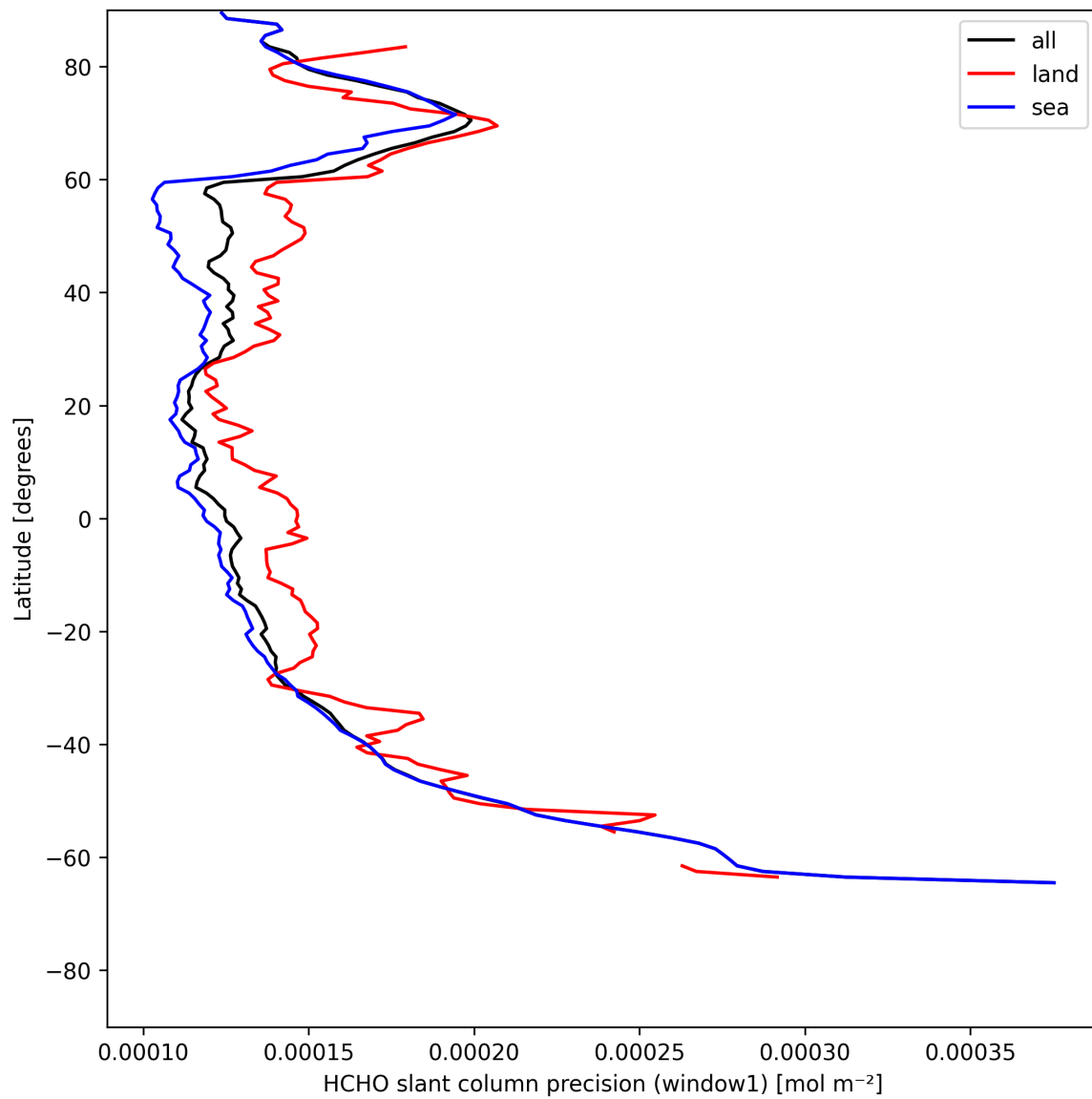
Figure 23: Zonal average of “HCHO slant column precision (window1)” for 2025-07-23 to 2025-07-24.
