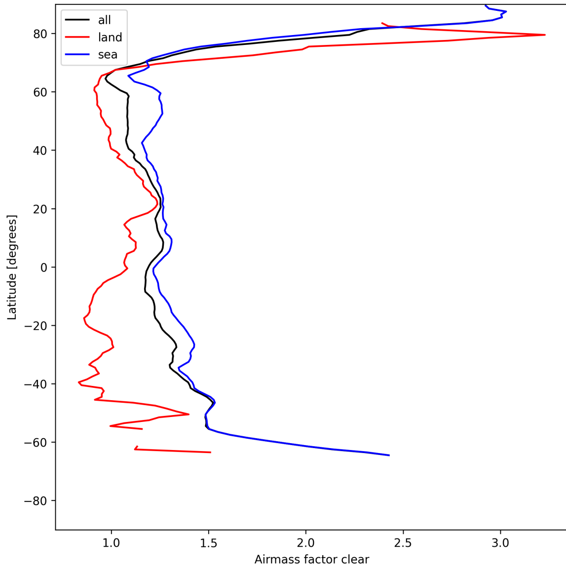
Figure 26: Zonal average of “Airmass factor clear” for 2025-07-23 to 2025-07-24.
