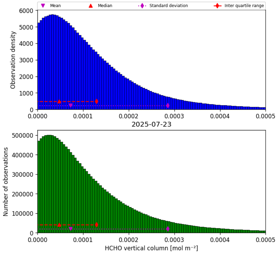
Figure 33: Histogram of “HCHO vertical column” for 2025-07-23 to 2025-07-24
