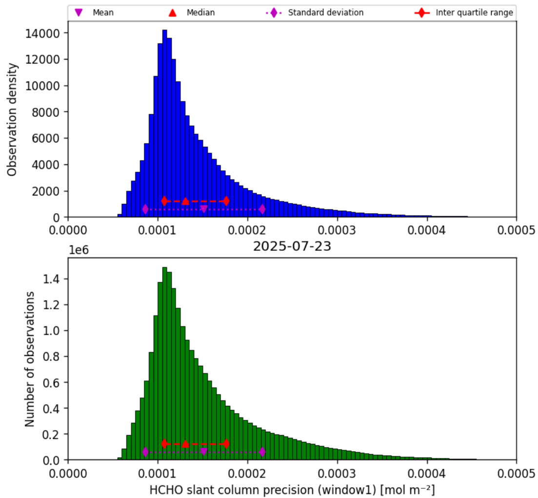
Figure 37: Histogram of “HCHO slant column precision (window1)” for 2025-07-23 to 2025-07-24
