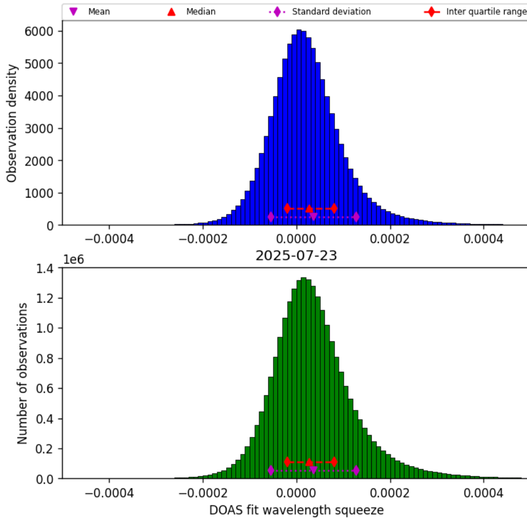
Figure 43: Histogram of “DOAS fit wavelength squeeze” for 2025-07-23 to 2025-07-24
