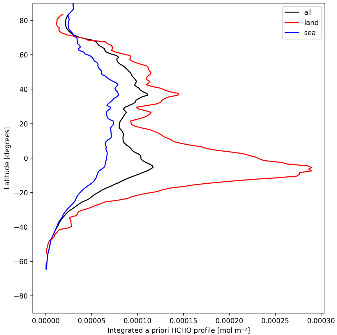
Figure 27: Zonal average of “Integrated a priori HCHO profile” for 2025-07-24 to 2025-07-25.
