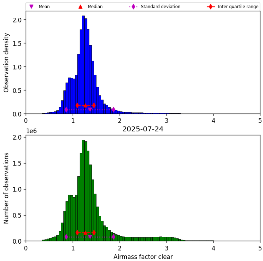
Figure 40: Histogram of “Airmass factor clear” for 2025-07-24 to 2025-07-25
