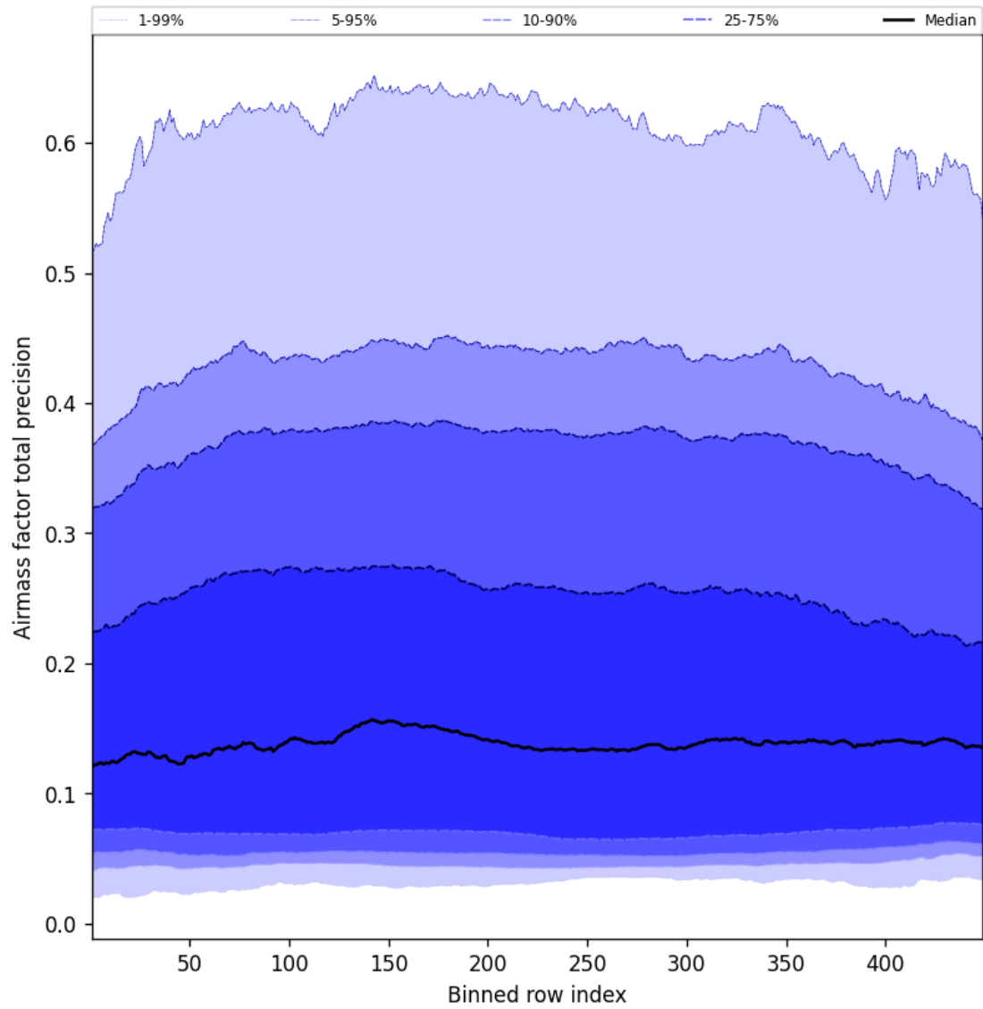
Figure 53: Along track statistics of “Airmass factor total precision” for 2025-07-24 to 2025-07-25
