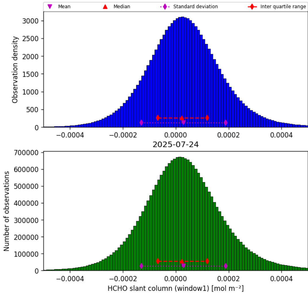
Figure 36: Histogram of “HCHO slant column (window1)” for 2025-07-24 to 2025-07-25
