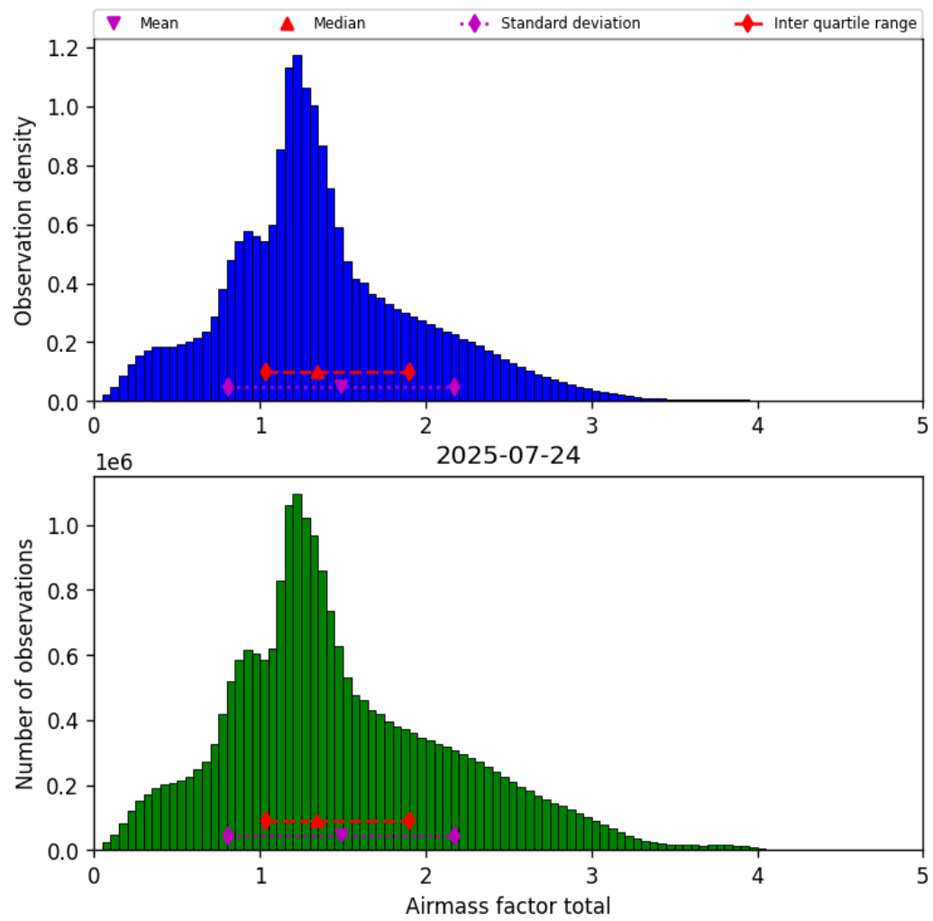
Figure 38: Histogram of “Airmass factor total” for 2025-07-24 to 2025-07-25
