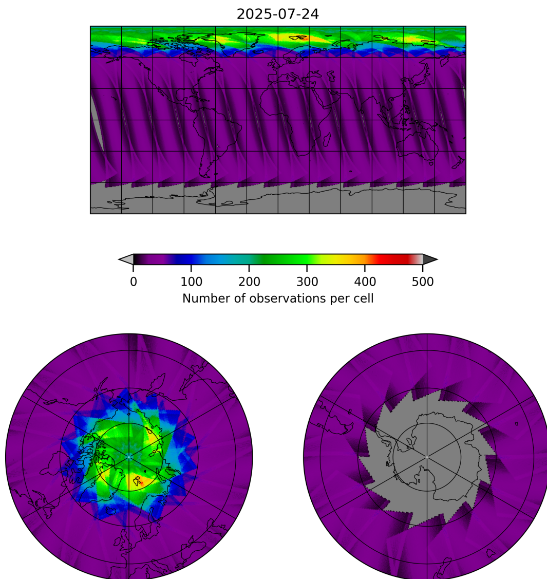
Figure 17: Map of the number of observations for 2025-07-24 to 2025-07-25
