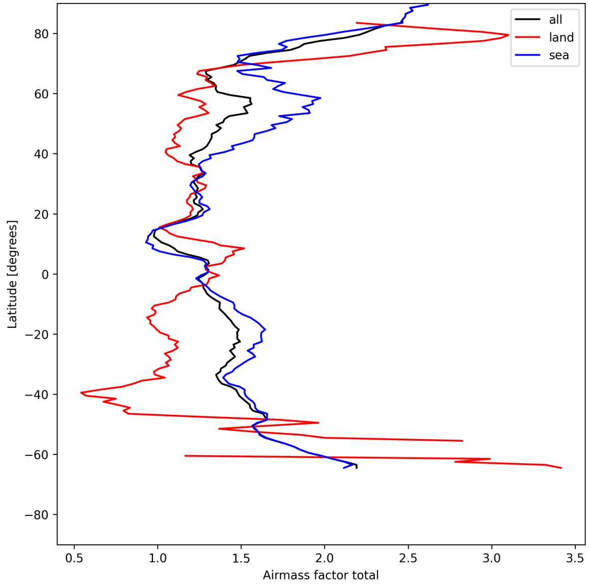
Figure 24: Zonal average of “Airmass factor total” for 2025-07-24 to 2025-07-25.
