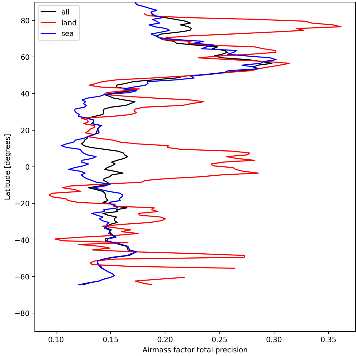
Figure 25: Zonal average of “Airmass factor total precision” for 2025-07-24 to 2025-07-25.
