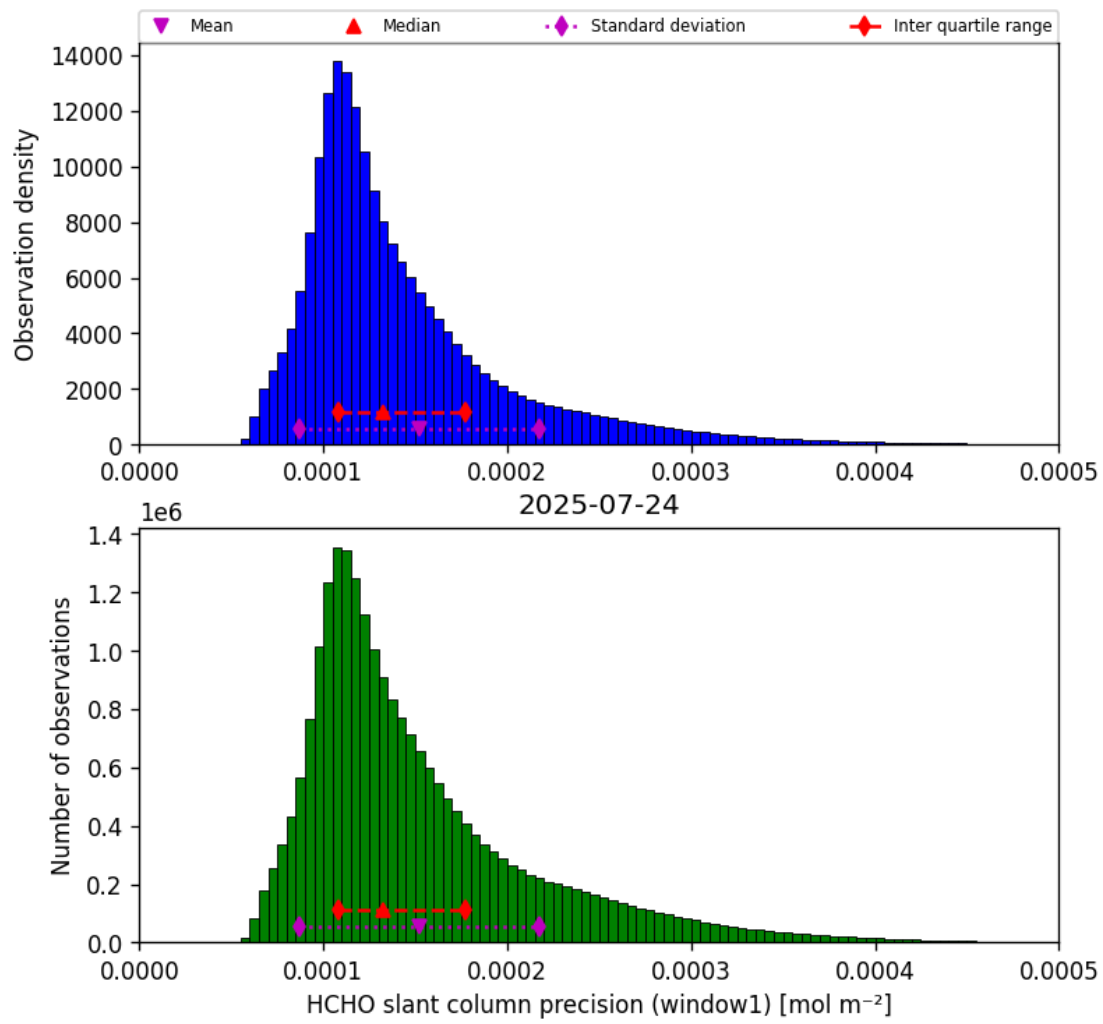
Figure 37: Histogram of “HCHO slant column precision (window1)” for 2025-07-24 to 2025-07-25
