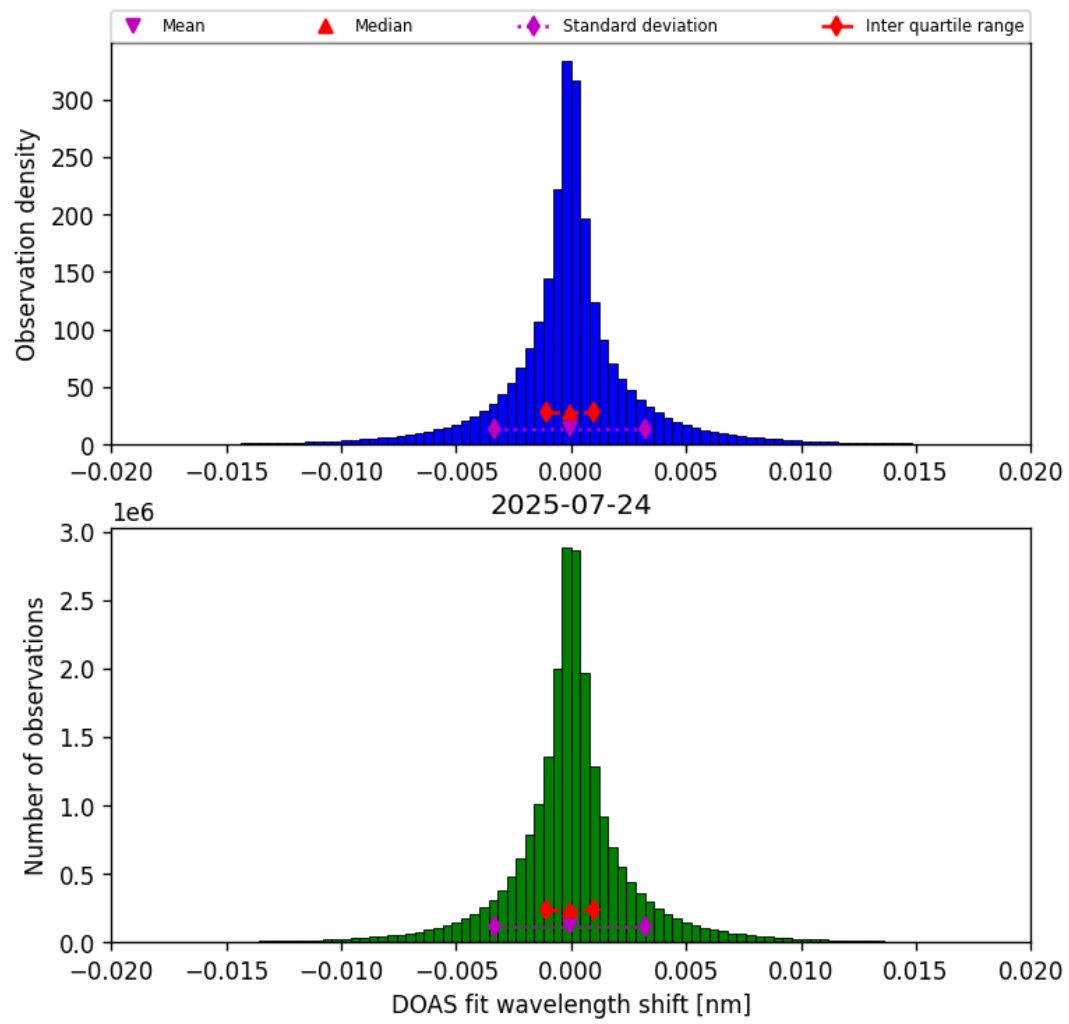
Figure 42: Histogram of “DOAS fit wavelength shift” for 2025-07-24 to 2025-07-25
