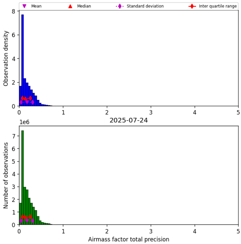
Figure 39: Histogram of “Airmass factor total precision” for 2025-07-24 to 2025-07-25
