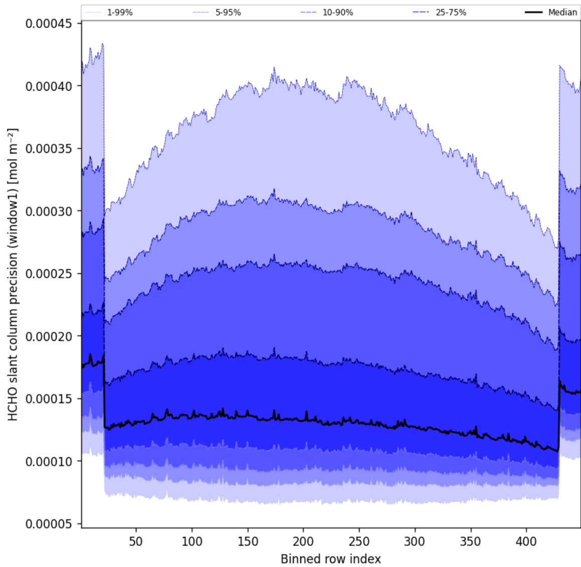
Figure 51: Along track statistics of “HCHO slant column precision (window1)” for 2025-07-24 to 2025-07-25
