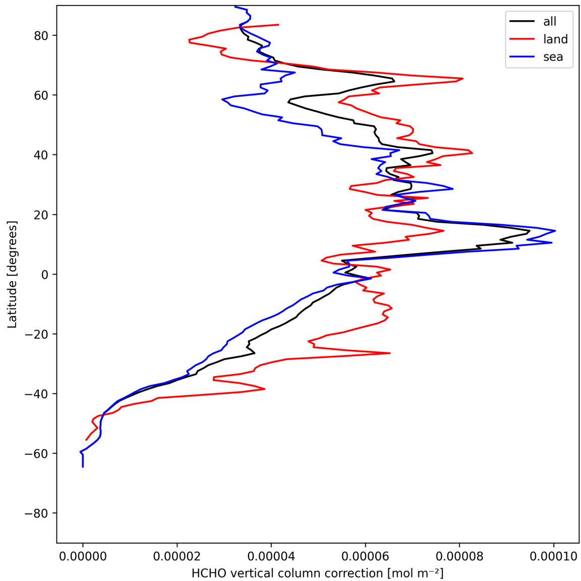
Figure 21: Zonal average of “HCHO vertical column correction” for 2025-07-24 to 2025-07-25.
