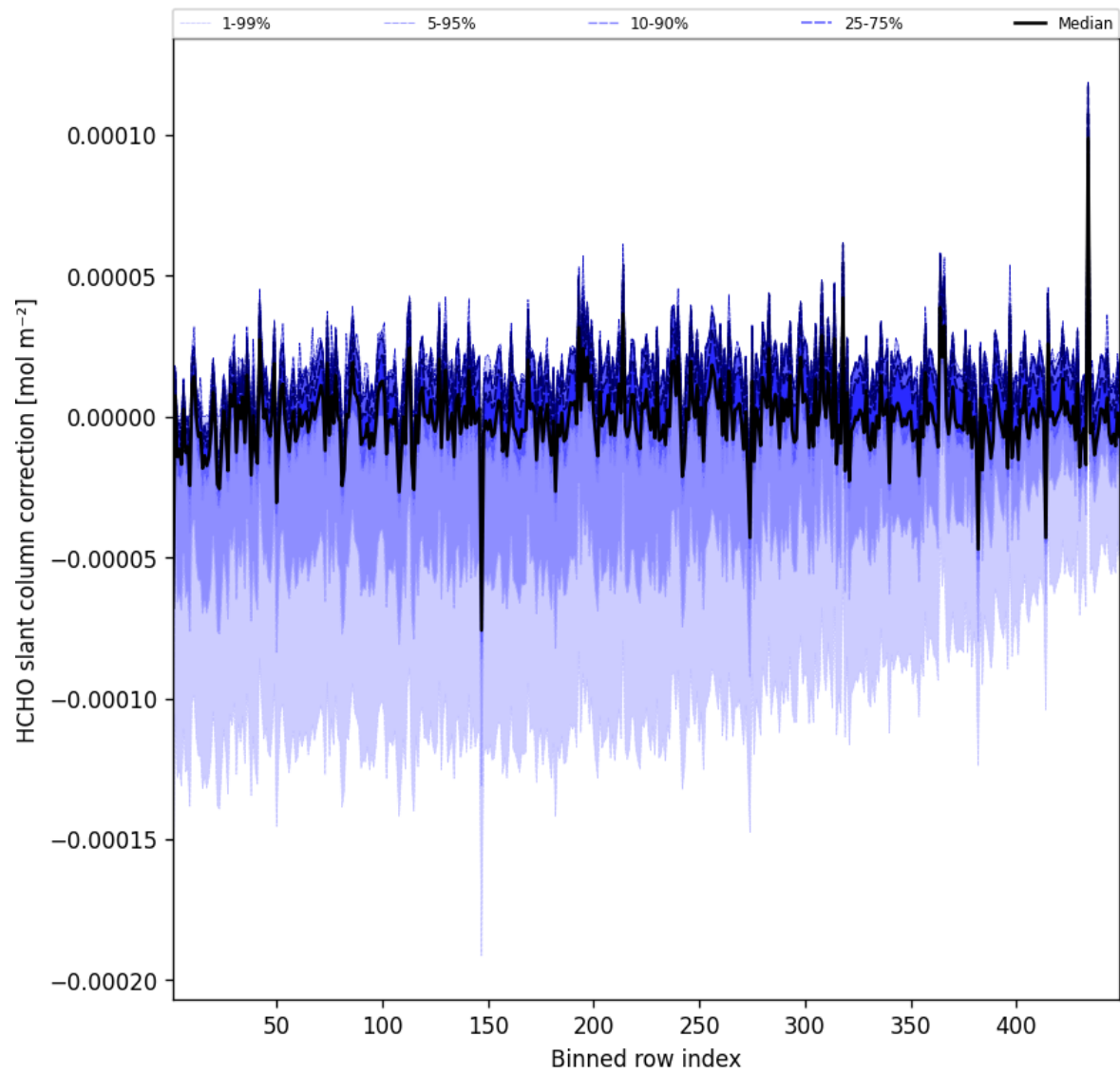
Figure 59: Along track statistics of “HCHO slant column correction” for 2025-07-24 to 2025-07-25
