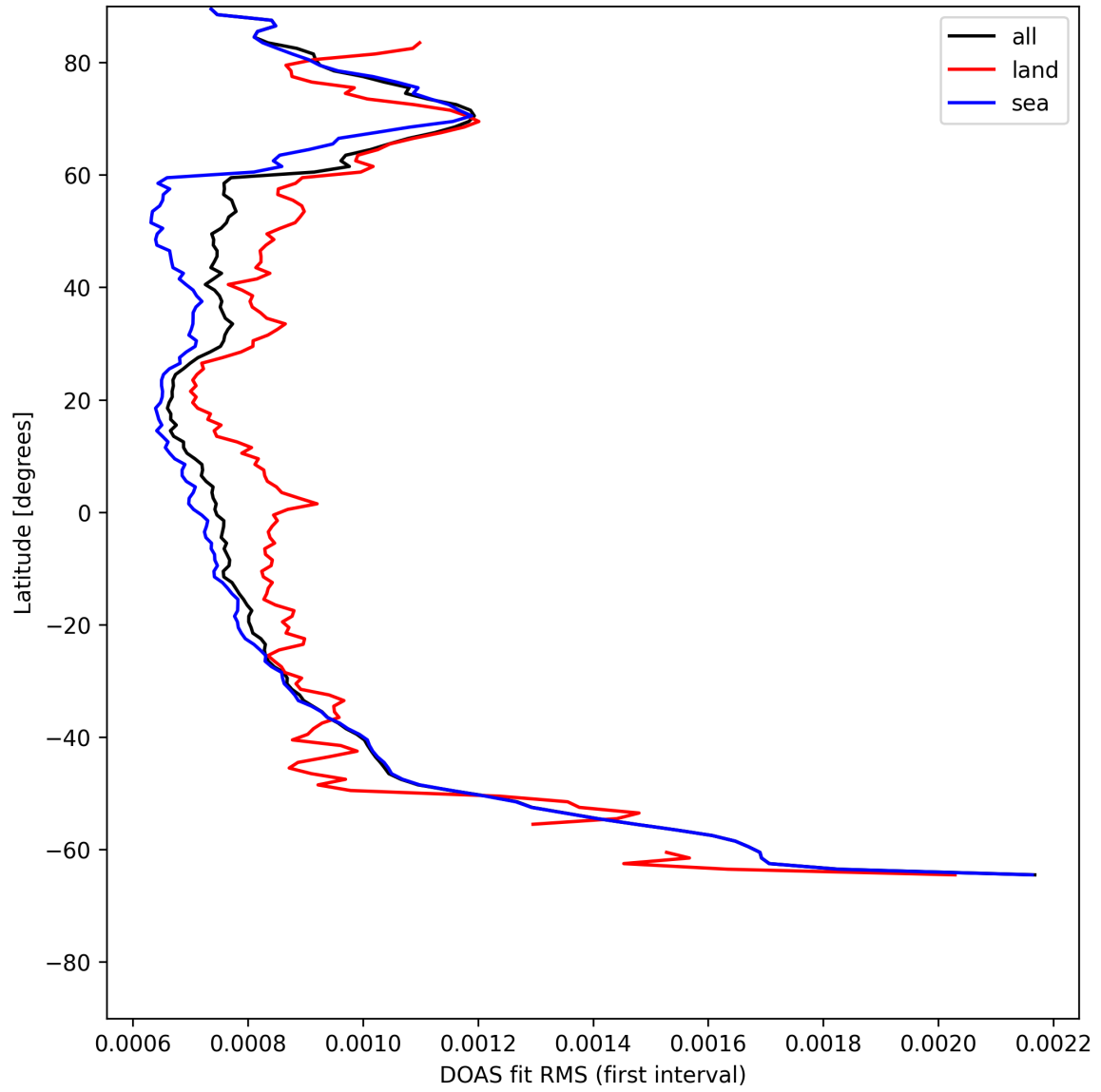
Figure 30: Zonal average of “DOAS fit RMS (first interval)” for 2025-07-24 to 2025-07-25.
