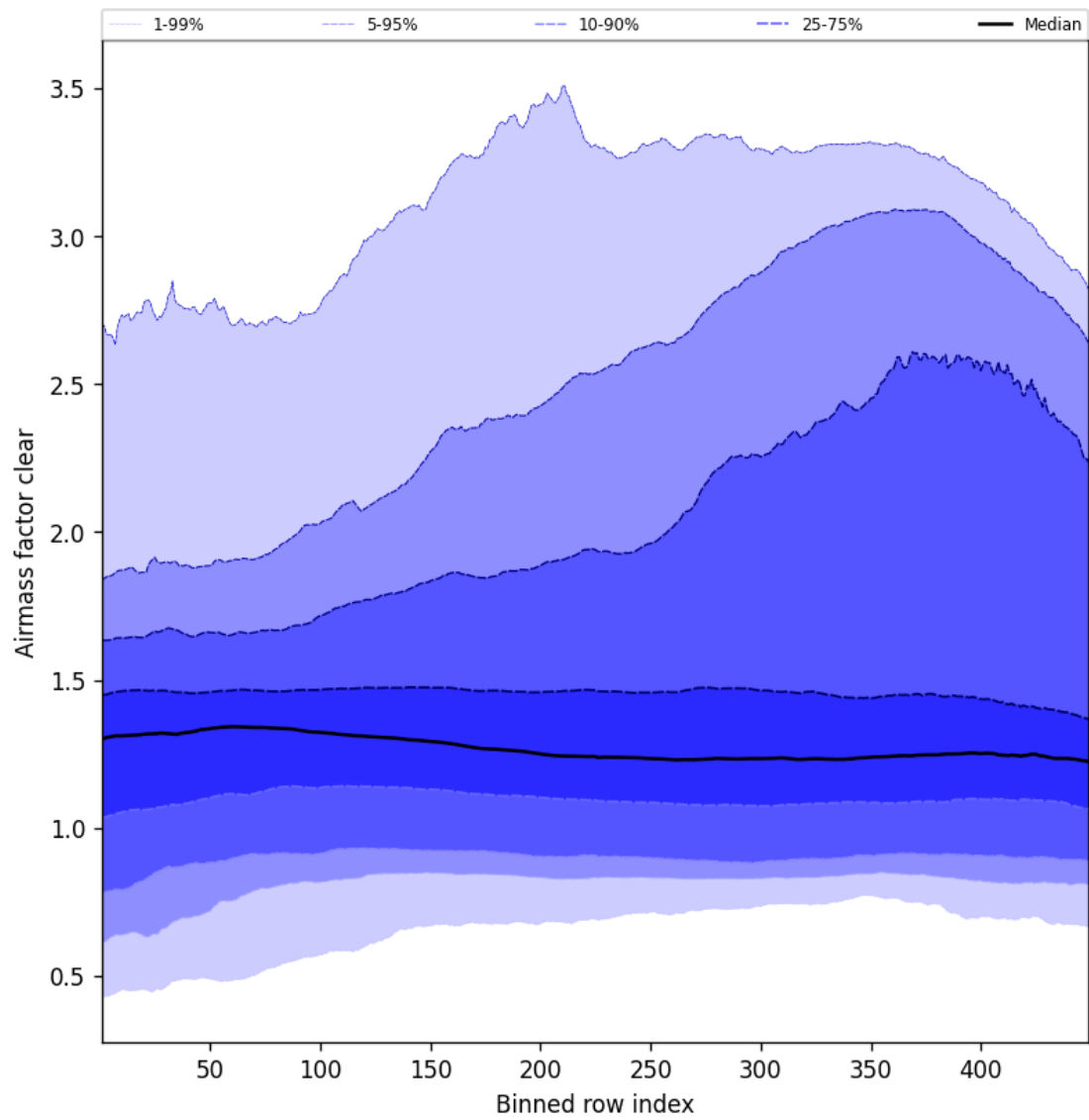
Figure 54: Along track statistics of “Airmass factor clear” for 2025-07-24 to 2025-07-25
