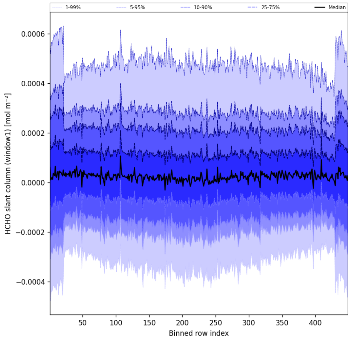
Figure 50: Along track statistics of “HCHO slant column (window1)” for 2025-07-24 to 2025-07-25
