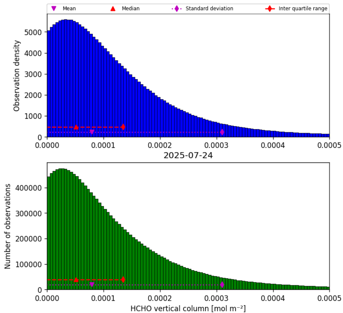
Figure 33: Histogram of “HCHO vertical column” for 2025-07-24 to 2025-07-25
