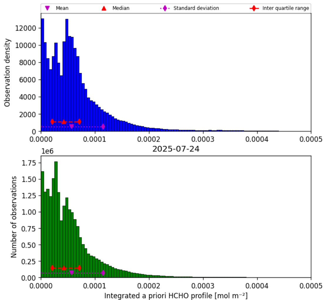
Figure 41: Histogram of “Integrated a priori HCHO profile” for 2025-07-24 to 2025-07-25
