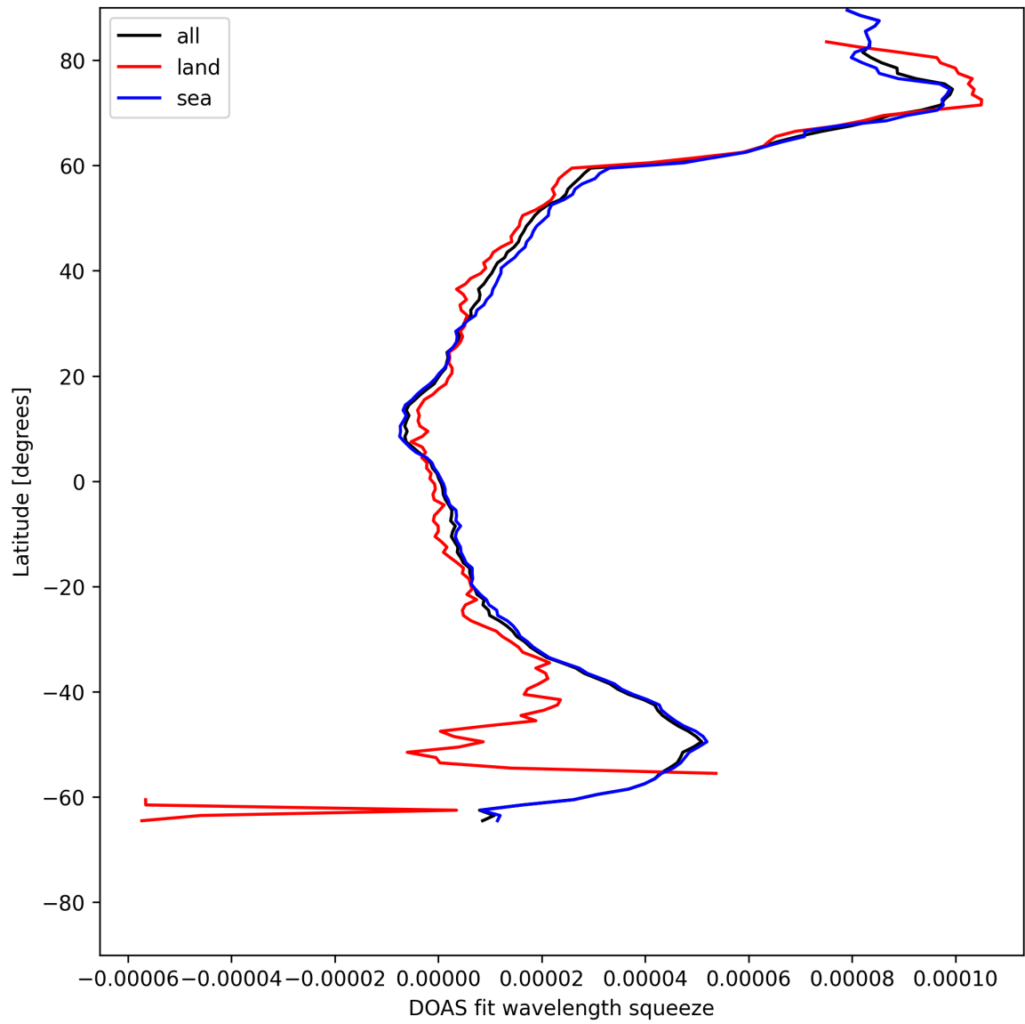
Figure 29: Zonal average of “DOAS fit wavelength squeeze” for 2025-07-24 to 2025-07-25.
