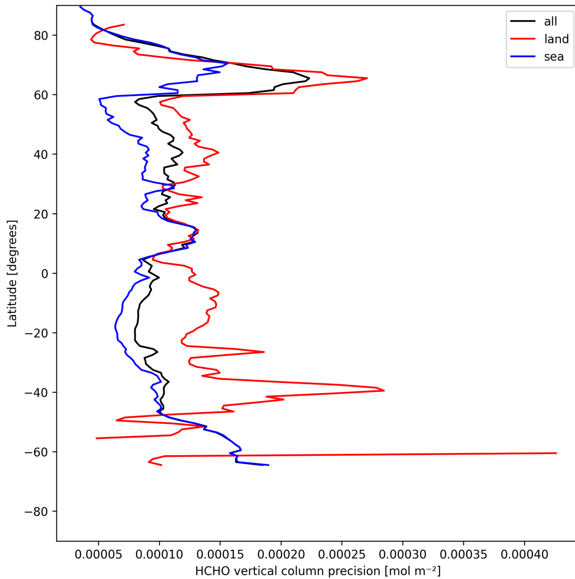
Figure 20: Zonal average of “HCHO vertical column precision” for 2025-07-24 to 2025-07-25.
