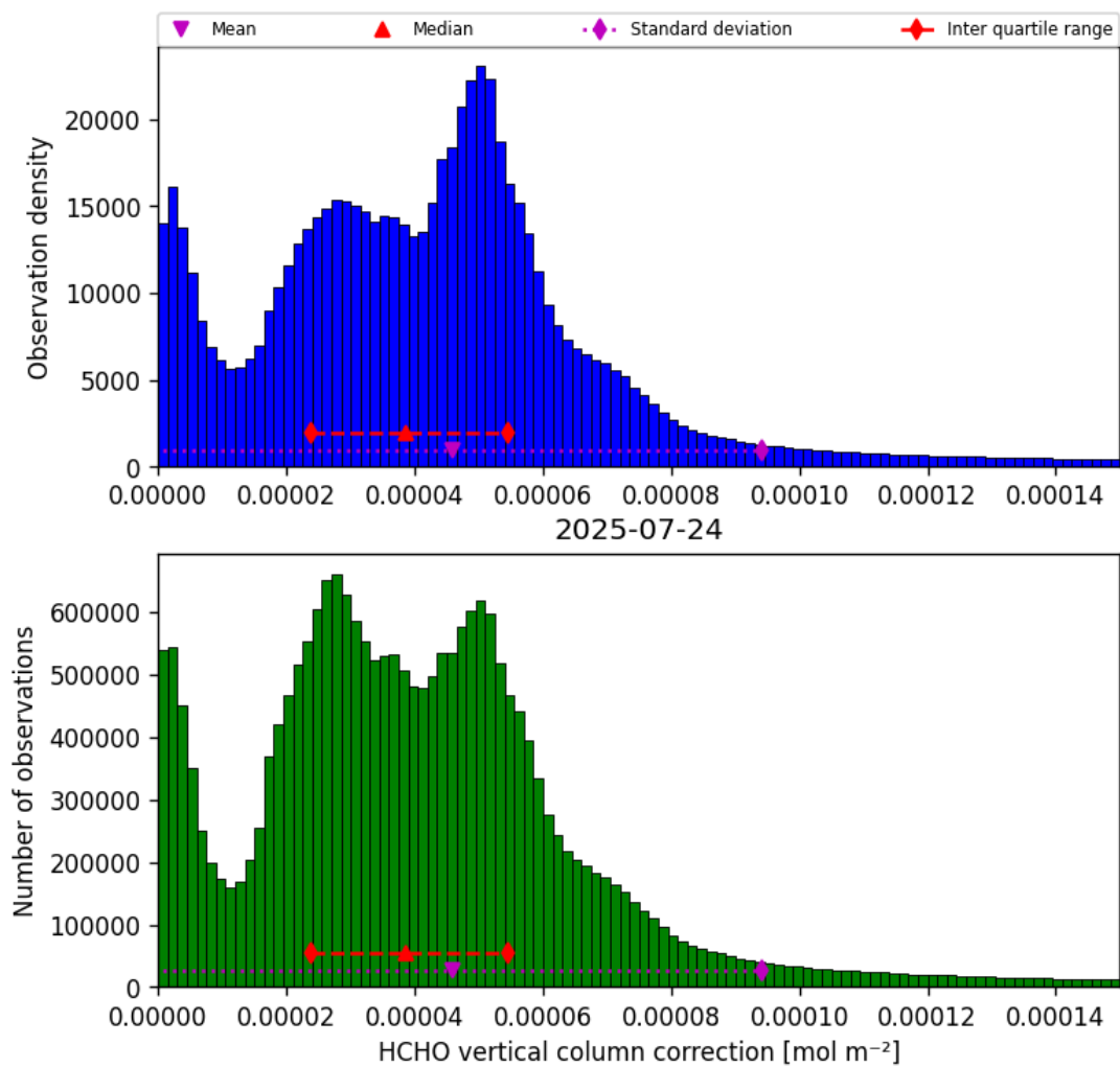
Figure 35: Histogram of “HCHO vertical column correction” for 2025-07-24 to 2025-07-25
