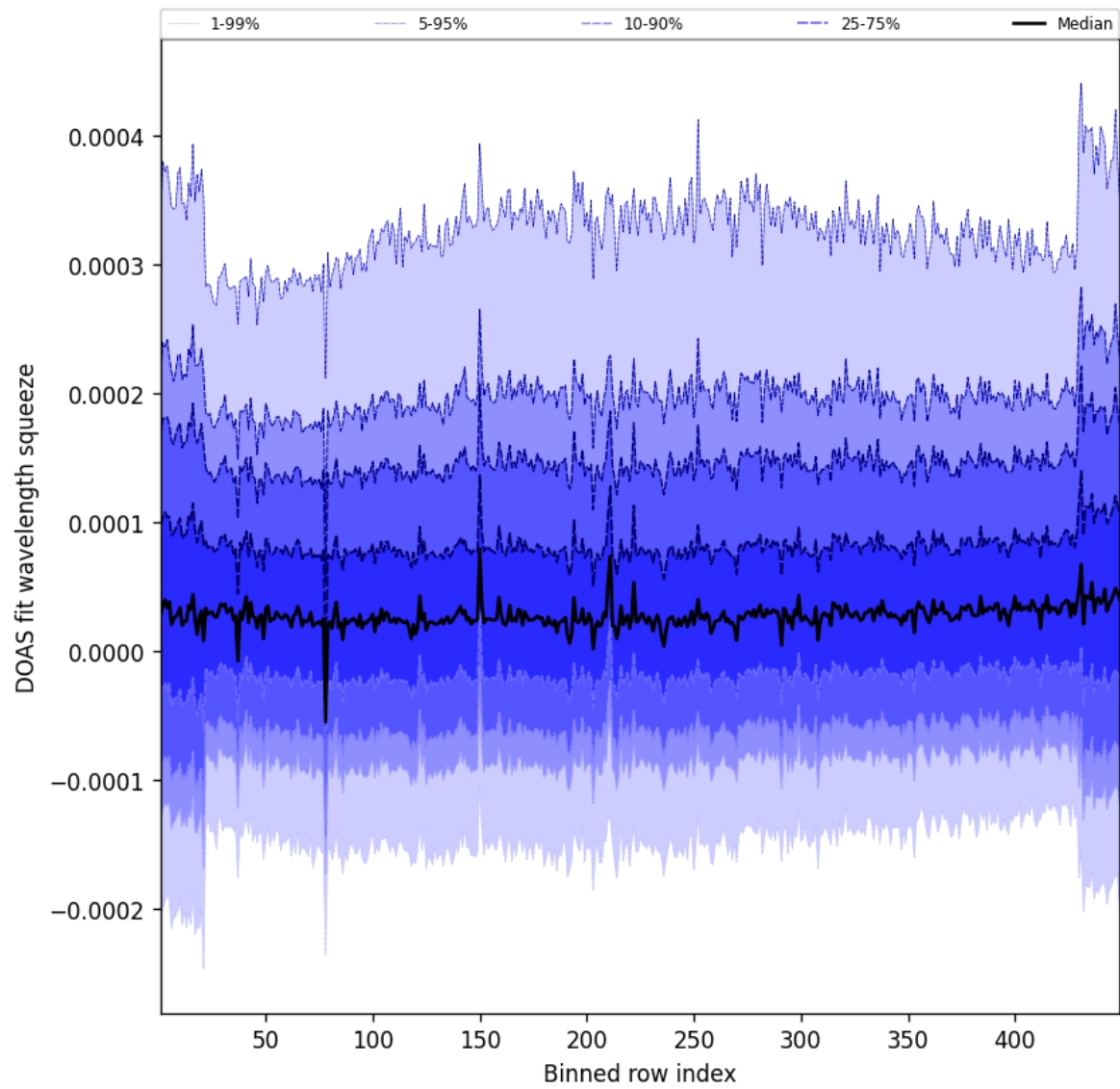
Figure 57: Along track statistics of “DOAS fit wavelength squeeze” for 2025-07-24 to 2025-07-25
