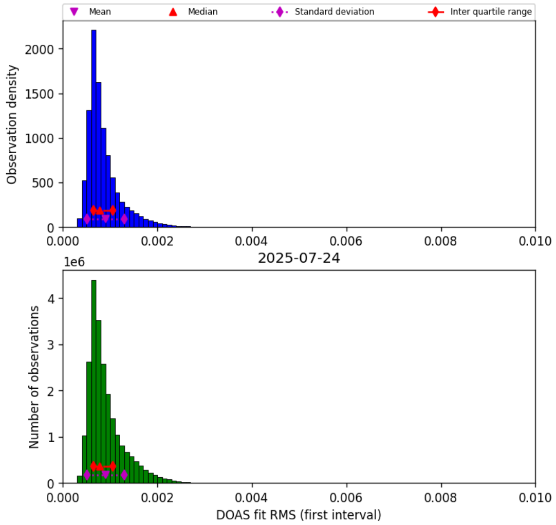
Figure 44: Histogram of “DOAS fit RMS (first interval)” for 2025-07-24 to 2025-07-25
