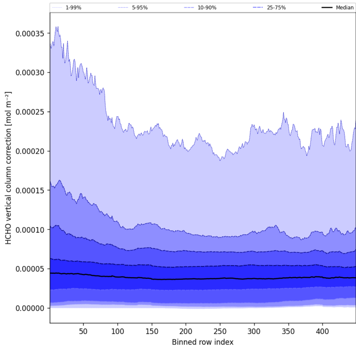
Figure 49: Along track statistics of “HCHO vertical column correction” for 2025-07-24 to 2025-07-25
