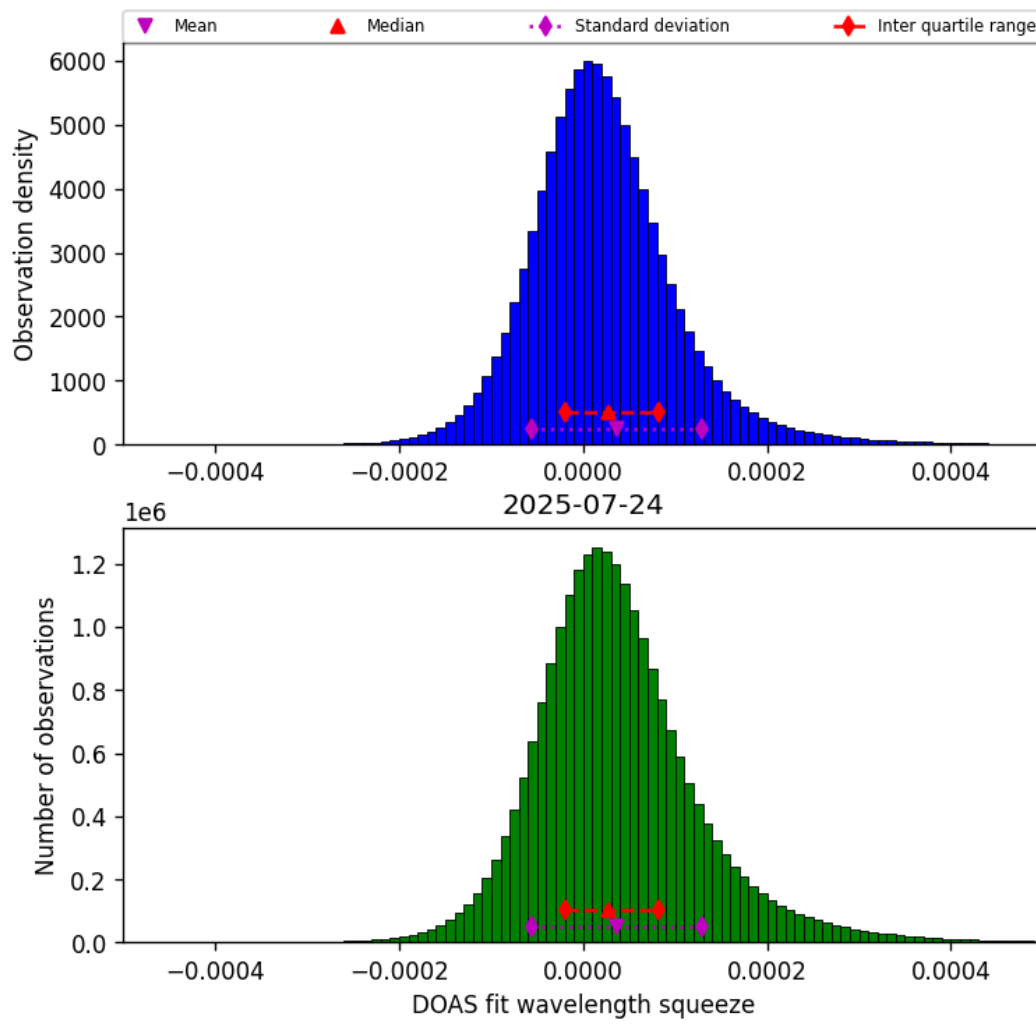
Figure 43: Histogram of “DOAS fit wavelength squeeze” for 2025-07-24 to 2025-07-25
