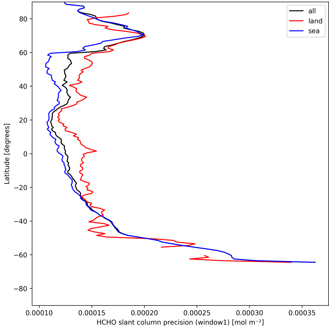
Figure 23: Zonal average of “HCHO slant column precision (window1)” for 2025-07-24 to 2025-07-25.
