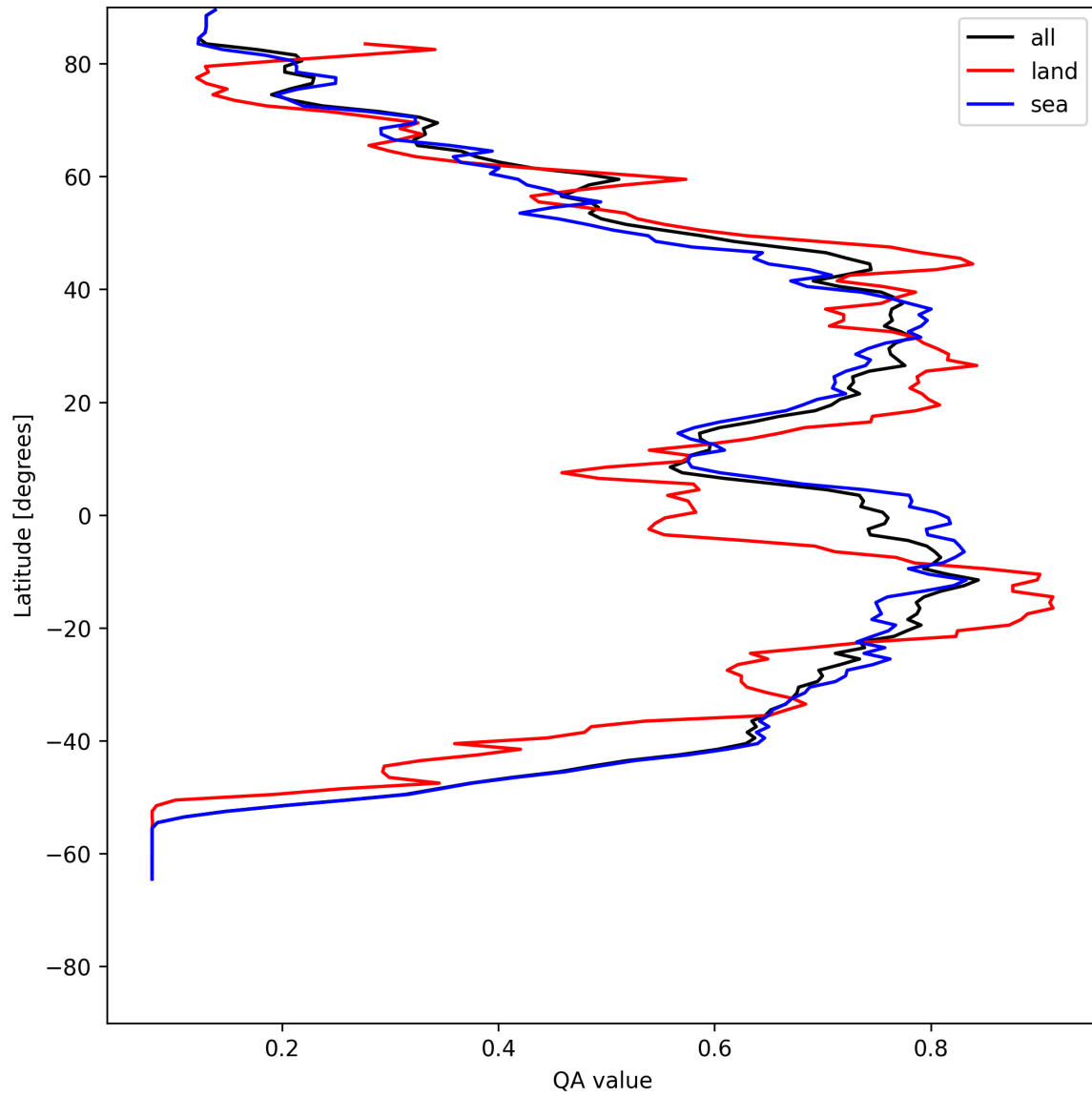
Figure 18: Zonal average of “QA value” for 2025-07-24 to 2025-07-25.
