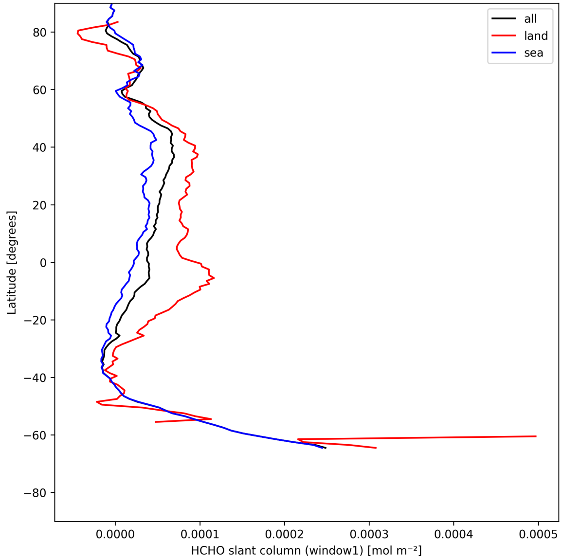
Figure 22: Zonal average of “HCHO slant column (window1)” for 2025-07-24 to 2025-07-25.
