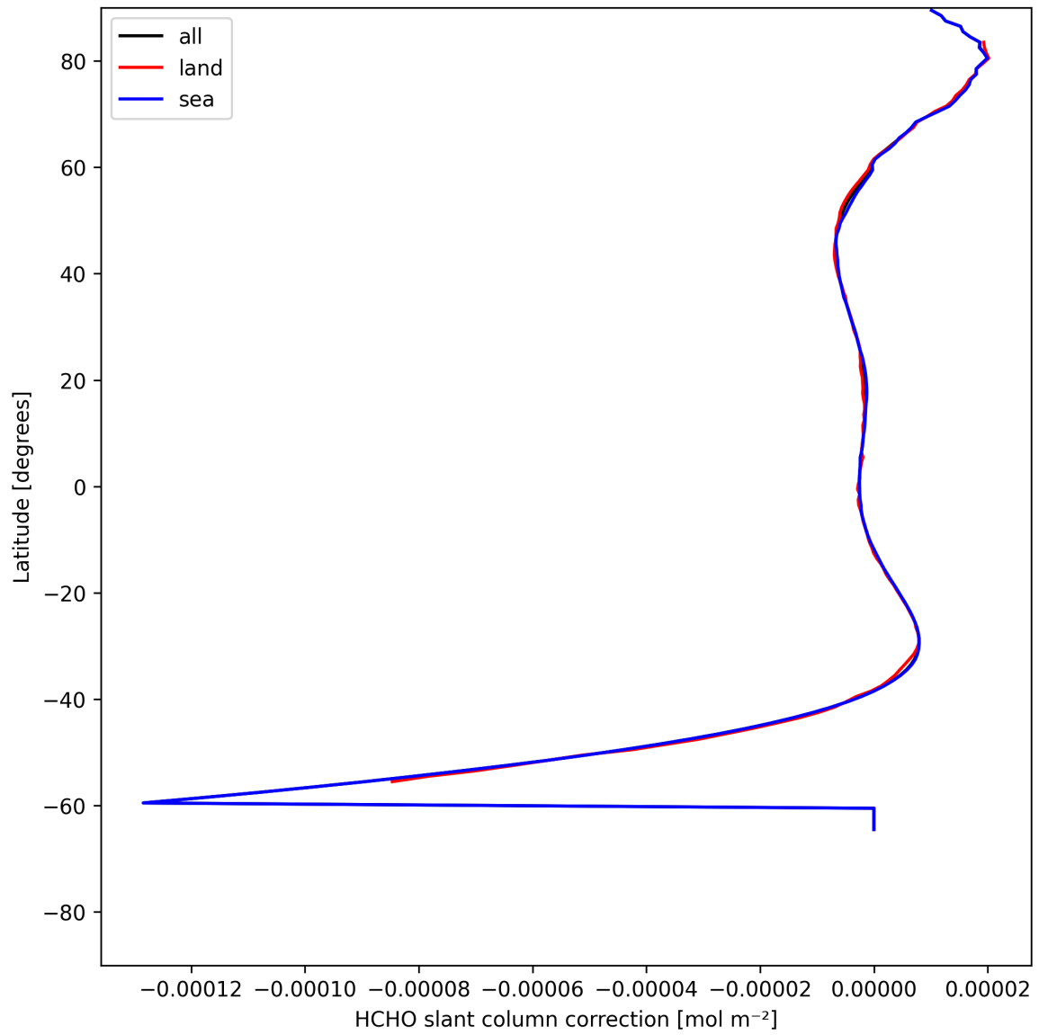
Figure 31: Zonal average of “HCHO slant column correction” for 2025-07-24 to 2025-07-25.
