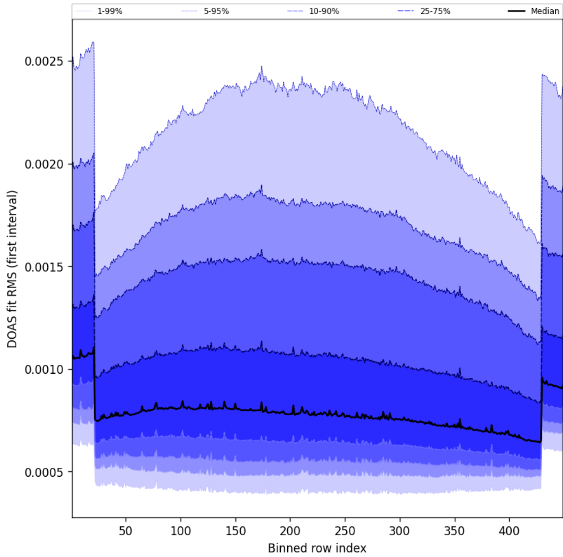
Figure 58: Along track statistics of “DOAS fit RMS (first interval)” for 2025-07-24 to 2025-07-25
