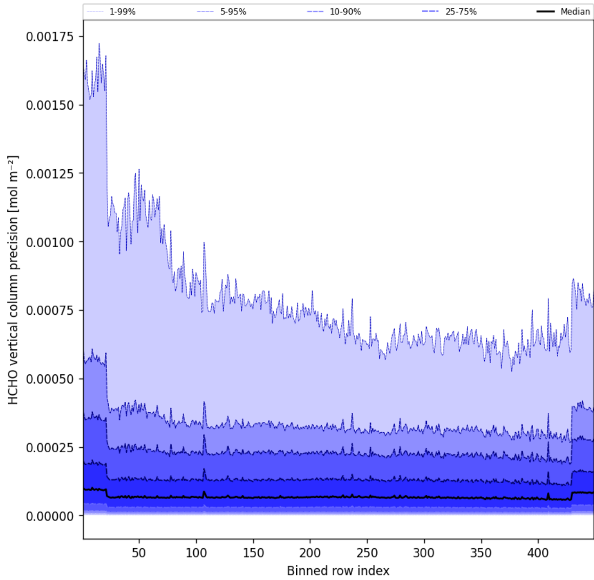
Figure 48: Along track statistics of “HCHO vertical column precision” for 2025-07-24 to 2025-07-25
