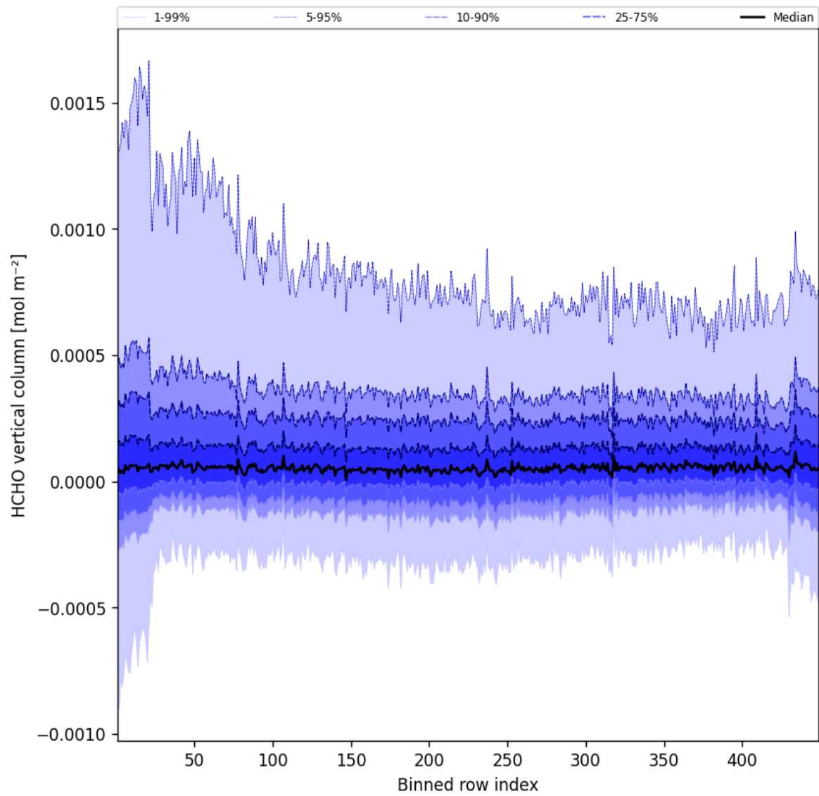
Figure 47: Along track statistics of “HCHO vertical column” for 2025-07-24 to 2025-07-25
