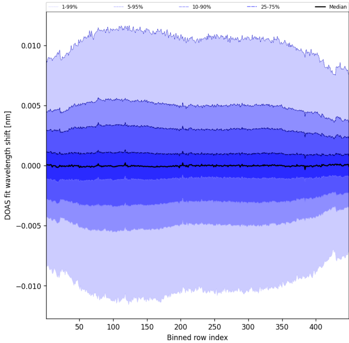
Figure 56: Along track statistics of “DOAS fit wavelength shift” for 2025-07-24 to 2025-07-25
