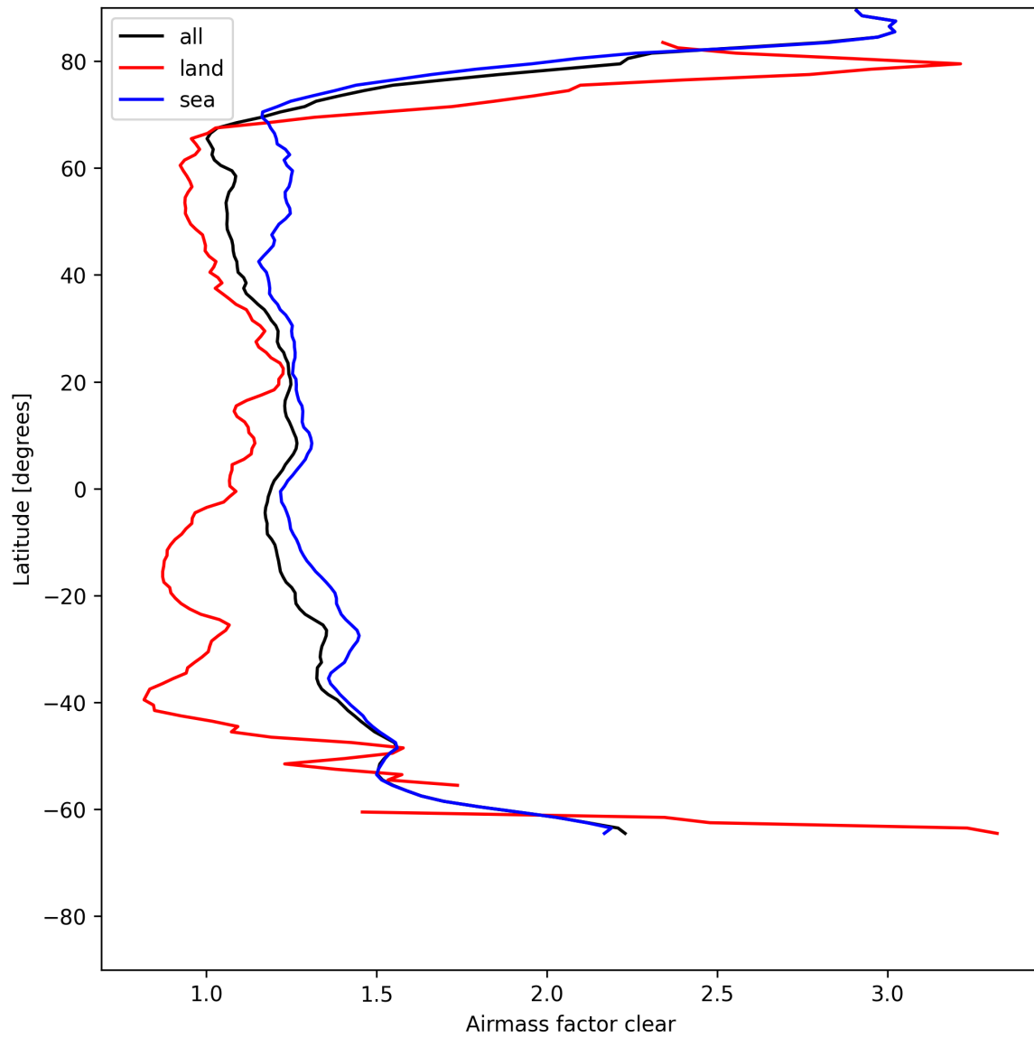
Figure 26: Zonal average of “Airmass factor clear” for 2025-07-24 to 2025-07-25.
