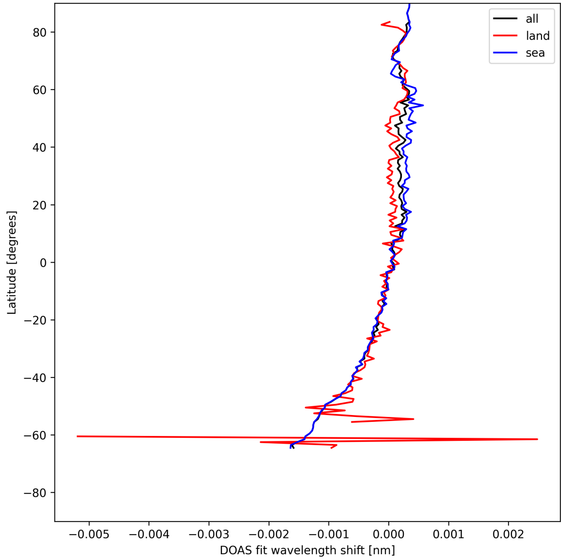
Figure 28: Zonal average of “DOAS fit wavelength shift” for 2025-07-24 to 2025-07-25.
