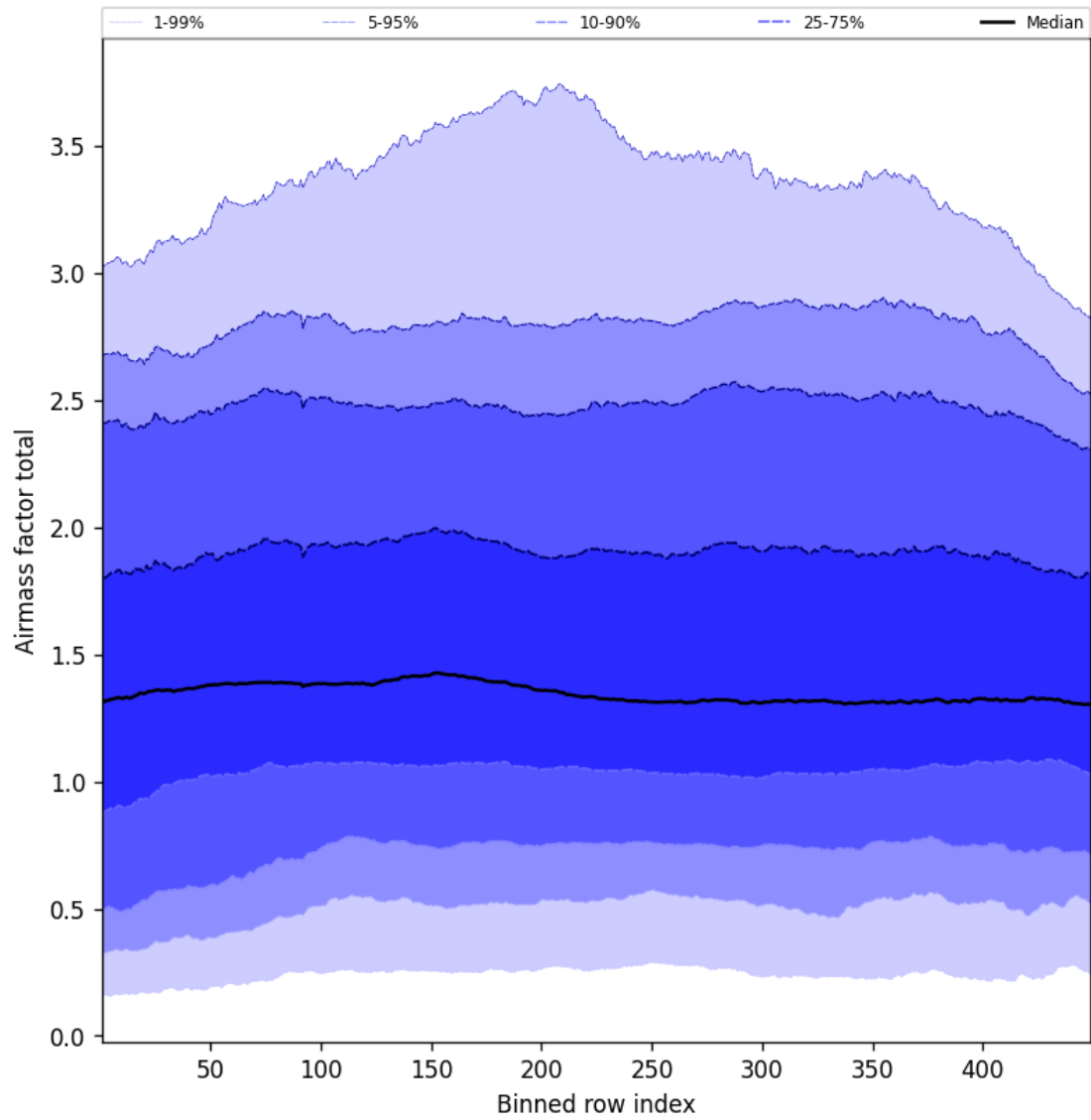
Figure 52: Along track statistics of “Airmass factor total” for 2025-07-24 to 2025-07-25
