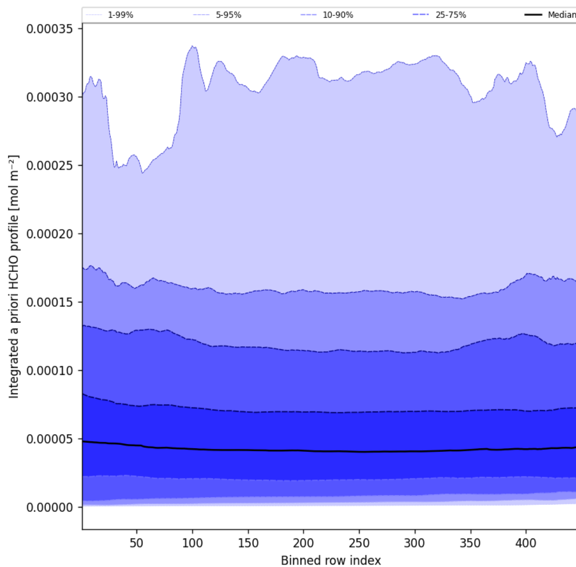
Figure 55: Along track statistics of “Integrated a priori HCHO profile” for 2025-07-24 to 2025-07-25
