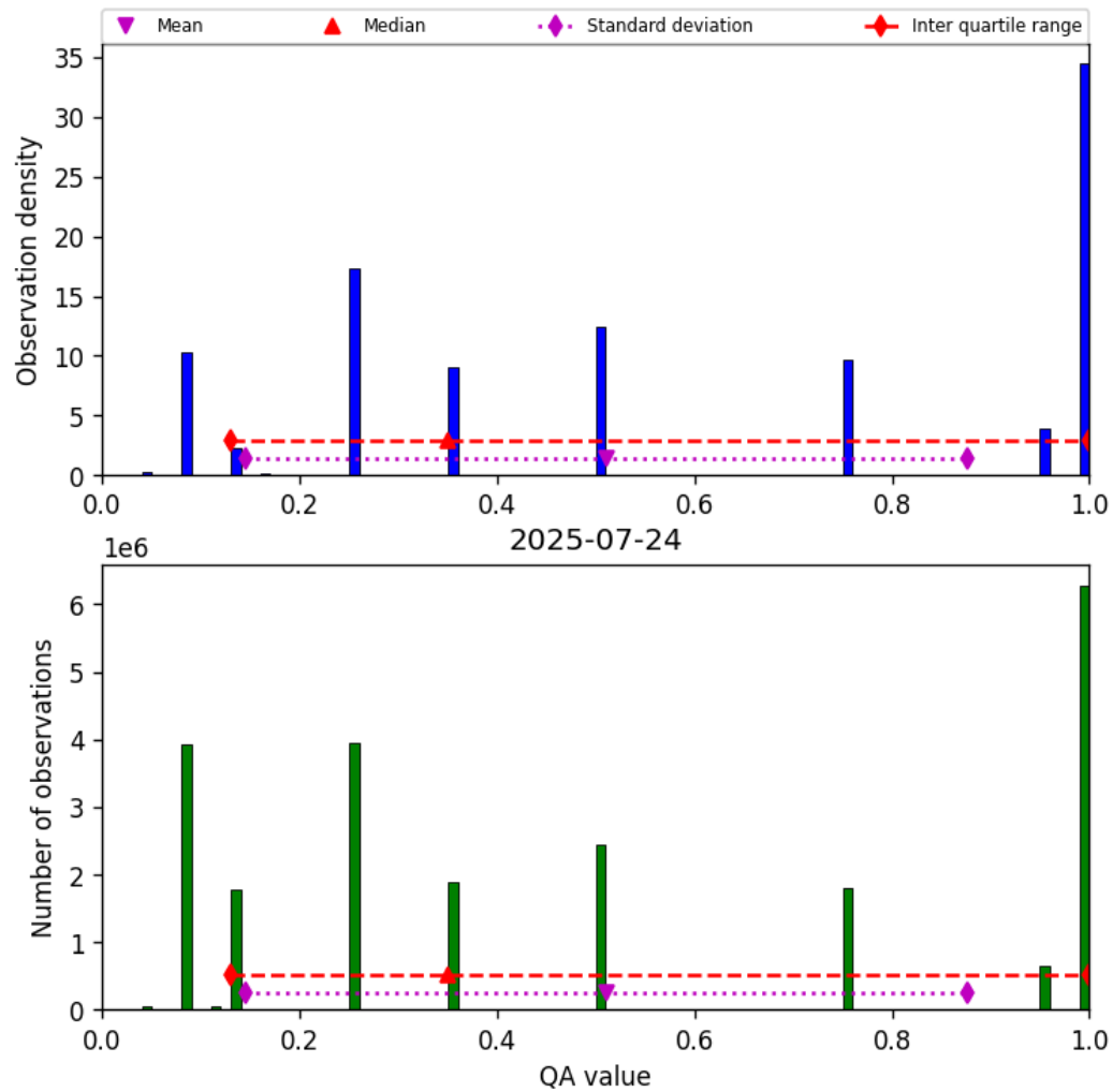
Figure 32: Histogram of “QA value” for 2025-07-24 to 2025-07-25
