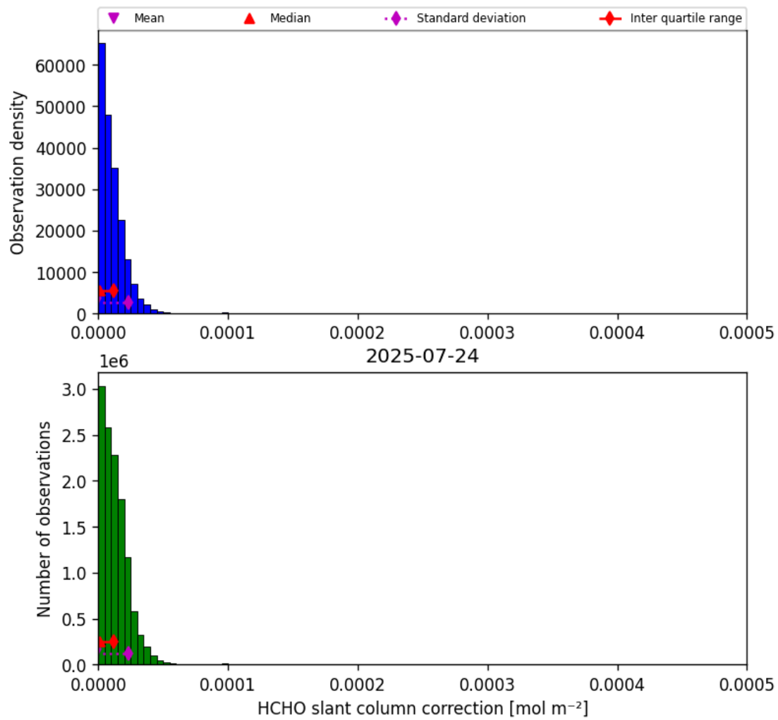
Figure 45: Histogram of “HCHO slant column correction” for 2025-07-24 to 2025-07-25
