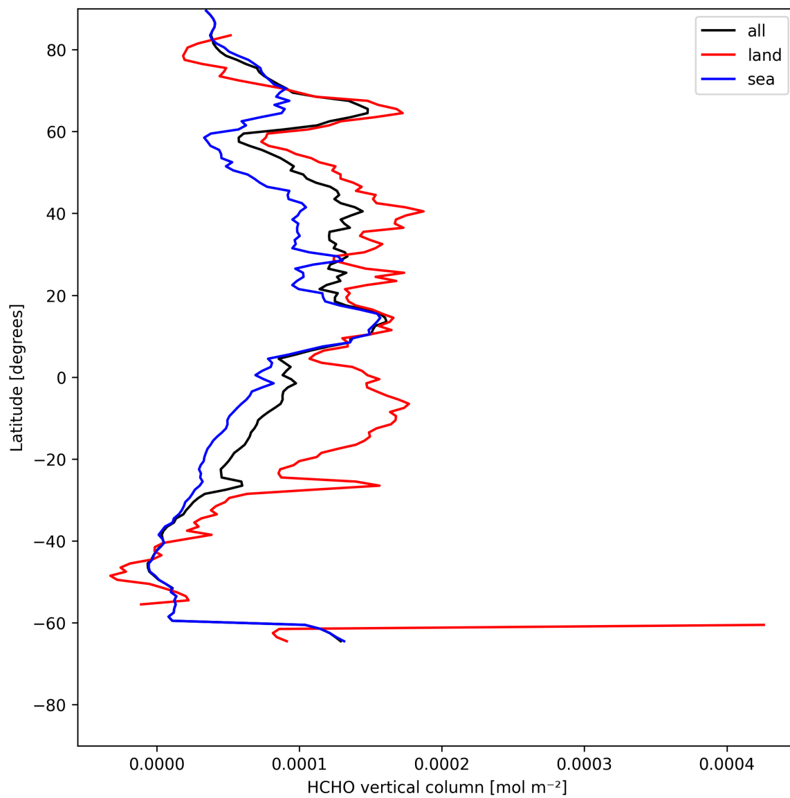
Figure 19: Zonal average of “HCHO vertical column” for 2025-07-24 to 2025-07-25.
