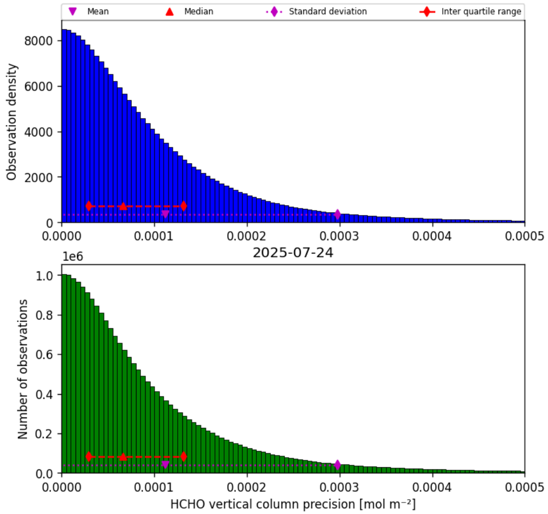
Figure 34: Histogram of “HCHO vertical column precision” for 2025-07-24 to 2025-07-25
