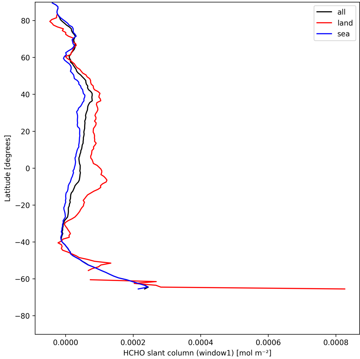
Figure 22: Zonal average of “HCHO slant column (window1)” for 2025-07-25 to 2025-07-26.
