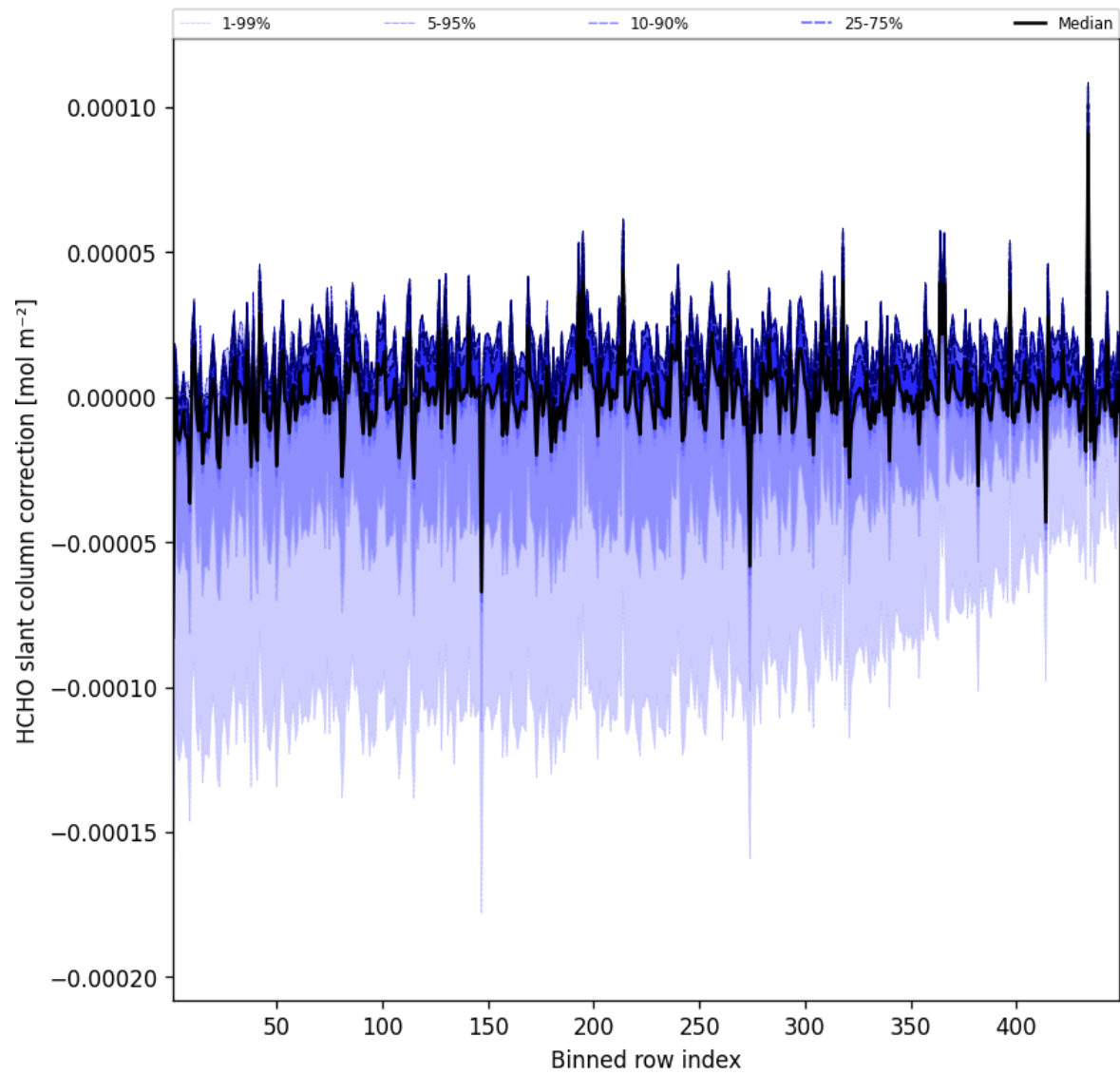
Figure 59: Along track statistics of “HCHO slant column correction” for 2025-07-25 to 2025-07-26
