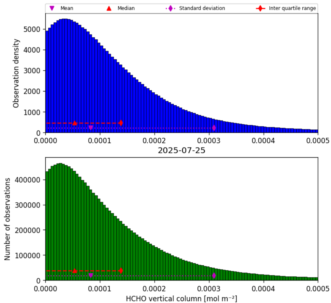
Figure 33: Histogram of “HCHO vertical column” for 2025-07-25 to 2025-07-26
