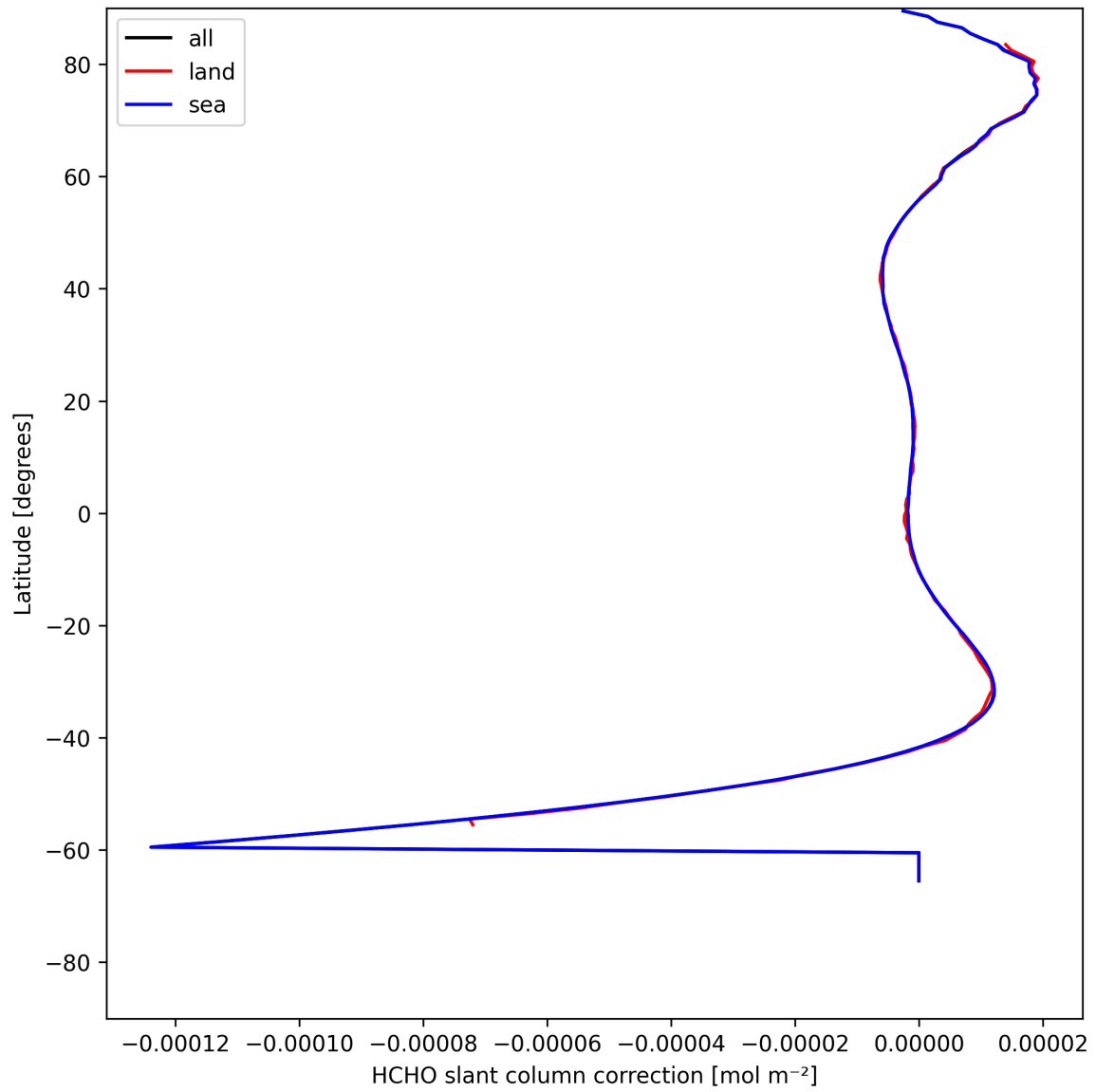
Figure 31: Zonal average of “HCHO slant column correction” for 2025-07-25 to 2025-07-26.
