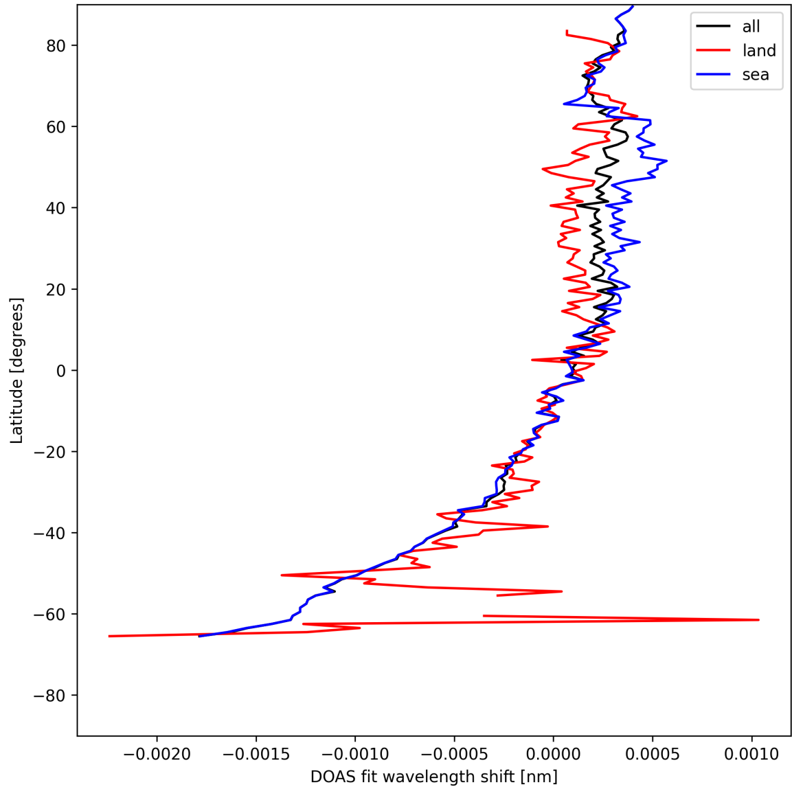
Figure 28: Zonal average of “DOAS fit wavelength shift” for 2025-07-25 to 2025-07-26.
