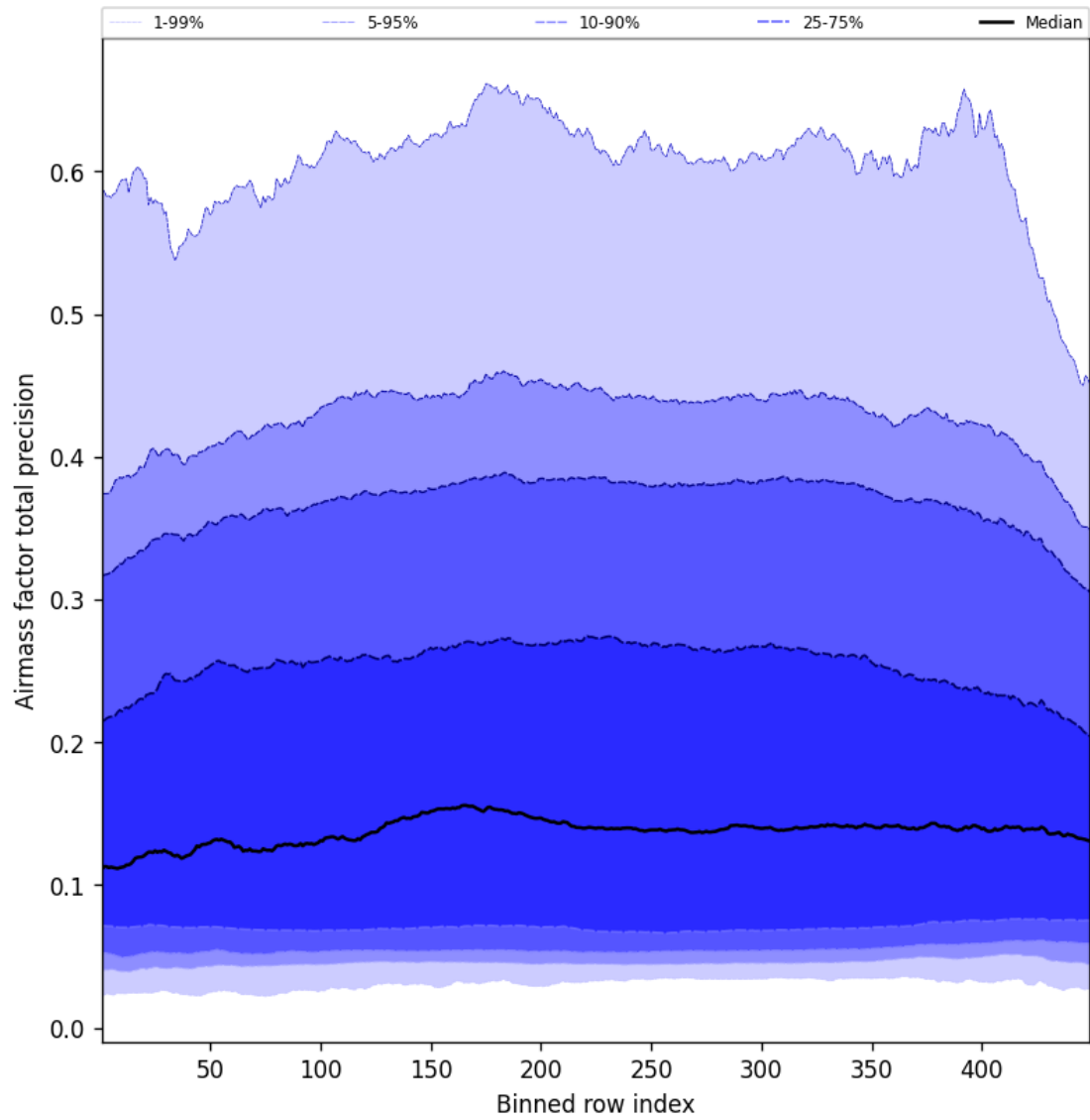
Figure 53: Along track statistics of “Airmass factor total precision” for 2025-07-25 to 2025-07-26
