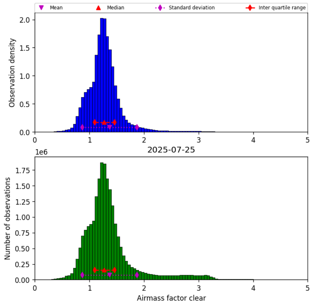
Figure 40: Histogram of “Airmass factor clear” for 2025-07-25 to 2025-07-26
