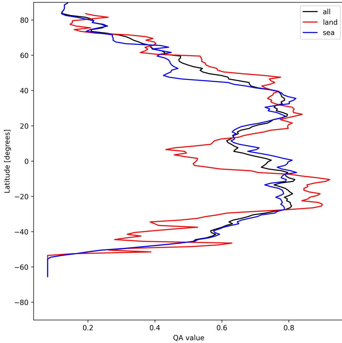
Figure 18: Zonal average of “QA value” for 2025-07-25 to 2025-07-26.
