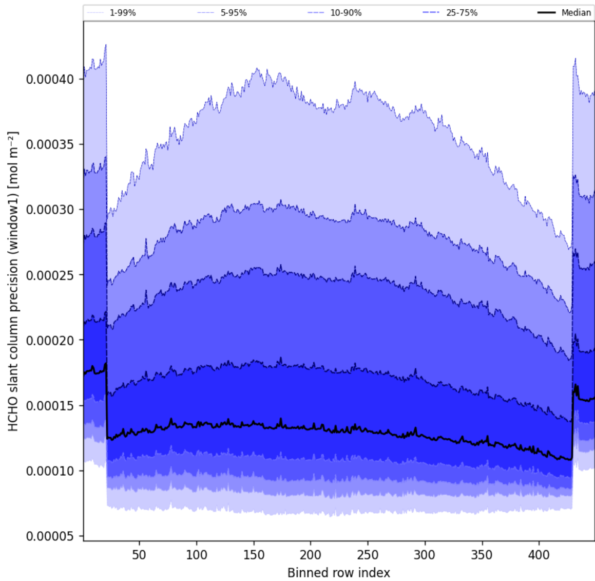
Figure 51: Along track statistics of “HCHO slant column precision (window1)” for 2025-07-25 to 2025-07-26
