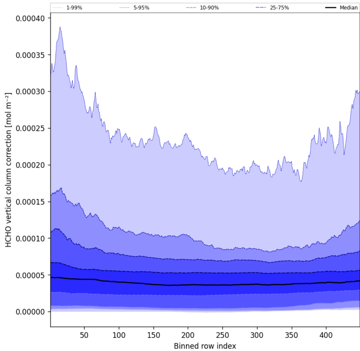
Figure 49: Along track statistics of “HCHO vertical column correction” for 2025-07-25 to 2025-07-26
