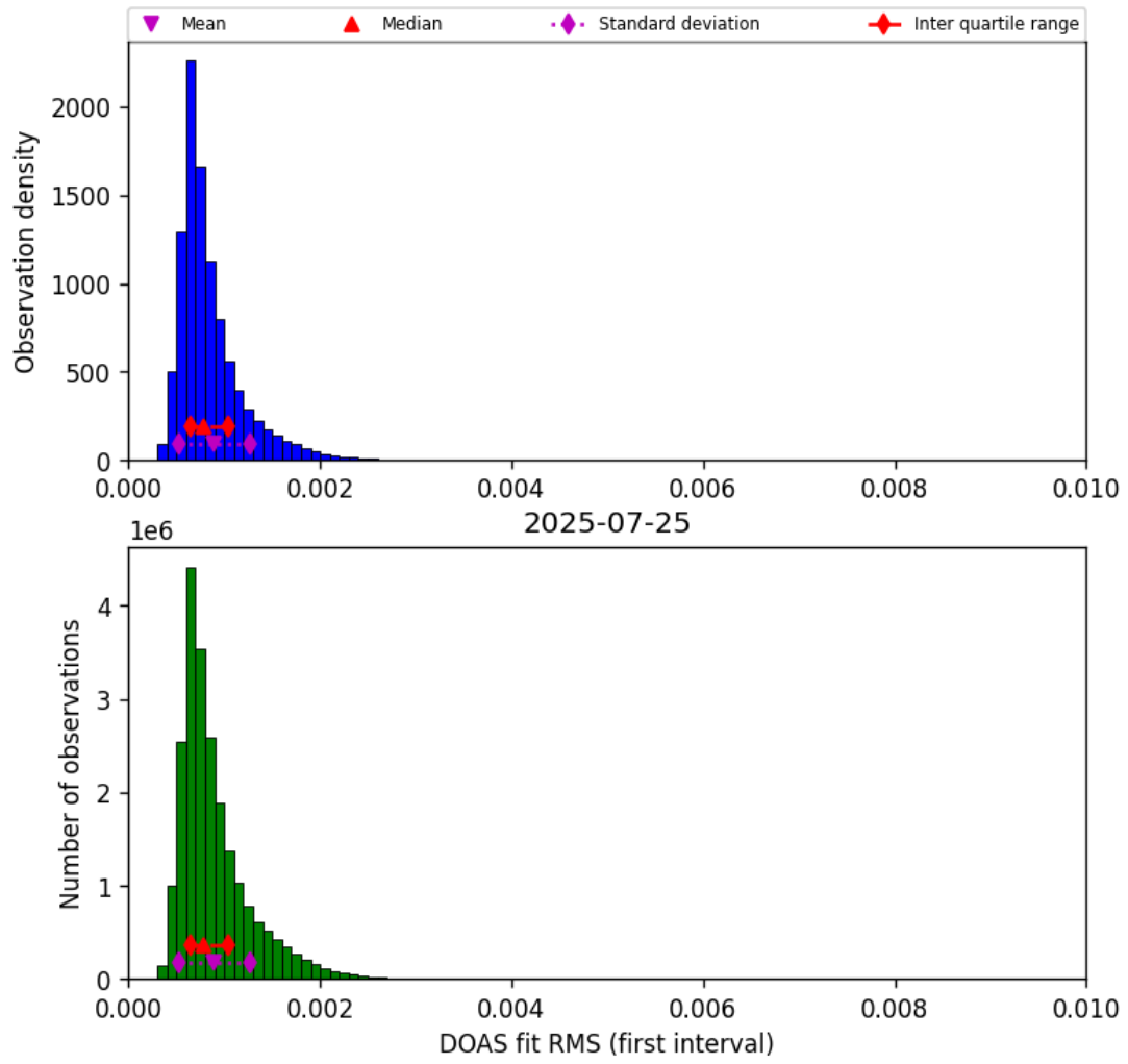
Figure 44: Histogram of “DOAS fit RMS (first interval)” for 2025-07-25 to 2025-07-26
