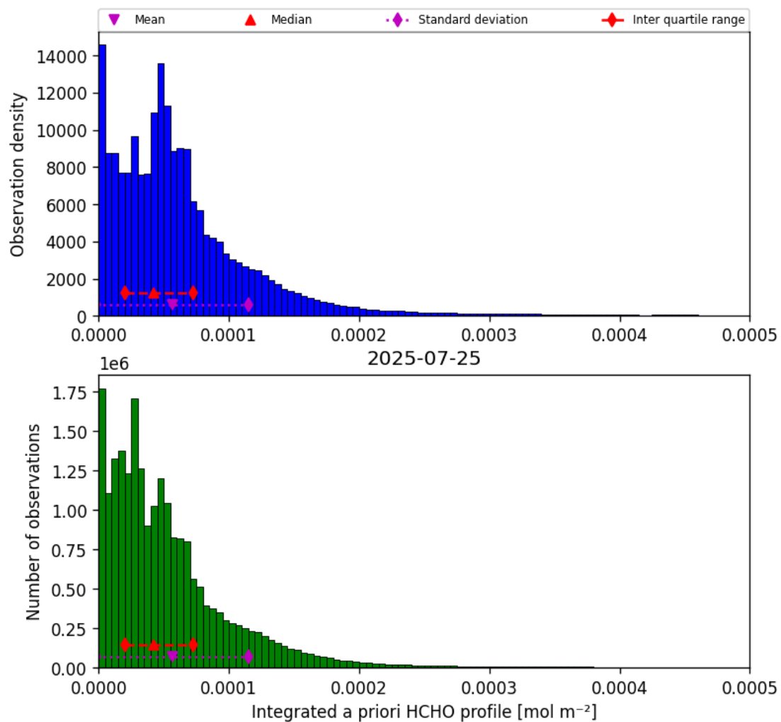
Figure 41: Histogram of “Integrated a priori HCHO profile” for 2025-07-25 to 2025-07-26
