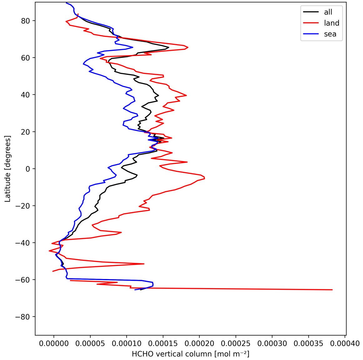
Figure 19: Zonal average of “HCHO vertical column” for 2025-07-25 to 2025-07-26.
