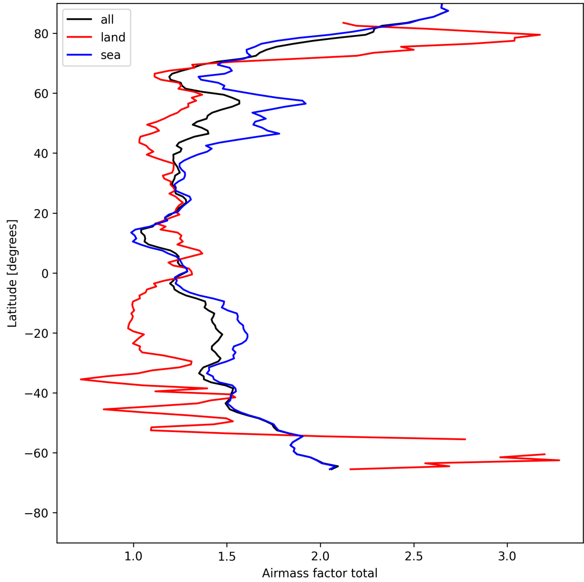
Figure 24: Zonal average of “Airmass factor total” for 2025-07-25 to 2025-07-26.
