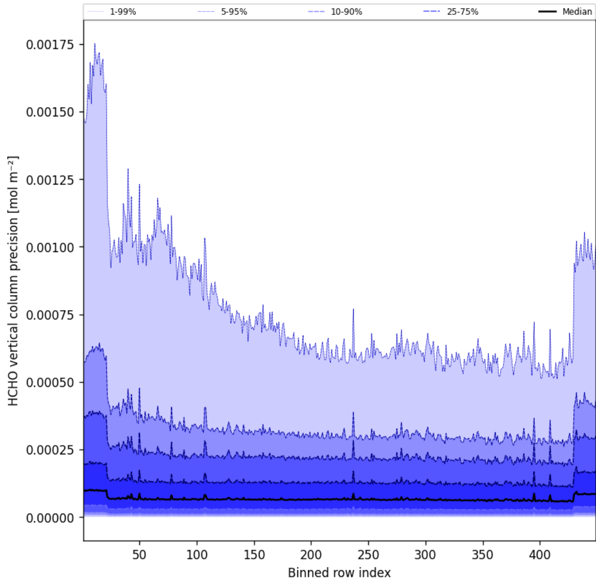
Figure 48: Along track statistics of “HCHO vertical column precision” for 2025-07-25 to 2025-07-26
