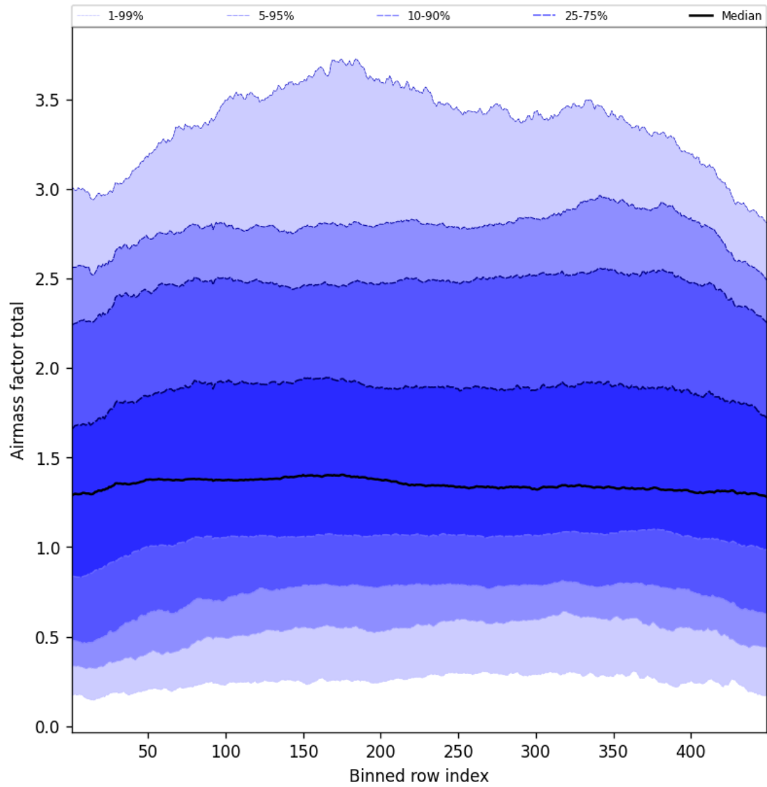
Figure 52: Along track statistics of “Airmass factor total” for 2025-07-25 to 2025-07-26
