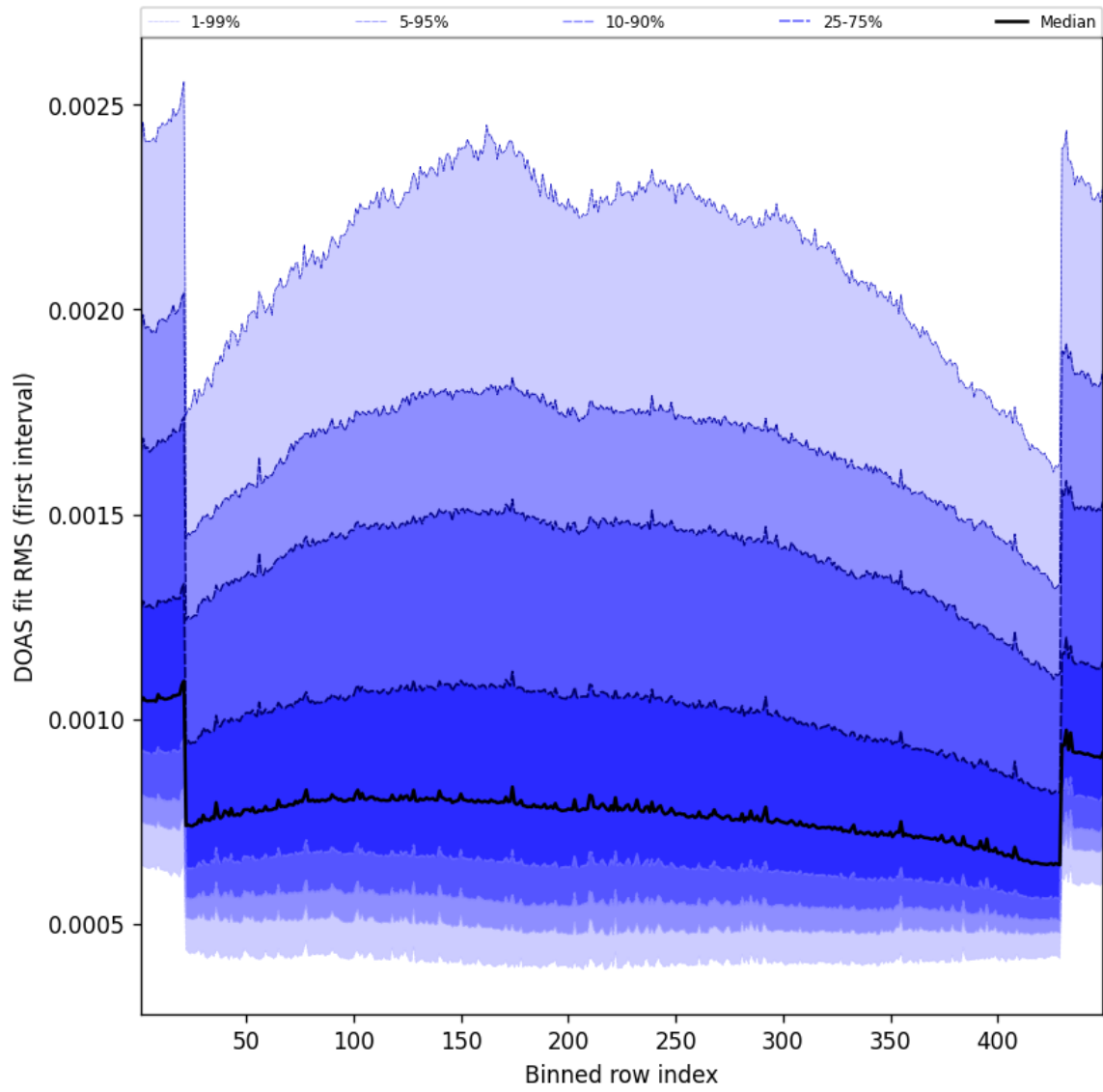
Figure 58: Along track statistics of “DOAS fit RMS (first interval)” for 2025-07-25 to 2025-07-26
