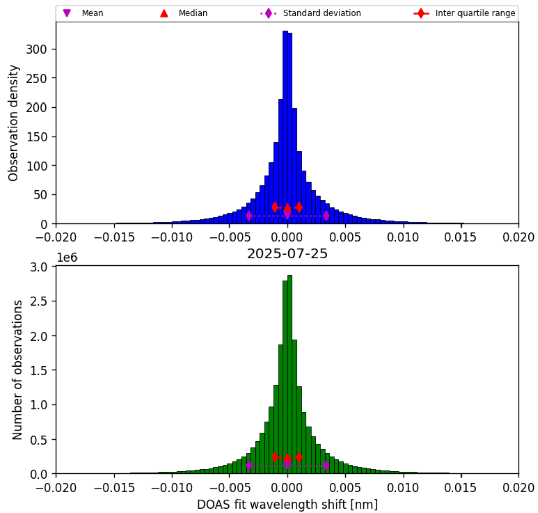
Figure 42: Histogram of “DOAS fit wavelength shift” for 2025-07-25 to 2025-07-26
