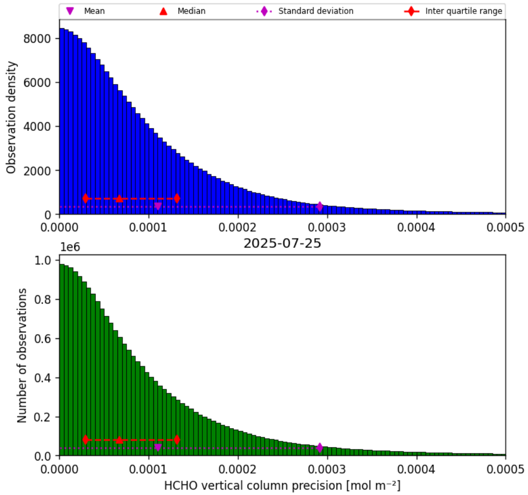
Figure 34: Histogram of “HCHO vertical column precision” for 2025-07-25 to 2025-07-26
