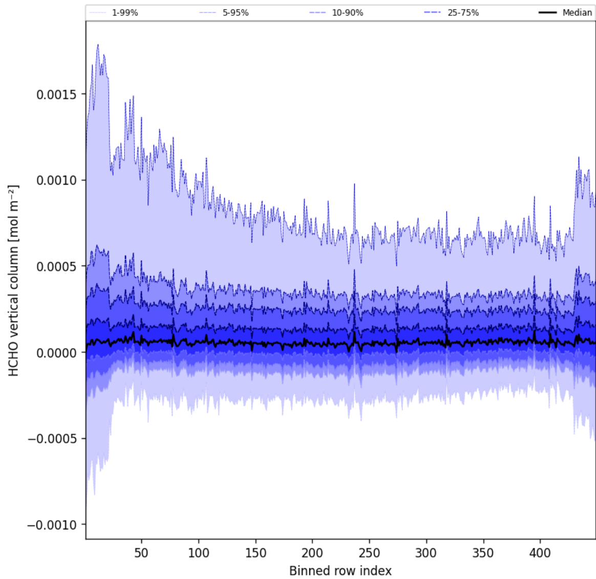
Figure 47: Along track statistics of “HCHO vertical column” for 2025-07-25 to 2025-07-26
