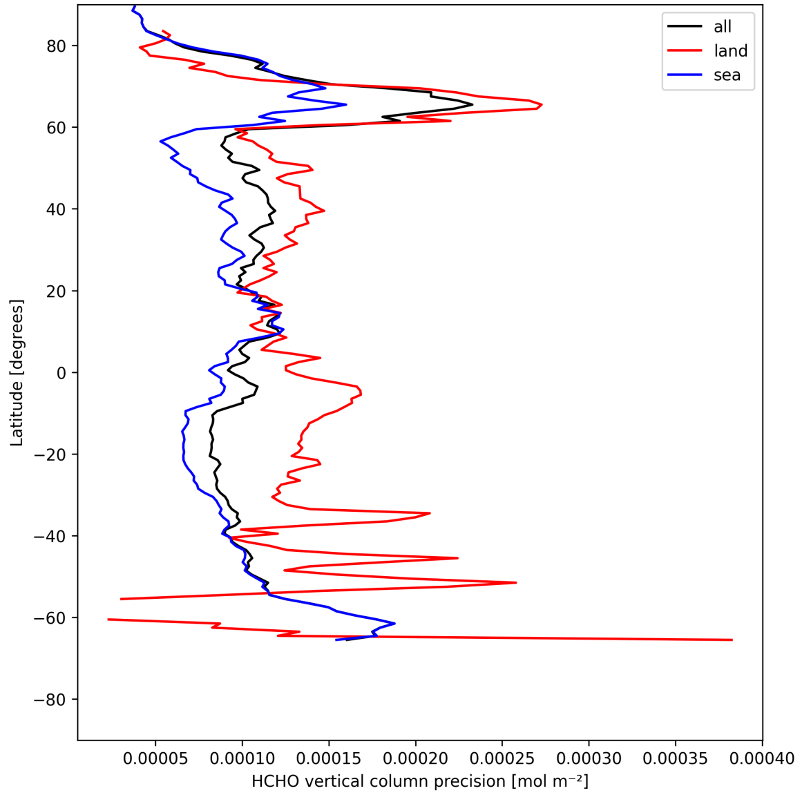
Figure 20: Zonal average of “HCHO vertical column precision” for 2025-07-25 to 2025-07-26.
