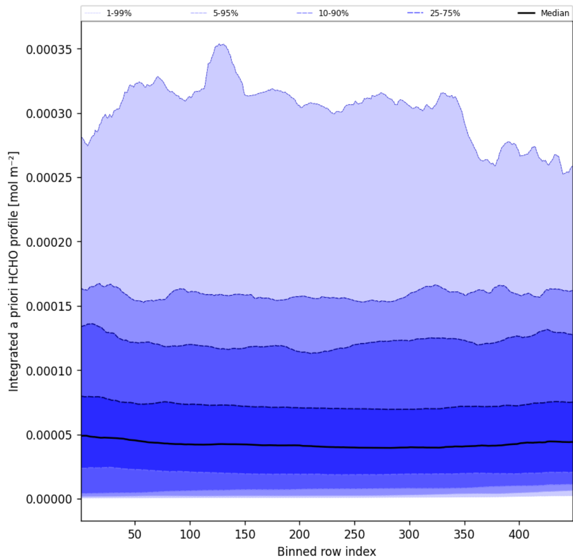
Figure 55: Along track statistics of “Integrated a priori HCHO profile” for 2025-07-25 to 2025-07-26
