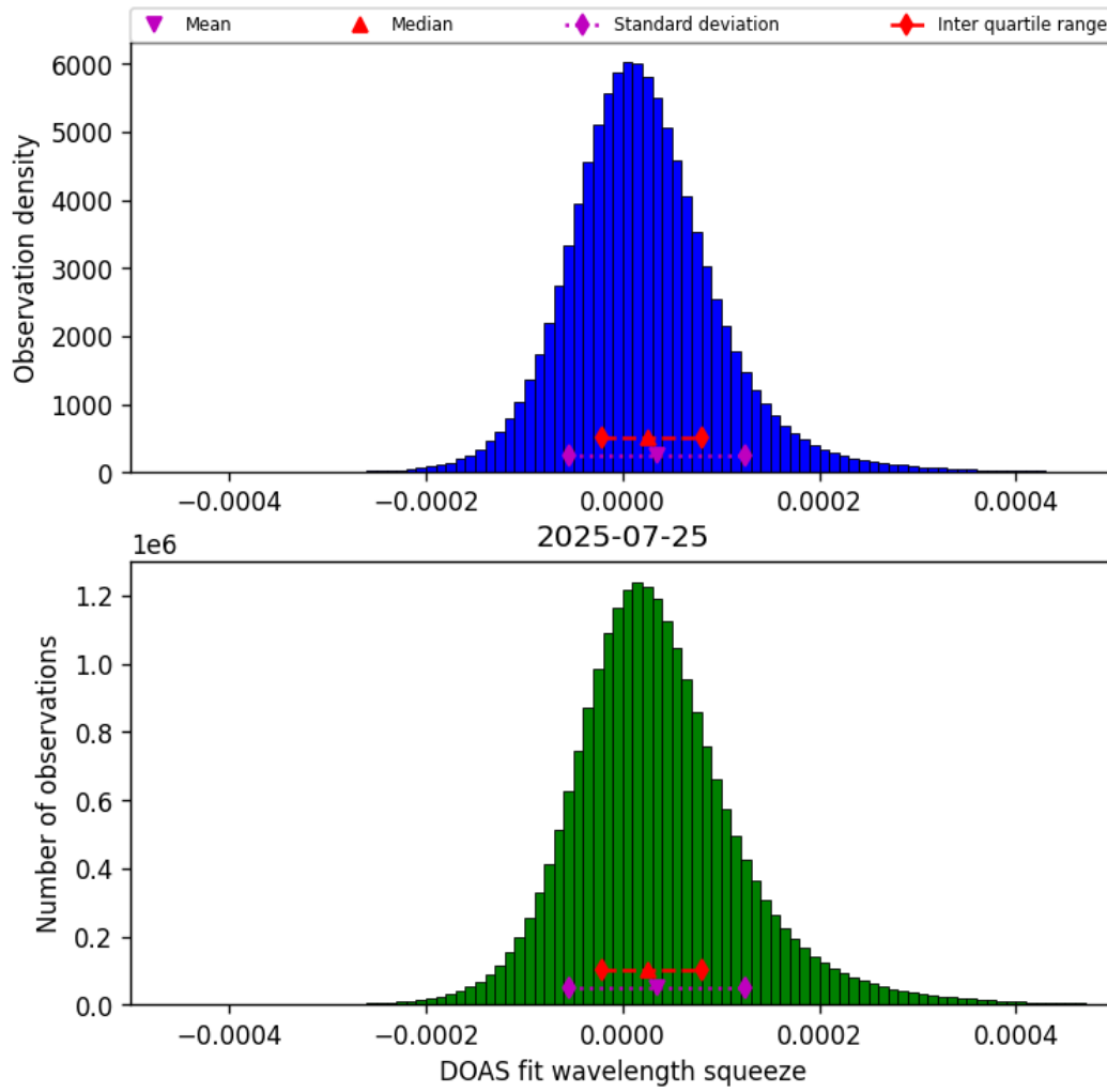
Figure 43: Histogram of “DOAS fit wavelength squeeze” for 2025-07-25 to 2025-07-26
