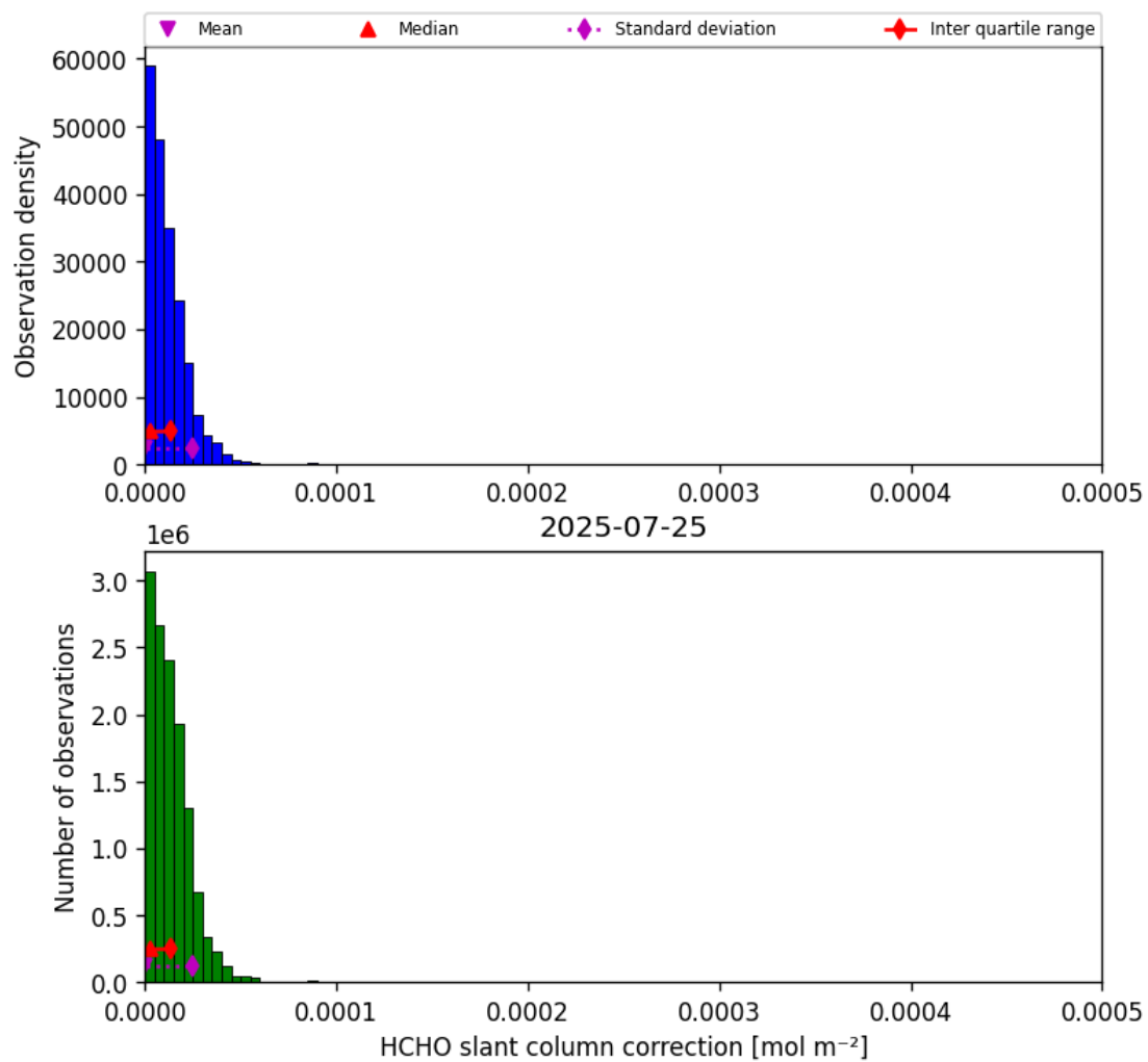
Figure 45: Histogram of “HCHO slant column correction” for 2025-07-25 to 2025-07-26
