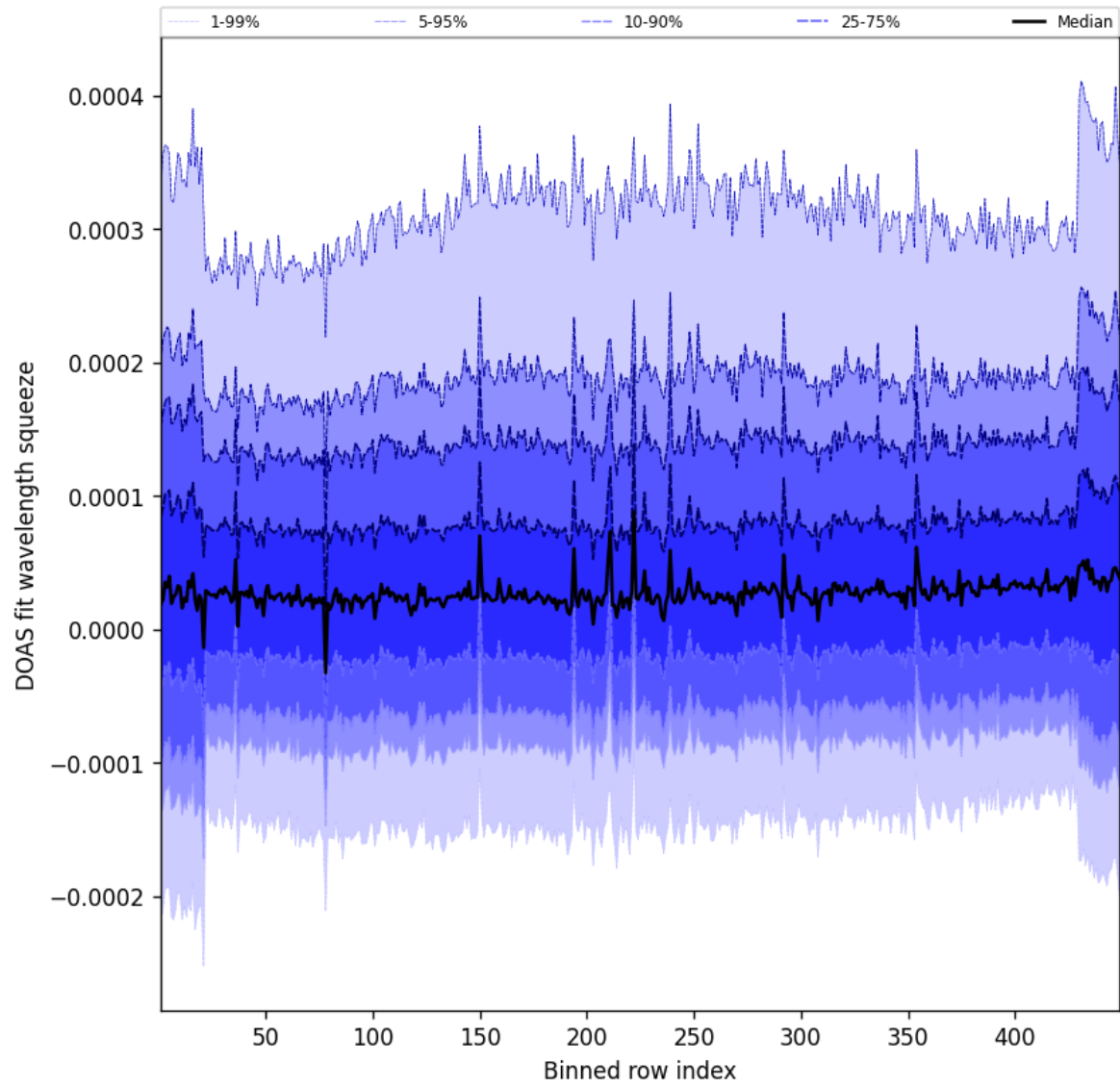
Figure 57: Along track statistics of “DOAS fit wavelength squeeze” for 2025-07-25 to 2025-07-26
