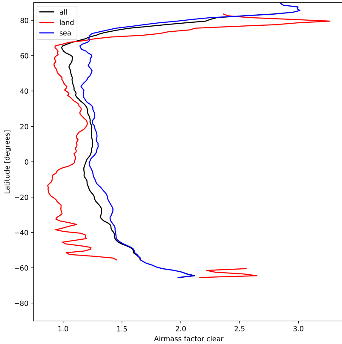
Figure 26: Zonal average of “Airmass factor clear” for 2025-07-25 to 2025-07-26.
