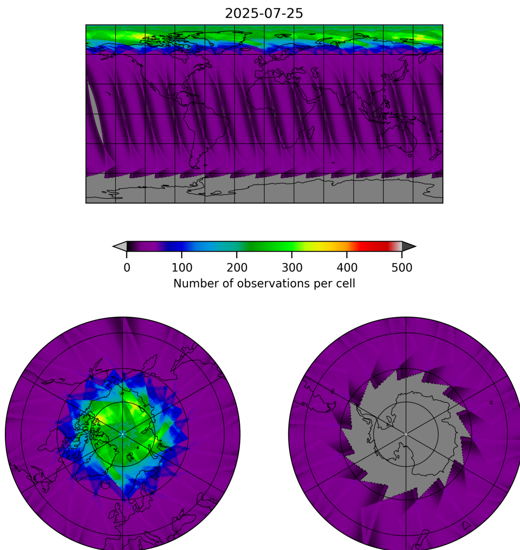
Figure 17: Map of the number of observations for 2025-07-25 to 2025-07-26
