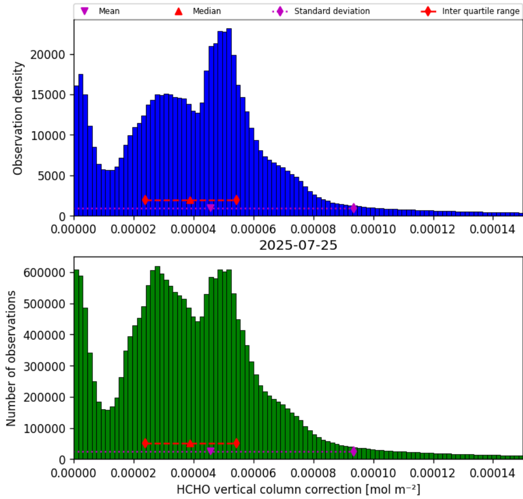
Figure 35: Histogram of “HCHO vertical column correction” for 2025-07-25 to 2025-07-26
