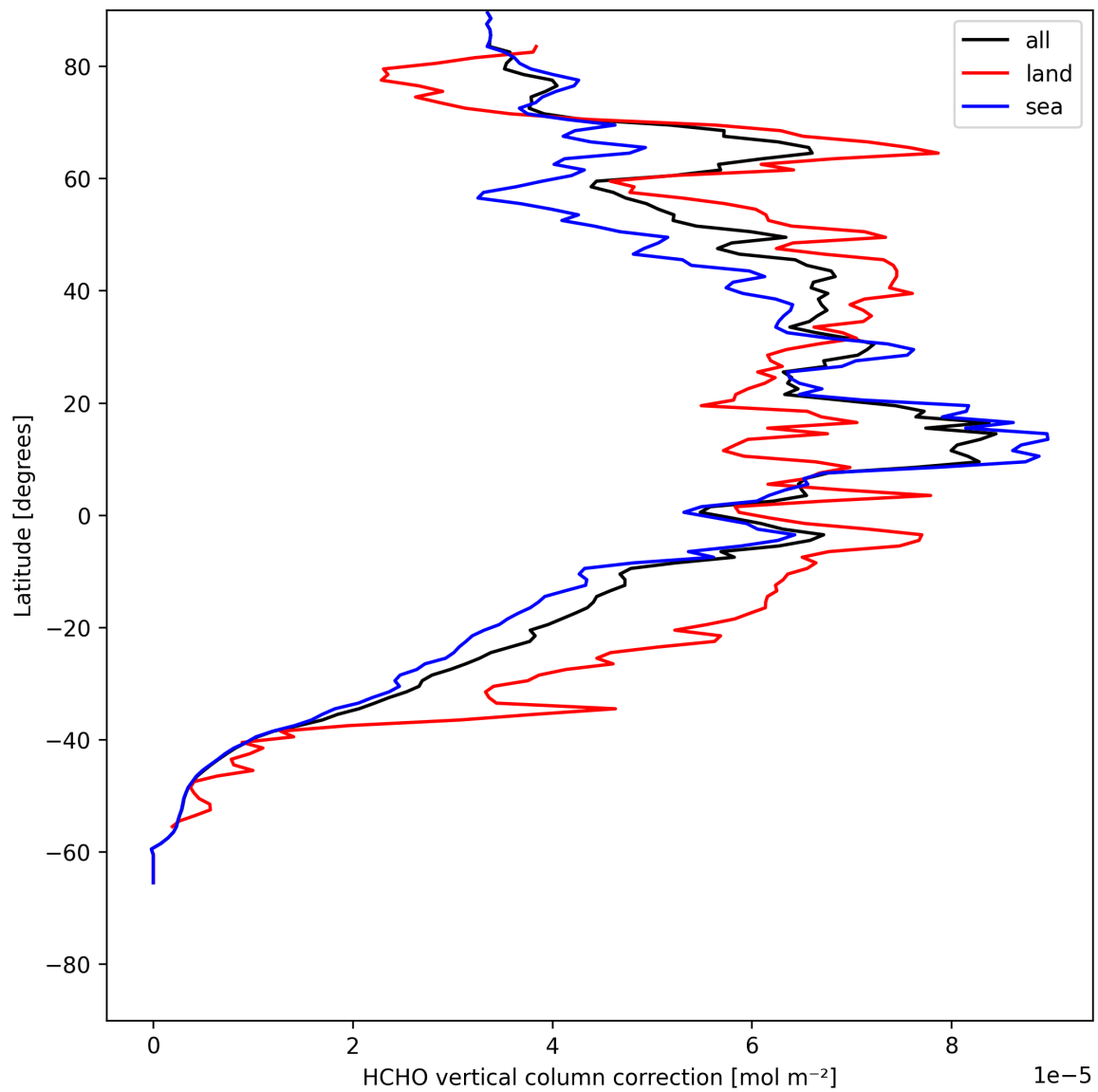
Figure 21: Zonal average of “HCHO vertical column correction” for 2025-07-25 to 2025-07-26.
