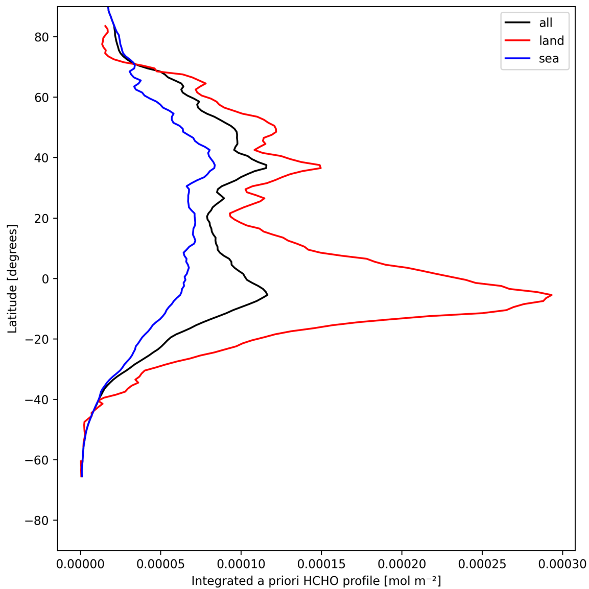
Figure 27: Zonal average of “Integrated a priori HCHO profile” for 2025-07-25 to 2025-07-26.
