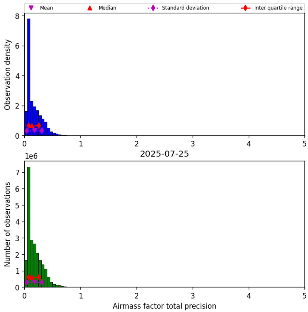
Figure 39: Histogram of “Airmass factor total precision” for 2025-07-25 to 2025-07-26
