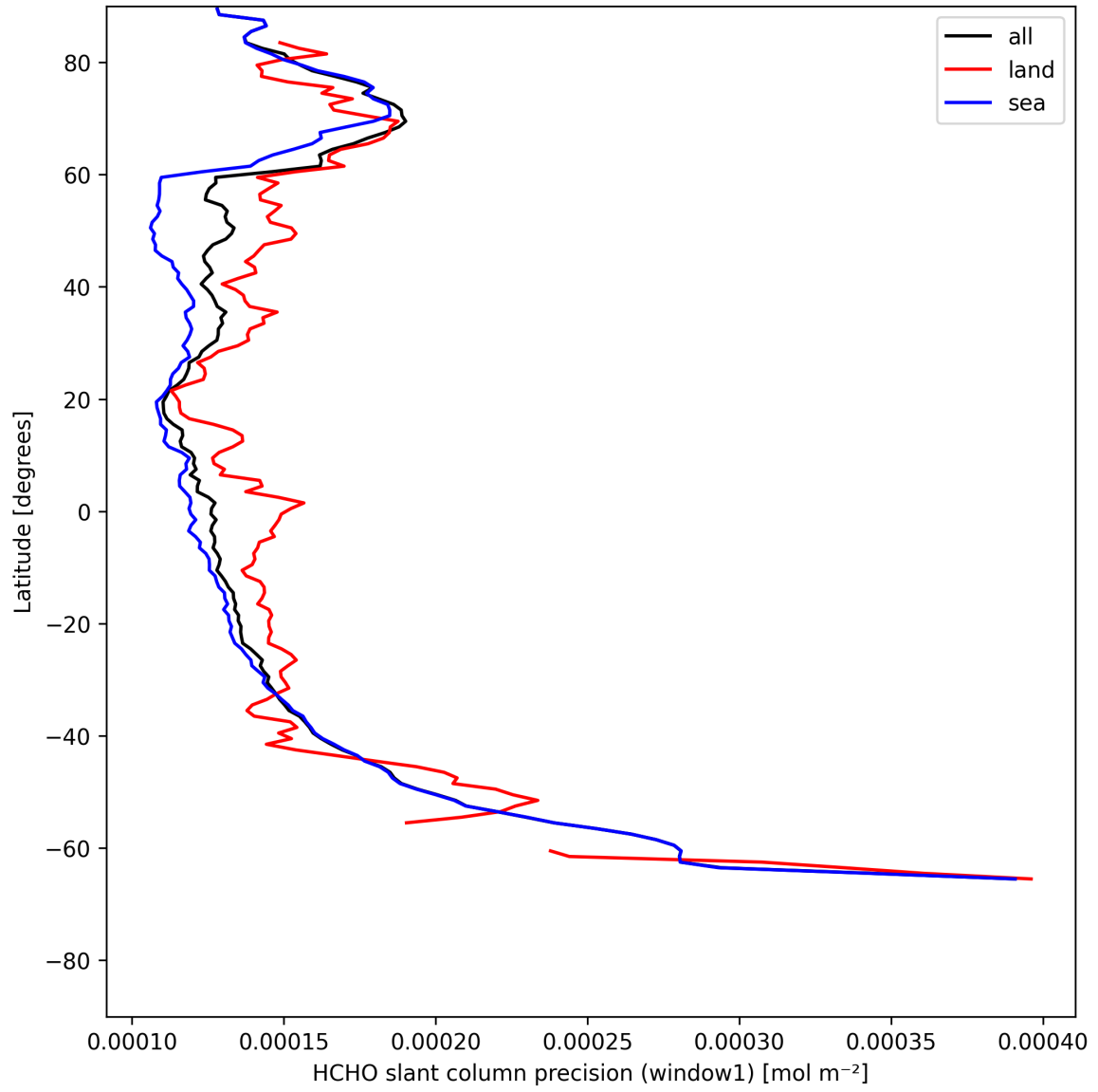
Figure 23: Zonal average of “HCHO slant column precision (window1)” for 2025-07-25 to 2025-07-26.
