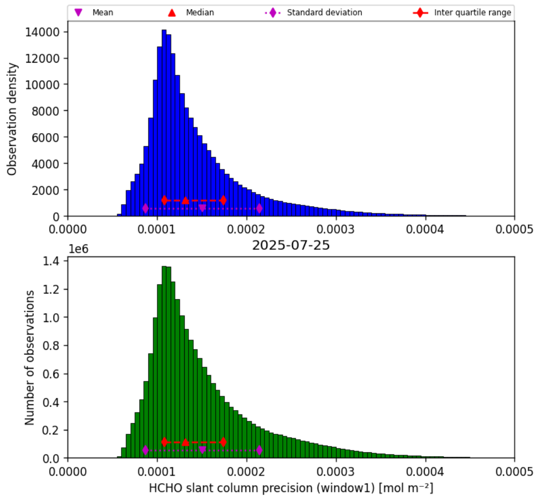
Figure 37: Histogram of “HCHO slant column precision (window1)” for 2025-07-25 to 2025-07-26
