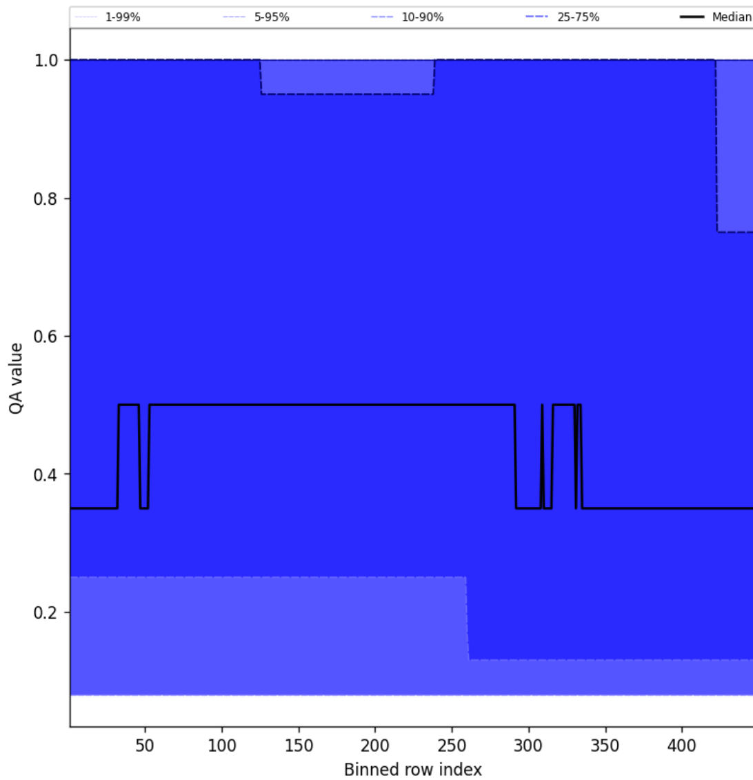
Figure 46: Along track statistics of “QA value” for 2025-07-25 to 2025-07-26
