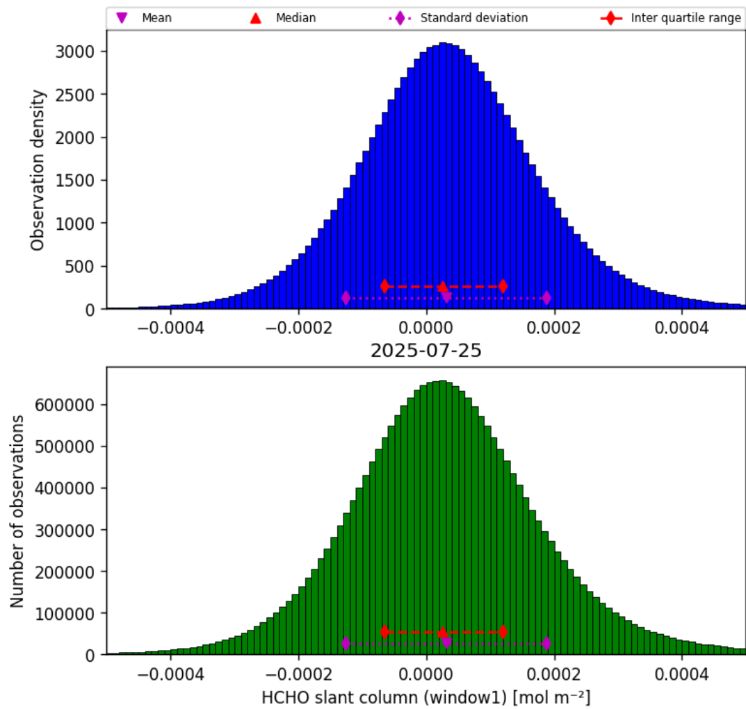
Figure 36: Histogram of “HCHO slant column (window1)” for 2025-07-25 to 2025-07-26
