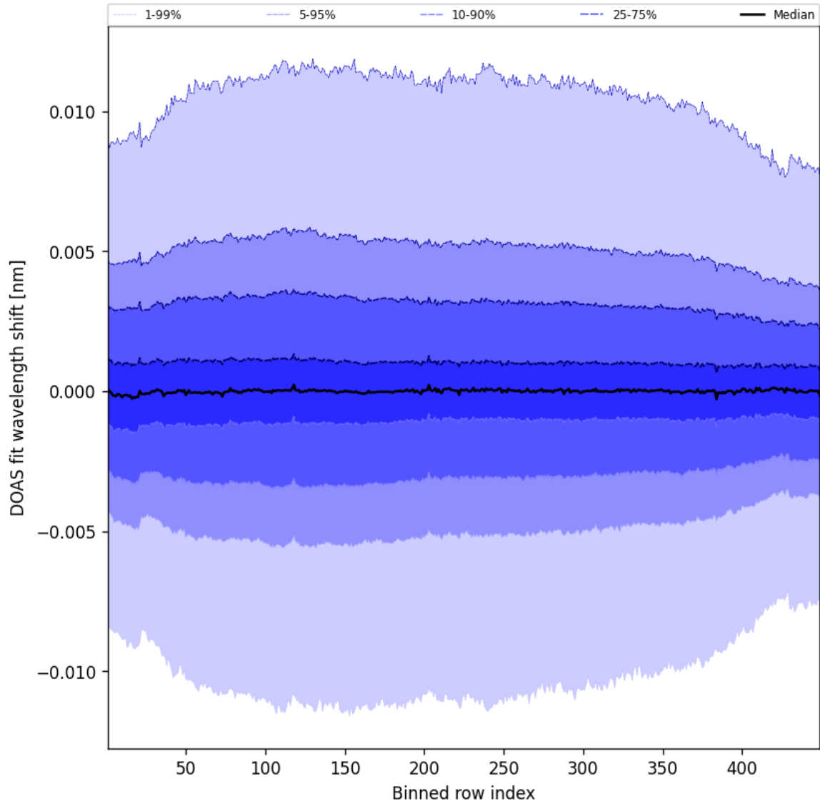
Figure 56: Along track statistics of “DOAS fit wavelength shift” for 2025-07-25 to 2025-07-26
