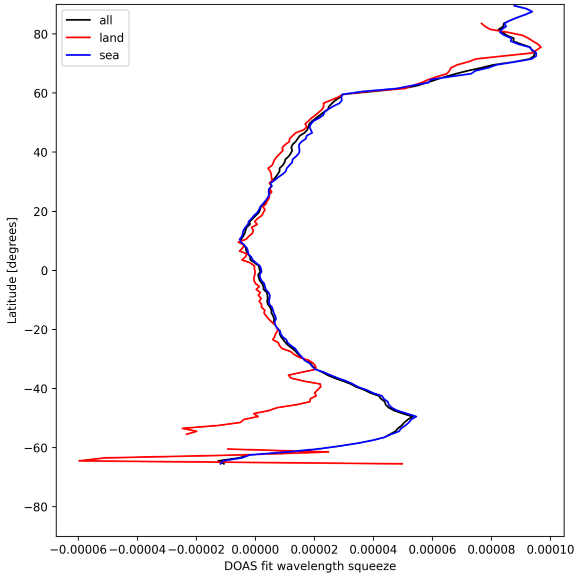
Figure 29: Zonal average of “DOAS fit wavelength squeeze” for 2025-07-25 to 2025-07-26.
