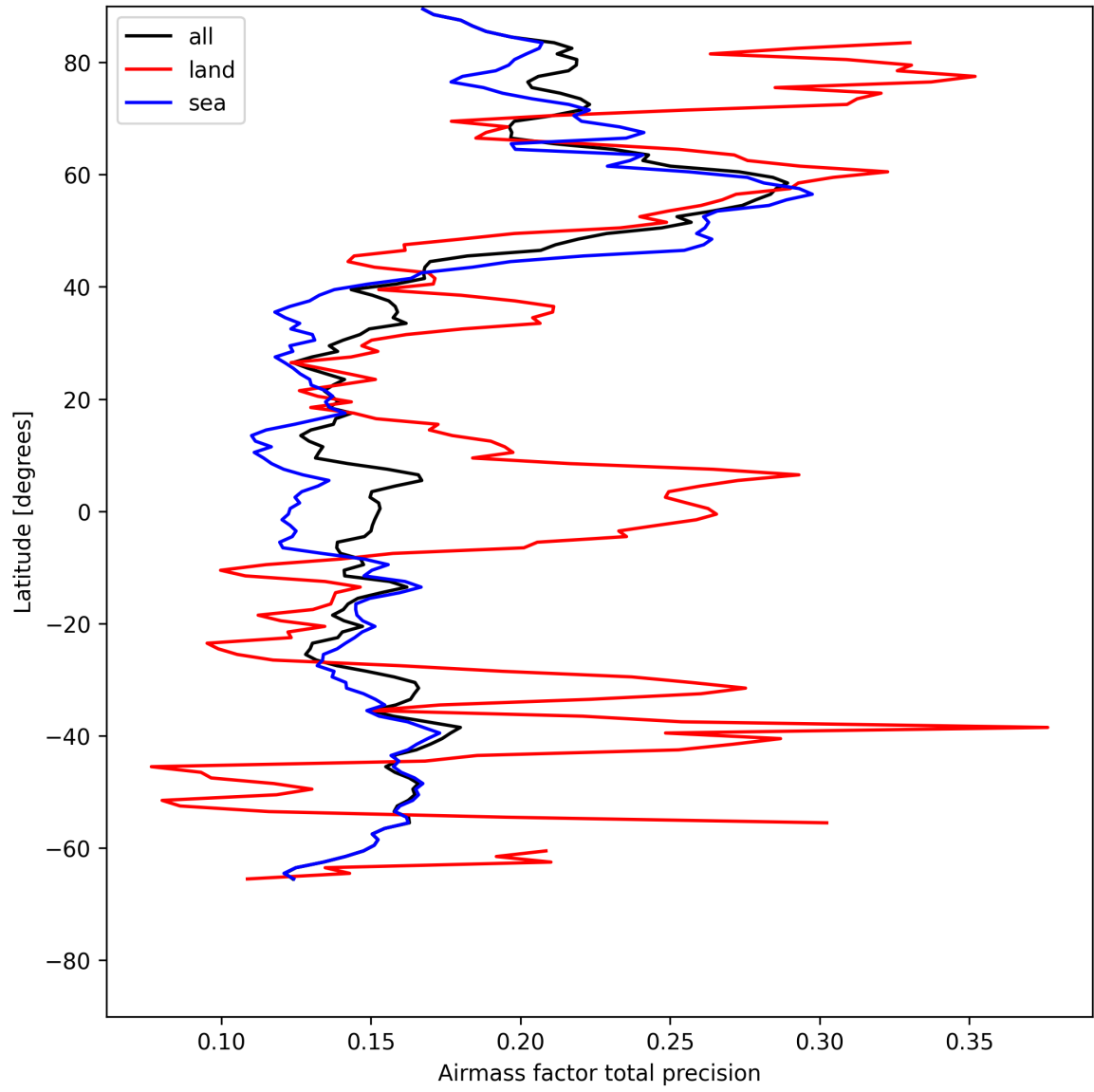
Figure 25: Zonal average of “Airmass factor total precision” for 2025-07-25 to 2025-07-26.
