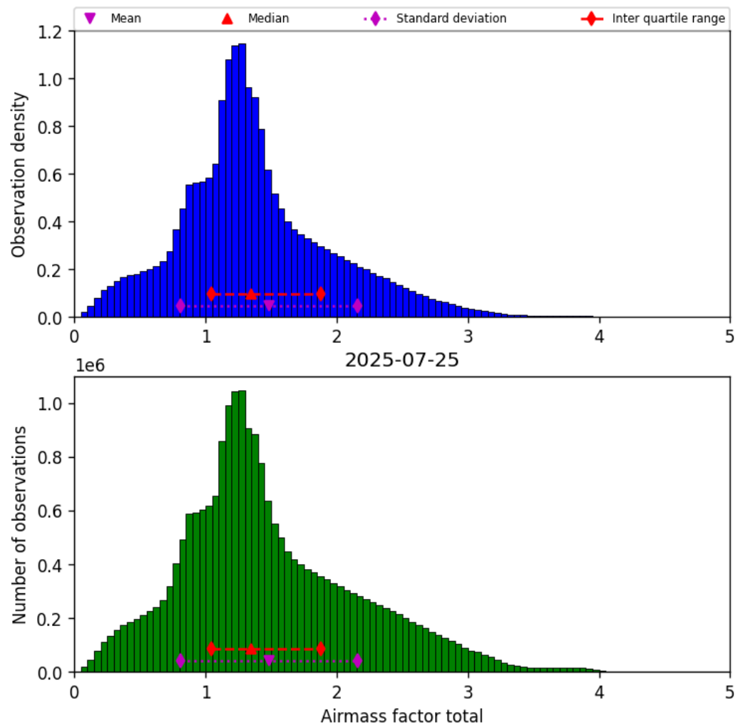
Figure 38: Histogram of “Airmass factor total” for 2025-07-25 to 2025-07-26
