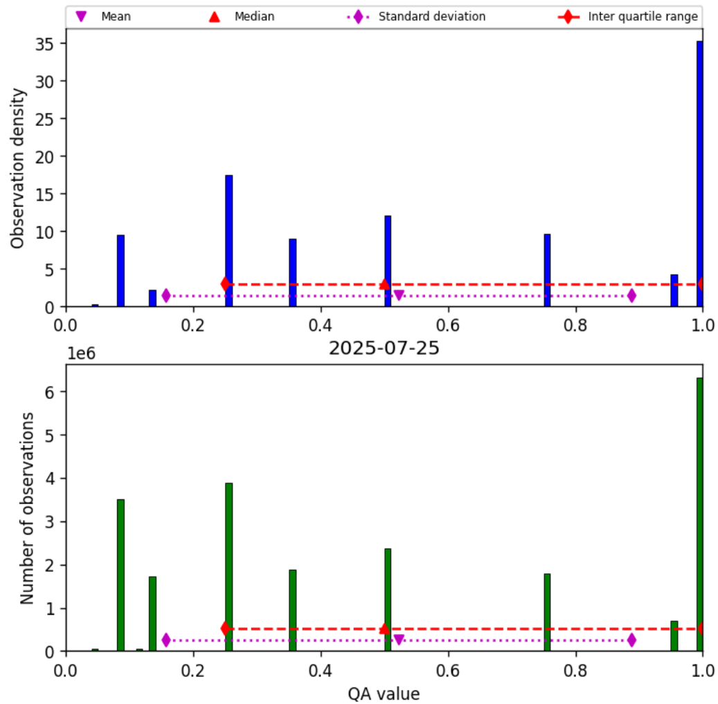
Figure 32: Histogram of “QA value” for 2025-07-25 to 2025-07-26
