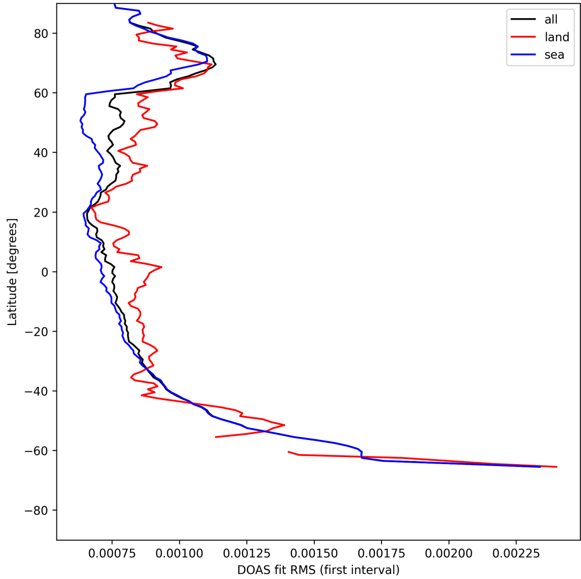
Figure 30: Zonal average of "DOAS fit RMS (first interval)" for 2025-07-25 to 2025-07-26.
