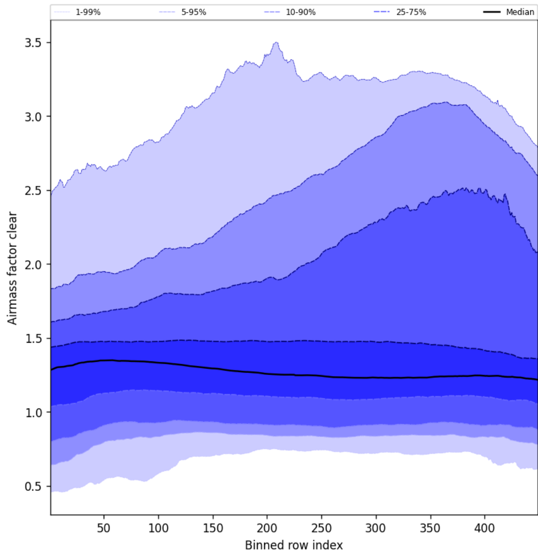
Figure 54: Along track statistics of “Airmass factor clear” for 2025-07-25 to 2025-07-26
