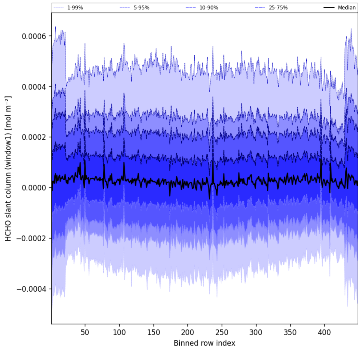
Figure 50: Along track statistics of “HCHO slant column (window1)” for 2025-07-25 to 2025-07-26
