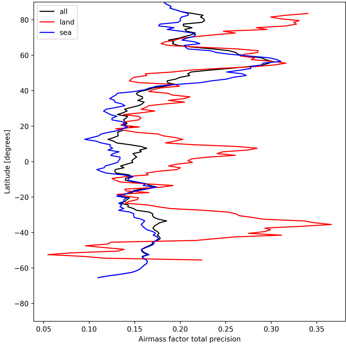
Figure 25: Zonal average of “Airmass factor total precision” for 2025-07-26 to 2025-07-27.
