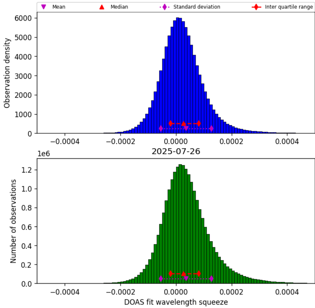
Figure 43: Histogram of “DOAS fit wavelength squeeze” for 2025-07-26 to 2025-07-27
