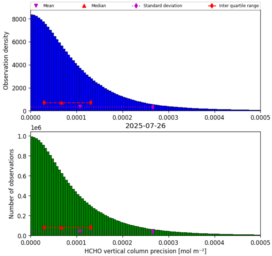
Figure 34: Histogram of “HCHO vertical column precision” for 2025-07-26 to 2025-07-27
