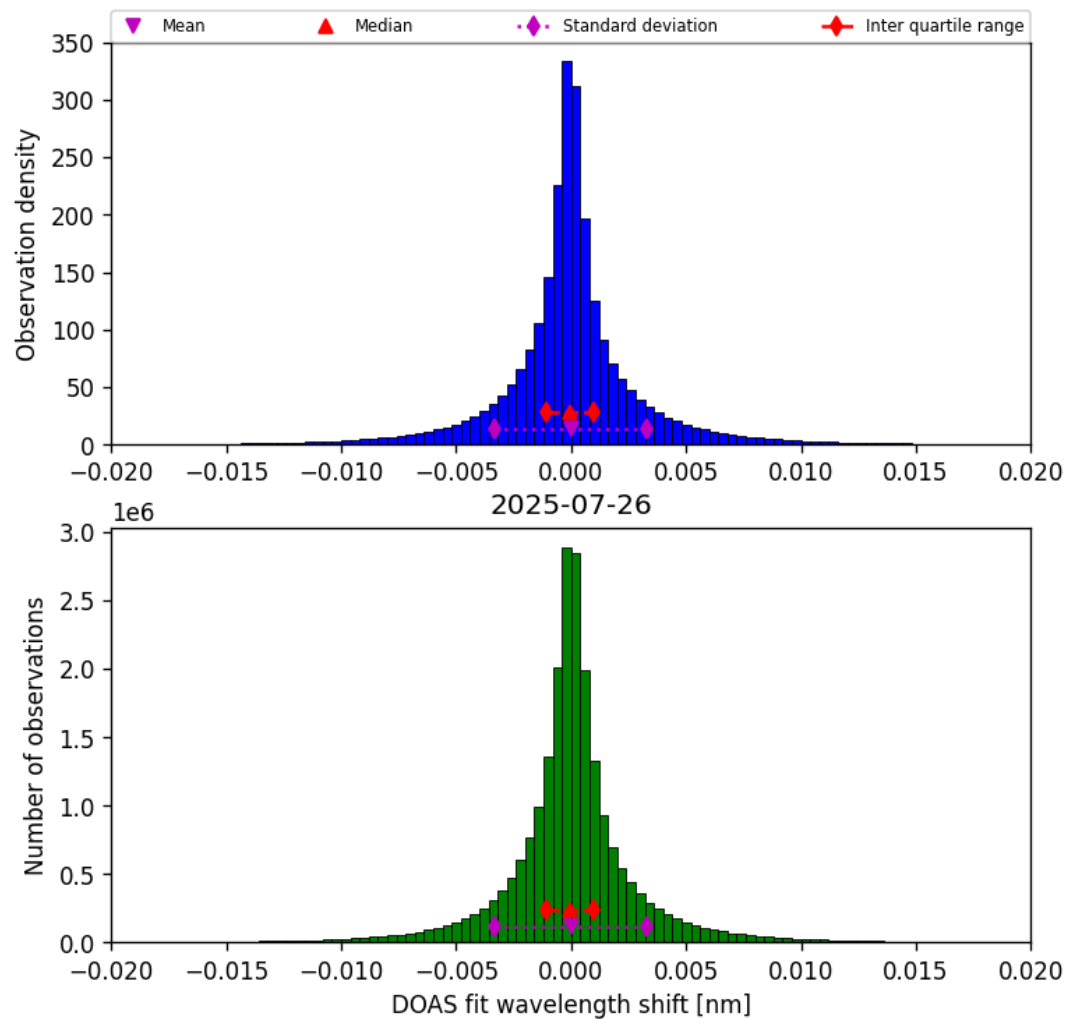
Figure 42: Histogram of “DOAS fit wavelength shift” for 2025-07-26 to 2025-07-27
