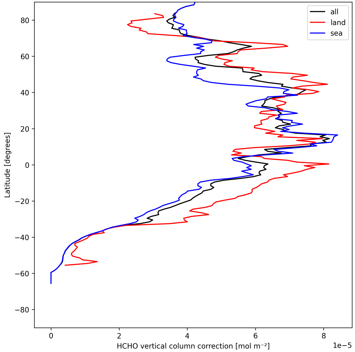
Figure 21: Zonal average of “HCHO vertical column correction” for 2025-07-26 to 2025-07-27.
