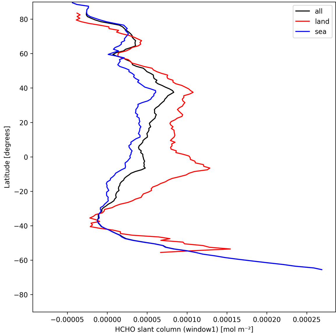
Figure 22: Zonal average of “HCHO slant column (window1)” for 2025-07-26 to 2025-07-27.
