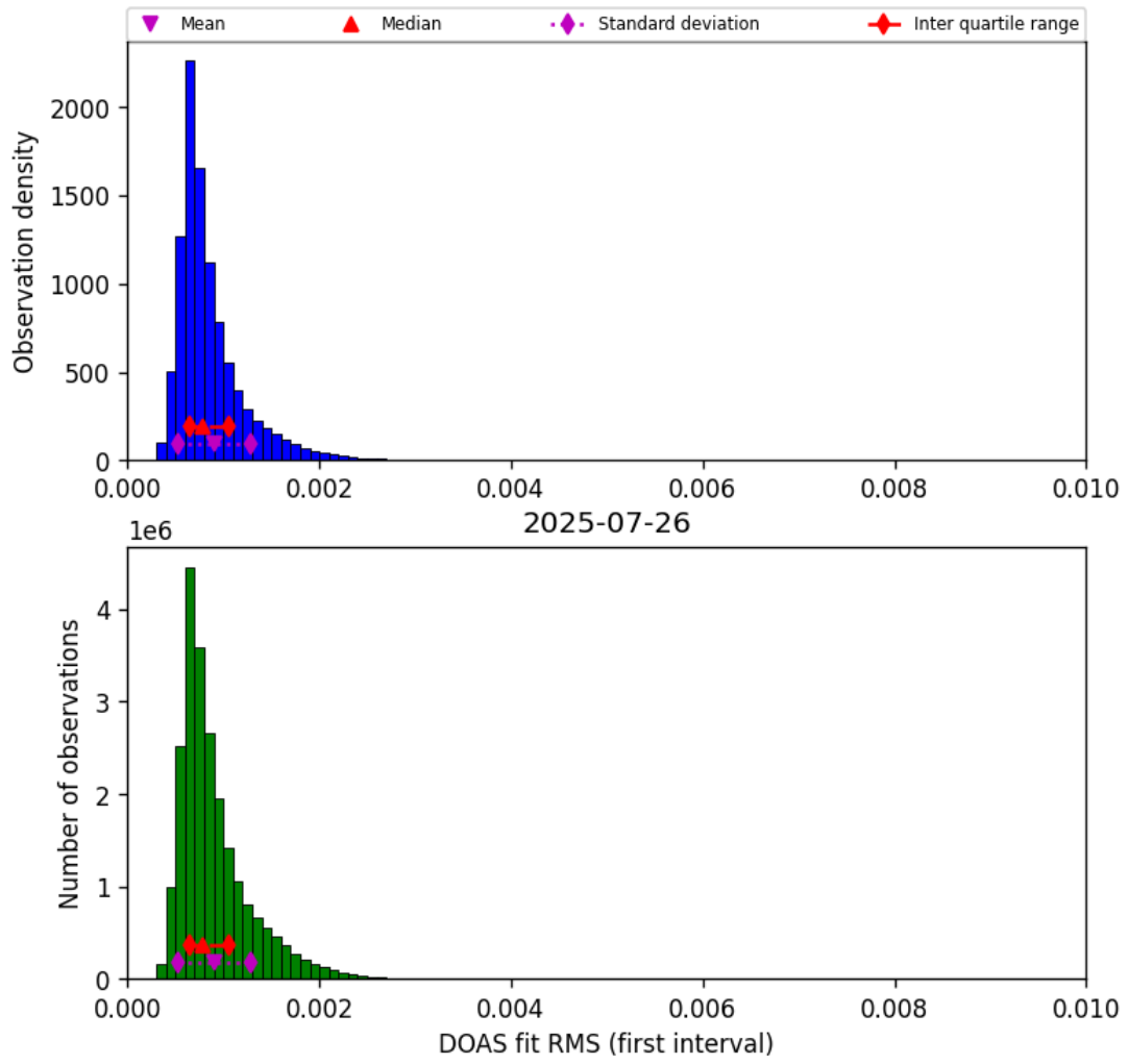
Figure 44: Histogram of “DOAS fit RMS (first interval)” for 2025-07-26 to 2025-07-27
