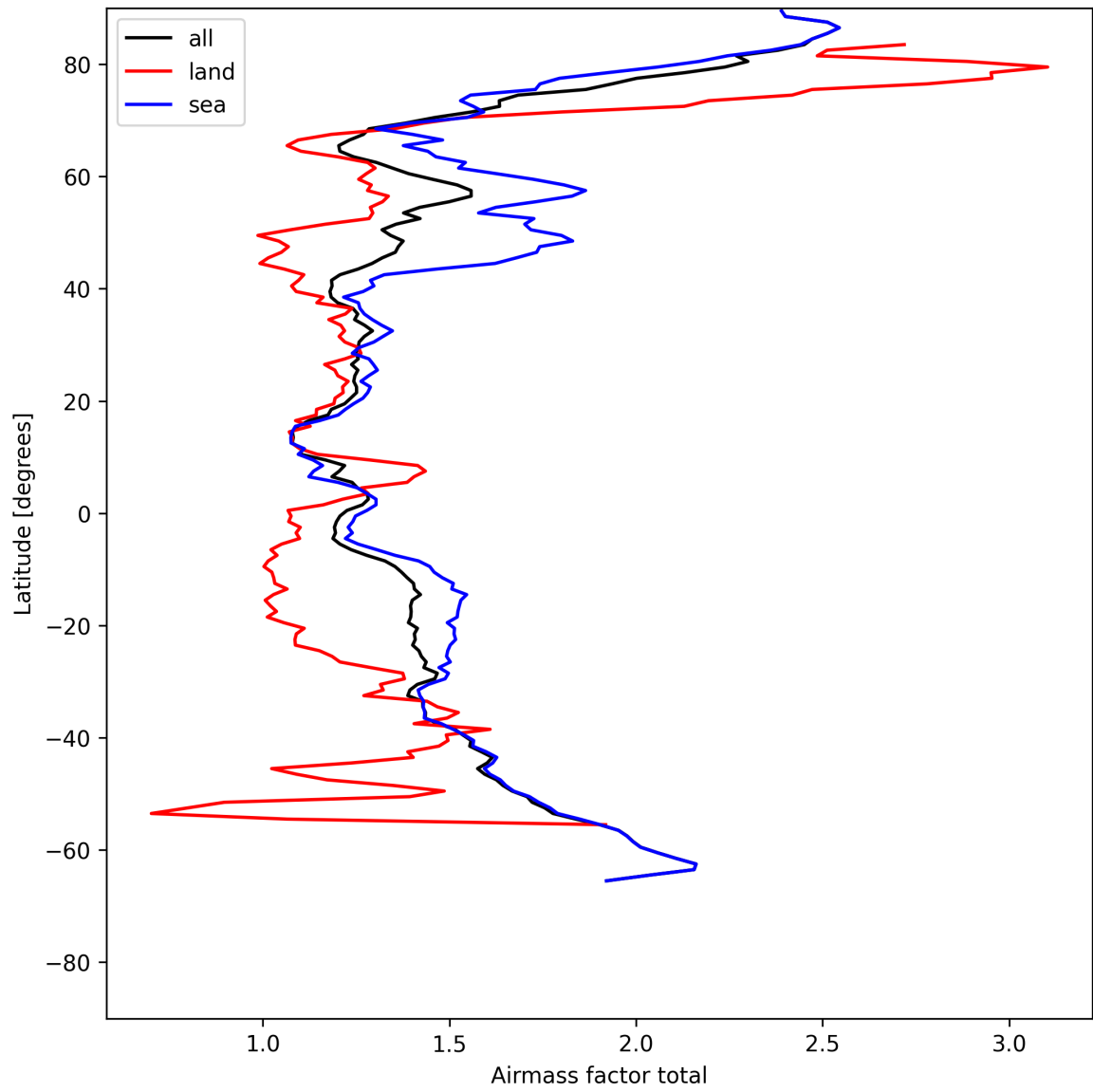
Figure 24: Zonal average of “Airmass factor total” for 2025-07-26 to 2025-07-27.
