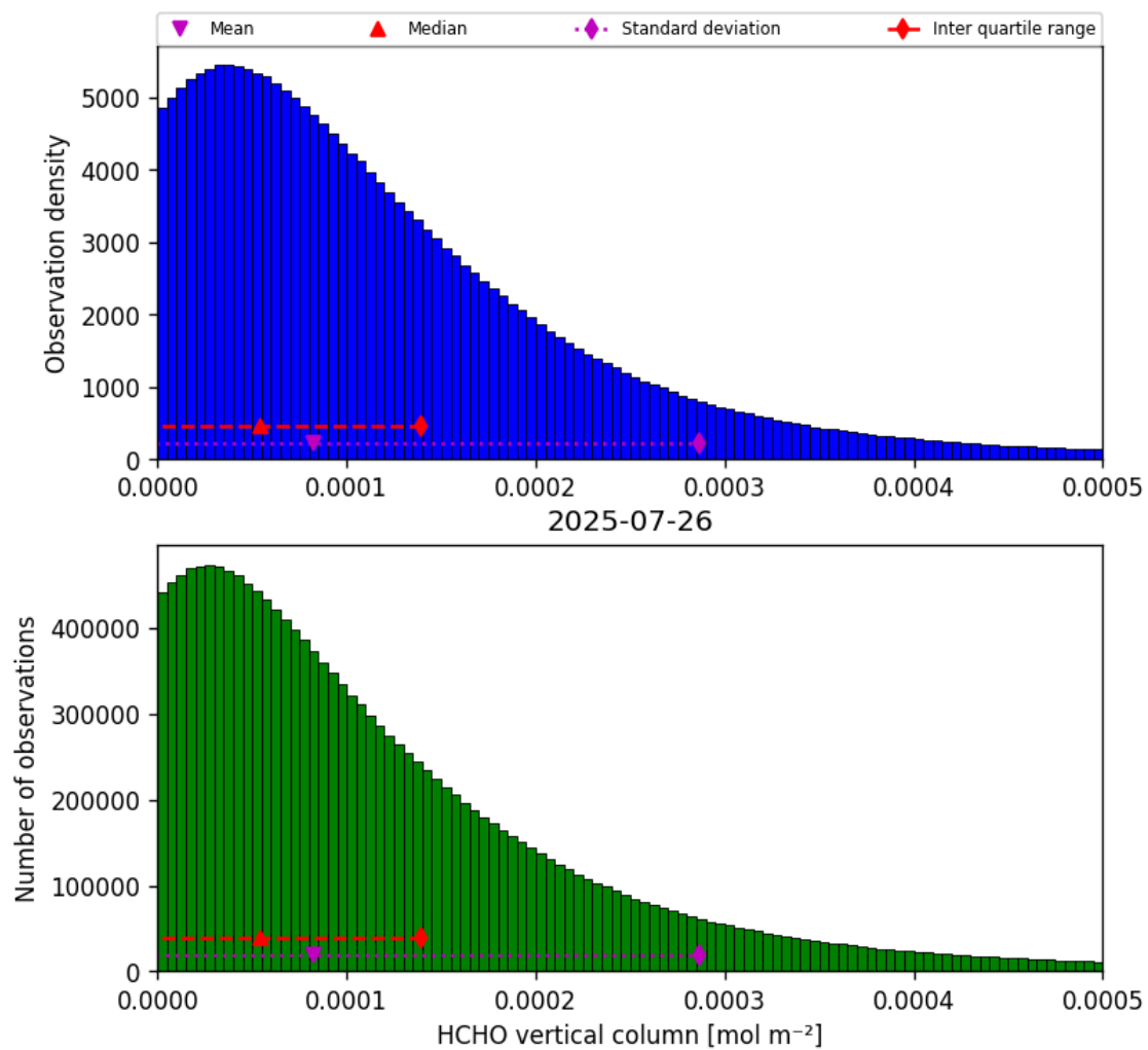
Figure 33: Histogram of “HCHO vertical column” for 2025-07-26 to 2025-07-27
