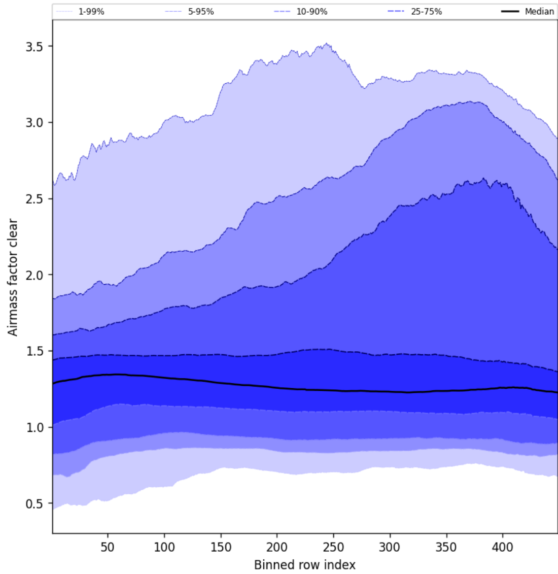
Figure 54: Along track statistics of “Airmass factor clear” for 2025-07-26 to 2025-07-27
