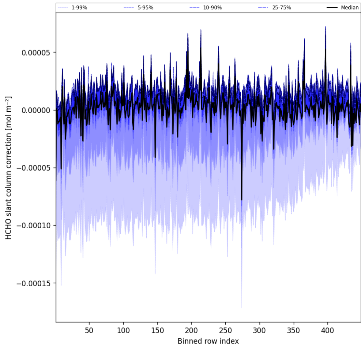
Figure 59: Along track statistics of “HCHO slant column correction” for 2025-07-26 to 2025-07-27
