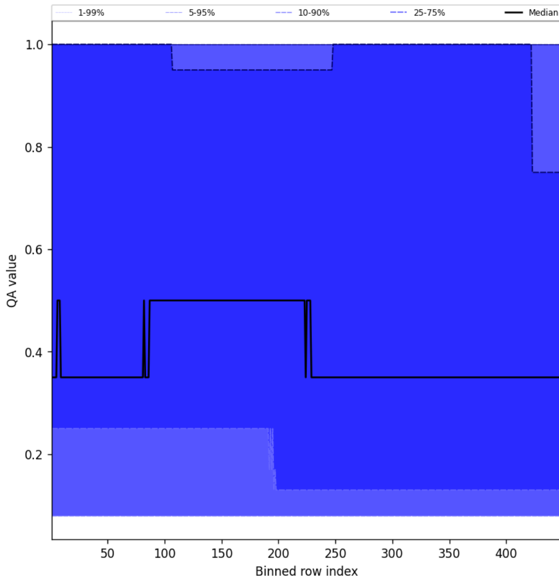
Figure 46: Along track statistics of “QA value” for 2025-07-26 to 2025-07-27
