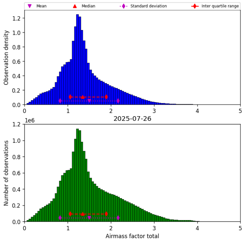
Figure 38: Histogram of “Airmass factor total” for 2025-07-26 to 2025-07-27
