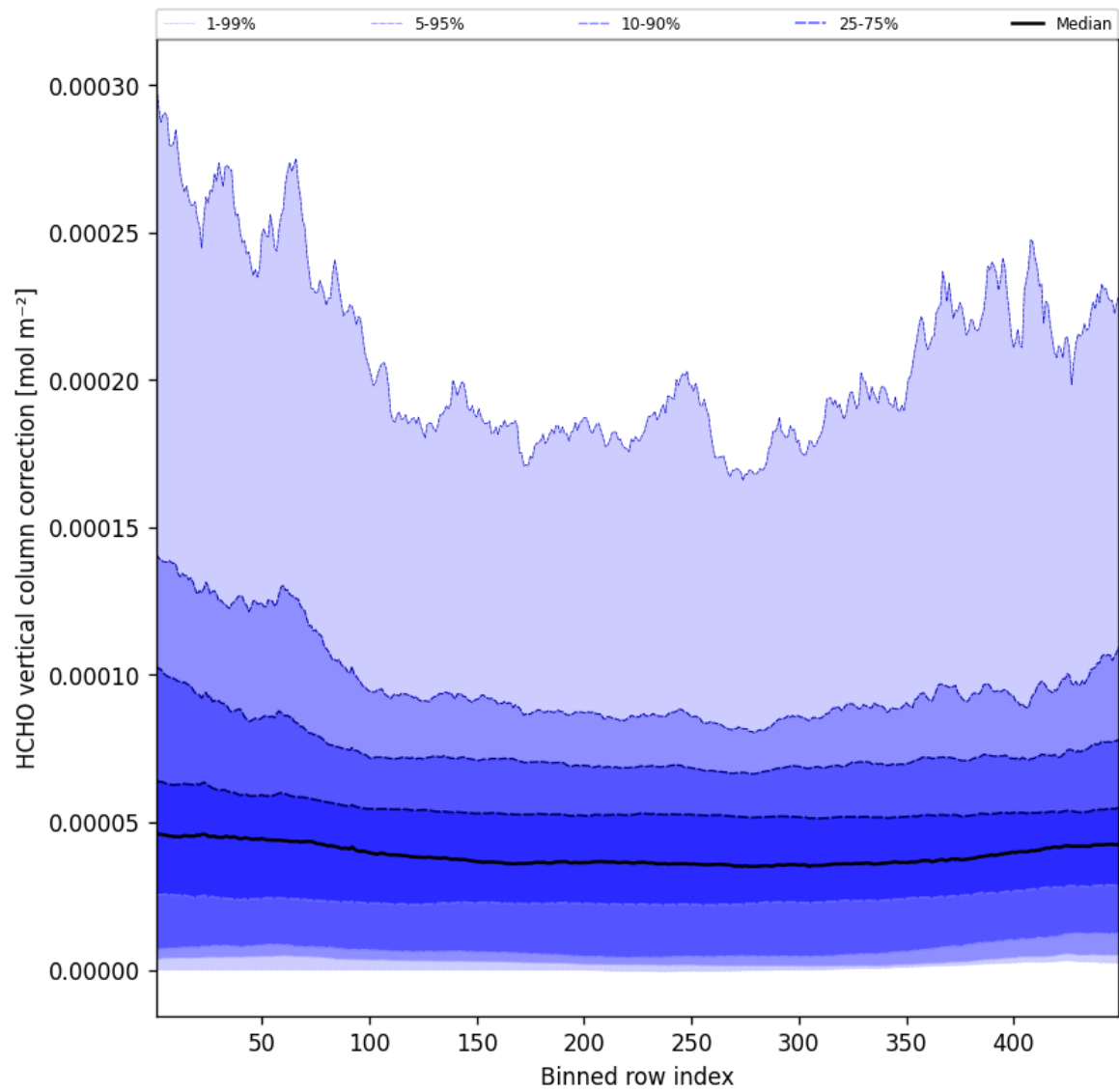
Figure 49: Along track statistics of “HCHO vertical column correction” for 2025-07-26 to 2025-07-27
