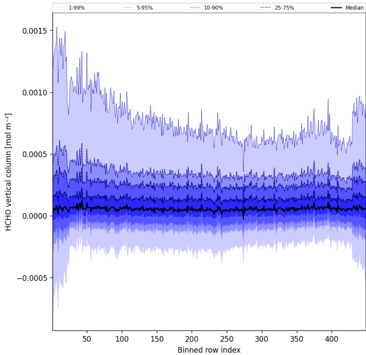
Figure 47: Along track statistics of “HCHO vertical column” for 2025-07-26 to 2025-07-27
