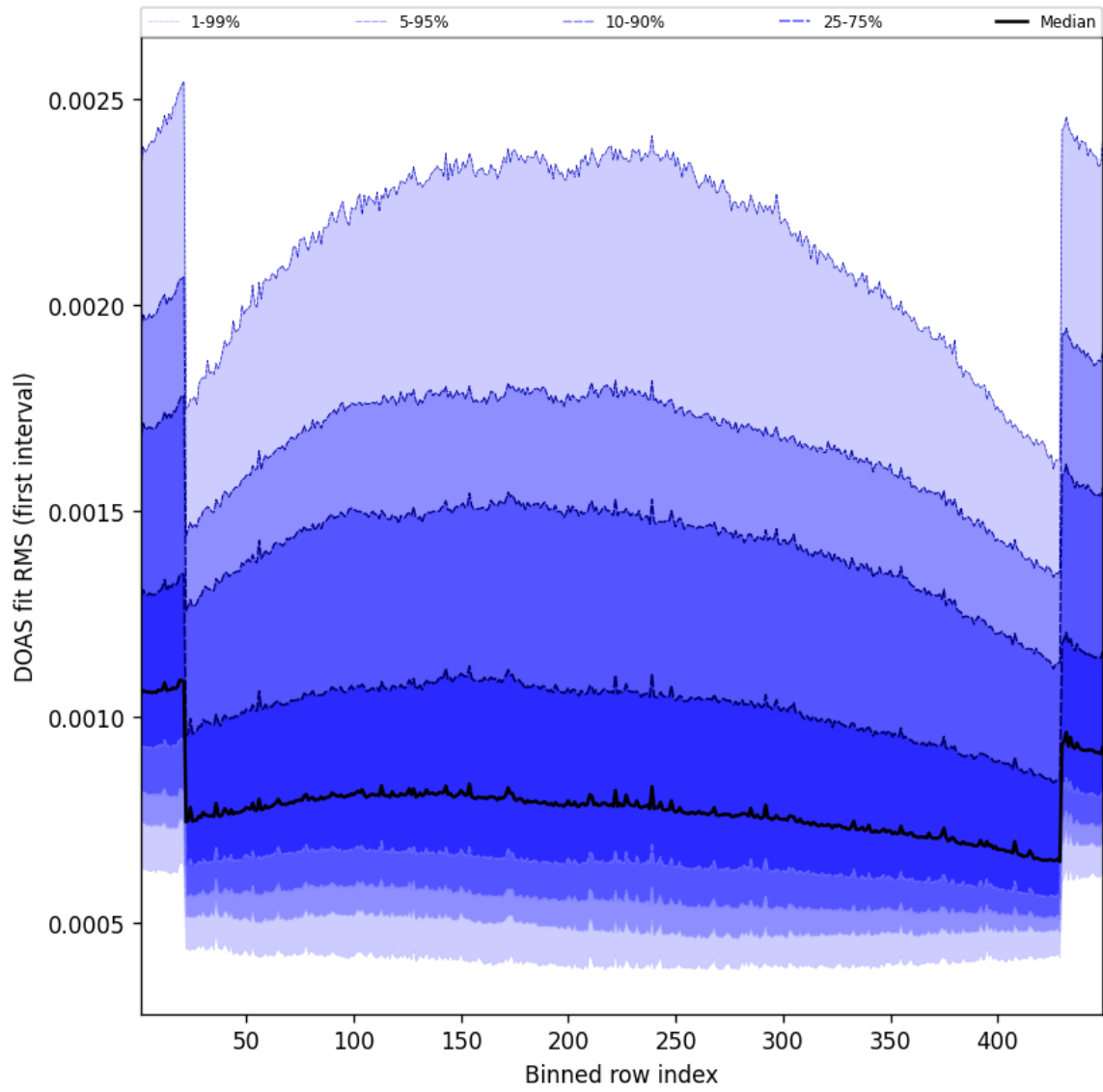
Figure 58: Along track statistics of “DOAS fit RMS (first interval)” for 2025-07-26 to 2025-07-27
