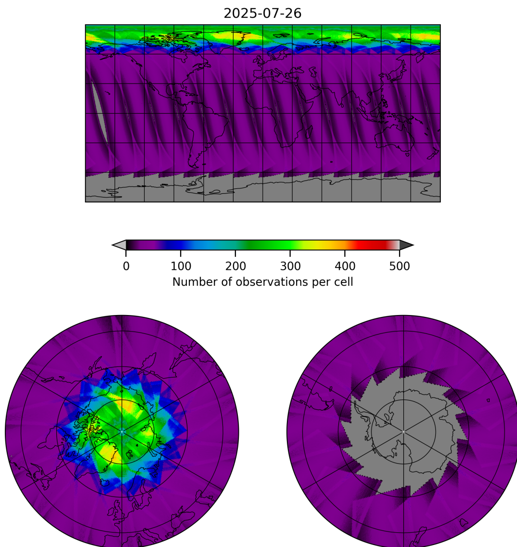
Figure 17: Map of the number of observations for 2025-07-26 to 2025-07-27
