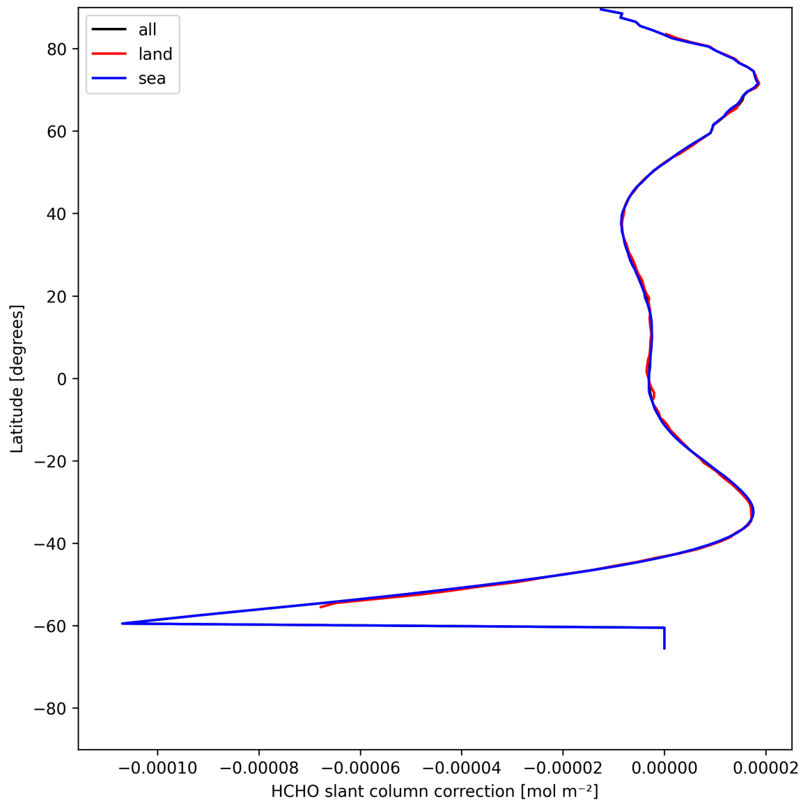
Figure 31: Zonal average of “HCHO slant column correction” for 2025-07-26 to 2025-07-27.
