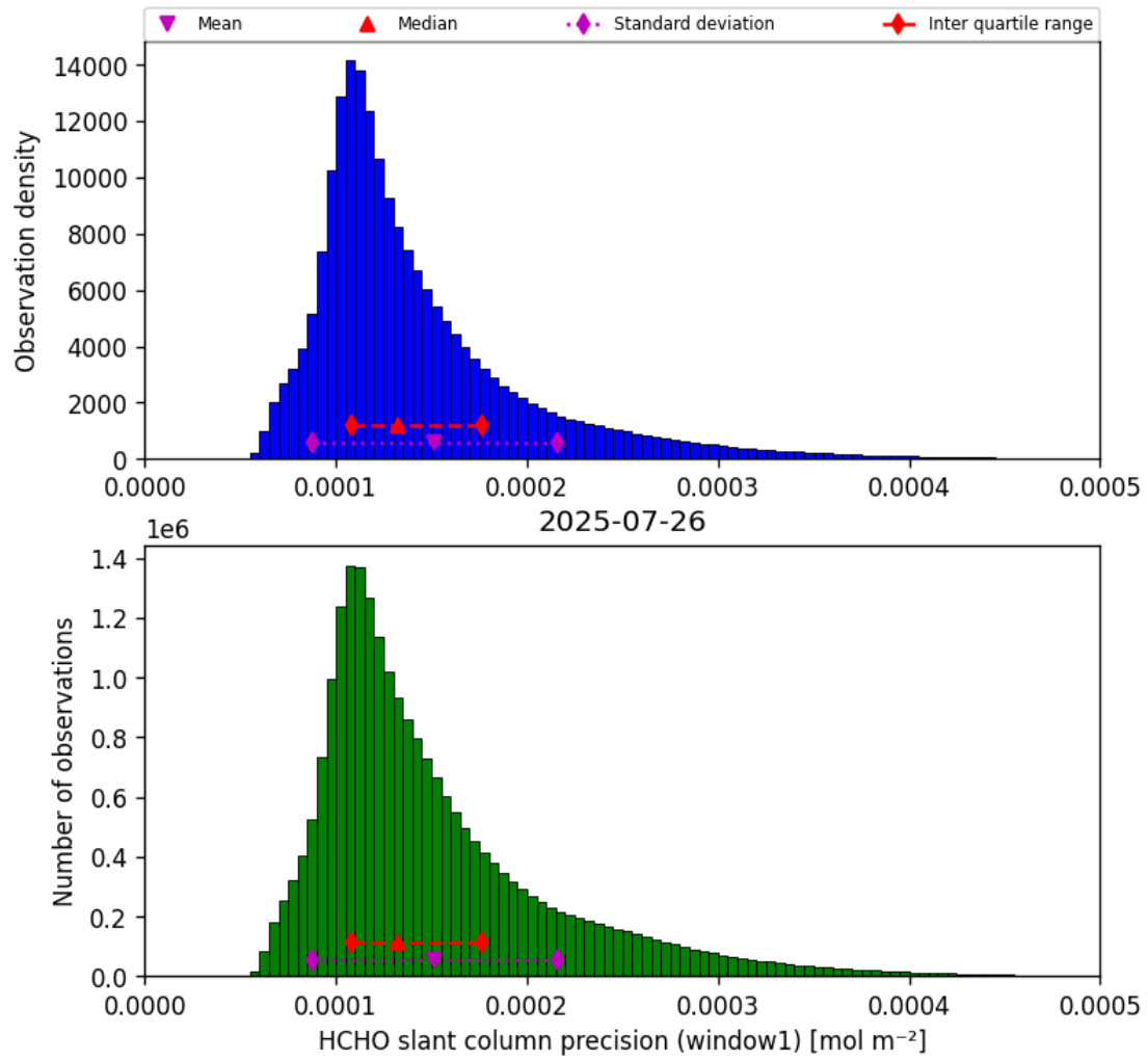
Figure 37: Histogram of “HCHO slant column precision (window1)” for 2025-07-26 to 2025-07-27
