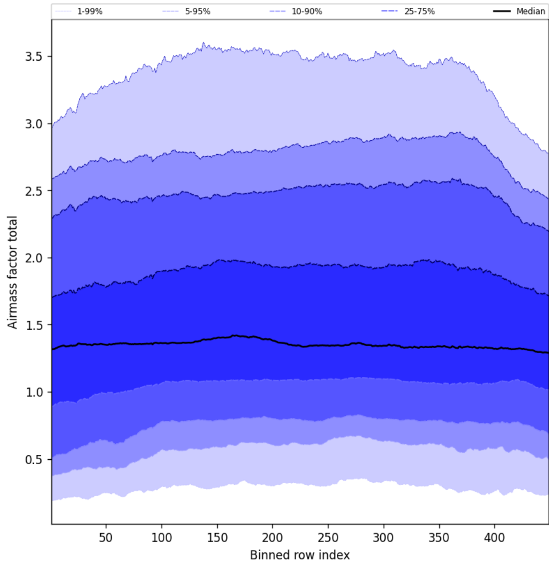
Figure 52: Along track statistics of “Airmass factor total” for 2025-07-26 to 2025-07-27
