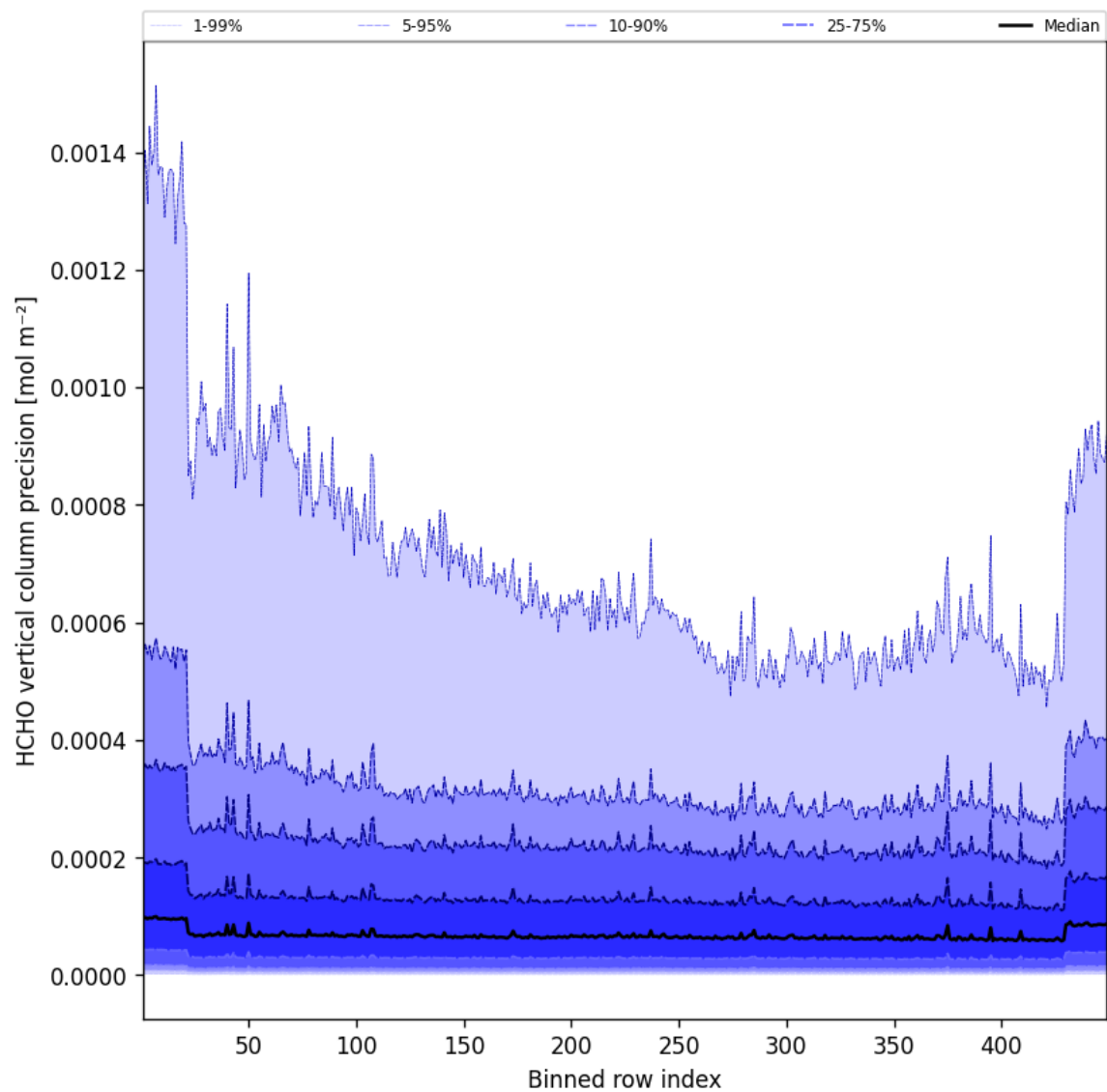
Figure 48: Along track statistics of “HCHO vertical column precision” for 2025-07-26 to 2025-07-27
