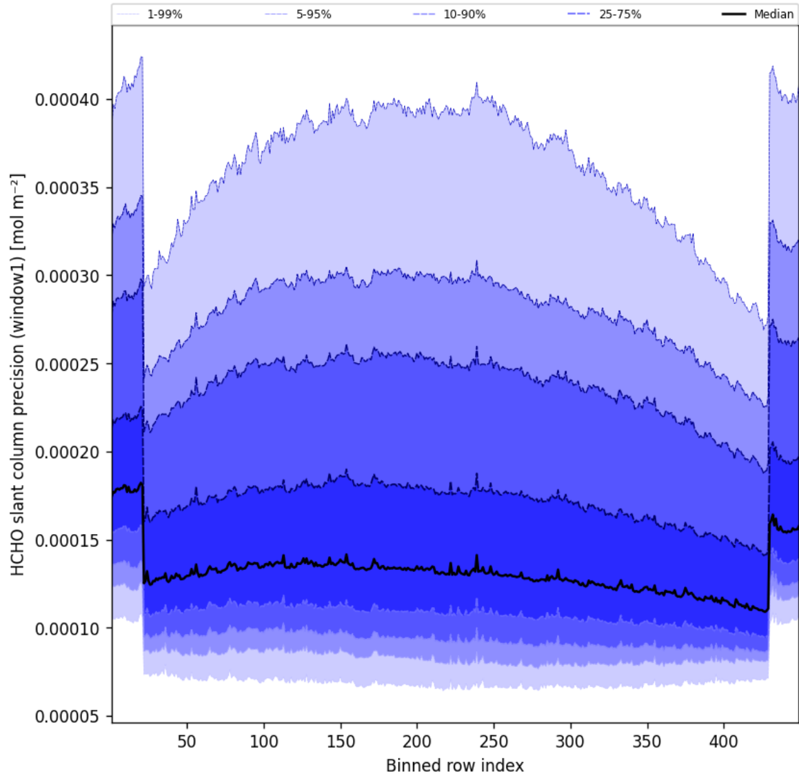
Figure 51: Along track statistics of “HCHO slant column precision (window1)” for 2025-07-26 to 2025-07-27
