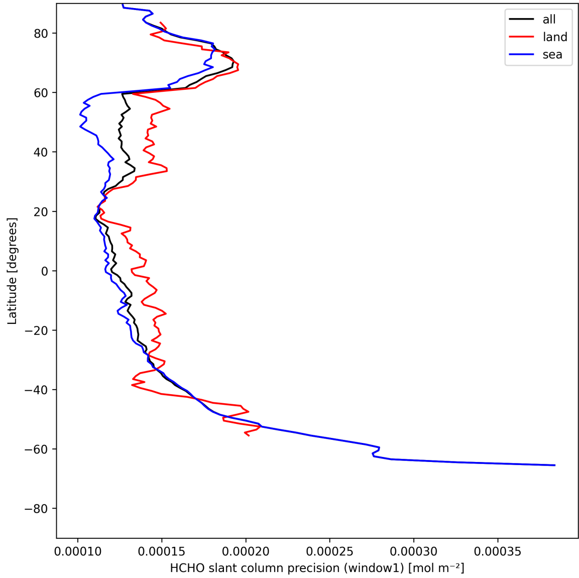
Figure 23: Zonal average of “HCHO slant column precision (window1)” for 2025-07-26 to 2025-07-27.
