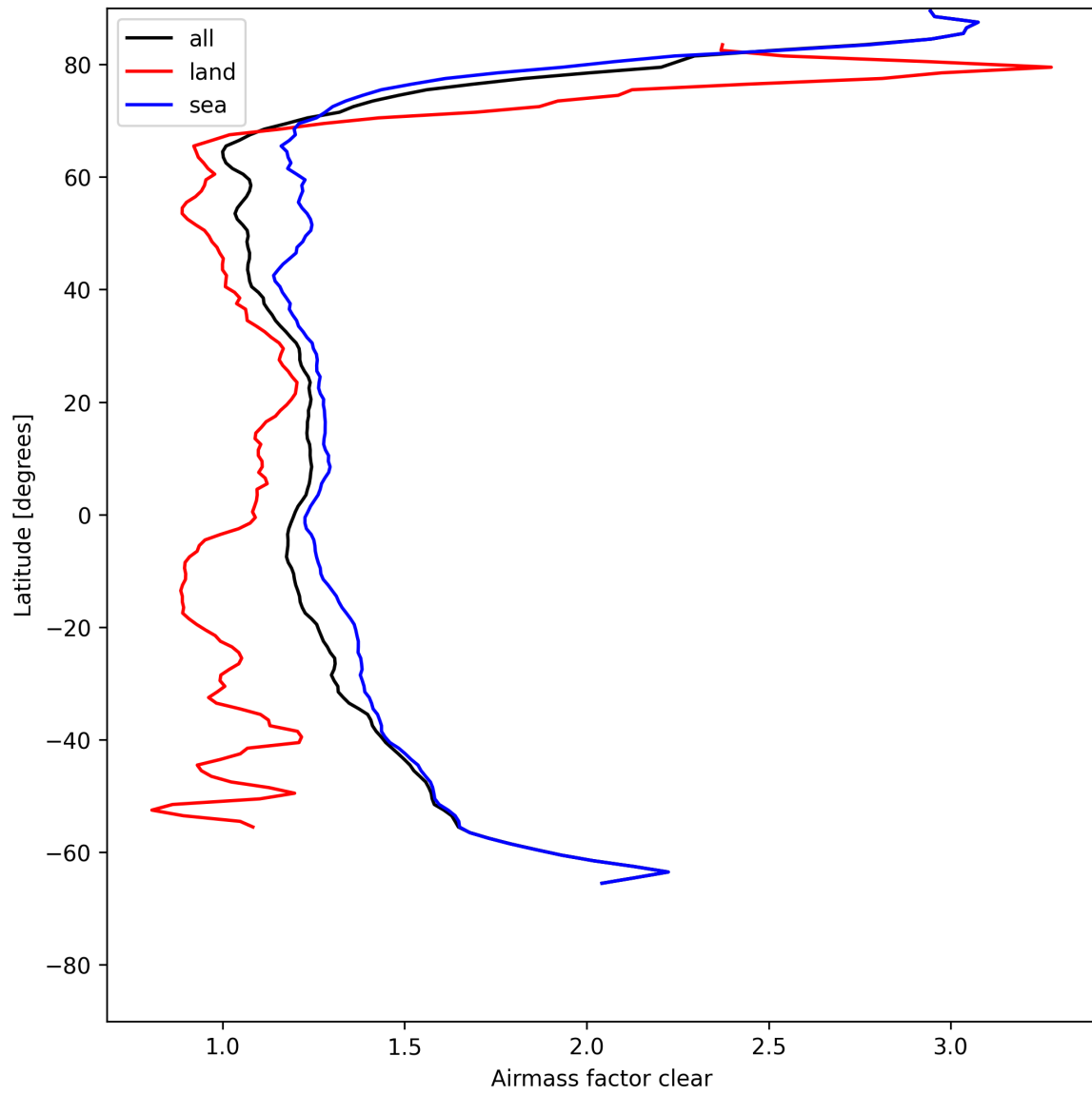
Figure 26: Zonal average of “Airmass factor clear” for 2025-07-26 to 2025-07-27.
