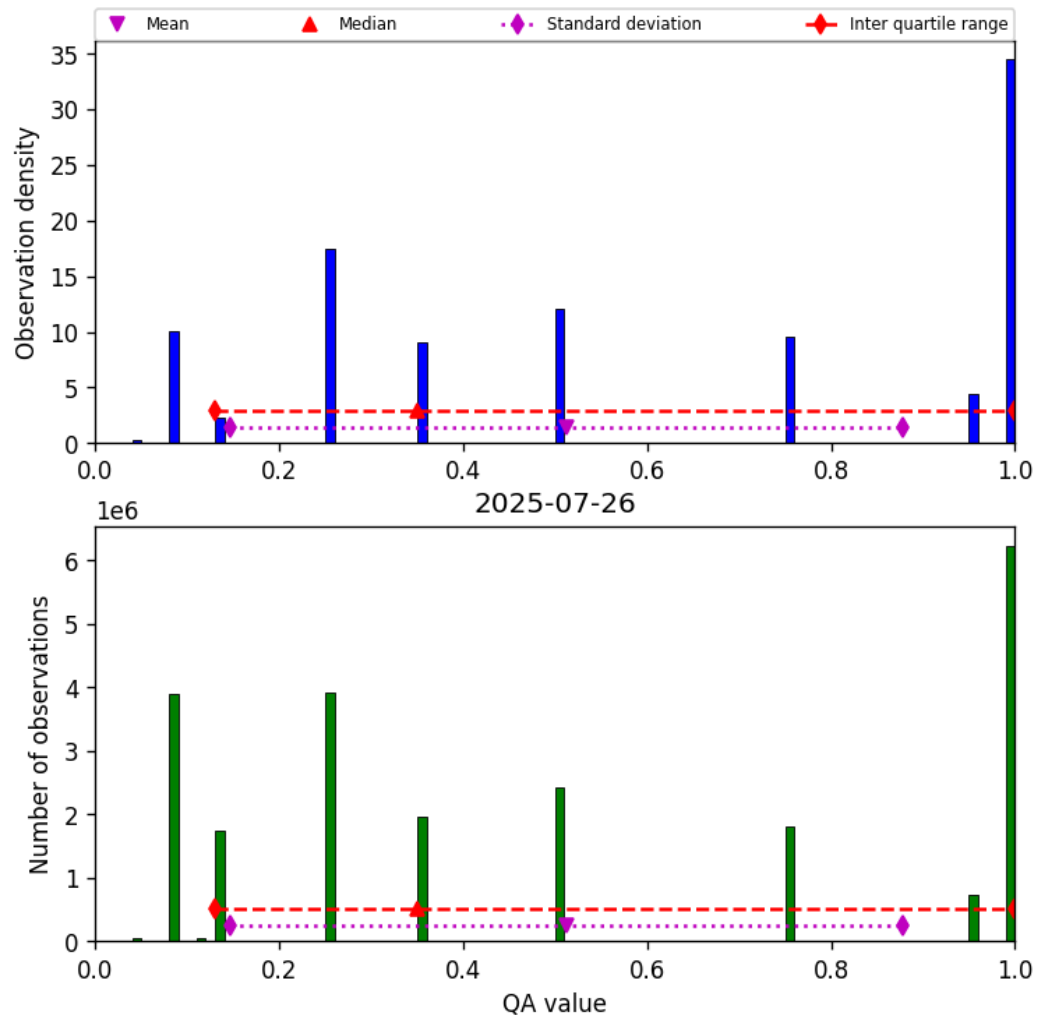
Figure 32: Histogram of “QA value” for 2025-07-26 to 2025-07-27
