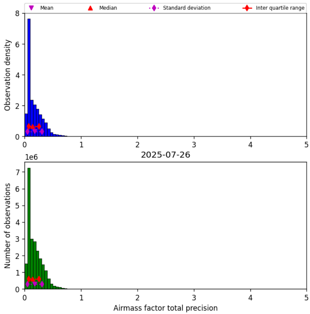
Figure 39: Histogram of “Airmass factor total precision” for 2025-07-26 to 2025-07-27
