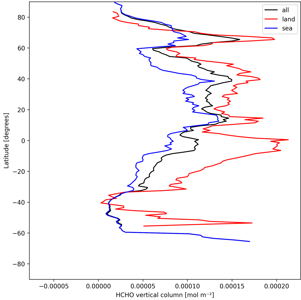
Figure 19: Zonal average of “HCHO vertical column” for 2025-07-26 to 2025-07-27.
