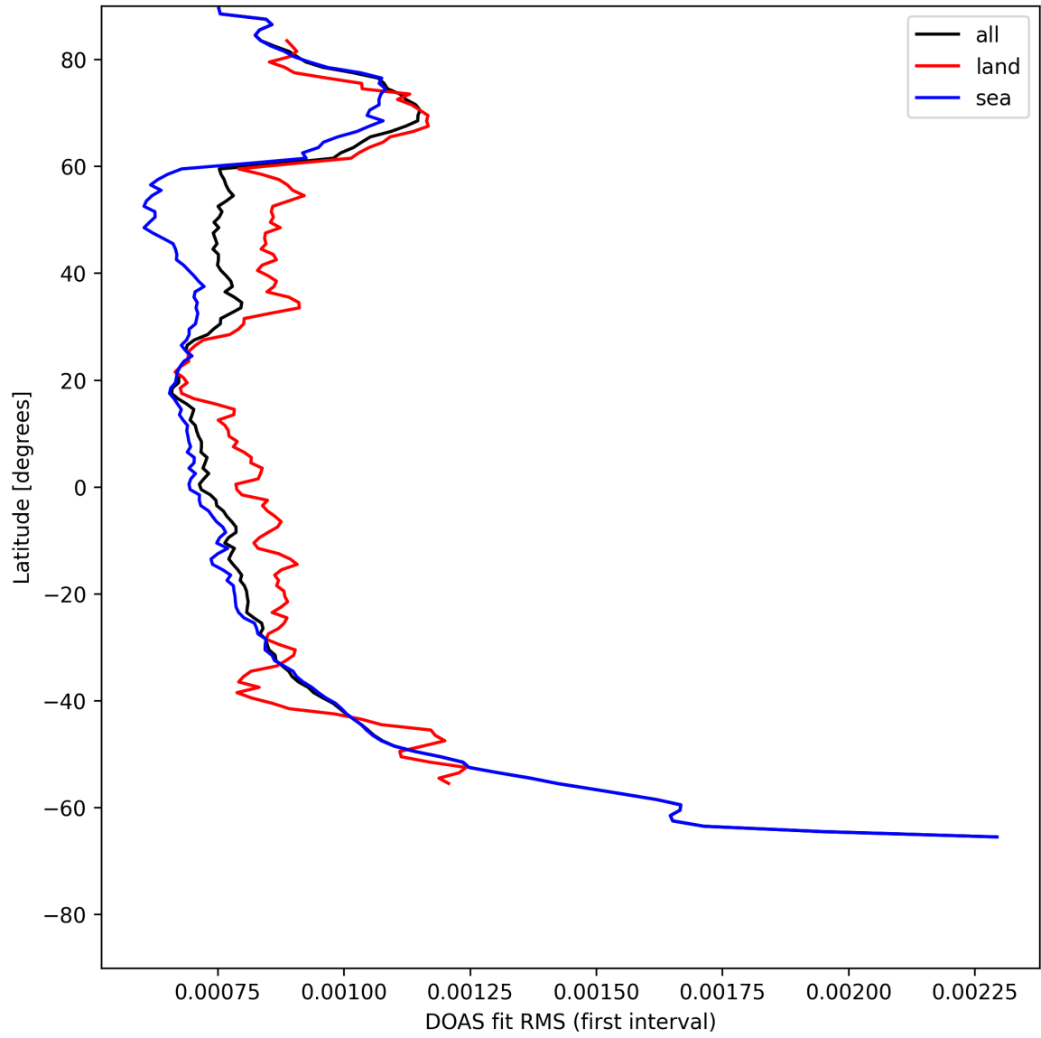
Figure 30: Zonal average of "DOAS fit RMS (first interval)" for 2025-07-26 to 2025-07-27.
