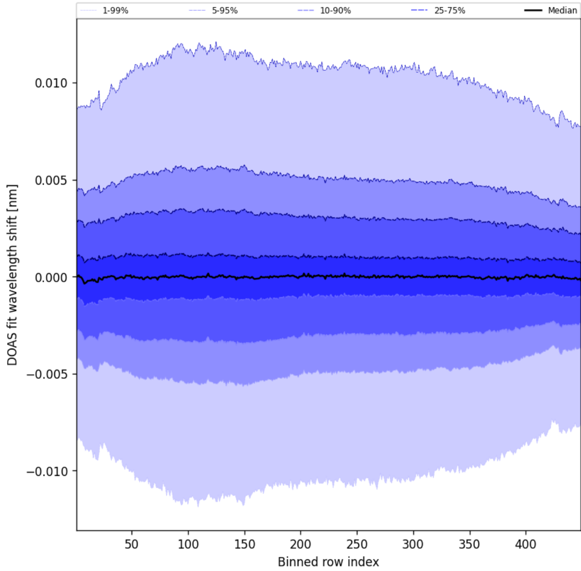
Figure 56: Along track statistics of “DOAS fit wavelength shift” for 2025-07-26 to 2025-07-27
