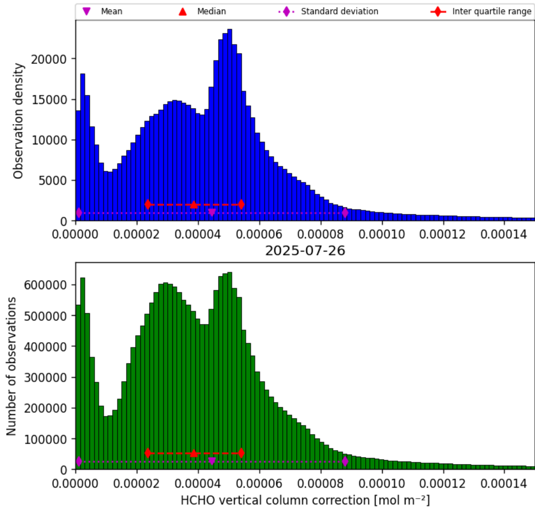
Figure 35: Histogram of “HCHO vertical column correction” for 2025-07-26 to 2025-07-27
