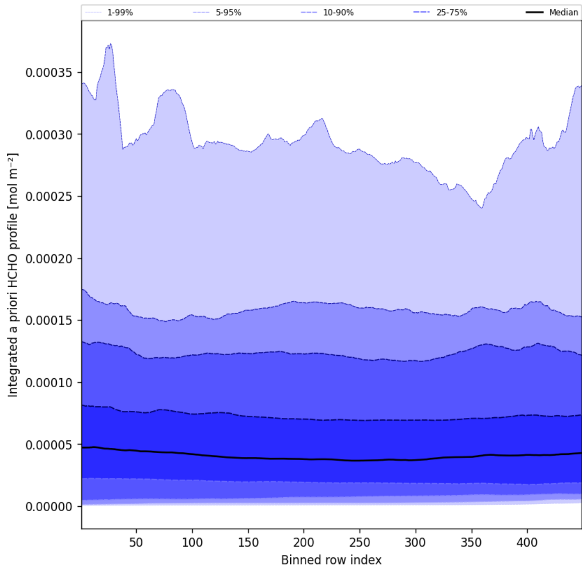
Figure 55: Along track statistics of “Integrated a priori HCHO profile” for 2025-07-26 to 2025-07-27
