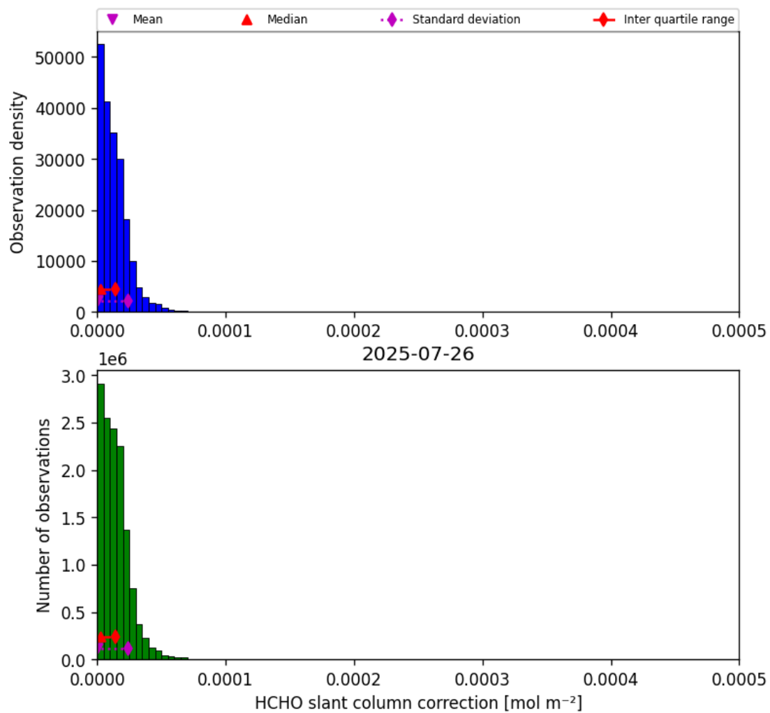
Figure 45: Histogram of “HCHO slant column correction” for 2025-07-26 to 2025-07-27
