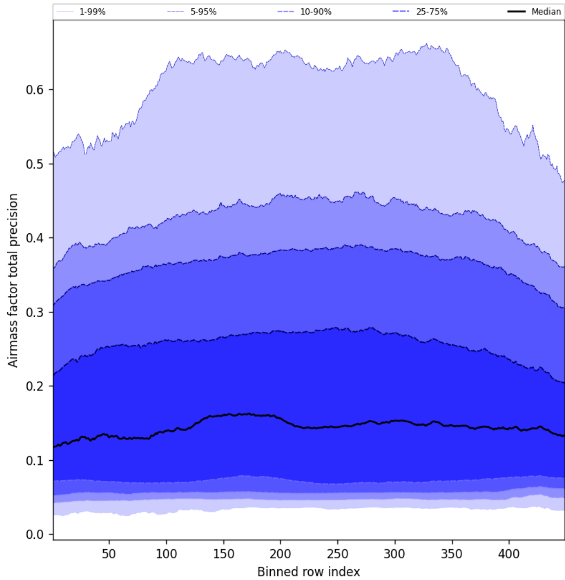
Figure 53: Along track statistics of “Airmass factor total precision” for 2025-07-26 to 2025-07-27
