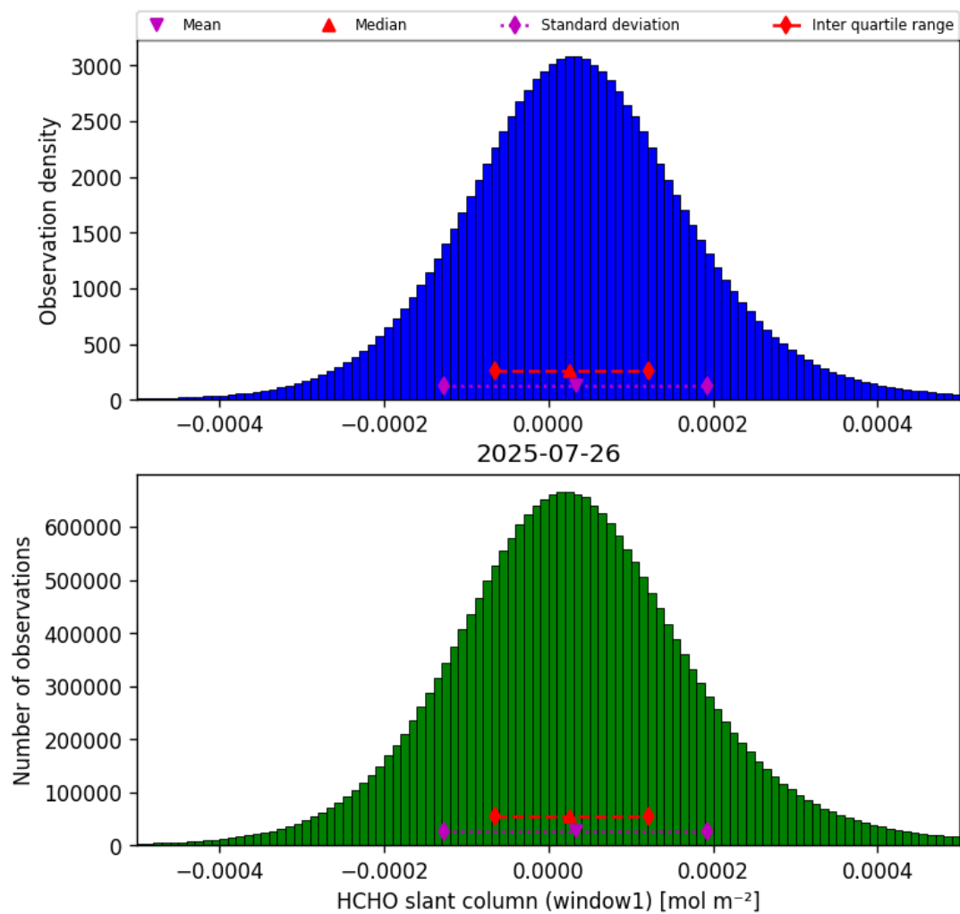
Figure 36: Histogram of “HCHO slant column (window1)” for 2025-07-26 to 2025-07-27
