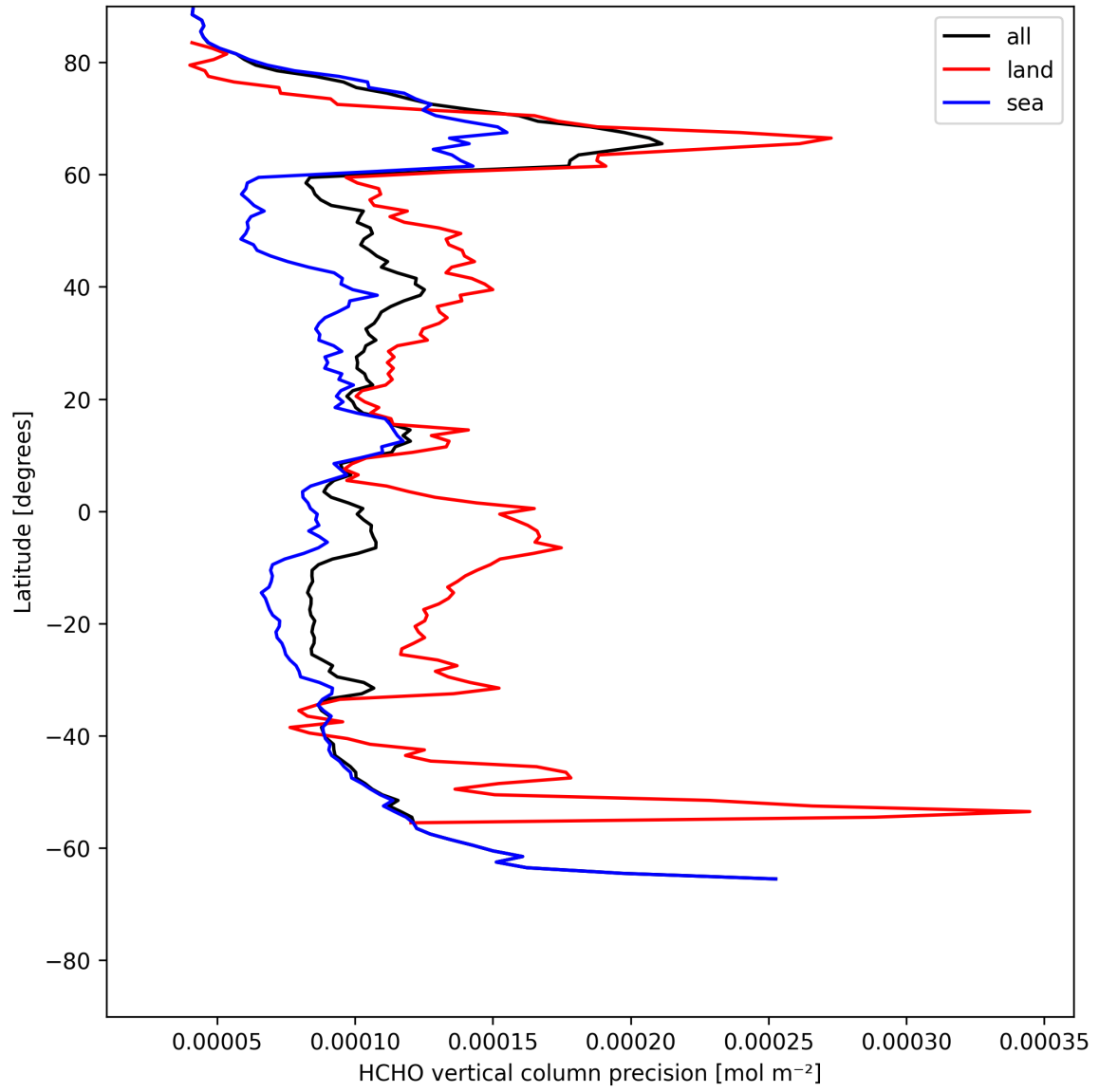
Figure 20: Zonal average of “HCHO vertical column precision” for 2025-07-26 to 2025-07-27.
