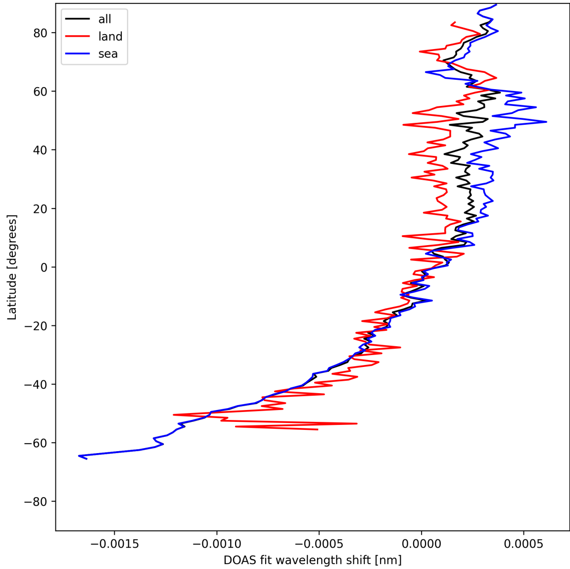
Figure 28: Zonal average of “DOAS fit wavelength shift” for 2025-07-26 to 2025-07-27.
