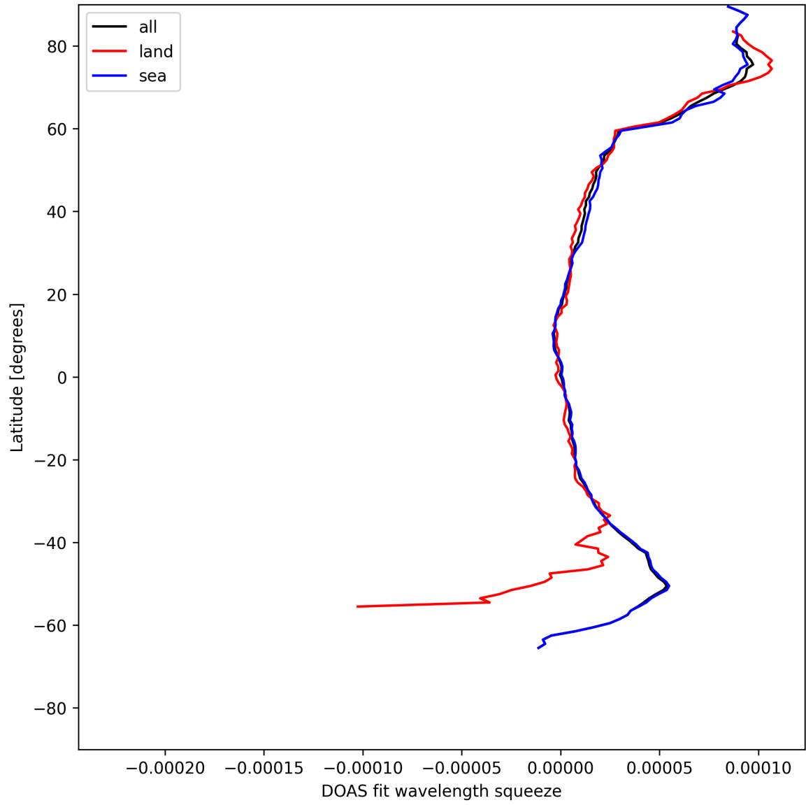
Figure 29: Zonal average of “DOAS fit wavelength squeeze” for 2025-07-26 to 2025-07-27.
