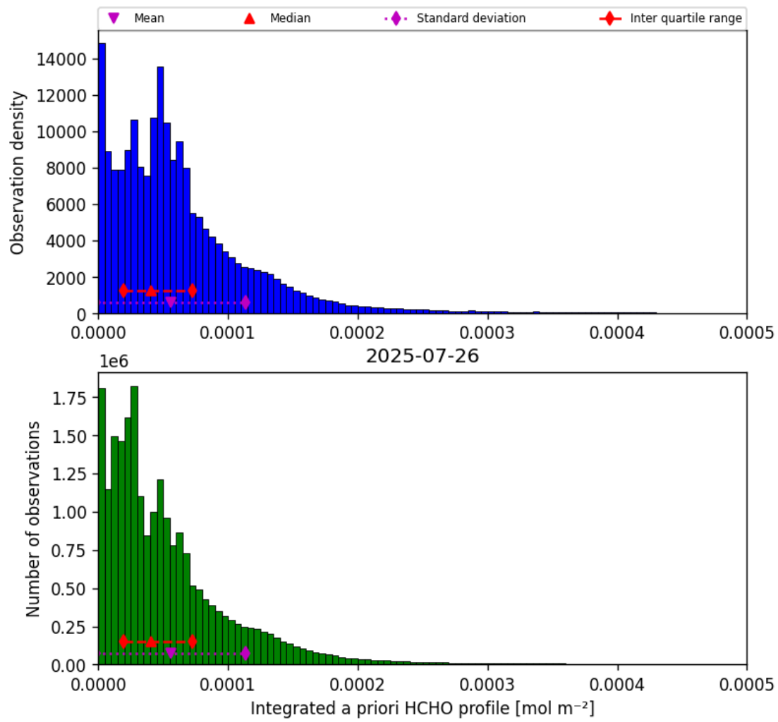
Figure 41: Histogram of “Integrated a priori HCHO profile” for 2025-07-26 to 2025-07-27
