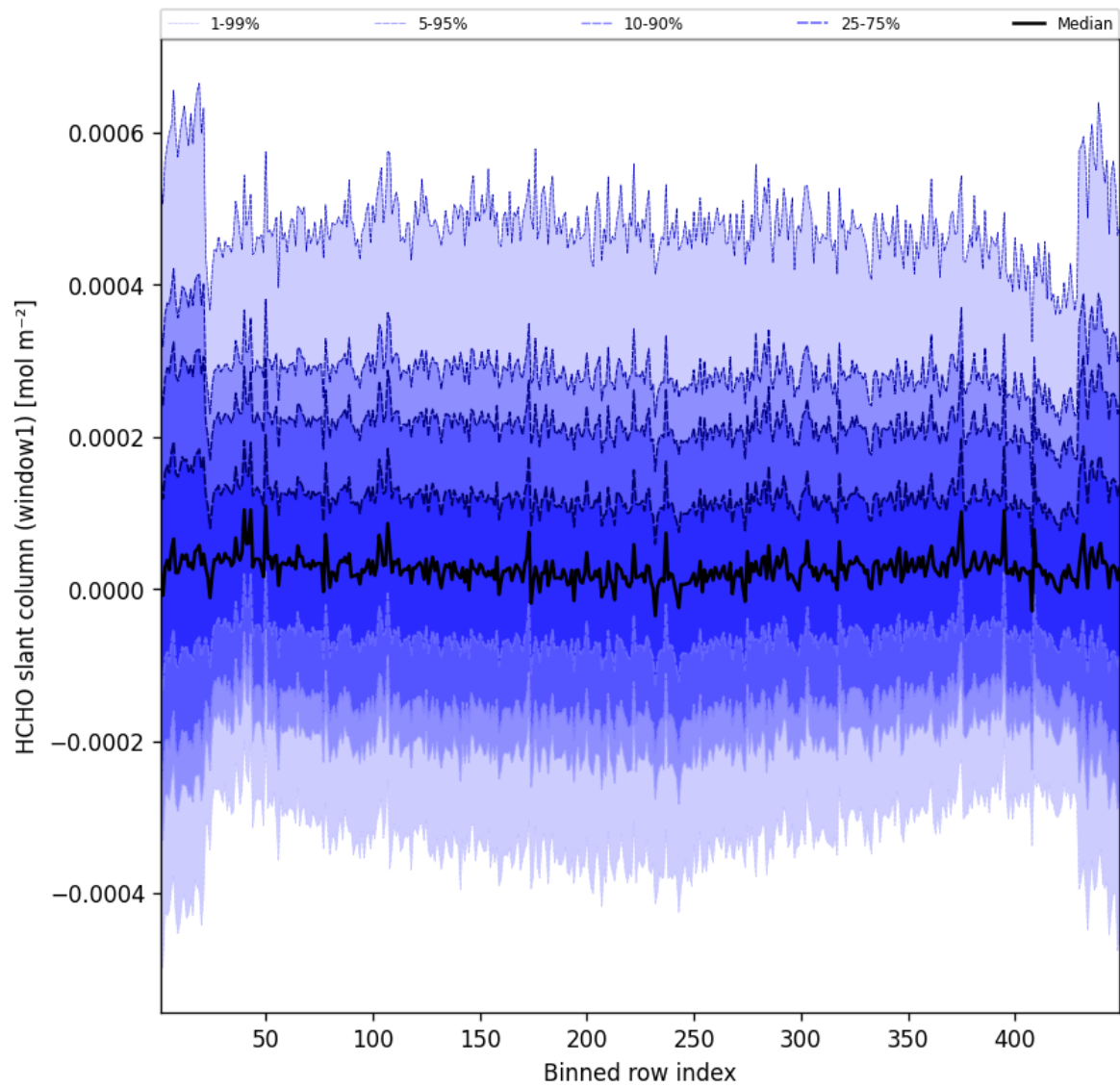
Figure 50: Along track statistics of “HCHO slant column (window1)” for 2025-07-26 to 2025-07-27
