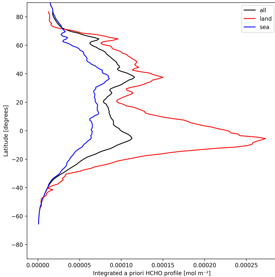
Figure 27: Zonal average of “Integrated a priori HCHO profile” for 2025-07-26 to 2025-07-27.
