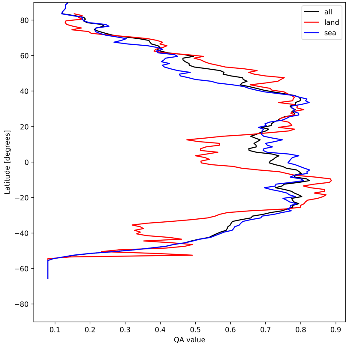
Figure 18: Zonal average of “QA value” for 2025-07-26 to 2025-07-27.
