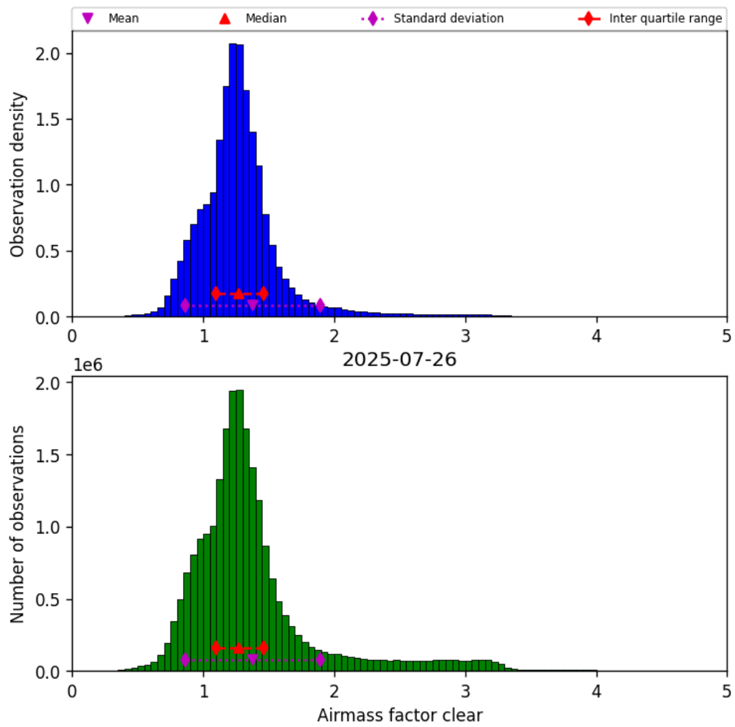
Figure 40: Histogram of “Airmass factor clear” for 2025-07-26 to 2025-07-27
