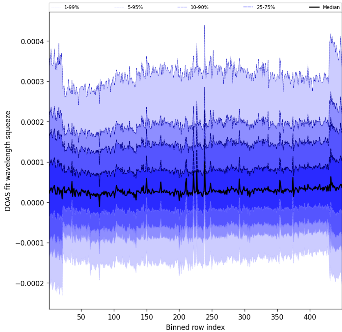
Figure 57: Along track statistics of “DOAS fit wavelength squeeze” for 2025-07-26 to 2025-07-27
